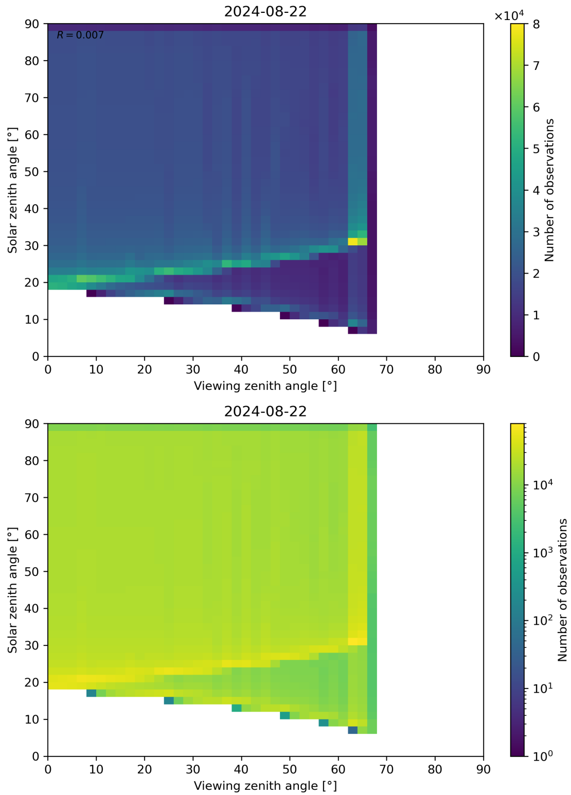
Figure 54: Scatter density plot of “Viewing zenith angle” against “Solar zenith angle” for 2024-08-22 to 2024-08-23.
