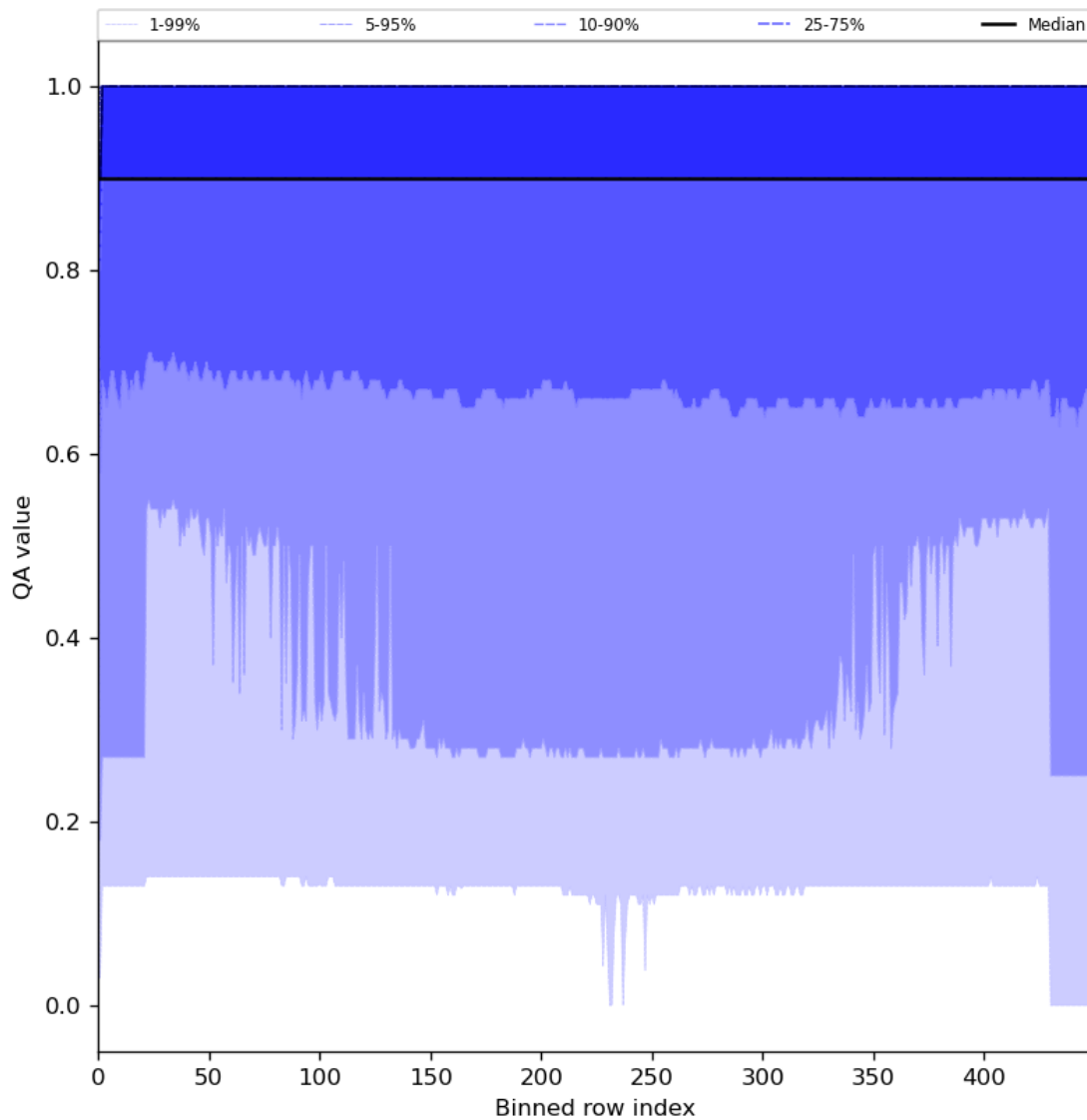
Figure 27: Along track statistics of “QA value” for 2024-08-22 to 2024-08-23
