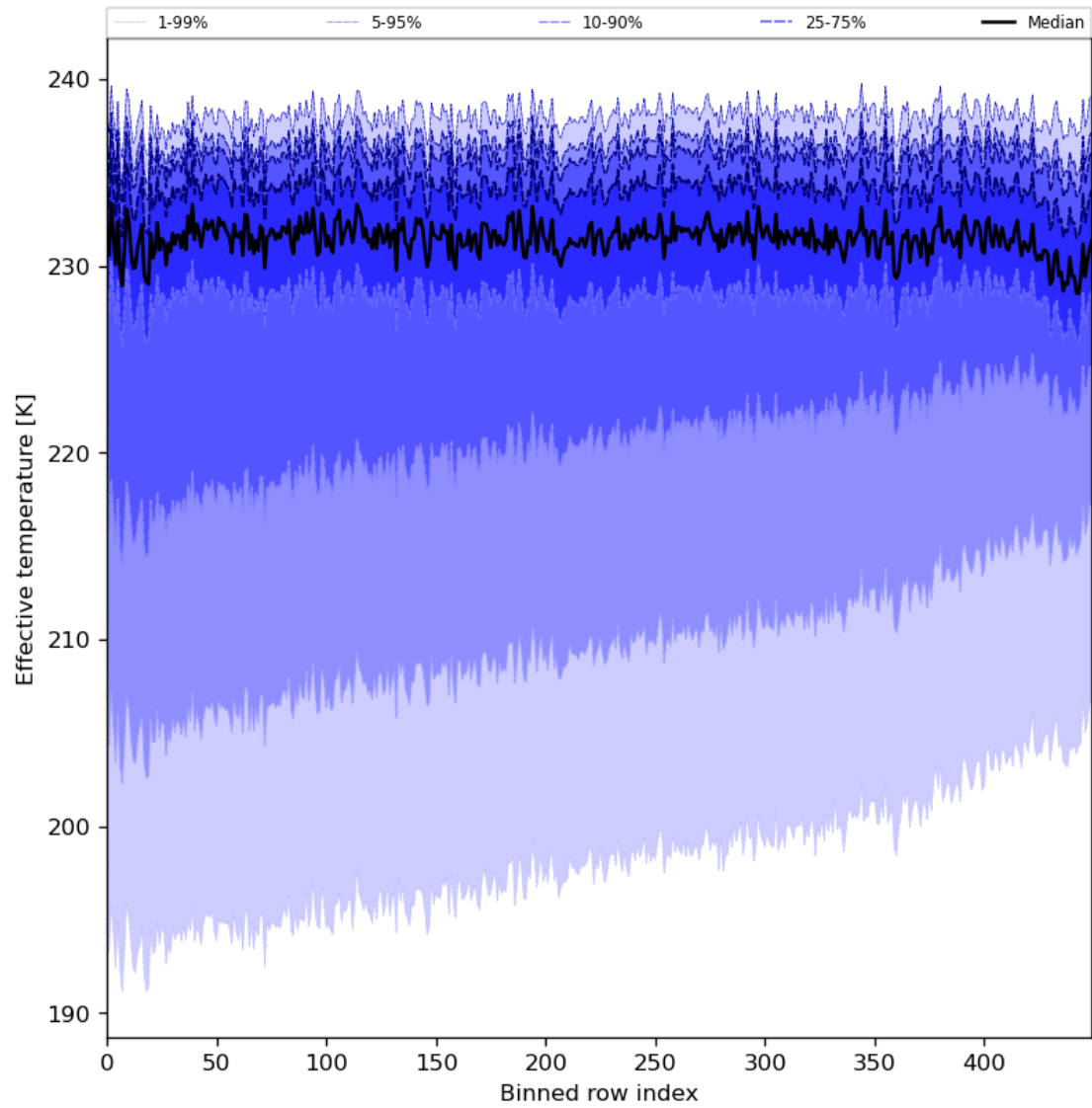
Figure 31: Along track statistics of “Effective temperature” for 2024-08-22 to 2024-08-23
