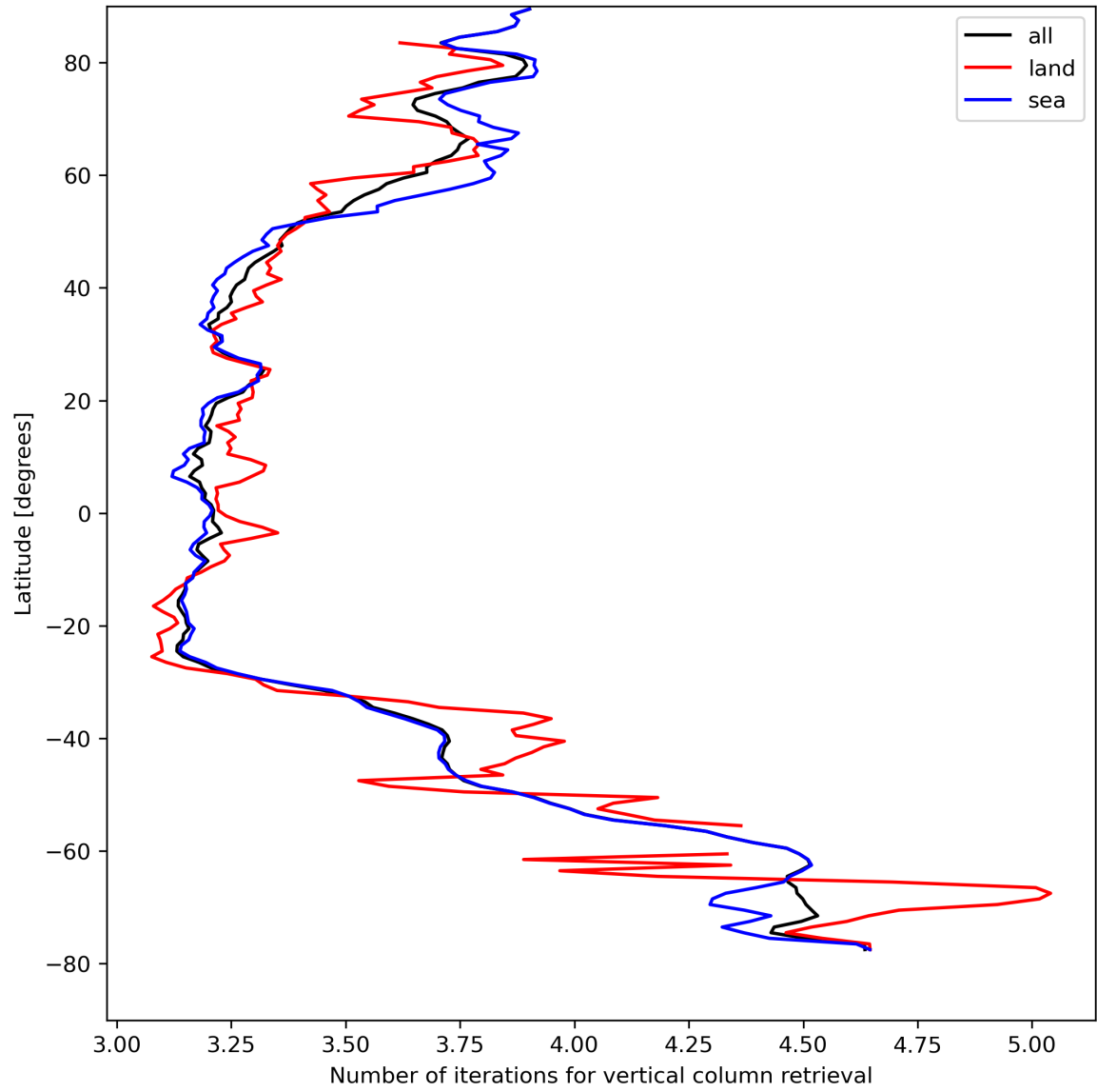
Figure 19: Zonal average of “Number of iterations for vertical column retrieval” for 2024-08-22 to 2024-08-23.
