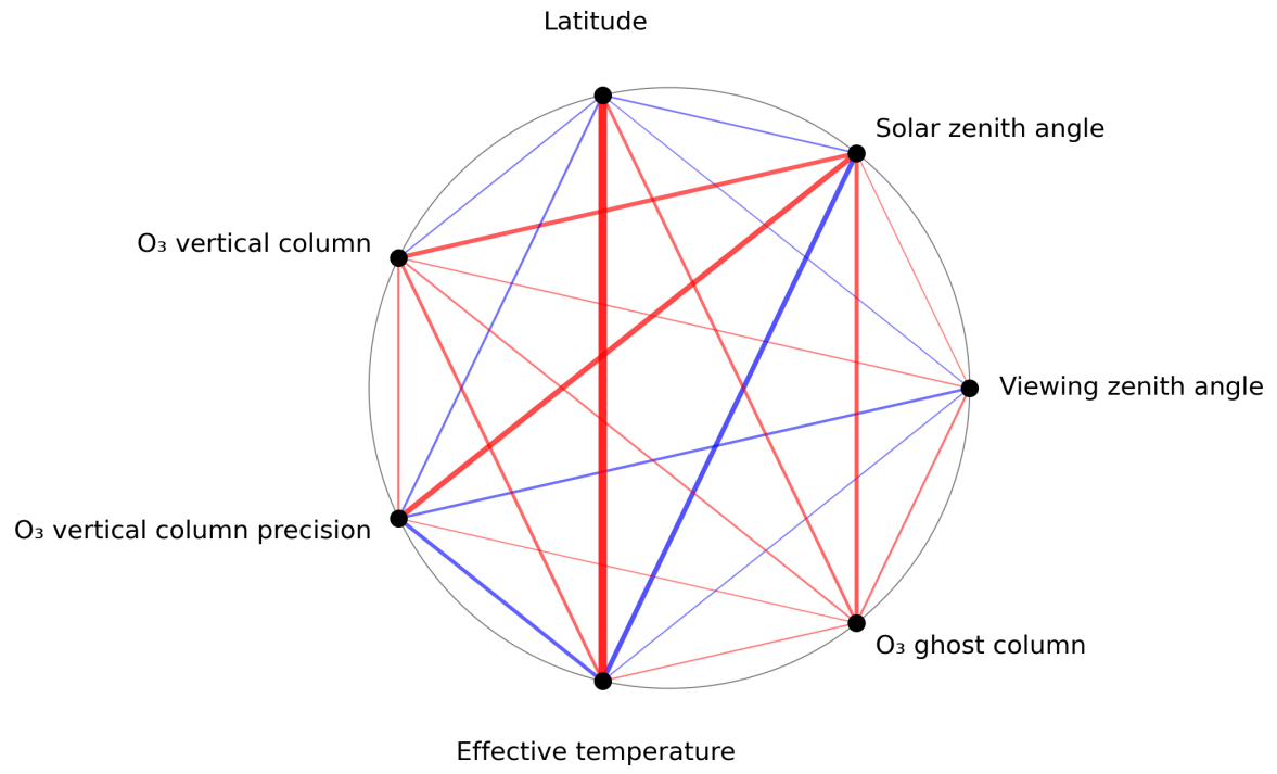
Figure 1: Map of correlation graph for 2024-08-22 to 2024-08-23.
