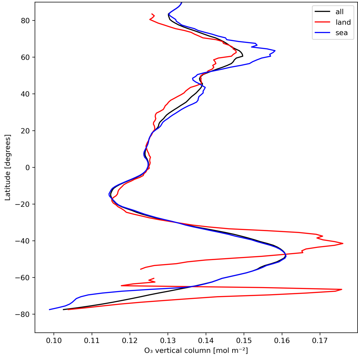
Figure 14: Zonal average of “O 3 vertical column” for 2024-08-22 to 2024-08-23.
