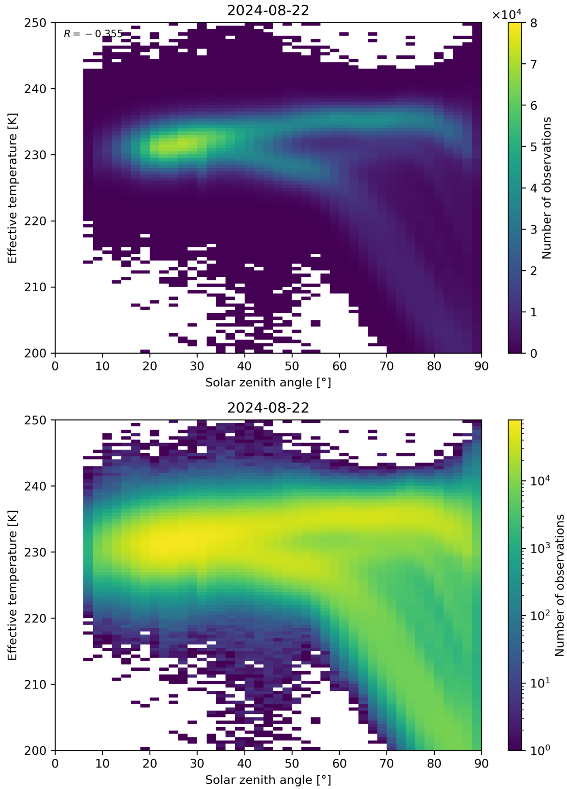
Figure 45: Scatter density plot of “Solar zenith angle” against “Effective temperature” for 2024-08-22 to 2024-08-23.
