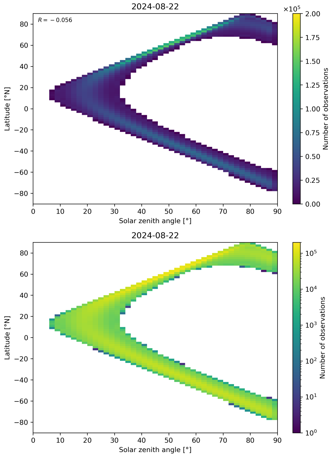
Figure 44: Scatter density plot of “Solar zenith angle” against “Latitude” for 2024-08-22 to 2024-08-23.
