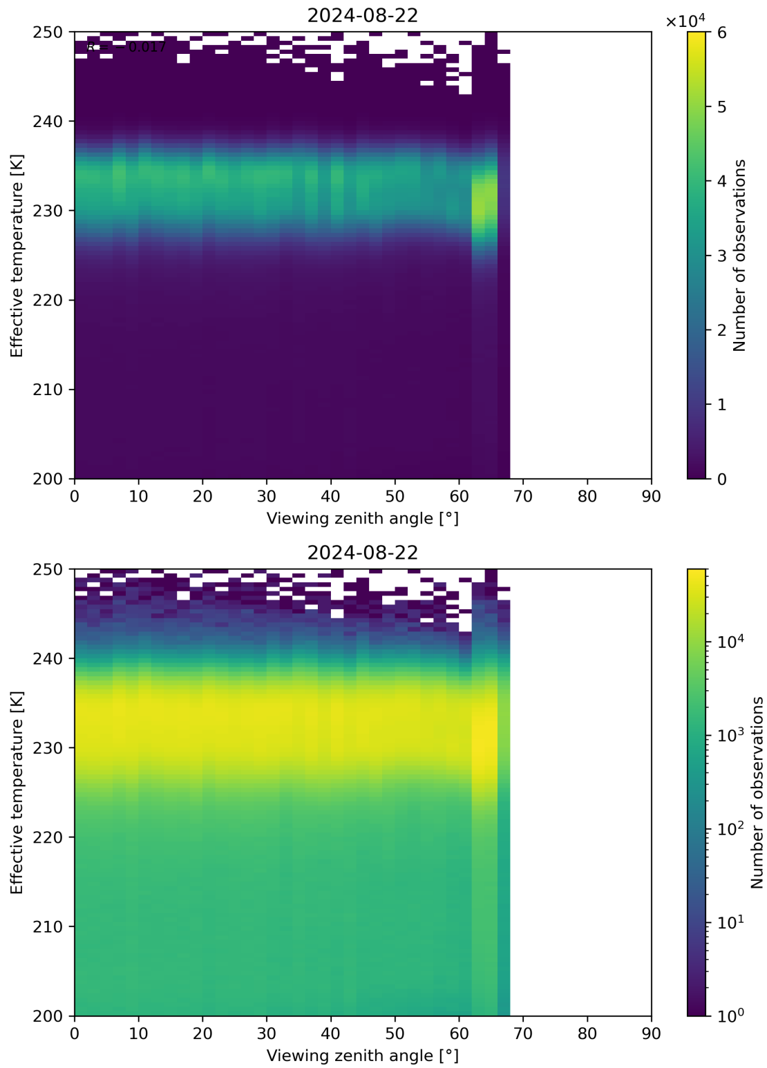
Figure 50: Scatter density plot of “Viewing zenith angle” against “Effective temperature” for 2024-08-22 to 2024-08-23.
