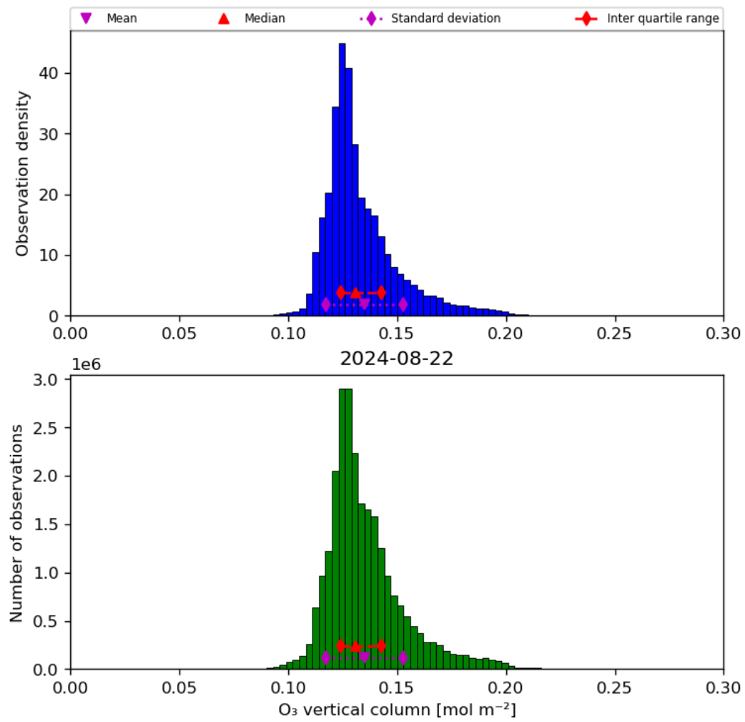
Figure 21: Histogram of “O 3 vertical column” for 2024-08-22 to 2024-08-23
