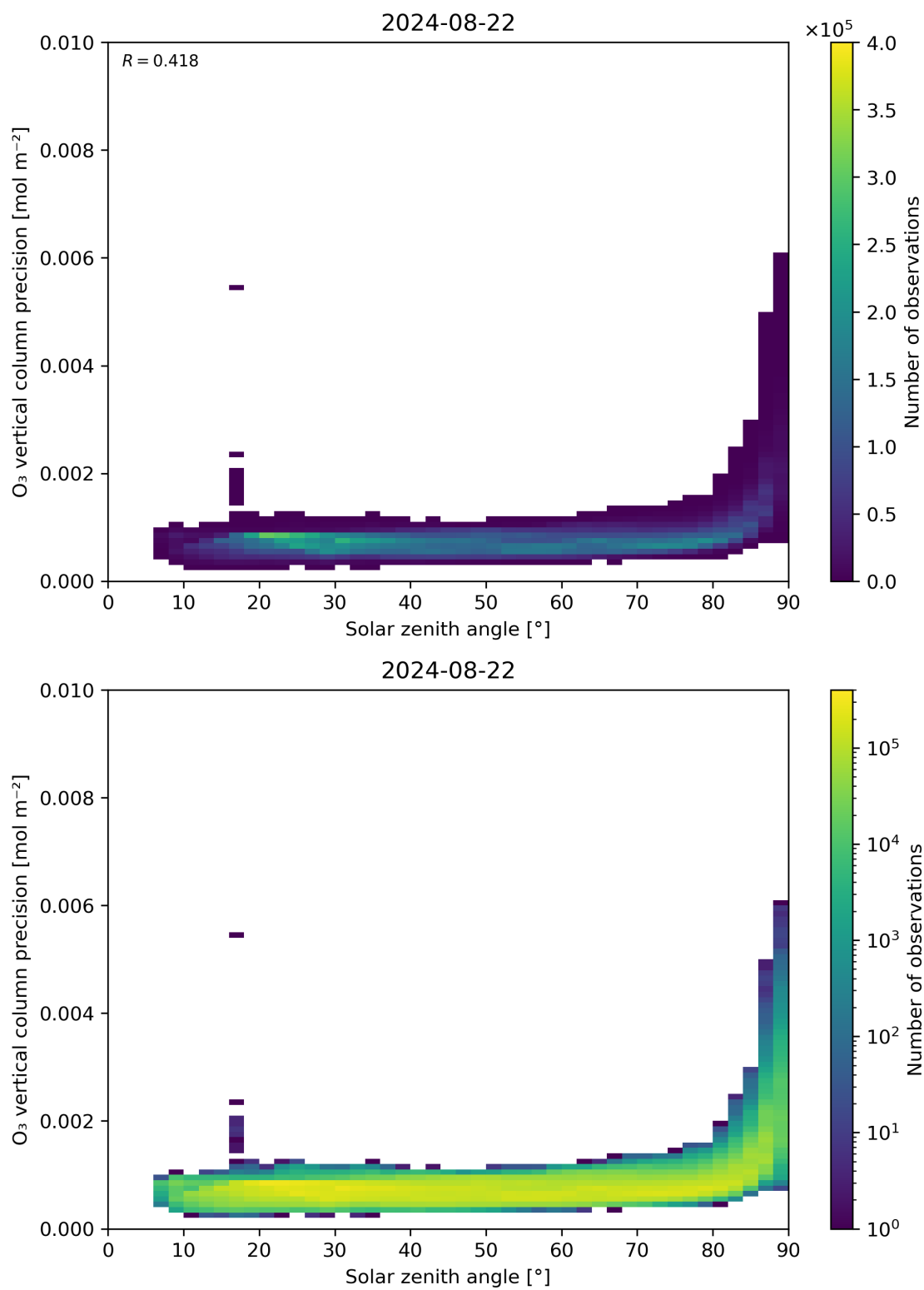
Figure 48: Scatter density plot of “Solar zenith angle” against “O 3 vertical column precision” for 2024-08-22 to 2024-08-23.
