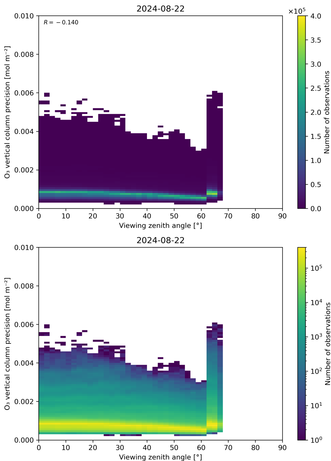
Figure 53: Scatter density plot of “Viewing zenith angle” against “O 3 vertical column precision” for 2024-08-22 to 2024-08-23.
