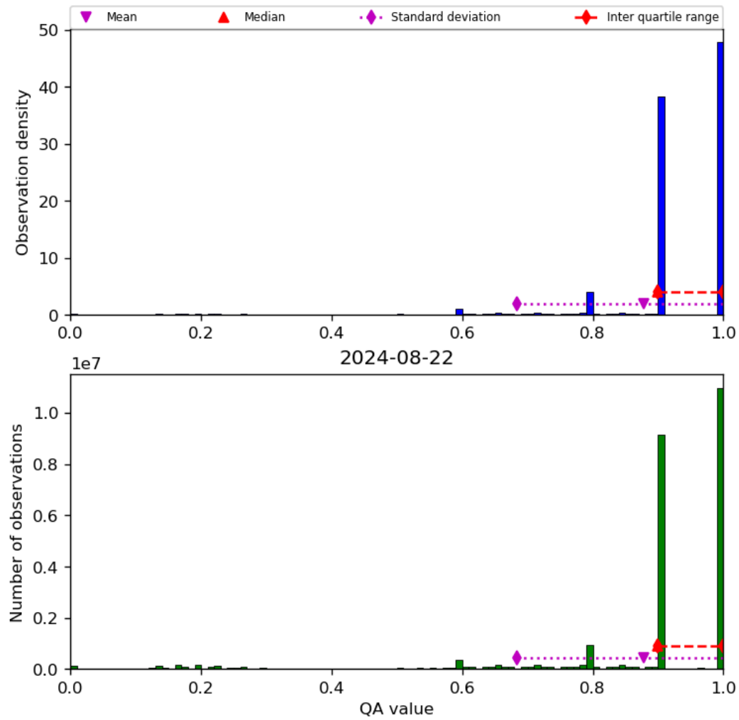
Figure 20: Histogram of “QA value” for 2024-08-22 to 2024-08-23
