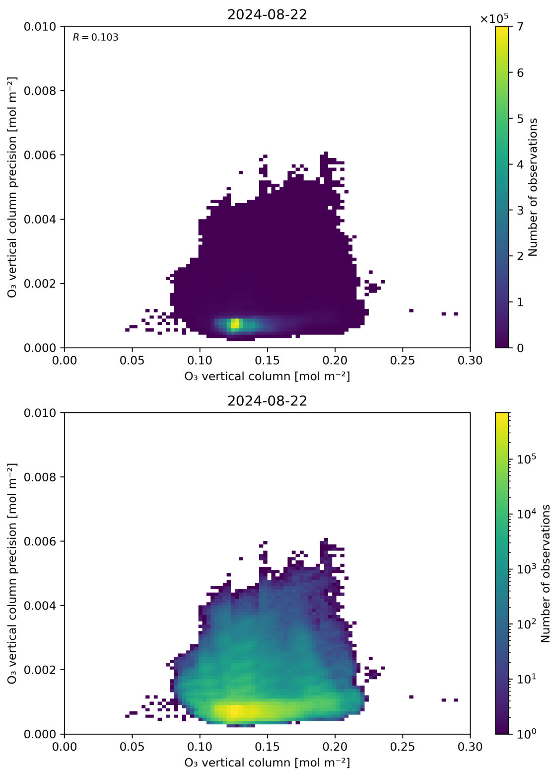
Figure 41: Scatter density plot of “O 3 vertical column” against “O 3 vertical column precision” for 2024-08-22 to 2024-08-23.
