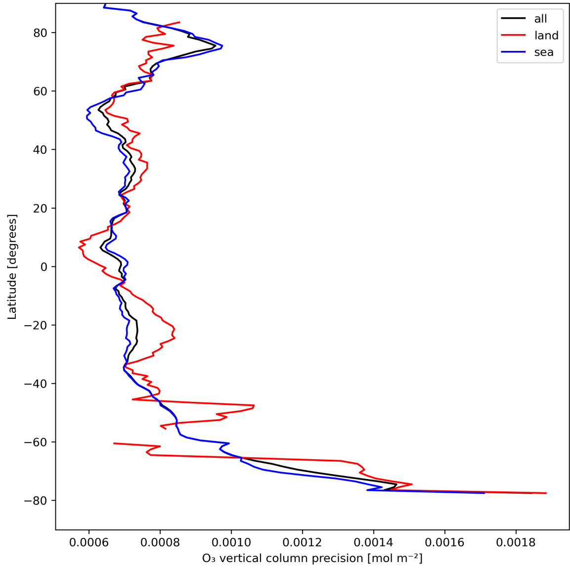
Figure 15: Zonal average of “O 3 vertical column precision” for 2024-08-22 to 2024-08-23.
