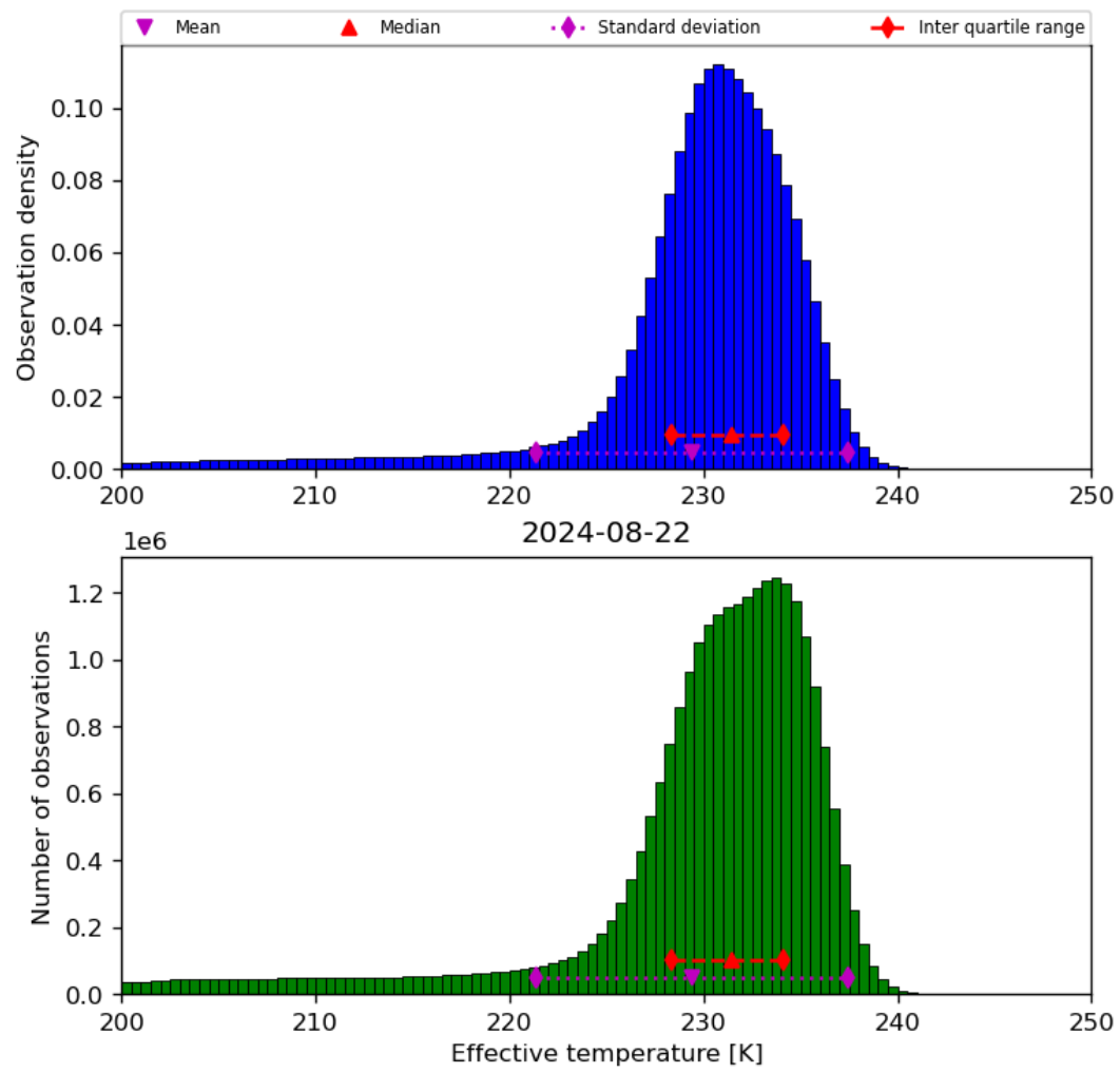
Figure 24: Histogram of “Effective temperature” for 2024-08-22 to 2024-08-23
