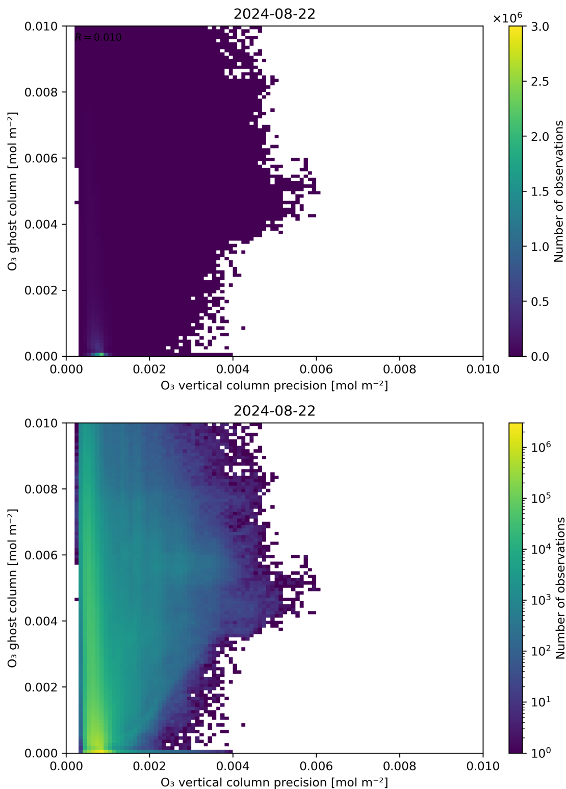
Figure 43: Scatter density plot of “ O_3 vertical column precision” against “ O_3 ghost column” for 2024-08-22 to 2024-08-23.
