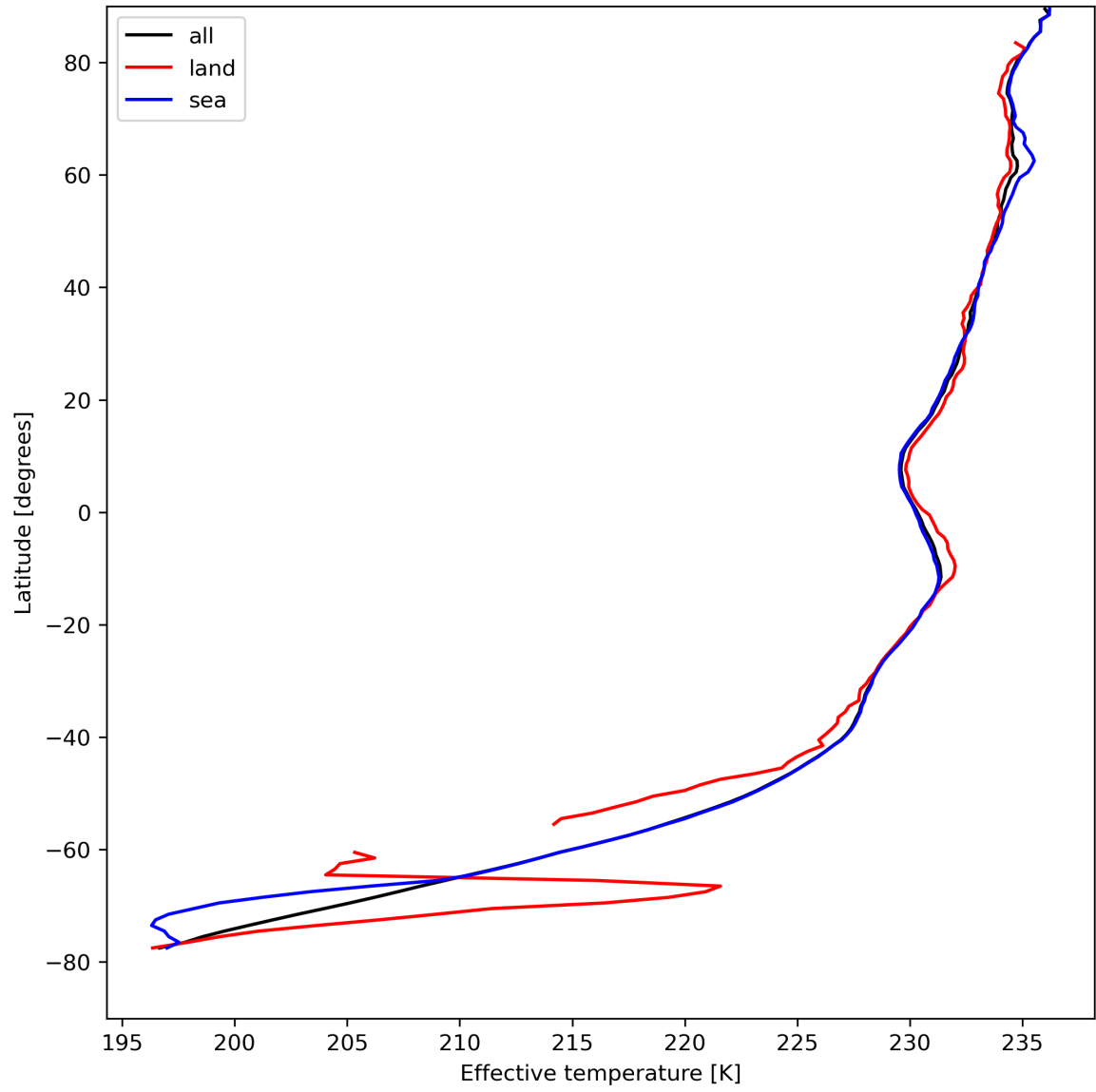
Figure 17: Zonal average of “Effective temperature” for 2024-08-22 to 2024-08-23.
