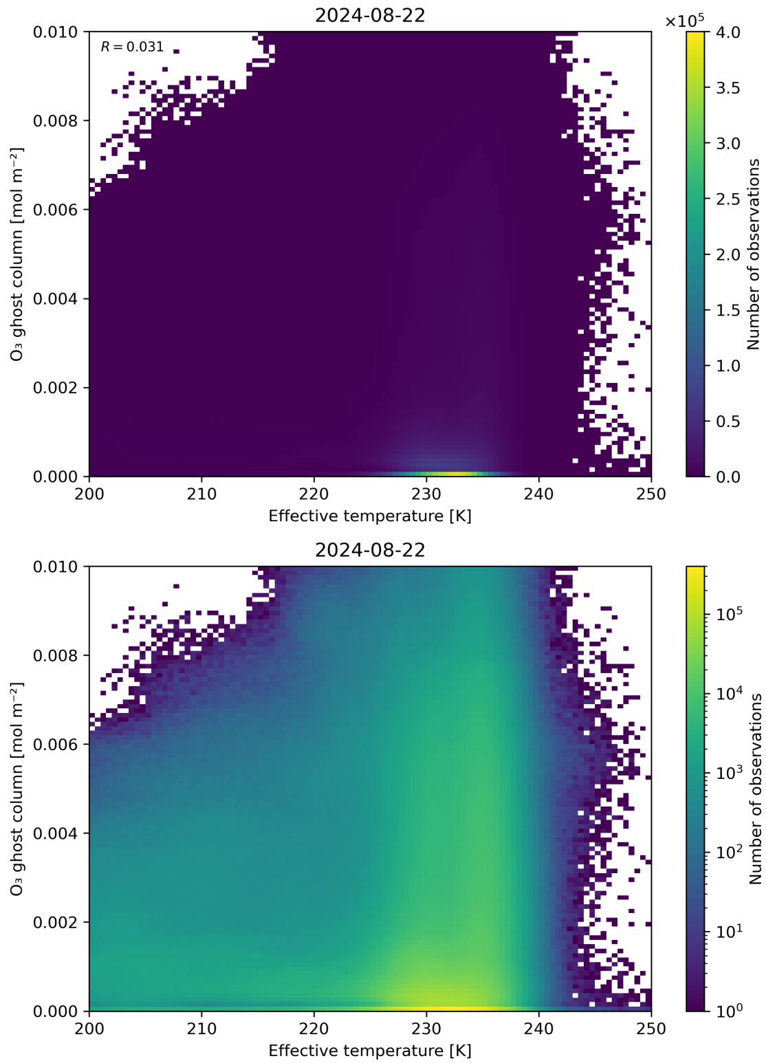
Figure 38: Scatter density plot of “Effective temperature” against “O 3 ghost column” for 2024-08-22 to 2024-08-23.
