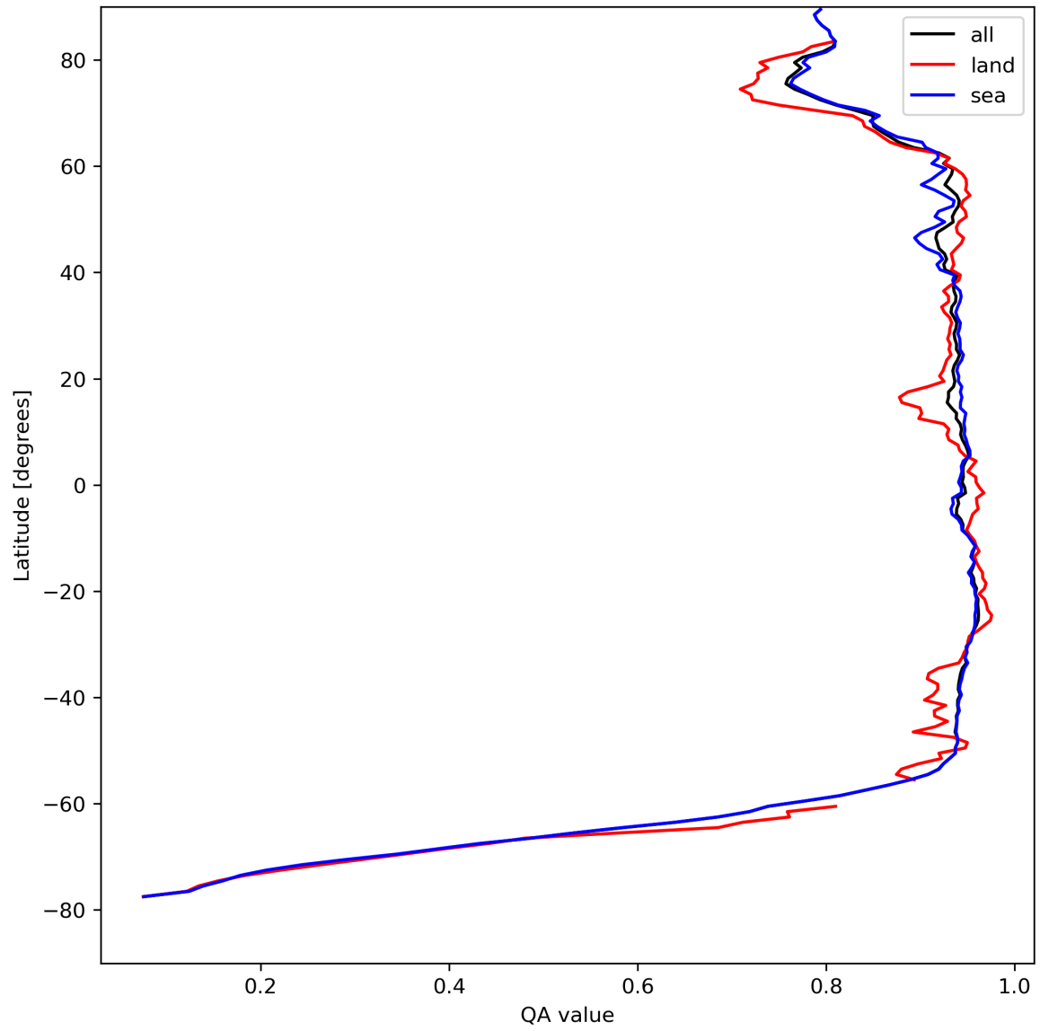
Figure 13: Zonal average of “QA value” for 2024-08-22 to 2024-08-23.
