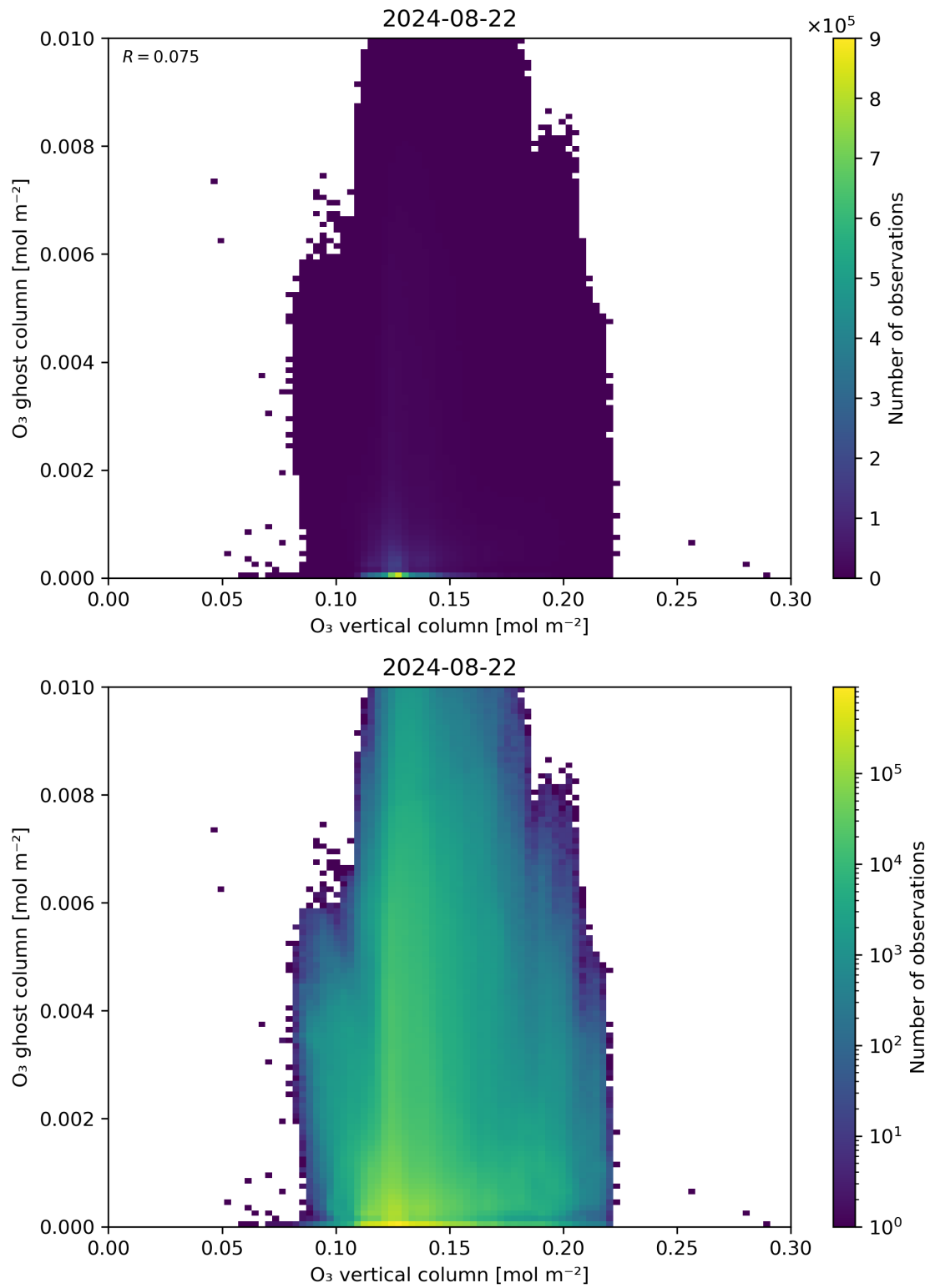
Figure 40: Scatter density plot of “O 3 vertical column” against “O 3 ghost column” for 2024-08-22 to 2024-08-23.
