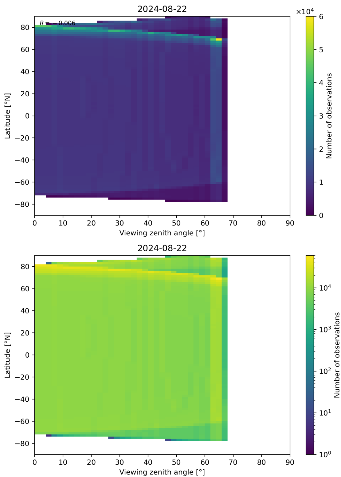
Figure 49: Scatter density plot of “Viewing zenith angle” against “Latitude” for 2024-08-22 to 2024-08-23.
