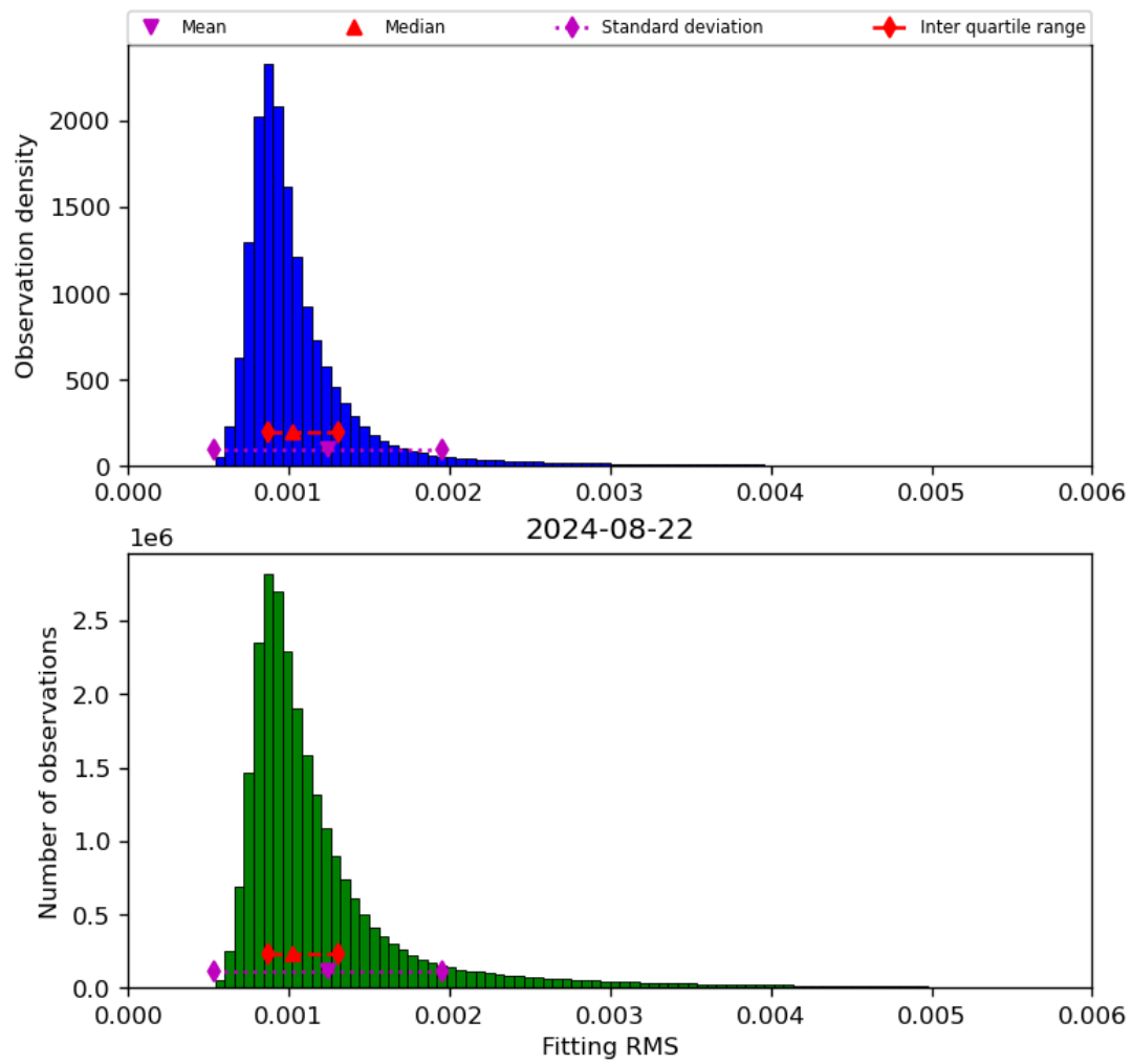
Figure 23: Histogram of “Fitting RMS” for 2024-08-22 to 2024-08-23
