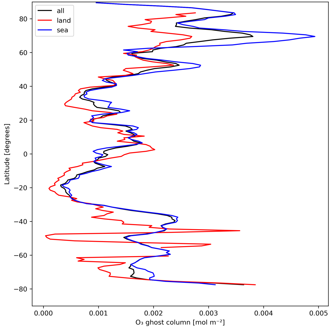
Figure 18: Zonal average of “O 3 ghost column” for 2024-08-22 to 2024-08-23.
