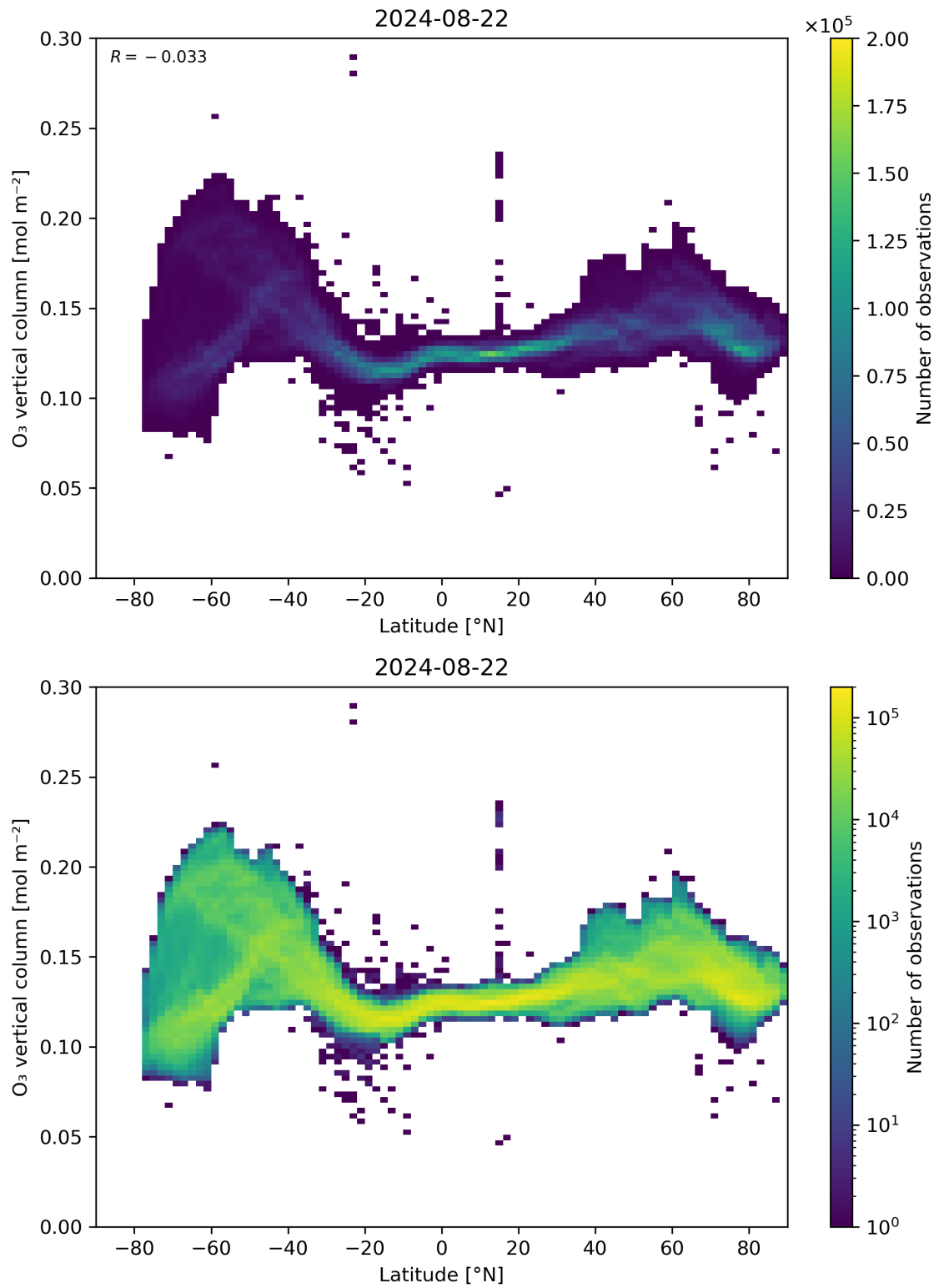
Figure 36: Scatter density plot of “Latitude” against “O 3 vertical column” for 2024-08-22 to 2024-08-23.
