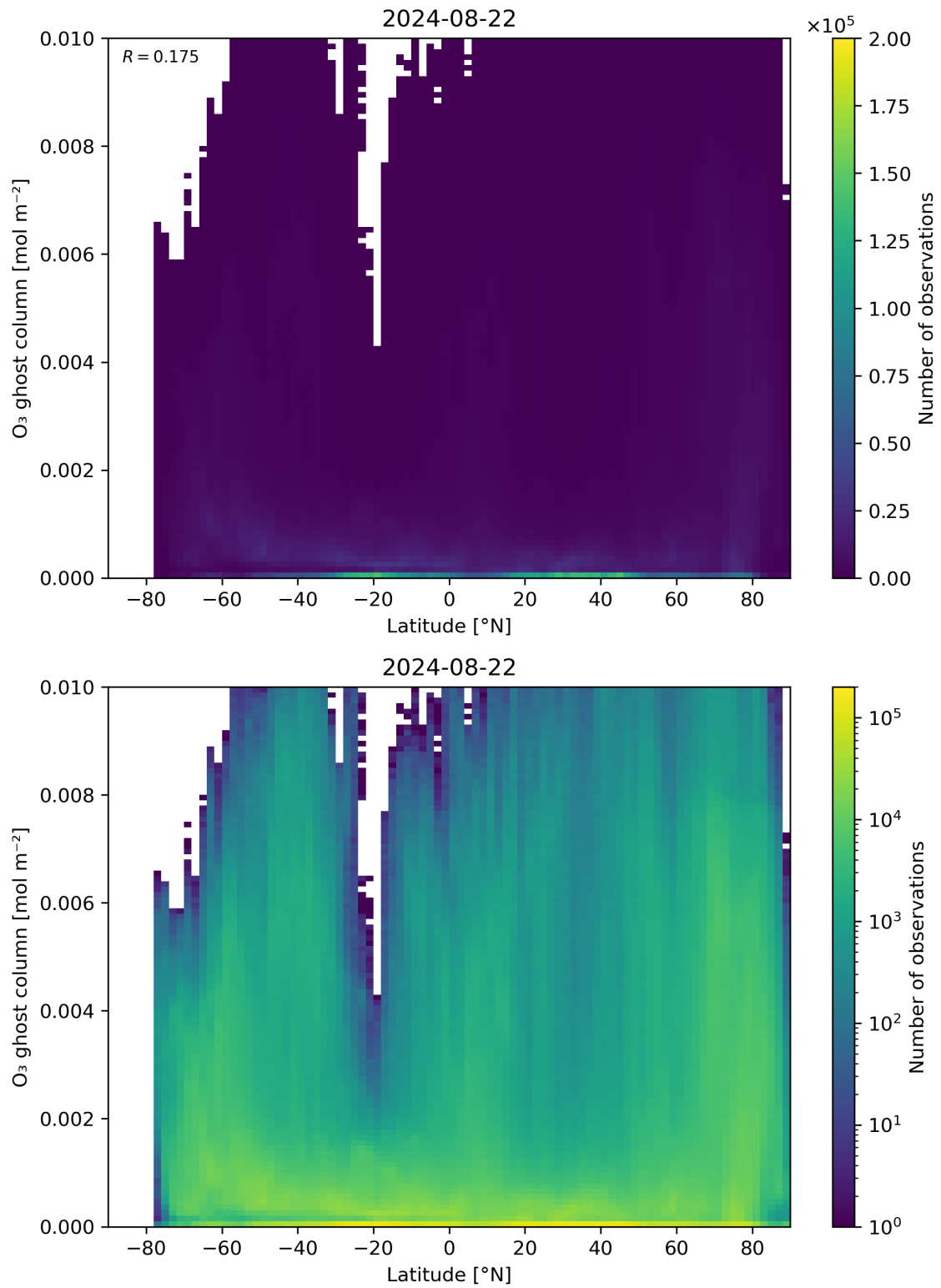
Figure 35: Scatter density plot of “Latitude” against “O 3 ghost column” for 2024-08-22 to 2024-08-23.
