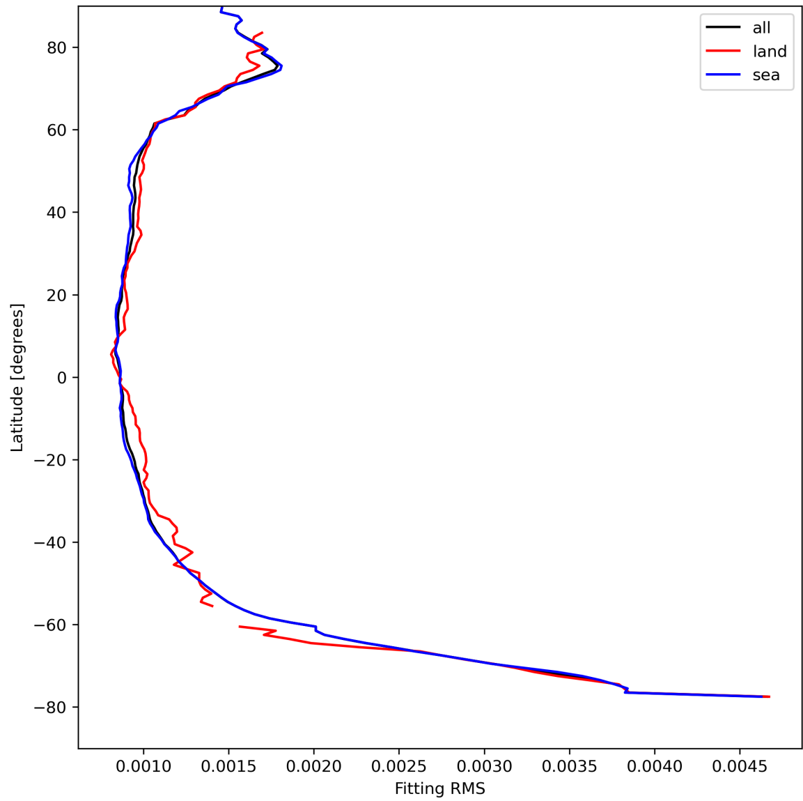
Figure 16: Zonal average of “Fitting RMS” for 2024-08-22 to 2024-08-23.
