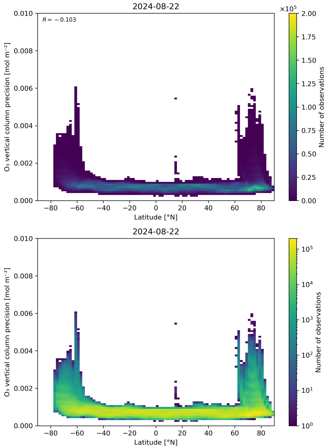
Figure 37: Scatter density plot of “Latitude” against “O 3 vertical column precision” for 2024-08-22 to 2024-08-23.
