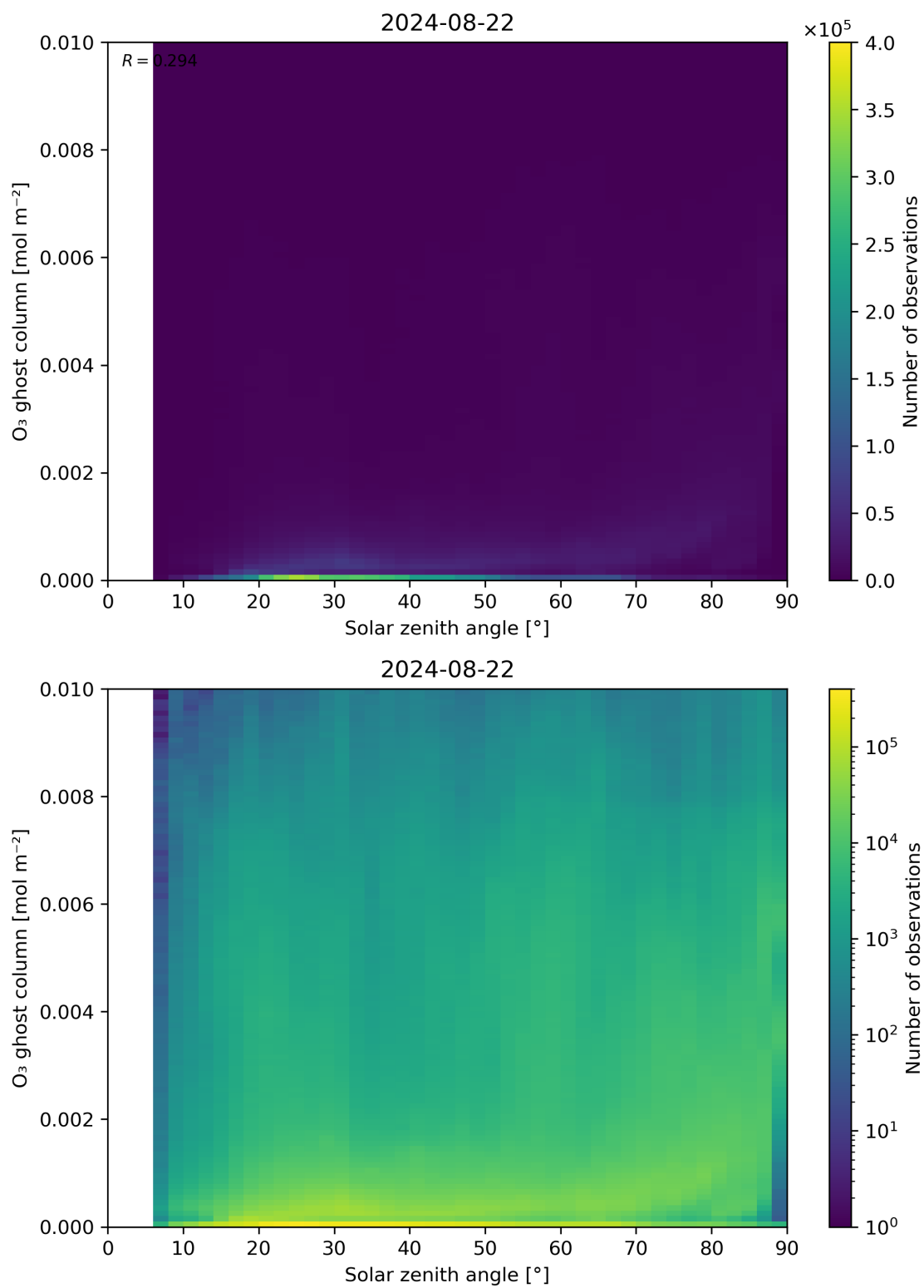
Figure 46: Scatter density plot of “Solar zenith angle” against “O 3 ghost column” for 2024-08-22 to 2024-08-23.
