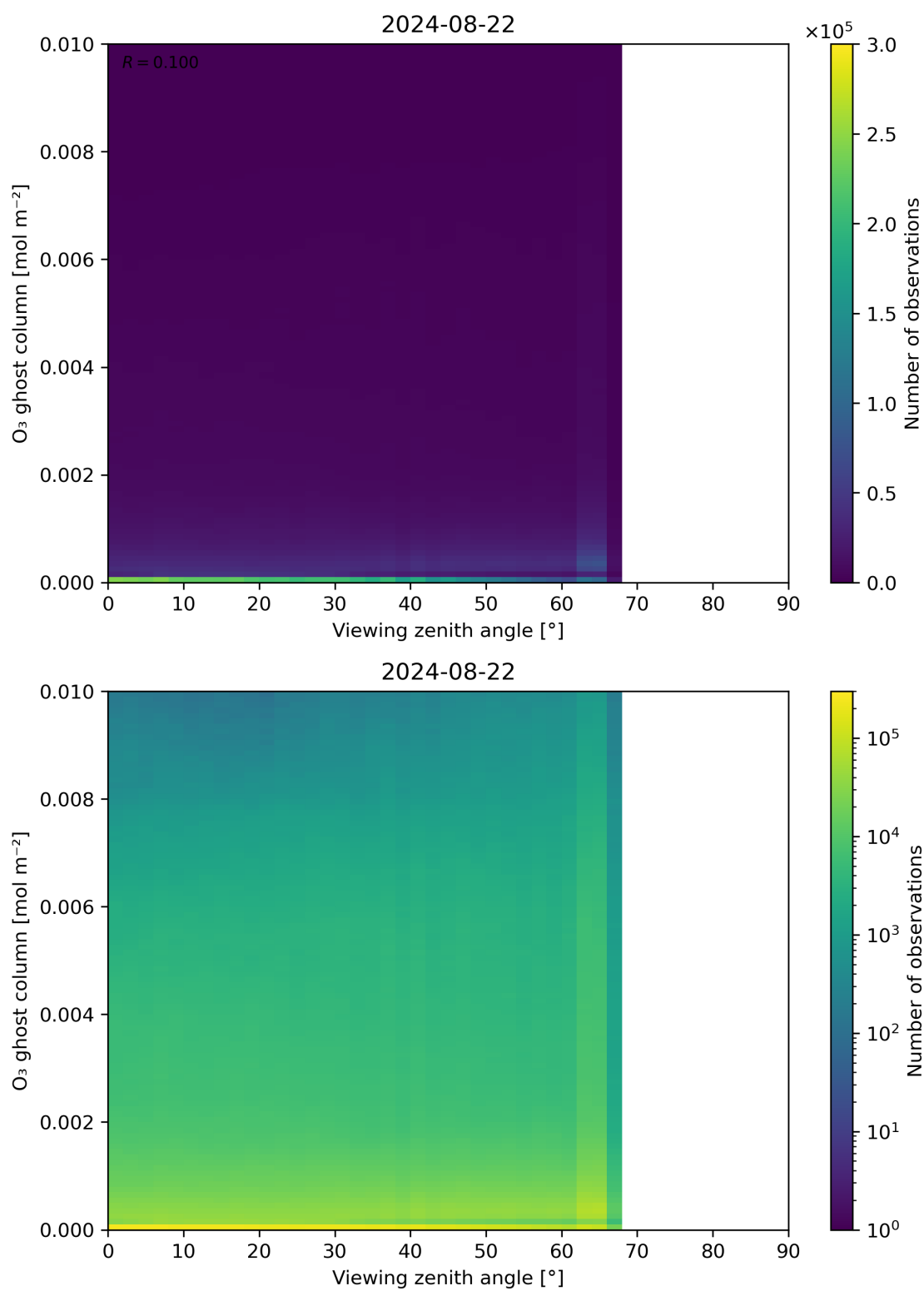
Figure 51: Scatter density plot of “Viewing zenith angle” against “O 3 ghost column” for 2024-08-22 to 2024-08-23.
