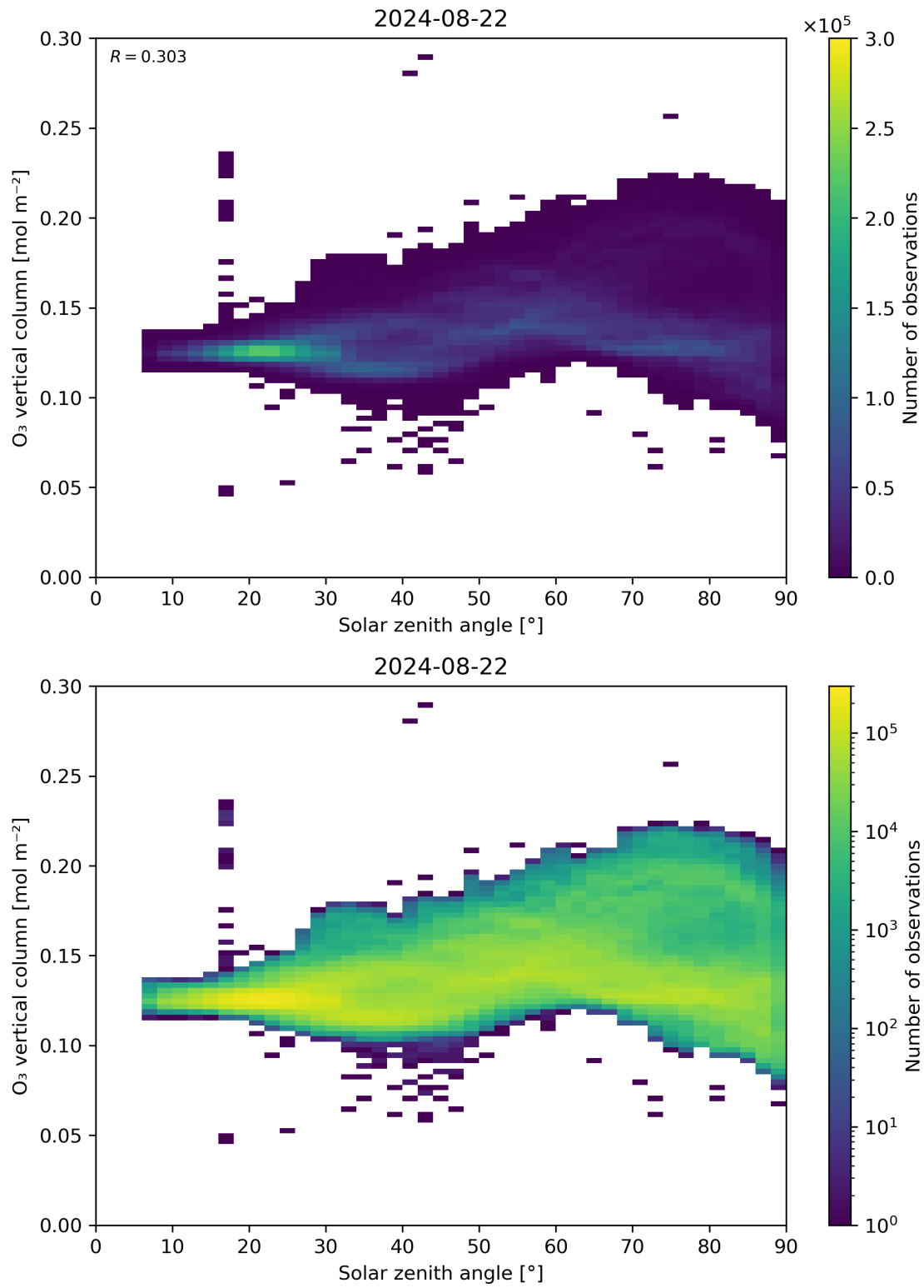
Figure 47: Scatter density plot of “Solar zenith angle” against “O 3 vertical column” for 2024-08-22 to 2024-08-23.
