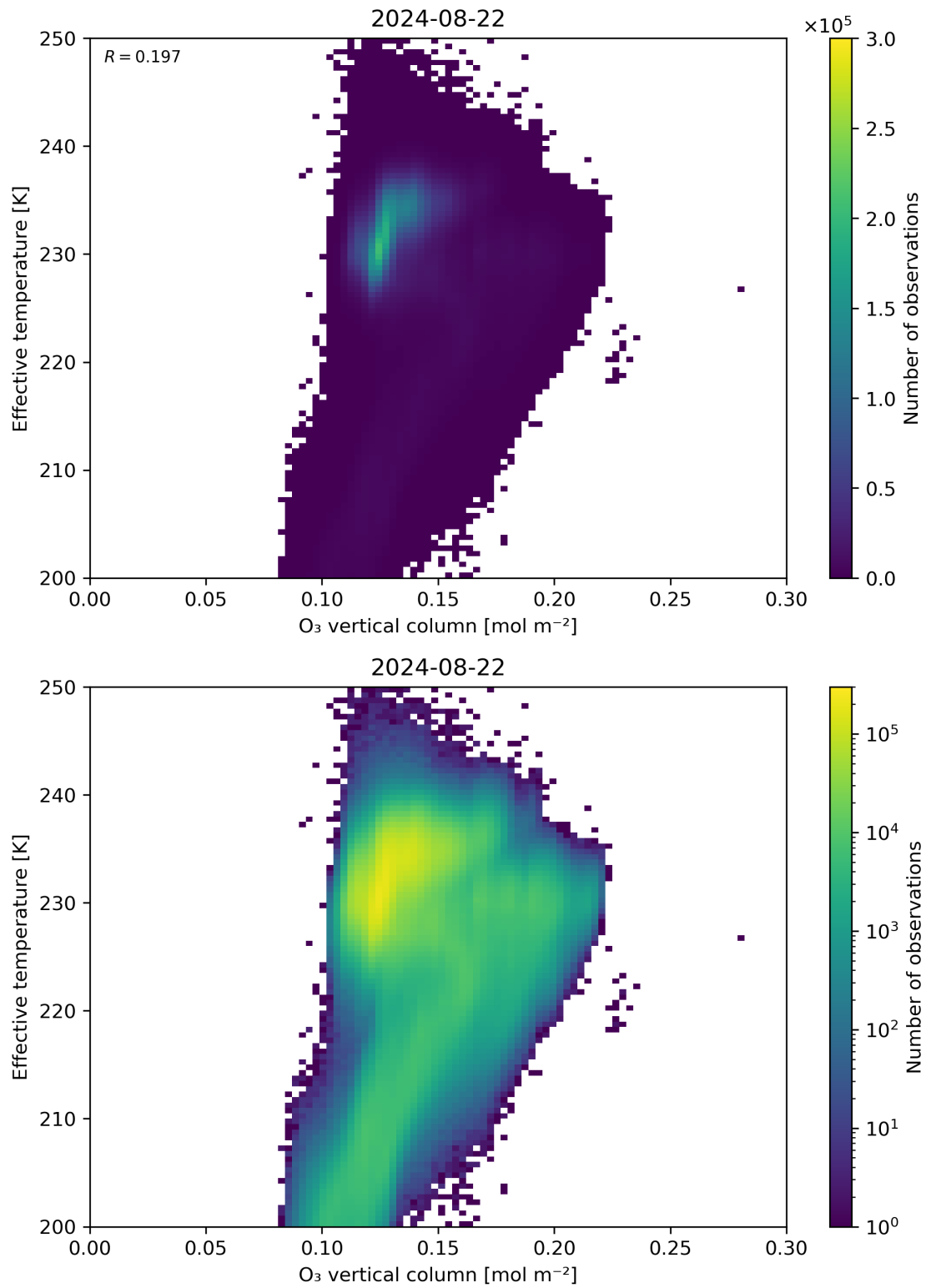
Figure 39: Scatter density plot of “O 3 vertical column” against “Effective temperature” for 2024-08-22 to 2024-08-23.
