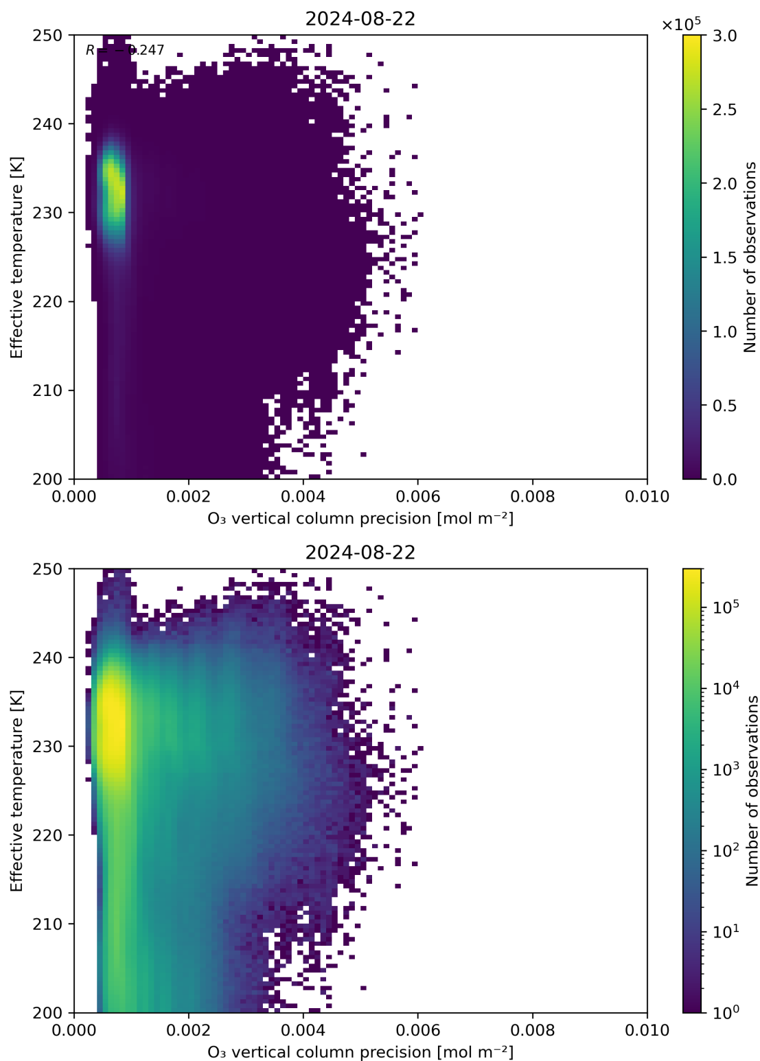
Figure 42: Scatter density plot of “O 3 vertical column precision” against “Effective temperature” for 2024-08-22 to 2024-08-23.
