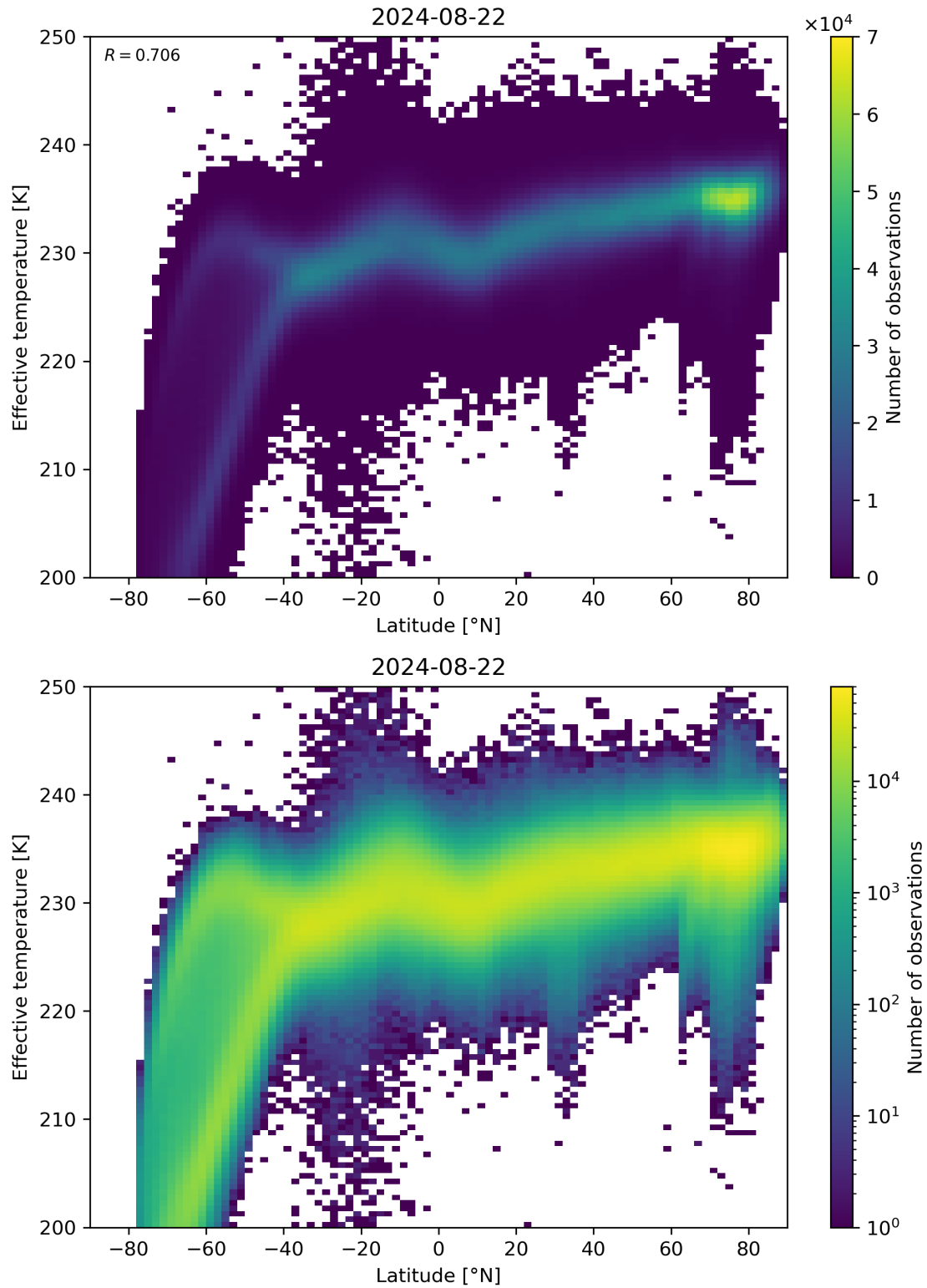
Figure 34: Scatter density plot of “Latitude” against “Effective temperature” for 2024-08-22 to 2024-08-23.
