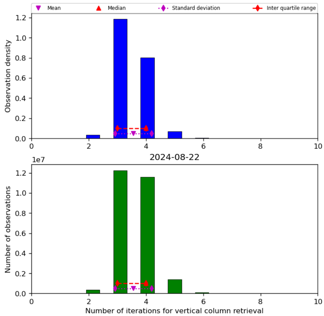
Figure 26: Histogram of “Number of iterations for vertical column retrieval” for 2024-08-22 to 2024-08-23
