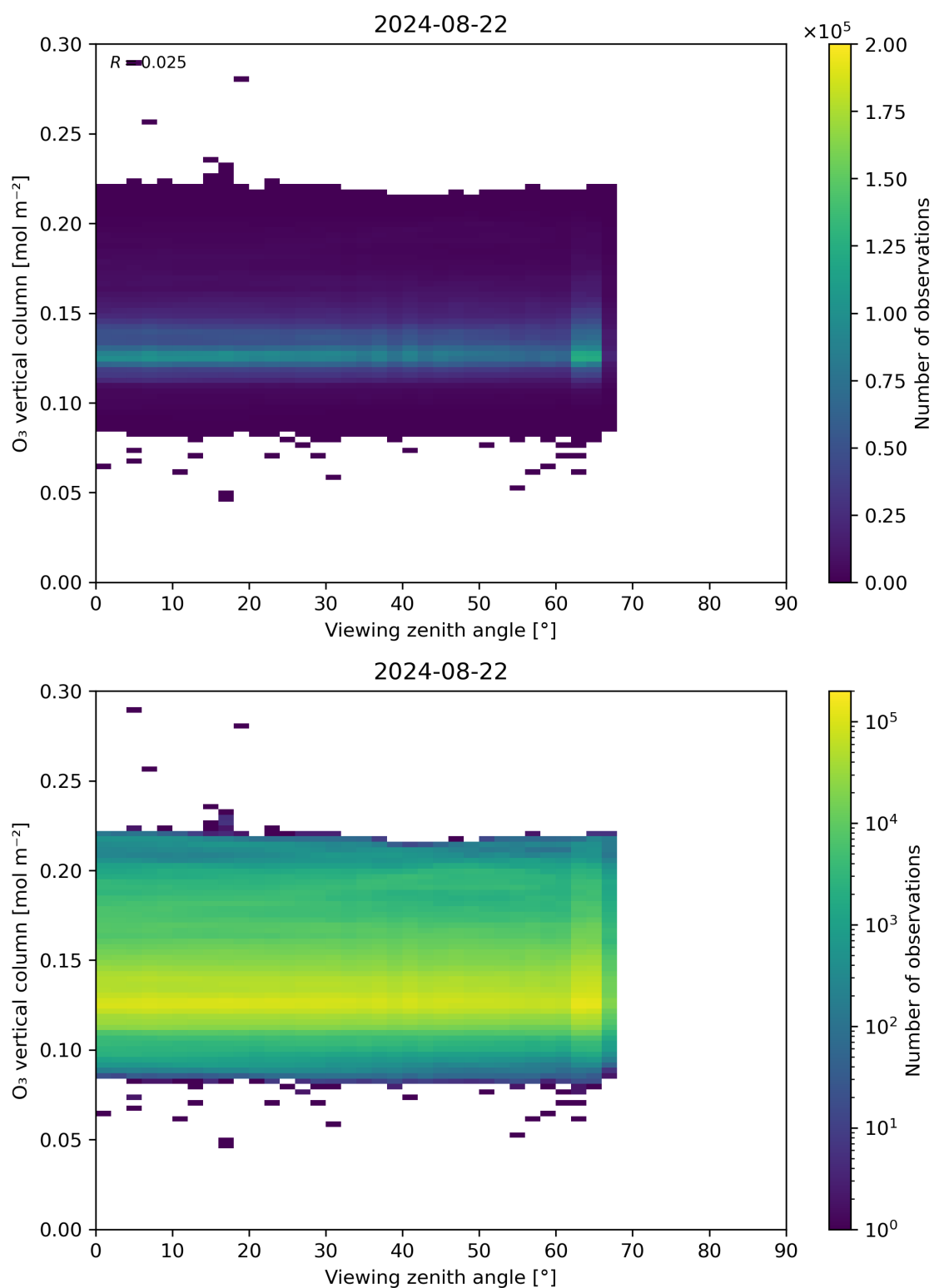
Figure 52: Scatter density plot of “Viewing zenith angle” against “O 3 vertical column” for 2024-08-22 to 2024-08-23.
