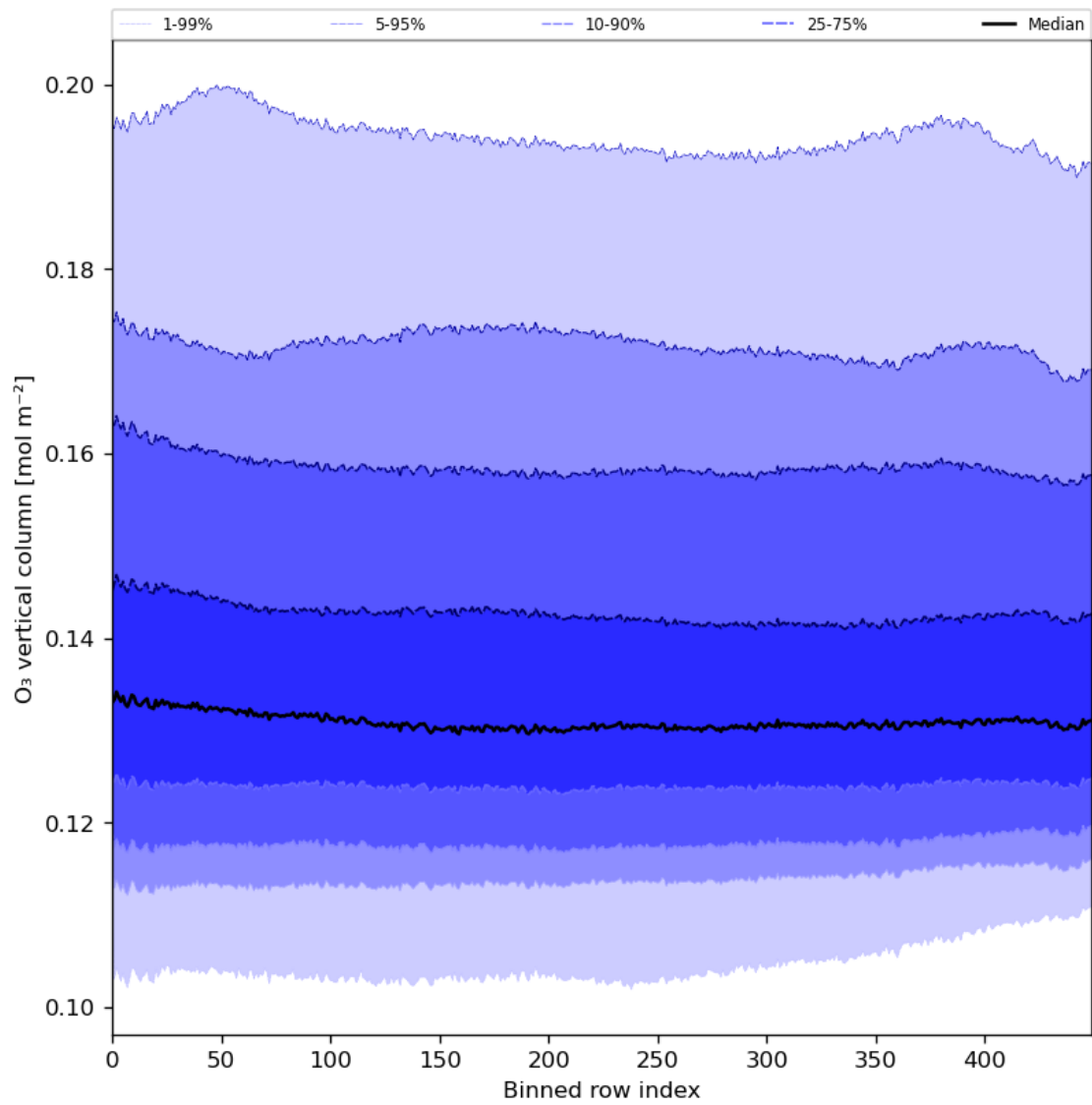
Figure 28: Along track statistics of “ \text{O}_3 vertical column” for 2024-08-22 to 2024-08-23
