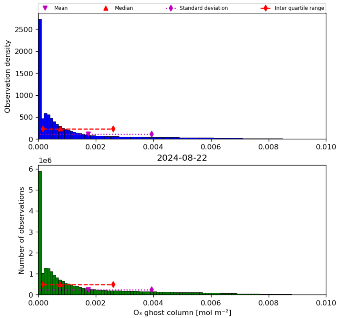
Figure 25: Histogram of “O 3 ghost column” for 2024-08-22 to 2024-08-23
