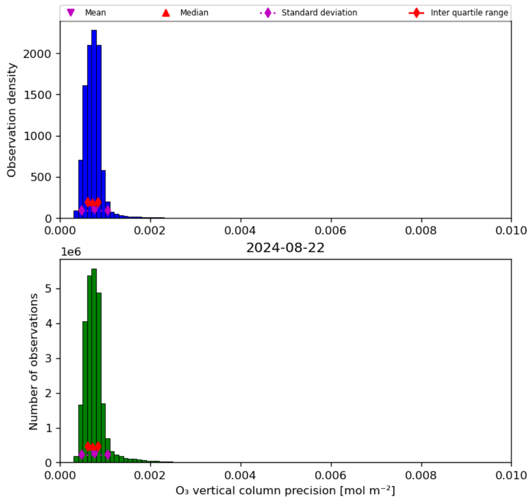
Figure 22: Histogram of “O 3 vertical column precision” for 2024-08-22 to 2024-08-23
