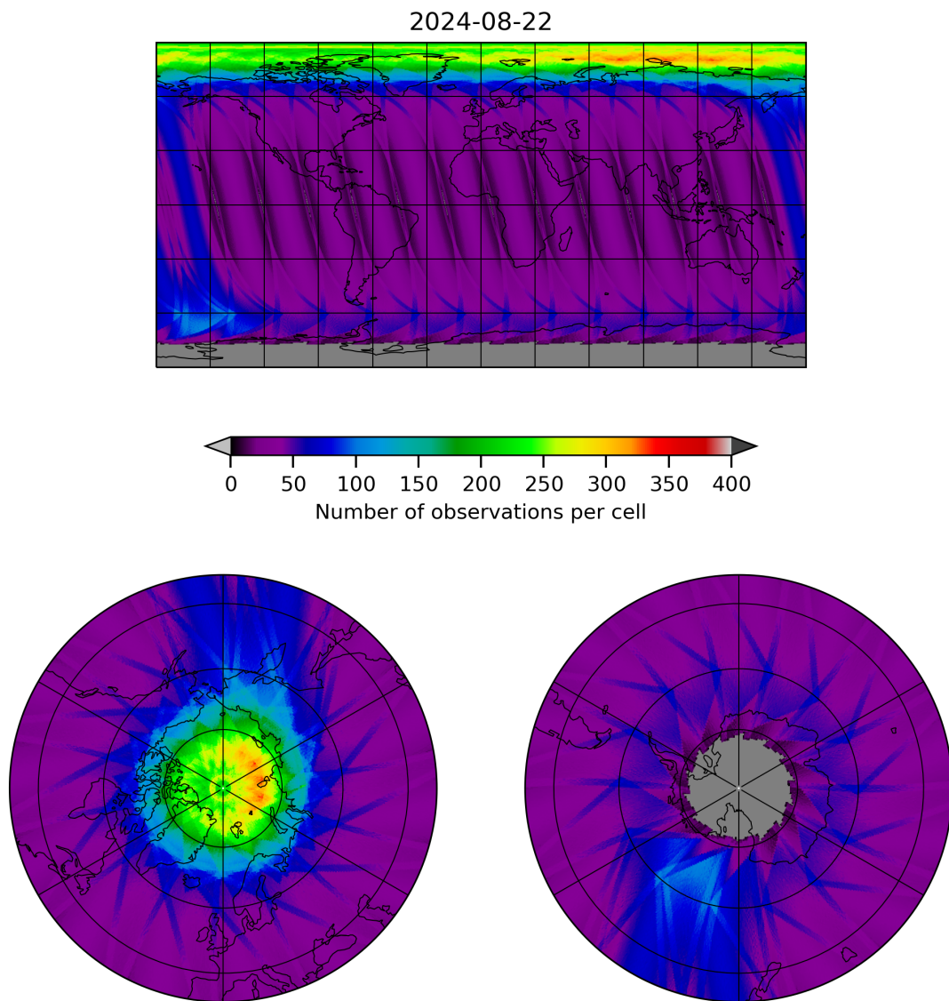
Figure 12: Map of the number of observations for 2024-08-22 to 2024-08-23
