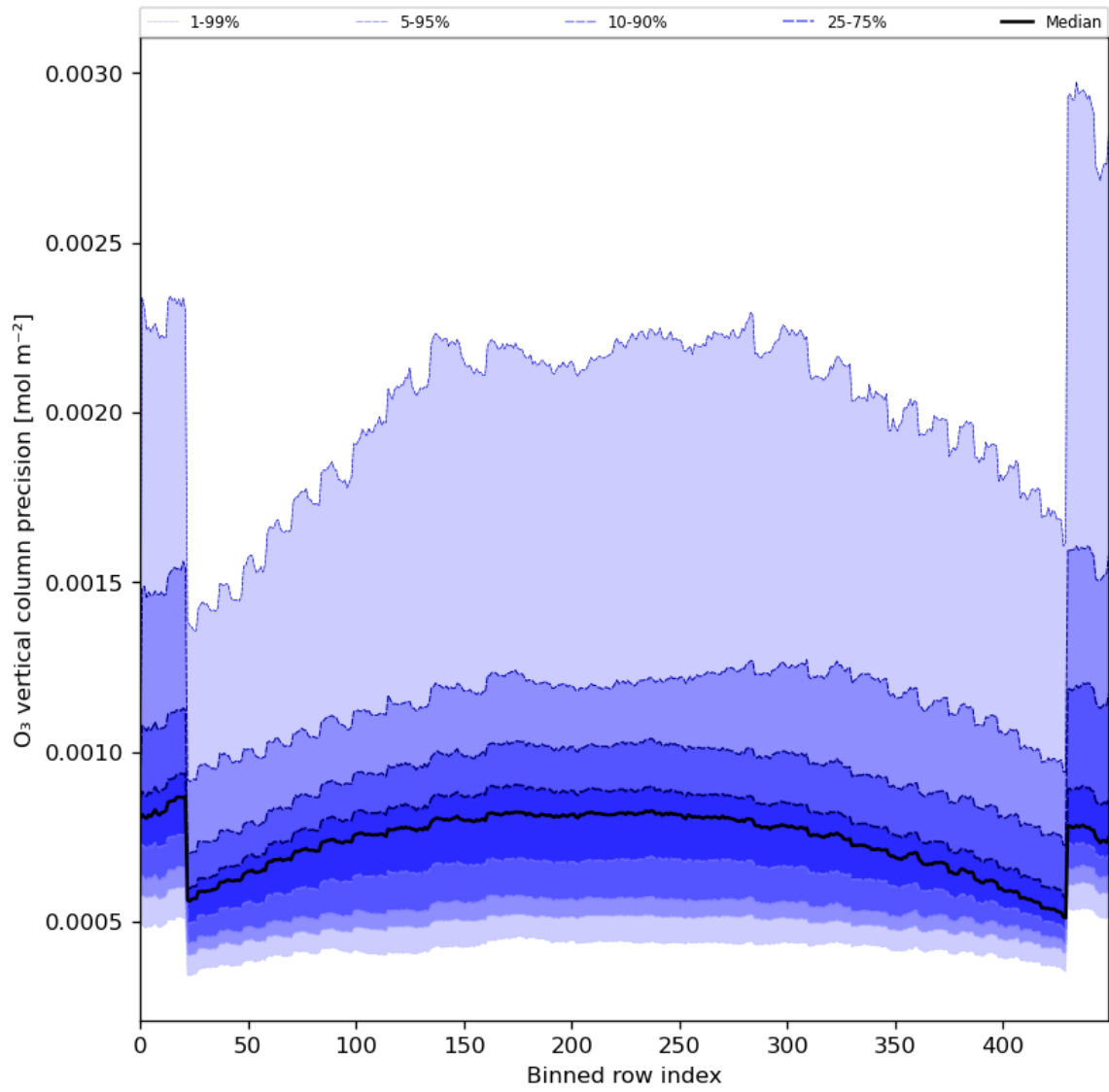
Figure 29: Along track statistics of “O 3 vertical column precision” for 2024-08-22 to 2024-08-23
