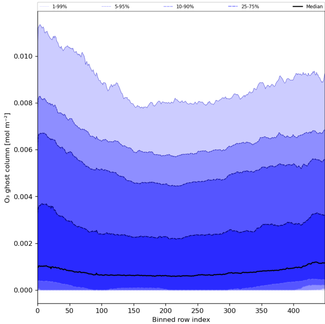
Figure 32: Along track statistics of “O 3 ghost column” for 2024-08-22 to 2024-08-23
