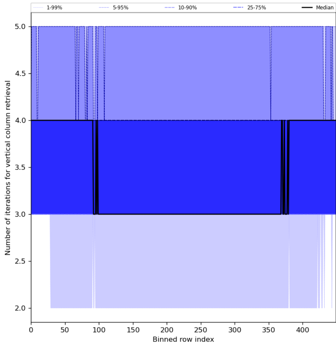
Figure 33: Along track statistics of “Number of iterations for vertical column retrieval” for 2024-08-22 to 2024-08-23
