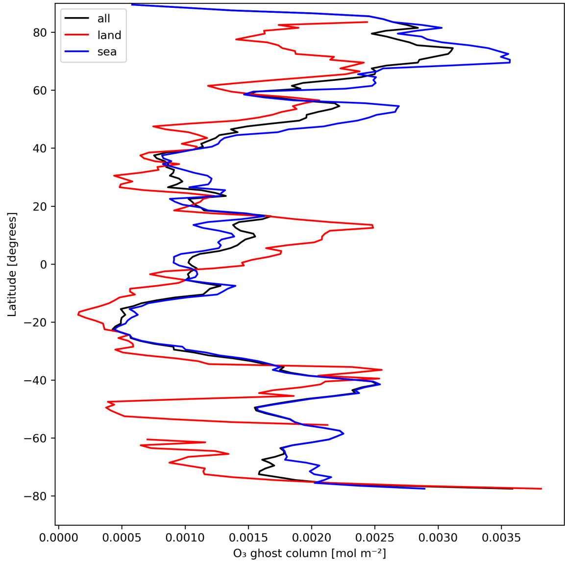
Figure 18: Zonal average of "O 3 ghost column" for 2024-08-22 to 2024-08-24.
