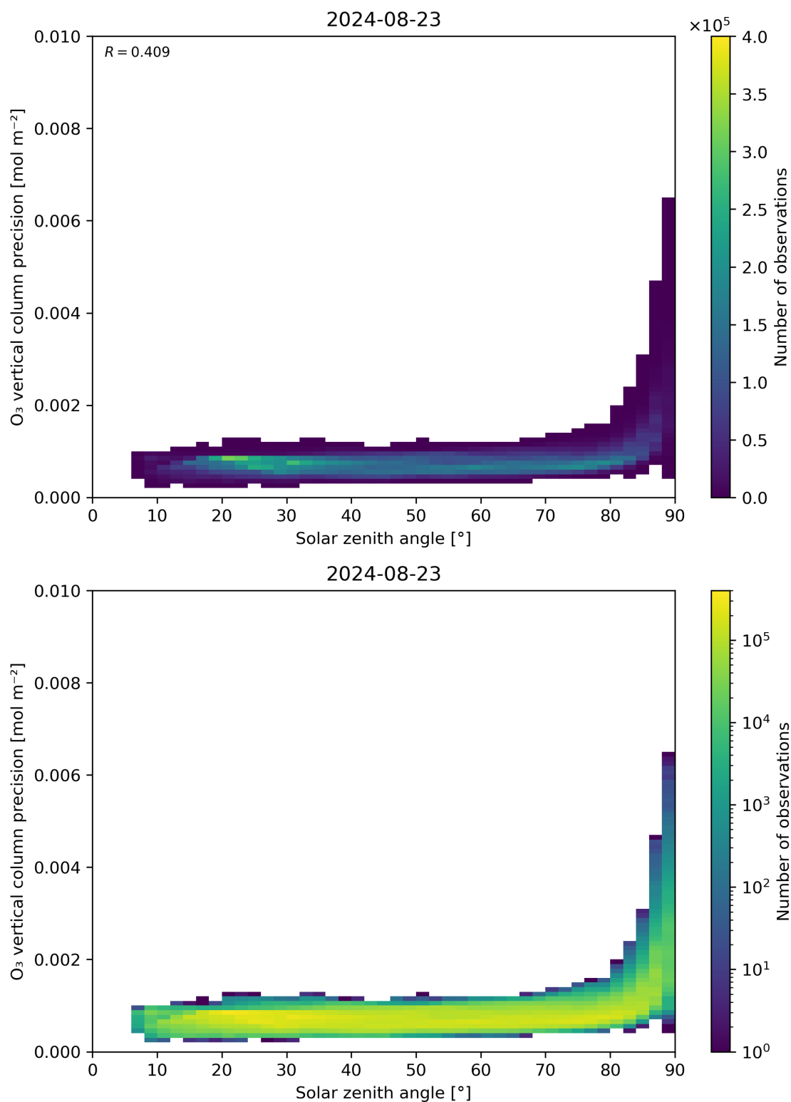
Figure 48: Scatter density plot of “Solar zenith angle” against “O 3 vertical column precision” for 2024-08-22 to 2024-08-24.
