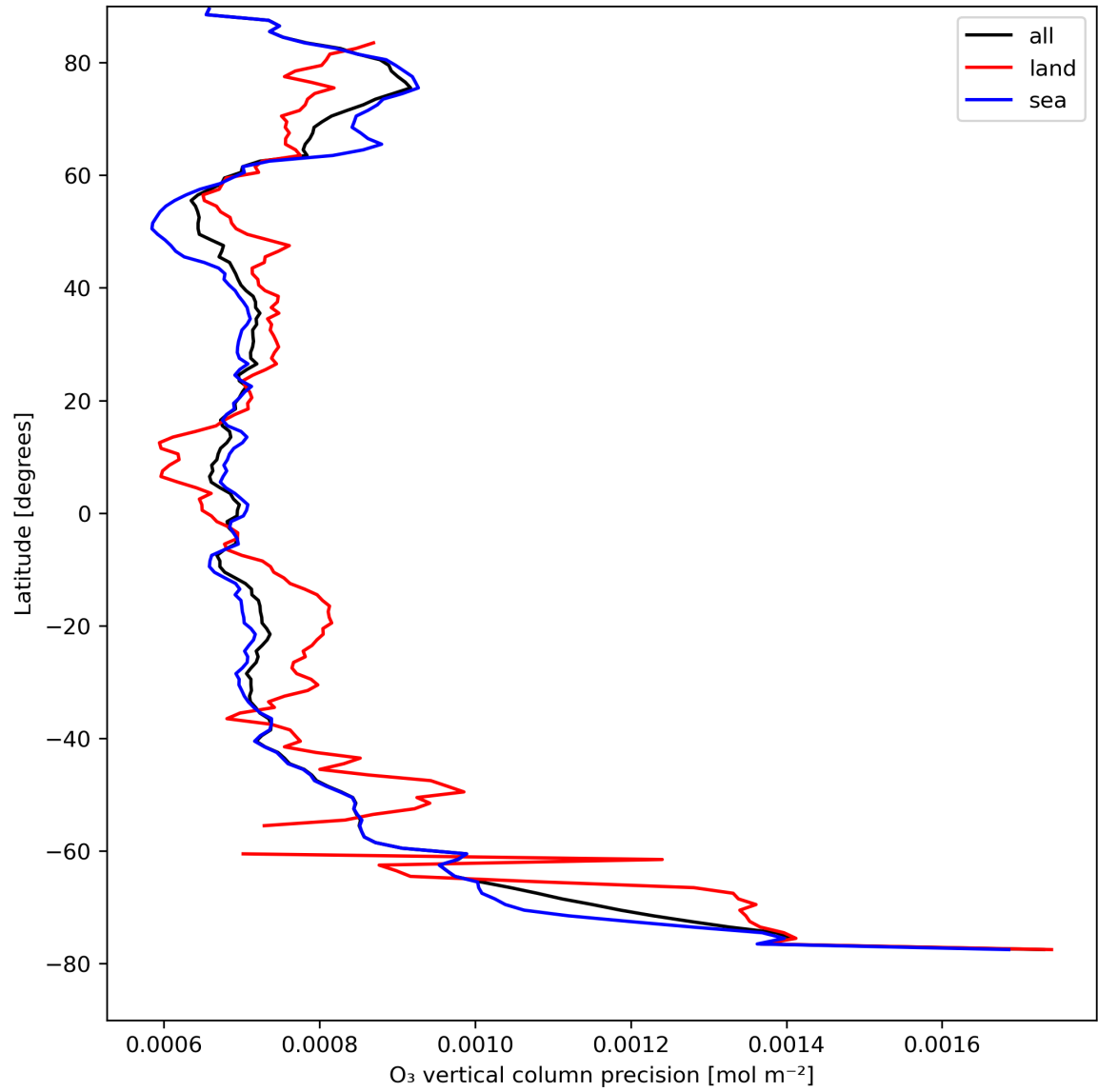
Figure 15: Zonal average of “O 3 vertical column precision” for 2024-08-22 to 2024-08-24.
