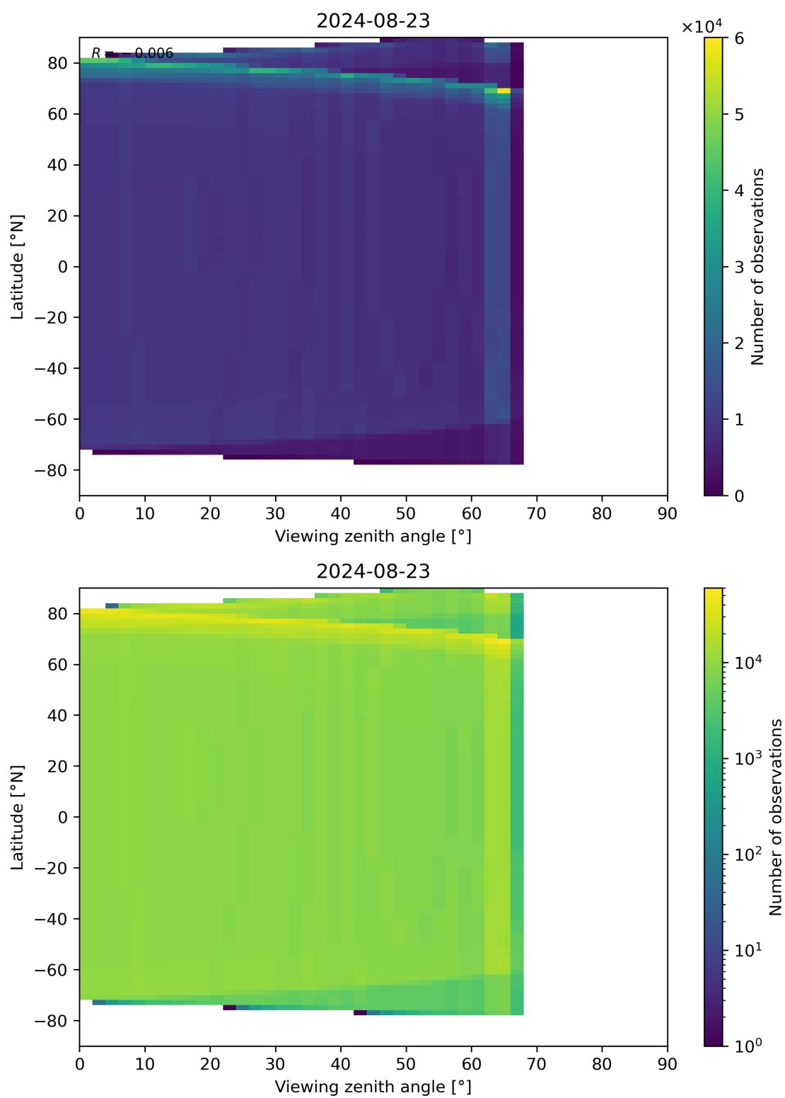
Figure 49: Scatter density plot of “Viewing zenith angle” against “Latitude” for 2024-08-22 to 2024-08-24.
