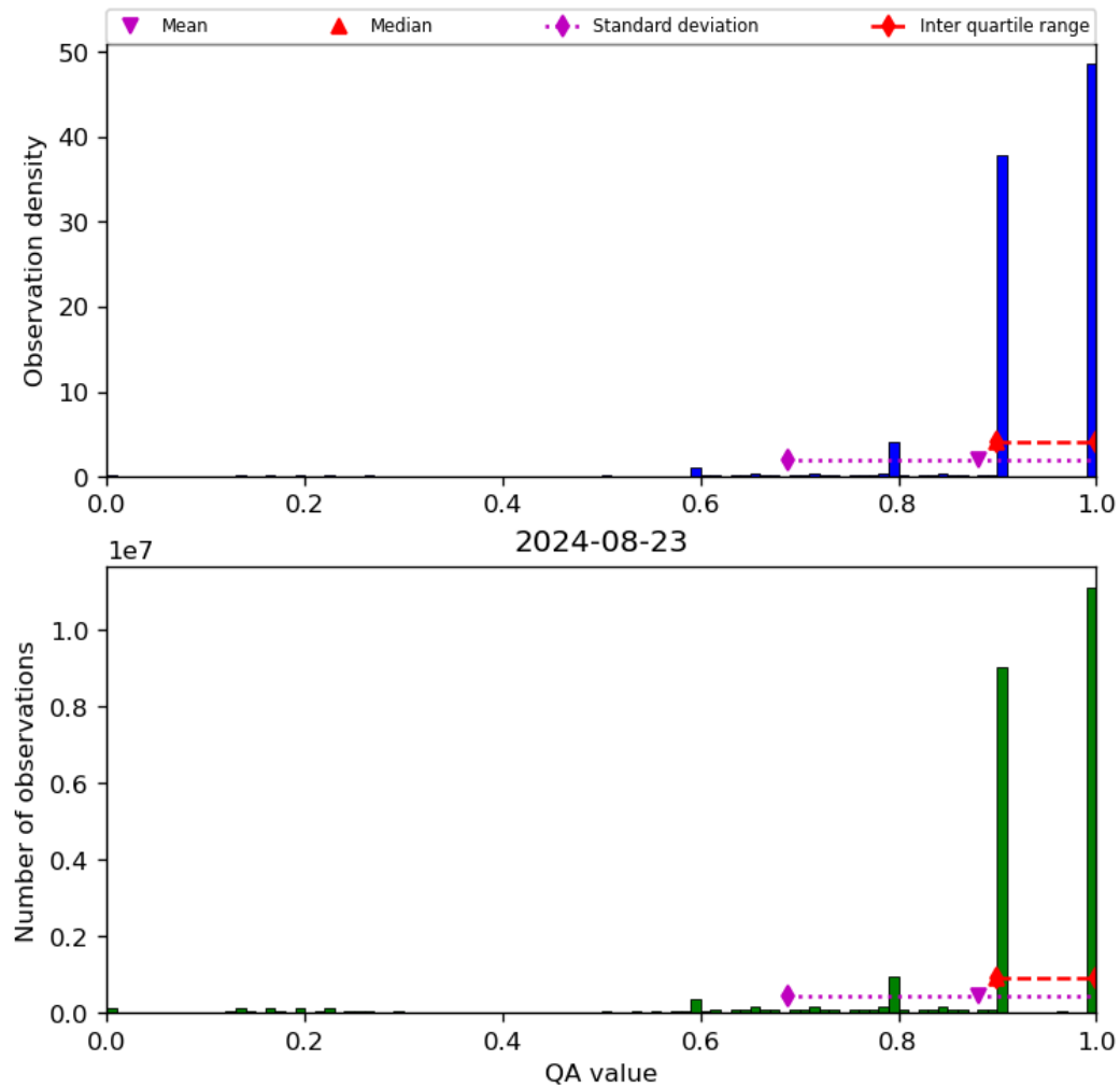
Figure 20: Histogram of “QA value” for 2024-08-22 to 2024-08-24
