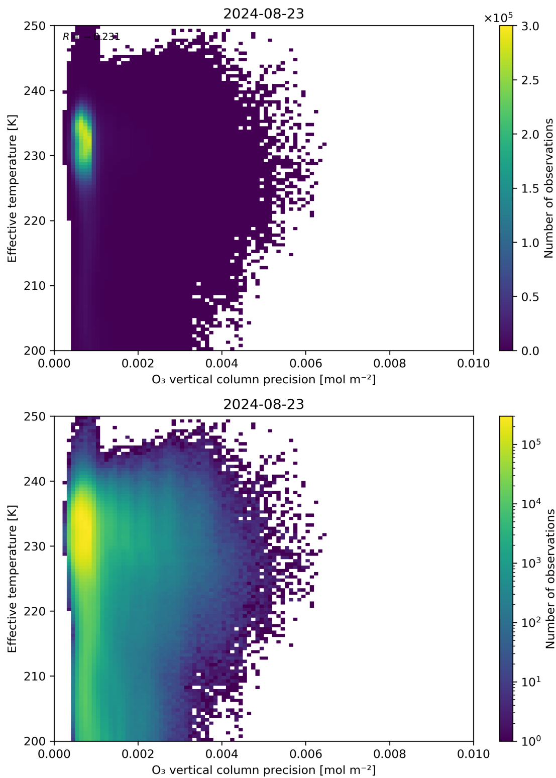
Figure 42: Scatter density plot of “O 3 vertical column precision” against “Effective temperature” for 2024-08-22 to 2024-08-24.
