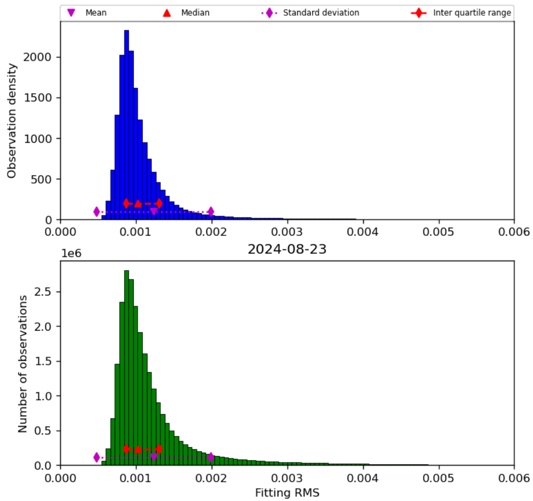
Figure 23: Histogram of “Fitting RMS” for 2024-08-22 to 2024-08-24
