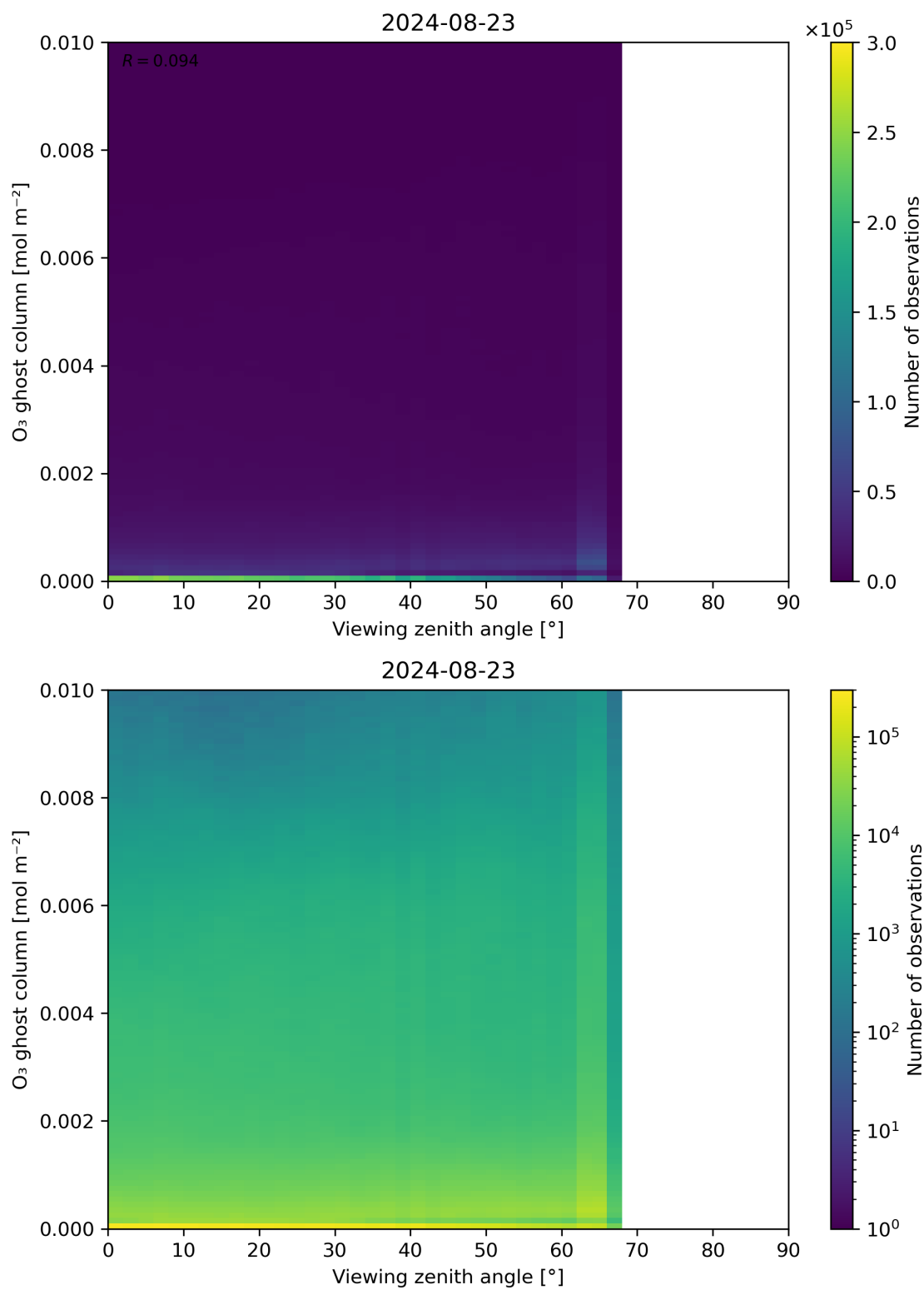
Figure 51: Scatter density plot of “Viewing zenith angle” against “O 3 ghost column” for 2024-08-22 to 2024-08-24.
