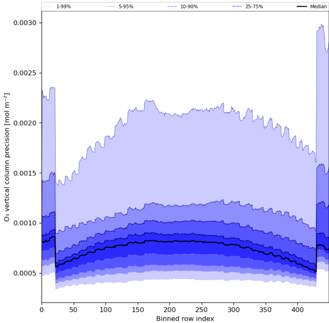
Figure 29: Along track statistics of “O 3 vertical column precision” for 2024-08-22 to 2024-08-24
