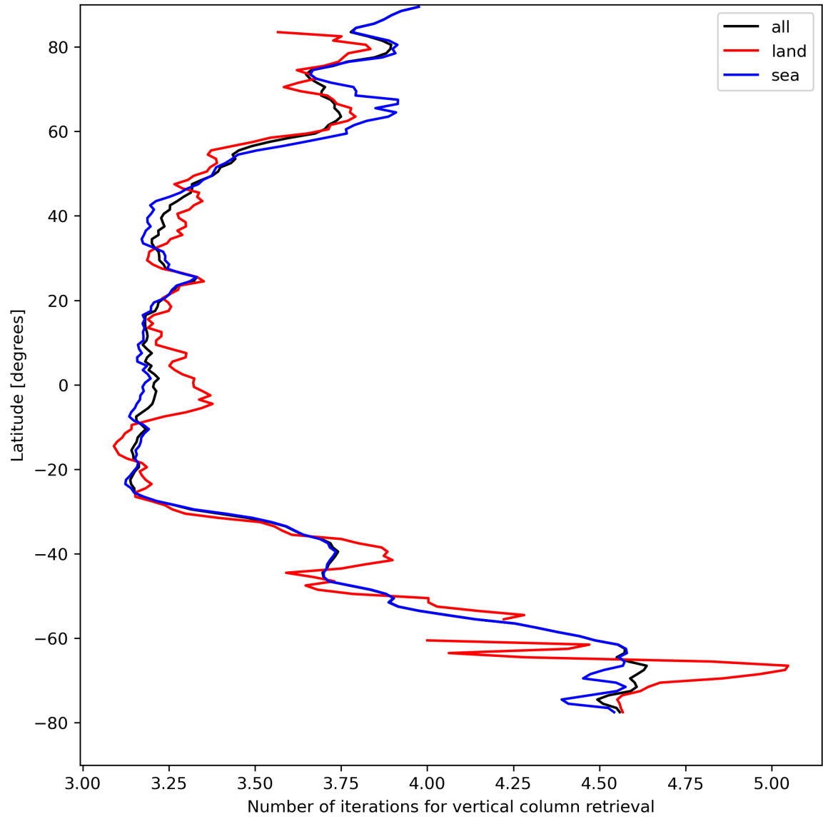
Figure 19: Zonal average of “Number of iterations for vertical column retrieval” for 2024-08-22 to 2024-08-24.
