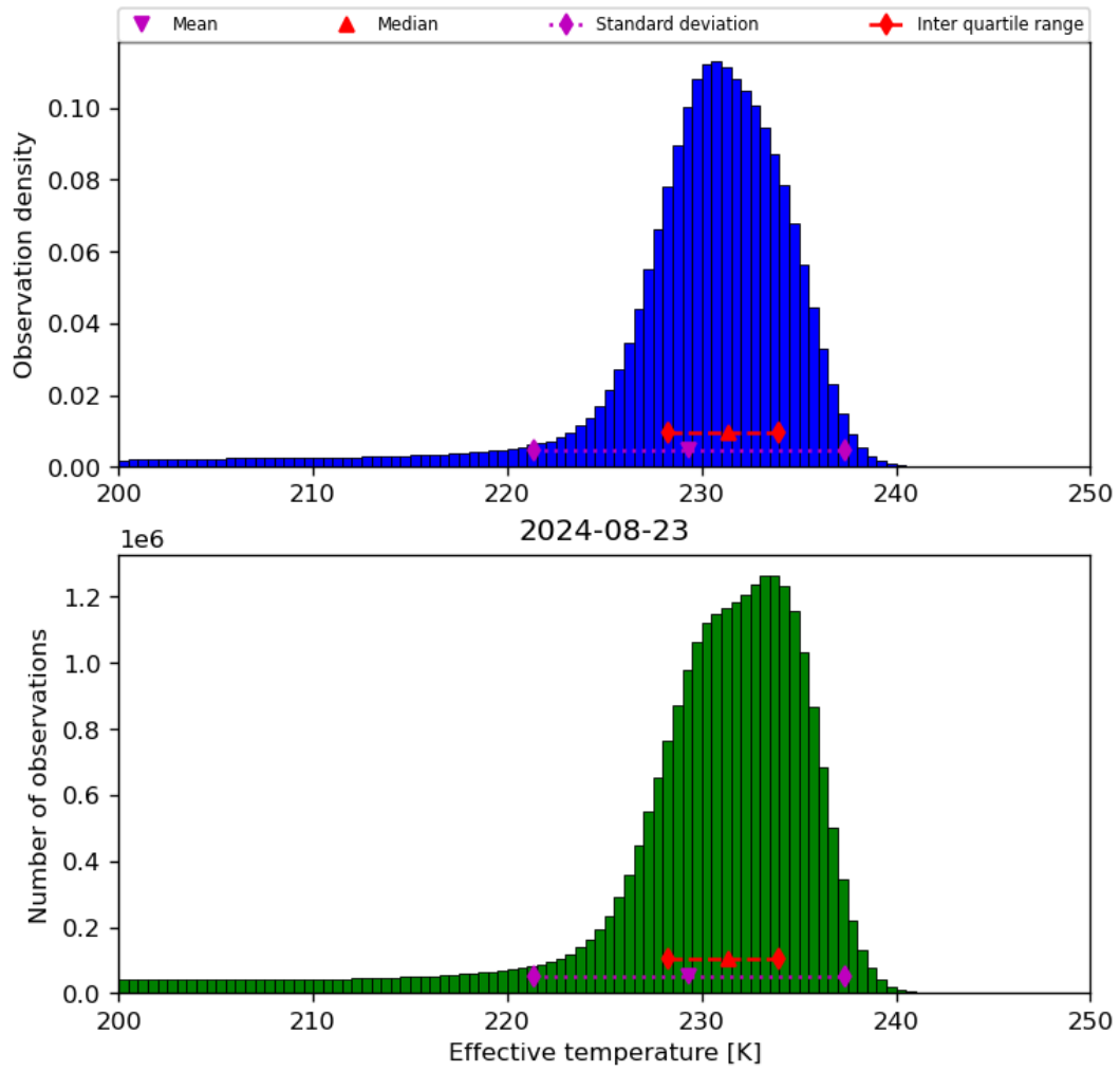
Figure 24: Histogram of “Effective temperature” for 2024-08-22 to 2024-08-24
