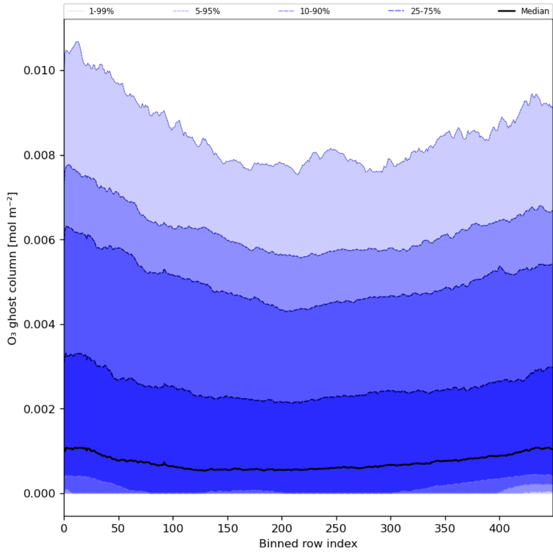
Figure 32: Along track statistics of “O 3 ghost column” for 2024-08-22 to 2024-08-24
