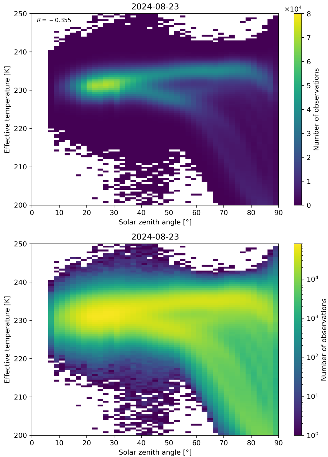
Figure 45: Scatter density plot of “Solar zenith angle” against “Effective temperature” for 2024-08-22 to 2024-08-24.
