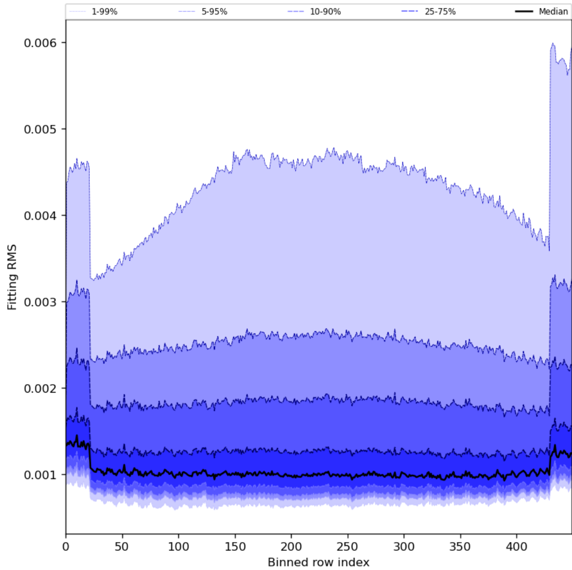
Figure 30: Along track statistics of “Fitting RMS” for 2024-08-22 to 2024-08-24
