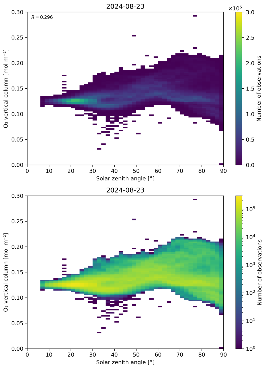
Figure 47: Scatter density plot of “Solar zenith angle” against “O 3 vertical column” for 2024-08-22 to 2024-08-24.
