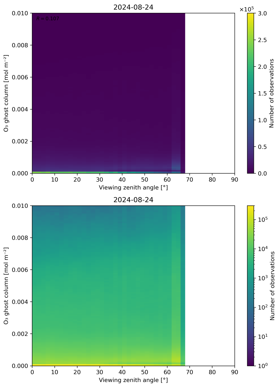
Figure 51: Scatter density plot of “Viewing zenith angle” against “O 3 ghost column” for 2024-08-23 to 2024-08-25.
