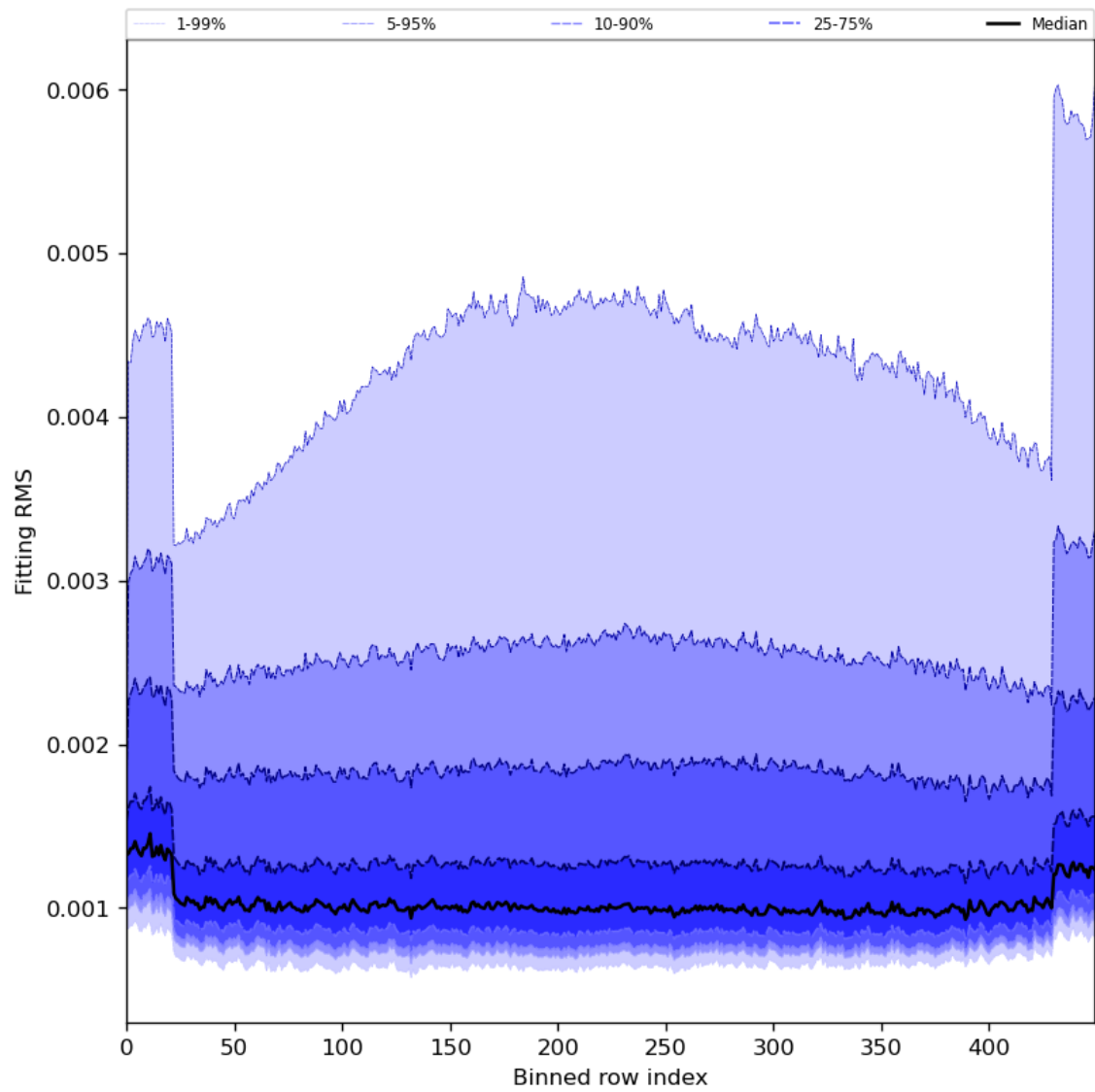
Figure 30: Along track statistics of “Fitting RMS” for 2024-08-23 to 2024-08-25
