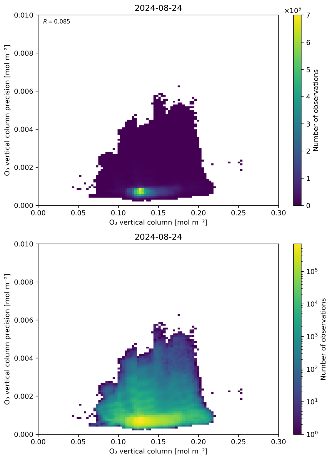
Figure 41: Scatter density plot of “O 3 vertical column” against “O 3 vertical column precision” for 2024-08-23 to 2024-08-25.
