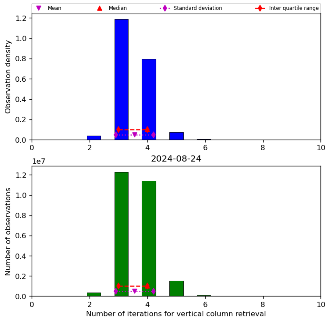
Figure 26: Histogram of “Number of iterations for vertical column retrieval” for 2024-08-23 to 2024-08-25
