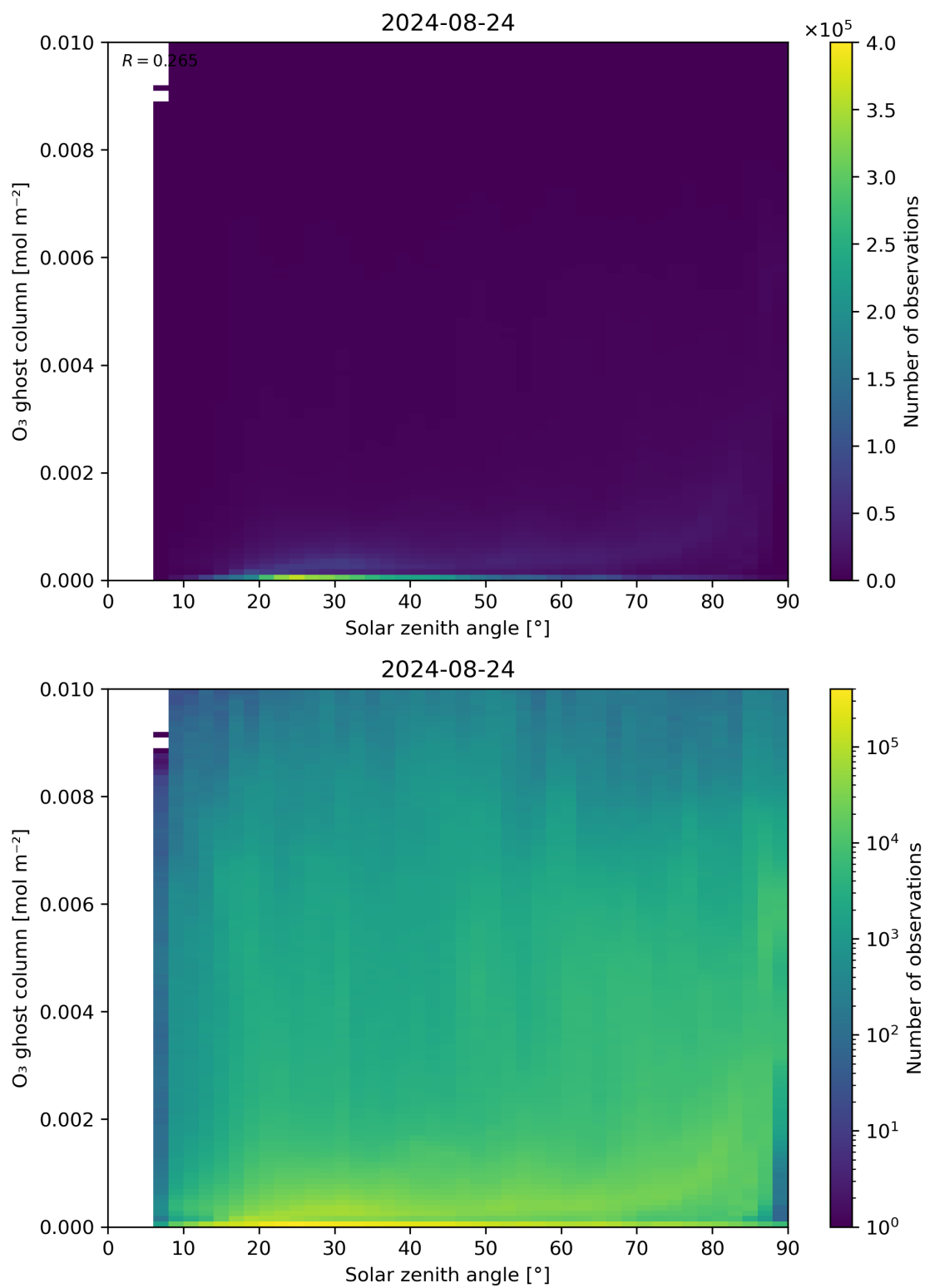
Figure 46: Scatter density plot of “Solar zenith angle” against “O 3 ghost column” for 2024-08-23 to 2024-08-25.
