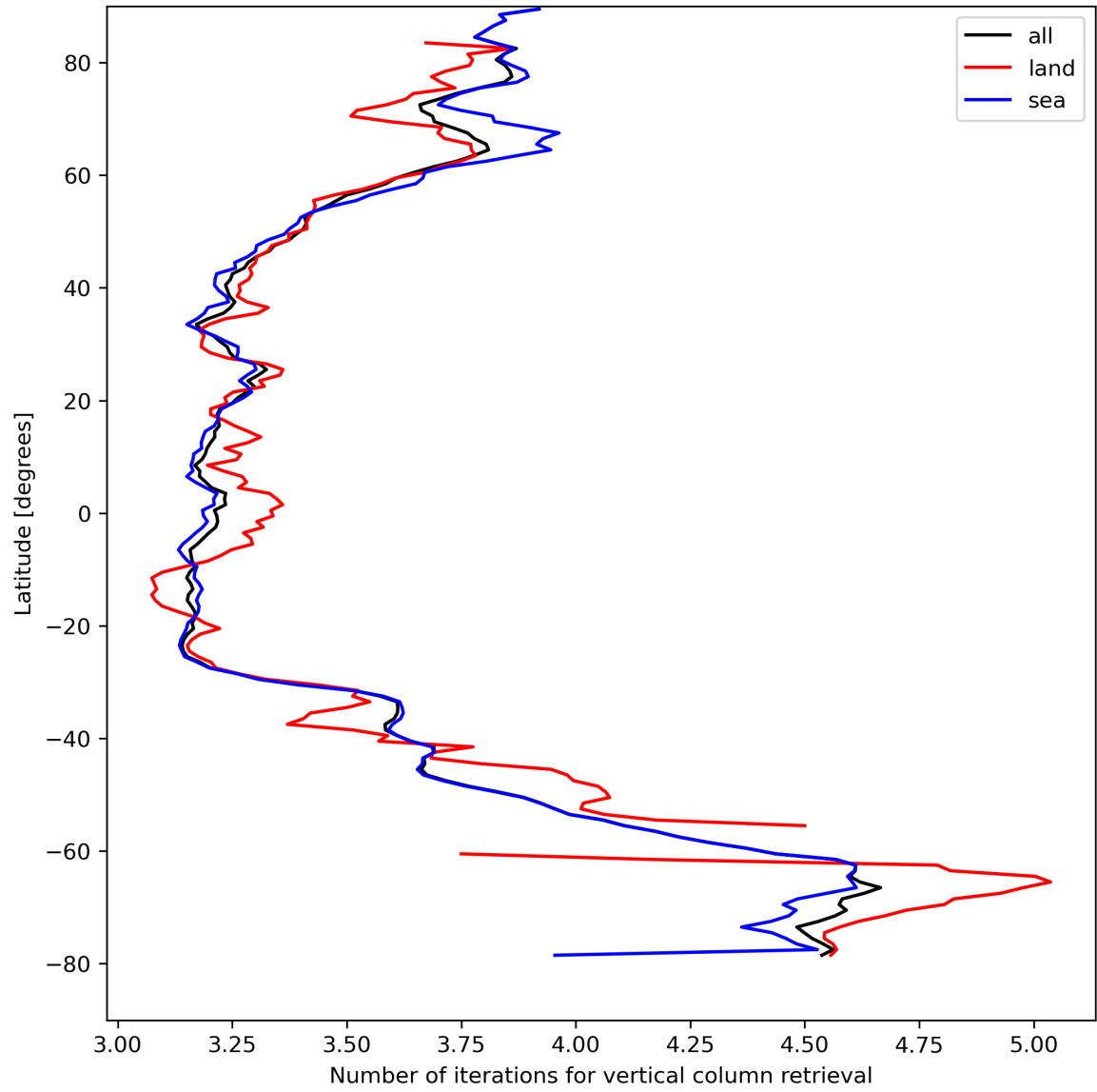
Figure 19: Zonal average of “Number of iterations for vertical column retrieval” for 2024-08-23 to 2024-08-25.
