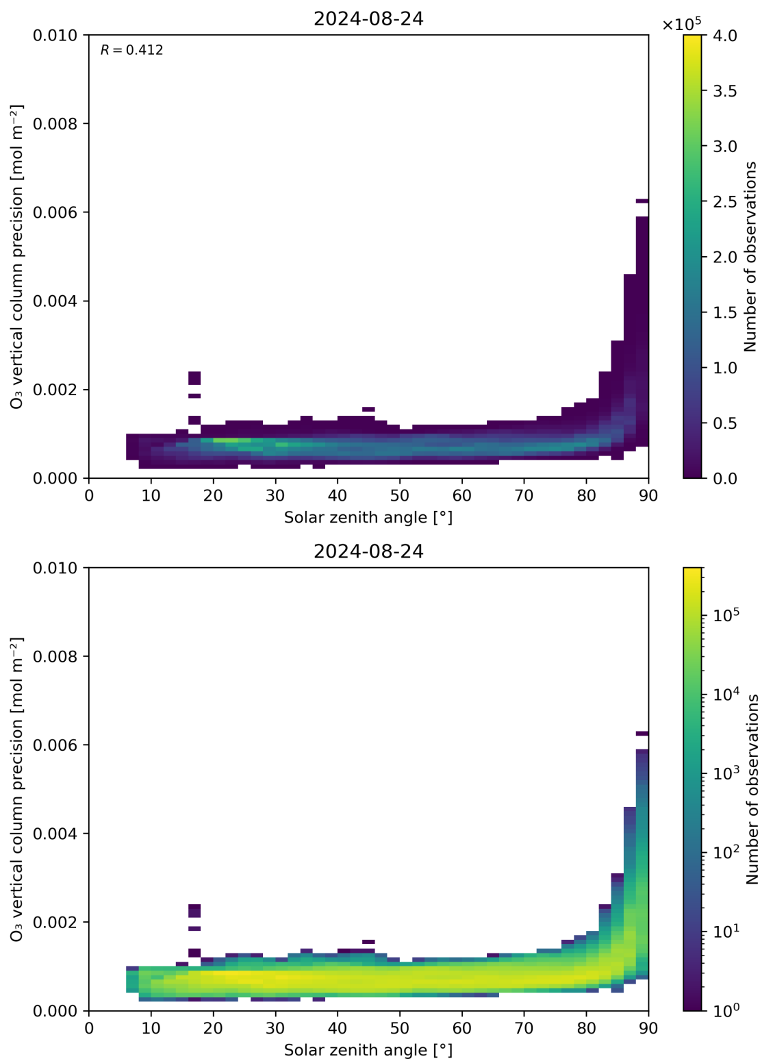
Figure 48: Scatter density plot of “Solar zenith angle” against “O 3 vertical column precision” for 2024-08-23 to 2024-08-25.
