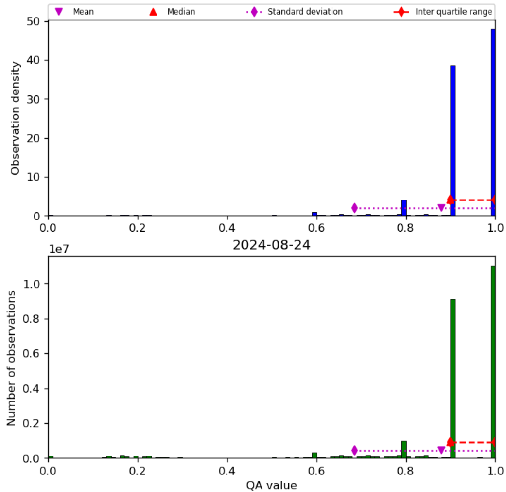
Figure 20: Histogram of “QA value” for 2024-08-23 to 2024-08-25
