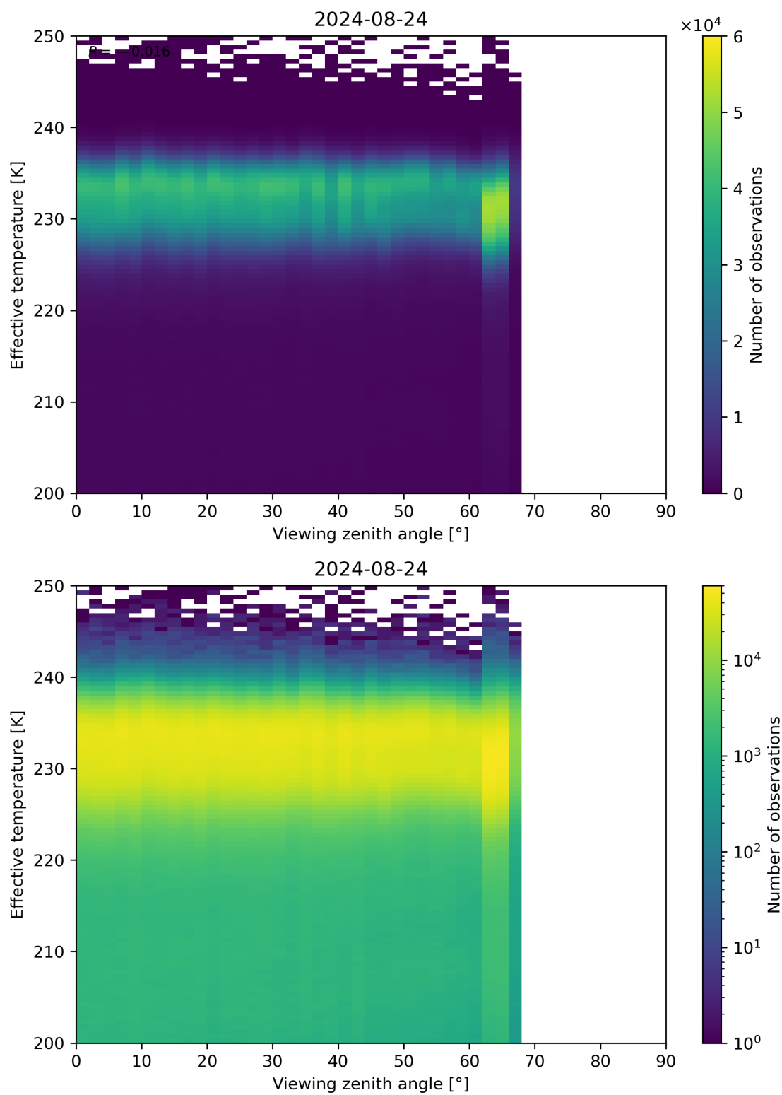
Figure 50: Scatter density plot of “Viewing zenith angle” against “Effective temperature” for 2024-08-23 to 2024-08-25.
