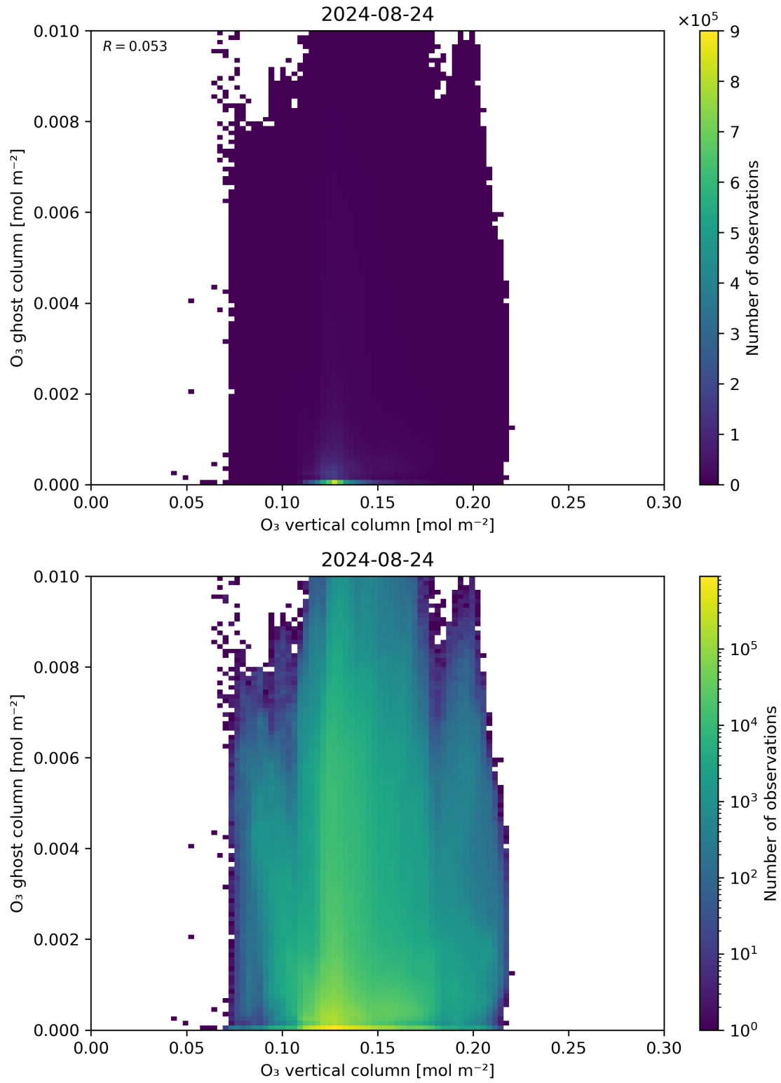
Figure 40: Scatter density plot of “O 3 vertical column” against “O 3 ghost column” for 2024-08-23 to 2024-08-25.
