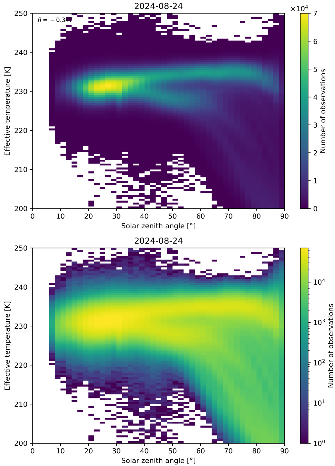
Figure 45: Scatter density plot of “Solar zenith angle” against “Effective temperature” for 2024-08-23 to 2024-08-25.
