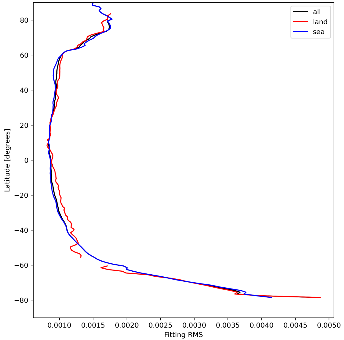
Figure 16: Zonal average of “Fitting RMS” for 2024-08-23 to 2024-08-25.
