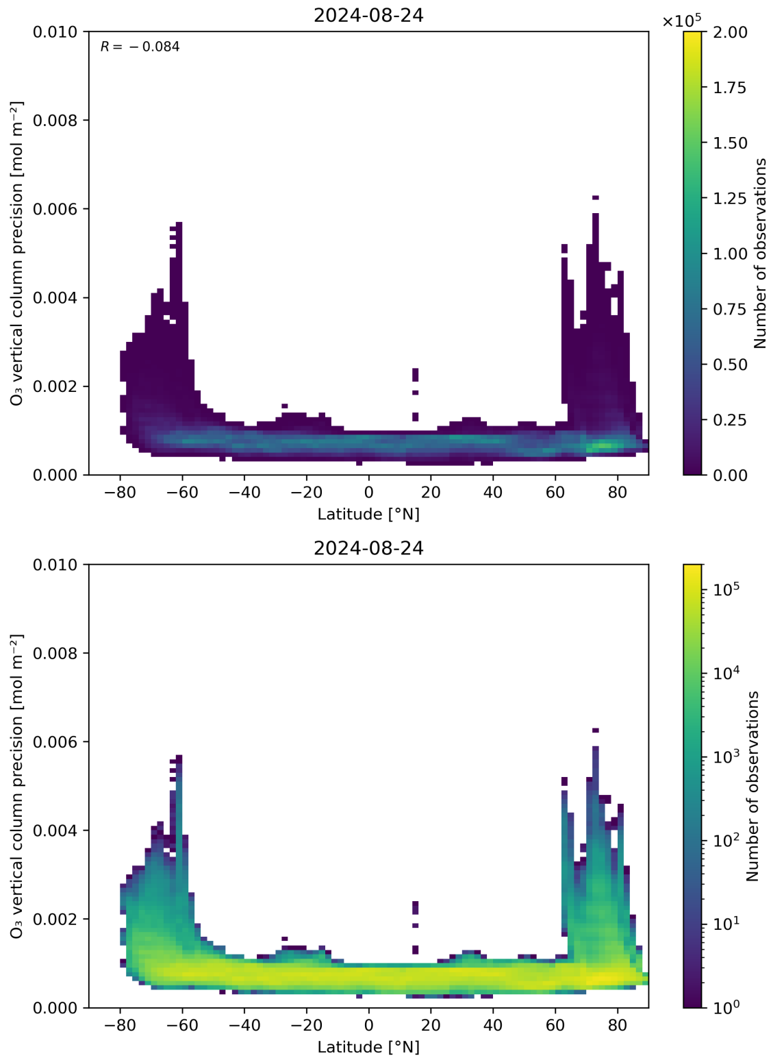
Figure 37: Scatter density plot of “Latitude” against “O 3 vertical column precision” for 2024-08-23 to 2024-08-25.
