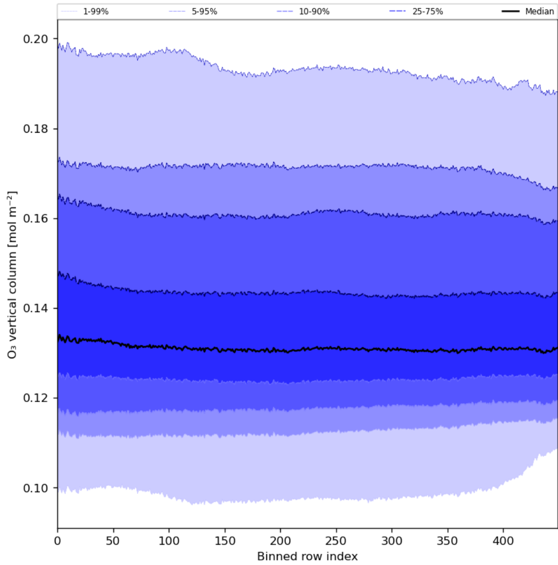
Figure 28: Along track statistics of “O 3 vertical column” for 2024-08-23 to 2024-08-25
