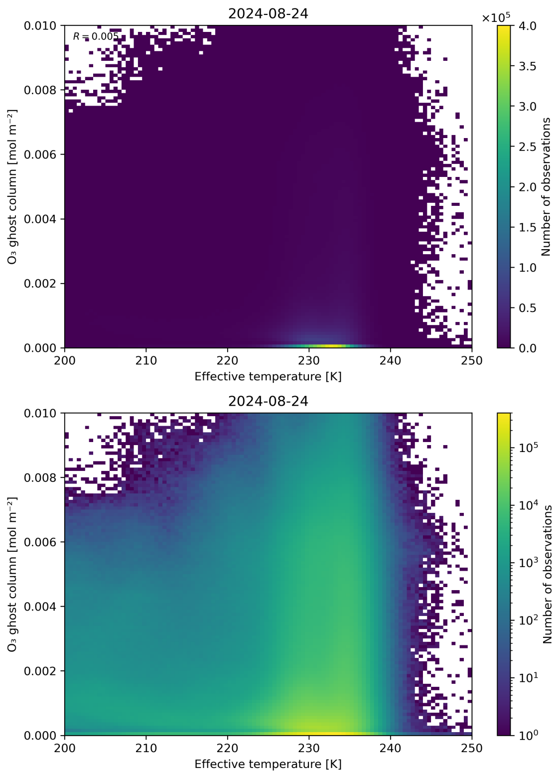
Figure 38: Scatter density plot of “Effective temperature” against “O 3 ghost column” for 2024-08-23 to 2024-08-25.
