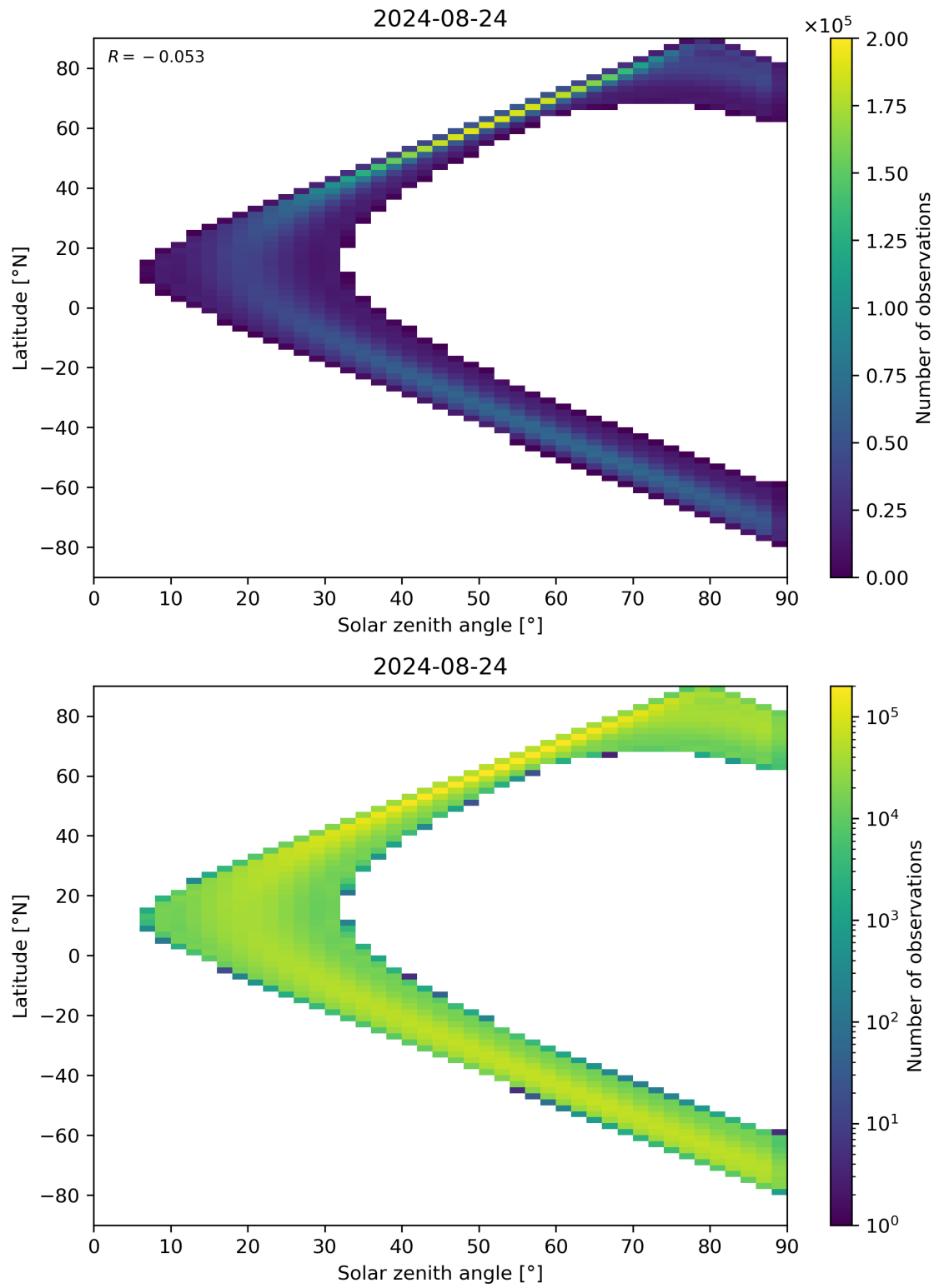
Figure 44: Scatter density plot of “Solar zenith angle” against “Latitude” for 2024-08-23 to 2024-08-25.
