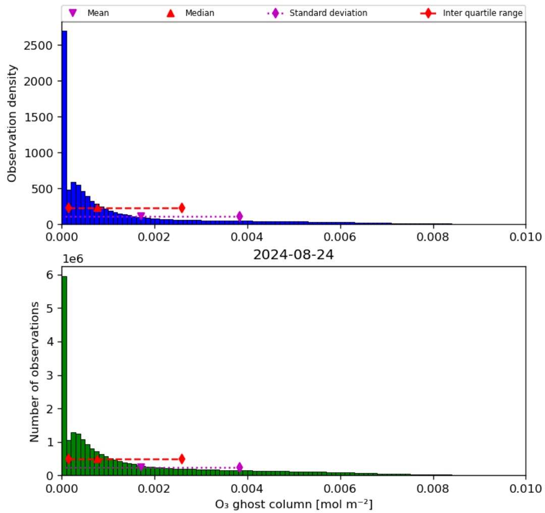
Figure 25: Histogram of “O 3 ghost column” for 2024-08-23 to 2024-08-25
