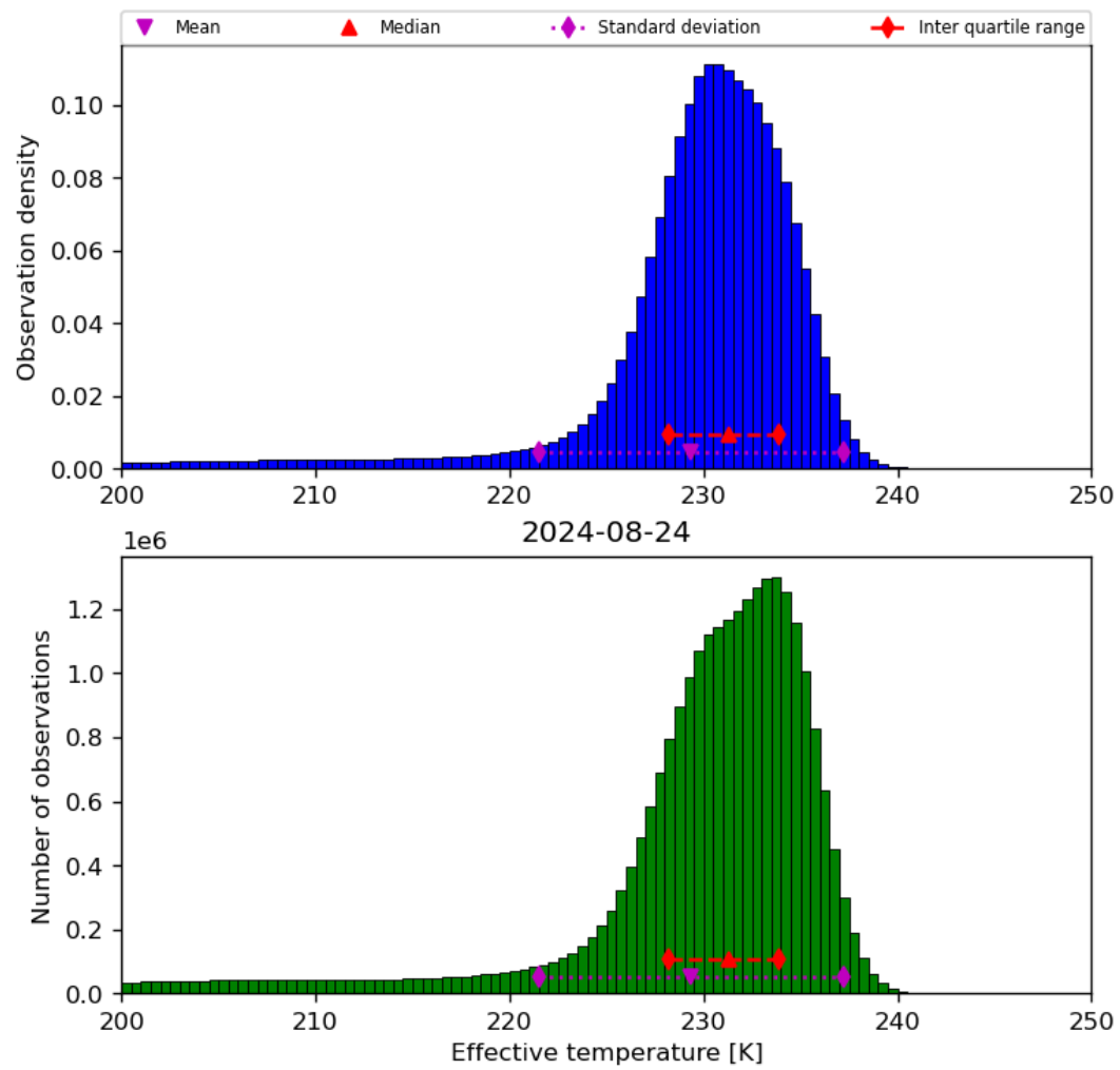
Figure 24: Histogram of “Effective temperature” for 2024-08-23 to 2024-08-25
