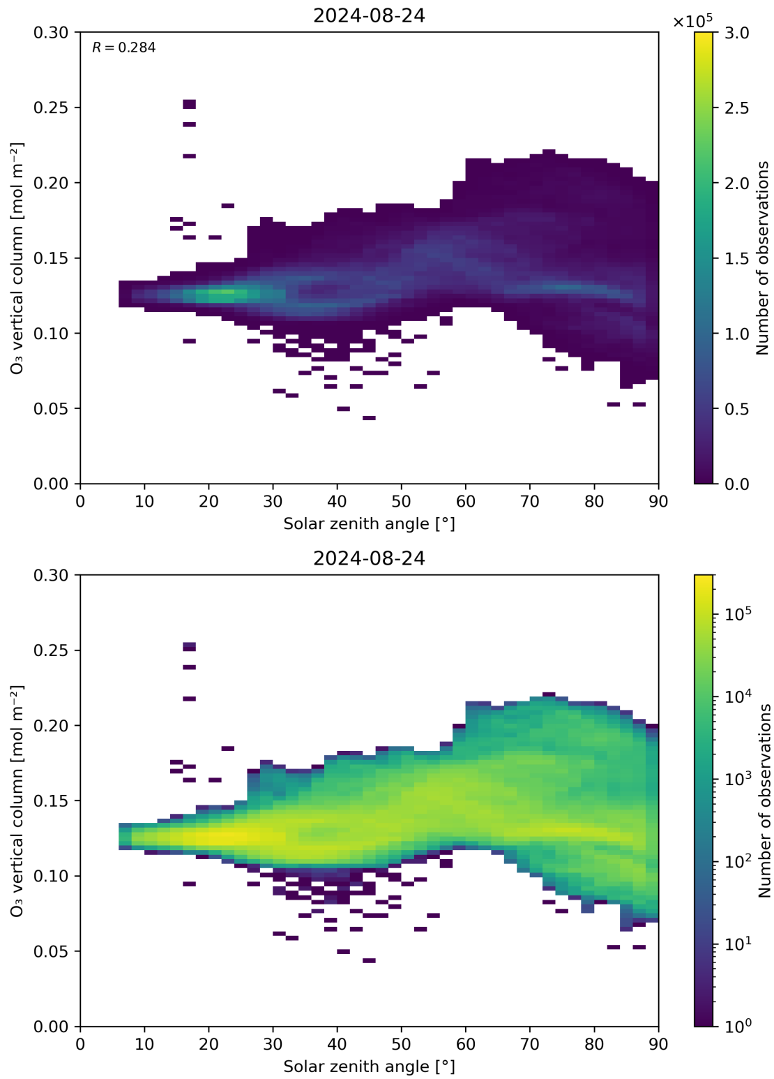
Figure 47: Scatter density plot of “Solar zenith angle” against “O 3 vertical column” for 2024-08-23 to 2024-08-25.
