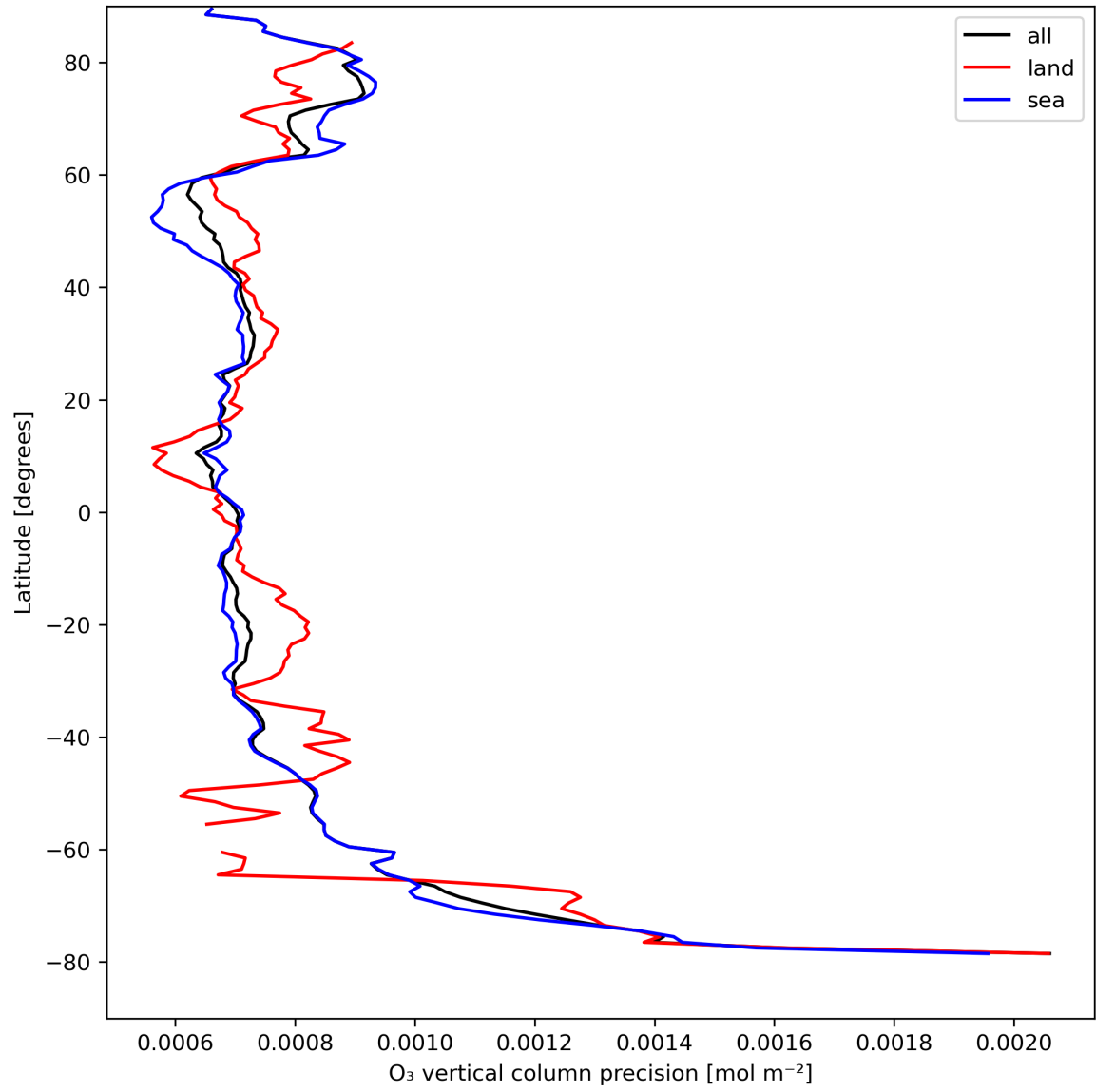
Figure 15: Zonal average of "O 3 vertical column precision" for 2024-08-23 to 2024-08-25.
