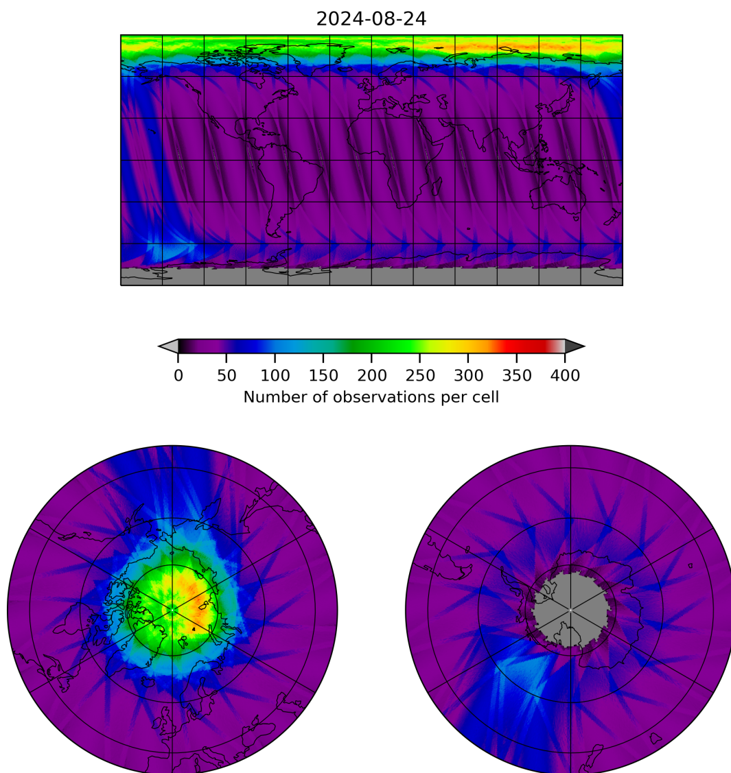
Figure 12: Map of the number of observations for 2024-08-23 to 2024-08-25
