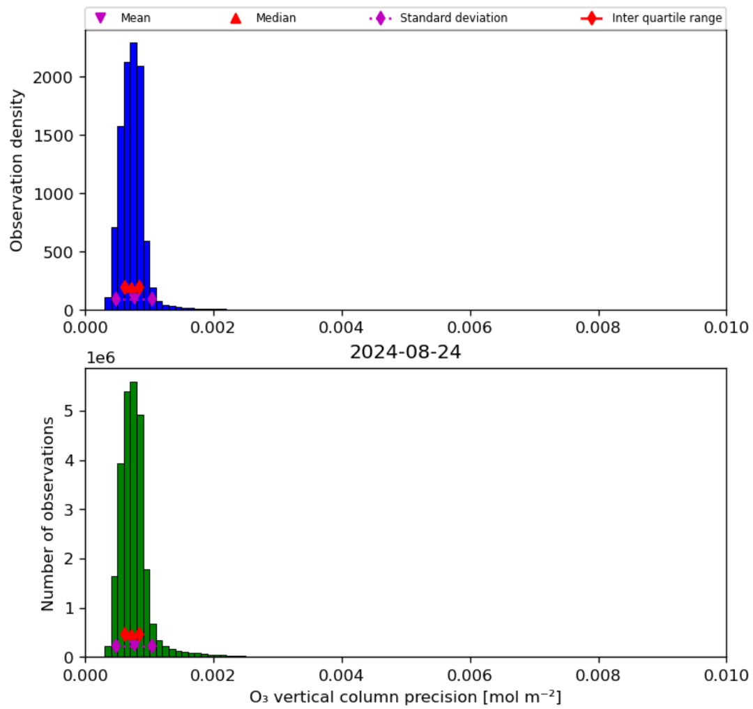
Figure 22: Histogram of “O 3 vertical column precision” for 2024-08-23 to 2024-08-25
