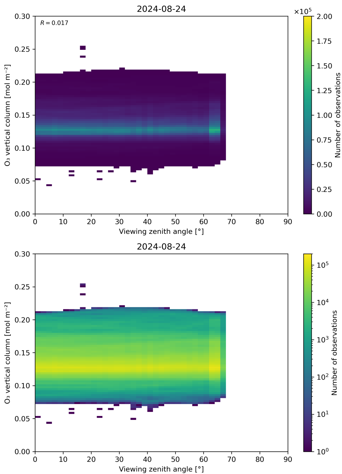
Figure 52: Scatter density plot of “Viewing zenith angle” against “O 3 vertical column” for 2024-08-23 to 2024-08-25.
