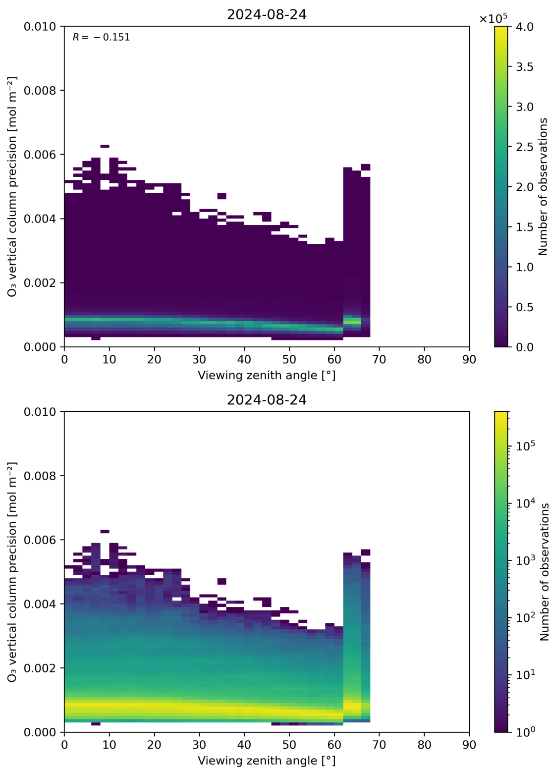
Figure 53: Scatter density plot of “Viewing zenith angle” against “O 3 vertical column precision” for 2024-08-23 to 2024-08-25.
