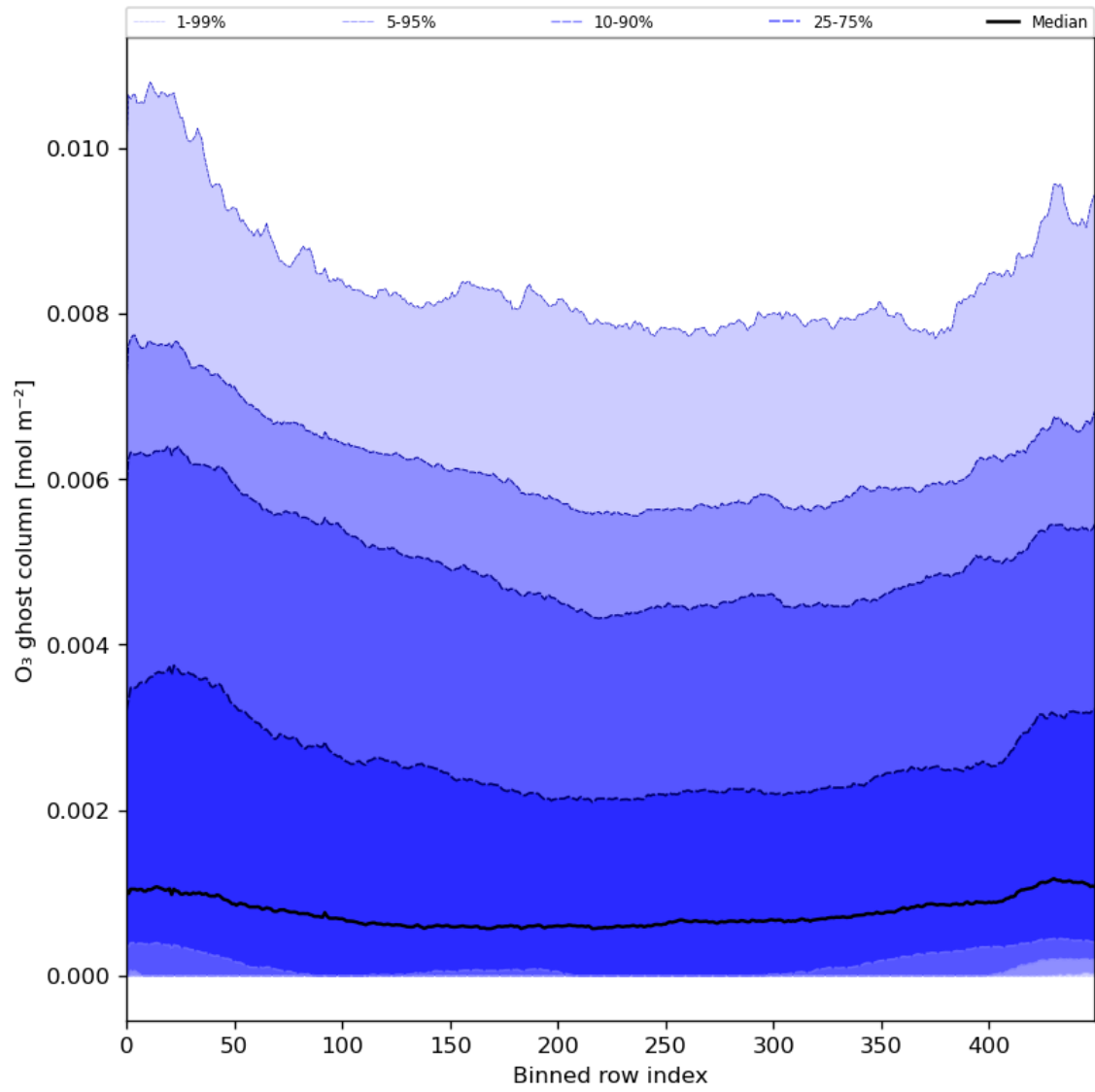
Figure 32: Along track statistics of "O 3 ghost column" for 2024-08-23 to 2024-08-25
