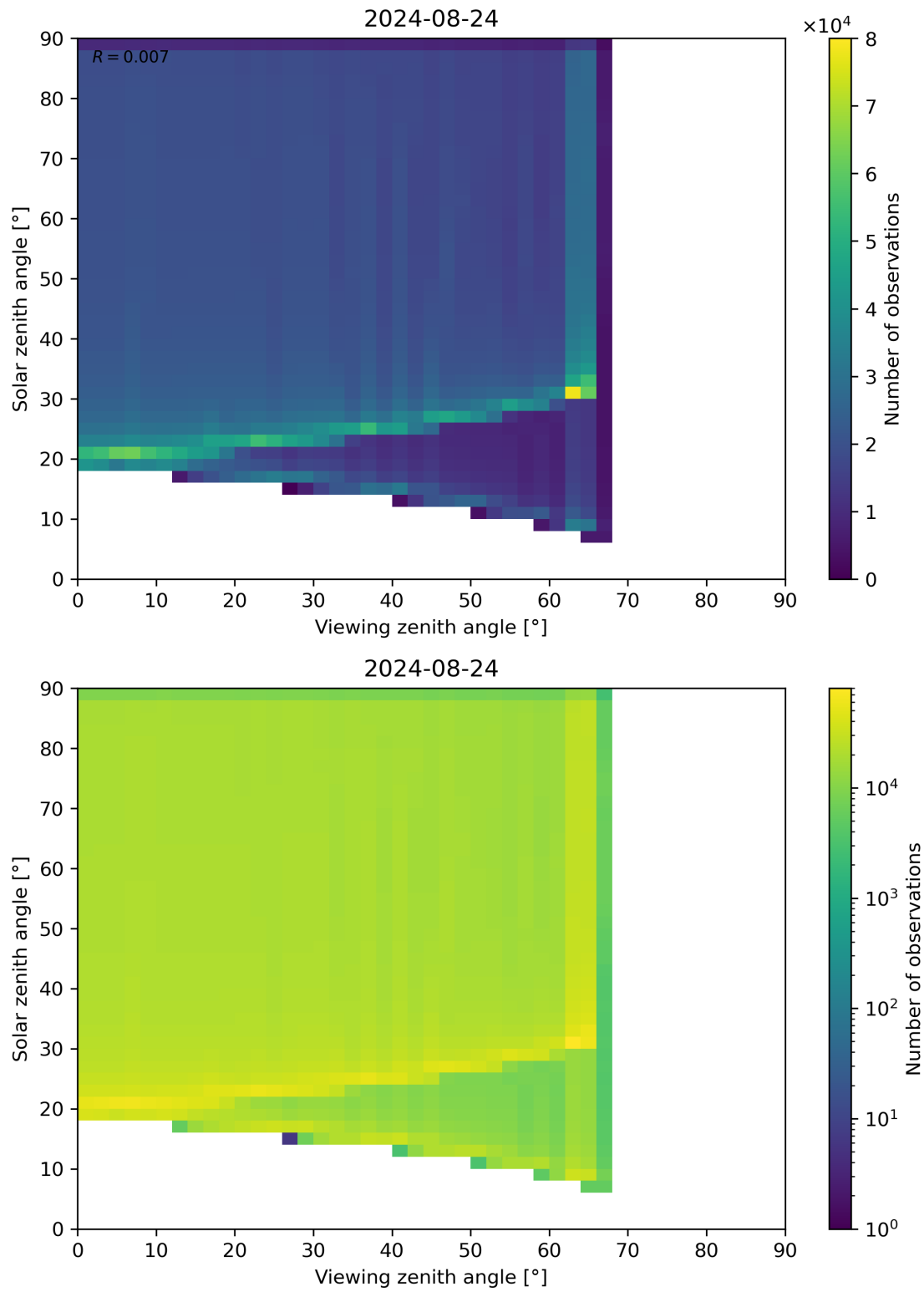
Figure 54: Scatter density plot of “Viewing zenith angle” against “Solar zenith angle” for 2024-08-23 to 2024-08-25.
