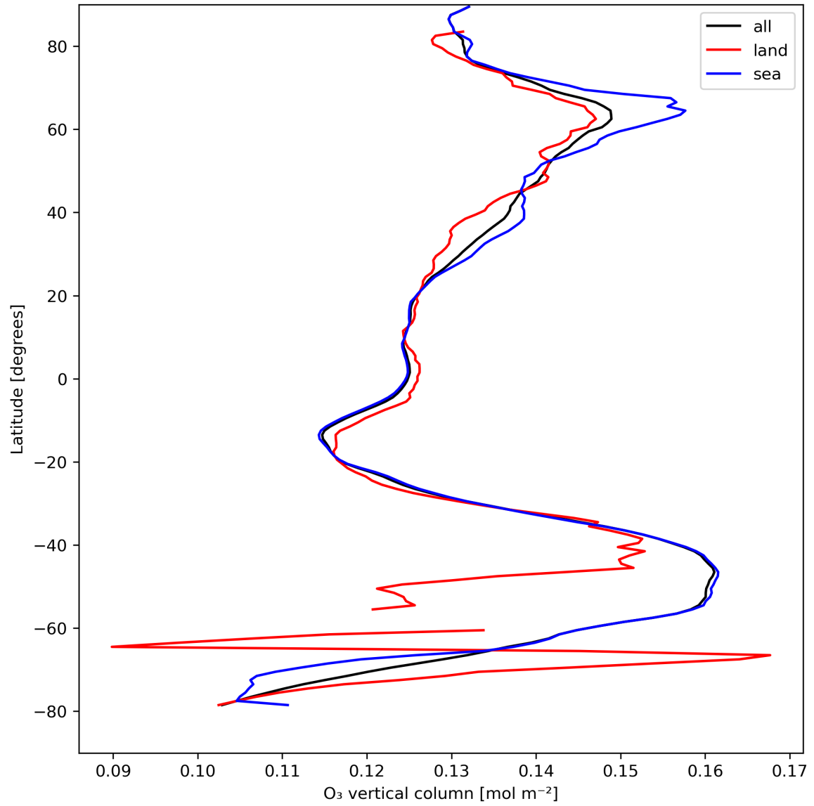
Figure 14: Zonal average of “O 3 vertical column” for 2024-08-23 to 2024-08-25.
