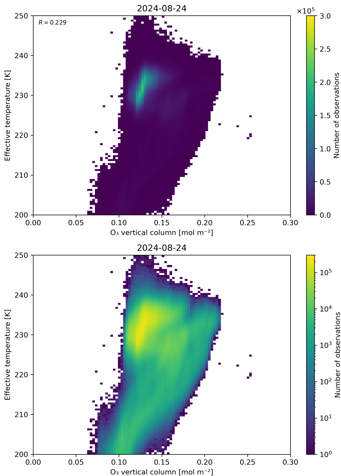
Figure 39: Scatter density plot of “O 3 vertical column” against “Effective temperature” for 2024-08-23 to 2024-08-25.
