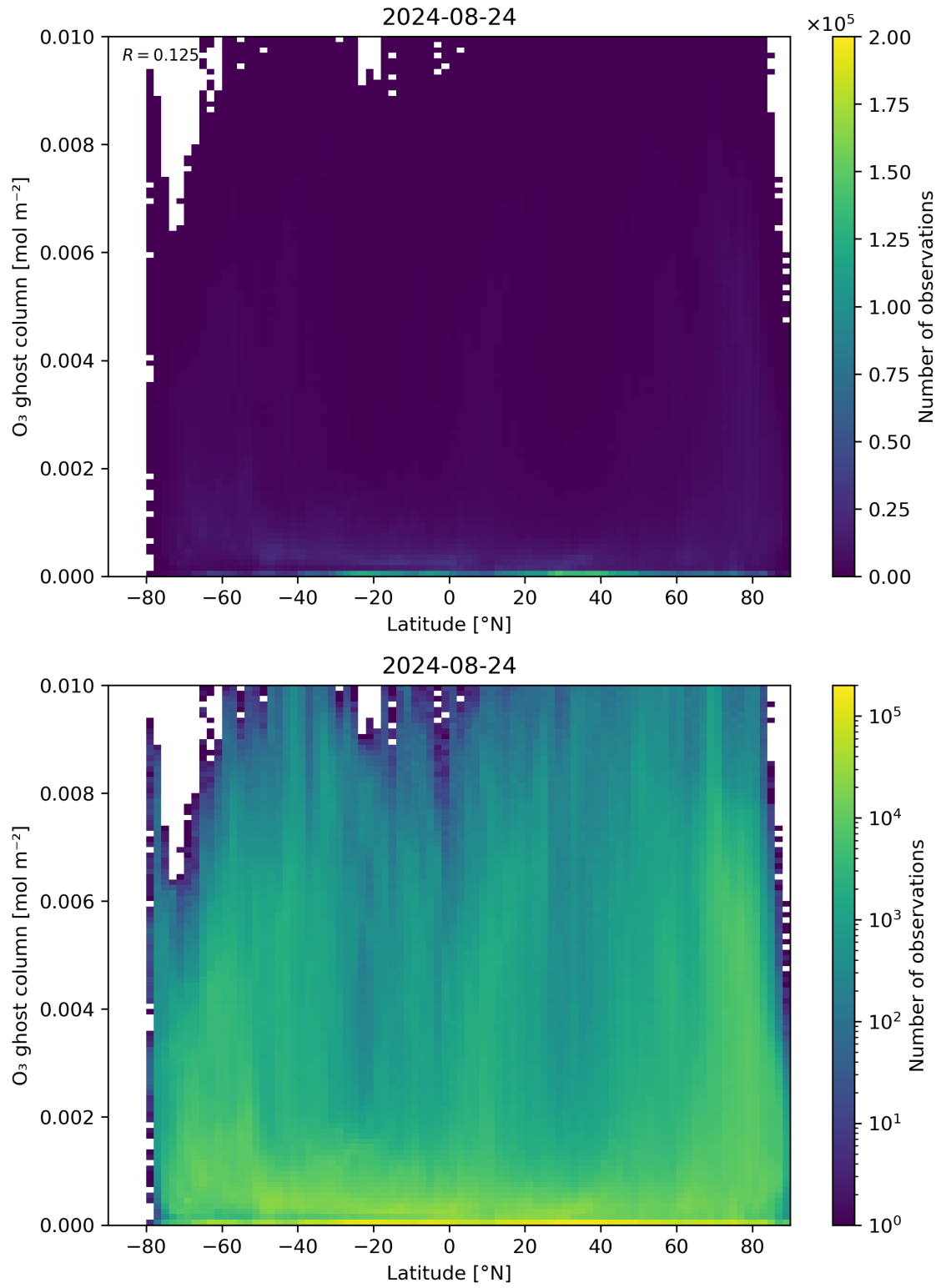
Figure 35: Scatter density plot of “Latitude” against “O 3 ghost column” for 2024-08-23 to 2024-08-25.
