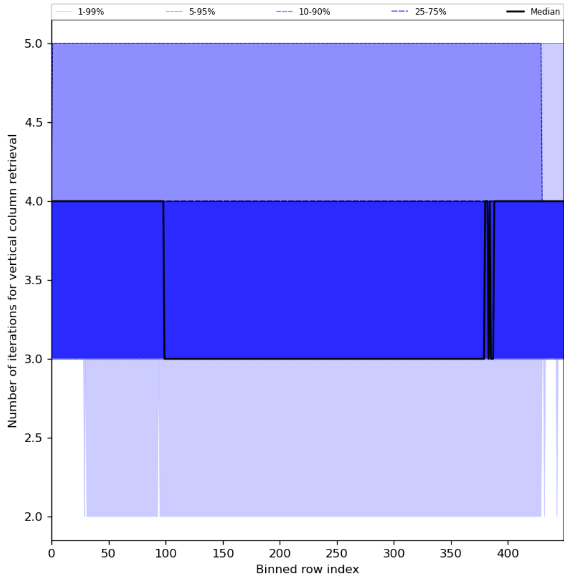
Figure 33: Along track statistics of “Number of iterations for vertical column retrieval” for 2024-08-23 to 2024-08-25
