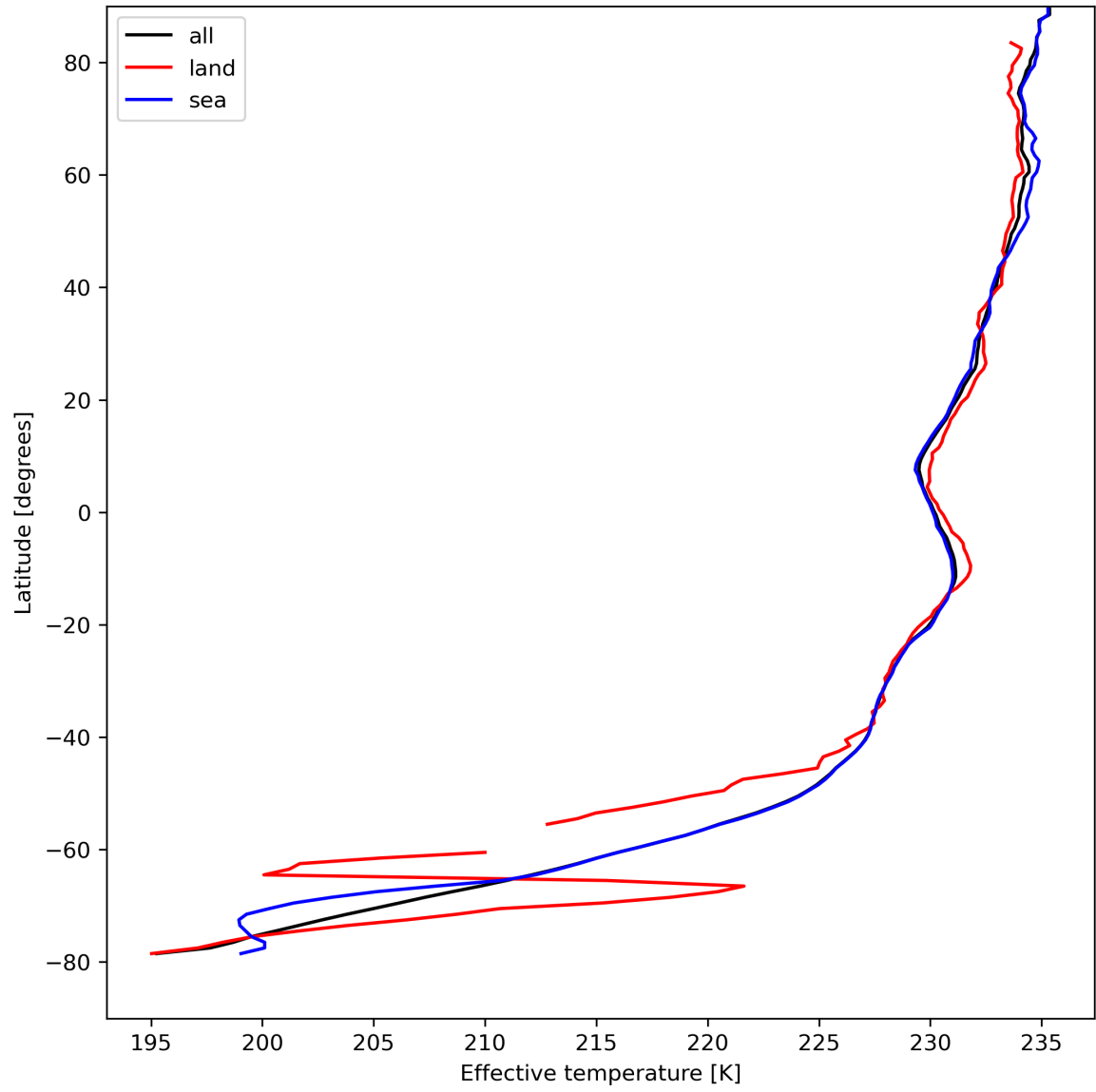
Figure 17: Zonal average of “Effective temperature” for 2024-08-23 to 2024-08-25.
