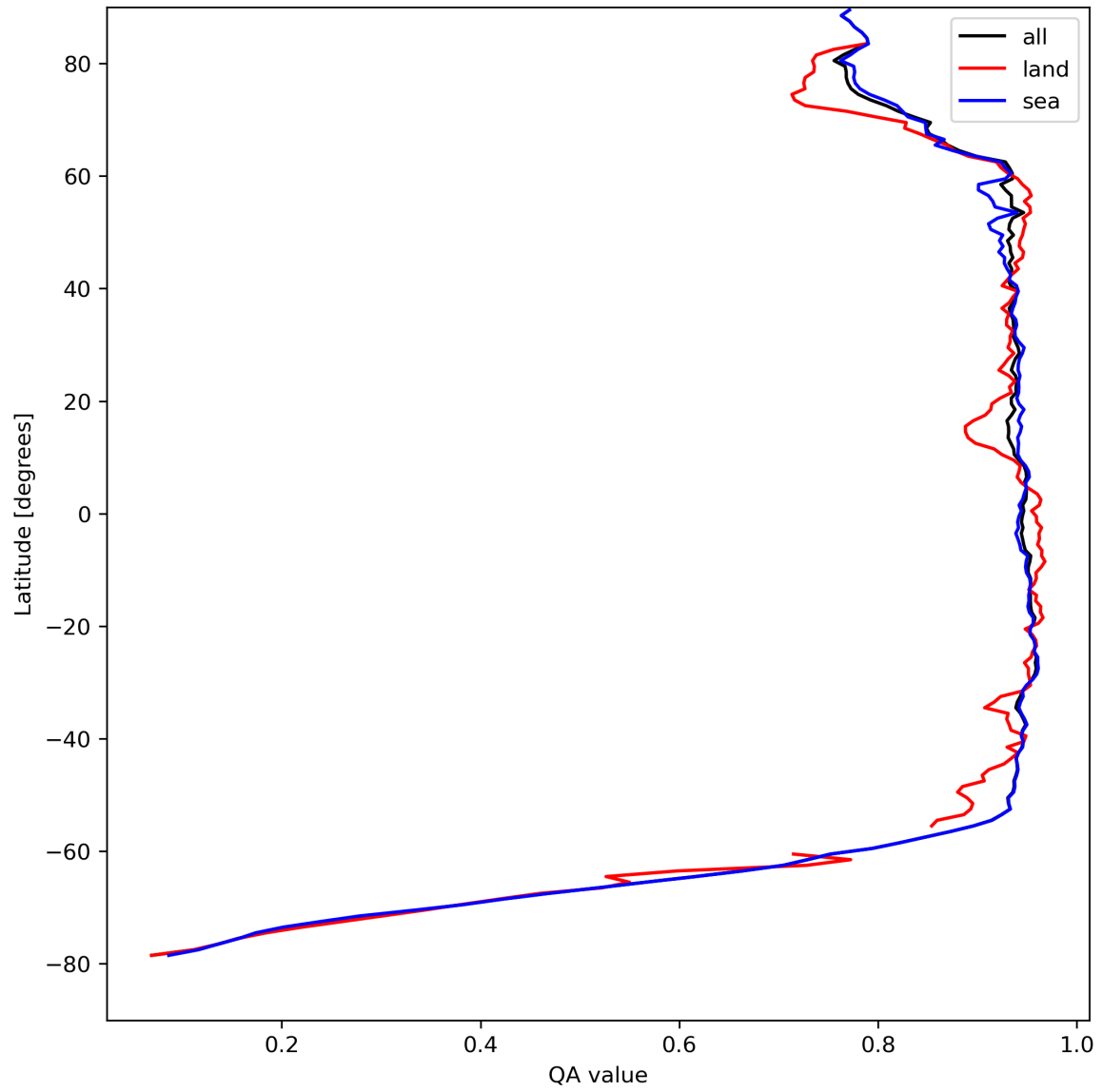
Figure 13: Zonal average of “QA value” for 2024-08-23 to 2024-08-25.
