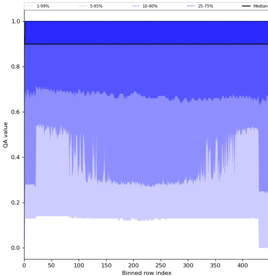
Figure 27: Along track statistics of “QA value” for 2024-08-23 to 2024-08-25
