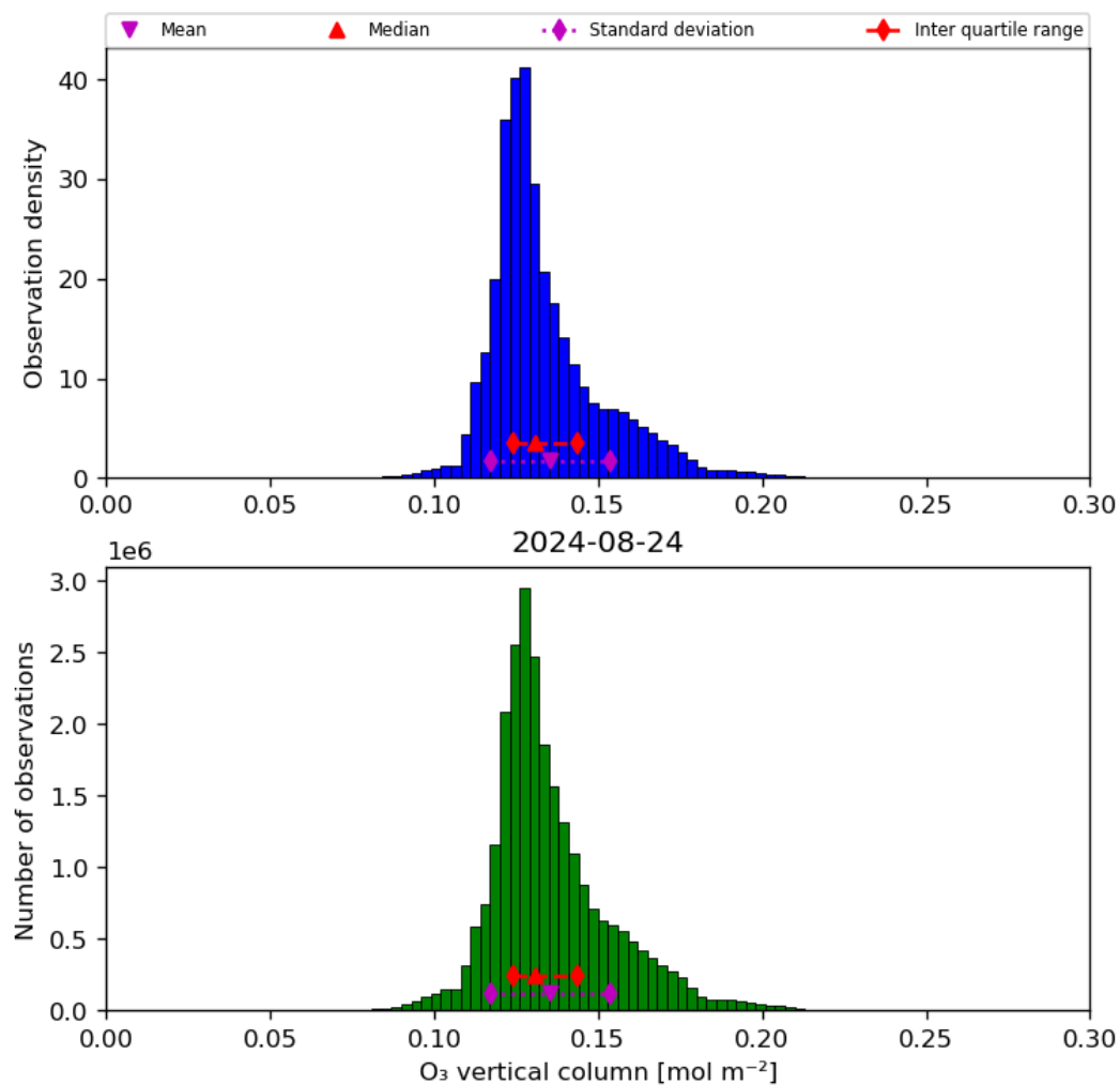
Figure 21: Histogram of “O 3 vertical column” for 2024-08-23 to 2024-08-25
