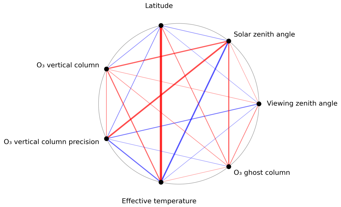
Figure 1: Map of correlation graph for 2024-08-23 to 2024-08-25.
