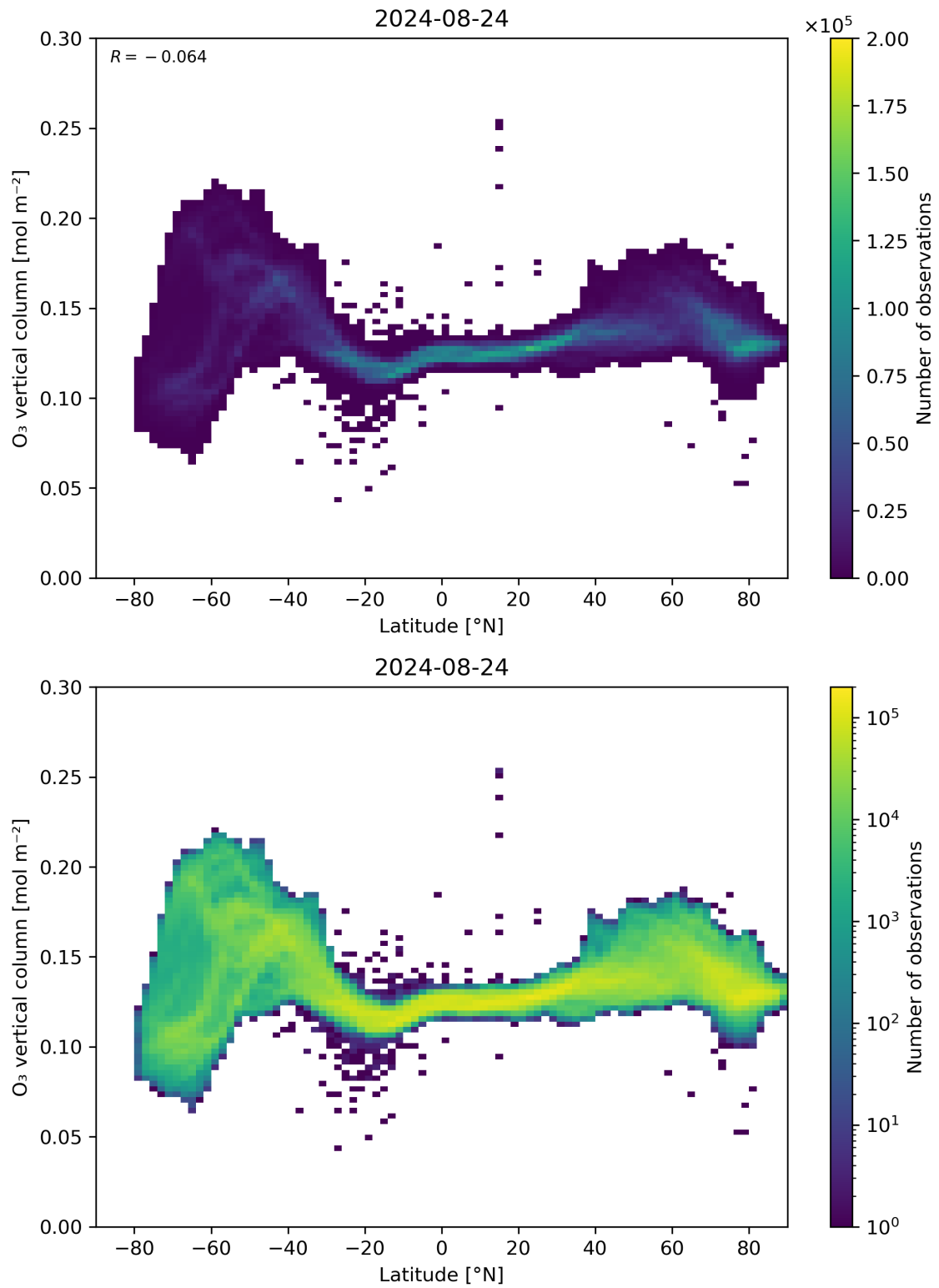
Figure 36: Scatter density plot of “Latitude” against “O 3 vertical column” for 2024-08-23 to 2024-08-25.
