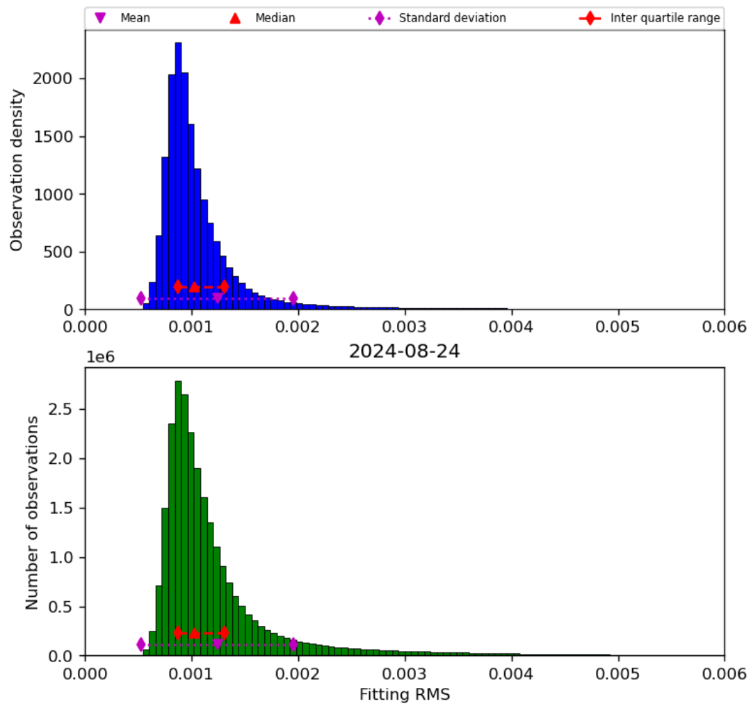
Figure 23: Histogram of “Fitting RMS” for 2024-08-23 to 2024-08-25
