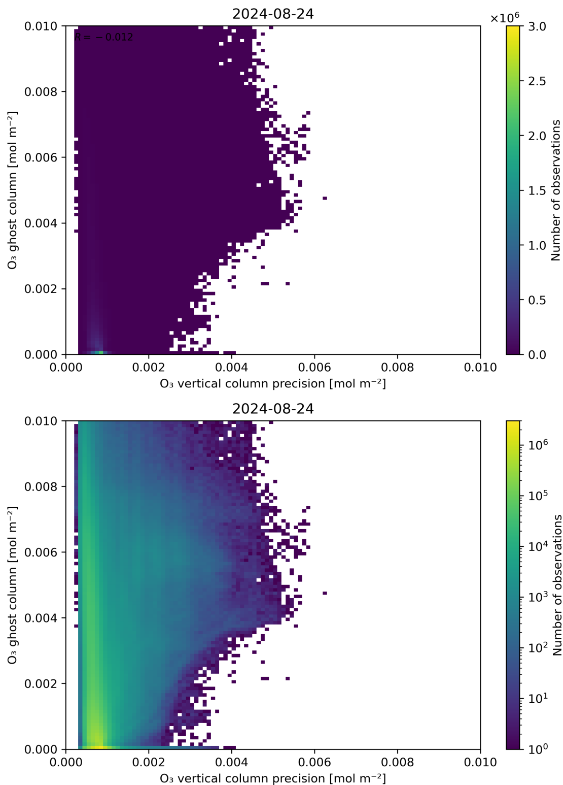
Figure 43: Scatter density plot of “ \text{O}_3 vertical column precision” against “ \text{O}_3 ghost column” for 2024-08-23 to 2024-08-25.
