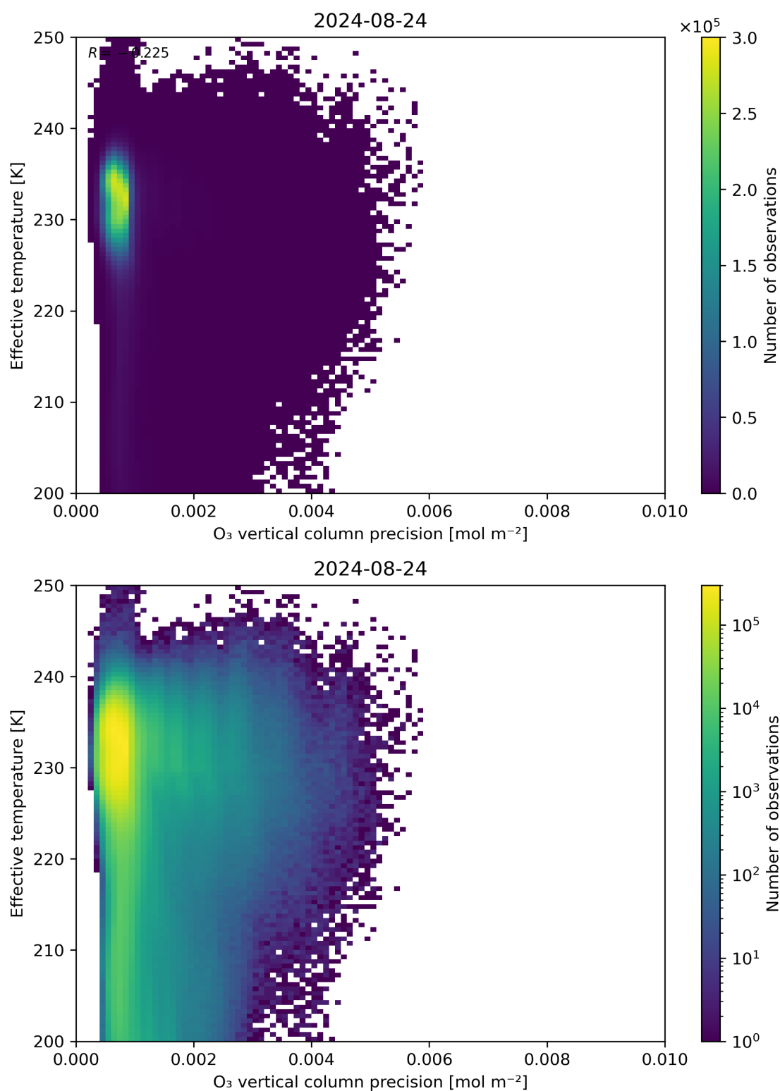
Figure 42: Scatter density plot of “O 3 vertical column precision” against “Effective temperature” for 2024-08-23 to 2024-08-25.
