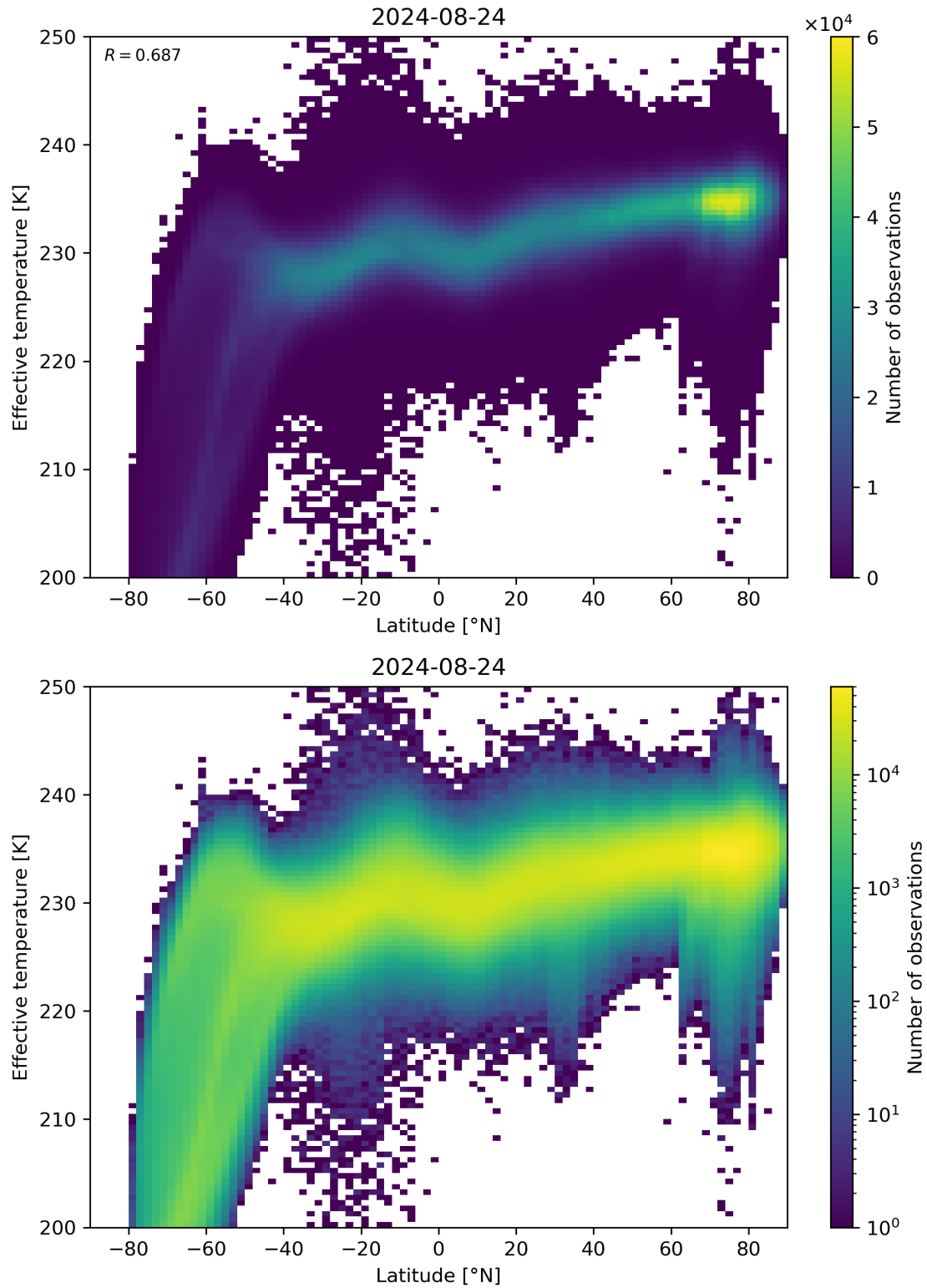
Figure 34: Scatter density plot of “Latitude” against “Effective temperature” for 2024-08-23 to 2024-08-25.
