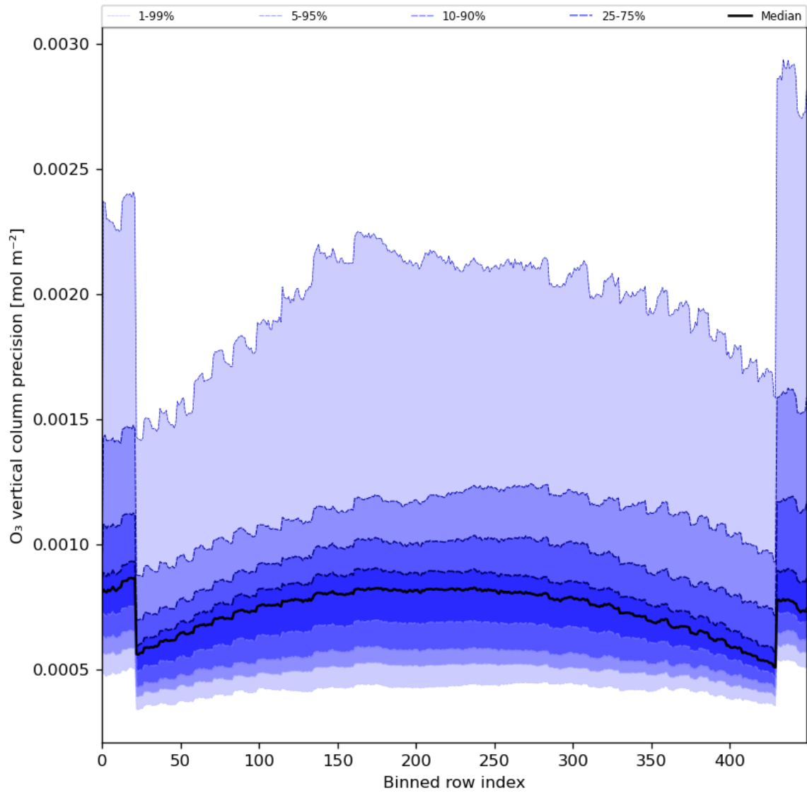
Figure 29: Along track statistics of “O 3 vertical column precision” for 2024-08-23 to 2024-08-25
