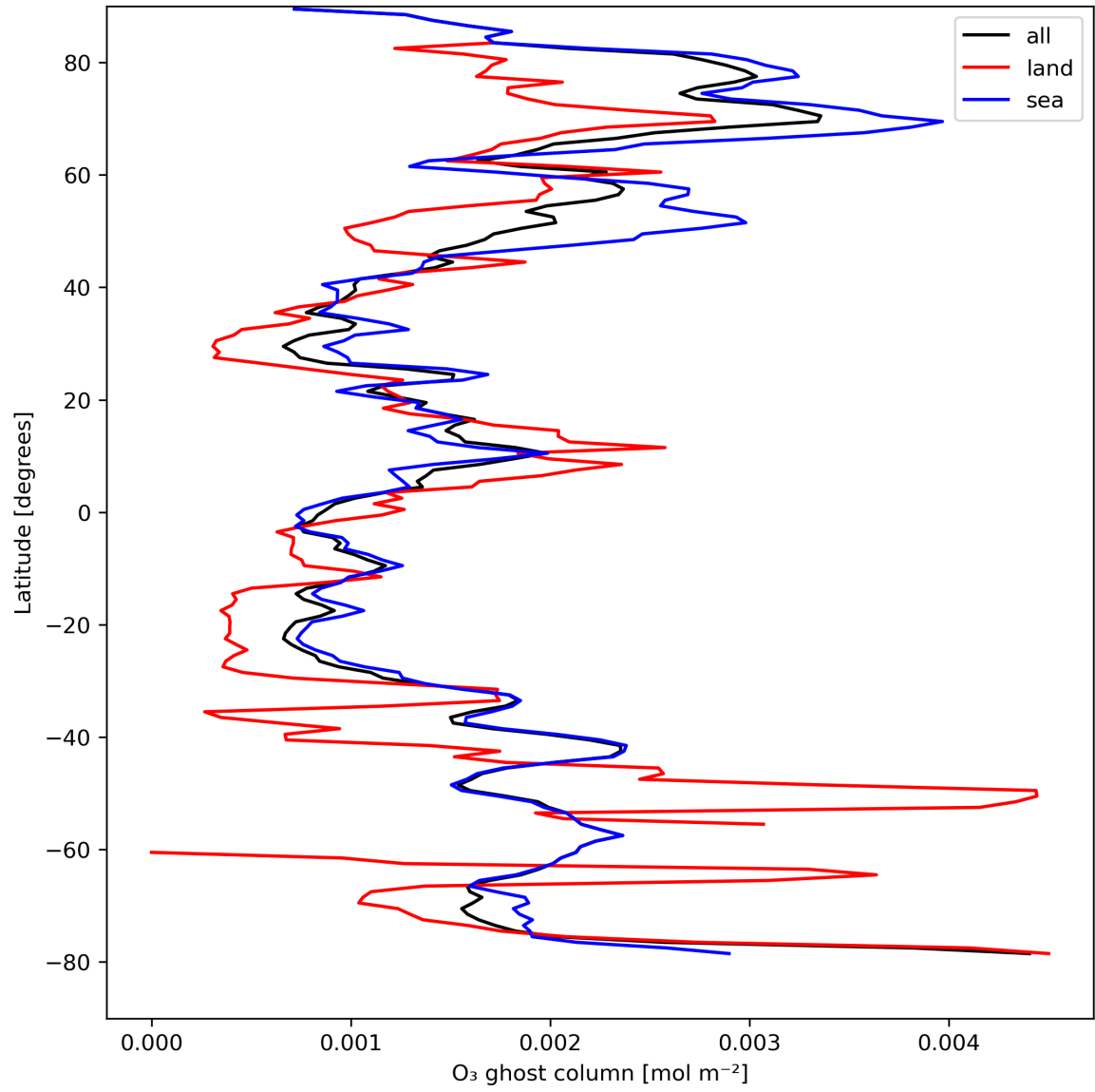
Figure 18: Zonal average of "O 3 ghost column" for 2024-08-23 to 2024-08-25.
