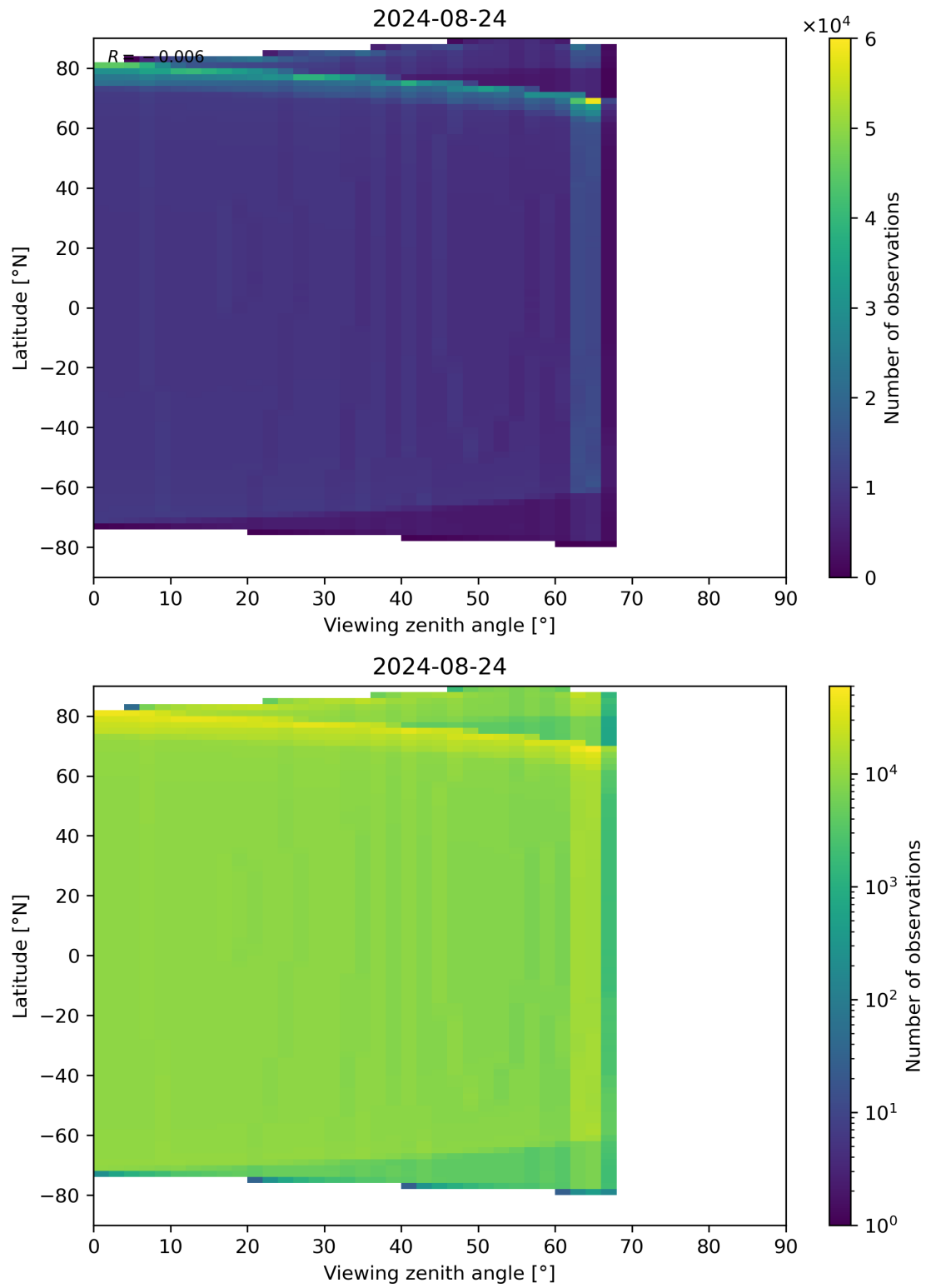
Figure 49: Scatter density plot of “Viewing zenith angle” against “Latitude” for 2024-08-23 to 2024-08-25.
