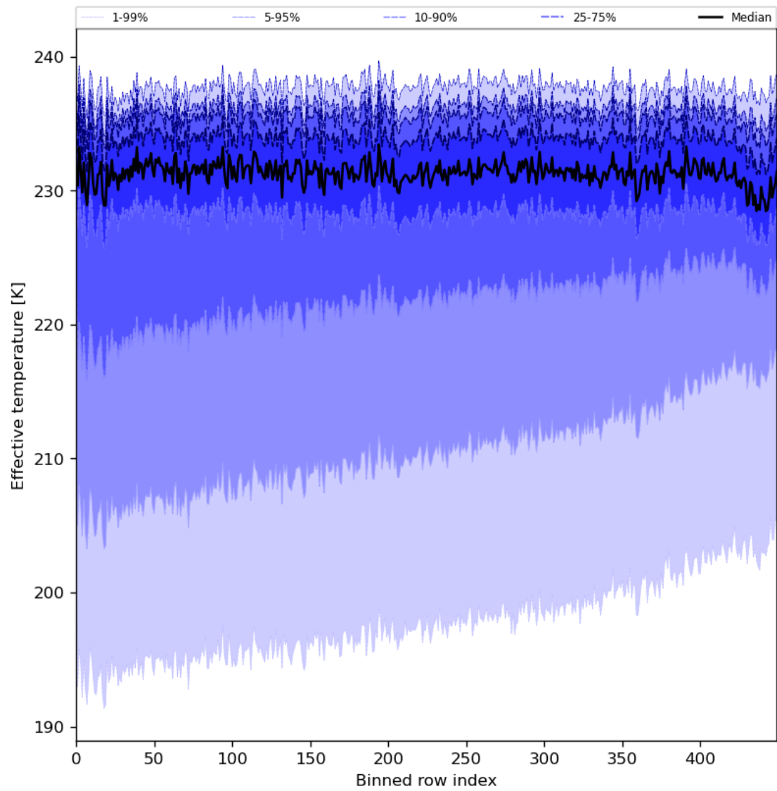
Figure 31: Along track statistics of “Effective temperature” for 2024-08-23 to 2024-08-25
