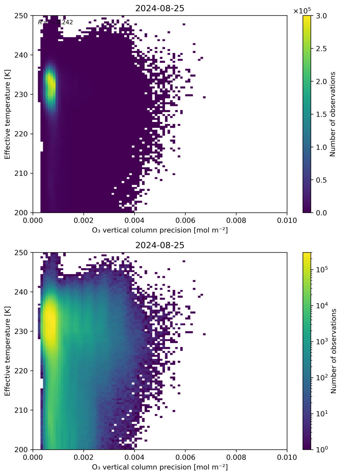
Figure 42: Scatter density plot of “O 3 vertical column precision” against “Effective temperature” for 2024-08-24 to 2024-08-26.
