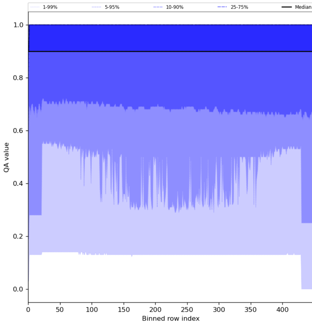
Figure 27: Along track statistics of “QA value” for 2024-08-24 to 2024-08-26
