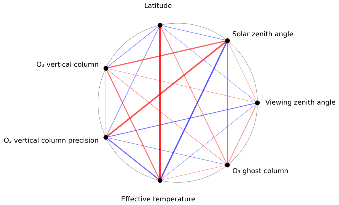
Figure 1: Map of correlation graph for 2024-08-24 to 2024-08-26.
