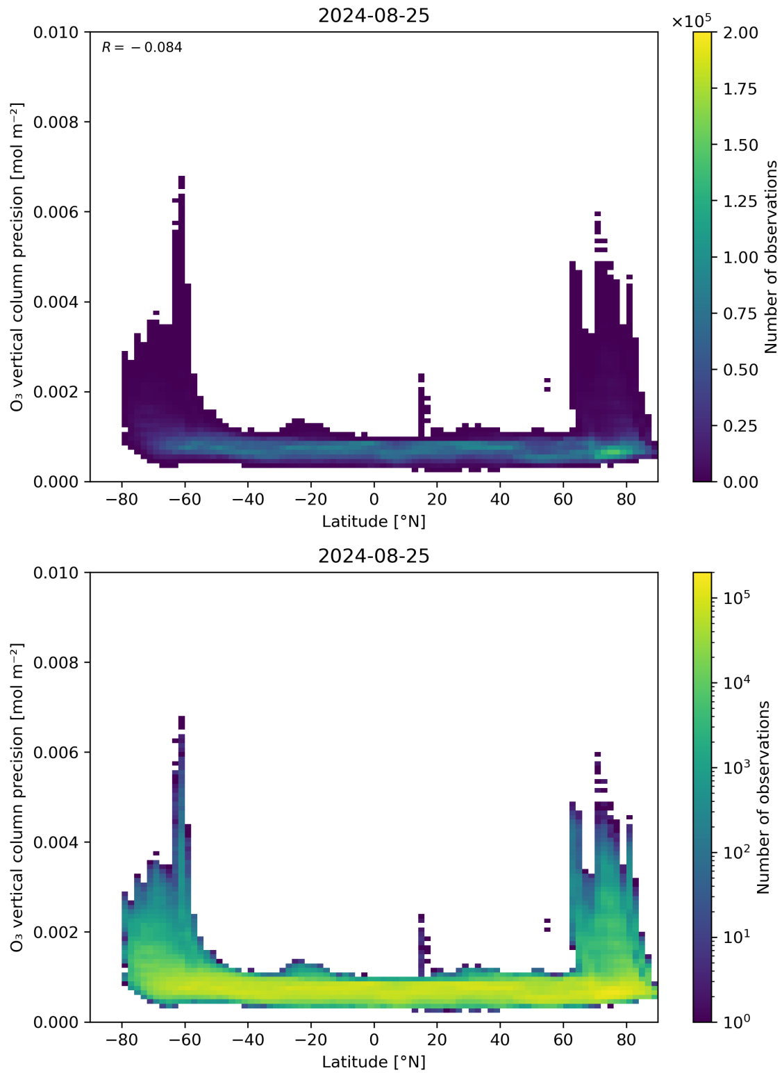
Figure 37: Scatter density plot of “Latitude” against “O 3 vertical column precision” for 2024-08-24 to 2024-08-26.
