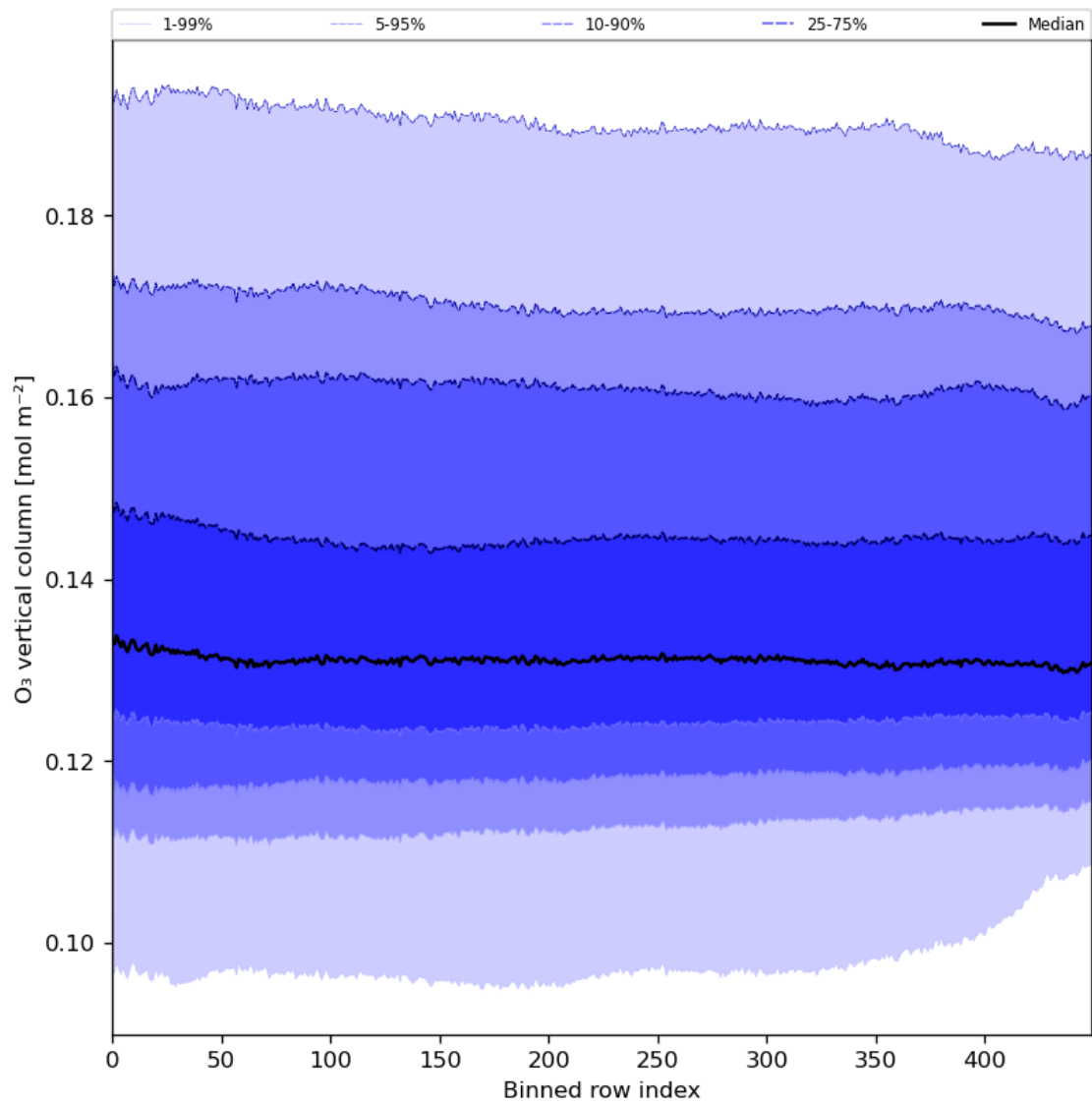
Figure 28: Along track statistics of “O 3 vertical column” for 2024-08-24 to 2024-08-26
