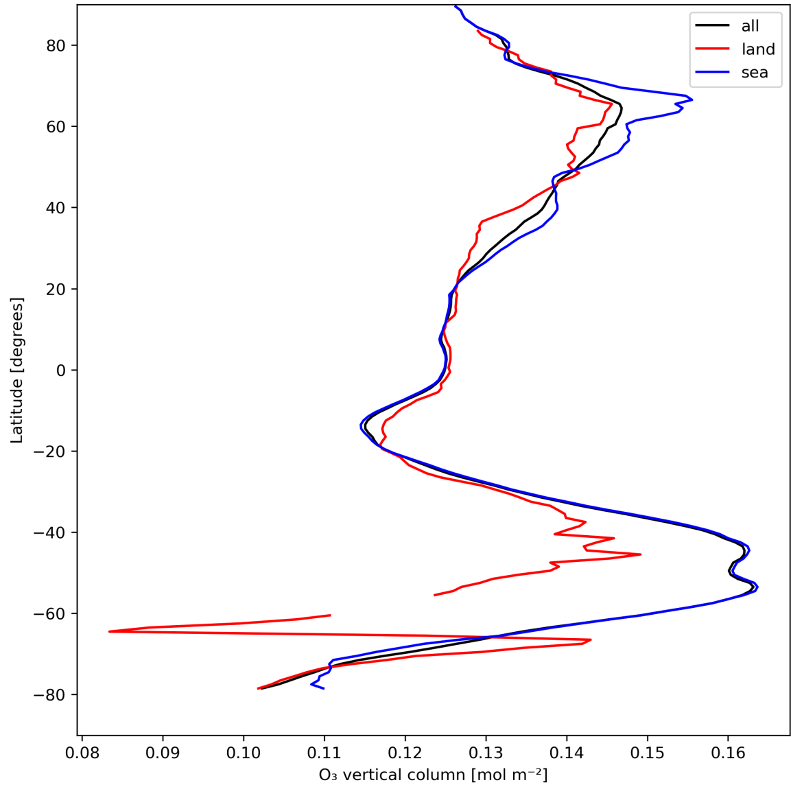
Figure 14: Zonal average of “O 3 vertical column” for 2024-08-24 to 2024-08-26.
