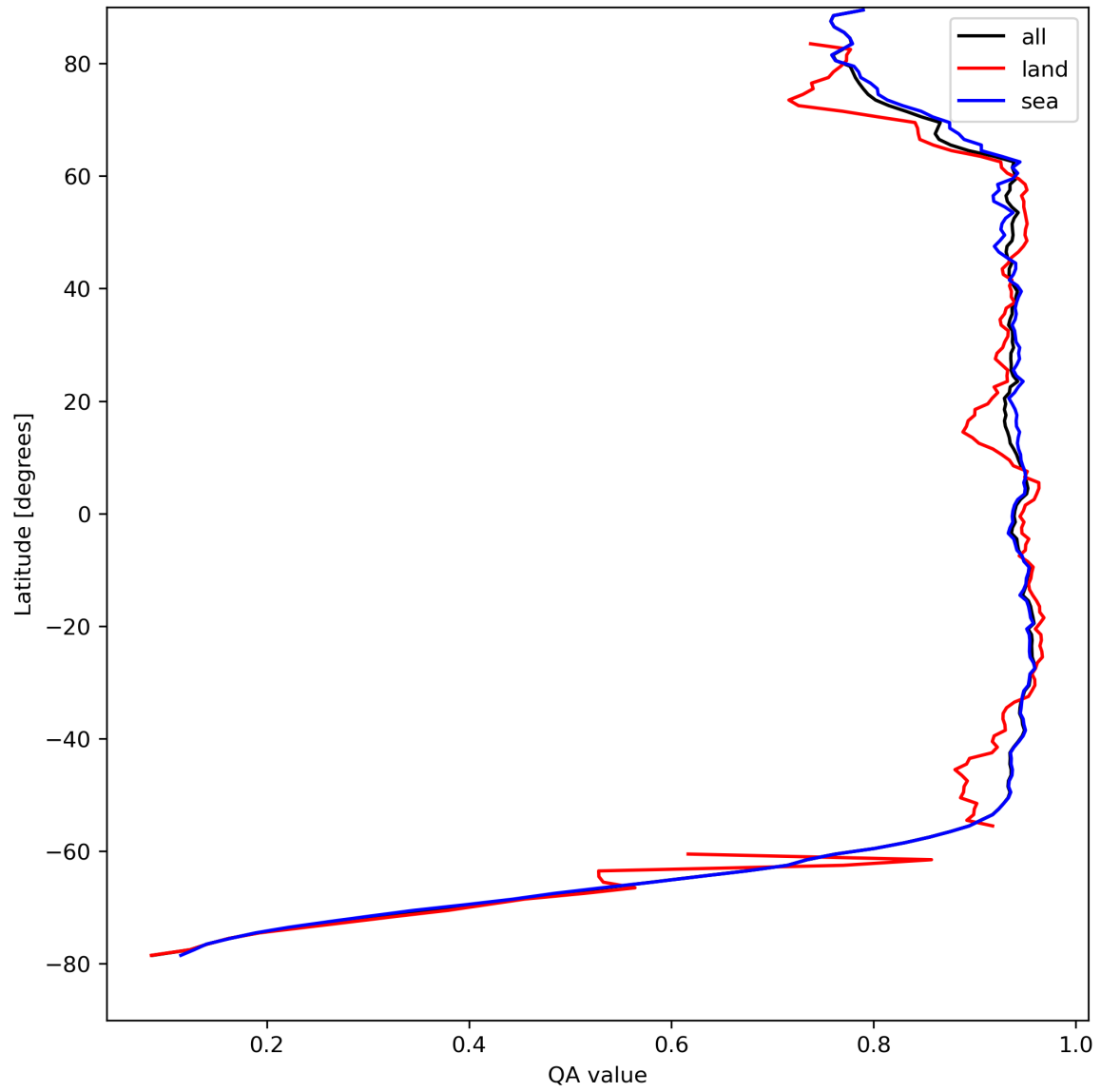
Figure 13: Zonal average of “QA value” for 2024-08-24 to 2024-08-26.
