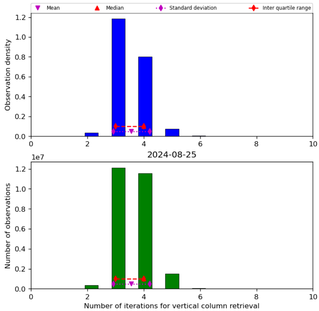
Figure 26: Histogram of “Number of iterations for vertical column retrieval” for 2024-08-24 to 2024-08-26
