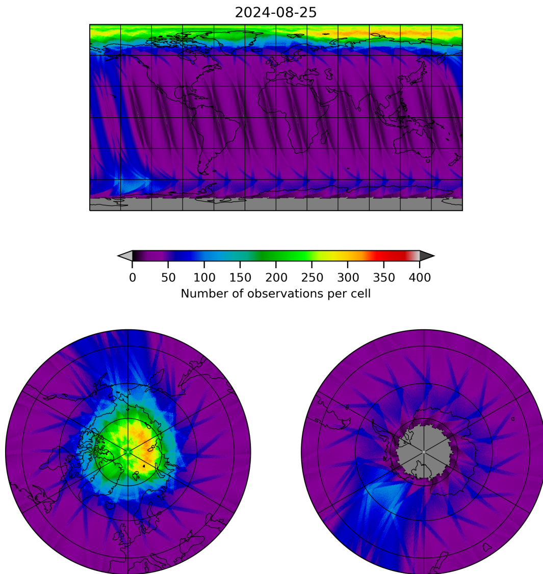
Figure 12: Map of the number of observations for 2024-08-24 to 2024-08-26
