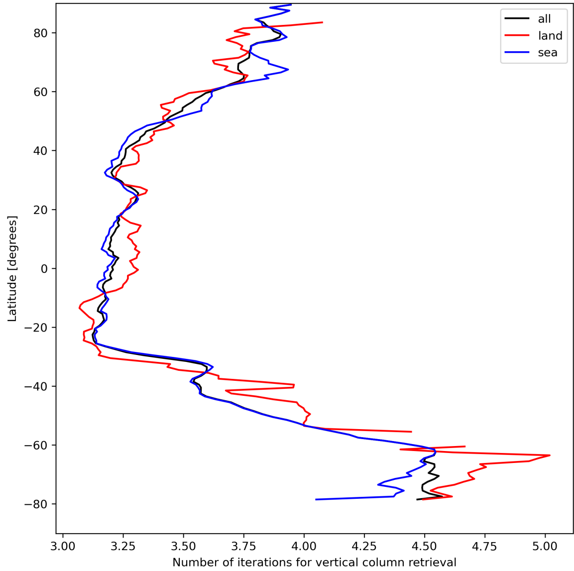
Figure 19: Zonal average of “Number of iterations for vertical column retrieval” for 2024-08-24 to 2024-08-26.
