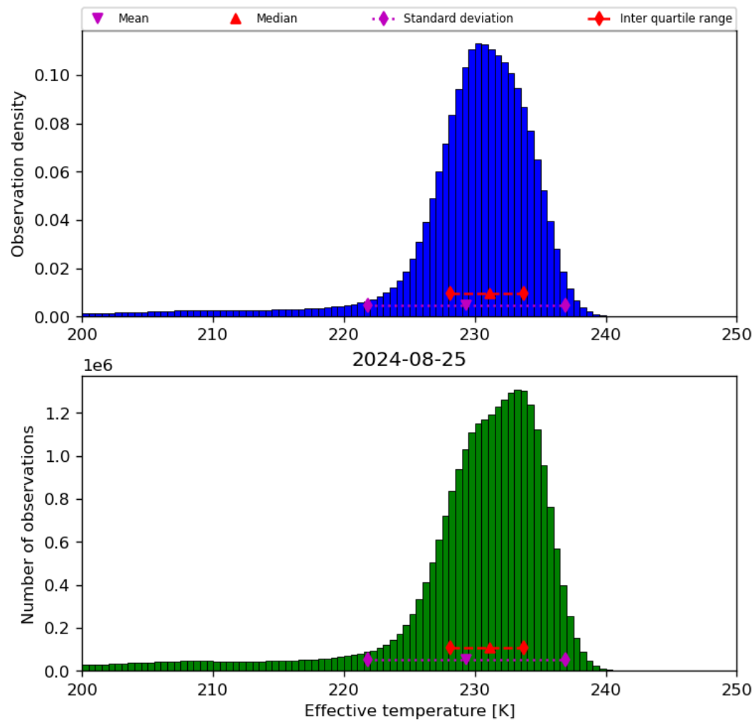
Figure 24: Histogram of “Effective temperature” for 2024-08-24 to 2024-08-26
