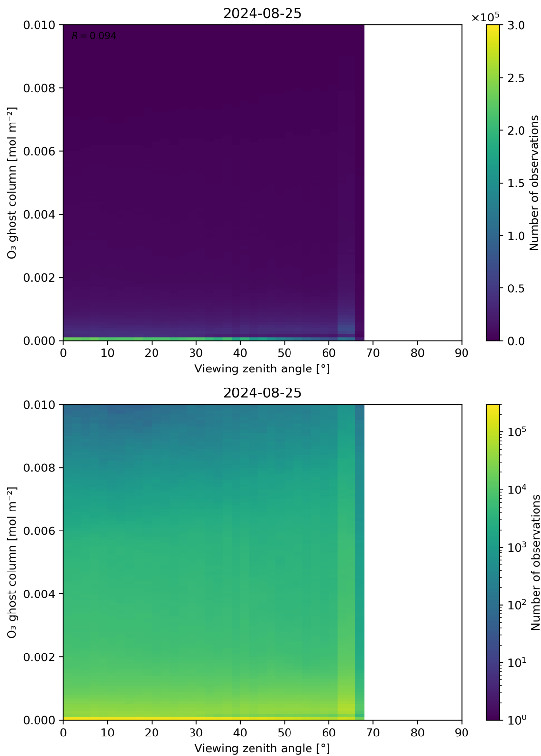
Figure 51: Scatter density plot of “Viewing zenith angle” against “O 3 ghost column” for 2024-08-24 to 2024-08-26.
