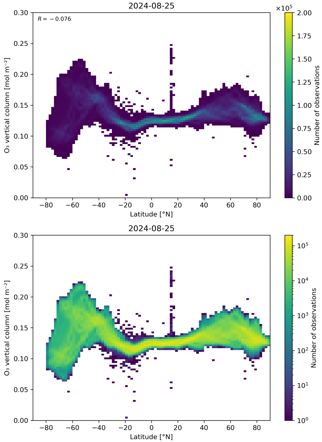
Figure 36: Scatter density plot of “Latitude” against “O 3 vertical column” for 2024-08-24 to 2024-08-26.
