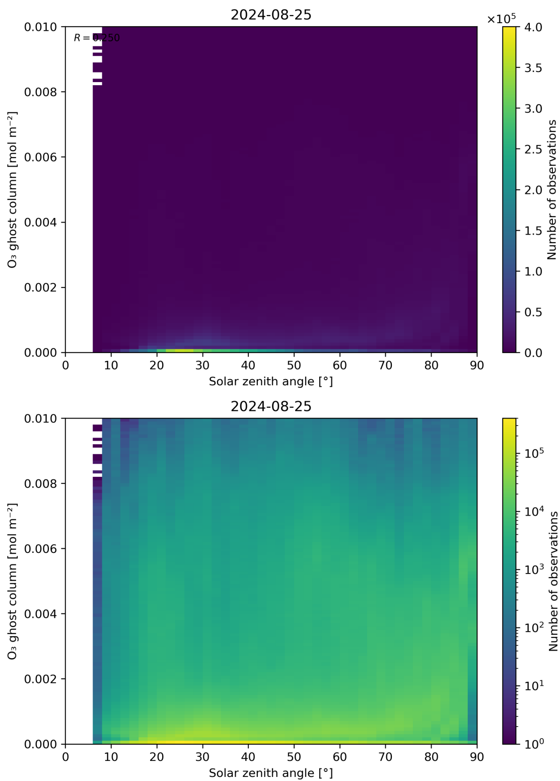
Figure 46: Scatter density plot of “Solar zenith angle” against “O 3 ghost column” for 2024-08-24 to 2024-08-26.
