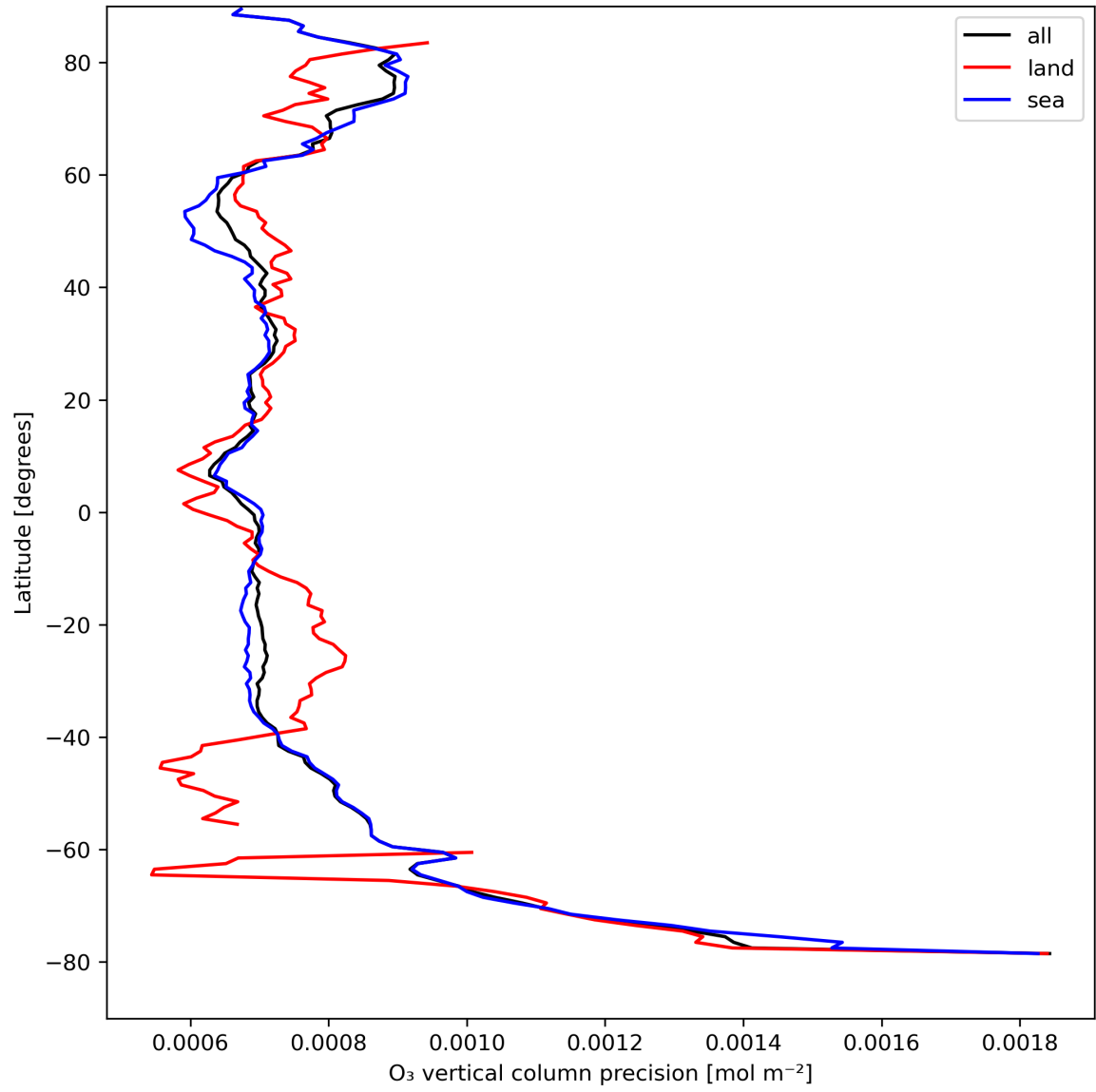
Figure 15: Zonal average of “O 3 vertical column precision” for 2024-08-24 to 2024-08-26.
