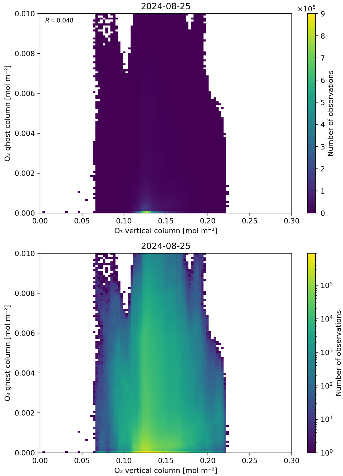
Figure 40: Scatter density plot of “O 3 vertical column” against “O 3 ghost column” for 2024-08-24 to 2024-08-26.
