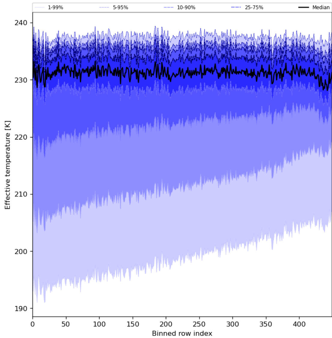
Figure 31: Along track statistics of “Effective temperature” for 2024-08-24 to 2024-08-26
