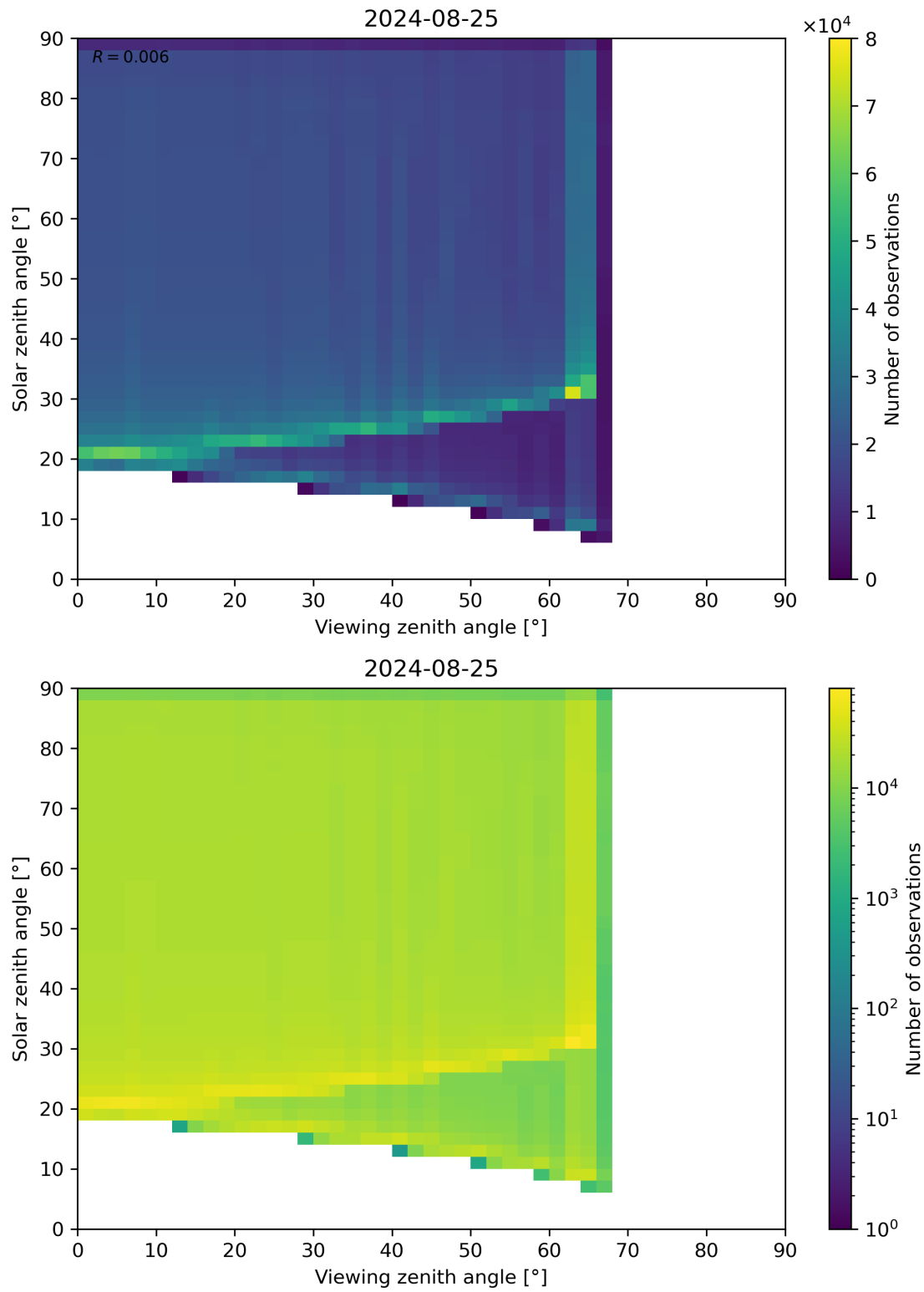
Figure 54: Scatter density plot of “Viewing zenith angle” against “Solar zenith angle” for 2024-08-24 to 2024-08-26.
