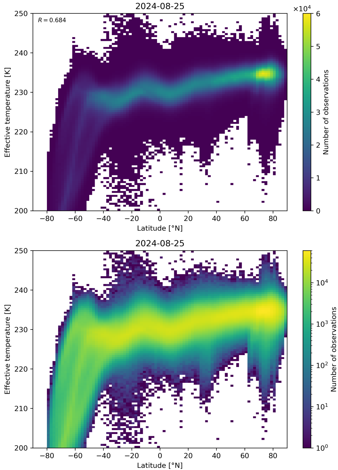
Figure 34: Scatter density plot of “Latitude” against “Effective temperature” for 2024-08-24 to 2024-08-26.
