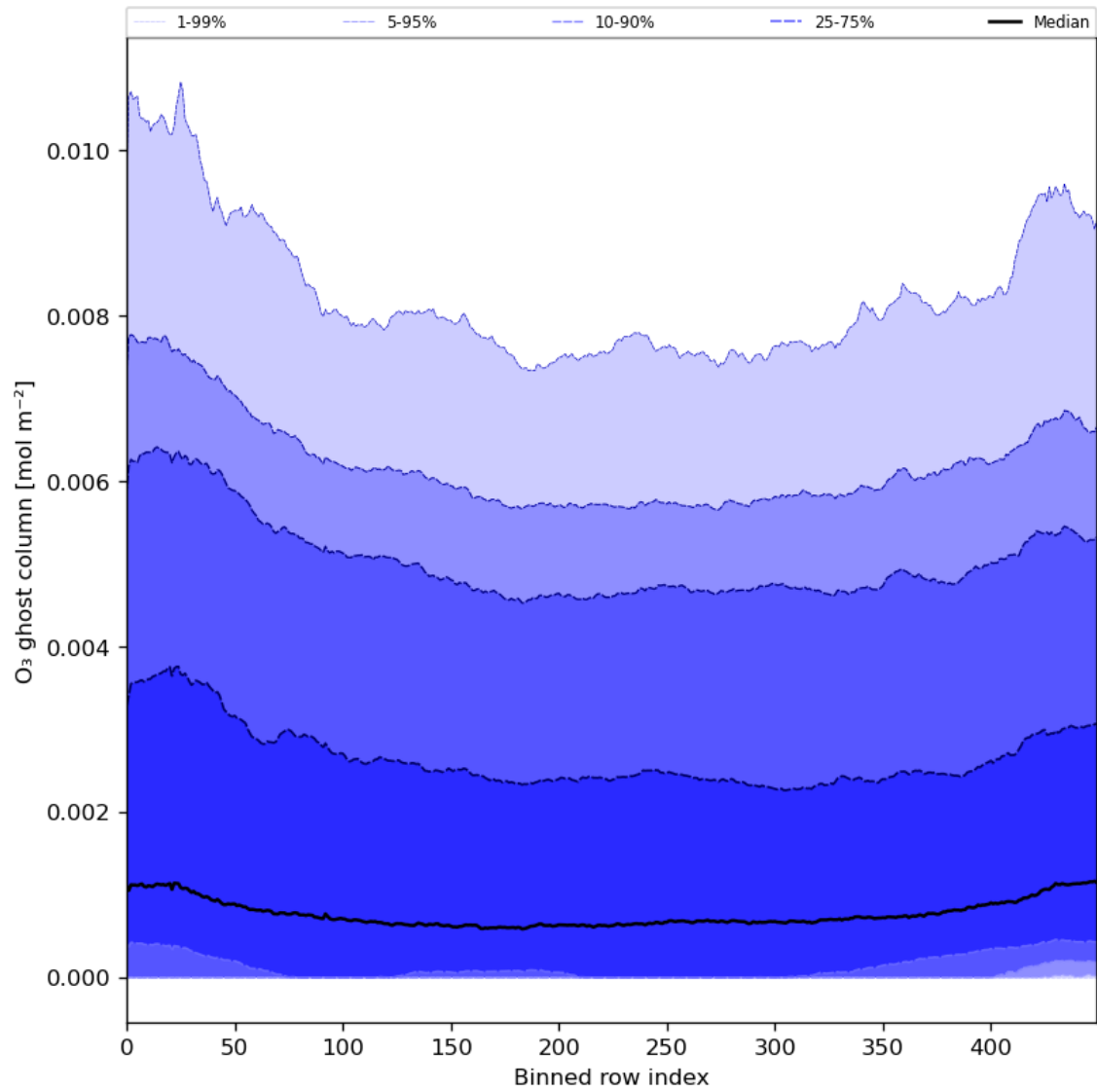
Figure 32: Along track statistics of “O 3 ghost column” for 2024-08-24 to 2024-08-26
