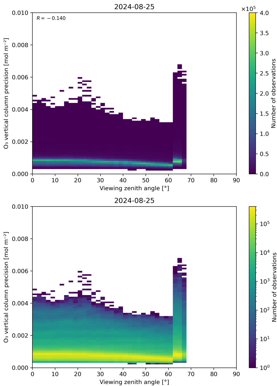
Figure 53: Scatter density plot of “Viewing zenith angle” against “O 3 vertical column precision” for 2024-08-24 to 2024-08-26.
