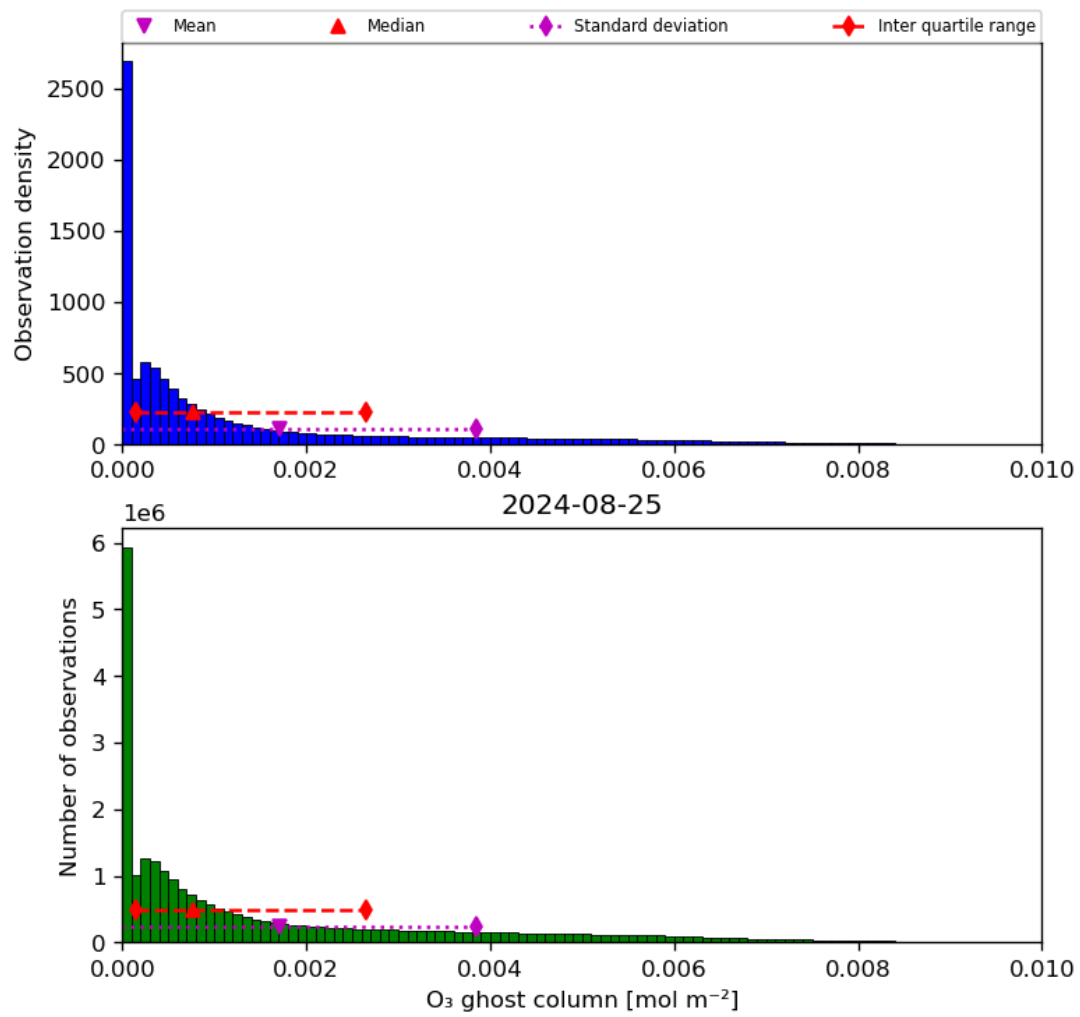
Figure 25: Histogram of “O 3 ghost column” for 2024-08-24 to 2024-08-26
