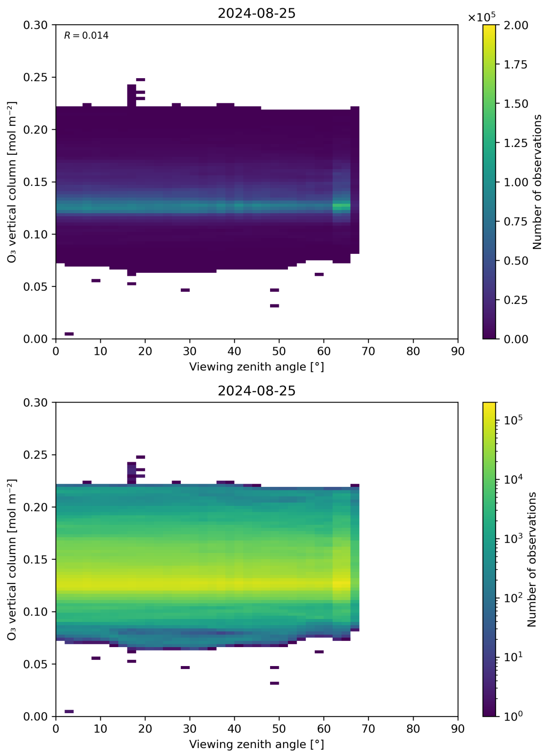
Figure 52: Scatter density plot of “Viewing zenith angle” against “O 3 vertical column” for 2024-08-24 to 2024-08-26.
