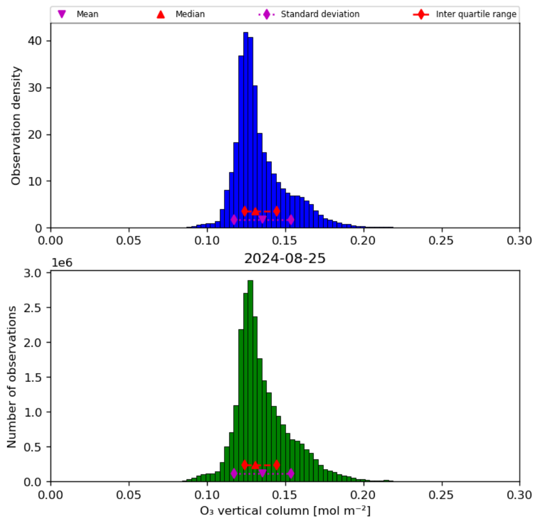
Figure 21: Histogram of “O 3 vertical column” for 2024-08-24 to 2024-08-26
