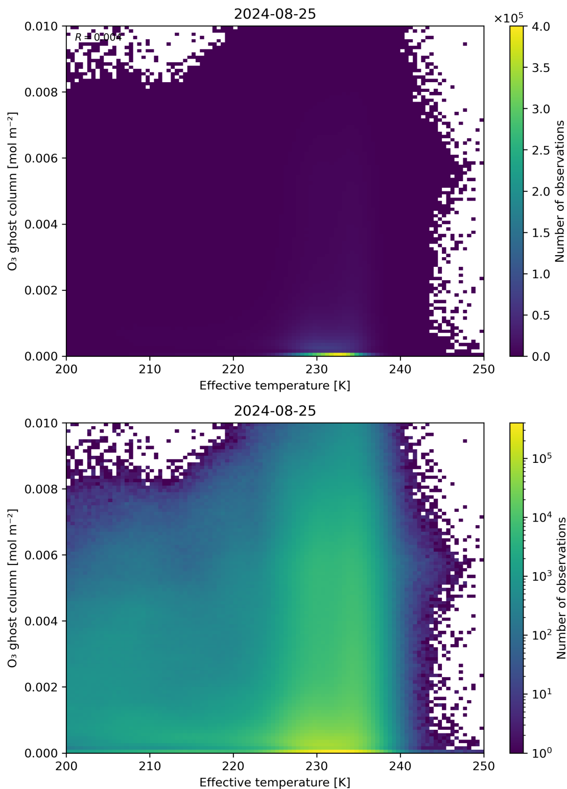
Figure 38: Scatter density plot of “Effective temperature” against “O 3 ghost column” for 2024-08-24 to 2024-08-26.
