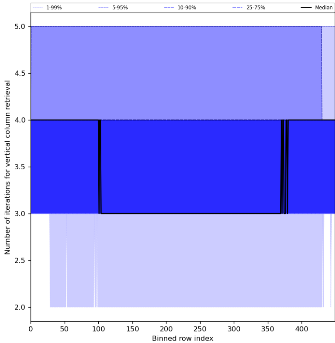
Figure 33: Along track statistics of “Number of iterations for vertical column retrieval” for 2024-08-24 to 2024-08-26
