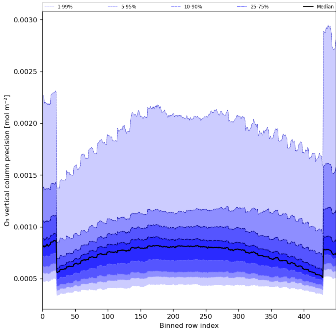
Figure 29: Along track statistics of “O 3 vertical column precision” for 2024-08-24 to 2024-08-26
