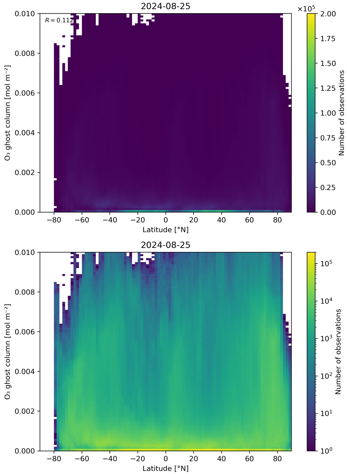
Figure 35: Scatter density plot of “Latitude” against “O 3 ghost column” for 2024-08-24 to 2024-08-26.
