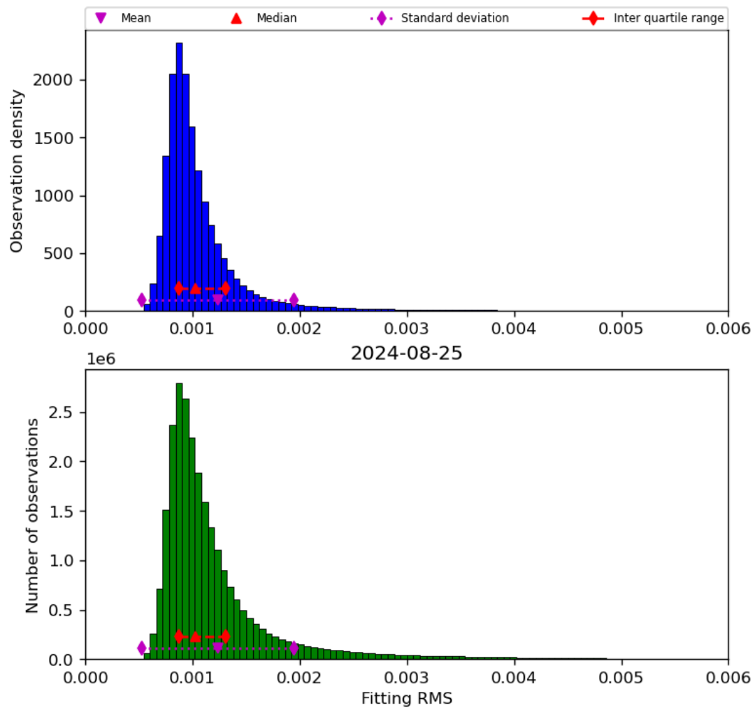
Figure 23: Histogram of “Fitting RMS” for 2024-08-24 to 2024-08-26
