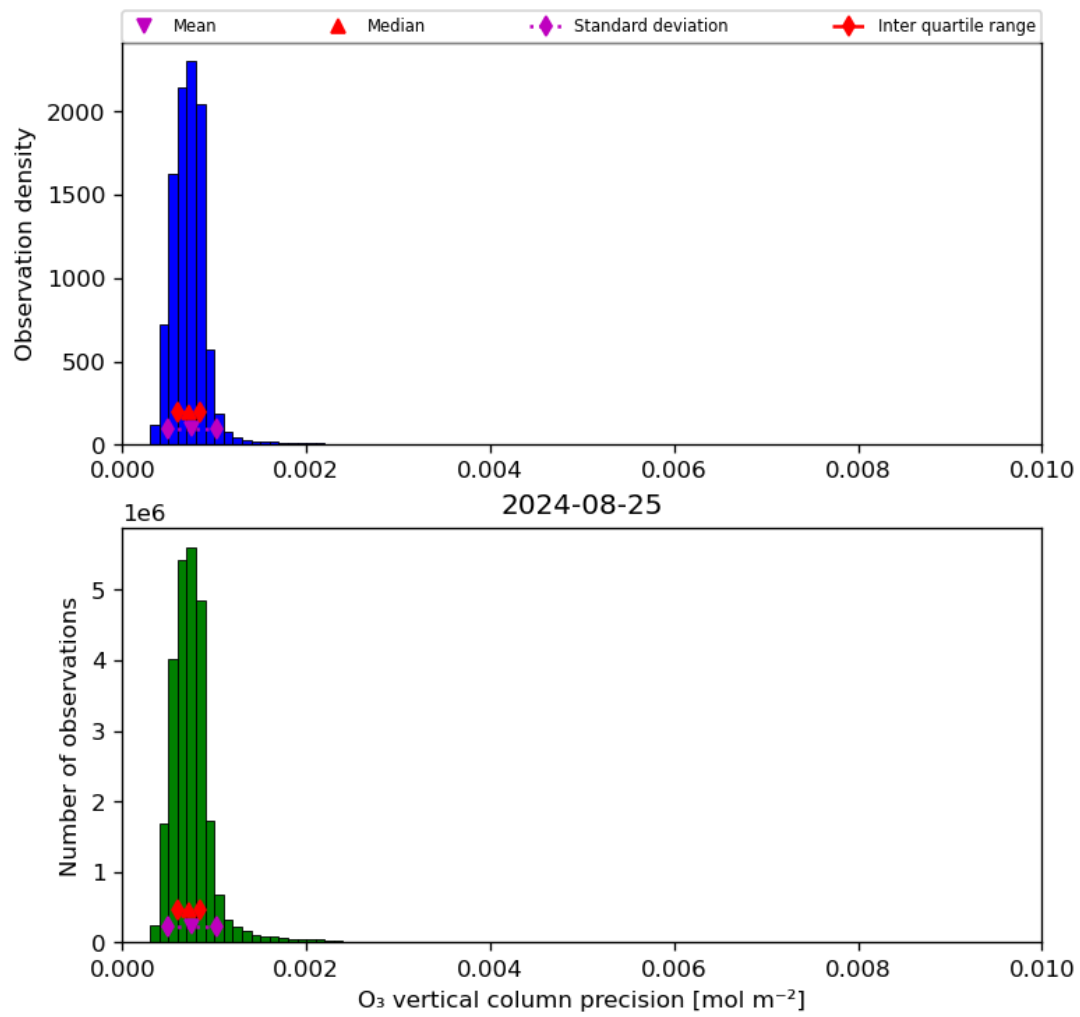
Figure 22: Histogram of “O 3 vertical column precision” for 2024-08-24 to 2024-08-26
