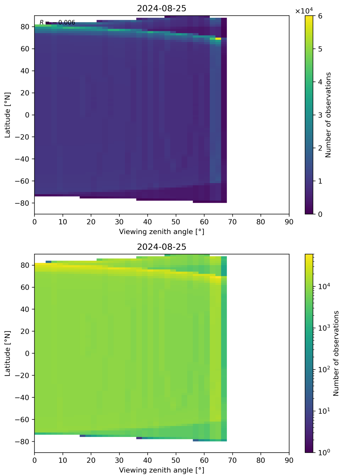
Figure 49: Scatter density plot of “Viewing zenith angle” against “Latitude” for 2024-08-24 to 2024-08-26.
