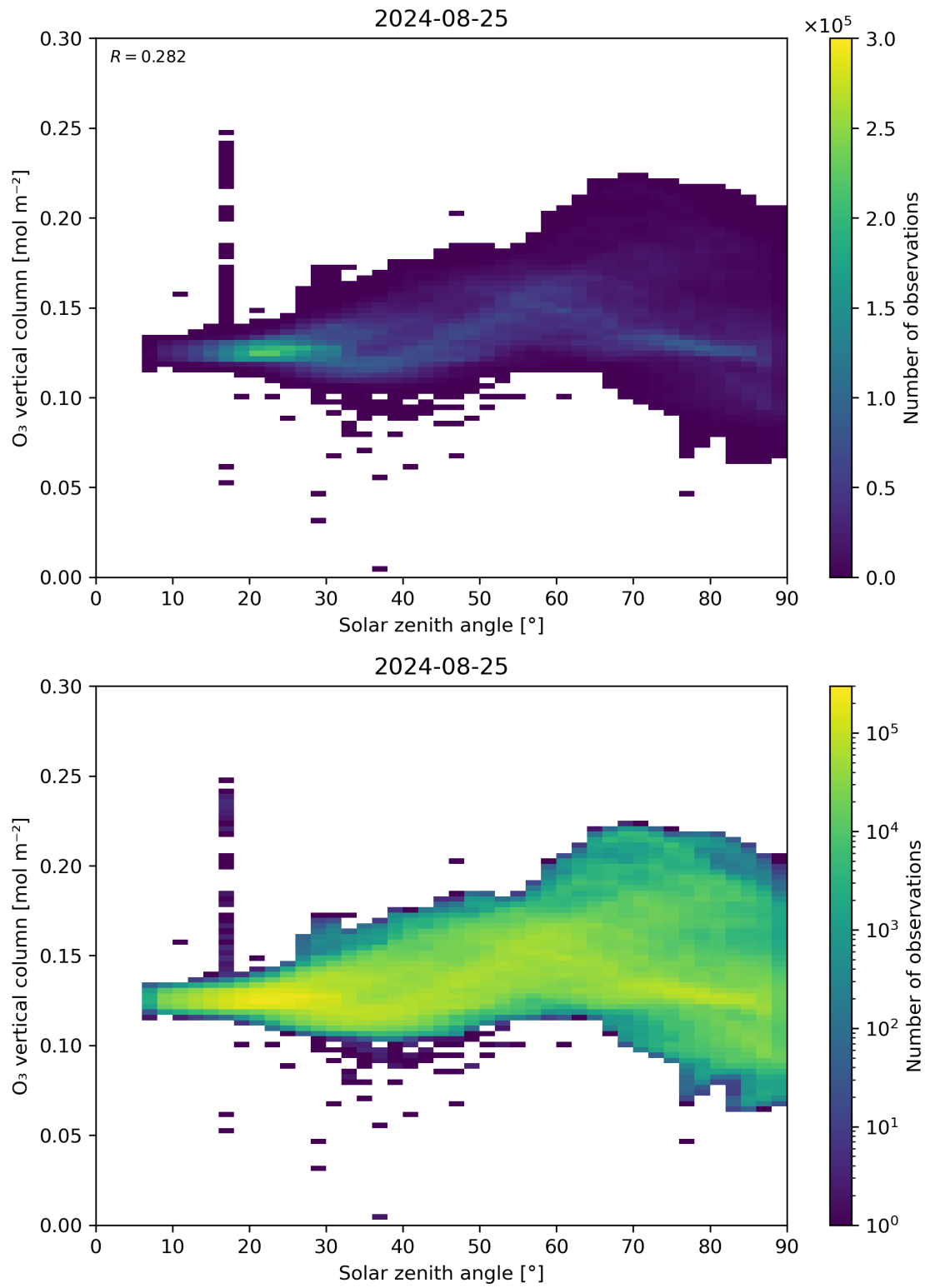
Figure 47: Scatter density plot of “Solar zenith angle” against “O 3 vertical column” for 2024-08-24 to 2024-08-26.
