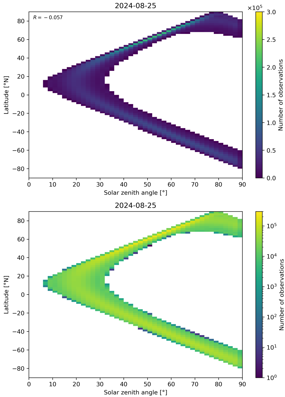
Figure 44: Scatter density plot of “Solar zenith angle” against “Latitude” for 2024-08-24 to 2024-08-26.
