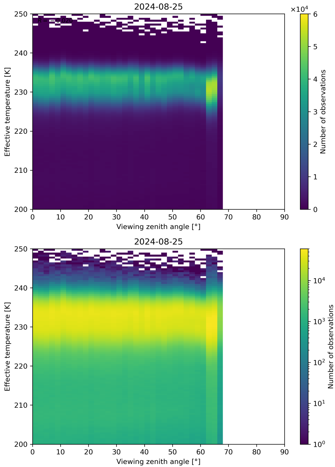
Figure 50: Scatter density plot of “Viewing zenith angle” against “Effective temperature” for 2024-08-24 to 2024-08-26.
