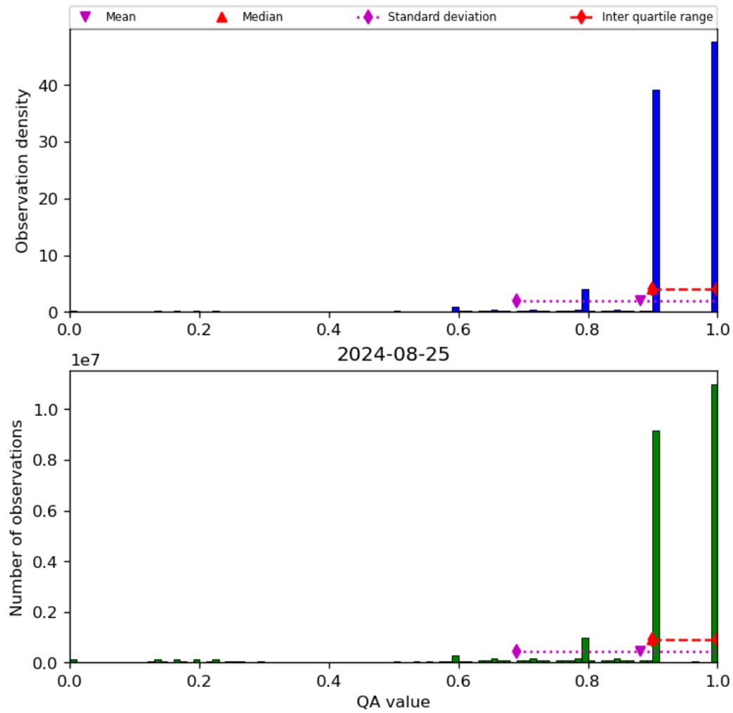
Figure 20: Histogram of “QA value” for 2024-08-24 to 2024-08-26
