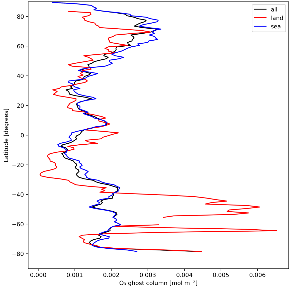
Figure 18: Zonal average of “O 3 ghost column” for 2024-08-24 to 2024-08-26.
