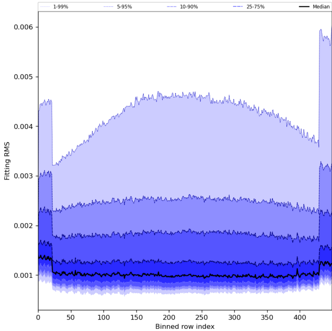
Figure 30: Along track statistics of “Fitting RMS” for 2024-08-24 to 2024-08-26
