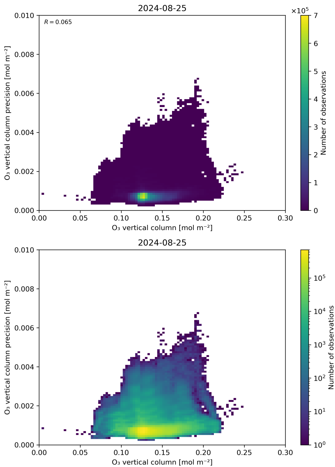
Figure 41: Scatter density plot of “O 3 vertical column” against “O 3 vertical column precision” for 2024-08-24 to 2024-08-26.
