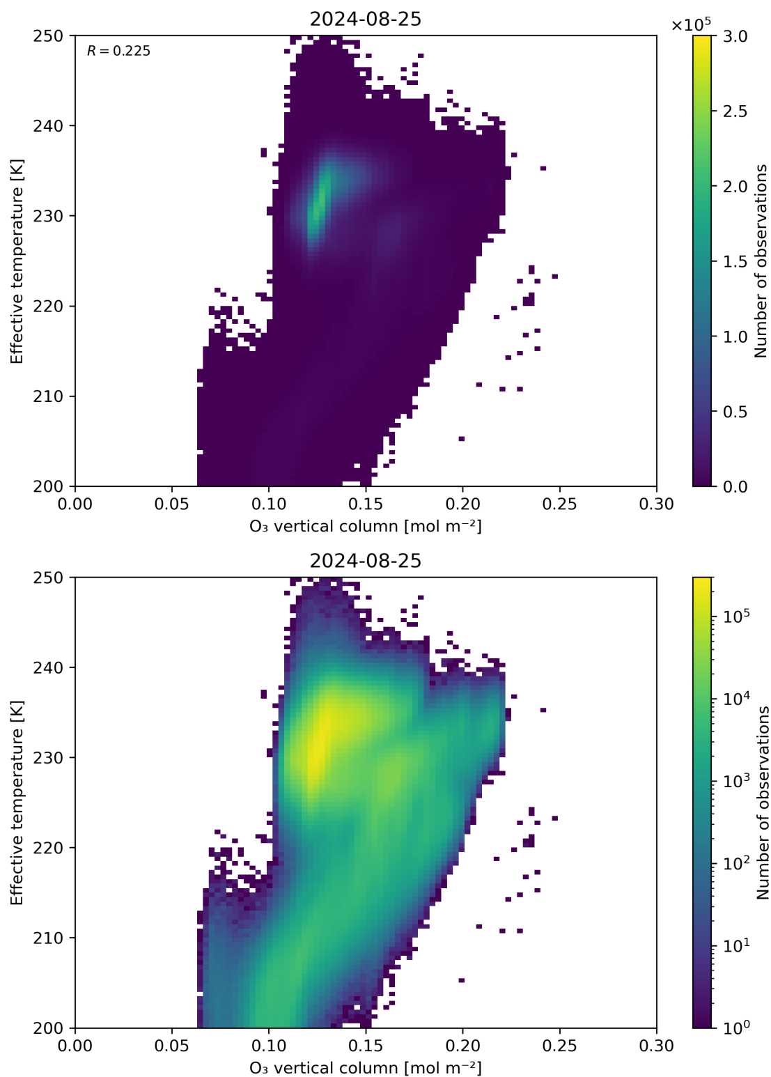
Figure 39: Scatter density plot of “O 3 vertical column” against “Effective temperature” for 2024-08-24 to 2024-08-26.
