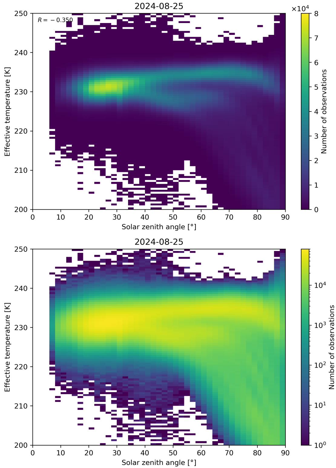
Figure 45: Scatter density plot of “Solar zenith angle” against “Effective temperature” for 2024-08-24 to 2024-08-26.
