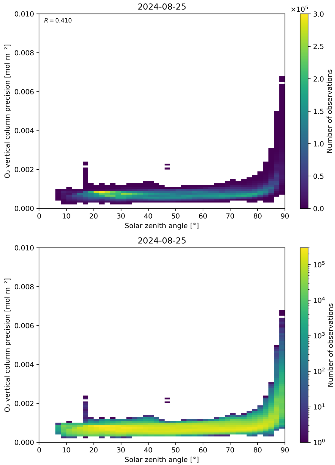
Figure 48: Scatter density plot of “Solar zenith angle” against “O 3 vertical column precision” for 2024-08-24 to 2024-08-26.
