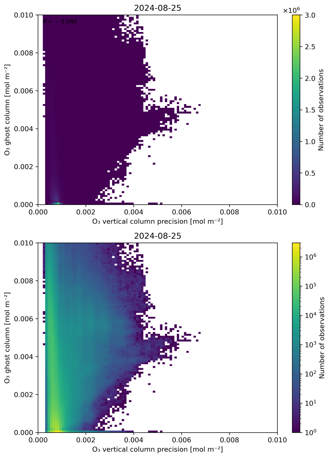
Figure 43: Scatter density plot of “ \text{O}_3 vertical column precision” against “ \text{O}_3 ghost column” for 2024-08-24 to 2024-08-26.
