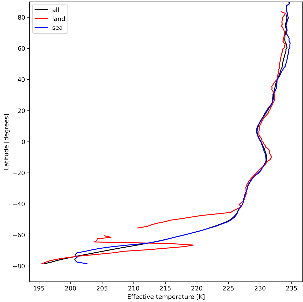
Figure 17: Zonal average of "Effective temperature" for 2024-08-24 to 2024-08-26.
