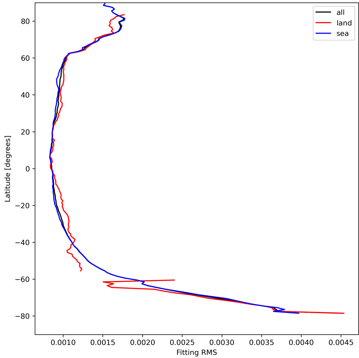
Figure 16: Zonal average of “Fitting RMS” for 2024-08-24 to 2024-08-26.
