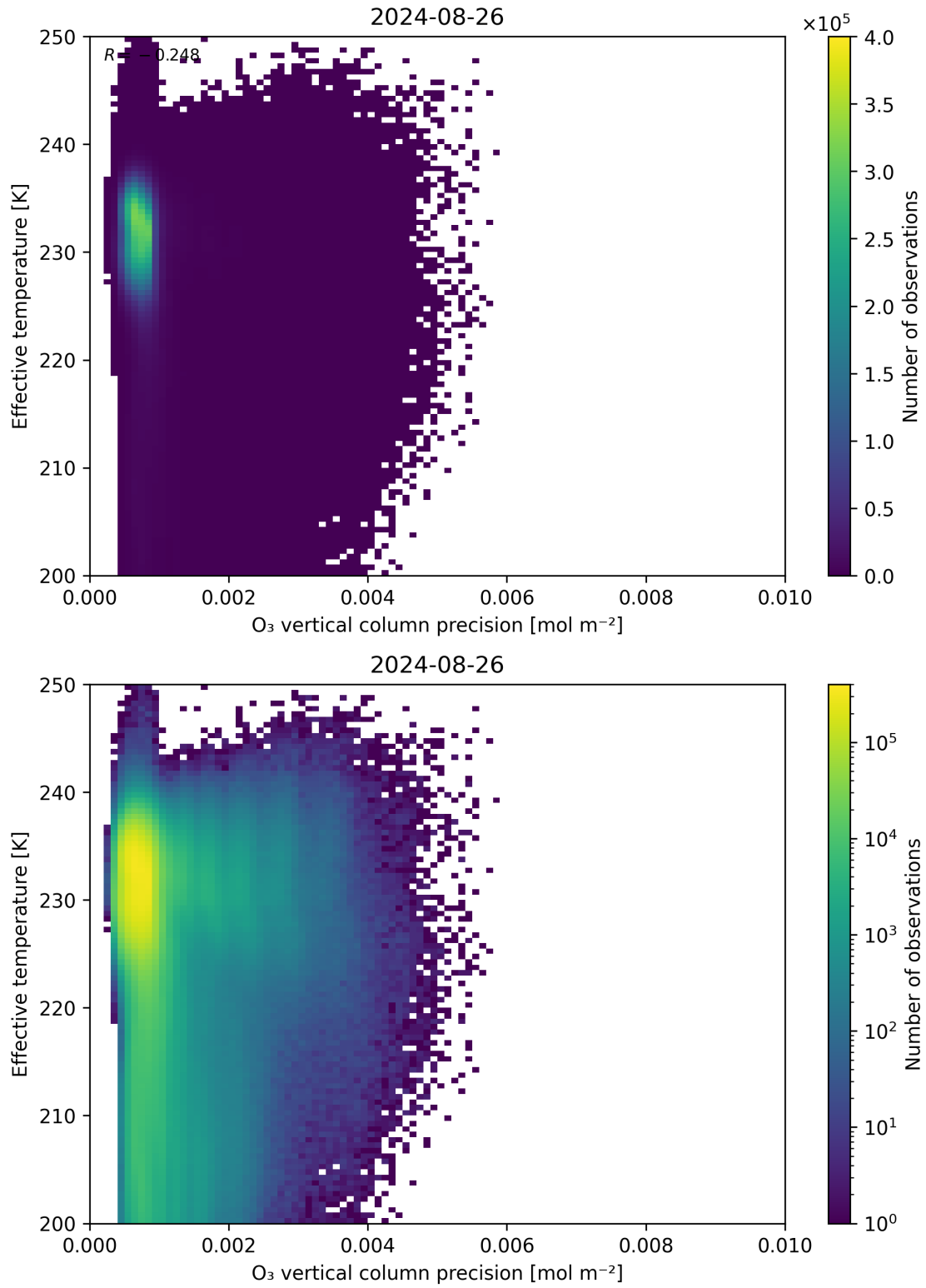
Figure 42: Scatter density plot of “O 3 vertical column precision” against “Effective temperature” for 2024-08-25 to 2024-08-27.
