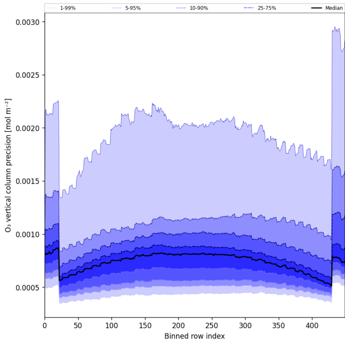
Figure 29: Along track statistics of “O 3 vertical column precision” for 2024-08-25 to 2024-08-27
