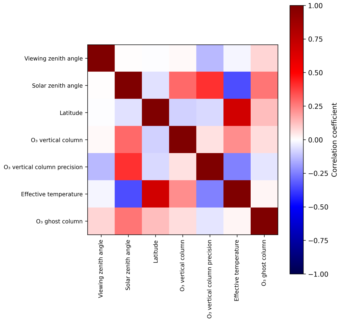
Figure 2: Map of correlation matrix for 2024-08-25 to 2024-08-27.
