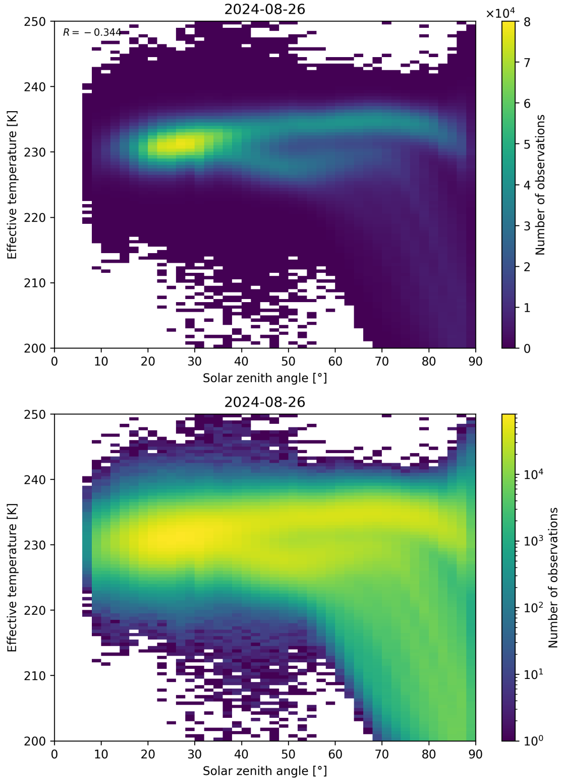
Figure 45: Scatter density plot of “Solar zenith angle” against “Effective temperature” for 2024-08-25 to 2024-08-27.
