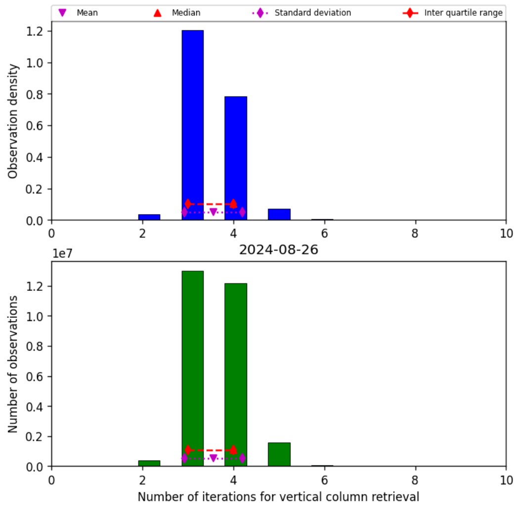
Figure 26: Histogram of “Number of iterations for vertical column retrieval” for 2024-08-25 to 2024-08-27
