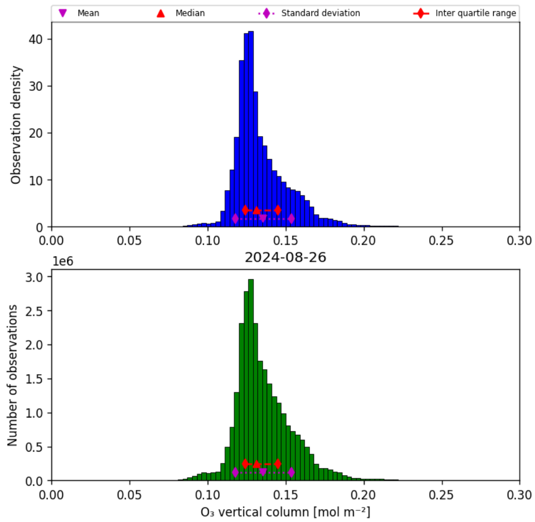
Figure 21: Histogram of “O 3 vertical column” for 2024-08-25 to 2024-08-27
