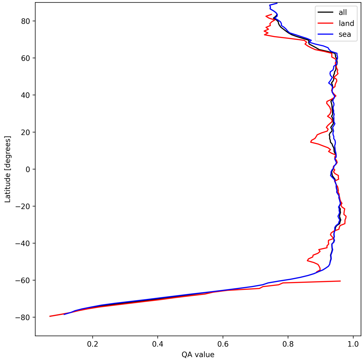
Figure 13: Zonal average of “QA value” for 2024-08-25 to 2024-08-27.
