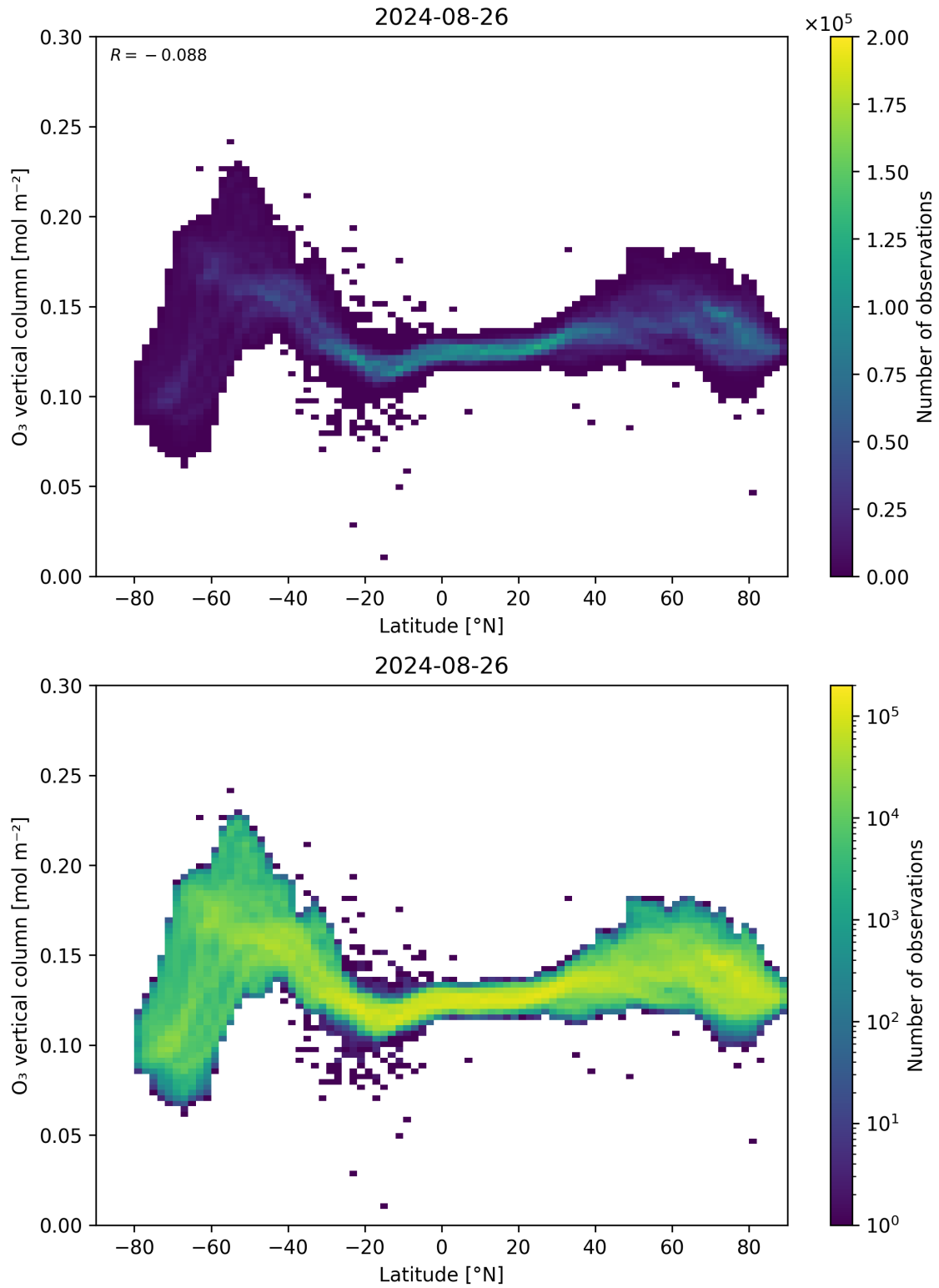
Figure 36: Scatter density plot of “Latitude” against “O 3 vertical column” for 2024-08-25 to 2024-08-27.
