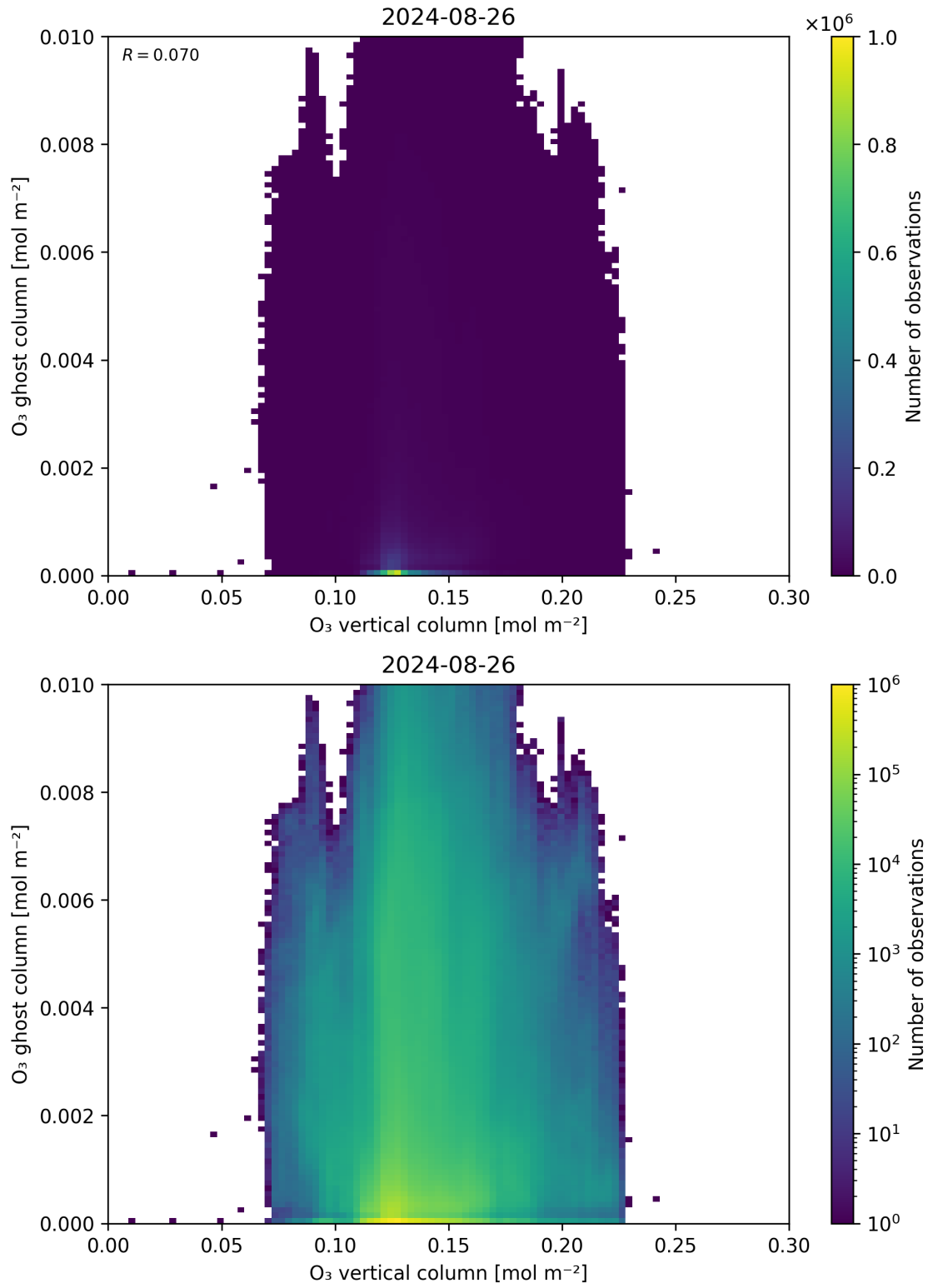
Figure 40: Scatter density plot of “O 3 vertical column” against “O 3 ghost column” for 2024-08-25 to 2024-08-27.
