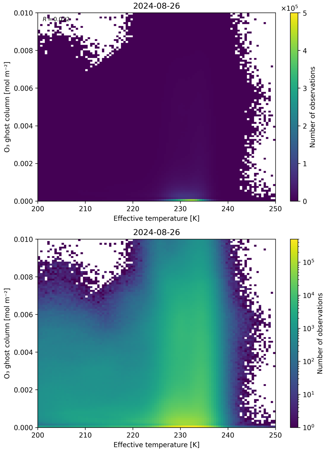
Figure 38: Scatter density plot of “Effective temperature” against “O 3 ghost column” for 2024-08-25 to 2024-08-27.
