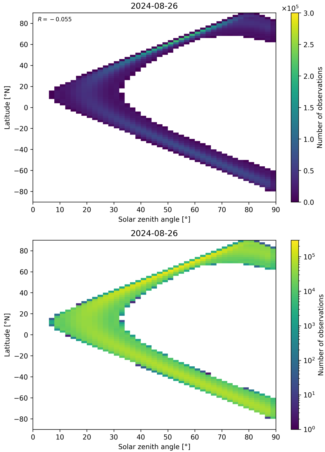
Figure 44: Scatter density plot of “Solar zenith angle” against “Latitude” for 2024-08-25 to 2024-08-27.
