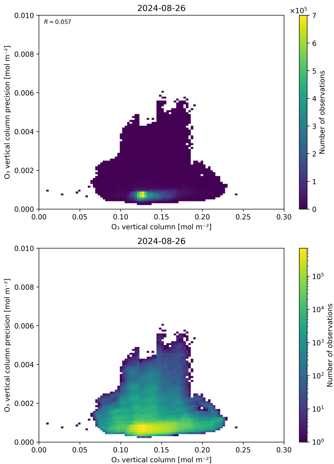
Figure 41: Scatter density plot of “O 3 vertical column” against “O 3 vertical column precision” for 2024-08-25 to 2024-08-27.
