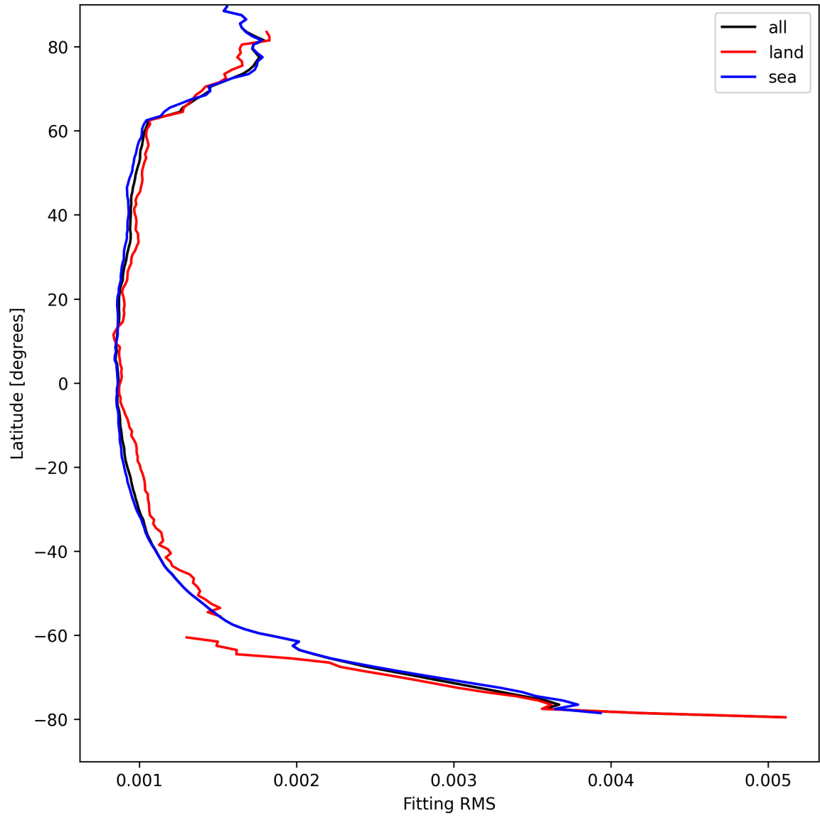
Figure 16: Zonal average of “Fitting RMS” for 2024-08-25 to 2024-08-27.
