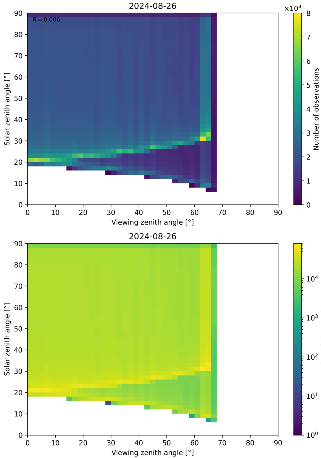
Figure 54: Scatter density plot of “Viewing zenith angle” against “Solar zenith angle” for 2024-08-25 to 2024-08-27.
