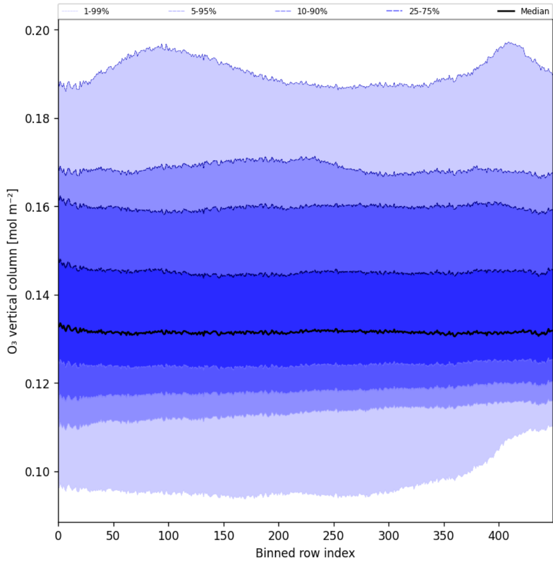
Figure 28: Along track statistics of “O 3 vertical column” for 2024-08-25 to 2024-08-27
