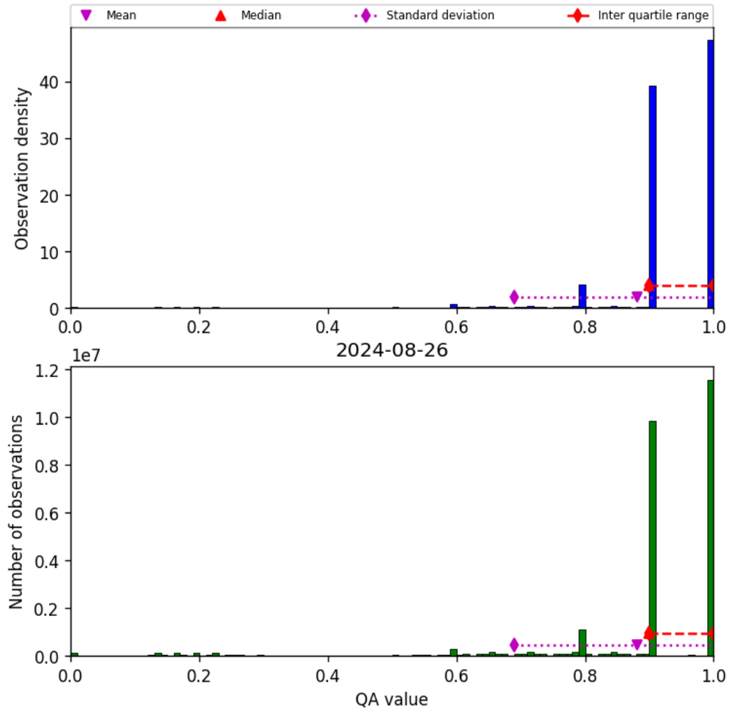
Figure 20: Histogram of “QA value” for 2024-08-25 to 2024-08-27
