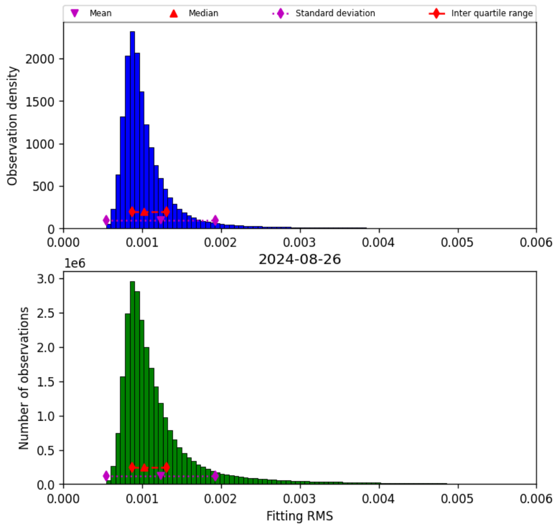
Figure 23: Histogram of “Fitting RMS” for 2024-08-25 to 2024-08-27
