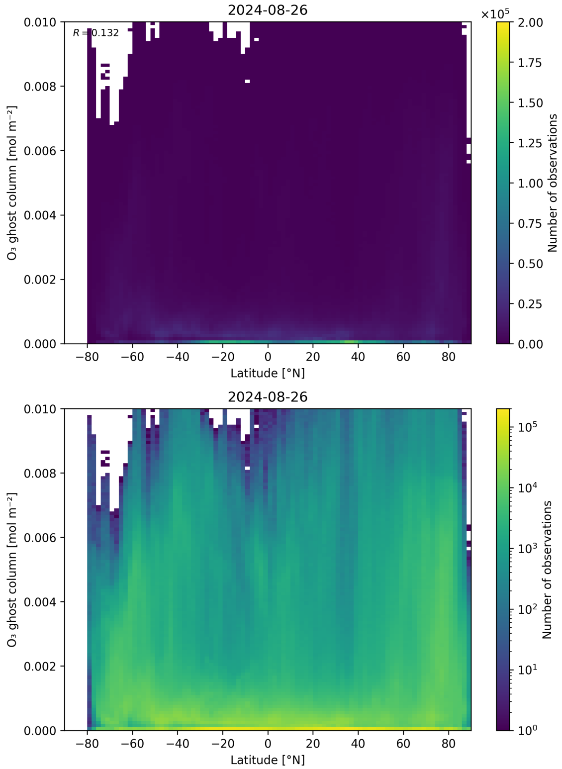
Figure 35: Scatter density plot of “Latitude” against “O 3 ghost column” for 2024-08-25 to 2024-08-27.
