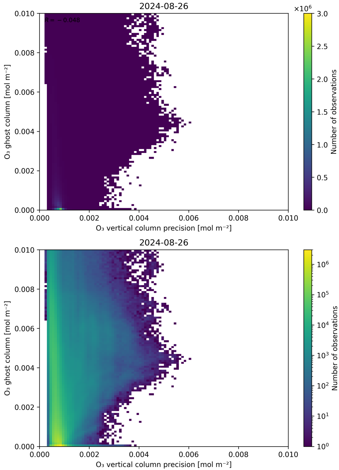
Figure 43: Scatter density plot of “ \text{O}_3 vertical column precision” against “ \text{O}_3 ghost column” for 2024-08-25 to 2024-08-27.
