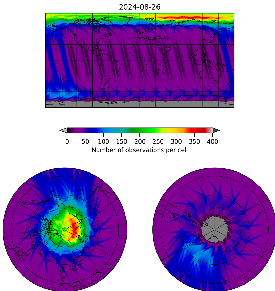
Figure 12: Map of the number of observations for 2024-08-25 to 2024-08-27
