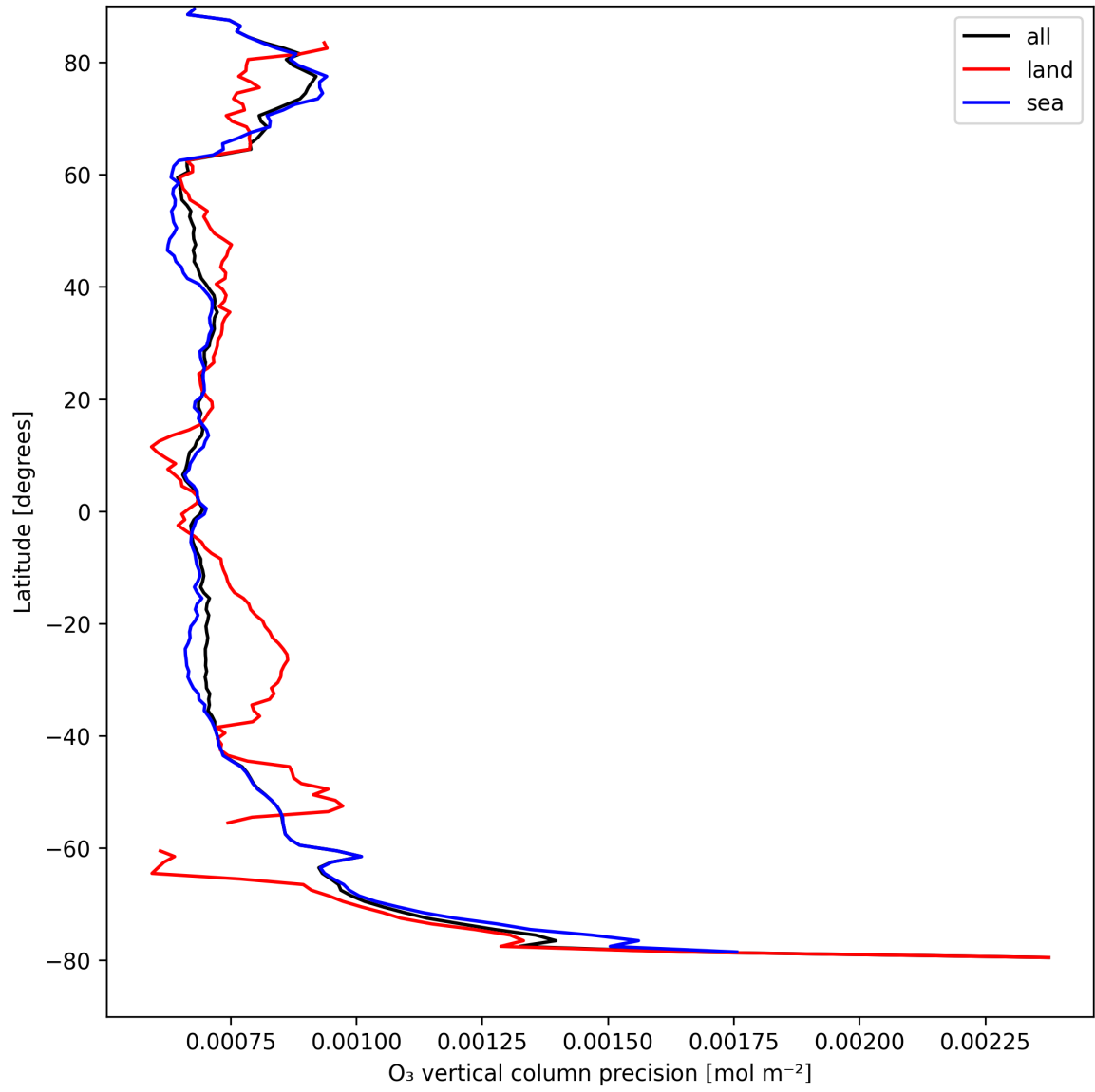
Figure 15: Zonal average of "O 3 vertical column precision" for 2024-08-25 to 2024-08-27.
