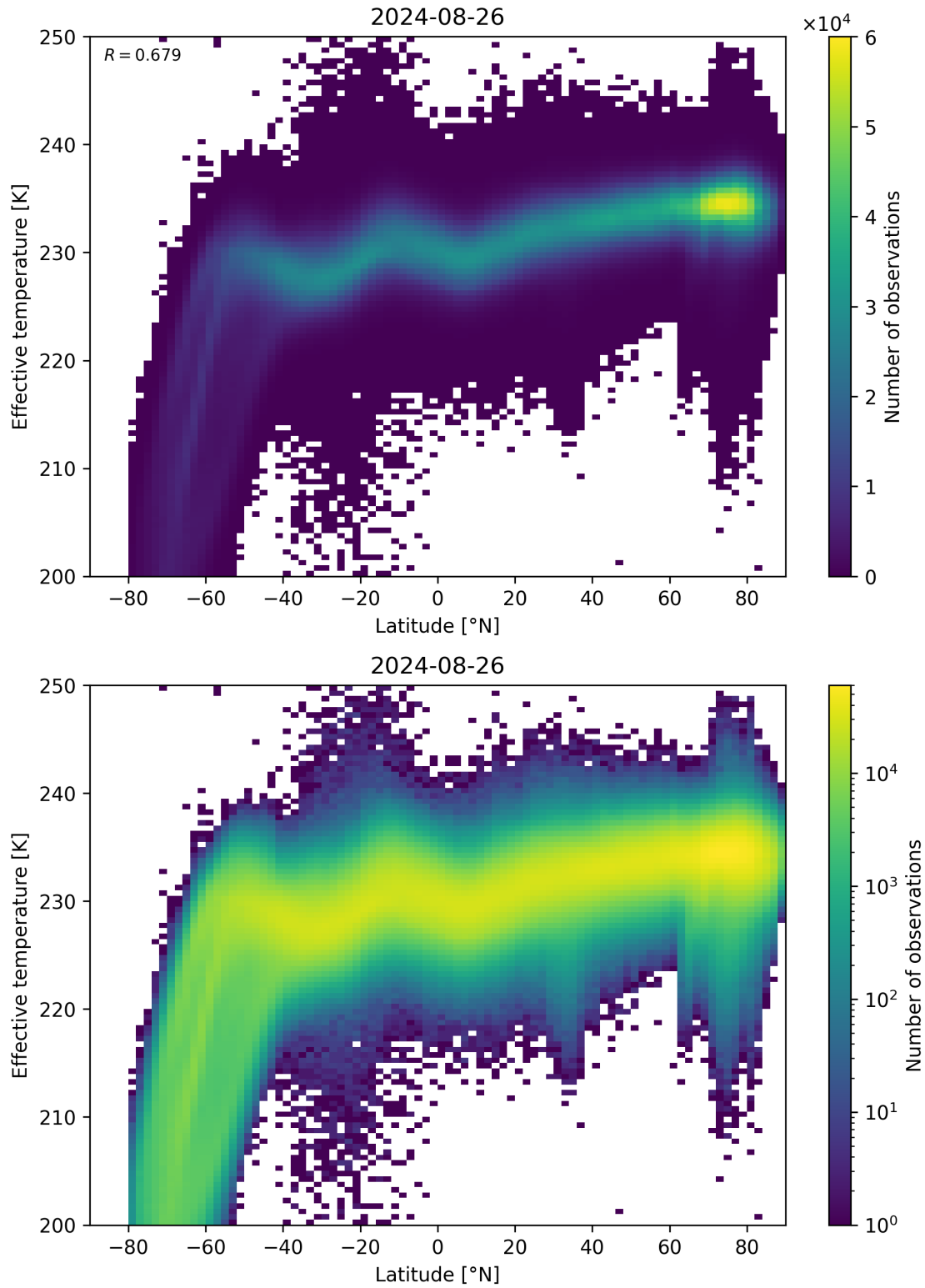
Figure 34: Scatter density plot of “Latitude” against “Effective temperature” for 2024-08-25 to 2024-08-27.
