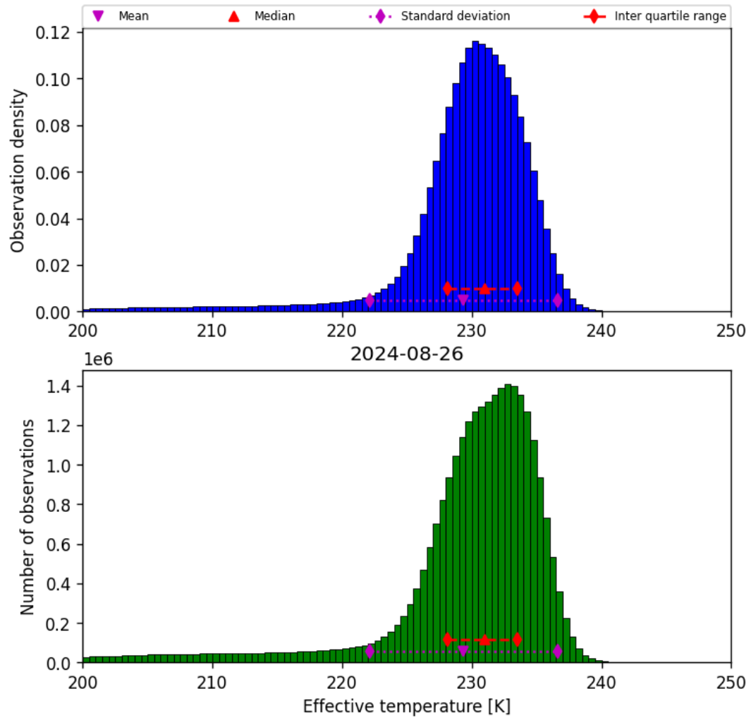
Figure 24: Histogram of “Effective temperature” for 2024-08-25 to 2024-08-27
