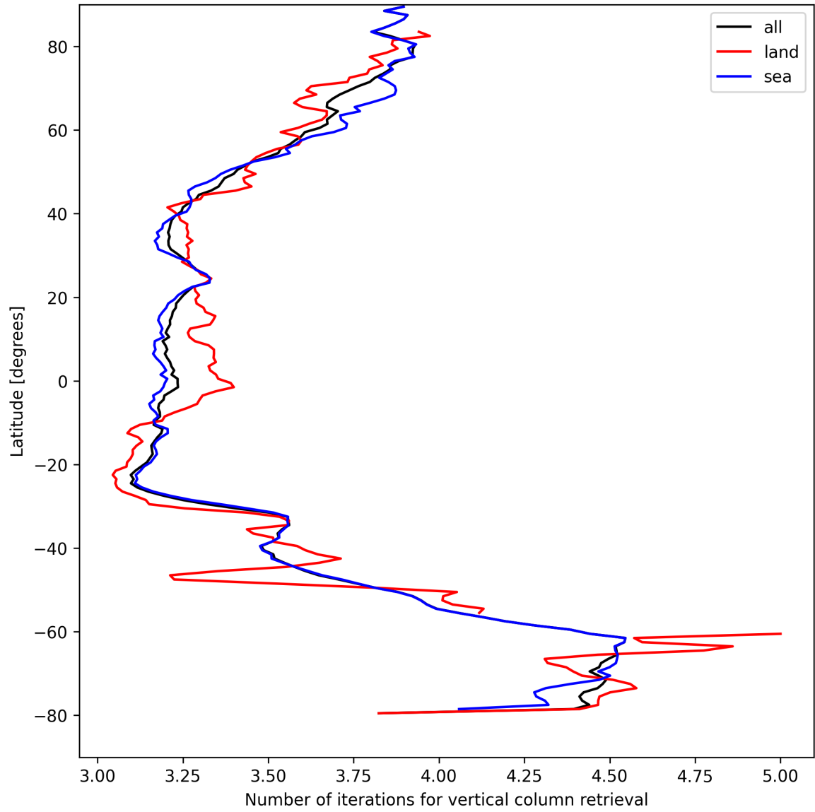
Figure 19: Zonal average of “Number of iterations for vertical column retrieval” for 2024-08-25 to 2024-08-27.
