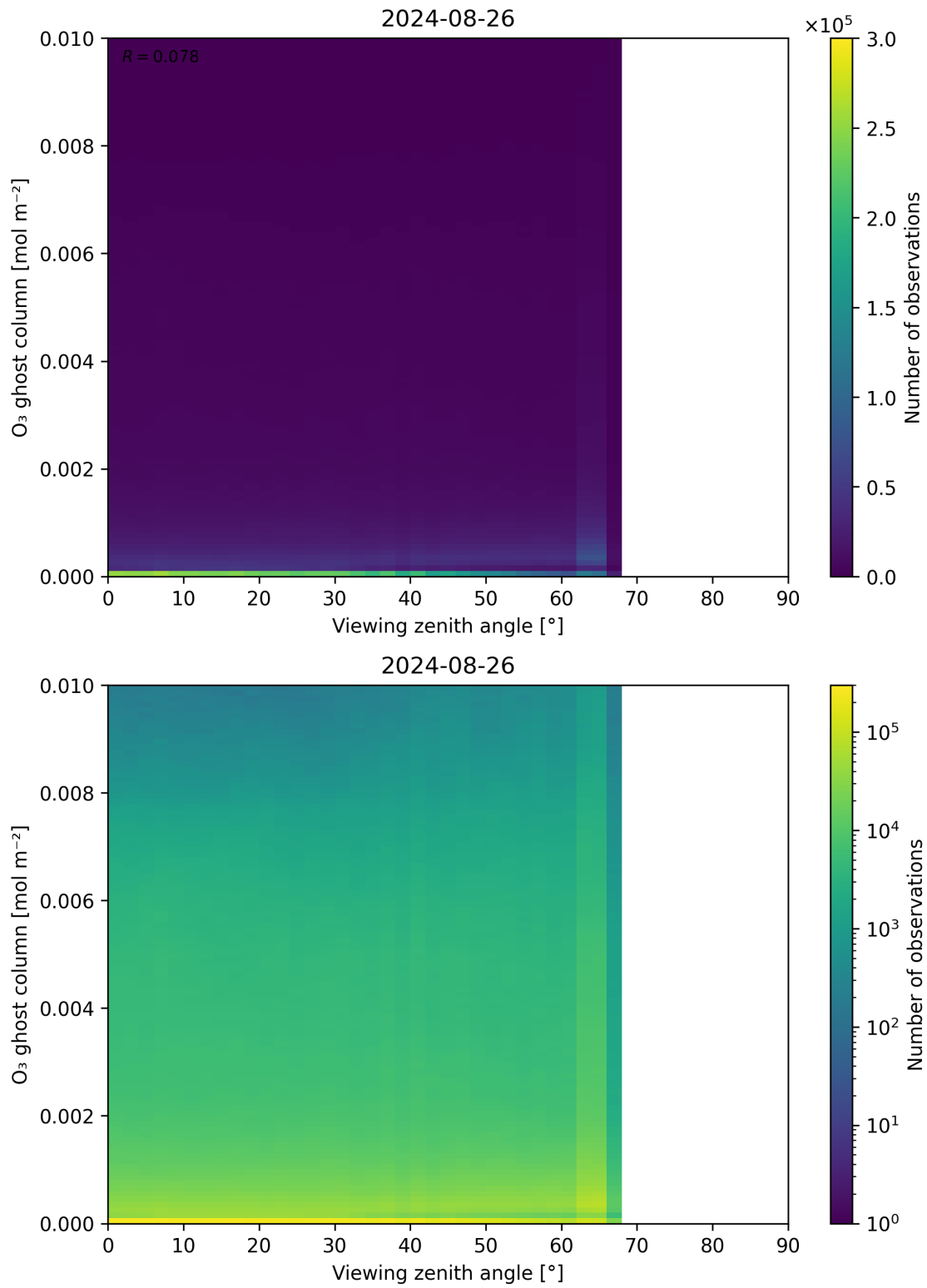
Figure 51: Scatter density plot of “Viewing zenith angle” against “O 3 ghost column” for 2024-08-25 to 2024-08-27.
