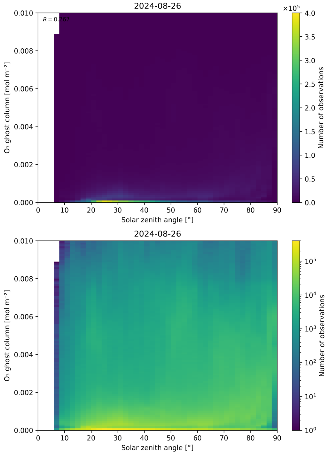
Figure 46: Scatter density plot of “Solar zenith angle” against “O 3 ghost column” for 2024-08-25 to 2024-08-27.
