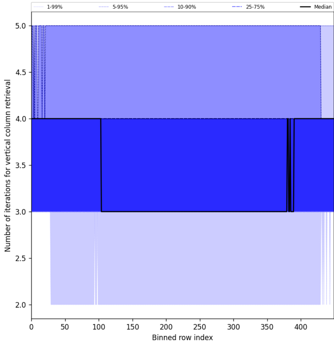
Figure 33: Along track statistics of “Number of iterations for vertical column retrieval” for 2024-08-25 to 2024-08-27
