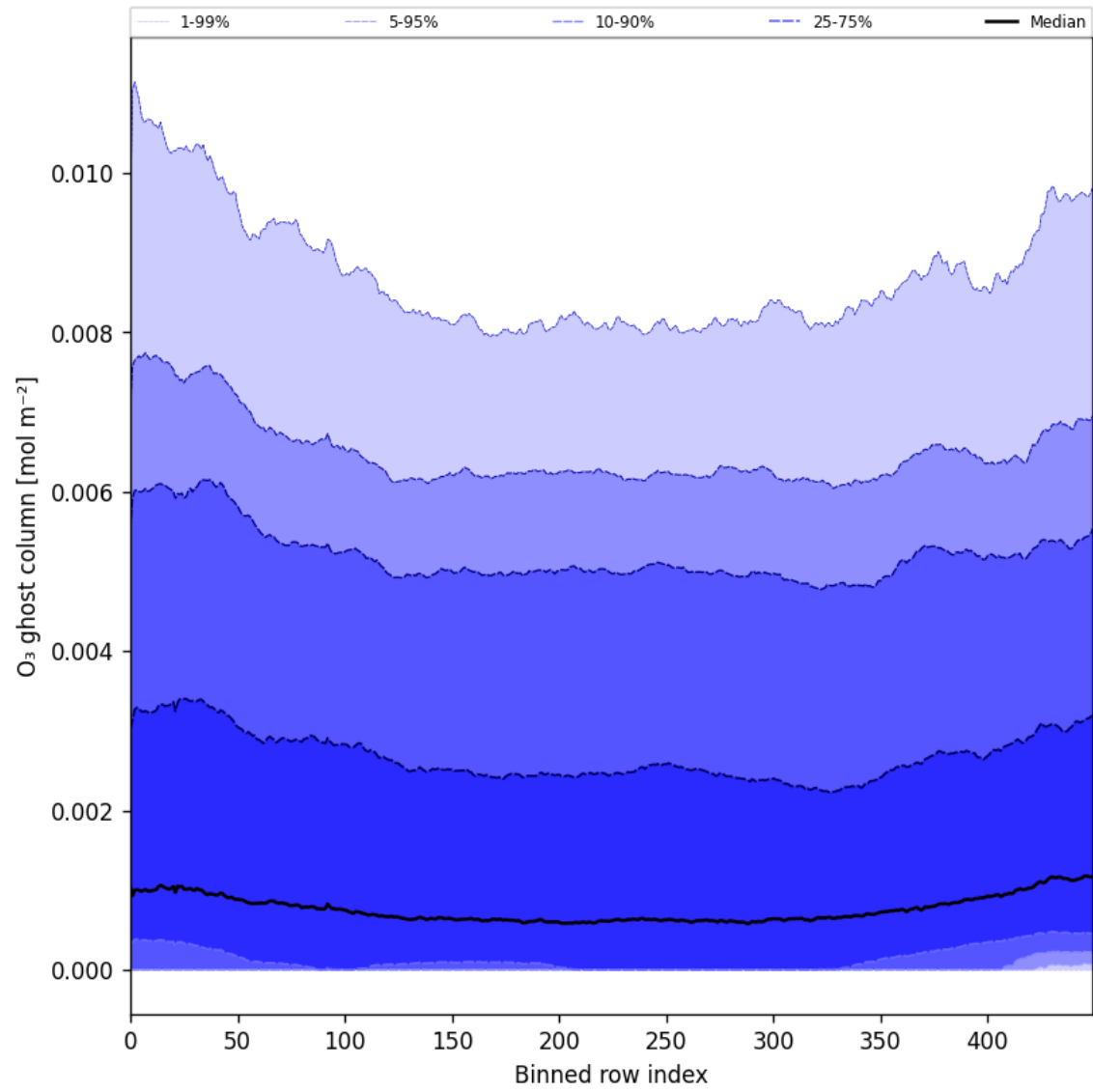
Figure 32: Along track statistics of “O 3 ghost column” for 2024-08-25 to 2024-08-27
