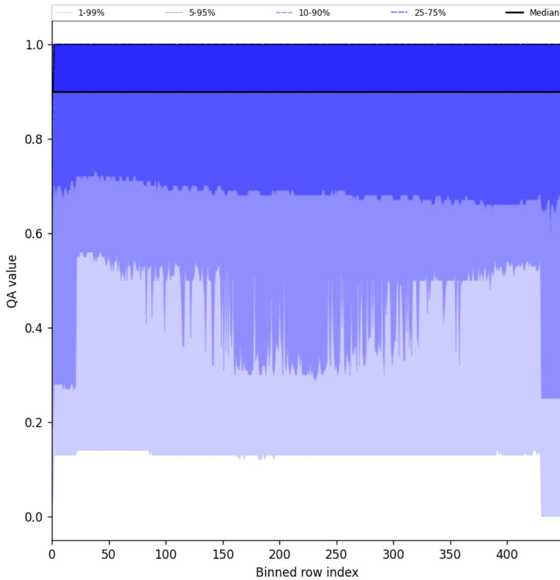
Figure 27: Along track statistics of “QA value” for 2024-08-25 to 2024-08-27
