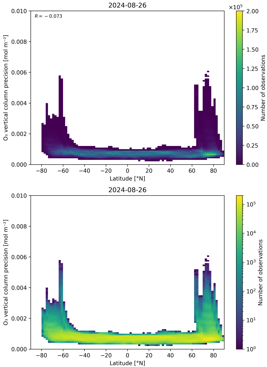
Figure 37: Scatter density plot of “Latitude” against “O 3 vertical column precision” for 2024-08-25 to 2024-08-27.
