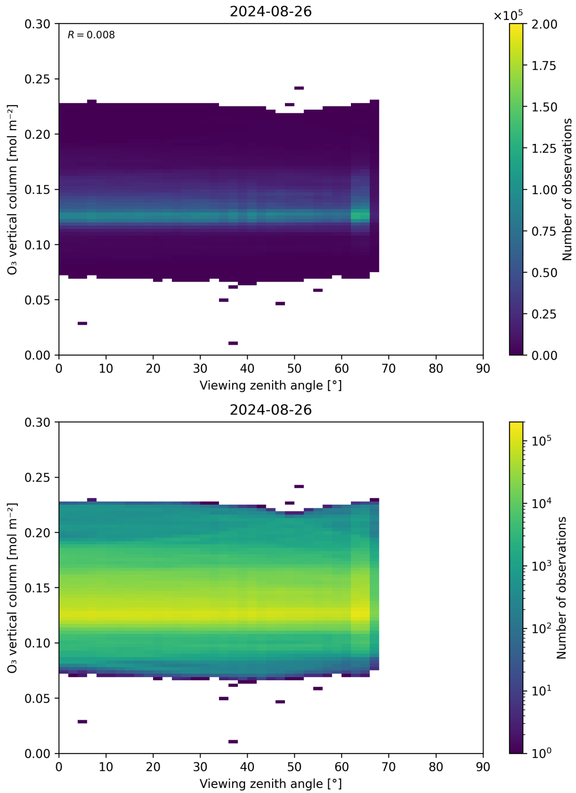
Figure 52: Scatter density plot of “Viewing zenith angle” against “O 3 vertical column” for 2024-08-25 to 2024-08-27.
