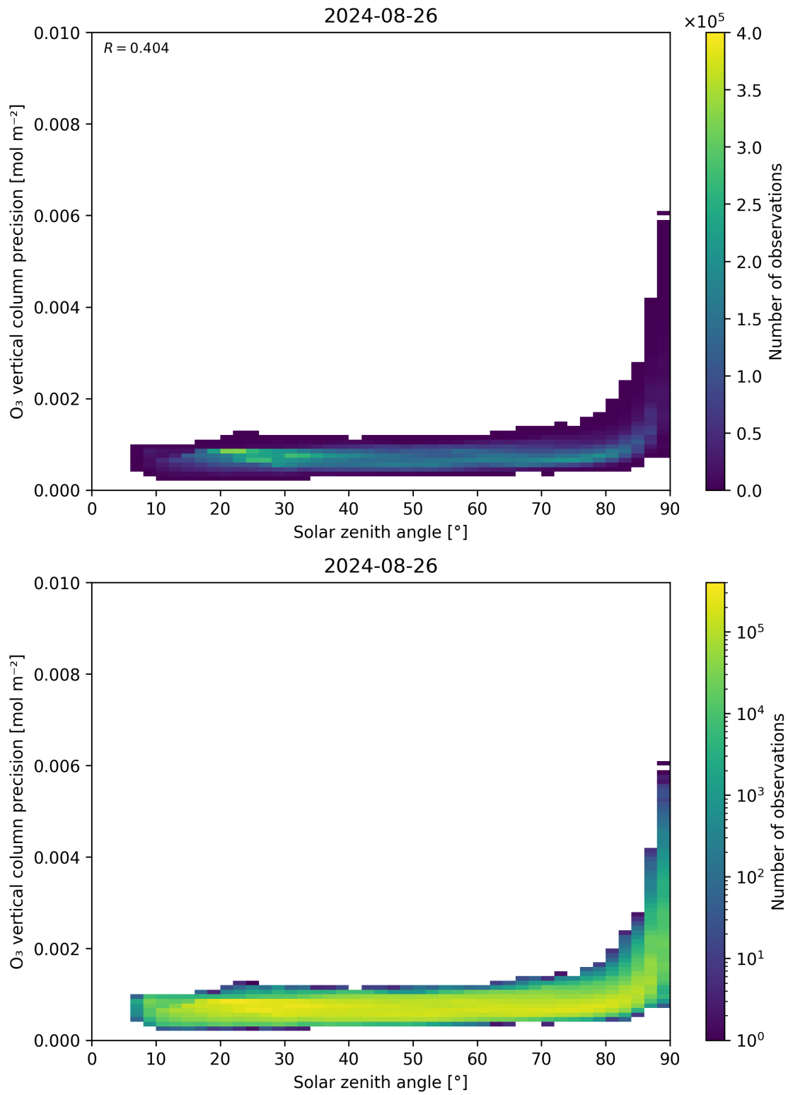
Figure 48: Scatter density plot of “Solar zenith angle” against “O 3 vertical column precision” for 2024-08-25 to 2024-08-27.
