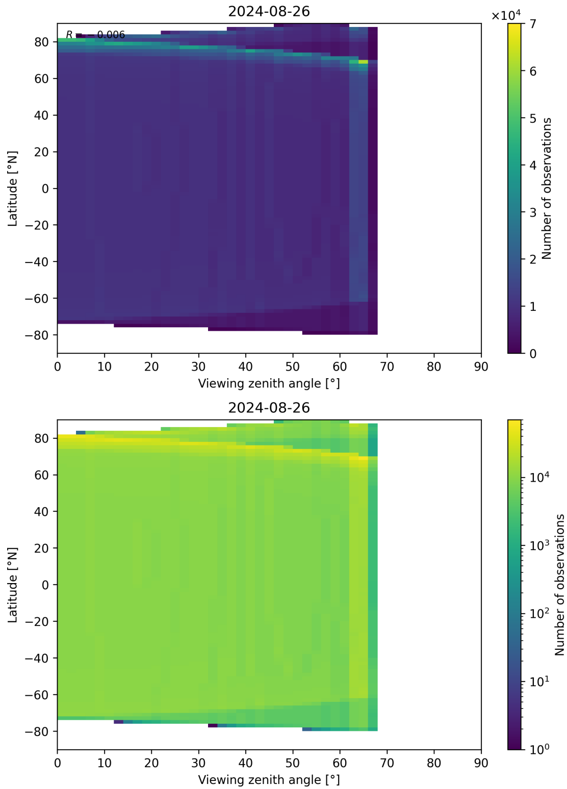
Figure 49: Scatter density plot of “Viewing zenith angle” against “Latitude” for 2024-08-25 to 2024-08-27.
