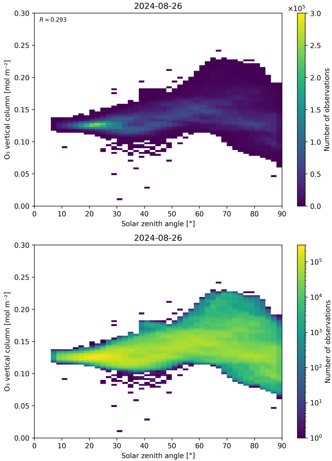
Figure 47: Scatter density plot of “Solar zenith angle” against “O 3 vertical column” for 2024-08-25 to 2024-08-27.
