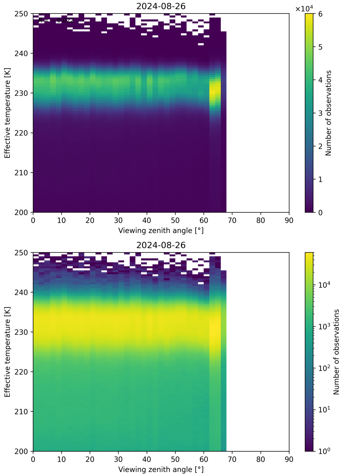
Figure 50: Scatter density plot of “Viewing zenith angle” against “Effective temperature” for 2024-08-25 to 2024-08-27.
