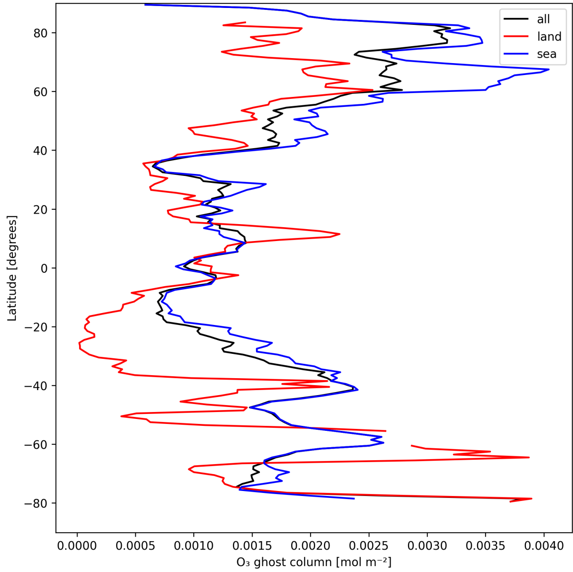
Figure 18: Zonal average of “O 3 ghost column” for 2024-08-25 to 2024-08-27.
