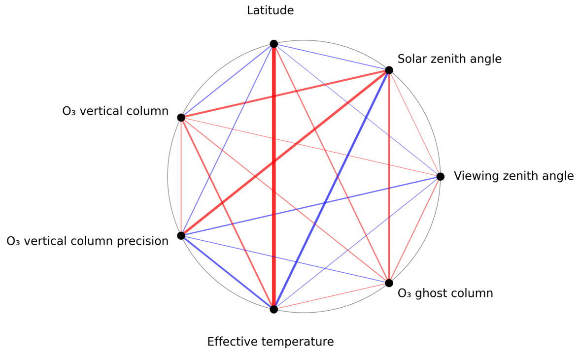
Figure 1: Map of correlation graph for 2024-08-25 to 2024-08-27.
