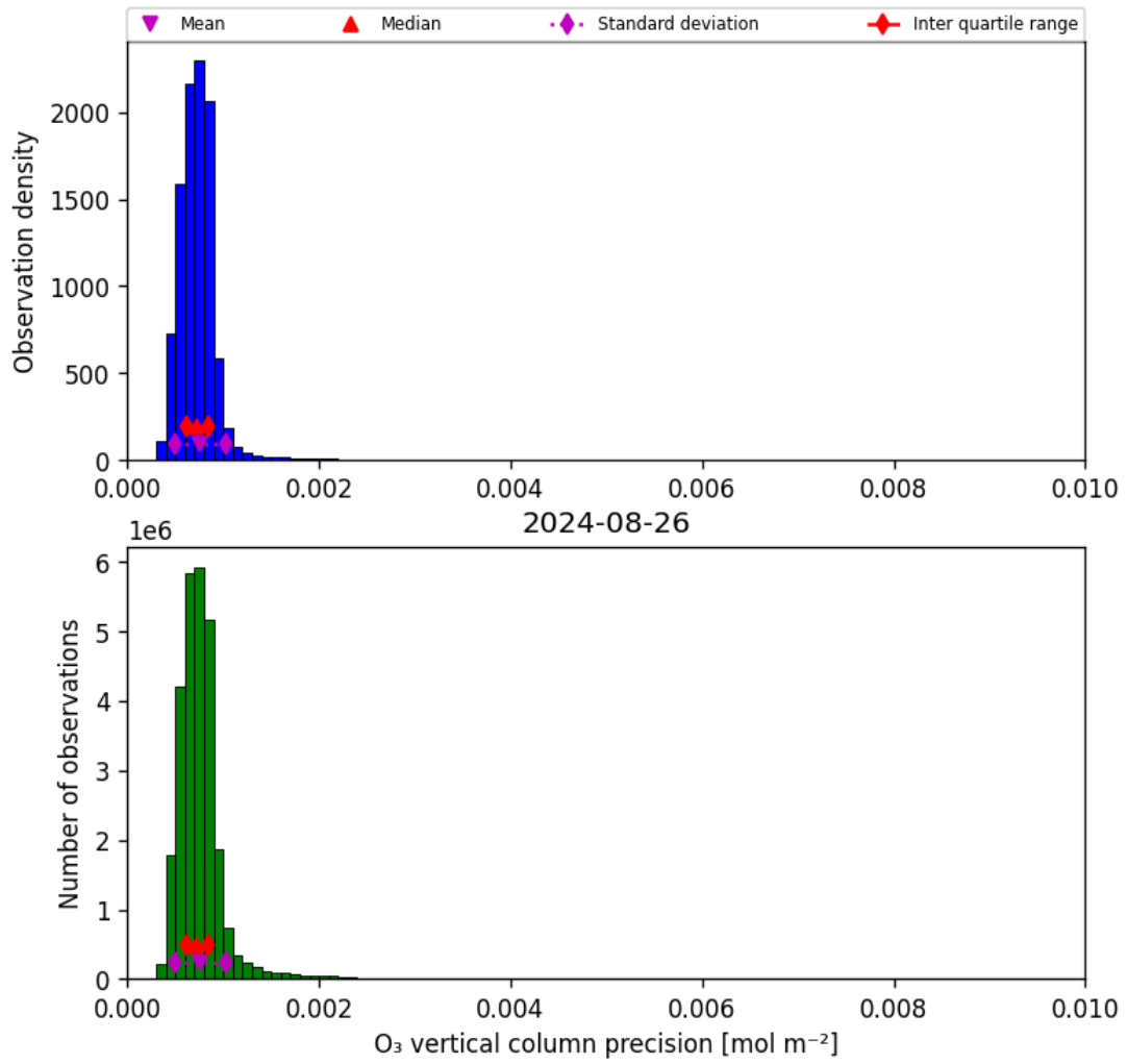
Figure 22: Histogram of “O 3 vertical column precision” for 2024-08-25 to 2024-08-27
