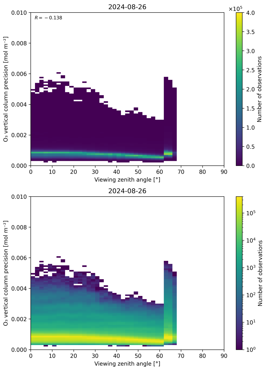
Figure 53: Scatter density plot of “Viewing zenith angle” against “O 3 vertical column precision” for 2024-08-25 to 2024-08-27.
