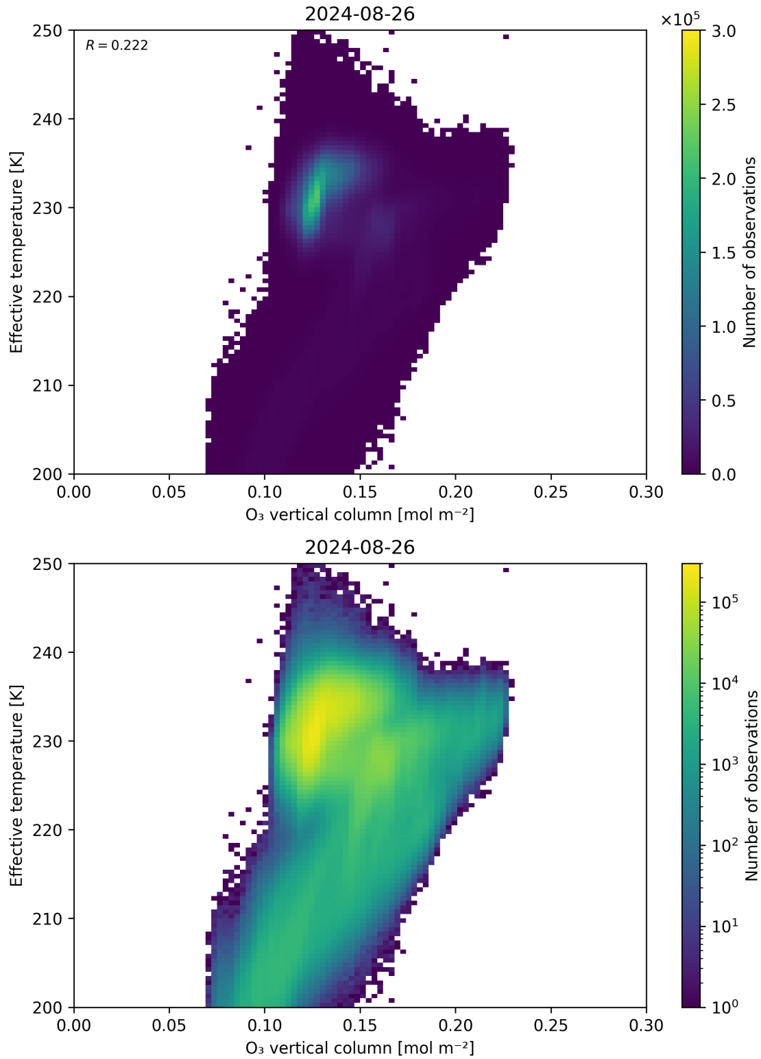
Figure 39: Scatter density plot of “O 3 vertical column” against “Effective temperature” for 2024-08-25 to 2024-08-27.
