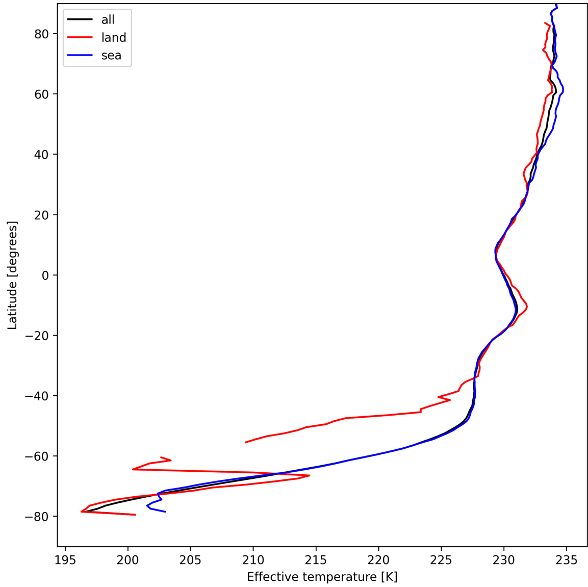
Figure 17: Zonal average of "Effective temperature" for 2024-08-25 to 2024-08-27.
