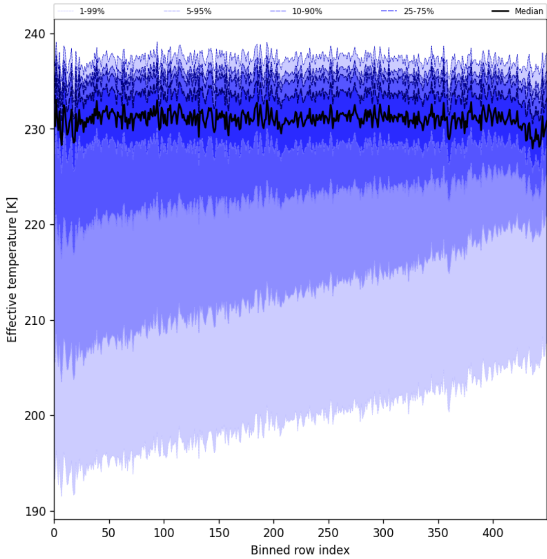
Figure 31: Along track statistics of “Effective temperature” for 2024-08-25 to 2024-08-27
