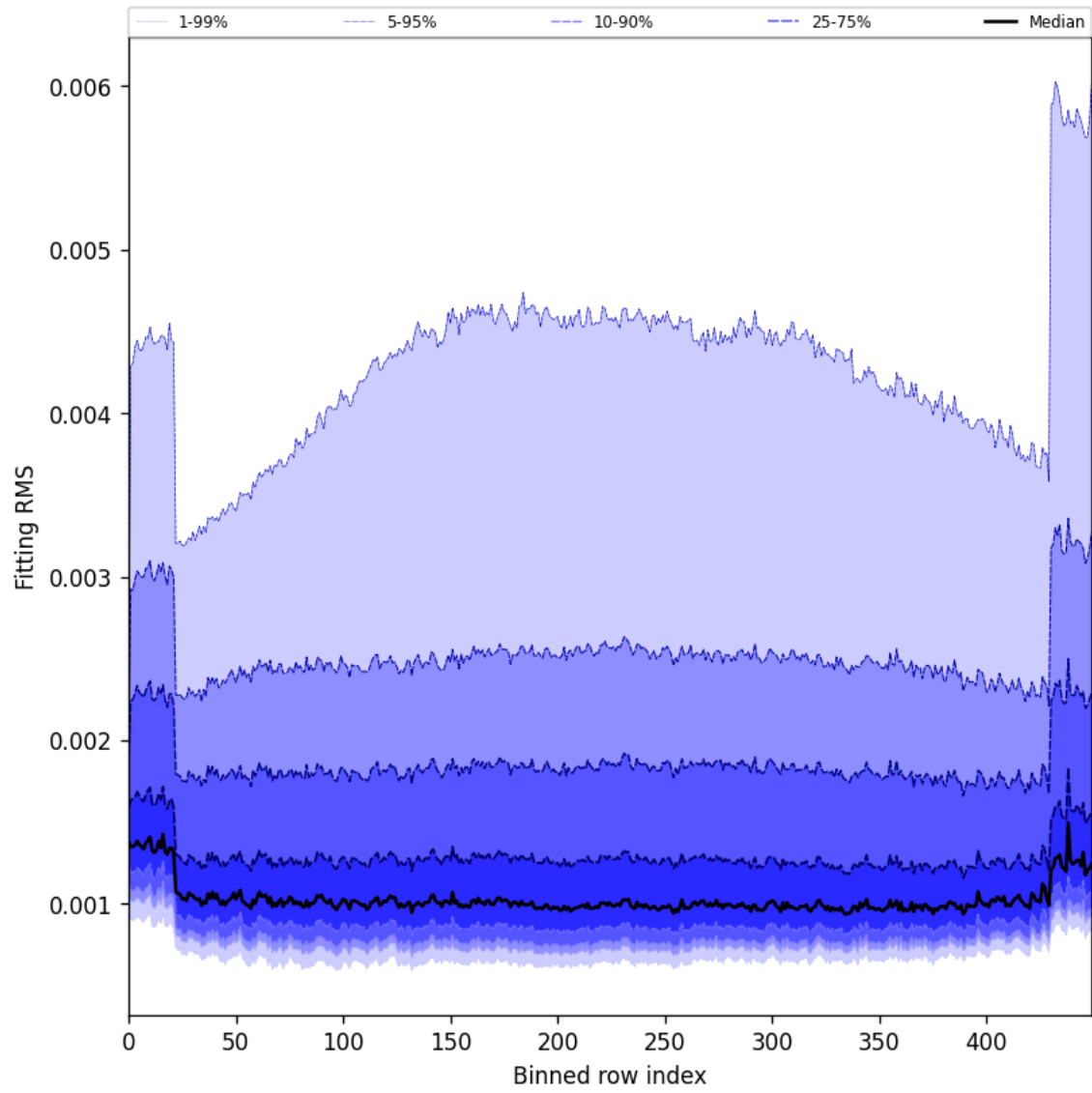
Figure 30: Along track statistics of “Fitting RMS” for 2024-08-25 to 2024-08-27
