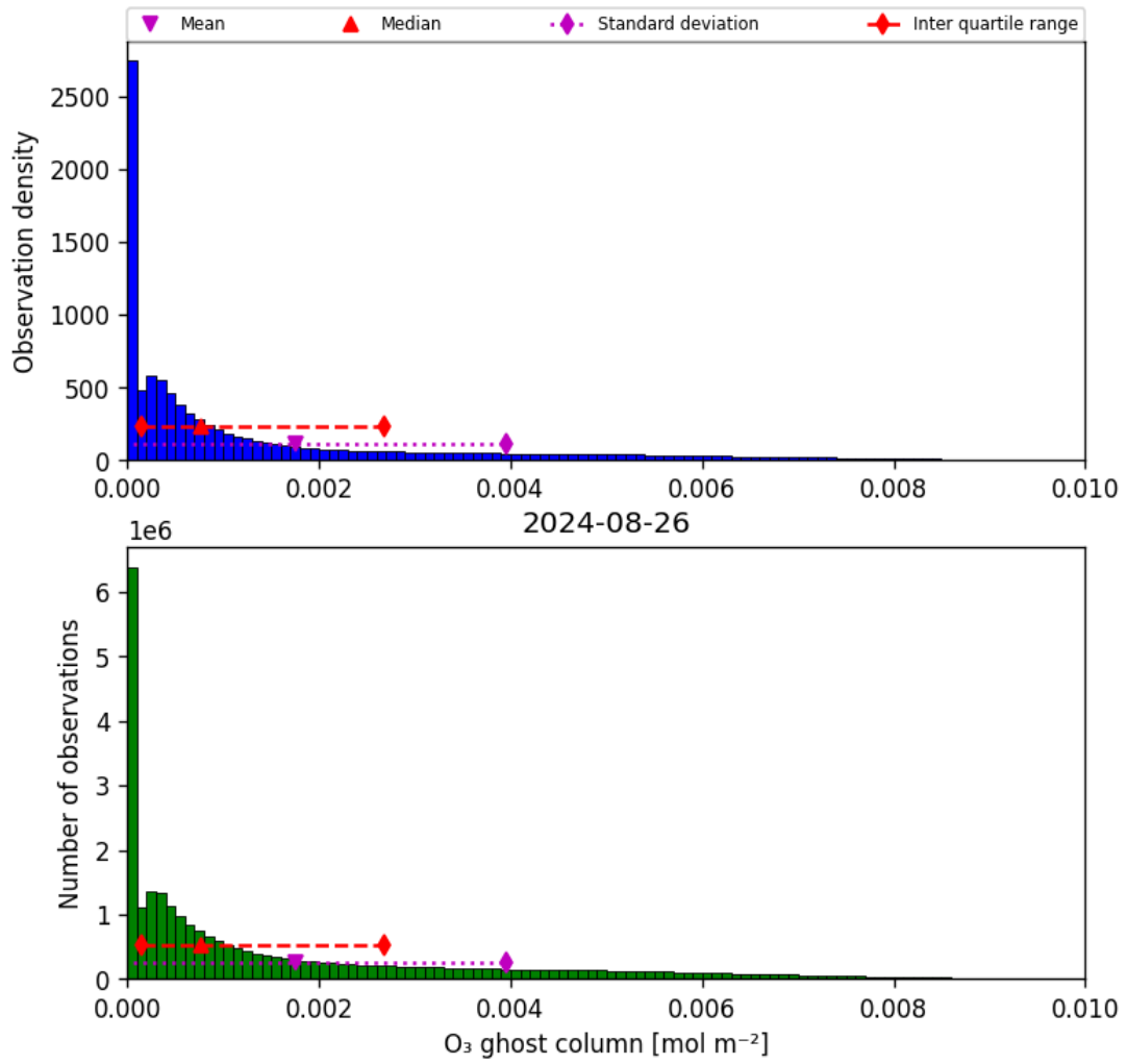
Figure 25: Histogram of “O 3 ghost column” for 2024-08-25 to 2024-08-27
