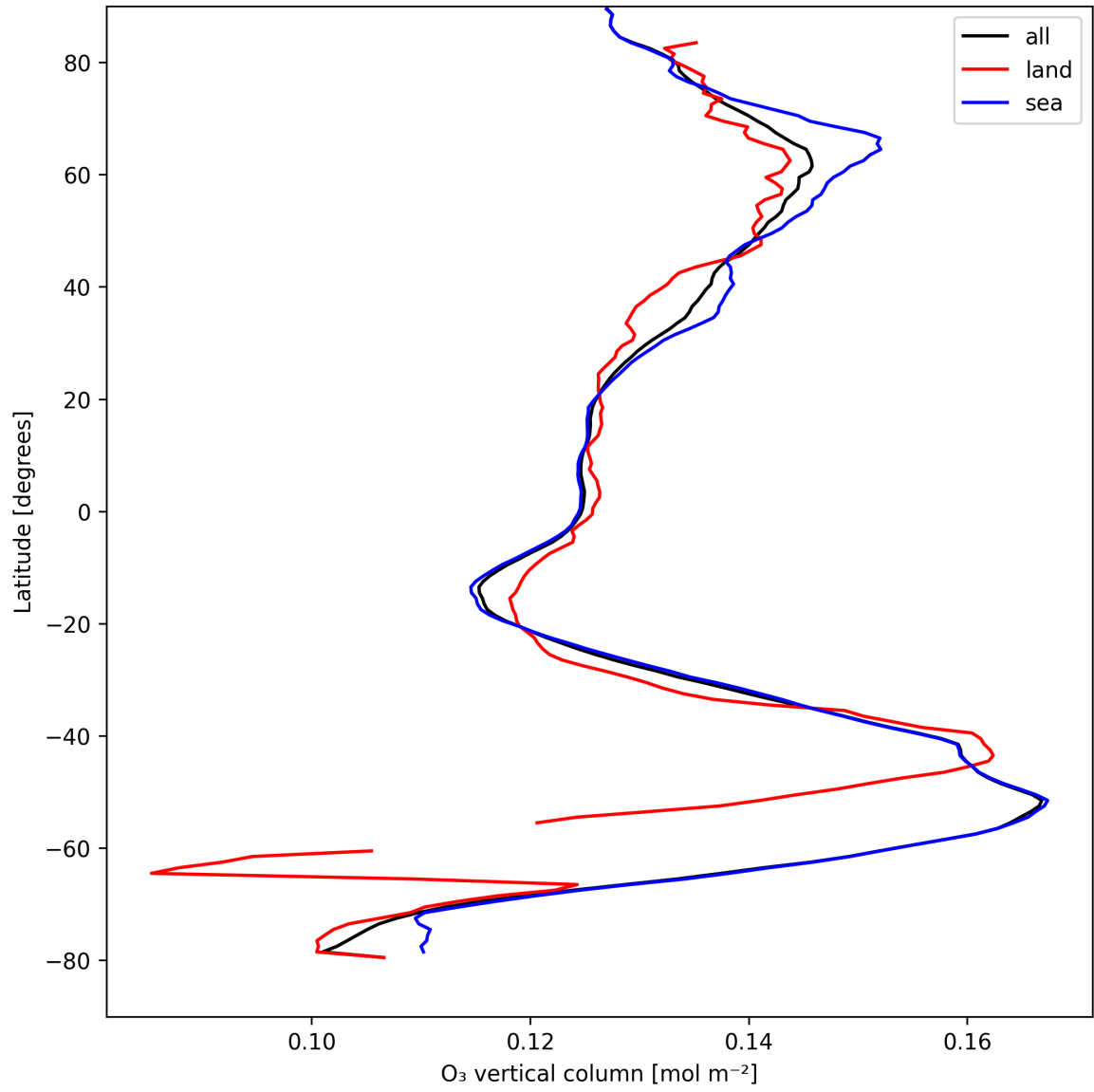
Figure 14: Zonal average of “O 3 vertical column” for 2024-08-25 to 2024-08-27.
