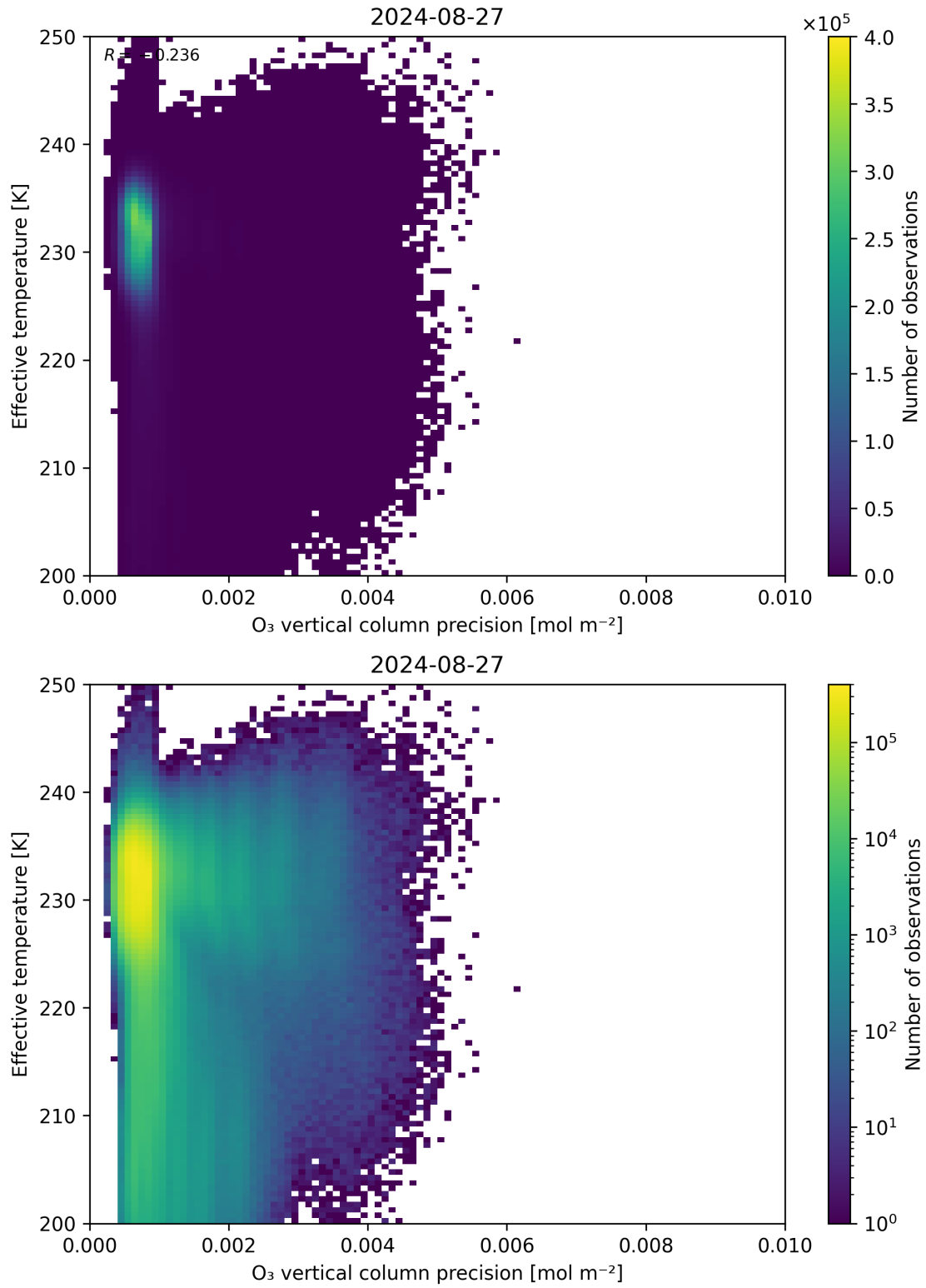
Figure 42: Scatter density plot of “O 3 vertical column precision” against “Effective temperature” for 2024-08-27 to 2024-08-28.
