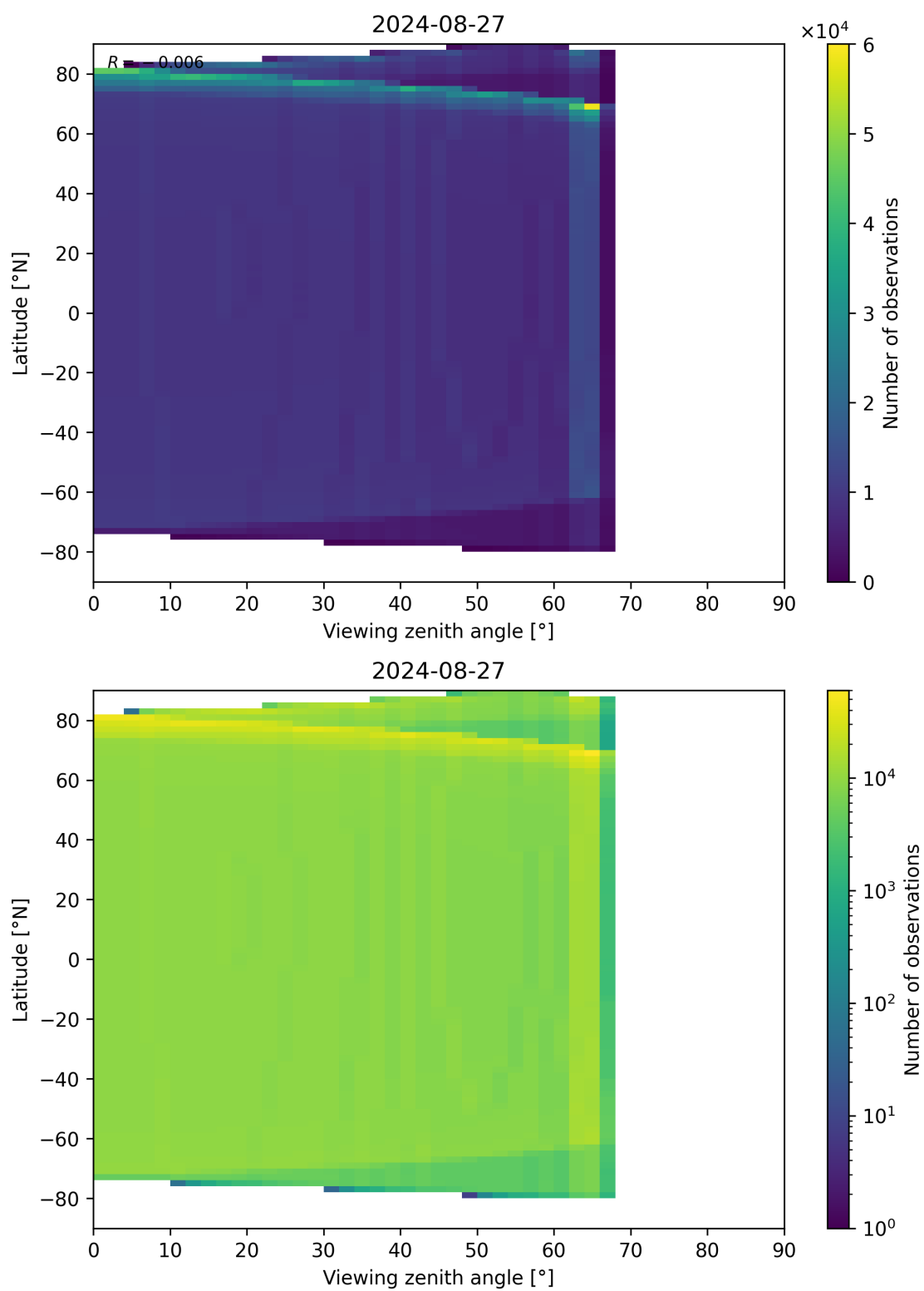
Figure 49: Scatter density plot of “Viewing zenith angle” against “Latitude” for 2024-08-27 to 2024-08-28.
