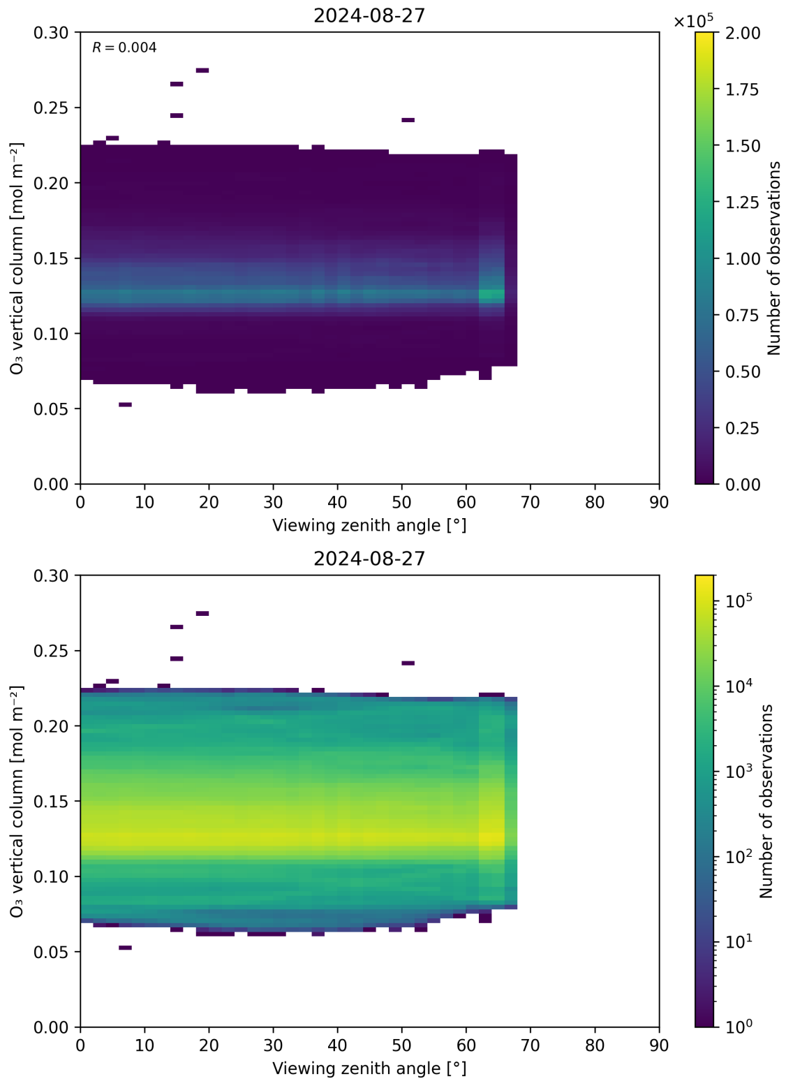
Figure 52: Scatter density plot of “Viewing zenith angle” against “O 3 vertical column” for 2024-08-27 to 2024-08-28.
