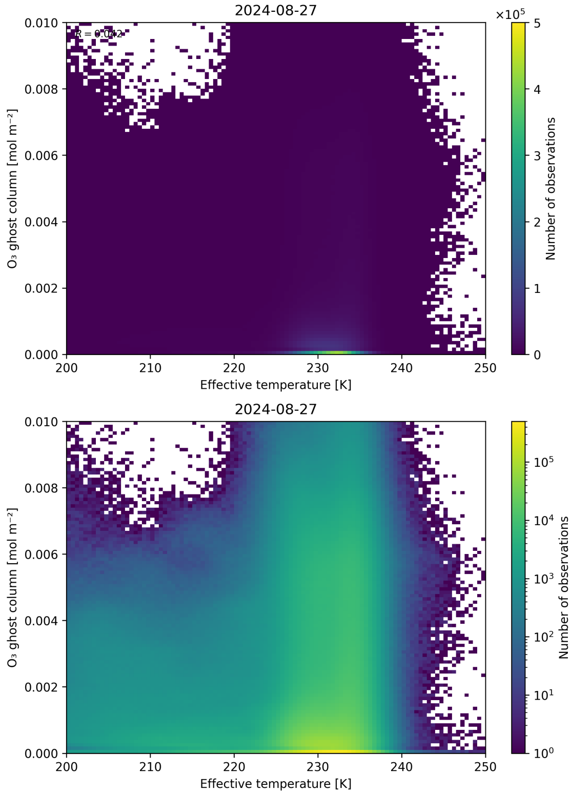
Figure 38: Scatter density plot of “Effective temperature” against “O 3 ghost column” for 2024-08-27 to 2024-08-28.
