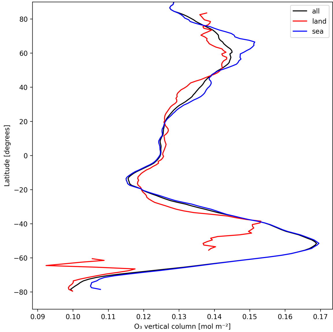
Figure 14: Zonal average of “O 3 vertical column” for 2024-08-27 to 2024-08-28.
