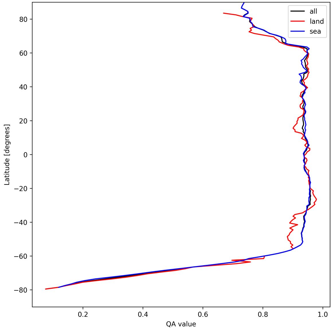
Figure 13: Zonal average of “QA value” for 2024-08-27 to 2024-08-28.
