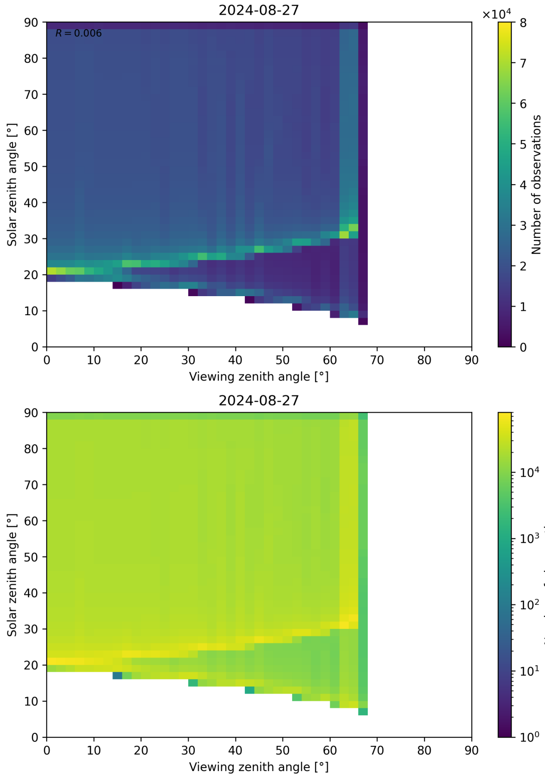
Figure 54: Scatter density plot of “Viewing zenith angle” against “Solar zenith angle” for 2024-08-27 to 2024-08-28.
