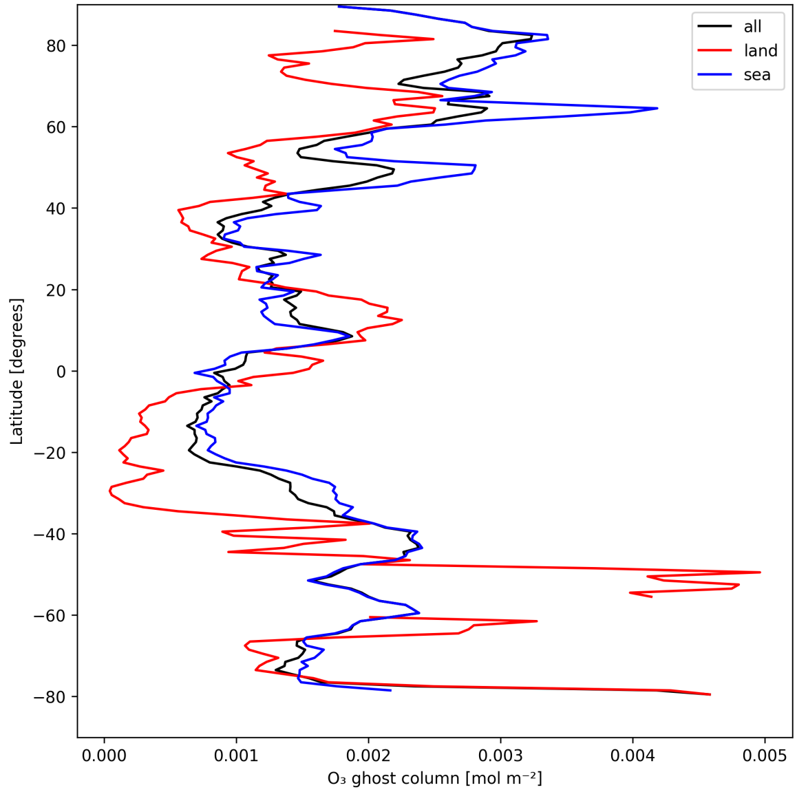
Figure 18: Zonal average of "O 3 ghost column" for 2024-08-27 to 2024-08-28.
