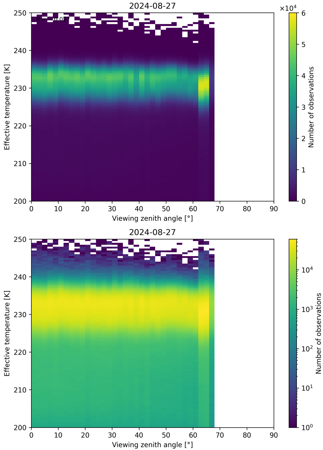
Figure 50: Scatter density plot of “Viewing zenith angle” against “Effective temperature” for 2024-08-27 to 2024-08-28.
