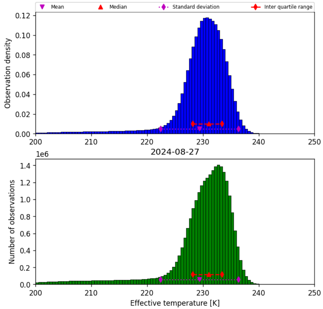
Figure 24: Histogram of “Effective temperature” for 2024-08-27 to 2024-08-28
