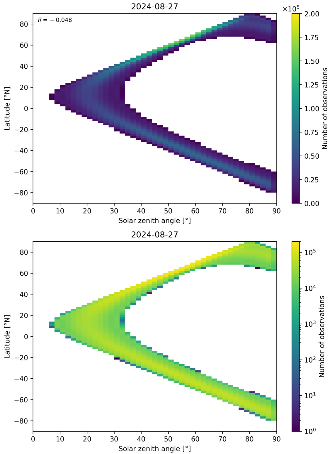
Figure 44: Scatter density plot of “Solar zenith angle” against “Latitude” for 2024-08-27 to 2024-08-28.
