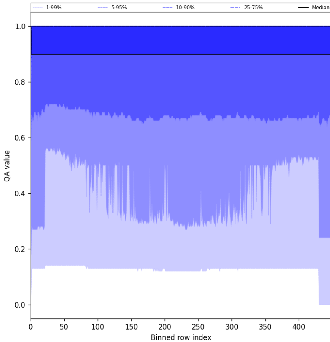
Figure 27: Along track statistics of “QA value” for 2024-08-27 to 2024-08-28
