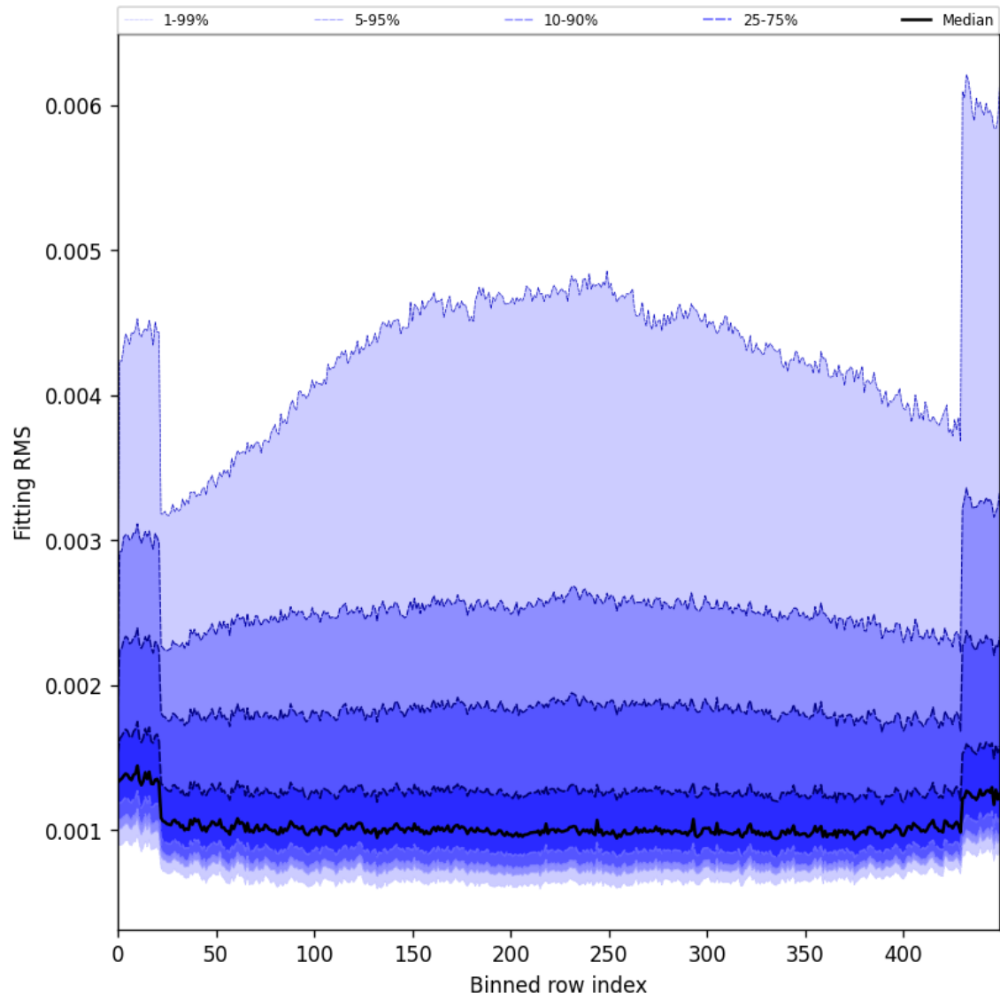
Figure 30: Along track statistics of “Fitting RMS” for 2024-08-27 to 2024-08-28
