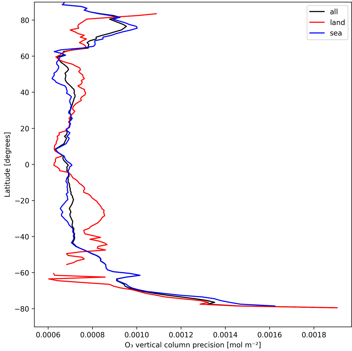
Figure 15: Zonal average of "O 3 vertical column precision" for 2024-08-27 to 2024-08-28.
