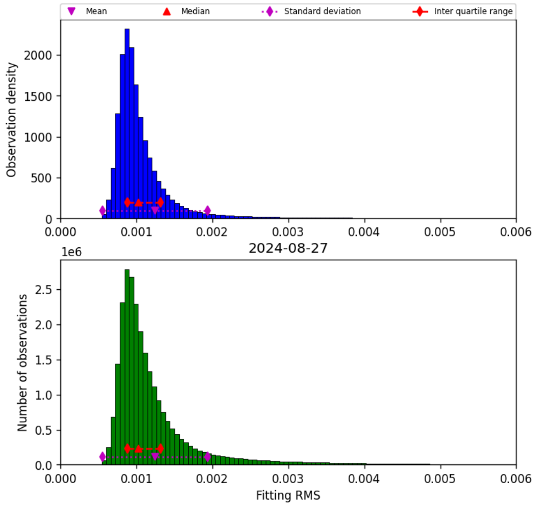
Figure 23: Histogram of “Fitting RMS” for 2024-08-27 to 2024-08-28
