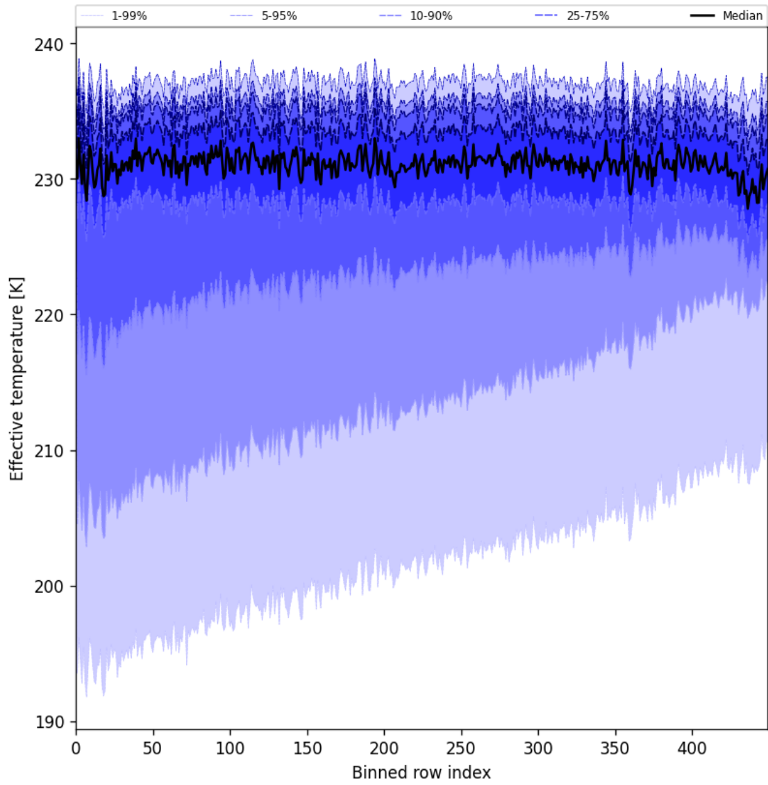
Figure 31: Along track statistics of “Effective temperature” for 2024-08-27 to 2024-08-28
