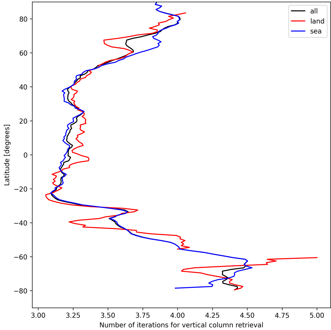
Figure 19: Zonal average of “Number of iterations for vertical column retrieval” for 2024-08-27 to 2024-08-28.
