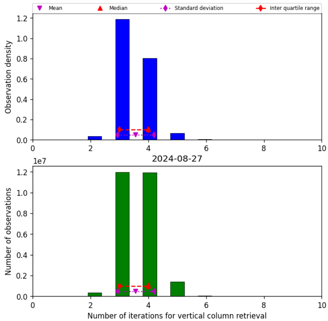
Figure 26: Histogram of “Number of iterations for vertical column retrieval” for 2024-08-27 to 2024-08-28
