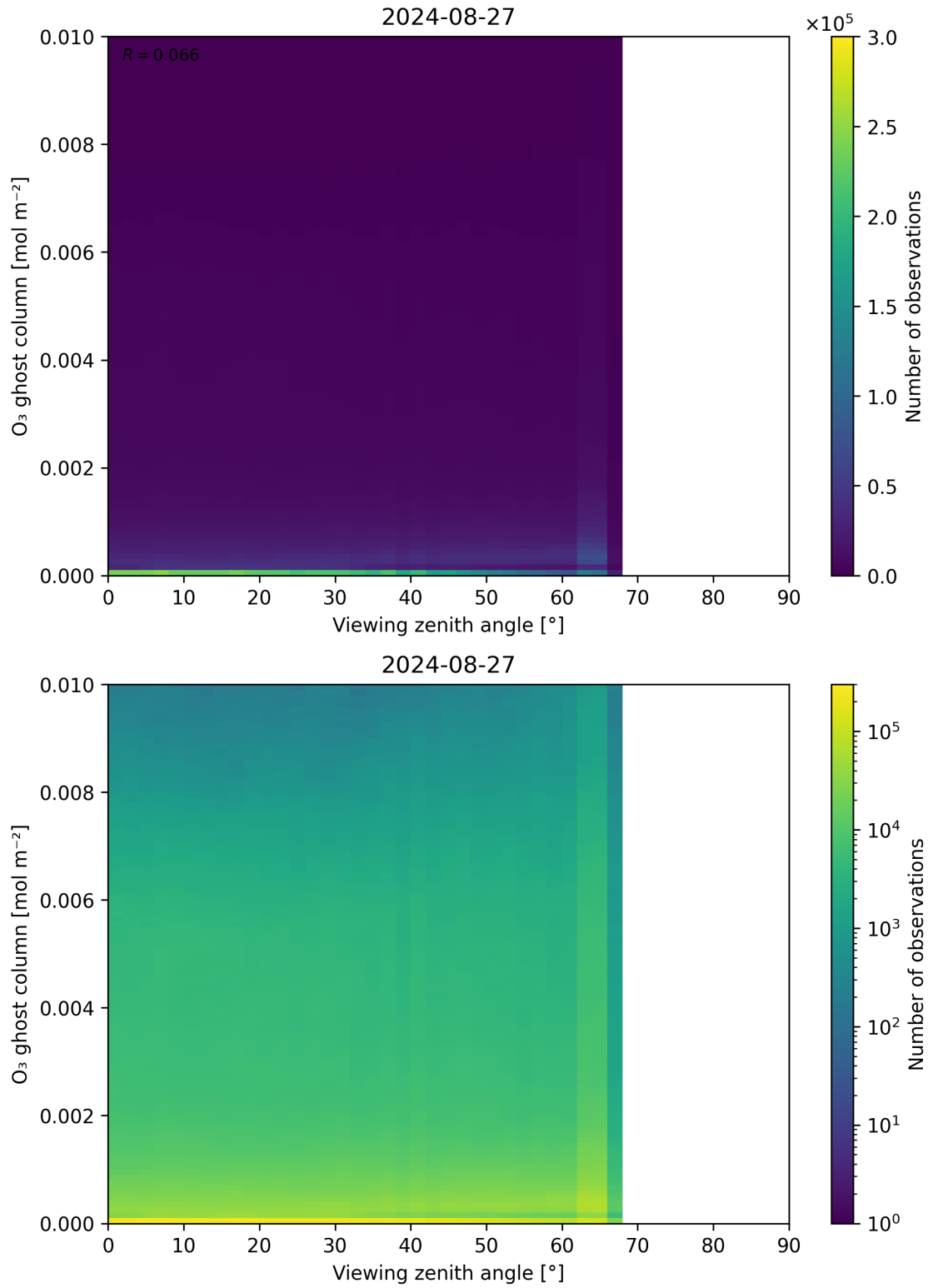
Figure 51: Scatter density plot of “Viewing zenith angle” against “O 3 ghost column” for 2024-08-27 to 2024-08-28.
