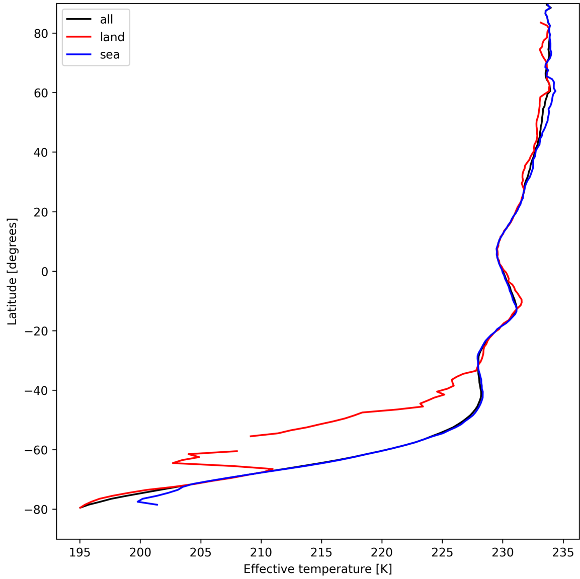
Figure 17: Zonal average of "Effective temperature" for 2024-08-27 to 2024-08-28.
