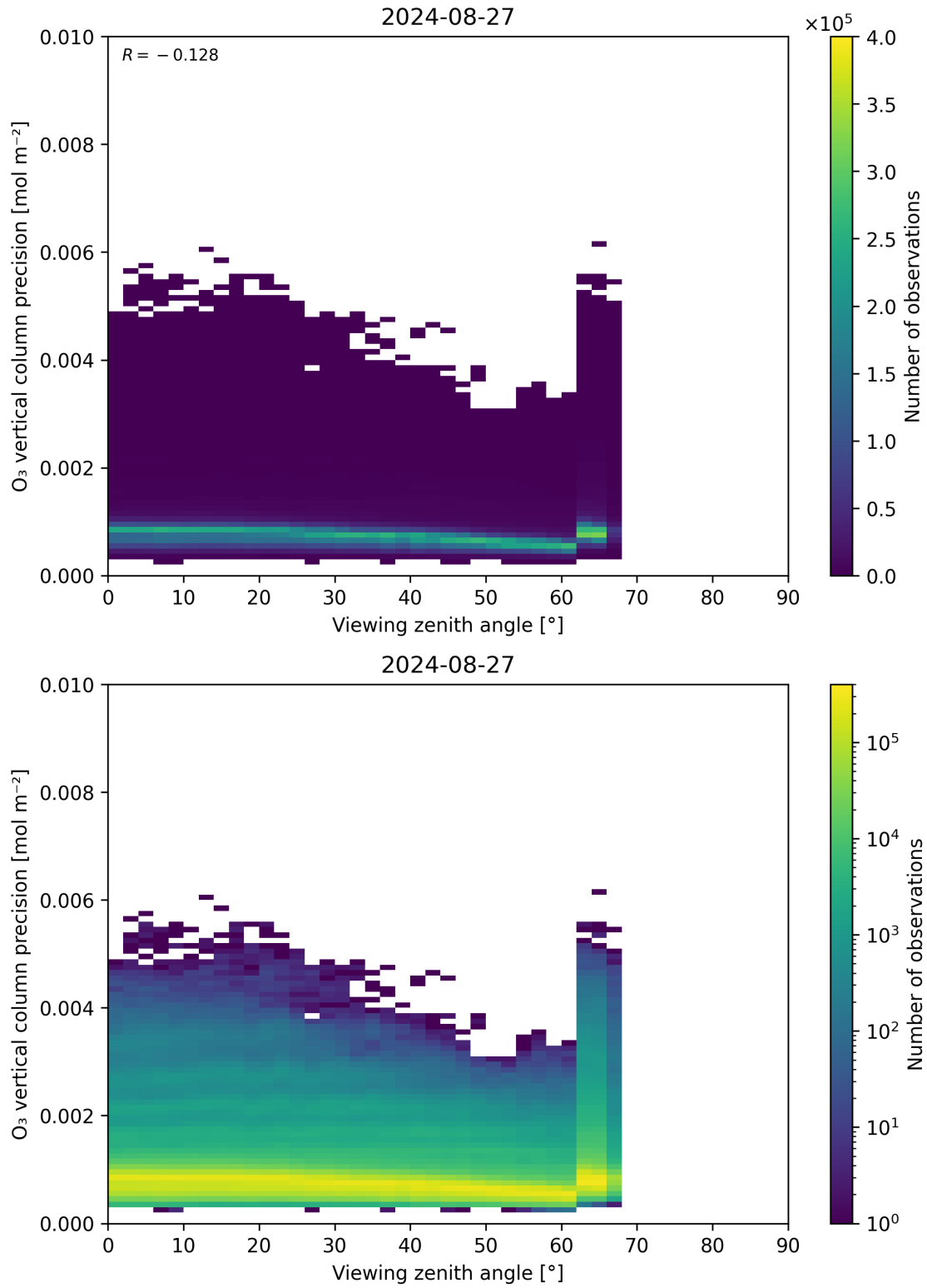
Figure 53: Scatter density plot of “Viewing zenith angle” against “O 3 vertical column precision” for 2024-08-27 to 2024-08-28.
