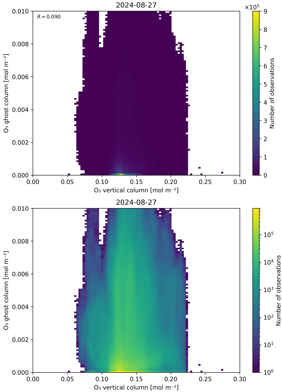
Figure 40: Scatter density plot of “O 3 vertical column” against “O 3 ghost column” for 2024-08-27 to 2024-08-28.
