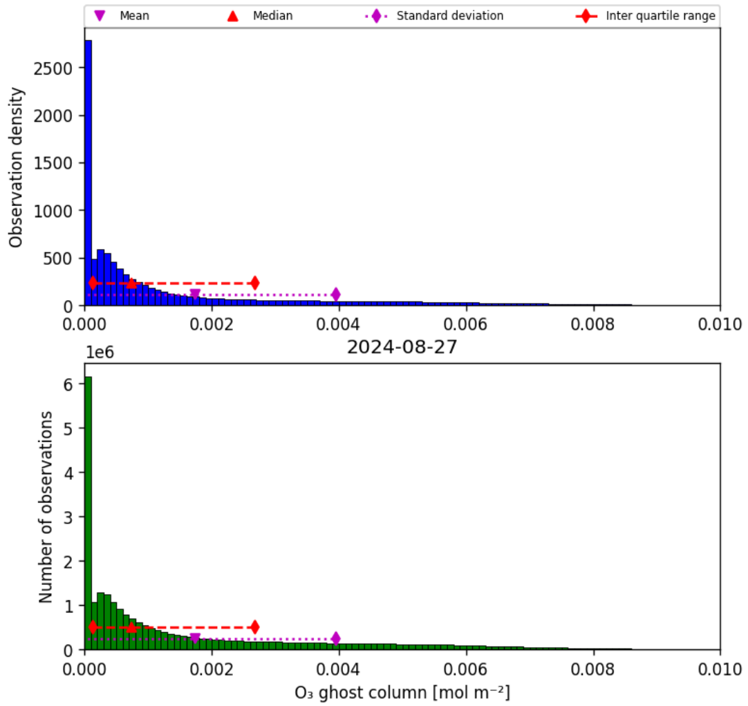
Figure 25: Histogram of “O 3 ghost column” for 2024-08-27 to 2024-08-28
