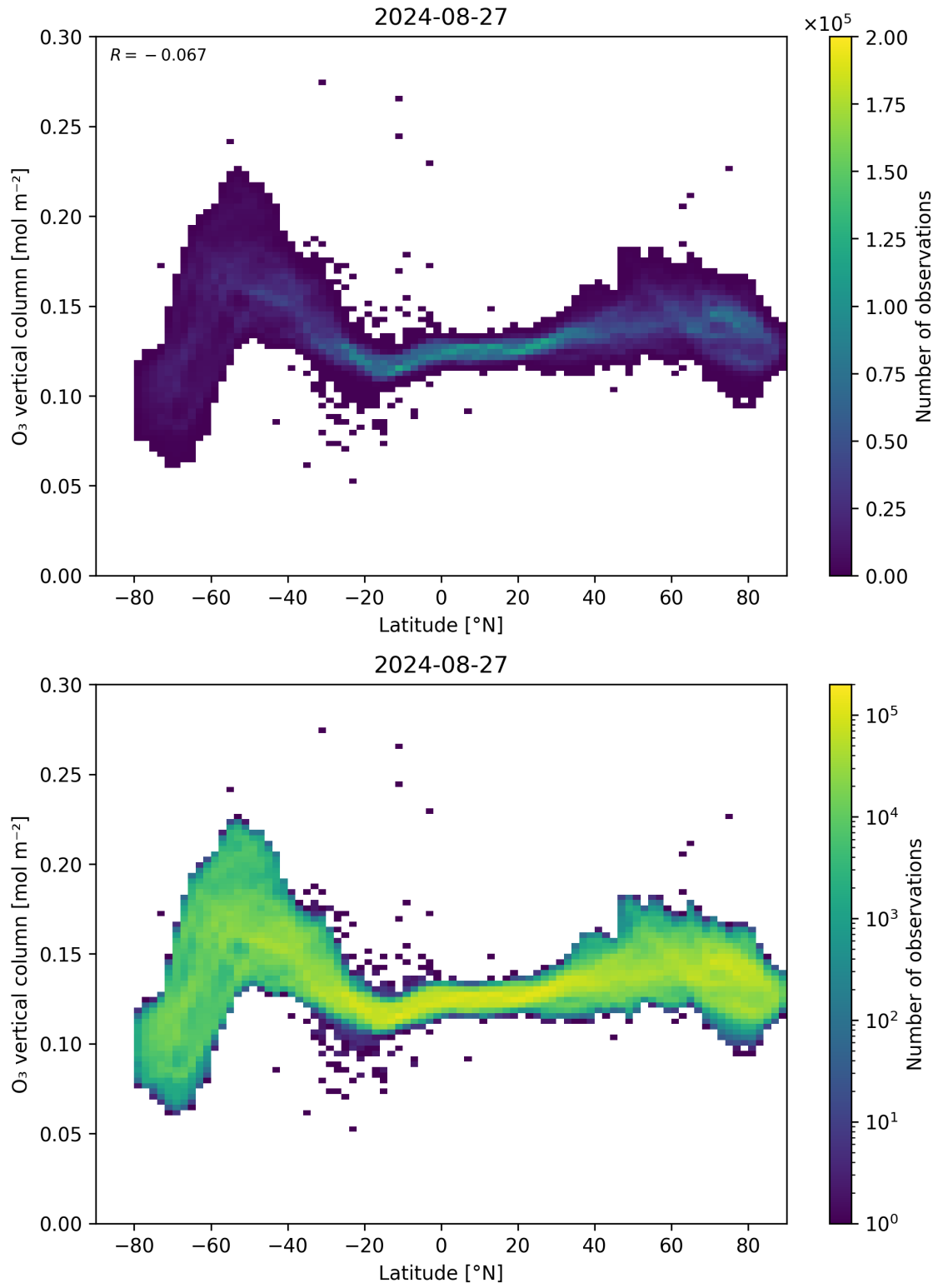
Figure 36: Scatter density plot of “Latitude” against “O 3 vertical column” for 2024-08-27 to 2024-08-28.
