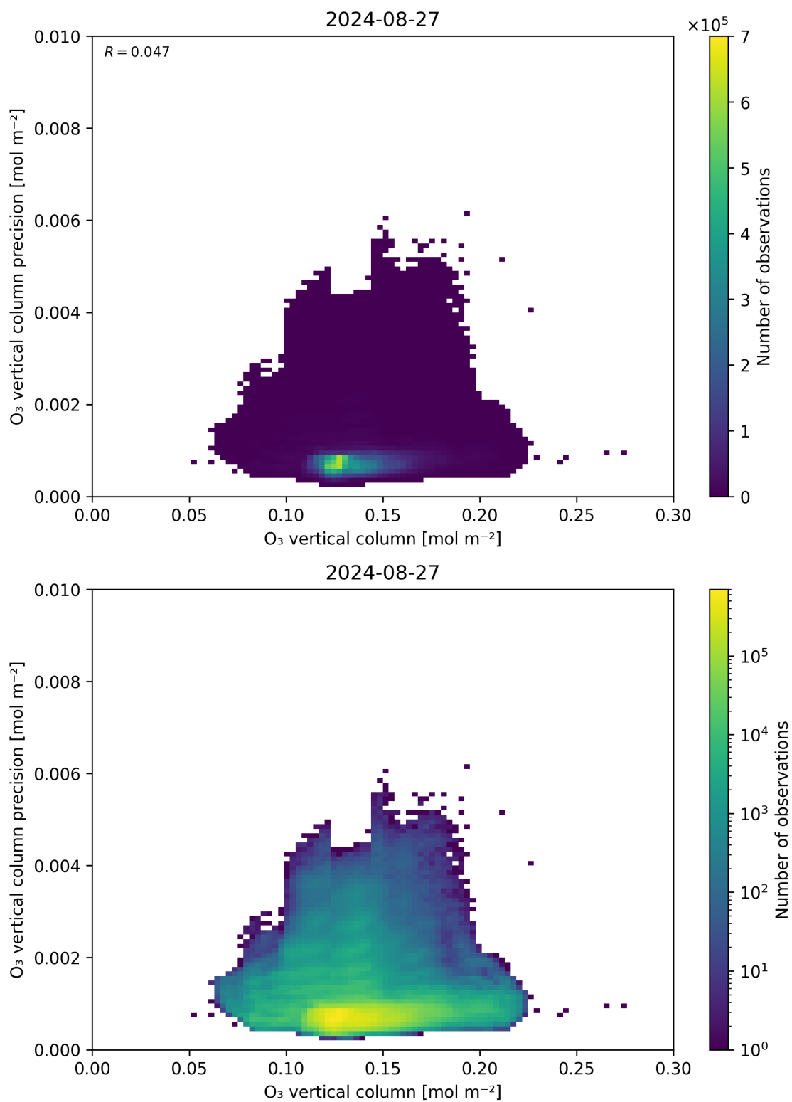
Figure 41: Scatter density plot of “O 3 vertical column” against “O 3 vertical column precision” for 2024-08-27 to 2024-08-28.
