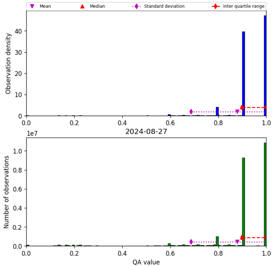
Figure 20: Histogram of “QA value” for 2024-08-27 to 2024-08-28
