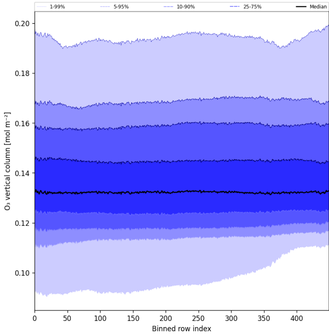
Figure 28: Along track statistics of “O 3 vertical column” for 2024-08-27 to 2024-08-28
