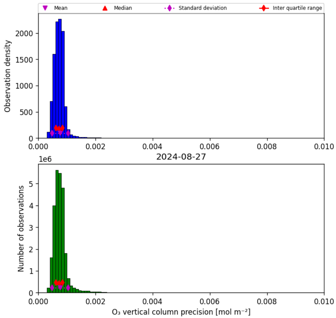
Figure 22: Histogram of “O 3 vertical column precision” for 2024-08-27 to 2024-08-28
