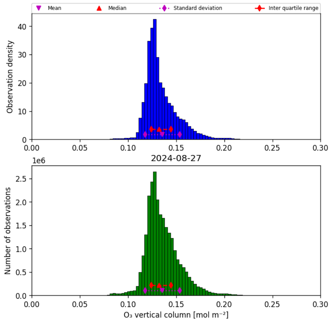
Figure 21: Histogram of “O 3 vertical column” for 2024-08-27 to 2024-08-28
