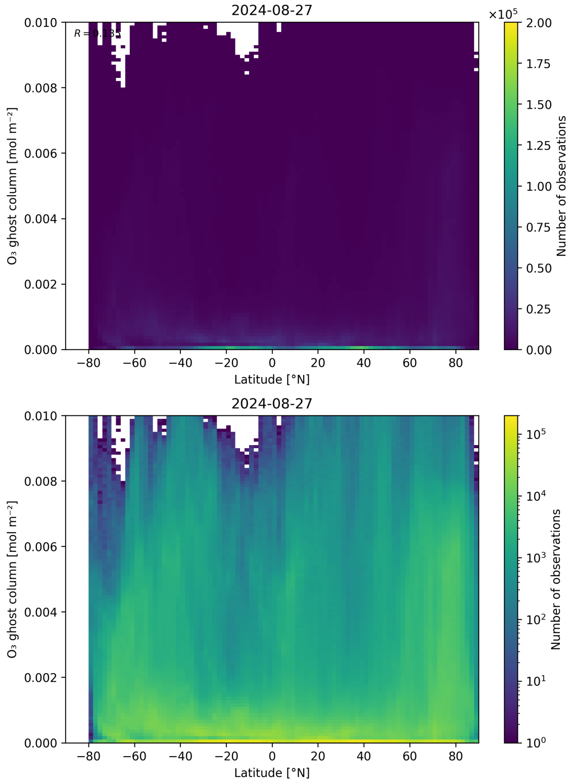
Figure 35: Scatter density plot of “Latitude” against “O 3 ghost column” for 2024-08-27 to 2024-08-28.
