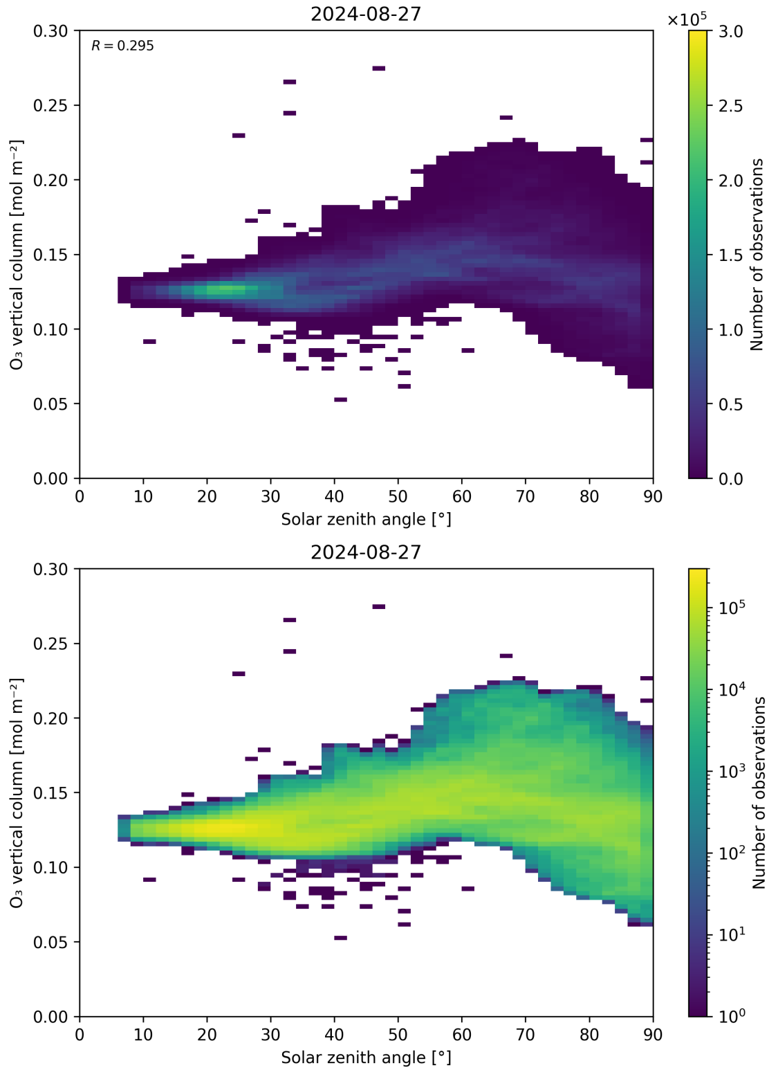
Figure 47: Scatter density plot of “Solar zenith angle” against “O 3 vertical column” for 2024-08-27 to 2024-08-28.
