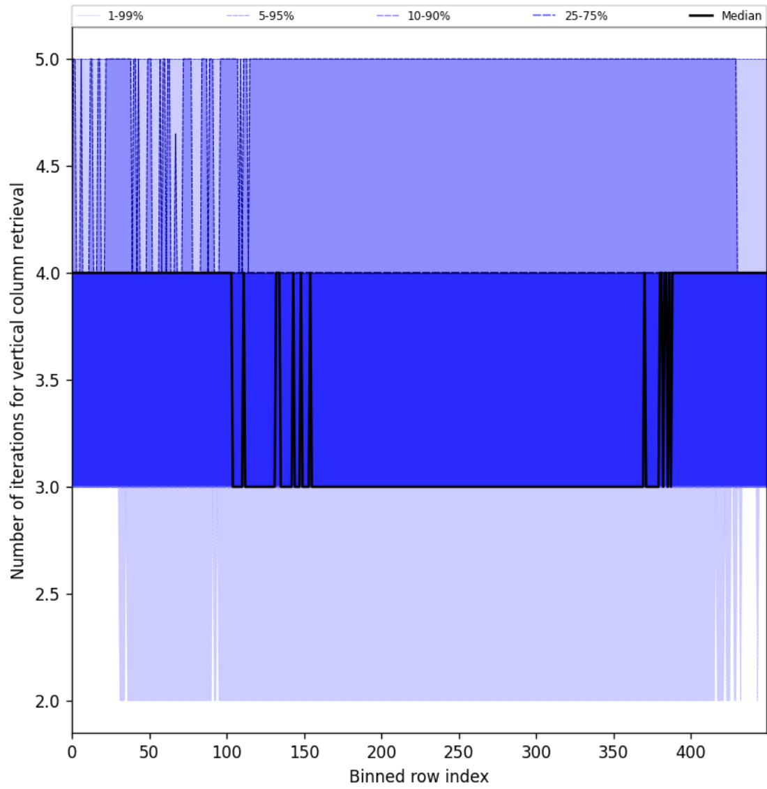
Figure 33: Along track statistics of “Number of iterations for vertical column retrieval” for 2024-08-27 to 2024-08-28
