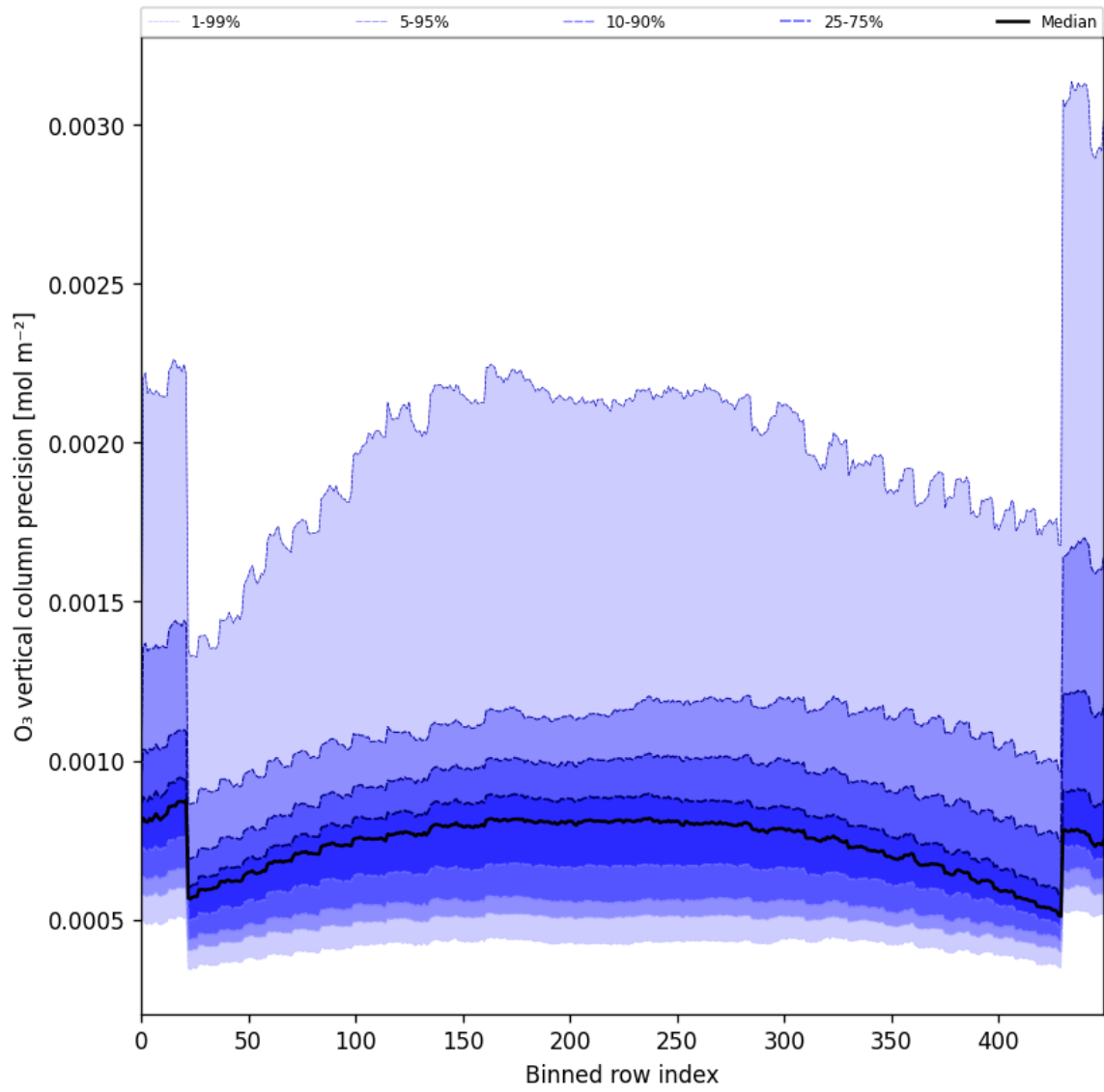
Figure 29: Along track statistics of “O 3 vertical column precision” for 2024-08-27 to 2024-08-28
