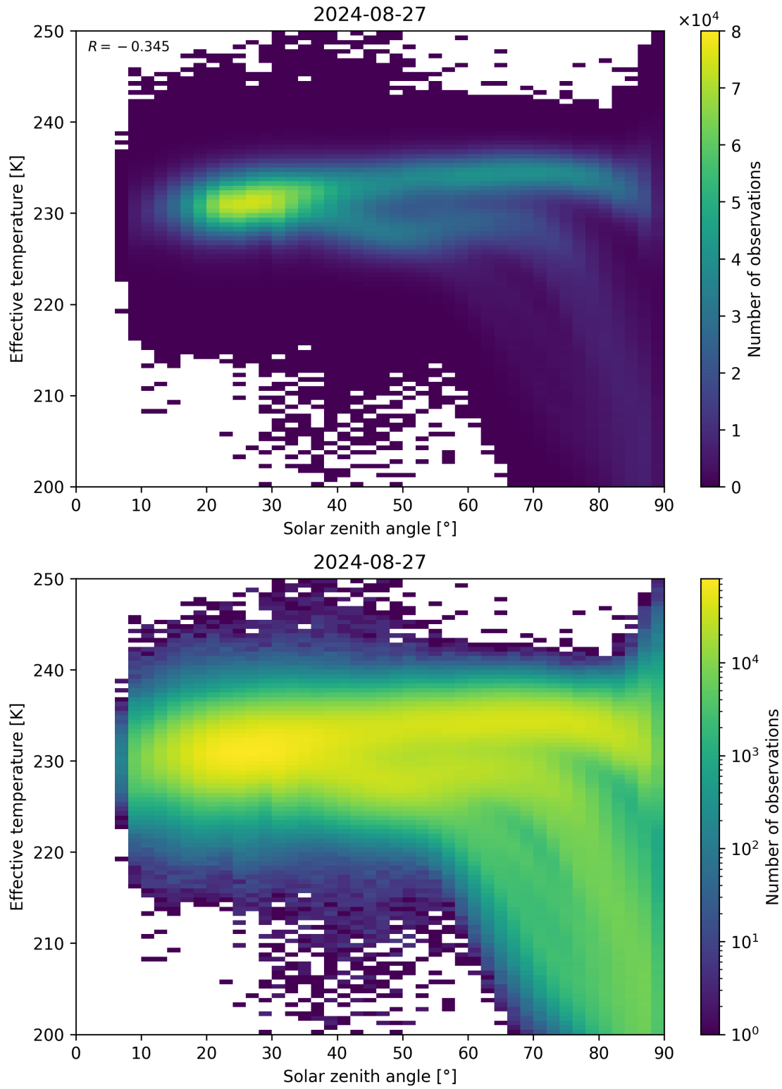
Figure 45: Scatter density plot of “Solar zenith angle” against “Effective temperature” for 2024-08-27 to 2024-08-28.
