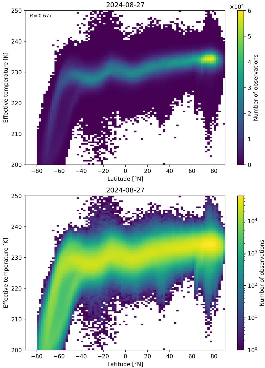
Figure 34: Scatter density plot of “Latitude” against “Effective temperature” for 2024-08-27 to 2024-08-28.
