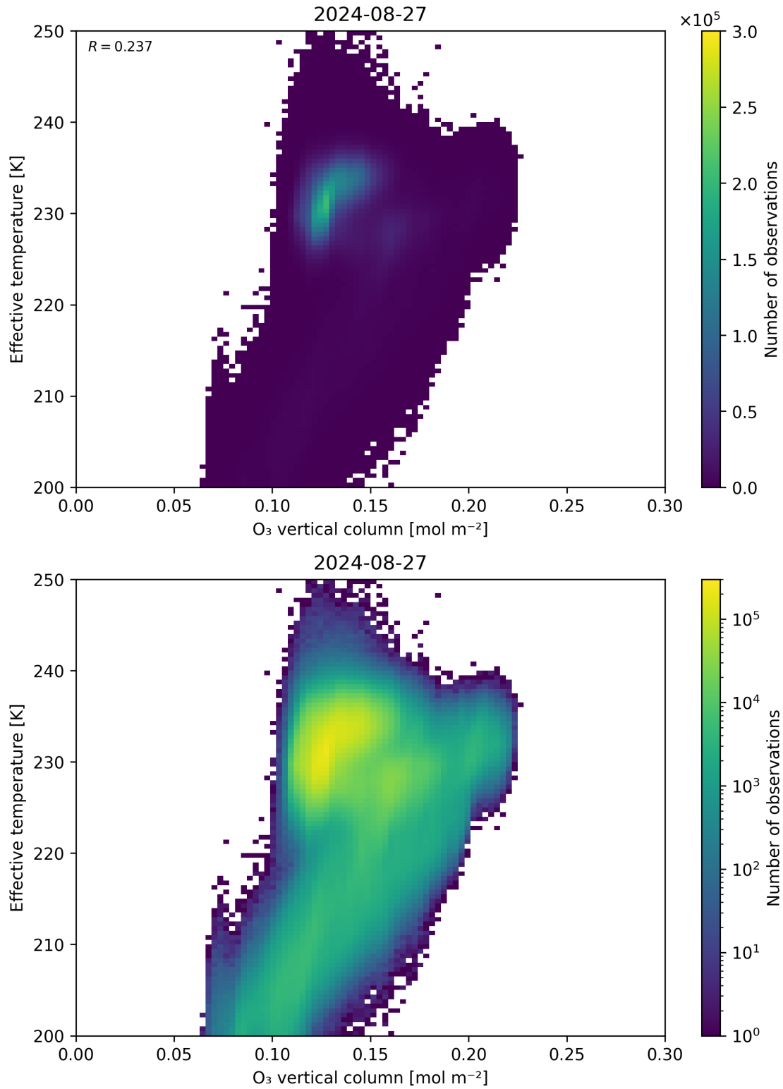
Figure 39: Scatter density plot of “O 3 vertical column” against “Effective temperature” for 2024-08-27 to 2024-08-28.
