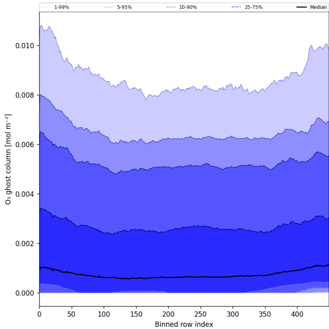
Figure 32: Along track statistics of “O 3 ghost column” for 2024-08-27 to 2024-08-28
