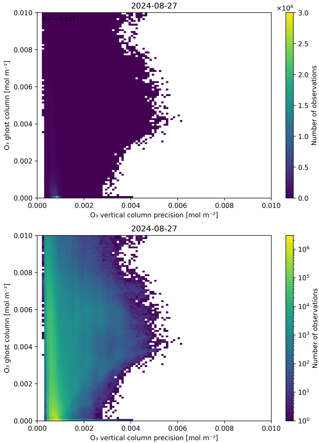
Figure 43: Scatter density plot of “ O_3 vertical column precision” against “ O_3 ghost column” for 2024-08-27 to 2024-08-28.
