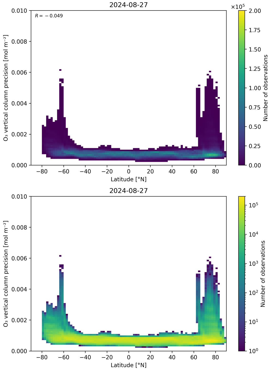
Figure 37: Scatter density plot of “Latitude” against “O 3 vertical column precision” for 2024-08-27 to 2024-08-28.
