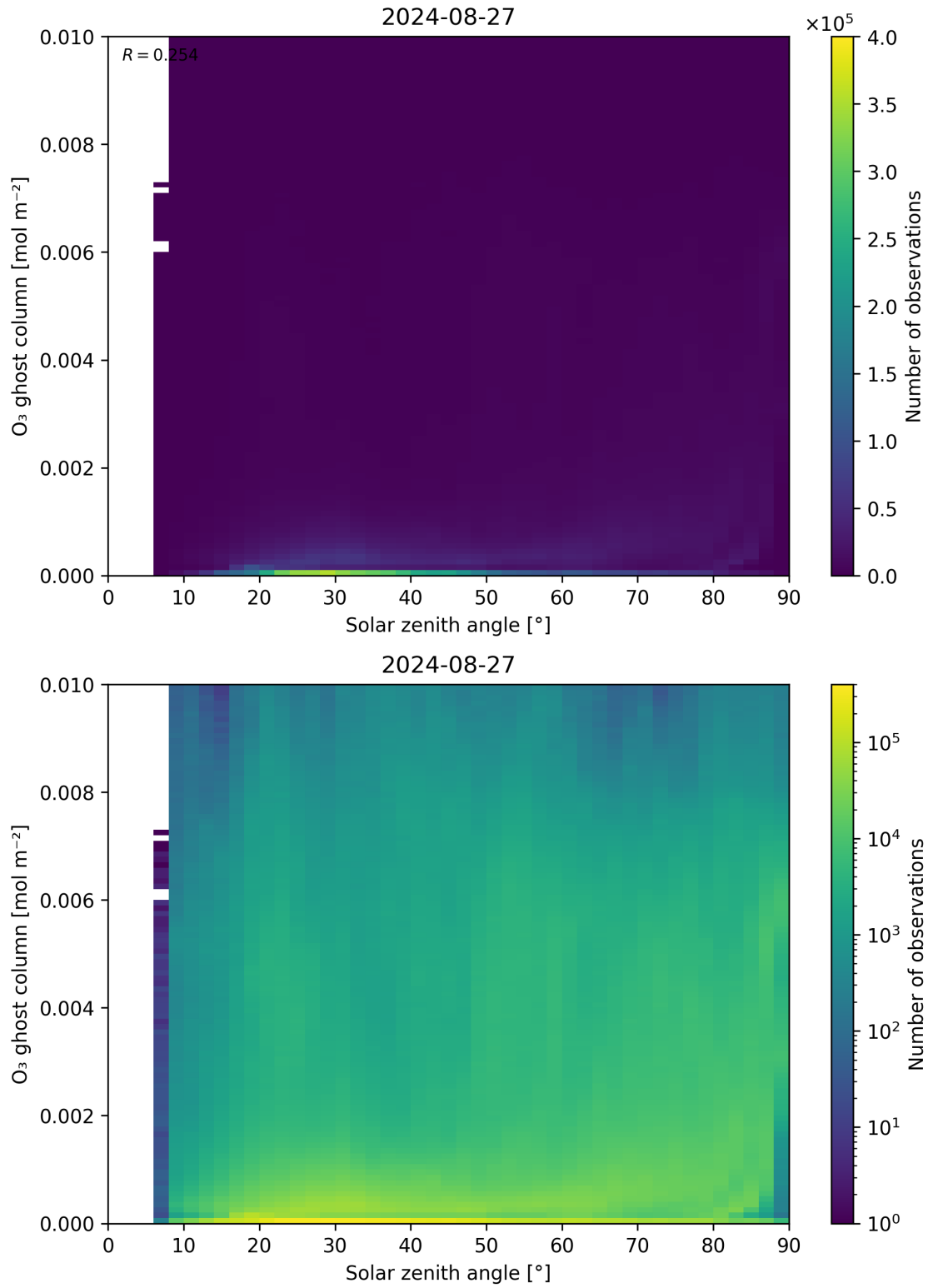
Figure 46: Scatter density plot of “Solar zenith angle” against “O 3 ghost column” for 2024-08-27 to 2024-08-28.
