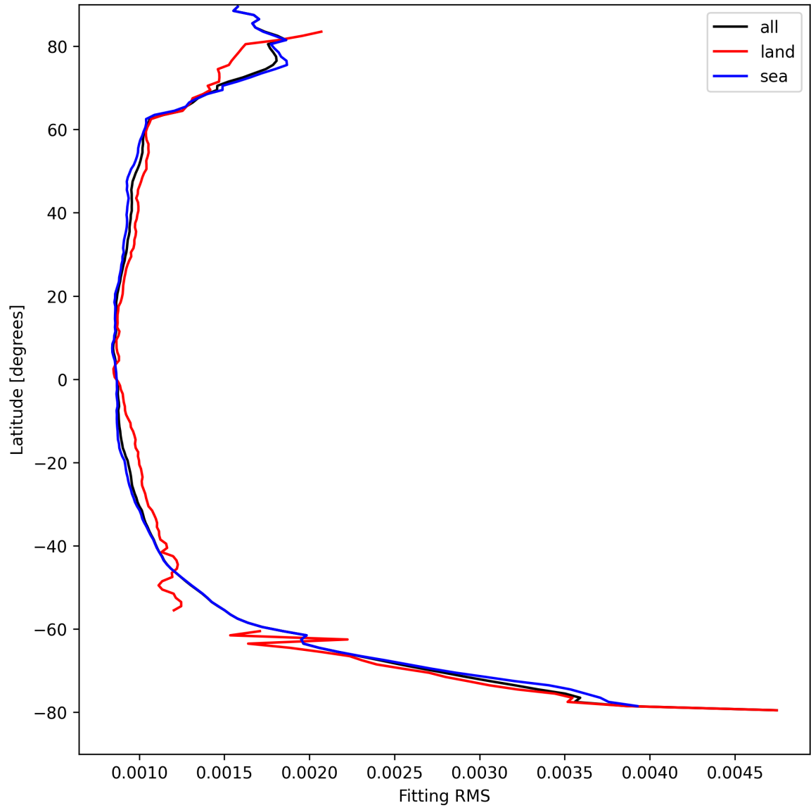
Figure 16: Zonal average of “Fitting RMS” for 2024-08-27 to 2024-08-28.
