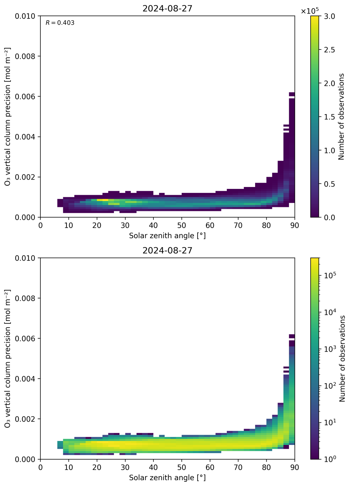
Figure 48: Scatter density plot of “Solar zenith angle” against “O 3 vertical column precision” for 2024-08-27 to 2024-08-28.
