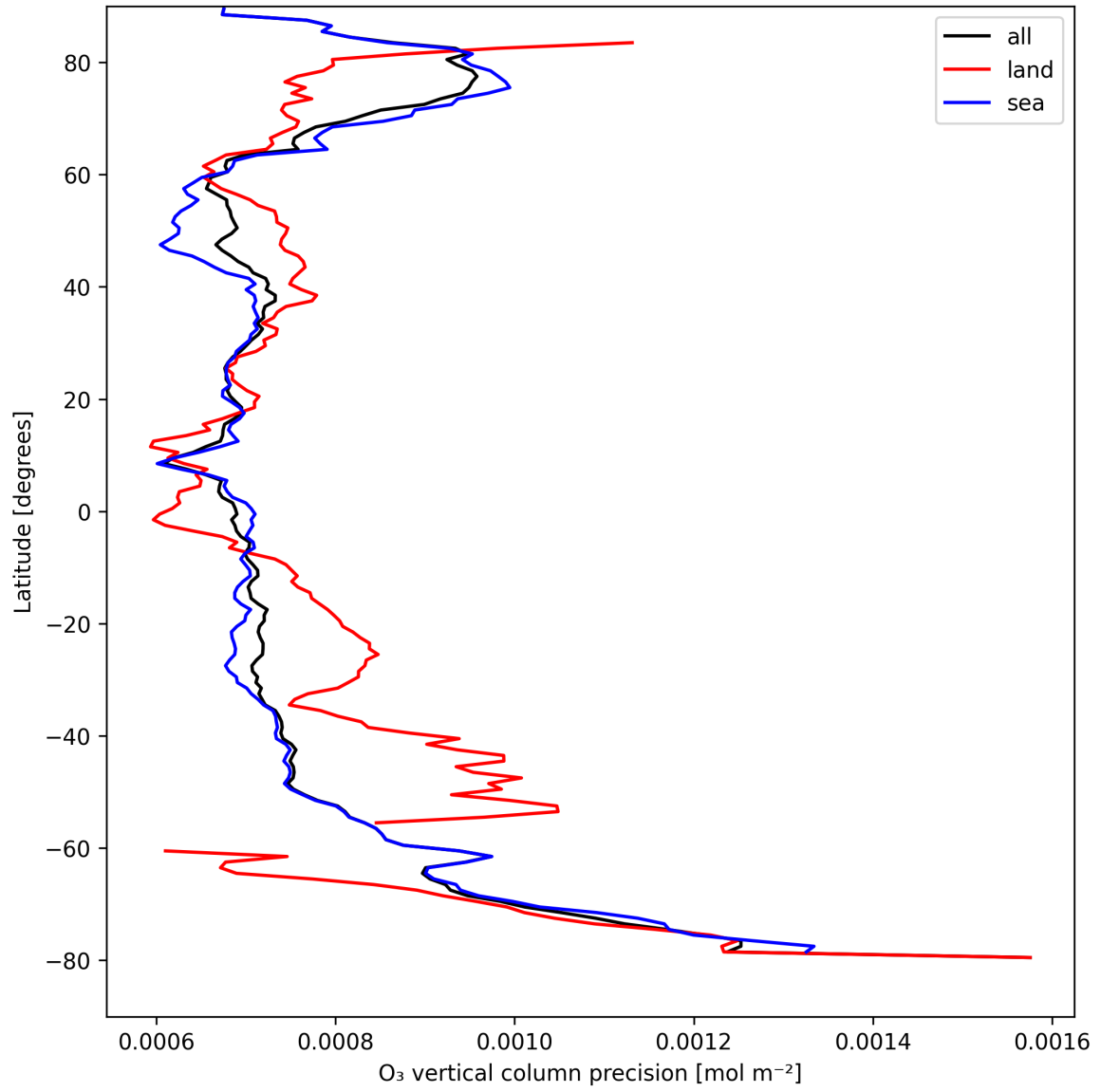
Figure 15: Zonal average of “O 3 vertical column precision” for 2024-08-27 to 2024-08-29.
