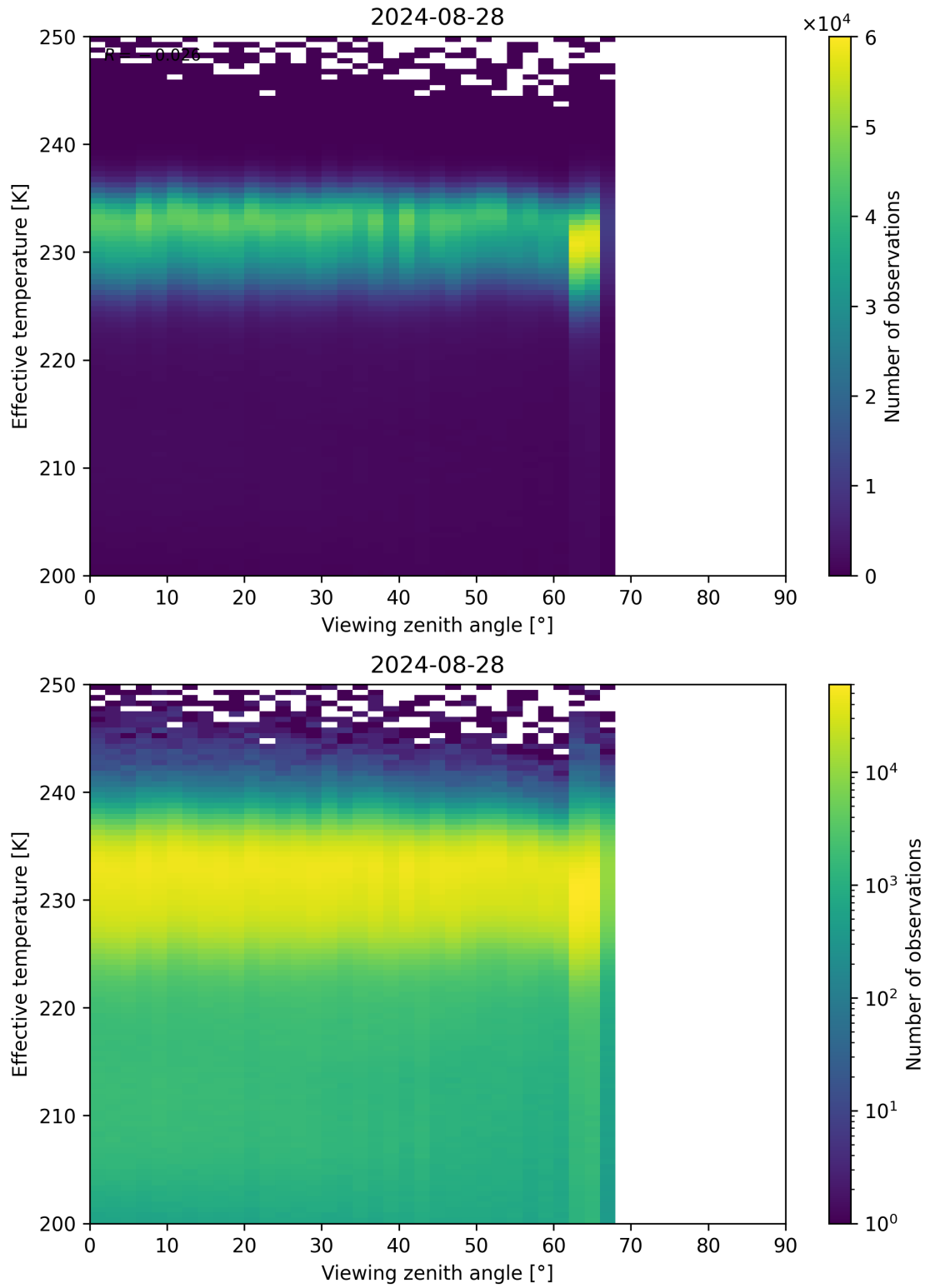
Figure 50: Scatter density plot of “Viewing zenith angle” against “Effective temperature” for 2024-08-27 to 2024-08-29.
