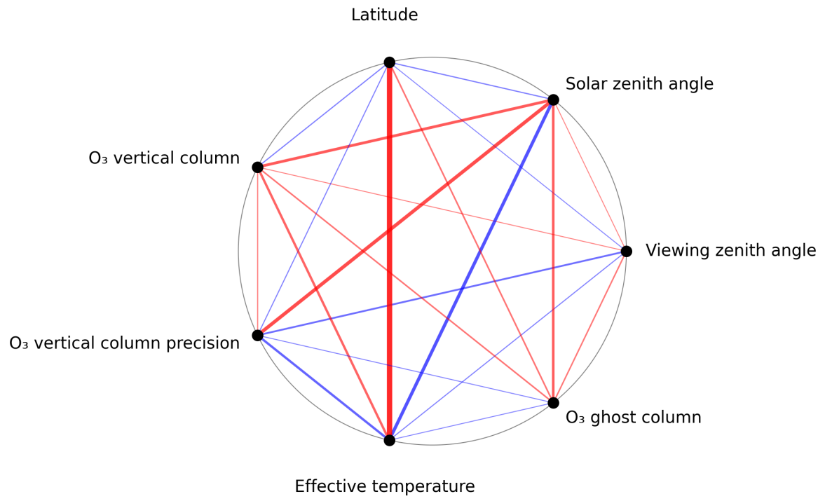
Figure 1: Map of correlation graph for 2024-08-27 to 2024-08-29.
