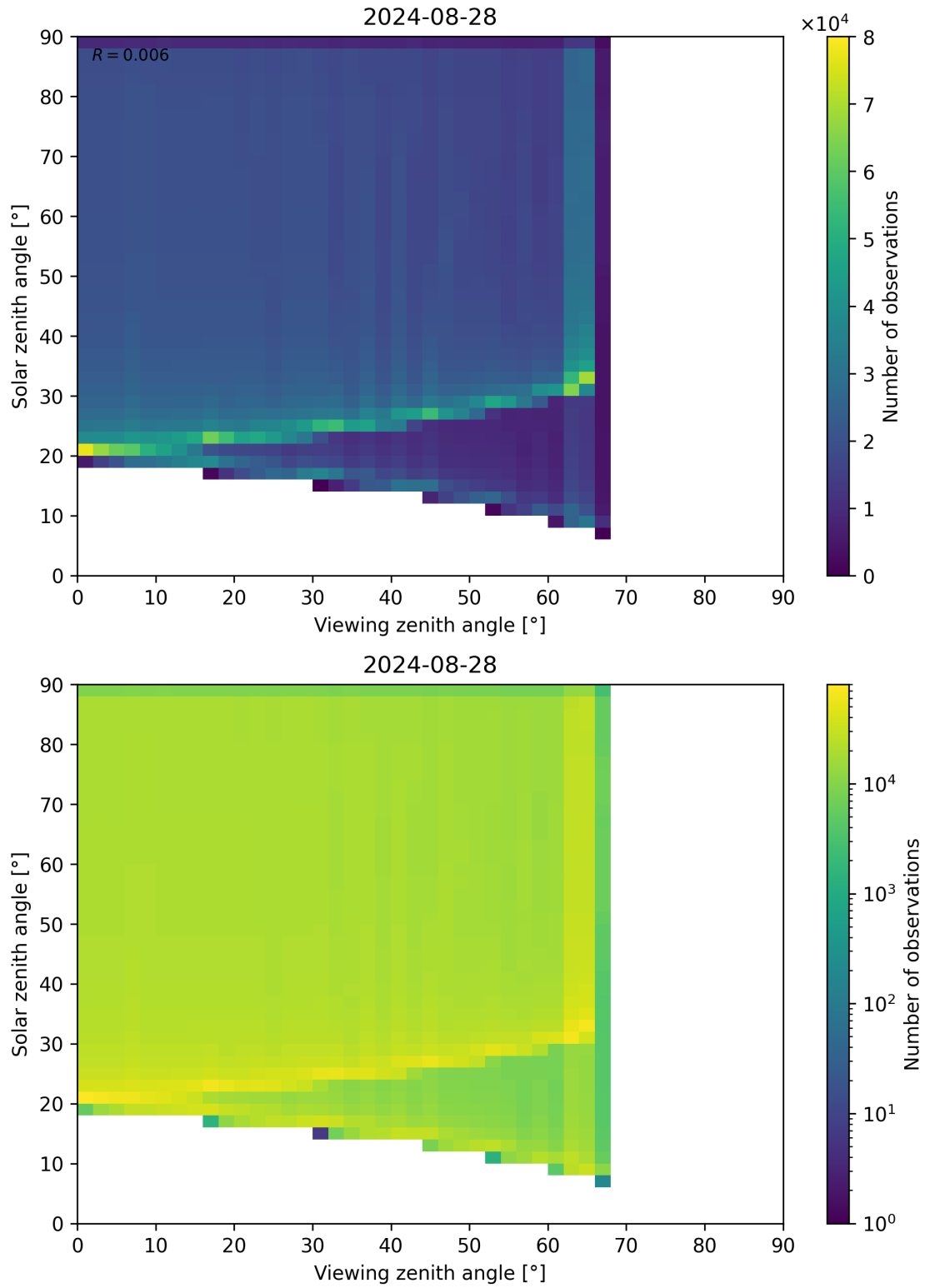
Figure 54: Scatter density plot of “Viewing zenith angle” against “Solar zenith angle” for 2024-08-27 to 2024-08-29.
