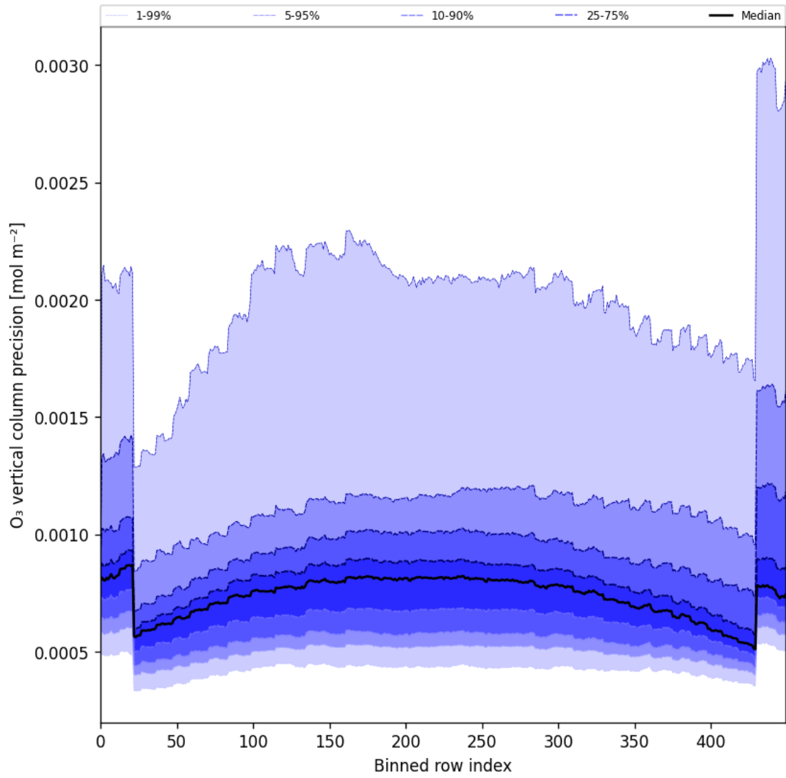
Figure 29: Along track statistics of “O 3 vertical column precision” for 2024-08-27 to 2024-08-29
