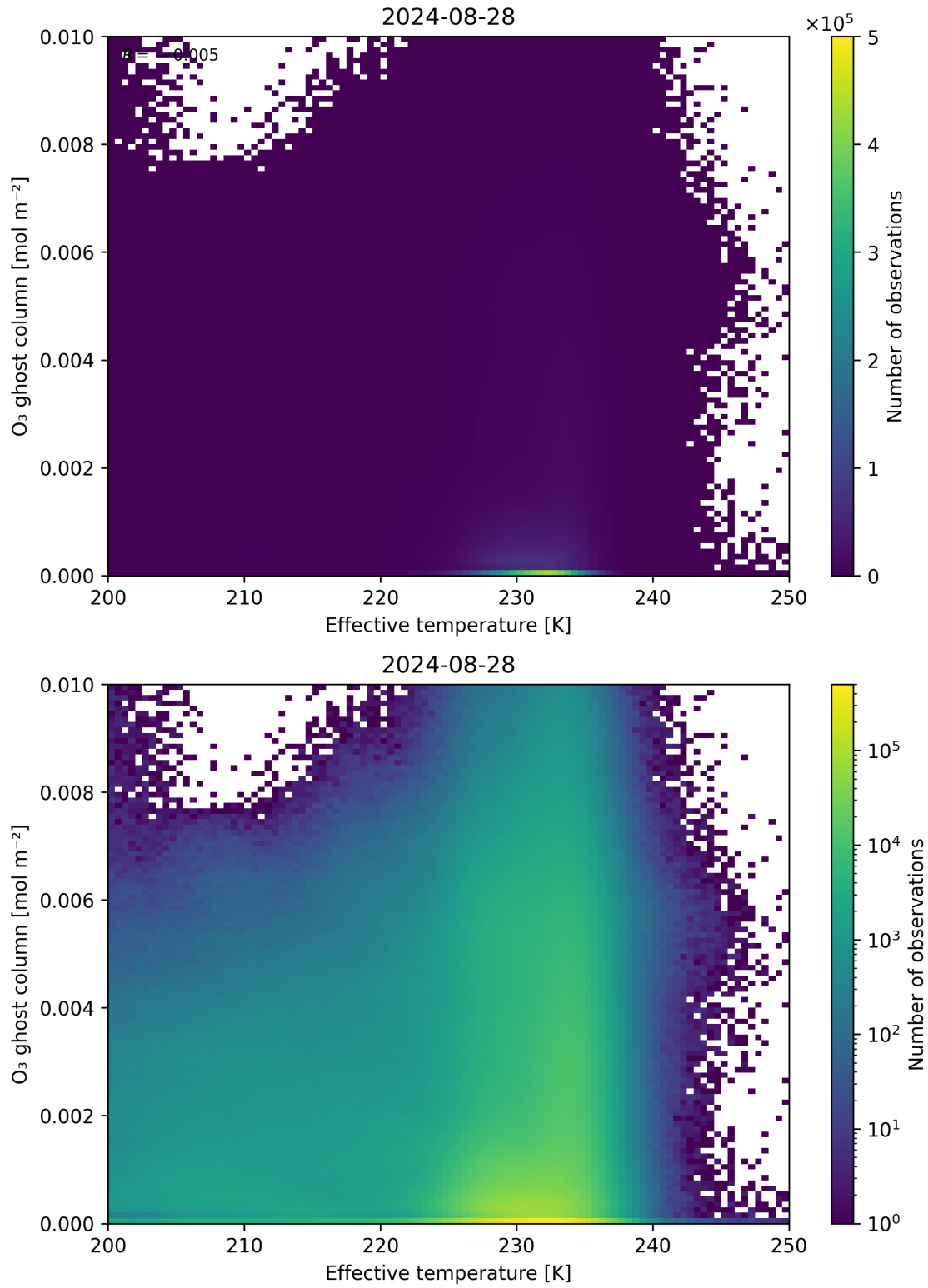
Figure 38: Scatter density plot of “Effective temperature” against “O 3 ghost column” for 2024-08-27 to 2024-08-29.
