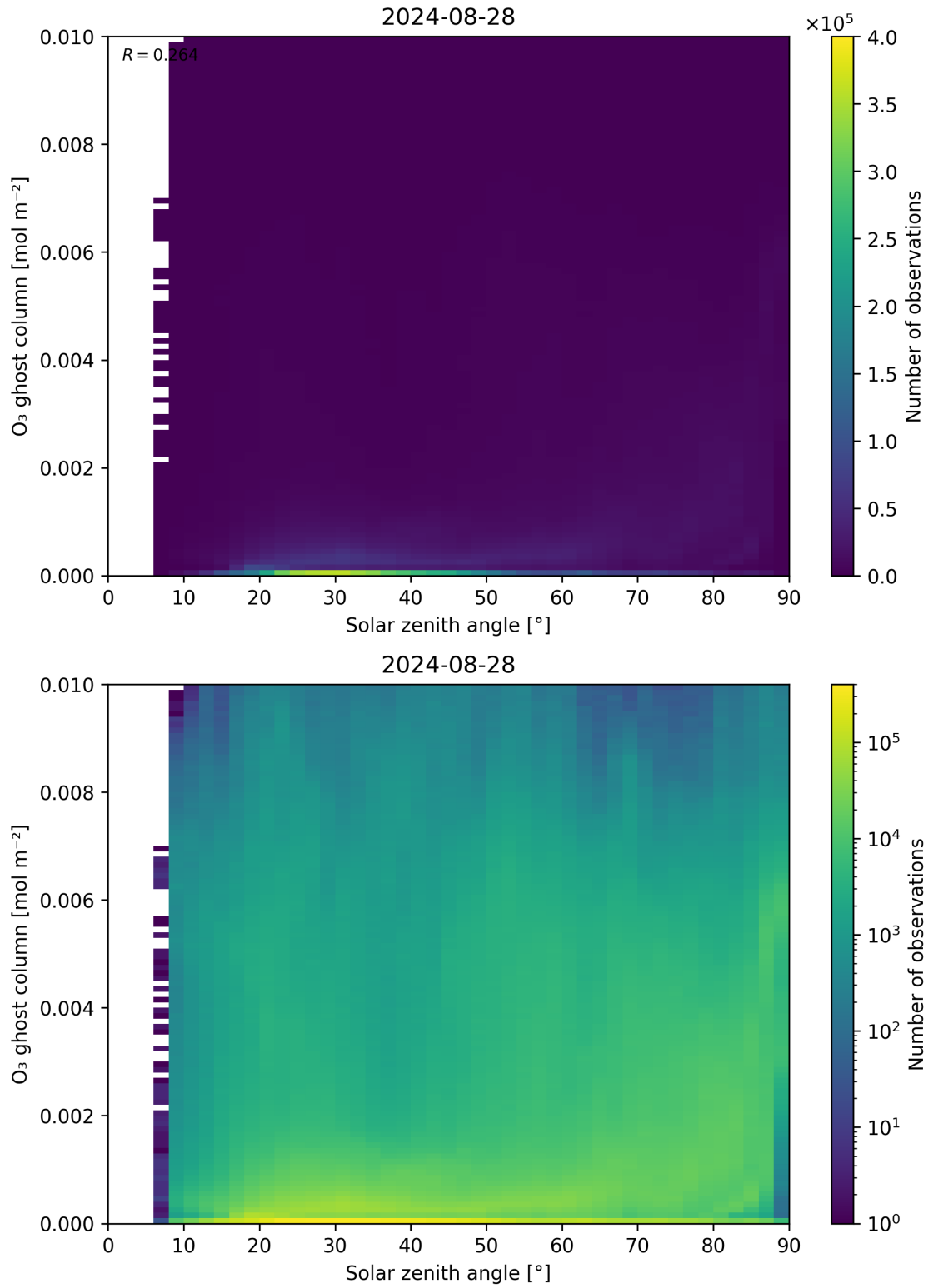
Figure 46: Scatter density plot of “Solar zenith angle” against “O 3 ghost column” for 2024-08-27 to 2024-08-29.
