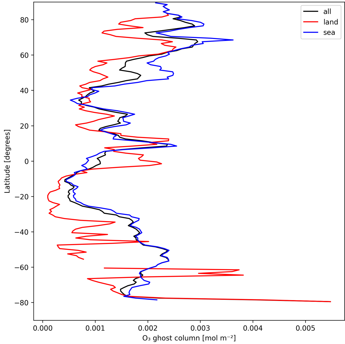
Figure 18: Zonal average of "O 3 ghost column" for 2024-08-27 to 2024-08-29.
