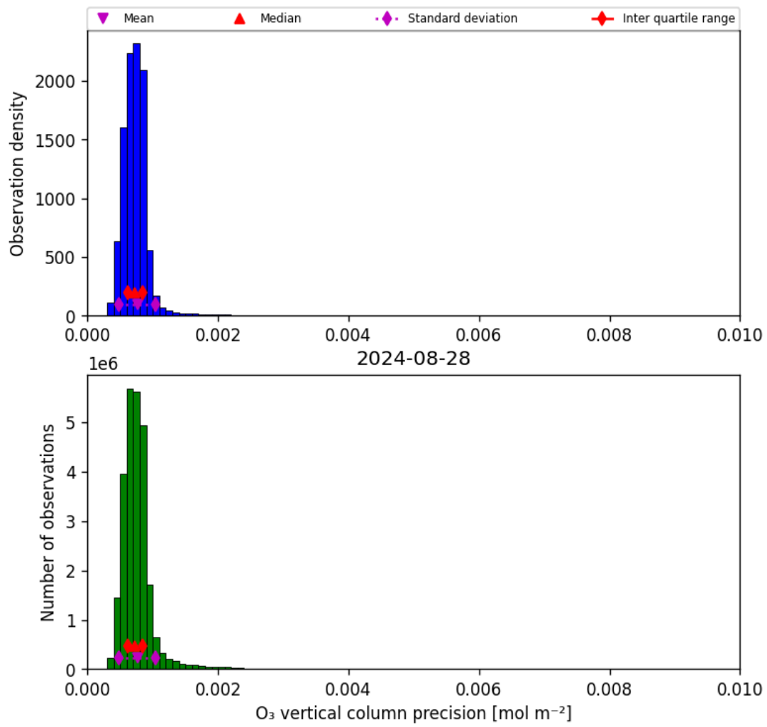
Figure 22: Histogram of “O 3 vertical column precision” for 2024-08-27 to 2024-08-29
