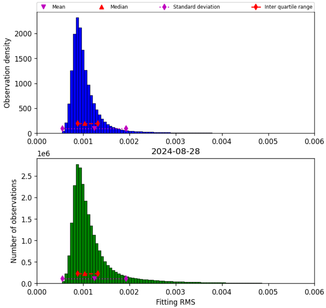
Figure 23: Histogram of “Fitting RMS” for 2024-08-27 to 2024-08-29
