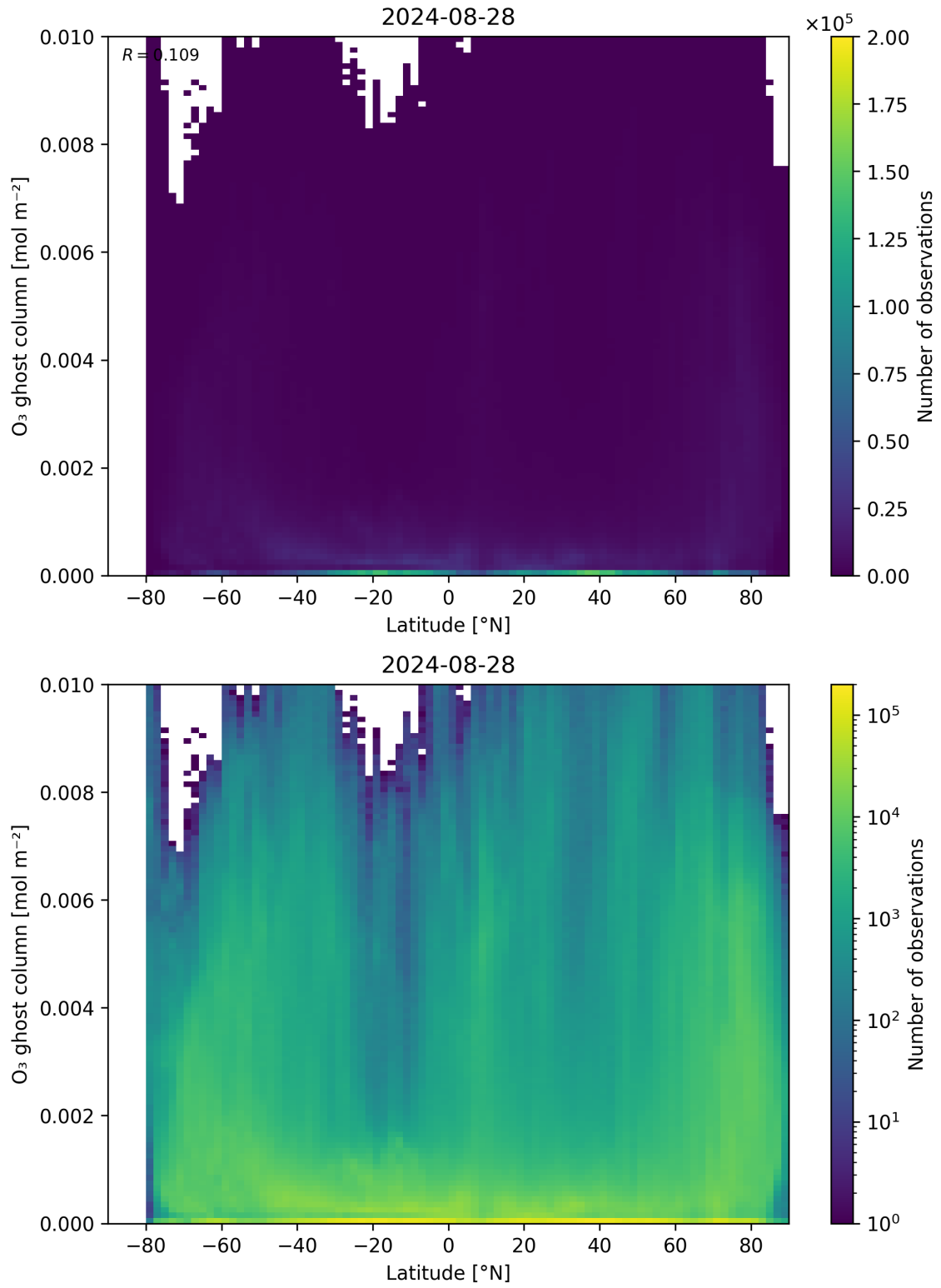
Figure 35: Scatter density plot of “Latitude” against “O 3 ghost column” for 2024-08-27 to 2024-08-29.
