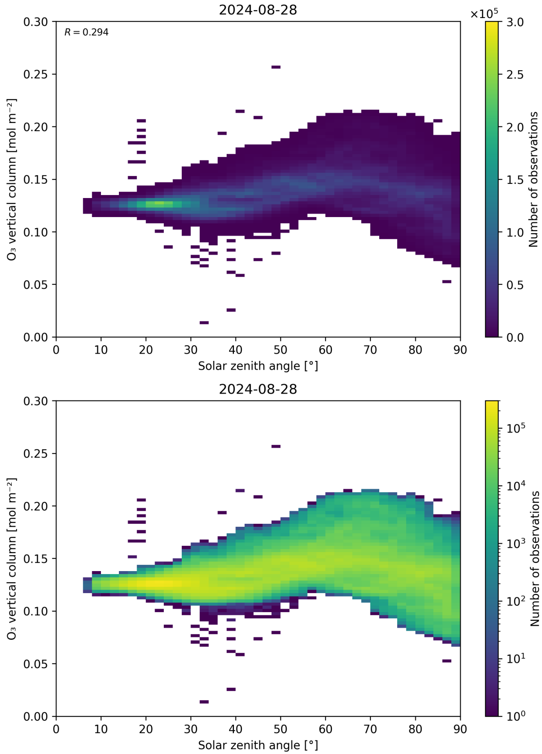
Figure 47: Scatter density plot of “Solar zenith angle” against “O 3 vertical column” for 2024-08-27 to 2024-08-29.
