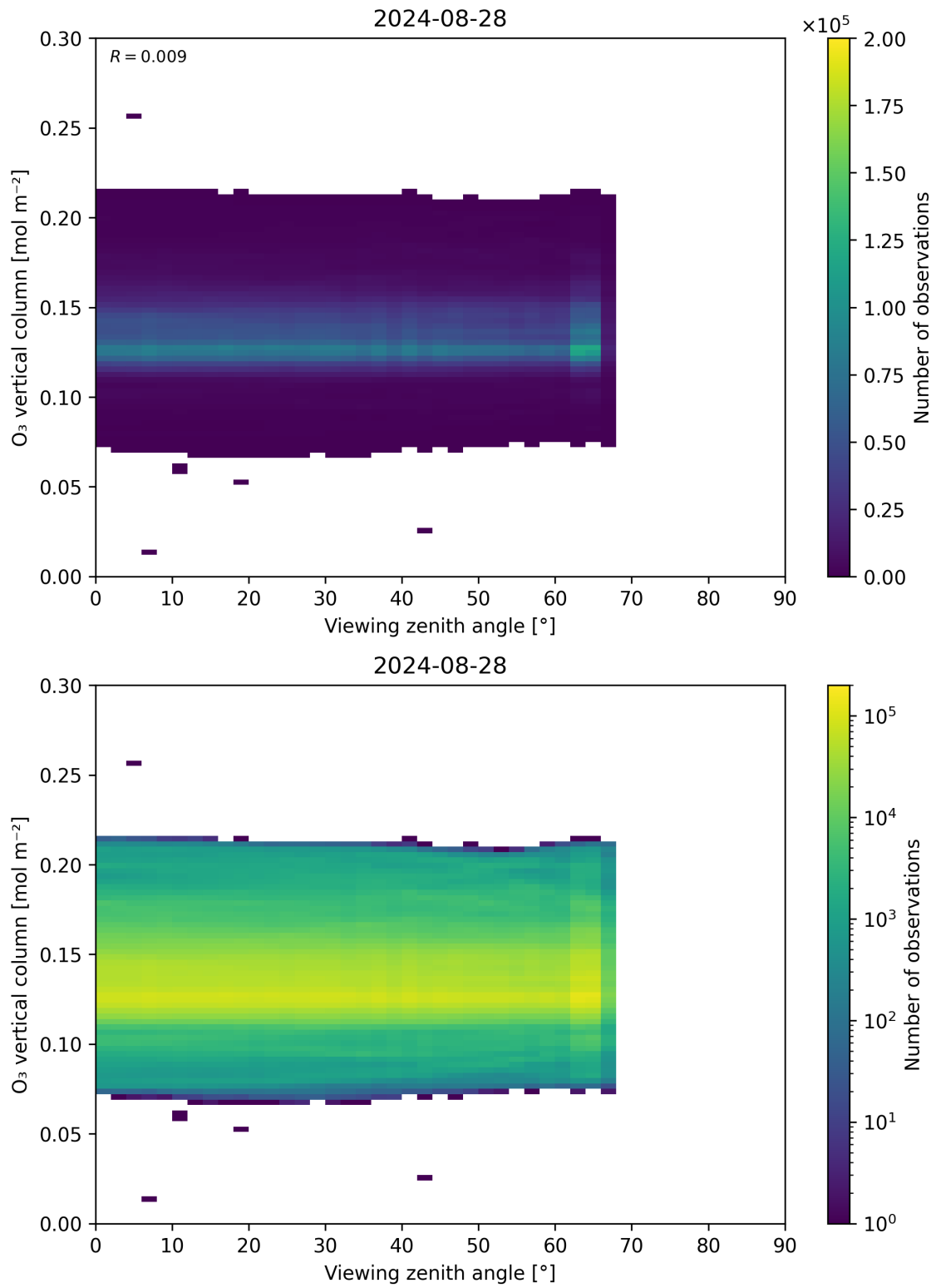
Figure 52: Scatter density plot of “Viewing zenith angle” against “O 3 vertical column” for 2024-08-27 to 2024-08-29.
