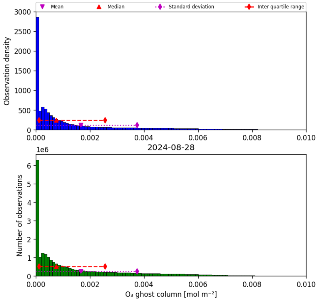
Figure 25: Histogram of “O 3 ghost column” for 2024-08-27 to 2024-08-29
