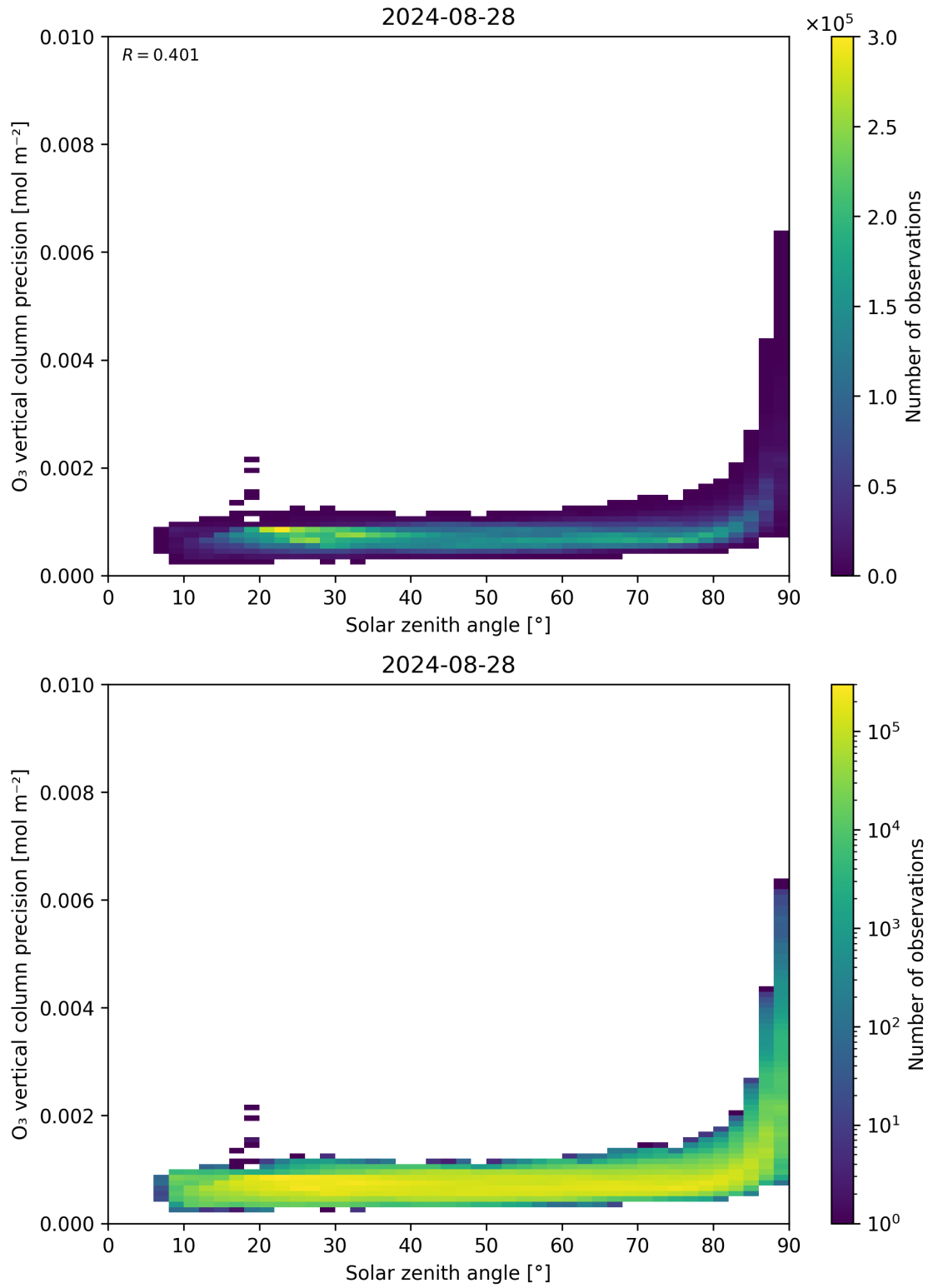
Figure 48: Scatter density plot of “Solar zenith angle” against “O 3 vertical column precision” for 2024-08-27 to 2024-08-29.
