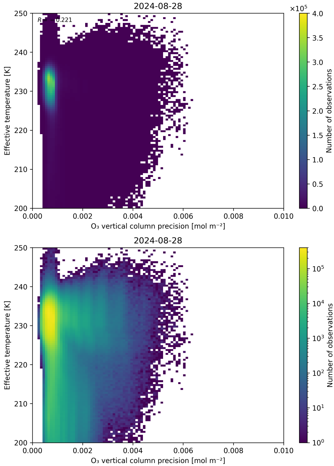
Figure 42: Scatter density plot of “O 3 vertical column precision” against “Effective temperature” for 2024-08-27 to 2024-08-29.
