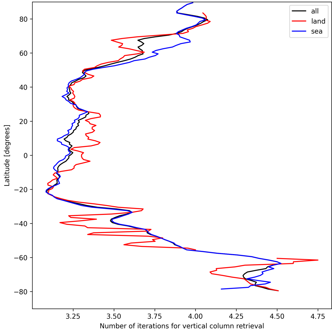
Figure 19: Zonal average of “Number of iterations for vertical column retrieval” for 2024-08-27 to 2024-08-29.
