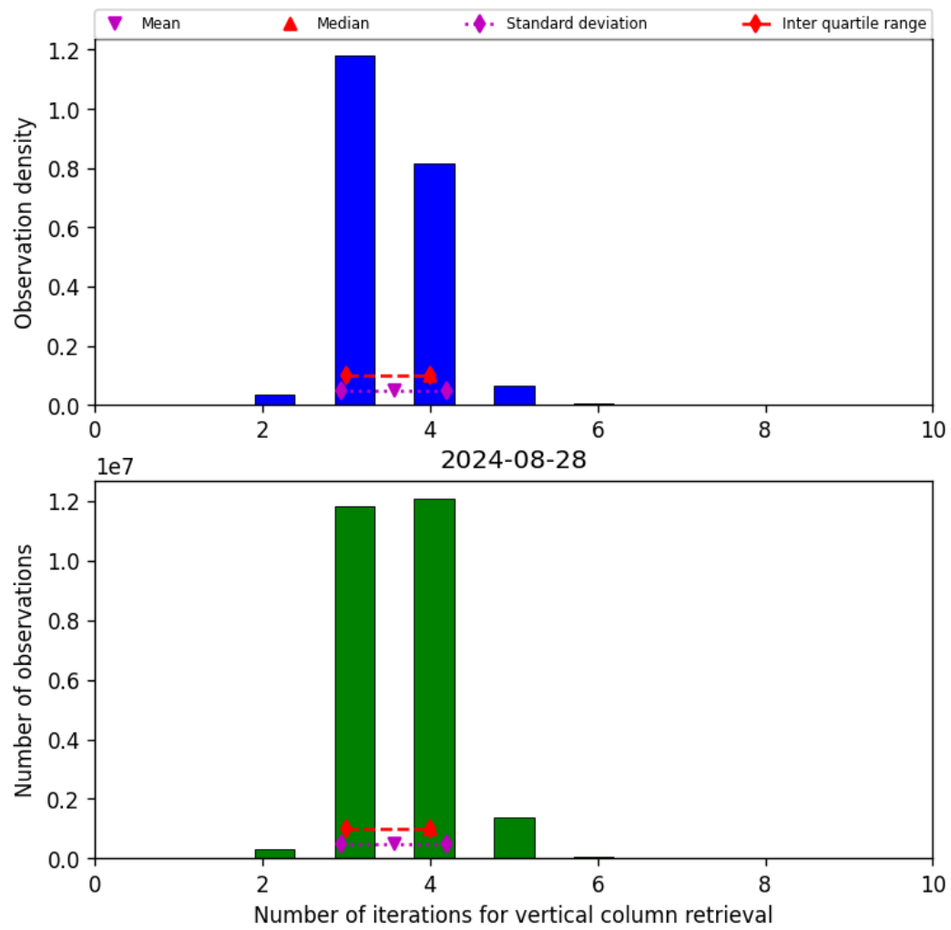
Figure 26: Histogram of “Number of iterations for vertical column retrieval” for 2024-08-27 to 2024-08-29
