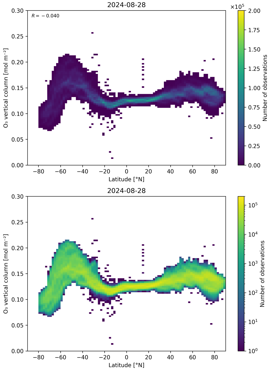
Figure 36: Scatter density plot of “Latitude” against “O 3 vertical column” for 2024-08-27 to 2024-08-29.
