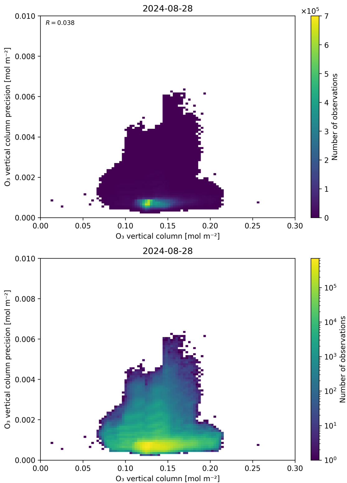
Figure 41: Scatter density plot of “O 3 vertical column” against “O 3 vertical column precision” for 2024-08-27 to 2024-08-29.
