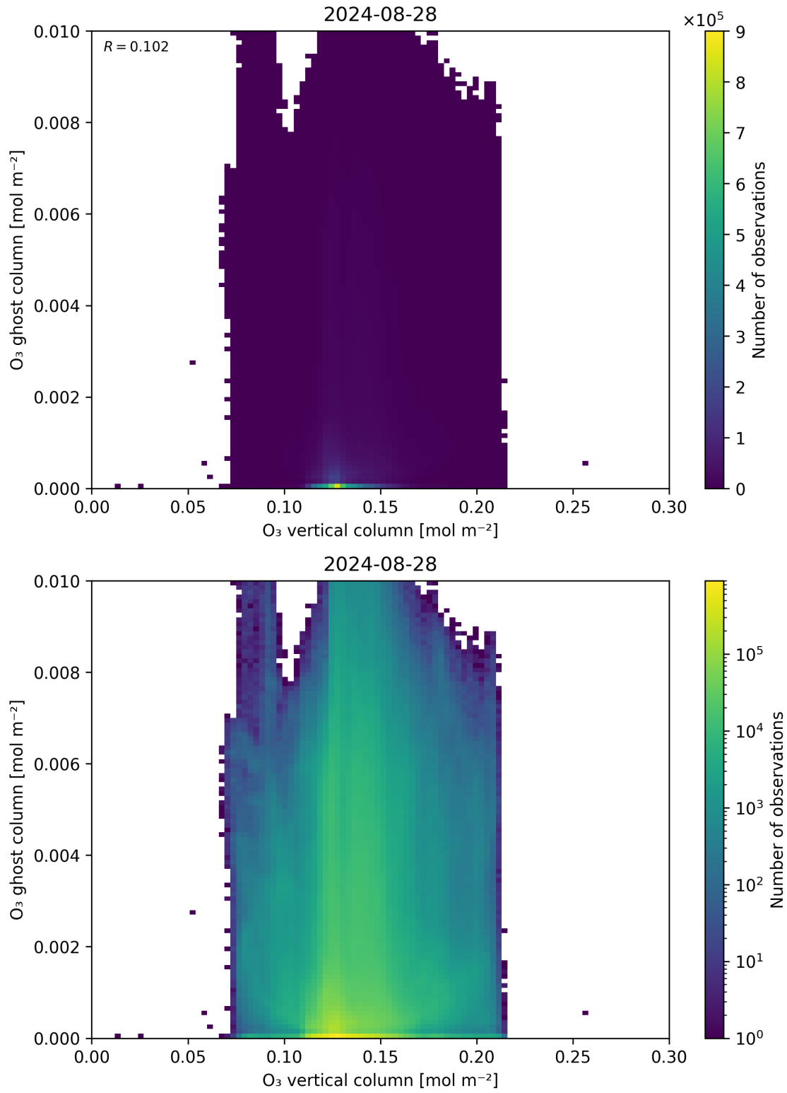
Figure 40: Scatter density plot of “O 3 vertical column” against “O 3 ghost column” for 2024-08-27 to 2024-08-29.
