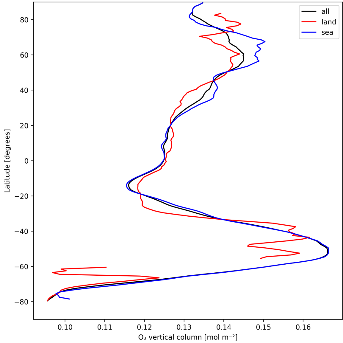
Figure 14: Zonal average of “O 3 vertical column” for 2024-08-27 to 2024-08-29.
