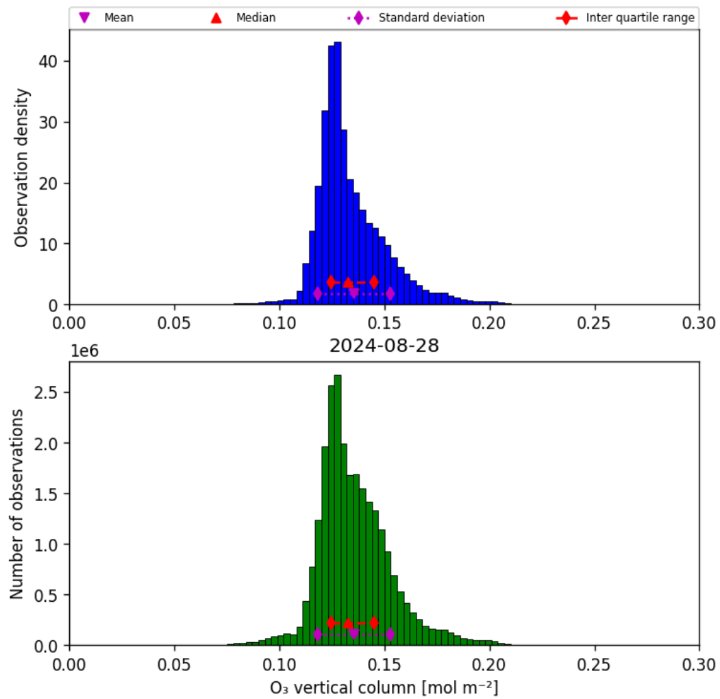
Figure 21: Histogram of “O 3 vertical column” for 2024-08-27 to 2024-08-29
