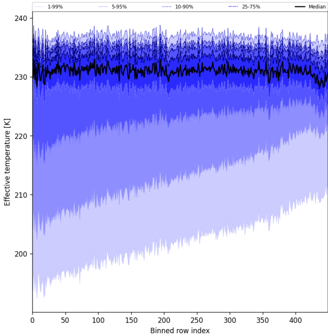
Figure 31: Along track statistics of “Effective temperature” for 2024-08-27 to 2024-08-29
