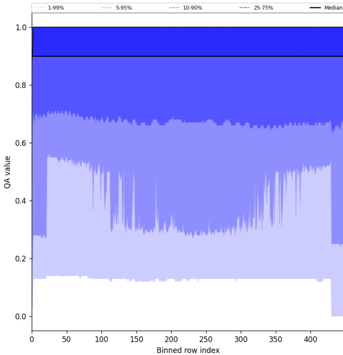
Figure 27: Along track statistics of “QA value” for 2024-08-27 to 2024-08-29
