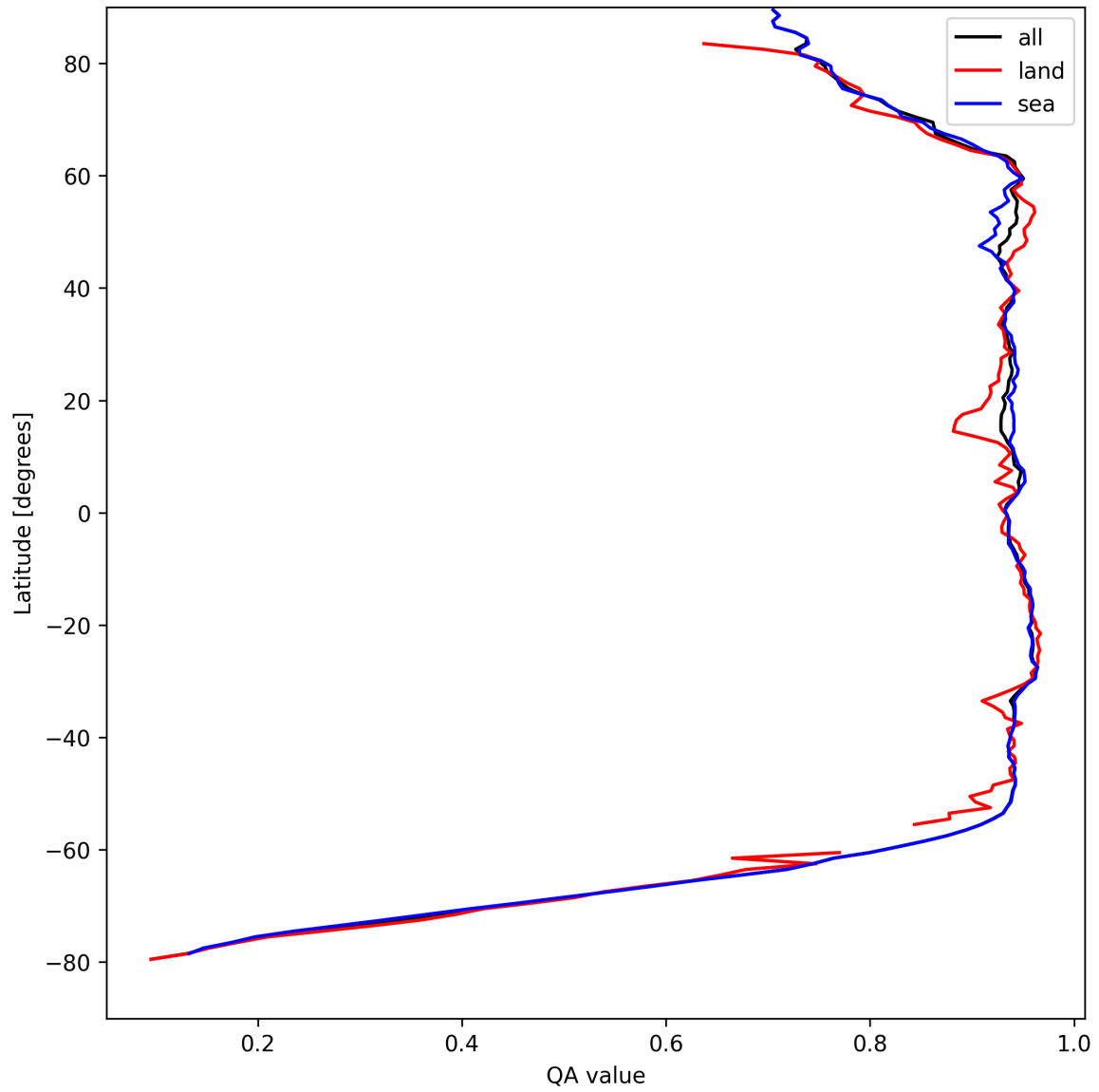
Figure 13: Zonal average of “QA value” for 2024-08-27 to 2024-08-29.
