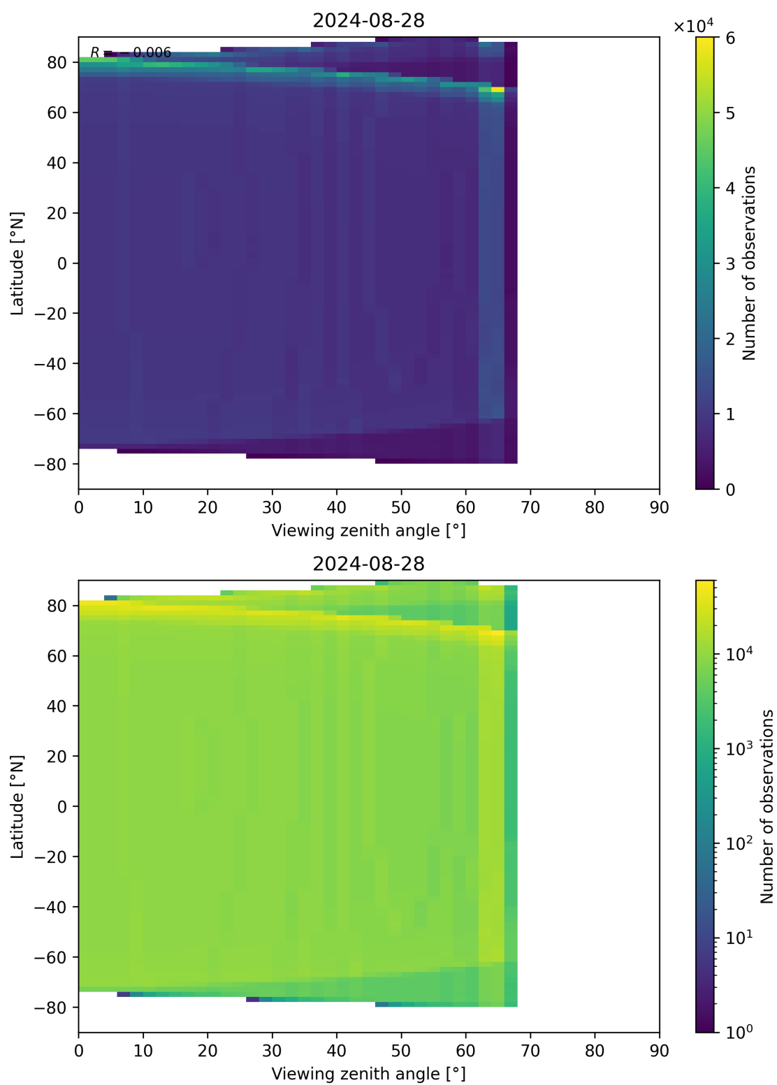
Figure 49: Scatter density plot of “Viewing zenith angle” against “Latitude” for 2024-08-27 to 2024-08-29.
