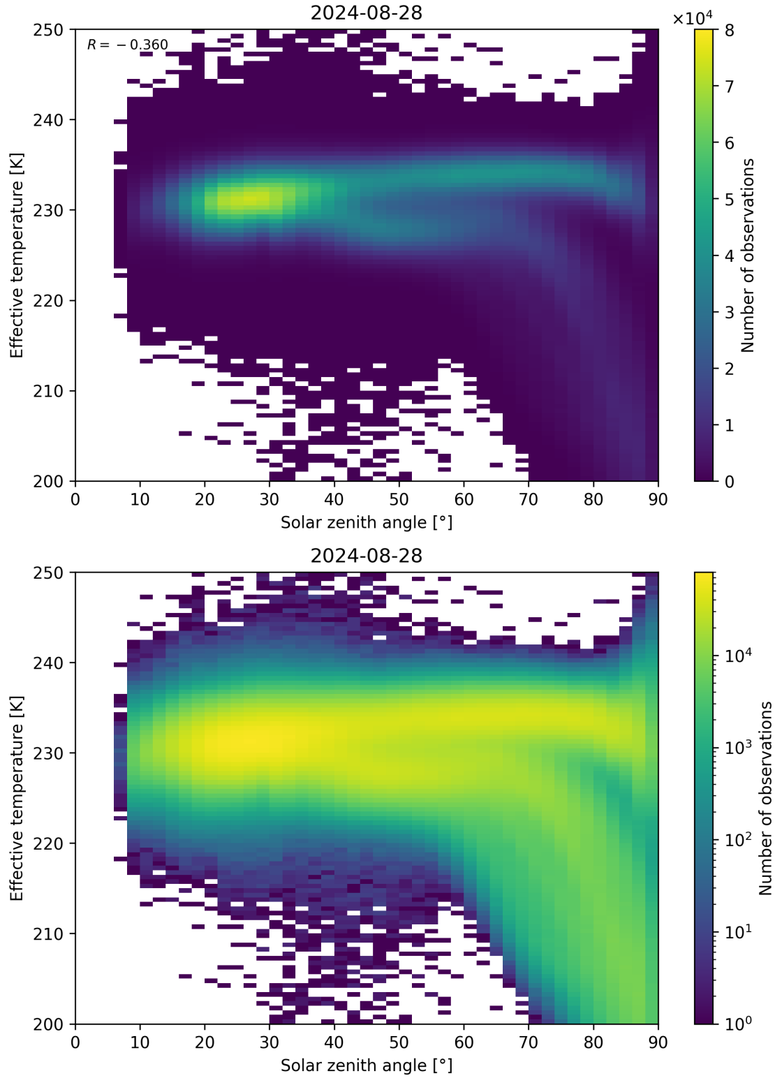
Figure 45: Scatter density plot of “Solar zenith angle” against “Effective temperature” for 2024-08-27 to 2024-08-29.
