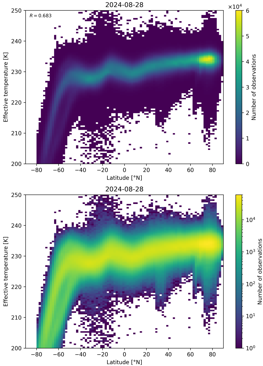
Figure 34: Scatter density plot of “Latitude” against “Effective temperature” for 2024-08-27 to 2024-08-29.
