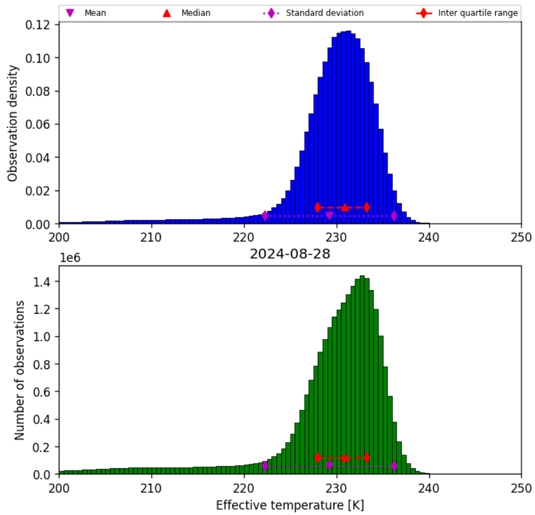
Figure 24: Histogram of “Effective temperature” for 2024-08-27 to 2024-08-29
