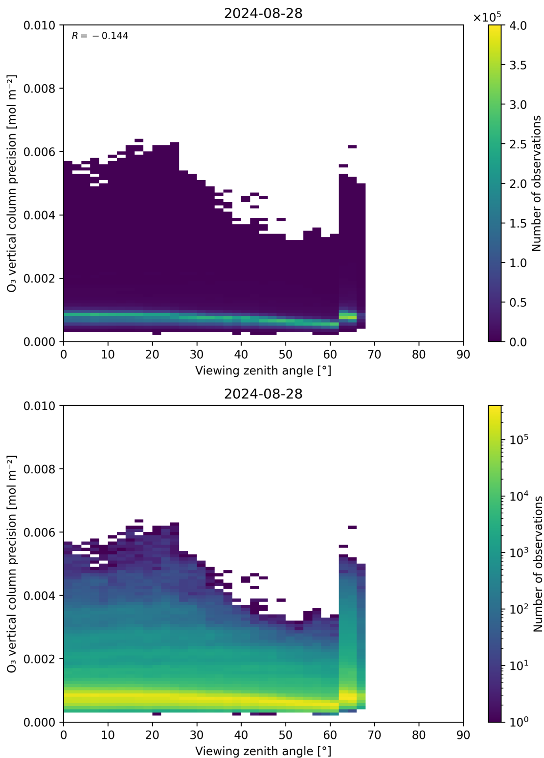
Figure 53: Scatter density plot of “Viewing zenith angle” against “O 3 vertical column precision” for 2024-08-27 to 2024-08-29.
