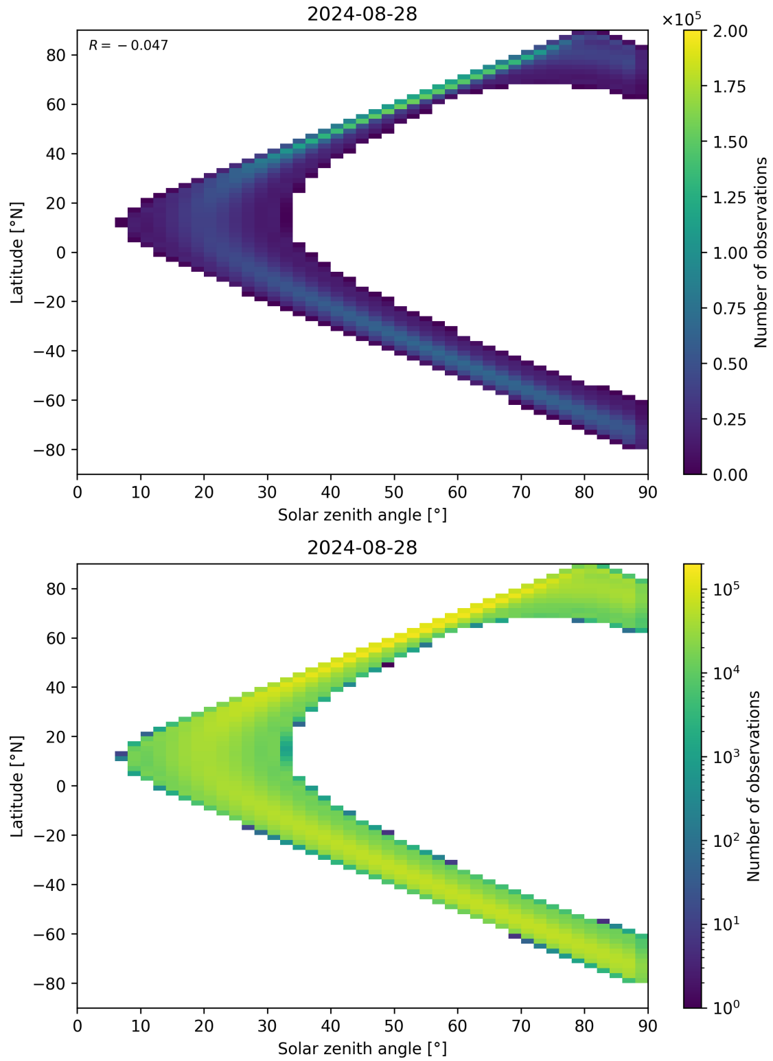
Figure 44: Scatter density plot of “Solar zenith angle” against “Latitude” for 2024-08-27 to 2024-08-29.
