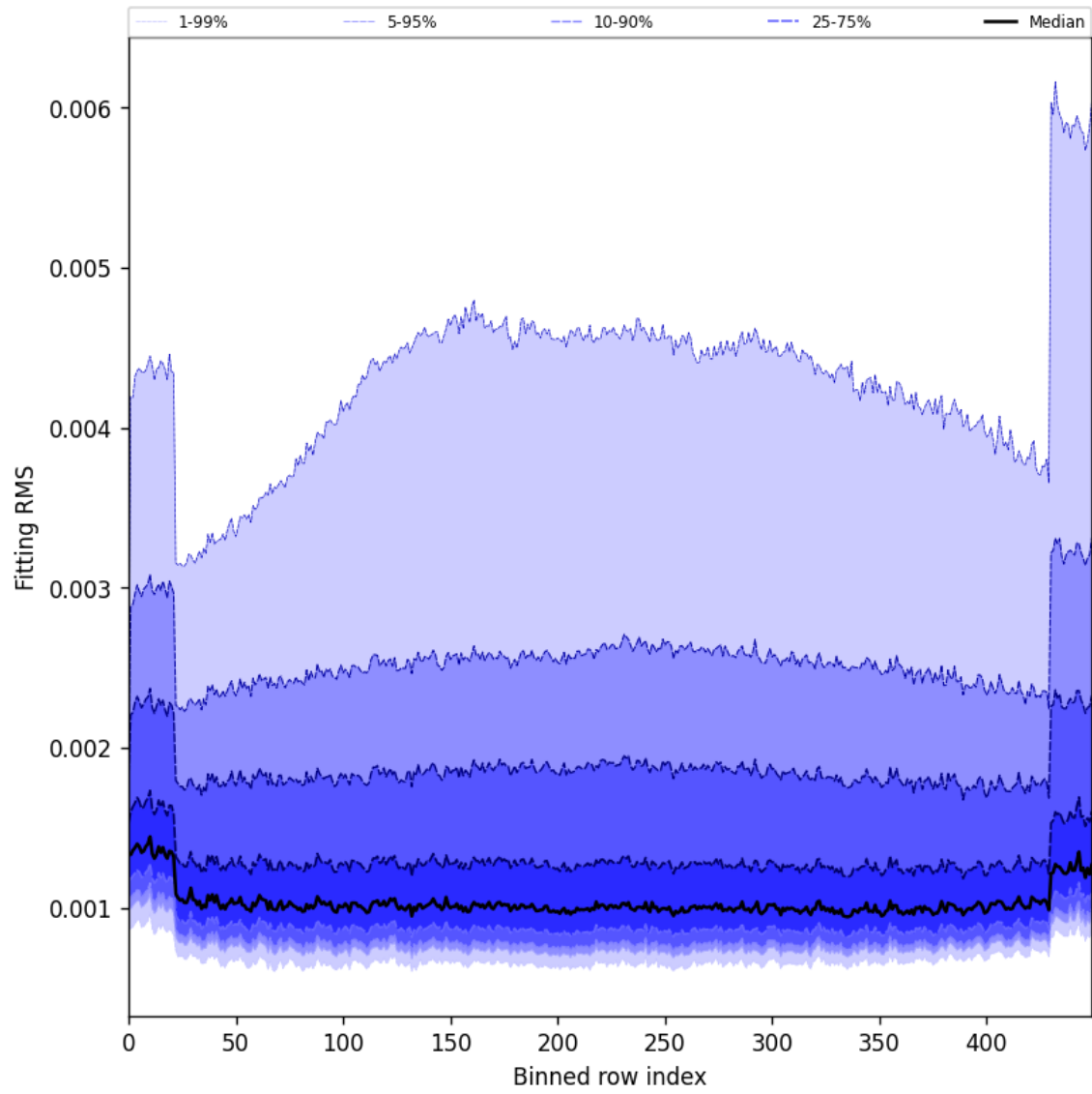
Figure 30: Along track statistics of “Fitting RMS” for 2024-08-27 to 2024-08-29
