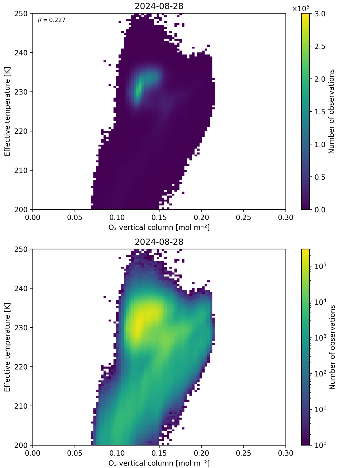
Figure 39: Scatter density plot of “O 3 vertical column” against “Effective temperature” for 2024-08-27 to 2024-08-29.
