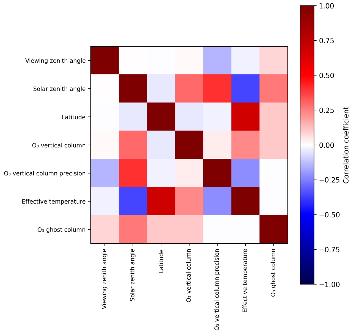
Figure 2: Map of correlation matrix for 2024-08-27 to 2024-08-29.
