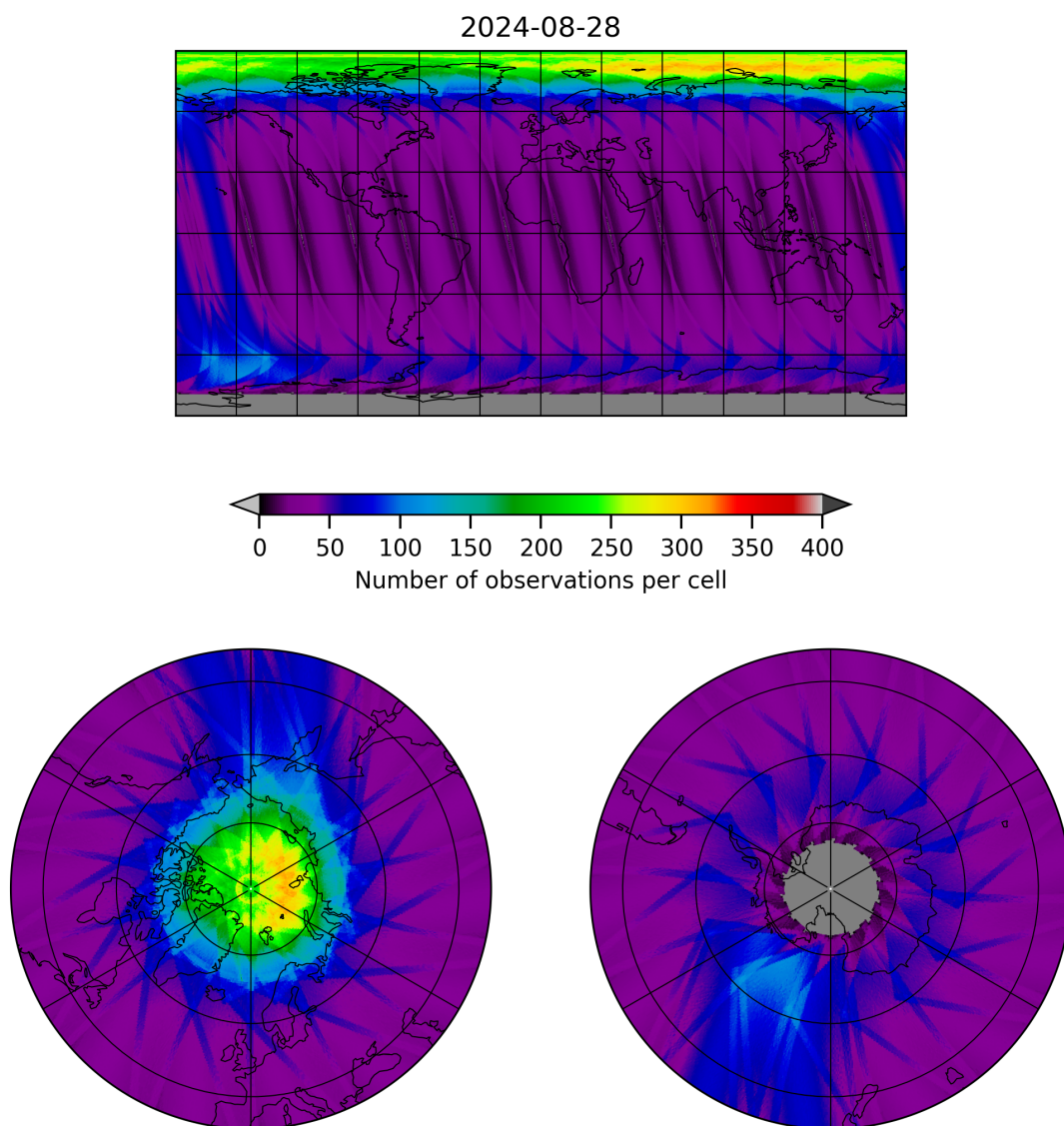
Figure 12: Map of the number of observations for 2024-08-27 to 2024-08-29
