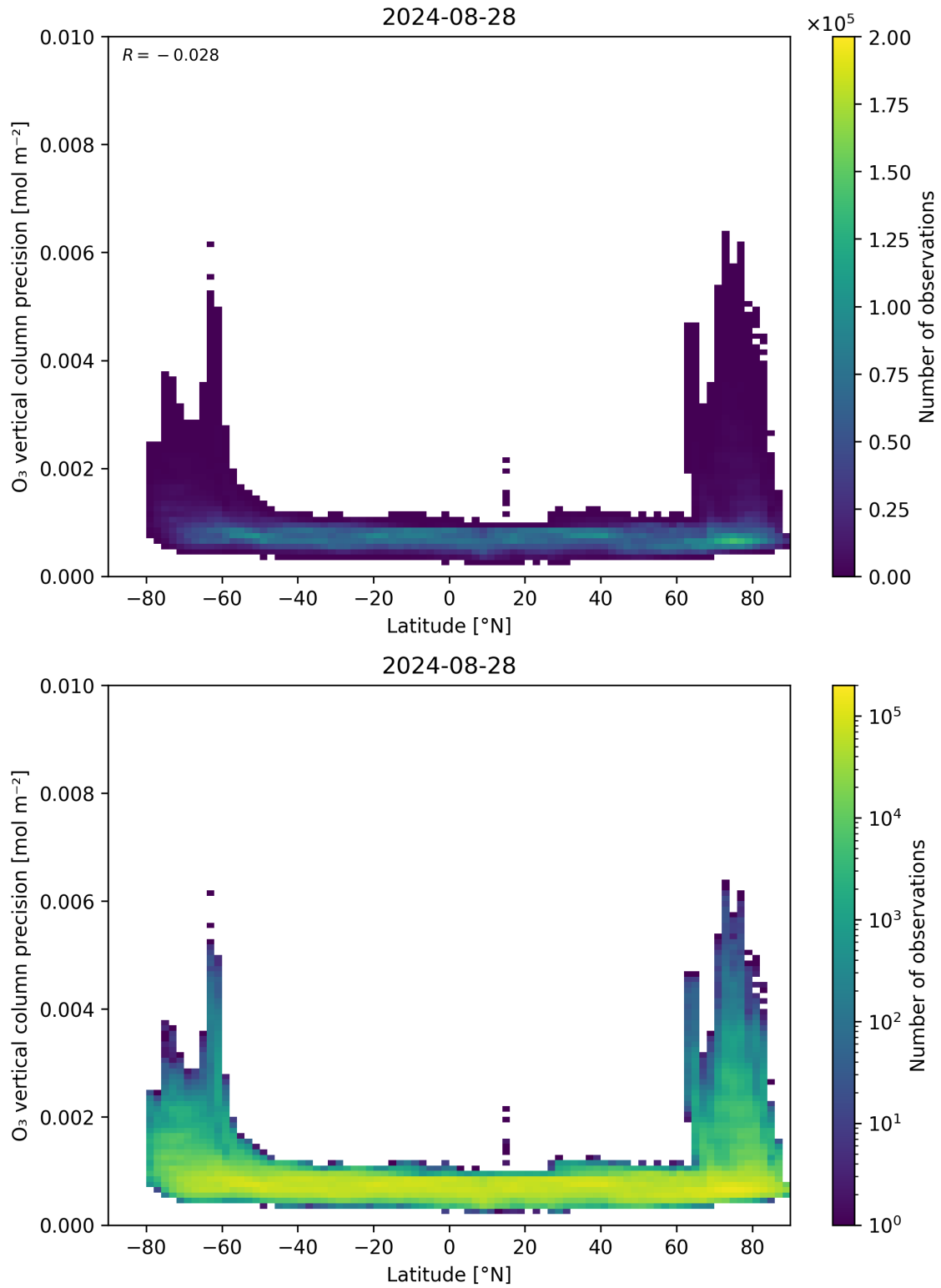
Figure 37: Scatter density plot of “Latitude” against “O 3 vertical column precision” for 2024-08-27 to 2024-08-29.
