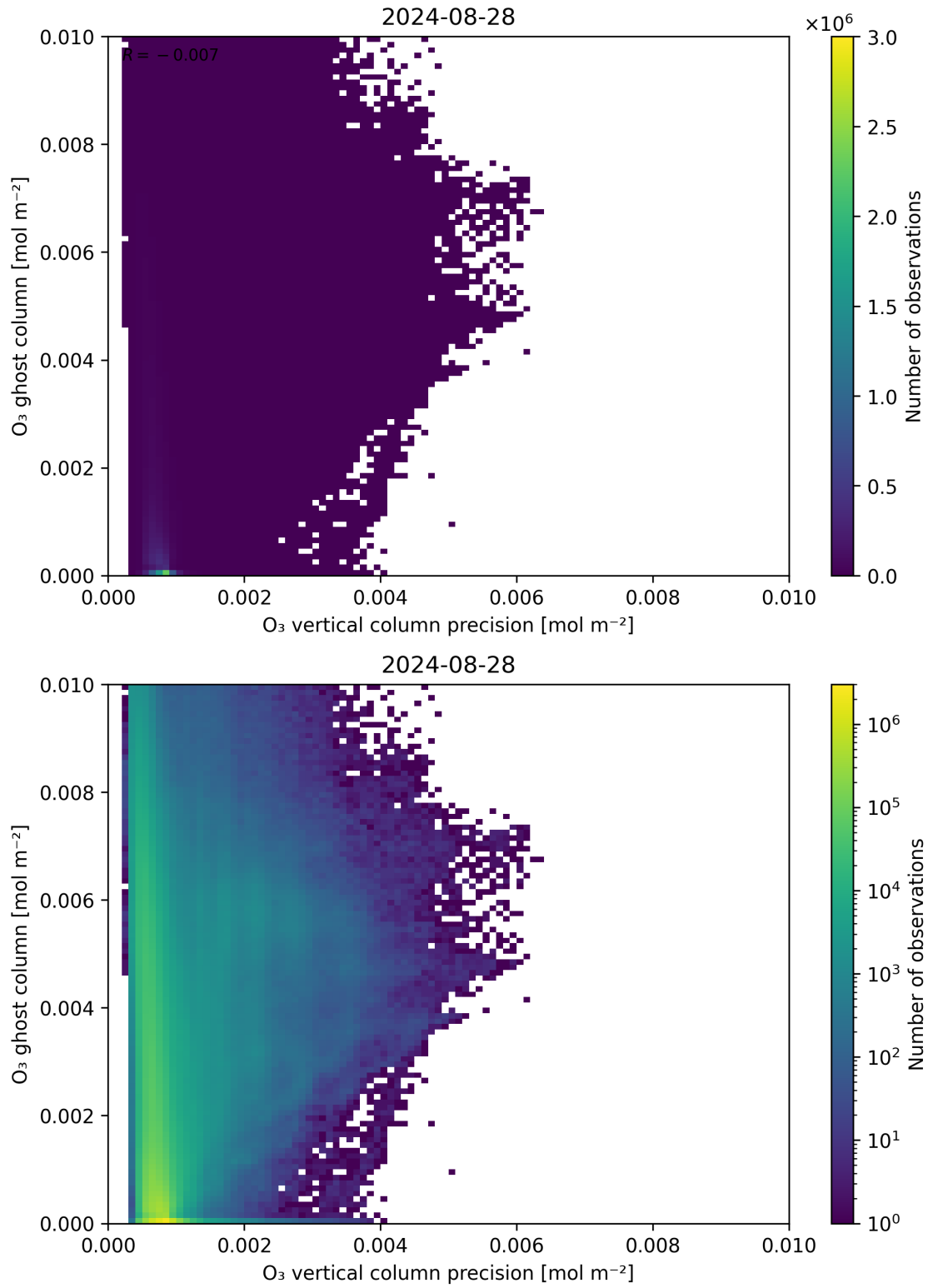
Figure 43: Scatter density plot of “ \text{O}_3 vertical column precision” against “ \text{O}_3 ghost column” for 2024-08-27 to 2024-08-29.
