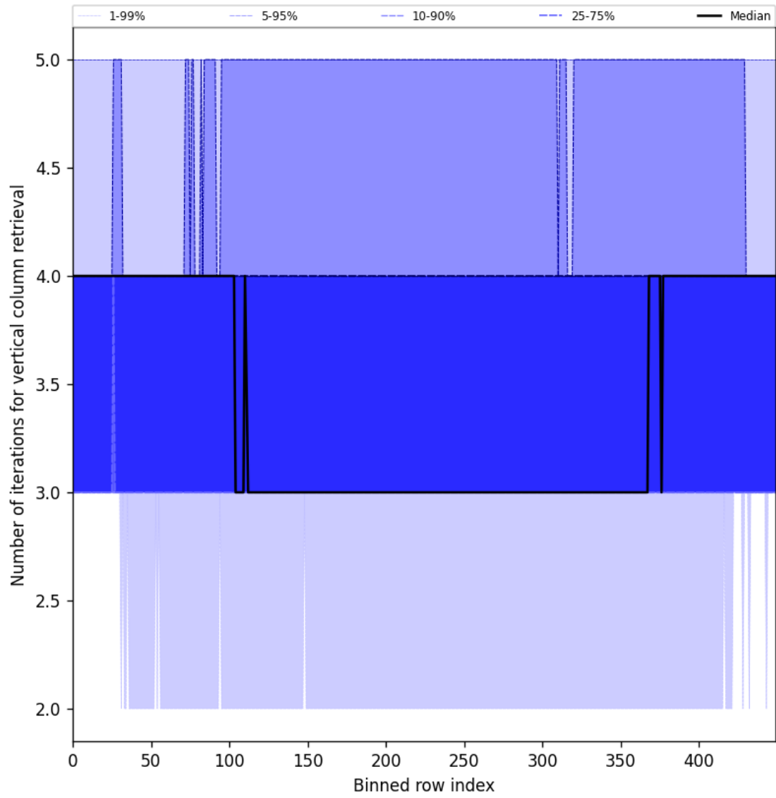
Figure 33: Along track statistics of “Number of iterations for vertical column retrieval” for 2024-08-27 to 2024-08-29
