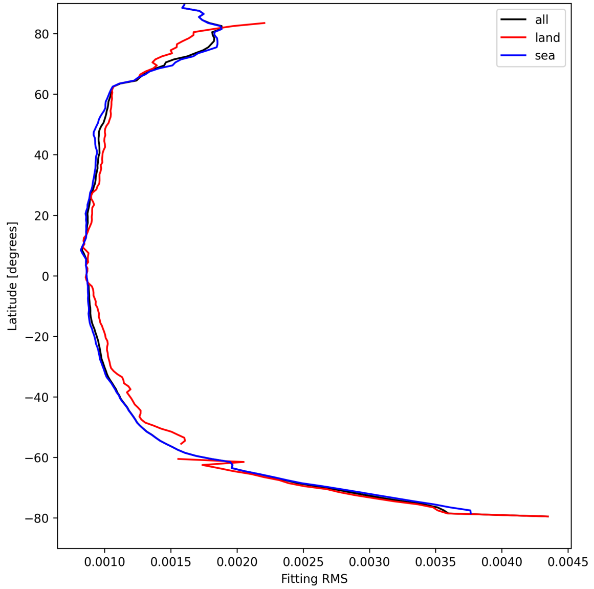
Figure 16: Zonal average of “Fitting RMS” for 2024-08-27 to 2024-08-29.
