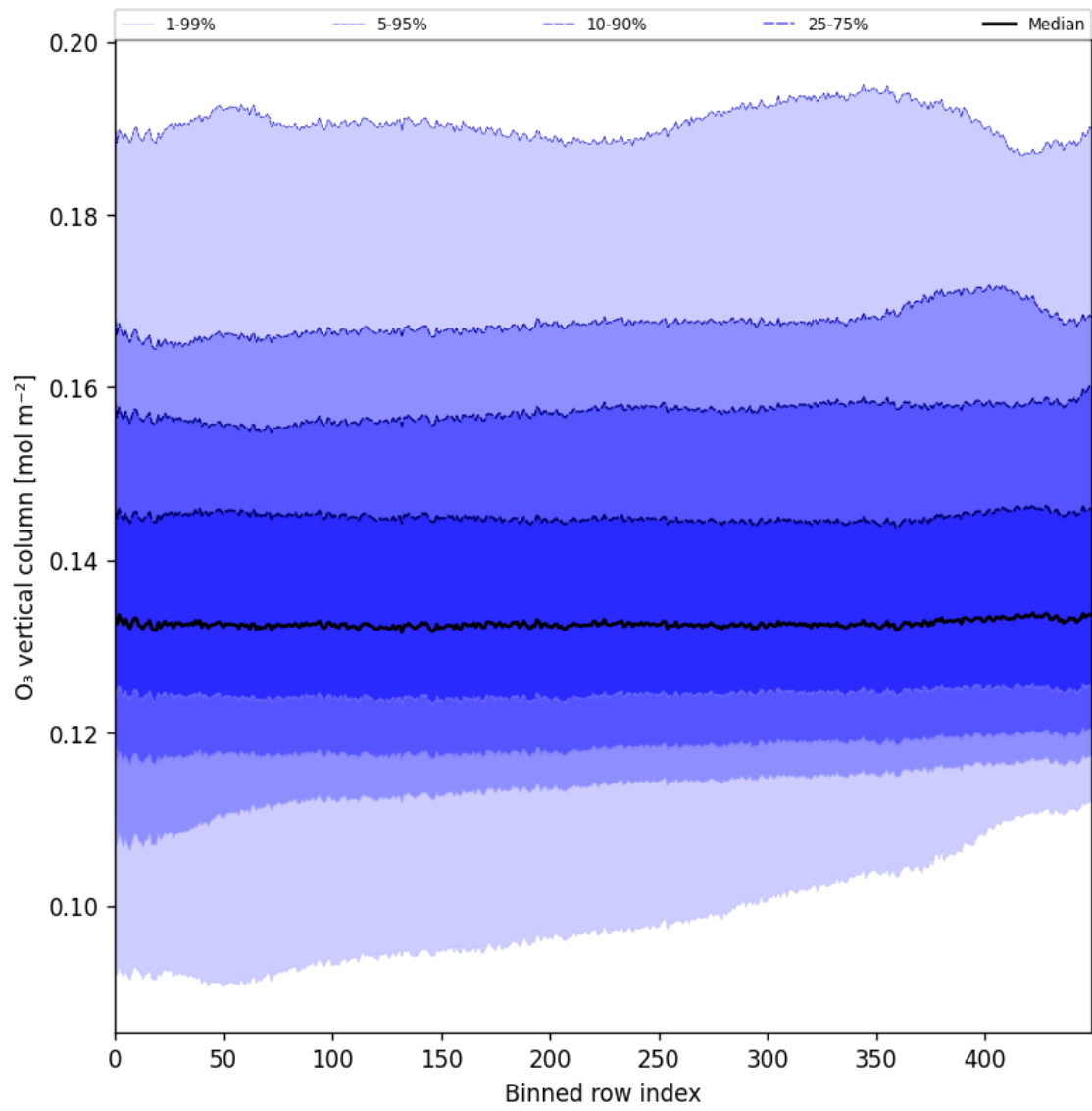
Figure 28: Along track statistics of “O 3 vertical column” for 2024-08-27 to 2024-08-29
