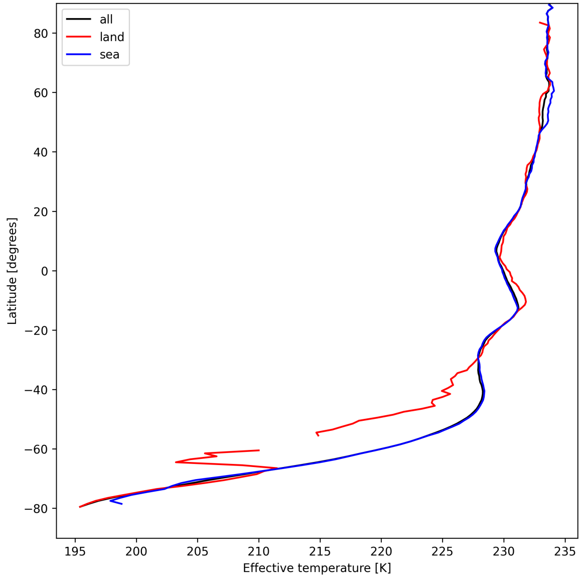
Figure 17: Zonal average of “Effective temperature” for 2024-08-27 to 2024-08-29.
