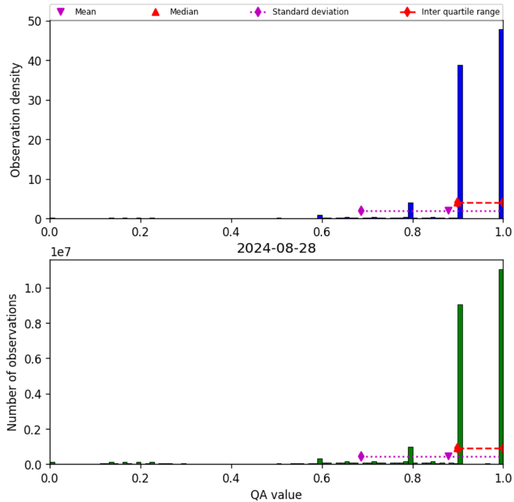
Figure 20: Histogram of “QA value” for 2024-08-27 to 2024-08-29
