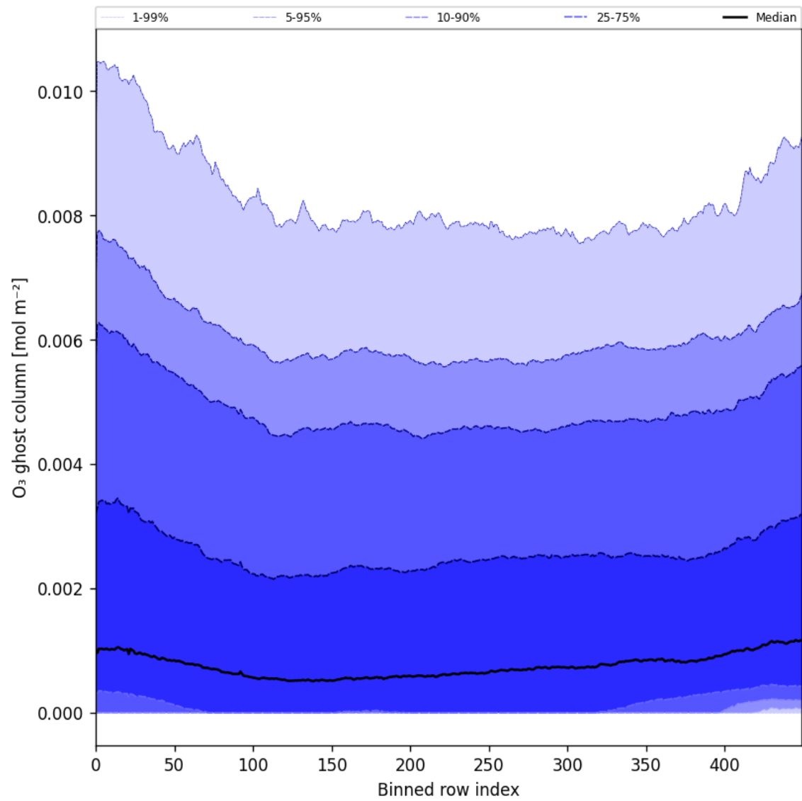
Figure 32: Along track statistics of “O 3 ghost column” for 2024-08-27 to 2024-08-29
