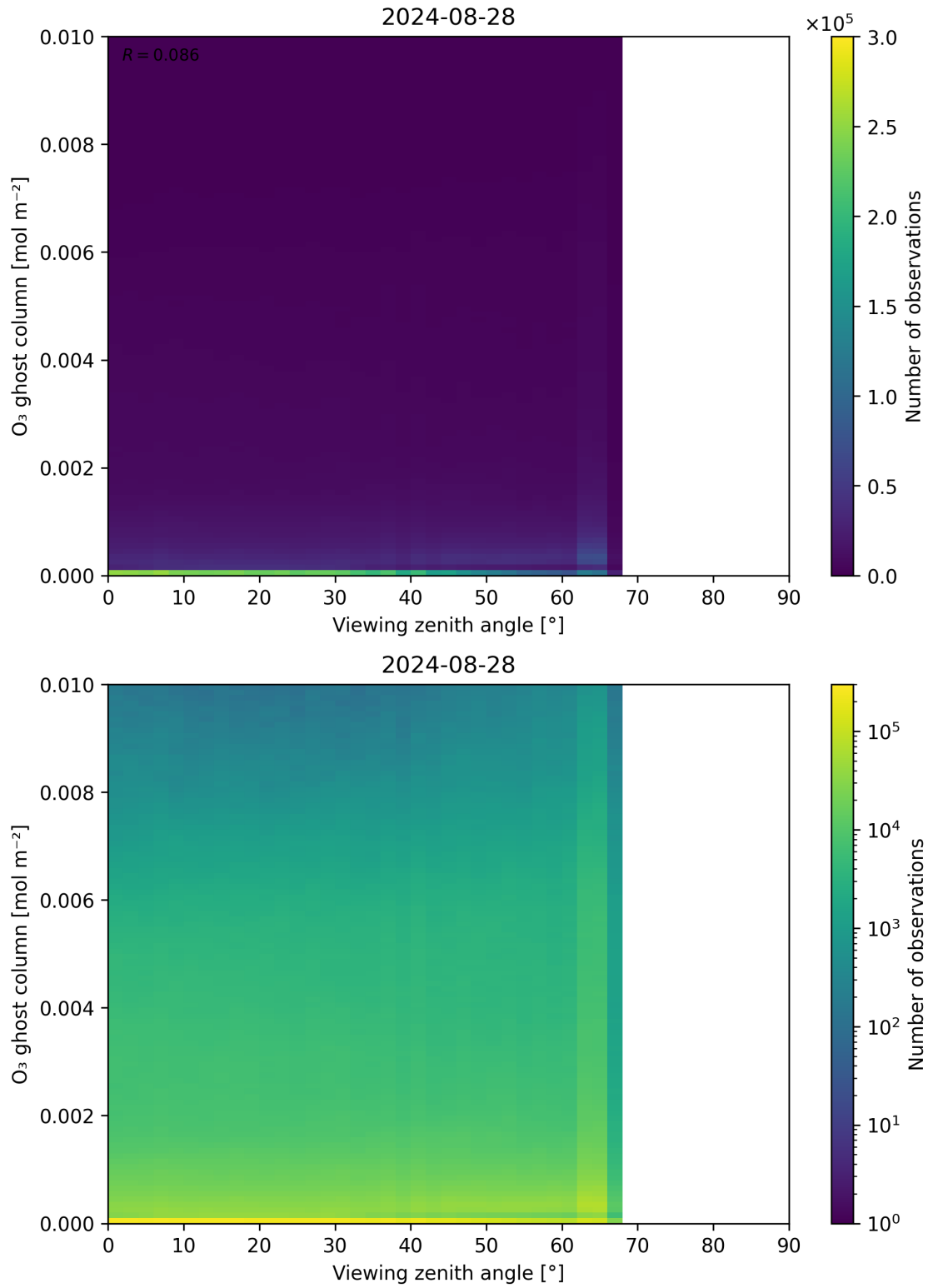
Figure 51: Scatter density plot of “Viewing zenith angle” against “O 3 ghost column” for 2024-08-27 to 2024-08-29.
