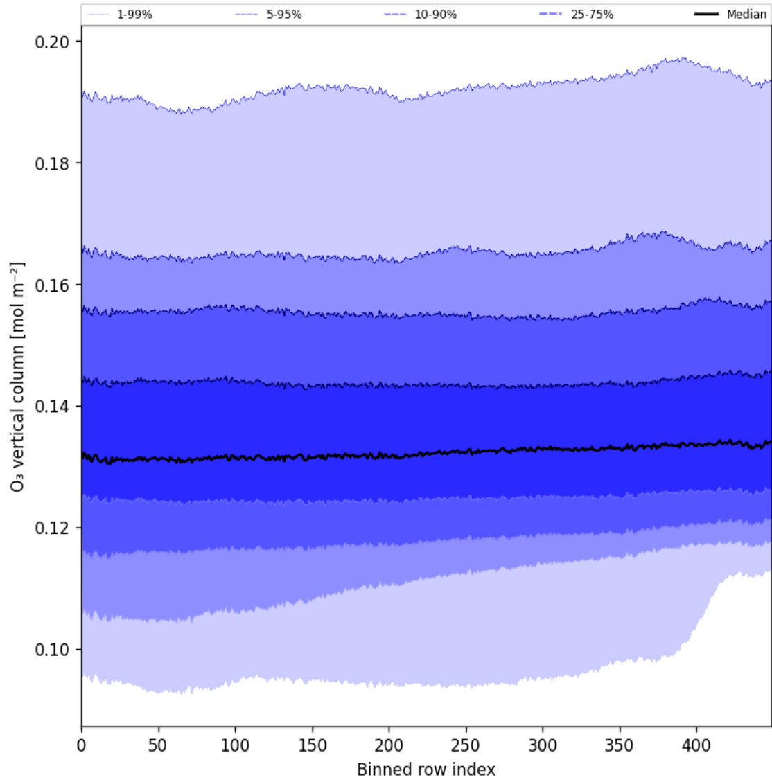
Figure 28: Along track statistics of “O 3 vertical column” for 2024-08-29 to 2024-08-31
