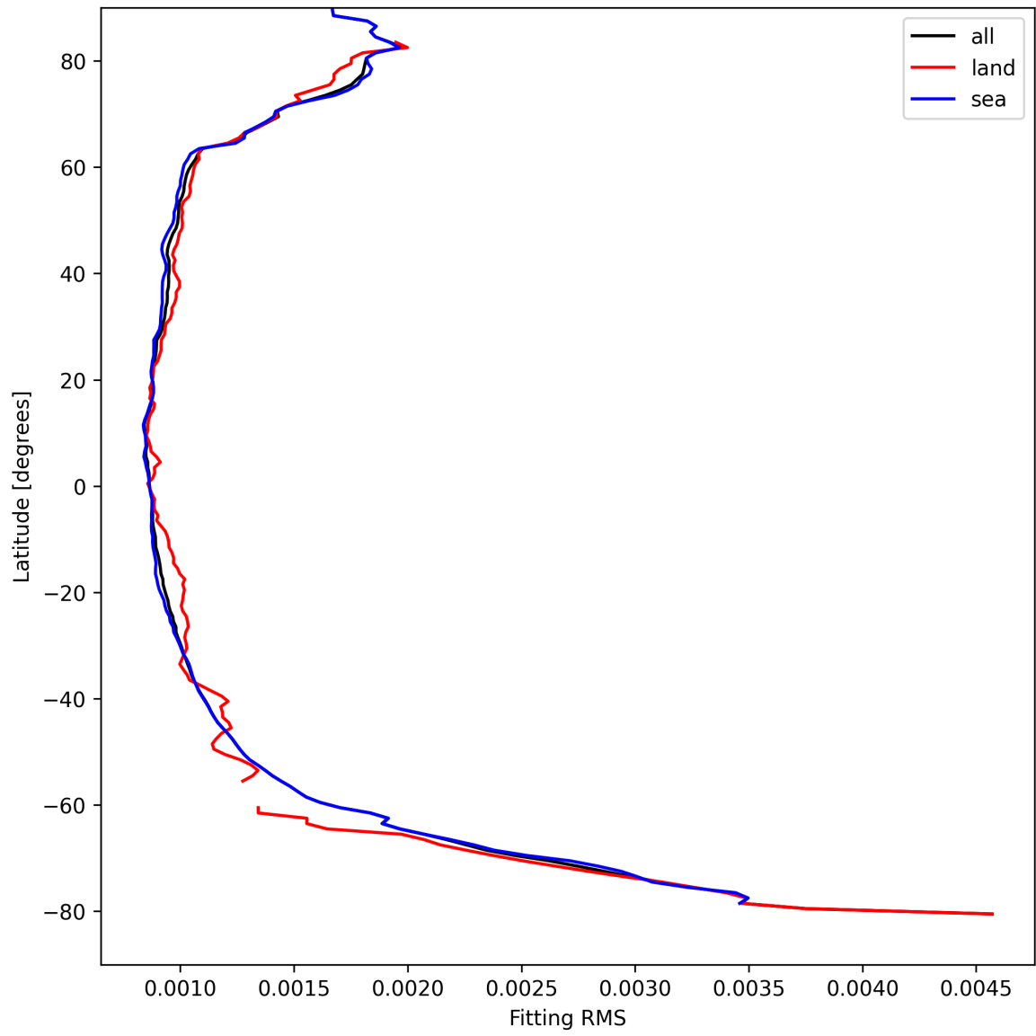
Figure 16: Zonal average of “Fitting RMS” for 2024-08-29 to 2024-08-31.
