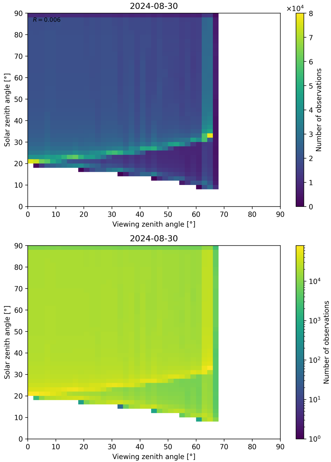
Figure 54: Scatter density plot of “Viewing zenith angle” against “Solar zenith angle” for 2024-08-29 to 2024-08-31.
