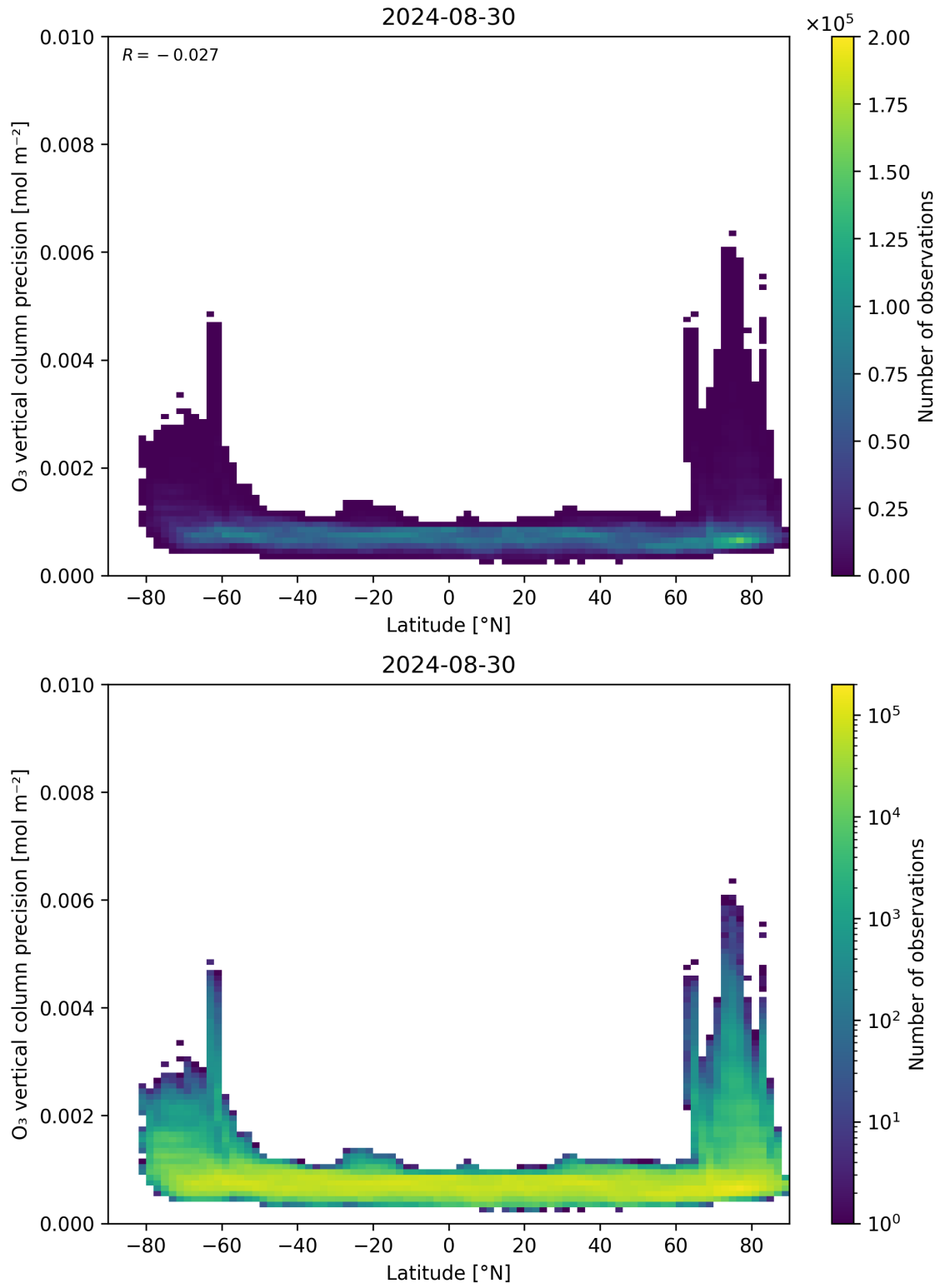
Figure 37: Scatter density plot of “Latitude” against “O 3 vertical column precision” for 2024-08-29 to 2024-08-31.
