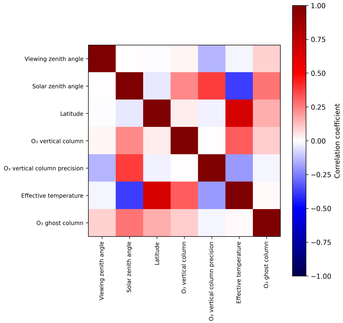
Figure 2: Map of correlation matrix for 2024-08-29 to 2024-08-31.
