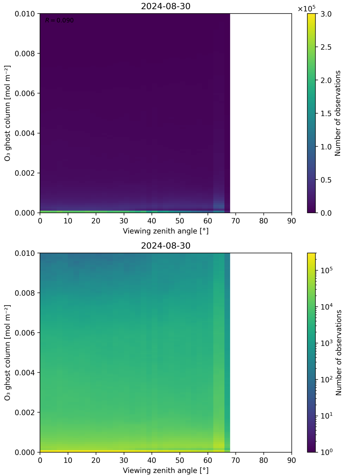
Figure 51: Scatter density plot of “Viewing zenith angle” against “O 3 ghost column” for 2024-08-29 to 2024-08-31.
