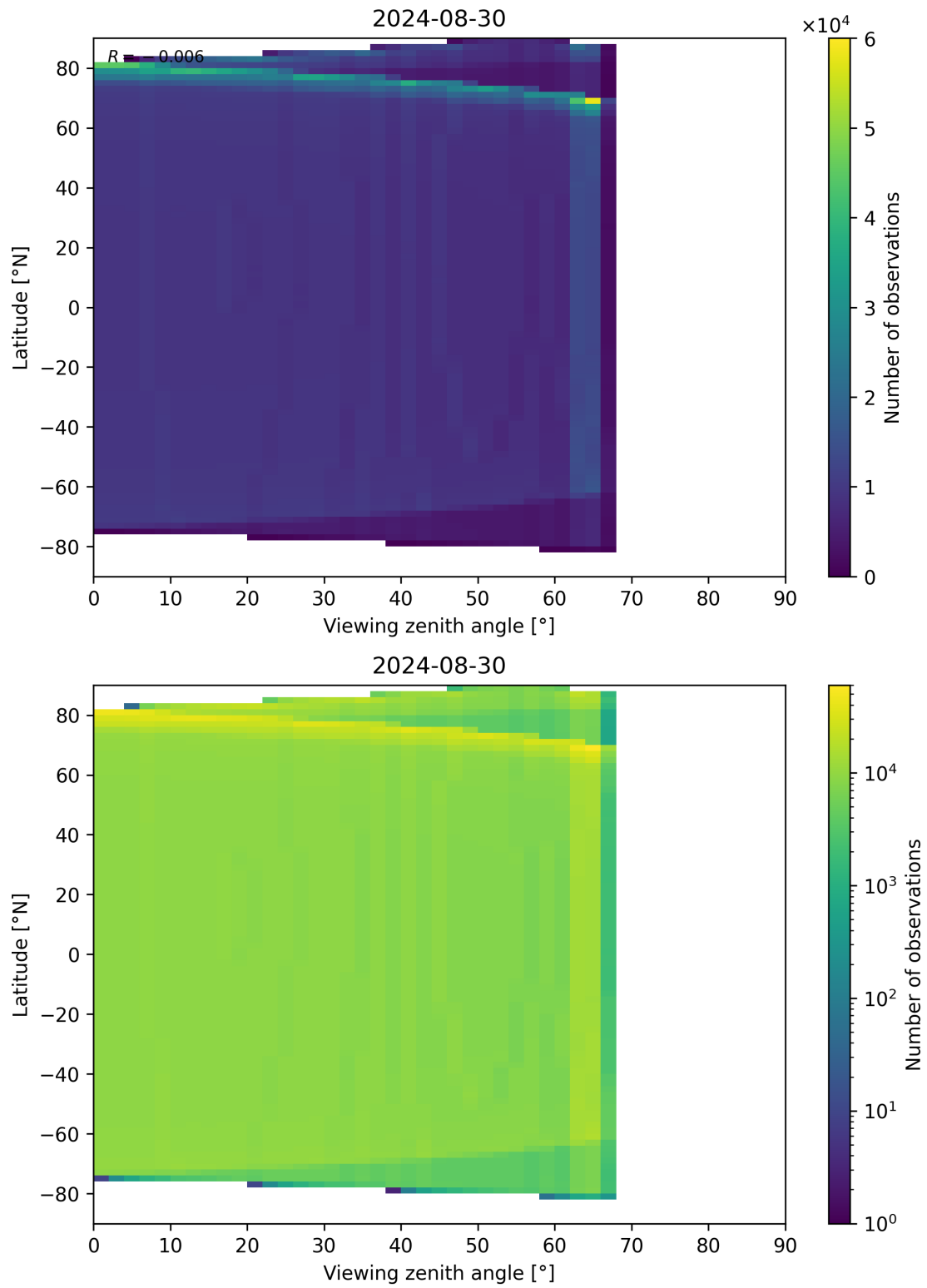
Figure 49: Scatter density plot of “Viewing zenith angle” against “Latitude” for 2024-08-29 to 2024-08-31.
