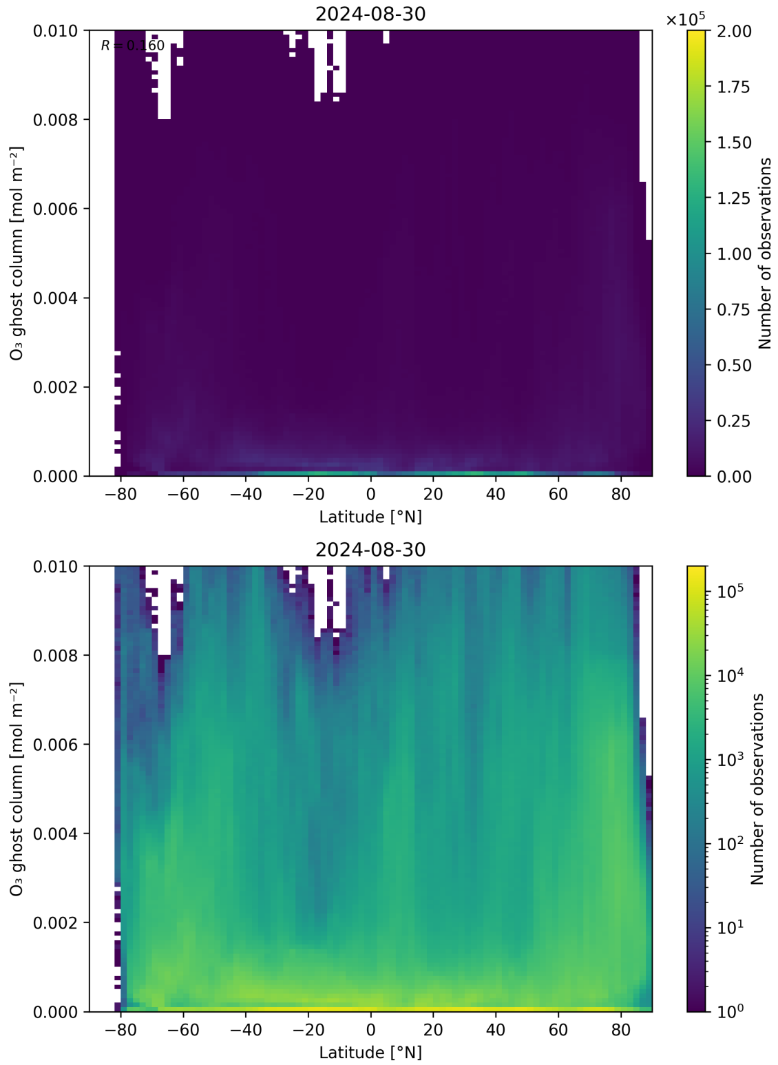
Figure 35: Scatter density plot of “Latitude” against “O 3 ghost column” for 2024-08-29 to 2024-08-31.
