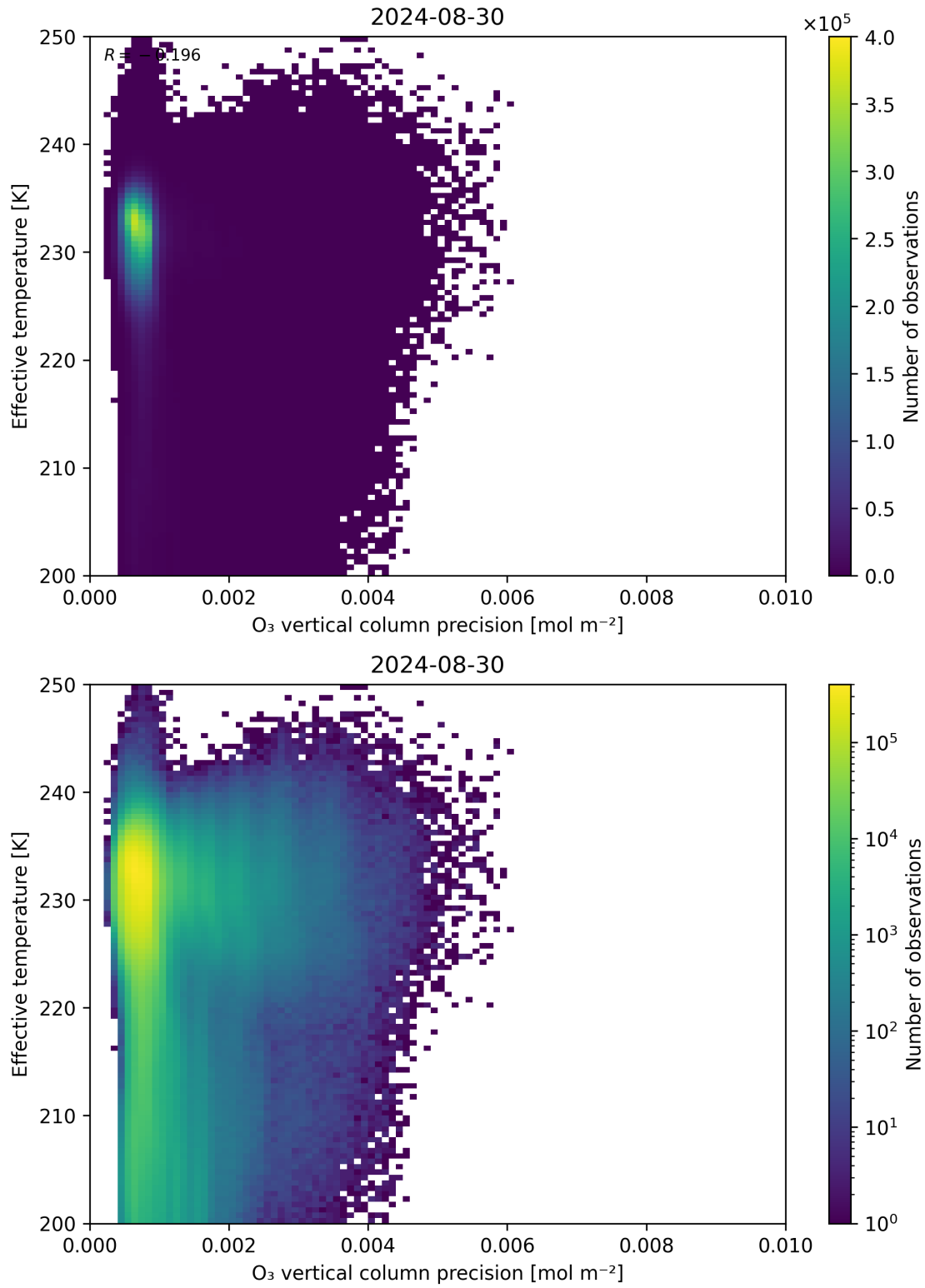
Figure 42: Scatter density plot of “O 3 vertical column precision” against “Effective temperature” for 2024-08-29 to 2024-08-31.
