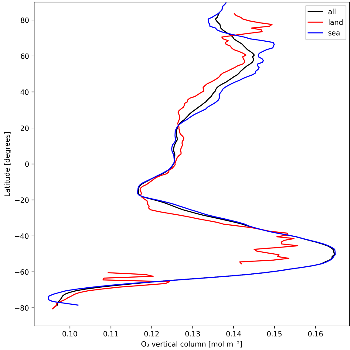
Figure 14: Zonal average of “O 3 vertical column” for 2024-08-29 to 2024-08-31.
