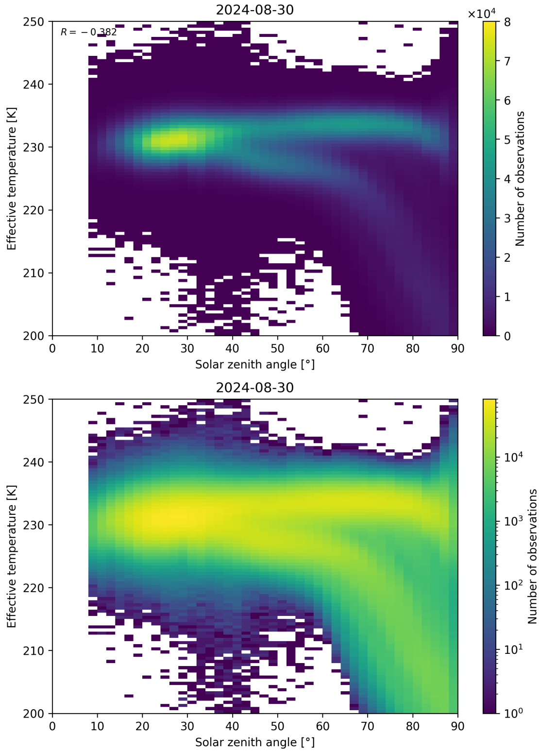
Figure 45: Scatter density plot of “Solar zenith angle” against “Effective temperature” for 2024-08-29 to 2024-08-31.
