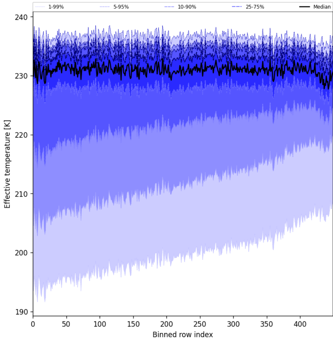
Figure 31: Along track statistics of “Effective temperature” for 2024-08-29 to 2024-08-31
