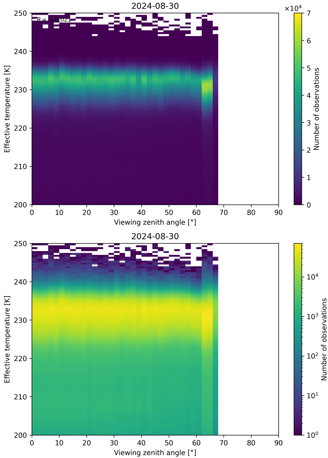
Figure 50: Scatter density plot of “Viewing zenith angle” against “Effective temperature” for 2024-08-29 to 2024-08-31.
