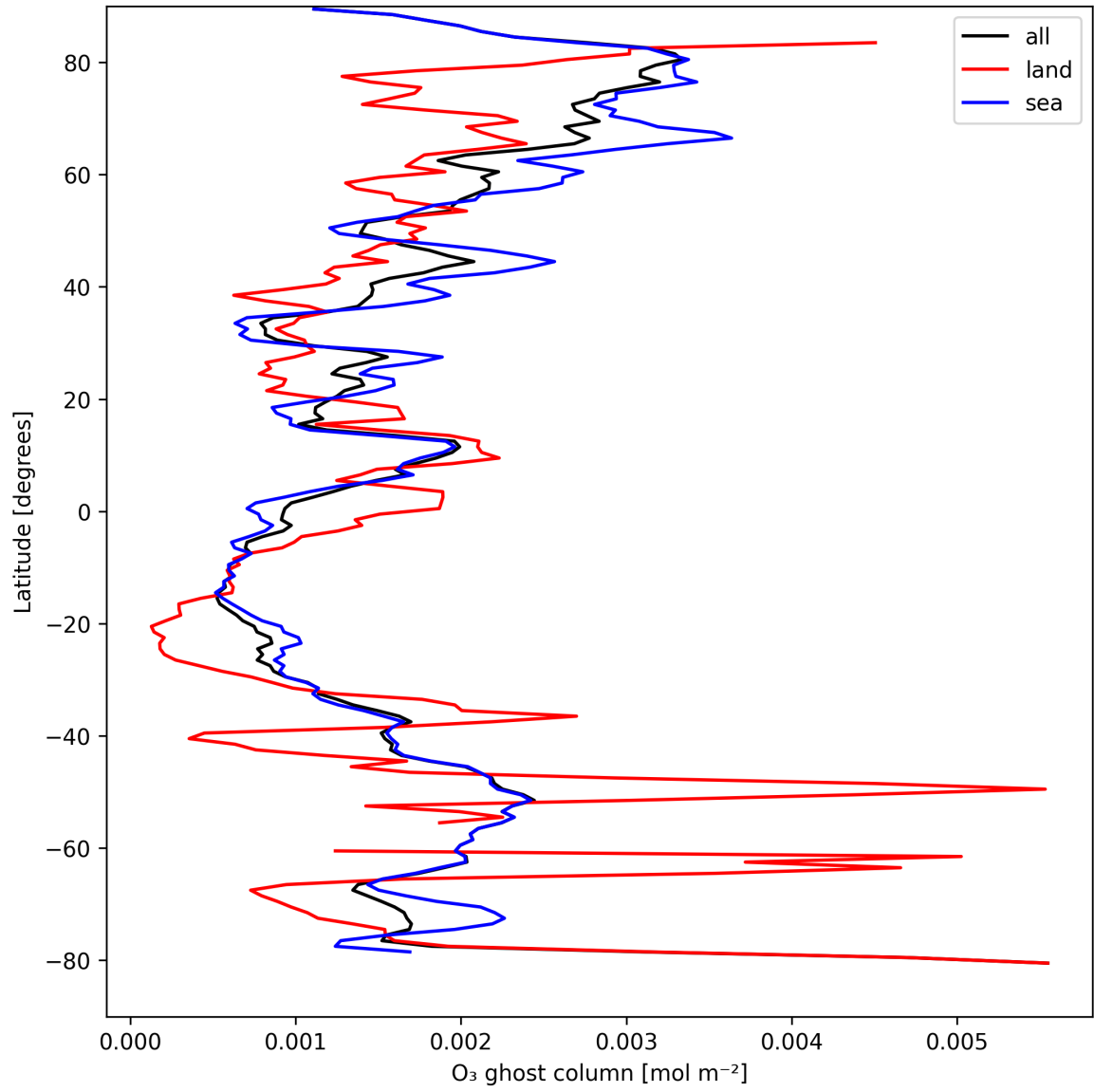
Figure 18: Zonal average of "O 3 ghost column" for 2024-08-29 to 2024-08-31.
