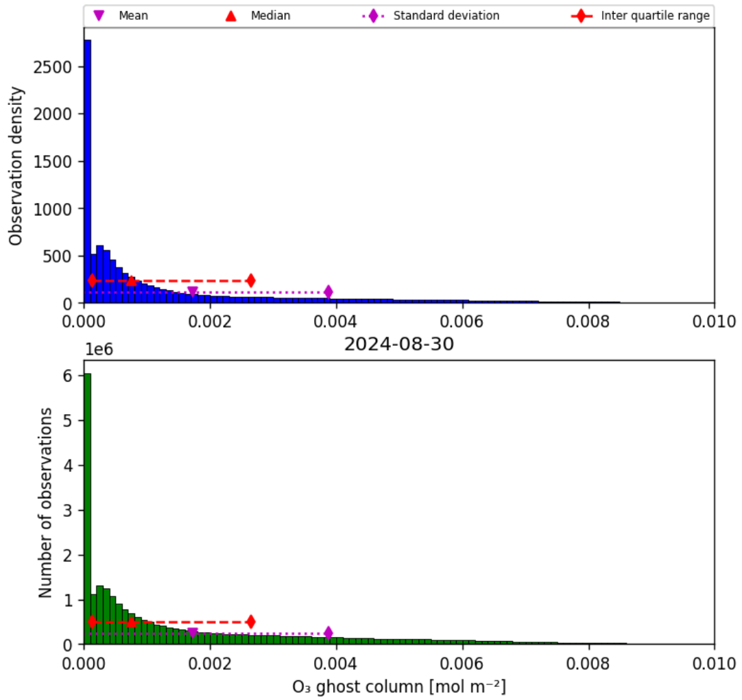
Figure 25: Histogram of “O 3 ghost column” for 2024-08-29 to 2024-08-31
