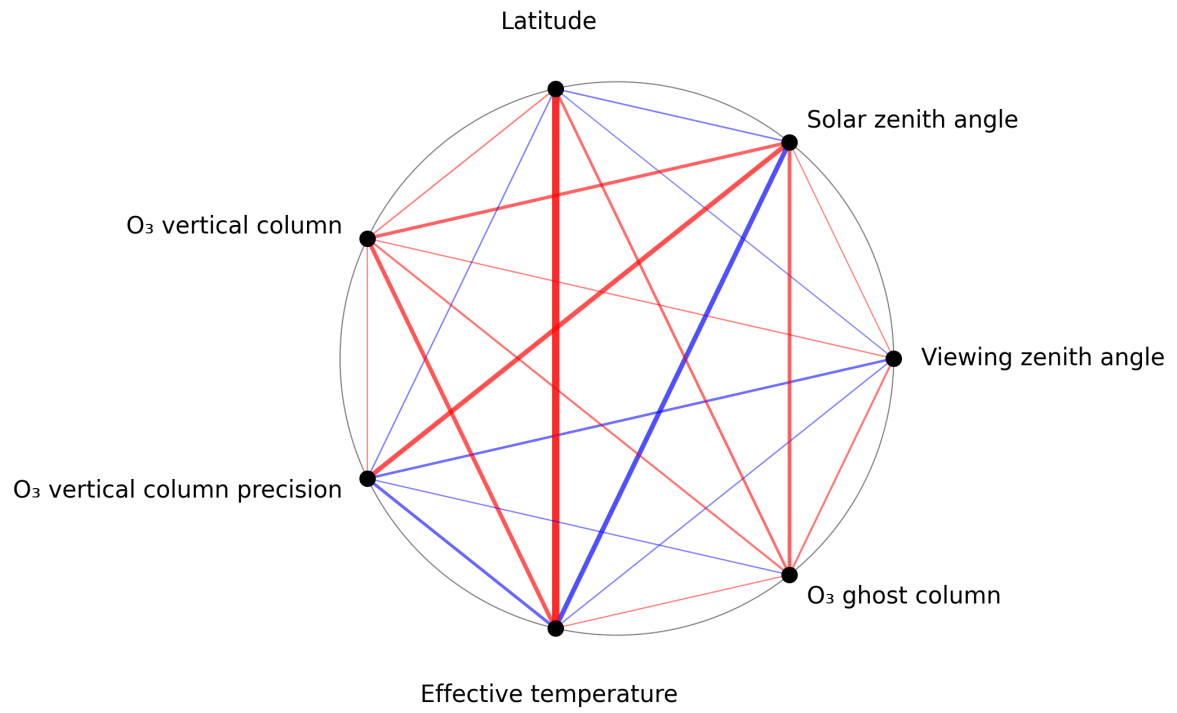
Figure 1: Map of correlation graph for 2024-08-29 to 2024-08-31.
