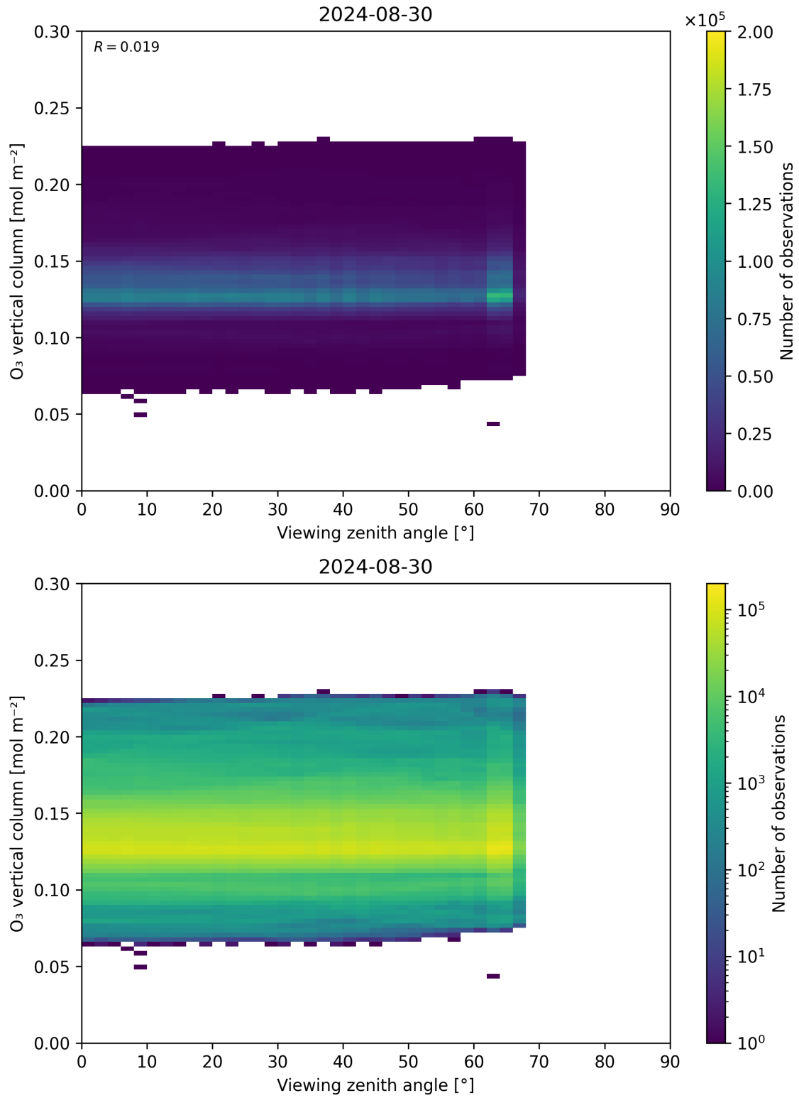
Figure 52: Scatter density plot of “Viewing zenith angle” against “O 3 vertical column” for 2024-08-29 to 2024-08-31.
