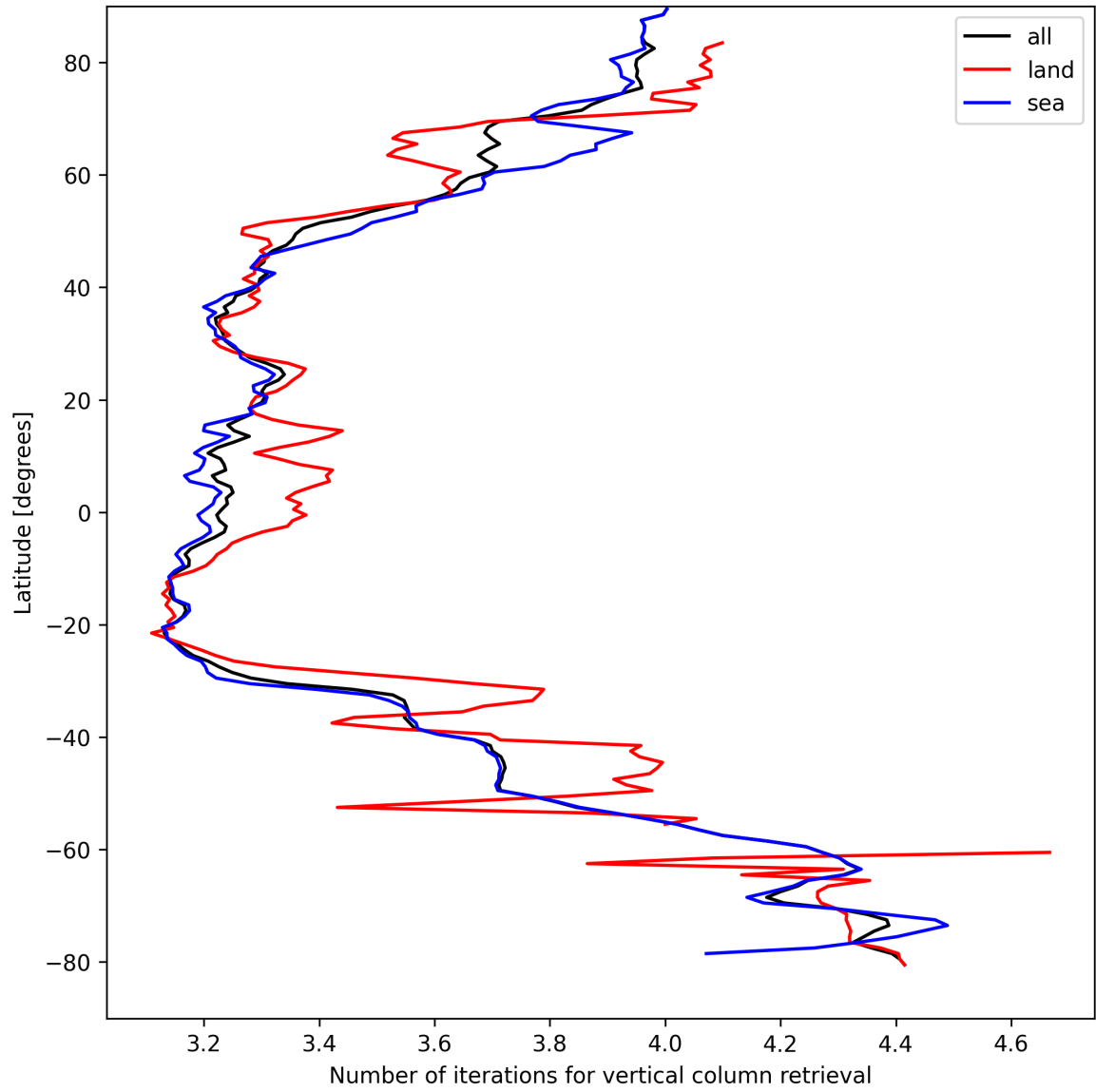
Figure 19: Zonal average of “Number of iterations for vertical column retrieval” for 2024-08-29 to 2024-08-31.
