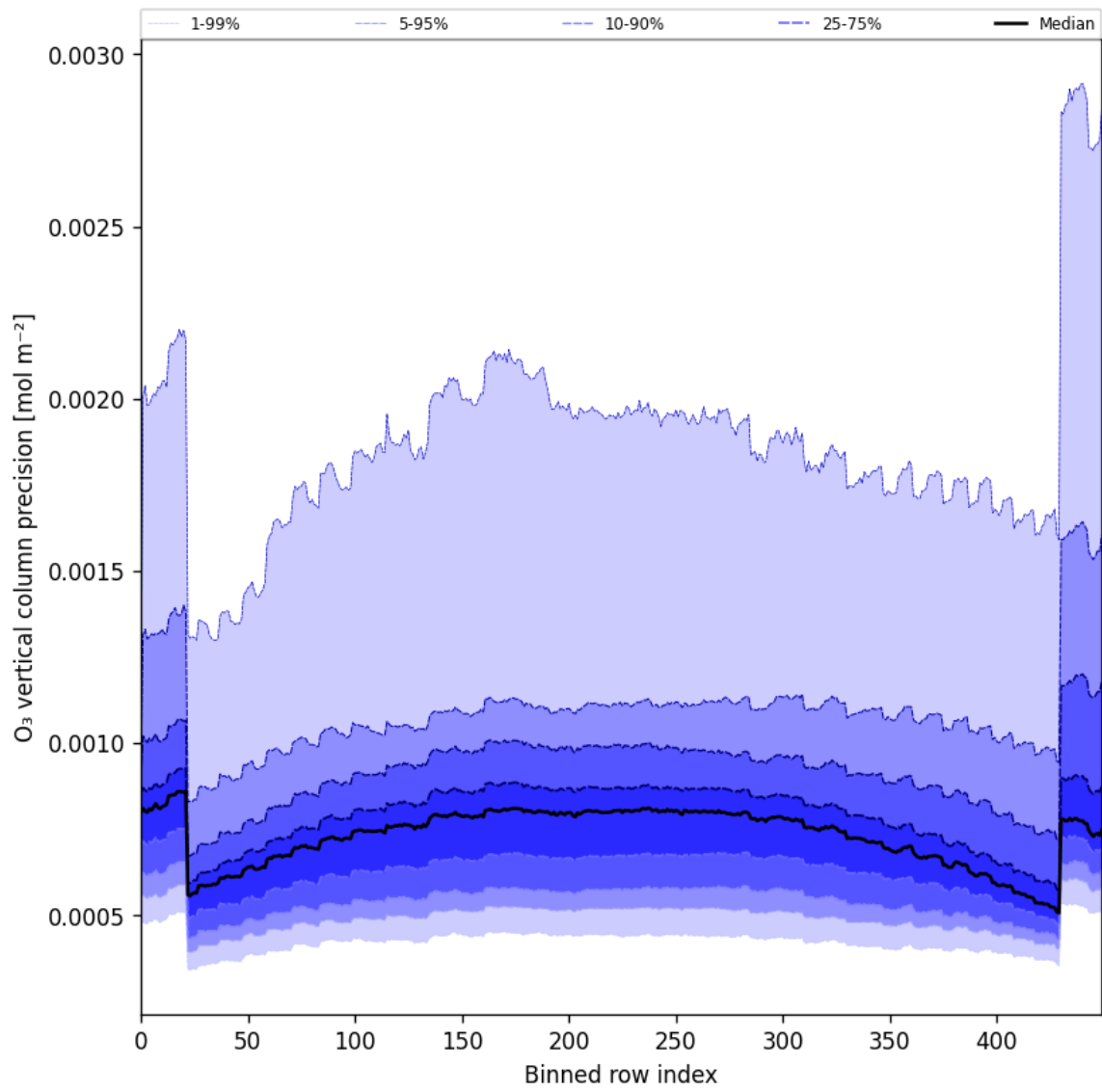
Figure 29: Along track statistics of “O 3 vertical column precision” for 2024-08-29 to 2024-08-31
