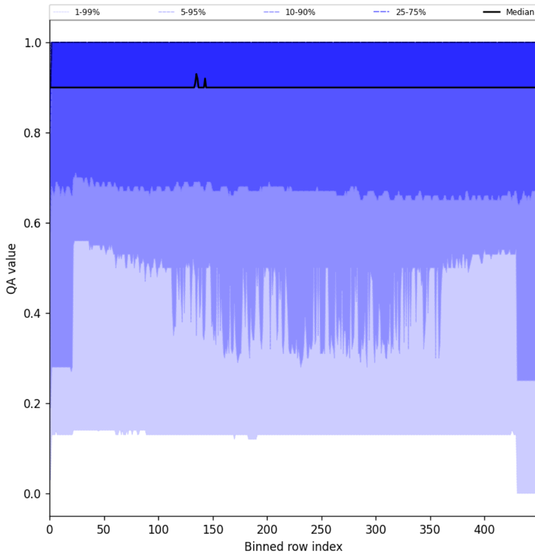
Figure 27: Along track statistics of “QA value” for 2024-08-29 to 2024-08-31
