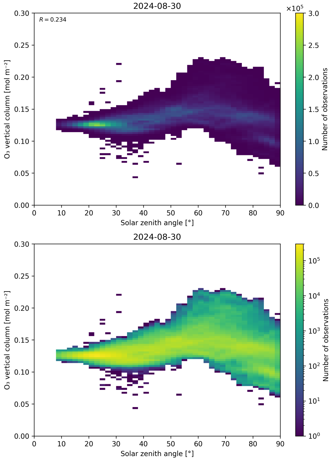
Figure 47: Scatter density plot of “Solar zenith angle” against “O 3 vertical column” for 2024-08-29 to 2024-08-31.
