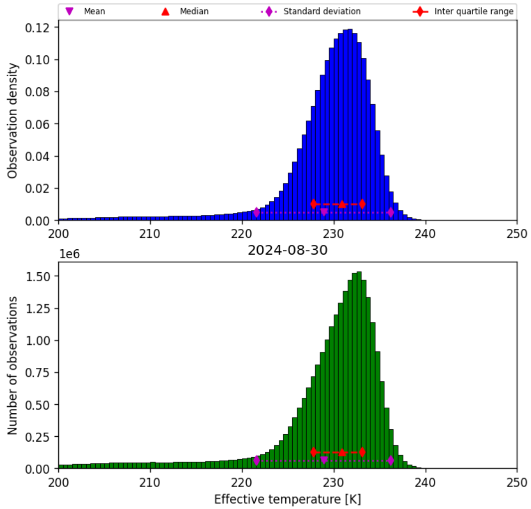
Figure 24: Histogram of “Effective temperature” for 2024-08-29 to 2024-08-31
