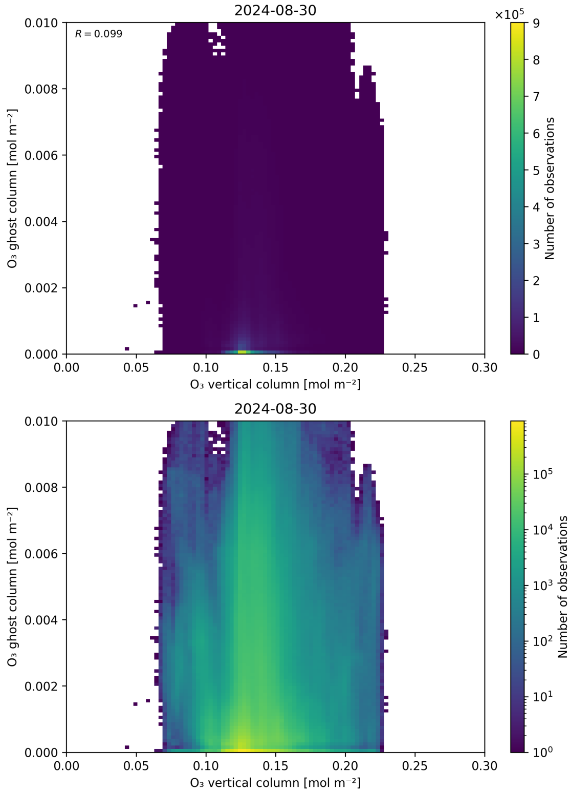
Figure 40: Scatter density plot of “O 3 vertical column” against “O 3 ghost column” for 2024-08-29 to 2024-08-31.
