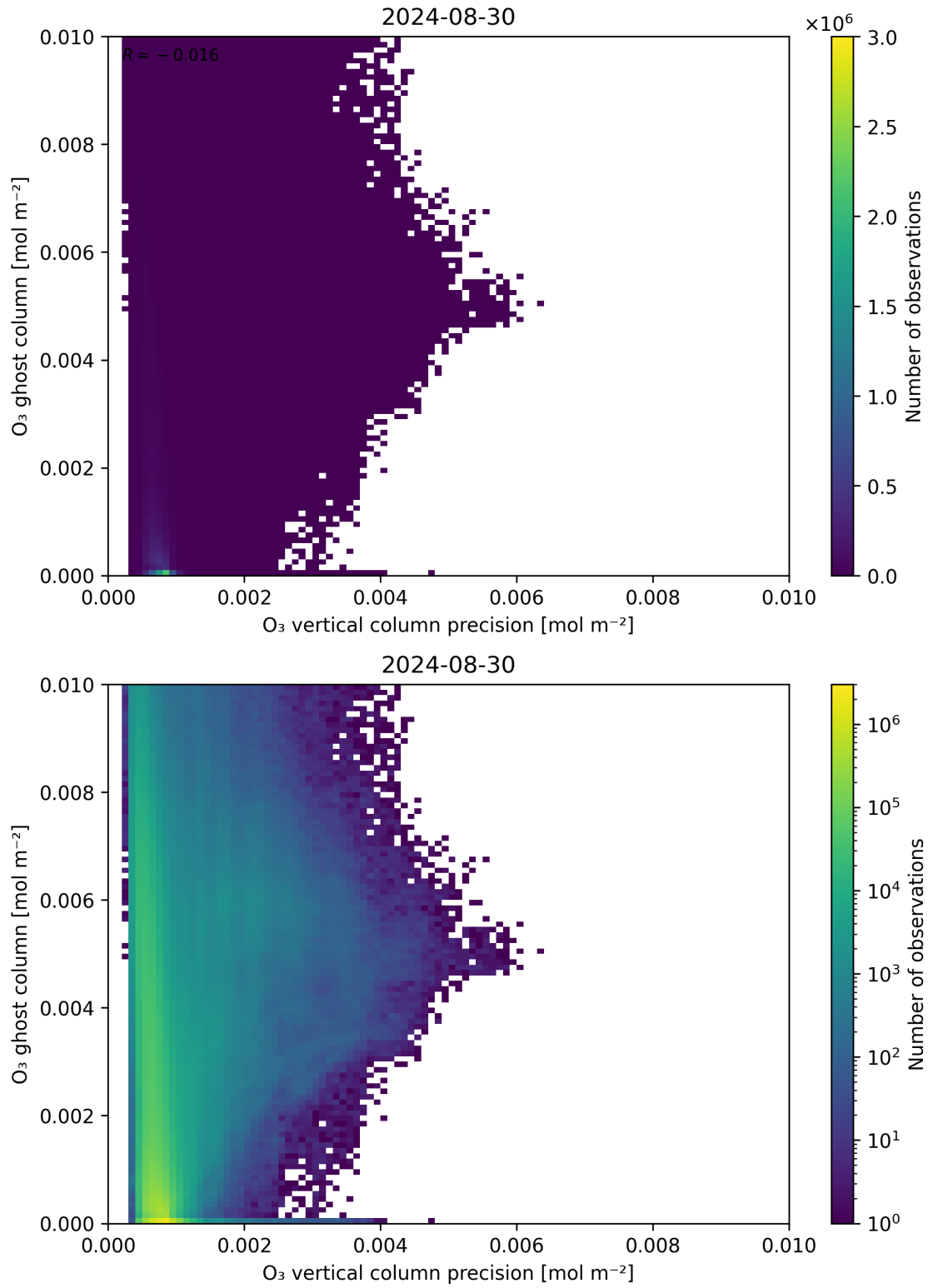
Figure 43: Scatter density plot of “ \text{O}_3 vertical column precision” against “ \text{O}_3 ghost column” for 2024-08-29 to 2024-08-31.
