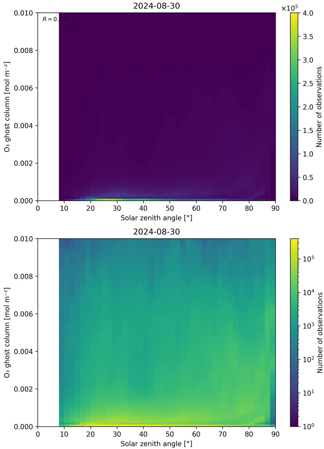
Figure 46: Scatter density plot of “Solar zenith angle” against “O 3 ghost column” for 2024-08-29 to 2024-08-31.
