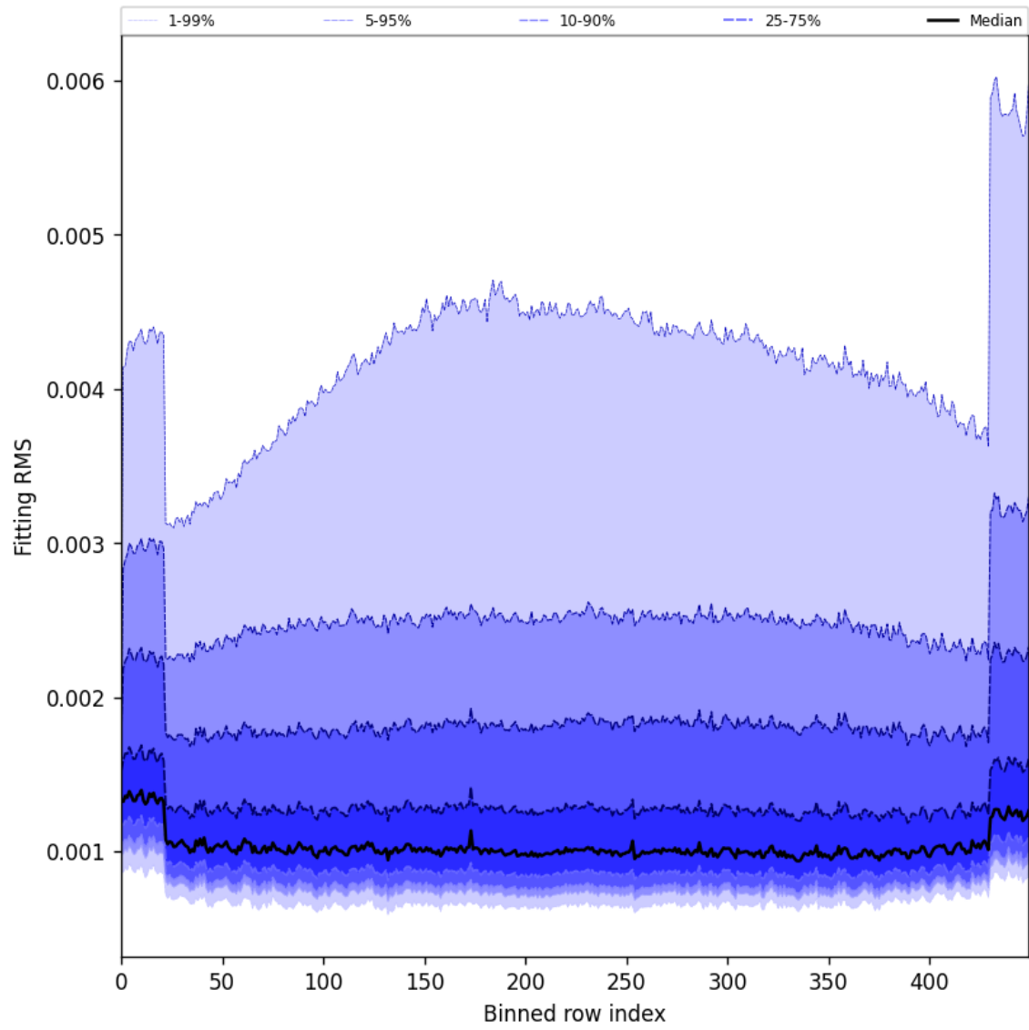
Figure 30: Along track statistics of “Fitting RMS” for 2024-08-29 to 2024-08-31
