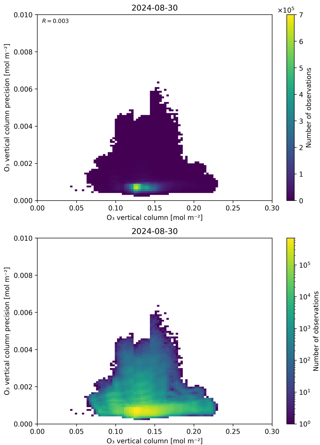
Figure 41: Scatter density plot of “O 3 vertical column” against “O 3 vertical column precision” for 2024-08-29 to 2024-08-31.
