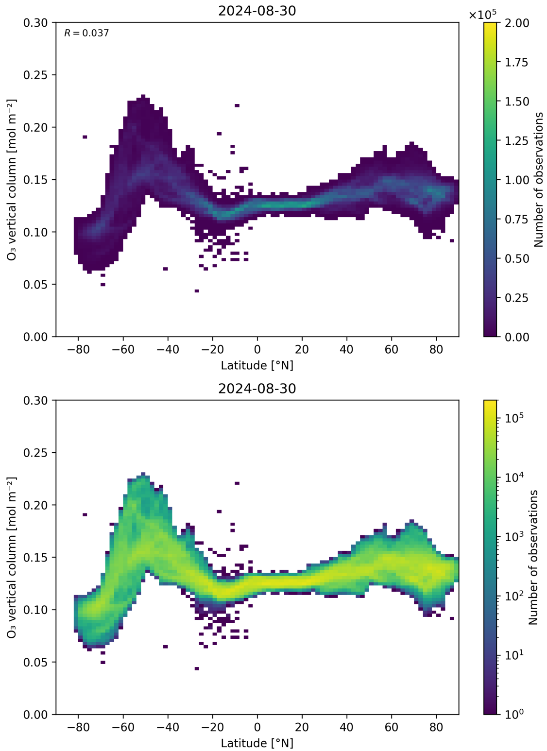
Figure 36: Scatter density plot of “Latitude” against “O 3 vertical column” for 2024-08-29 to 2024-08-31.
