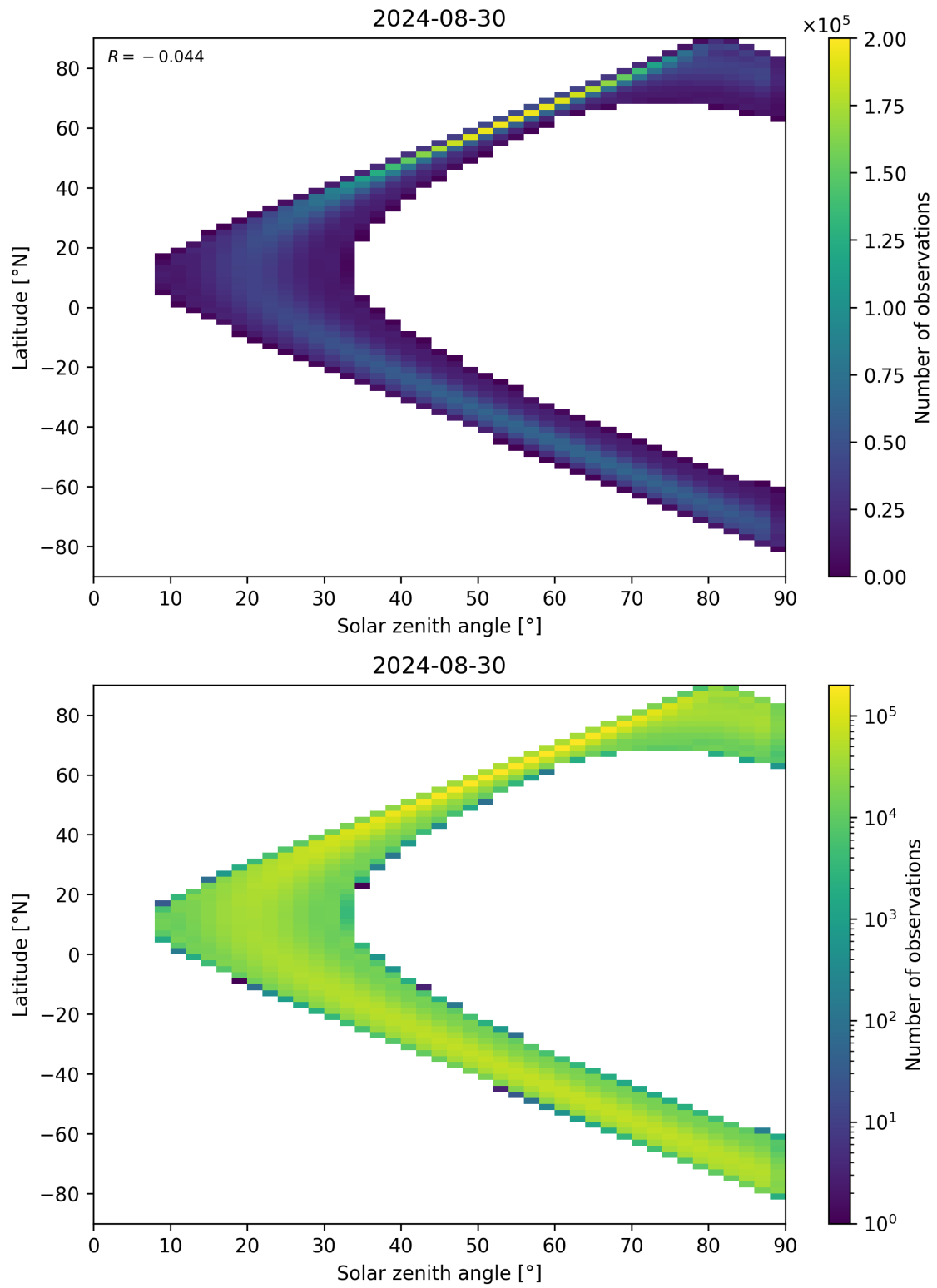
Figure 44: Scatter density plot of “Solar zenith angle” against “Latitude” for 2024-08-29 to 2024-08-31.
