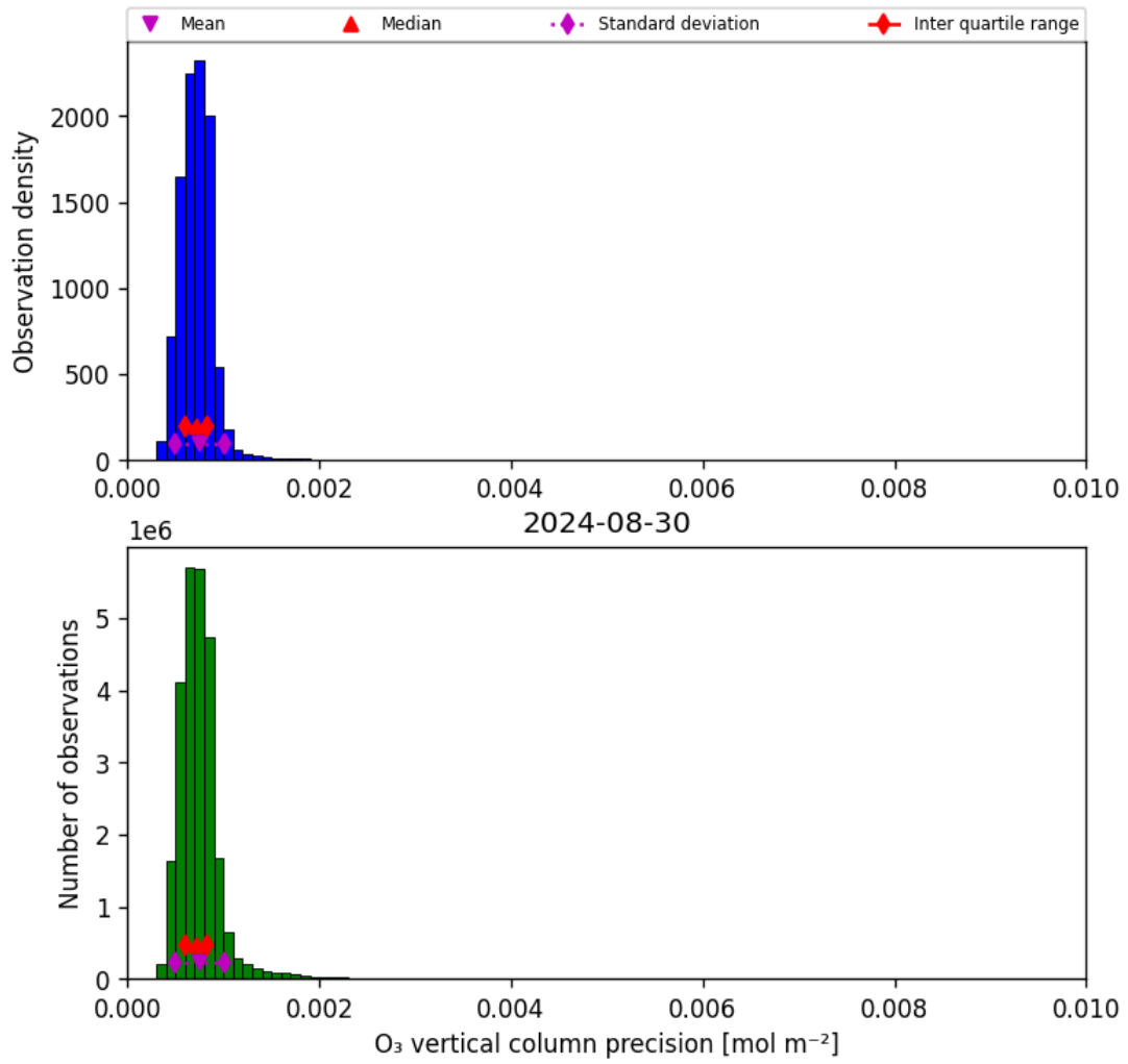
Figure 22: Histogram of “O 3 vertical column precision” for 2024-08-29 to 2024-08-31
