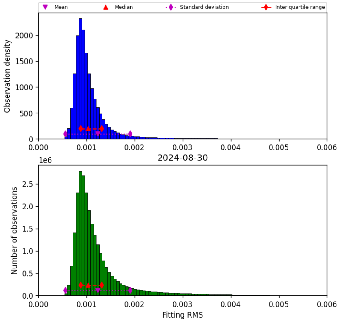
Figure 23: Histogram of “Fitting RMS” for 2024-08-29 to 2024-08-31
