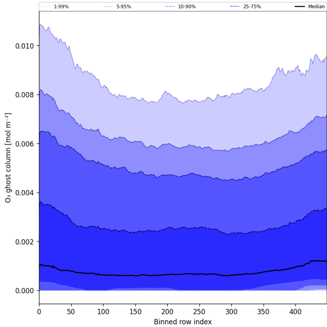
Figure 32: Along track statistics of “O 3 ghost column” for 2024-08-29 to 2024-08-31
