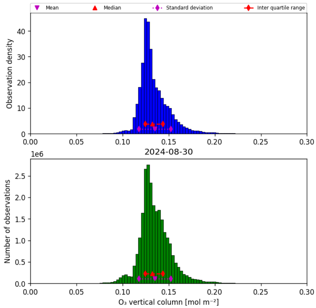
Figure 21: Histogram of “O 3 vertical column” for 2024-08-29 to 2024-08-31
