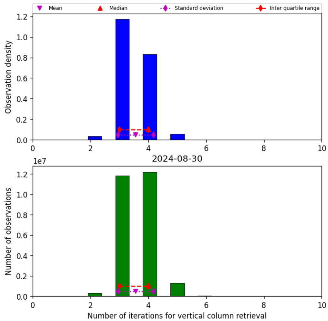
Figure 26: Histogram of “Number of iterations for vertical column retrieval” for 2024-08-29 to 2024-08-31
