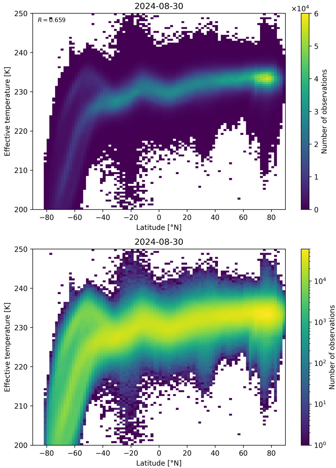
Figure 34: Scatter density plot of “Latitude” against “Effective temperature” for 2024-08-29 to 2024-08-31.
