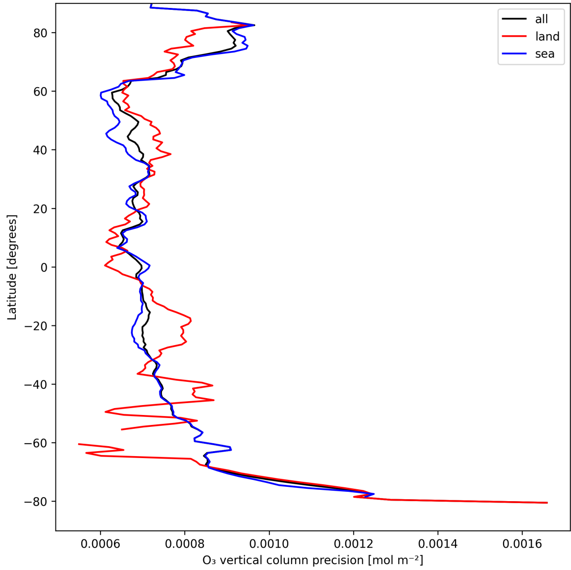
Figure 15: Zonal average of “O 3 vertical column precision” for 2024-08-29 to 2024-08-31.
