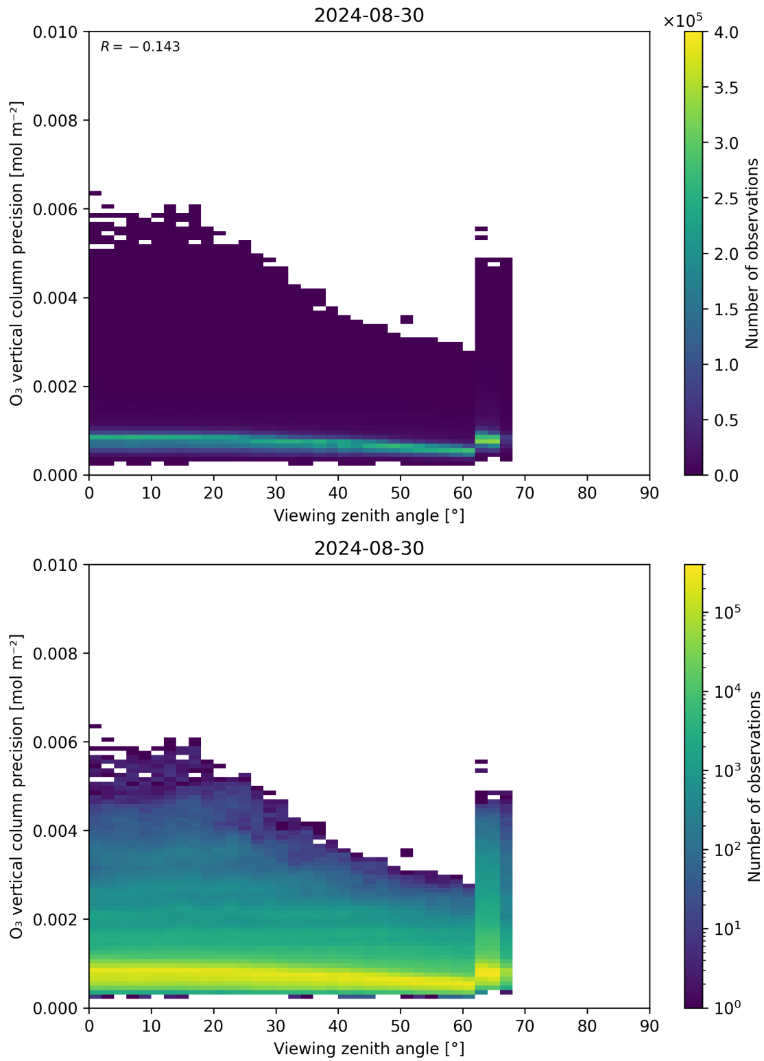
Figure 53: Scatter density plot of “Viewing zenith angle” against “O 3 vertical column precision” for 2024-08-29 to 2024-08-31.
