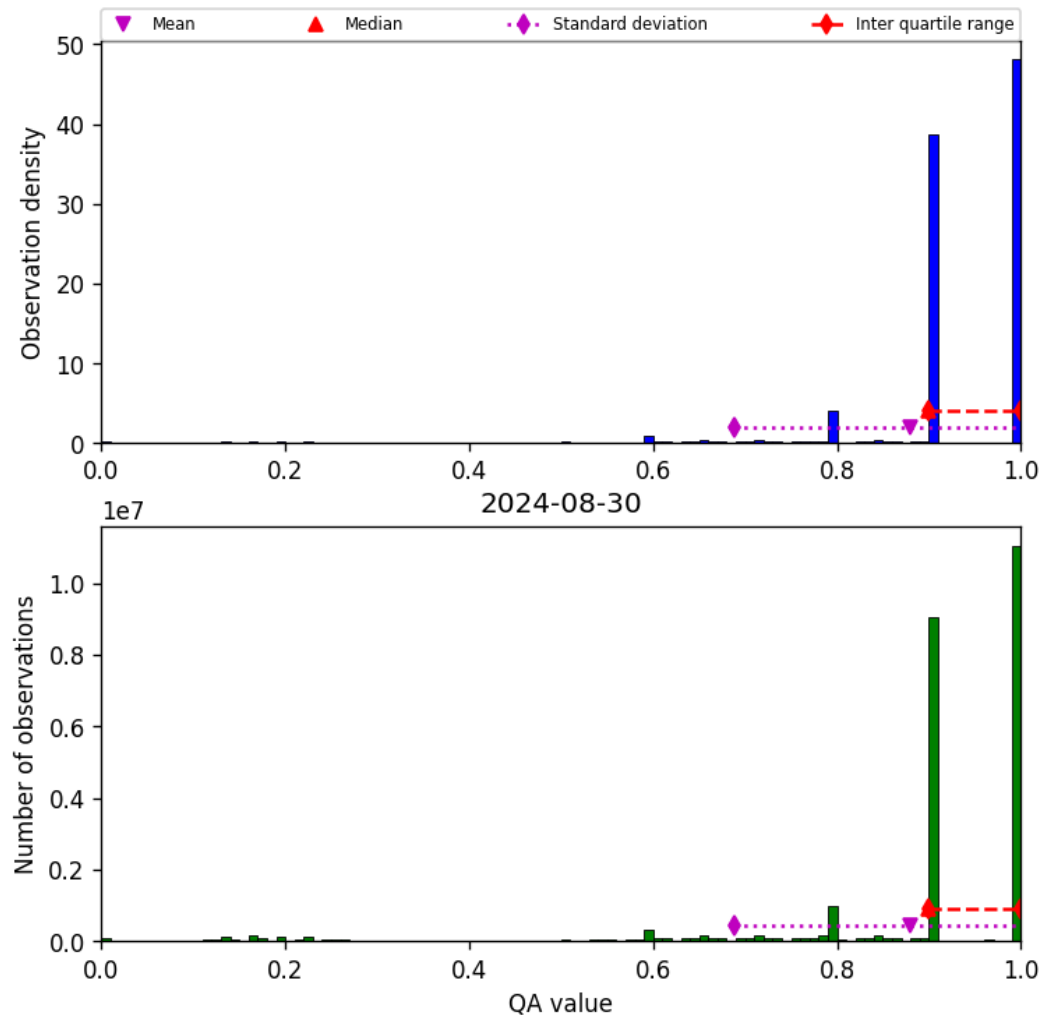
Figure 20: Histogram of “QA value” for 2024-08-29 to 2024-08-31
