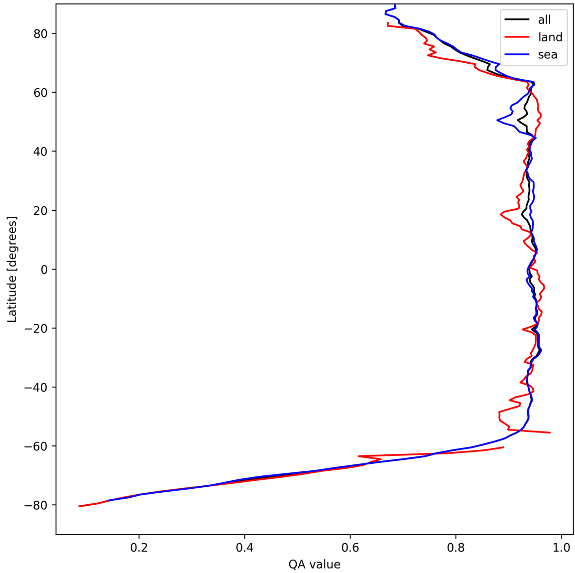
Figure 13: Zonal average of “QA value” for 2024-08-29 to 2024-08-31.
