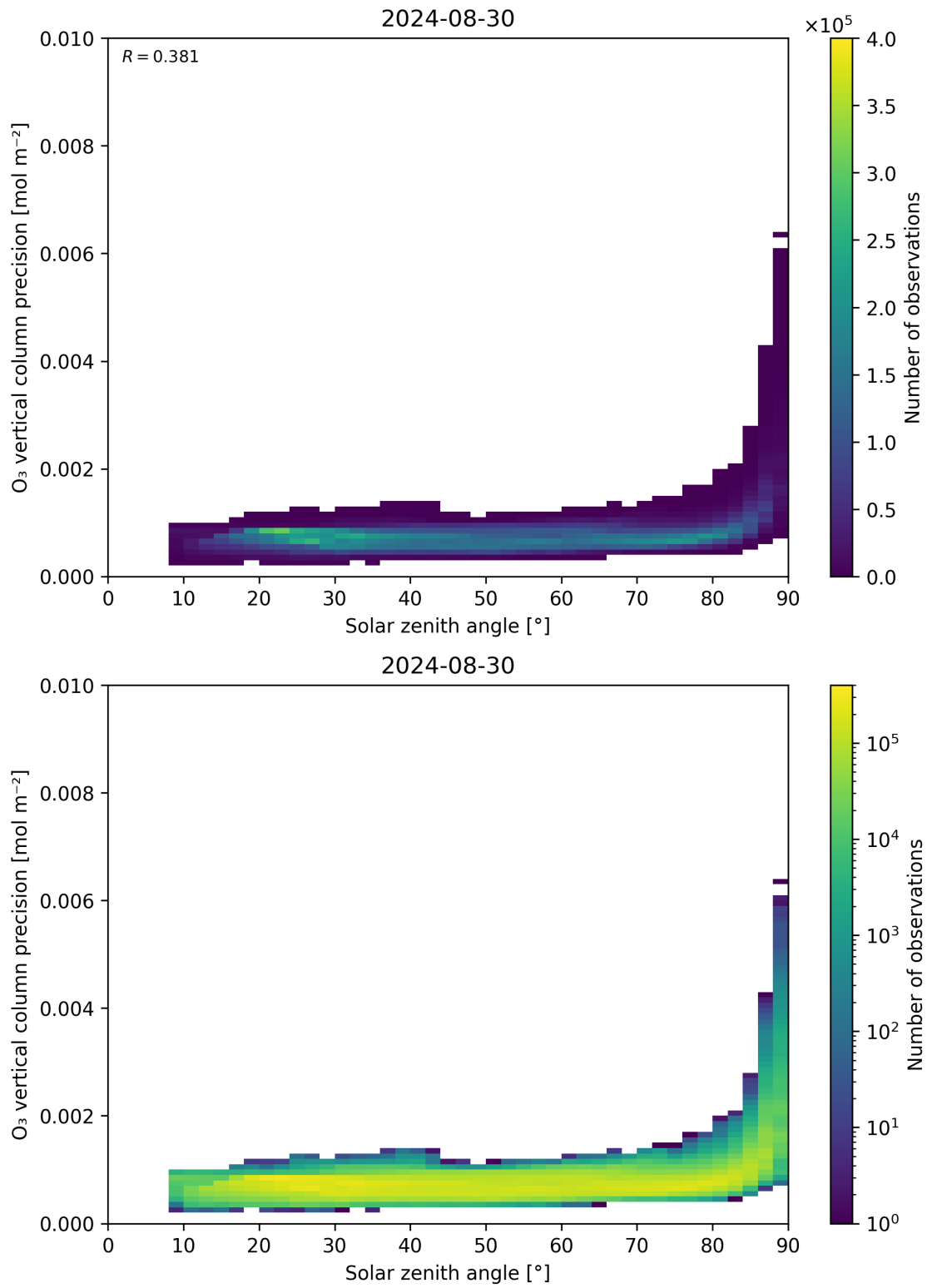
Figure 48: Scatter density plot of “Solar zenith angle” against “O 3 vertical column precision” for 2024-08-29 to 2024-08-31.
