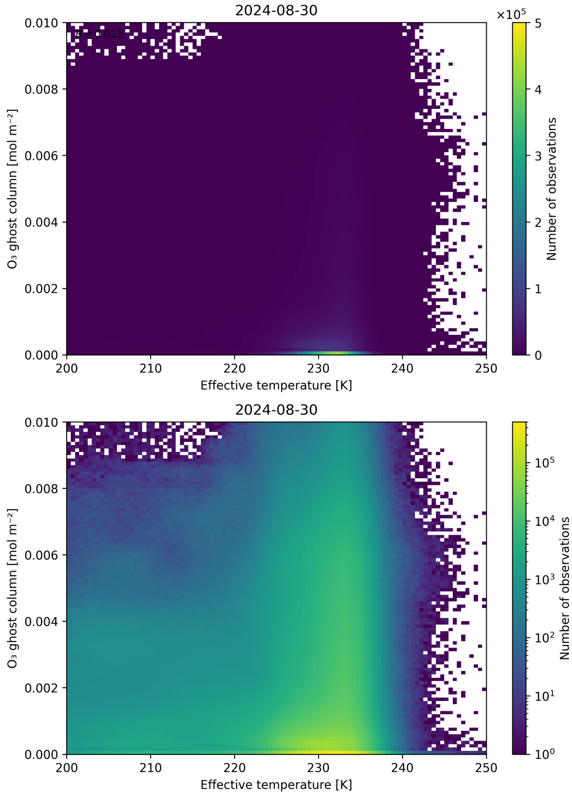
Figure 38: Scatter density plot of “Effective temperature” against “O 3 ghost column” for 2024-08-29 to 2024-08-31.
