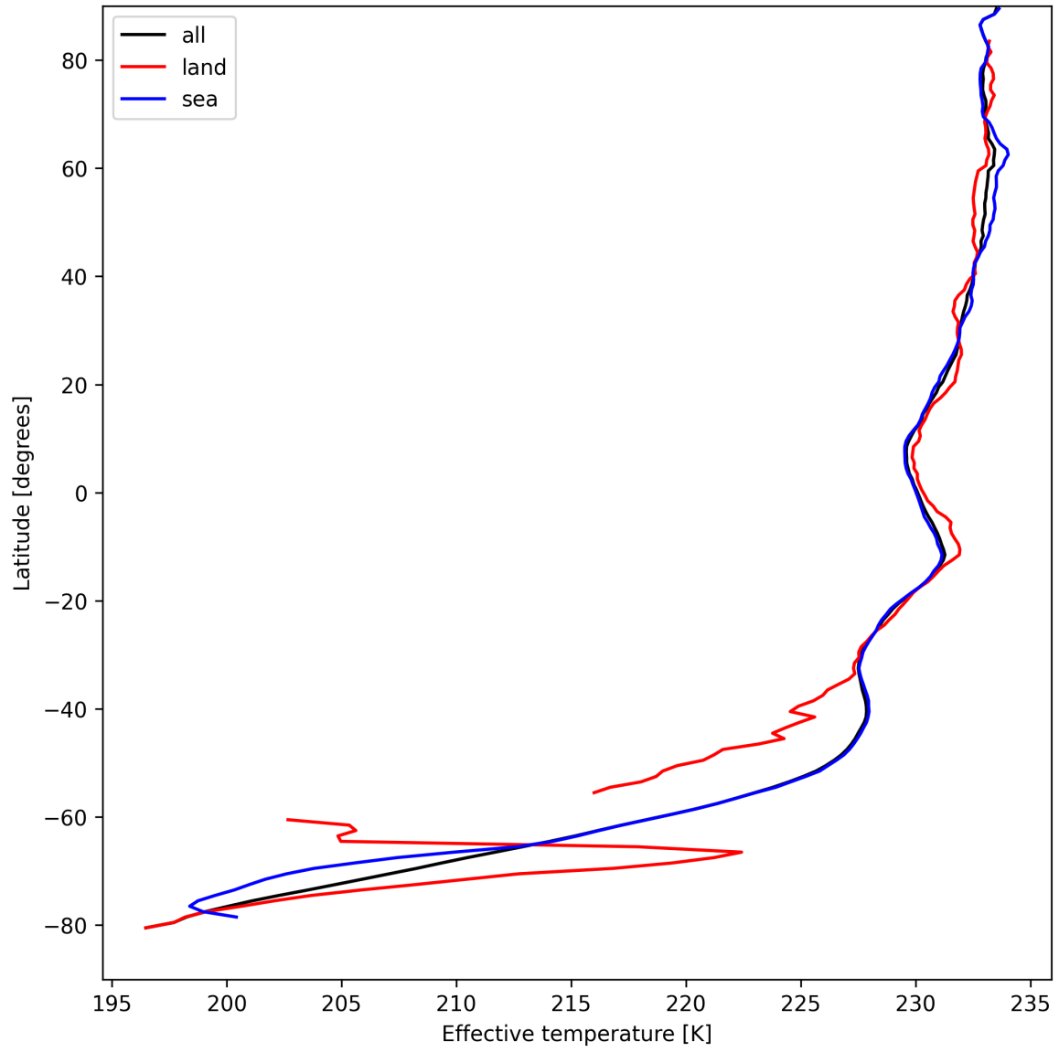
Figure 17: Zonal average of "Effective temperature" for 2024-08-29 to 2024-08-31.
