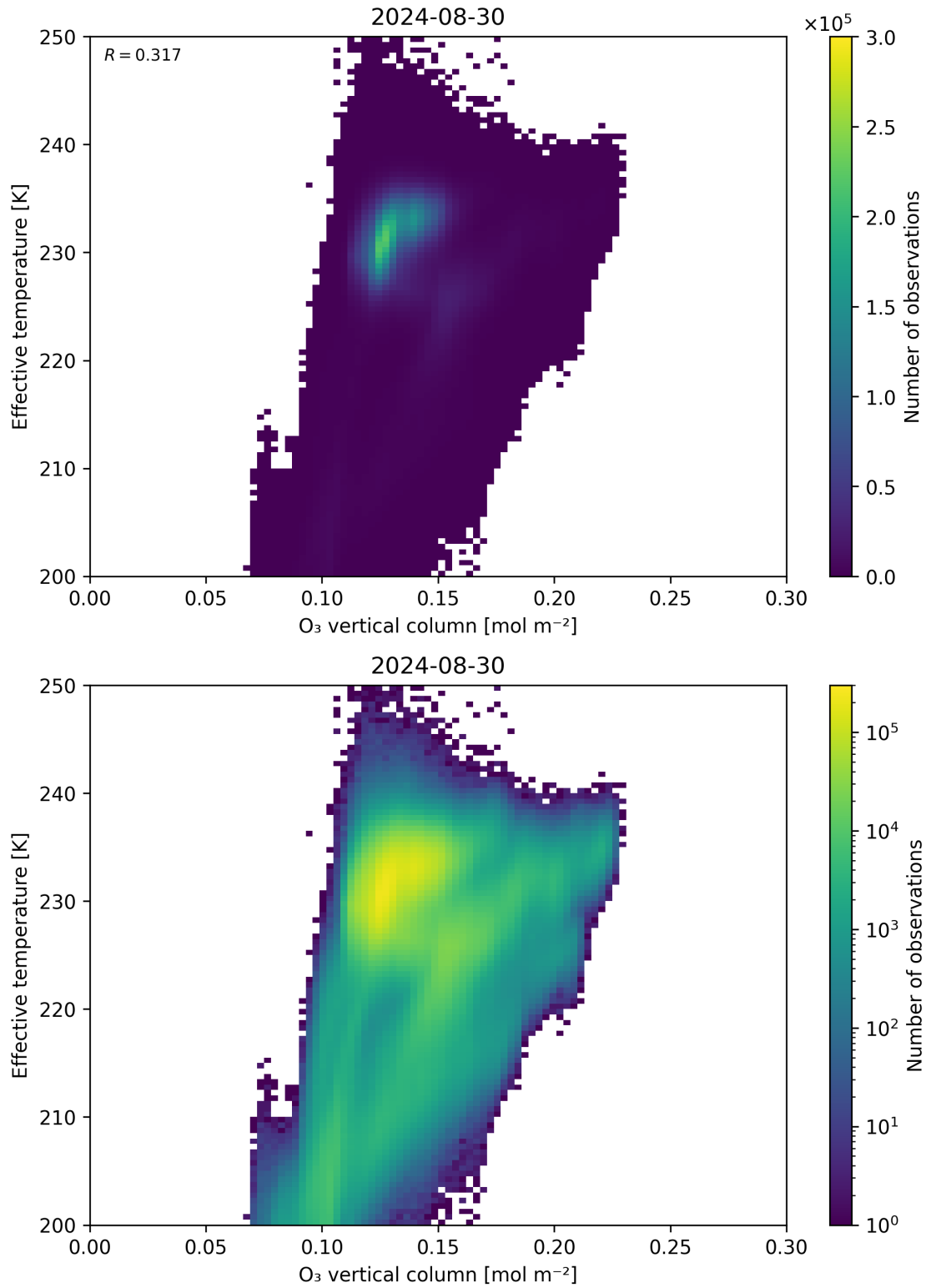
Figure 39: Scatter density plot of “O 3 vertical column” against “Effective temperature” for 2024-08-29 to 2024-08-31.
