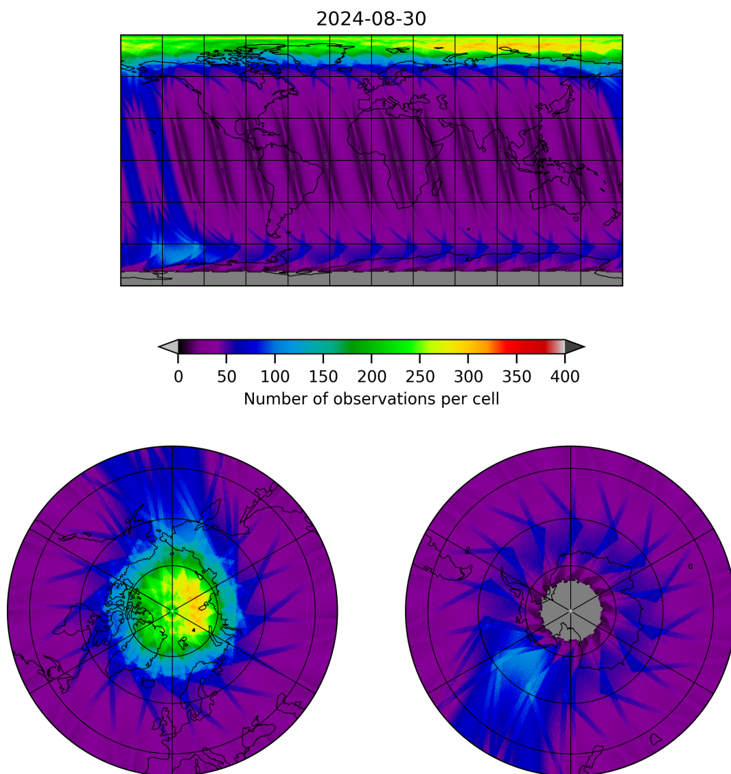
Figure 12: Map of the number of observations for 2024-08-29 to 2024-08-31
