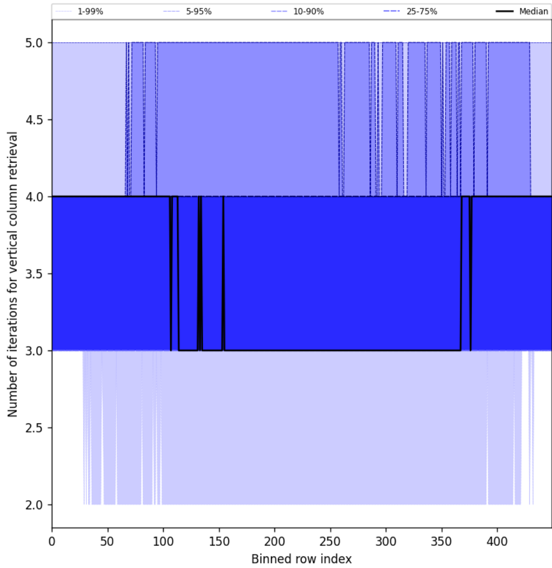
Figure 33: Along track statistics of “Number of iterations for vertical column retrieval” for 2024-08-29 to 2024-08-31
