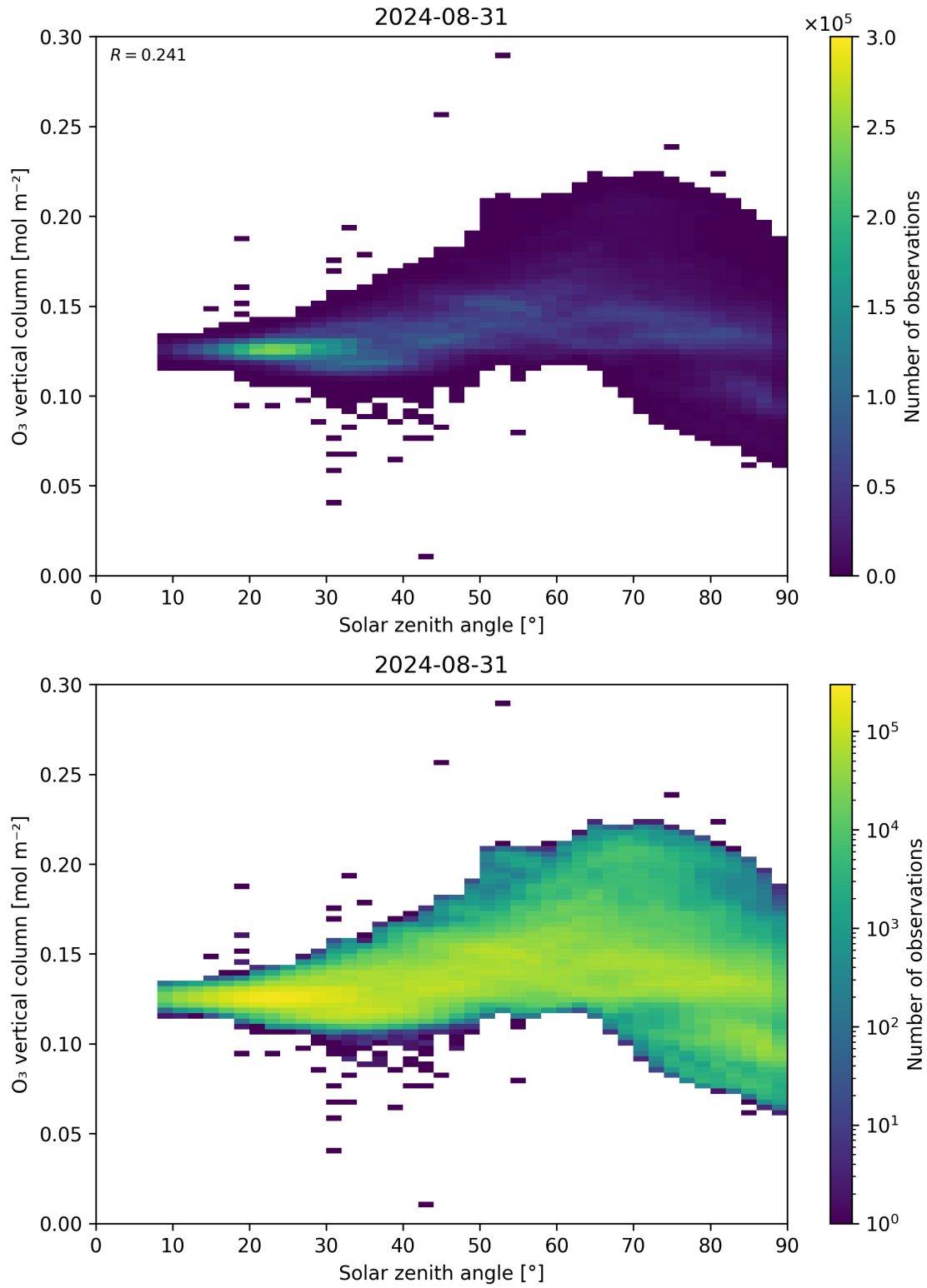
Figure 47: Scatter density plot of “Solar zenith angle” against “O 3 vertical column” for 2024-08-30 to 2024-09-01.
