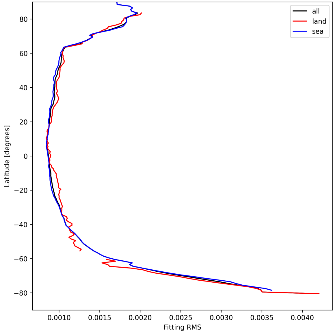
Figure 16: Zonal average of “Fitting RMS” for 2024-08-30 to 2024-09-01.
