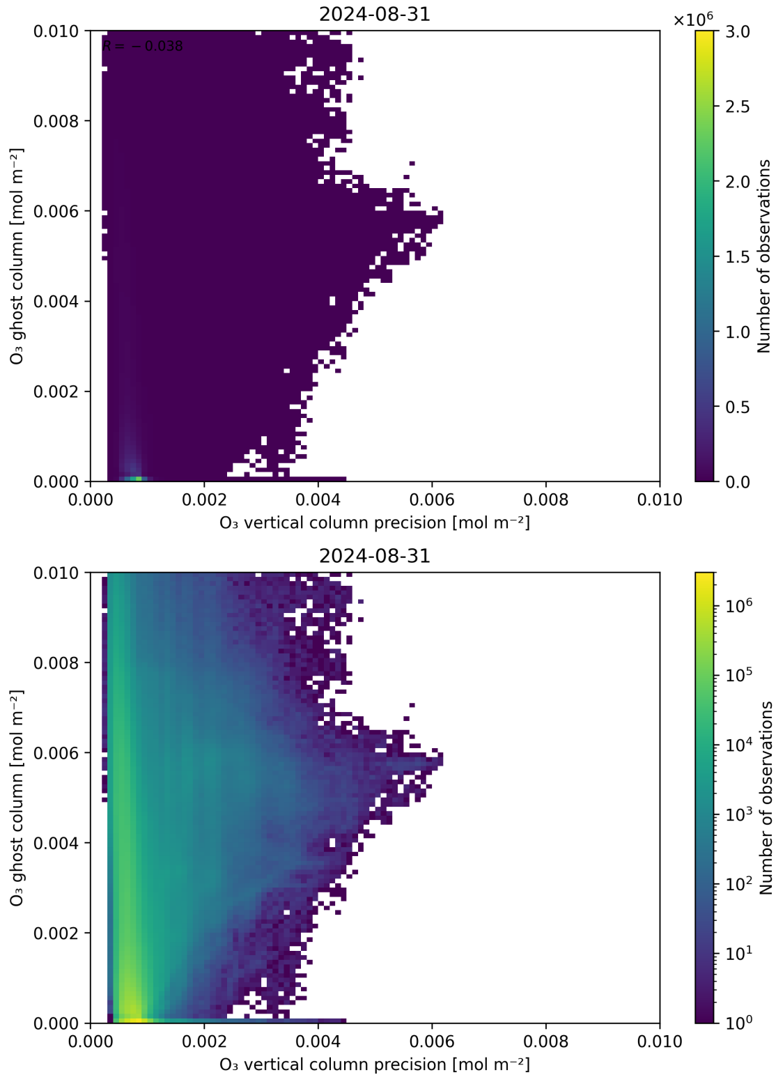
Figure 43: Scatter density plot of “ \text{O}_3 vertical column precision” against “ \text{O}_3 ghost column” for 2024-08-30 to 2024-09-01.
