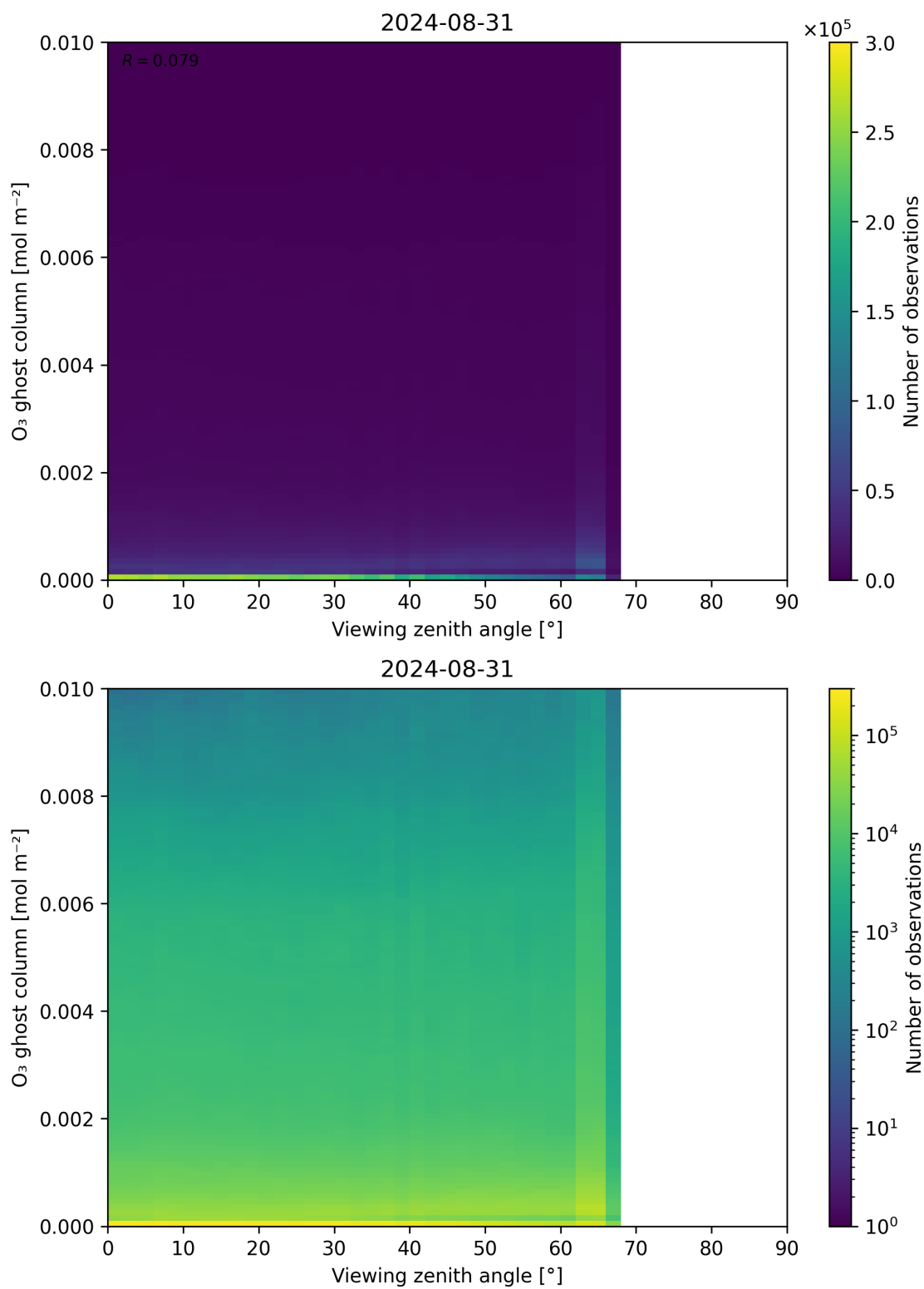
Figure 51: Scatter density plot of “Viewing zenith angle” against “O 3 ghost column” for 2024-08-30 to 2024-09-01.
