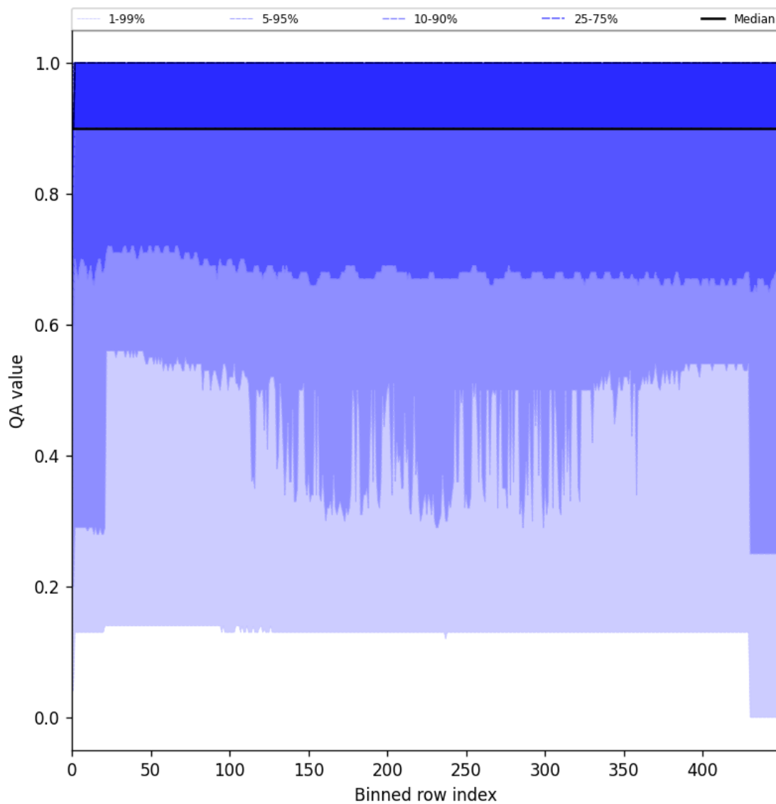
Figure 27: Along track statistics of “QA value” for 2024-08-30 to 2024-09-01
