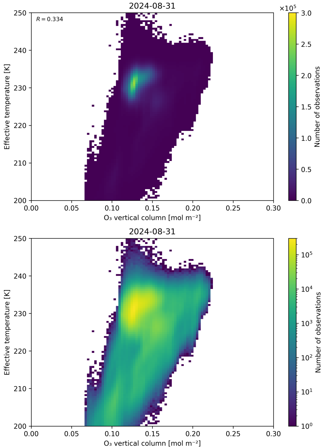
Figure 39: Scatter density plot of “O 3 vertical column” against “Effective temperature” for 2024-08-30 to 2024-09-01.
