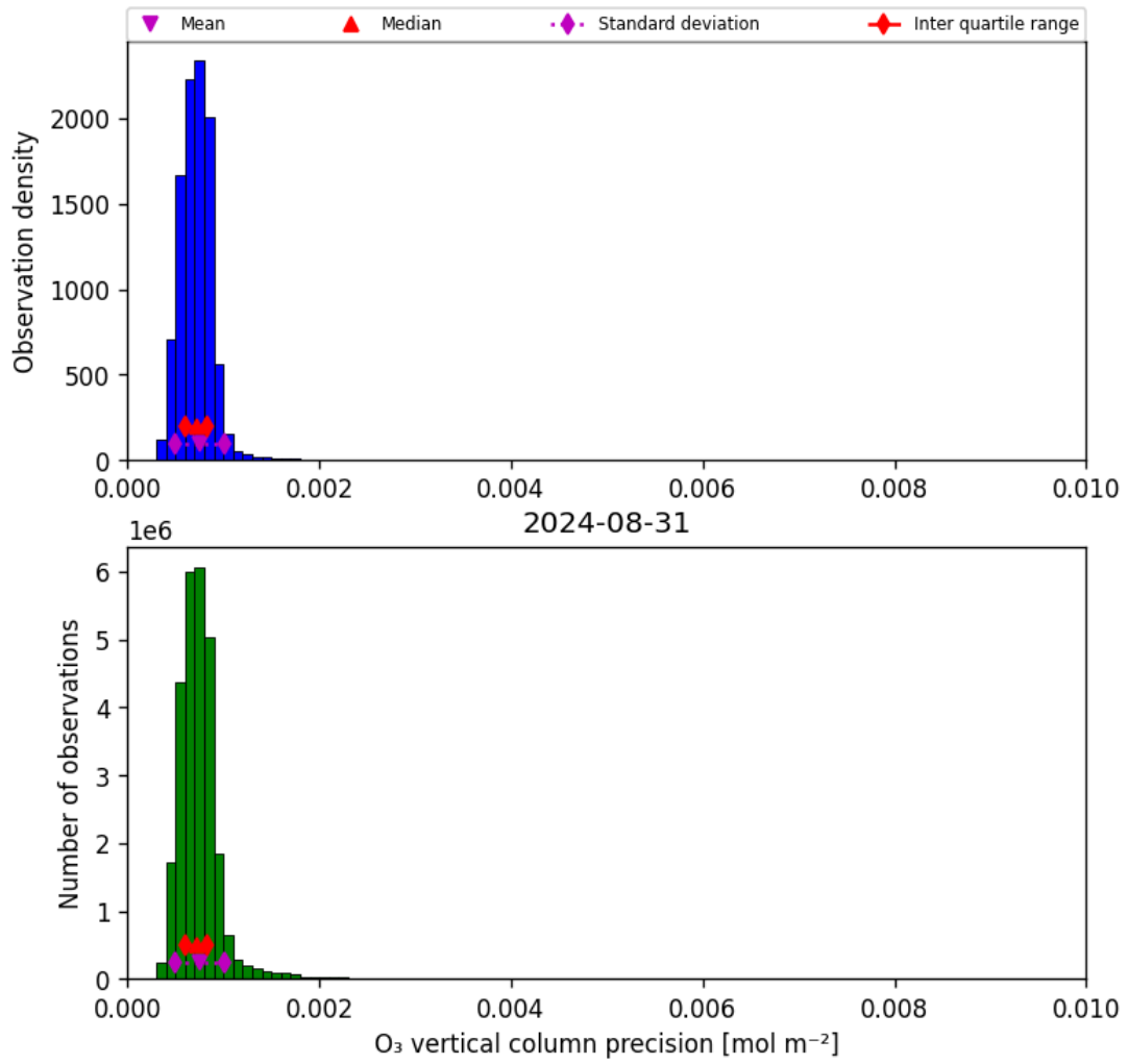
Figure 22: Histogram of “O 3 vertical column precision” for 2024-08-30 to 2024-09-01
