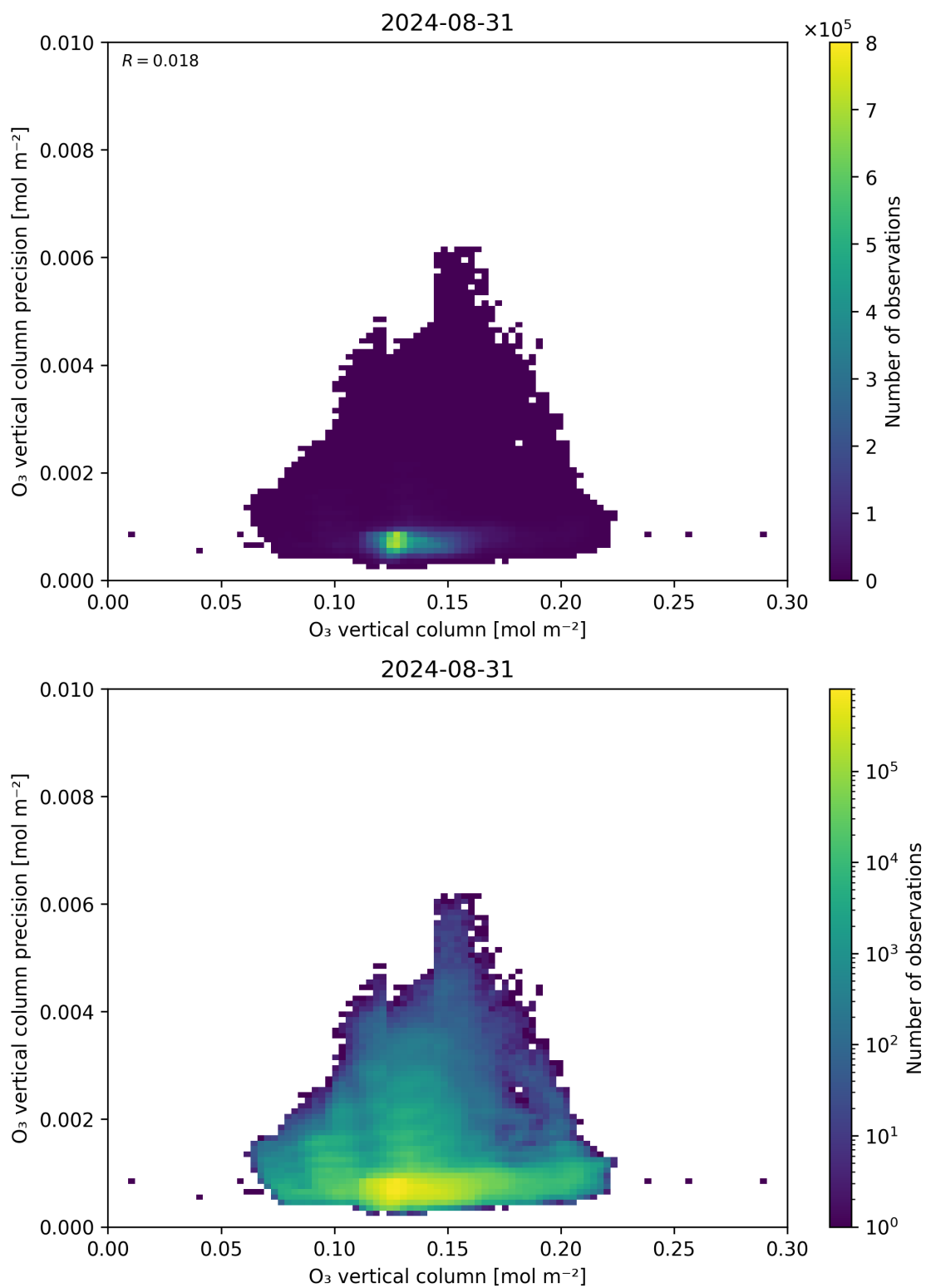
Figure 41: Scatter density plot of “O 3 vertical column” against “O 3 vertical column precision” for 2024-08-30 to 2024-09-01.
