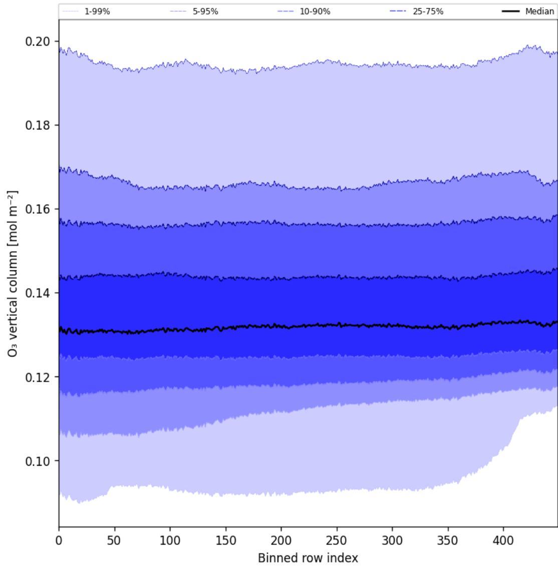
Figure 28: Along track statistics of “O 3 vertical column” for 2024-08-30 to 2024-09-01
