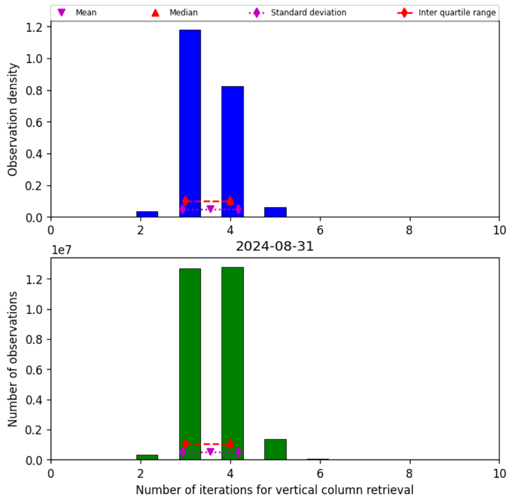
Figure 26: Histogram of “Number of iterations for vertical column retrieval” for 2024-08-30 to 2024-09-01
