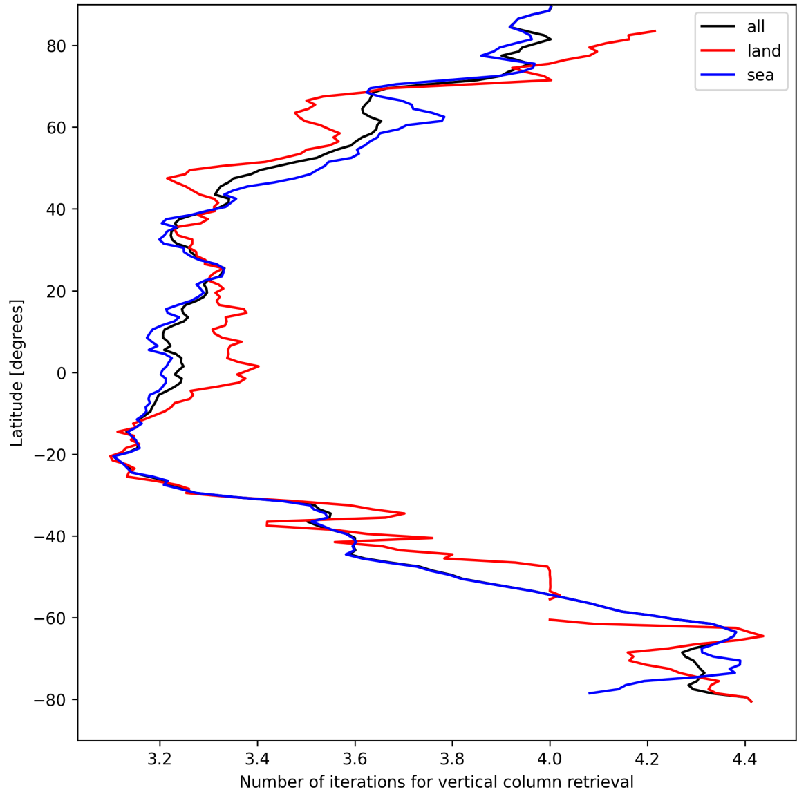
Figure 19: Zonal average of “Number of iterations for vertical column retrieval” for 2024-08-30 to 2024-09-01.
