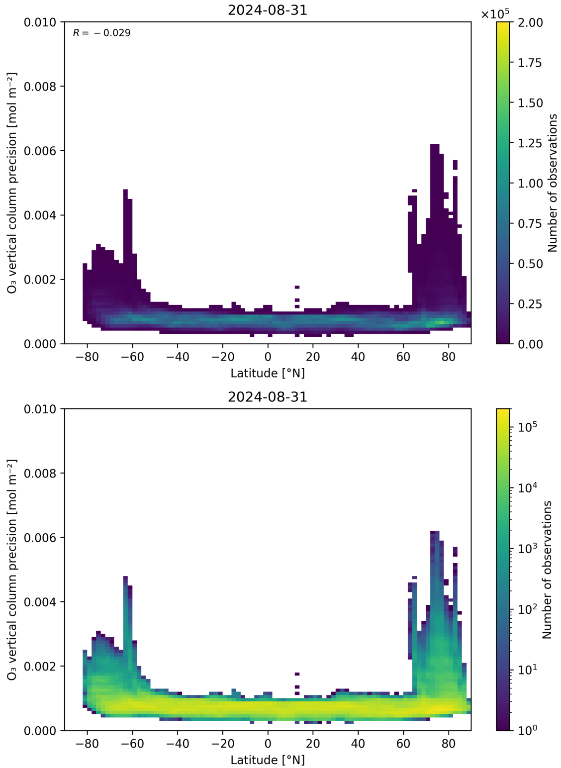
Figure 37: Scatter density plot of “Latitude” against “O 3 vertical column precision” for 2024-08-30 to 2024-09-01.
