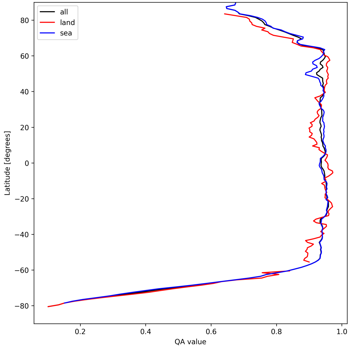
Figure 13: Zonal average of “QA value” for 2024-08-30 to 2024-09-01.
