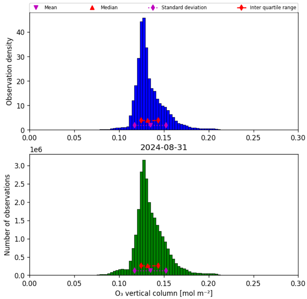
Figure 21: Histogram of “O 3 vertical column” for 2024-08-30 to 2024-09-01
