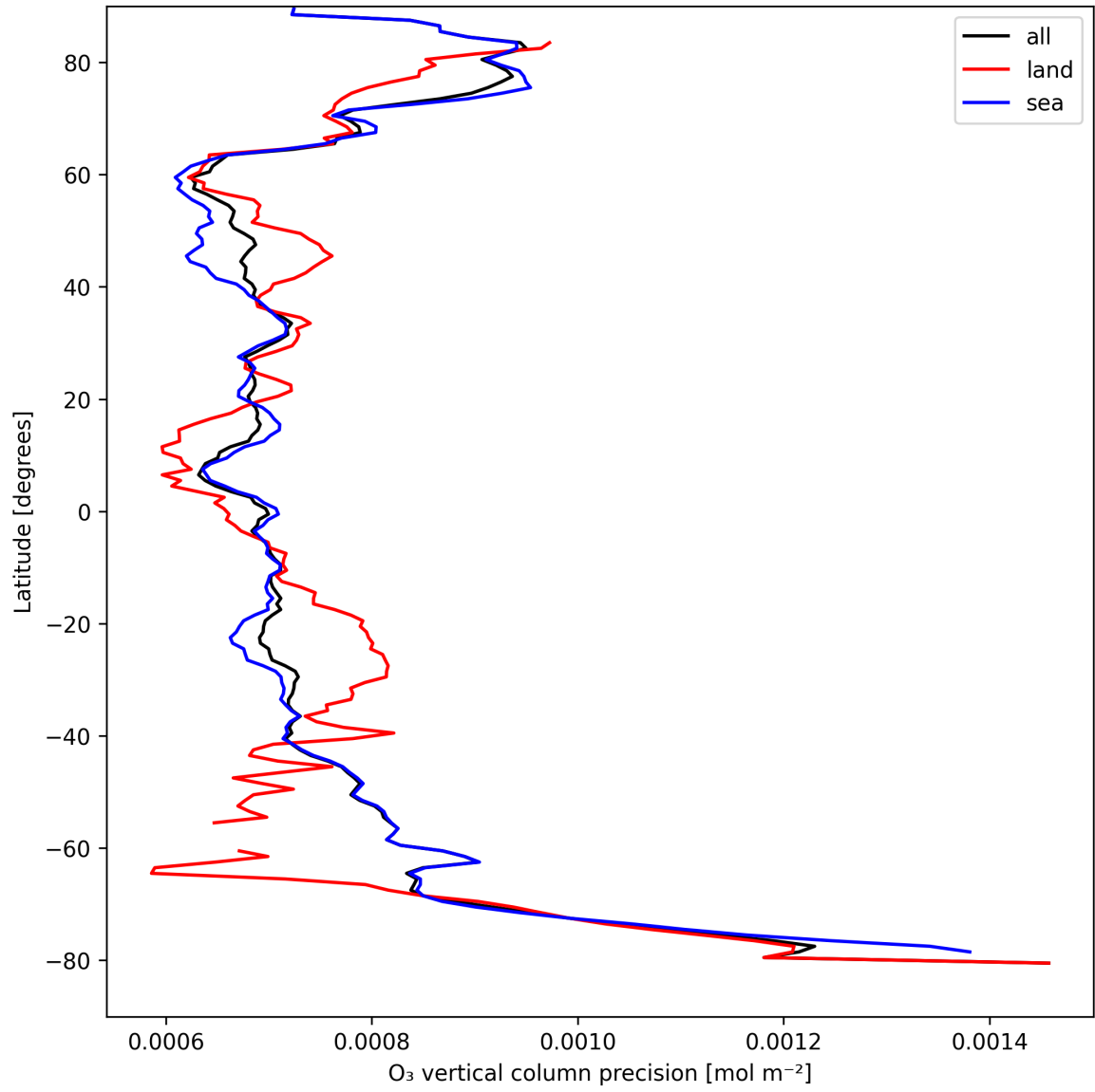
Figure 15: Zonal average of “O 3 vertical column precision” for 2024-08-30 to 2024-09-01.
