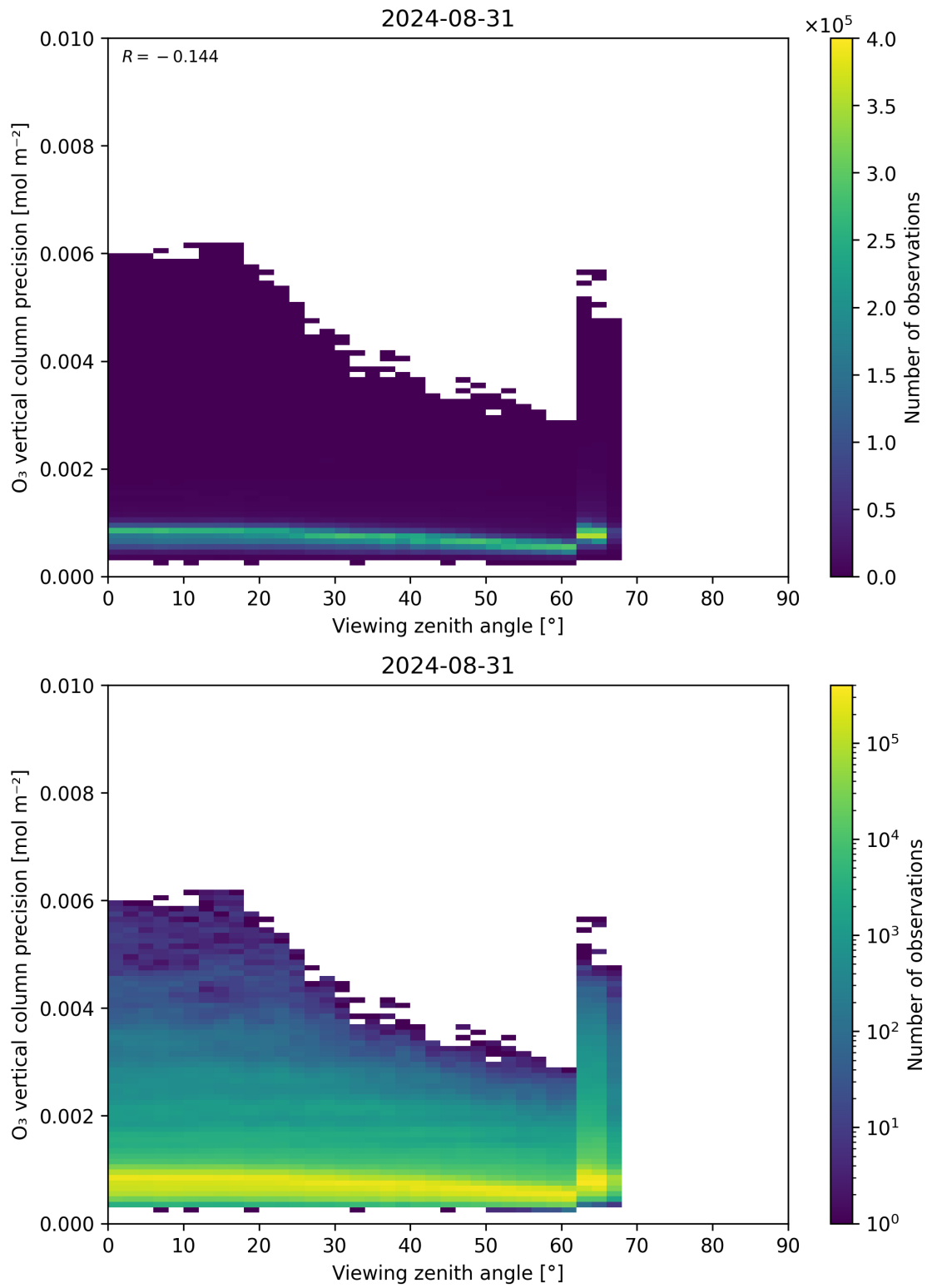
Figure 53: Scatter density plot of “Viewing zenith angle” against “O 3 vertical column precision” for 2024-08-30 to 2024-09-01.
