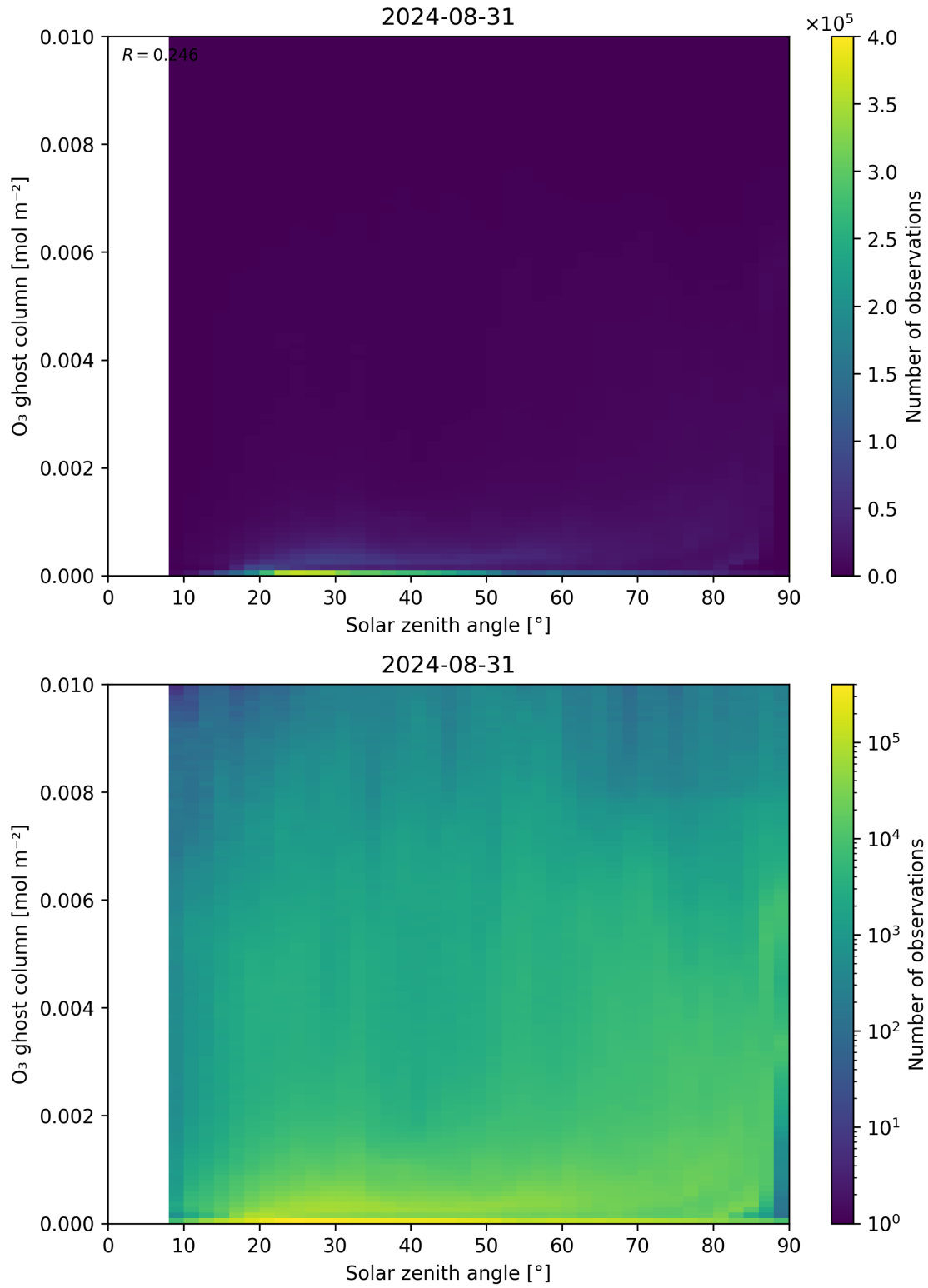
Figure 46: Scatter density plot of “Solar zenith angle” against “O 3 ghost column” for 2024-08-30 to 2024-09-01.
