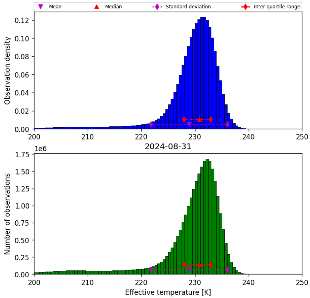
Figure 24: Histogram of “Effective temperature” for 2024-08-30 to 2024-09-01
