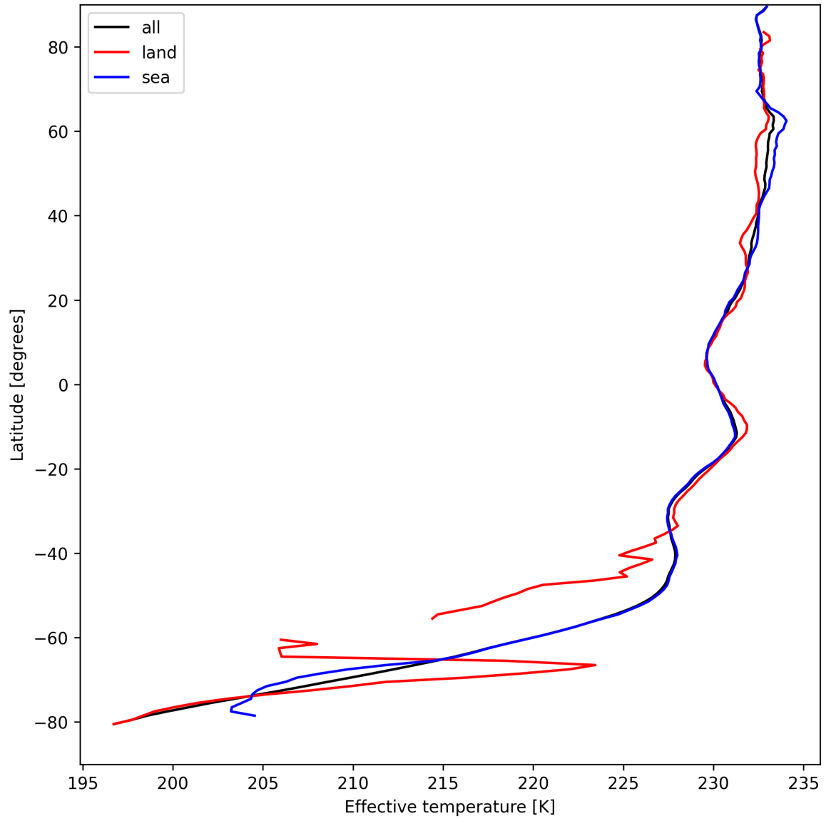
Figure 17: Zonal average of "Effective temperature" for 2024-08-30 to 2024-09-01.
