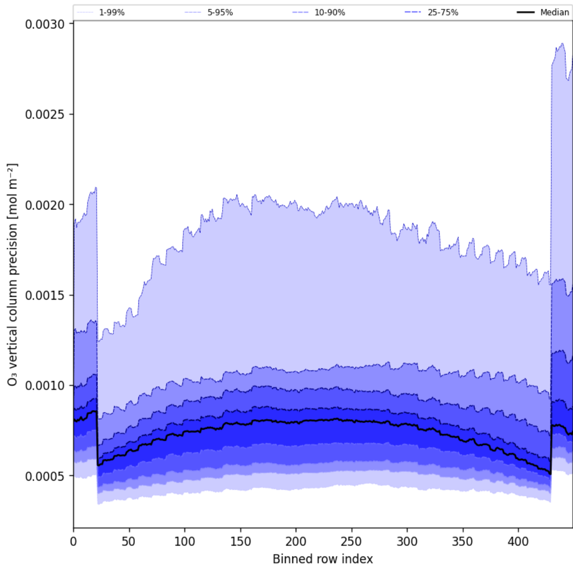
Figure 29: Along track statistics of “O 3 vertical column precision” for 2024-08-30 to 2024-09-01
