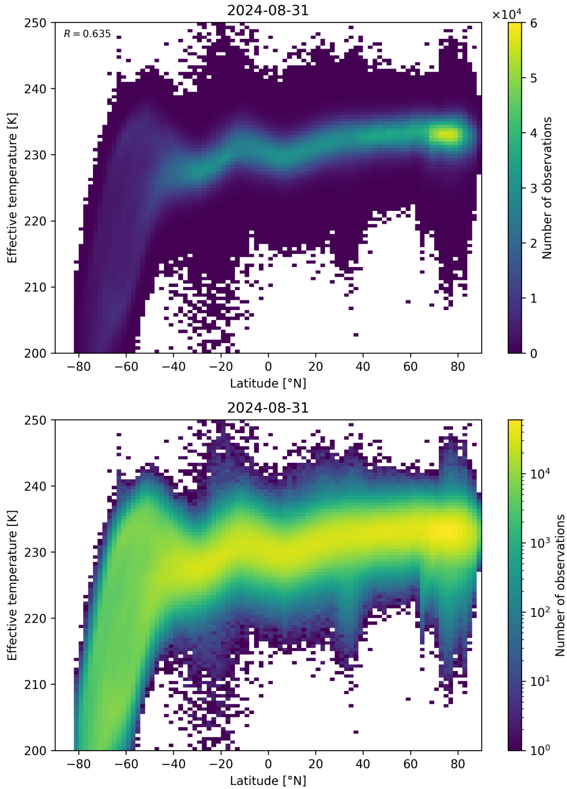
Figure 34: Scatter density plot of “Latitude” against “Effective temperature” for 2024-08-30 to 2024-09-01.
