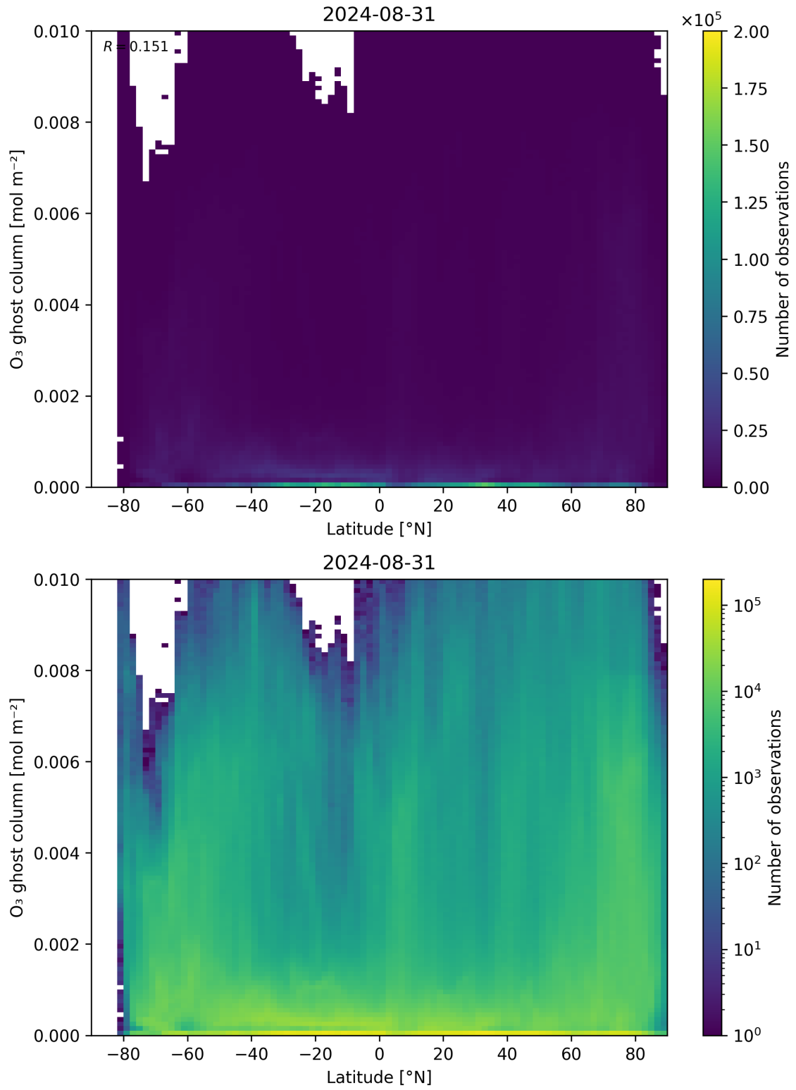
Figure 35: Scatter density plot of “Latitude” against “O 3 ghost column” for 2024-08-30 to 2024-09-01.
