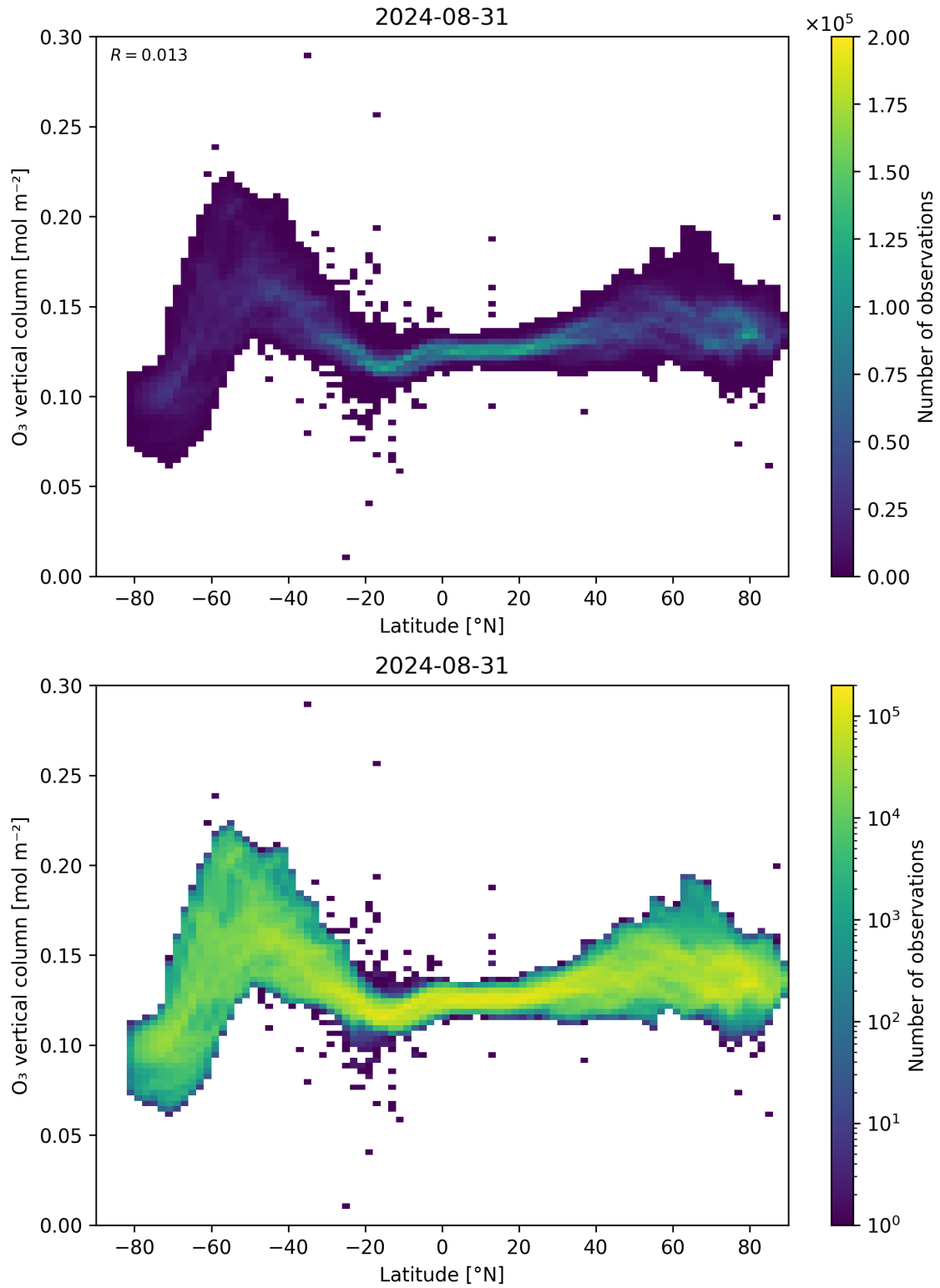
Figure 36: Scatter density plot of “Latitude” against “O 3 vertical column” for 2024-08-30 to 2024-09-01.
