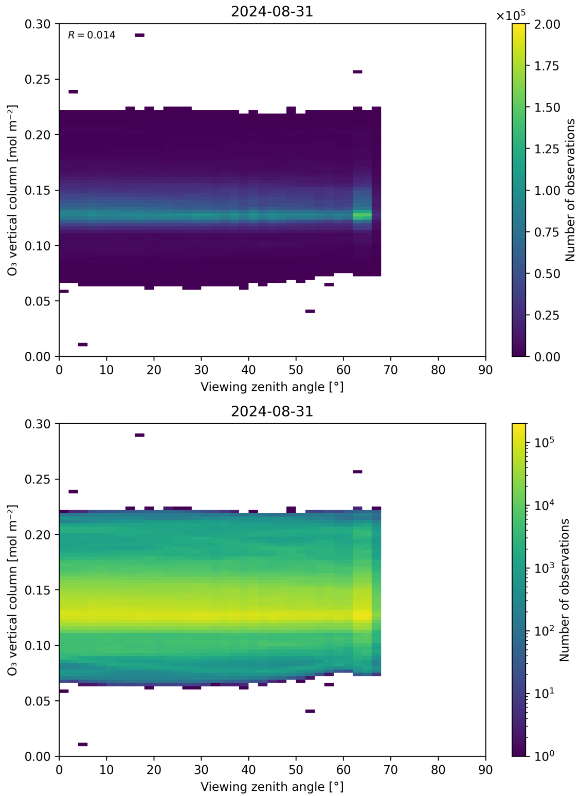
Figure 52: Scatter density plot of “Viewing zenith angle” against “O 3 vertical column” for 2024-08-30 to 2024-09-01.
