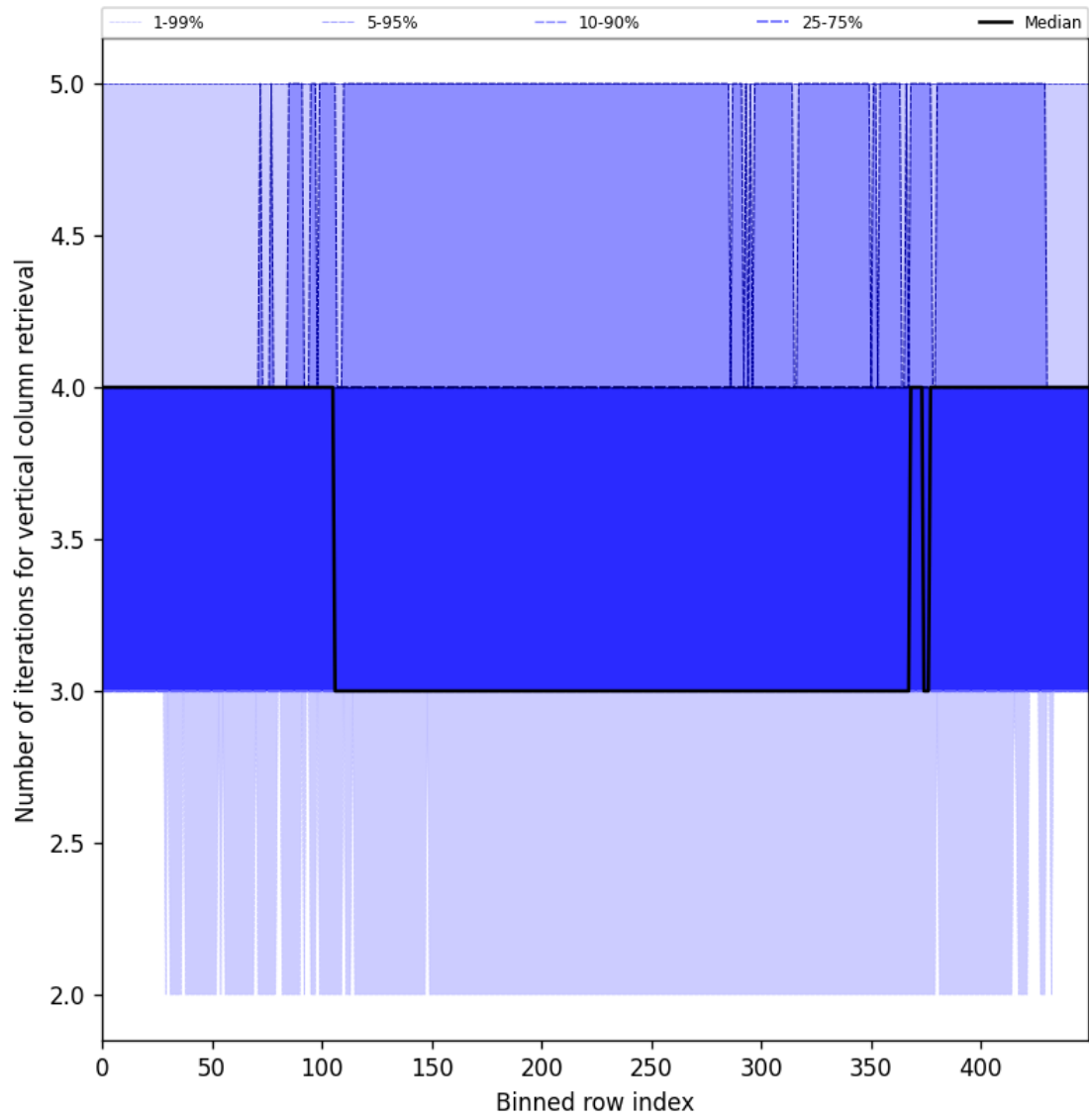
Figure 33: Along track statistics of “Number of iterations for vertical column retrieval” for 2024-08-30 to 2024-09-01
