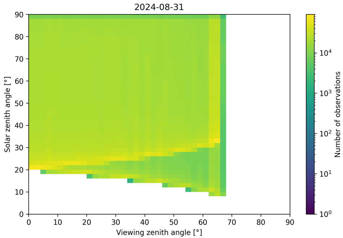
Figure 54: Scatter density plot of “Viewing zenith angle” against “Solar zenith angle” for 2024-08-30 to 2024-09-01.
