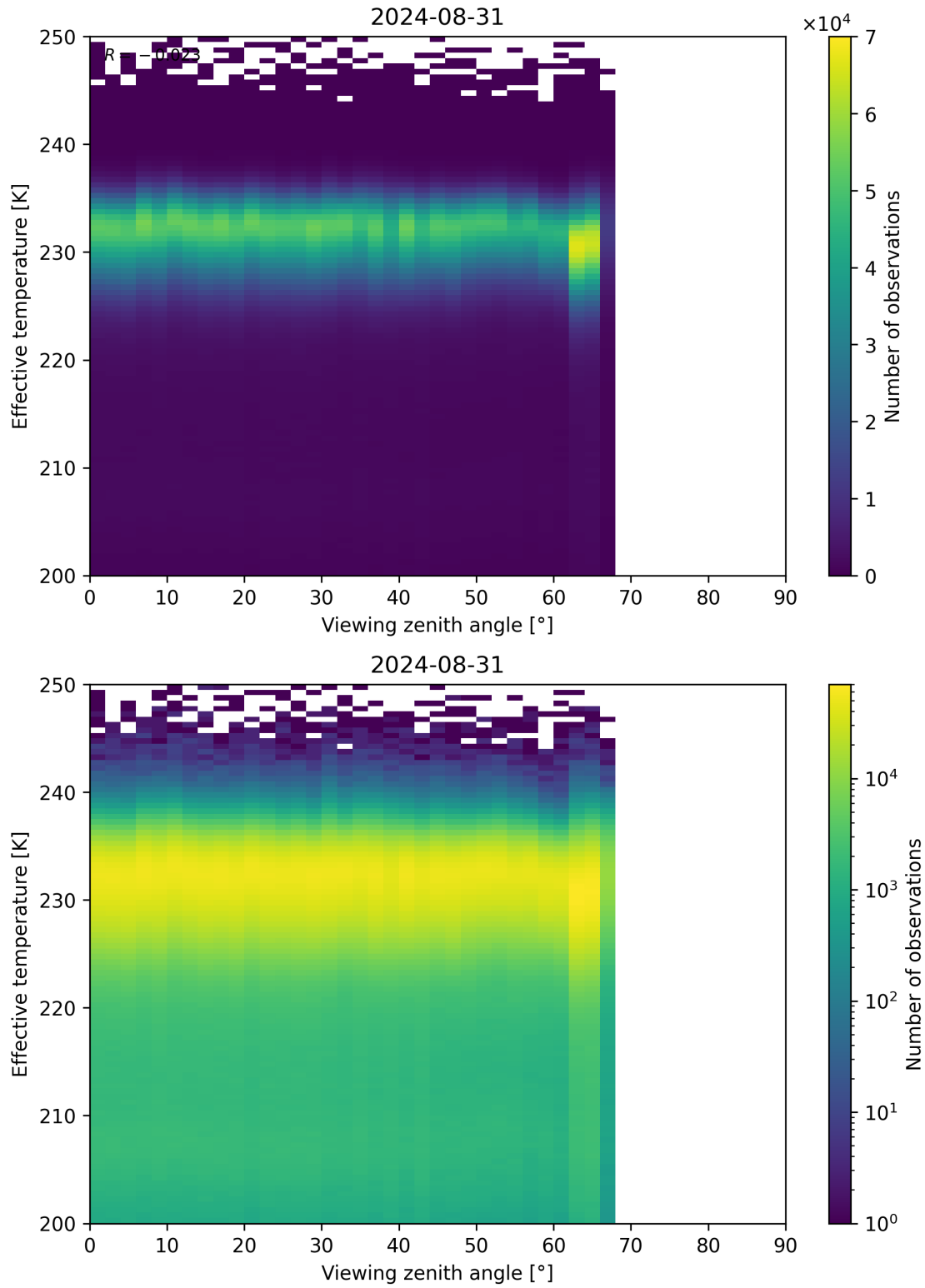
Figure 50: Scatter density plot of “Viewing zenith angle” against “Effective temperature” for 2024-08-30 to 2024-09-01.
