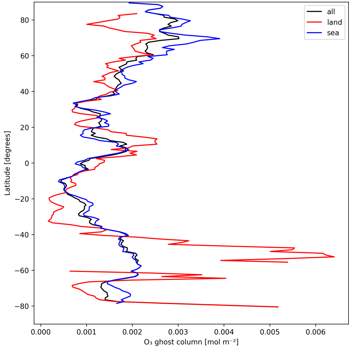
Figure 18: Zonal average of “O 3 ghost column” for 2024-08-30 to 2024-09-01.
