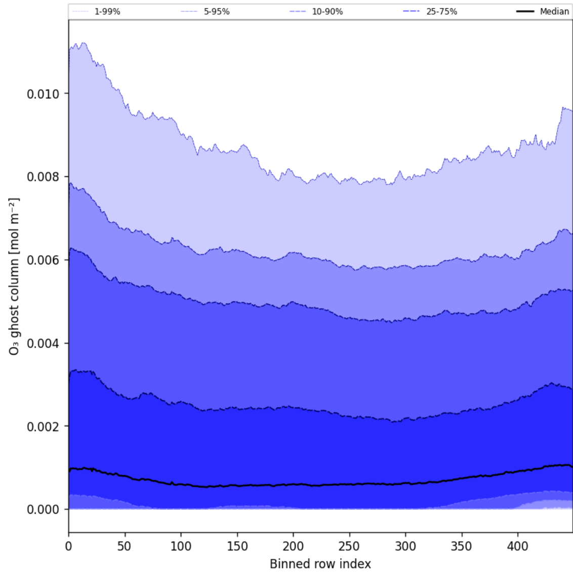
Figure 32: Along track statistics of “O 3 ghost column” for 2024-08-30 to 2024-09-01
