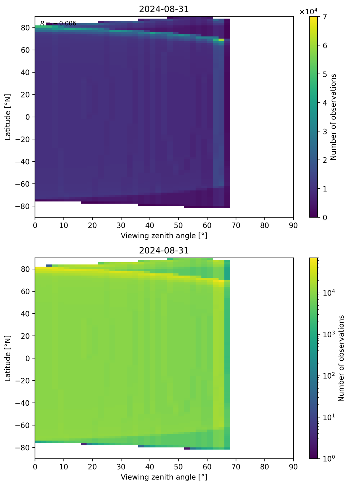
Figure 49: Scatter density plot of “Viewing zenith angle” against “Latitude” for 2024-08-30 to 2024-09-01.
