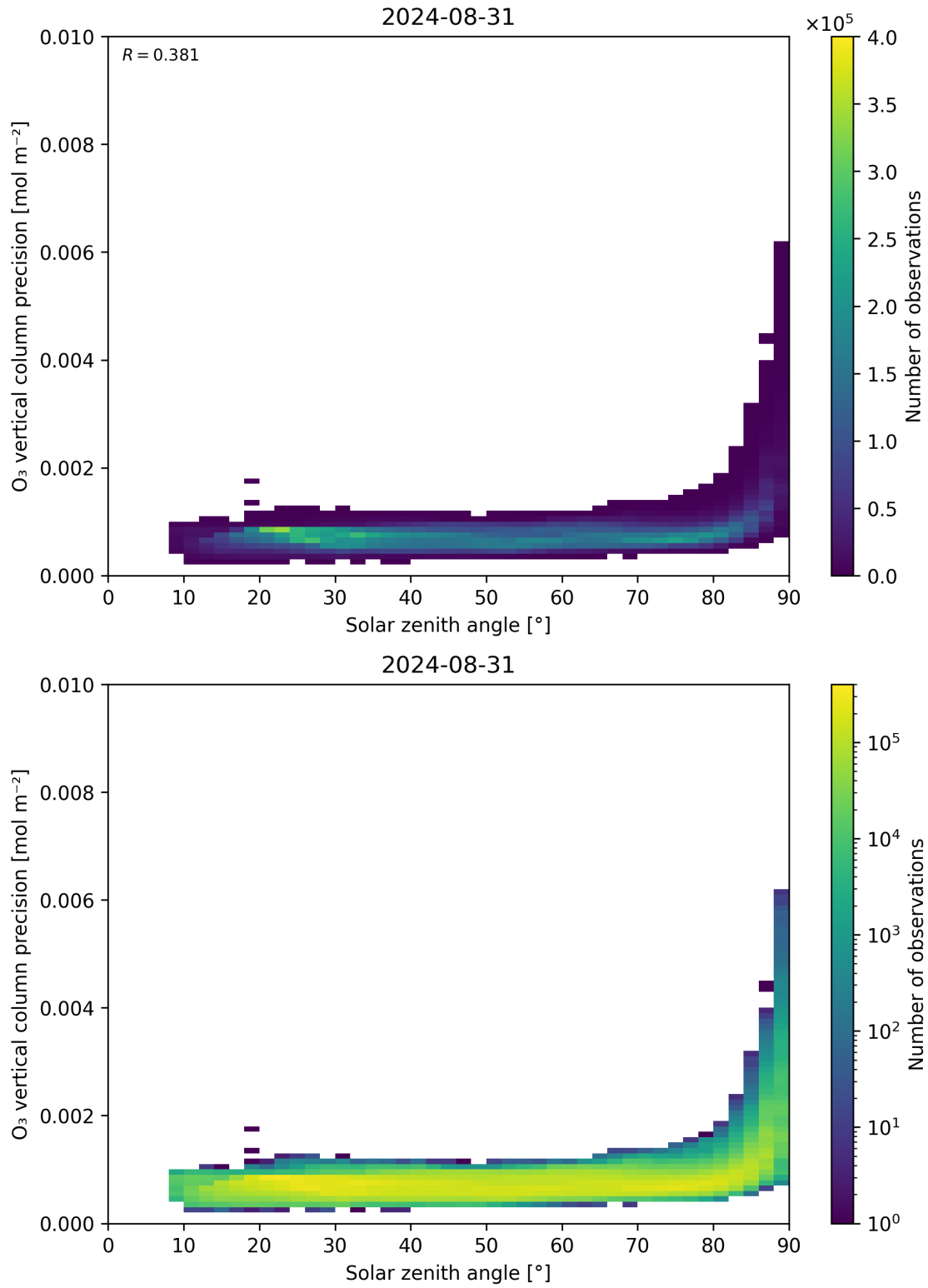
Figure 48: Scatter density plot of “Solar zenith angle” against “O 3 vertical column precision” for 2024-08-30 to 2024-09-01.
