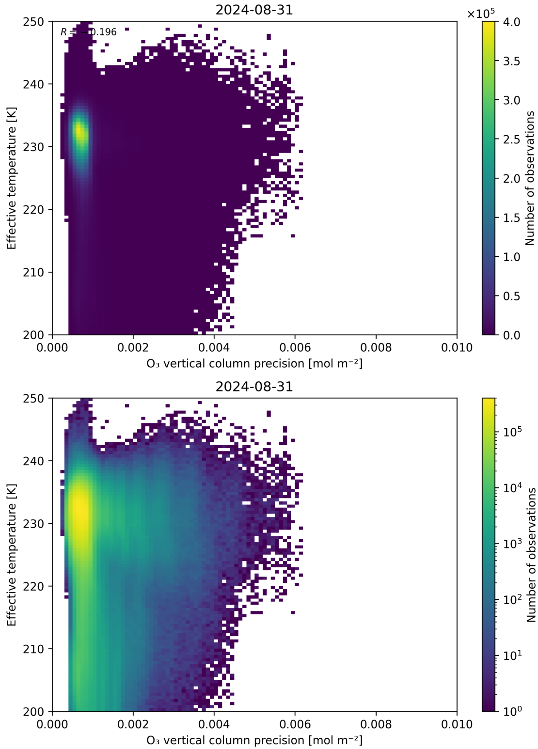
Figure 42: Scatter density plot of “O 3 vertical column precision” against “Effective temperature” for 2024-08-30 to 2024-09-01.
