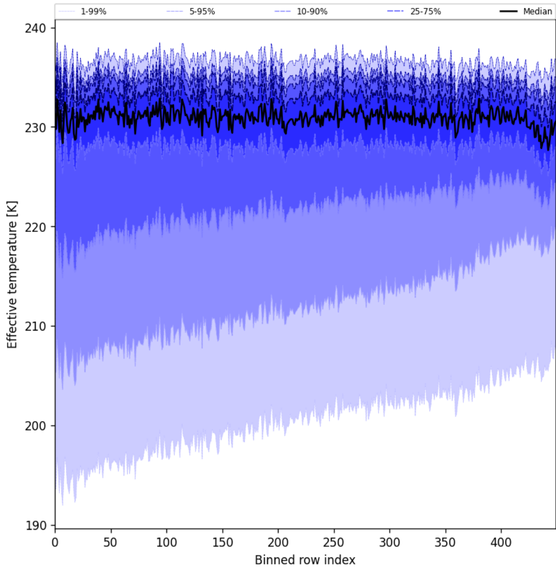
Figure 31: Along track statistics of “Effective temperature” for 2024-08-30 to 2024-09-01
