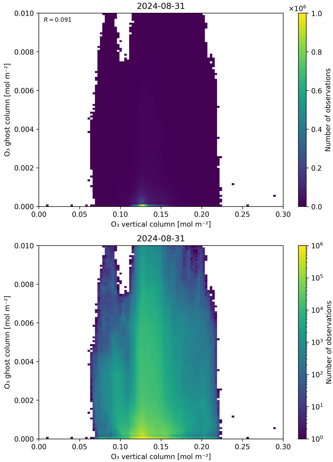
Figure 40: Scatter density plot of “ O_3 vertical column” against “ O_3 ghost column” for 2024-08-30 to 2024-09-01.
