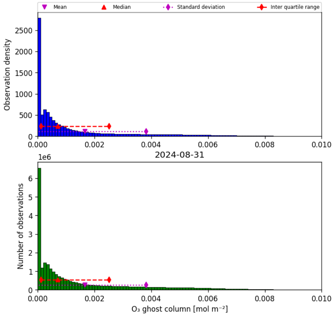
Figure 25: Histogram of “O 3 ghost column” for 2024-08-30 to 2024-09-01
