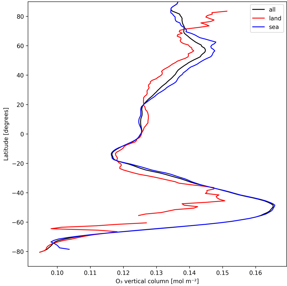
Figure 14: Zonal average of “O 3 vertical column” for 2024-08-30 to 2024-09-01.
