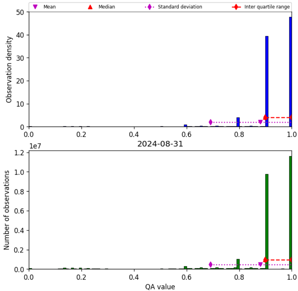
Figure 20: Histogram of “QA value” for 2024-08-30 to 2024-09-01
