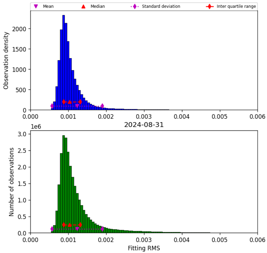
Figure 23: Histogram of “Fitting RMS” for 2024-08-30 to 2024-09-01
