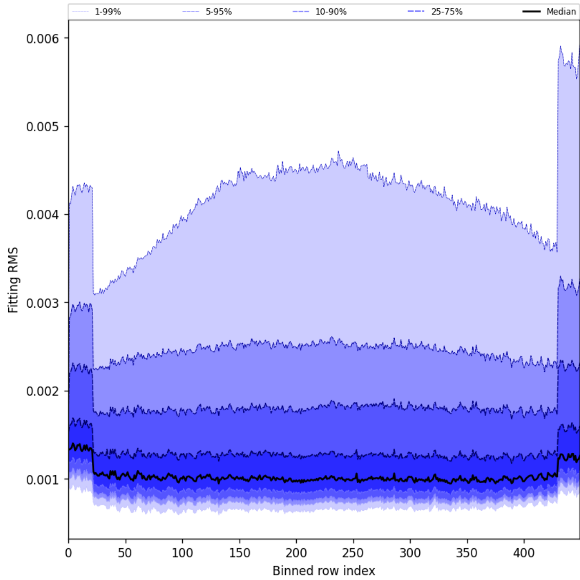
Figure 30: Along track statistics of “Fitting RMS” for 2024-08-30 to 2024-09-01
