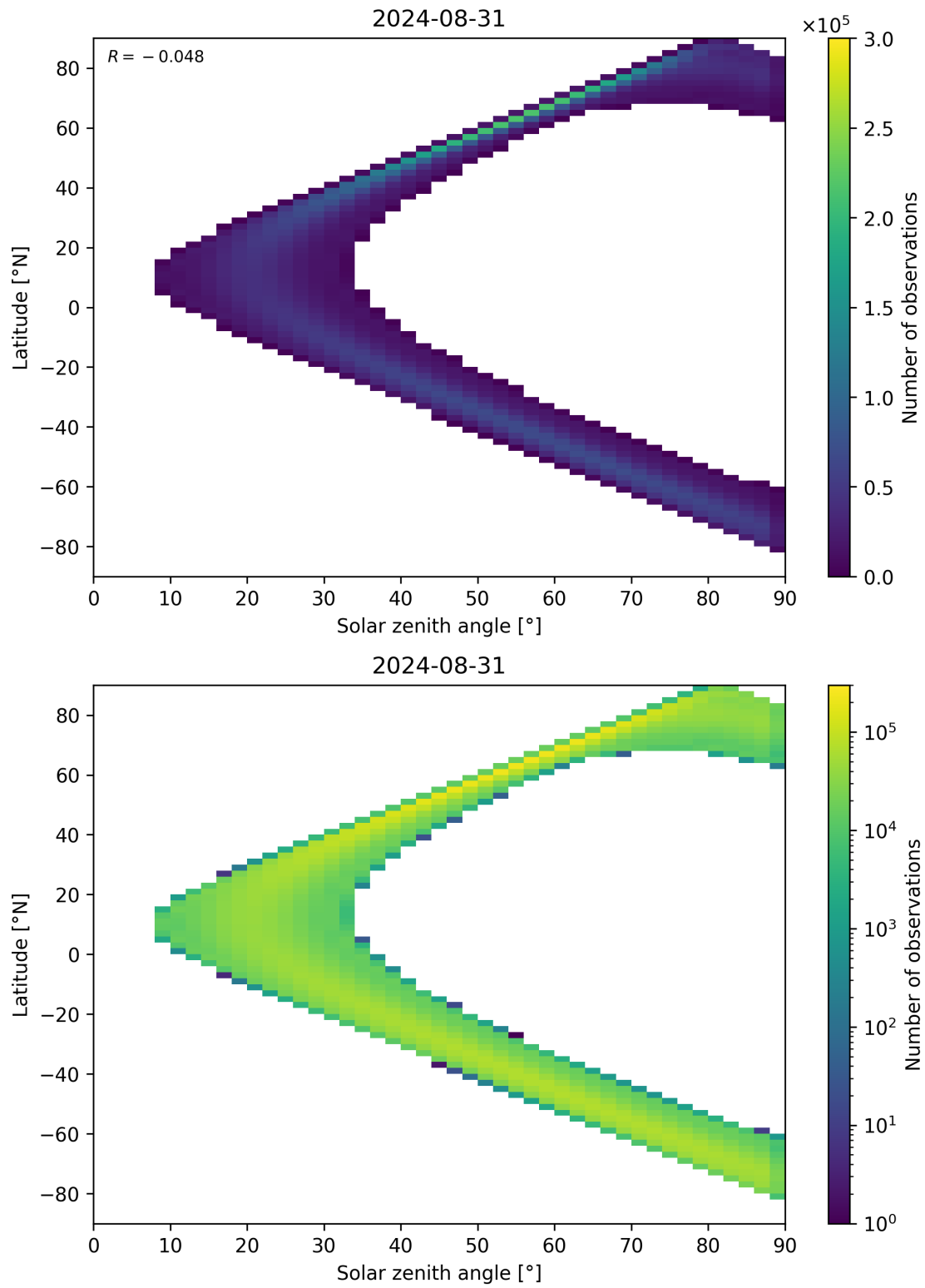
Figure 44: Scatter density plot of “Solar zenith angle” against “Latitude” for 2024-08-30 to 2024-09-01.
