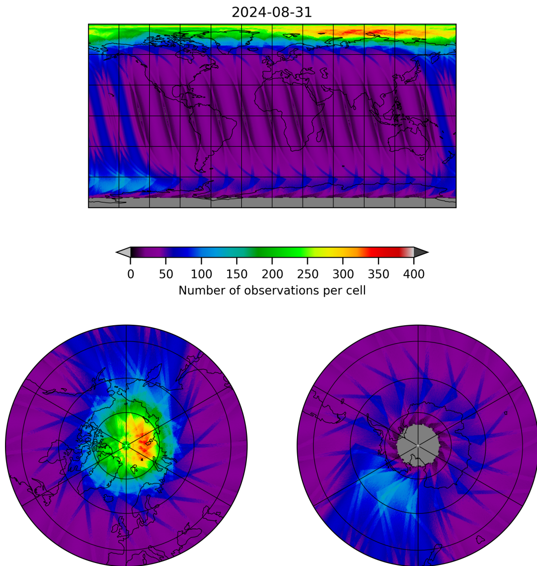
Figure 12: Map of the number of observations for 2024-08-30 to 2024-09-01
