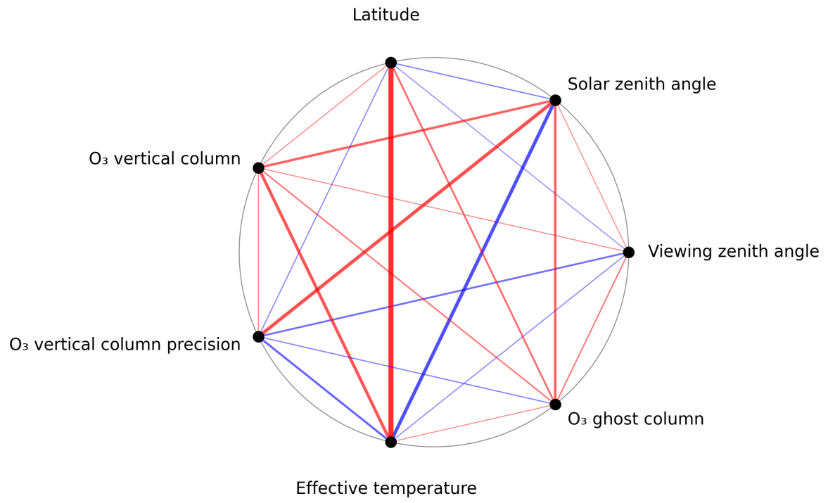
Figure 1: Map of correlation graph for 2024-08-30 to 2024-09-01.
