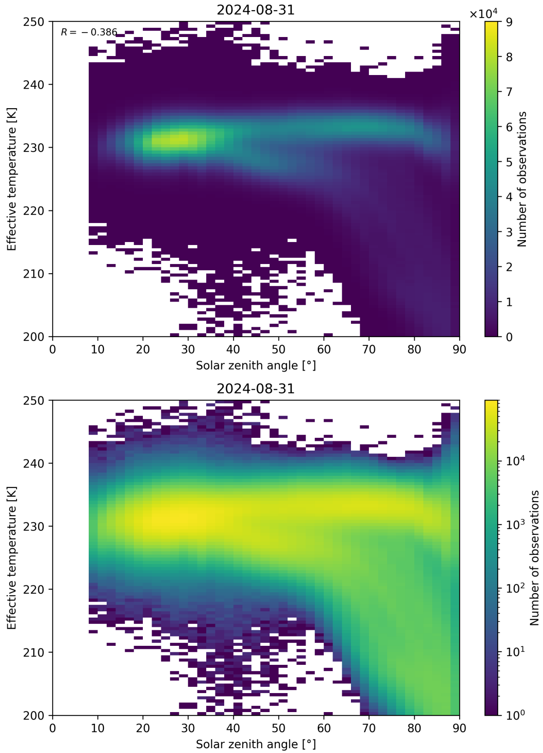
Figure 45: Scatter density plot of “Solar zenith angle” against “Effective temperature” for 2024-08-30 to 2024-09-01.
