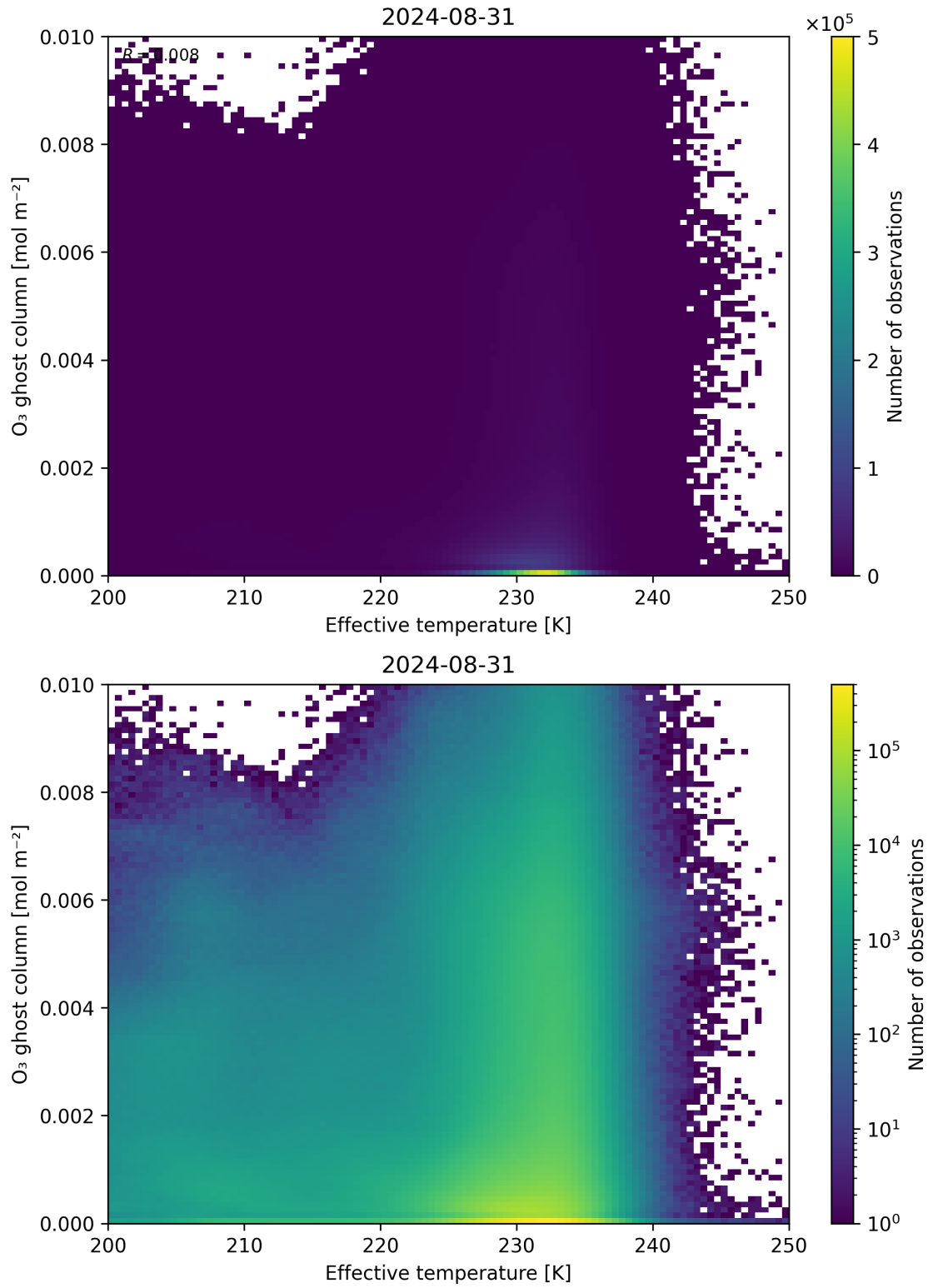
Figure 38: Scatter density plot of “Effective temperature” against “O 3 ghost column” for 2024-08-30 to 2024-09-01.
