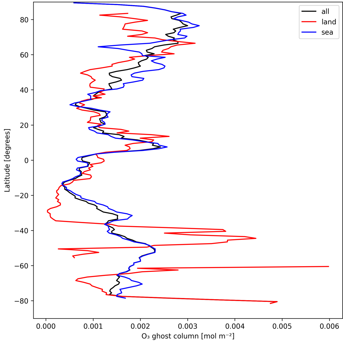
Figure 18: Zonal average of “O 3 ghost column” for 2024-09-01 to 2024-09-02.
