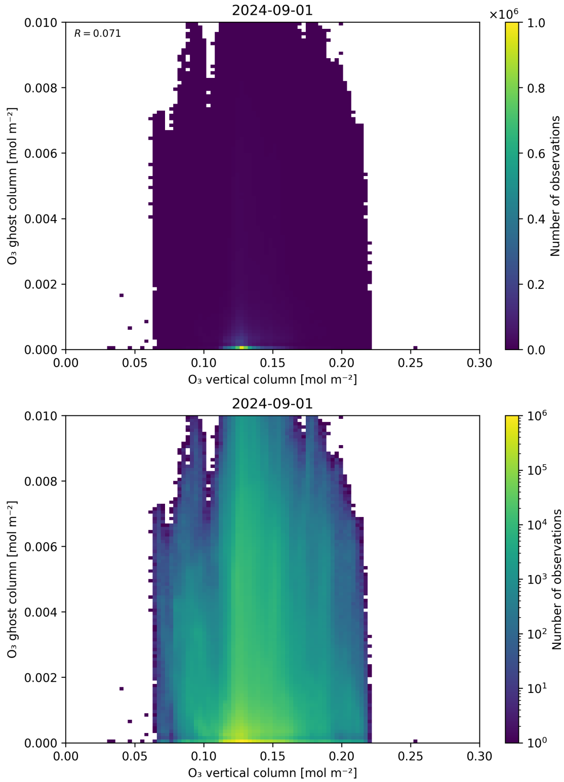
Figure 40: Scatter density plot of “O 3 vertical column” against “O 3 ghost column” for 2024-09-01 to 2024-09-02.
