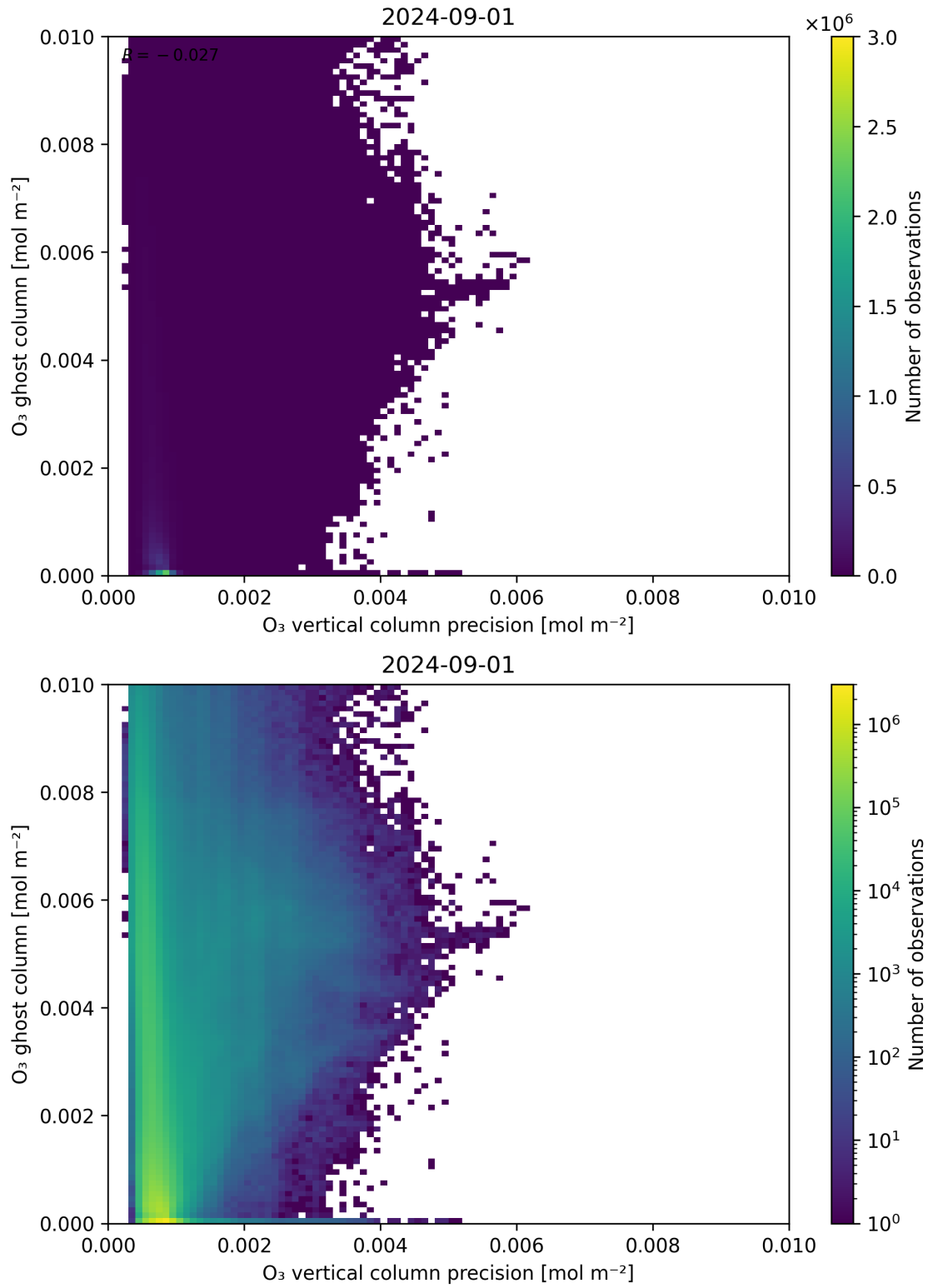
Figure 43: Scatter density plot of “ \text{O}_3 vertical column precision” against “ \text{O}_3 ghost column” for 2024-09-01 to 2024-09-02.
