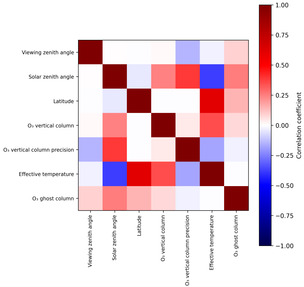
Figure 2: Map of correlation matrix for 2024-09-01 to 2024-09-02.
