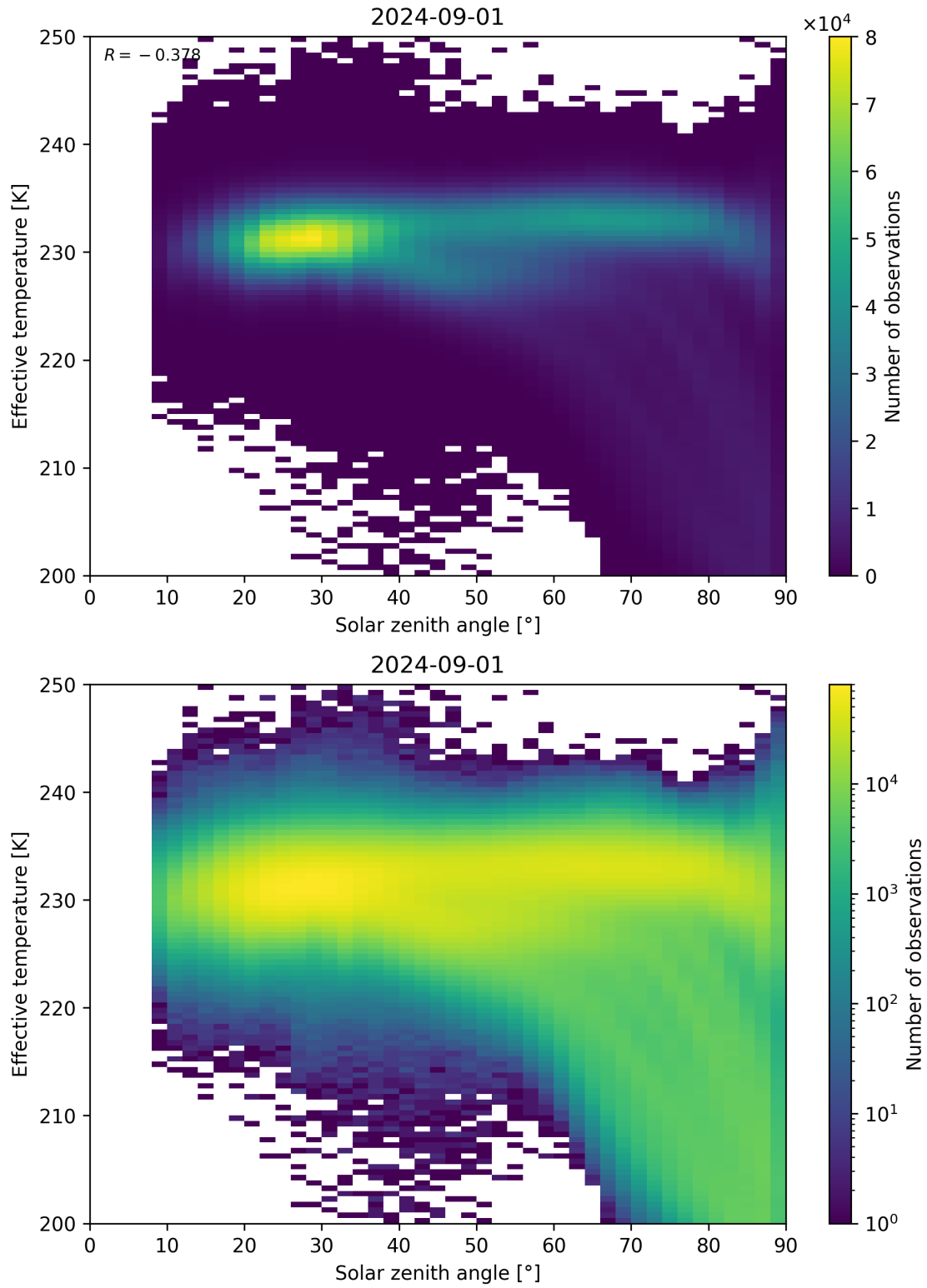
Figure 45: Scatter density plot of “Solar zenith angle” against “Effective temperature” for 2024-09-01 to 2024-09-02.
