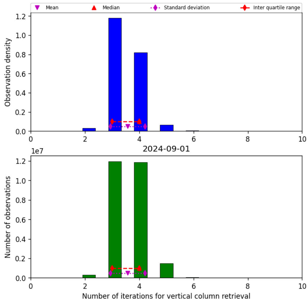
Figure 26: Histogram of “Number of iterations for vertical column retrieval” for 2024-09-01 to 2024-09-02
