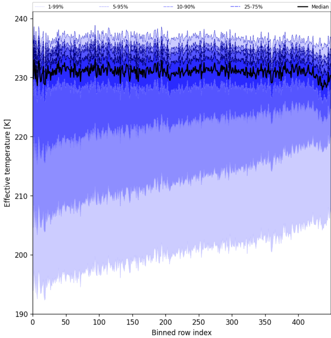
Figure 31: Along track statistics of “Effective temperature” for 2024-09-01 to 2024-09-02
