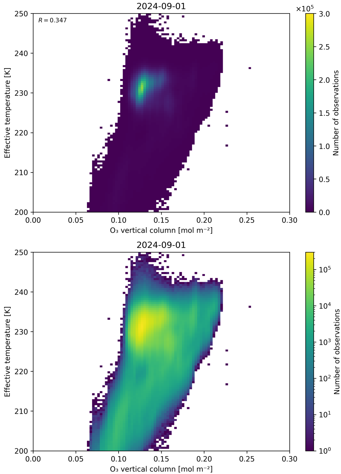
Figure 39: Scatter density plot of “O 3 vertical column” against “Effective temperature” for 2024-09-01 to 2024-09-02.
