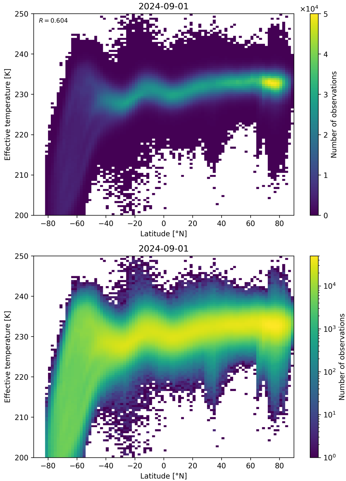
Figure 34: Scatter density plot of “Latitude” against “Effective temperature” for 2024-09-01 to 2024-09-02.
