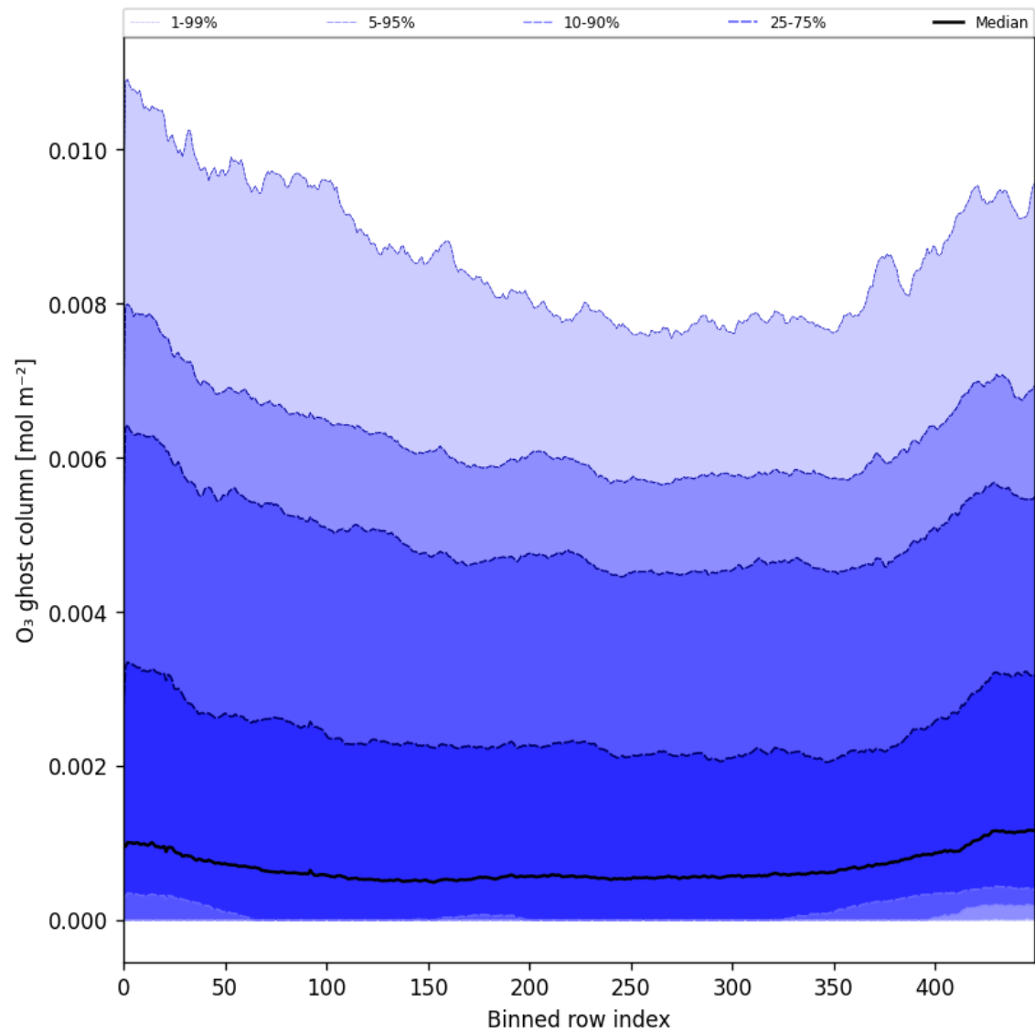
Figure 32: Along track statistics of “O 3 ghost column” for 2024-09-01 to 2024-09-02
