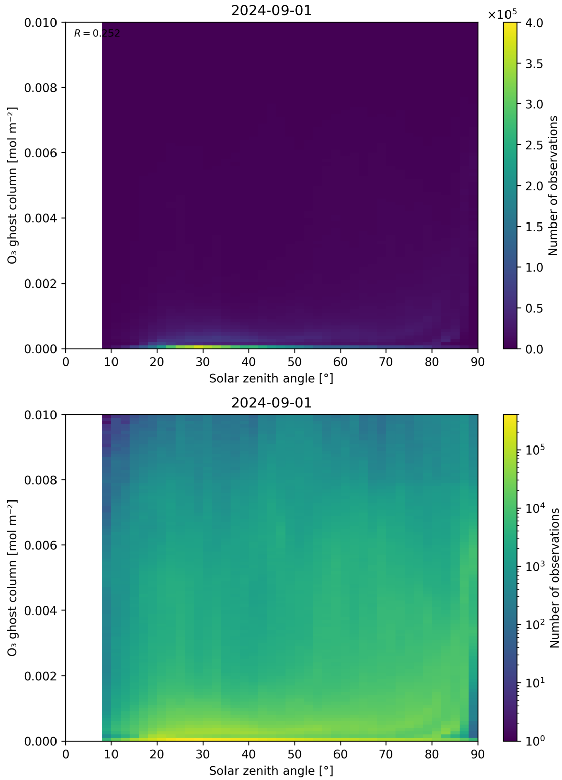
Figure 46: Scatter density plot of “Solar zenith angle” against “O 3 ghost column” for 2024-09-01 to 2024-09-02.
