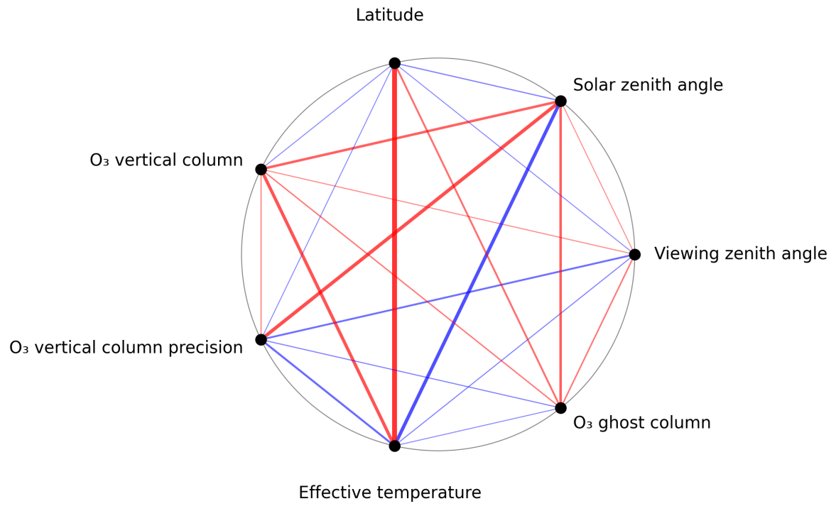
Figure 1: Map of correlation graph for 2024-09-01 to 2024-09-02.
