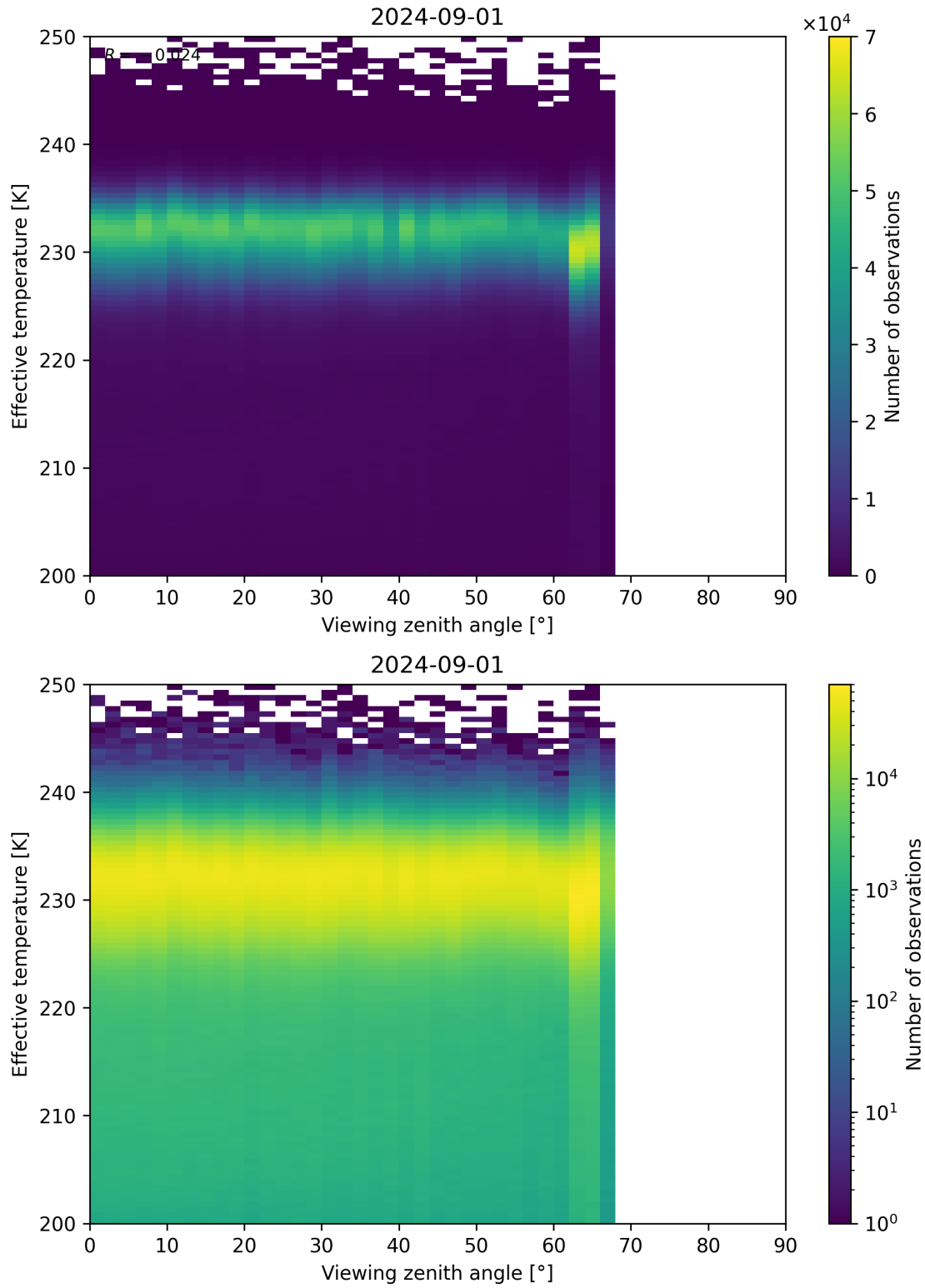
Figure 50: Scatter density plot of “Viewing zenith angle” against “Effective temperature” for 2024-09-01 to 2024-09-02.
