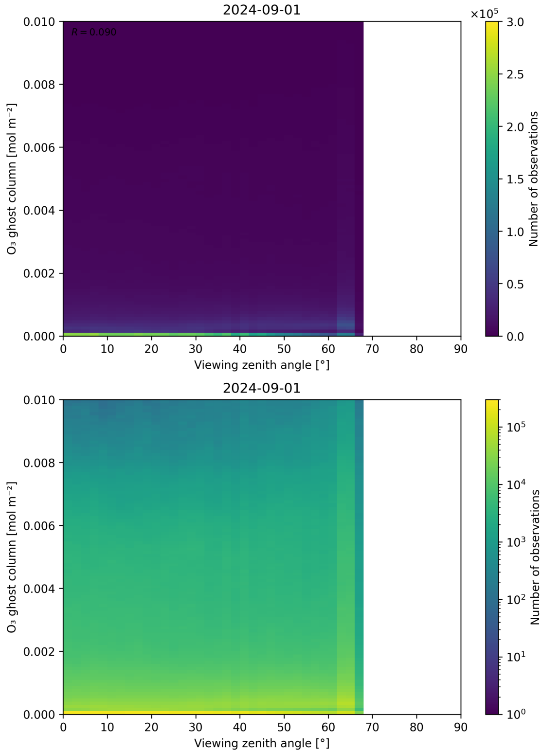
Figure 51: Scatter density plot of “Viewing zenith angle” against “O 3 ghost column” for 2024-09-01 to 2024-09-02.
