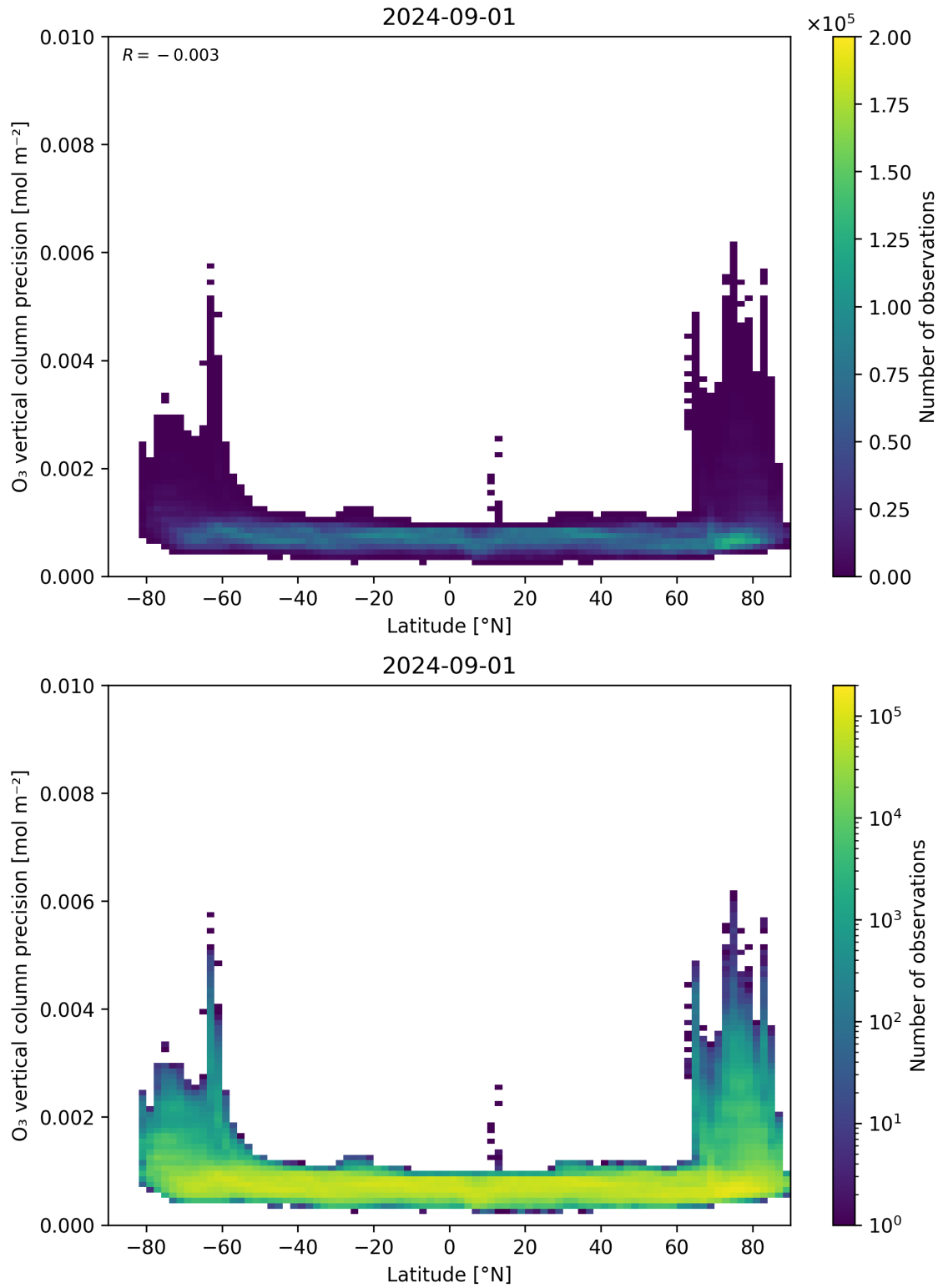
Figure 37: Scatter density plot of “Latitude” against “O 3 vertical column precision” for 2024-09-01 to 2024-09-02.
