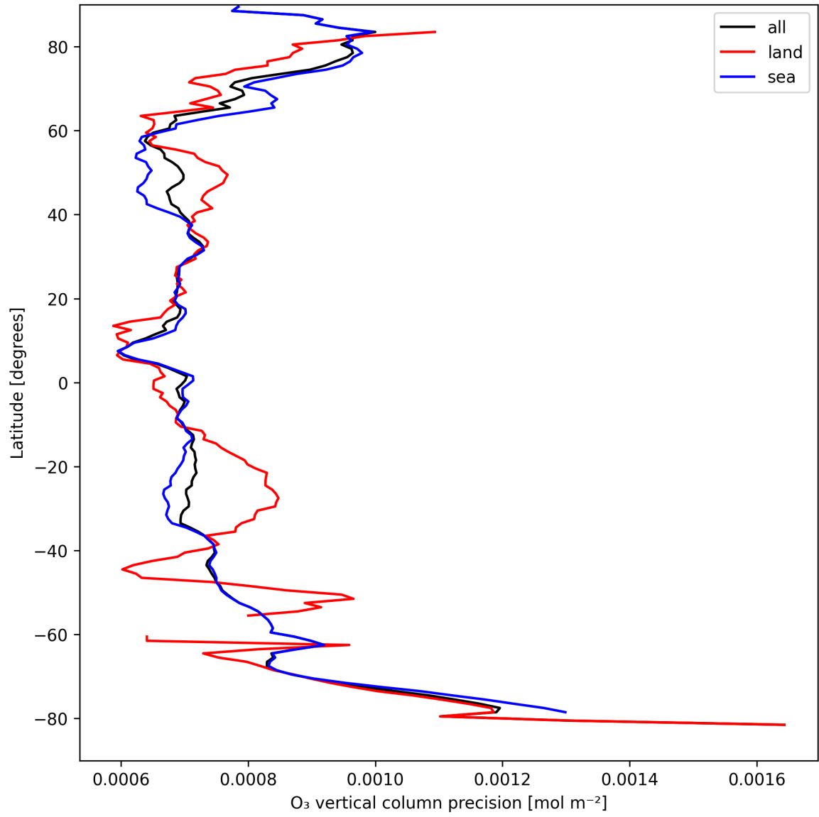
Figure 15: Zonal average of “O 3 vertical column precision” for 2024-09-01 to 2024-09-02.
