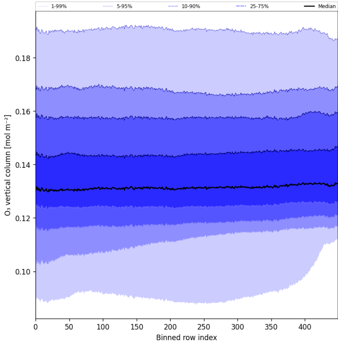
Figure 28: Along track statistics of “O 3 vertical column” for 2024-09-01 to 2024-09-02
