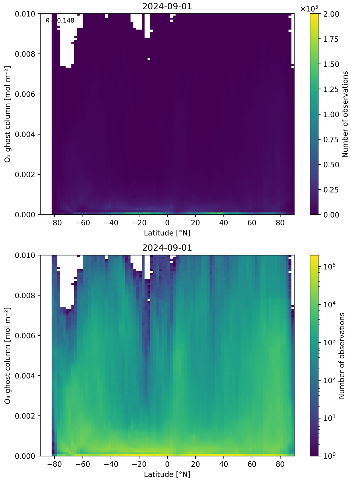
Figure 35: Scatter density plot of “Latitude” against “O 3 ghost column” for 2024-09-01 to 2024-09-02.
