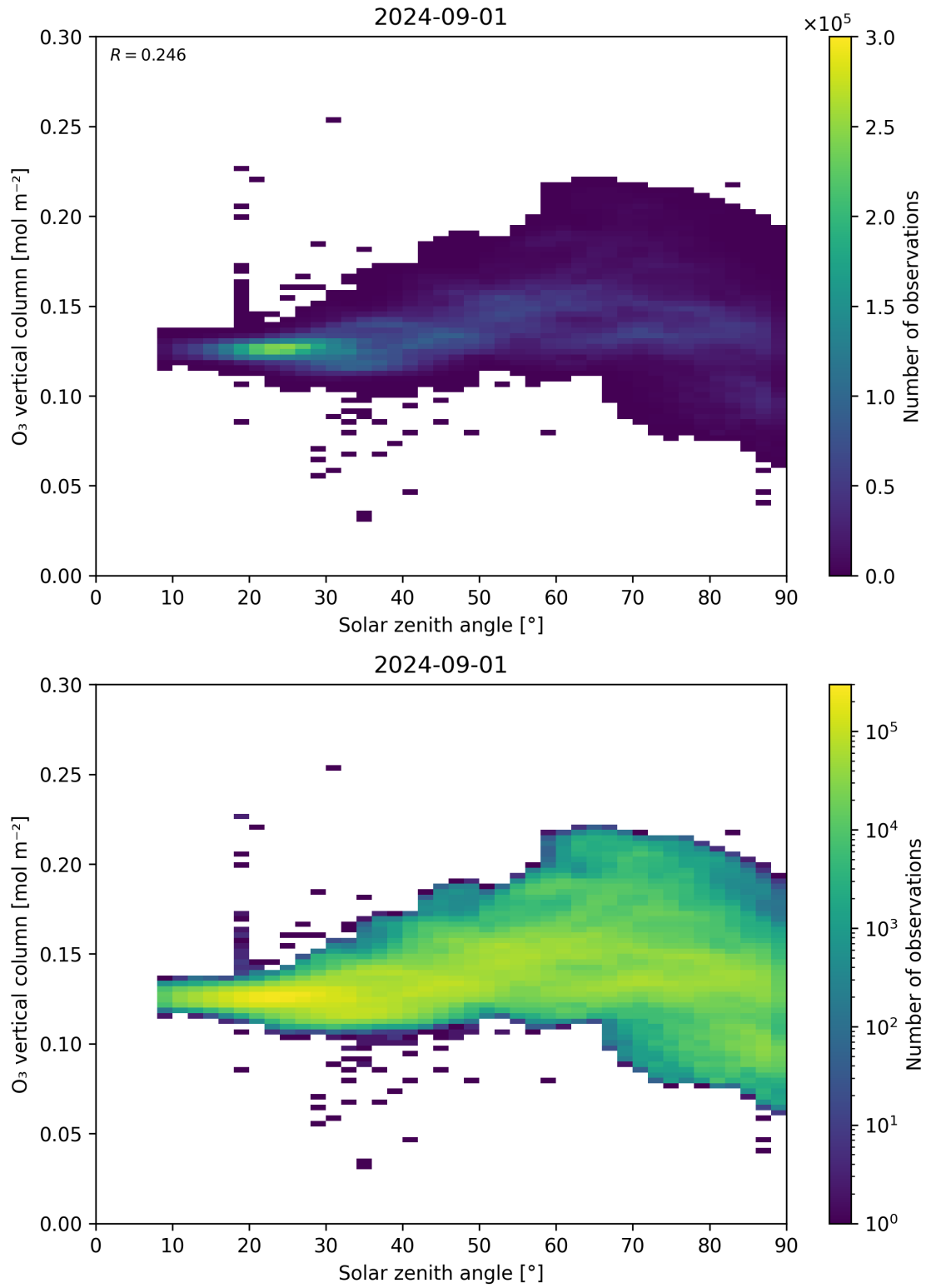
Figure 47: Scatter density plot of “Solar zenith angle” against “O 3 vertical column” for 2024-09-01 to 2024-09-02.
