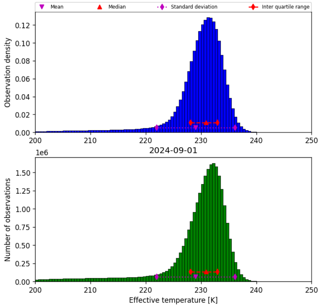
Figure 24: Histogram of “Effective temperature” for 2024-09-01 to 2024-09-02
