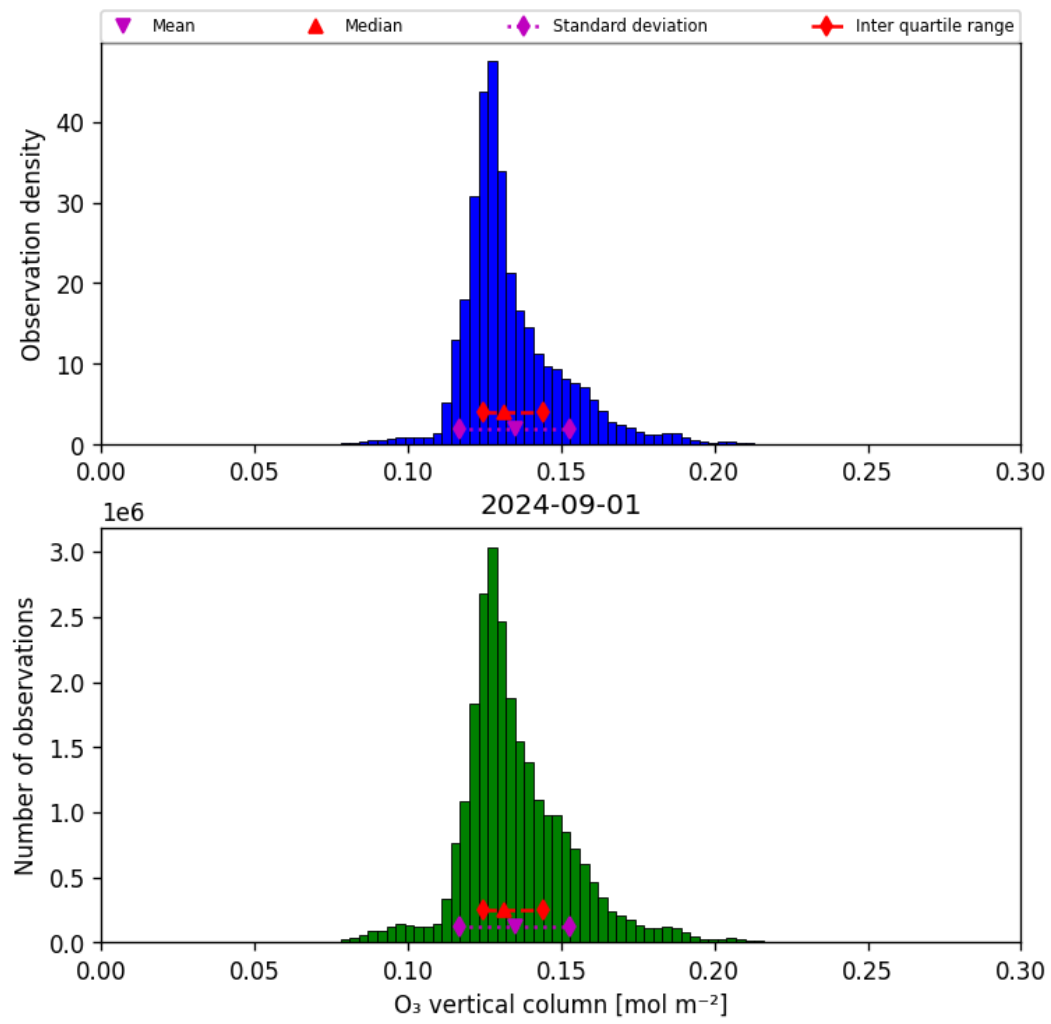
Figure 21: Histogram of “O 3 vertical column” for 2024-09-01 to 2024-09-02
