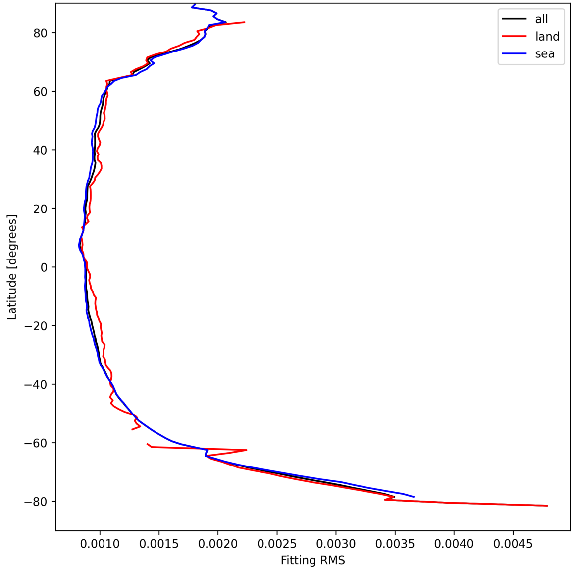
Figure 16: Zonal average of “Fitting RMS” for 2024-09-01 to 2024-09-02.
