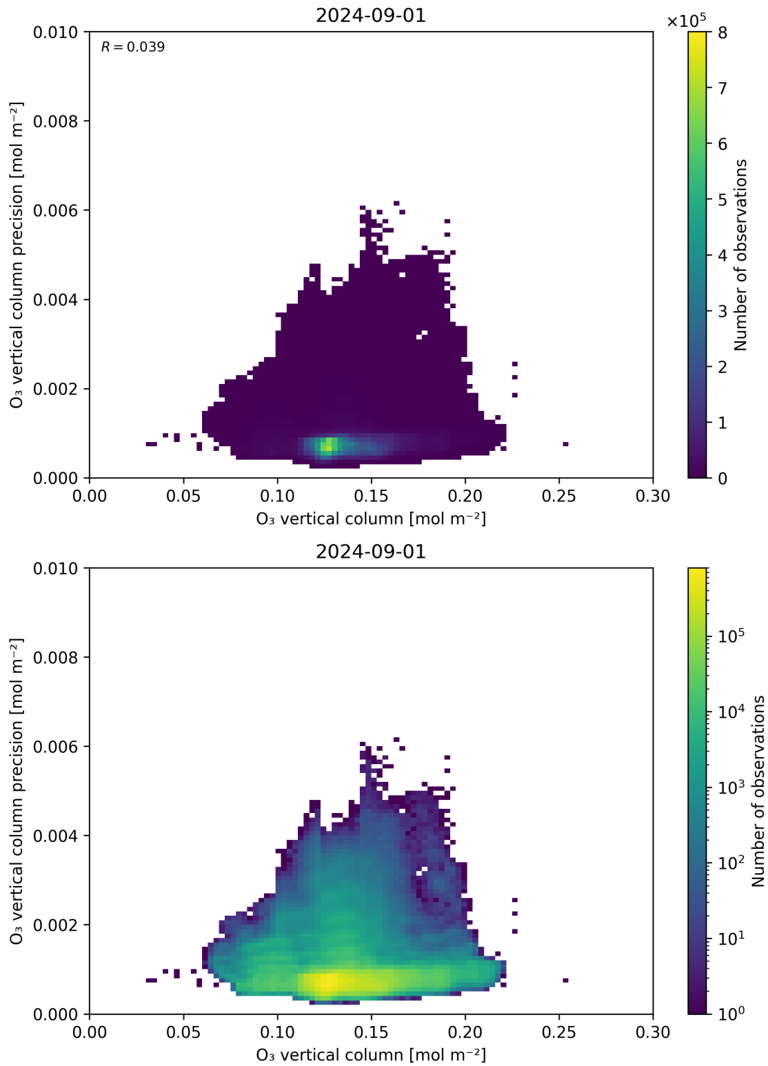
Figure 41: Scatter density plot of “O 3 vertical column” against “O 3 vertical column precision” for 2024-09-01 to 2024-09-02.
