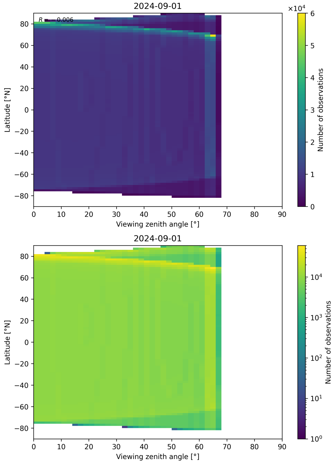
Figure 49: Scatter density plot of “Viewing zenith angle” against “Latitude” for 2024-09-01 to 2024-09-02.
