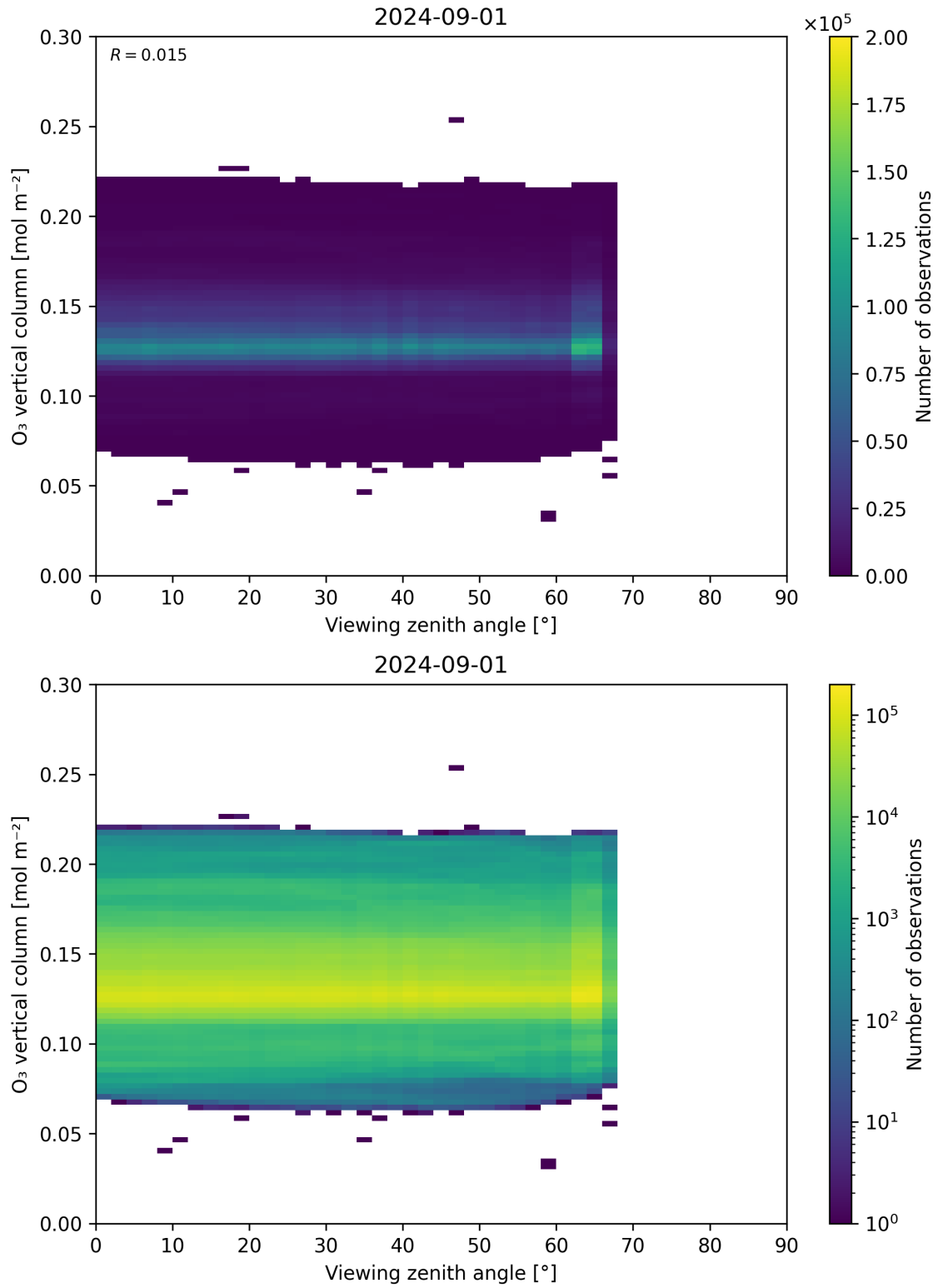
Figure 52: Scatter density plot of “Viewing zenith angle” against “O 3 vertical column” for 2024-09-01 to 2024-09-02.
