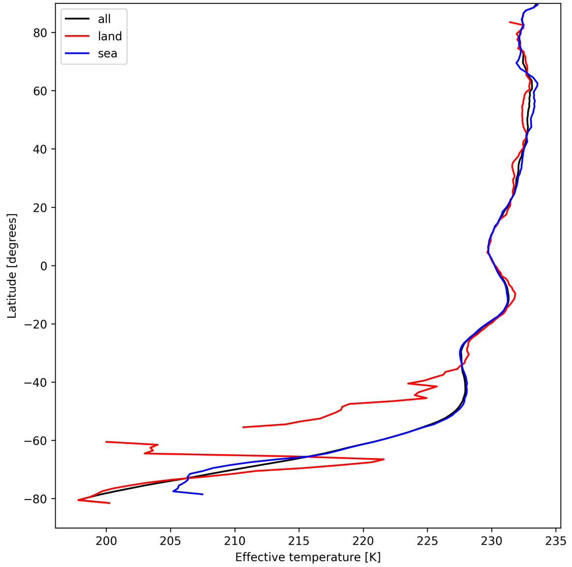
Figure 17: Zonal average of "Effective temperature" for 2024-09-01 to 2024-09-02.
