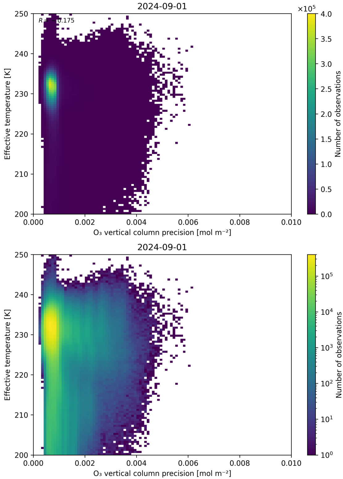
Figure 42: Scatter density plot of “O 3 vertical column precision” against “Effective temperature” for 2024-09-01 to 2024-09-02.
