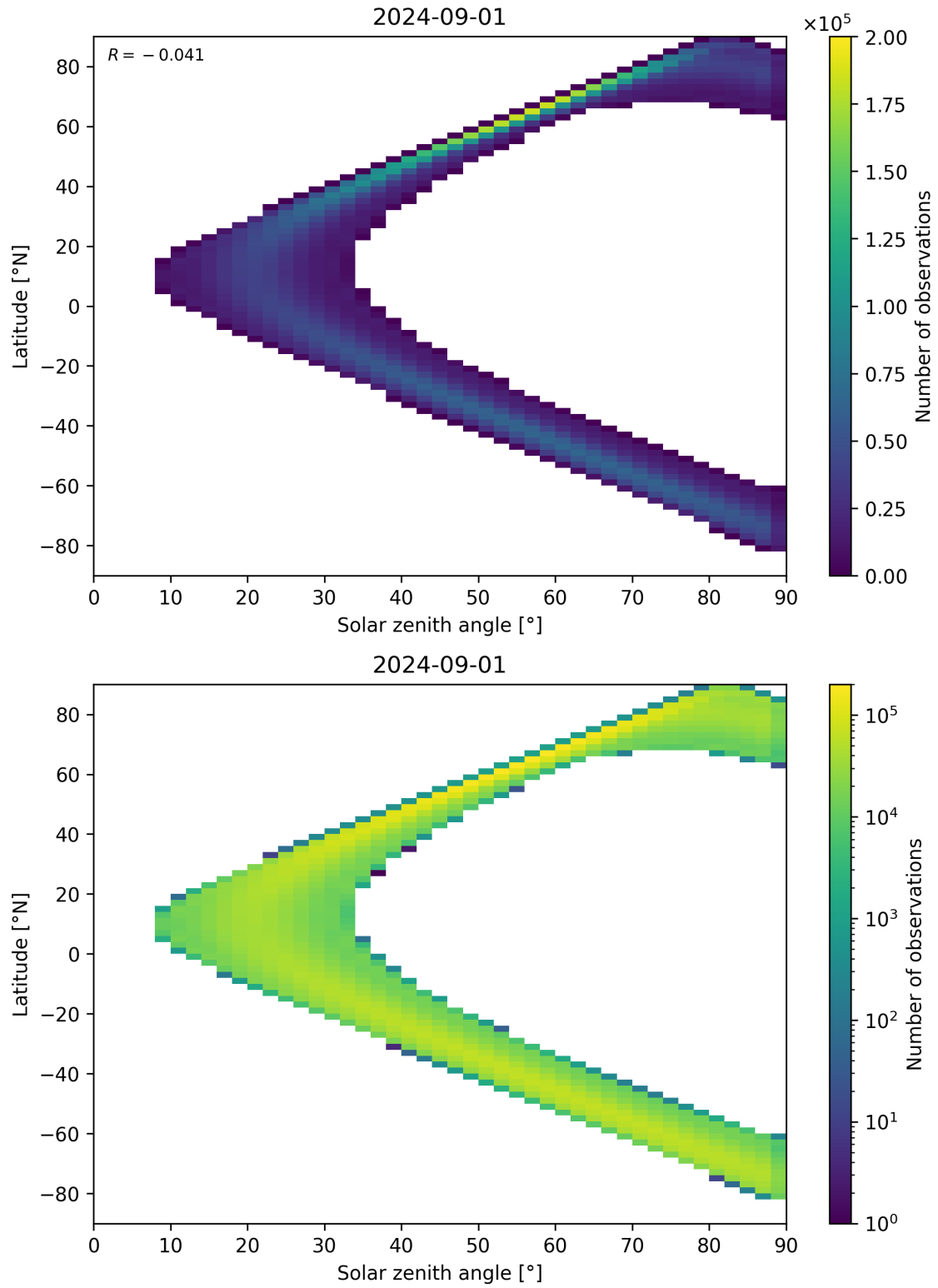
Figure 44: Scatter density plot of “Solar zenith angle” against “Latitude” for 2024-09-01 to 2024-09-02.
