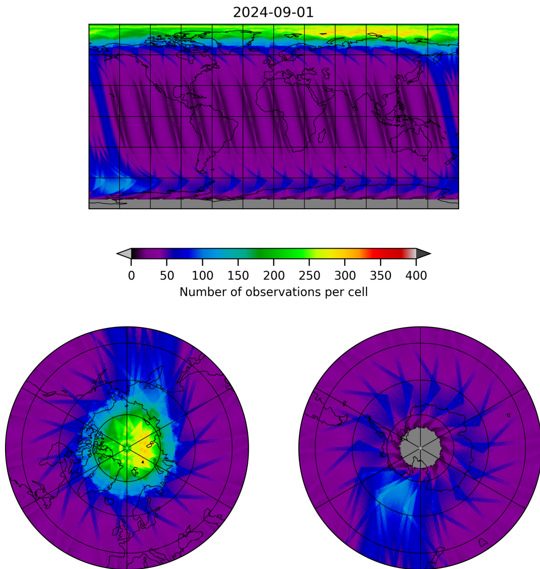
Figure 12: Map of the number of observations for 2024-09-01 to 2024-09-02
