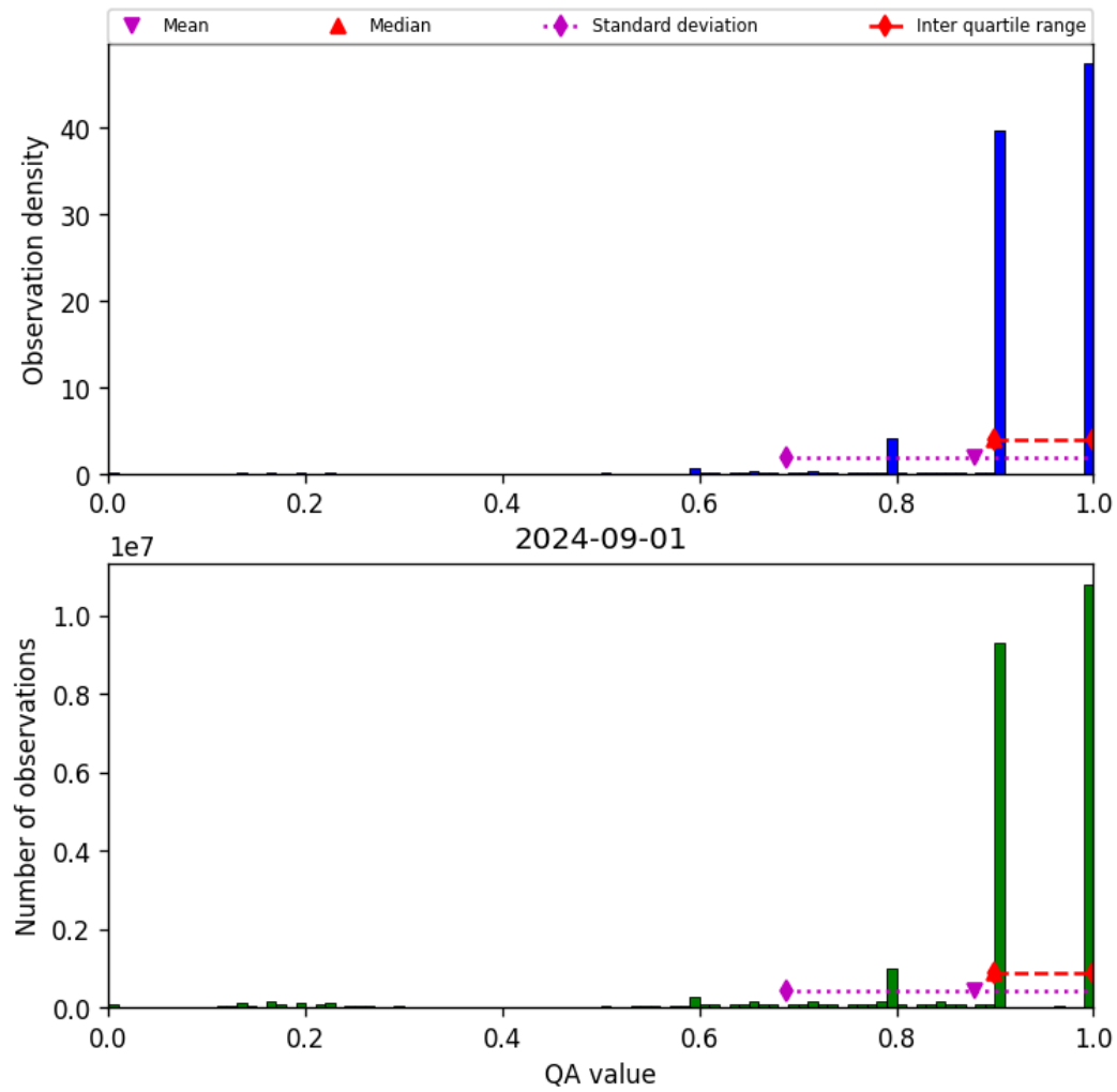
Figure 20: Histogram of “QA value” for 2024-09-01 to 2024-09-02
