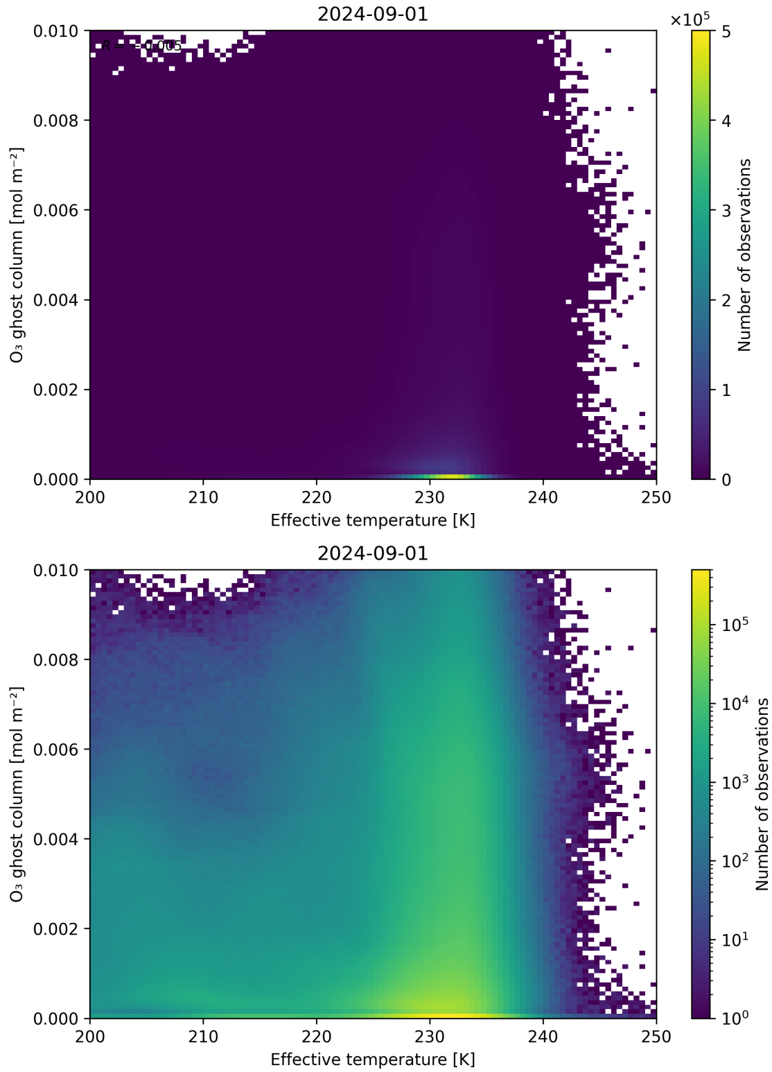
Figure 38: Scatter density plot of “Effective temperature” against “O 3 ghost column” for 2024-09-01 to 2024-09-02.
