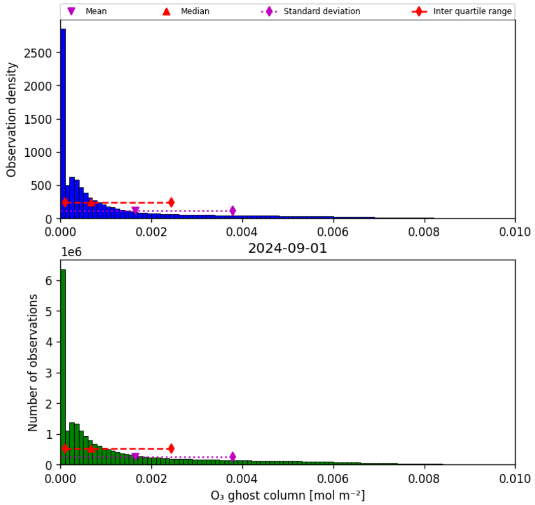
Figure 25: Histogram of “O 3 ghost column” for 2024-09-01 to 2024-09-02
