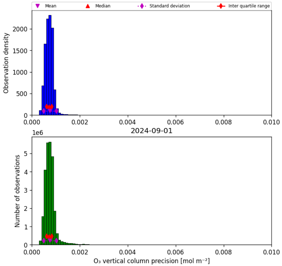
Figure 22: Histogram of “O 3 vertical column precision” for 2024-09-01 to 2024-09-02
