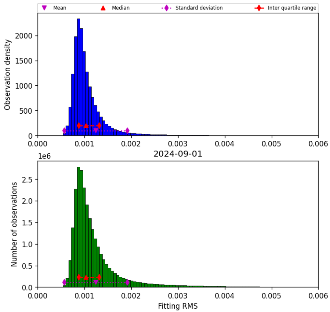
Figure 23: Histogram of “Fitting RMS” for 2024-09-01 to 2024-09-02
