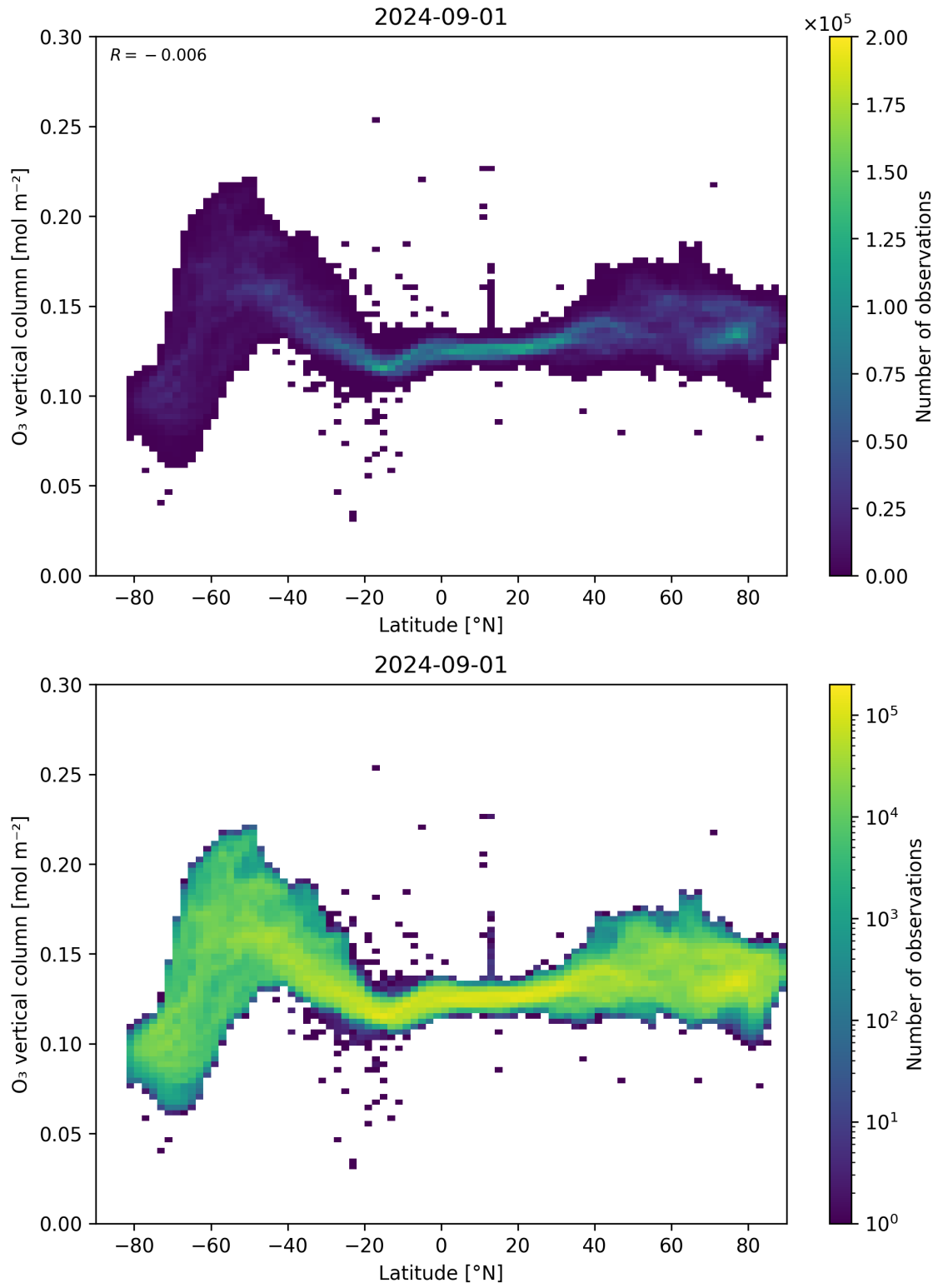
Figure 36: Scatter density plot of “Latitude” against “O 3 vertical column” for 2024-09-01 to 2024-09-02.
