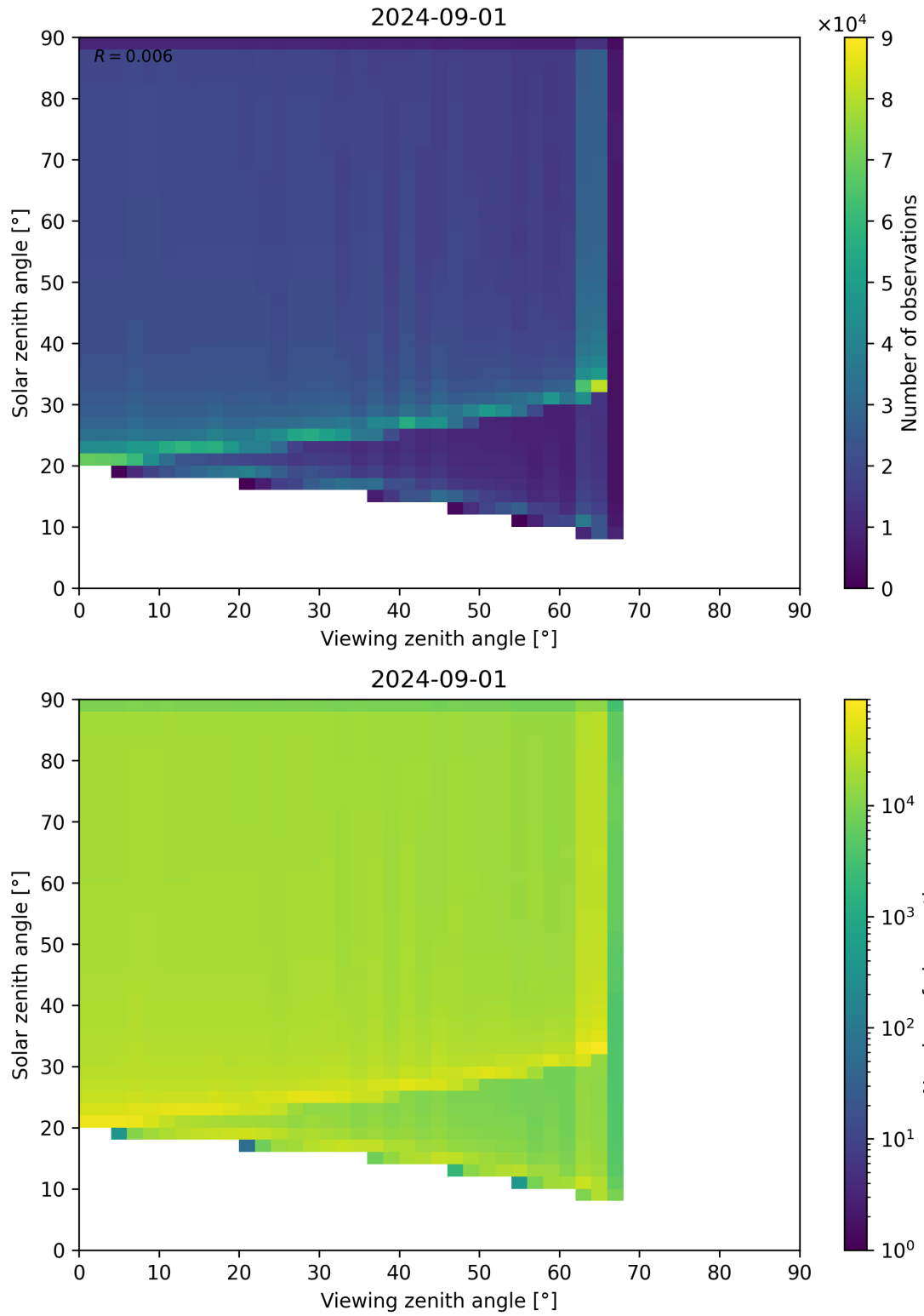
Figure 54: Scatter density plot of “Viewing zenith angle” against “Solar zenith angle” for 2024-09-01 to 2024-09-02.
