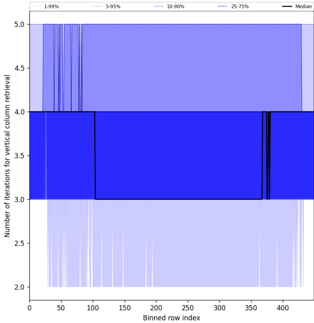
Figure 33: Along track statistics of “Number of iterations for vertical column retrieval” for 2024-09-01 to 2024-09-02
