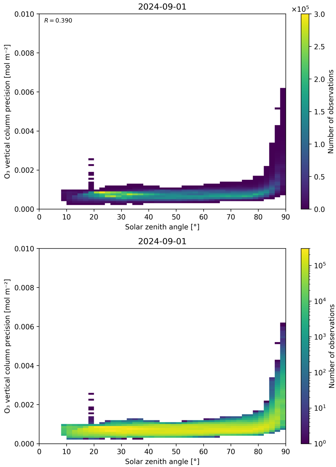
Figure 48: Scatter density plot of “Solar zenith angle” against “O 3 vertical column precision” for 2024-09-01 to 2024-09-02.
