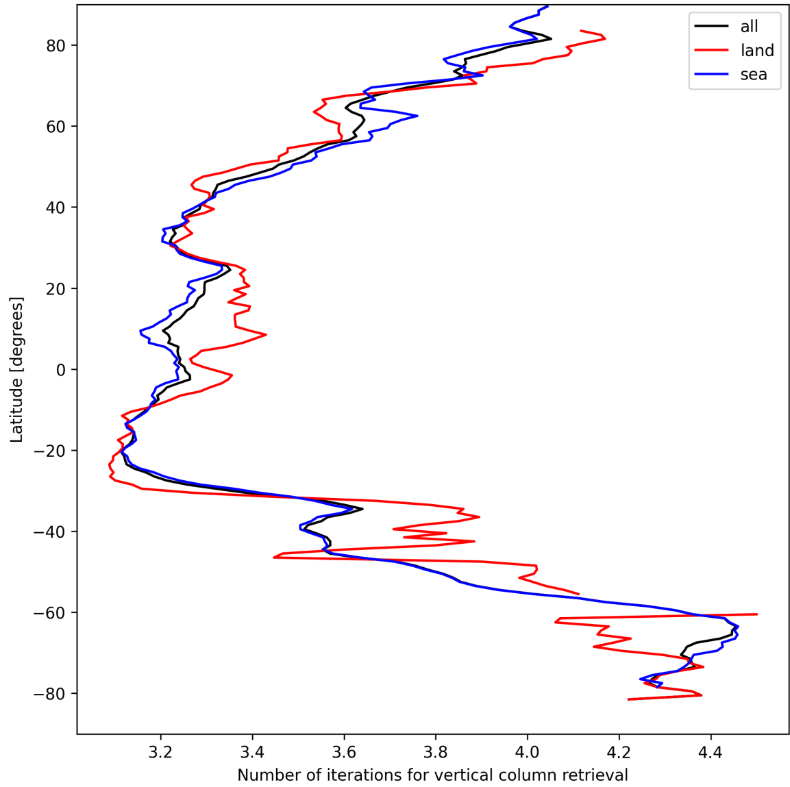
Figure 19: Zonal average of “Number of iterations for vertical column retrieval” for 2024-09-01 to 2024-09-02.
