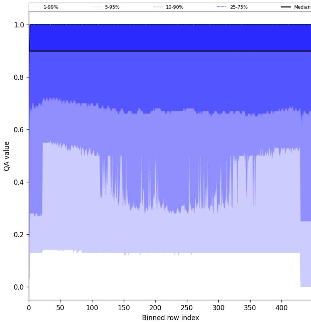
Figure 27: Along track statistics of “QA value” for 2024-09-01 to 2024-09-02
