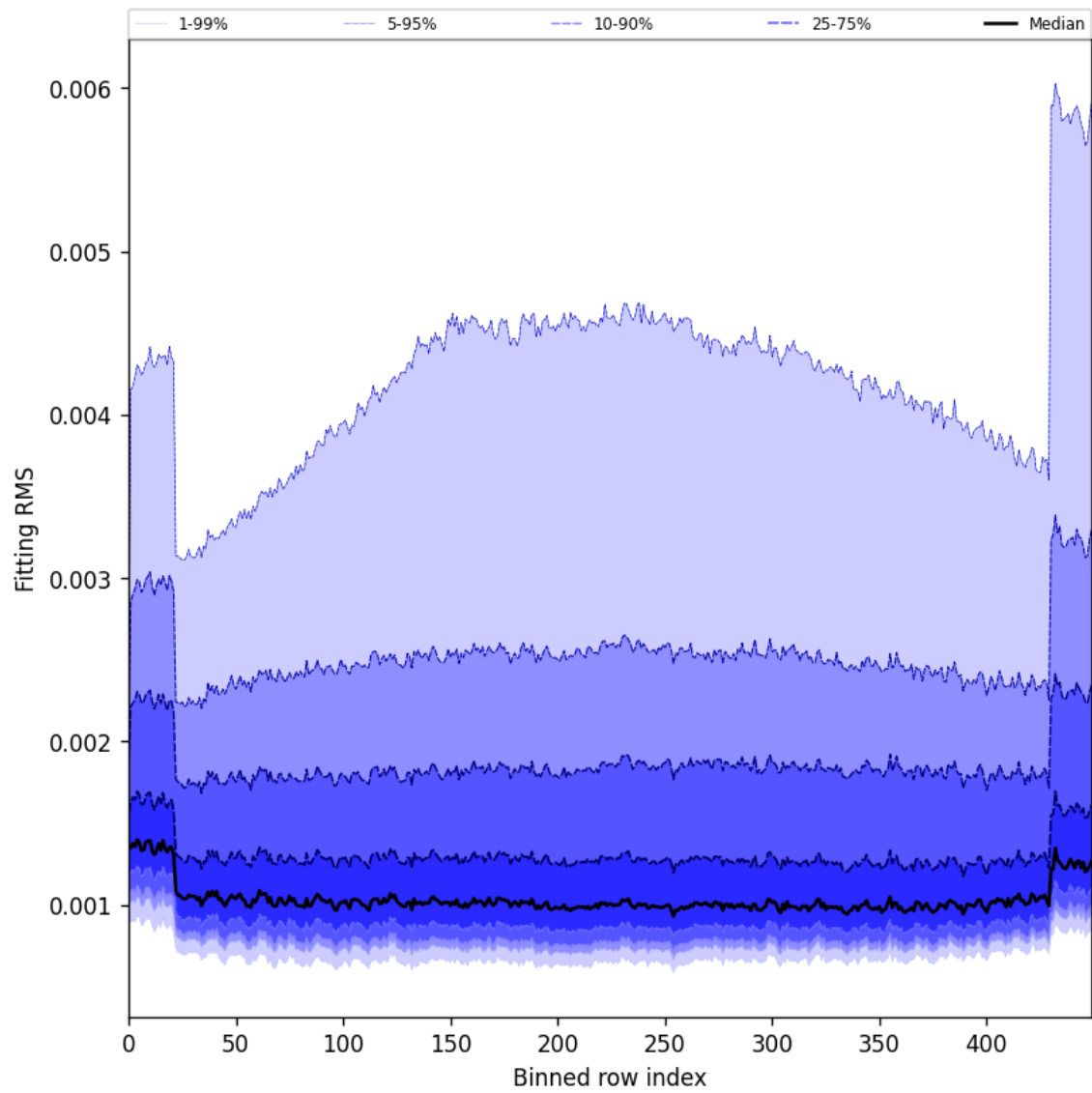
Figure 30: Along track statistics of “Fitting RMS” for 2024-09-01 to 2024-09-02
