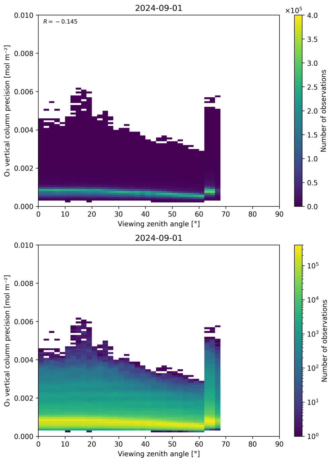
Figure 53: Scatter density plot of “Viewing zenith angle” against “O 3 vertical column precision” for 2024-09-01 to 2024-09-02.
