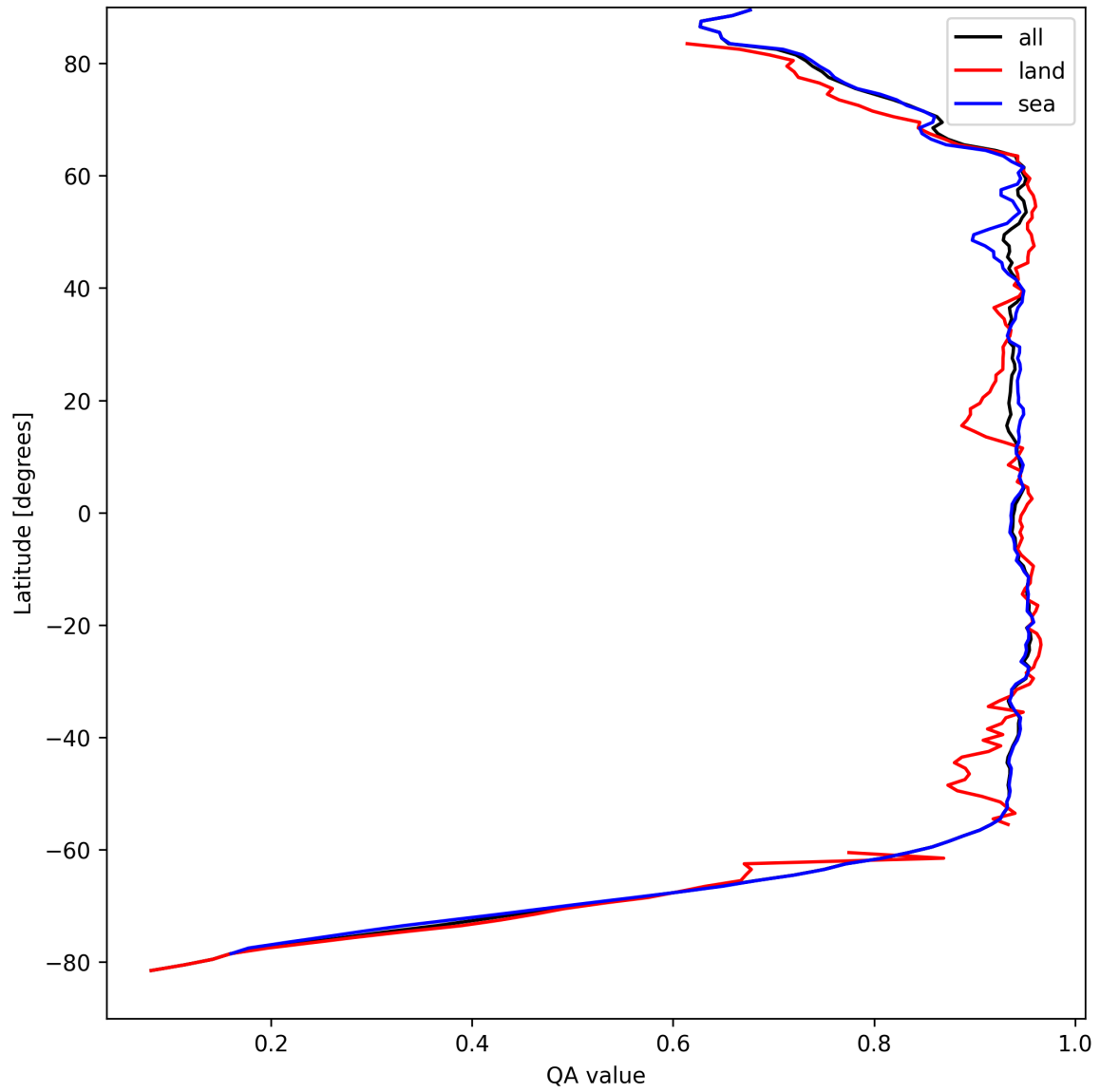
Figure 13: Zonal average of “QA value” for 2024-09-01 to 2024-09-02.
