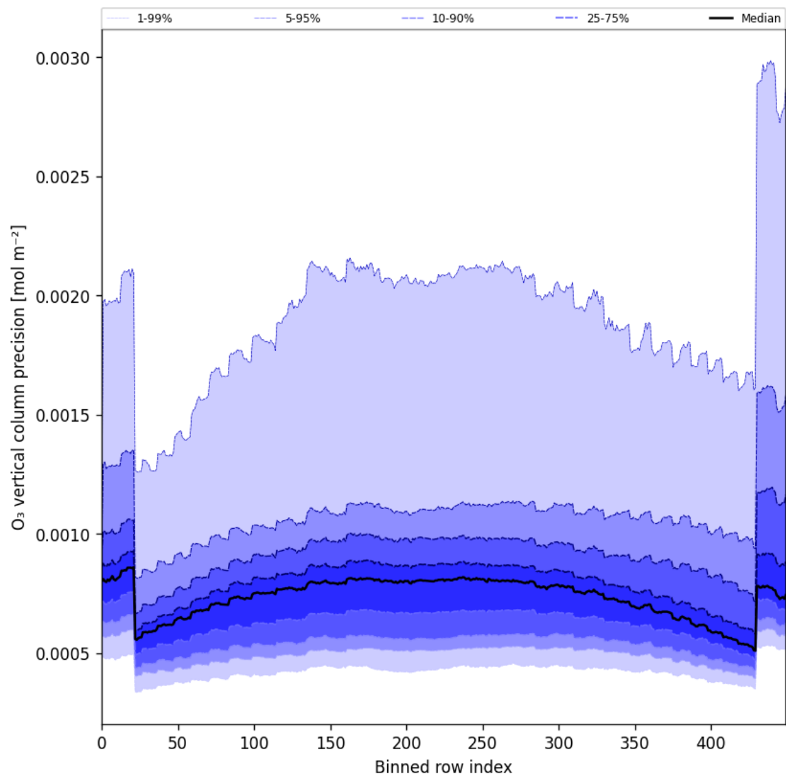
Figure 29: Along track statistics of “O 3 vertical column precision” for 2024-09-01 to 2024-09-02
