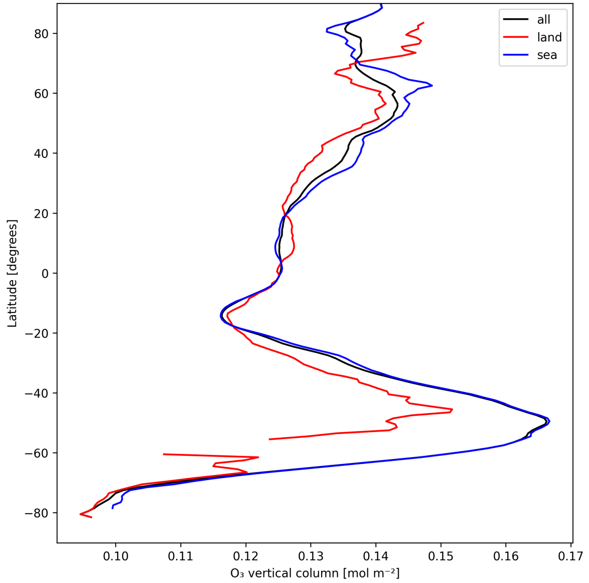
Figure 14: Zonal average of “O 3 vertical column” for 2024-09-01 to 2024-09-02.
