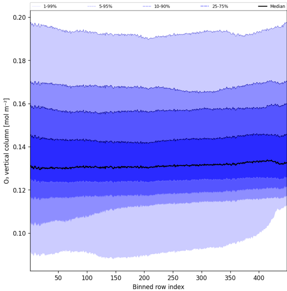
Figure 28: Along track statistics of “O 3 vertical column” for 2024-09-01 to 2024-09-03
