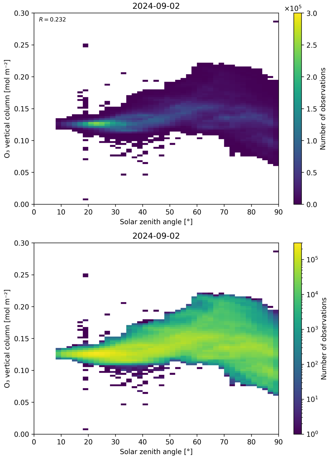
Figure 47: Scatter density plot of “Solar zenith angle” against “O 3 vertical column” for 2024-09-01 to 2024-09-03.
