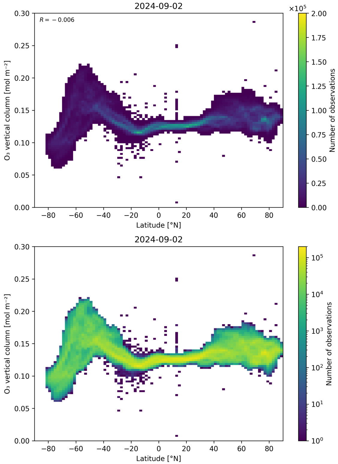
Figure 36: Scatter density plot of “Latitude” against “O 3 vertical column” for 2024-09-01 to 2024-09-03.
