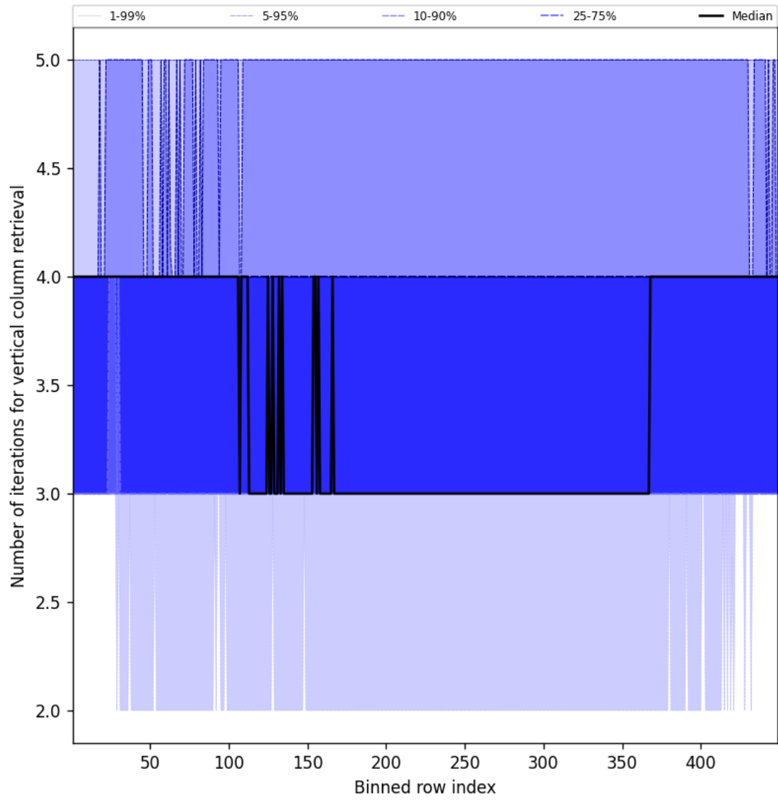
Figure 33: Along track statistics of “Number of iterations for vertical column retrieval” for 2024-09-01 to 2024-09-03
