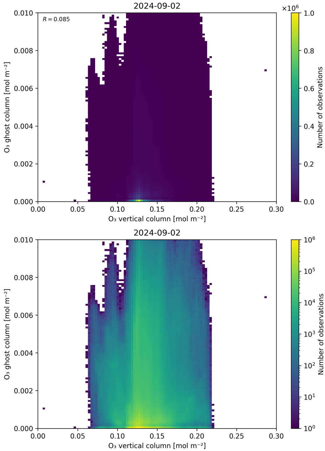
Figure 40: Scatter density plot of “ \text{O}_3 vertical column” against “ \text{O}_3 ghost column” for 2024-09-01 to 2024-09-03.
