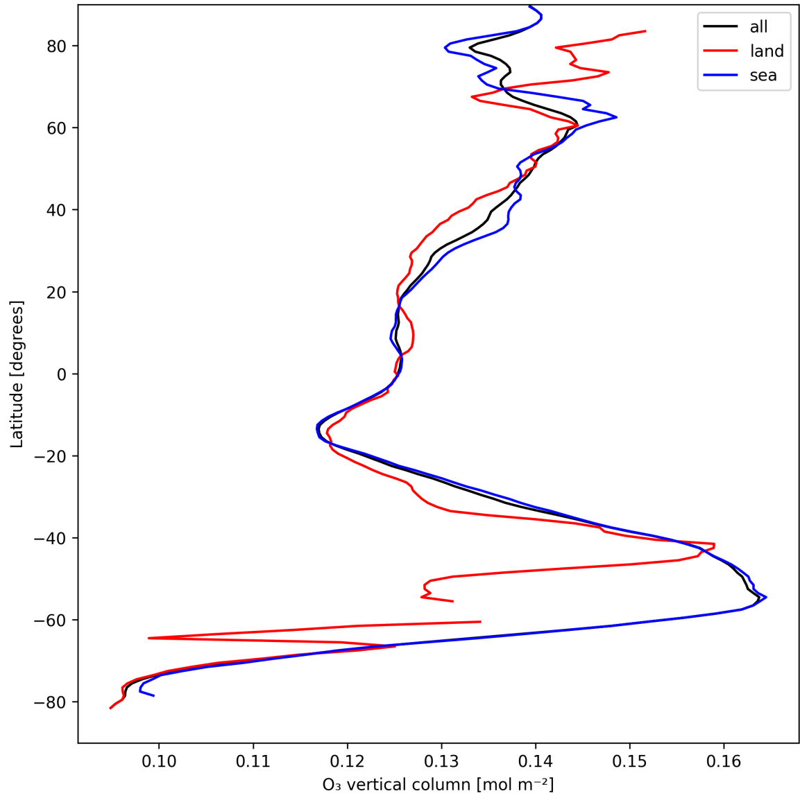
Figure 14: Zonal average of “O 3 vertical column” for 2024-09-01 to 2024-09-03.
