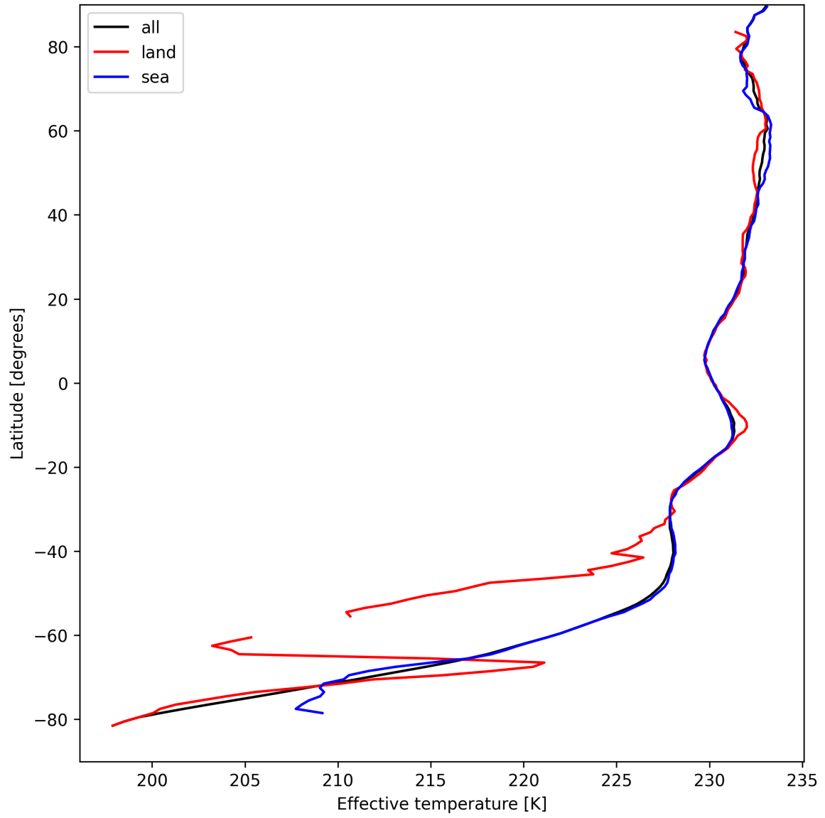
Figure 17: Zonal average of “Effective temperature” for 2024-09-01 to 2024-09-03.
