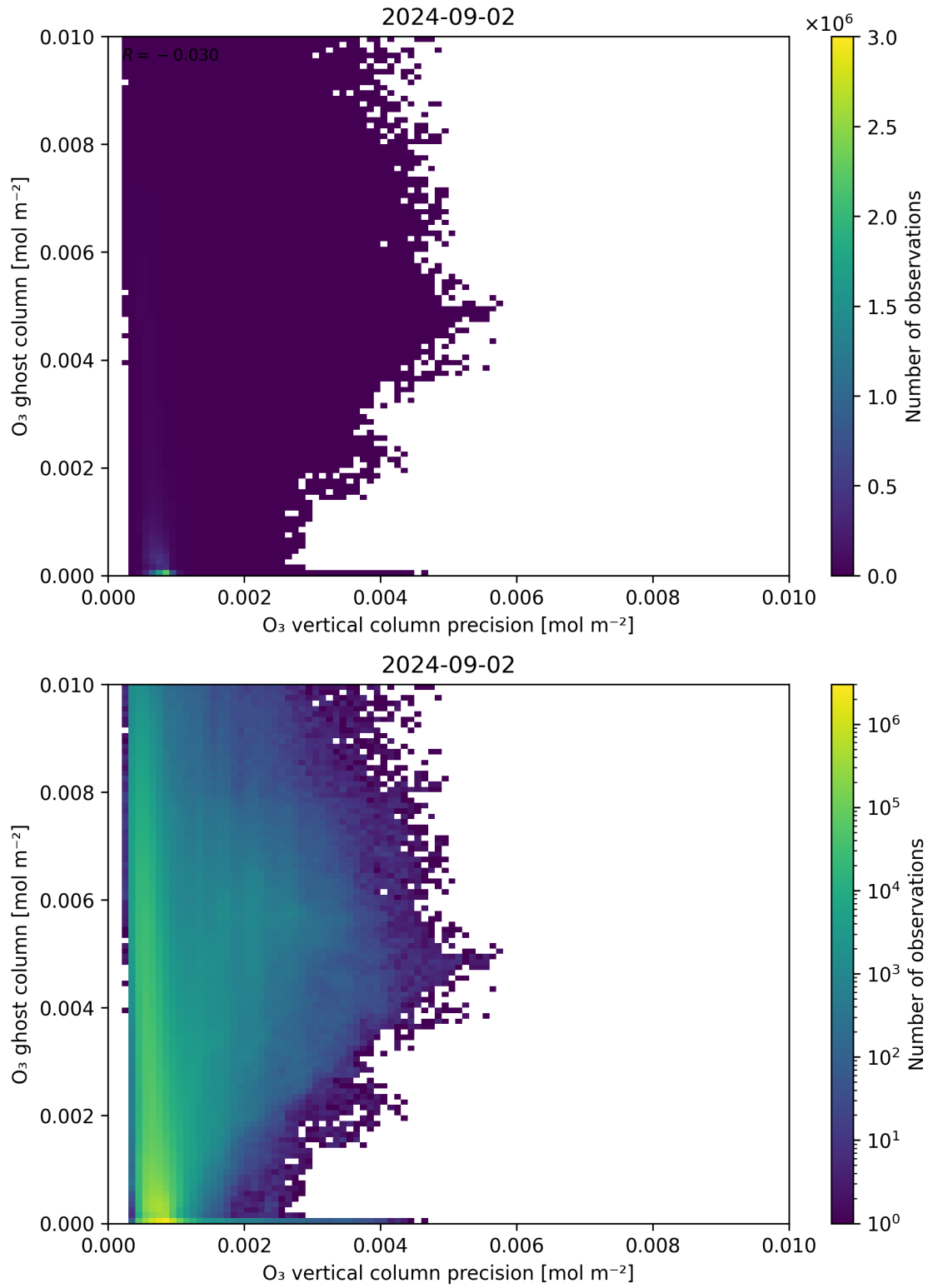
Figure 43: Scatter density plot of “ \text{O}_3 vertical column precision” against “ \text{O}_3 ghost column” for 2024-09-01 to 2024-09-03.
