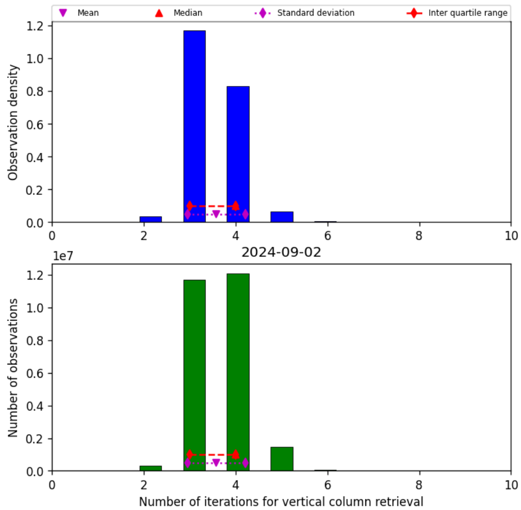
Figure 26: Histogram of “Number of iterations for vertical column retrieval” for 2024-09-01 to 2024-09-03
