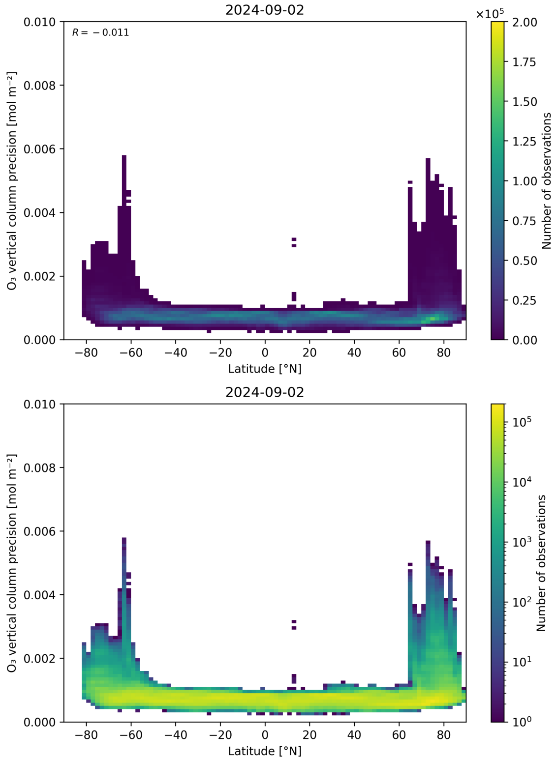
Figure 37: Scatter density plot of “Latitude” against “O 3 vertical column precision” for 2024-09-01 to 2024-09-03.
