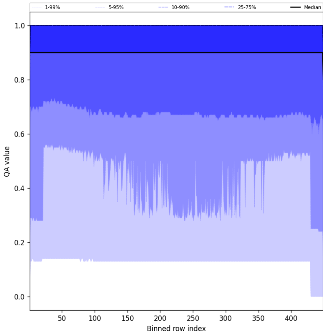
Figure 27: Along track statistics of “QA value” for 2024-09-01 to 2024-09-03
