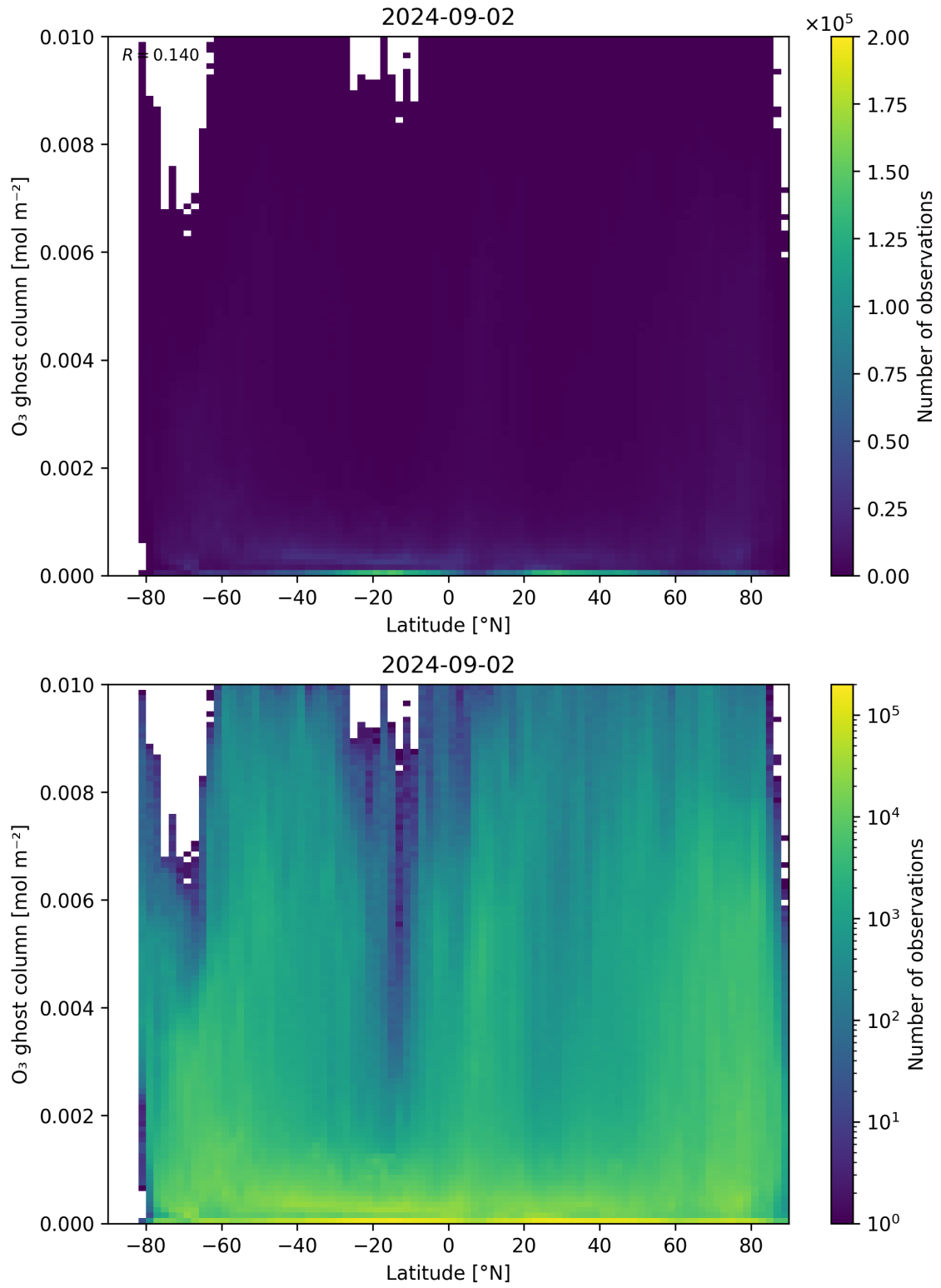
Figure 35: Scatter density plot of “Latitude” against “O 3 ghost column” for 2024-09-01 to 2024-09-03.
