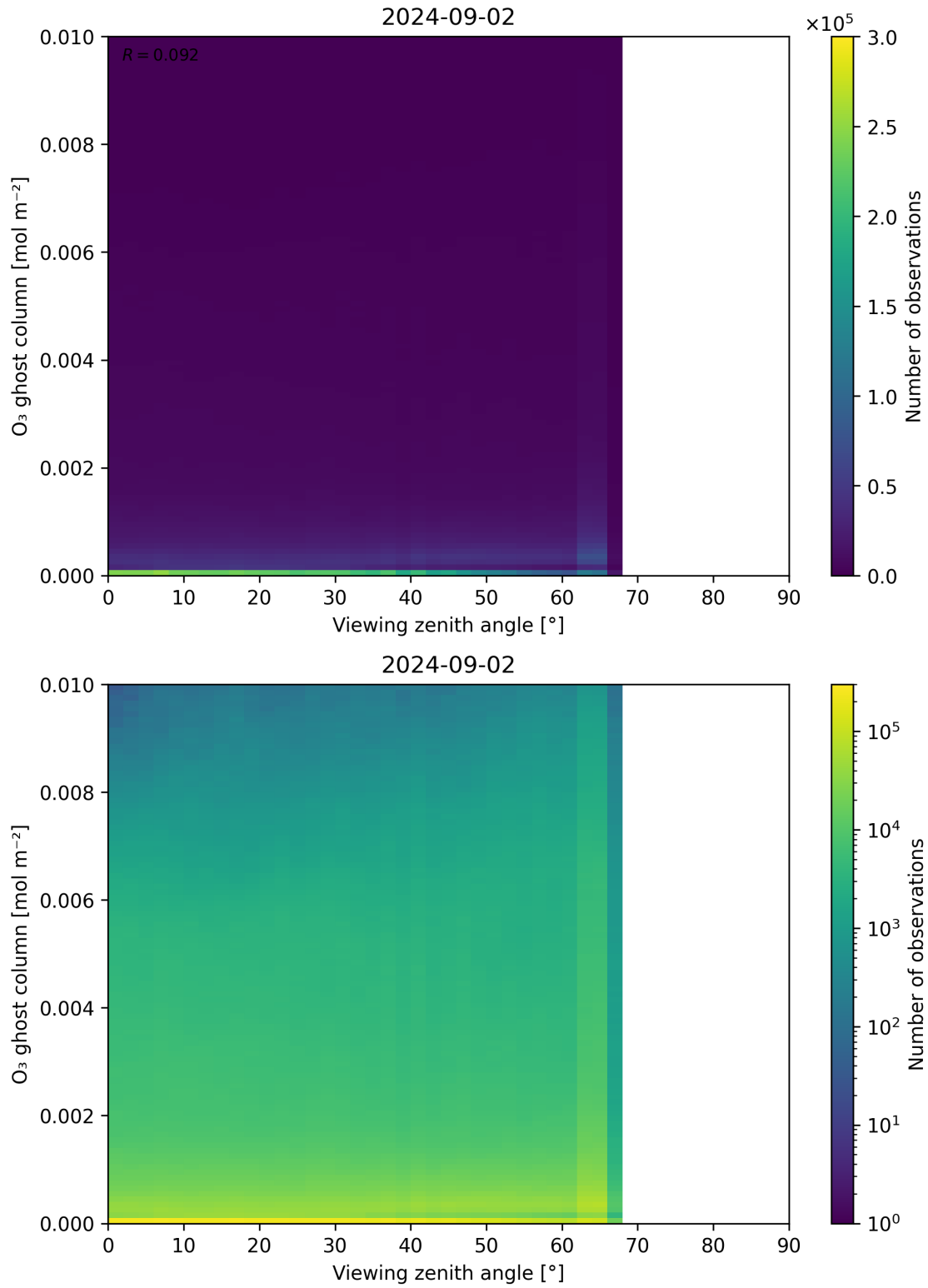
Figure 51: Scatter density plot of “Viewing zenith angle” against “O 3 ghost column” for 2024-09-01 to 2024-09-03.
