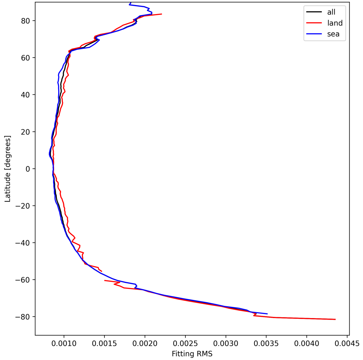
Figure 16: Zonal average of “Fitting RMS” for 2024-09-01 to 2024-09-03.
