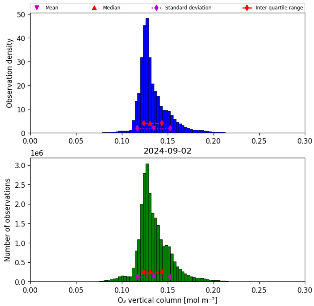
Figure 21: Histogram of “O 3 vertical column” for 2024-09-01 to 2024-09-03
