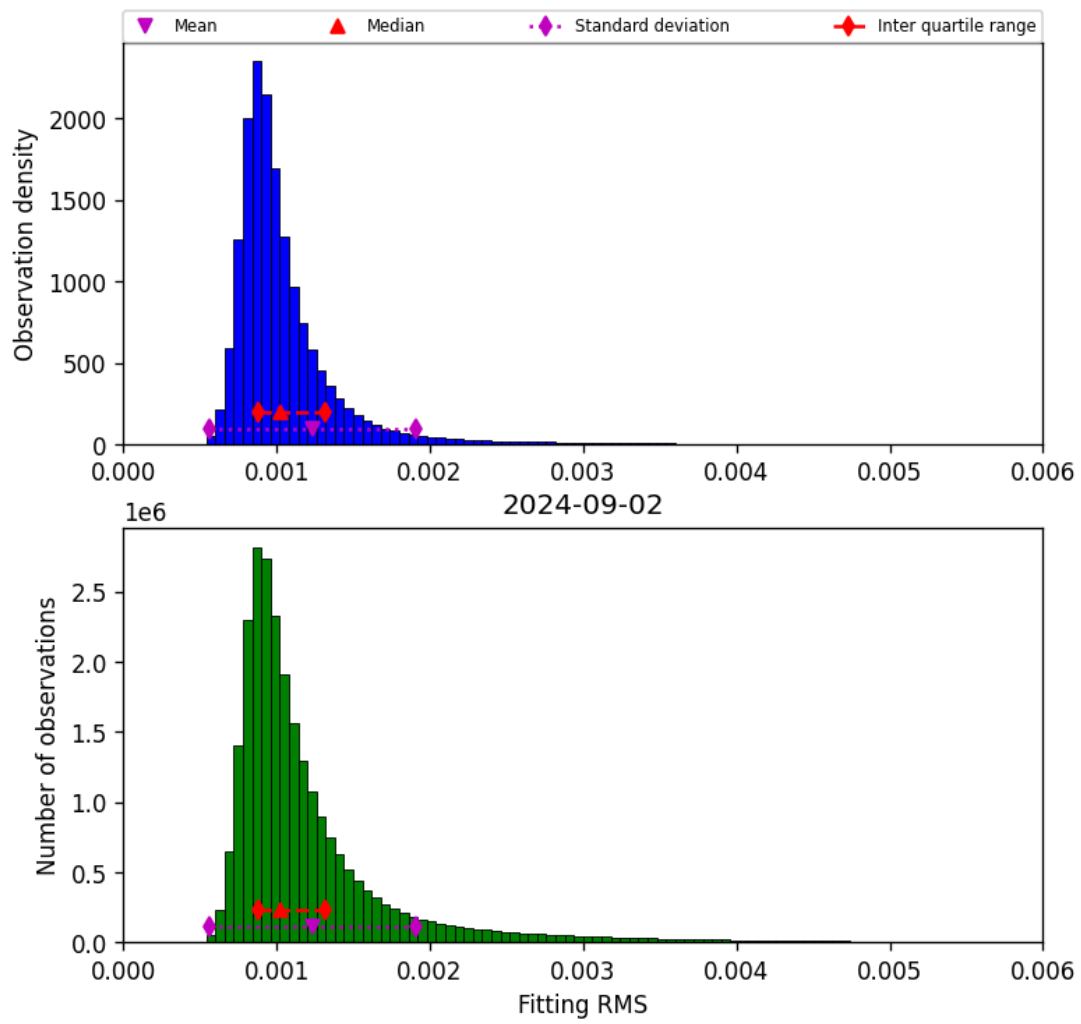
Figure 23: Histogram of “Fitting RMS” for 2024-09-01 to 2024-09-03
