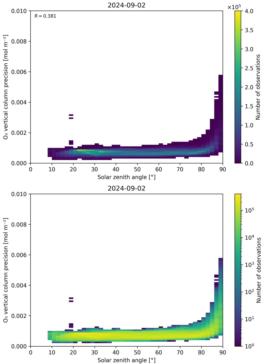
Figure 48: Scatter density plot of “Solar zenith angle” against “O 3 vertical column precision” for 2024-09-01 to 2024-09-03.
