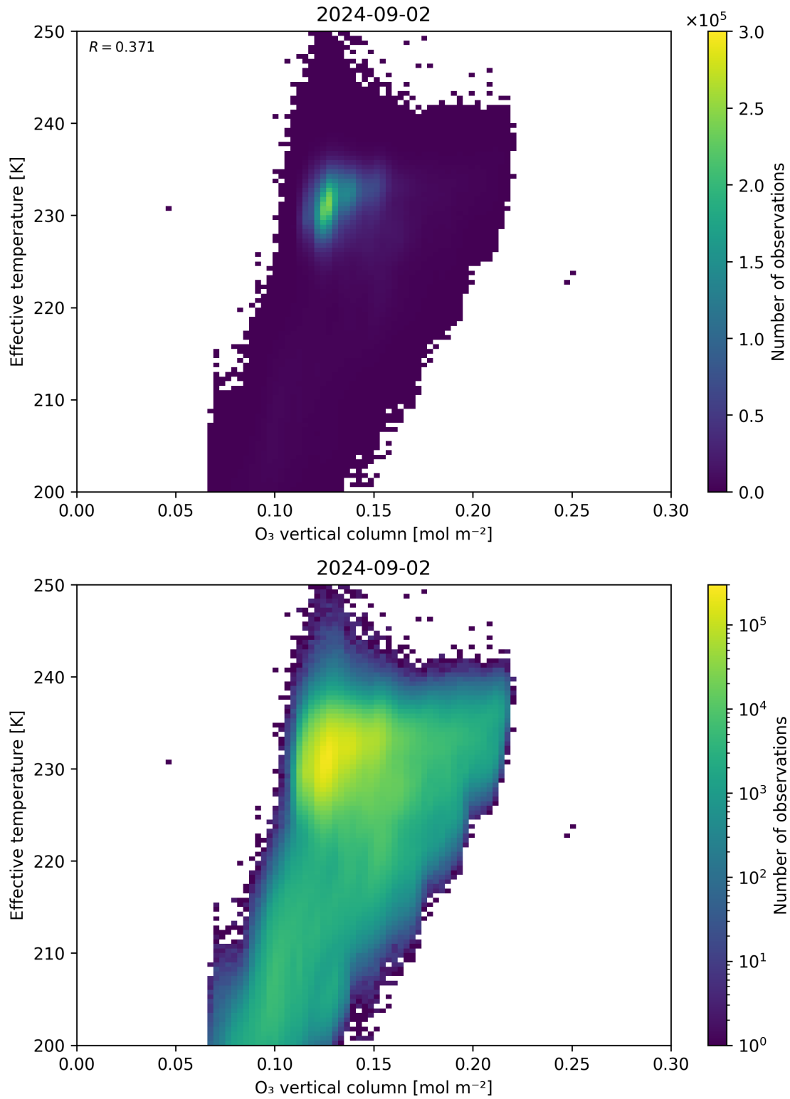
Figure 39: Scatter density plot of “O 3 vertical column” against “Effective temperature” for 2024-09-01 to 2024-09-03.
