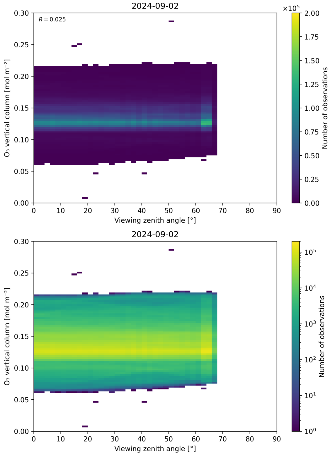
Figure 52: Scatter density plot of “Viewing zenith angle” against “O 3 vertical column” for 2024-09-01 to 2024-09-03.
