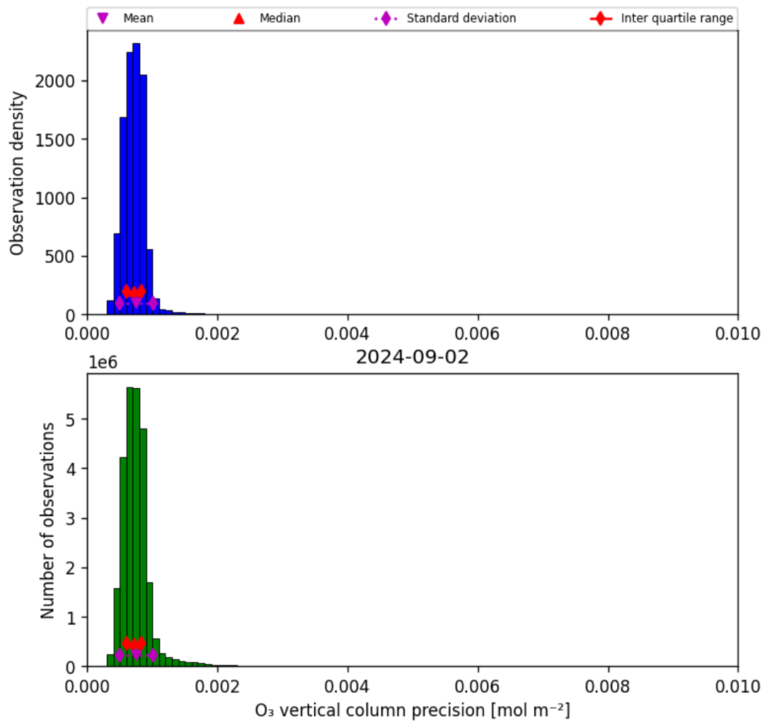
Figure 22: Histogram of “O 3 vertical column precision” for 2024-09-01 to 2024-09-03
