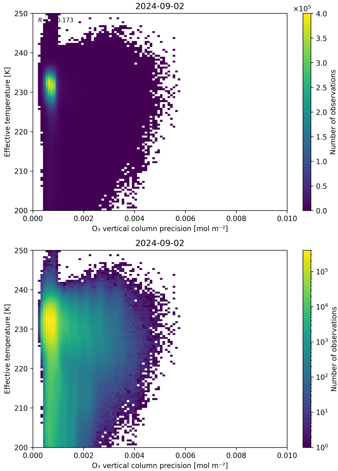
Figure 42: Scatter density plot of “O 3 vertical column precision” against “Effective temperature” for 2024-09-01 to 2024-09-03.
