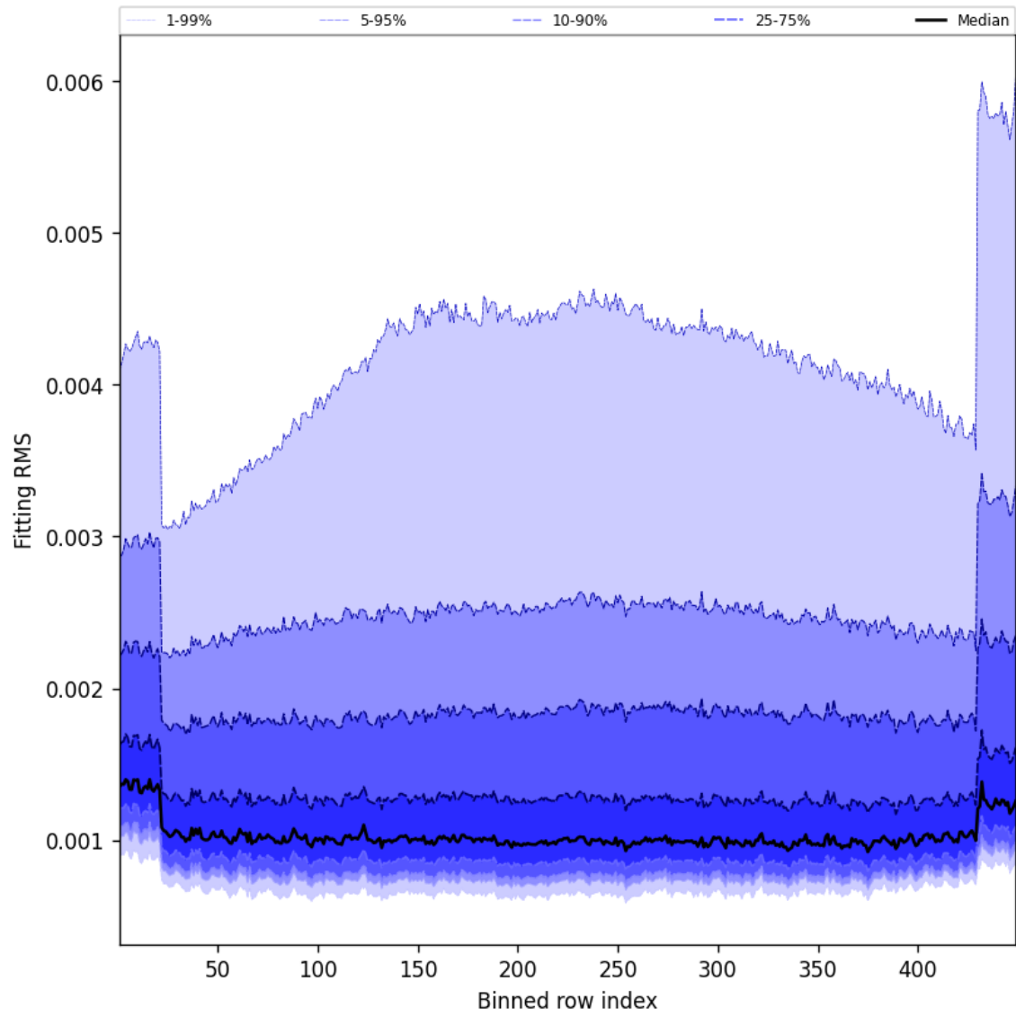
Figure 30: Along track statistics of “Fitting RMS” for 2024-09-01 to 2024-09-03
