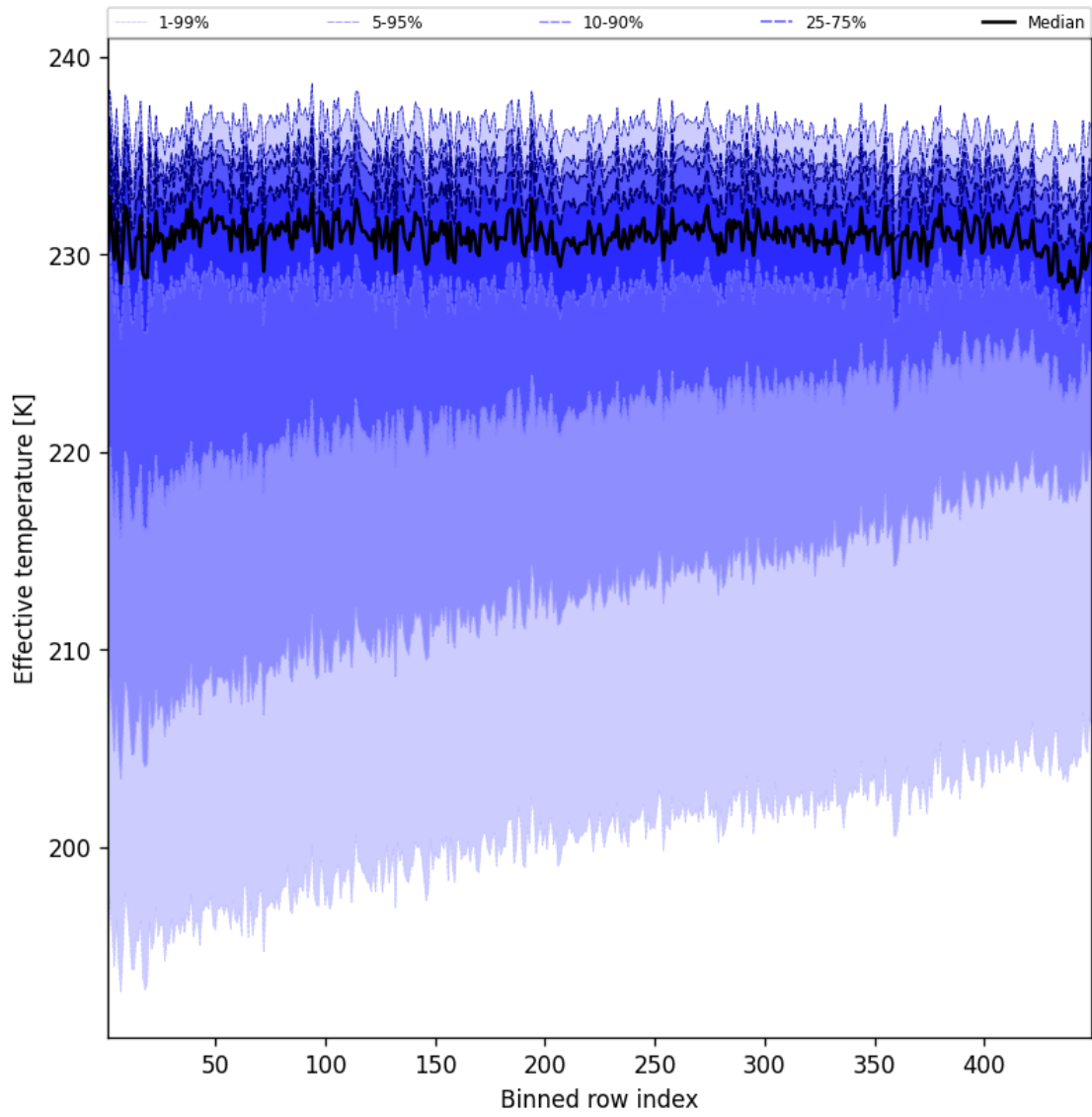
Figure 31: Along track statistics of “Effective temperature” for 2024-09-01 to 2024-09-03
