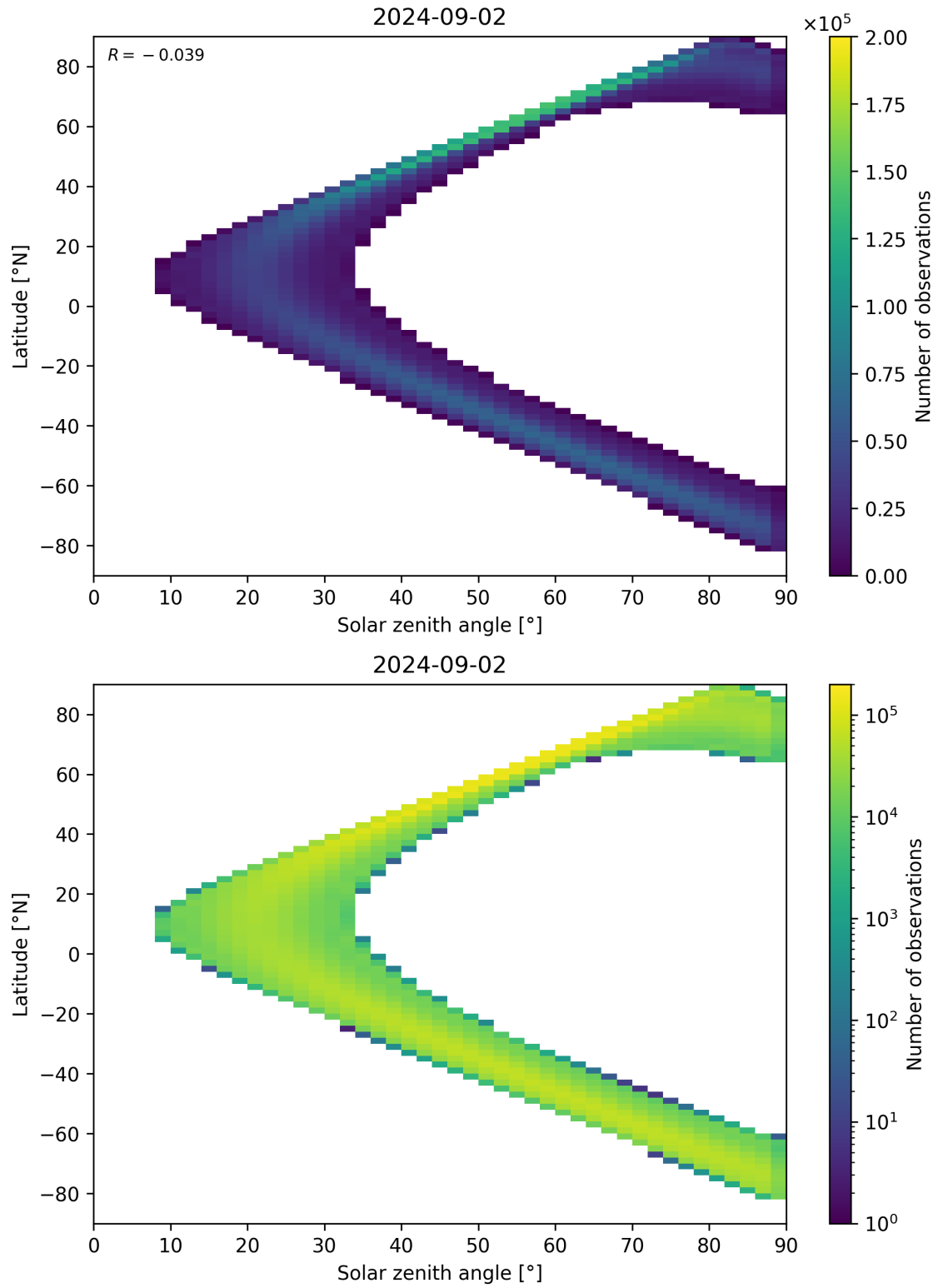
Figure 44: Scatter density plot of “Solar zenith angle” against “Latitude” for 2024-09-01 to 2024-09-03.
