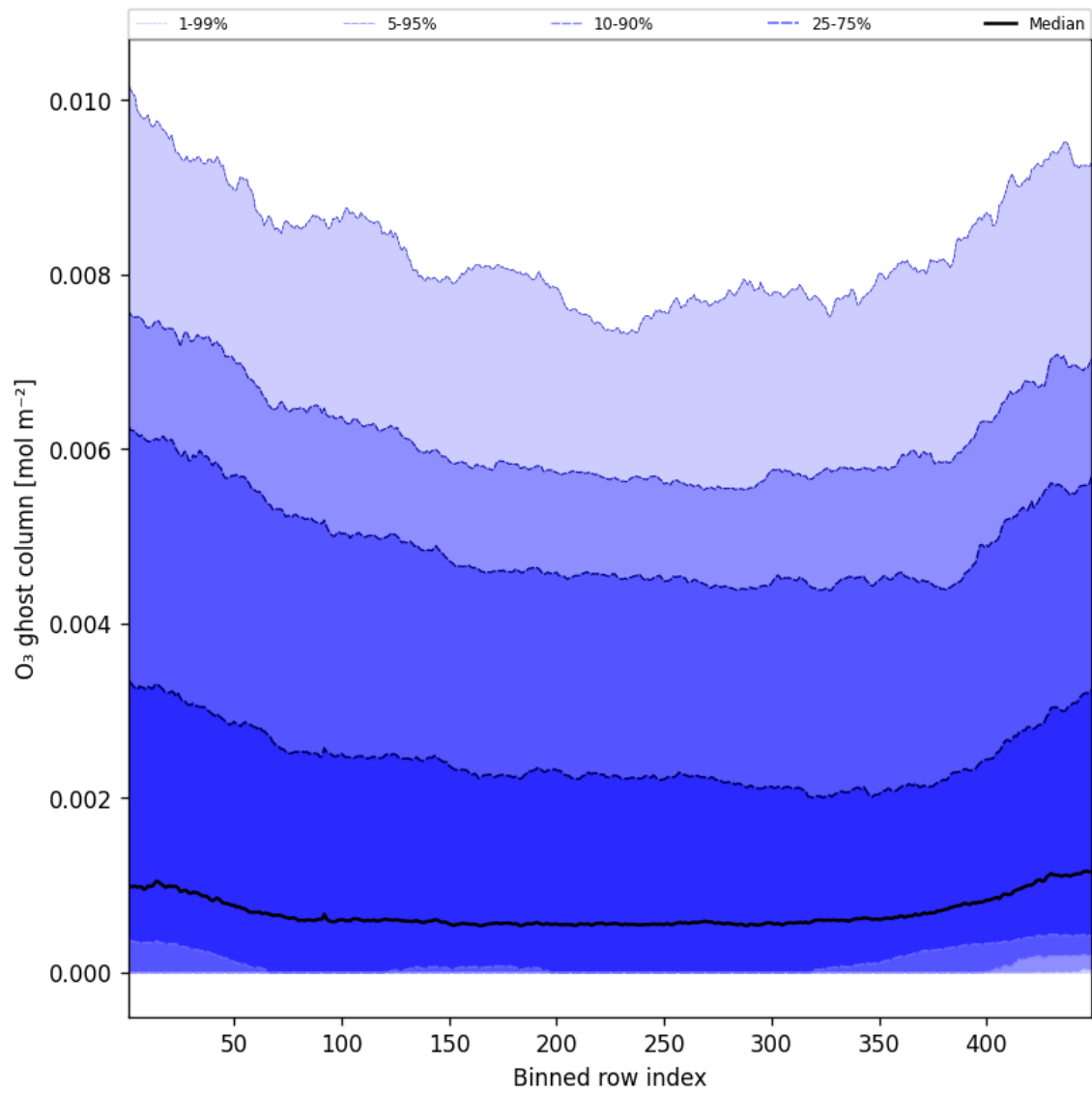
Figure 32: Along track statistics of “O 3 ghost column” for 2024-09-01 to 2024-09-03
