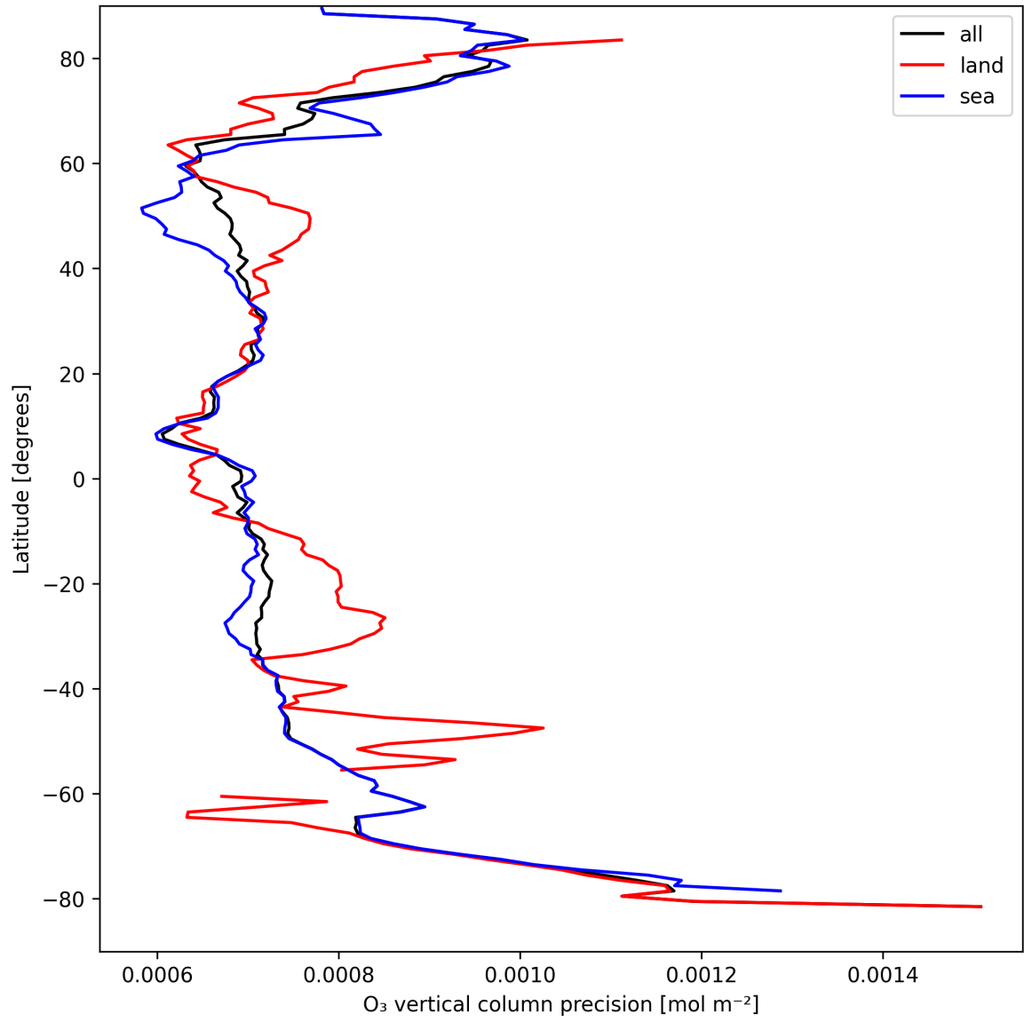
Figure 15: Zonal average of "O 3 vertical column precision" for 2024-09-01 to 2024-09-03.
