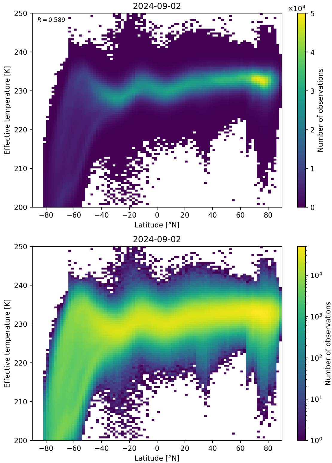
Figure 34: Scatter density plot of “Latitude” against “Effective temperature” for 2024-09-01 to 2024-09-03.
