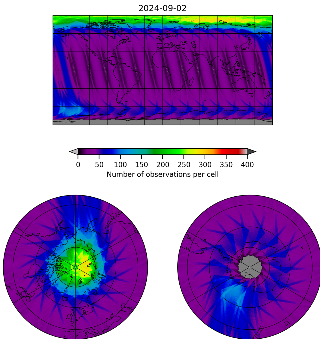
Figure 12: Map of the number of observations for 2024-09-01 to 2024-09-03
