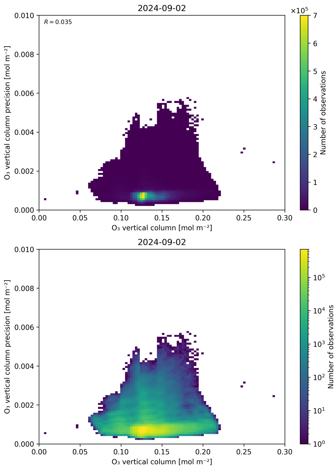
Figure 41: Scatter density plot of “O 3 vertical column” against “O 3 vertical column precision” for 2024-09-01 to 2024-09-03.
