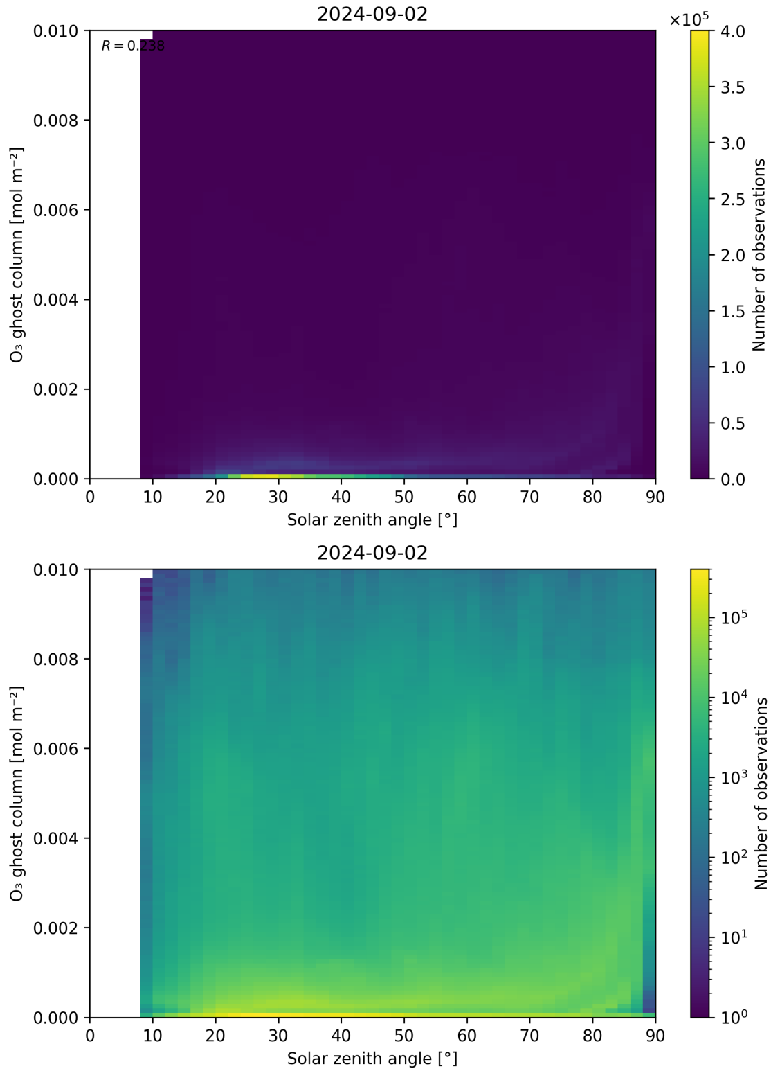
Figure 46: Scatter density plot of “Solar zenith angle” against “O 3 ghost column” for 2024-09-01 to 2024-09-03.
