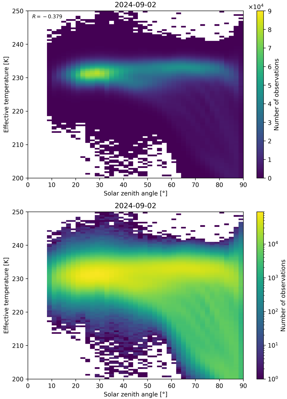
Figure 45: Scatter density plot of “Solar zenith angle” against “Effective temperature” for 2024-09-01 to 2024-09-03.
