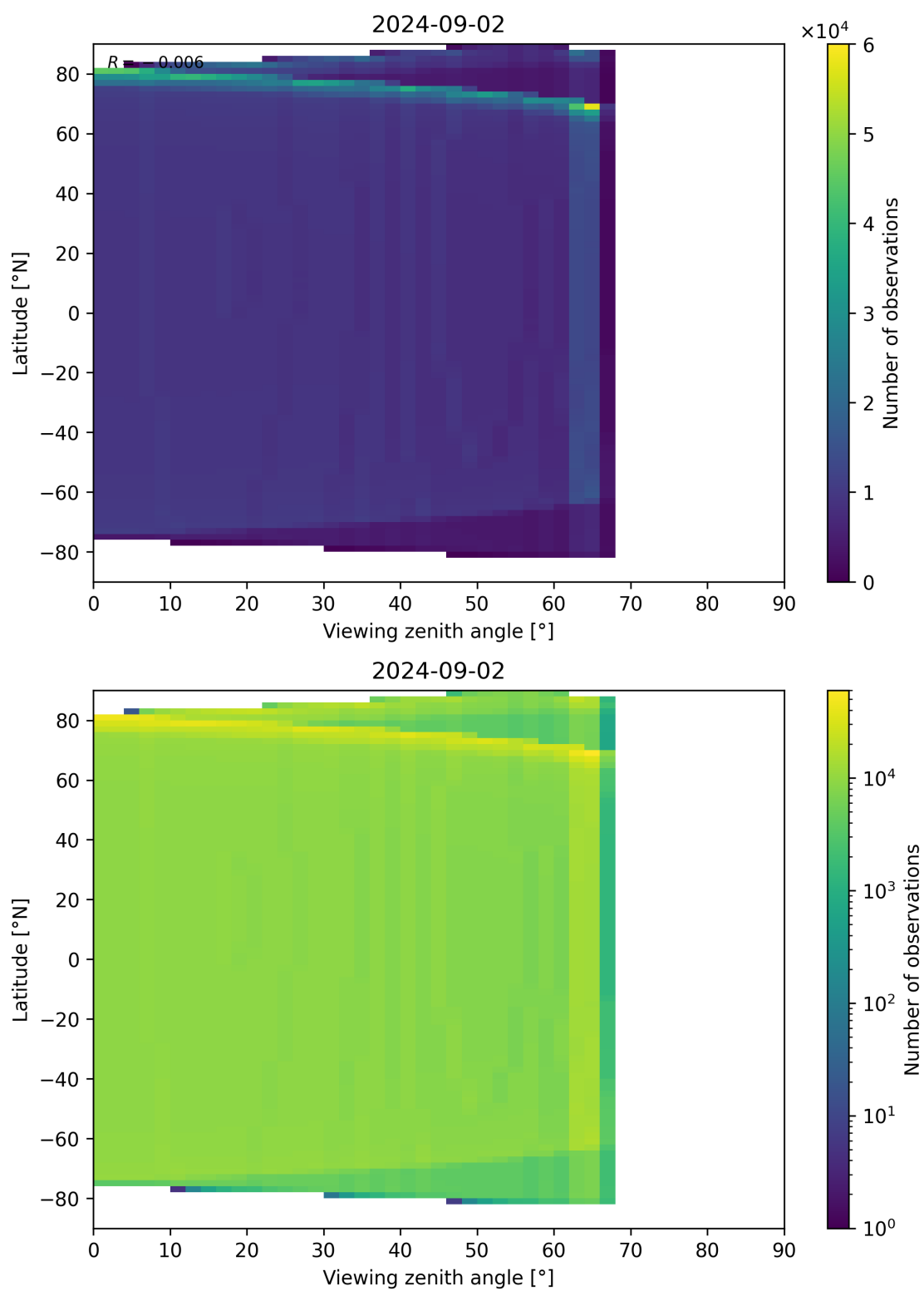
Figure 49: Scatter density plot of “Viewing zenith angle” against “Latitude” for 2024-09-01 to 2024-09-03.
