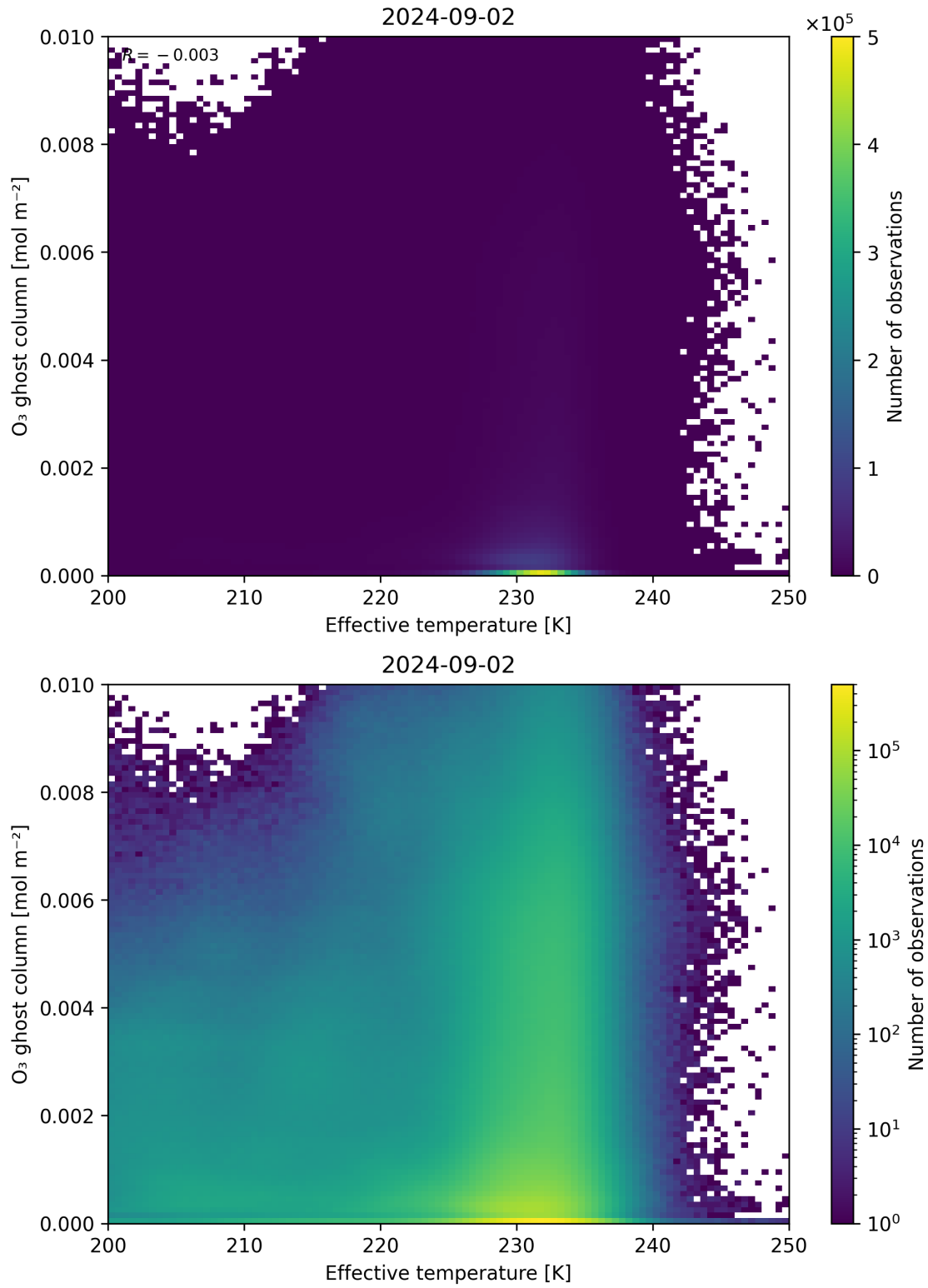
Figure 38: Scatter density plot of “Effective temperature” against “O 3 ghost column” for 2024-09-01 to 2024-09-03.
