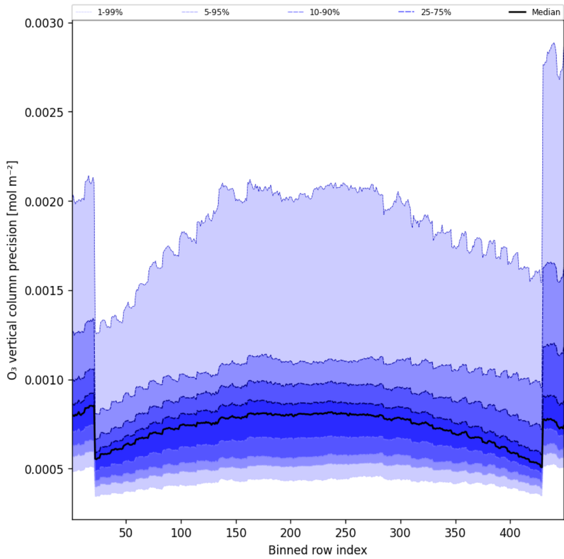
Figure 29: Along track statistics of “O 3 vertical column precision” for 2024-09-01 to 2024-09-03
