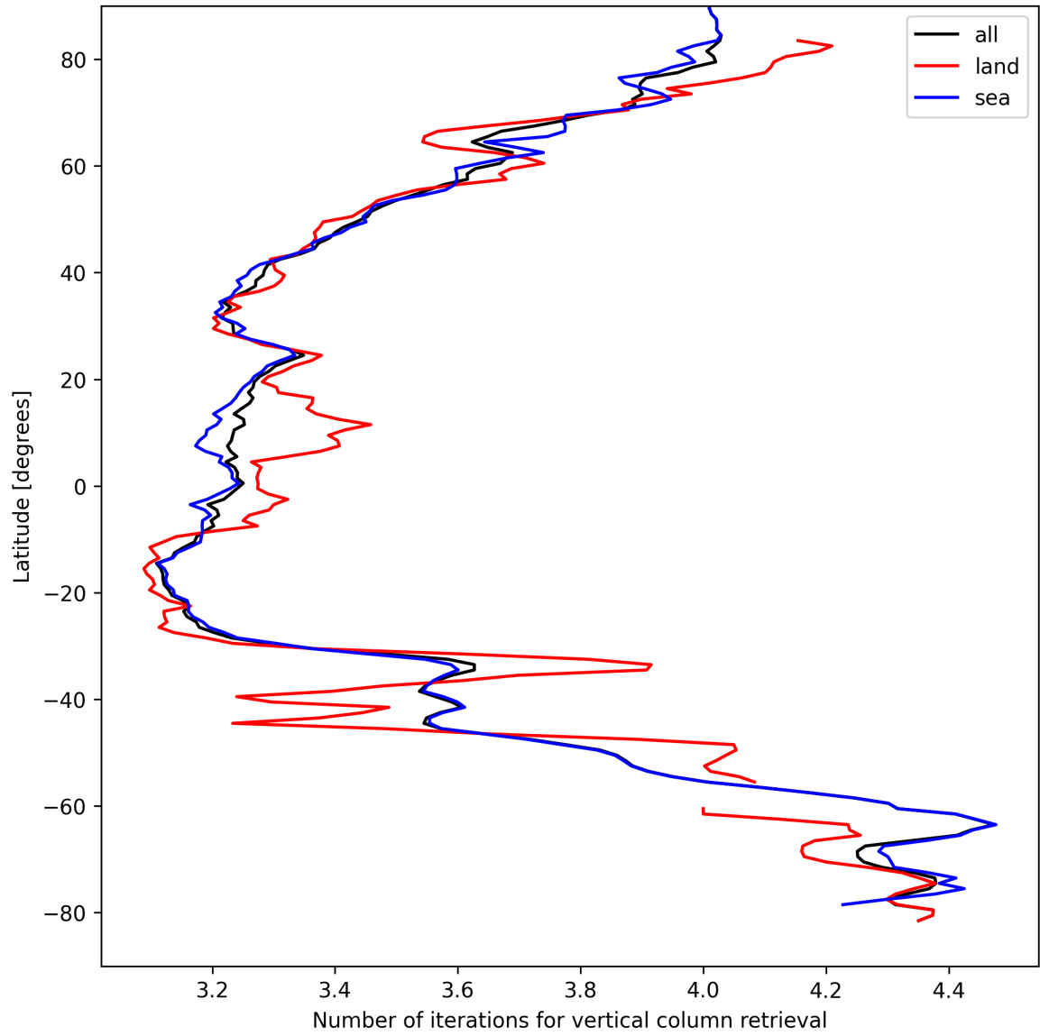
Figure 19: Zonal average of “Number of iterations for vertical column retrieval” for 2024-09-01 to 2024-09-03.
