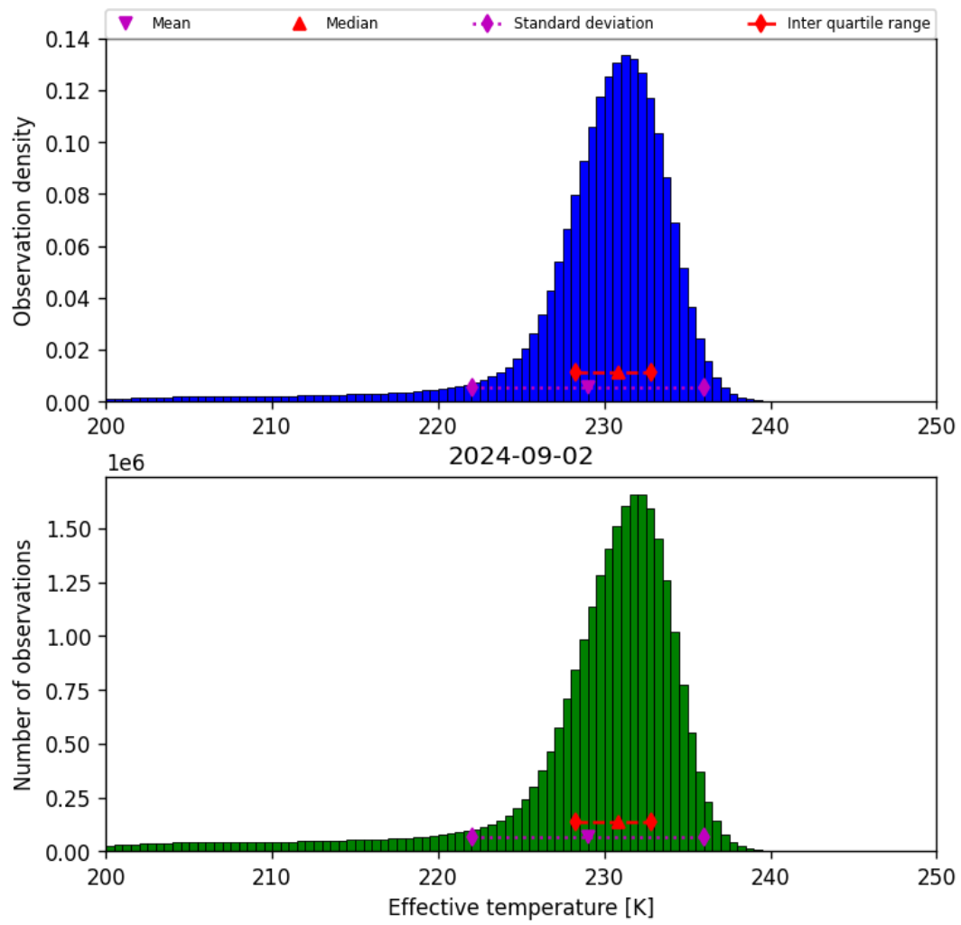
Figure 24: Histogram of “Effective temperature” for 2024-09-01 to 2024-09-03
