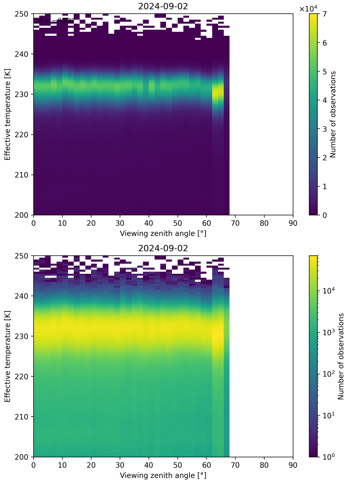
Figure 50: Scatter density plot of “Viewing zenith angle” against “Effective temperature” for 2024-09-01 to 2024-09-03.
