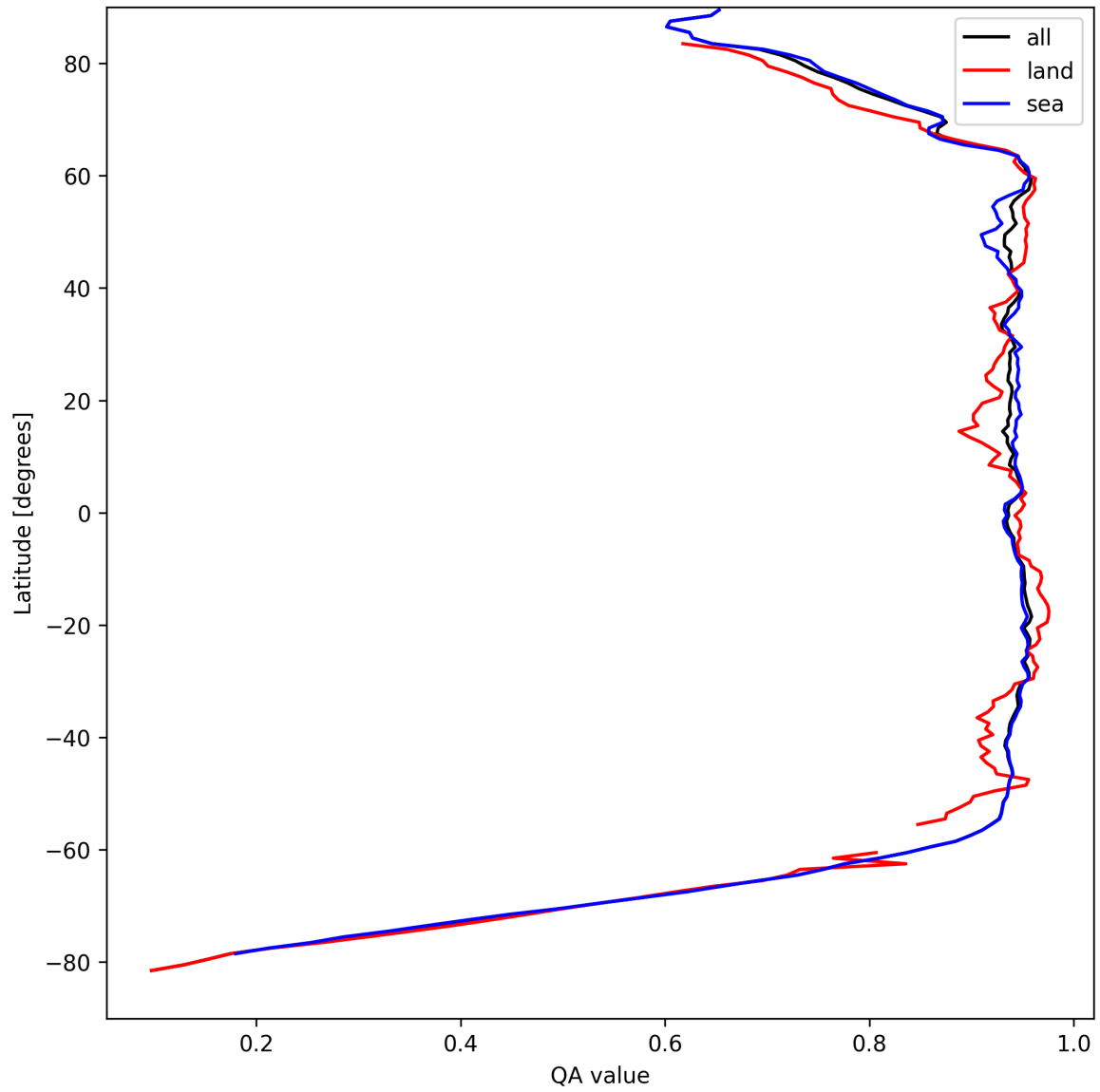
Figure 13: Zonal average of “QA value” for 2024-09-01 to 2024-09-03.
