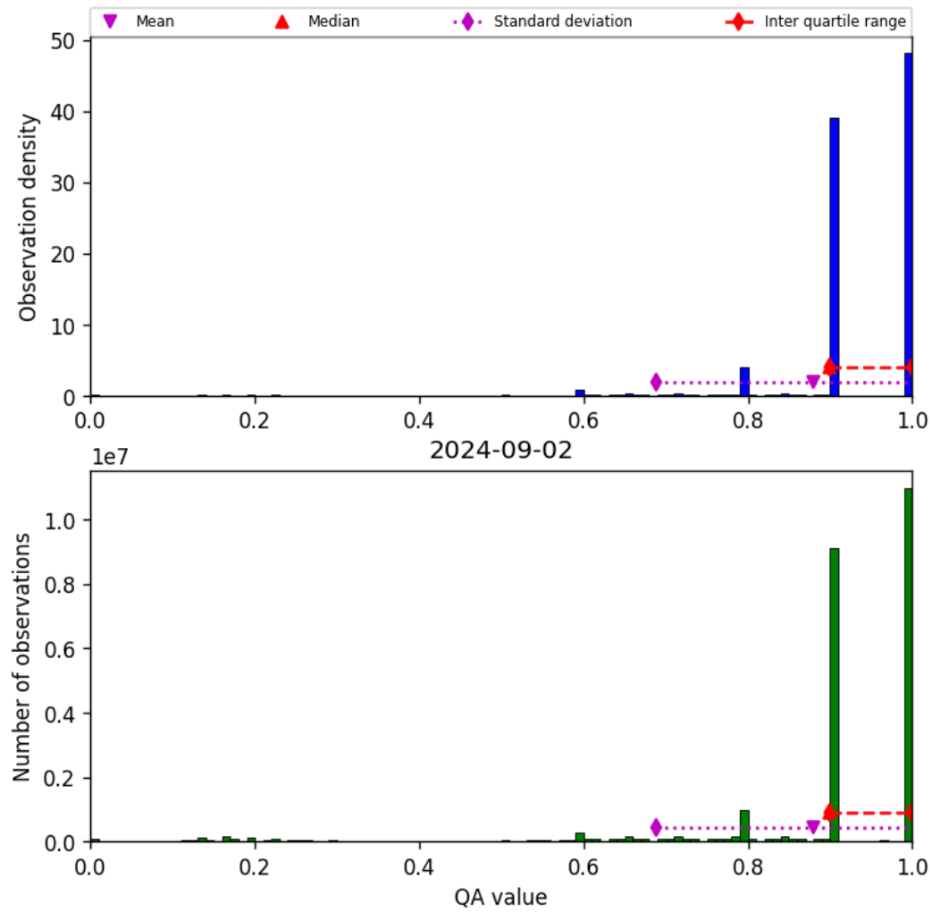
Figure 20: Histogram of “QA value” for 2024-09-01 to 2024-09-03
