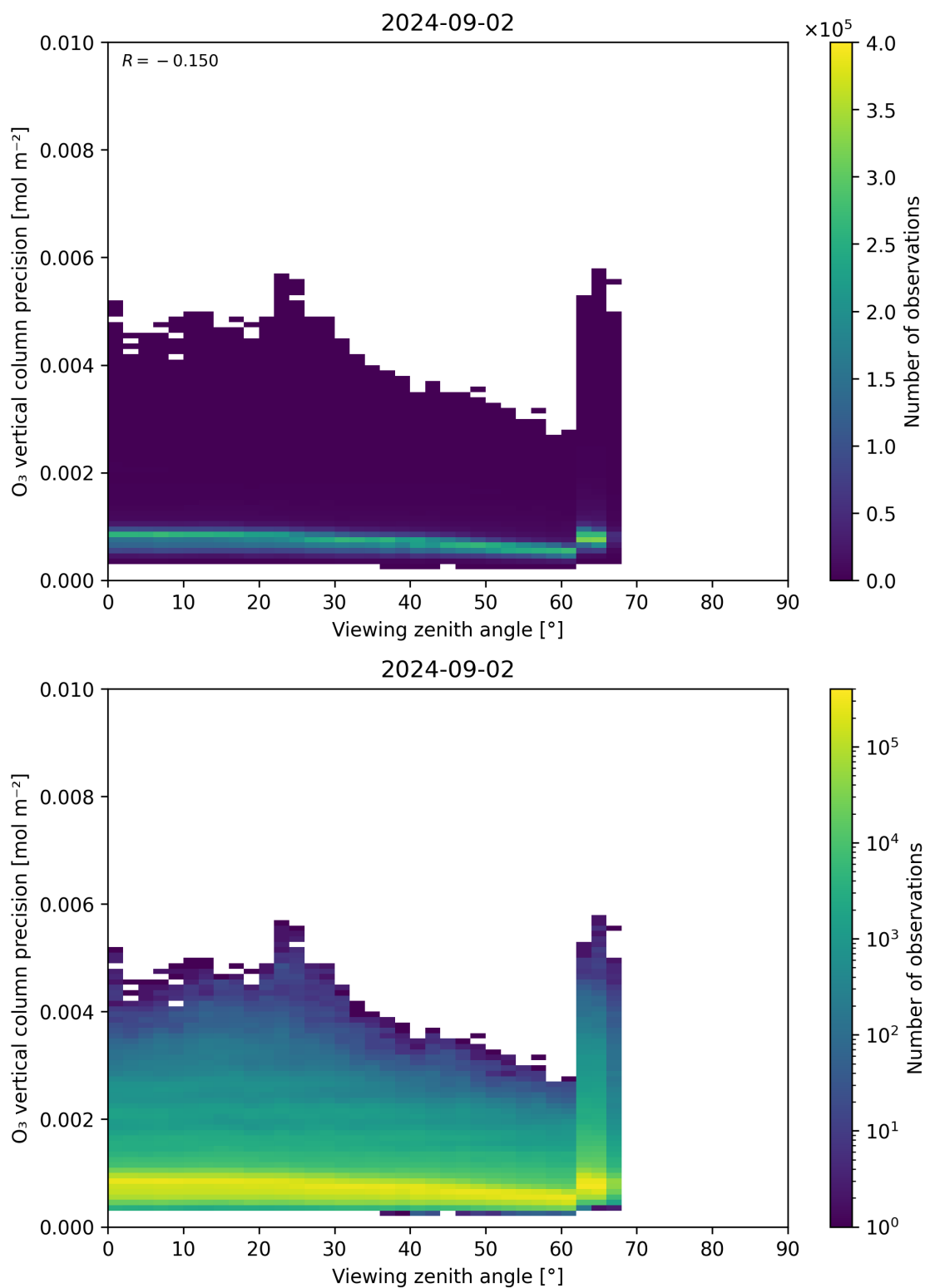
Figure 53: Scatter density plot of “Viewing zenith angle” against “O 3 vertical column precision” for 2024-09-01 to 2024-09-03.
