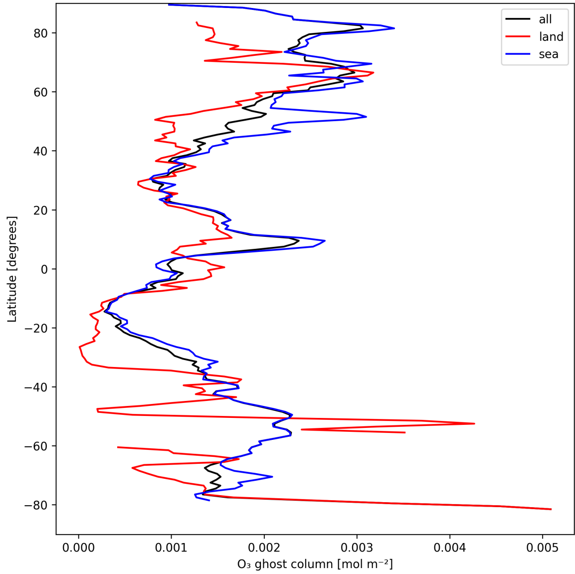
Figure 18: Zonal average of “O 3 ghost column” for 2024-09-01 to 2024-09-03.
