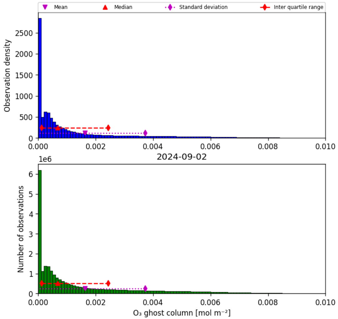
Figure 25: Histogram of “O 3 ghost column” for 2024-09-01 to 2024-09-03
