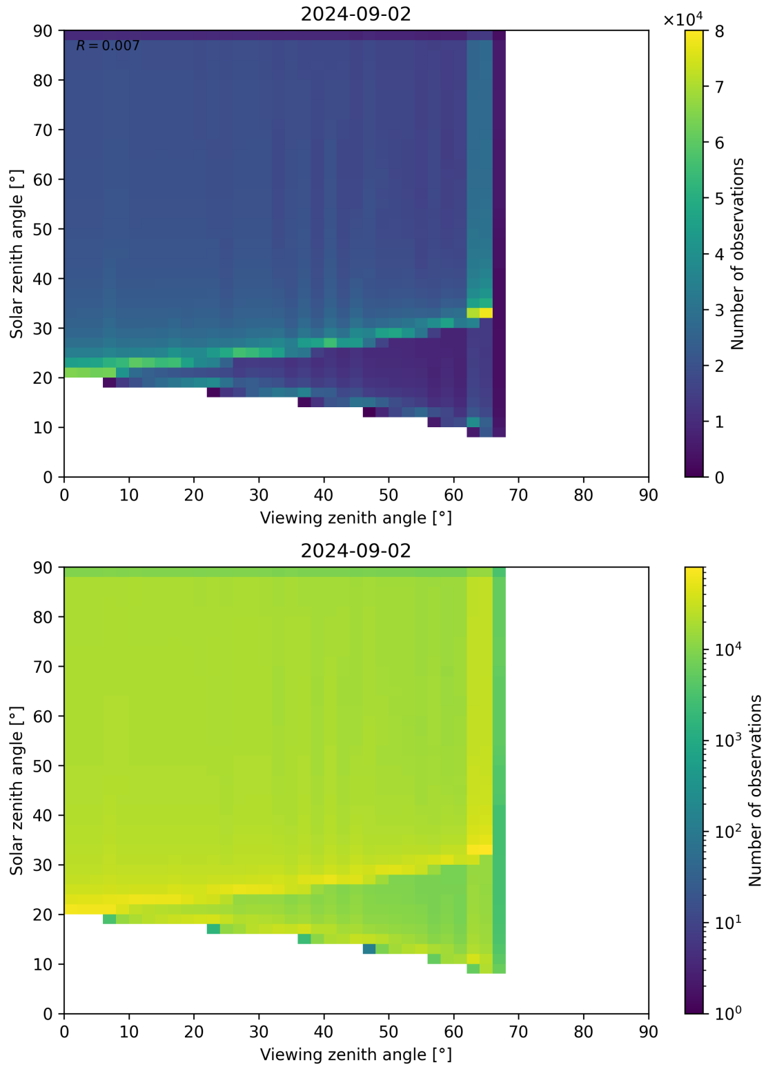
Figure 54: Scatter density plot of “Viewing zenith angle” against “Solar zenith angle” for 2024-09-01 to 2024-09-03.
