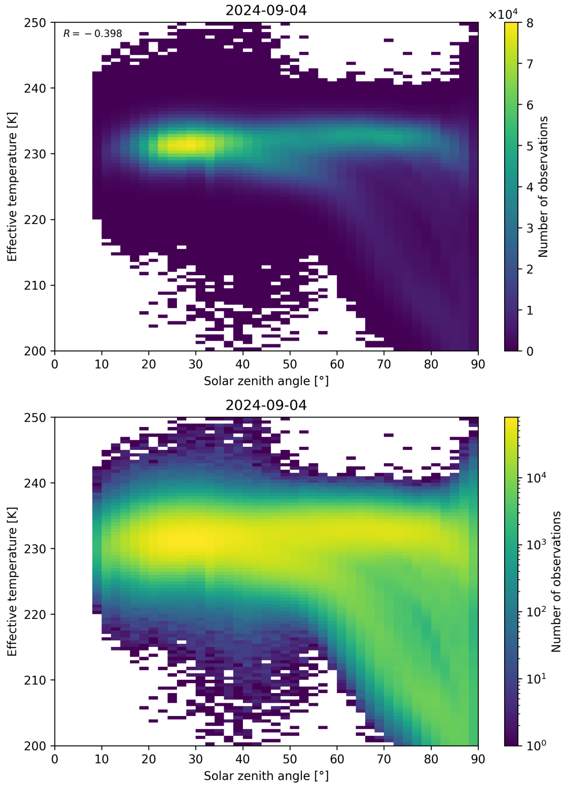
Figure 45: Scatter density plot of “Solar zenith angle” against “Effective temperature” for 2024-09-03 to 2024-09-05.
