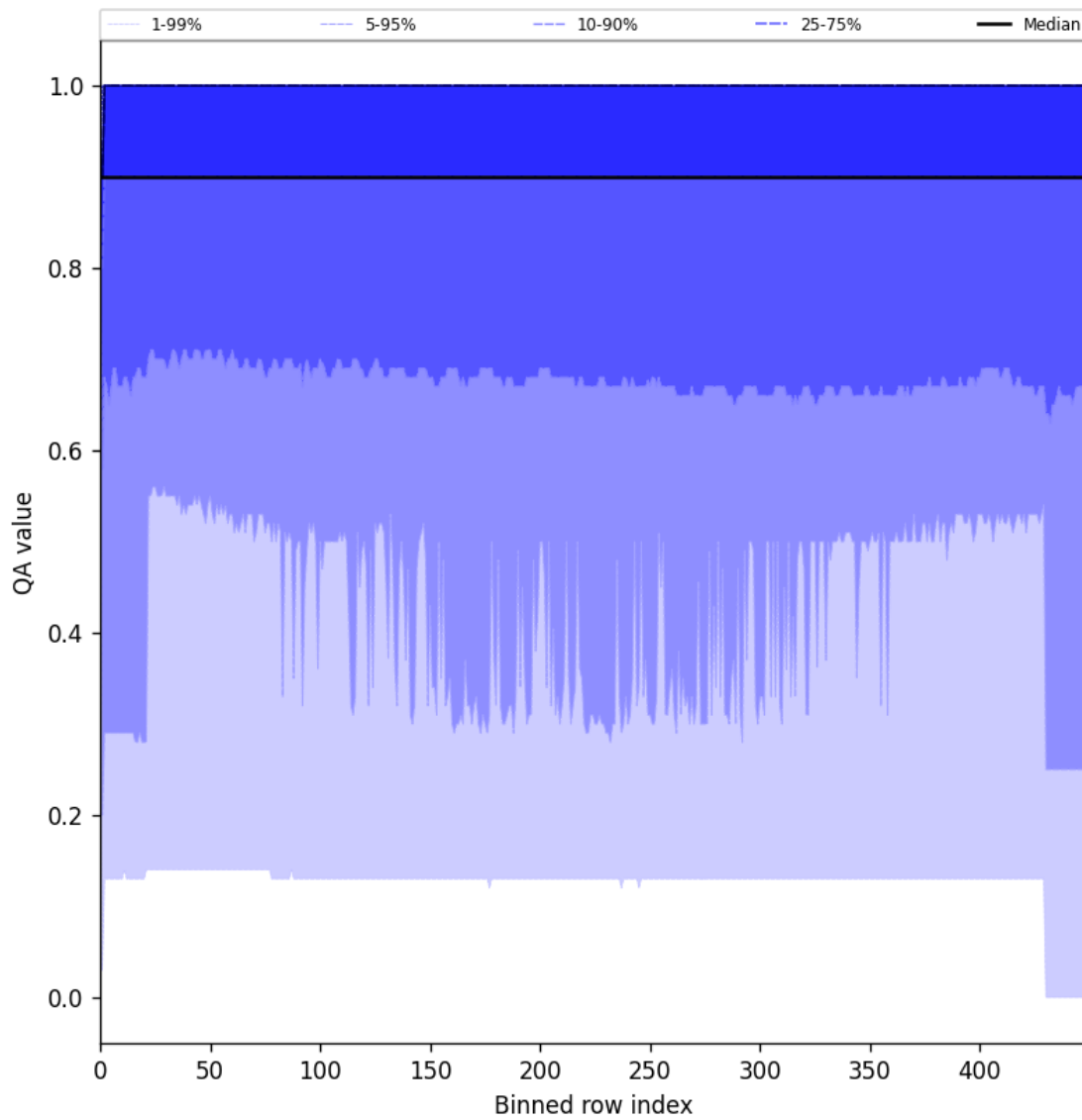
Figure 27: Along track statistics of “QA value” for 2024-09-03 to 2024-09-05
