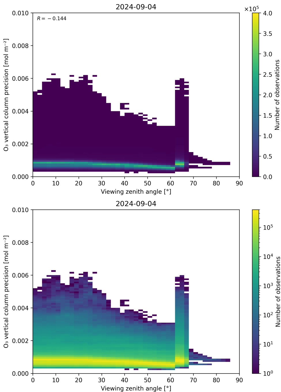
Figure 53: Scatter density plot of “Viewing zenith angle” against “O 3 vertical column precision” for 2024-09-03 to 2024-09-05.
