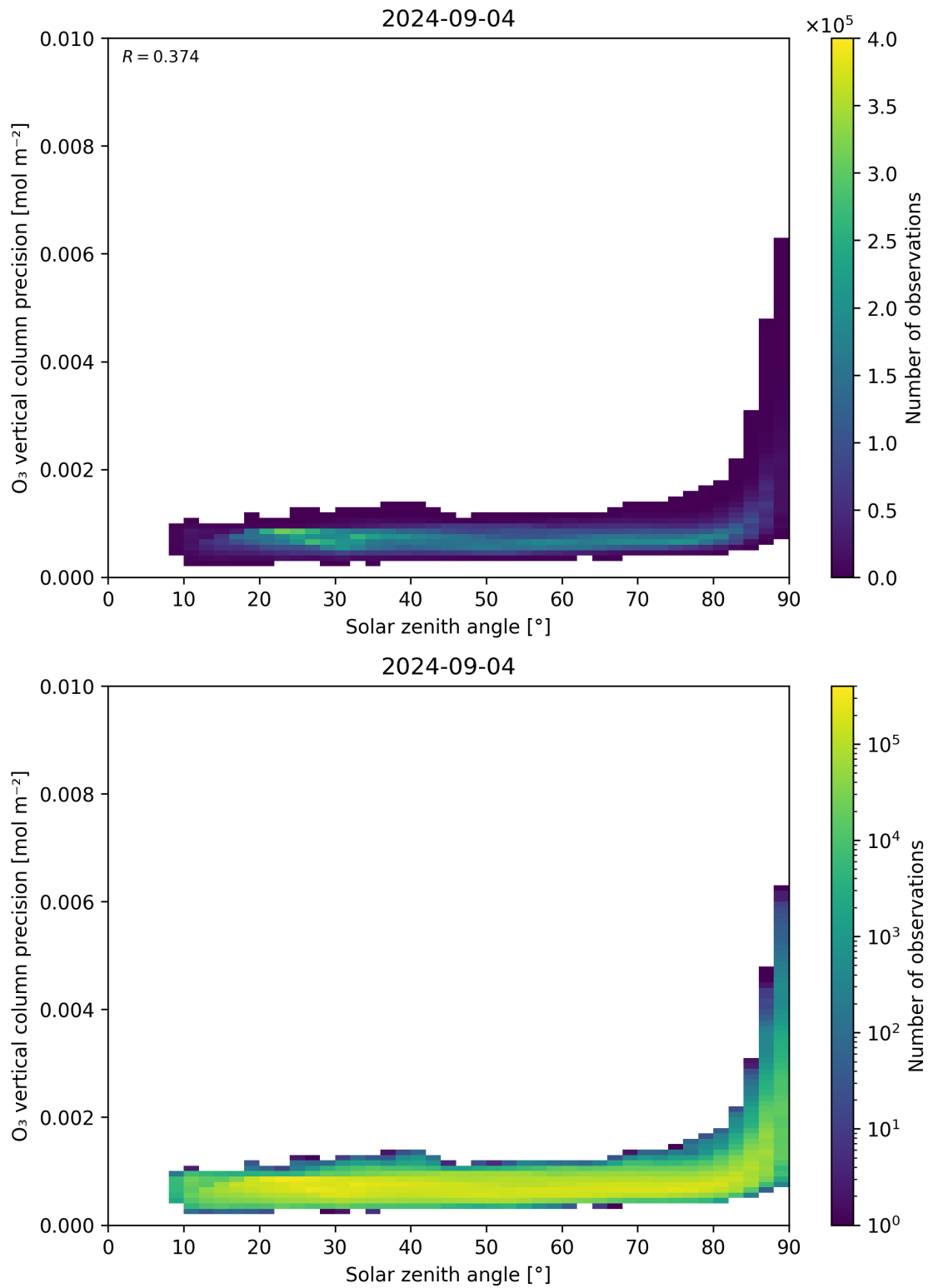
Figure 48: Scatter density plot of “Solar zenith angle” against “O 3 vertical column precision” for 2024-09-03 to 2024-09-05.
