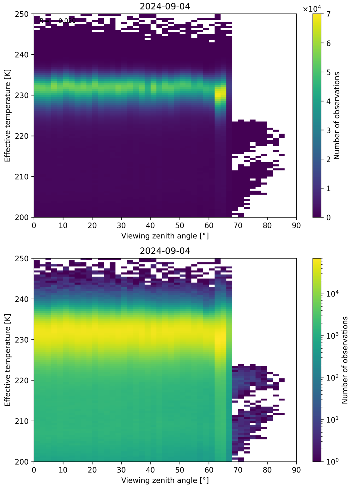
Figure 50: Scatter density plot of “Viewing zenith angle” against “Effective temperature” for 2024-09-03 to 2024-09-05.
