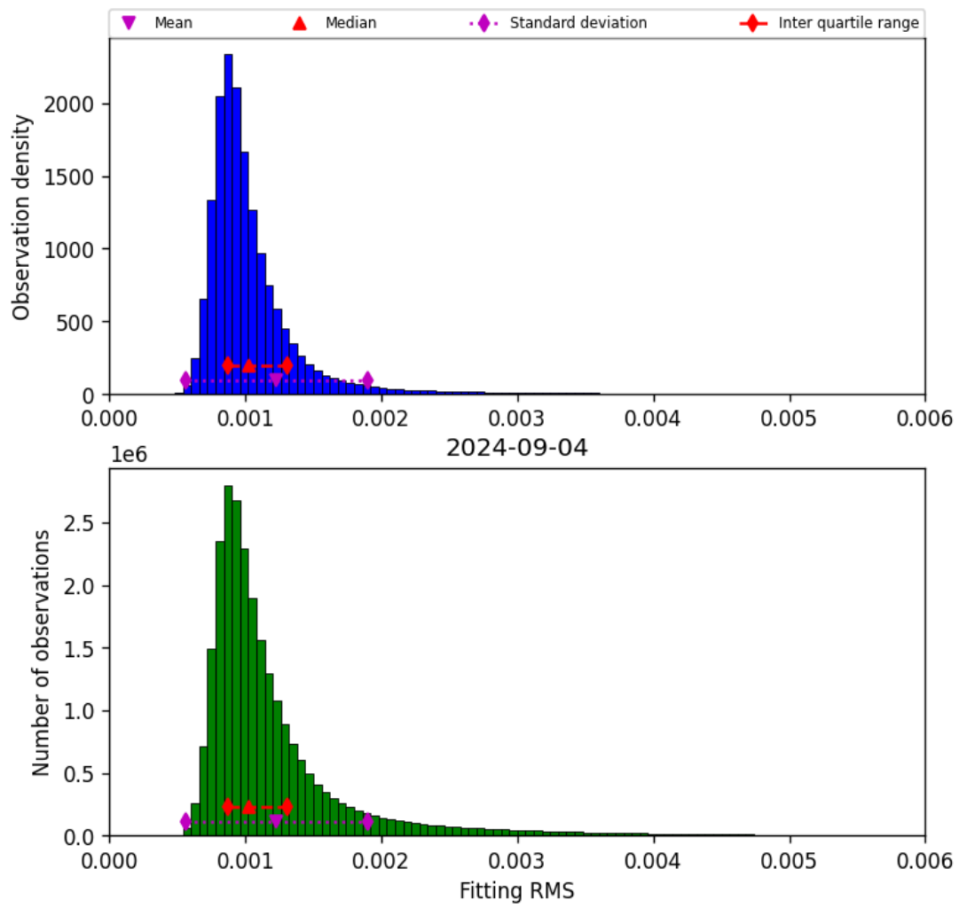
Figure 23: Histogram of “Fitting RMS” for 2024-09-03 to 2024-09-05
