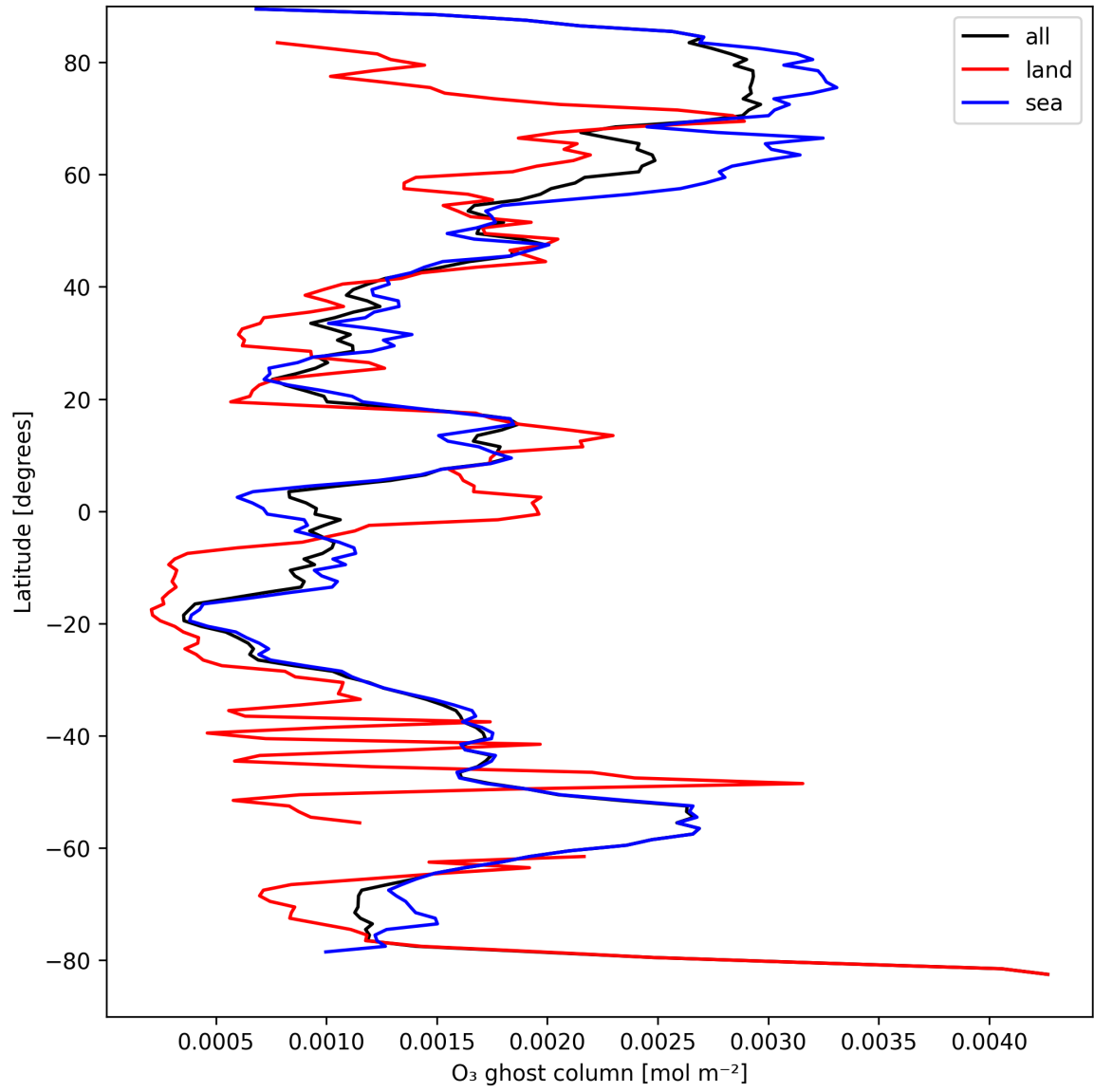
Figure 18: Zonal average of “O 3 ghost column” for 2024-09-03 to 2024-09-05.
