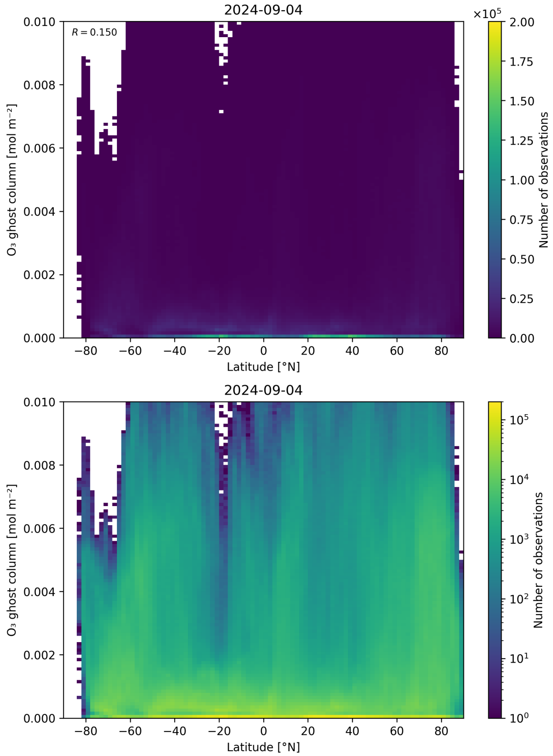
Figure 35: Scatter density plot of “Latitude” against “O 3 ghost column” for 2024-09-03 to 2024-09-05.
