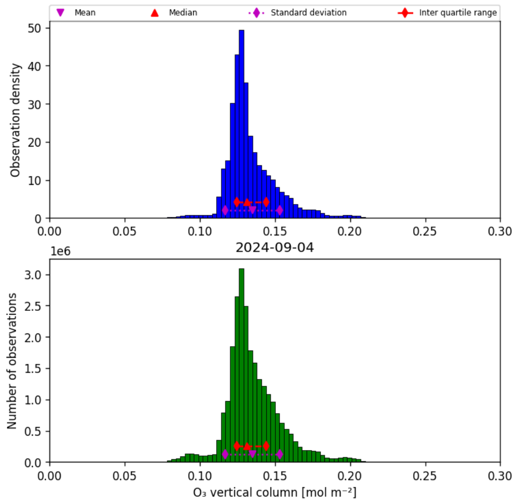
Figure 21: Histogram of “O 3 vertical column” for 2024-09-03 to 2024-09-05
