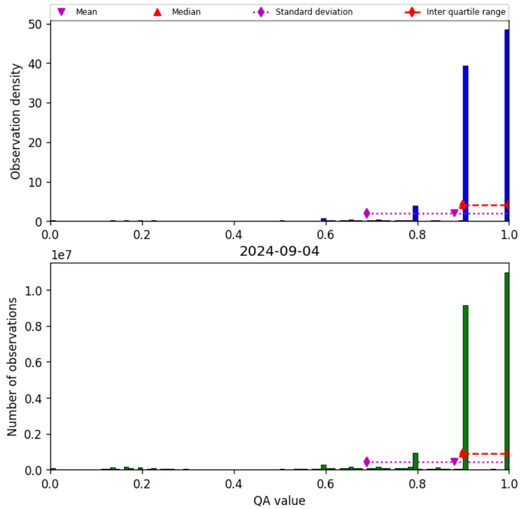
Figure 20: Histogram of “QA value” for 2024-09-03 to 2024-09-05
