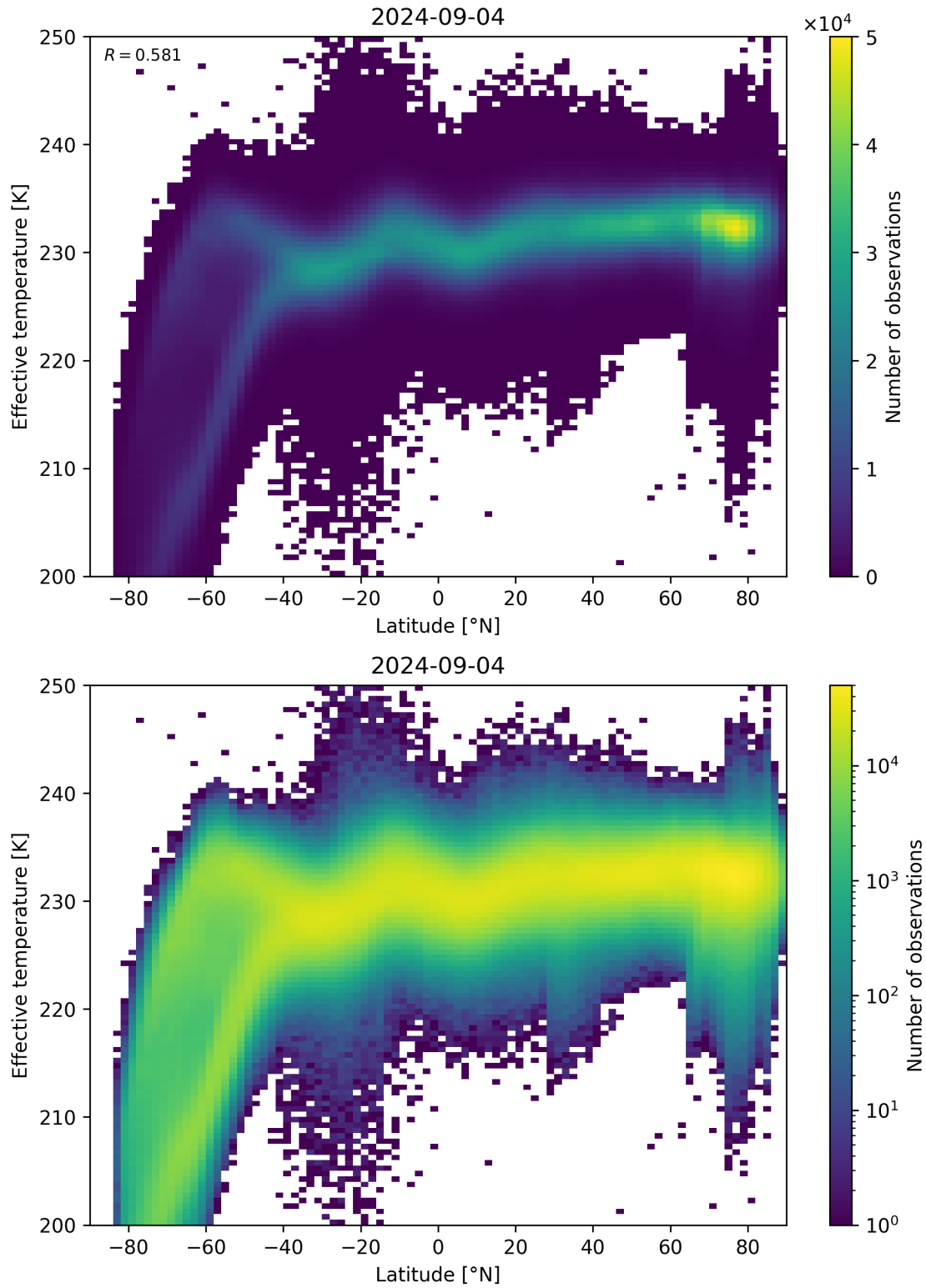
Figure 34: Scatter density plot of “Latitude” against “Effective temperature” for 2024-09-03 to 2024-09-05.
