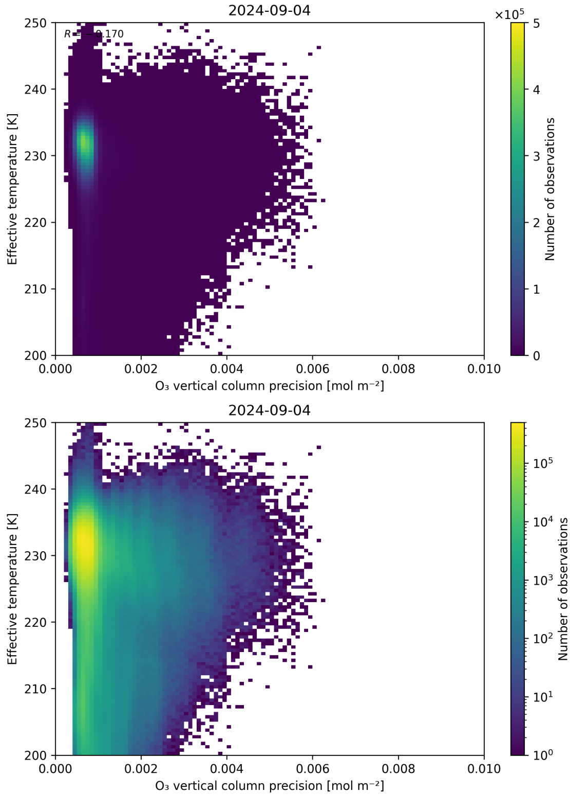
Figure 42: Scatter density plot of “O 3 vertical column precision” against “Effective temperature” for 2024-09-03 to 2024-09-05.
