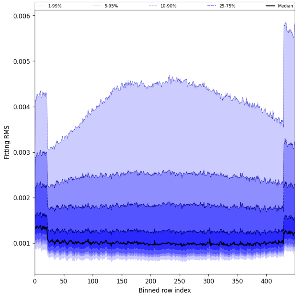
Figure 30: Along track statistics of “Fitting RMS” for 2024-09-03 to 2024-09-05
