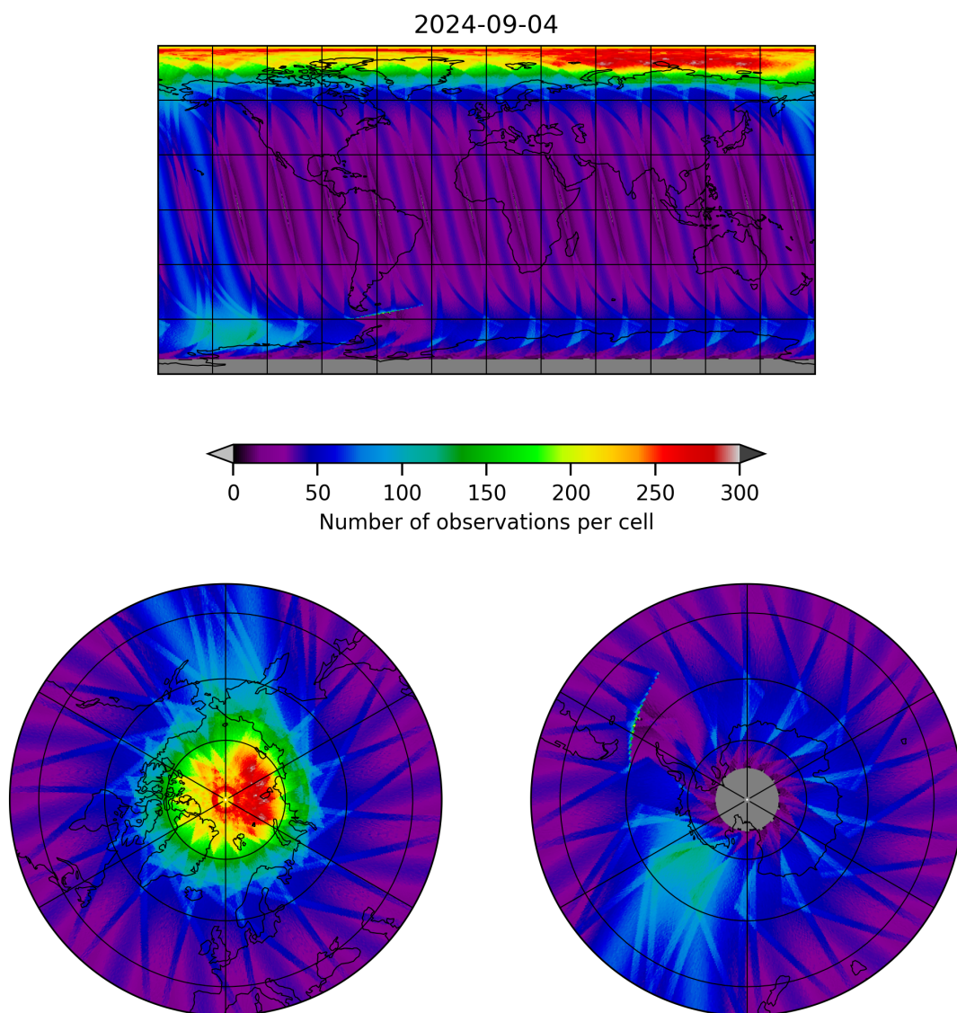
Figure 12: Map of the number of observations for 2024-09-03 to 2024-09-05
