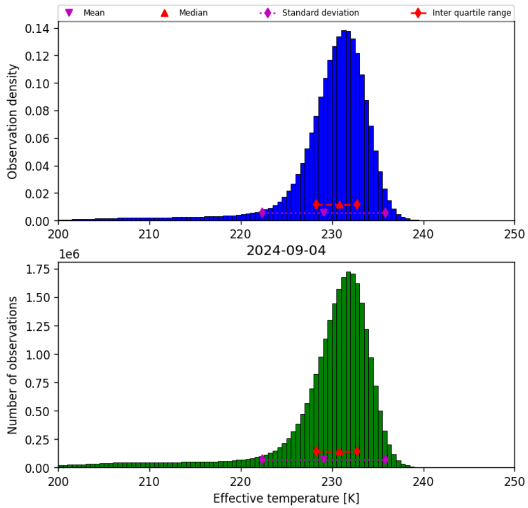
Figure 24: Histogram of “Effective temperature” for 2024-09-03 to 2024-09-05
