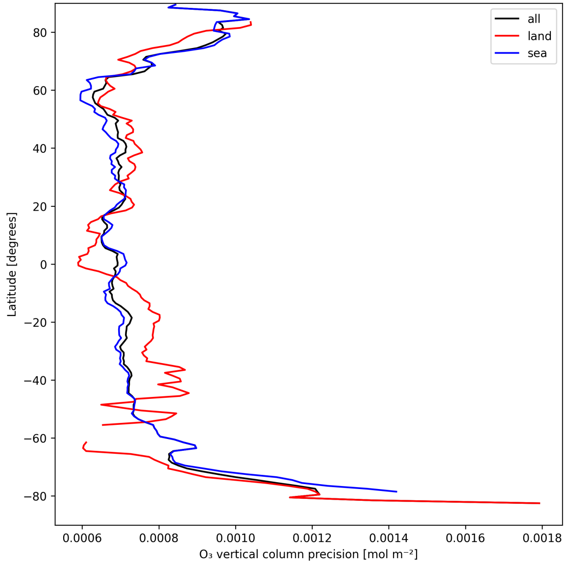
Figure 15: Zonal average of “O 3 vertical column precision” for 2024-09-03 to 2024-09-05.
