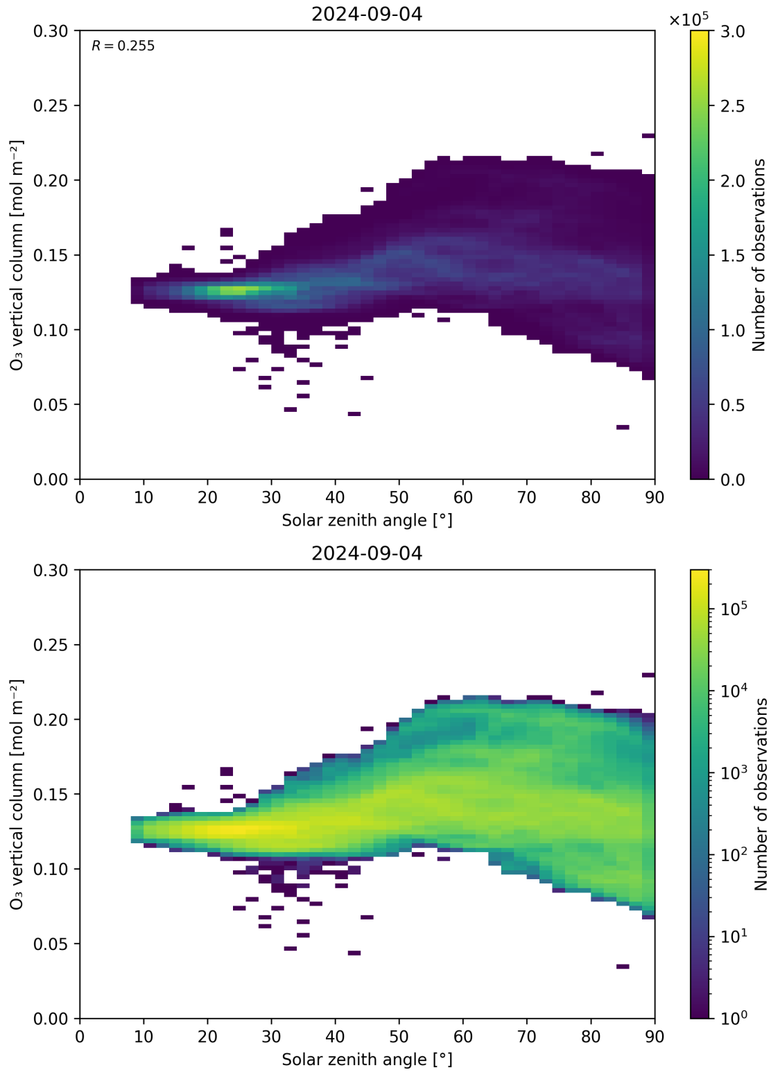
Figure 47: Scatter density plot of “Solar zenith angle” against “O 3 vertical column” for 2024-09-03 to 2024-09-05.
