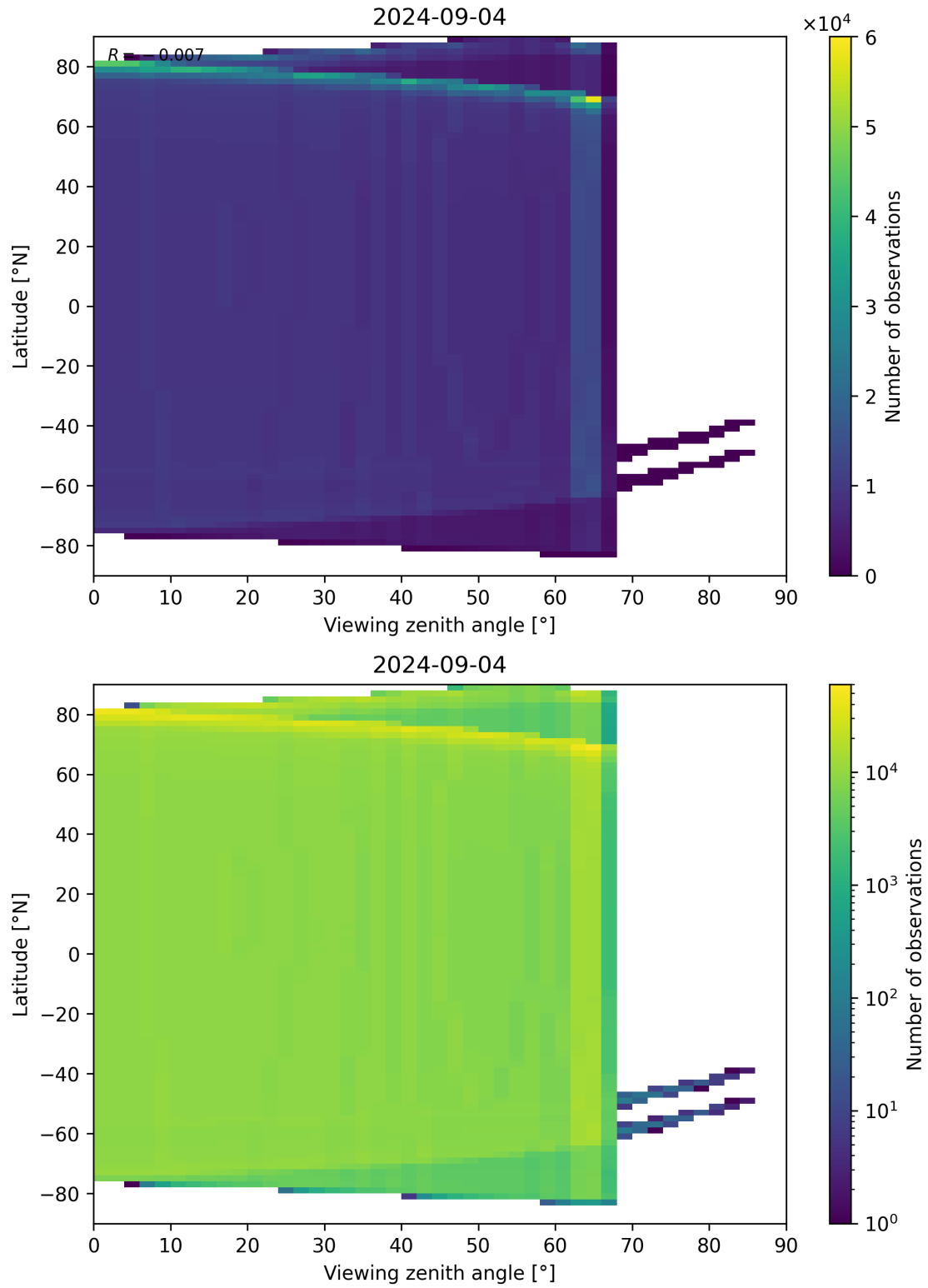
Figure 49: Scatter density plot of “Viewing zenith angle” against “Latitude” for 2024-09-03 to 2024-09-05.
