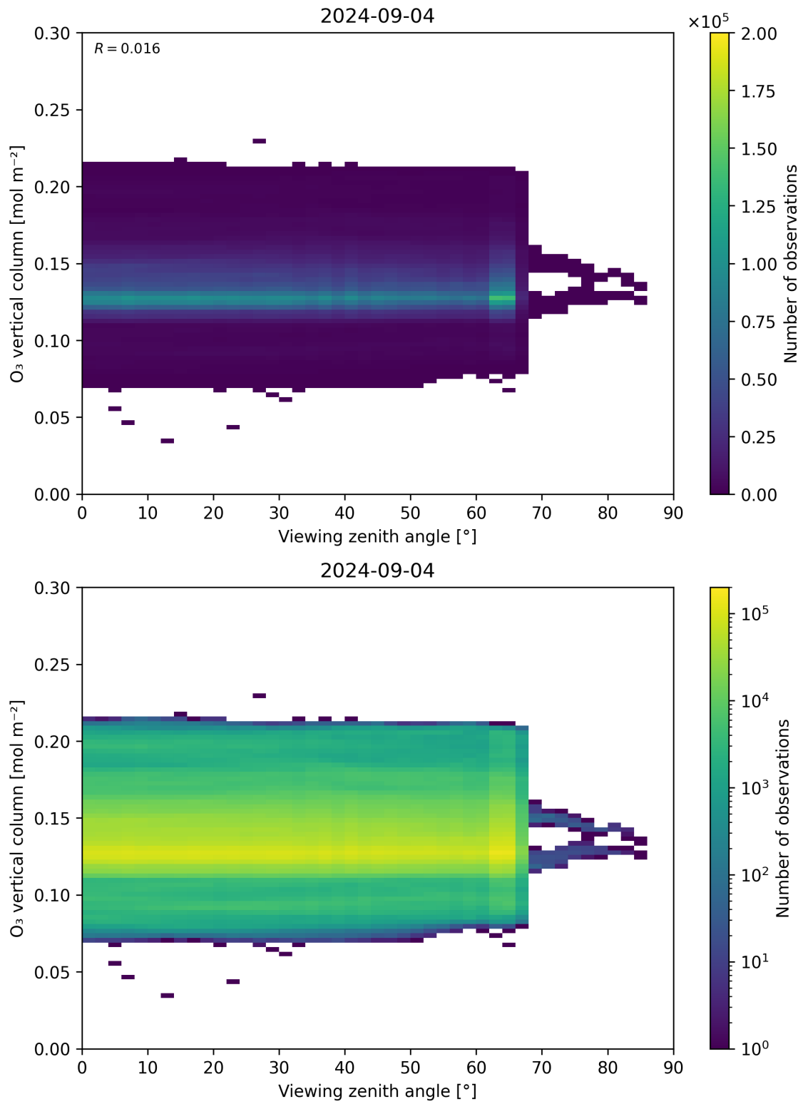
Figure 52: Scatter density plot of “Viewing zenith angle” against “O 3 vertical column” for 2024-09-03 to 2024-09-05.
