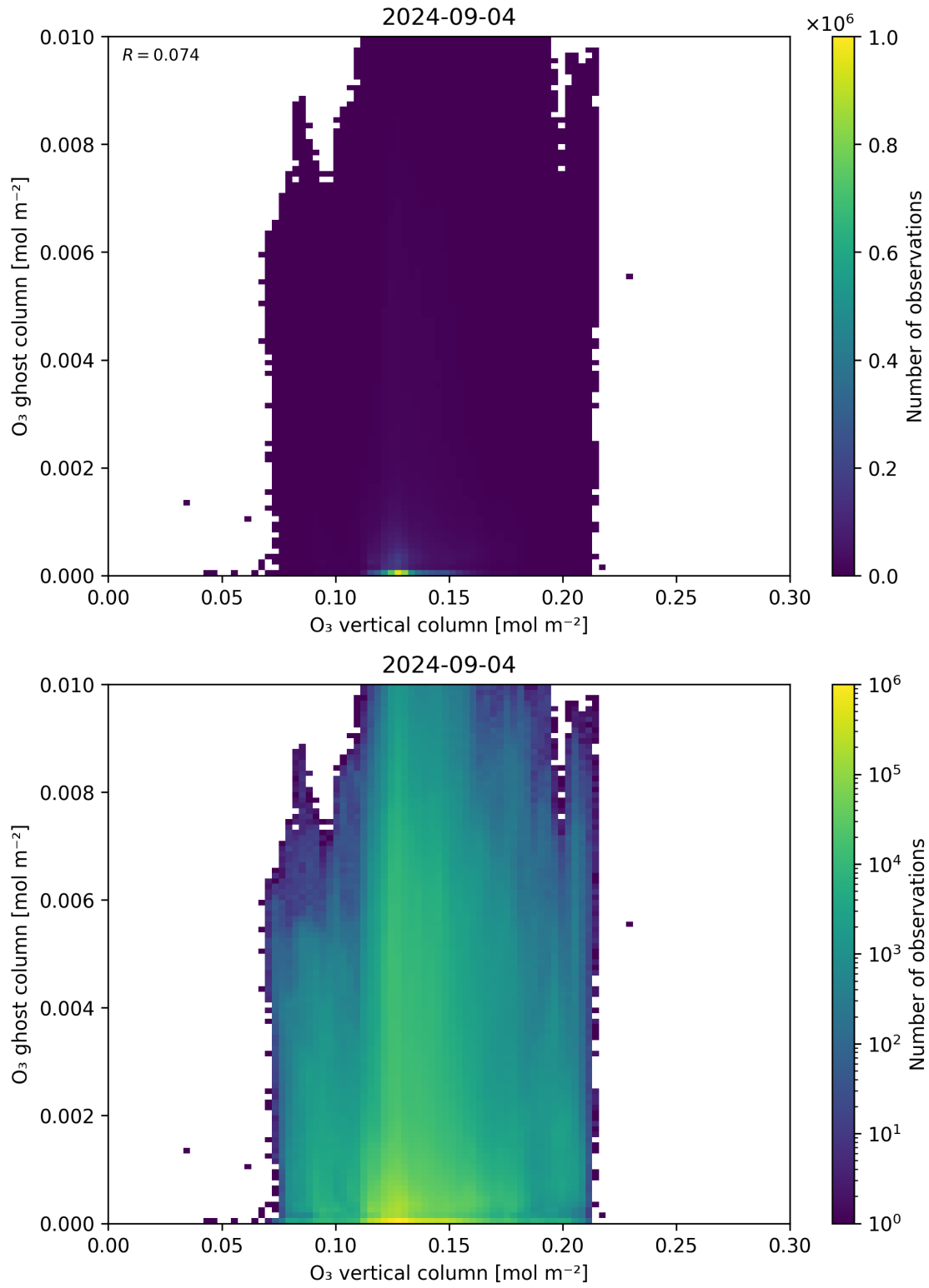
Figure 40: Scatter density plot of “ \text{O}_3 vertical column” against “ \text{O}_3 ghost column” for 2024-09-03 to 2024-09-05.
