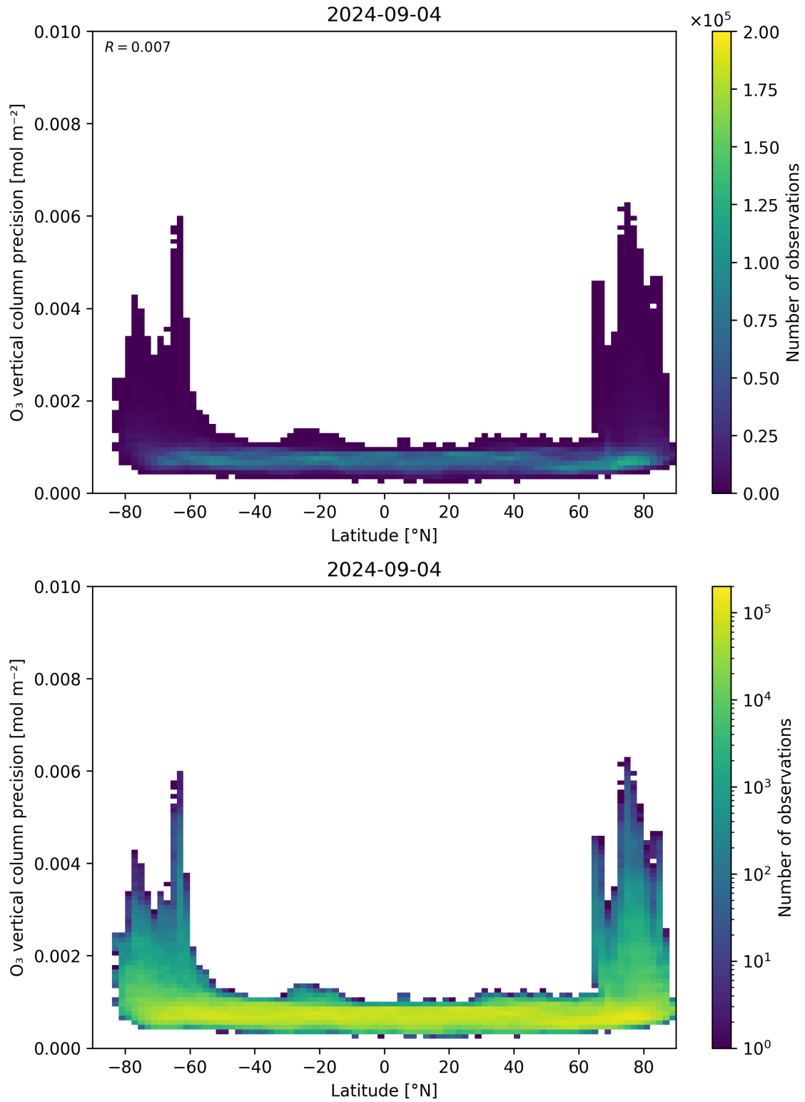
Figure 37: Scatter density plot of “Latitude” against “O 3 vertical column precision” for 2024-09-03 to 2024-09-05.
