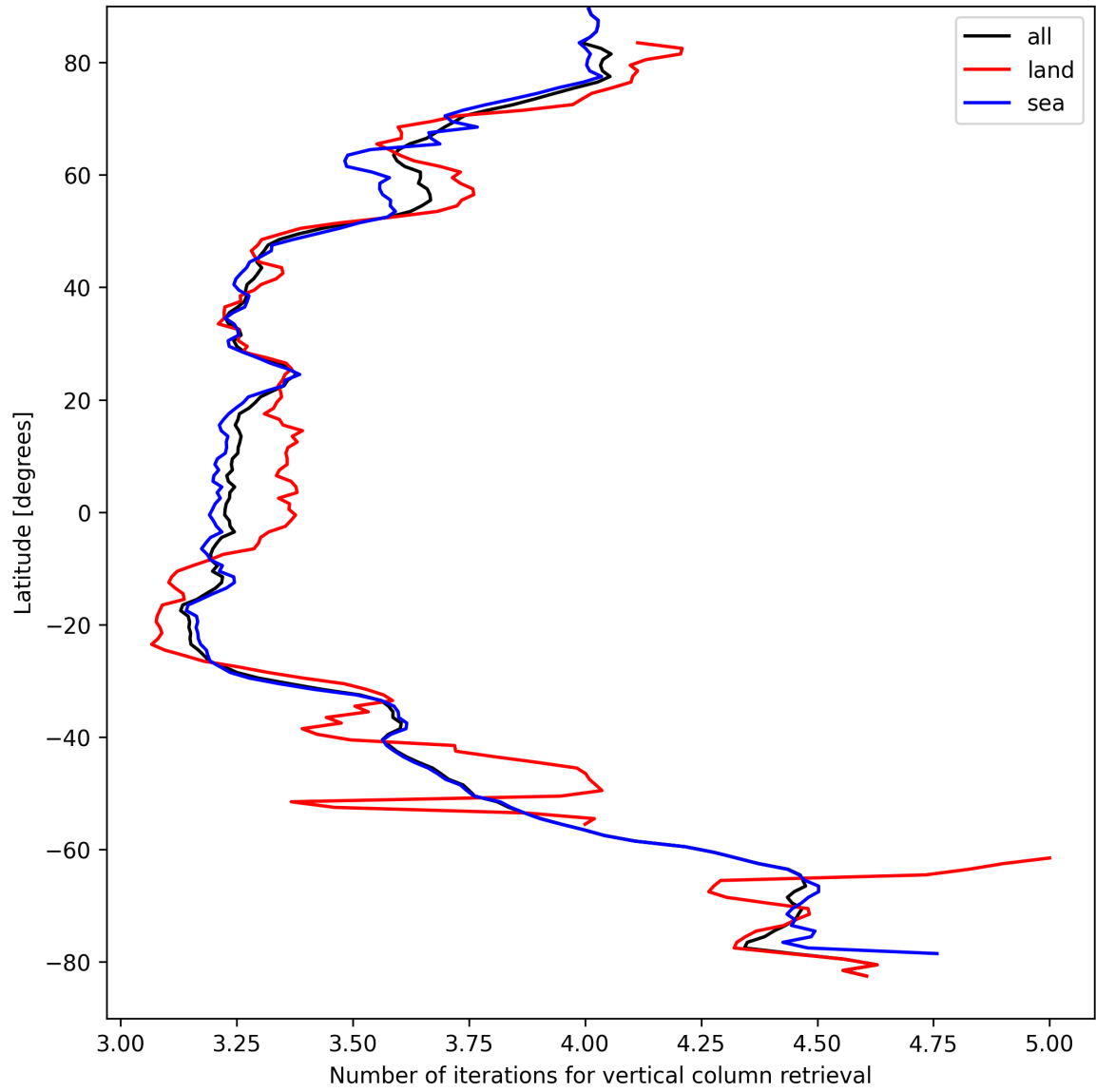
Figure 19: Zonal average of “Number of iterations for vertical column retrieval” for 2024-09-03 to 2024-09-05.
