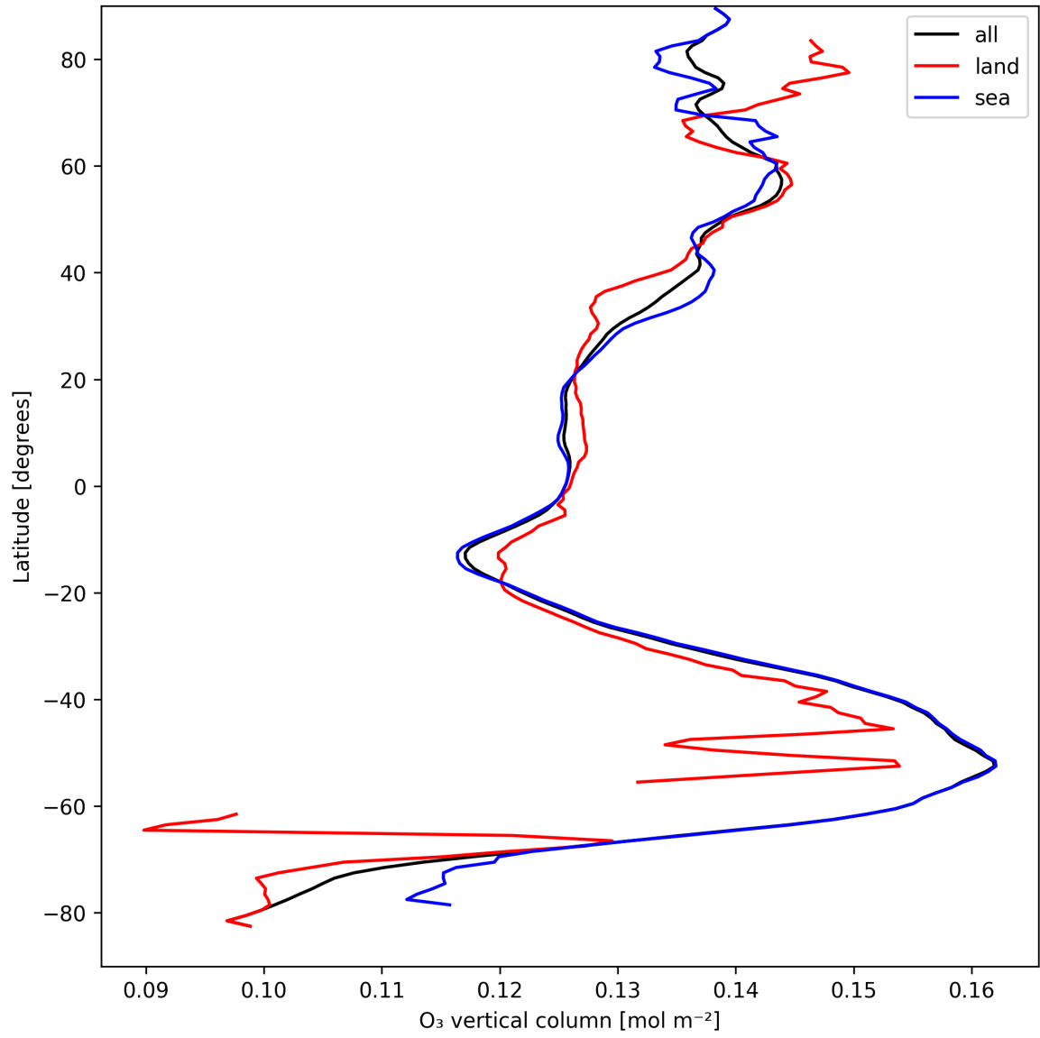
Figure 14: Zonal average of “O 3 vertical column” for 2024-09-03 to 2024-09-05.
