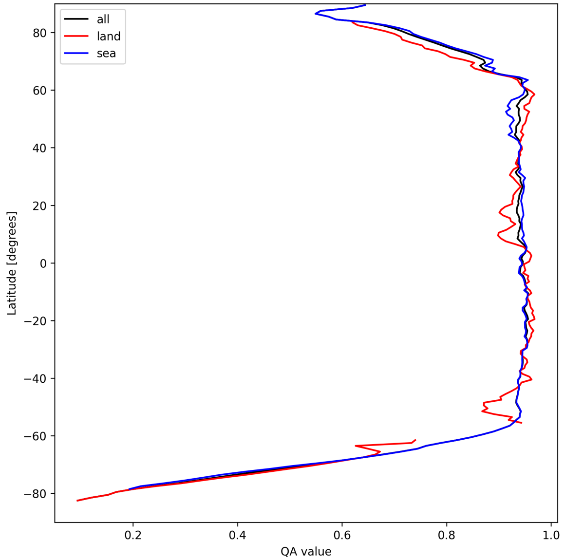
Figure 13: Zonal average of “QA value” for 2024-09-03 to 2024-09-05.
