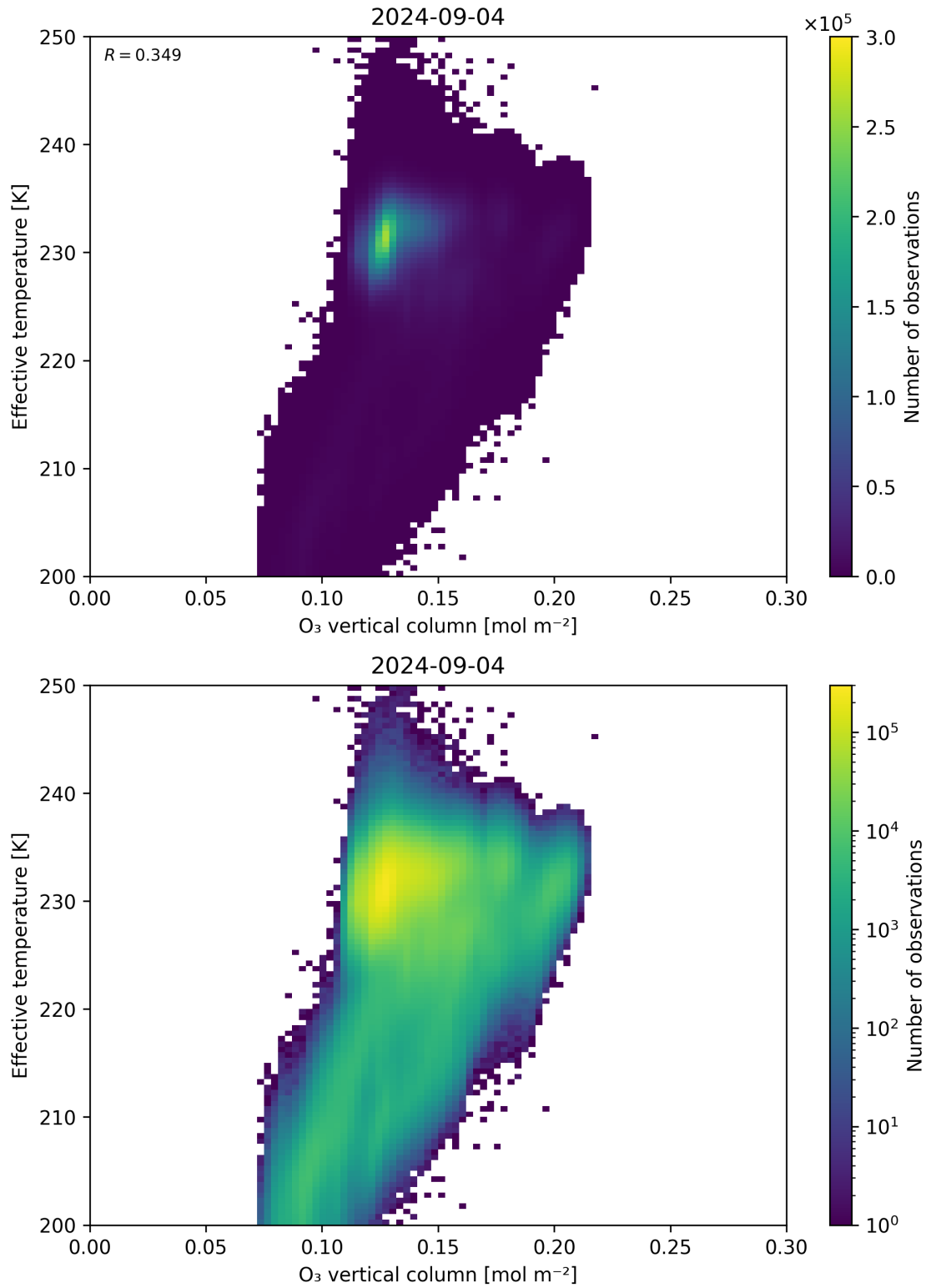
Figure 39: Scatter density plot of “O 3 vertical column” against “Effective temperature” for 2024-09-03 to 2024-09-05.
