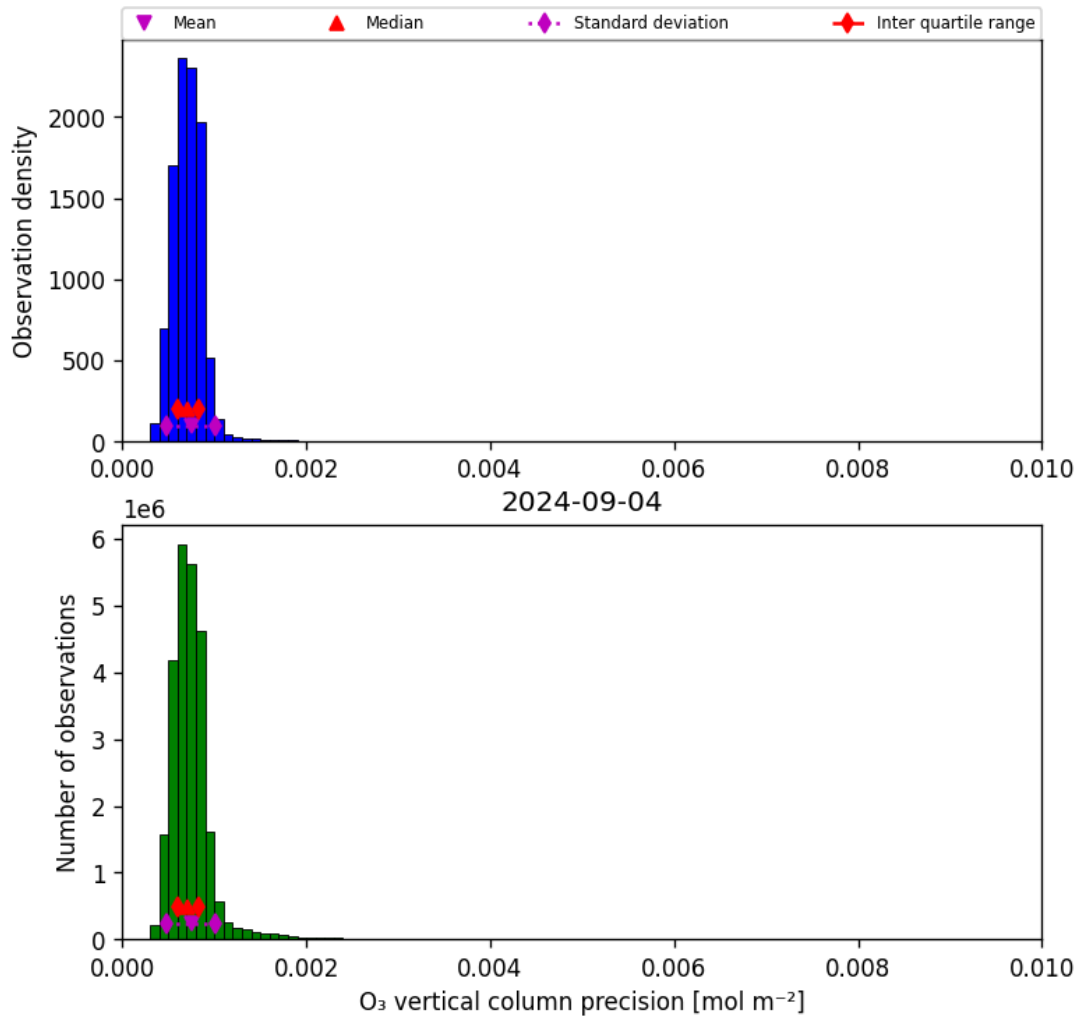
Figure 22: Histogram of “O 3 vertical column precision” for 2024-09-03 to 2024-09-05
