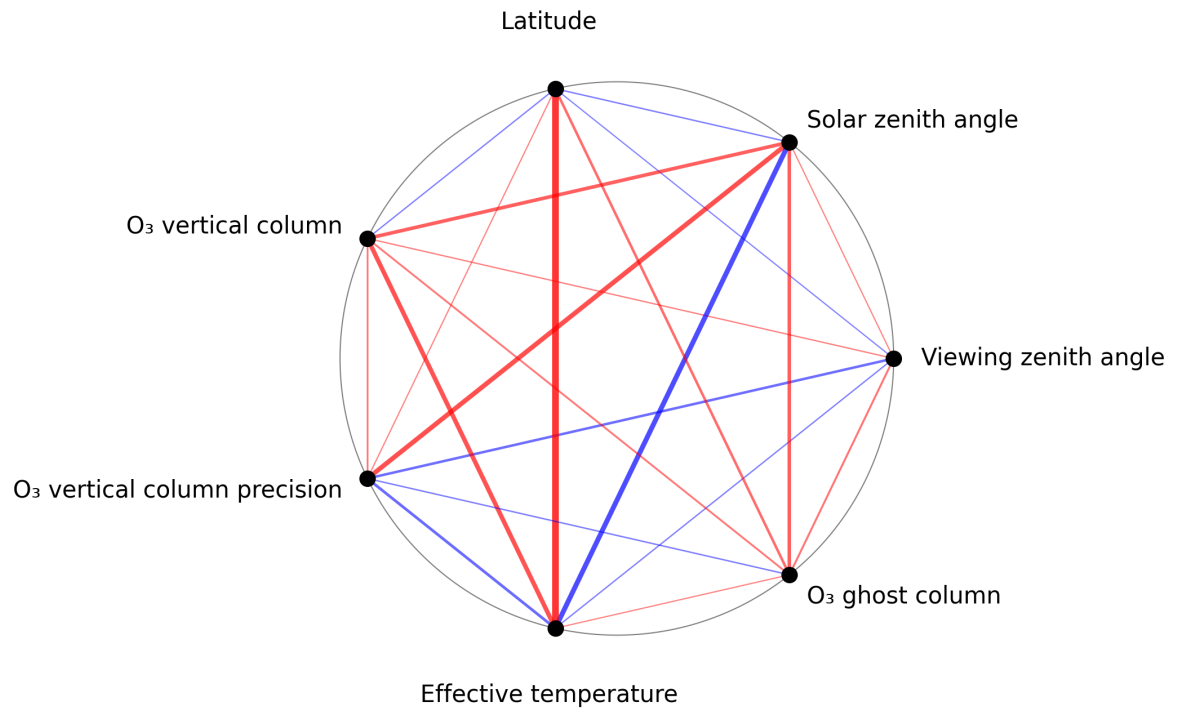
Figure 1: Map of correlation graph for 2024-09-03 to 2024-09-05.
