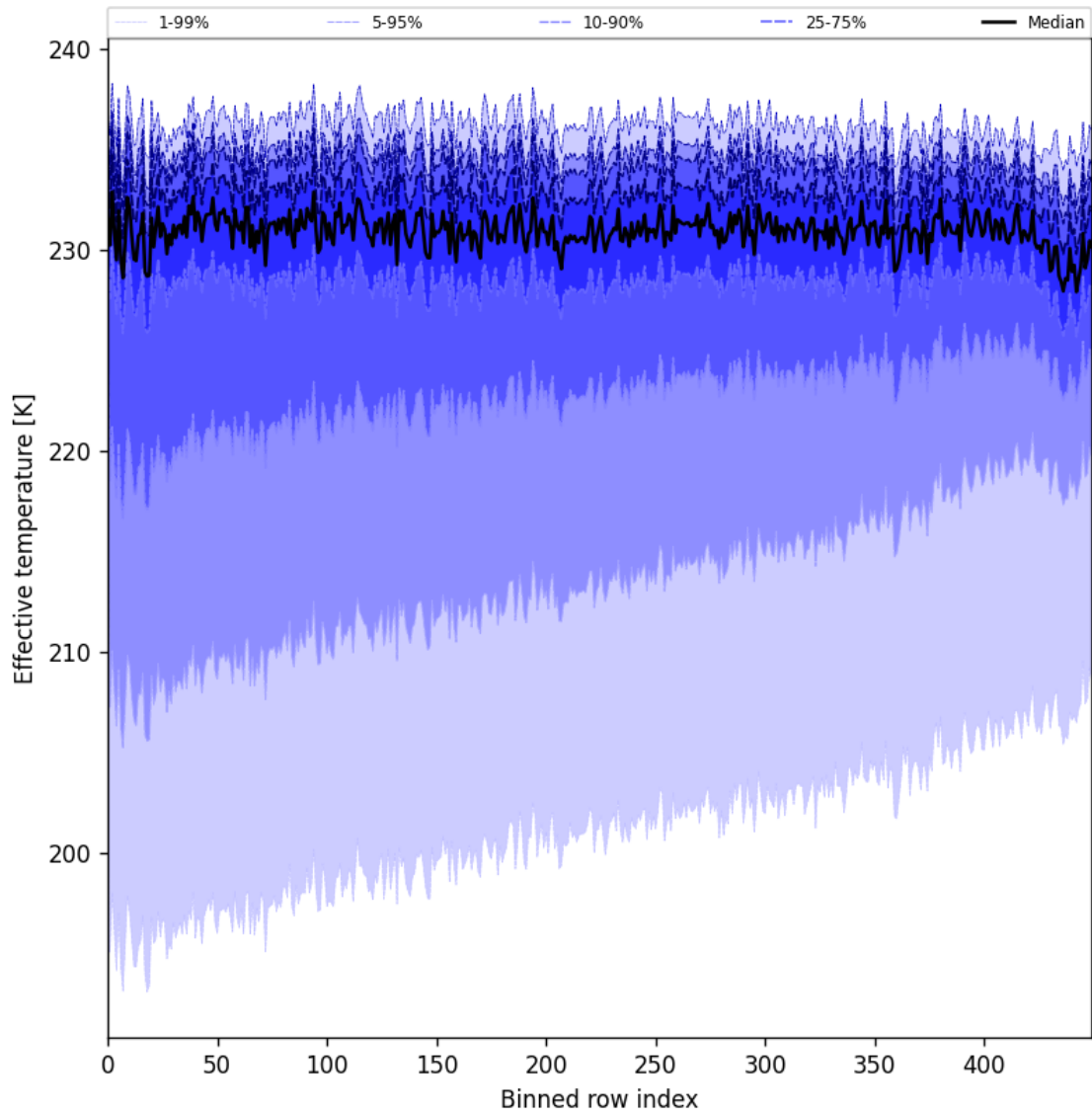
Figure 31: Along track statistics of “Effective temperature” for 2024-09-03 to 2024-09-05
