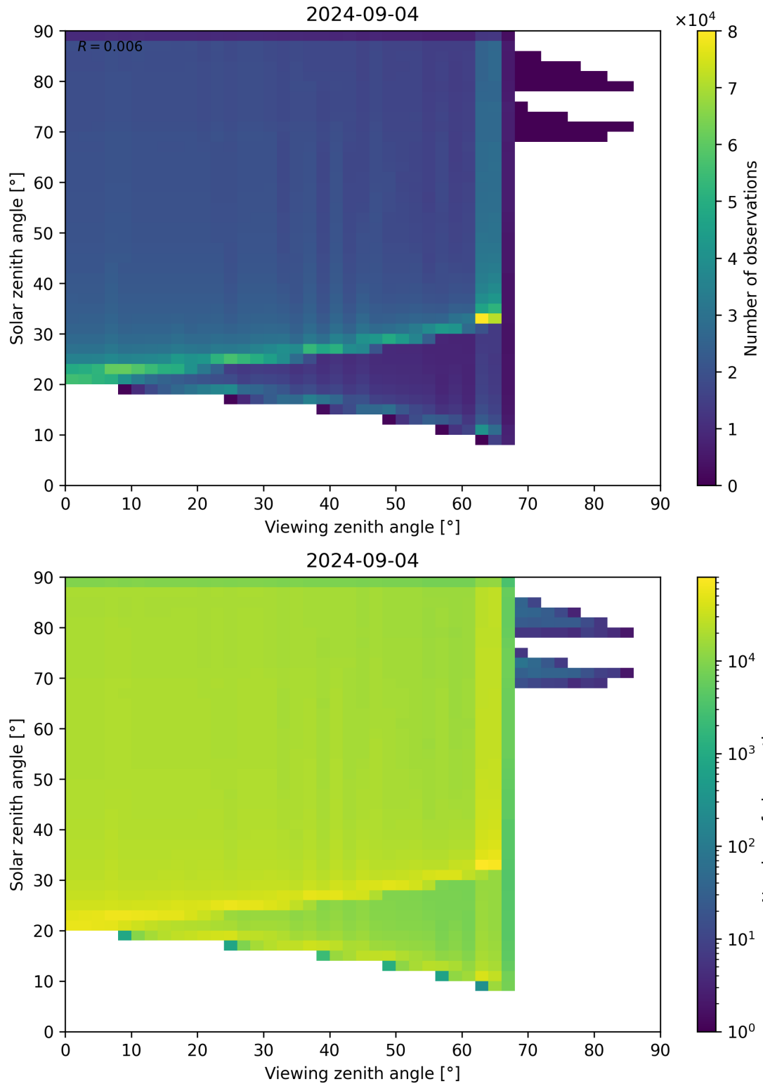
Figure 54: Scatter density plot of “Viewing zenith angle” against “Solar zenith angle” for 2024-09-03 to 2024-09-05.
