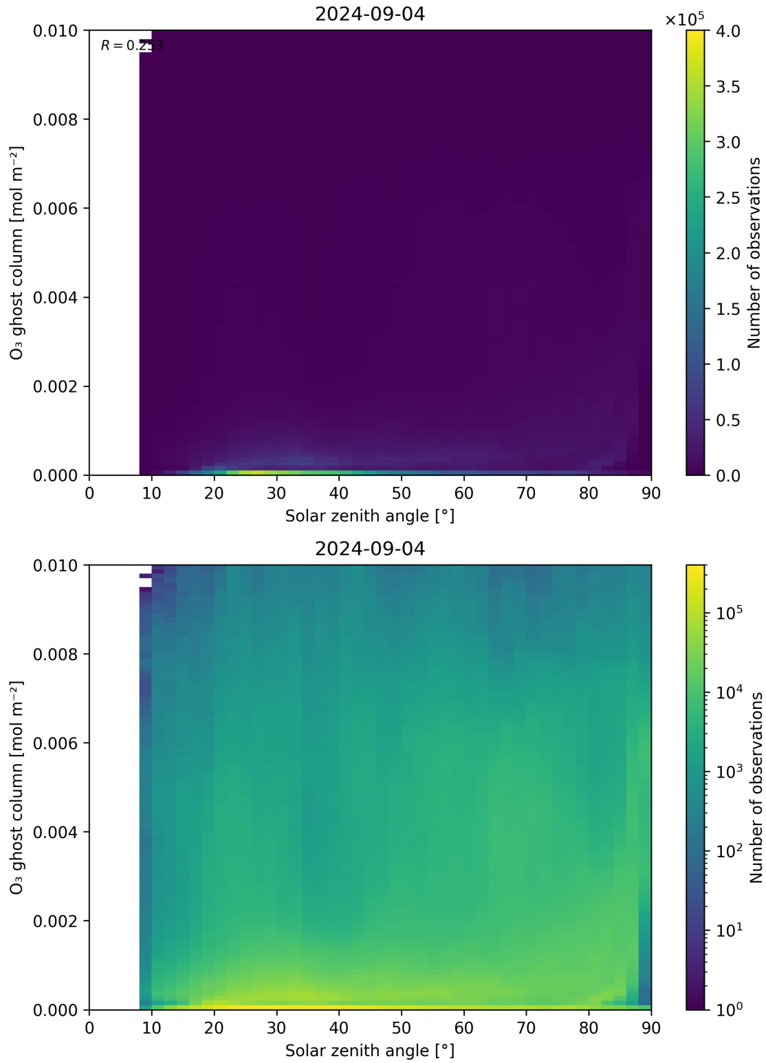
Figure 46: Scatter density plot of “Solar zenith angle” against “O 3 ghost column” for 2024-09-03 to 2024-09-05.
