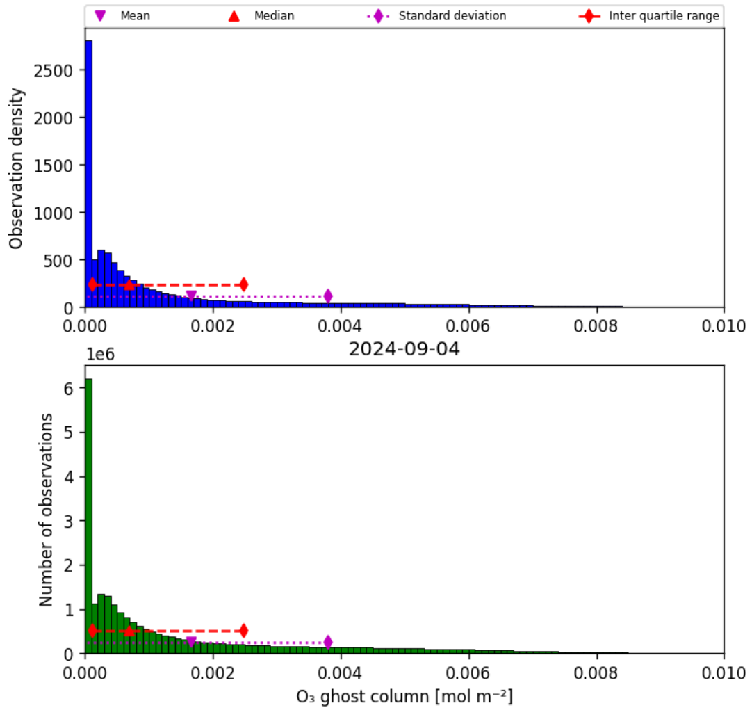
Figure 25: Histogram of “O 3 ghost column” for 2024-09-03 to 2024-09-05
