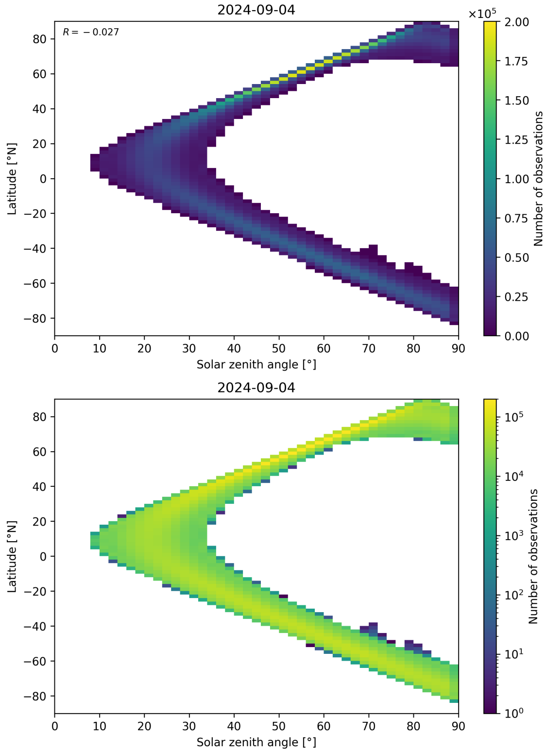
Figure 44: Scatter density plot of “Solar zenith angle” against “Latitude” for 2024-09-03 to 2024-09-05.
