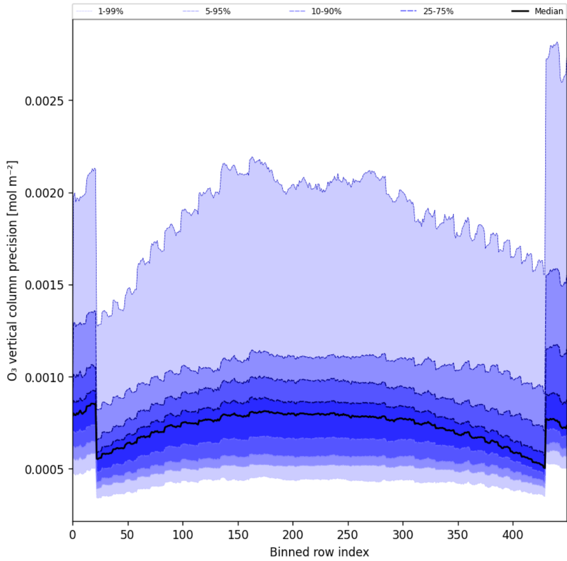
Figure 29: Along track statistics of “O 3 vertical column precision” for 2024-09-03 to 2024-09-05
