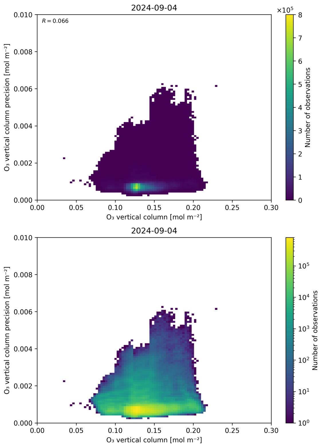
Figure 41: Scatter density plot of “O 3 vertical column” against “O 3 vertical column precision” for 2024-09-03 to 2024-09-05.
