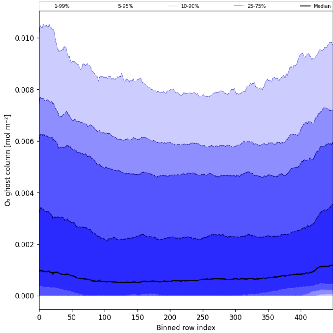
Figure 32: Along track statistics of “O 3 ghost column” for 2024-09-03 to 2024-09-05
