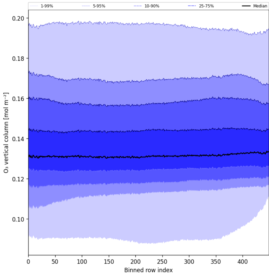
Figure 28: Along track statistics of “O 3 vertical column” for 2024-09-03 to 2024-09-05
