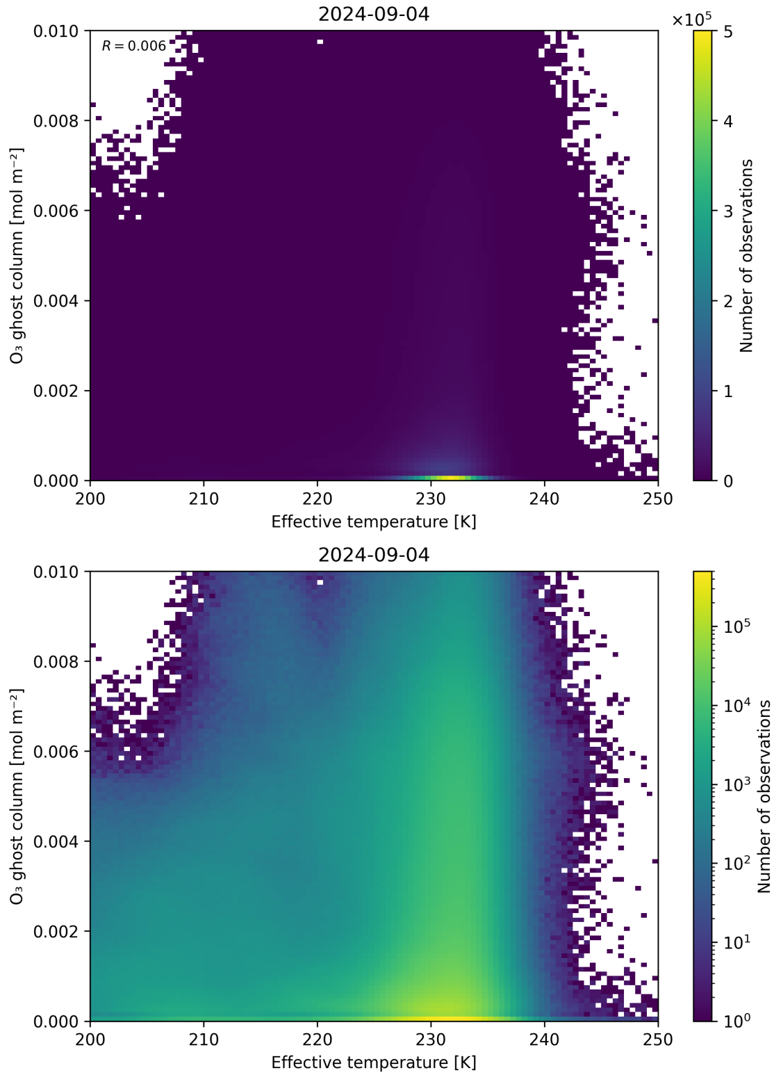
Figure 38: Scatter density plot of “Effective temperature” against “O 3 ghost column” for 2024-09-03 to 2024-09-05.
