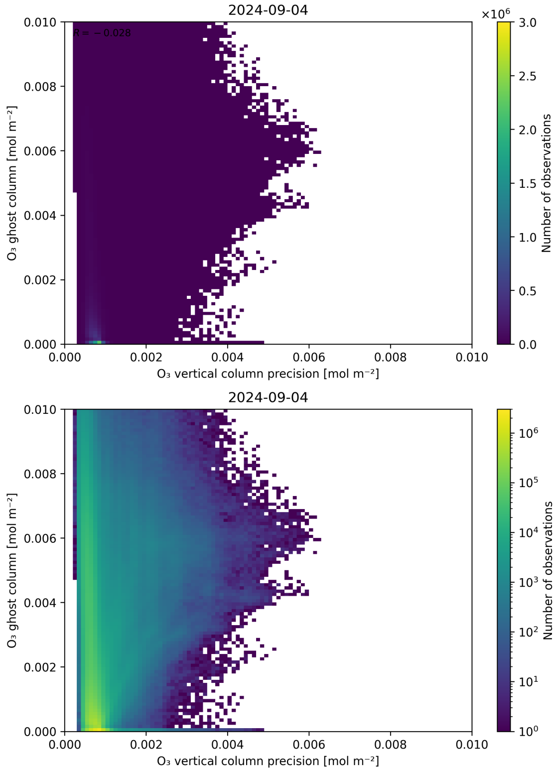
Figure 43: Scatter density plot of “ \text{O}_3 vertical column precision” against “ \text{O}_3 ghost column” for 2024-09-03 to 2024-09-05.
