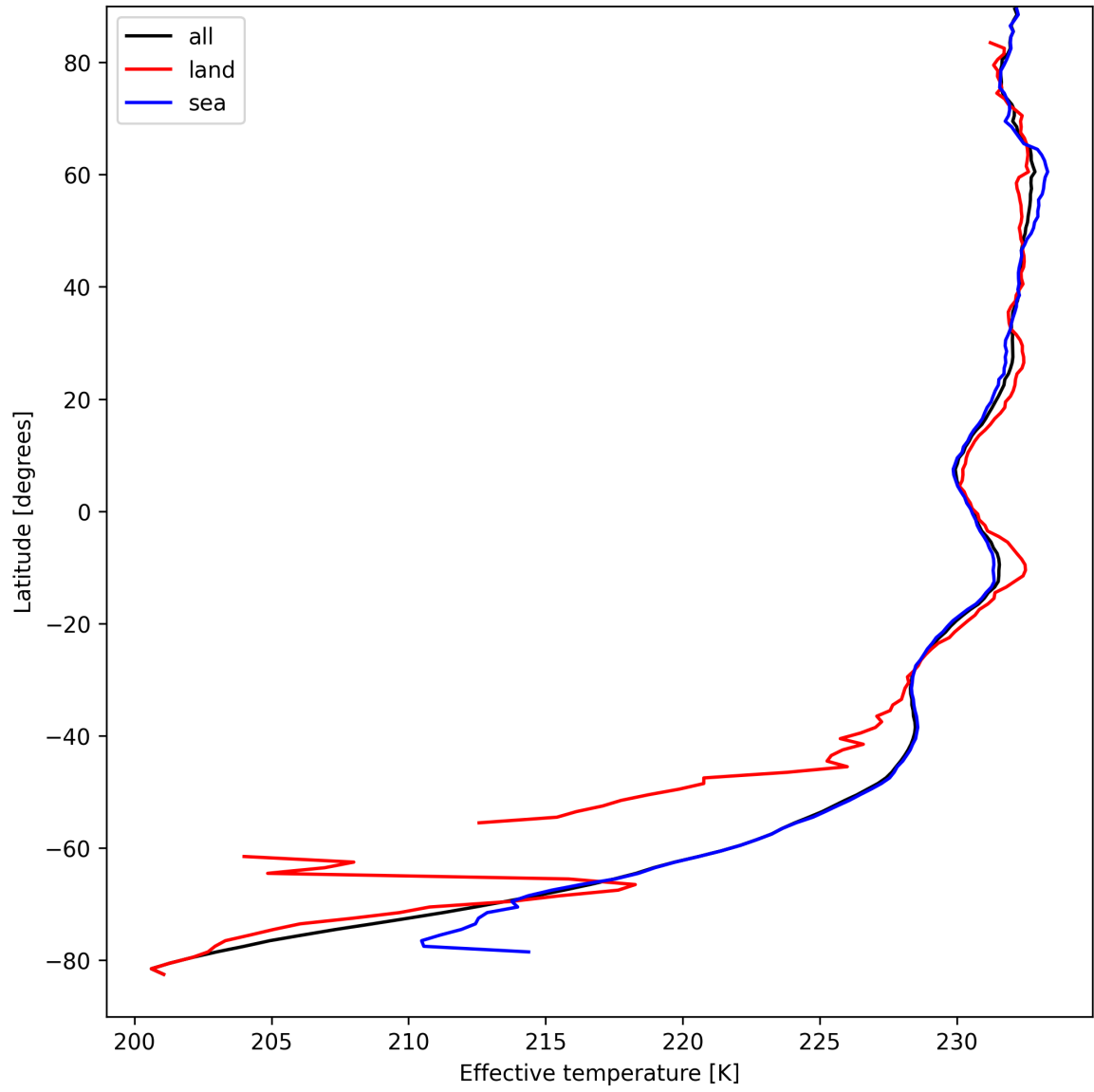
Figure 17: Zonal average of "Effective temperature" for 2024-09-03 to 2024-09-05.
