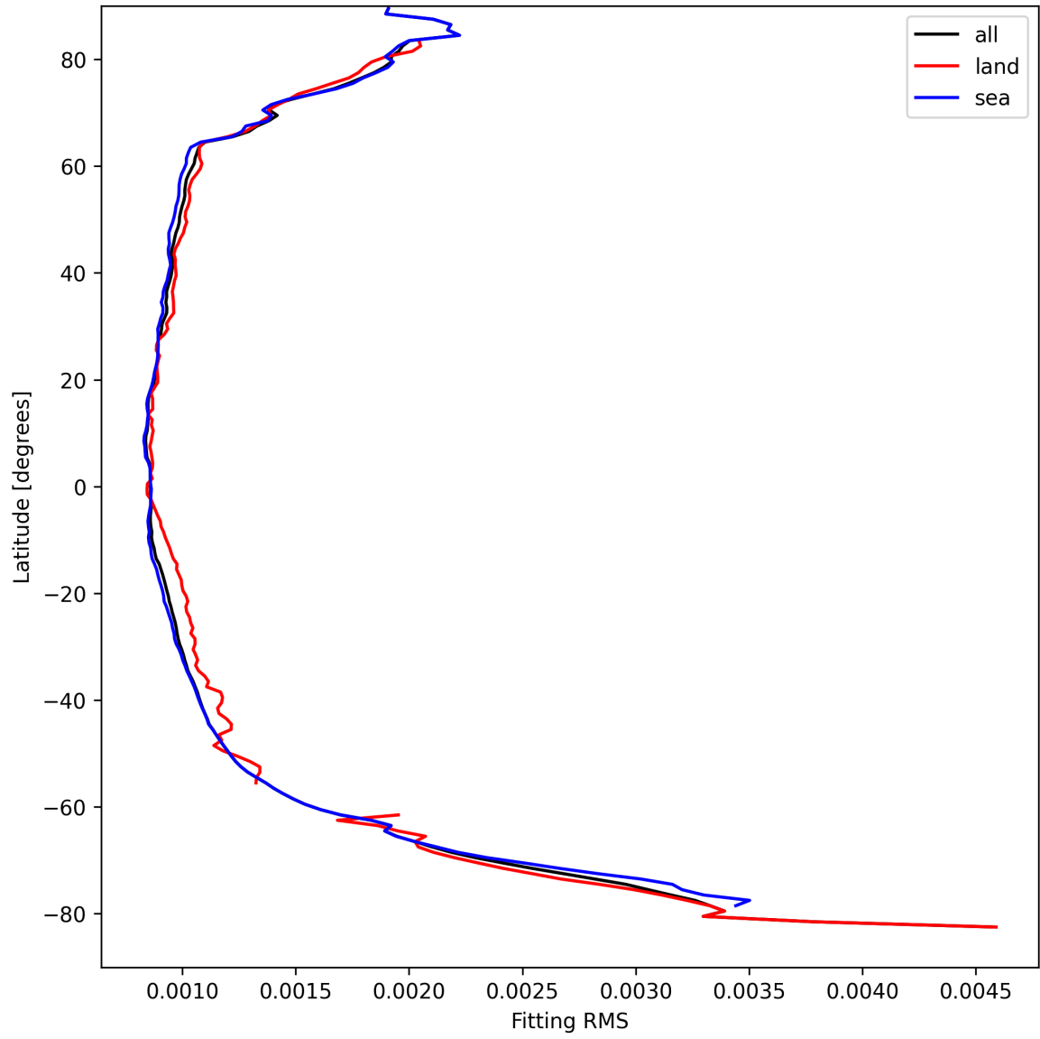
Figure 16: Zonal average of “Fitting RMS” for 2024-09-03 to 2024-09-05.
