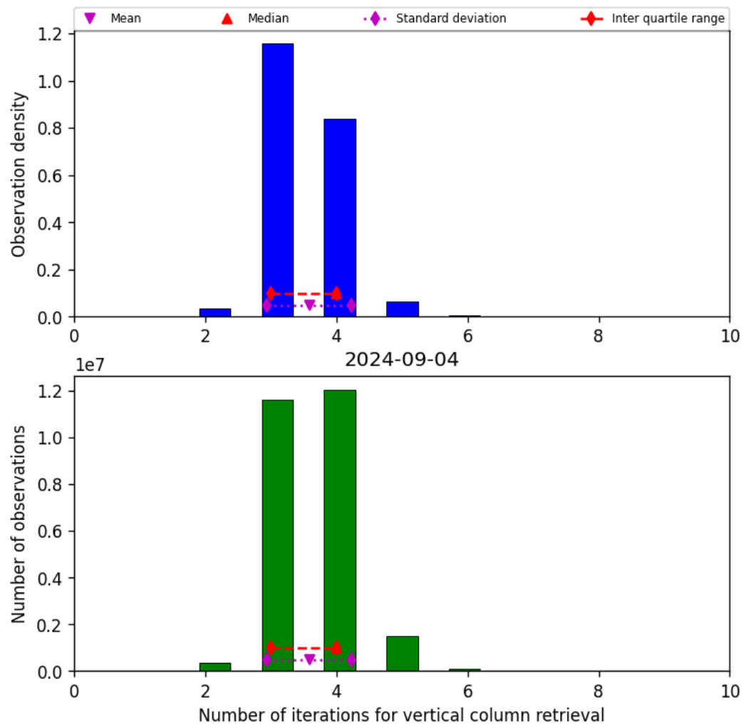
Figure 26: Histogram of “Number of iterations for vertical column retrieval” for 2024-09-03 to 2024-09-05
