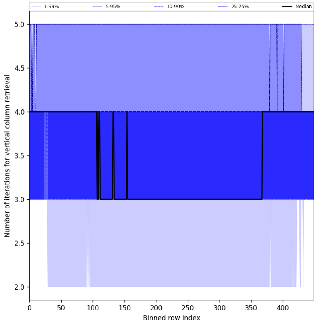
Figure 33: Along track statistics of “Number of iterations for vertical column retrieval” for 2024-09-03 to 2024-09-05
