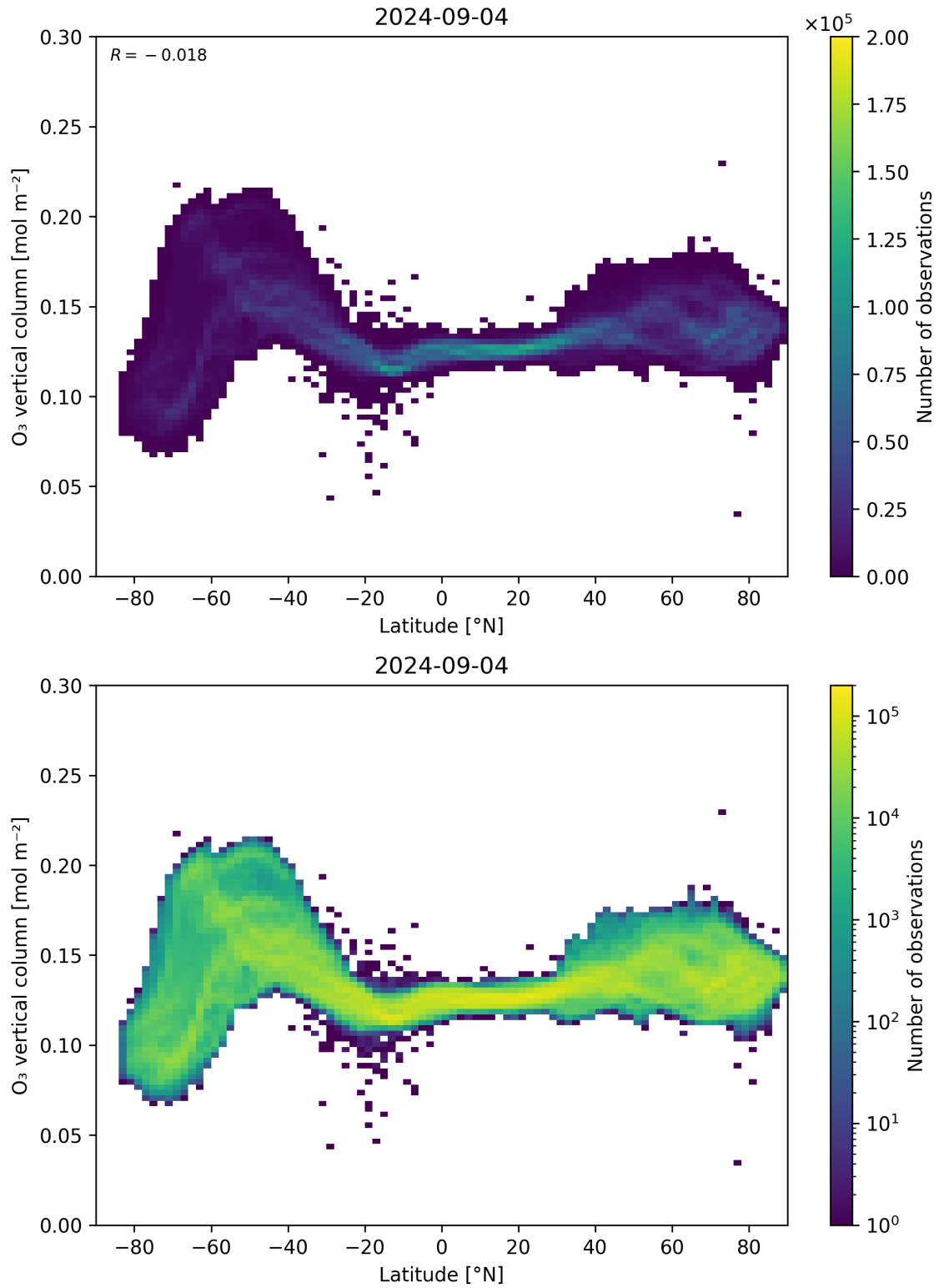
Figure 36: Scatter density plot of “Latitude” against “O 3 vertical column” for 2024-09-03 to 2024-09-05.
