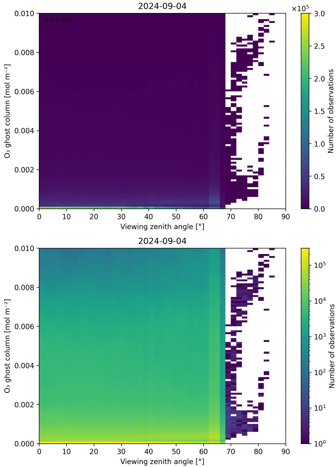
Figure 51: Scatter density plot of “Viewing zenith angle” against “O 3 ghost column” for 2024-09-03 to 2024-09-05.
