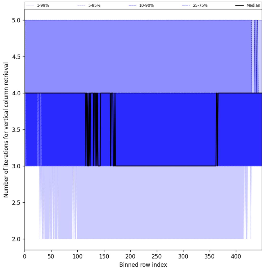
Figure 33: Along track statistics of “Number of iterations for vertical column retrieval” for 2024-09-04 to 2024-09-06
