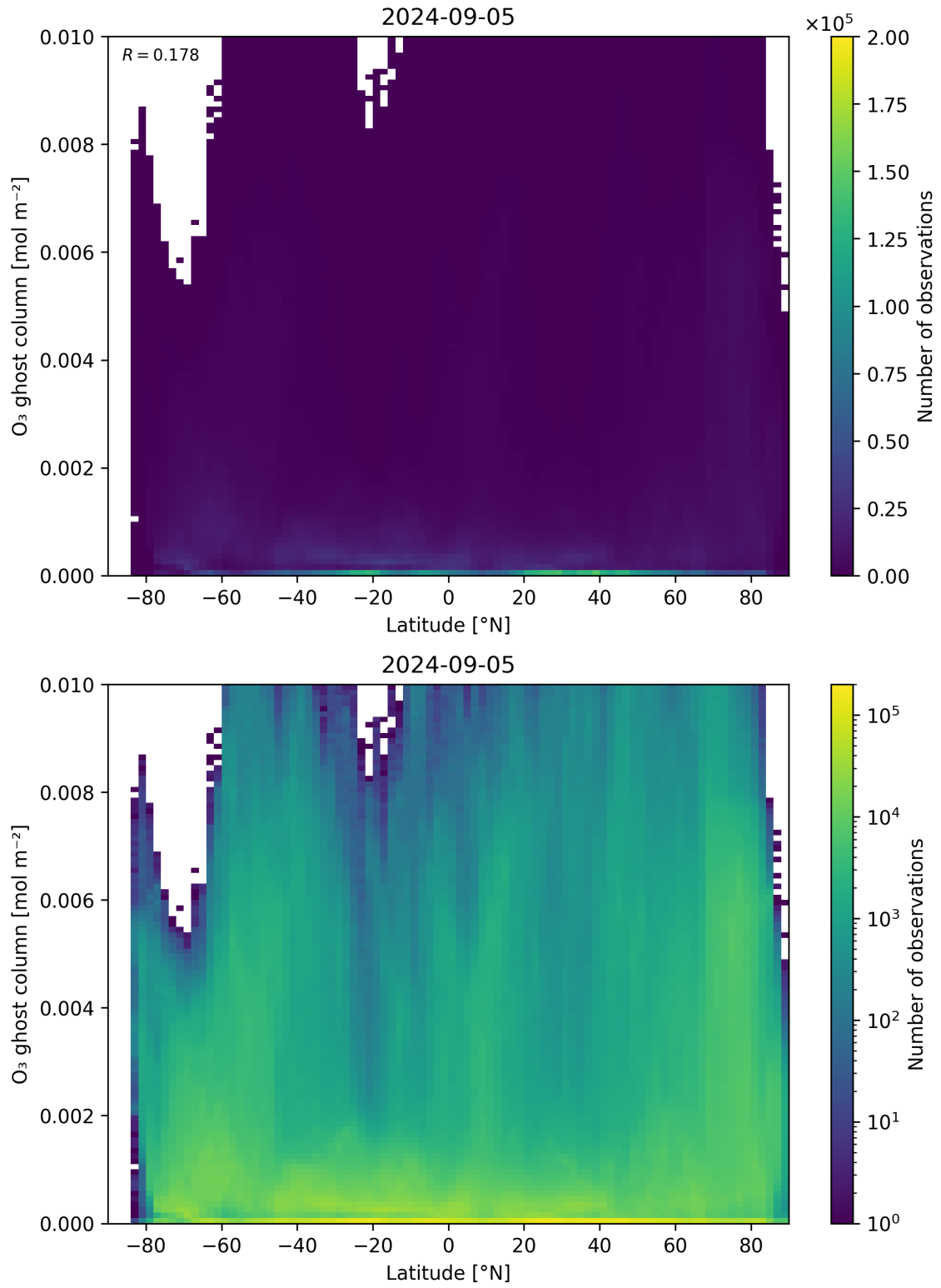
Figure 35: Scatter density plot of “Latitude” against “O 3 ghost column” for 2024-09-04 to 2024-09-06.
