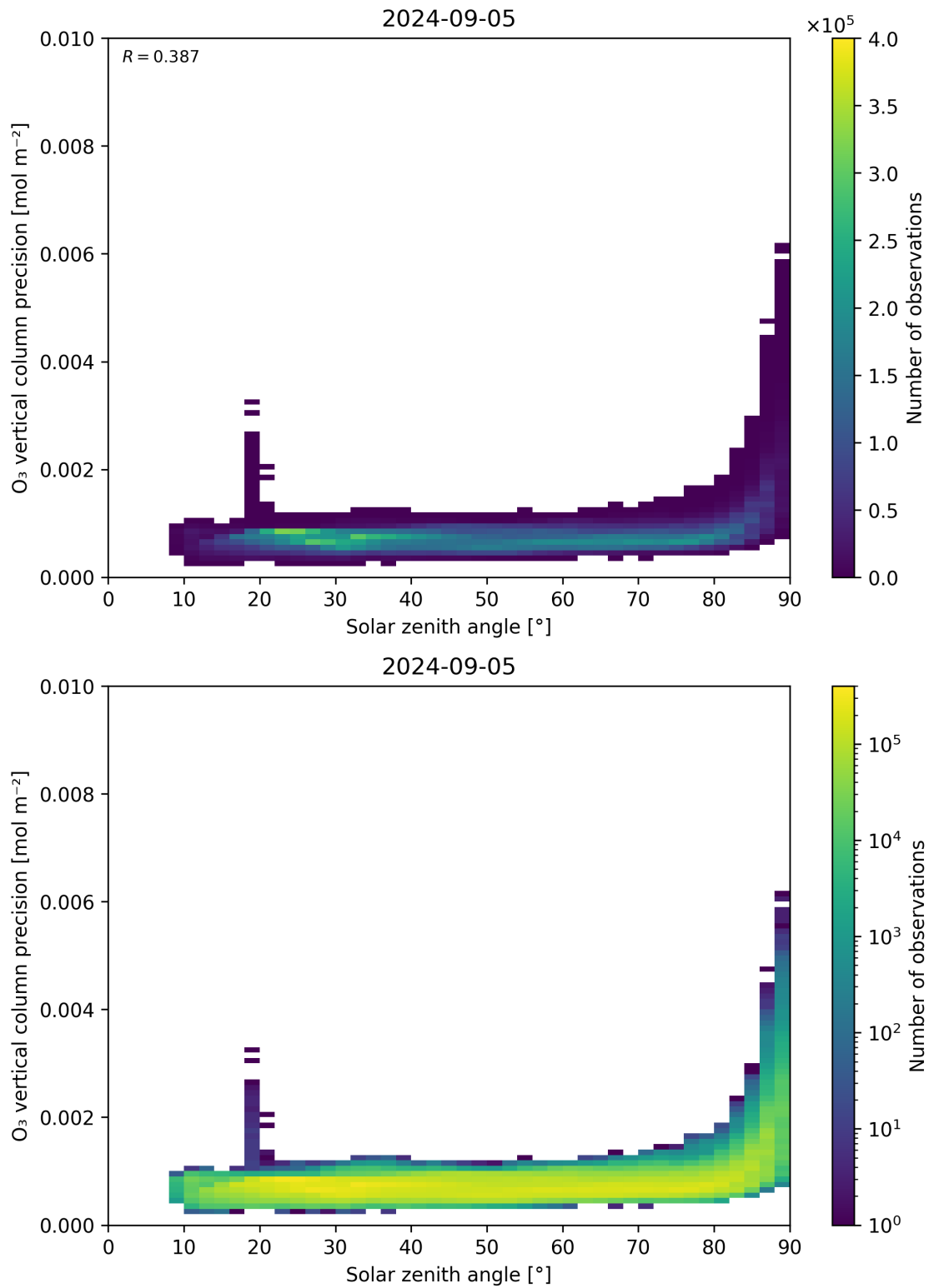
Figure 48: Scatter density plot of “Solar zenith angle” against “O 3 vertical column precision” for 2024-09-04 to 2024-09-06.
