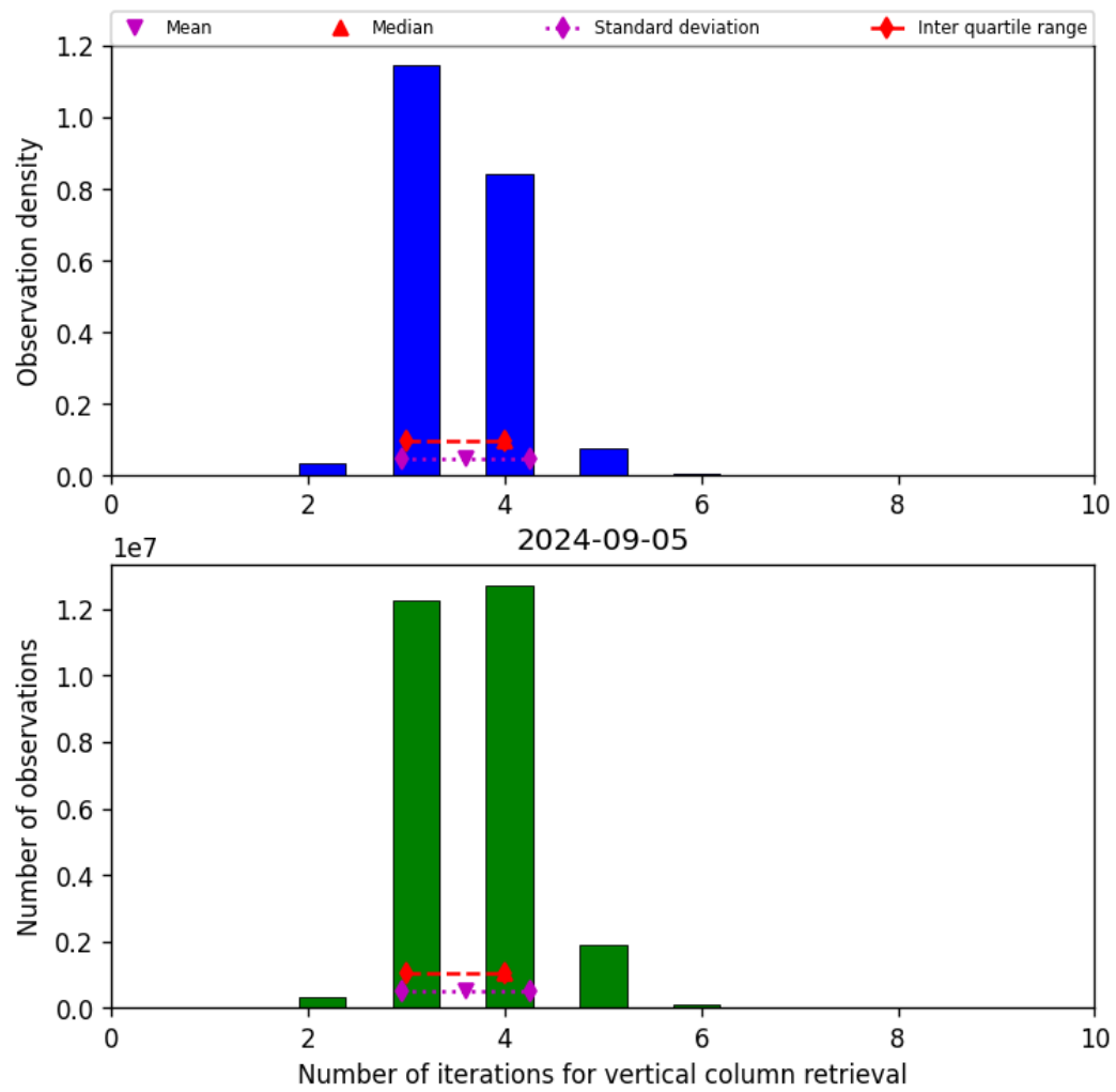
Figure 26: Histogram of “Number of iterations for vertical column retrieval” for 2024-09-04 to 2024-09-06
