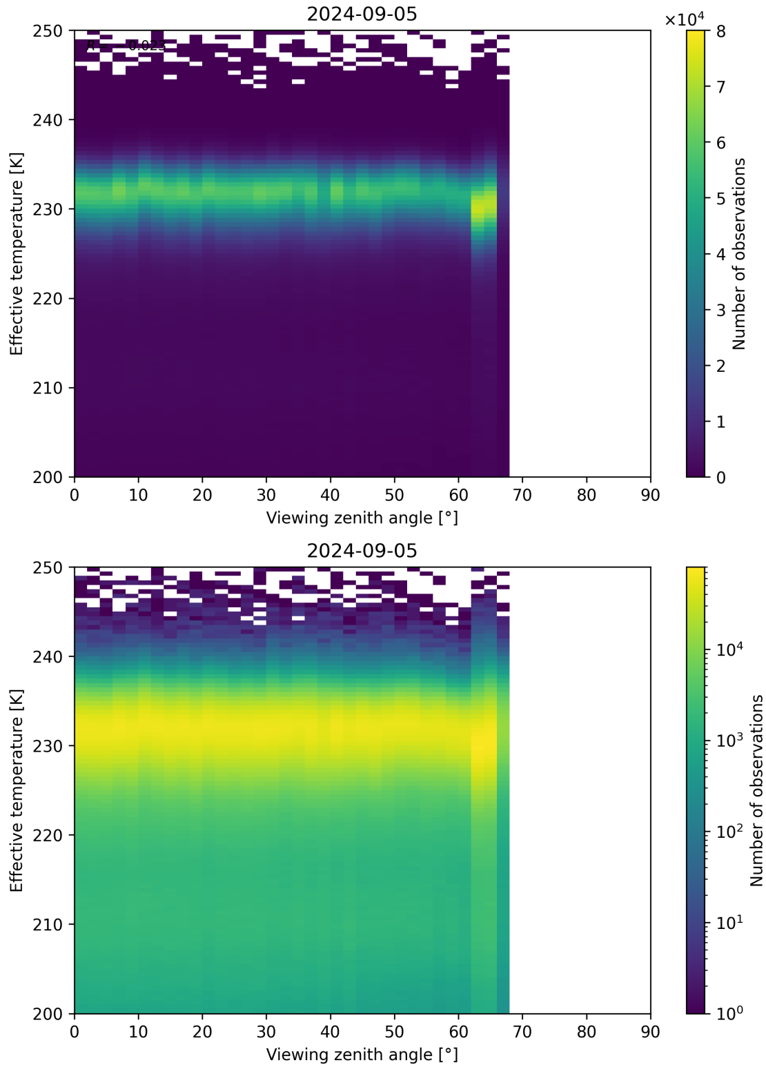
Figure 50: Scatter density plot of “Viewing zenith angle” against “Effective temperature” for 2024-09-04 to 2024-09-06.
