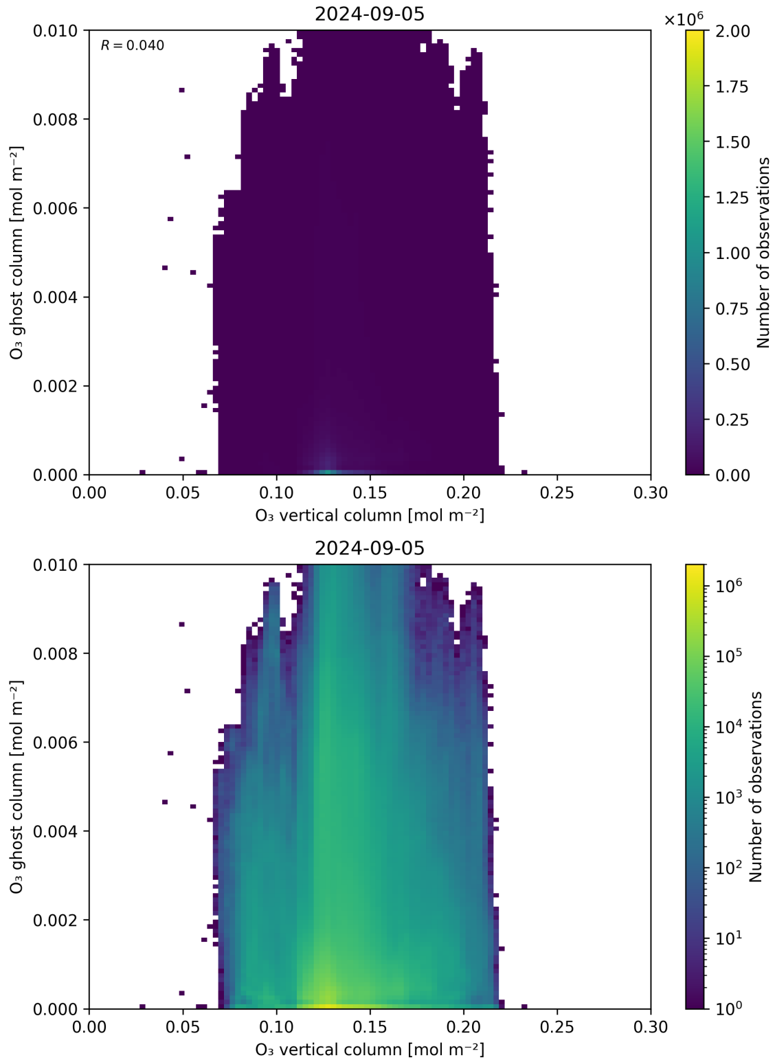
Figure 40: Scatter density plot of “O 3 vertical column” against “O 3 ghost column” for 2024-09-04 to 2024-09-06.
