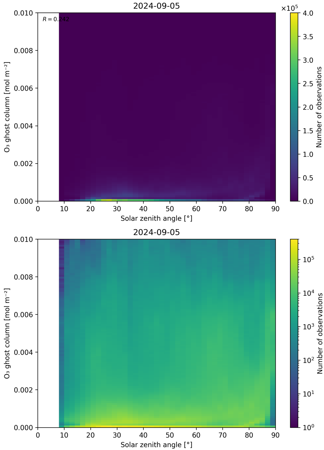
Figure 46: Scatter density plot of “Solar zenith angle” against “O 3 ghost column” for 2024-09-04 to 2024-09-06.
