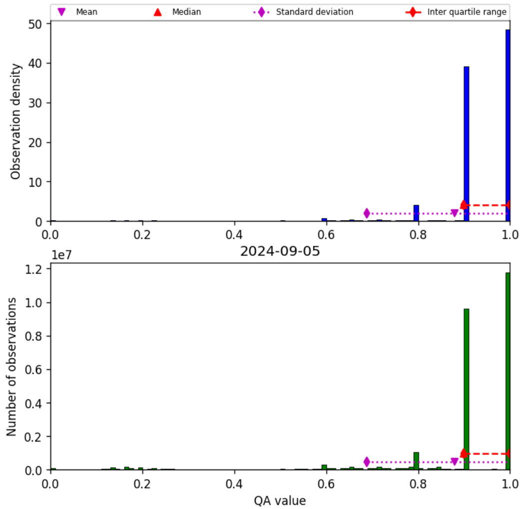
Figure 20: Histogram of “QA value” for 2024-09-04 to 2024-09-06
