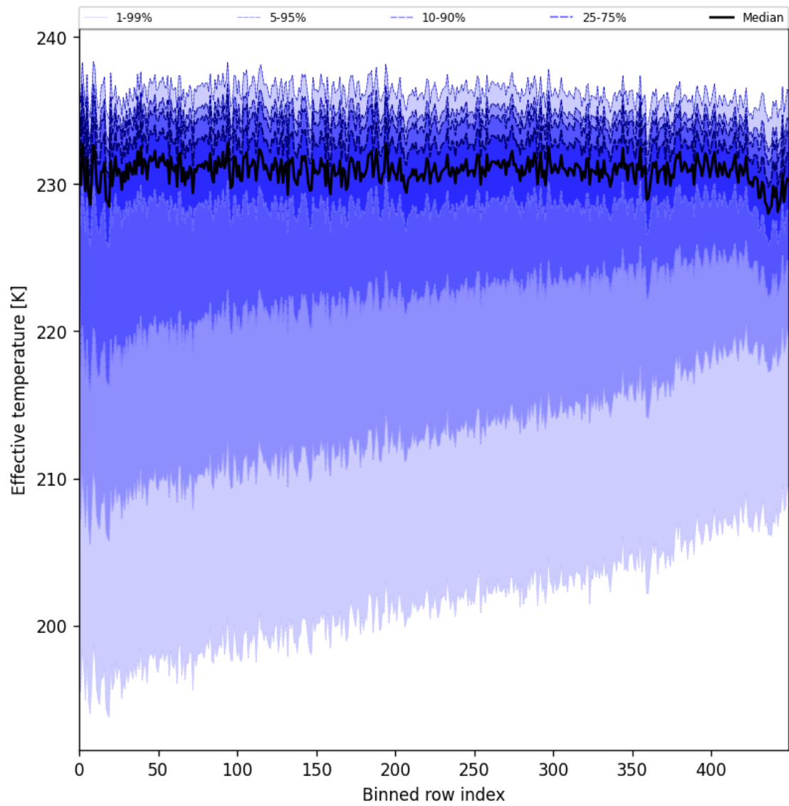
Figure 31: Along track statistics of “Effective temperature” for 2024-09-04 to 2024-09-06
