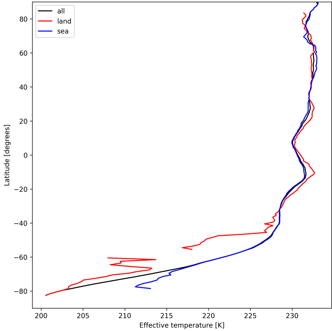
Figure 17: Zonal average of "Effective temperature" for 2024-09-04 to 2024-09-06.
