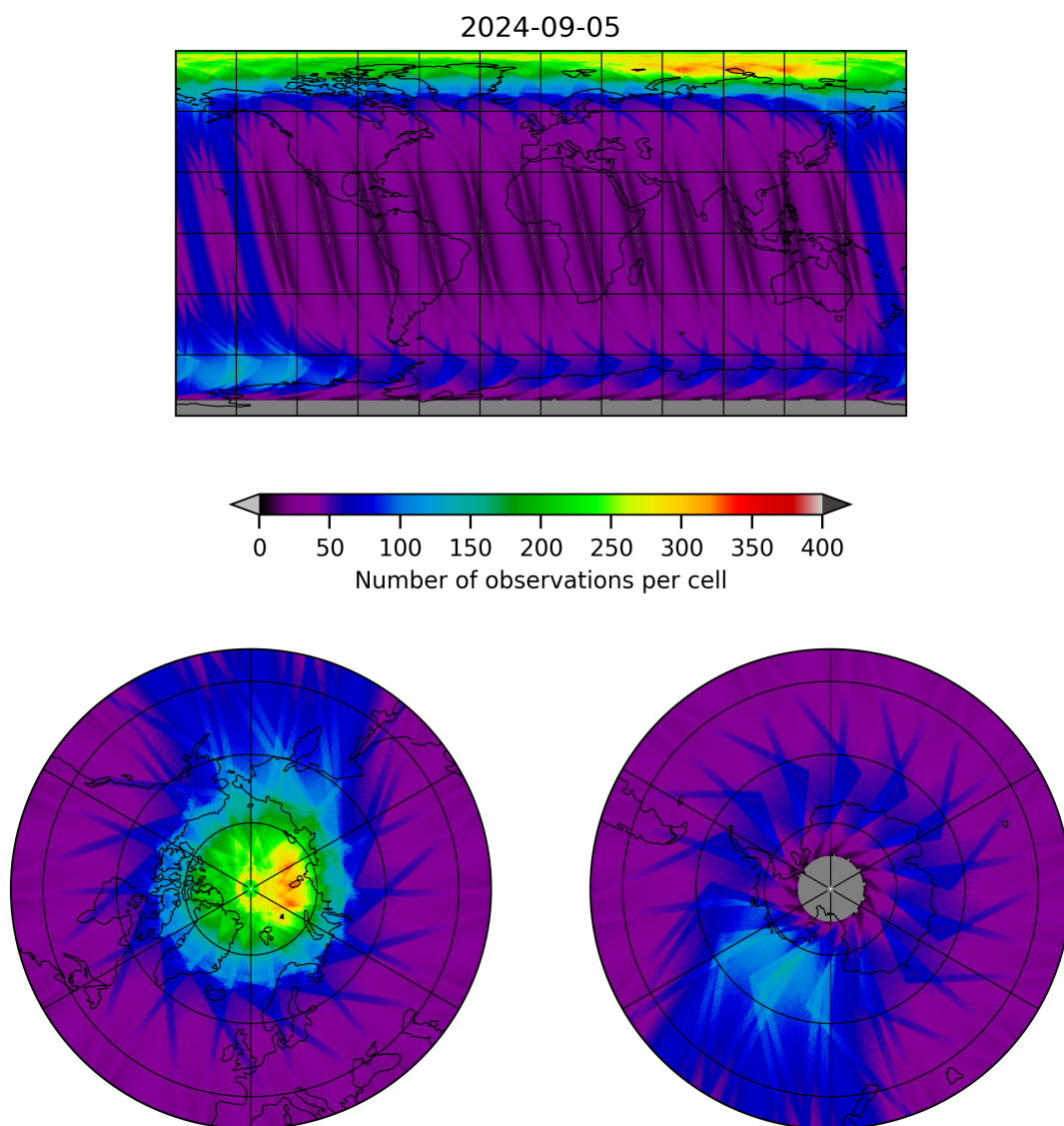
Figure 12: Map of the number of observations for 2024-09-04 to 2024-09-06
