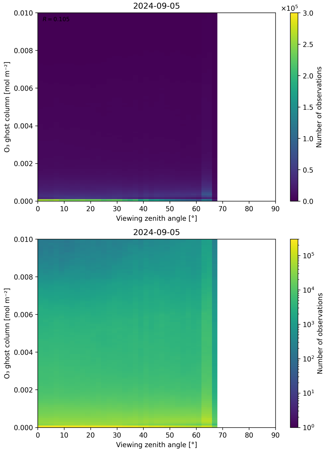
Figure 51: Scatter density plot of “Viewing zenith angle” against “O 3 ghost column” for 2024-09-04 to 2024-09-06.
