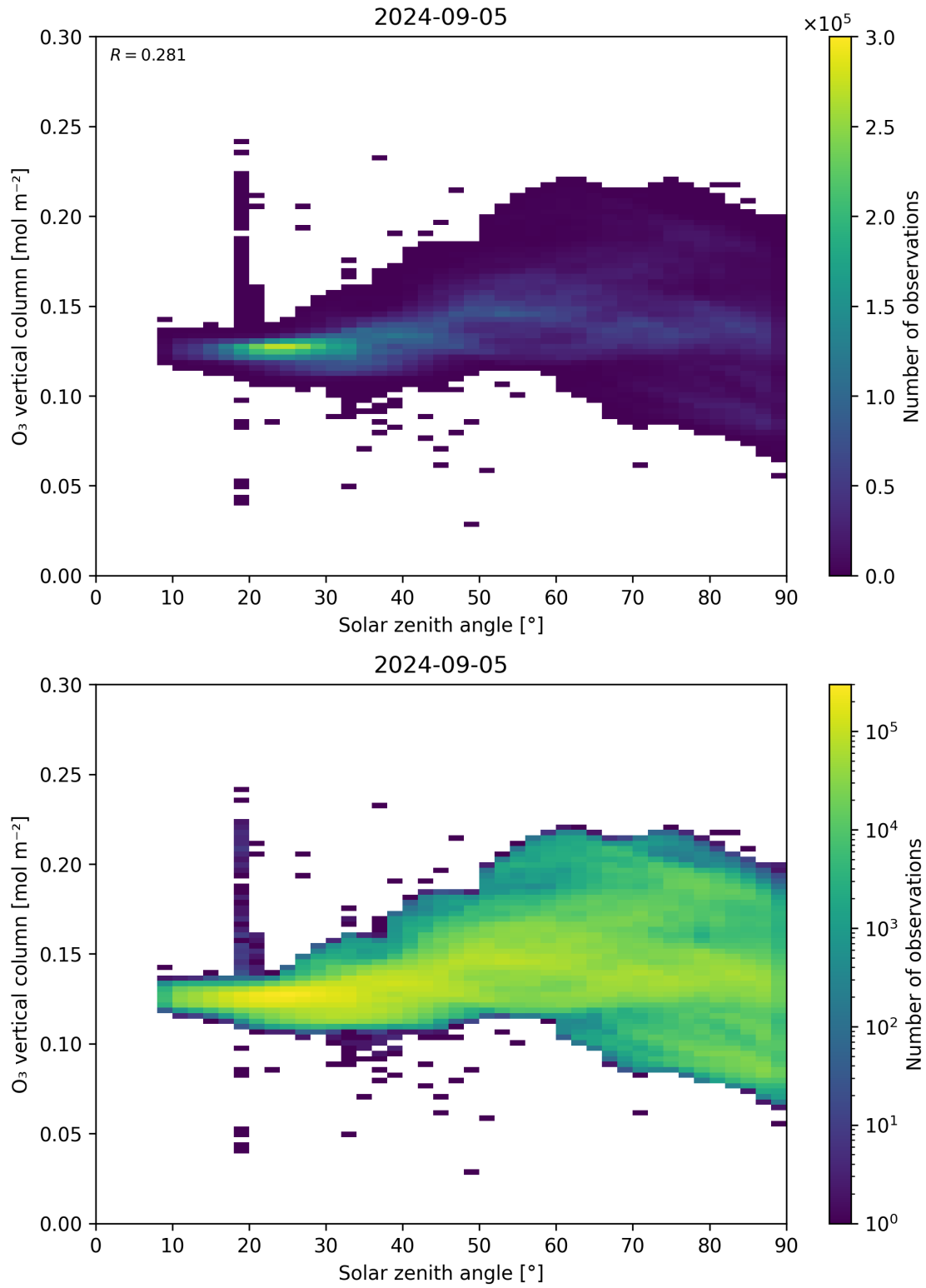
Figure 47: Scatter density plot of “Solar zenith angle” against “O 3 vertical column” for 2024-09-04 to 2024-09-06.
