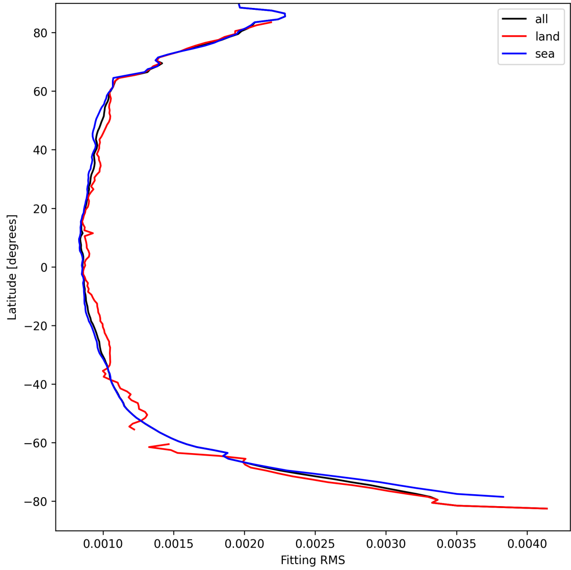
Figure 16: Zonal average of “Fitting RMS” for 2024-09-04 to 2024-09-06.
