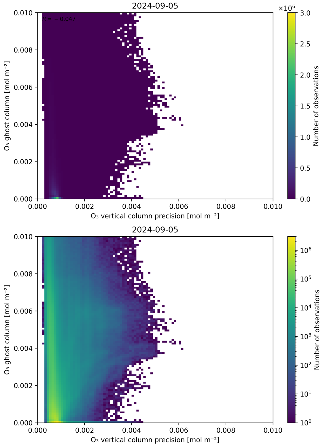
Figure 43: Scatter density plot of “ \text{O}_3 vertical column precision” against “ \text{O}_3 ghost column” for 2024-09-04 to 2024-09-06.
