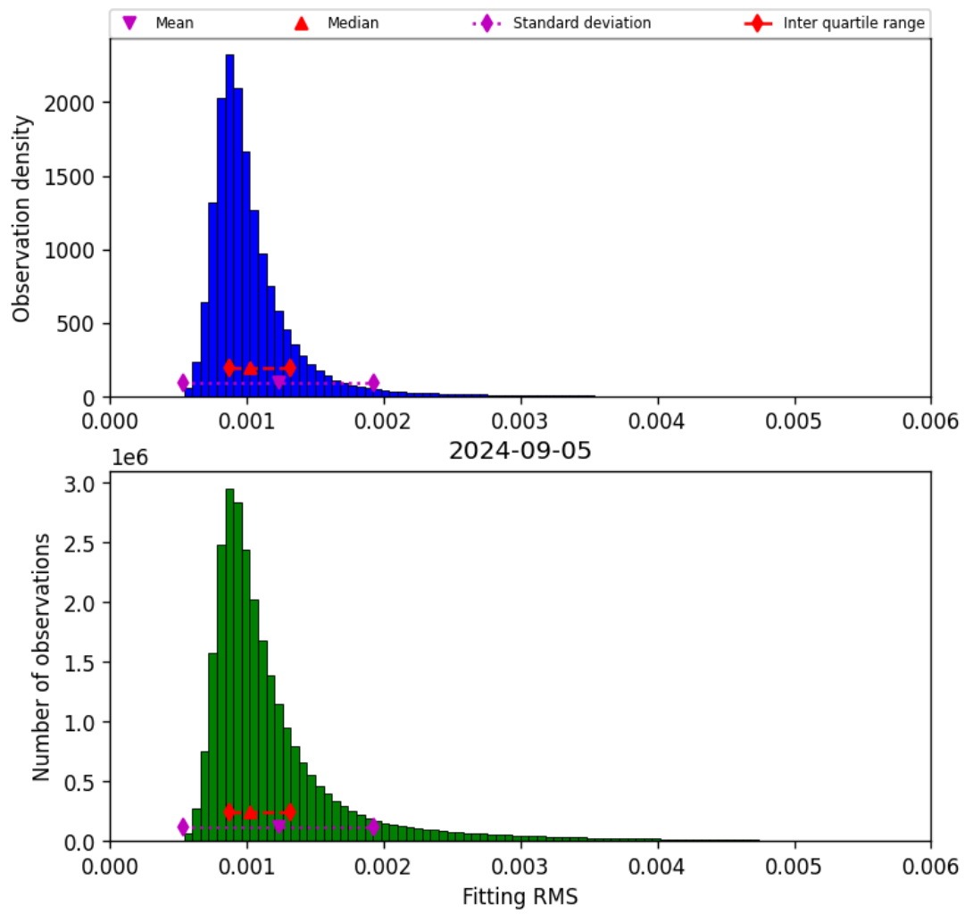
Figure 23: Histogram of “Fitting RMS” for 2024-09-04 to 2024-09-06
