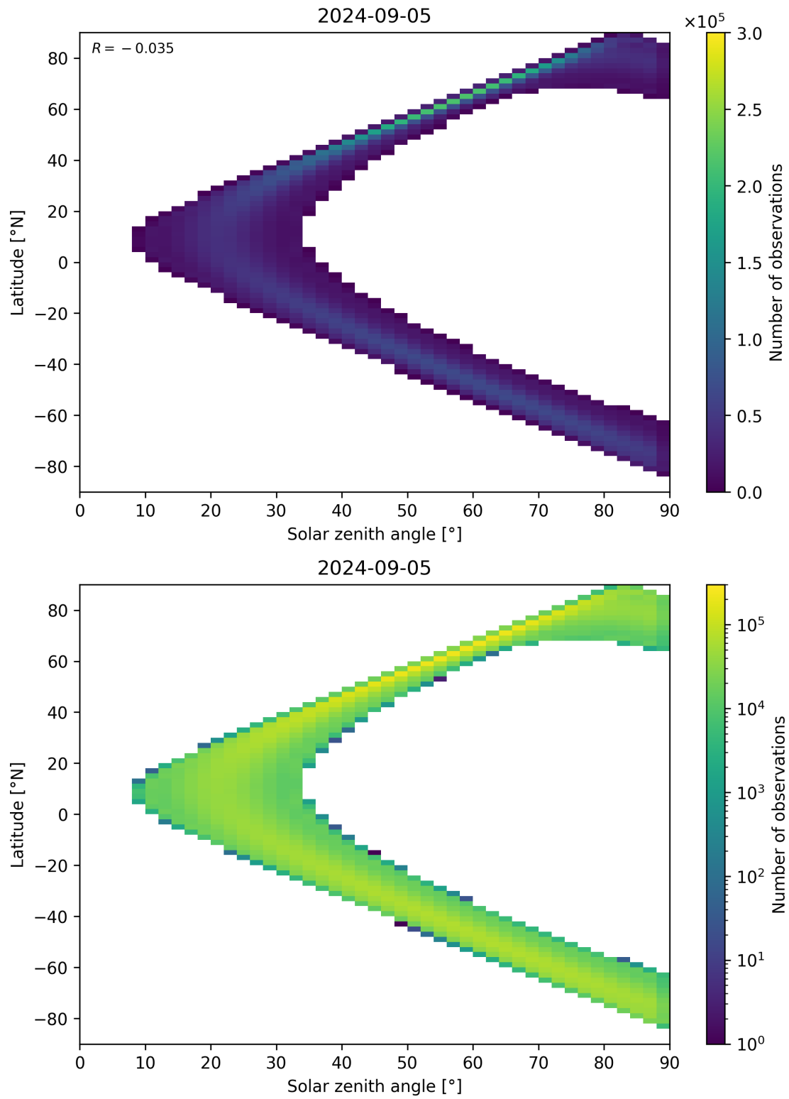
Figure 44: Scatter density plot of “Solar zenith angle” against “Latitude” for 2024-09-04 to 2024-09-06.
