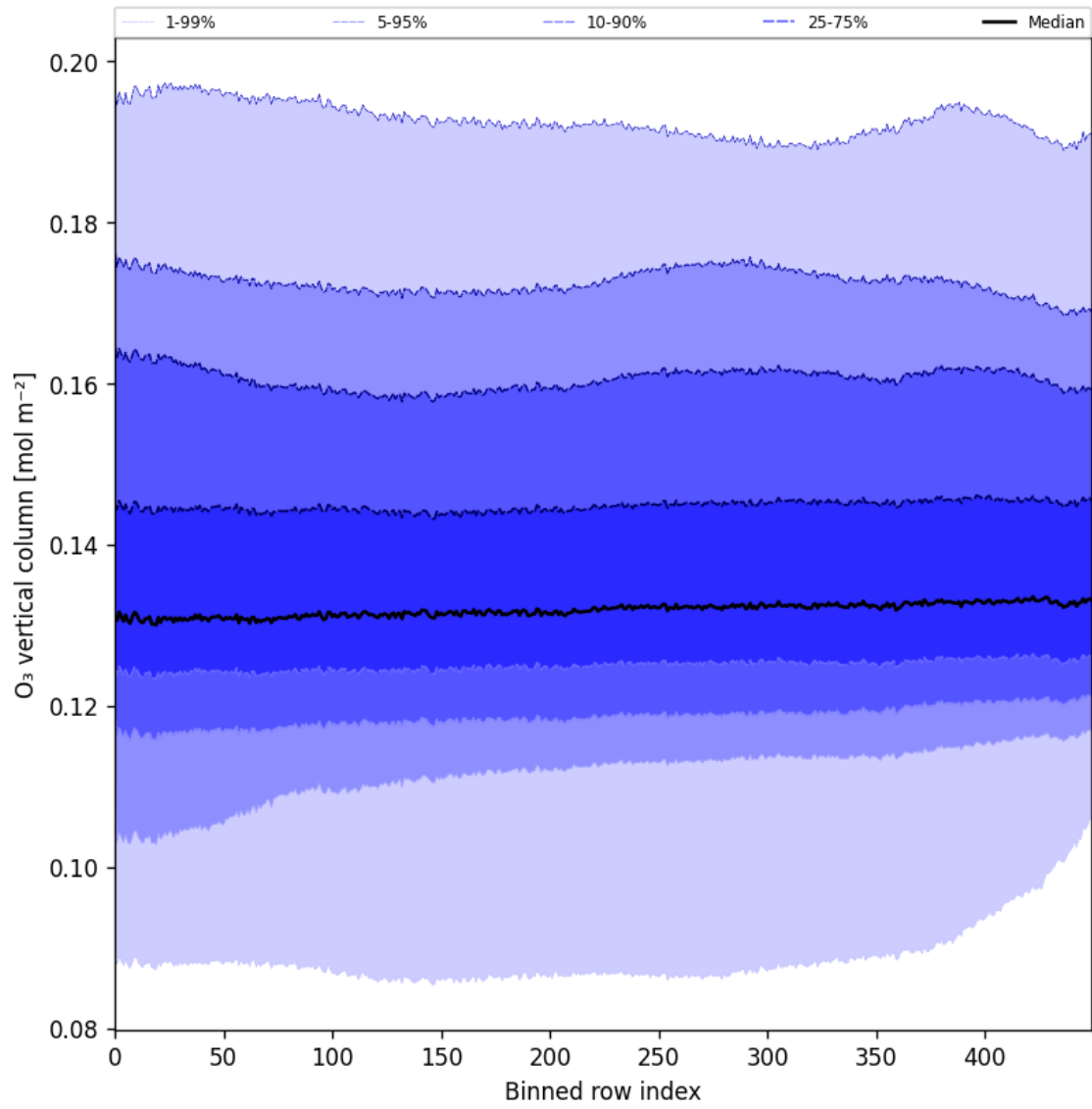
Figure 28: Along track statistics of “O 3 vertical column” for 2024-09-04 to 2024-09-06
