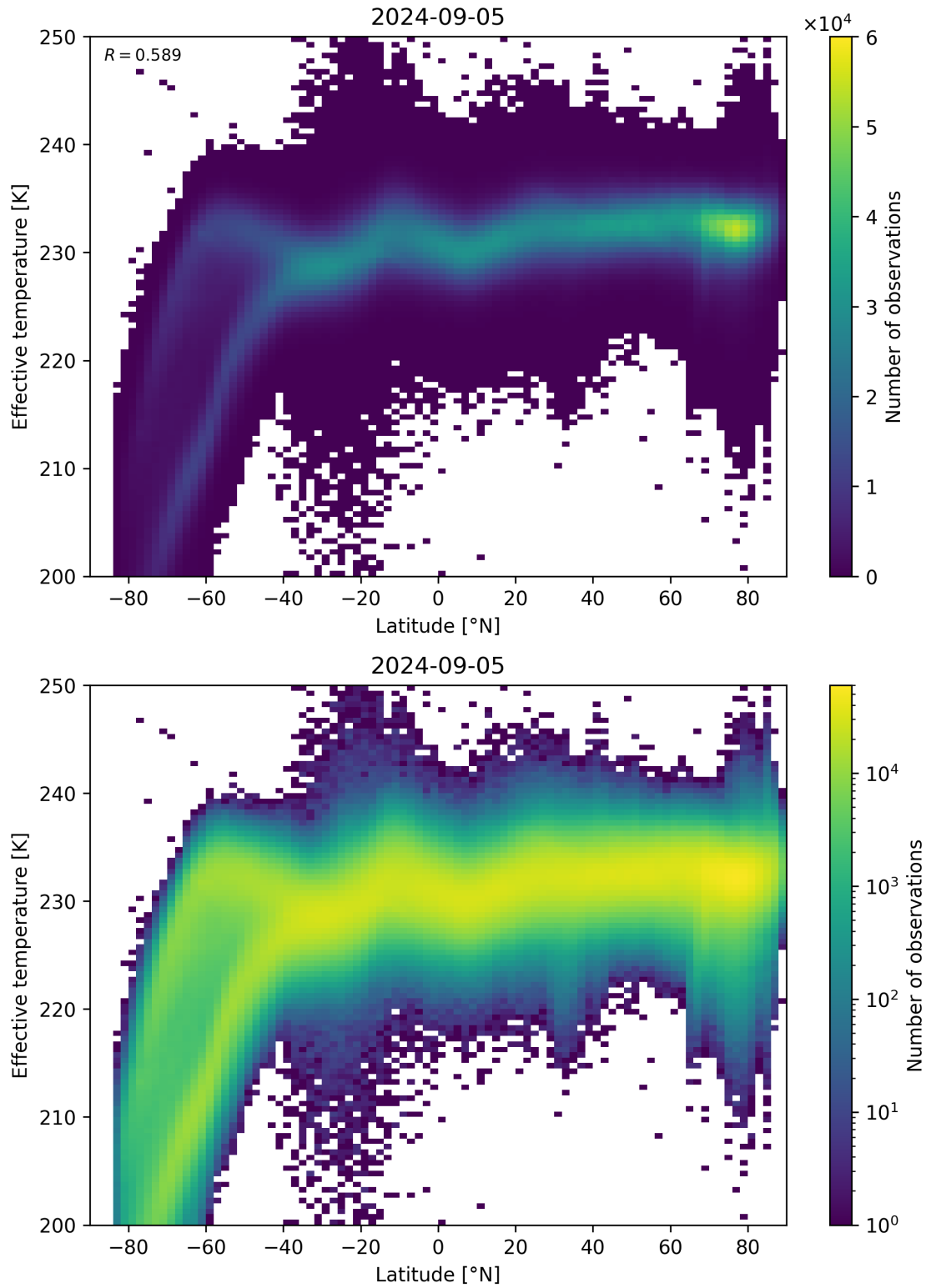
Figure 34: Scatter density plot of “Latitude” against “Effective temperature” for 2024-09-04 to 2024-09-06.
