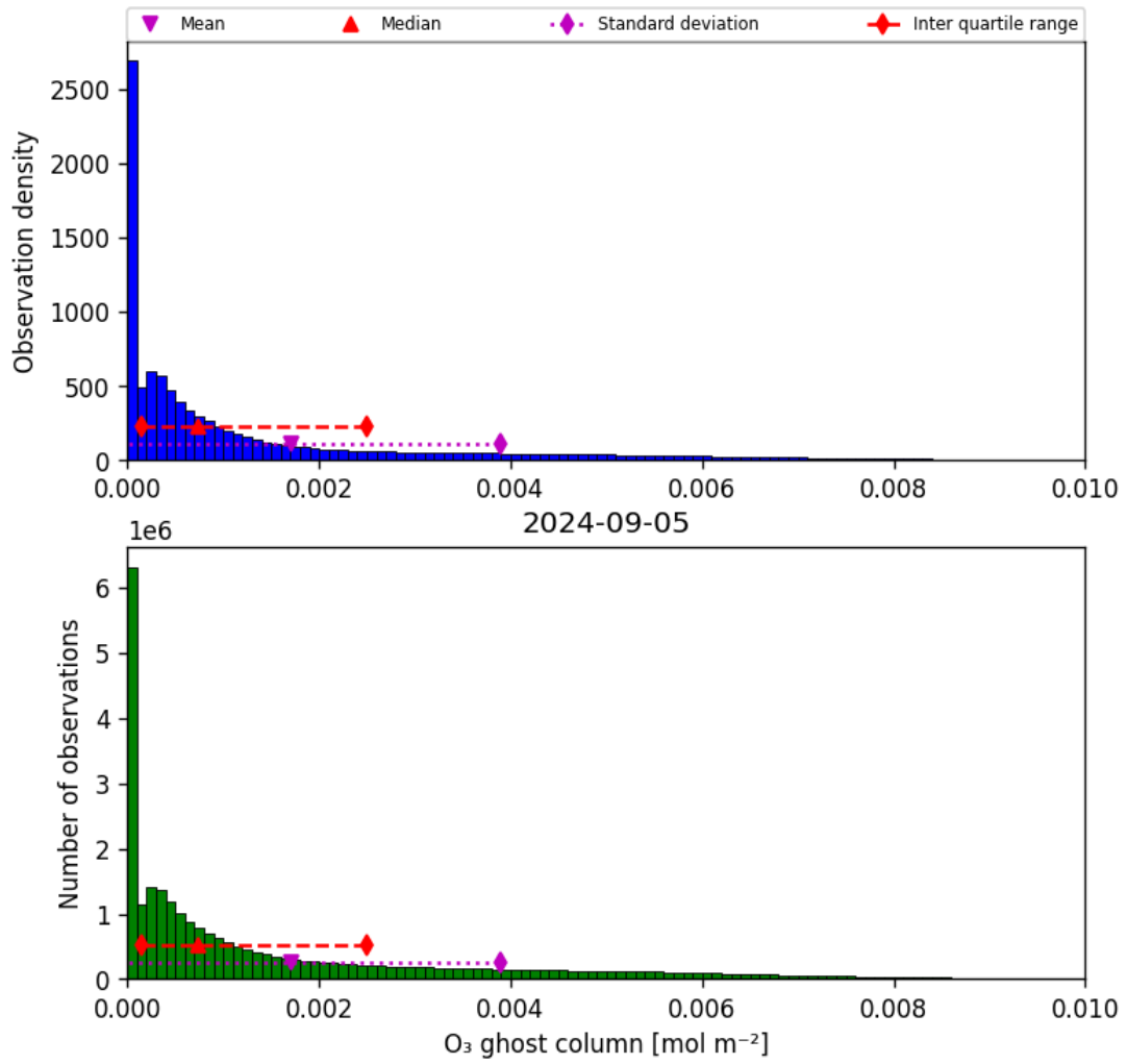
Figure 25: Histogram of “O 3 ghost column” for 2024-09-04 to 2024-09-06
