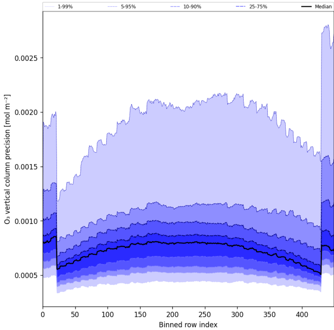
Figure 29: Along track statistics of “O 3 vertical column precision” for 2024-09-04 to 2024-09-06
