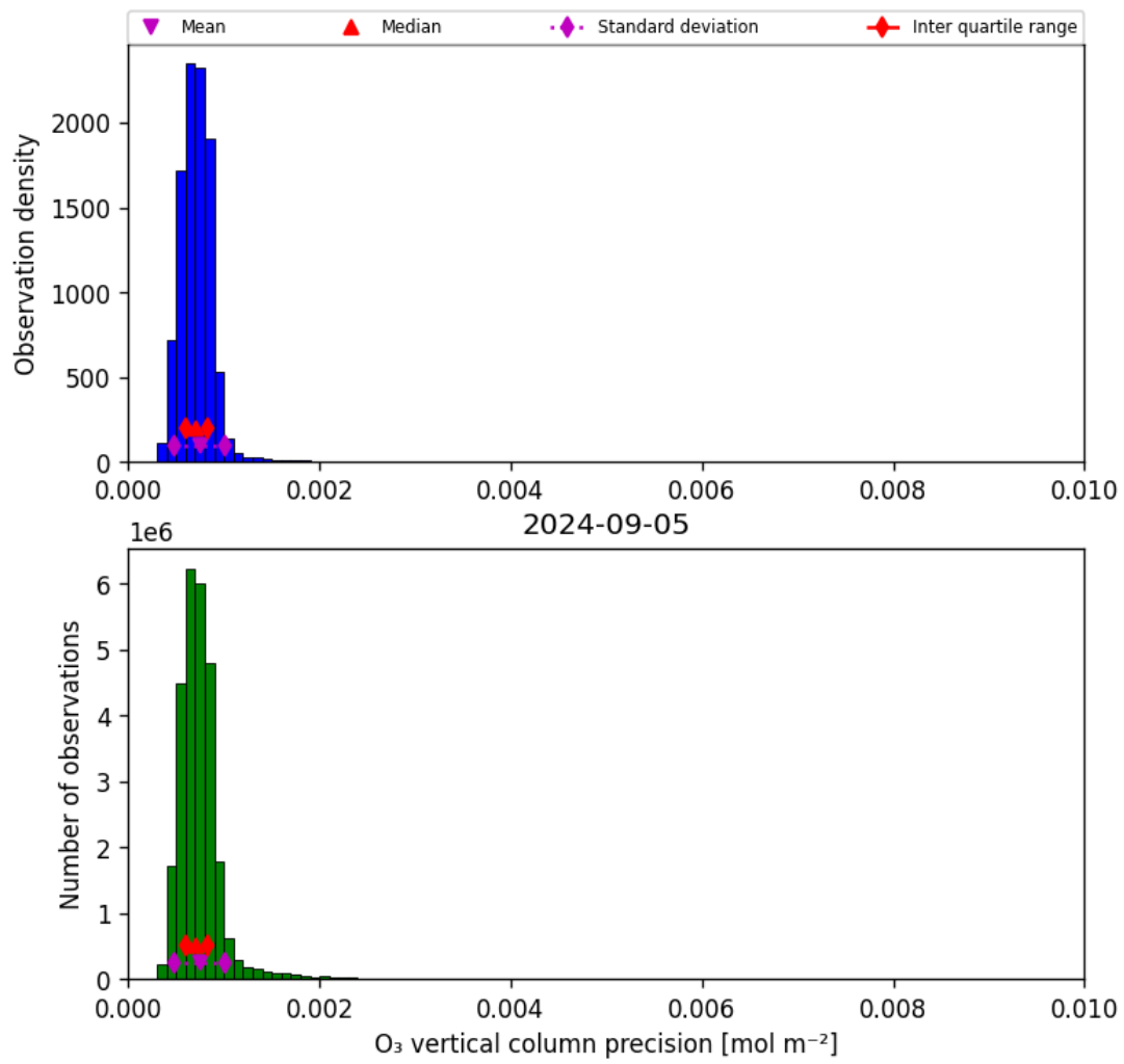
Figure 22: Histogram of “O 3 vertical column precision” for 2024-09-04 to 2024-09-06
