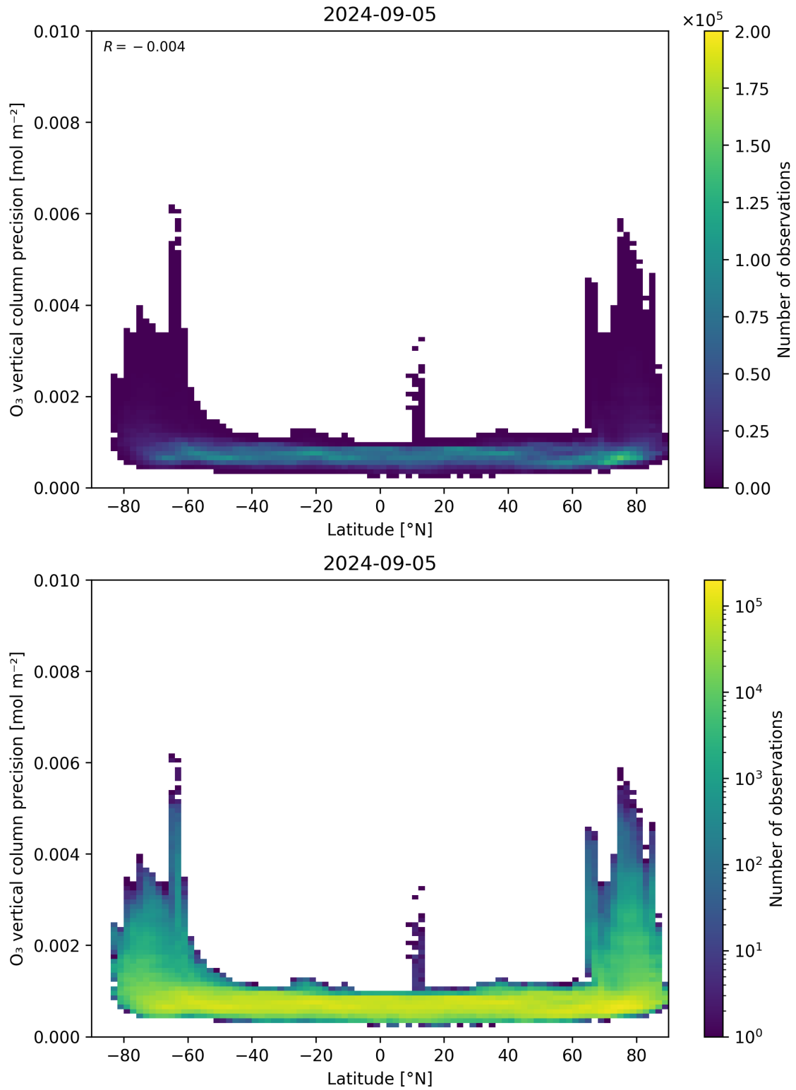
Figure 37: Scatter density plot of “Latitude” against “O 3 vertical column precision” for 2024-09-04 to 2024-09-06.
