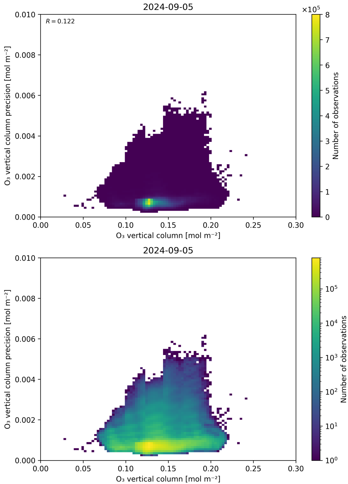
Figure 41: Scatter density plot of “O 3 vertical column” against “O 3 vertical column precision” for 2024-09-04 to 2024-09-06.
