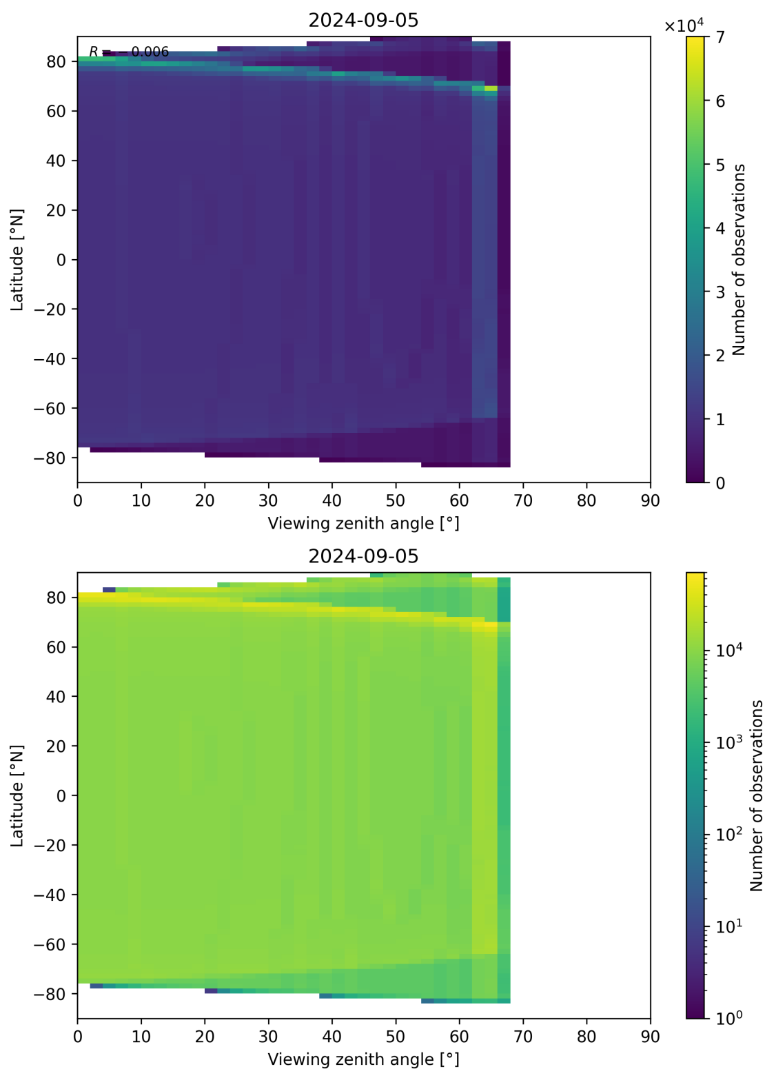
Figure 49: Scatter density plot of “Viewing zenith angle” against “Latitude” for 2024-09-04 to 2024-09-06.
