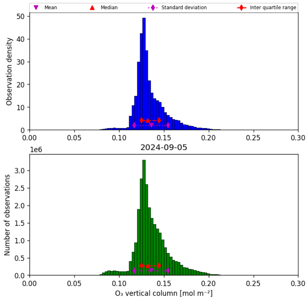
Figure 21: Histogram of “O 3 vertical column” for 2024-09-04 to 2024-09-06
