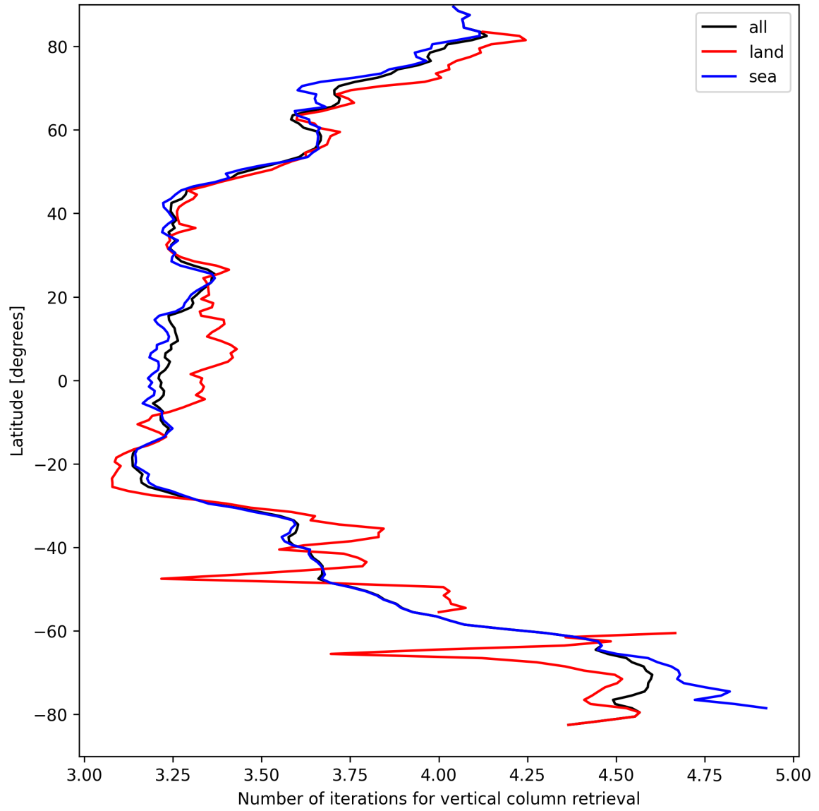
Figure 19: Zonal average of “Number of iterations for vertical column retrieval” for 2024-09-04 to 2024-09-06.
