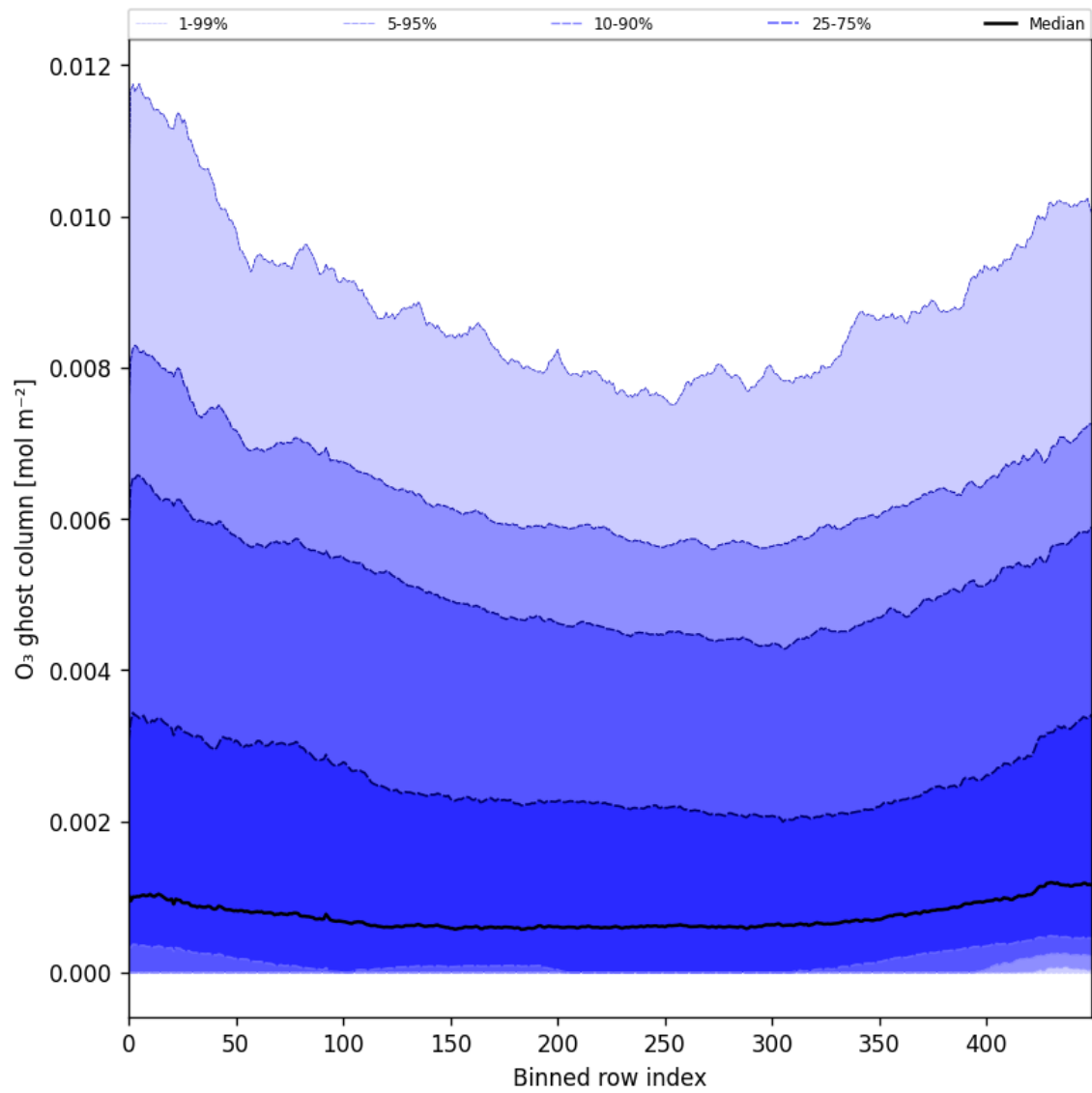
Figure 32: Along track statistics of “O 3 ghost column” for 2024-09-04 to 2024-09-06
