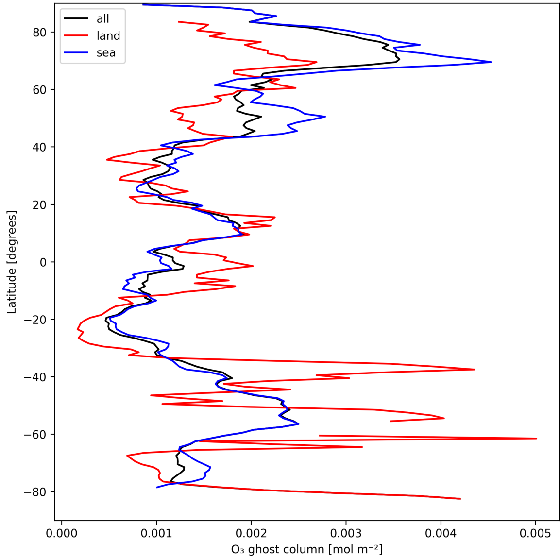
Figure 18: Zonal average of "O 3 ghost column" for 2024-09-04 to 2024-09-06.
