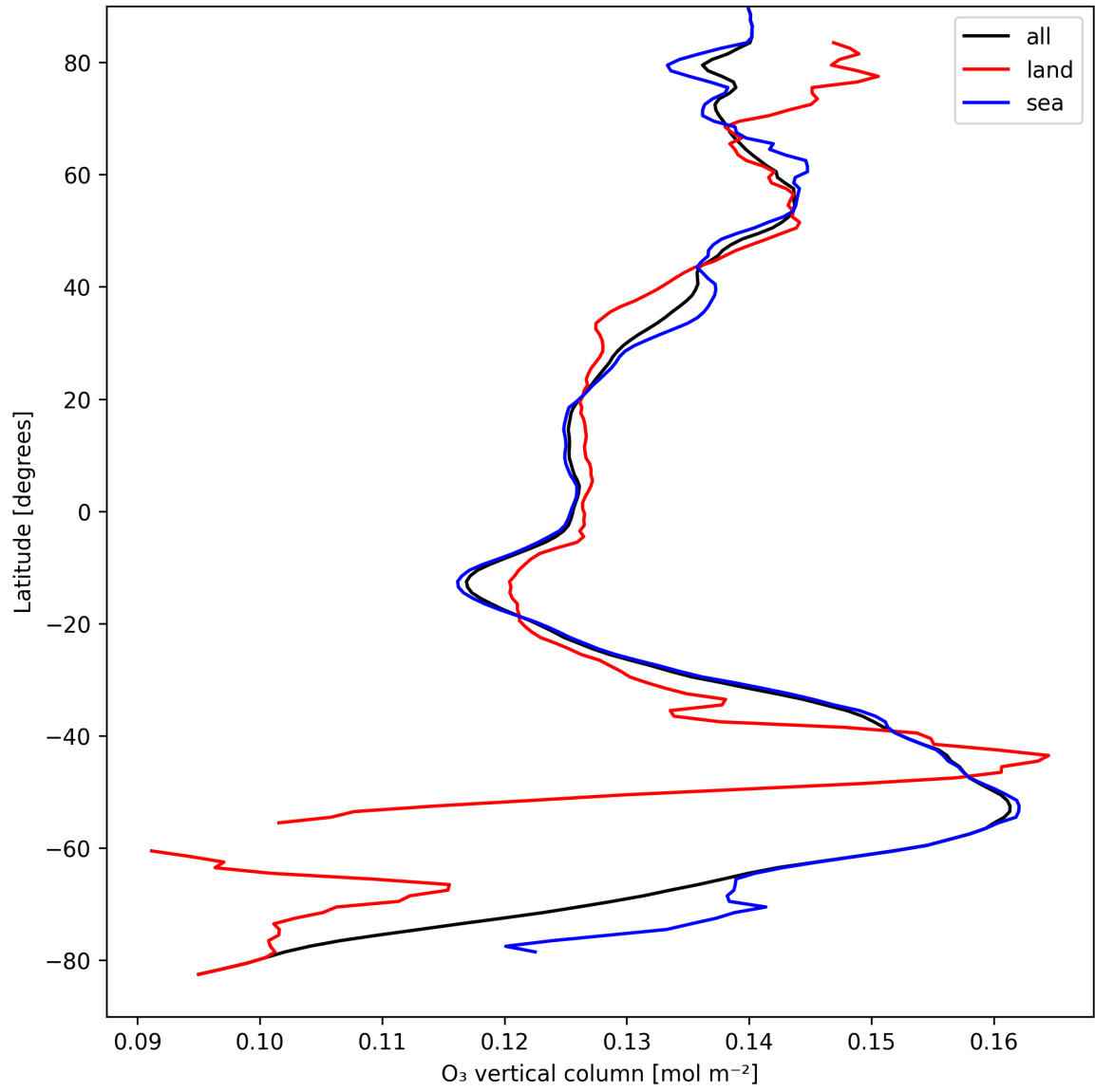
Figure 14: Zonal average of “O 3 vertical column” for 2024-09-04 to 2024-09-06.
