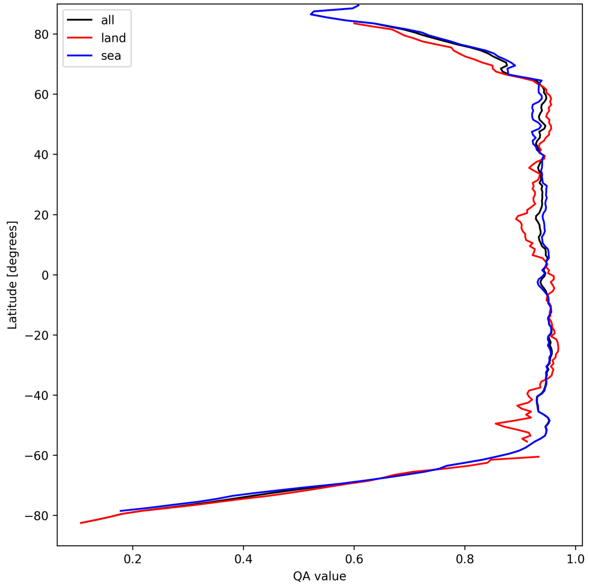
Figure 13: Zonal average of “QA value” for 2024-09-04 to 2024-09-06.
