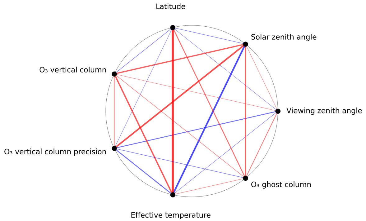
Figure 1: Map of correlation graph for 2024-09-04 to 2024-09-06.
