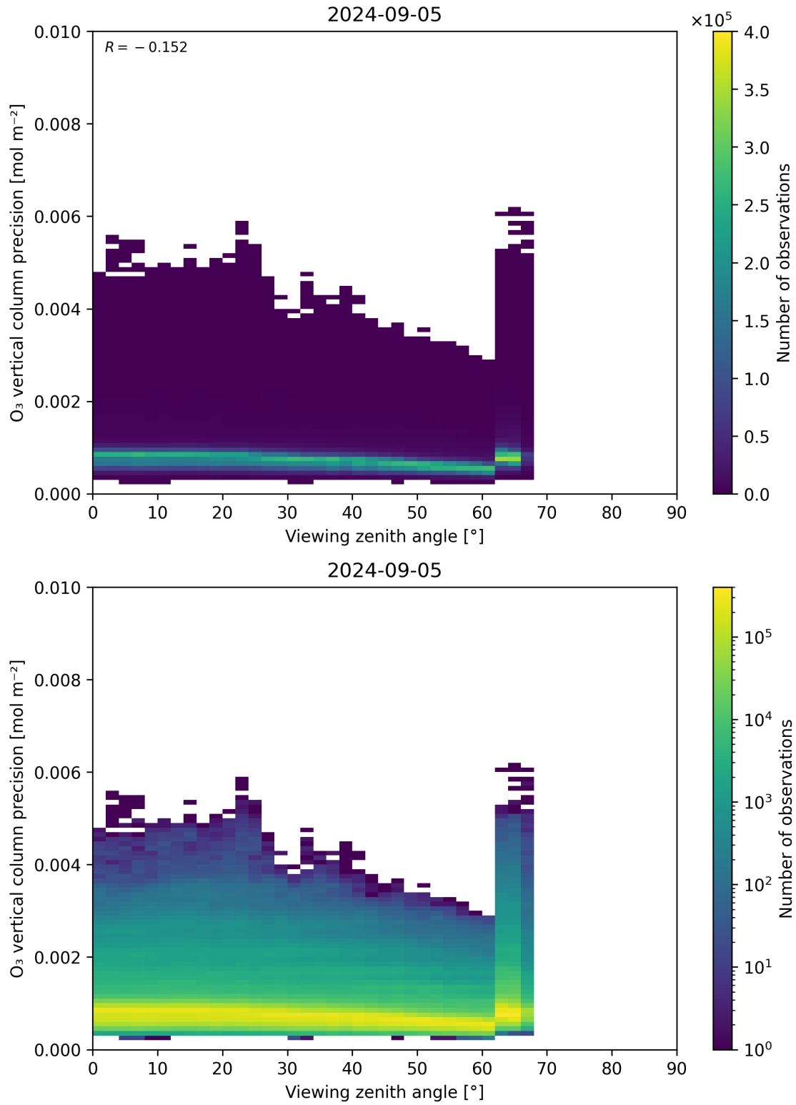
Figure 53: Scatter density plot of “Viewing zenith angle” against “O 3 vertical column precision” for 2024-09-04 to 2024-09-06.
