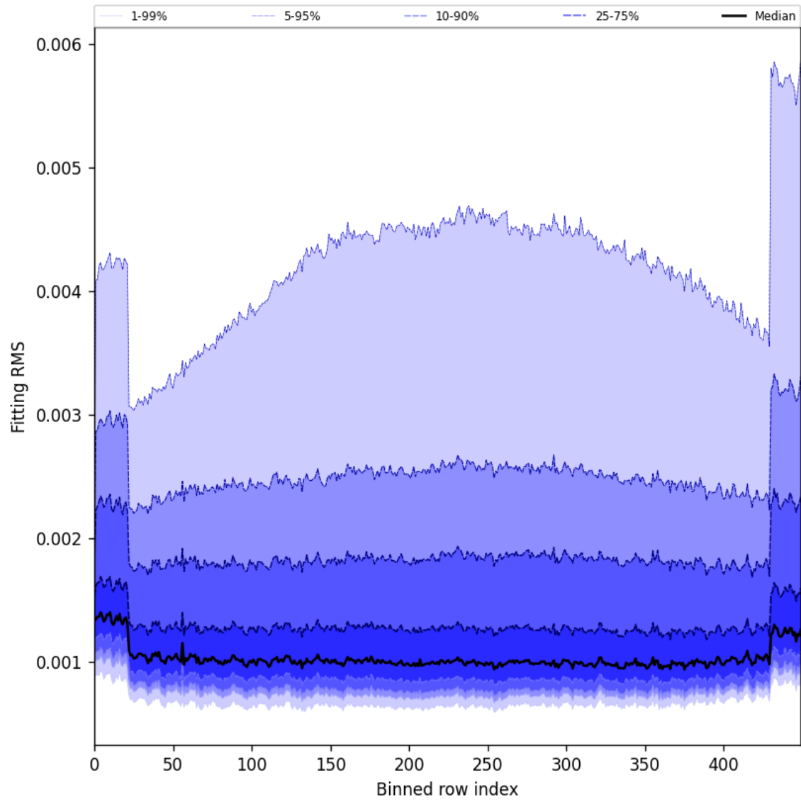
Figure 30: Along track statistics of “Fitting RMS” for 2024-09-04 to 2024-09-06
