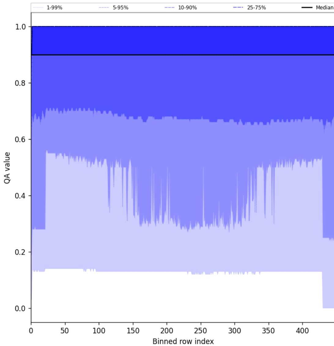
Figure 27: Along track statistics of “QA value” for 2024-09-04 to 2024-09-06
