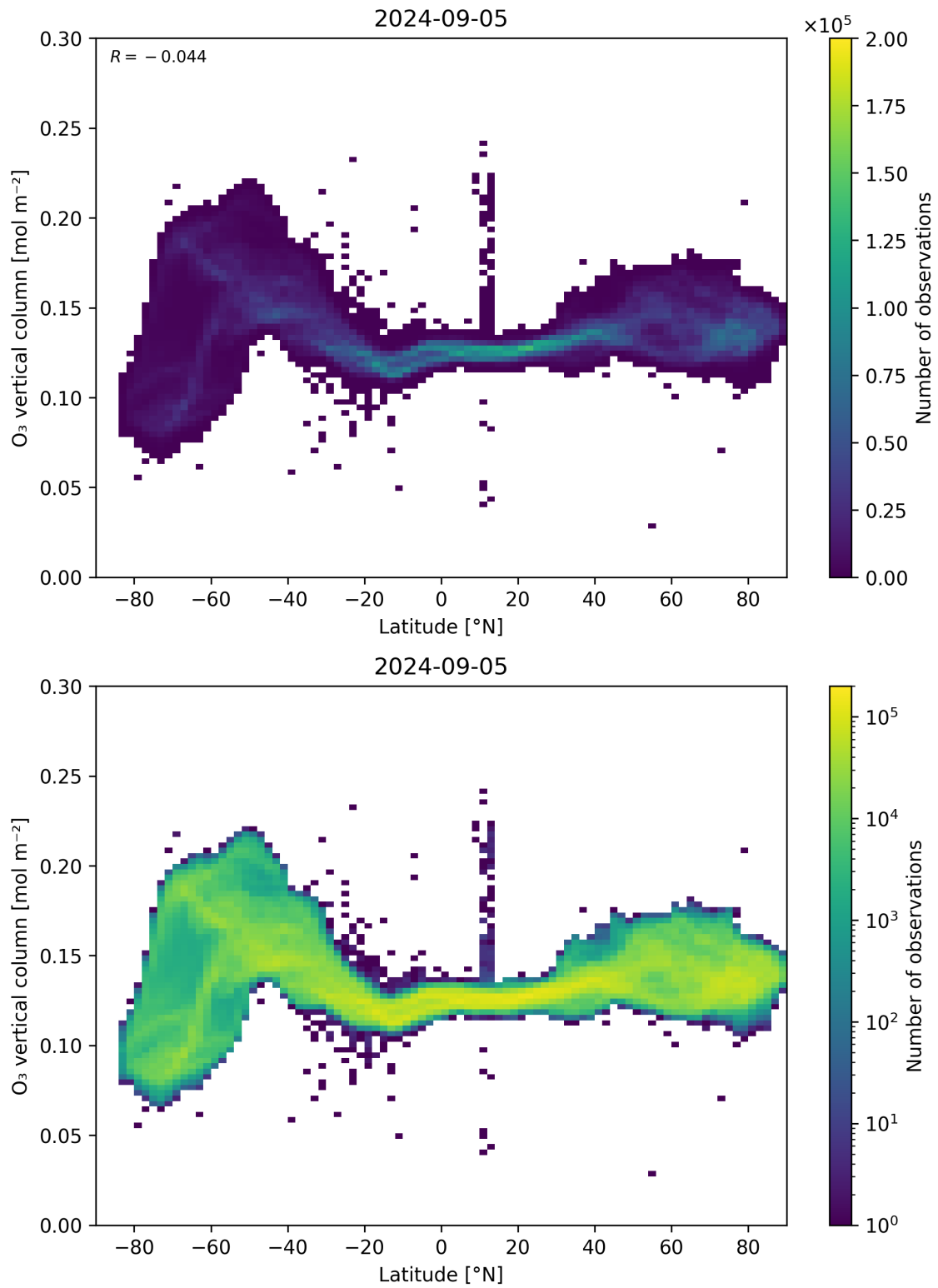
Figure 36: Scatter density plot of “Latitude” against “O 3 vertical column” for 2024-09-04 to 2024-09-06.
