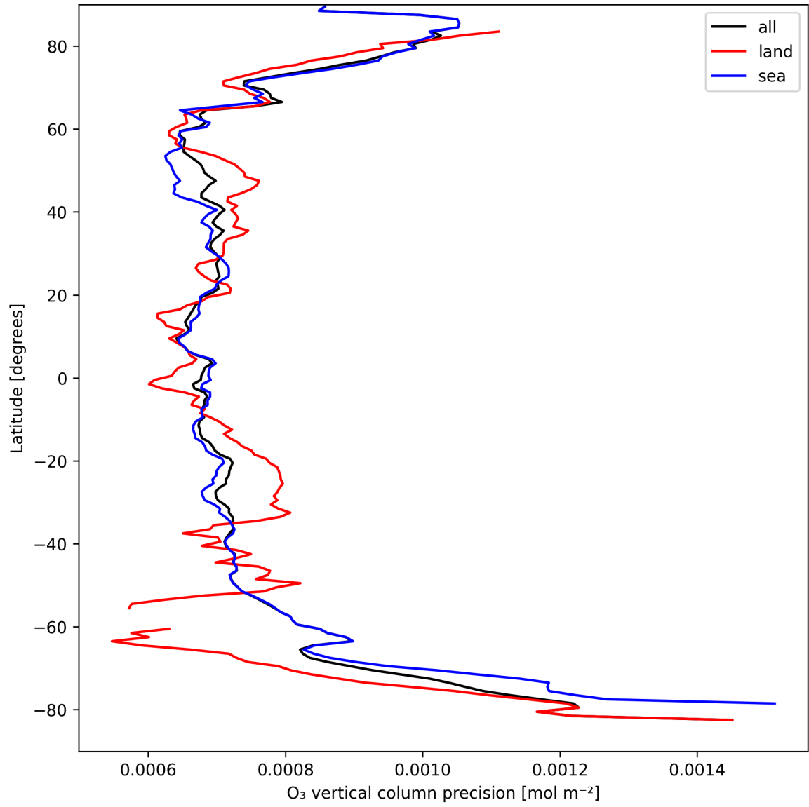
Figure 15: Zonal average of “O 3 vertical column precision” for 2024-09-04 to 2024-09-06.
