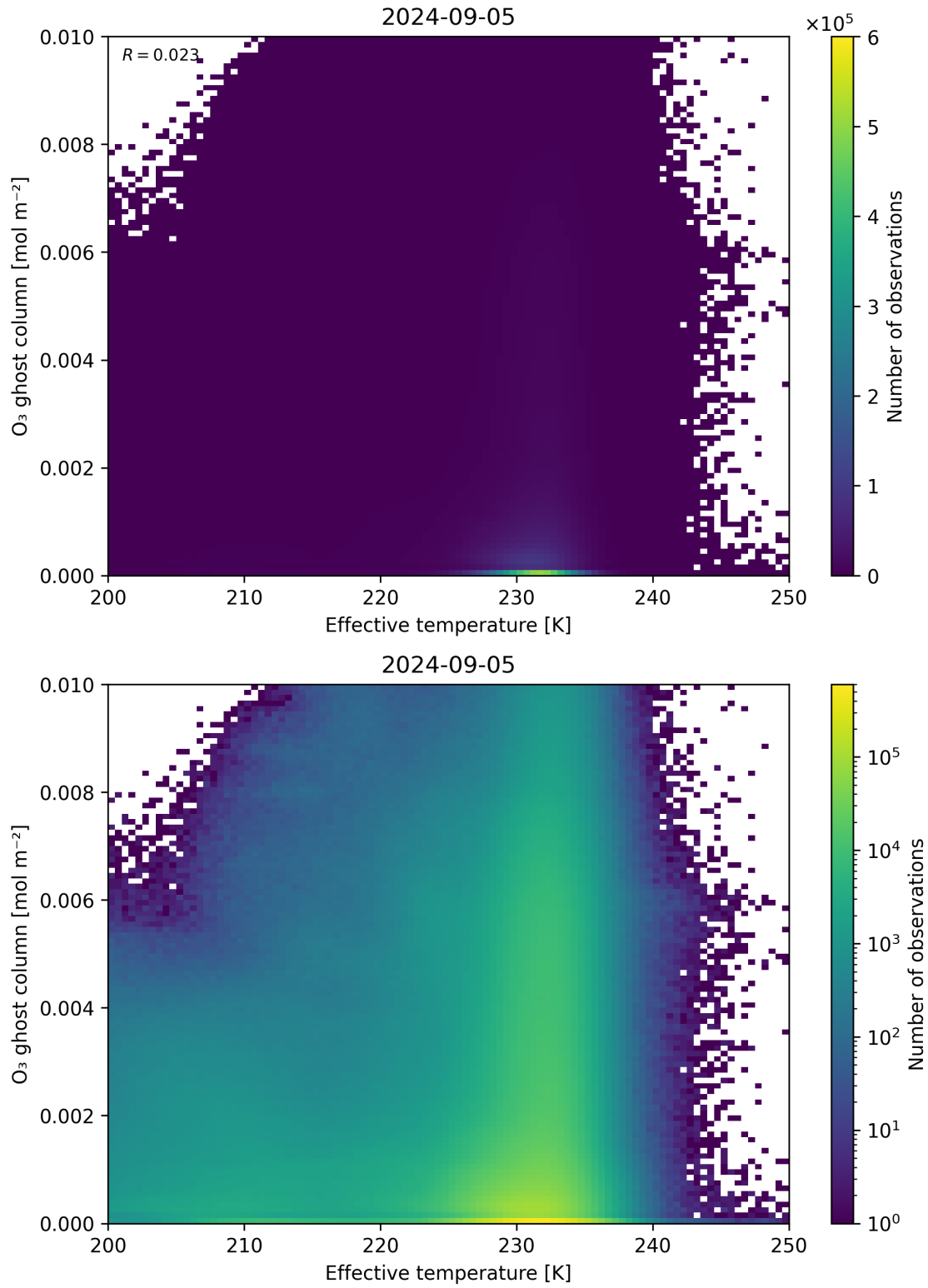
Figure 38: Scatter density plot of “Effective temperature” against “O 3 ghost column” for 2024-09-04 to 2024-09-06.
