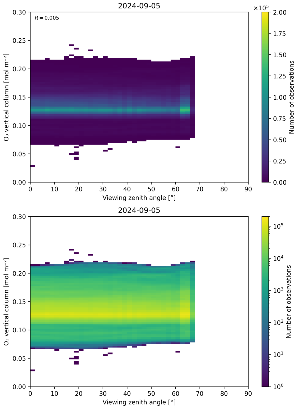
Figure 52: Scatter density plot of “Viewing zenith angle” against “O 3 vertical column” for 2024-09-04 to 2024-09-06.
