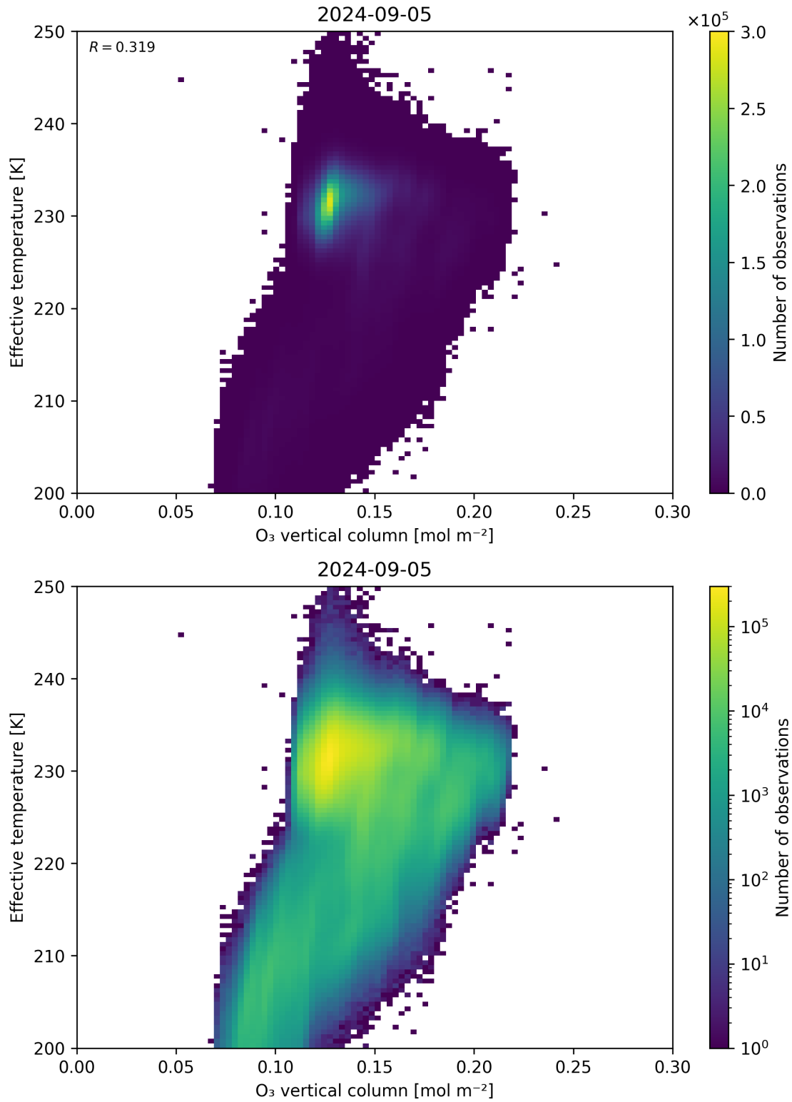
Figure 39: Scatter density plot of “O 3 vertical column” against “Effective temperature” for 2024-09-04 to 2024-09-06.
