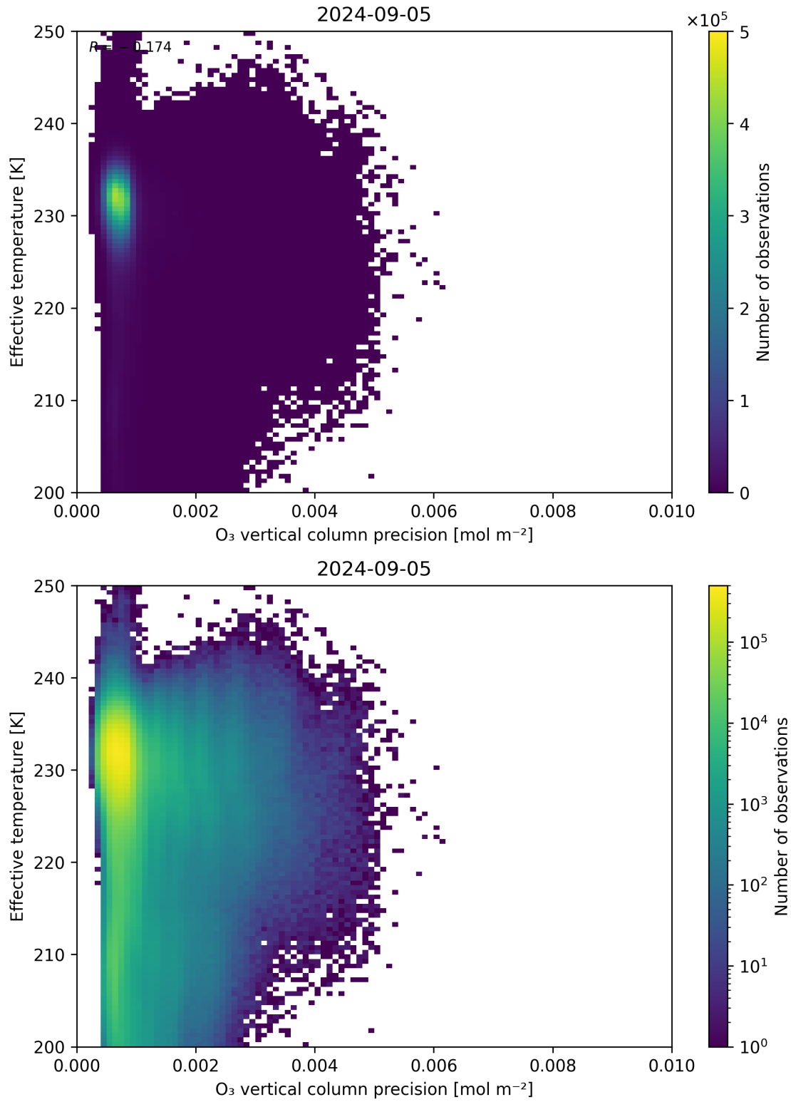
Figure 42: Scatter density plot of “O 3 vertical column precision” against “Effective temperature” for 2024-09-04 to 2024-09-06.
