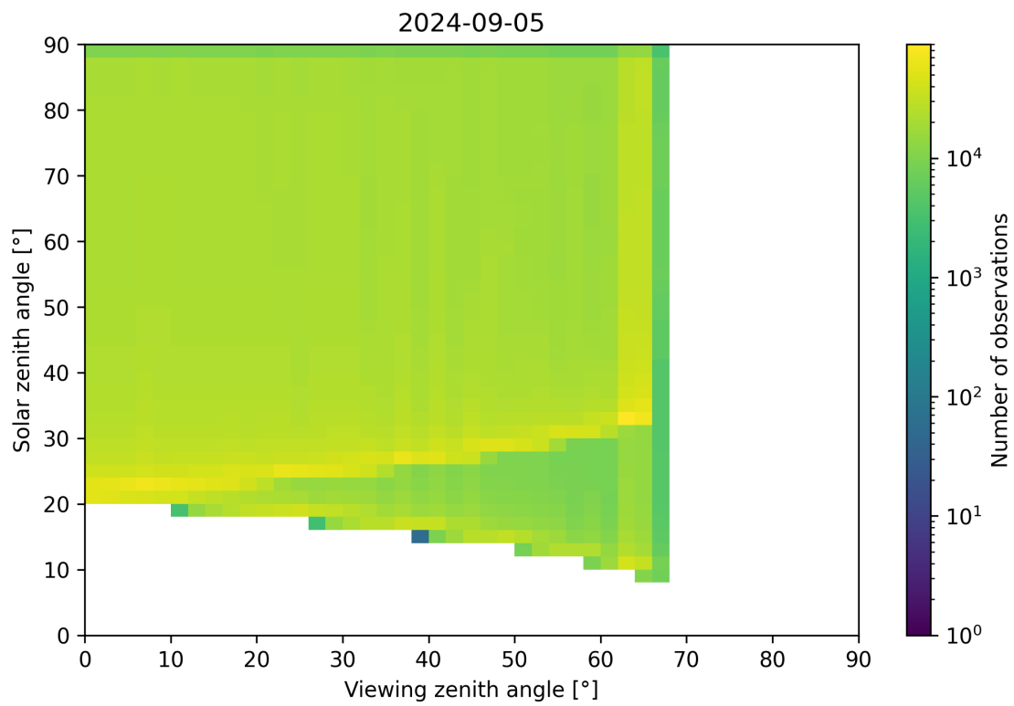
Figure 54: Scatter density plot of “Viewing zenith angle” against “Solar zenith angle” for 2024-09-04 to 2024-09-06.
