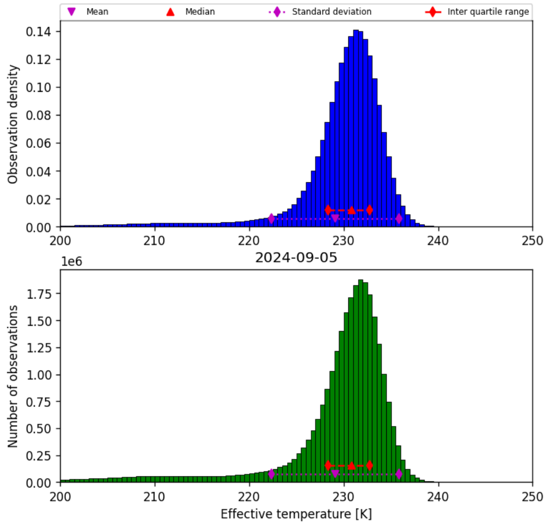
Figure 24: Histogram of “Effective temperature” for 2024-09-04 to 2024-09-06
