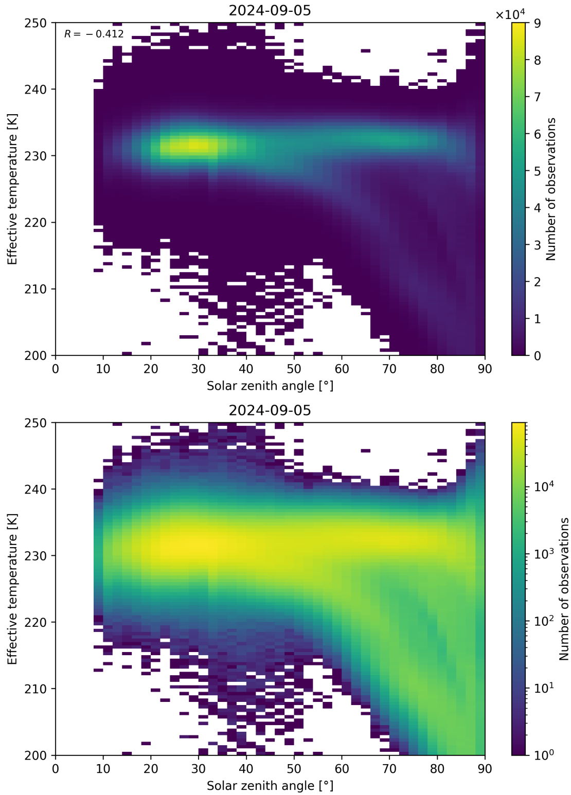
Figure 45: Scatter density plot of “Solar zenith angle” against “Effective temperature” for 2024-09-04 to 2024-09-06.
