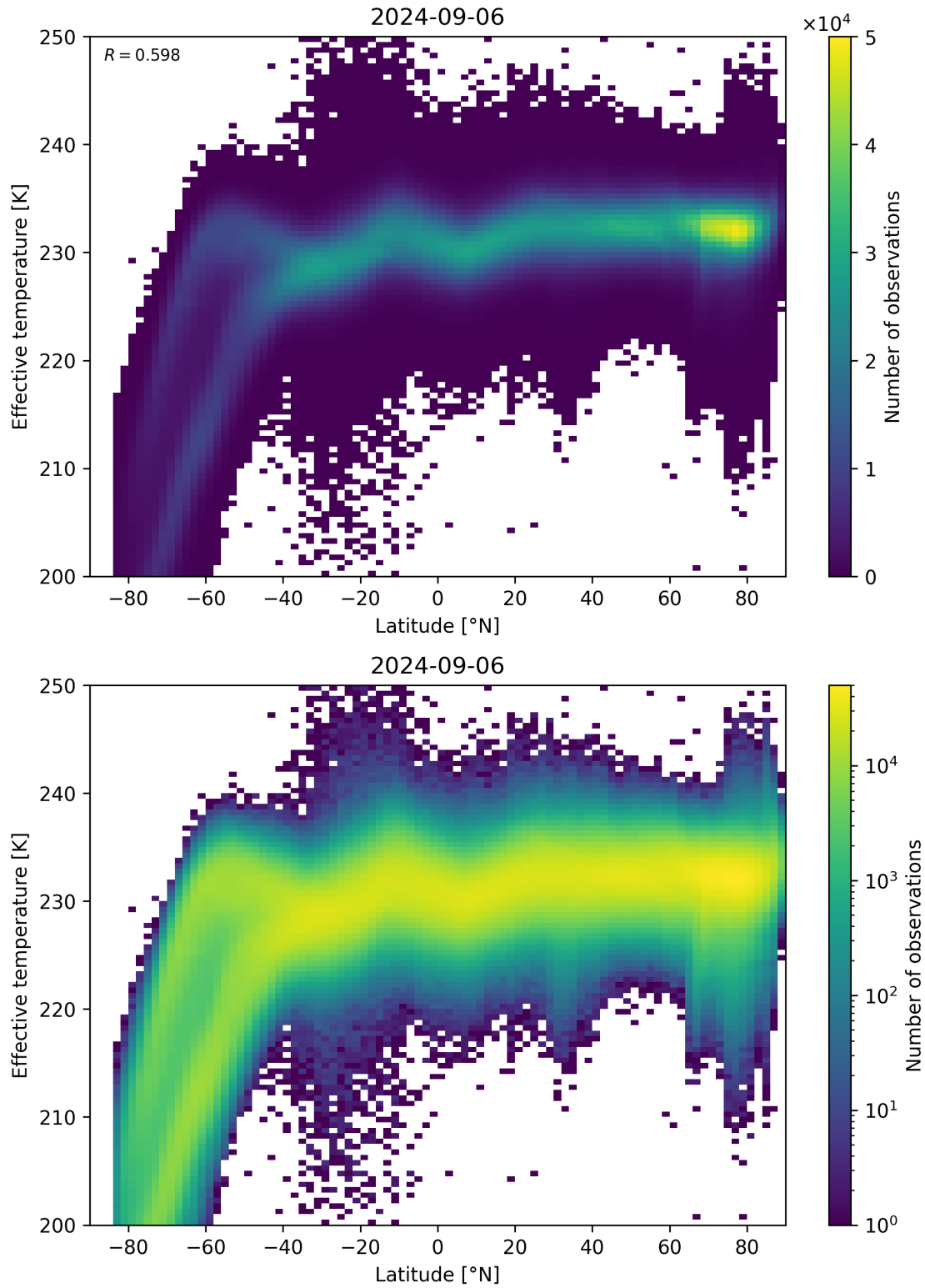
Figure 34: Scatter density plot of “Latitude” against “Effective temperature” for 2024-09-06 to 2024-09-07.
