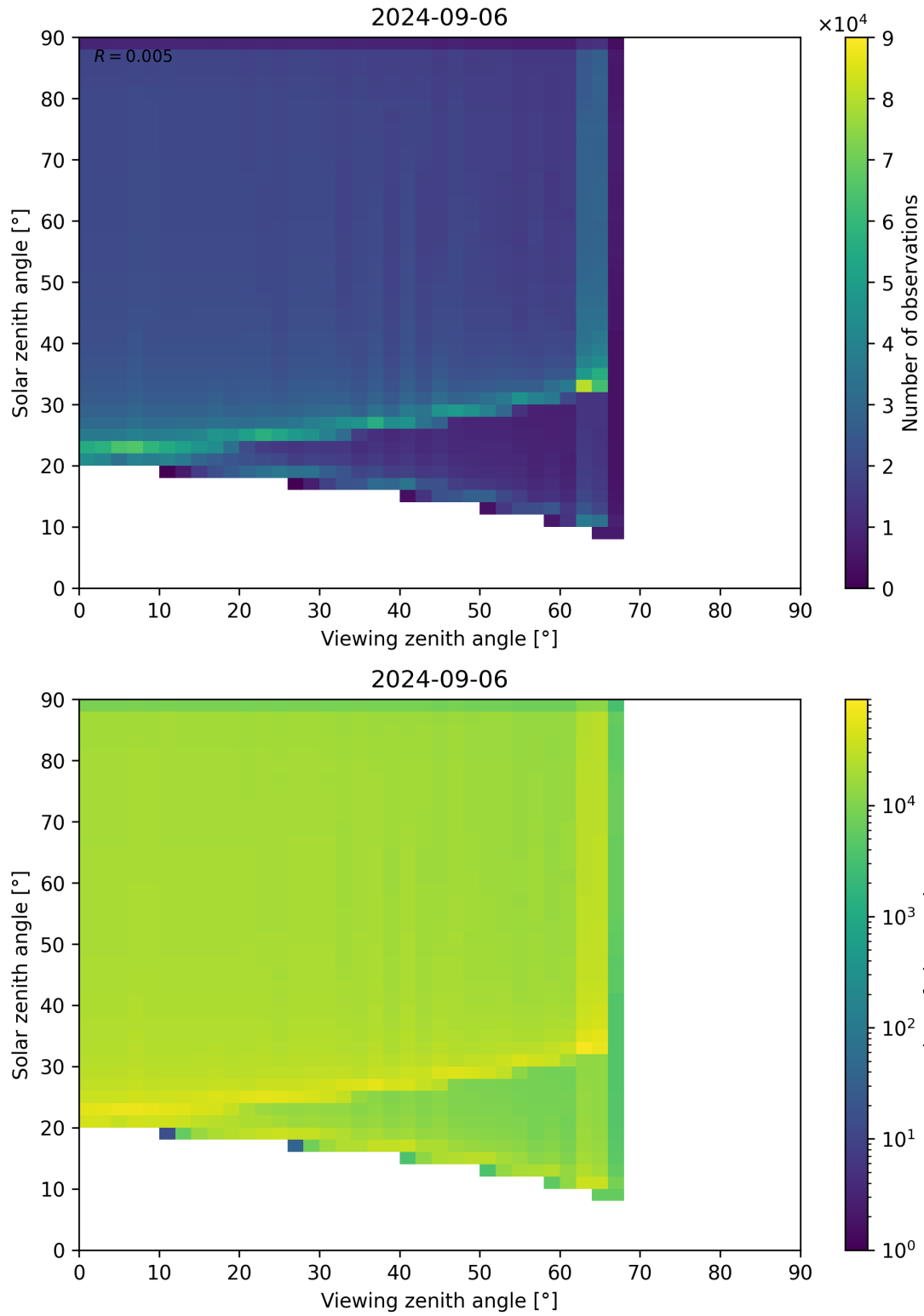
Figure 54: Scatter density plot of “Viewing zenith angle” against “Solar zenith angle” for 2024-09-06 to 2024-09-07.
