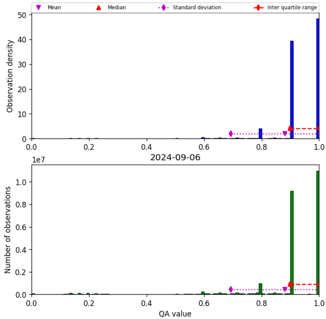
Figure 20: Histogram of “QA value” for 2024-09-06 to 2024-09-07
