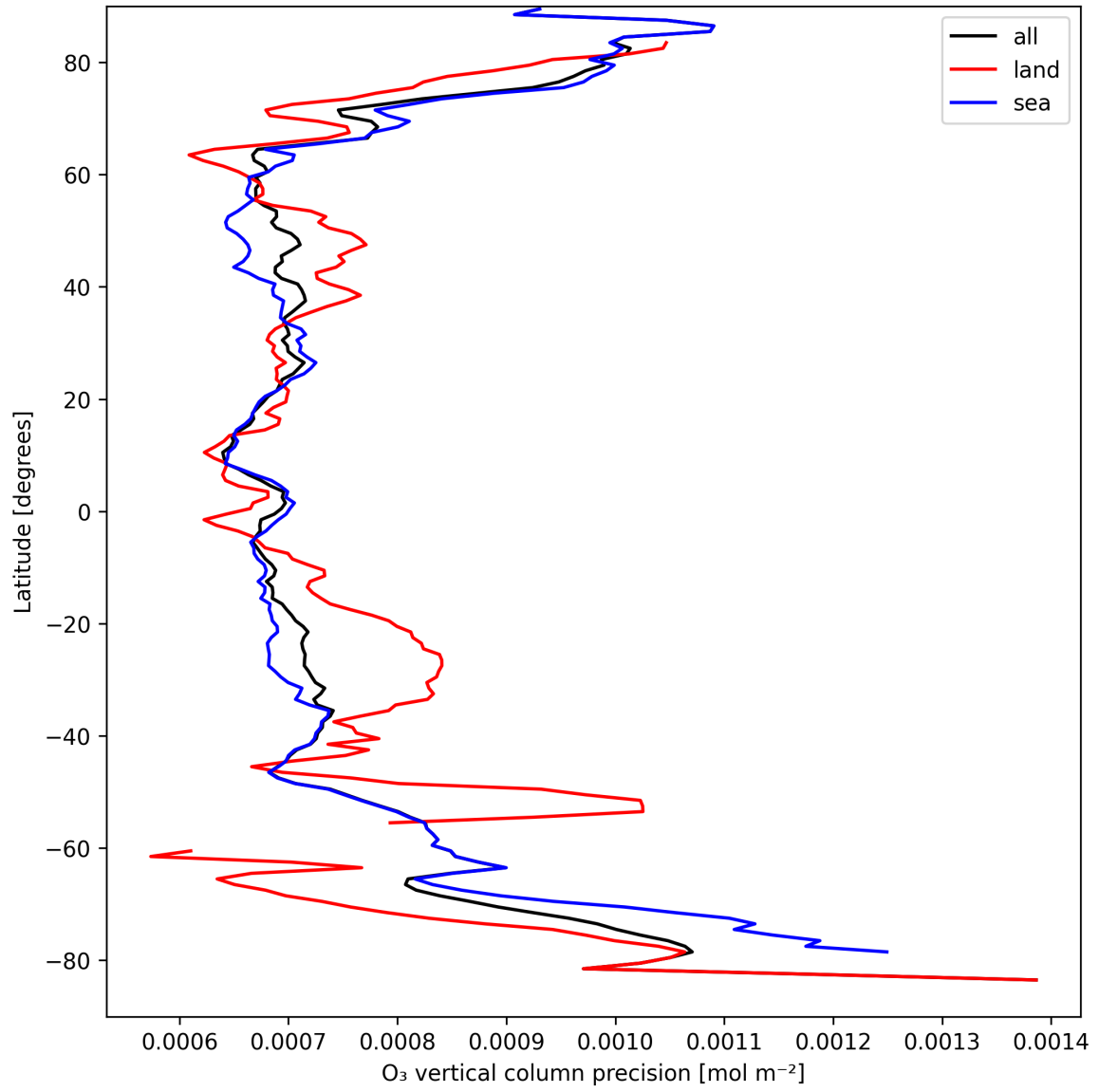
Figure 15: Zonal average of “O 3 vertical column precision” for 2024-09-06 to 2024-09-07.
