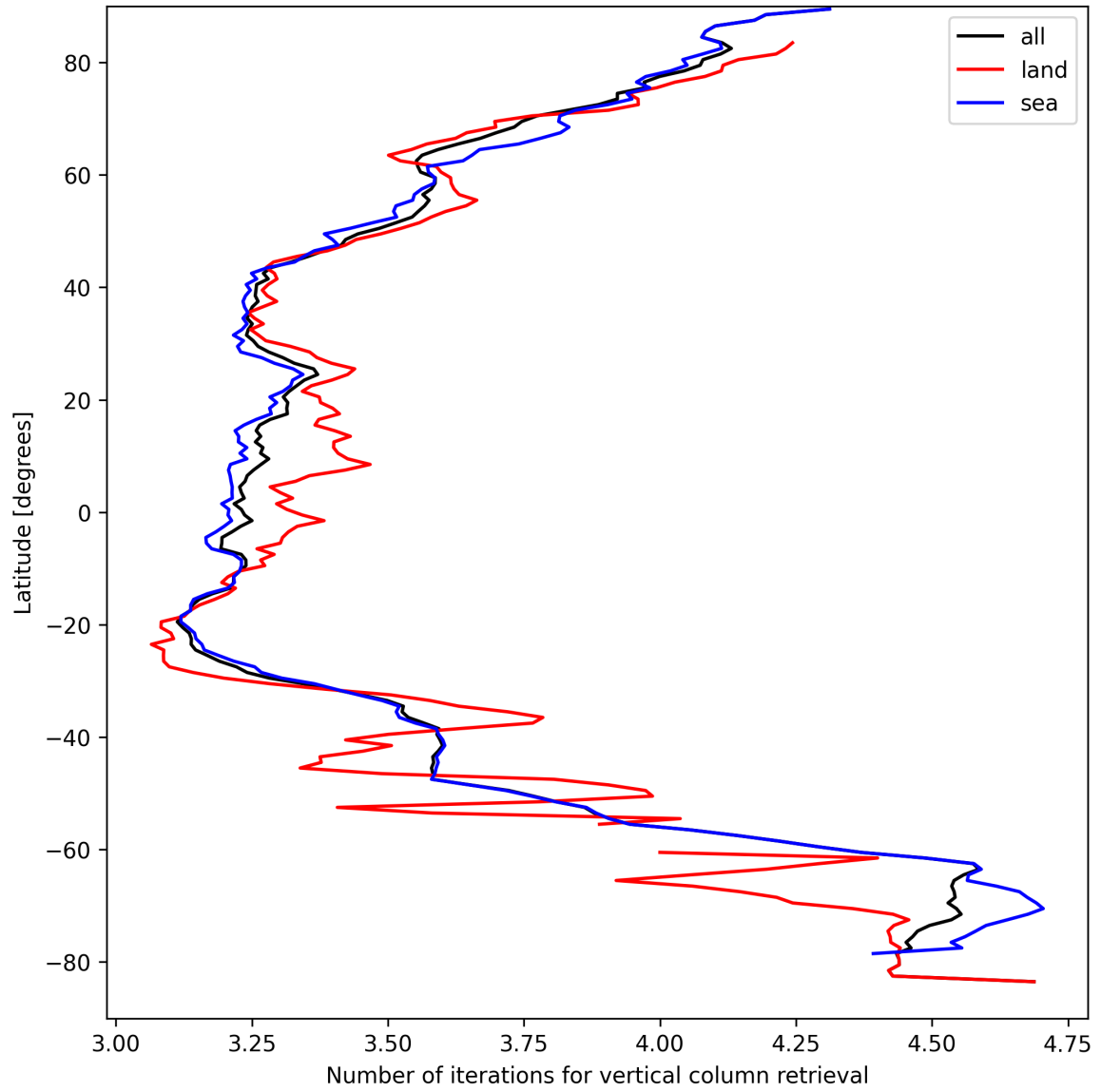
Figure 19: Zonal average of “Number of iterations for vertical column retrieval” for 2024-09-06 to 2024-09-07.
