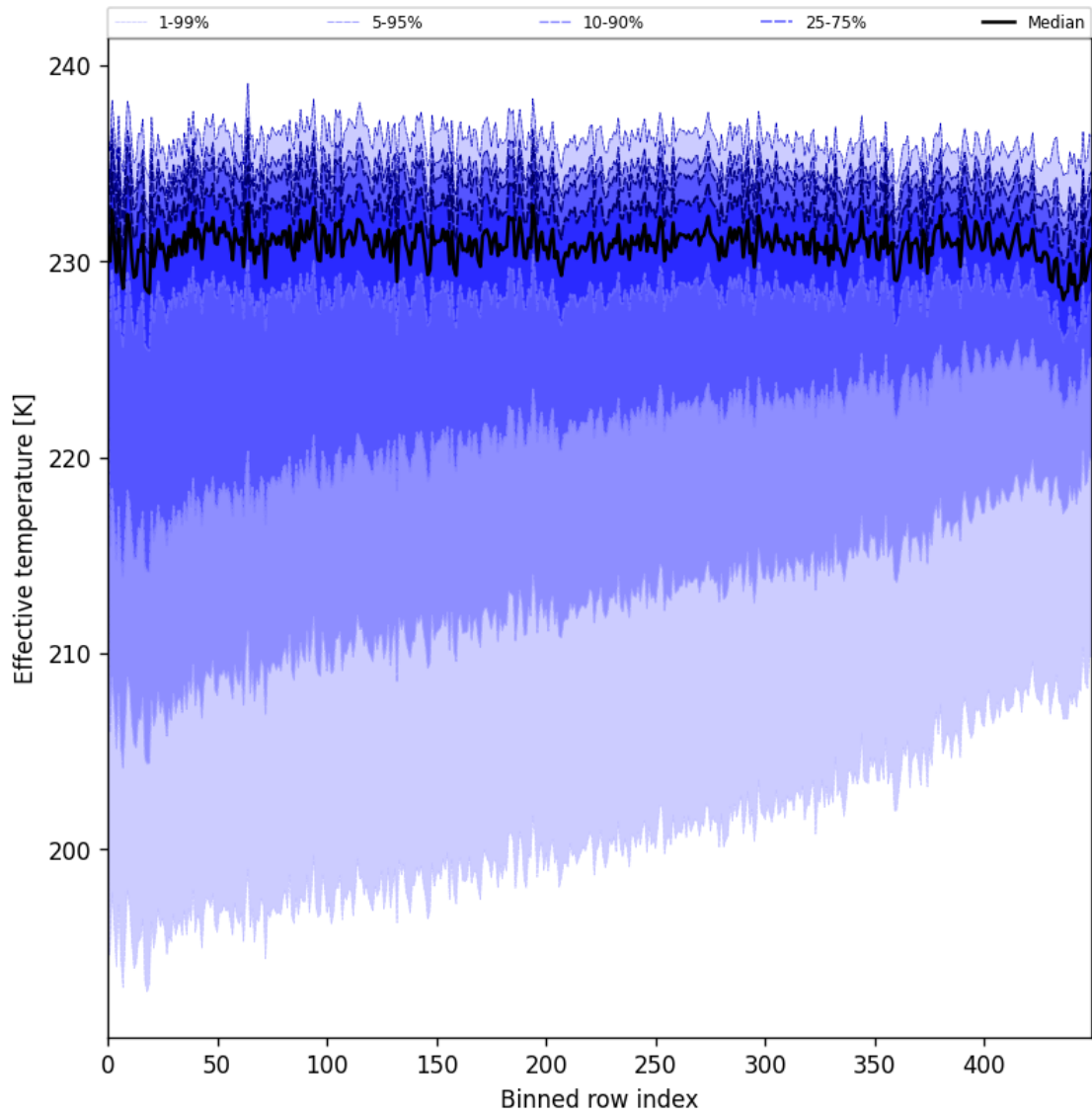
Figure 31: Along track statistics of “Effective temperature” for 2024-09-06 to 2024-09-07
