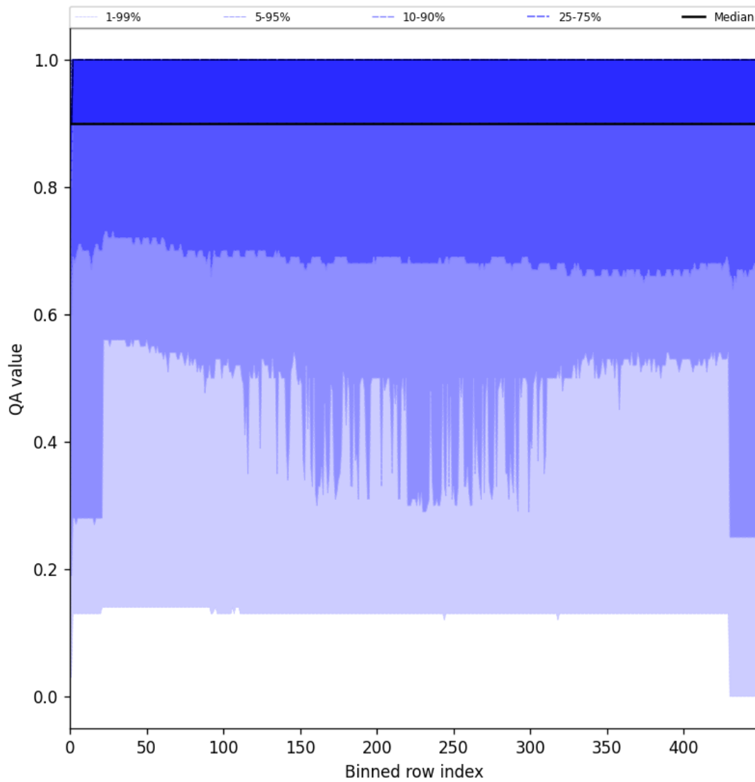
Figure 27: Along track statistics of “QA value” for 2024-09-06 to 2024-09-07
