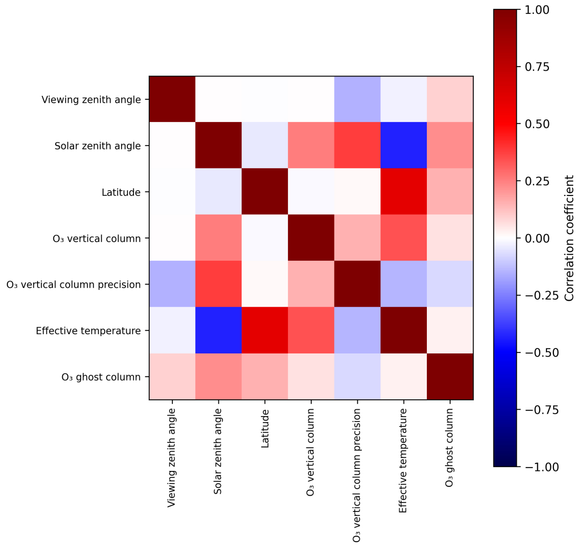
Figure 2: Map of correlation matrix for 2024-09-06 to 2024-09-07.
