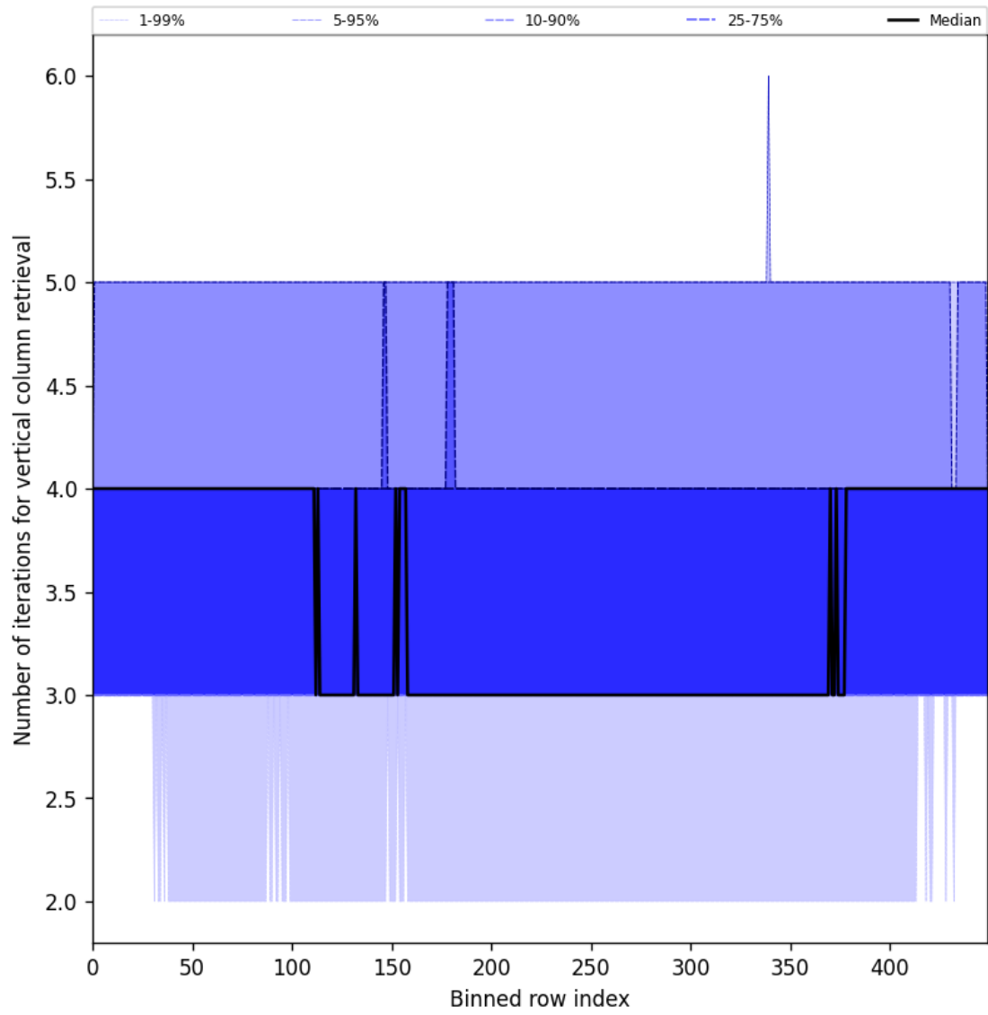
Figure 33: Along track statistics of “Number of iterations for vertical column retrieval” for 2024-09-06 to 2024-09-07
