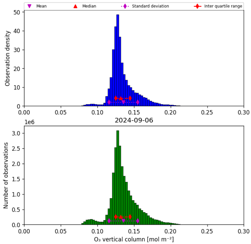
Figure 21: Histogram of “O 3 vertical column” for 2024-09-06 to 2024-09-07
