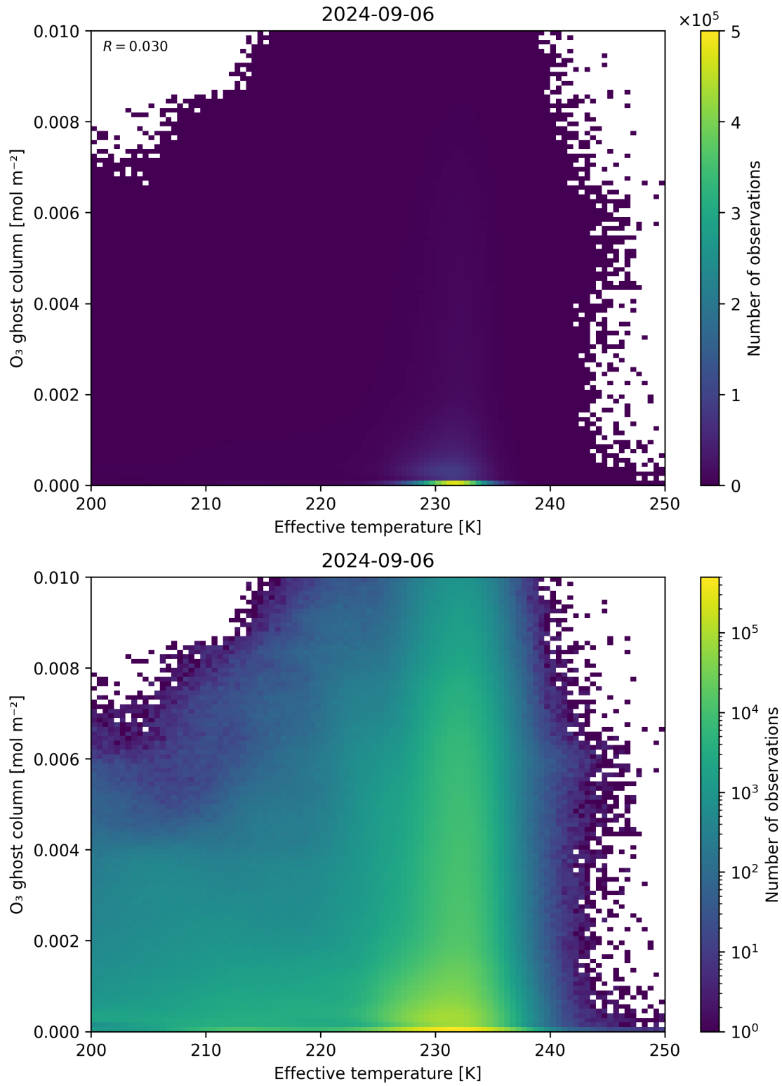
Figure 38: Scatter density plot of “Effective temperature” against “O 3 ghost column” for 2024-09-06 to 2024-09-07.
