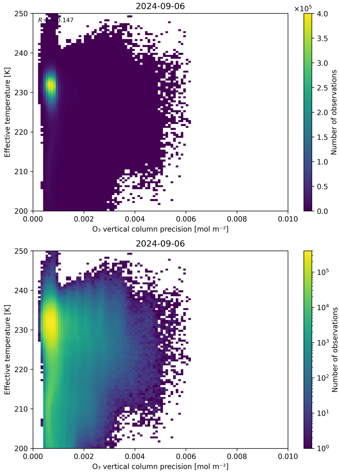
Figure 42: Scatter density plot of “O 3 vertical column precision” against “Effective temperature” for 2024-09-06 to 2024-09-07.
