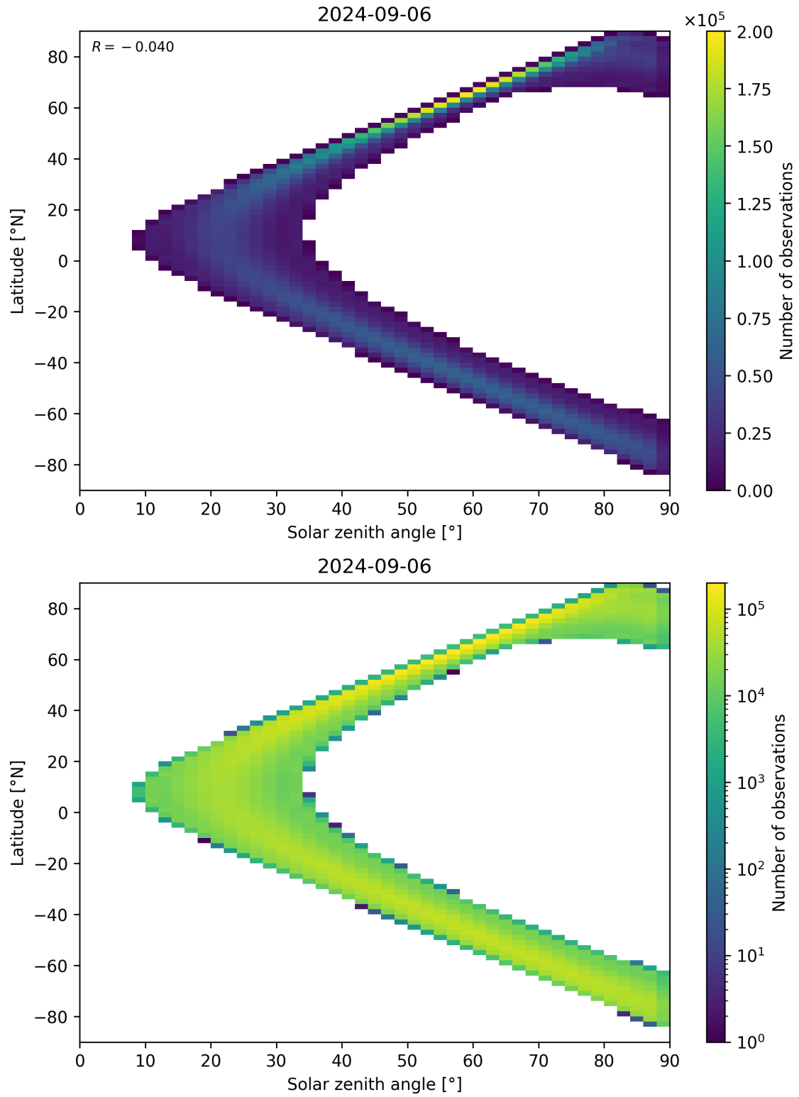
Figure 44: Scatter density plot of “Solar zenith angle” against “Latitude” for 2024-09-06 to 2024-09-07.
