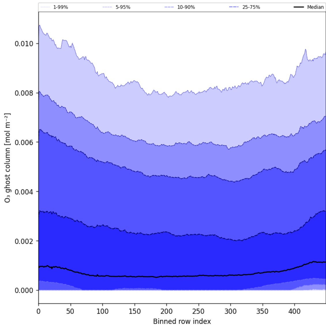
Figure 32: Along track statistics of “O 3 ghost column” for 2024-09-06 to 2024-09-07
