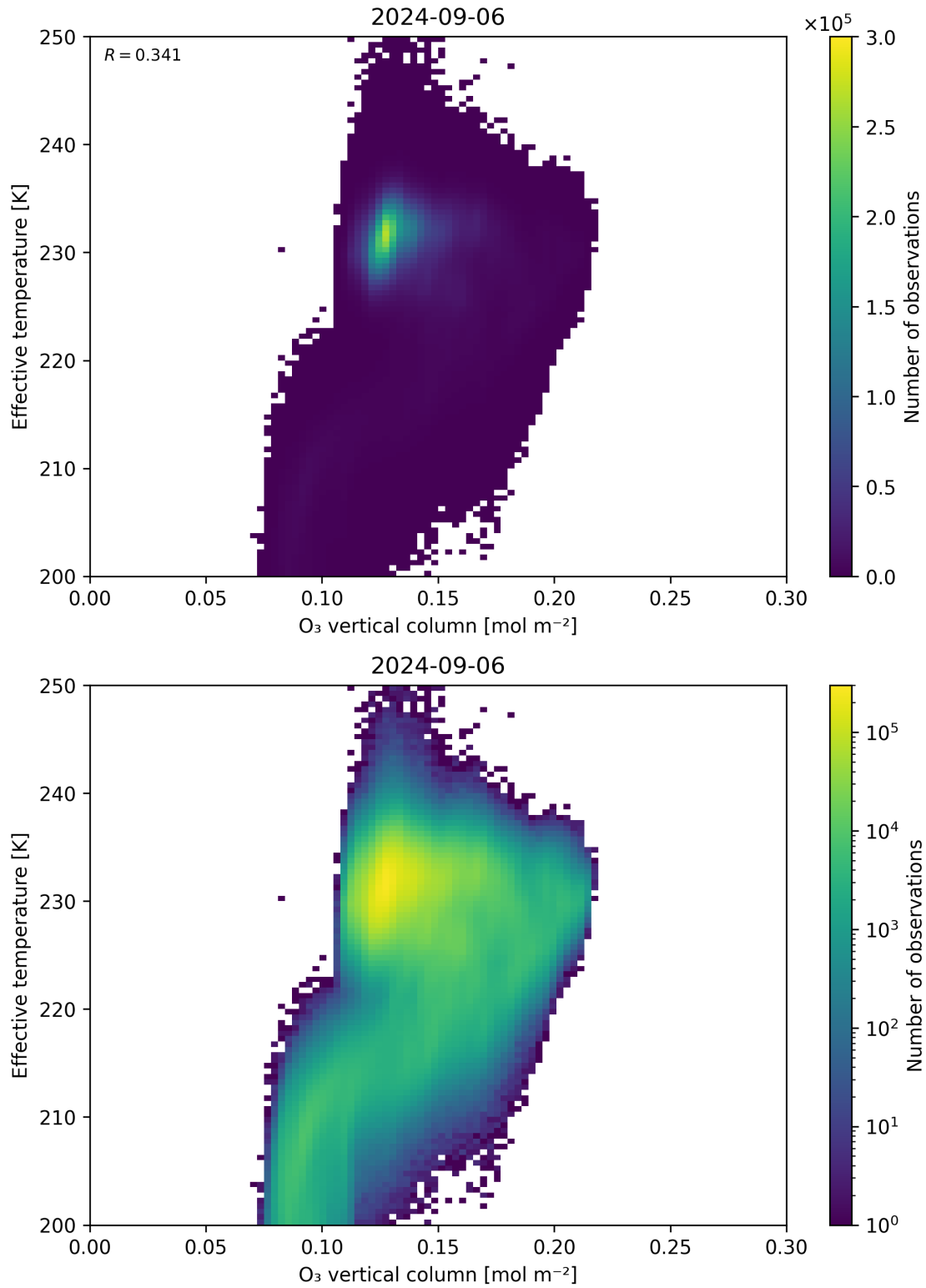
Figure 39: Scatter density plot of “O 3 vertical column” against “Effective temperature” for 2024-09-06 to 2024-09-07.
