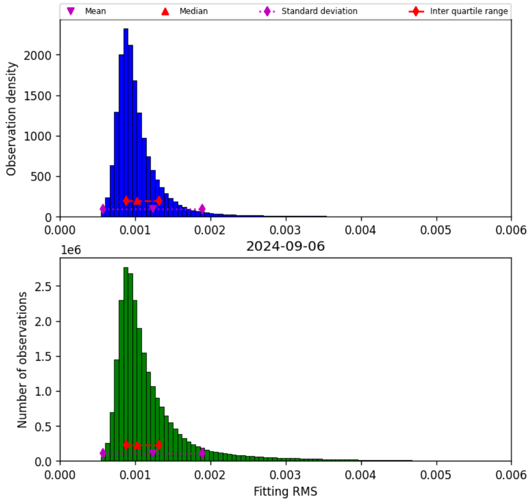
Figure 23: Histogram of “Fitting RMS” for 2024-09-06 to 2024-09-07
