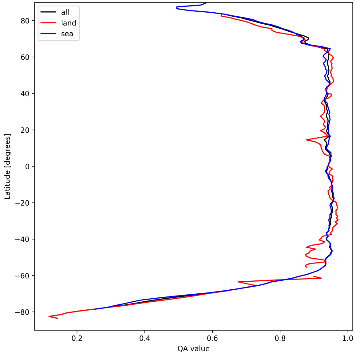
Figure 13: Zonal average of “QA value” for 2024-09-06 to 2024-09-07.
