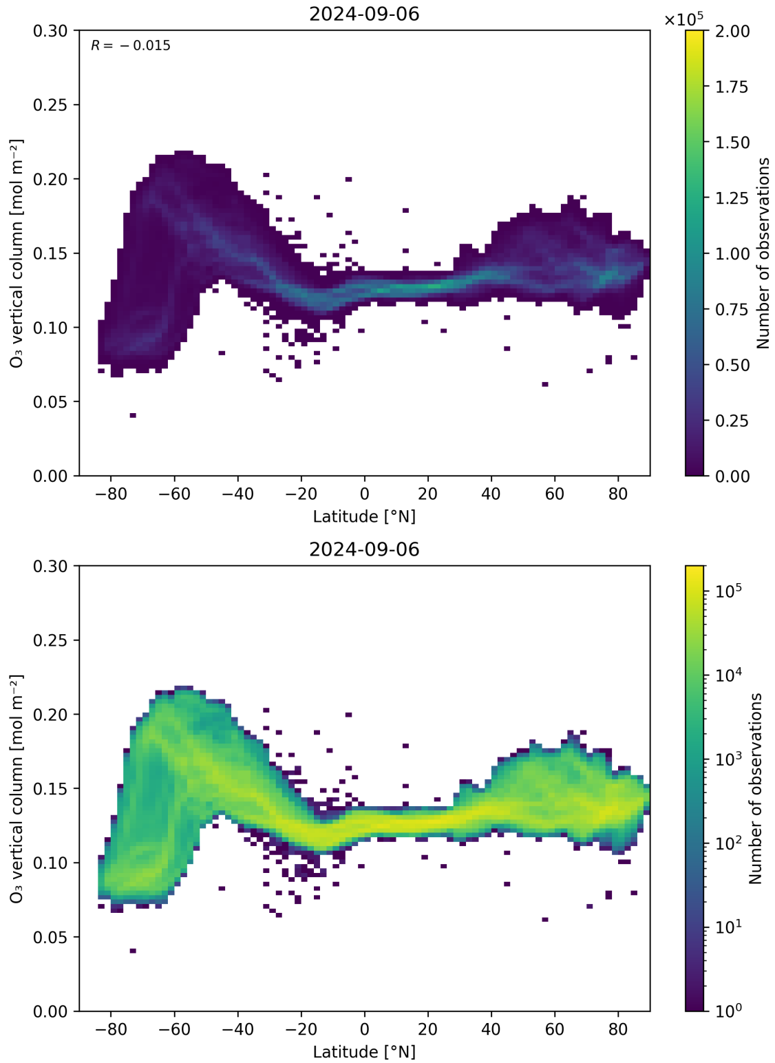
Figure 36: Scatter density plot of “Latitude” against “O 3 vertical column” for 2024-09-06 to 2024-09-07.
