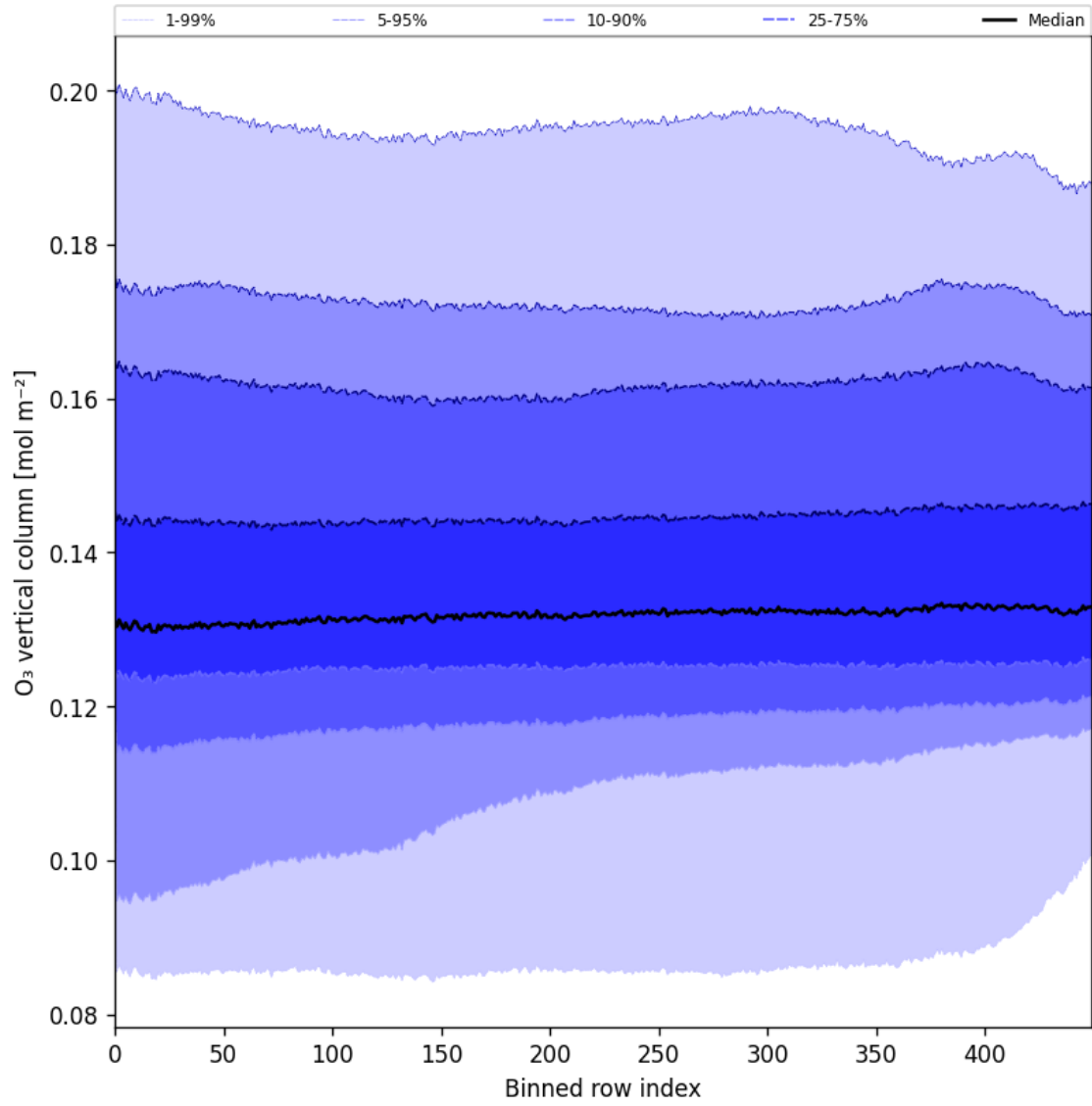
Figure 28: Along track statistics of “O 3 vertical column” for 2024-09-06 to 2024-09-07
