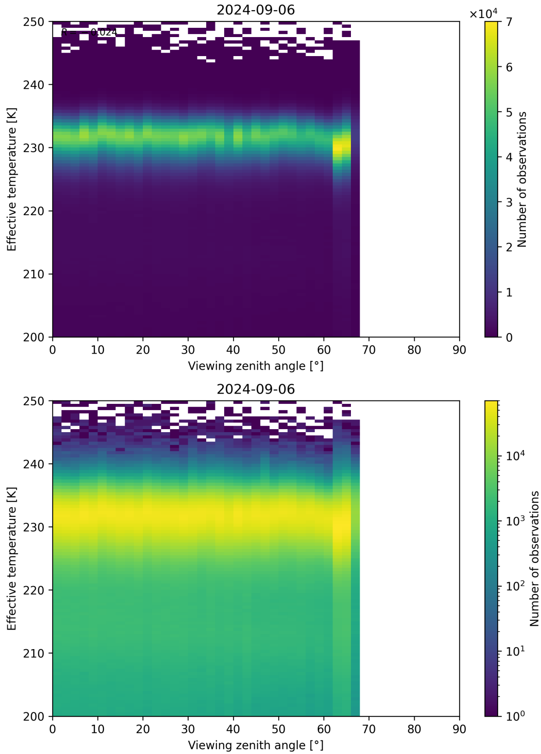
Figure 50: Scatter density plot of “Viewing zenith angle” against “Effective temperature” for 2024-09-06 to 2024-09-07.
