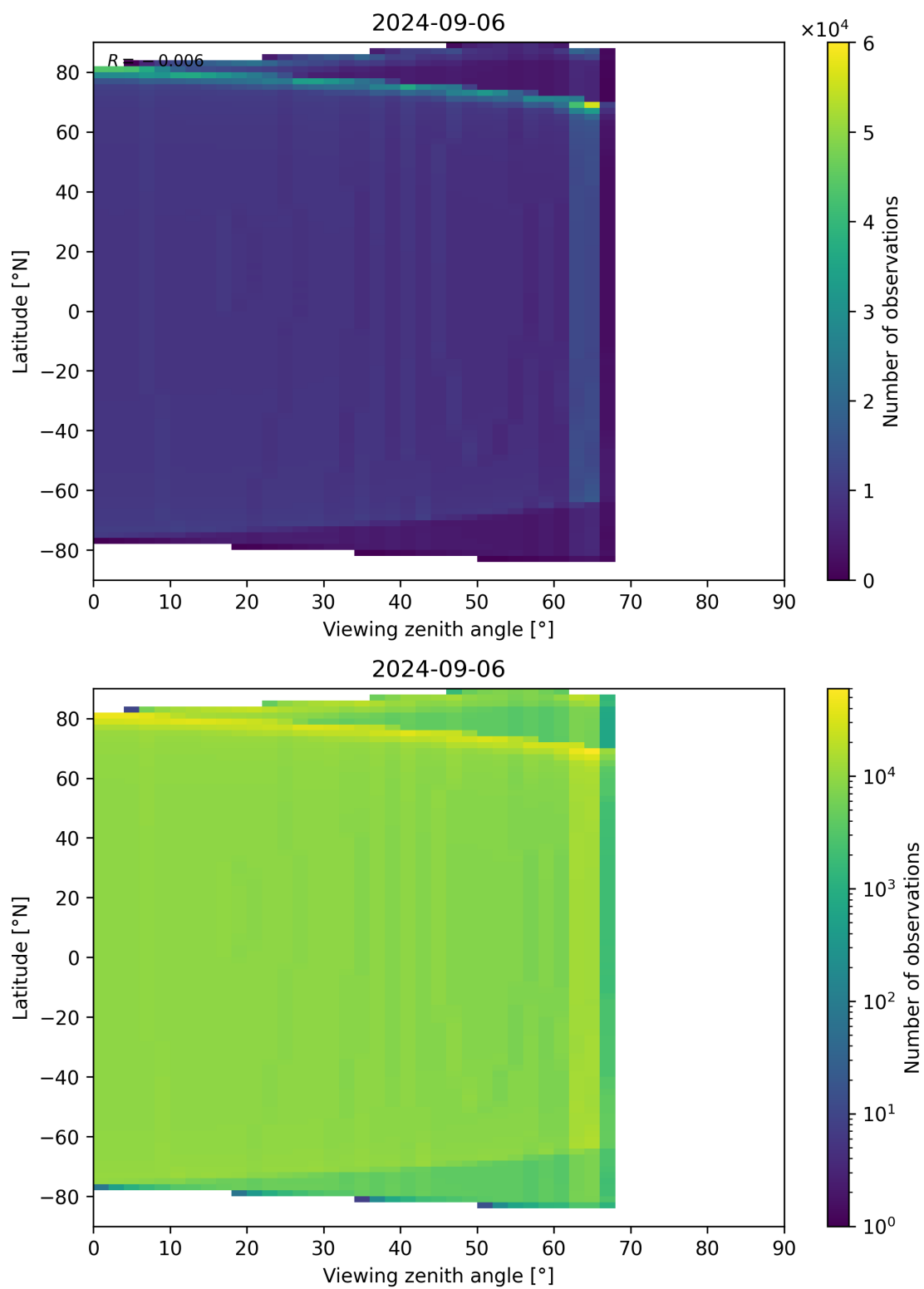
Figure 49: Scatter density plot of “Viewing zenith angle” against “Latitude” for 2024-09-06 to 2024-09-07.
