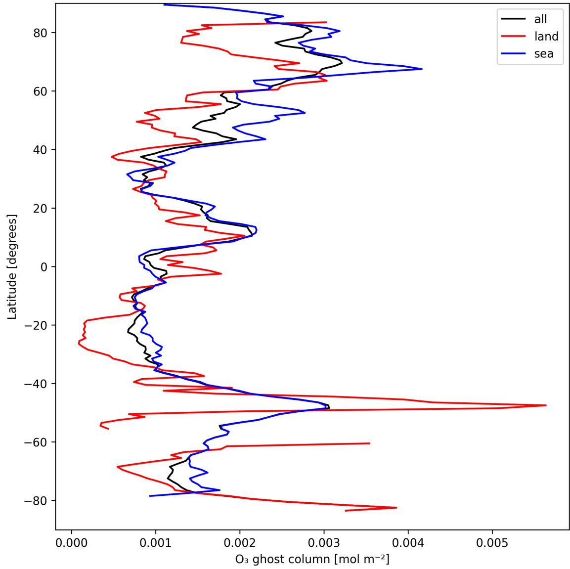
Figure 18: Zonal average of "O 3 ghost column" for 2024-09-06 to 2024-09-07.
