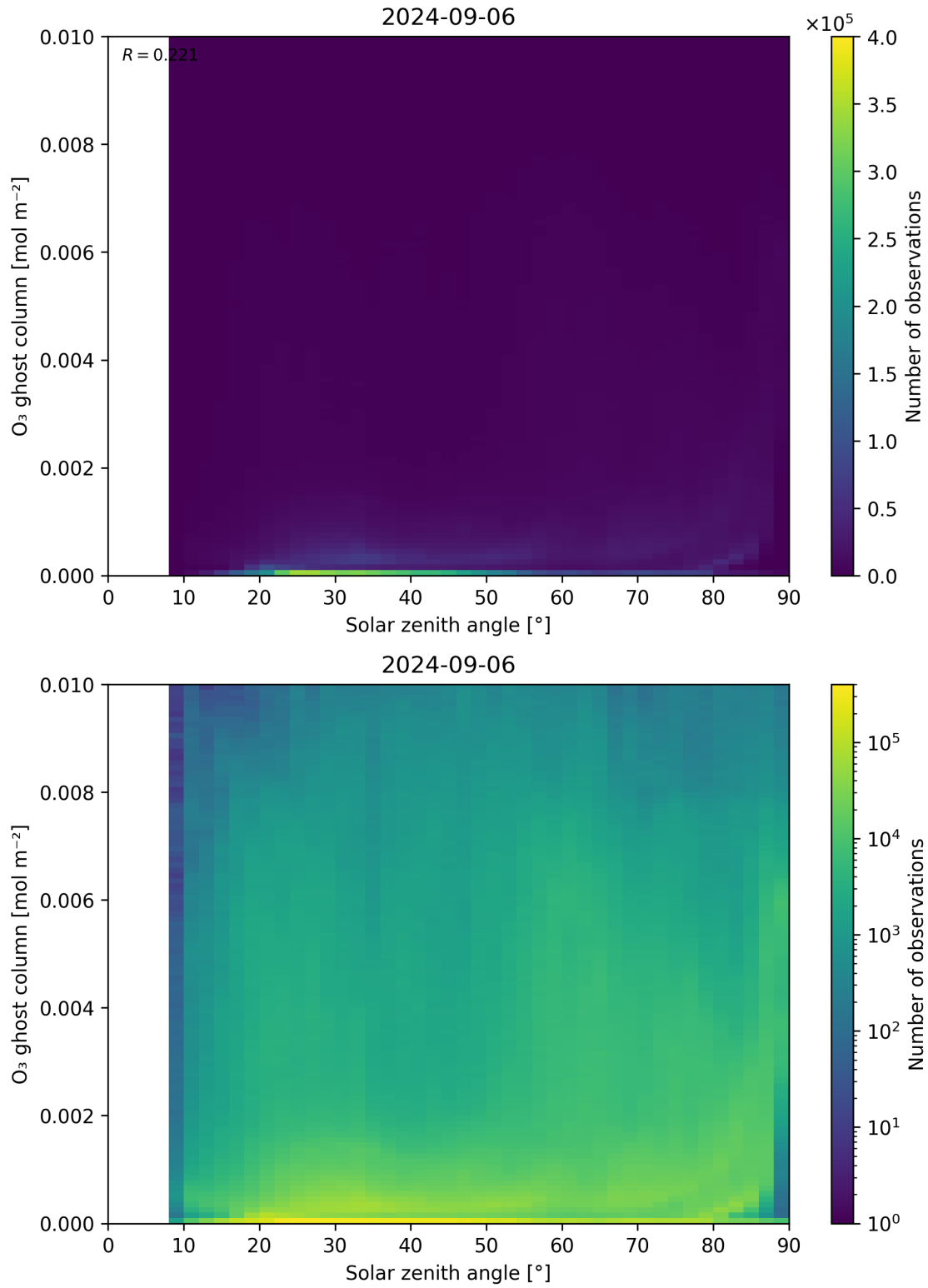
Figure 46: Scatter density plot of “Solar zenith angle” against “O 3 ghost column” for 2024-09-06 to 2024-09-07.
