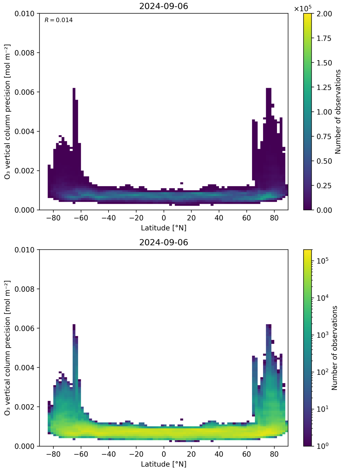
Figure 37: Scatter density plot of “Latitude” against “O 3 vertical column precision” for 2024-09-06 to 2024-09-07.
