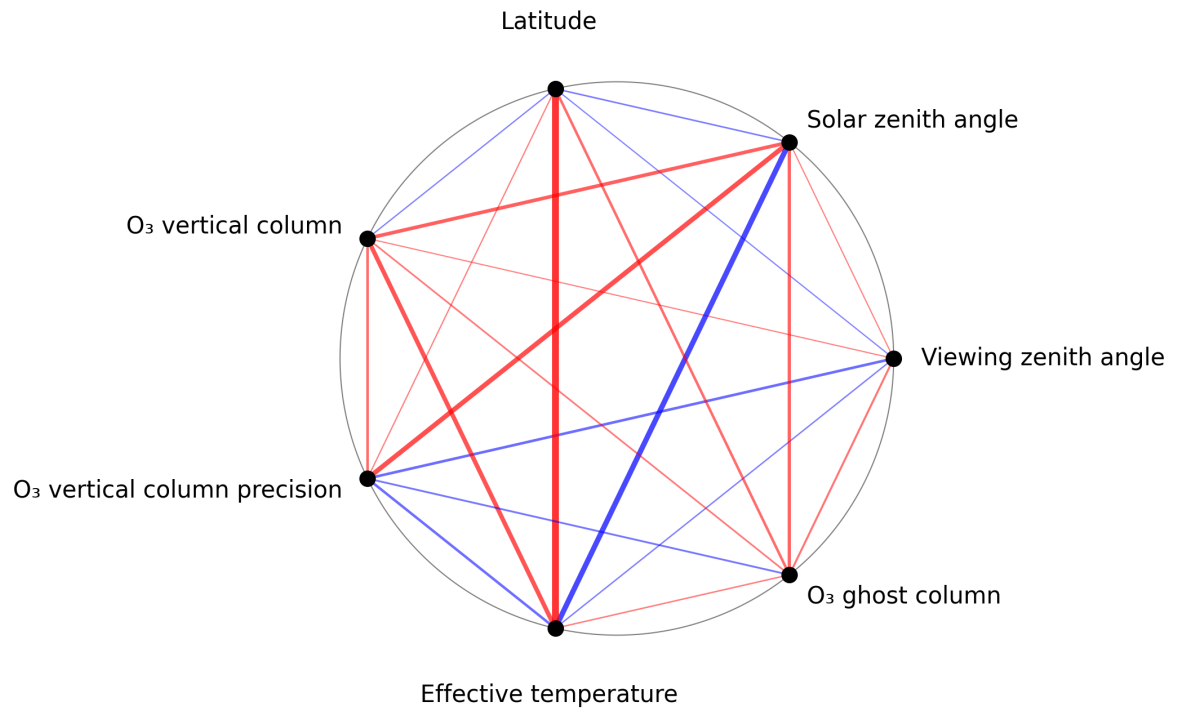
Figure 1: Map of correlation graph for 2024-09-06 to 2024-09-07.
