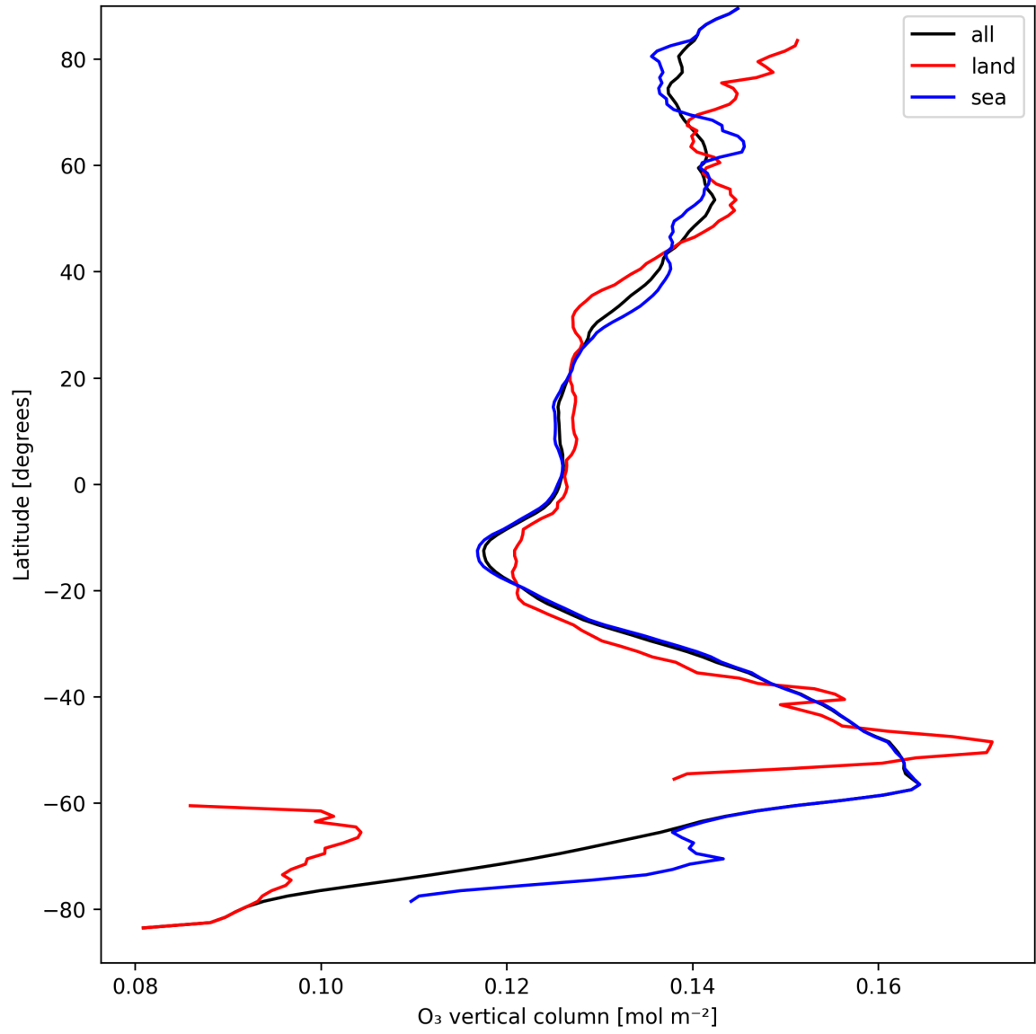
Figure 14: Zonal average of “O 3 vertical column” for 2024-09-06 to 2024-09-07.
