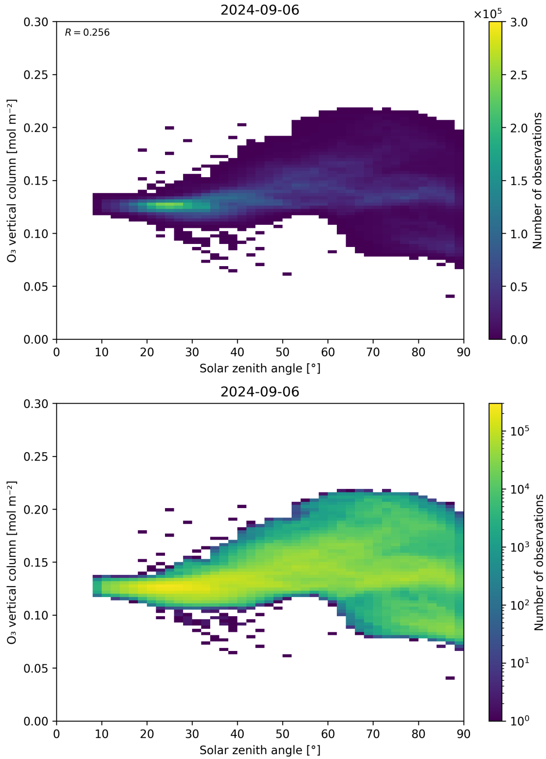
Figure 47: Scatter density plot of “Solar zenith angle” against “O 3 vertical column” for 2024-09-06 to 2024-09-07.
