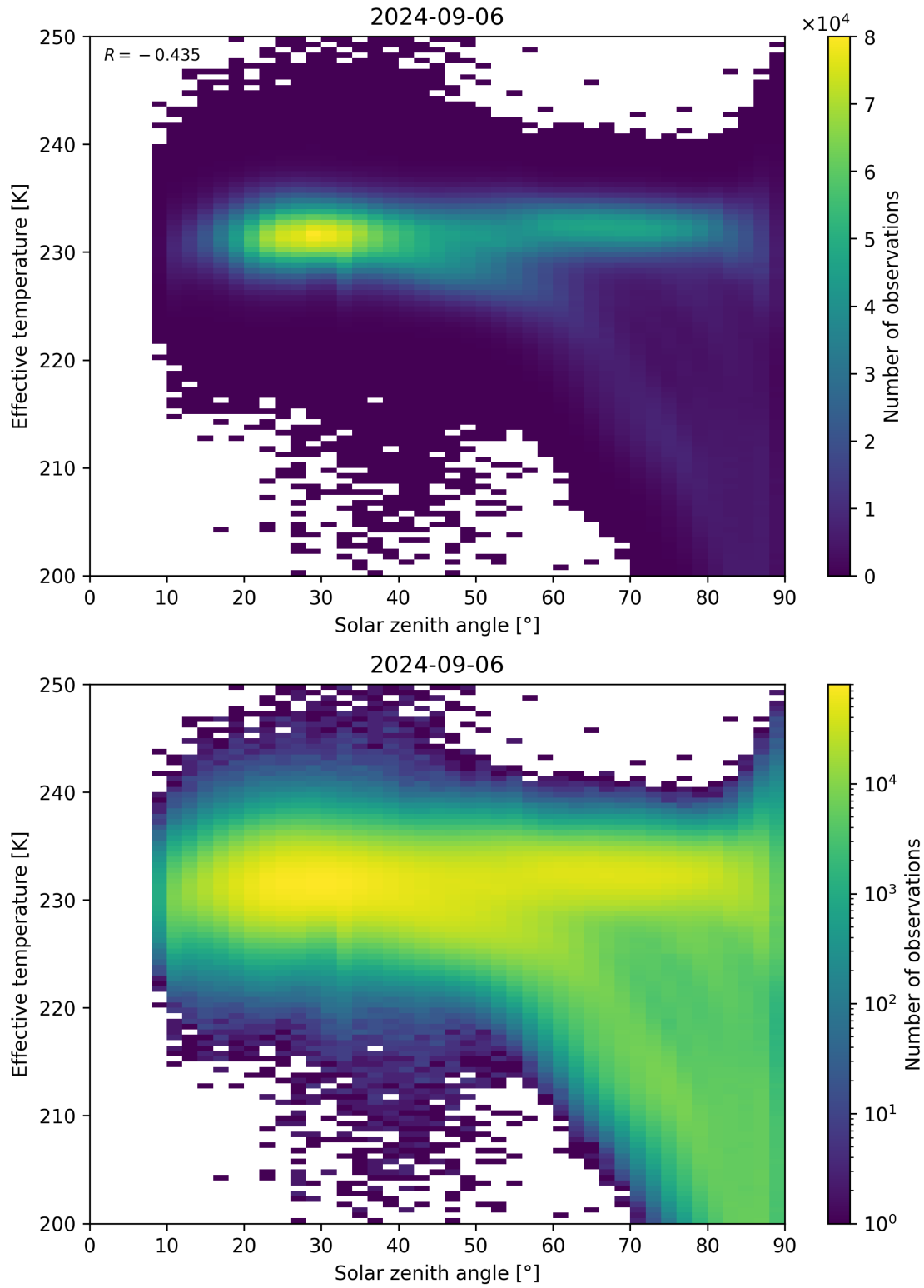
Figure 45: Scatter density plot of “Solar zenith angle” against “Effective temperature” for 2024-09-06 to 2024-09-07.
