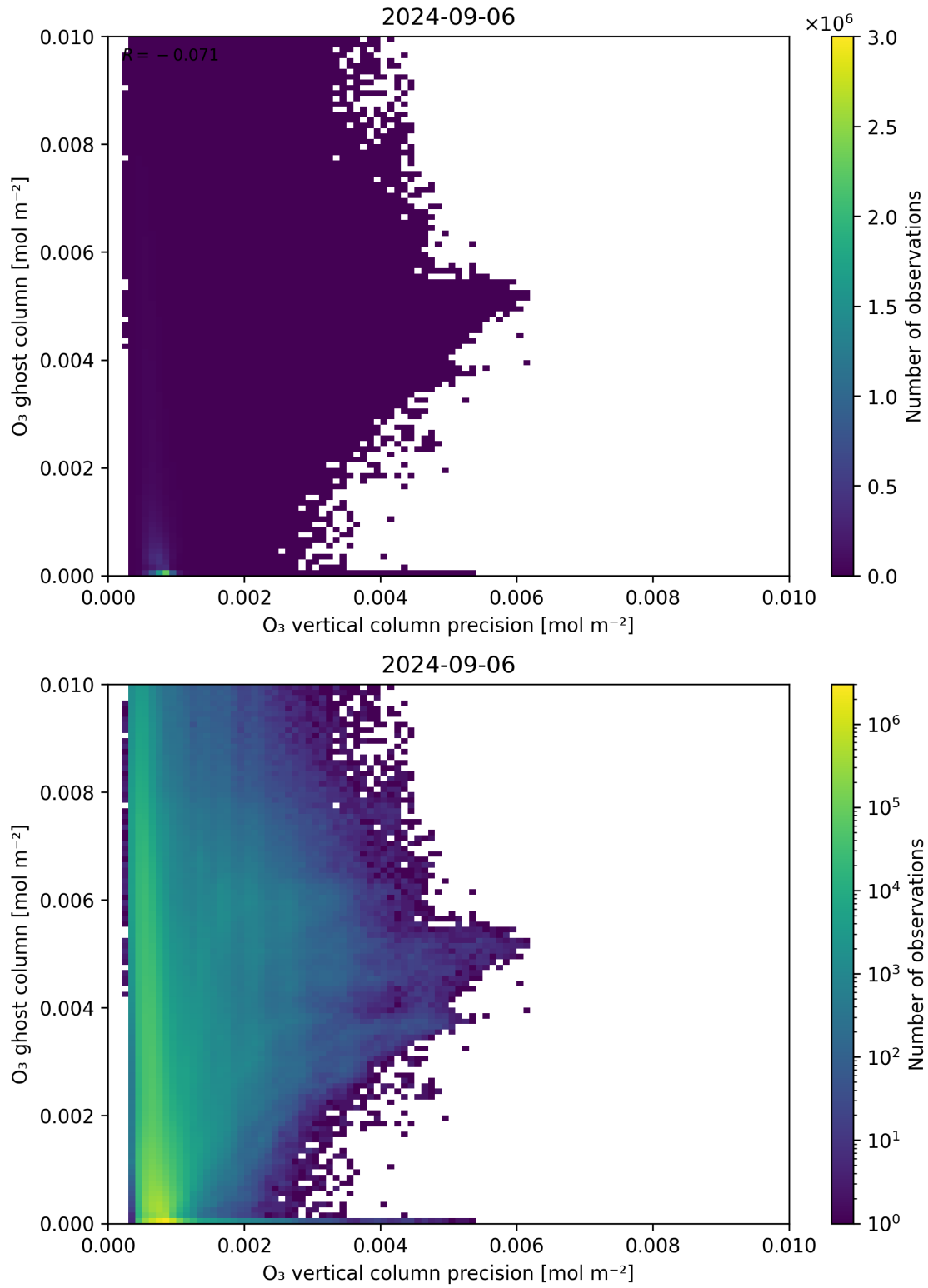
Figure 43: Scatter density plot of “O 3 vertical column precision” against “O 3 ghost column” for 2024-09-06 to 2024-09-07.
