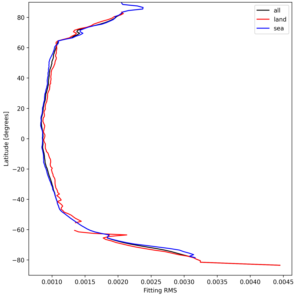
Figure 16: Zonal average of “Fitting RMS” for 2024-09-06 to 2024-09-07.
