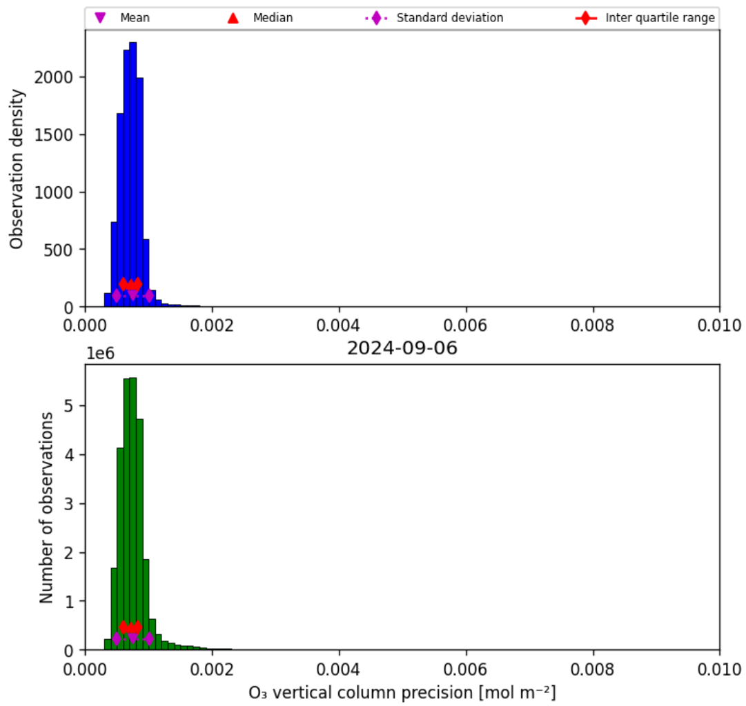
Figure 22: Histogram of “O 3 vertical column precision” for 2024-09-06 to 2024-09-07
