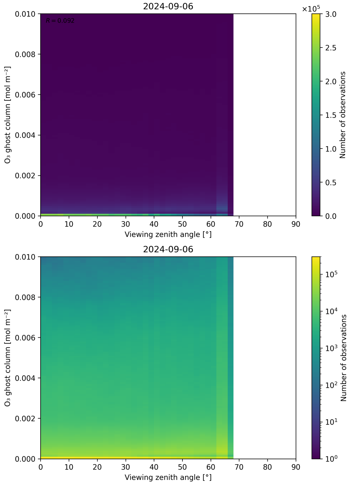
Figure 51: Scatter density plot of “Viewing zenith angle” against “O 3 ghost column” for 2024-09-06 to 2024-09-07.
