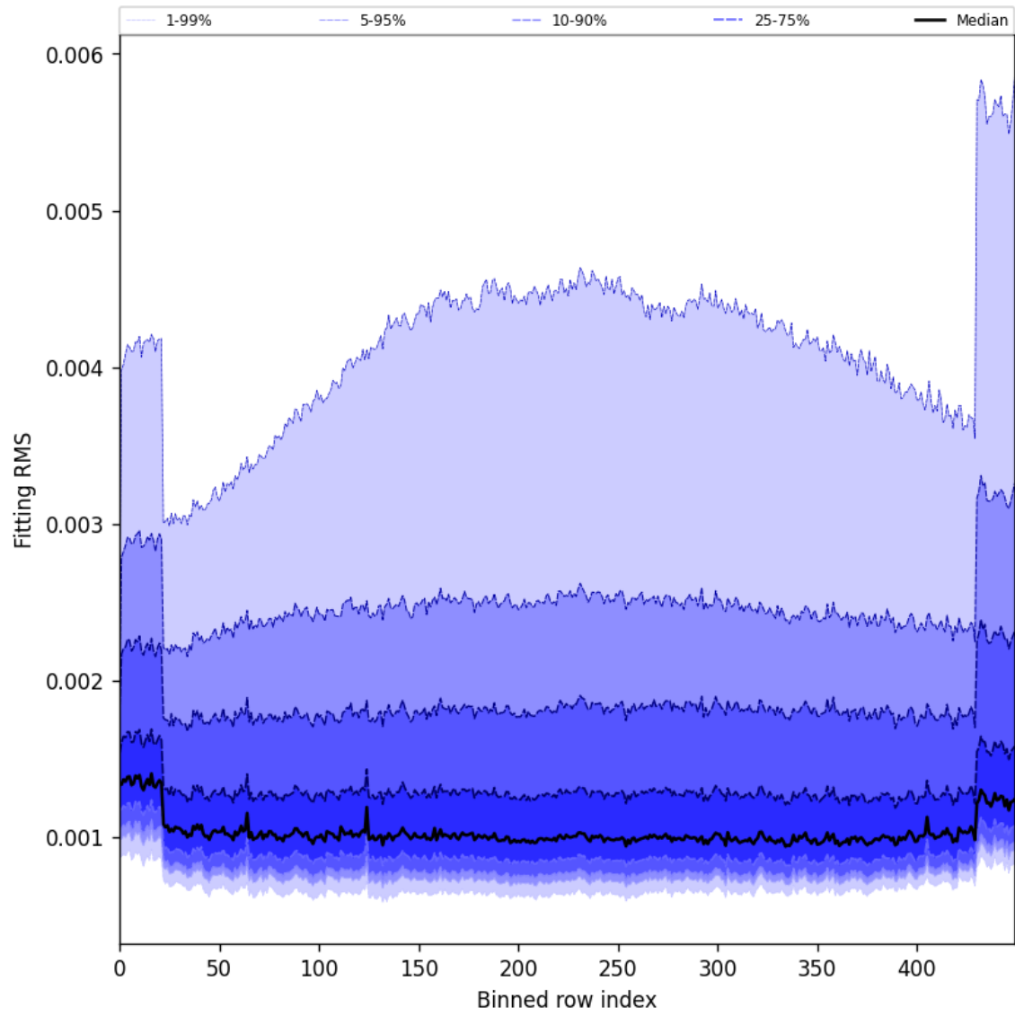
Figure 30: Along track statistics of “Fitting RMS” for 2024-09-06 to 2024-09-07
