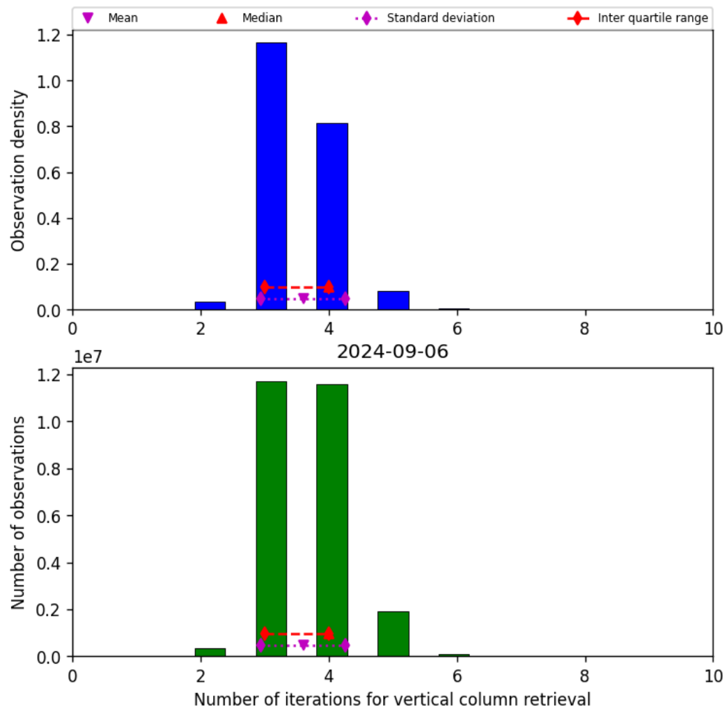
Figure 26: Histogram of “Number of iterations for vertical column retrieval” for 2024-09-06 to 2024-09-07
