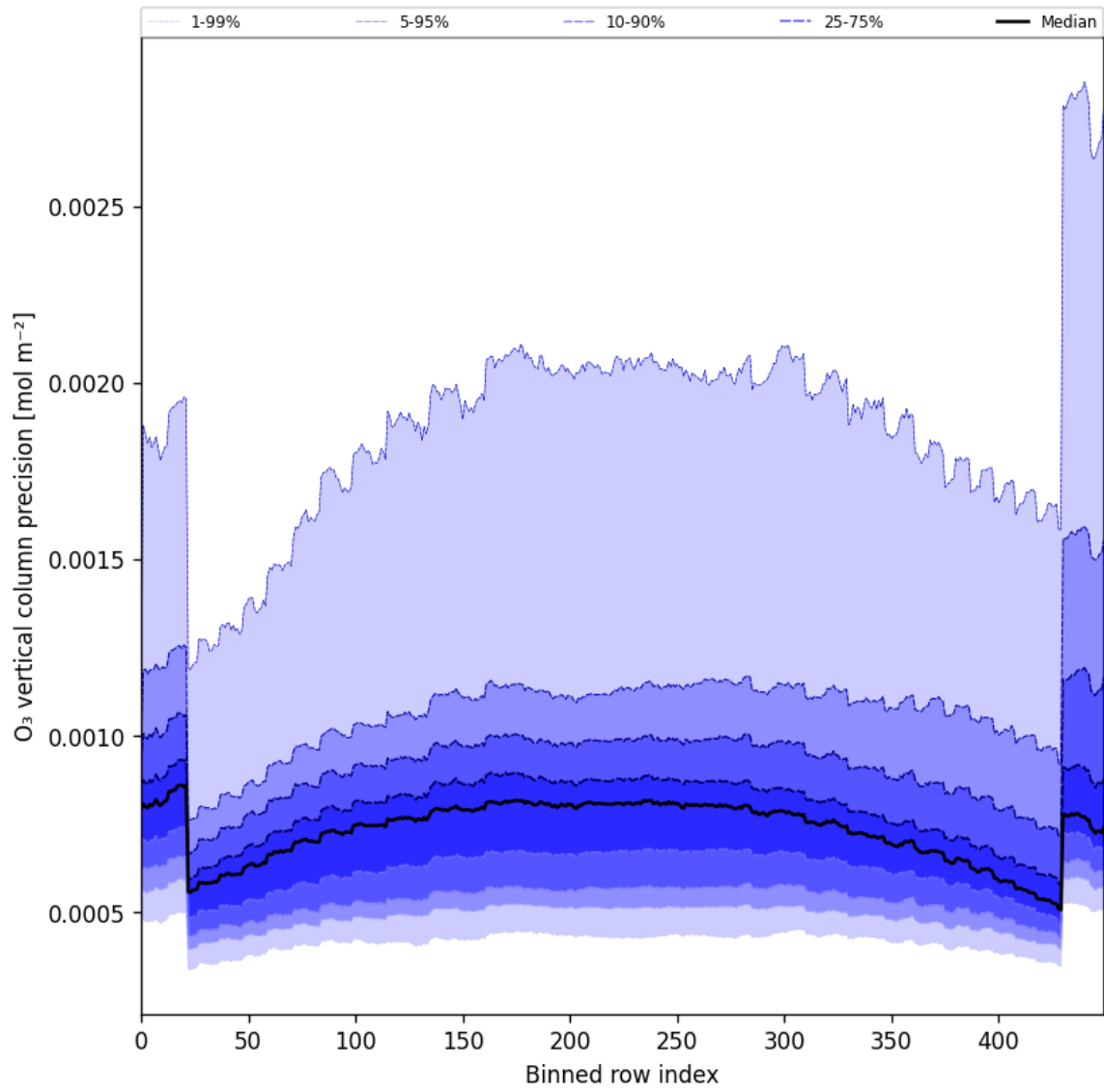
Figure 29: Along track statistics of “O 3 vertical column precision” for 2024-09-06 to 2024-09-07
