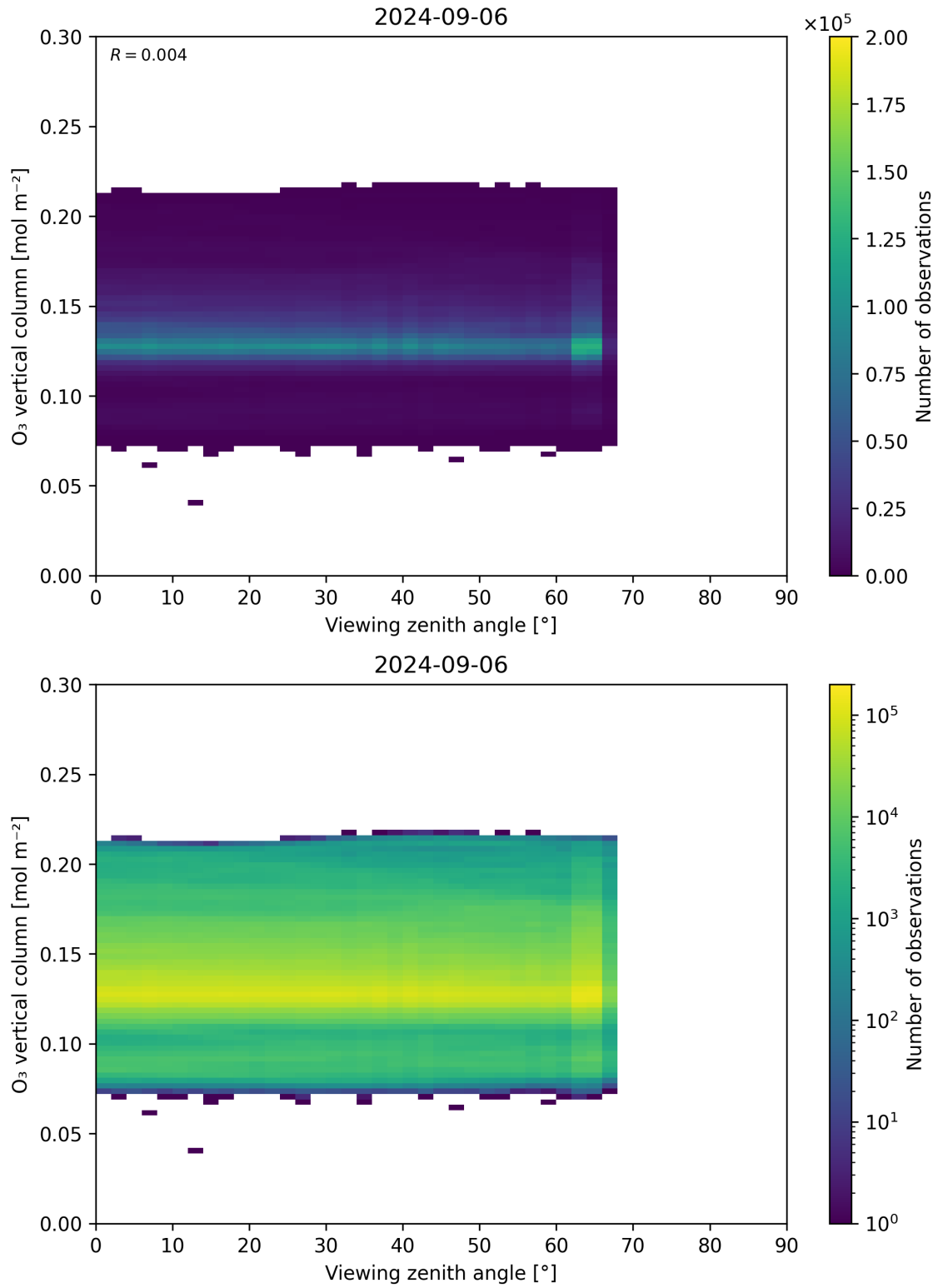
Figure 52: Scatter density plot of “Viewing zenith angle” against “O 3 vertical column” for 2024-09-06 to 2024-09-07.
