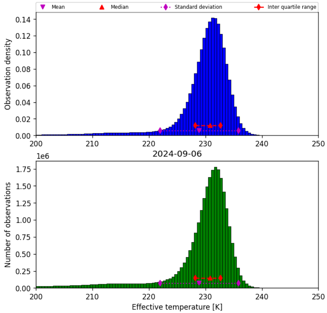
Figure 24: Histogram of “Effective temperature” for 2024-09-06 to 2024-09-07
