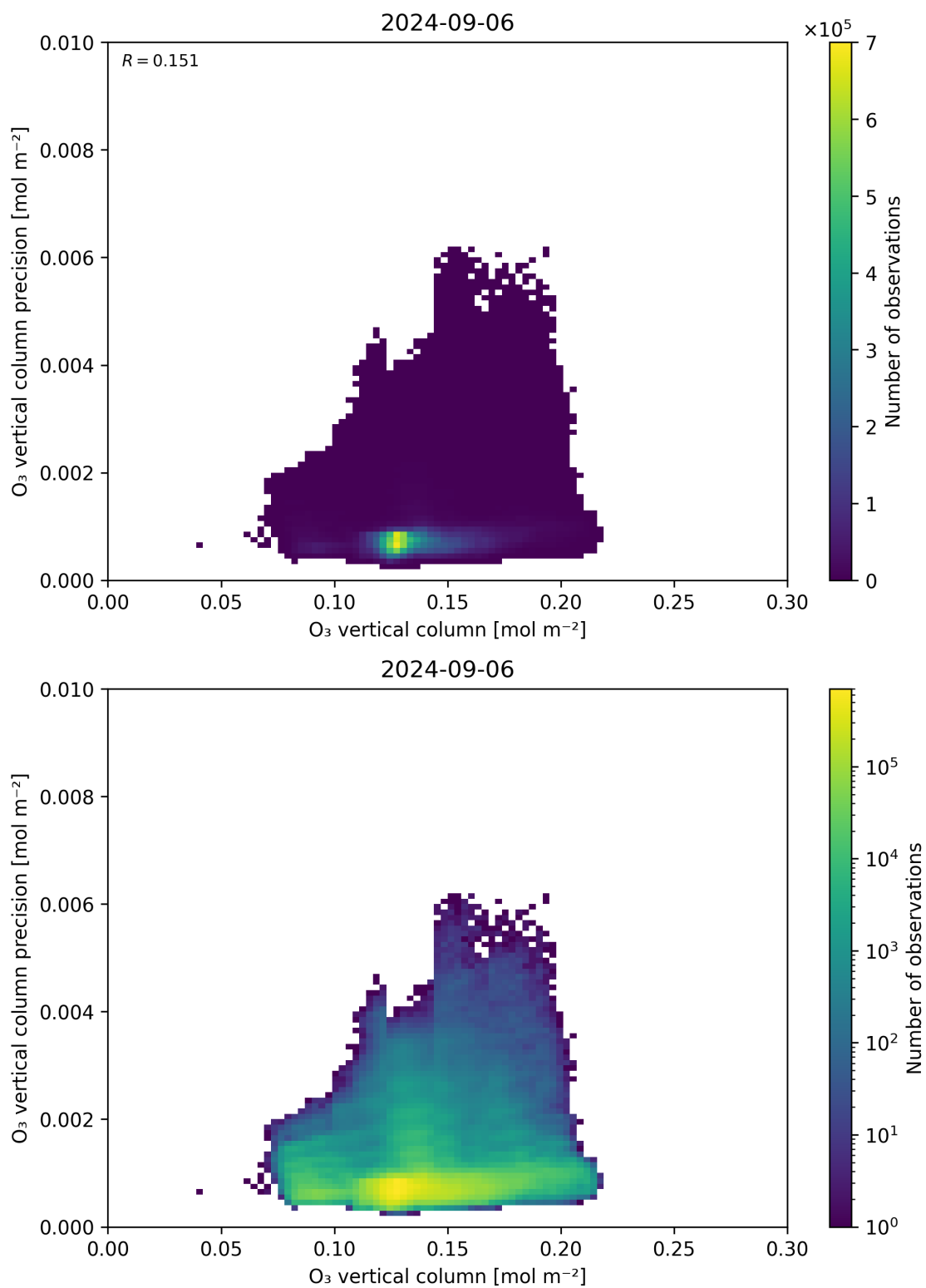
Figure 41: Scatter density plot of “O 3 vertical column” against “O 3 vertical column precision” for 2024-09-06 to 2024-09-07.
