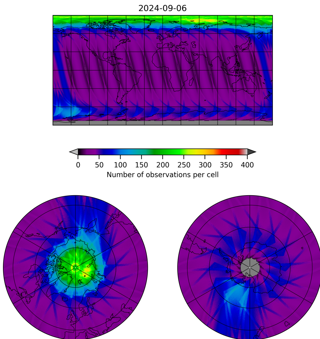
Figure 12: Map of the number of observations for 2024-09-06 to 2024-09-07
