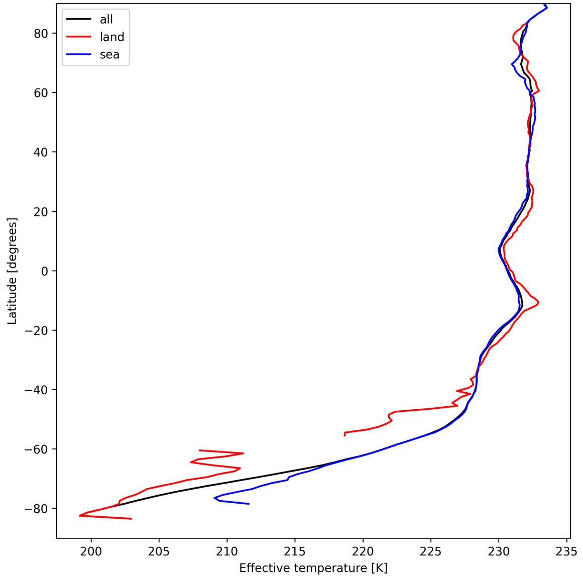
Figure 17: Zonal average of "Effective temperature" for 2024-09-06 to 2024-09-07.
