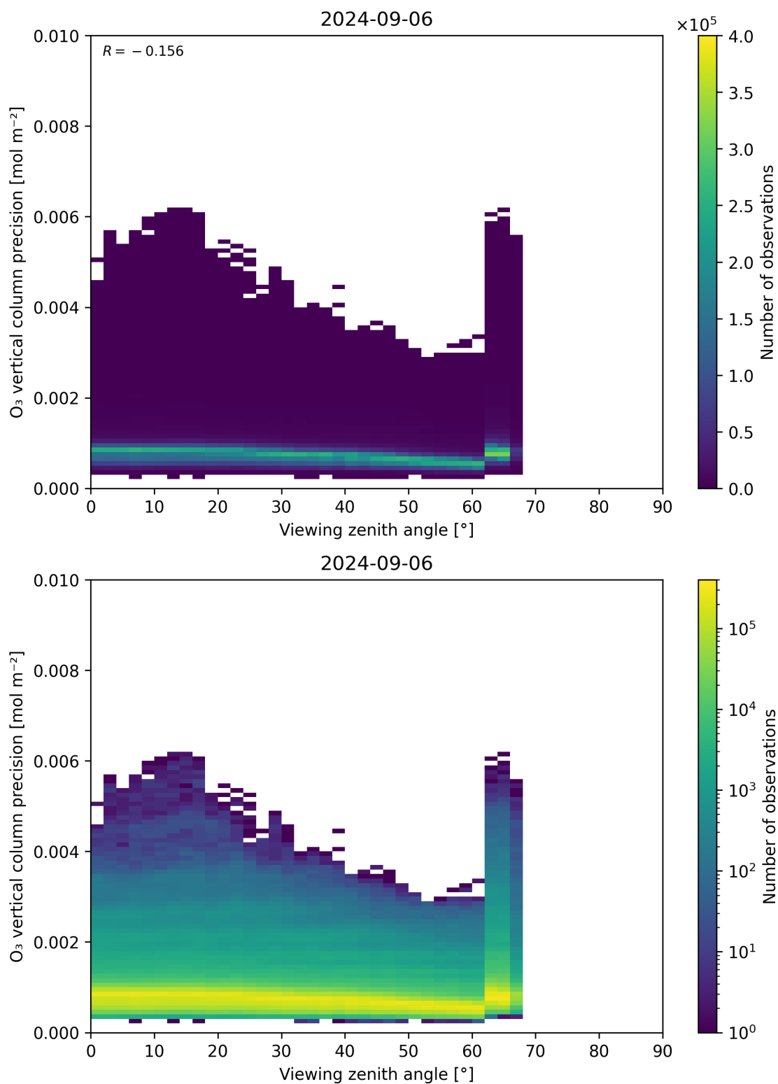
Figure 53: Scatter density plot of “Viewing zenith angle” against “O 3 vertical column precision” for 2024-09-06 to 2024-09-07.
