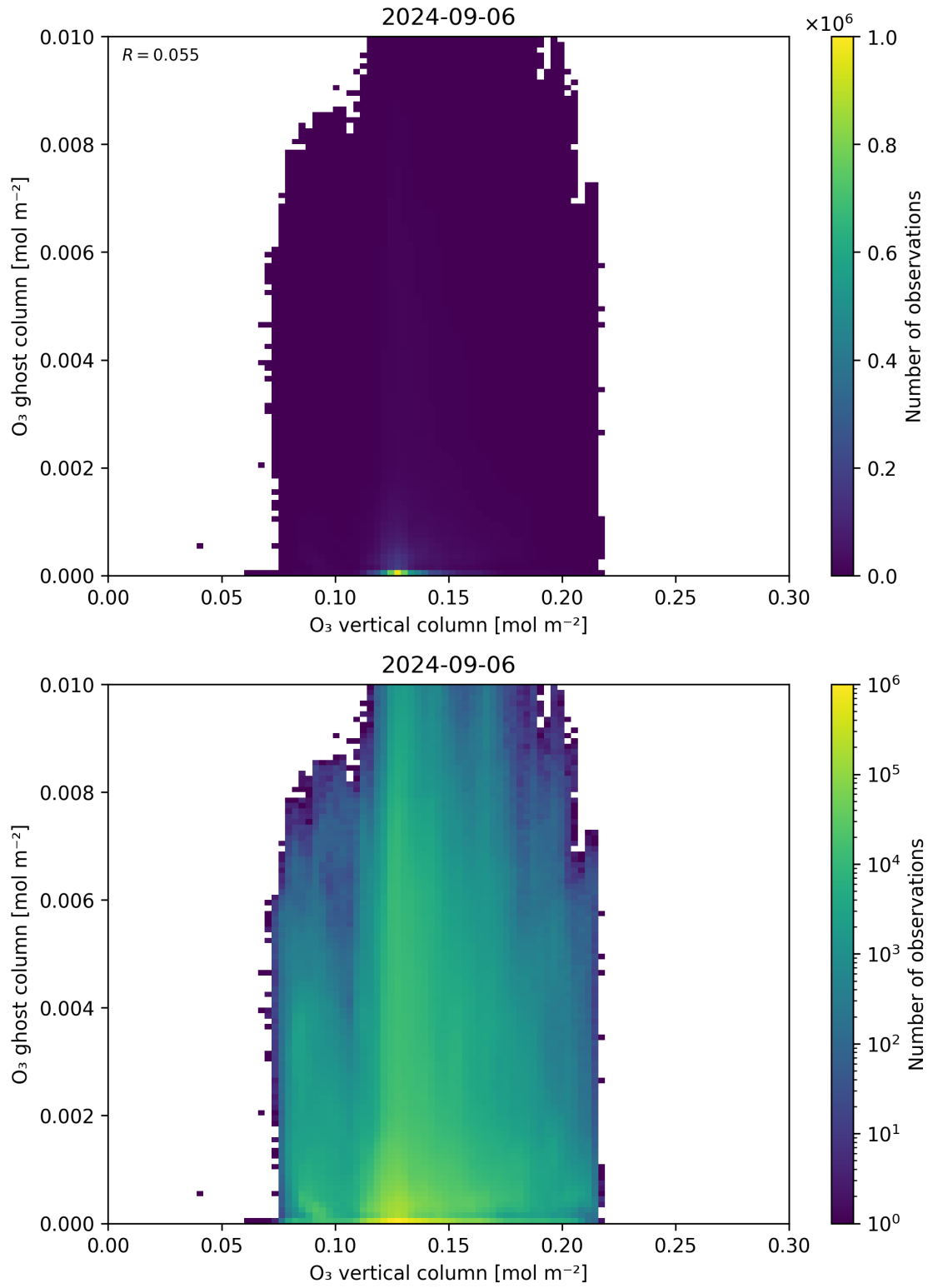
Figure 40: Scatter density plot of “O 3 vertical column” against “O 3 ghost column” for 2024-09-06 to 2024-09-07.
