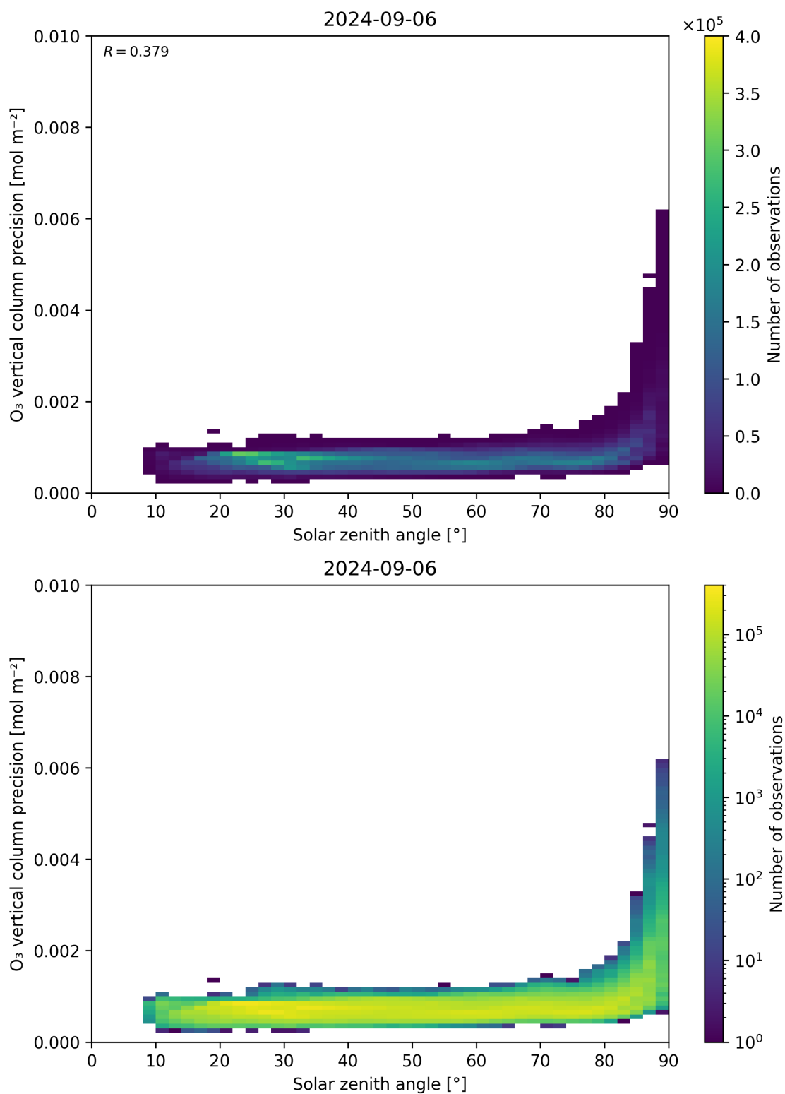
Figure 48: Scatter density plot of “Solar zenith angle” against “O 3 vertical column precision” for 2024-09-06 to 2024-09-07.
