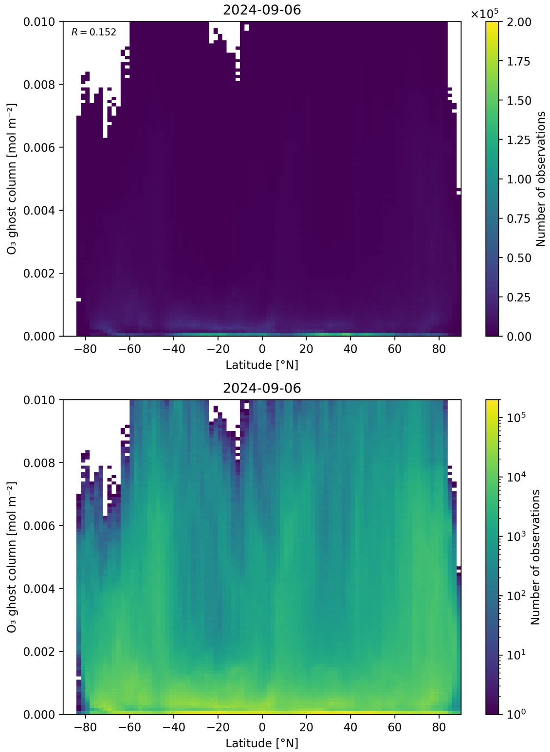
Figure 35: Scatter density plot of “Latitude” against “O 3 ghost column” for 2024-09-06 to 2024-09-07.
