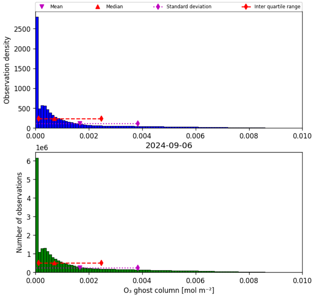
Figure 25: Histogram of “O 3 ghost column” for 2024-09-06 to 2024-09-07
