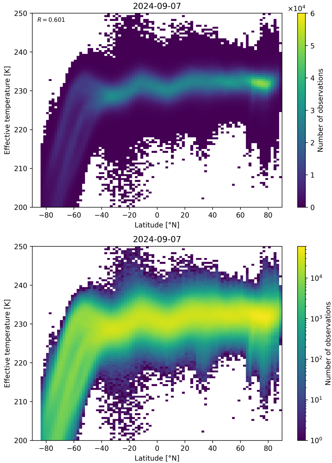
Figure 34: Scatter density plot of “Latitude” against “Effective temperature” for 2024-09-06 to 2024-09-08.
