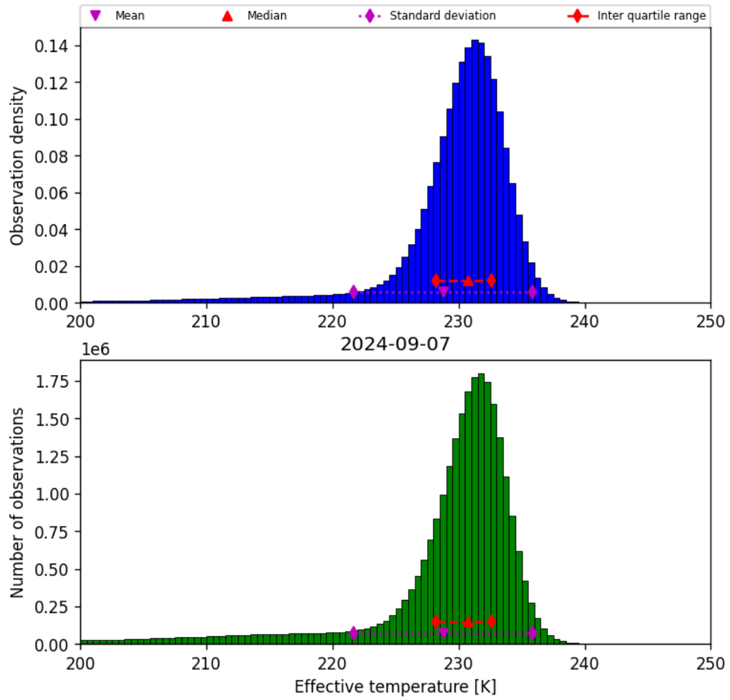
Figure 24: Histogram of “Effective temperature” for 2024-09-06 to 2024-09-08
