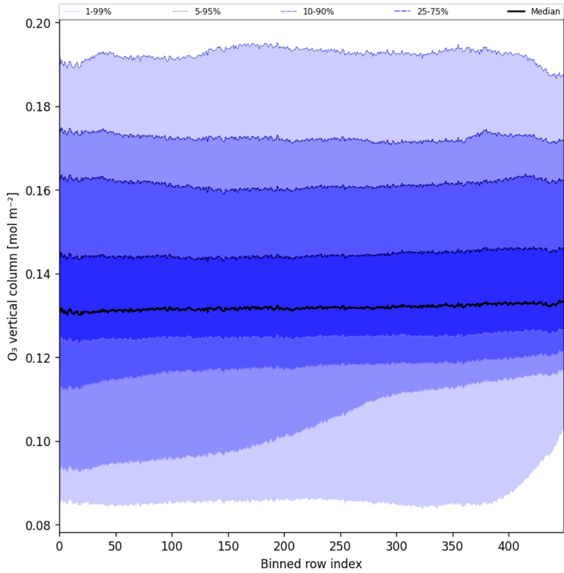
Figure 28: Along track statistics of “O 3 vertical column” for 2024-09-06 to 2024-09-08
