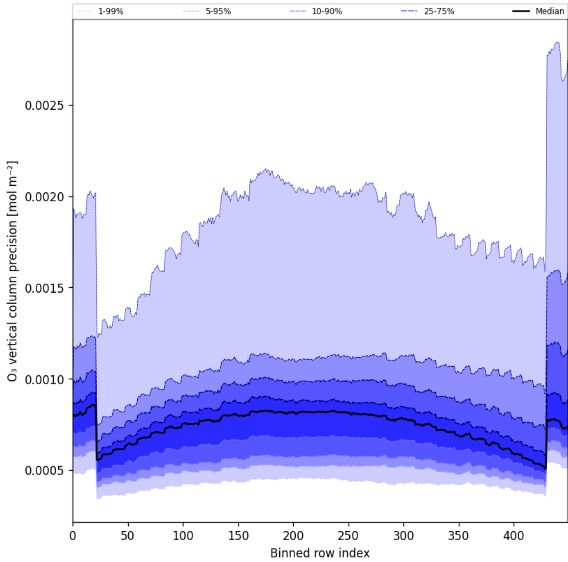
Figure 29: Along track statistics of “O 3 vertical column precision” for 2024-09-06 to 2024-09-08
