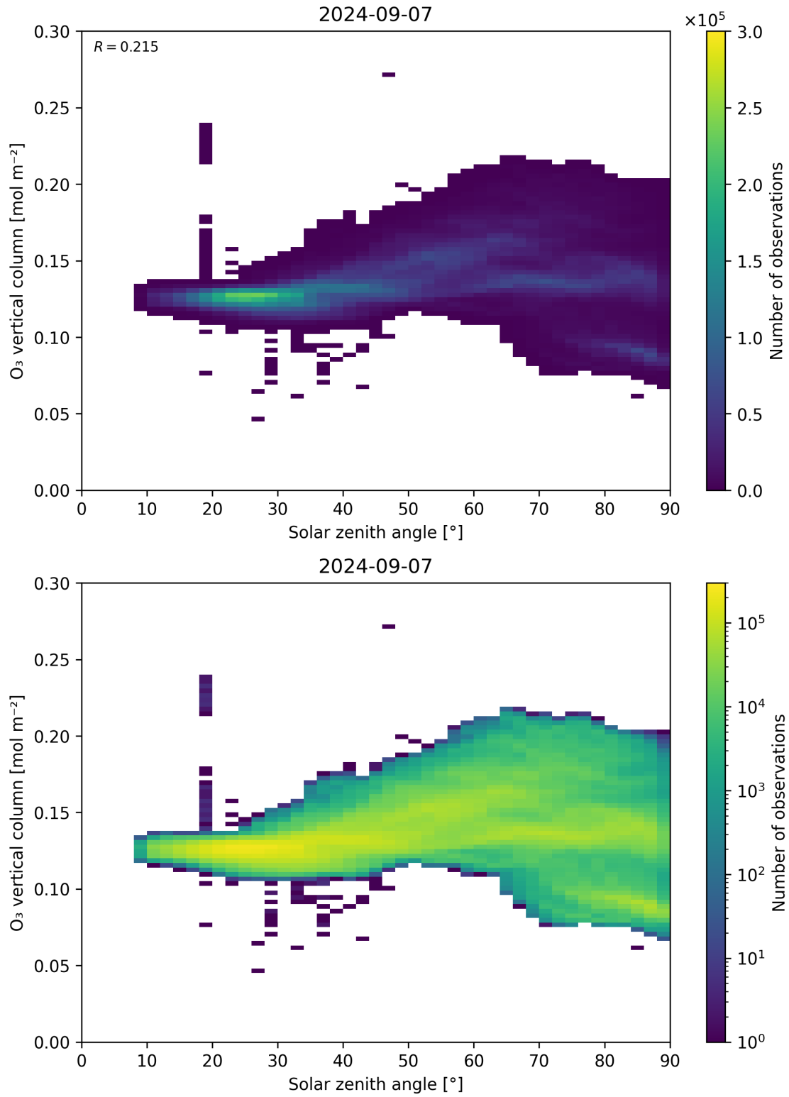
Figure 47: Scatter density plot of “Solar zenith angle” against “O 3 vertical column” for 2024-09-06 to 2024-09-08.
