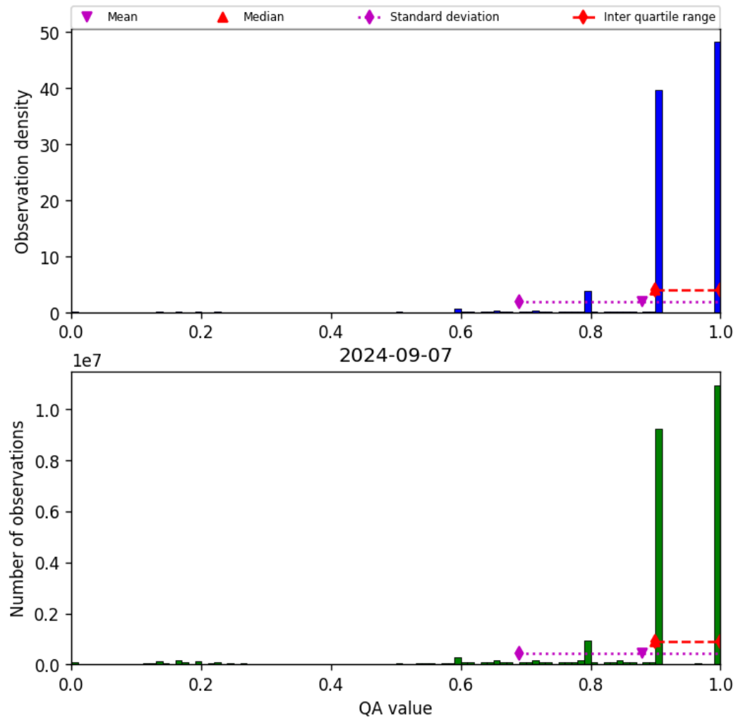
Figure 20: Histogram of “QA value” for 2024-09-06 to 2024-09-08
