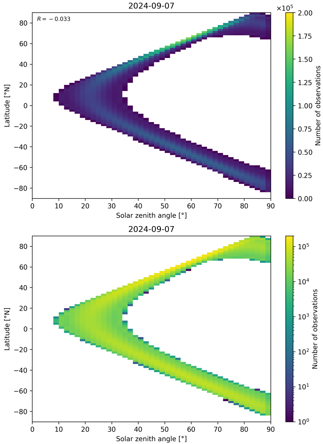
Figure 44: Scatter density plot of “Solar zenith angle” against “Latitude” for 2024-09-06 to 2024-09-08.
