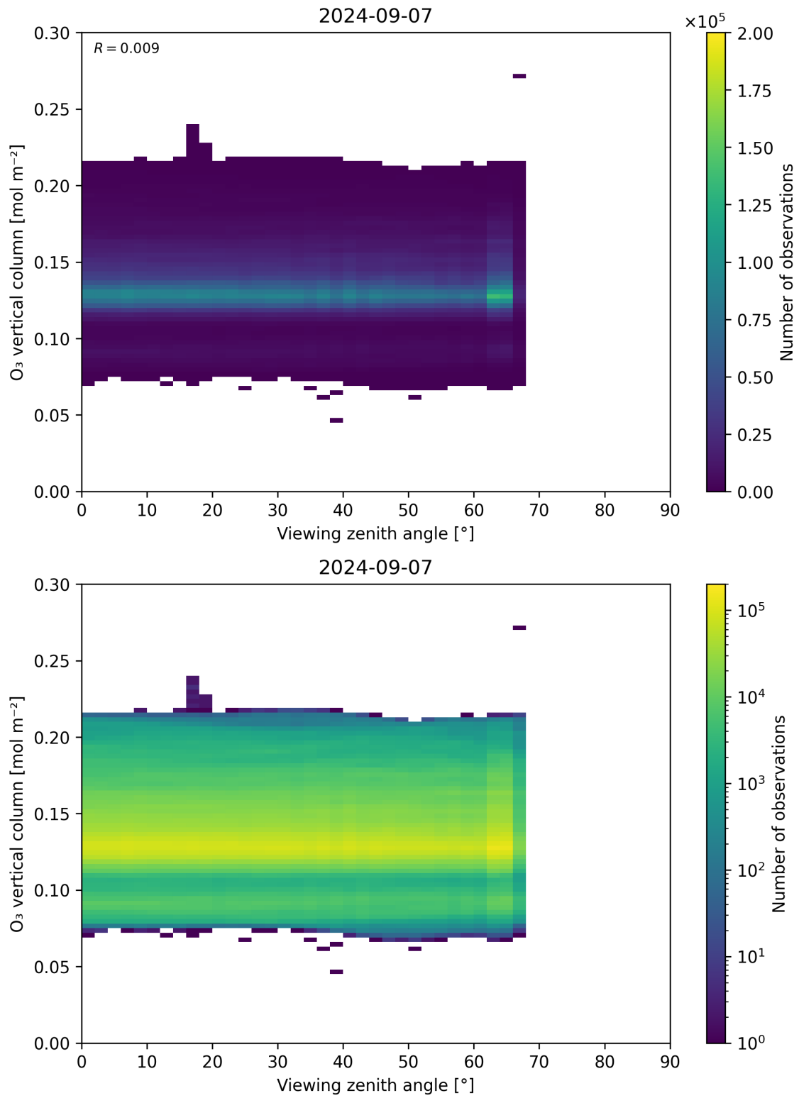
Figure 52: Scatter density plot of “Viewing zenith angle” against “O 3 vertical column” for 2024-09-06 to 2024-09-08.
