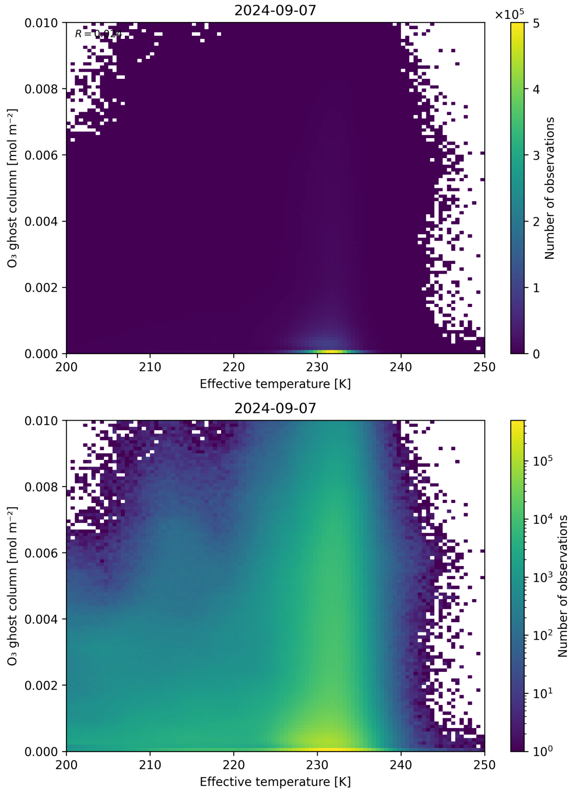
Figure 38: Scatter density plot of “Effective temperature” against “O 3 ghost column” for 2024-09-06 to 2024-09-08.
