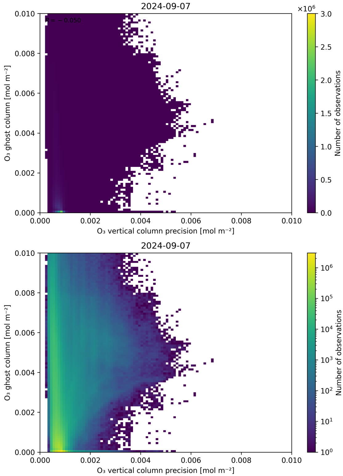
Figure 43: Scatter density plot of “ \text{O}_3 vertical column precision” against “ \text{O}_3 ghost column” for 2024-09-06 to 2024-09-08.
