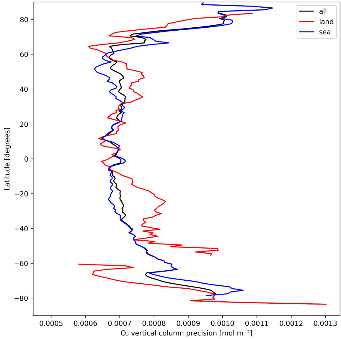
Figure 15: Zonal average of “O 3 vertical column precision” for 2024-09-06 to 2024-09-08.
