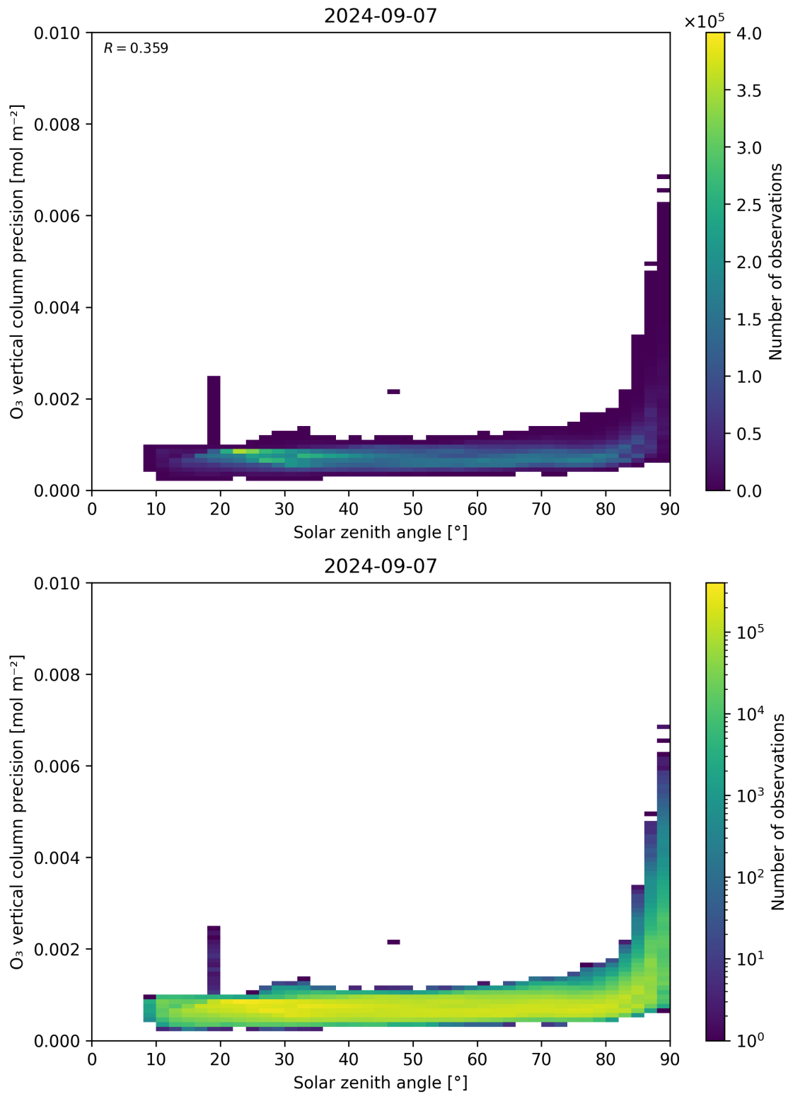
Figure 48: Scatter density plot of “Solar zenith angle” against “O 3 vertical column precision” for 2024-09-06 to 2024-09-08.
