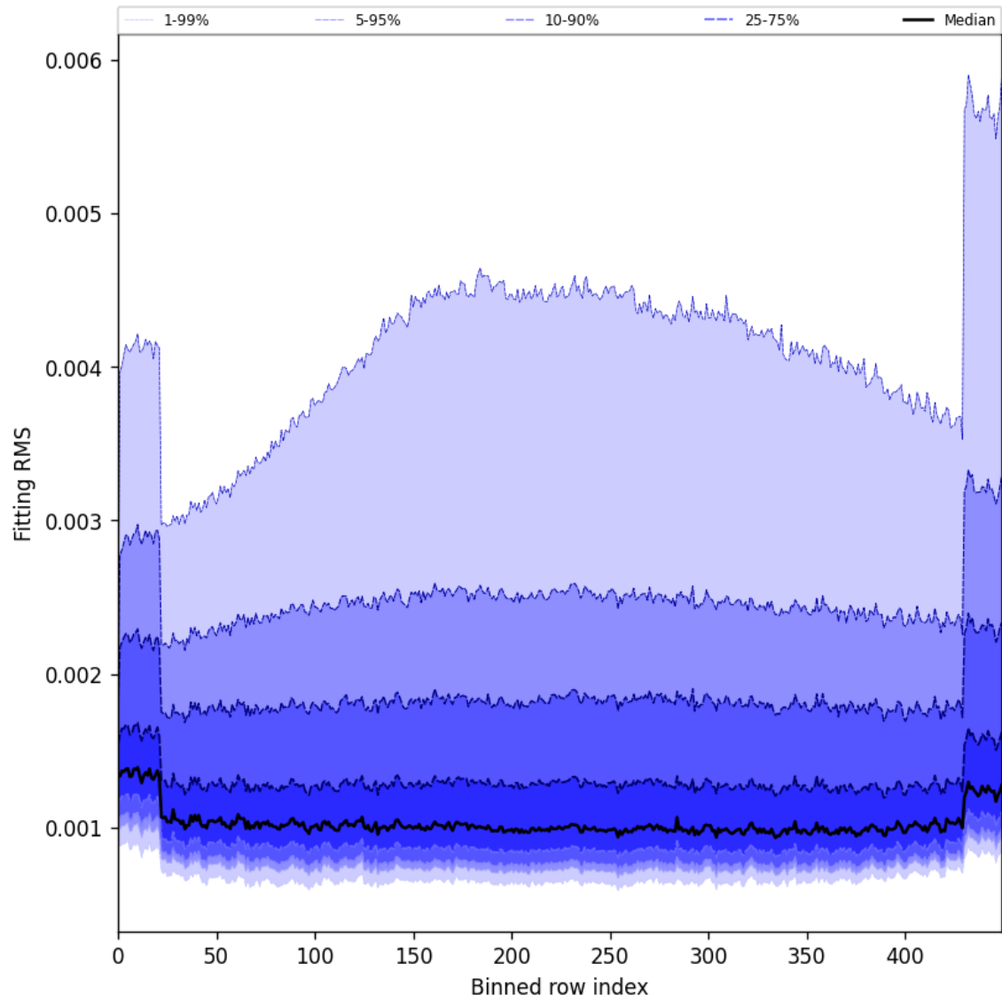
Figure 30: Along track statistics of “Fitting RMS” for 2024-09-06 to 2024-09-08
