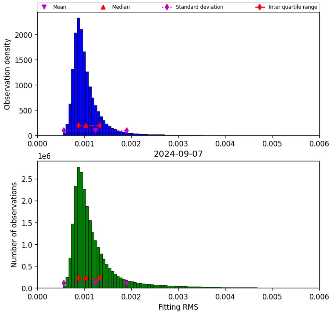
Figure 23: Histogram of “Fitting RMS” for 2024-09-06 to 2024-09-08
