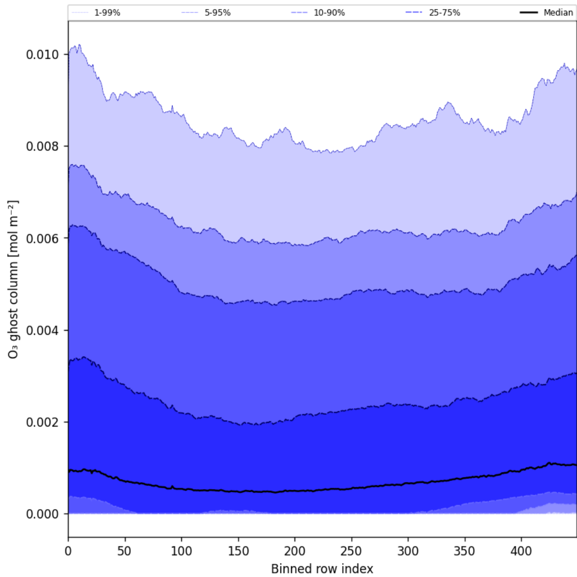
Figure 32: Along track statistics of “O 3 ghost column” for 2024-09-06 to 2024-09-08
