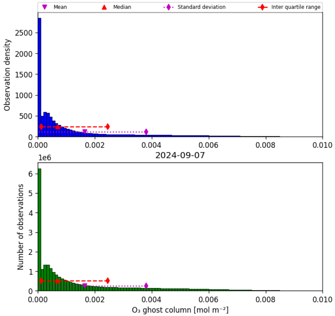
Figure 25: Histogram of “O 3 ghost column” for 2024-09-06 to 2024-09-08
