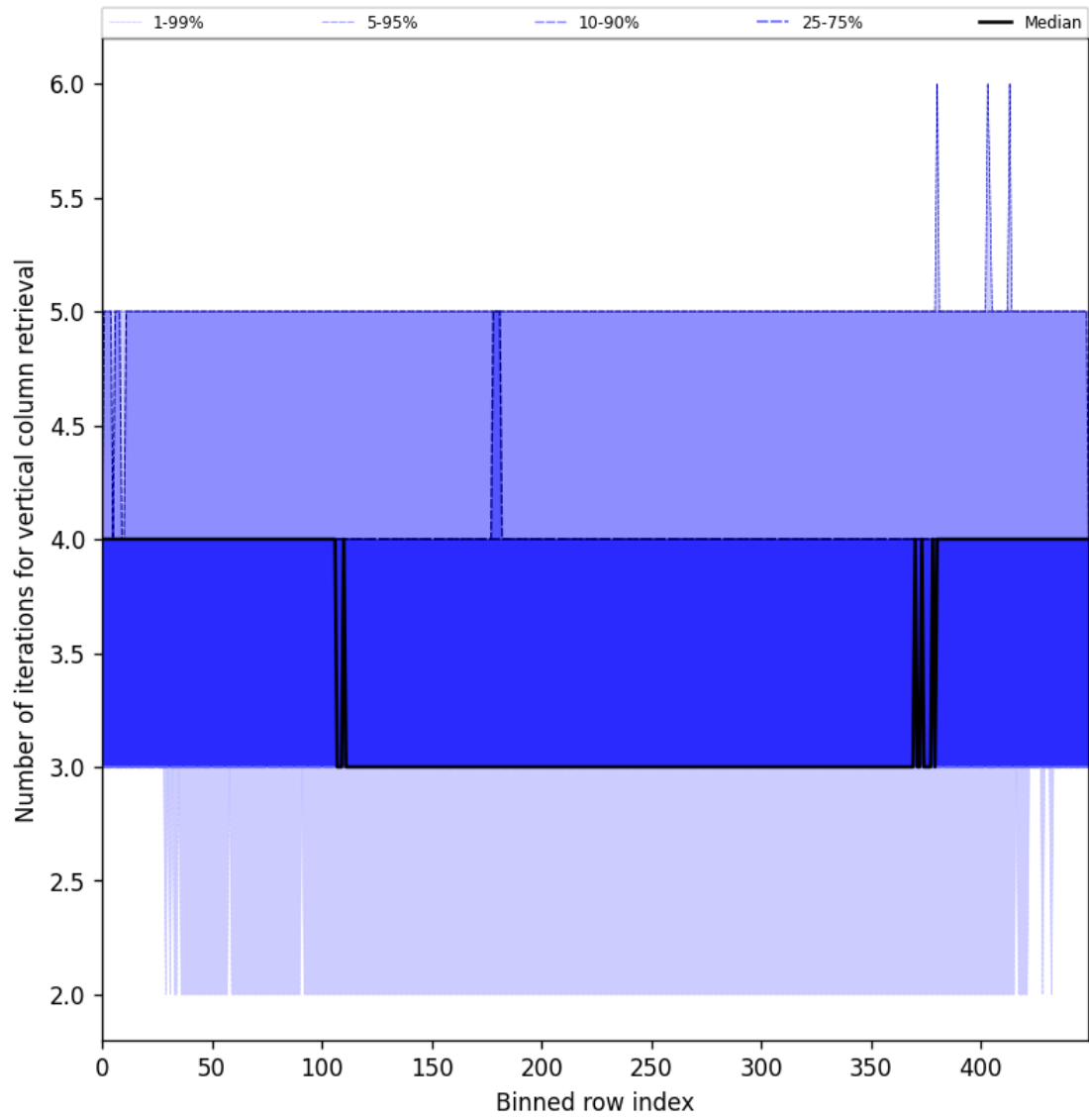
Figure 33: Along track statistics of “Number of iterations for vertical column retrieval” for 2024-09-06 to 2024-09-08
