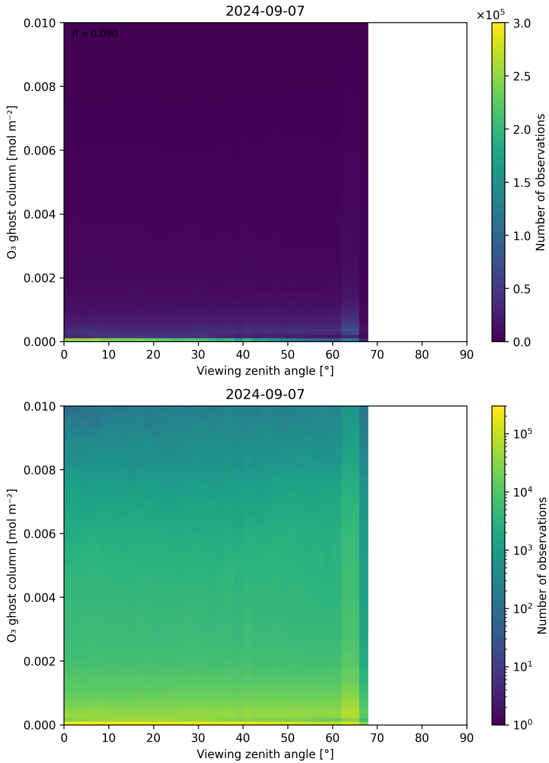
Figure 51: Scatter density plot of “Viewing zenith angle” against “O 3 ghost column” for 2024-09-06 to 2024-09-08.
