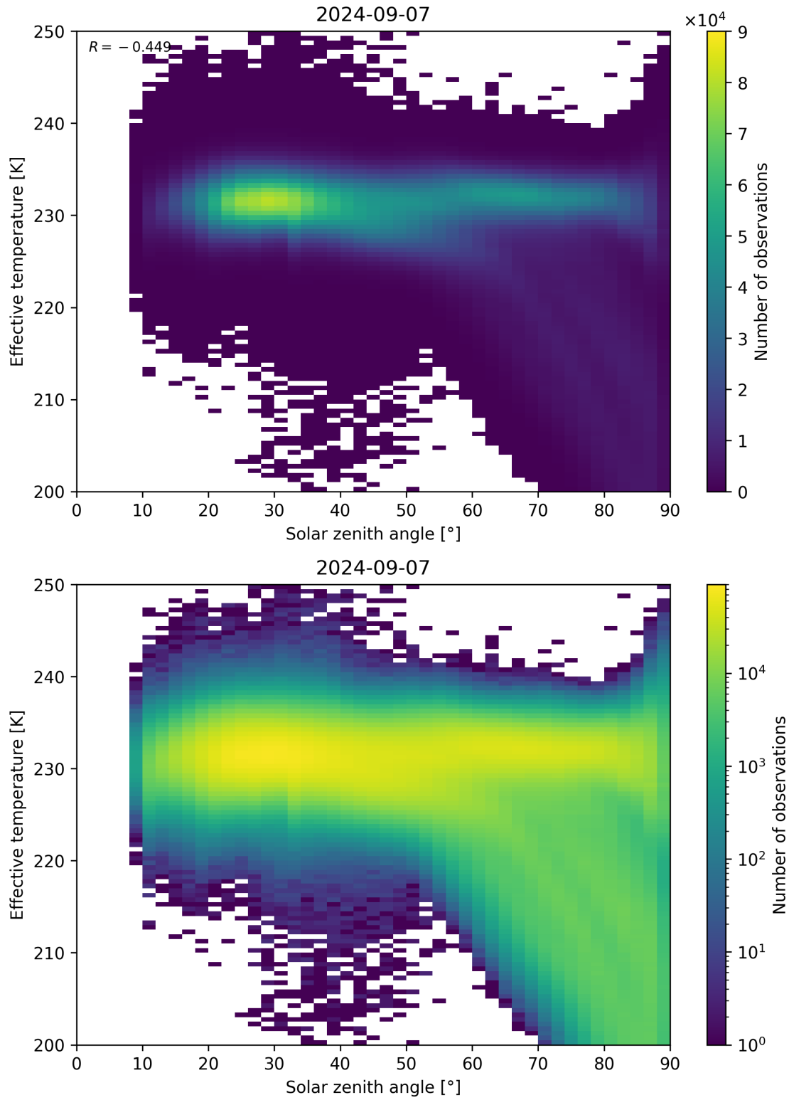
Figure 45: Scatter density plot of “Solar zenith angle” against “Effective temperature” for 2024-09-06 to 2024-09-08.
