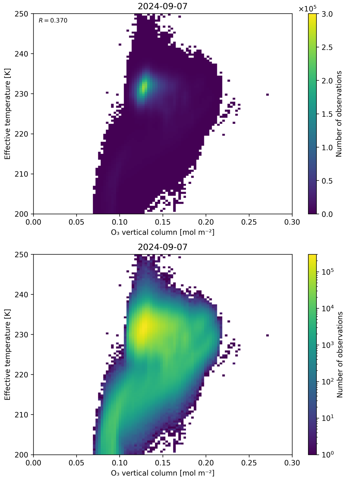
Figure 39: Scatter density plot of “O 3 vertical column” against “Effective temperature” for 2024-09-06 to 2024-09-08.
