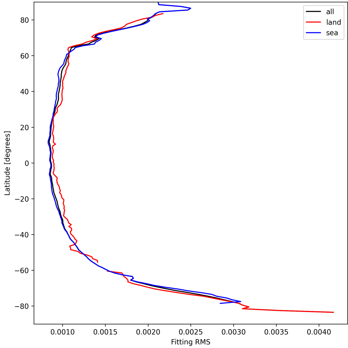
Figure 16: Zonal average of “Fitting RMS” for 2024-09-06 to 2024-09-08.
