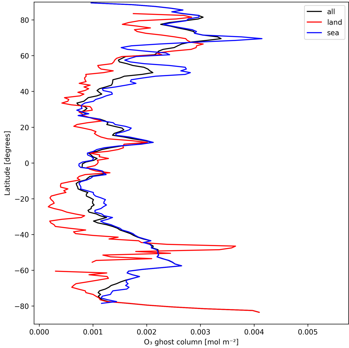
Figure 18: Zonal average of “O 3 ghost column” for 2024-09-06 to 2024-09-08.
