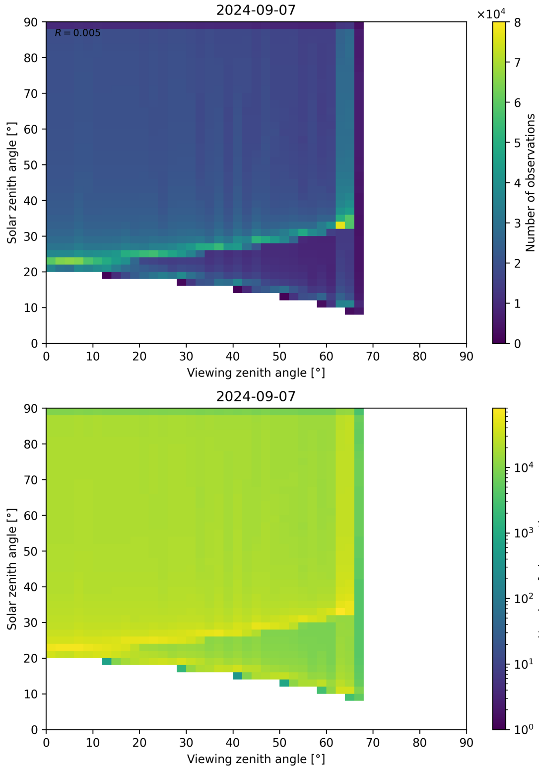
Figure 54: Scatter density plot of “Viewing zenith angle” against “Solar zenith angle” for 2024-09-06 to 2024-09-08.
