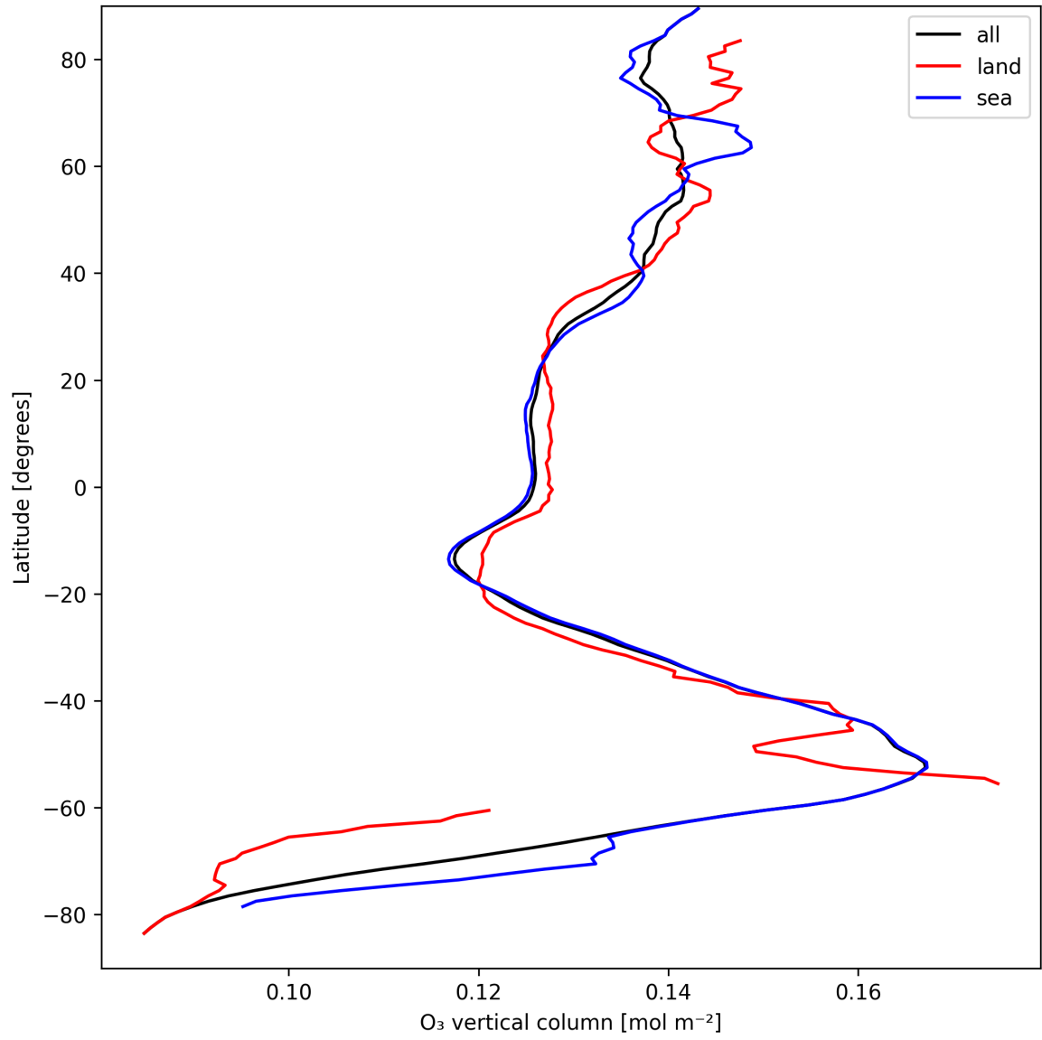
Figure 14: Zonal average of “O 3 vertical column” for 2024-09-06 to 2024-09-08.
