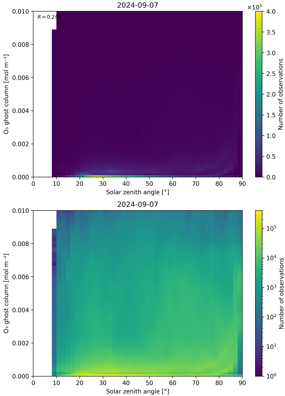
Figure 46: Scatter density plot of “Solar zenith angle” against “O 3 ghost column” for 2024-09-06 to 2024-09-08.
