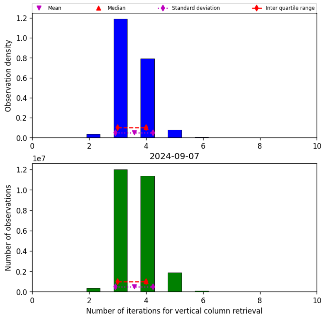
Figure 26: Histogram of “Number of iterations for vertical column retrieval” for 2024-09-06 to 2024-09-08
