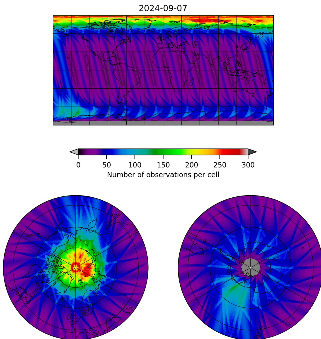
Figure 12: Map of the number of observations for 2024-09-06 to 2024-09-08
