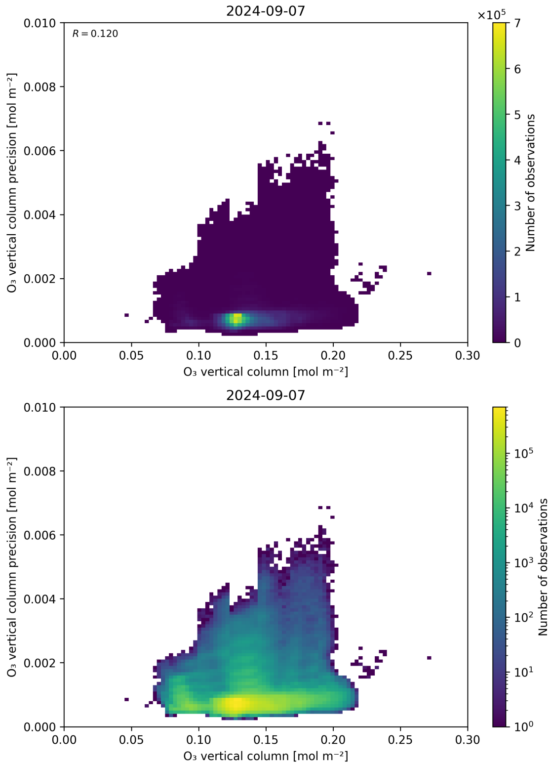
Figure 41: Scatter density plot of “O 3 vertical column” against “O 3 vertical column precision” for 2024-09-06 to 2024-09-08.
