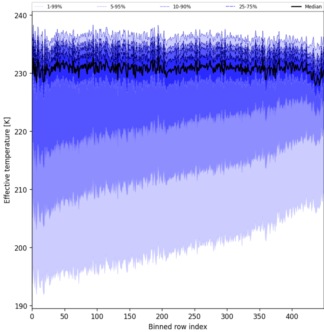
Figure 31: Along track statistics of “Effective temperature” for 2024-09-06 to 2024-09-08
