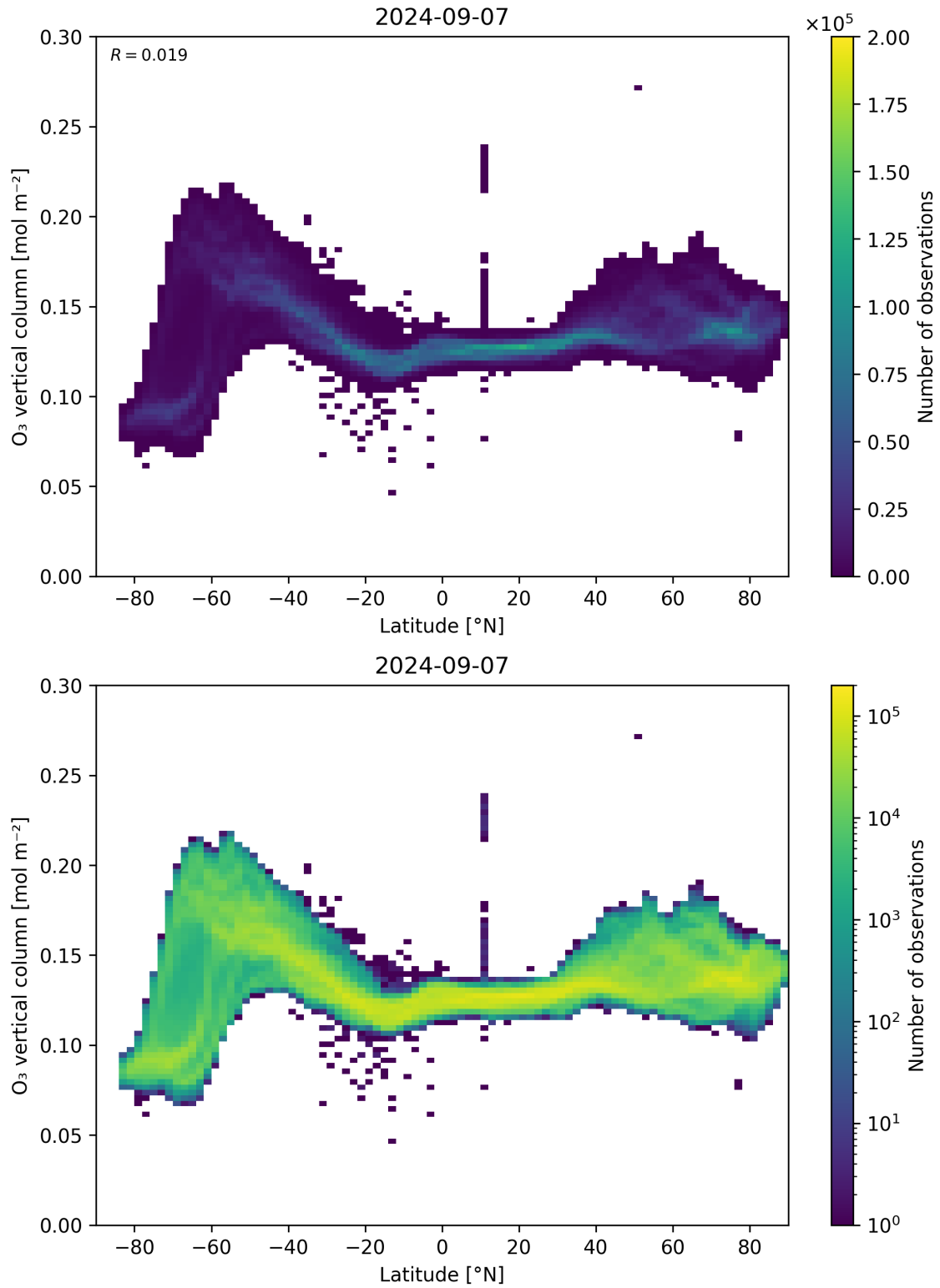
Figure 36: Scatter density plot of “Latitude” against “O 3 vertical column” for 2024-09-06 to 2024-09-08.
