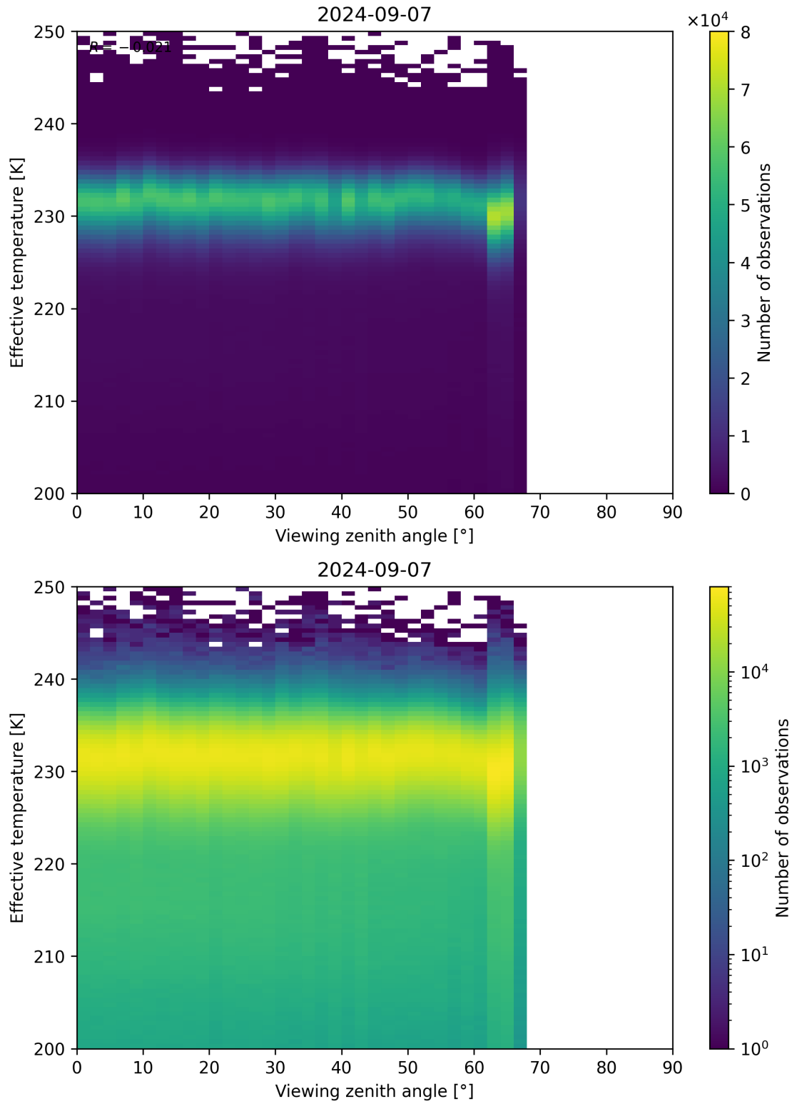
Figure 50: Scatter density plot of “Viewing zenith angle” against “Effective temperature” for 2024-09-06 to 2024-09-08.
