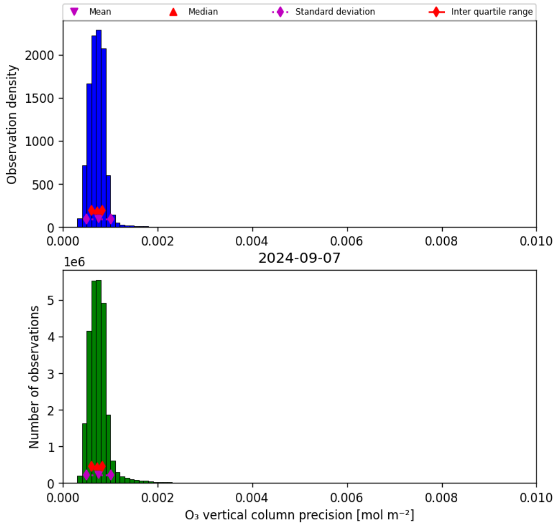
Figure 22: Histogram of “O 3 vertical column precision” for 2024-09-06 to 2024-09-08
