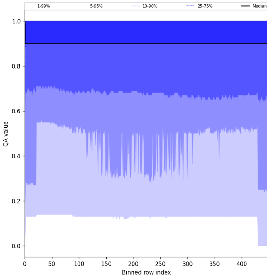
Figure 27: Along track statistics of “QA value” for 2024-09-06 to 2024-09-08
