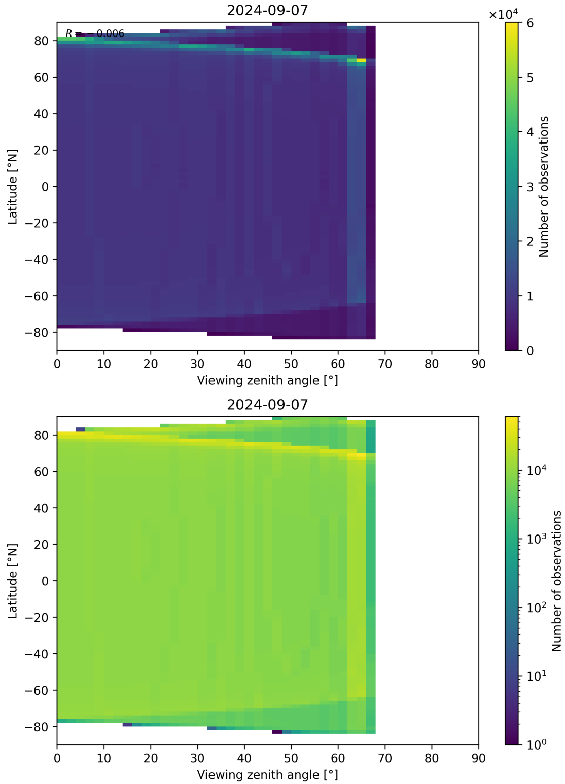
Figure 49: Scatter density plot of “Viewing zenith angle” against “Latitude” for 2024-09-06 to 2024-09-08.
