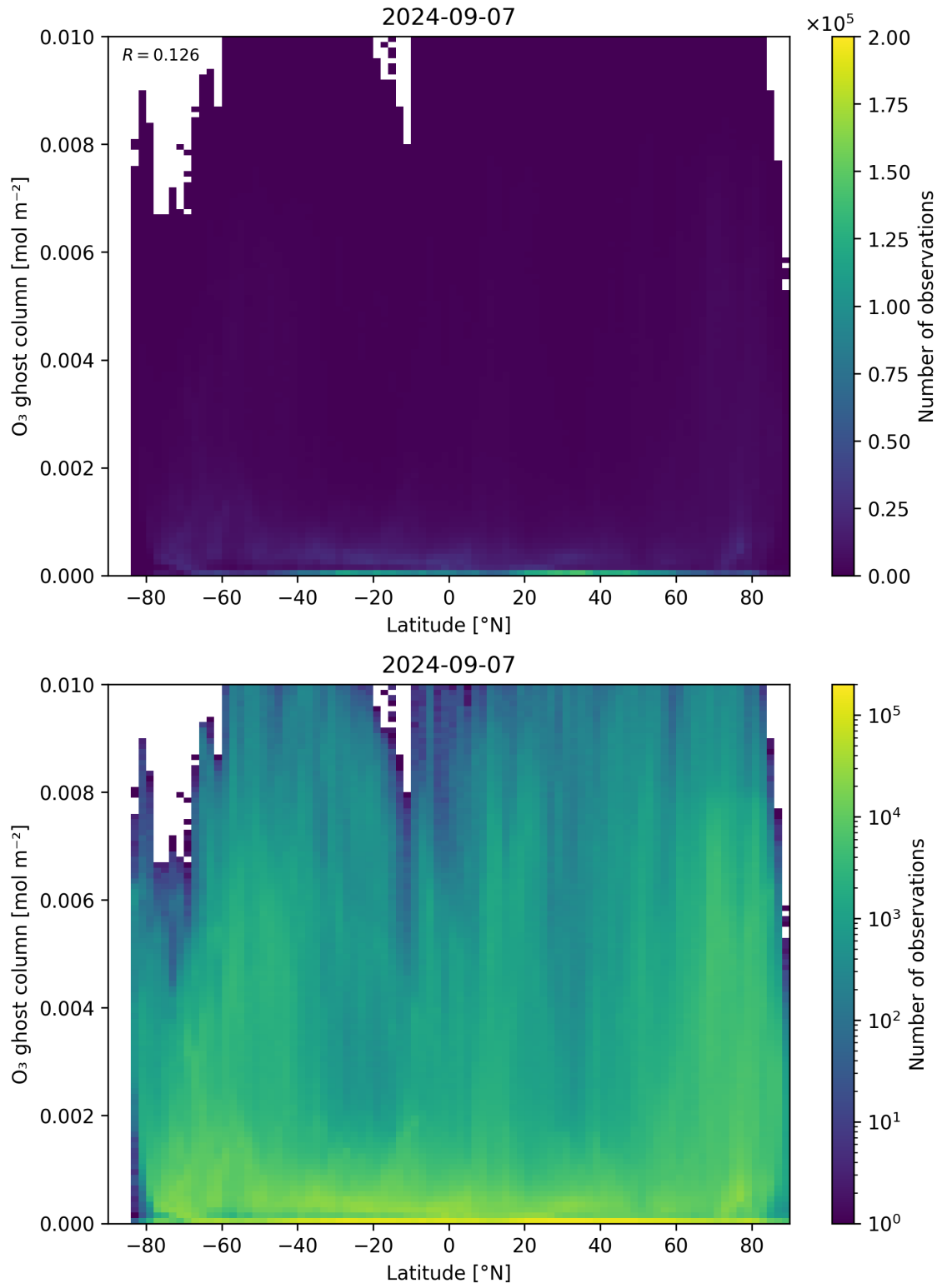
Figure 35: Scatter density plot of “Latitude” against “O 3 ghost column” for 2024-09-06 to 2024-09-08.
