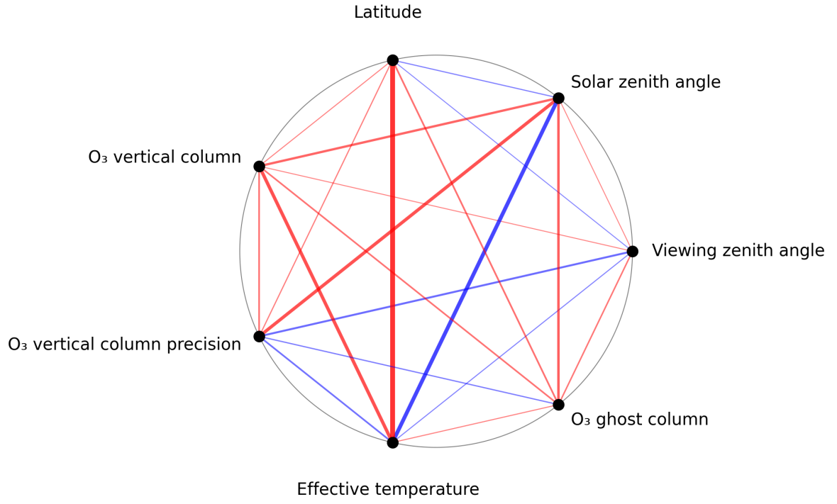
Figure 1: Map of correlation graph for 2024-09-06 to 2024-09-08.
