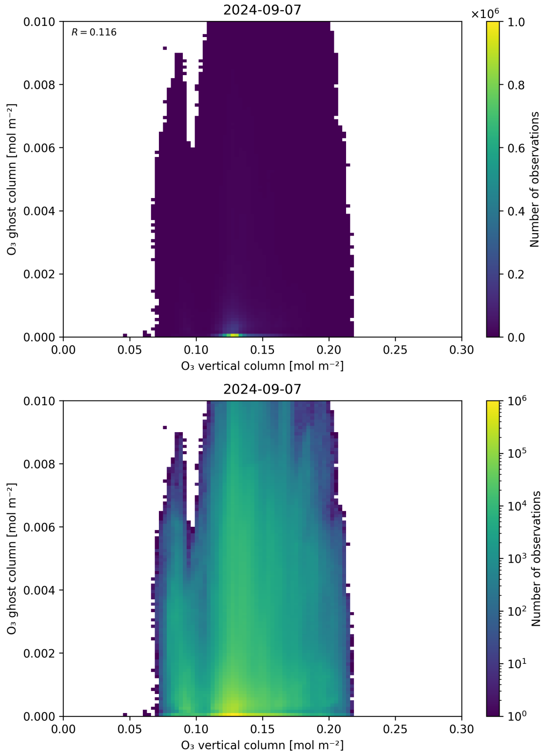
Figure 40: Scatter density plot of “O 3 vertical column” against “O 3 ghost column” for 2024-09-06 to 2024-09-08.
