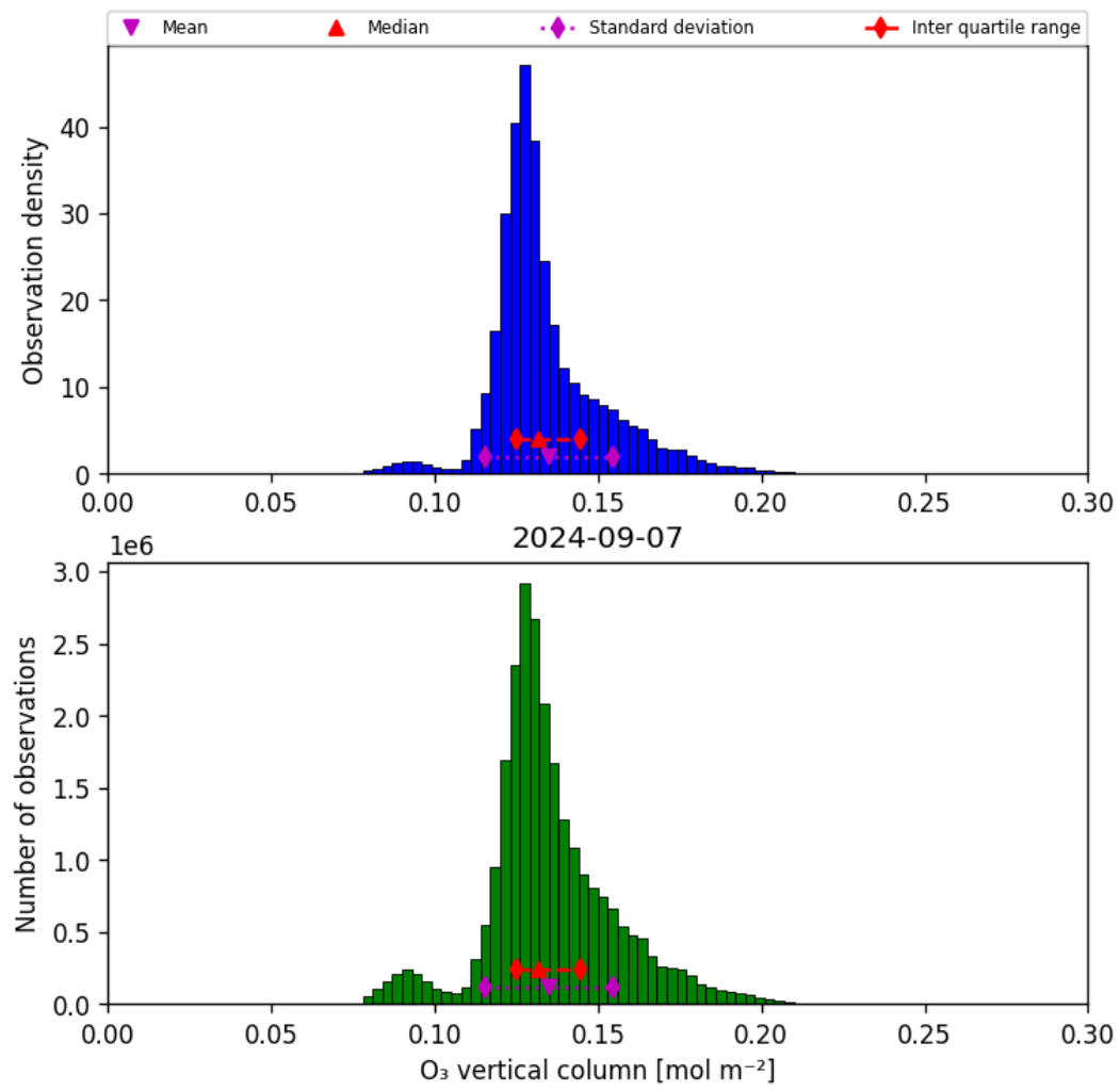
Figure 21: Histogram of “O 3 vertical column” for 2024-09-06 to 2024-09-08
