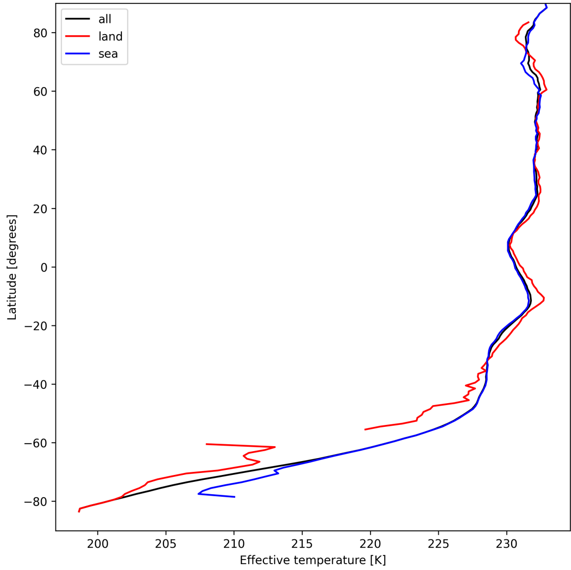
Figure 17: Zonal average of “Effective temperature” for 2024-09-06 to 2024-09-08.
