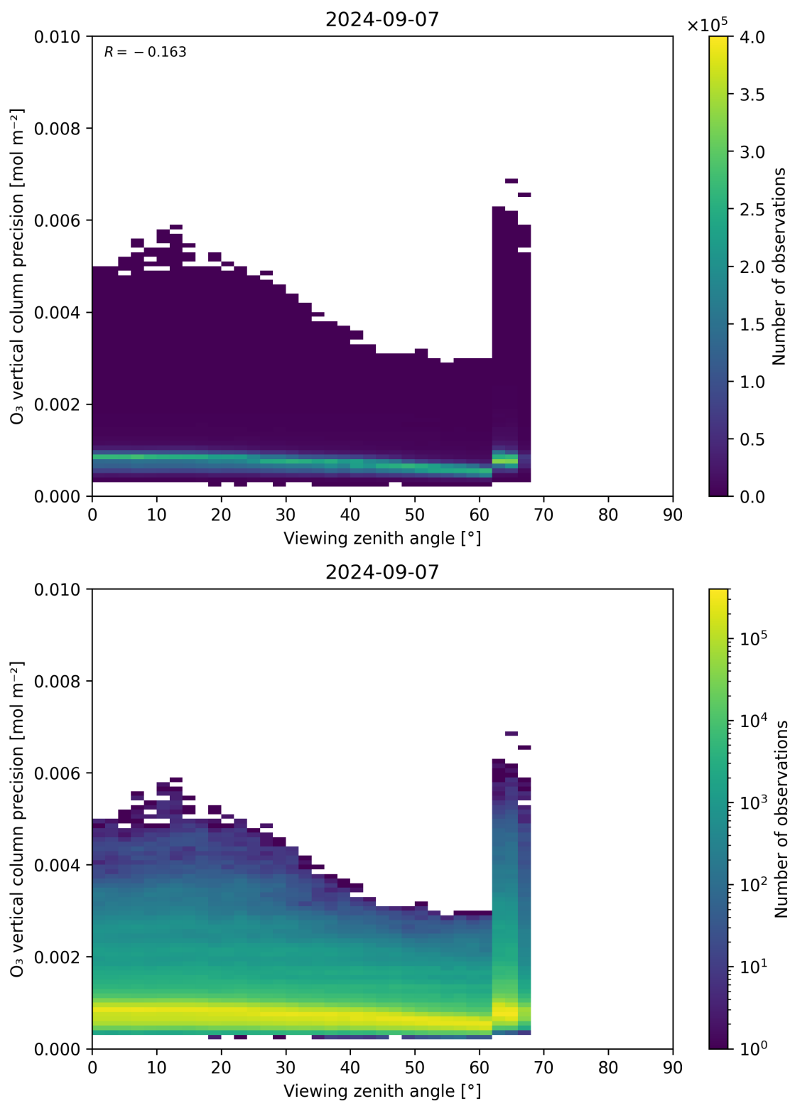
Figure 53: Scatter density plot of “Viewing zenith angle” against “O 3 vertical column precision” for 2024-09-06 to 2024-09-08.
