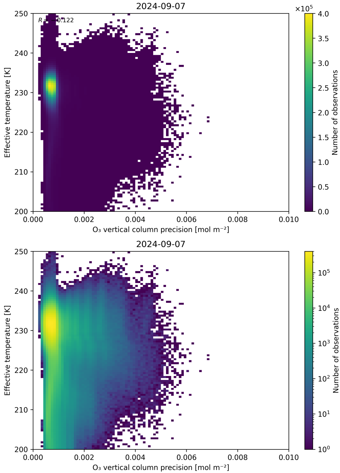
Figure 42: Scatter density plot of “O 3 vertical column precision” against “Effective temperature” for 2024-09-06 to 2024-09-08.
