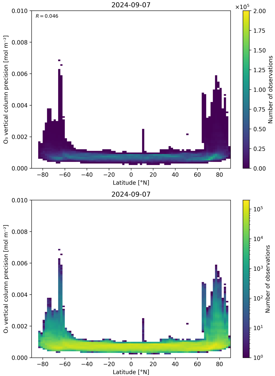
Figure 37: Scatter density plot of “Latitude” against “O 3 vertical column precision” for 2024-09-06 to 2024-09-08.
