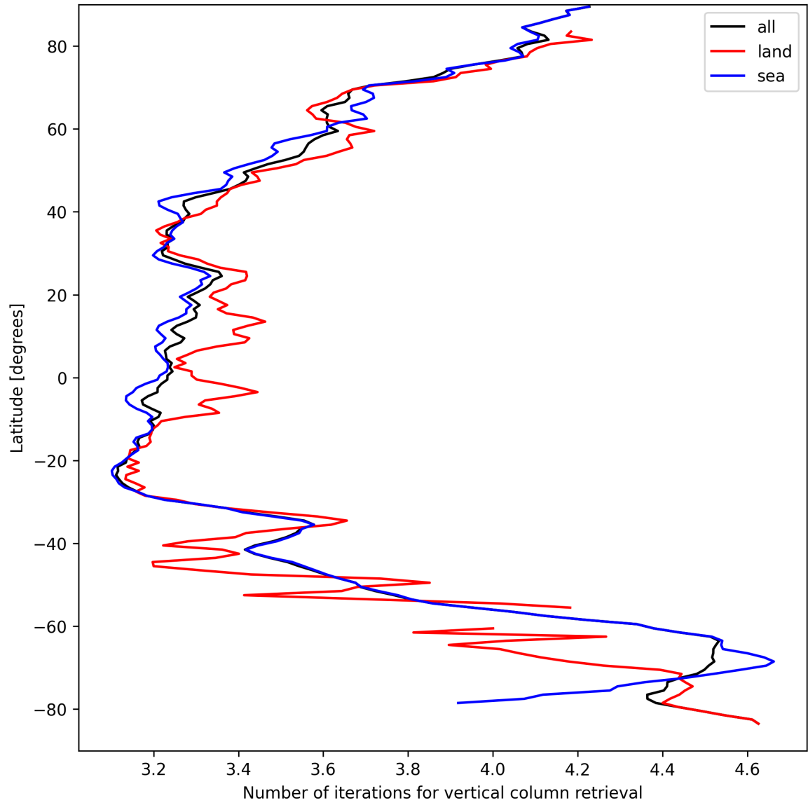
Figure 19: Zonal average of “Number of iterations for vertical column retrieval” for 2024-09-06 to 2024-09-08.
