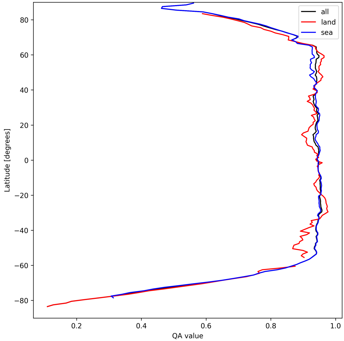
Figure 13: Zonal average of “QA value” for 2024-09-06 to 2024-09-08.
