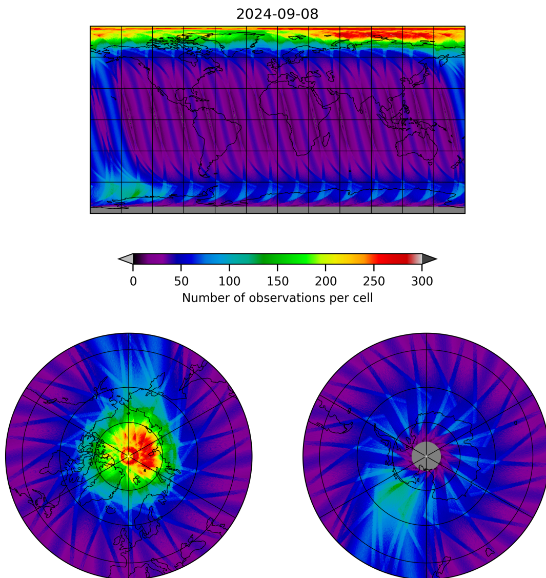
Figure 12: Map of the number of observations for 2024-09-07 to 2024-09-09
