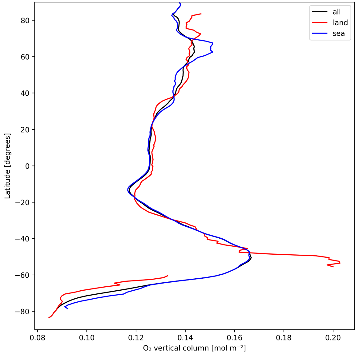
Figure 14: Zonal average of “O 3 vertical column” for 2024-09-07 to 2024-09-09.
