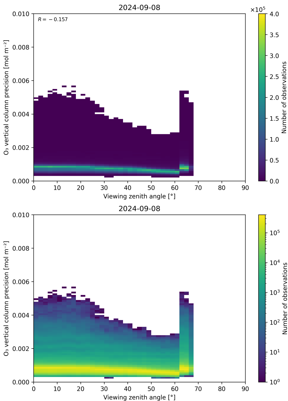
Figure 53: Scatter density plot of “Viewing zenith angle” against “O 3 vertical column precision” for 2024-09-07 to 2024-09-09.
