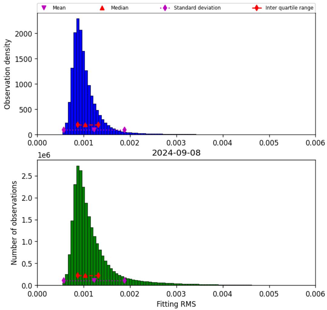
Figure 23: Histogram of “Fitting RMS” for 2024-09-07 to 2024-09-09
