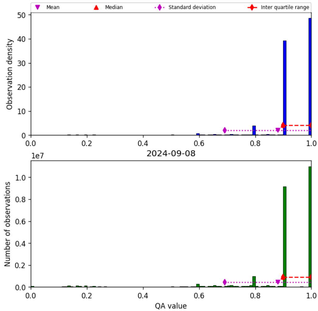
Figure 20: Histogram of “QA value” for 2024-09-07 to 2024-09-09
