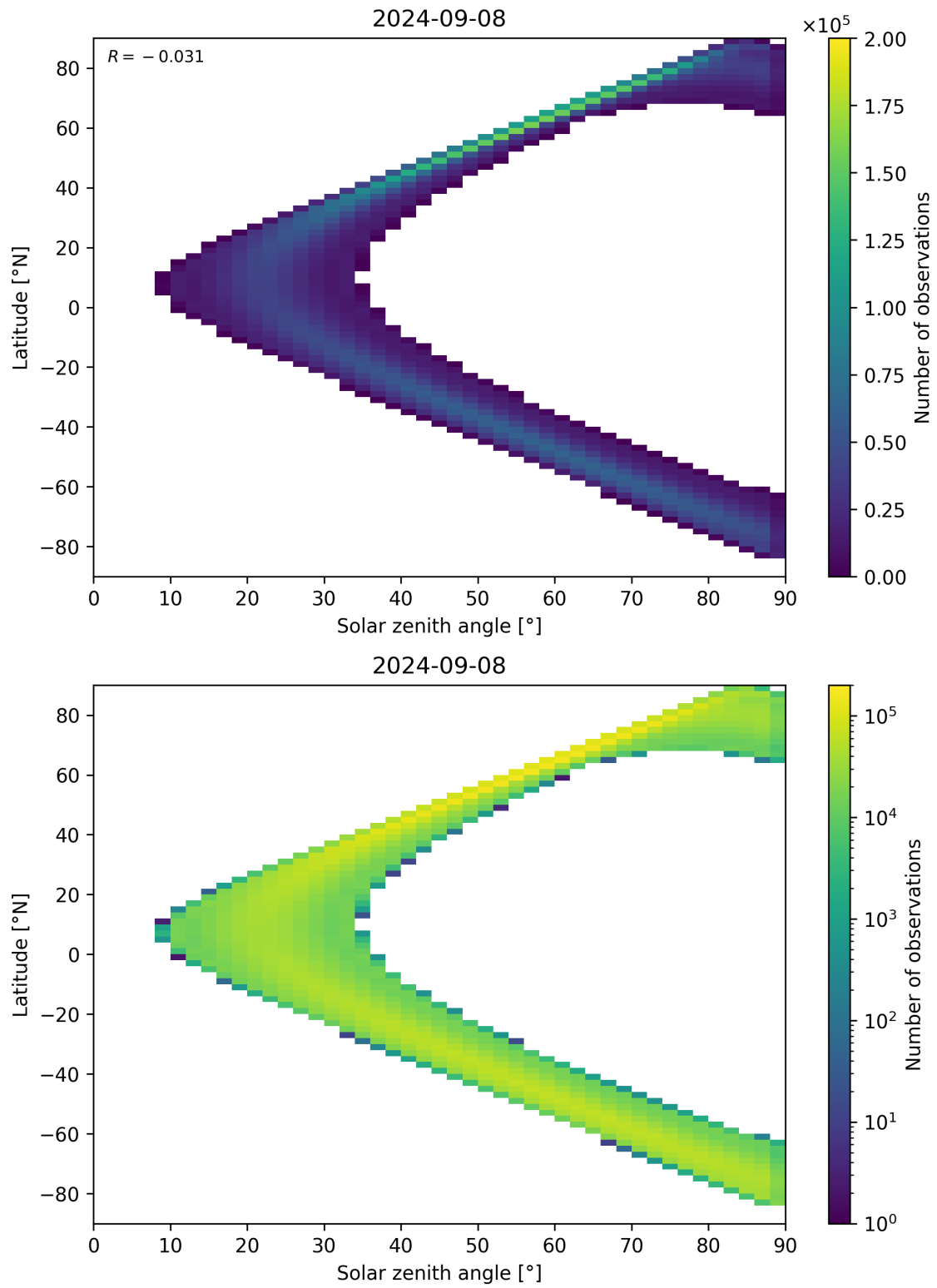
Figure 44: Scatter density plot of “Solar zenith angle” against “Latitude” for 2024-09-07 to 2024-09-09.
