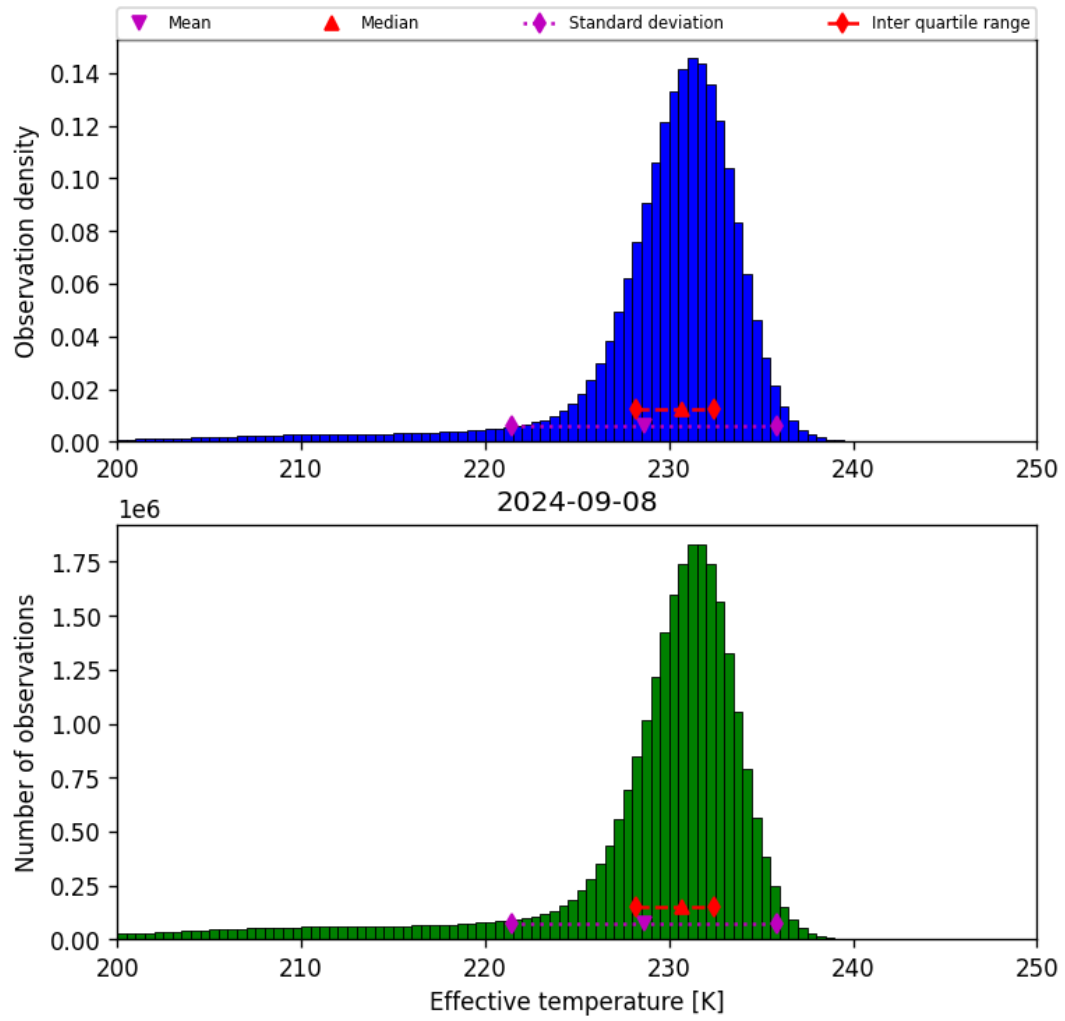
Figure 24: Histogram of “Effective temperature” for 2024-09-07 to 2024-09-09
