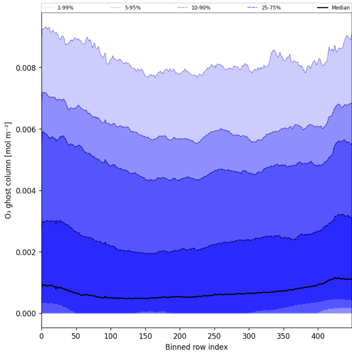
Figure 32: Along track statistics of “O 3 ghost column” for 2024-09-07 to 2024-09-09
