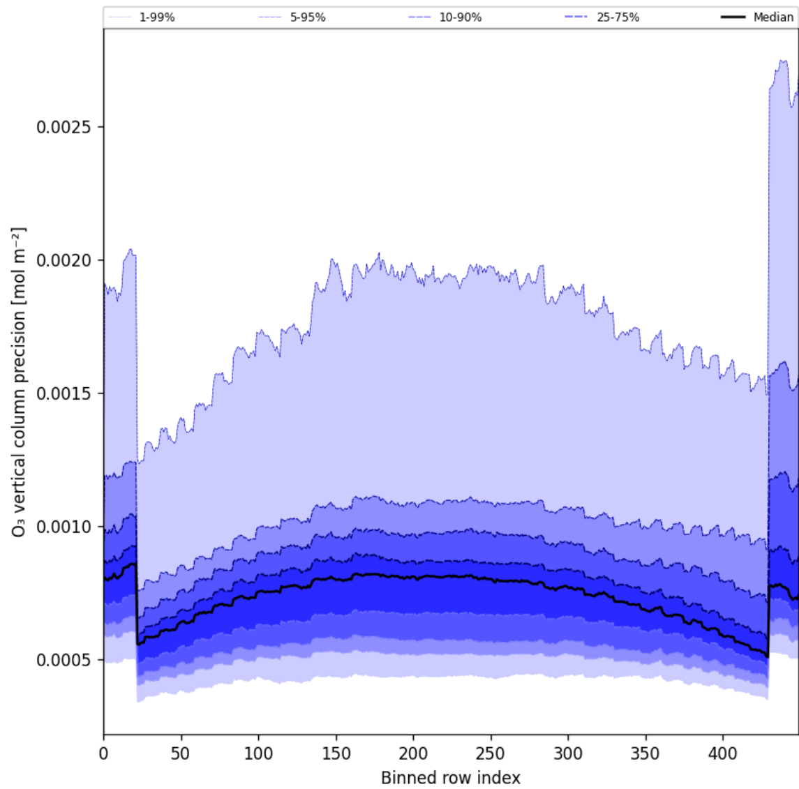
Figure 29: Along track statistics of “O 3 vertical column precision” for 2024-09-07 to 2024-09-09
