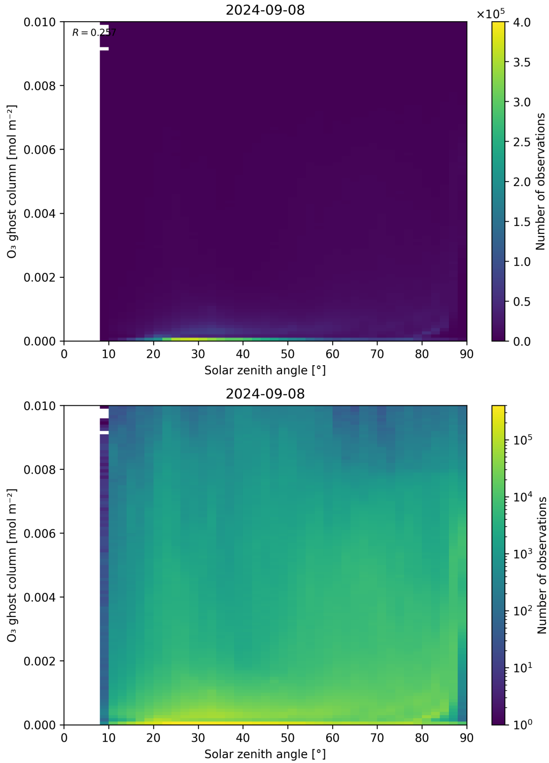
Figure 46: Scatter density plot of “Solar zenith angle” against “O 3 ghost column” for 2024-09-07 to 2024-09-09.
