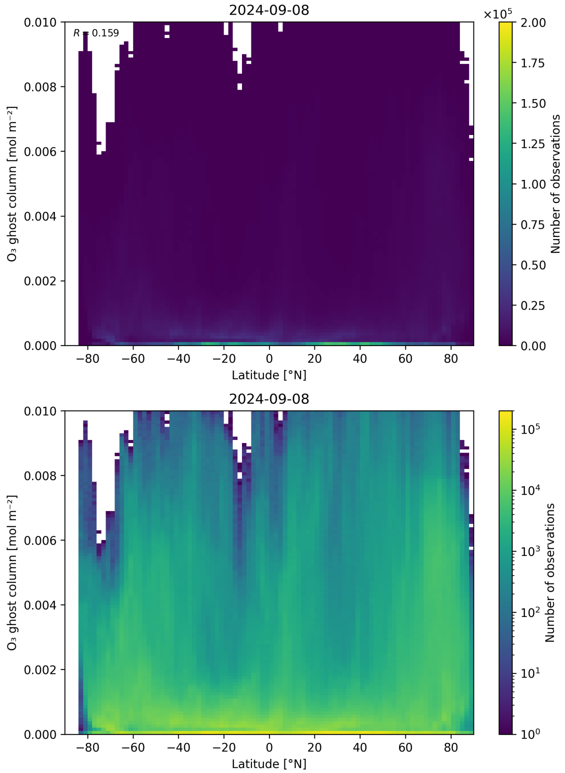
Figure 35: Scatter density plot of “Latitude” against “O 3 ghost column” for 2024-09-07 to 2024-09-09.
