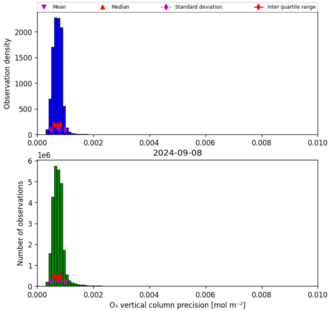
Figure 22: Histogram of “O 3 vertical column precision” for 2024-09-07 to 2024-09-09
