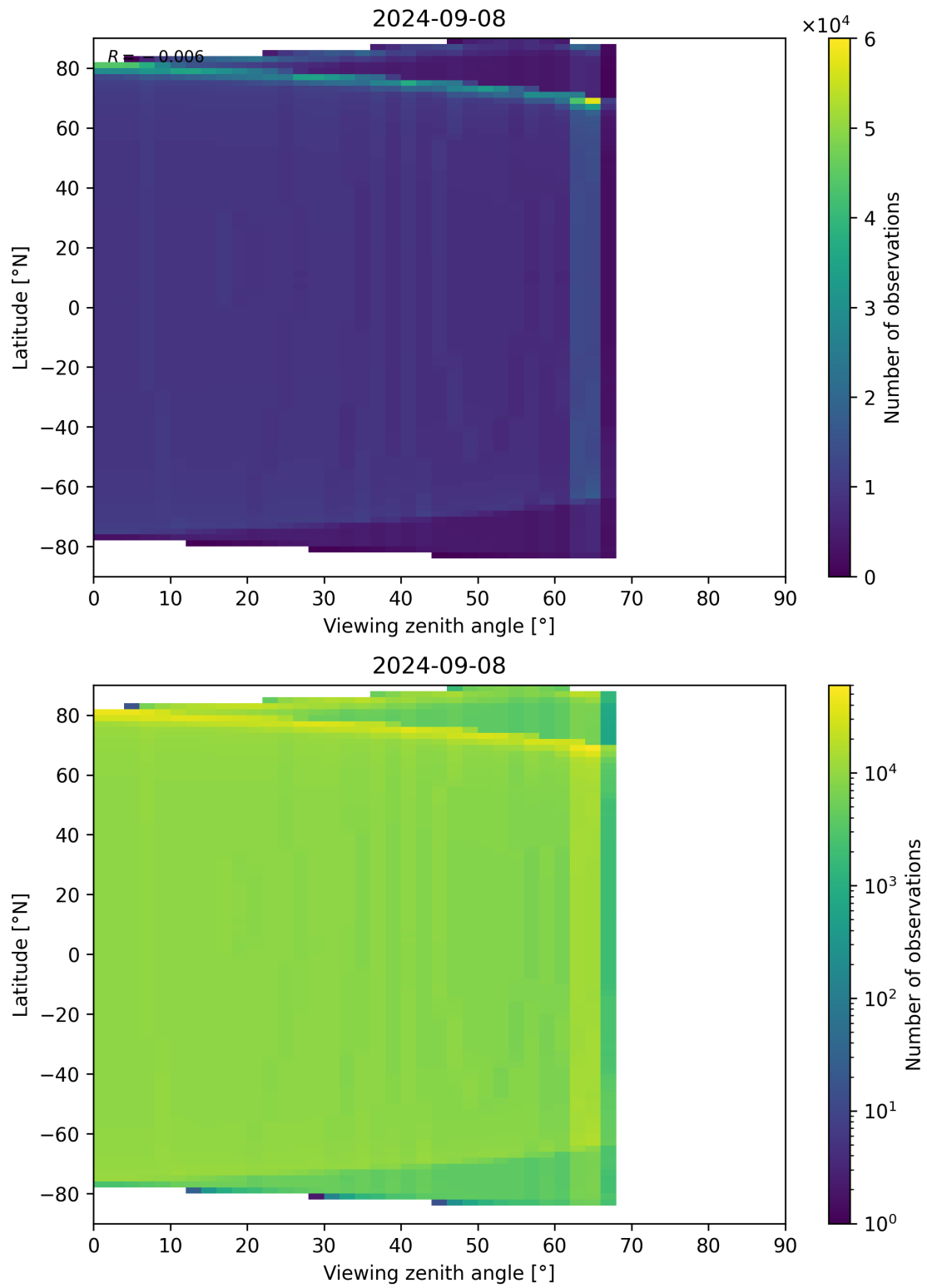
Figure 49: Scatter density plot of “Viewing zenith angle” against “Latitude” for 2024-09-07 to 2024-09-09.
