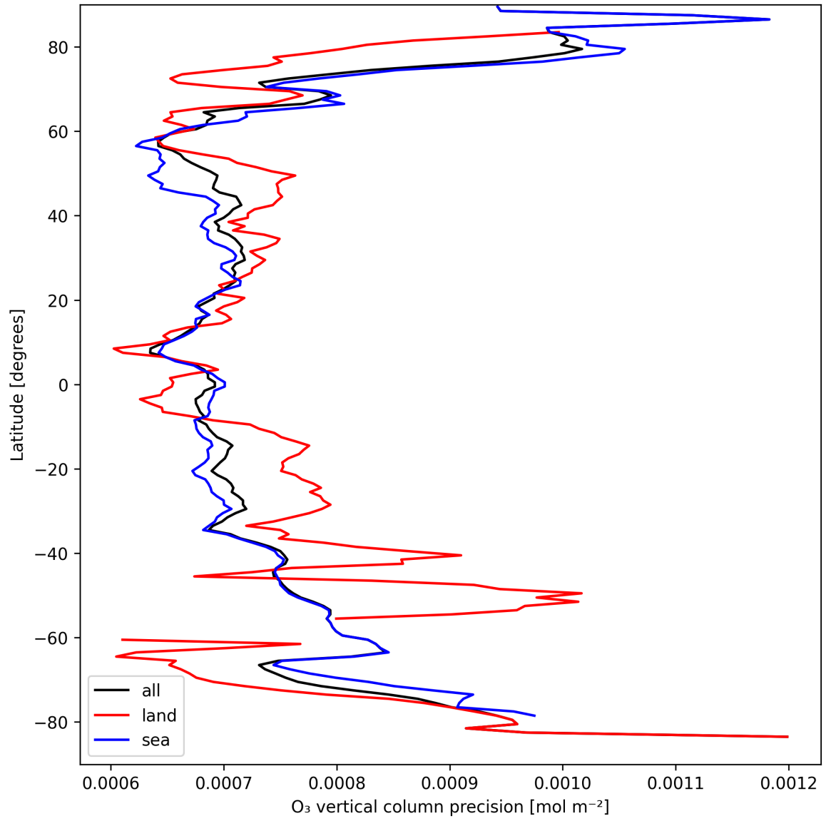
Figure 15: Zonal average of “O 3 vertical column precision” for 2024-09-07 to 2024-09-09.
