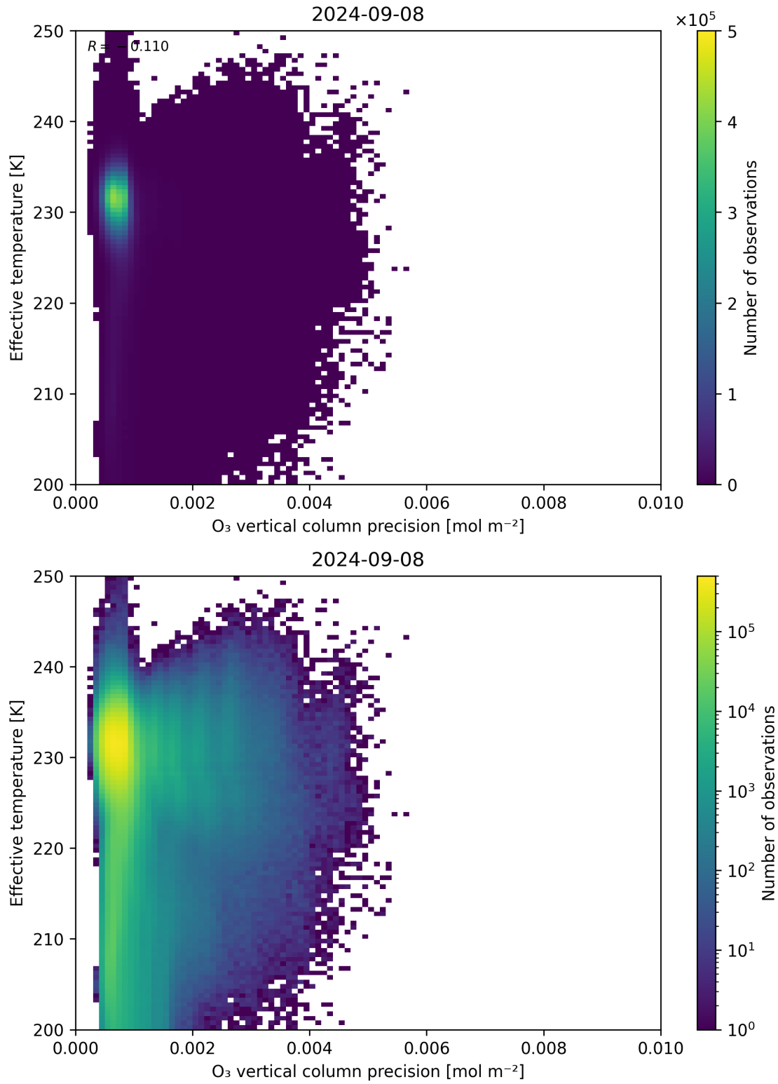
Figure 42: Scatter density plot of “O 3 vertical column precision” against “Effective temperature” for 2024-09-07 to 2024-09-09.
