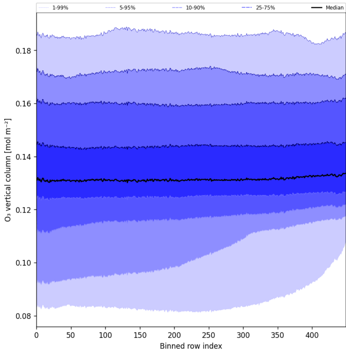
Figure 28: Along track statistics of “O 3 vertical column” for 2024-09-07 to 2024-09-09
