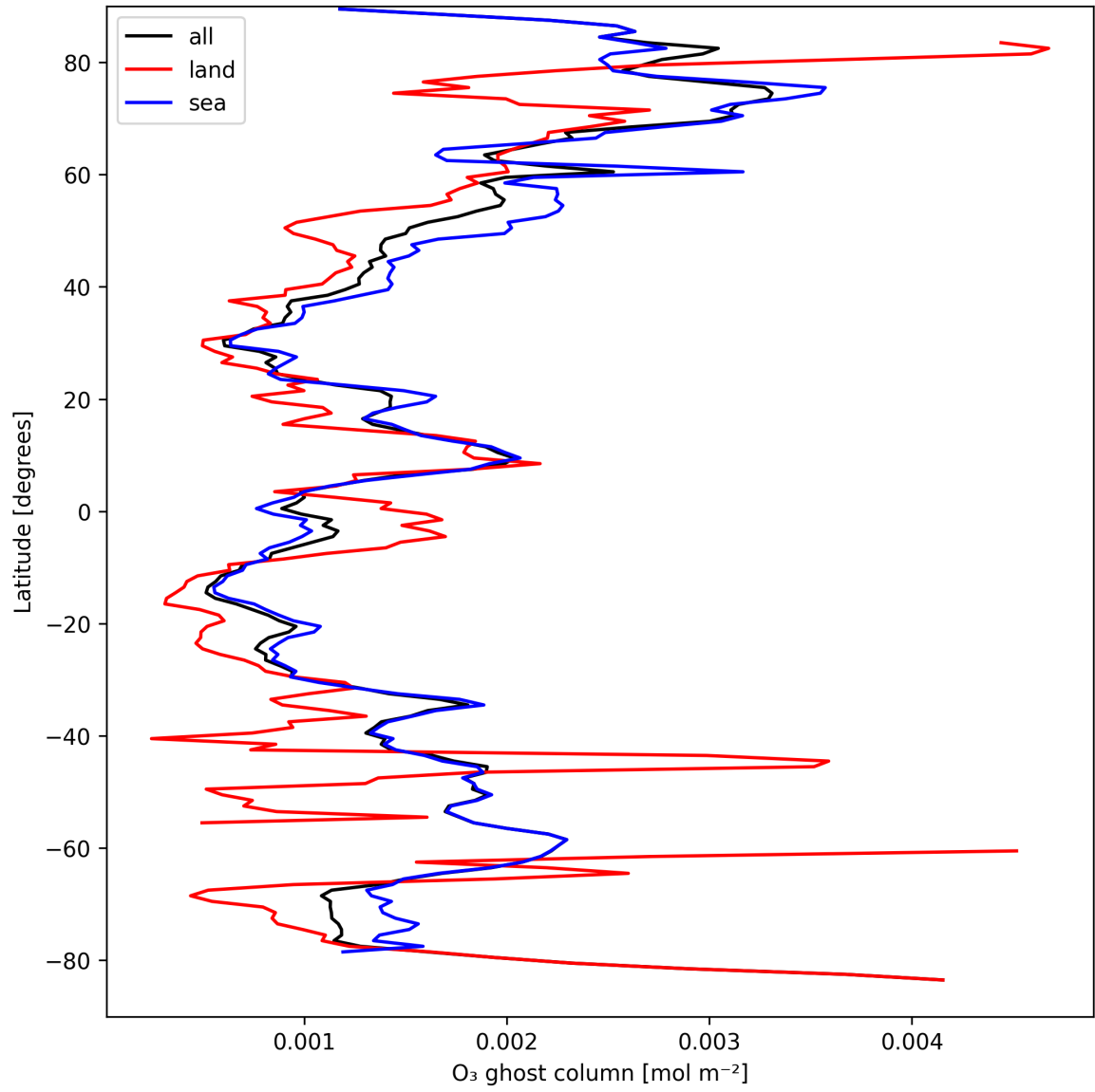
Figure 18: Zonal average of "O 3 ghost column" for 2024-09-07 to 2024-09-09.
