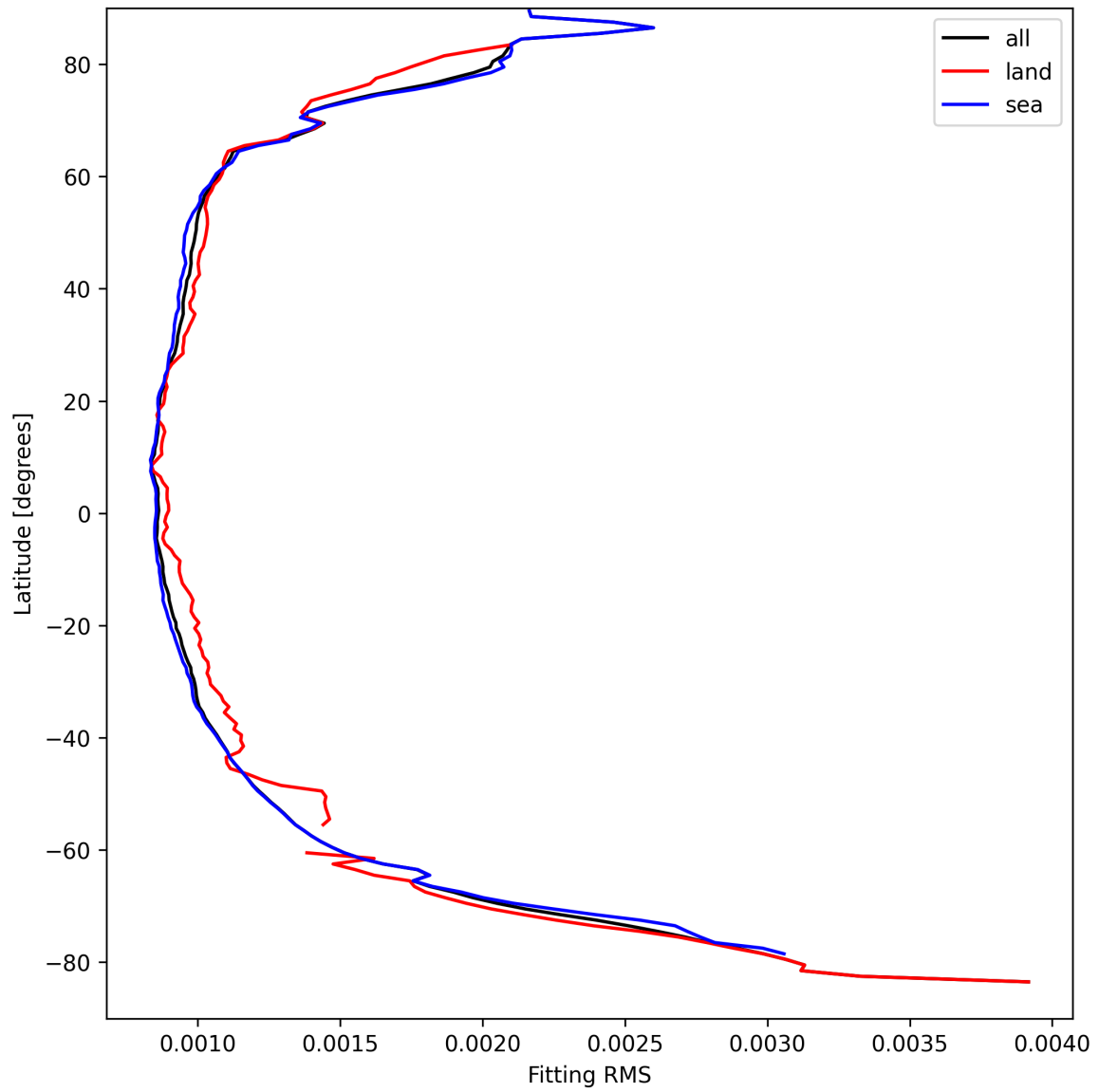
Figure 16: Zonal average of “Fitting RMS” for 2024-09-07 to 2024-09-09.
