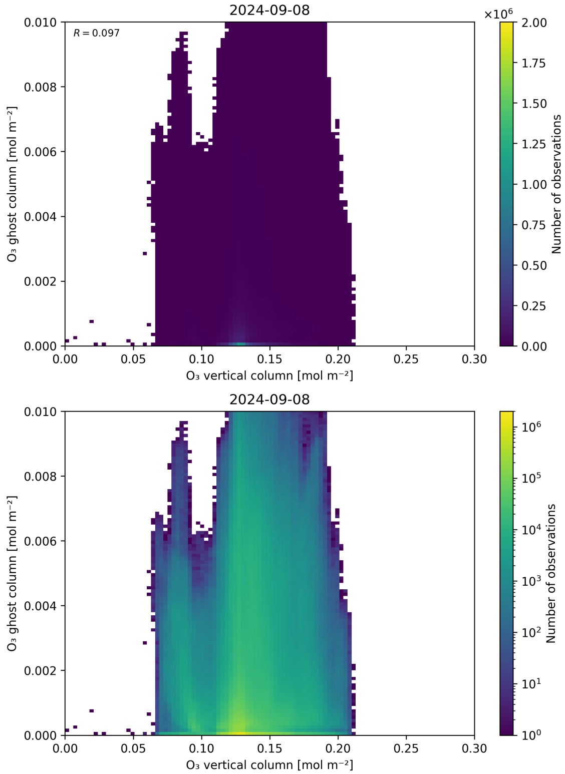
Figure 40: Scatter density plot of “O 3 vertical column” against “O 3 ghost column” for 2024-09-07 to 2024-09-09.
