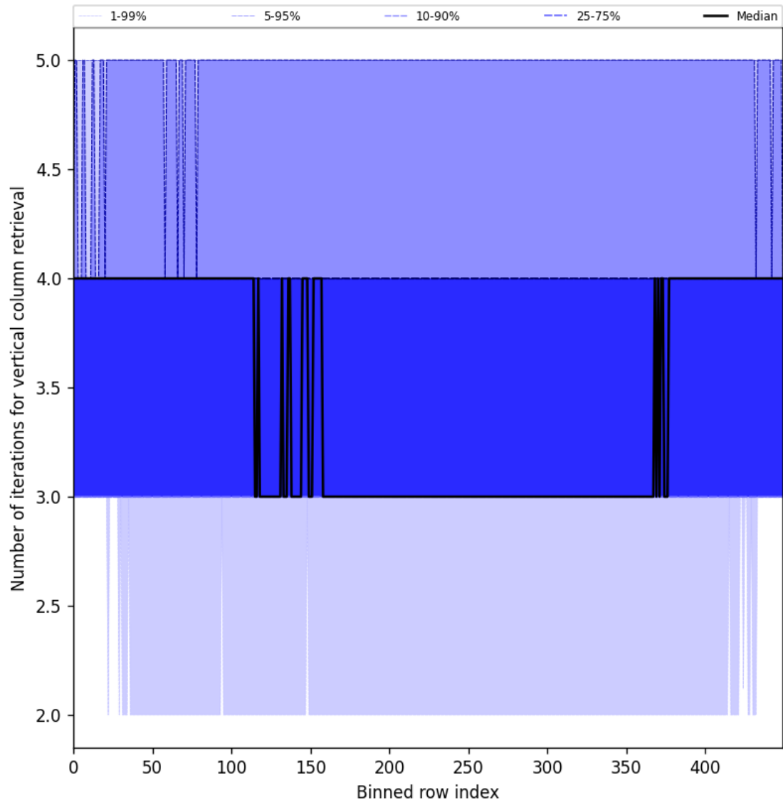
Figure 33: Along track statistics of “Number of iterations for vertical column retrieval” for 2024-09-07 to 2024-09-09
