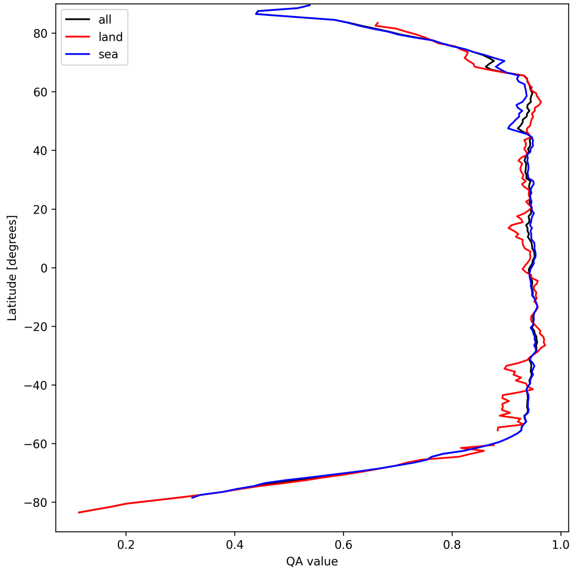
Figure 13: Zonal average of “QA value” for 2024-09-07 to 2024-09-09.
