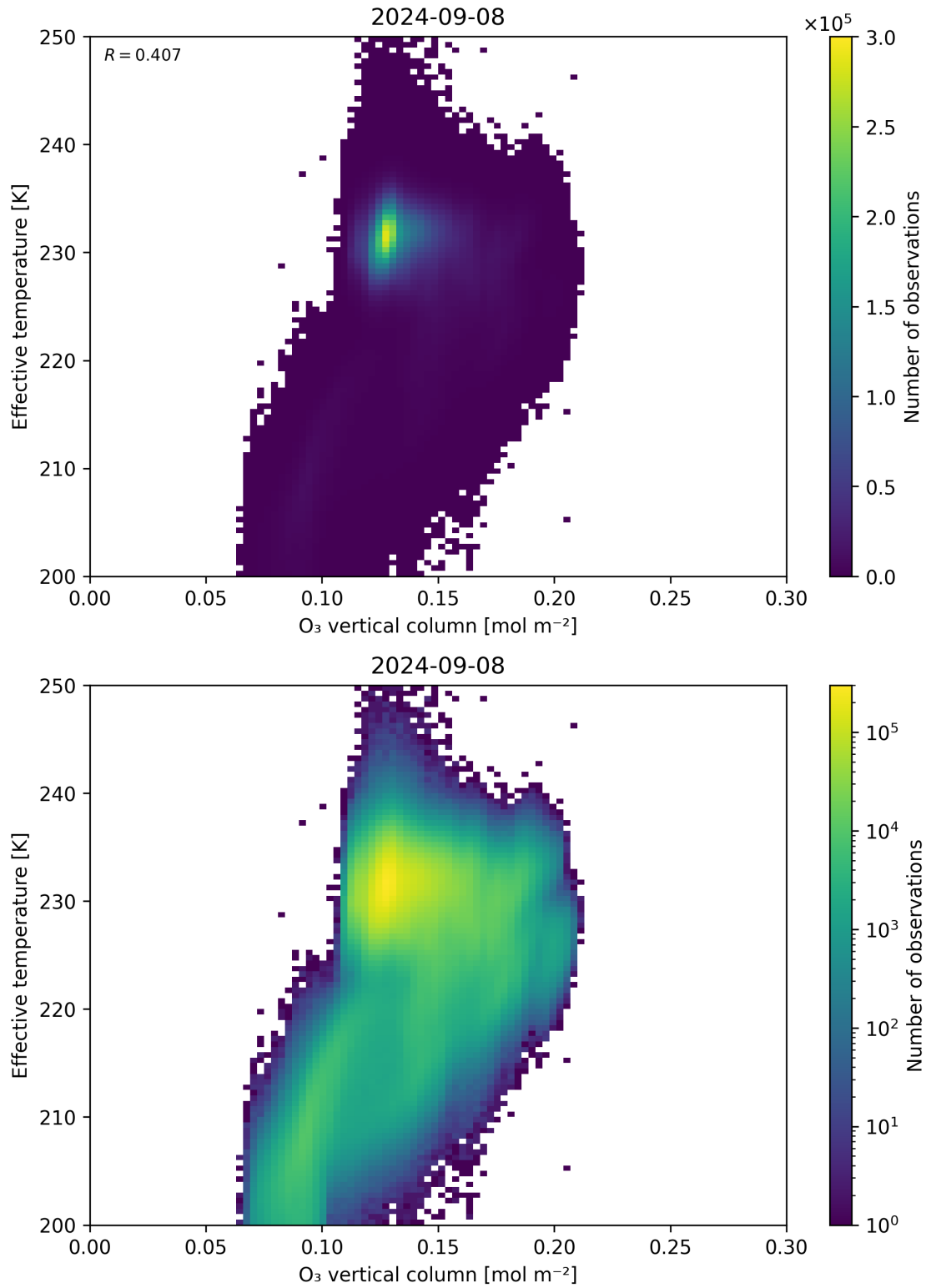
Figure 39: Scatter density plot of “O 3 vertical column” against “Effective temperature” for 2024-09-07 to 2024-09-09.
