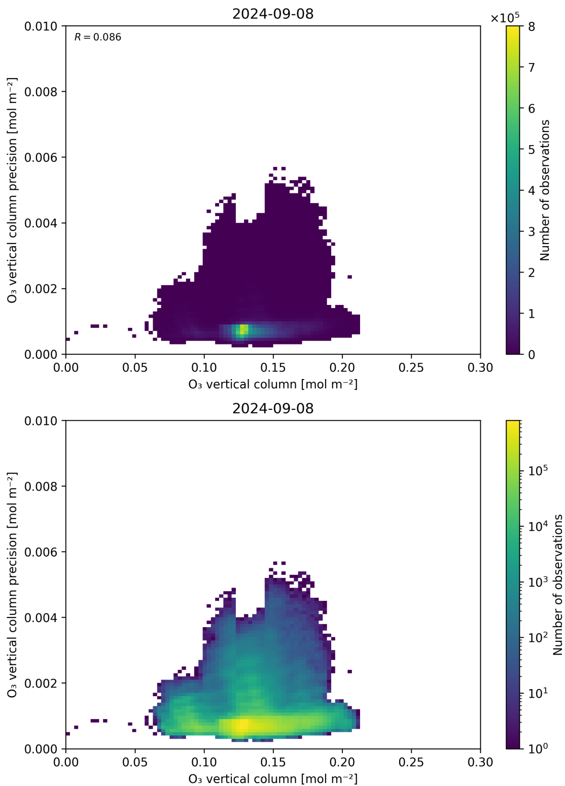
Figure 41: Scatter density plot of “O 3 vertical column” against “O 3 vertical column precision” for 2024-09-07 to 2024-09-09.
