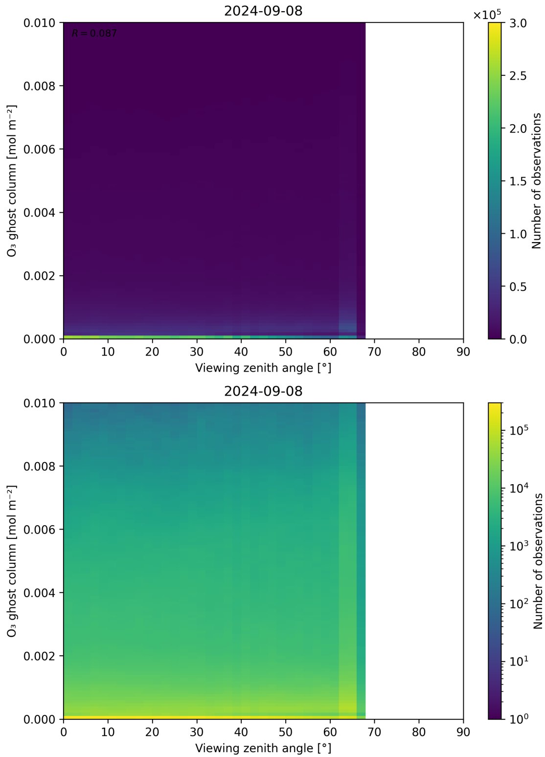
Figure 51: Scatter density plot of “Viewing zenith angle” against “O 3 ghost column” for 2024-09-07 to 2024-09-09.
