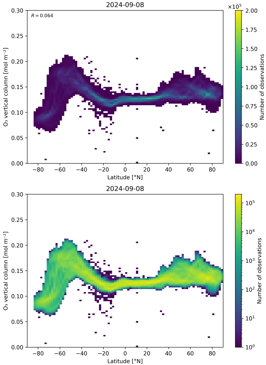
Figure 36: Scatter density plot of “Latitude” against “O 3 vertical column” for 2024-09-07 to 2024-09-09.
