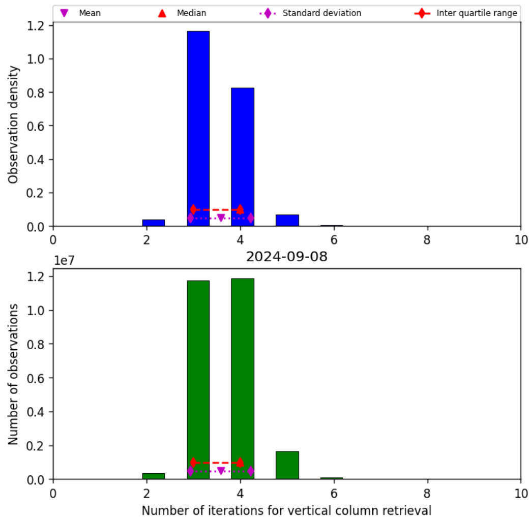
Figure 26: Histogram of “Number of iterations for vertical column retrieval” for 2024-09-07 to 2024-09-09
