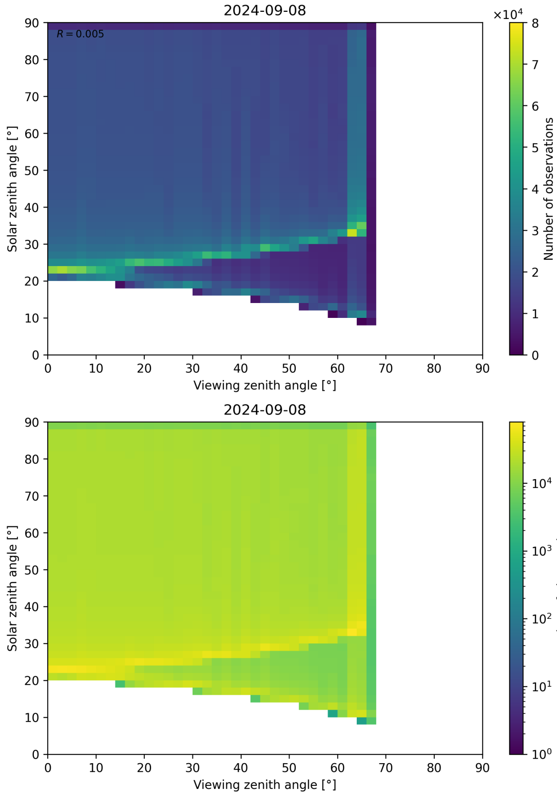
Figure 54: Scatter density plot of “Viewing zenith angle” against “Solar zenith angle” for 2024-09-07 to 2024-09-09.
