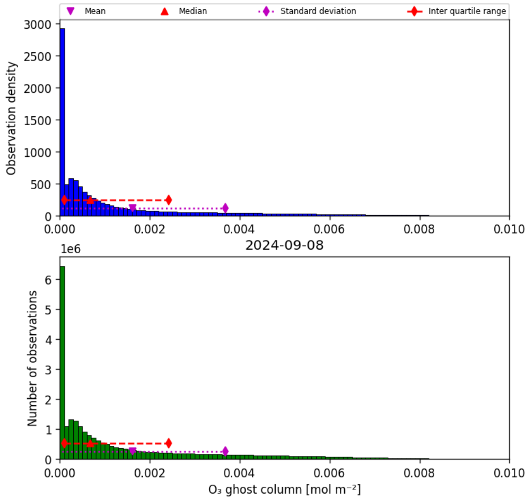
Figure 25: Histogram of “O 3 ghost column” for 2024-09-07 to 2024-09-09
