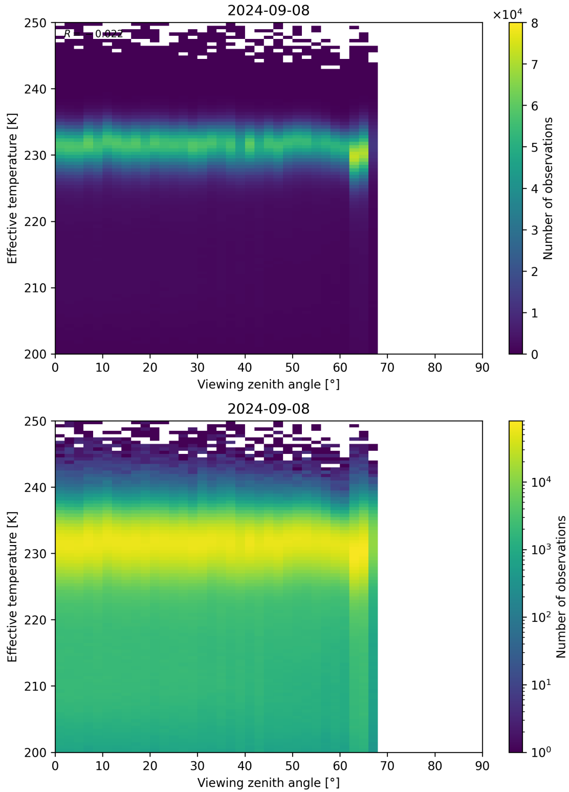
Figure 50: Scatter density plot of “Viewing zenith angle” against “Effective temperature” for 2024-09-07 to 2024-09-09.
