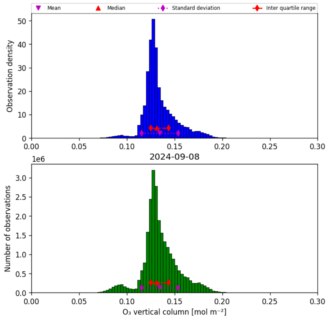
Figure 21: Histogram of “O 3 vertical column” for 2024-09-07 to 2024-09-09
