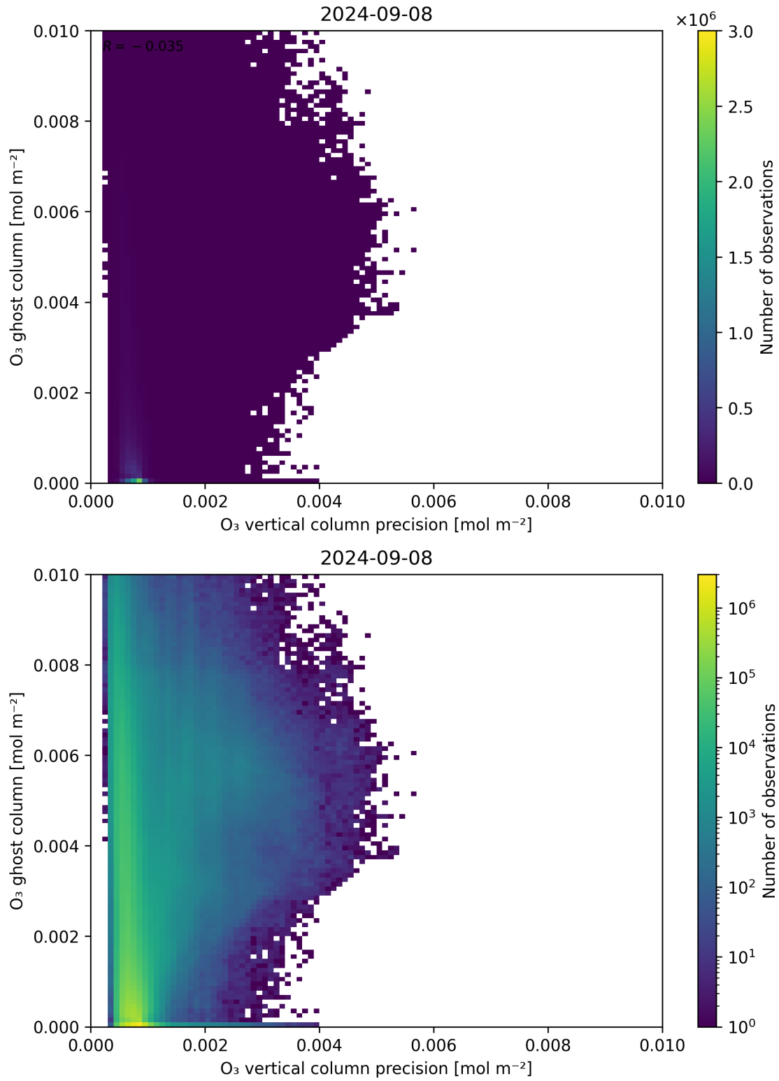
Figure 43: Scatter density plot of “ \text{O}_3 vertical column precision” against “ \text{O}_3 ghost column” for 2024-09-07 to 2024-09-09.
