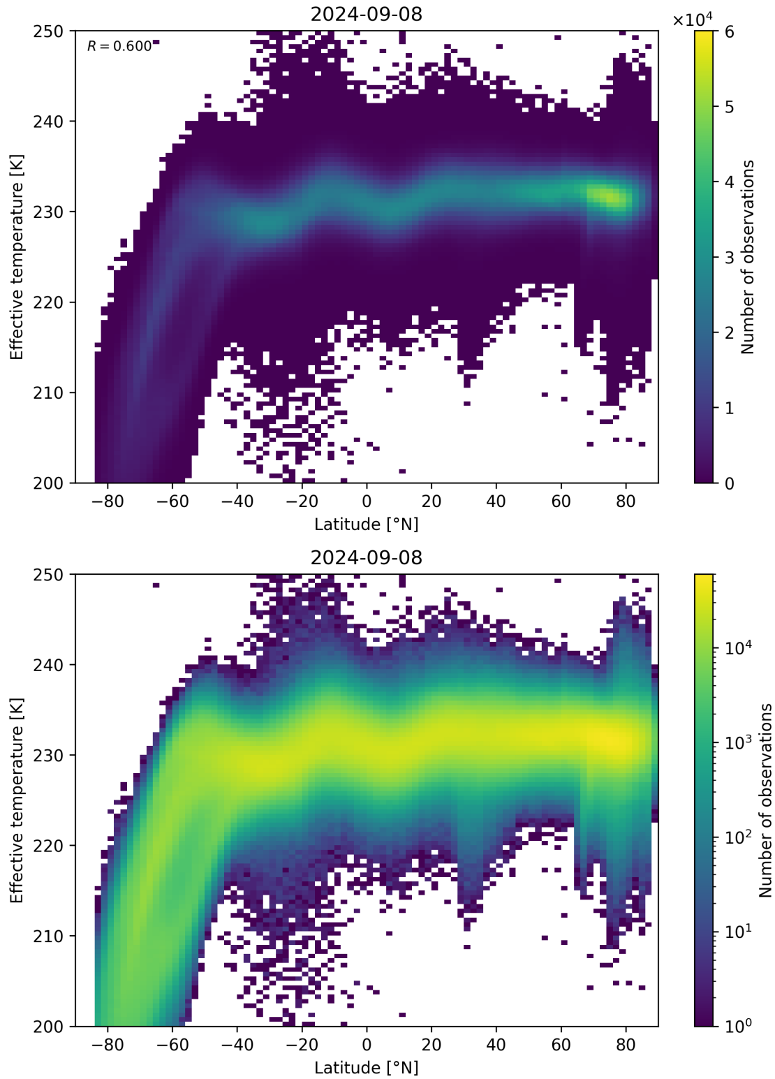
Figure 34: Scatter density plot of “Latitude” against “Effective temperature” for 2024-09-07 to 2024-09-09.
