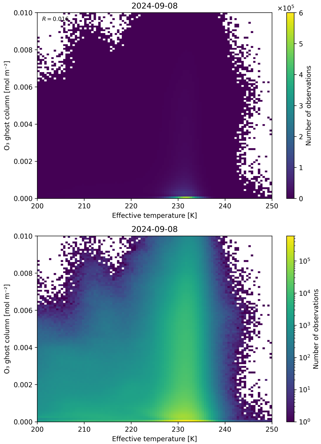
Figure 38: Scatter density plot of “Effective temperature” against “O 3 ghost column” for 2024-09-07 to 2024-09-09.
