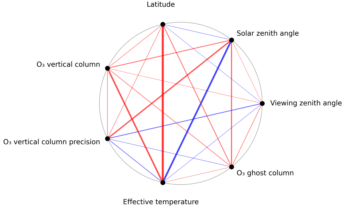
Figure 1: Map of correlation graph for 2024-09-07 to 2024-09-09.
