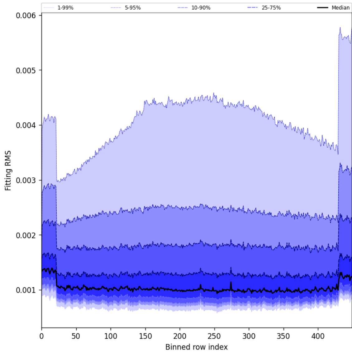
Figure 30: Along track statistics of “Fitting RMS” for 2024-09-07 to 2024-09-09
