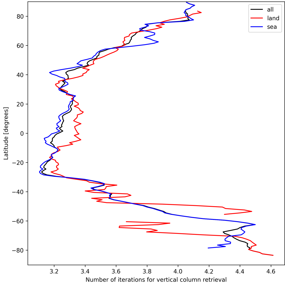
Figure 19: Zonal average of “Number of iterations for vertical column retrieval” for 2024-09-07 to 2024-09-09.
