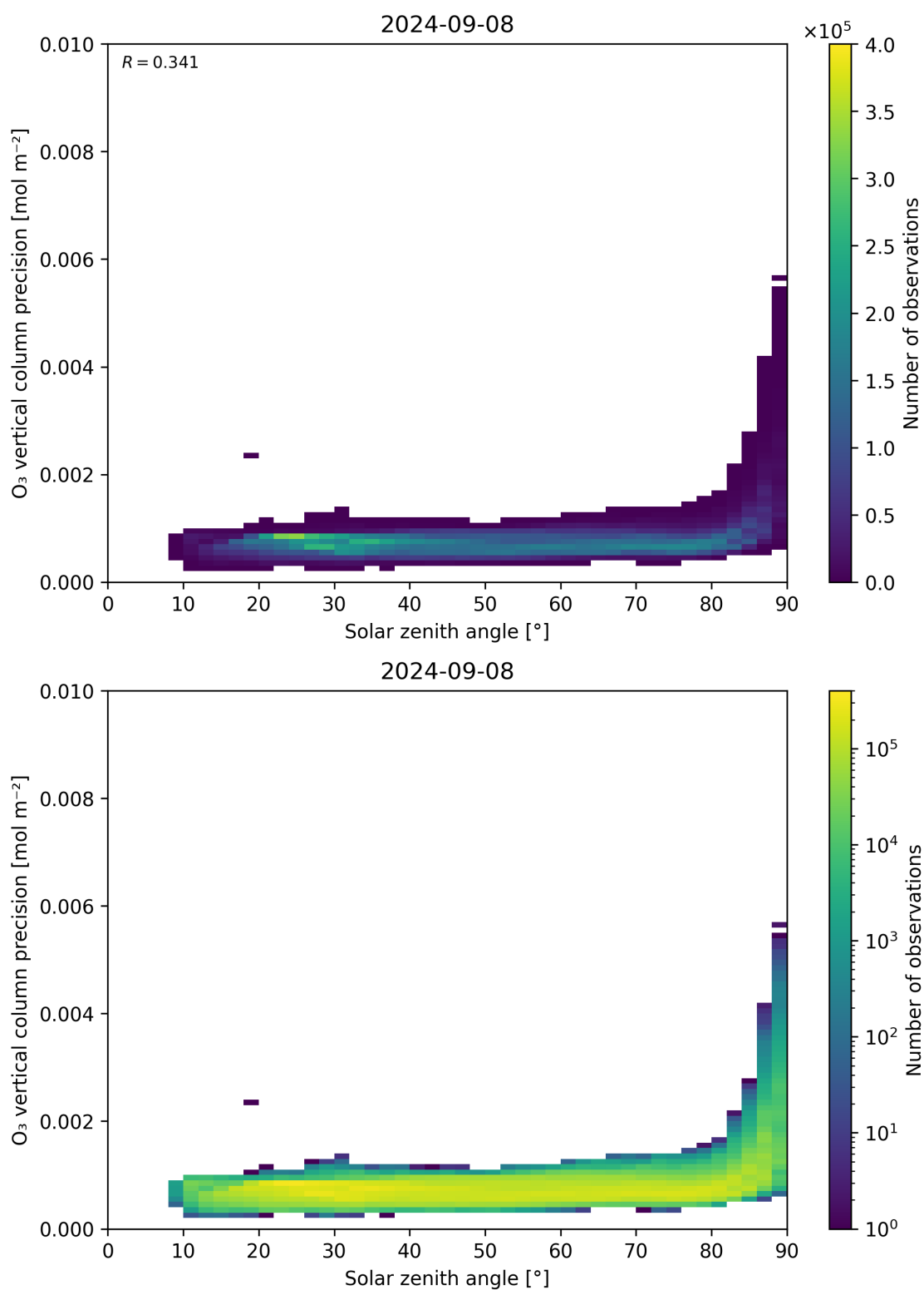
Figure 48: Scatter density plot of “Solar zenith angle” against “O 3 vertical column precision” for 2024-09-07 to 2024-09-09.
