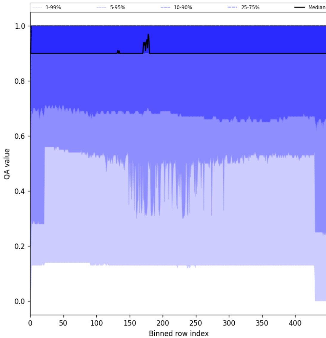
Figure 27: Along track statistics of “QA value” for 2024-09-07 to 2024-09-09
