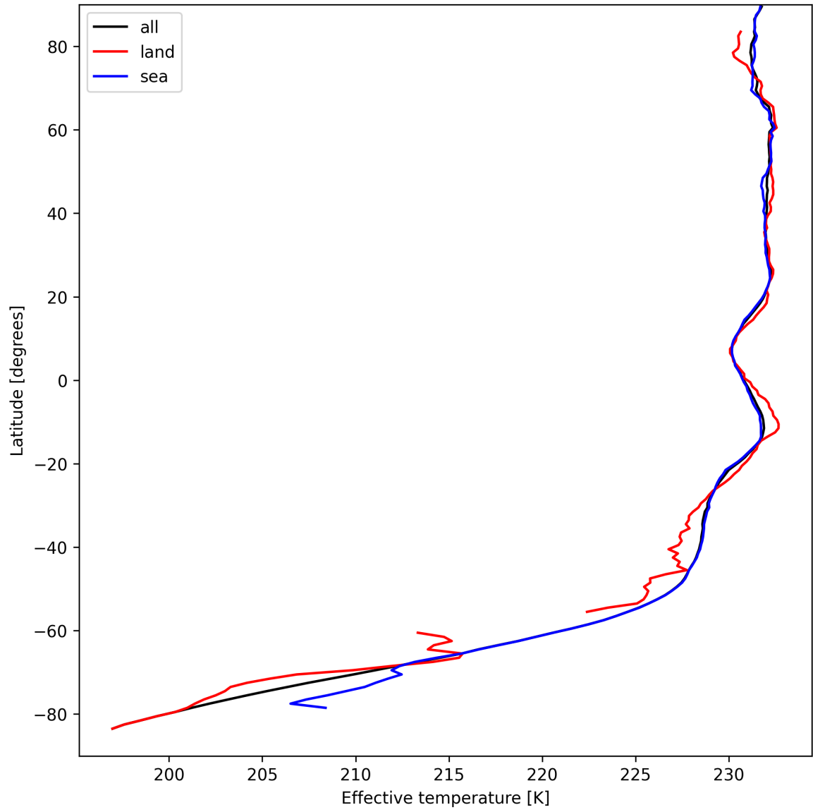
Figure 17: Zonal average of "Effective temperature" for 2024-09-07 to 2024-09-09.
