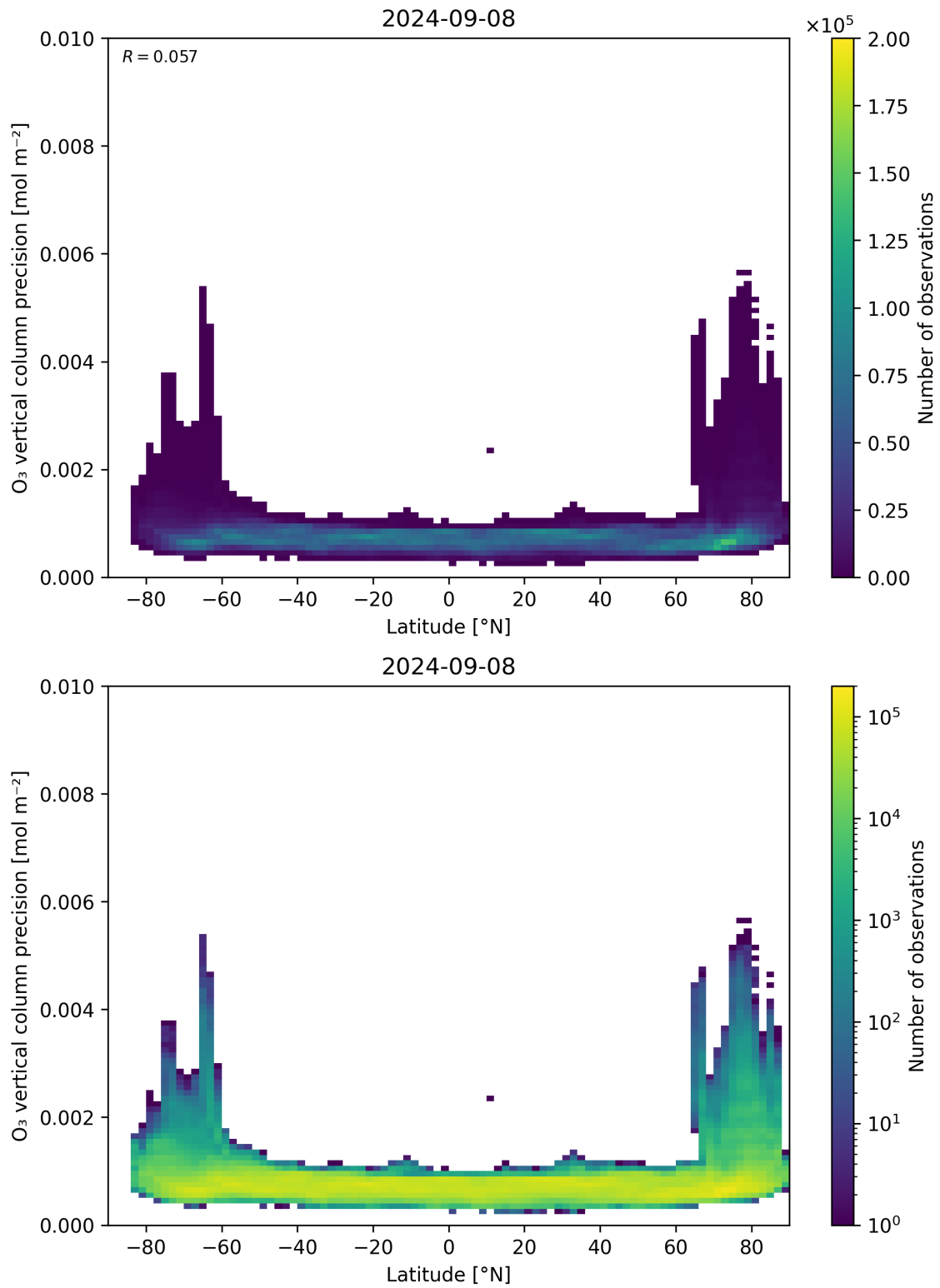
Figure 37: Scatter density plot of “Latitude” against “O 3 vertical column precision” for 2024-09-07 to 2024-09-09.
