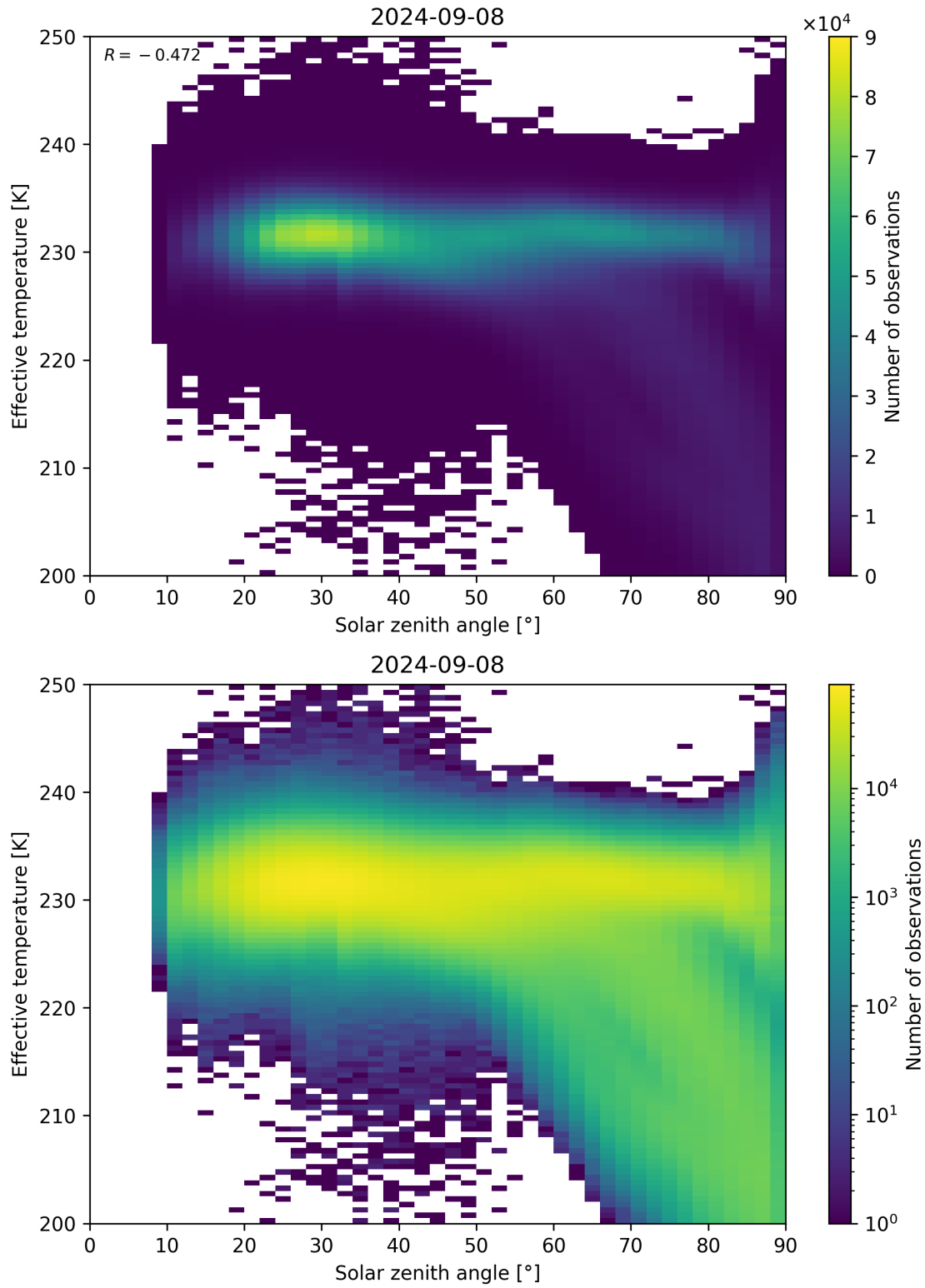
Figure 45: Scatter density plot of “Solar zenith angle” against “Effective temperature” for 2024-09-07 to 2024-09-09.
