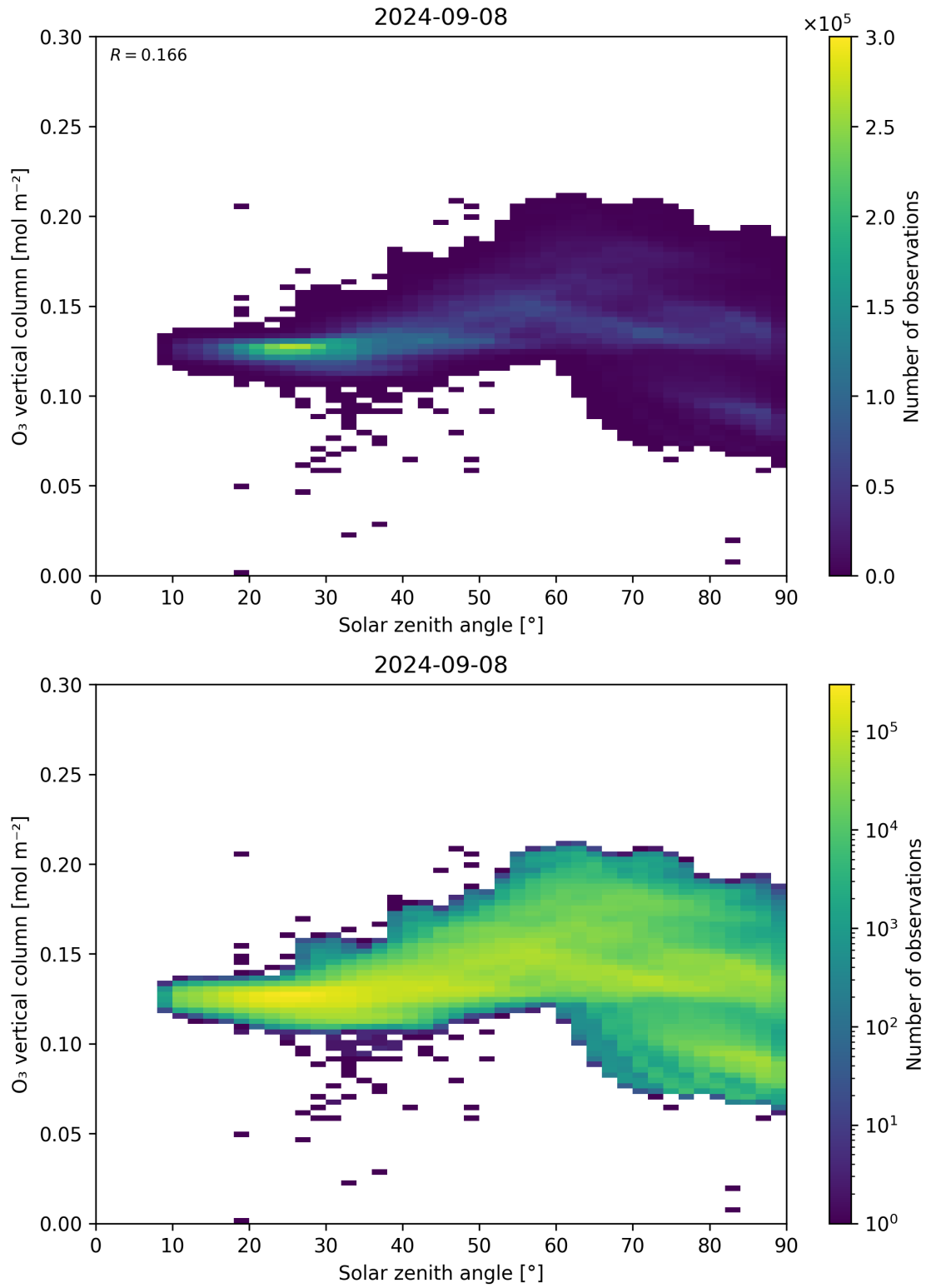
Figure 47: Scatter density plot of “Solar zenith angle” against “O 3 vertical column” for 2024-09-07 to 2024-09-09.
