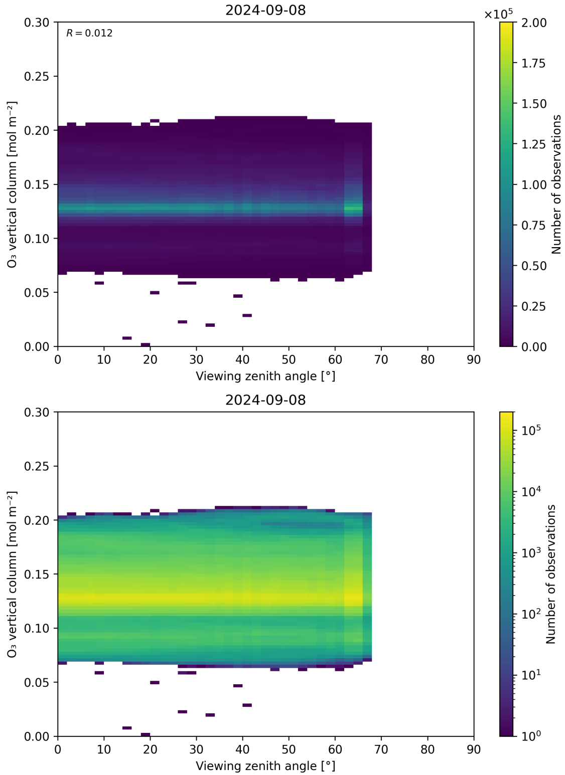
Figure 52: Scatter density plot of “Viewing zenith angle” against “O 3 vertical column” for 2024-09-07 to 2024-09-09.
