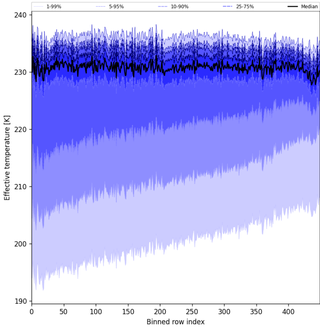
Figure 31: Along track statistics of “Effective temperature” for 2024-09-07 to 2024-09-09
