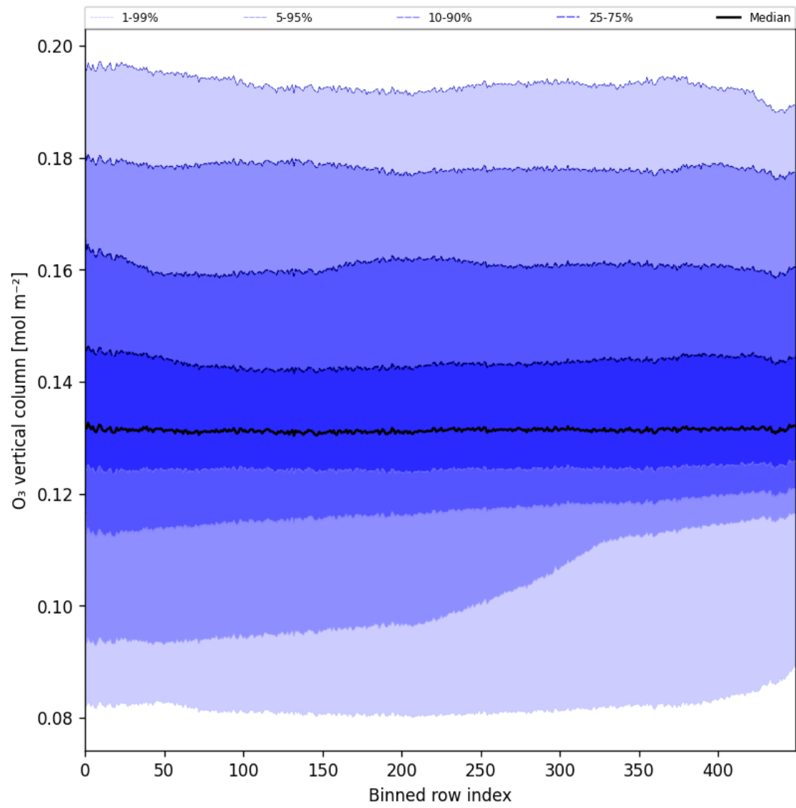
Figure 28: Along track statistics of “O 3 vertical column” for 2024-09-09 to 2024-09-11
