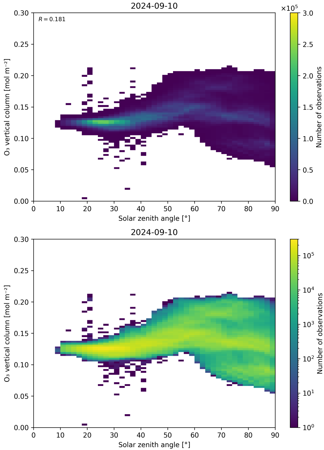
Figure 47: Scatter density plot of “Solar zenith angle” against “O 3 vertical column” for 2024-09-09 to 2024-09-11.
