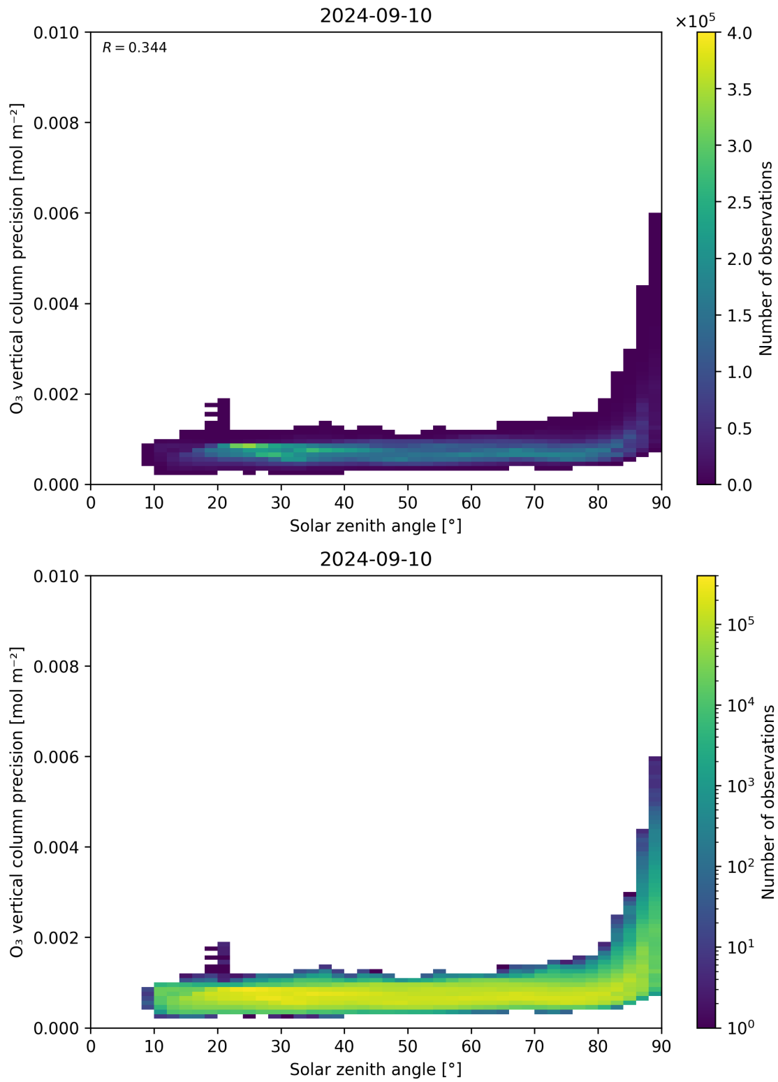
Figure 48: Scatter density plot of “Solar zenith angle” against “O 3 vertical column precision” for 2024-09-09 to 2024-09-11.
