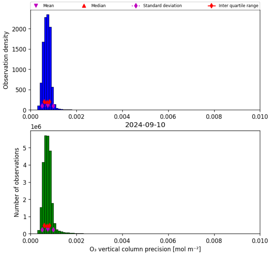
Figure 22: Histogram of “O 3 vertical column precision” for 2024-09-09 to 2024-09-11
