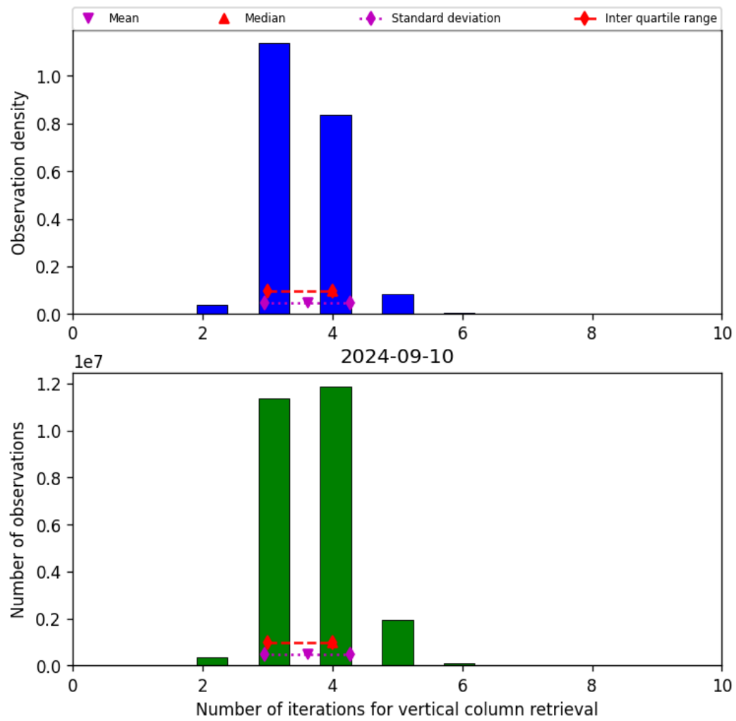
Figure 26: Histogram of “Number of iterations for vertical column retrieval” for 2024-09-09 to 2024-09-11
