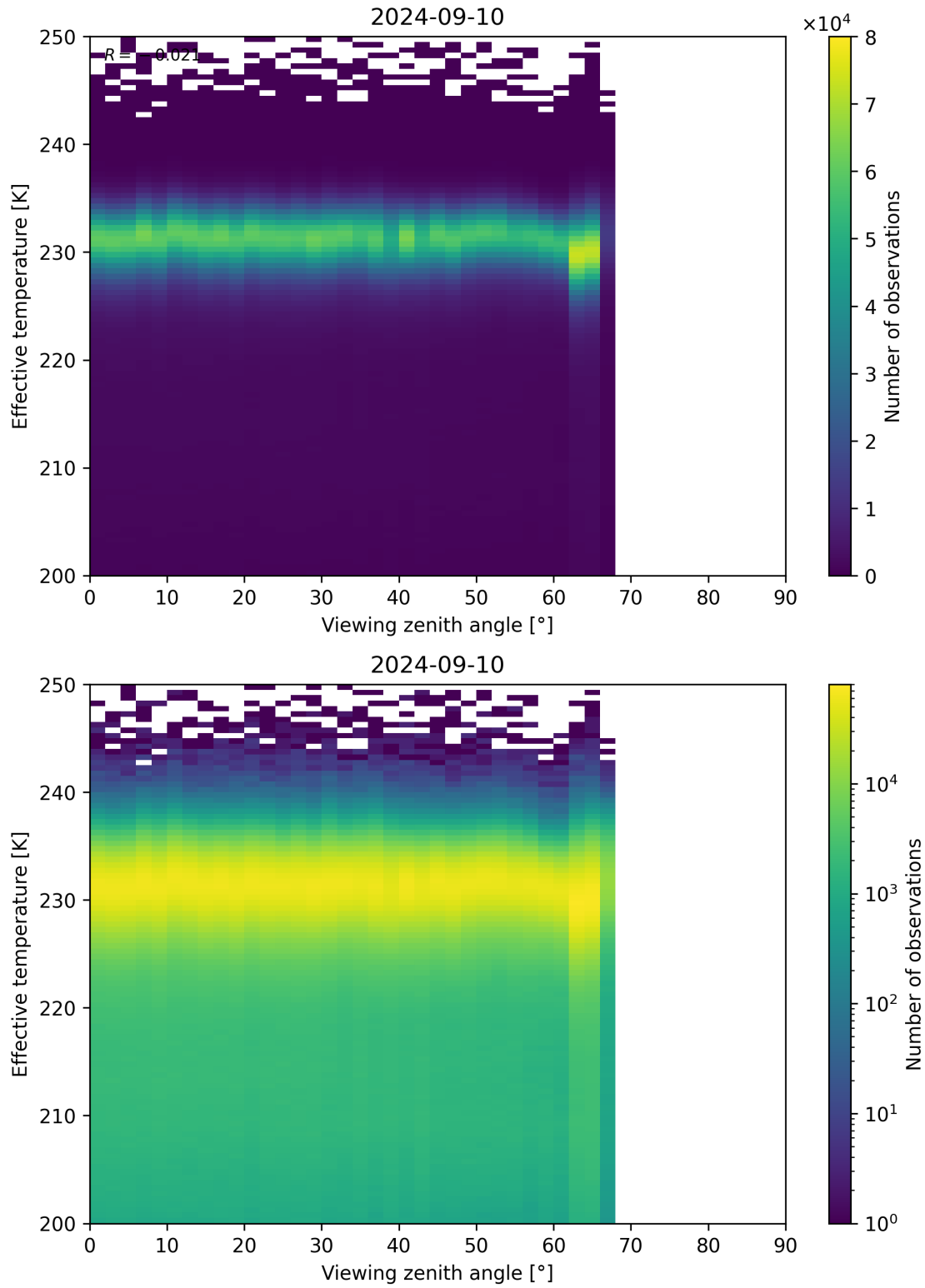
Figure 50: Scatter density plot of “Viewing zenith angle” against “Effective temperature” for 2024-09-09 to 2024-09-11.
