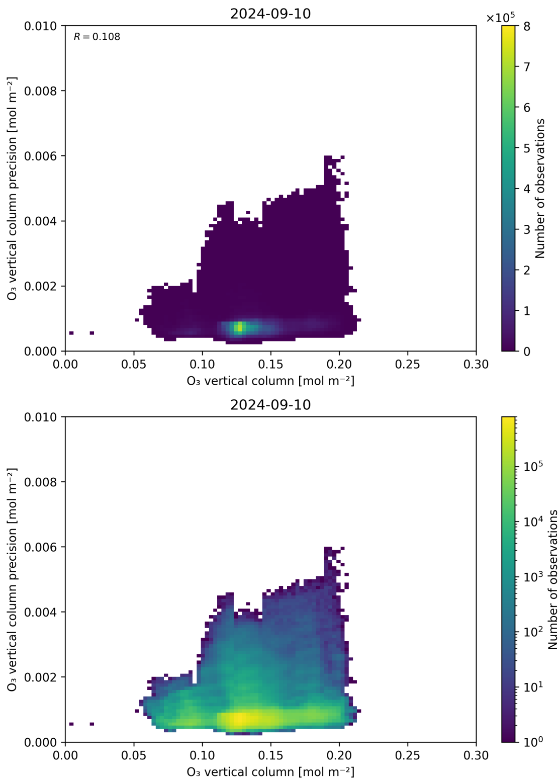
Figure 41: Scatter density plot of “O 3 vertical column” against “O 3 vertical column precision” for 2024-09-09 to 2024-09-11.
