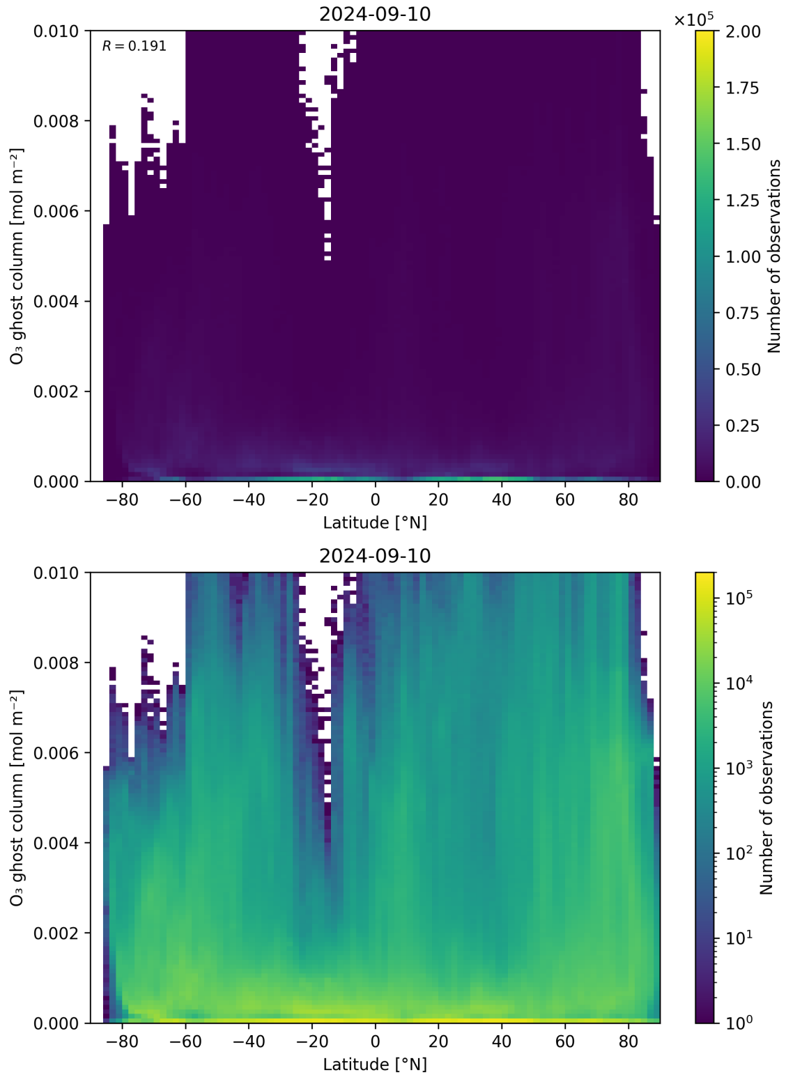
Figure 35: Scatter density plot of “Latitude” against “O 3 ghost column” for 2024-09-09 to 2024-09-11.
