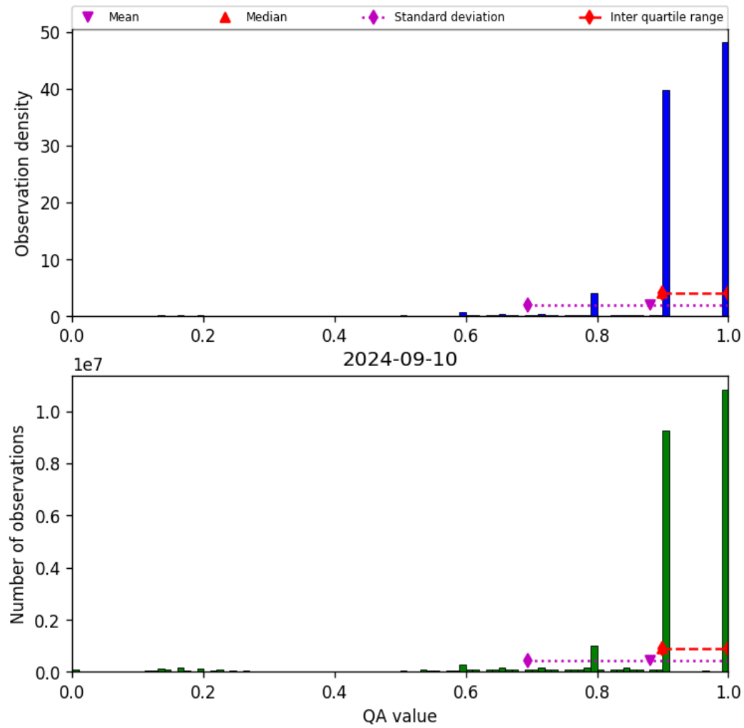
Figure 20: Histogram of “QA value” for 2024-09-09 to 2024-09-11
