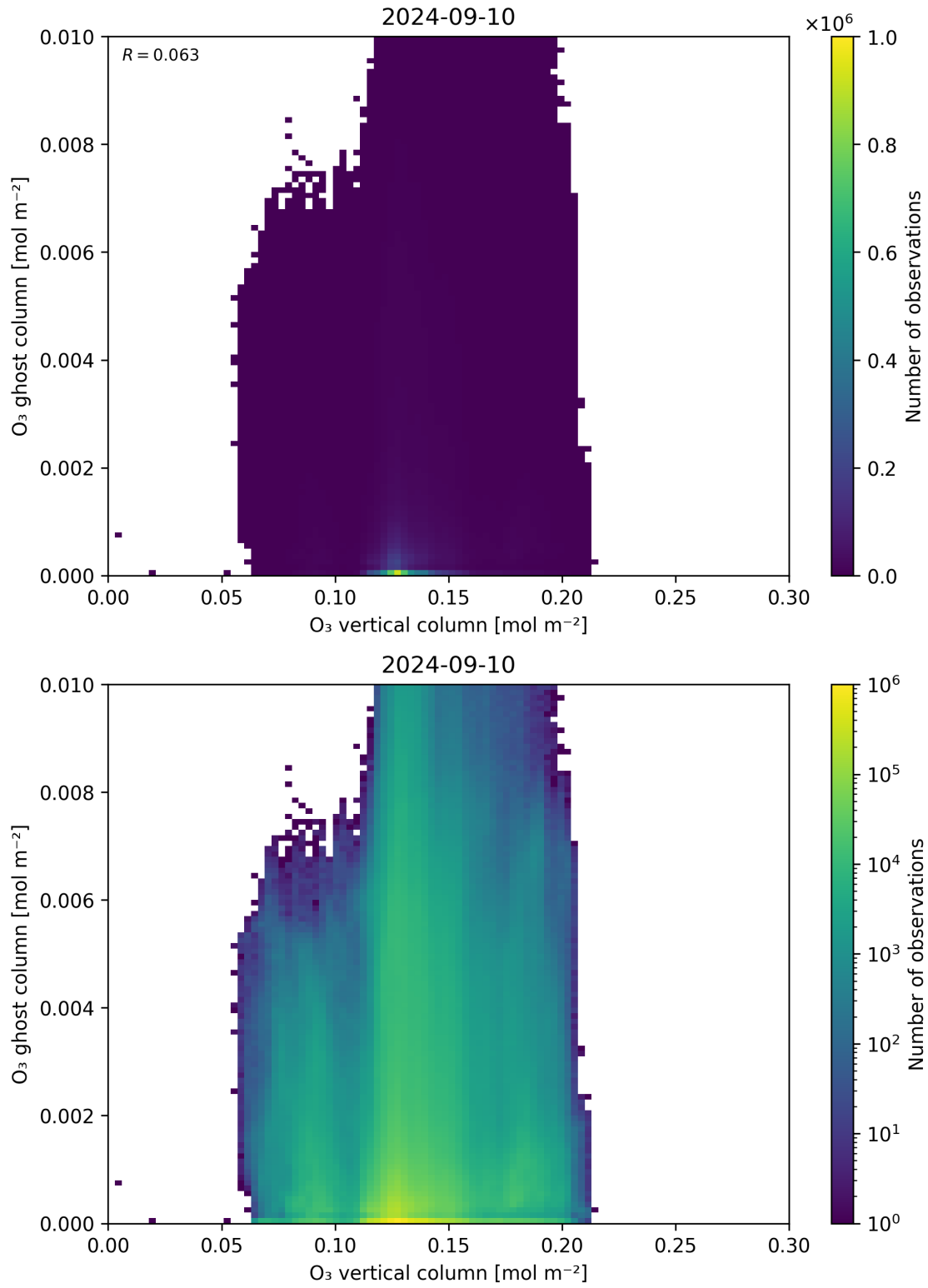
Figure 40: Scatter density plot of “O 3 vertical column” against “O 3 ghost column” for 2024-09-09 to 2024-09-11.
