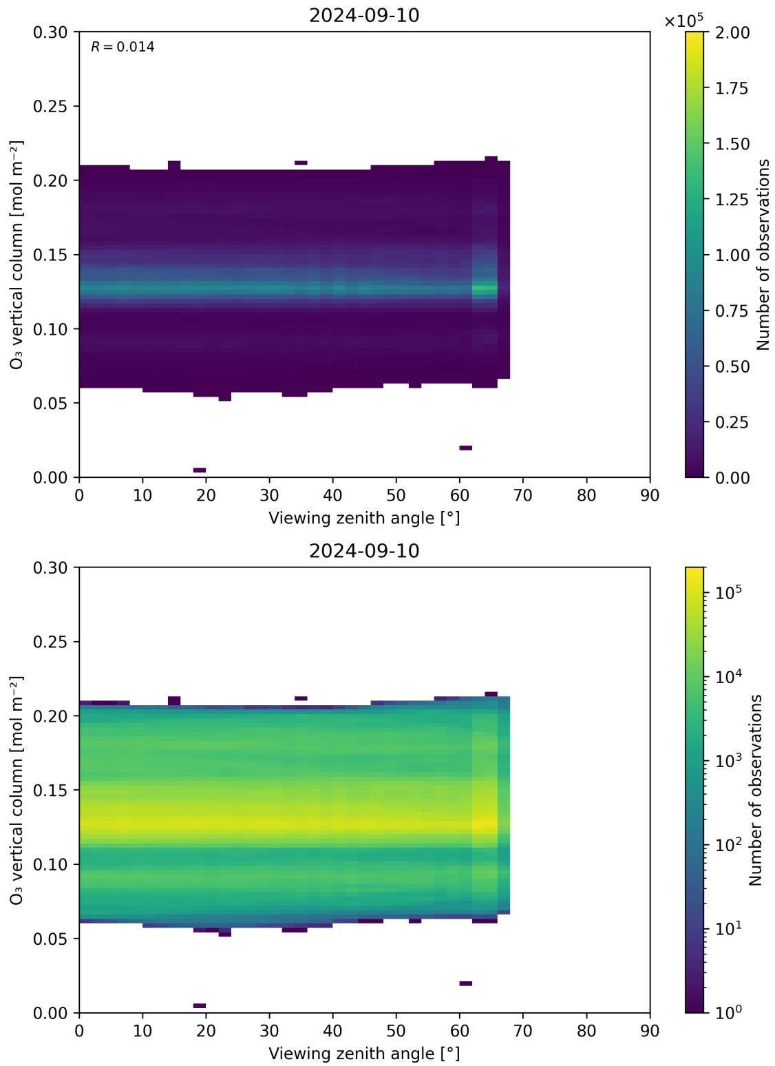
Figure 52: Scatter density plot of “Viewing zenith angle” against “O 3 vertical column” for 2024-09-09 to 2024-09-11.
