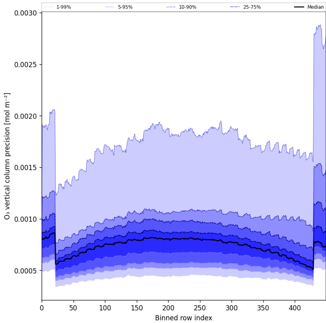
Figure 29: Along track statistics of “O 3 vertical column precision” for 2024-09-09 to 2024-09-11
