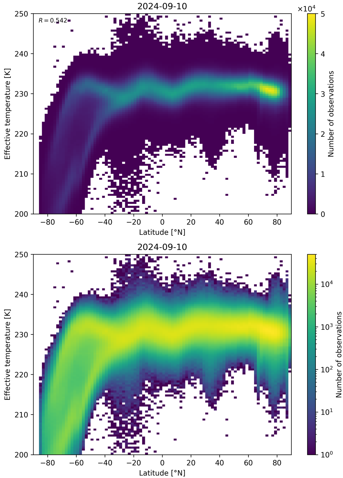
Figure 34: Scatter density plot of “Latitude” against “Effective temperature” for 2024-09-09 to 2024-09-11.
