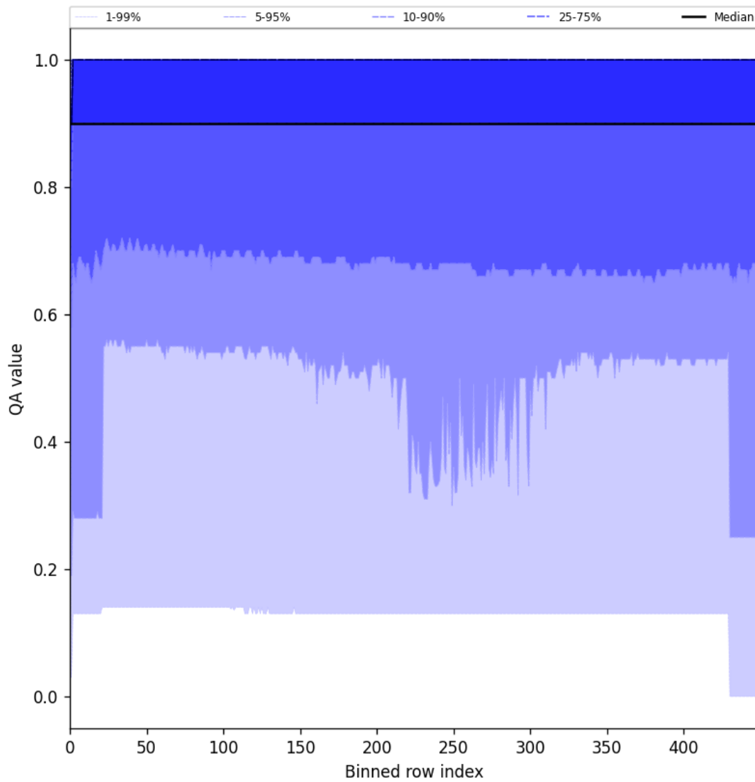
Figure 27: Along track statistics of “QA value” for 2024-09-09 to 2024-09-11
