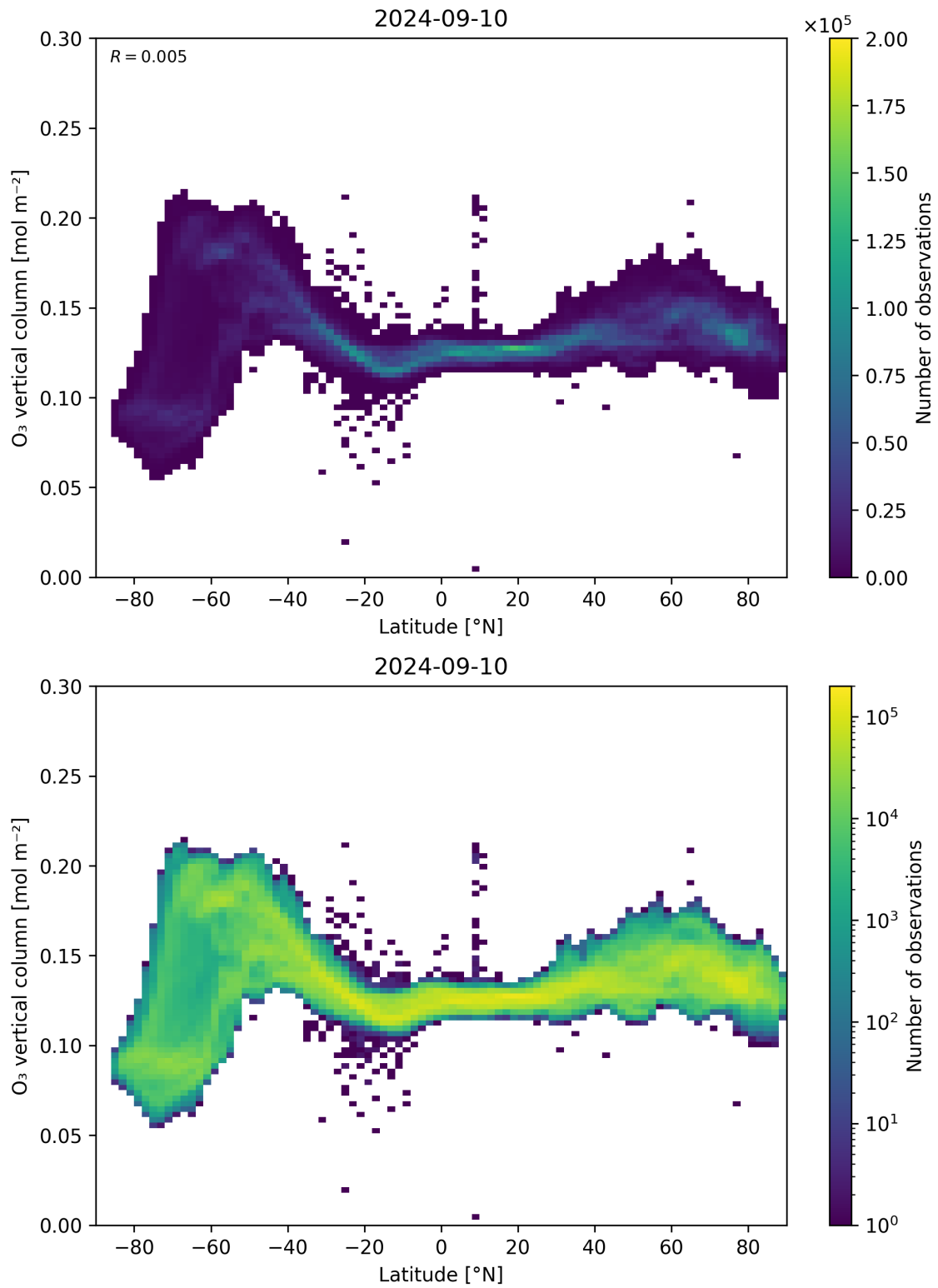
Figure 36: Scatter density plot of “Latitude” against “O 3 vertical column” for 2024-09-09 to 2024-09-11.
