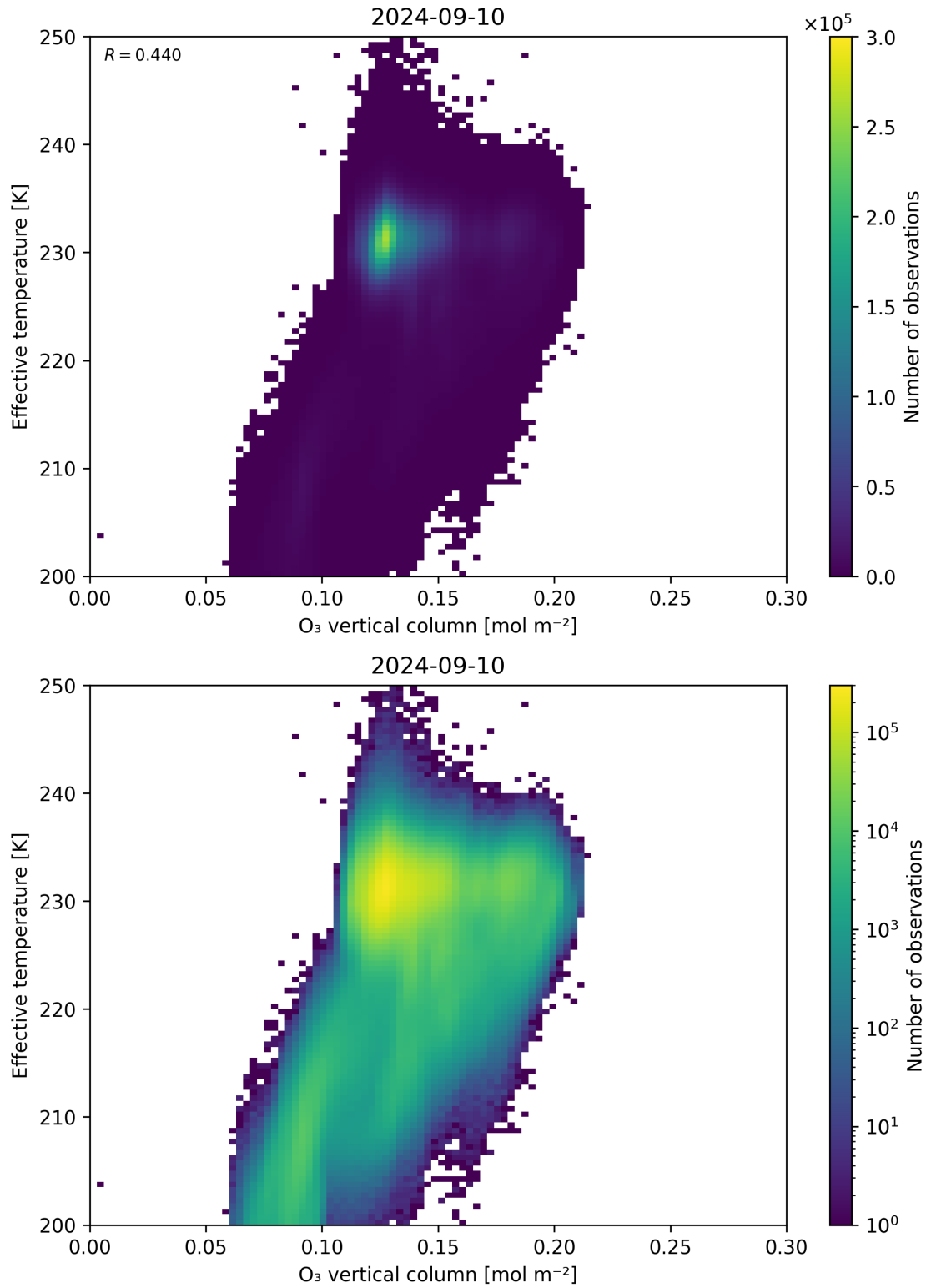
Figure 39: Scatter density plot of “O 3 vertical column” against “Effective temperature” for 2024-09-09 to 2024-09-11.
