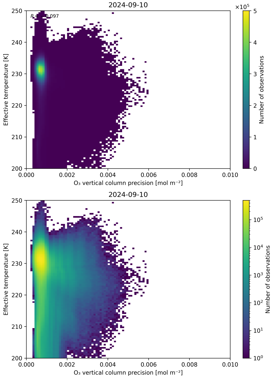
Figure 42: Scatter density plot of “ O_3 vertical column precision” against “Effective temperature” for 2024-09-09 to 2024-09-11.
