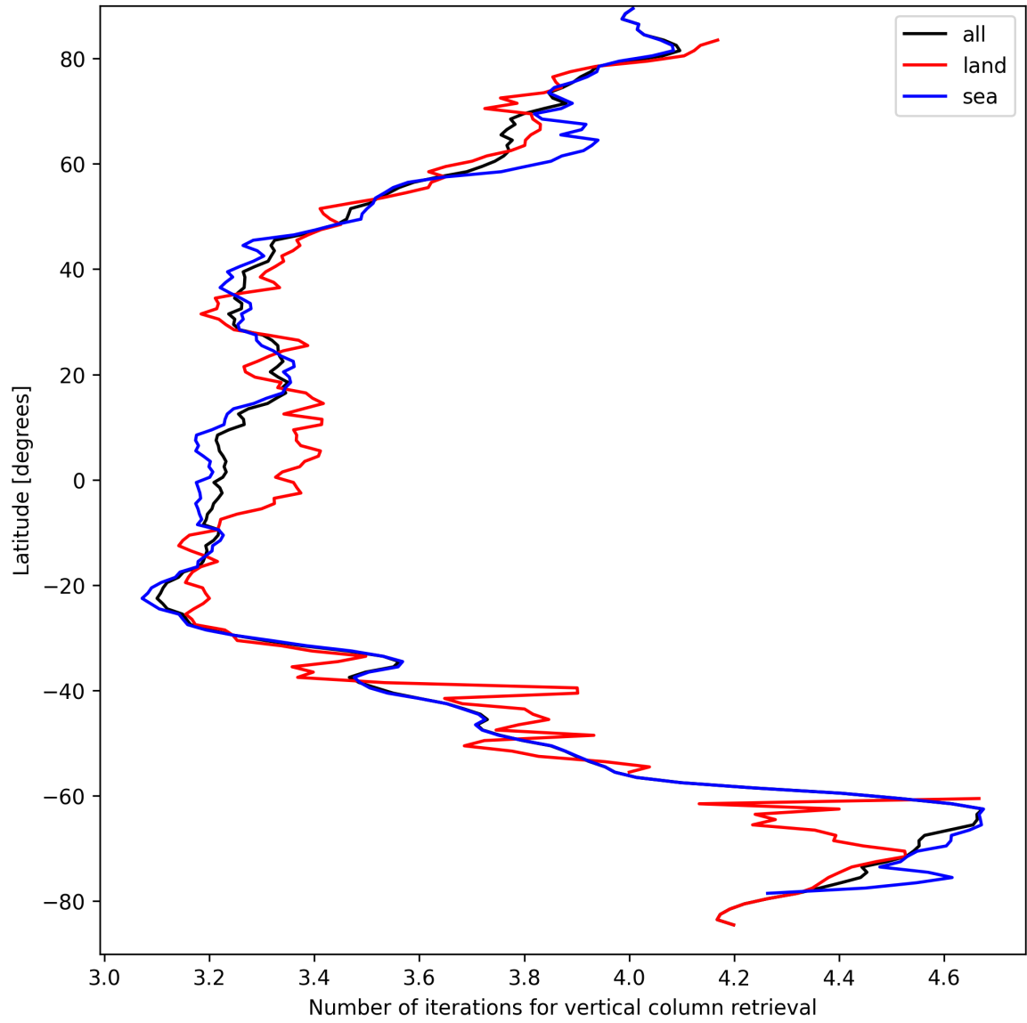
Figure 19: Zonal average of “Number of iterations for vertical column retrieval” for 2024-09-09 to 2024-09-11.
