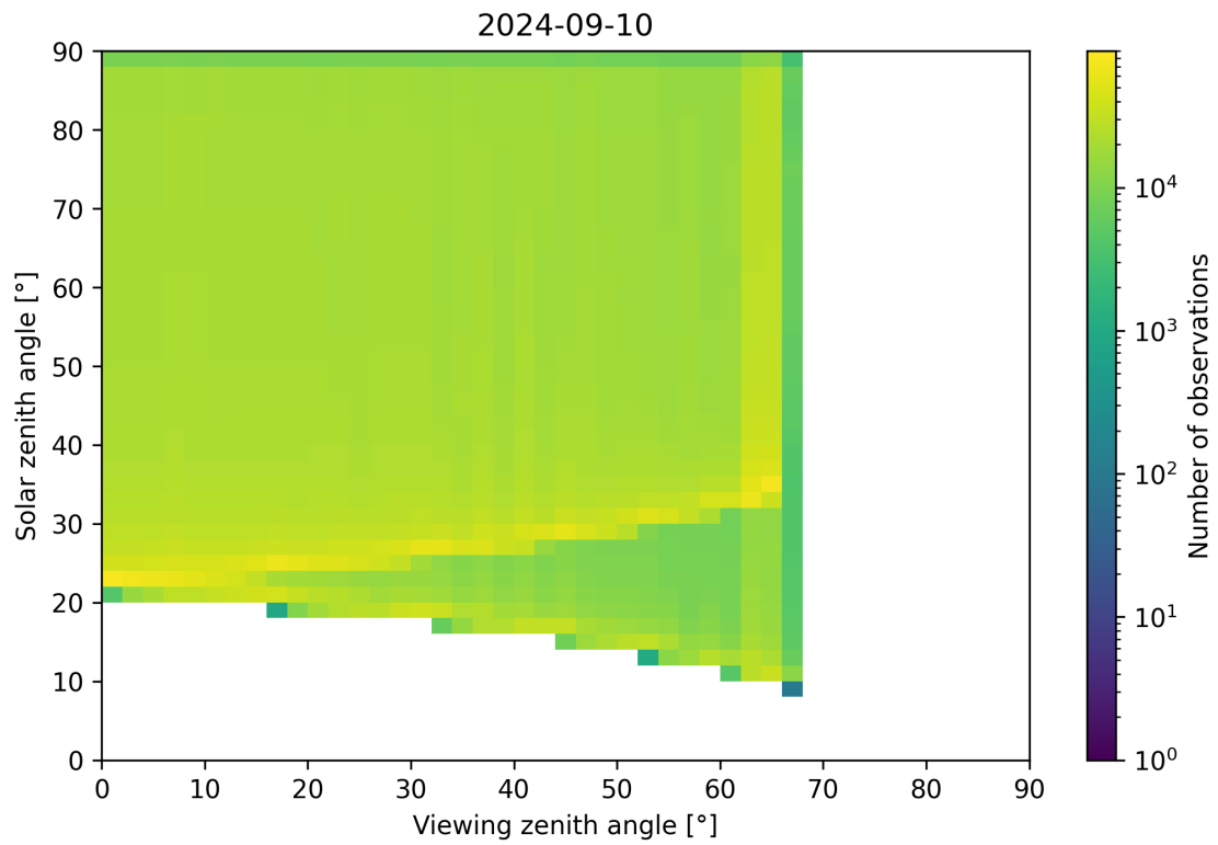
Figure 54: Scatter density plot of “Viewing zenith angle” against “Solar zenith angle” for 2024-09-09 to 2024-09-11.
