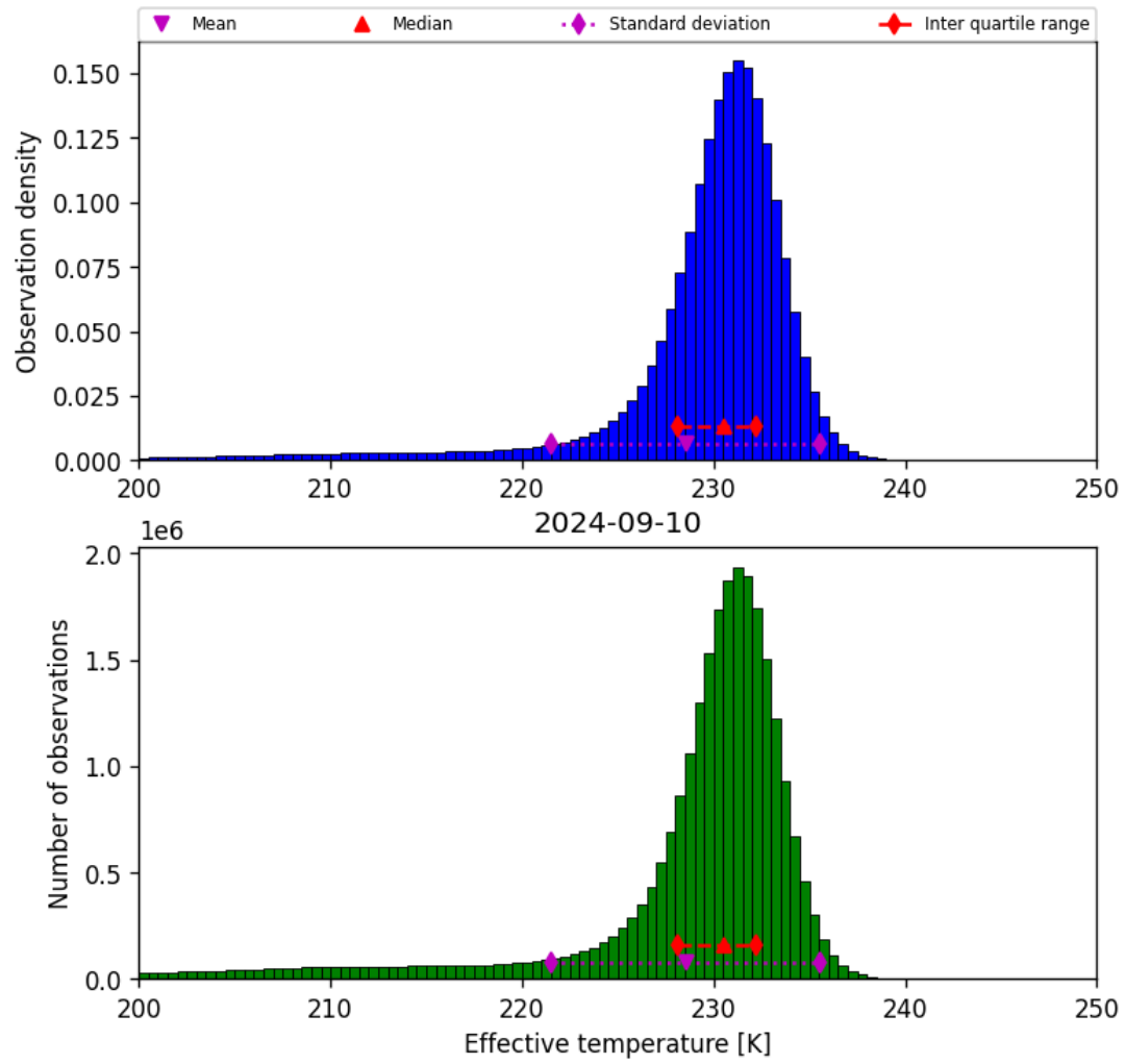
Figure 24: Histogram of “Effective temperature” for 2024-09-09 to 2024-09-11
