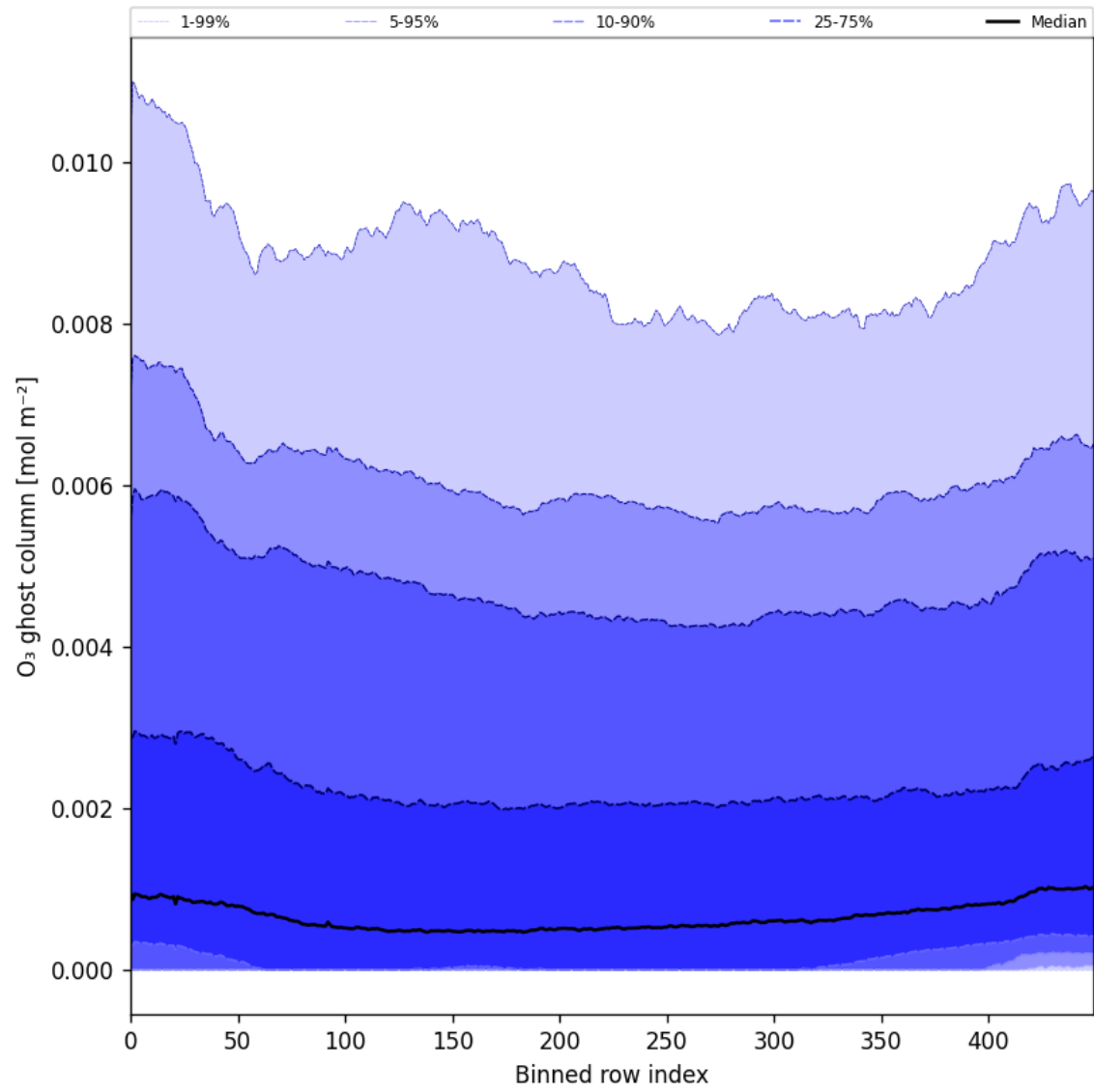
Figure 32: Along track statistics of “O 3 ghost column” for 2024-09-09 to 2024-09-11
