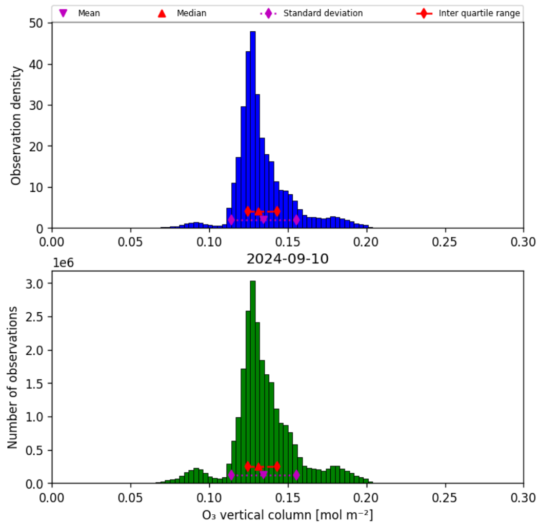
Figure 21: Histogram of “O 3 vertical column” for 2024-09-09 to 2024-09-11
