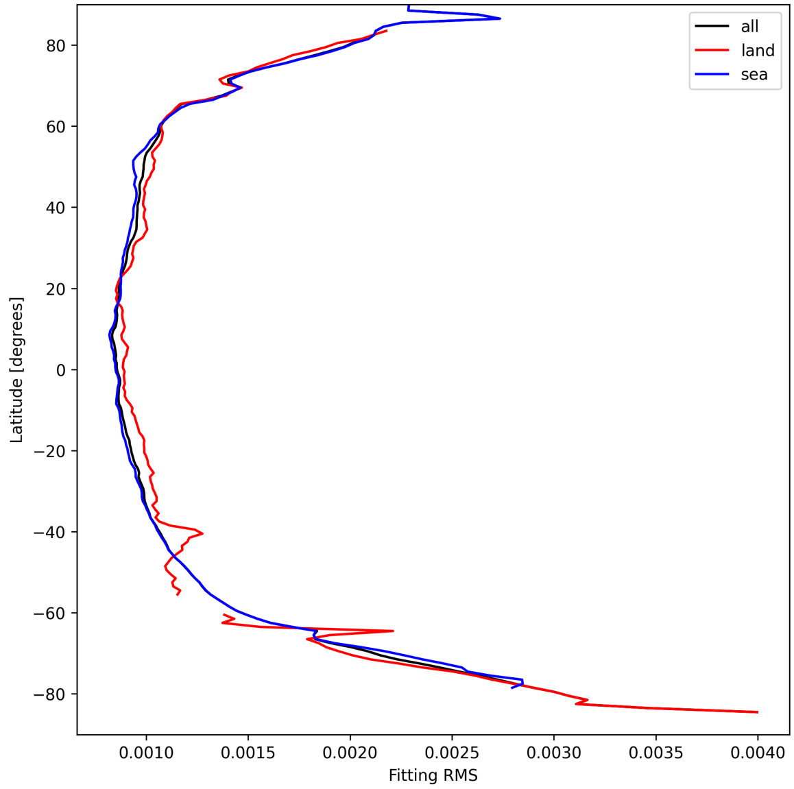
Figure 16: Zonal average of “Fitting RMS” for 2024-09-09 to 2024-09-11.
