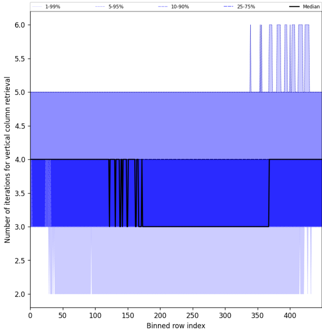
Figure 33: Along track statistics of “Number of iterations for vertical column retrieval” for 2024-09-09 to 2024-09-11
