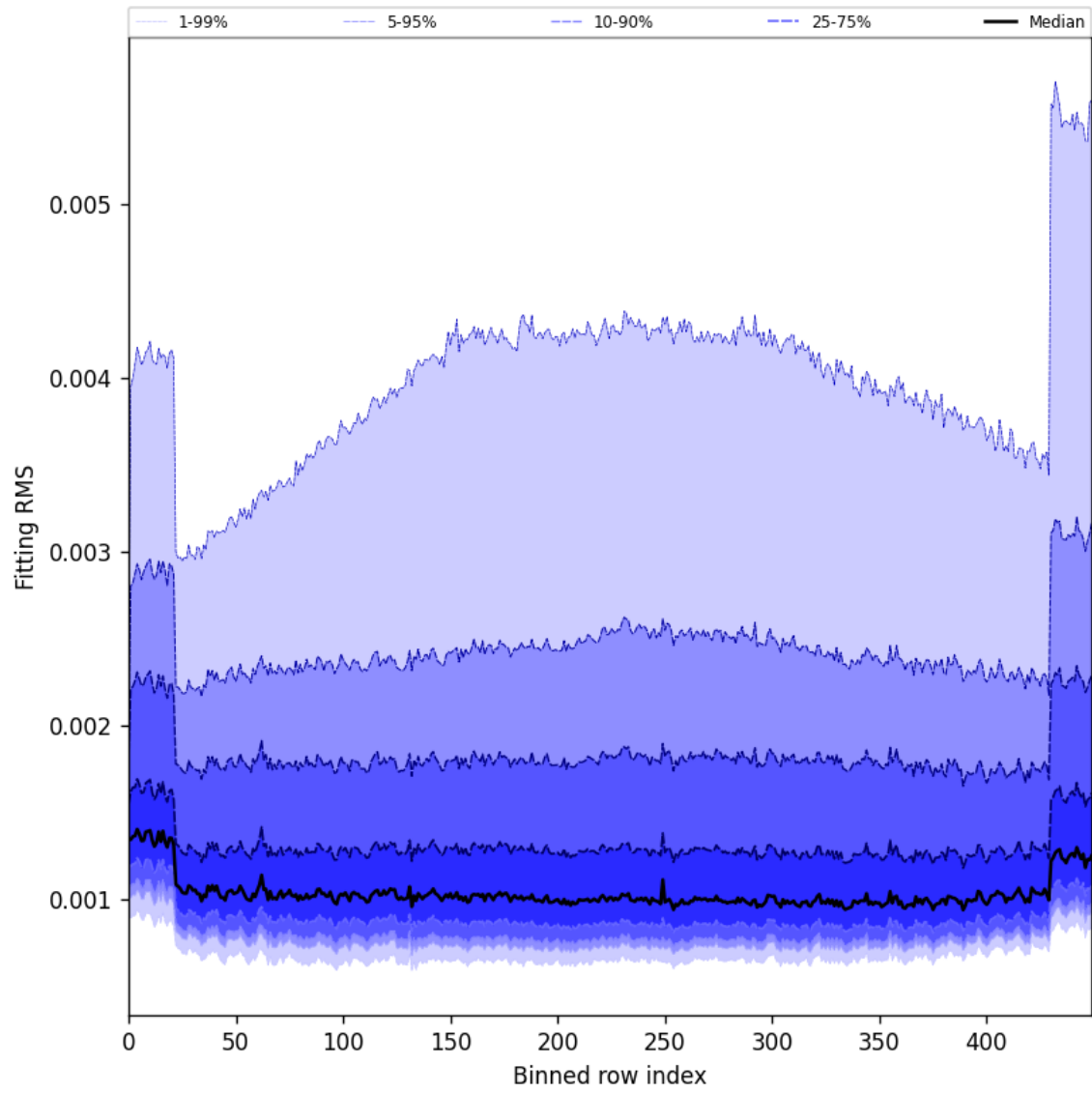
Figure 30: Along track statistics of “Fitting RMS” for 2024-09-09 to 2024-09-11
