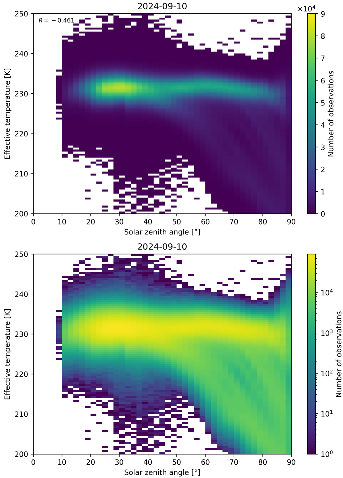
Figure 45: Scatter density plot of “Solar zenith angle” against “Effective temperature” for 2024-09-09 to 2024-09-11.
