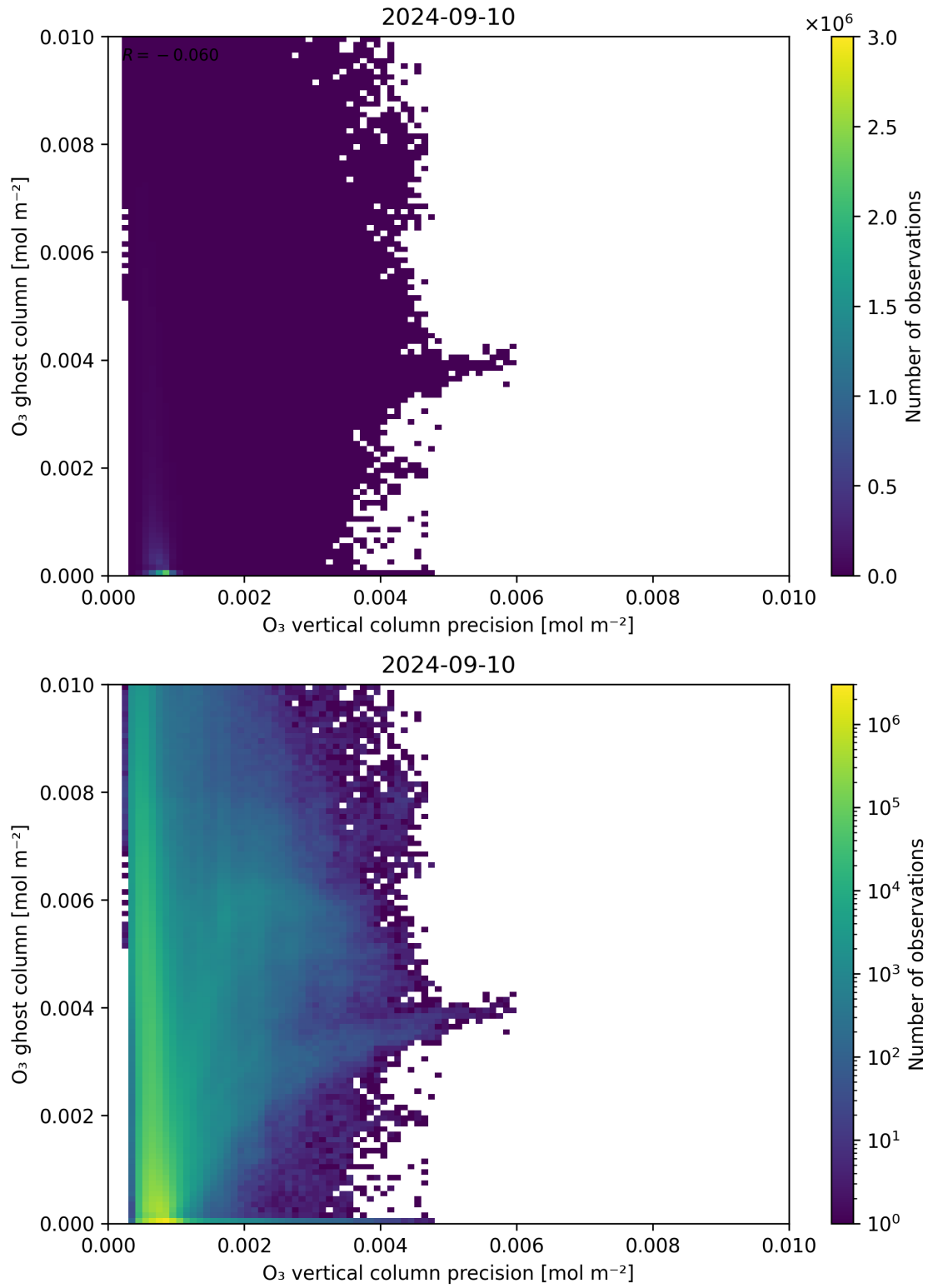
Figure 43: Scatter density plot of “ \text{O}_3 vertical column precision” against “ \text{O}_3 ghost column” for 2024-09-09 to 2024-09-11.
