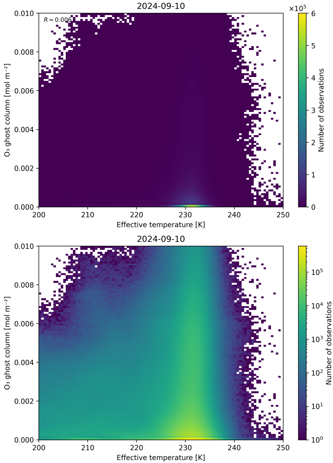
Figure 38: Scatter density plot of “Effective temperature” against “O 3 ghost column” for 2024-09-09 to 2024-09-11.
