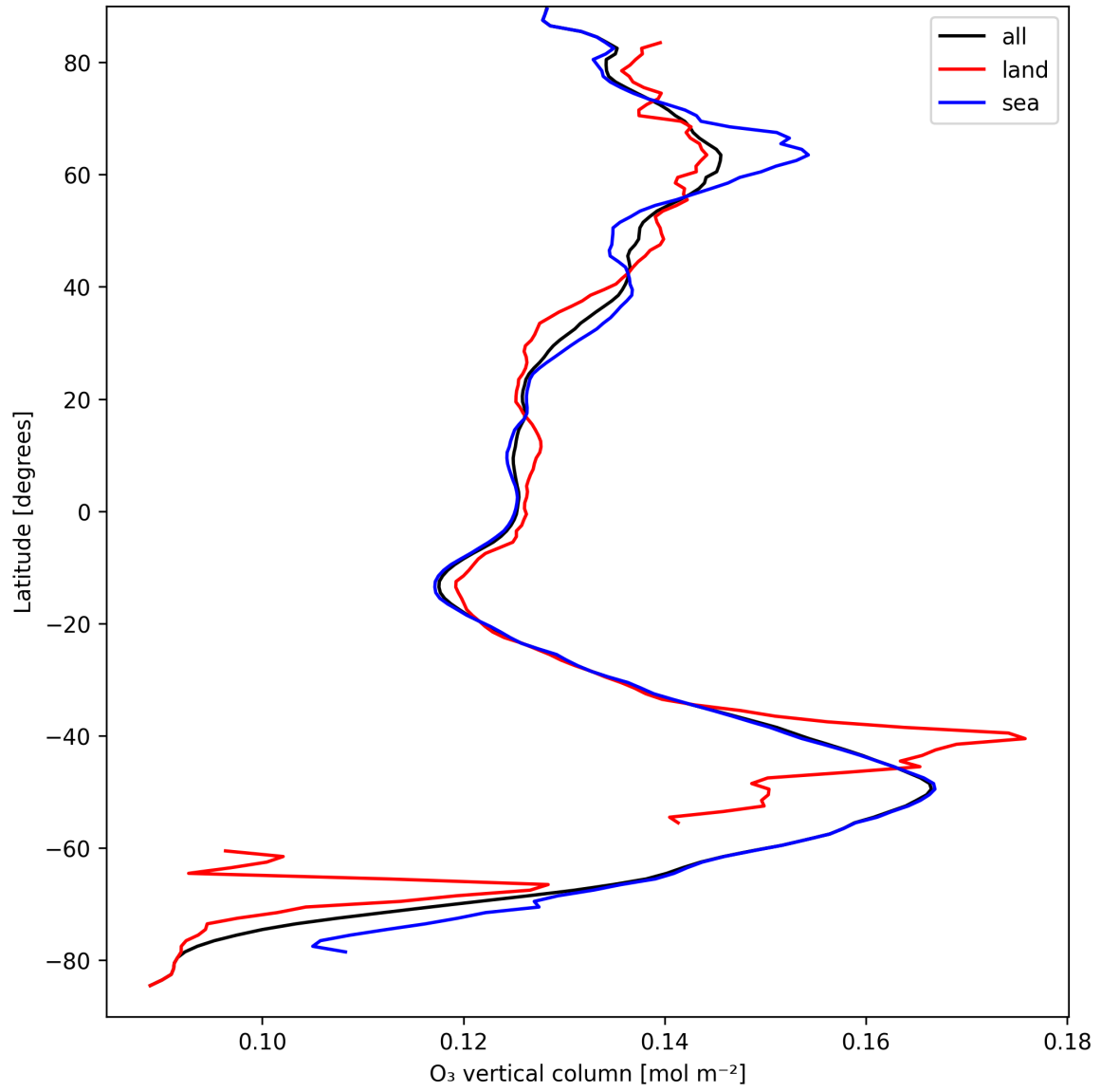
Figure 14: Zonal average of “O 3 vertical column” for 2024-09-09 to 2024-09-11.
