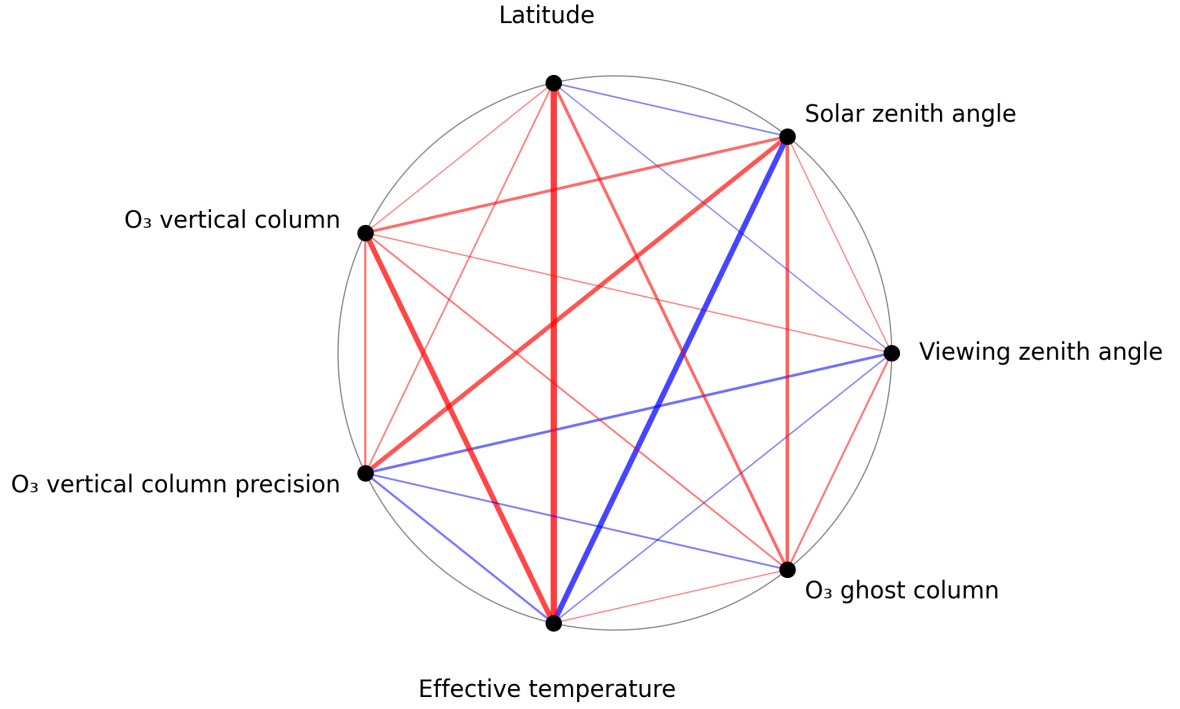
Figure 1: Map of correlation graph for 2024-09-09 to 2024-09-11.
