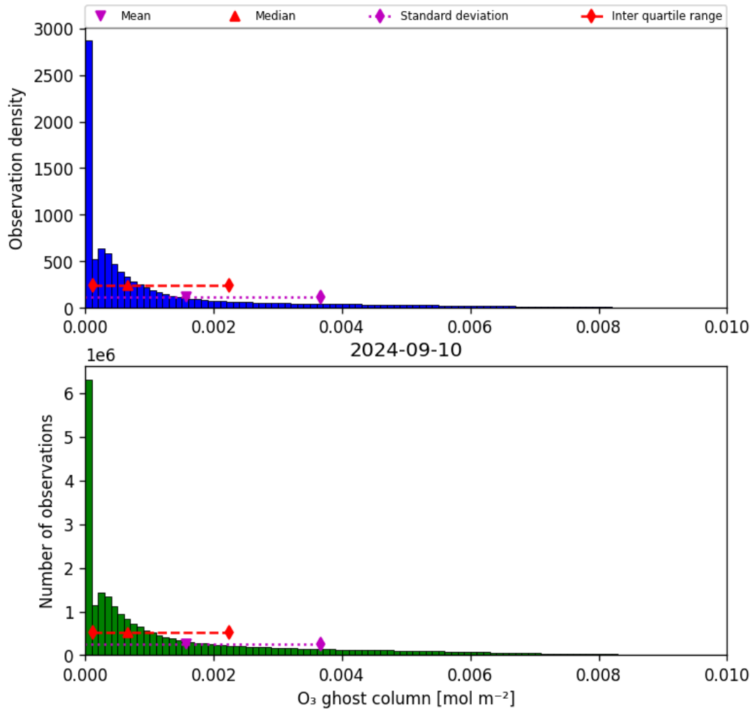
Figure 25: Histogram of “O 3 ghost column” for 2024-09-09 to 2024-09-11
