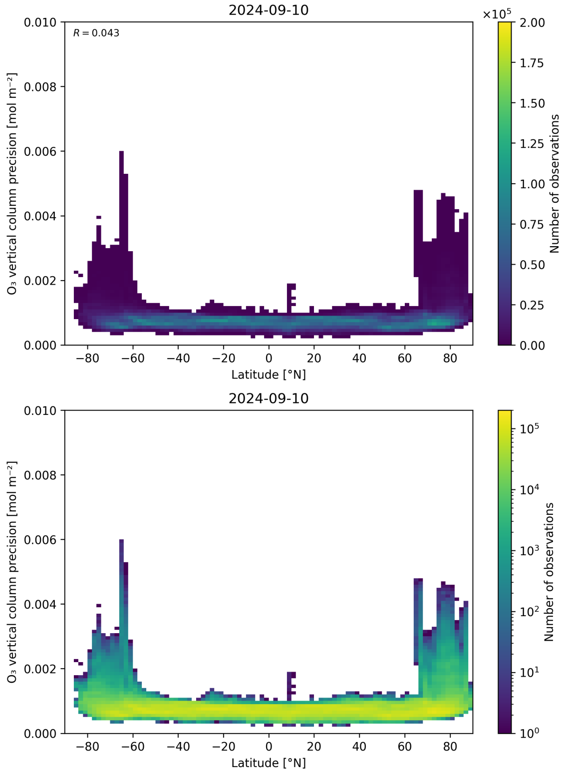
Figure 37: Scatter density plot of “Latitude” against “O 3 vertical column precision” for 2024-09-09 to 2024-09-11.
