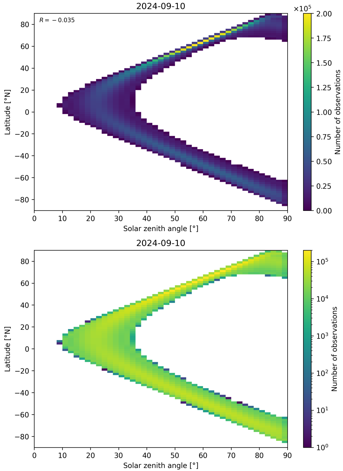
Figure 44: Scatter density plot of “Solar zenith angle” against “Latitude” for 2024-09-09 to 2024-09-11.
