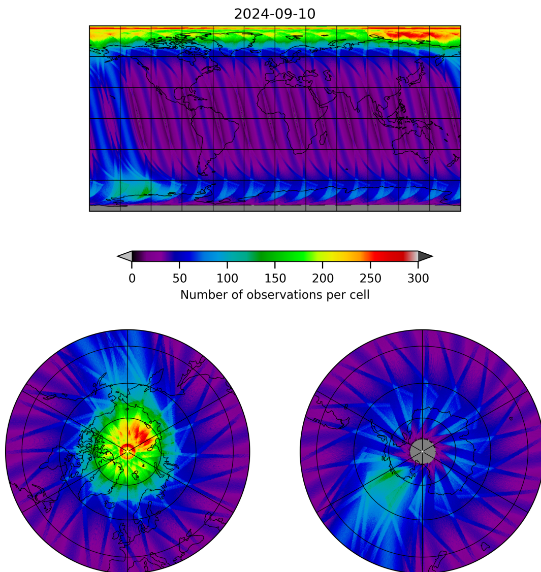
Figure 12: Map of the number of observations for 2024-09-09 to 2024-09-11
