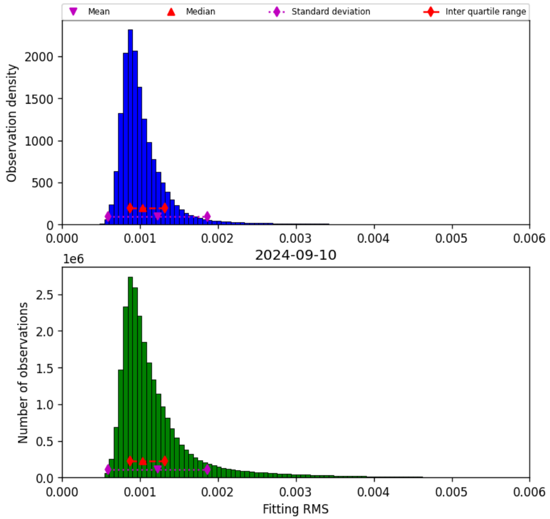
Figure 23: Histogram of “Fitting RMS” for 2024-09-09 to 2024-09-11
