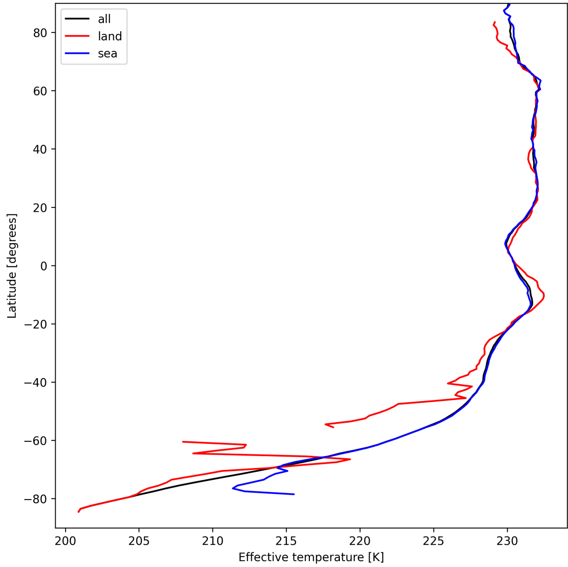
Figure 17: Zonal average of "Effective temperature" for 2024-09-09 to 2024-09-11.
