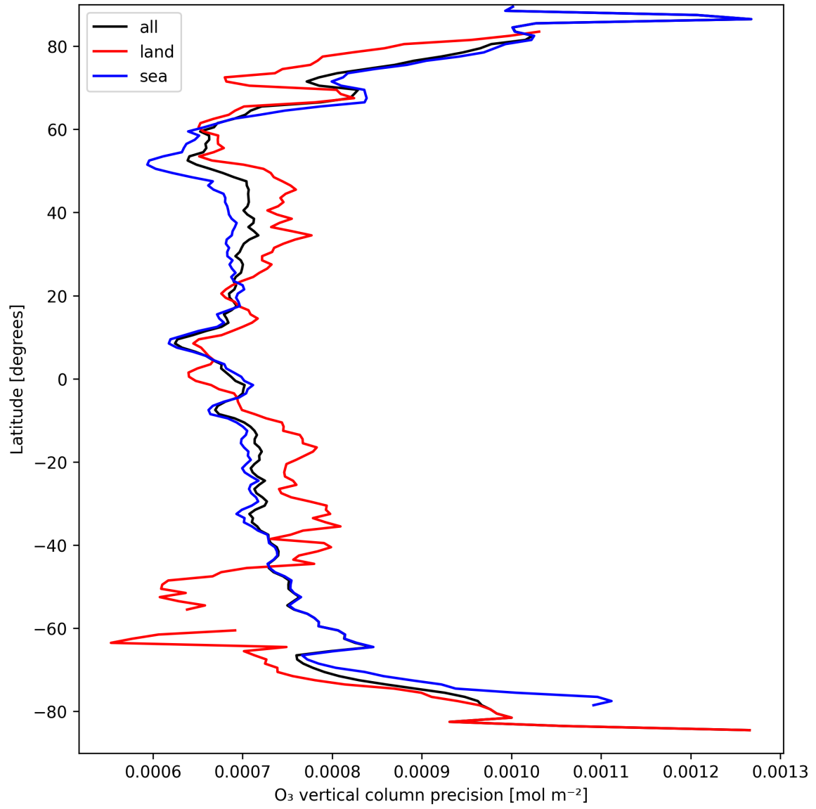
Figure 15: Zonal average of “O 3 vertical column precision” for 2024-09-09 to 2024-09-11.
