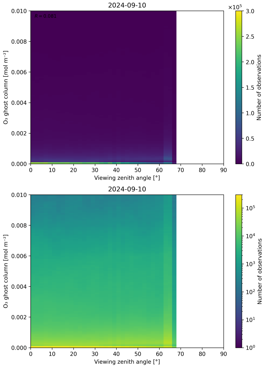
Figure 51: Scatter density plot of “Viewing zenith angle” against “O 3 ghost column” for 2024-09-09 to 2024-09-11.
