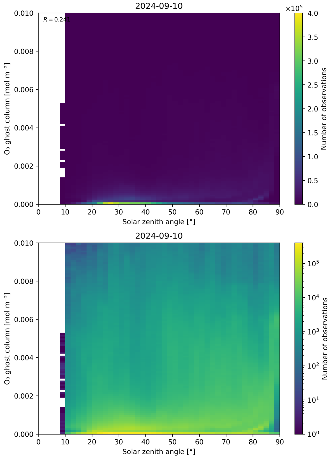
Figure 46: Scatter density plot of “Solar zenith angle” against “O 3 ghost column” for 2024-09-09 to 2024-09-11.
