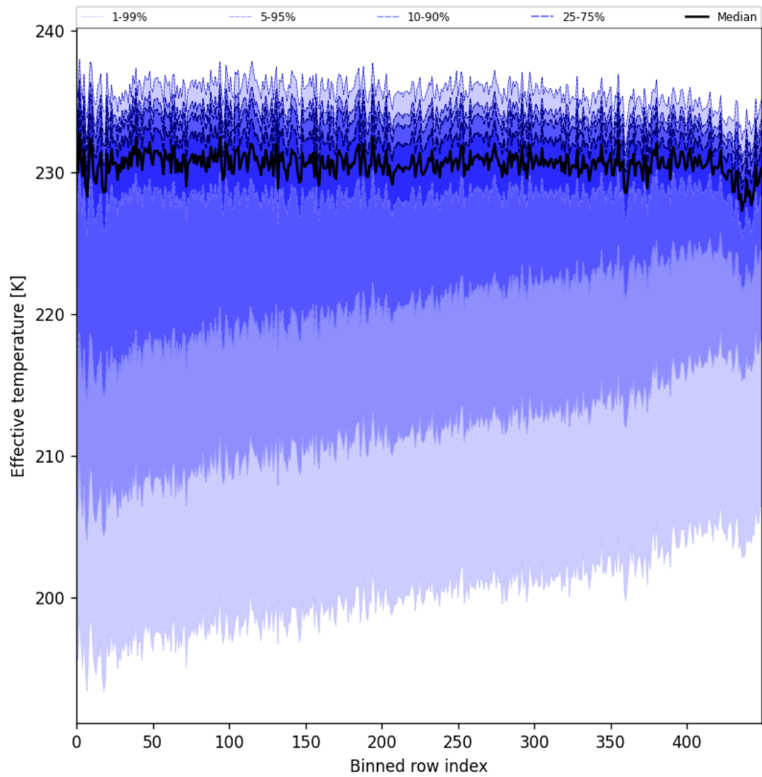
Figure 31: Along track statistics of “Effective temperature” for 2024-09-09 to 2024-09-11
