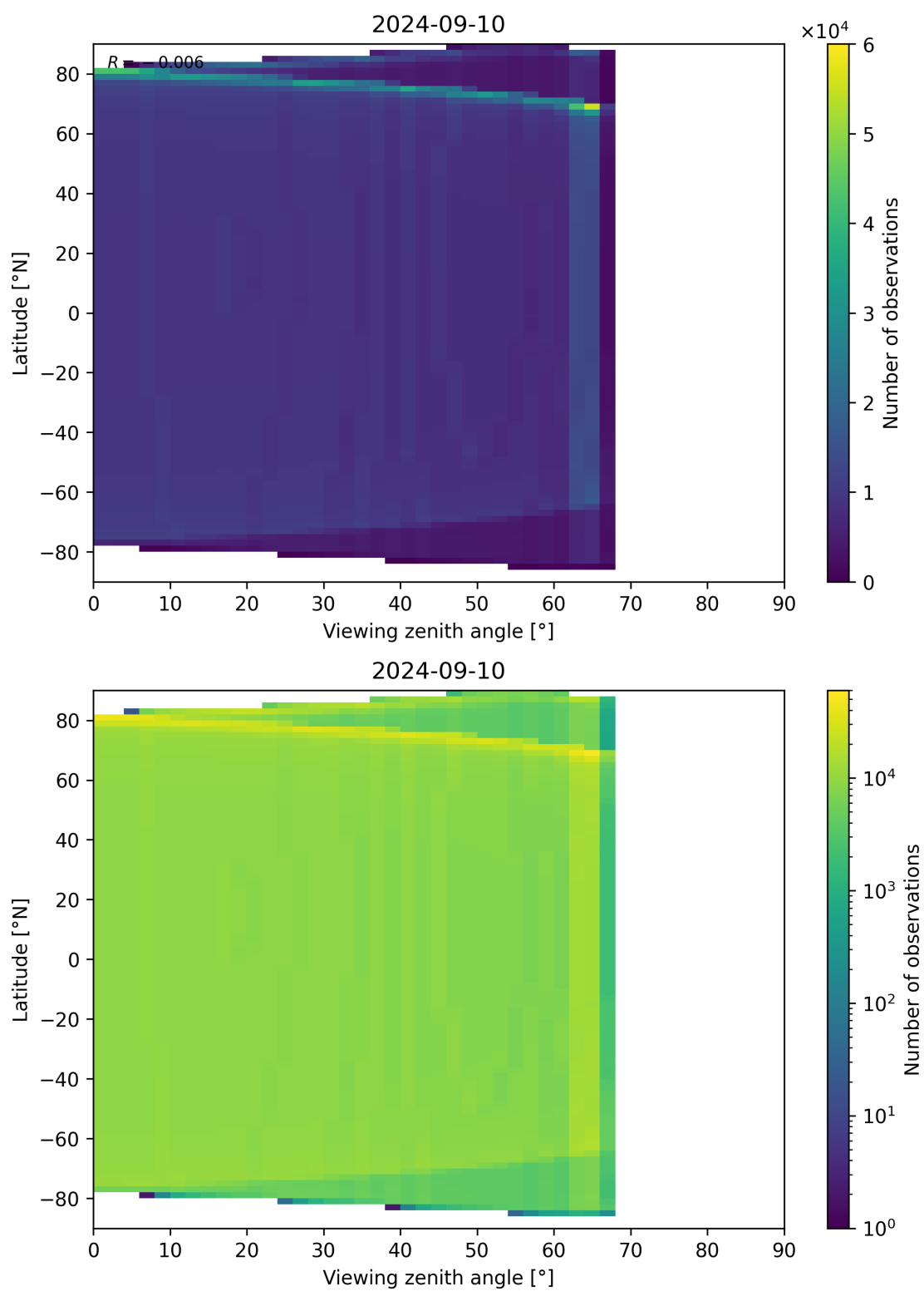
Figure 49: Scatter density plot of “Viewing zenith angle” against “Latitude” for 2024-09-09 to 2024-09-11.
