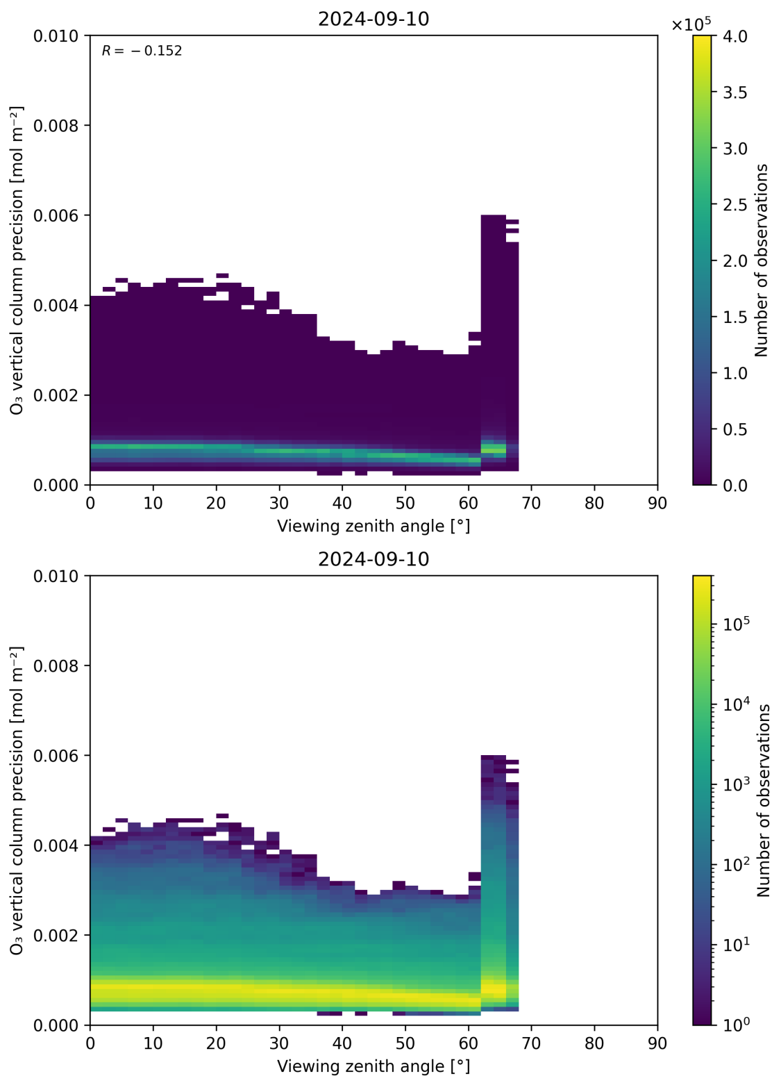
Figure 53: Scatter density plot of “Viewing zenith angle” against “O 3 vertical column precision” for 2024-09-09 to 2024-09-11.
