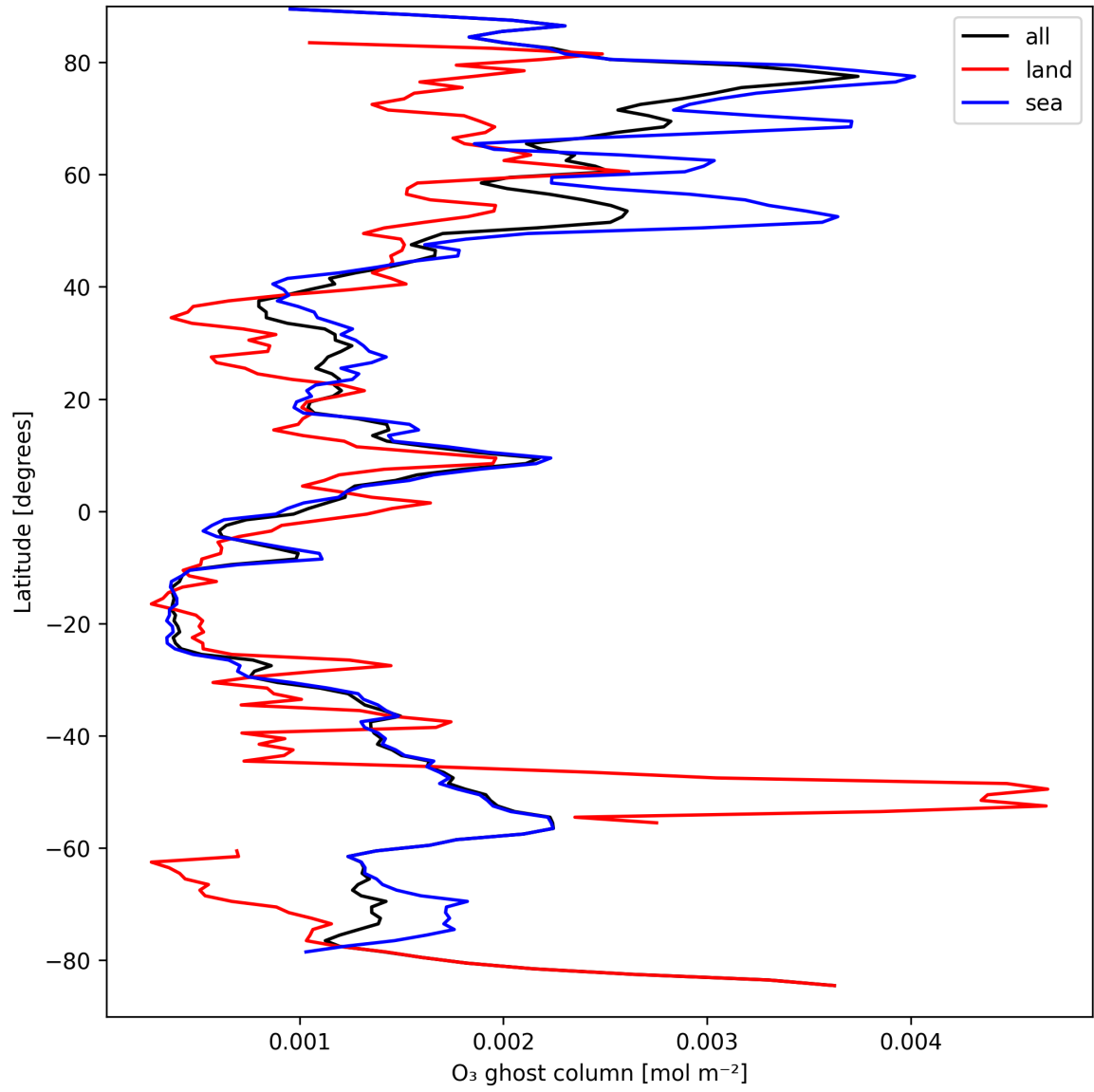
Figure 18: Zonal average of "O 3 ghost column" for 2024-09-09 to 2024-09-11.
