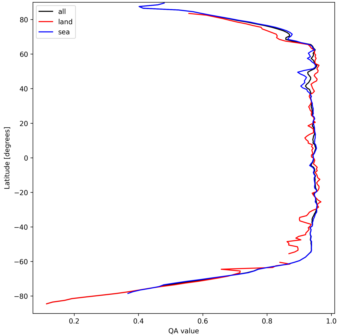
Figure 13: Zonal average of “QA value” for 2024-09-09 to 2024-09-11.
