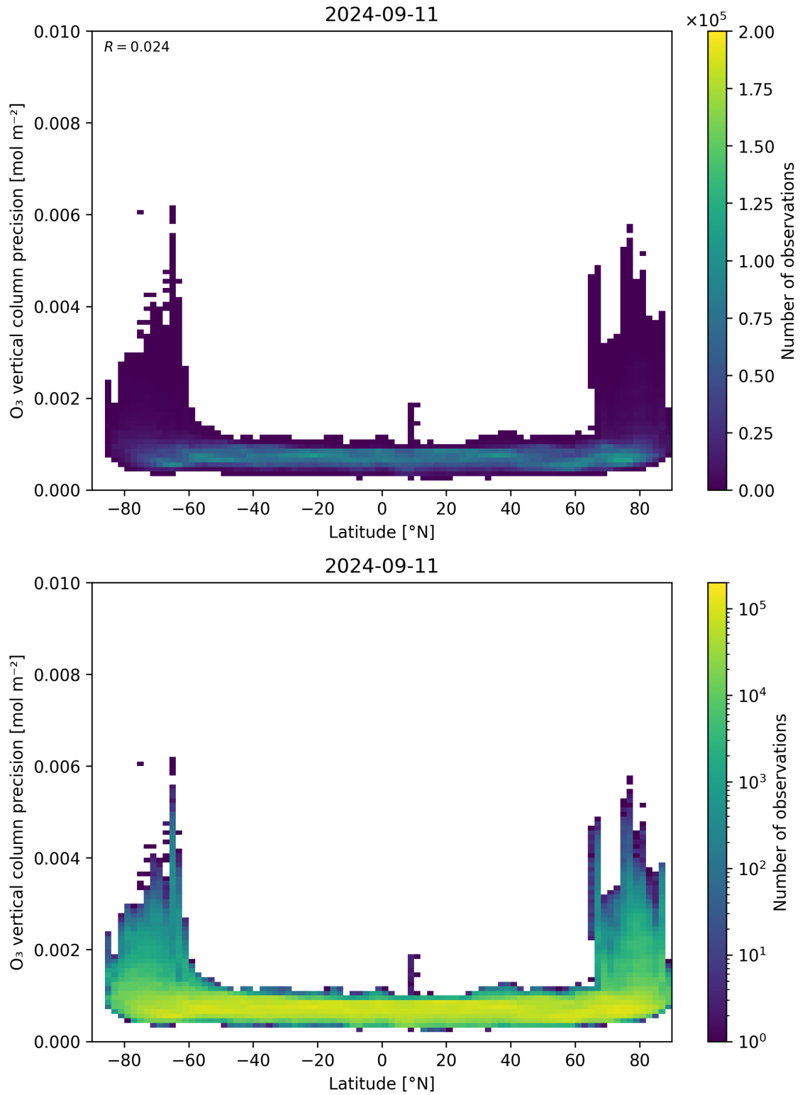
Figure 37: Scatter density plot of “Latitude” against “O 3 vertical column precision” for 2024-09-10 to 2024-09-12.
