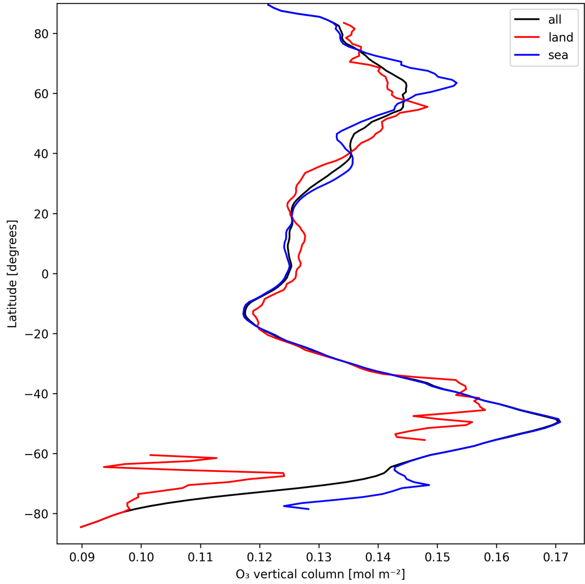
Figure 14: Zonal average of “O 3 vertical column” for 2024-09-10 to 2024-09-12.
