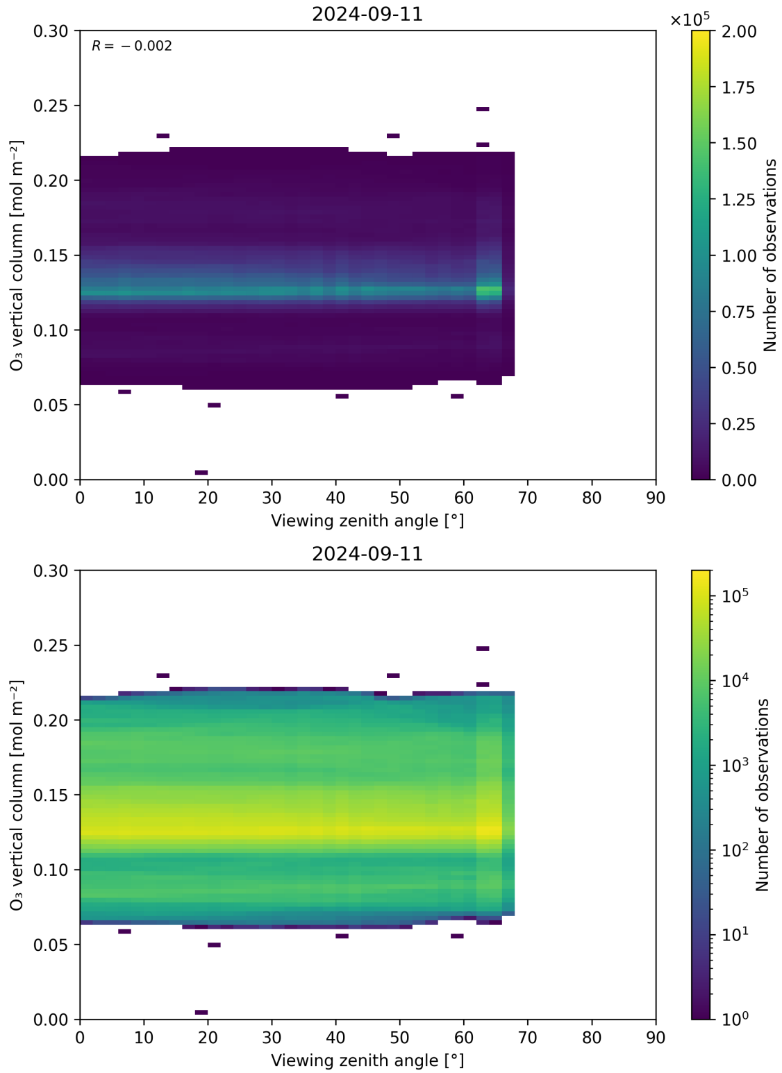
Figure 52: Scatter density plot of “Viewing zenith angle” against “O 3 vertical column” for 2024-09-10 to 2024-09-12.
