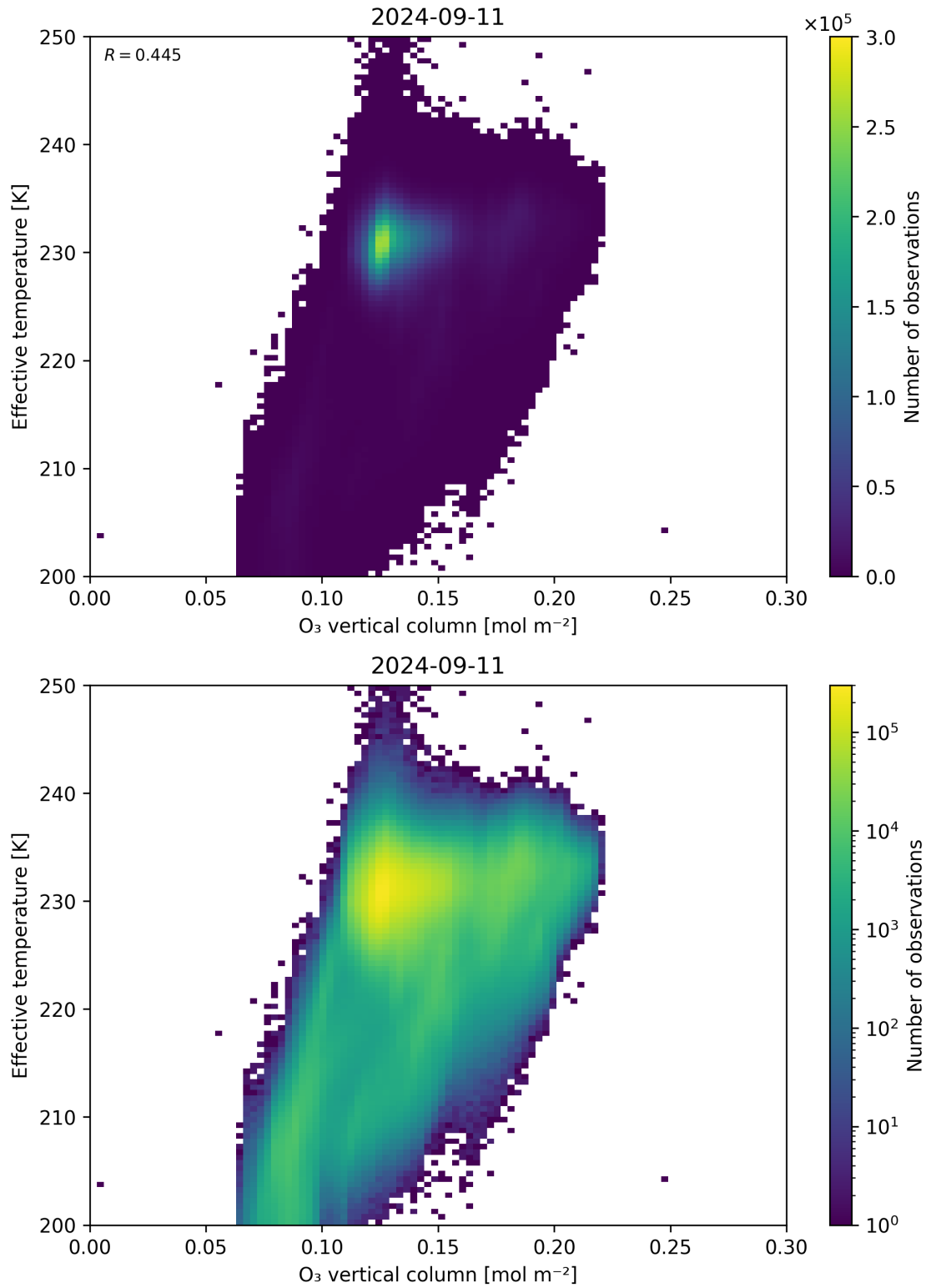
Figure 39: Scatter density plot of “O 3 vertical column” against “Effective temperature” for 2024-09-10 to 2024-09-12.
