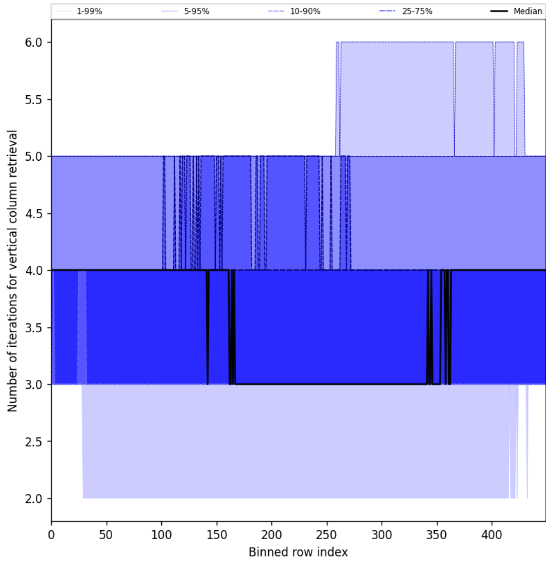
Figure 33: Along track statistics of “Number of iterations for vertical column retrieval” for 2024-09-10 to 2024-09-12
