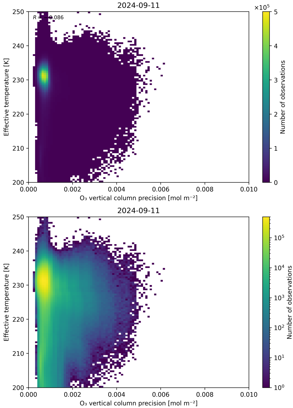
Figure 42: Scatter density plot of “O 3 vertical column precision” against “Effective temperature” for 2024-09-10 to 2024-09-12.
