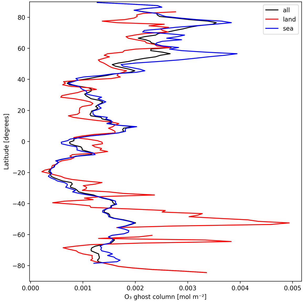
Figure 18: Zonal average of "O 3 ghost column" for 2024-09-10 to 2024-09-12.
