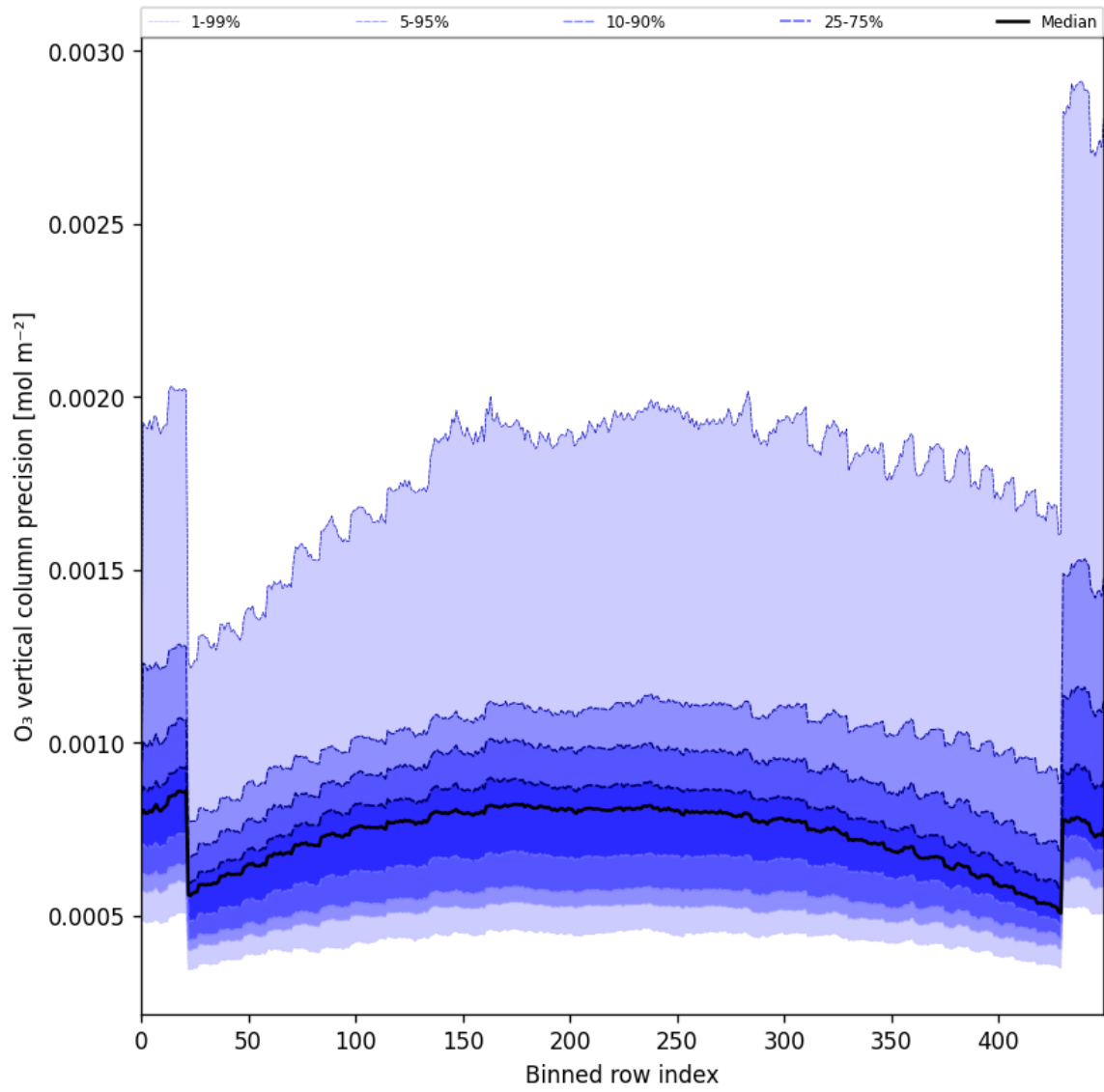
Figure 29: Along track statistics of “O 3 vertical column precision” for 2024-09-10 to 2024-09-12
