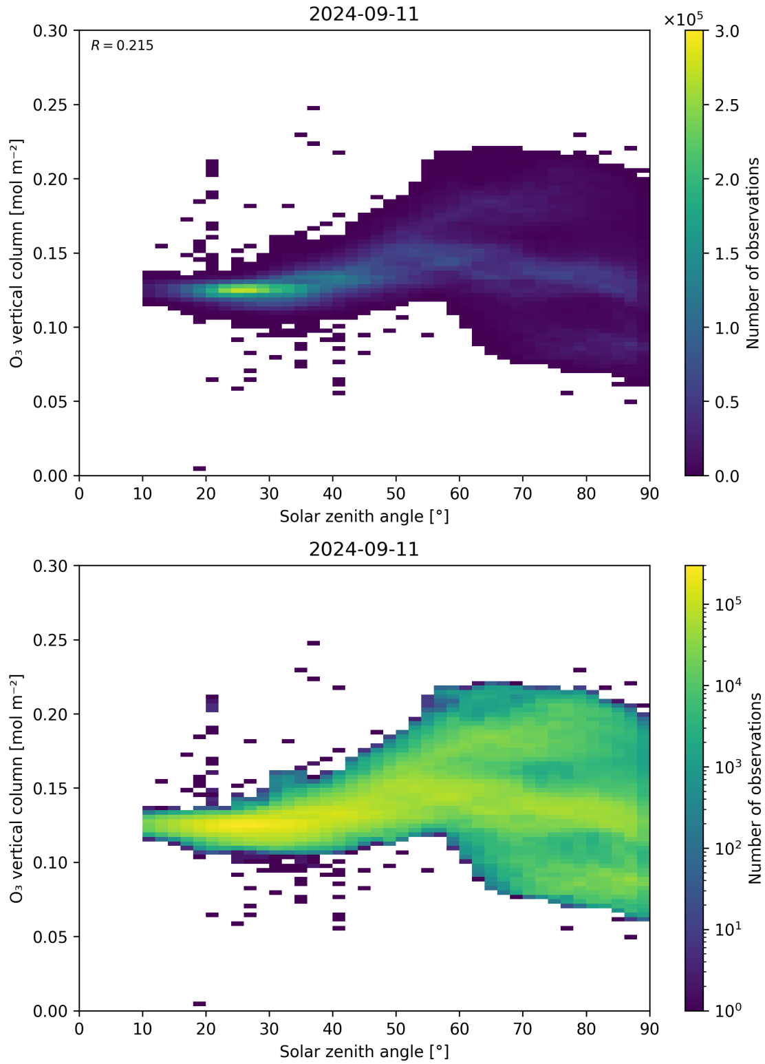
Figure 47: Scatter density plot of “Solar zenith angle” against “O 3 vertical column” for 2024-09-10 to 2024-09-12.
