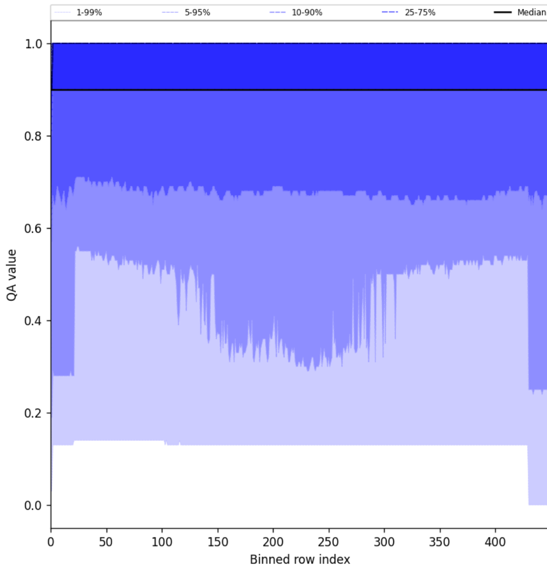
Figure 27: Along track statistics of “QA value” for 2024-09-10 to 2024-09-12
