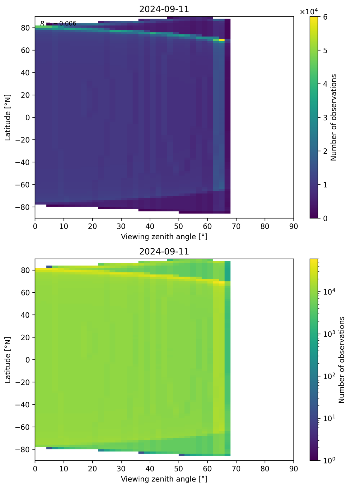
Figure 49: Scatter density plot of “Viewing zenith angle” against “Latitude” for 2024-09-10 to 2024-09-12.
