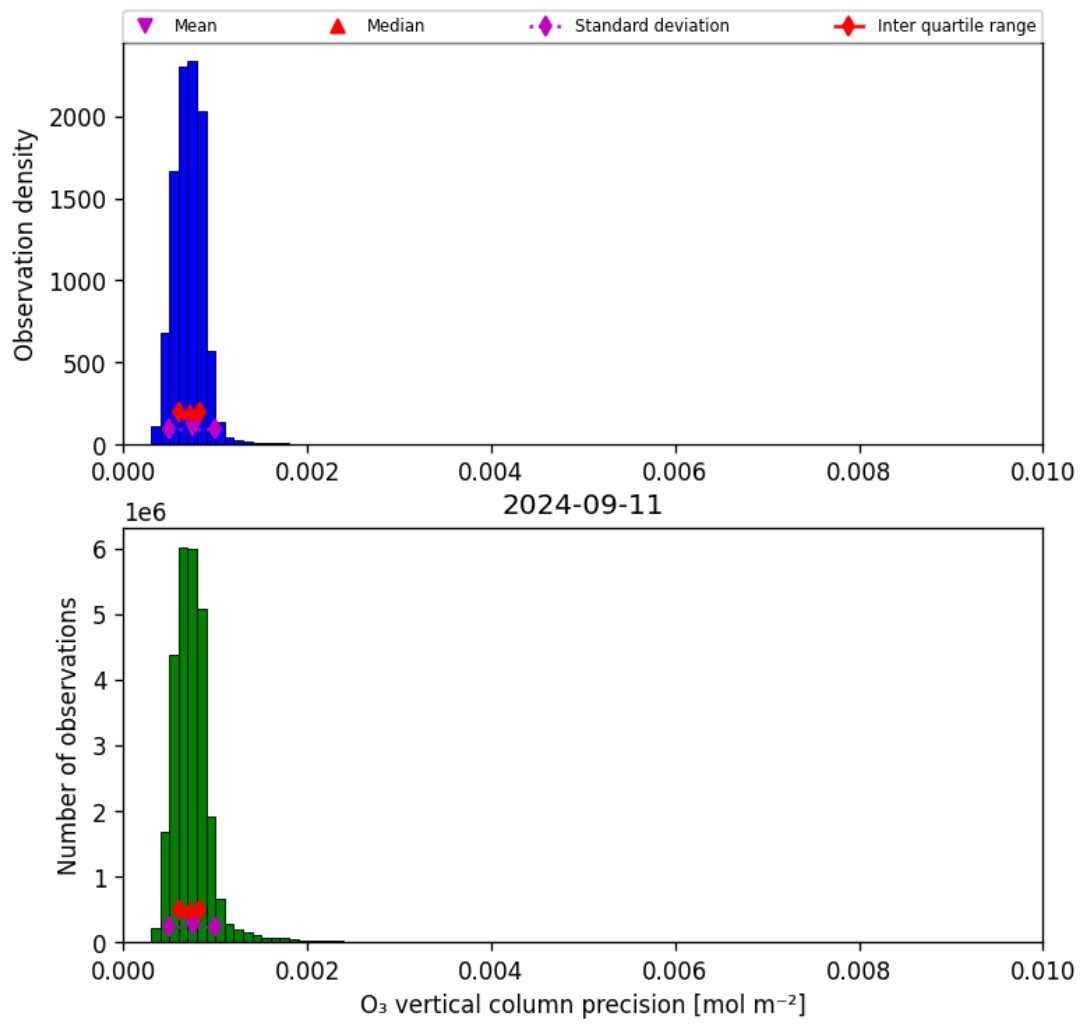
Figure 22: Histogram of “O 3 vertical column precision” for 2024-09-10 to 2024-09-12
