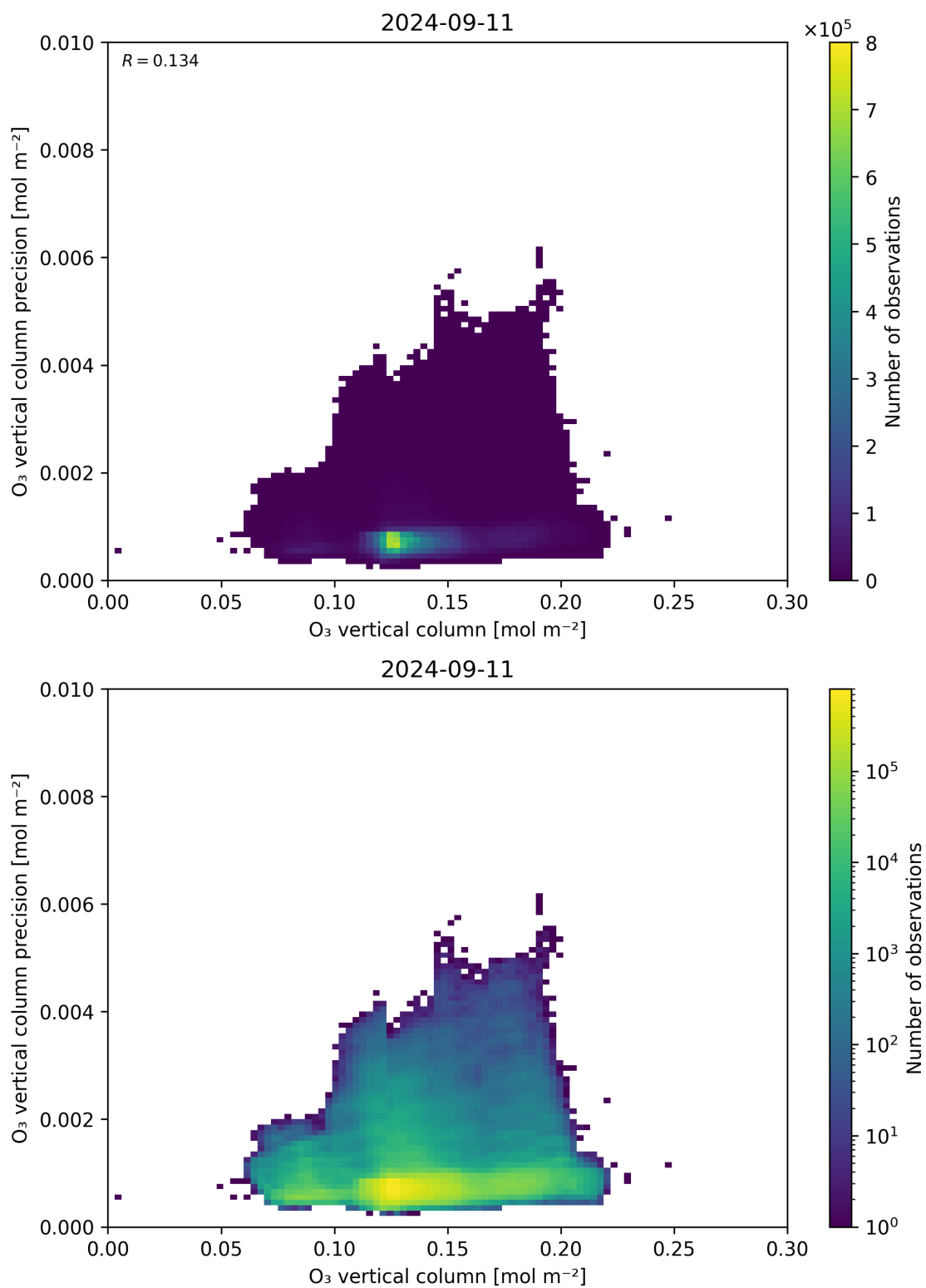
Figure 41: Scatter density plot of “O 3 vertical column” against “O 3 vertical column precision” for 2024-09-10 to 2024-09-12.
