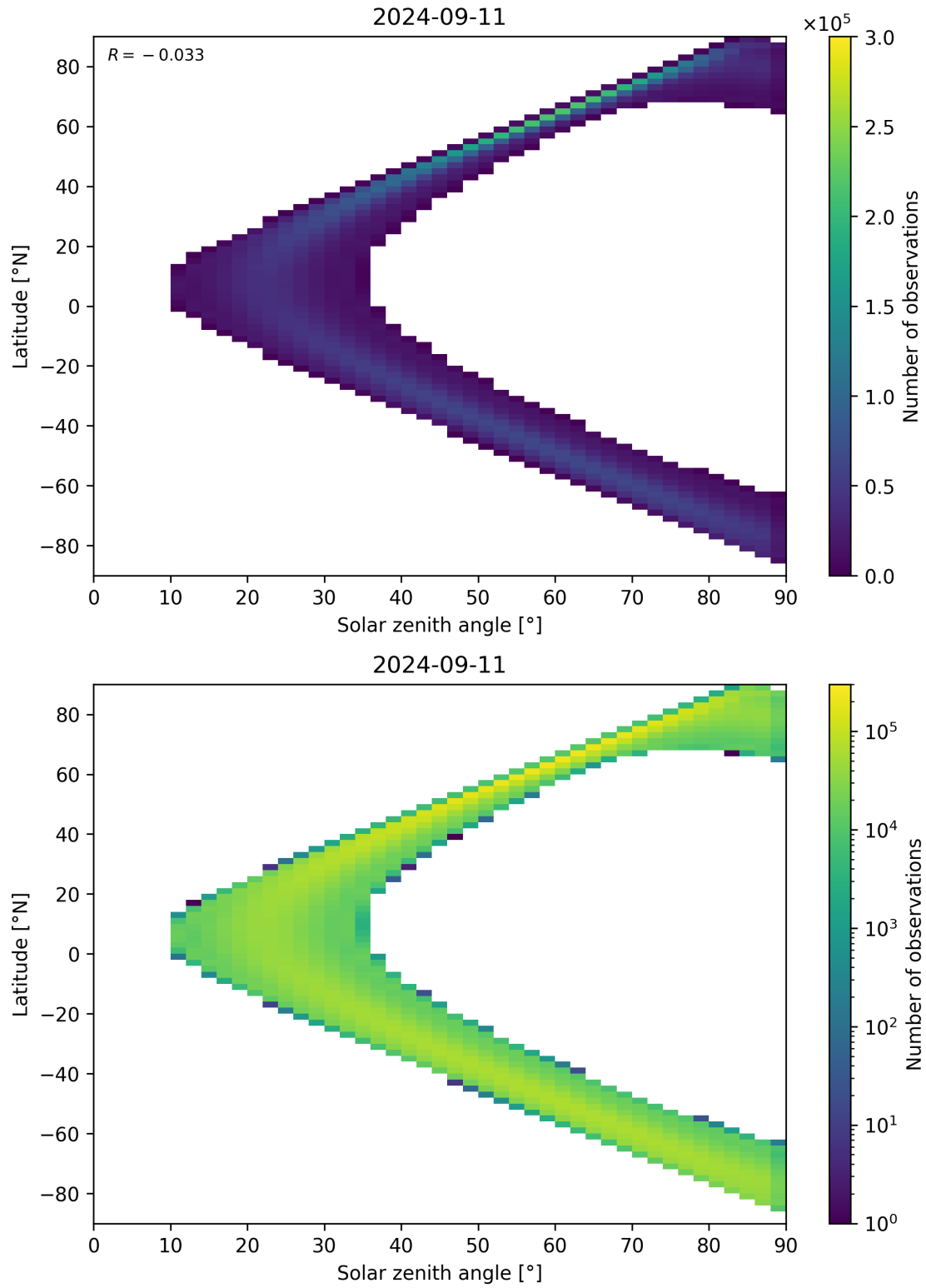
Figure 44: Scatter density plot of “Solar zenith angle” against “Latitude” for 2024-09-10 to 2024-09-12.
