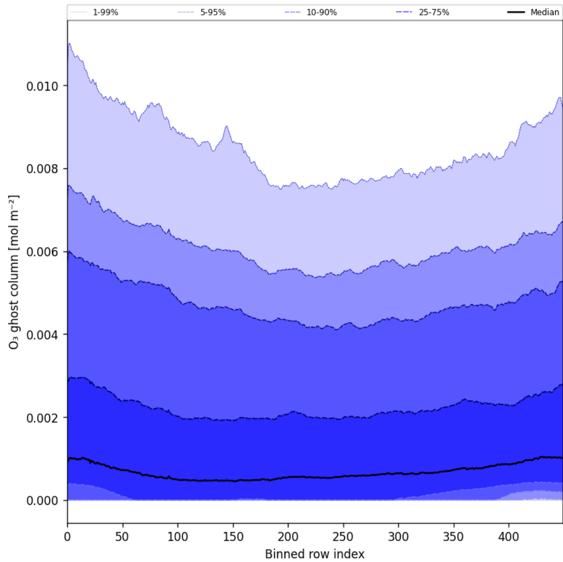
Figure 32: Along track statistics of “O 3 ghost column” for 2024-09-10 to 2024-09-12
