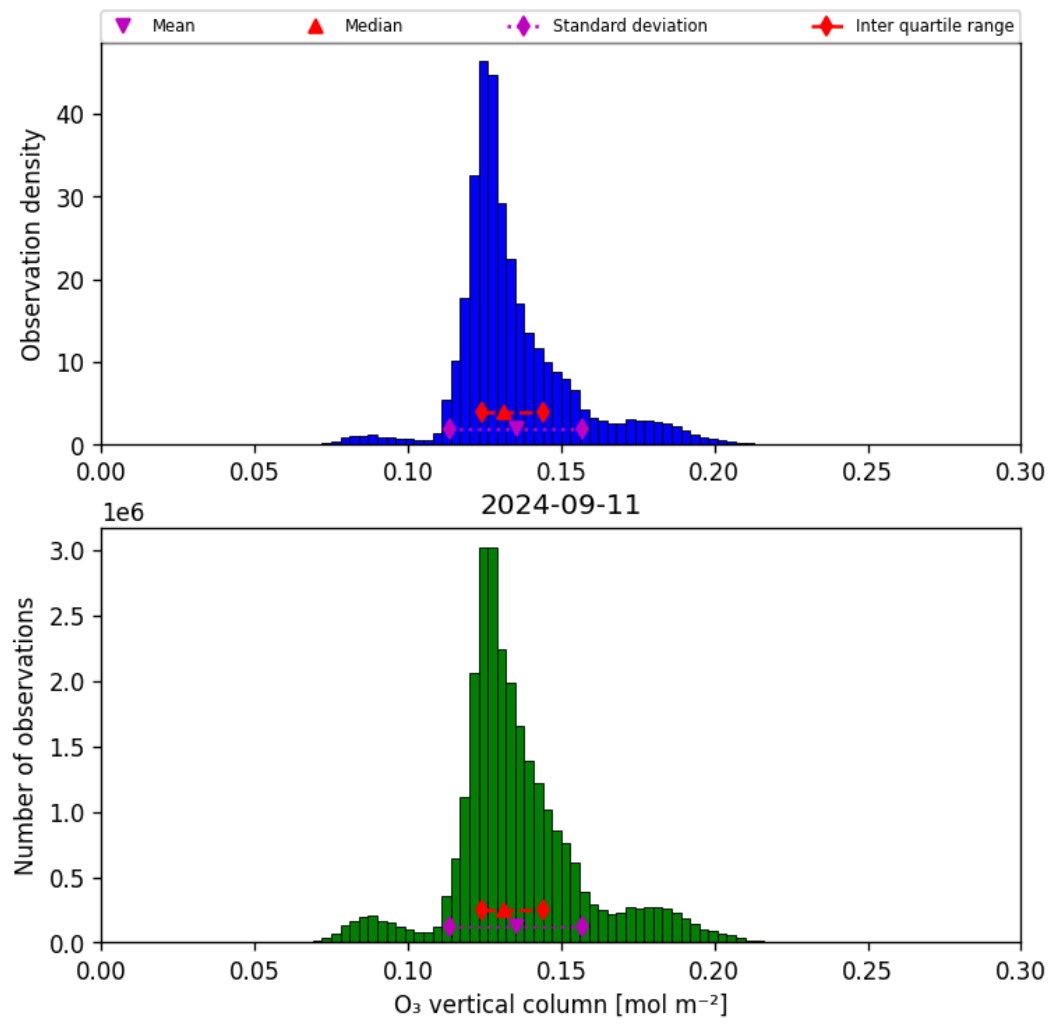
Figure 21: Histogram of “O 3 vertical column” for 2024-09-10 to 2024-09-12
