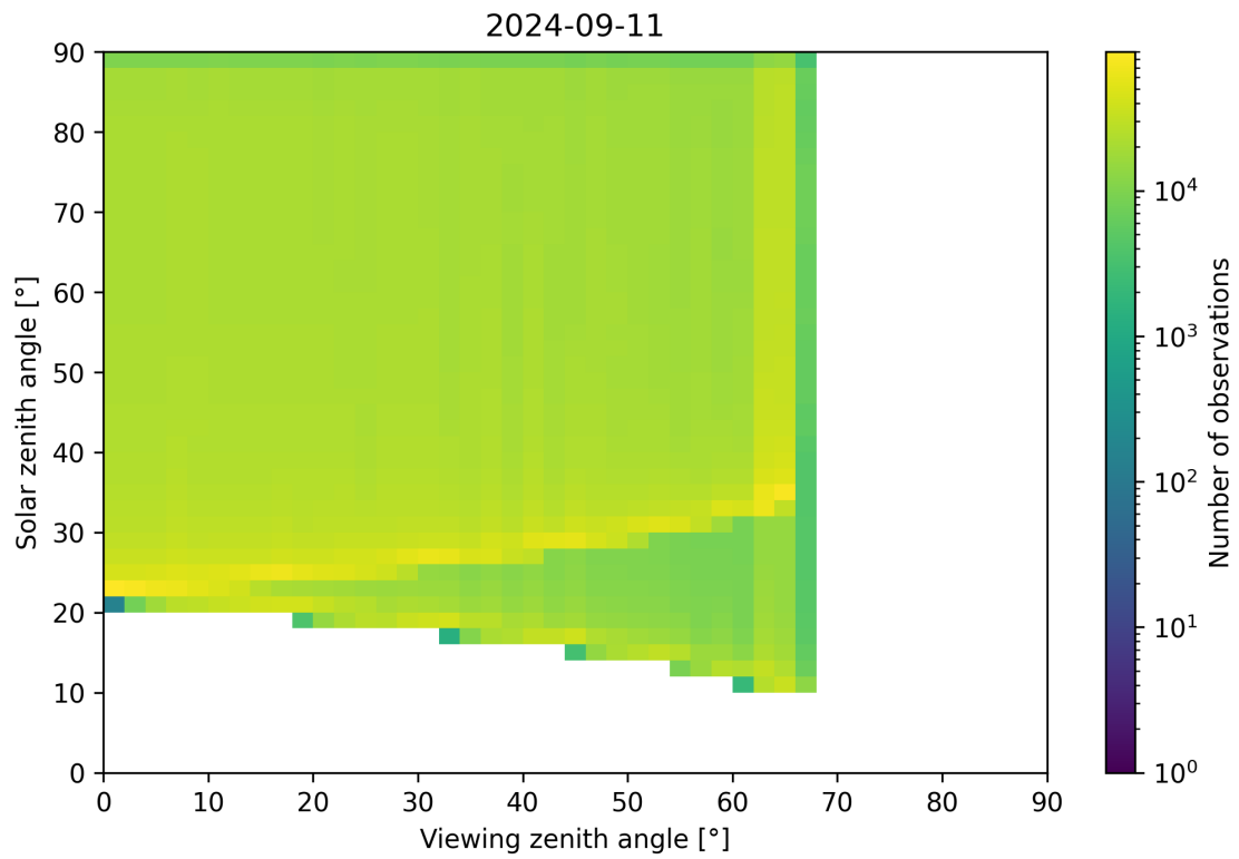
Figure 54: Scatter density plot of “Viewing zenith angle” against “Solar zenith angle” for 2024-09-10 to 2024-09-12.
