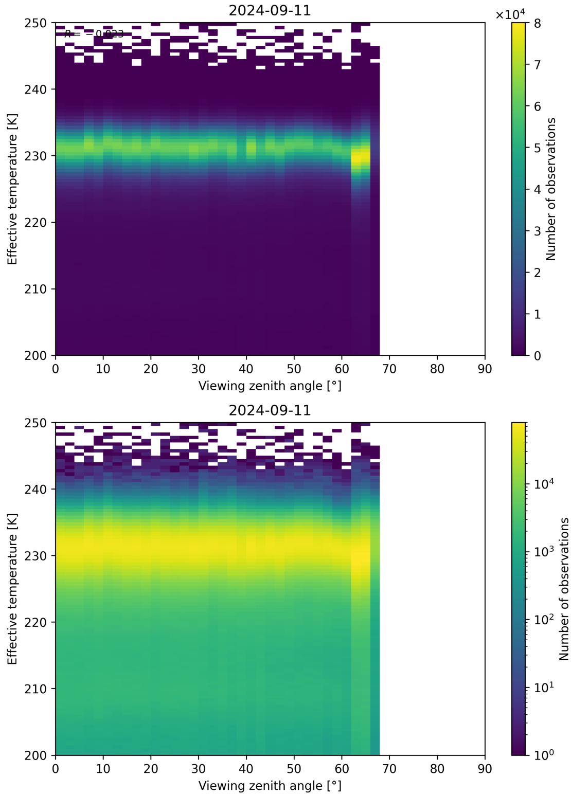
Figure 50: Scatter density plot of “Viewing zenith angle” against “Effective temperature” for 2024-09-10 to 2024-09-12.
