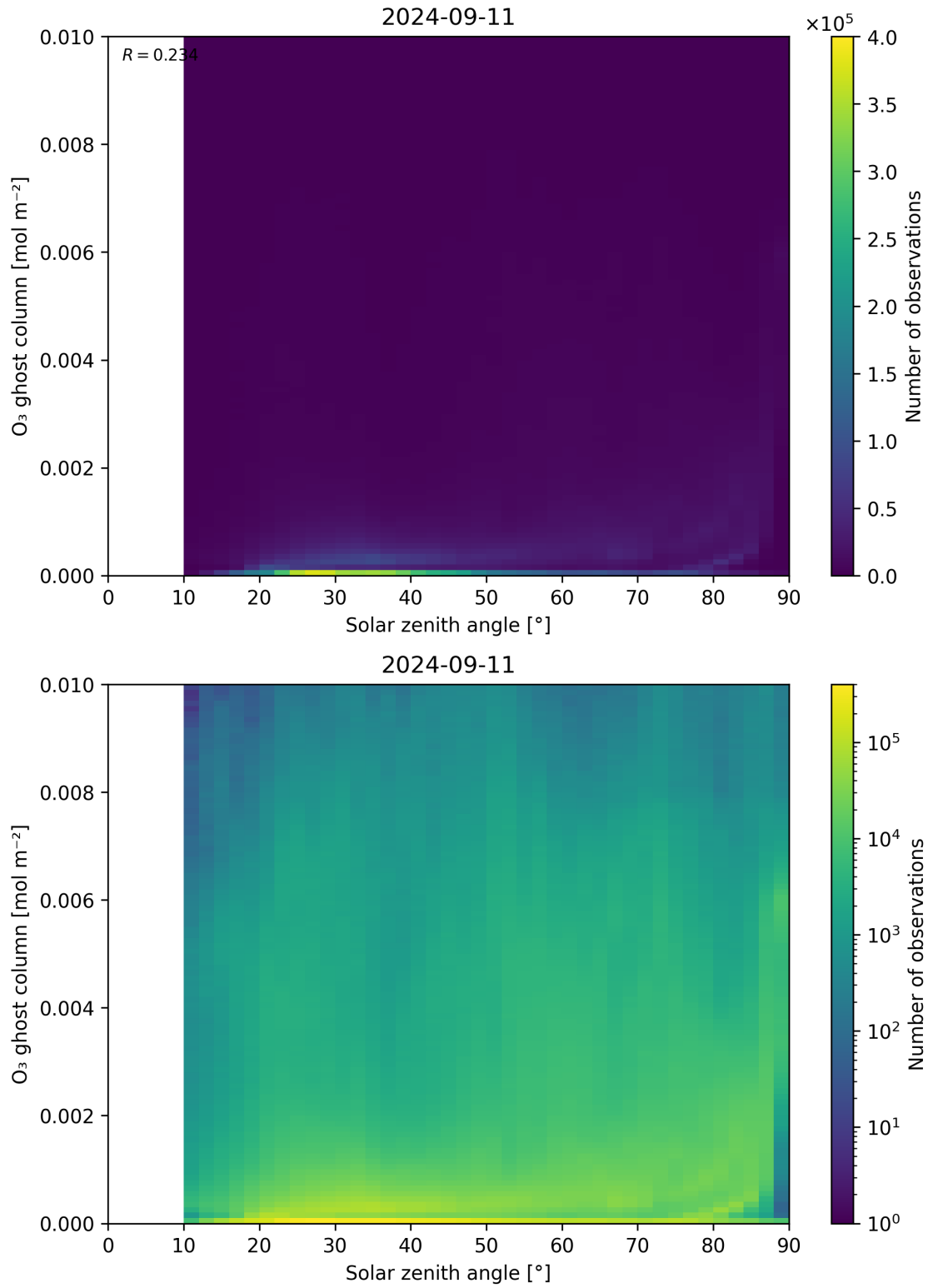
Figure 46: Scatter density plot of “Solar zenith angle” against “O 3 ghost column” for 2024-09-10 to 2024-09-12.
