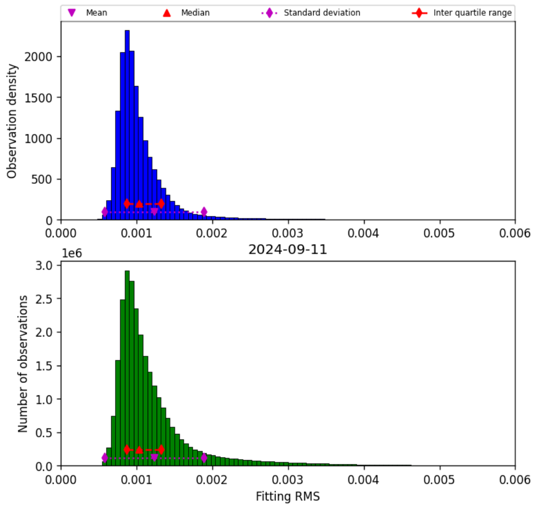
Figure 23: Histogram of “Fitting RMS” for 2024-09-10 to 2024-09-12
