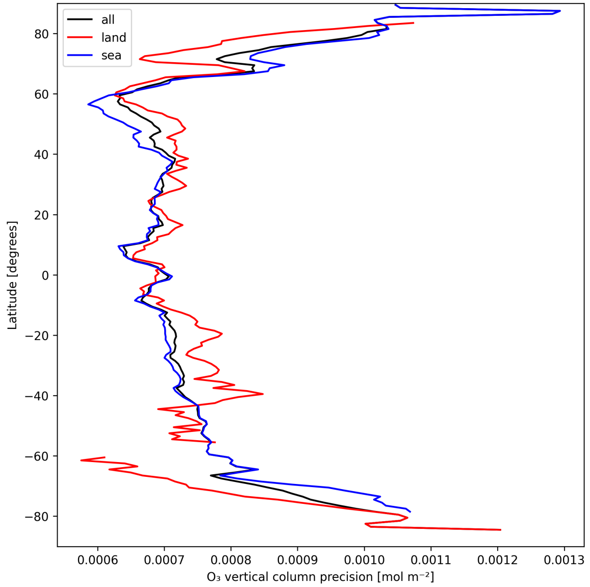
Figure 15: Zonal average of “O 3 vertical column precision” for 2024-09-10 to 2024-09-12.
