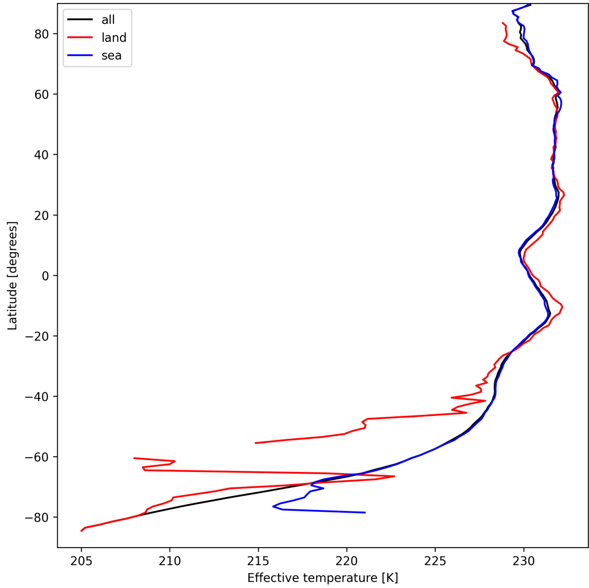
Figure 17: Zonal average of "Effective temperature" for 2024-09-10 to 2024-09-12.
