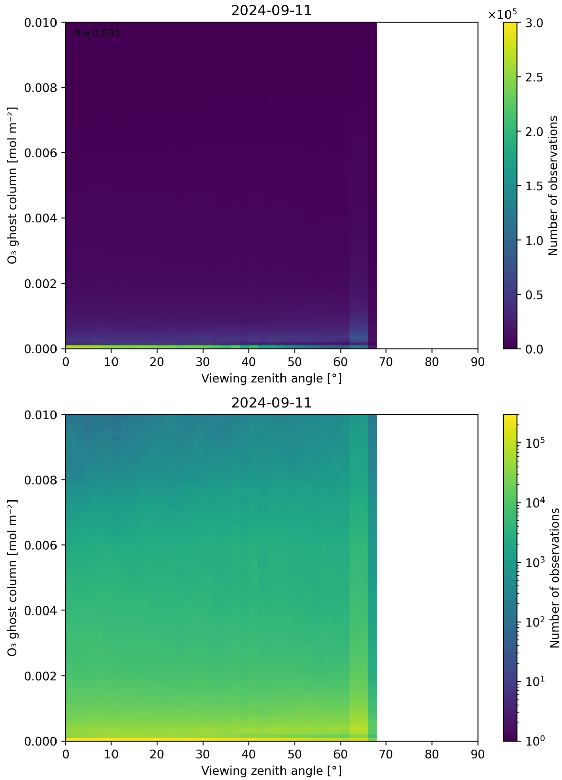
Figure 51: Scatter density plot of “Viewing zenith angle” against “O 3 ghost column” for 2024-09-10 to 2024-09-12.
