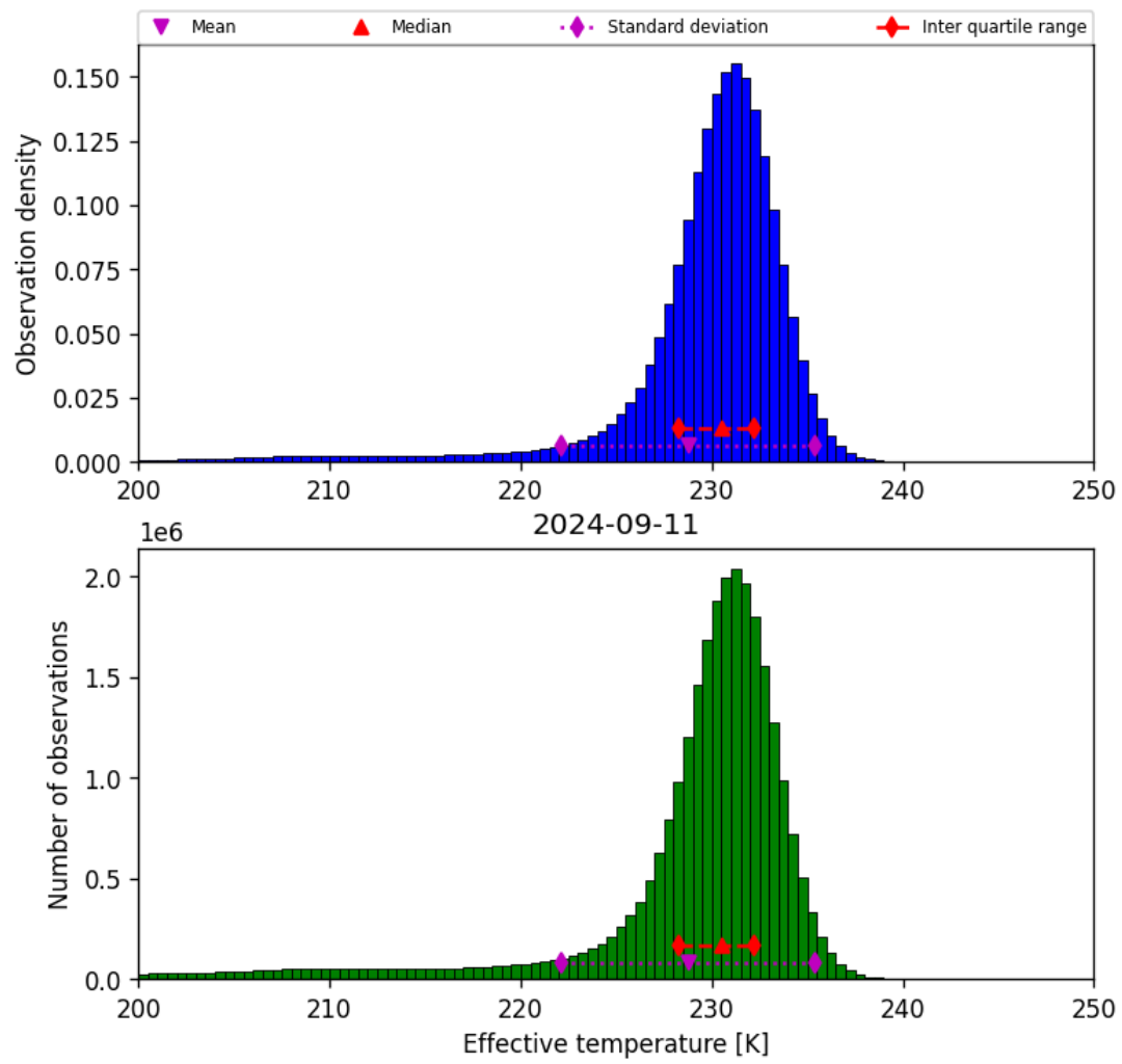
Figure 24: Histogram of “Effective temperature” for 2024-09-10 to 2024-09-12
