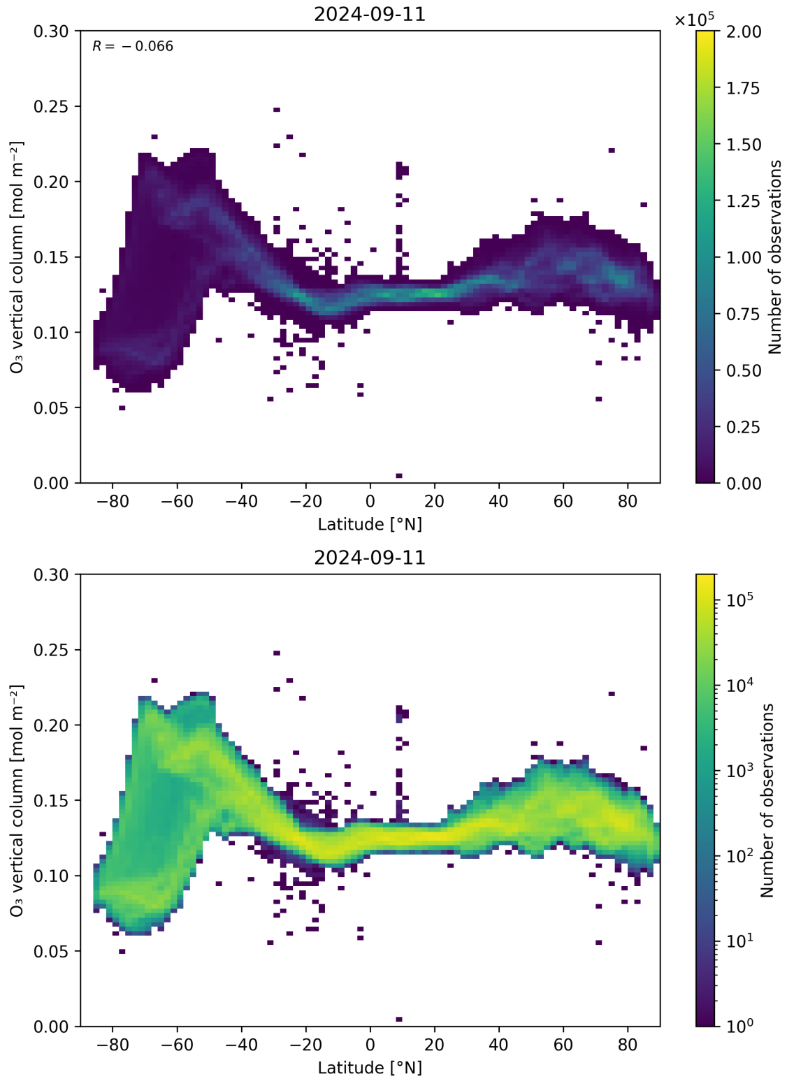
Figure 36: Scatter density plot of “Latitude” against “O 3 vertical column” for 2024-09-10 to 2024-09-12.
