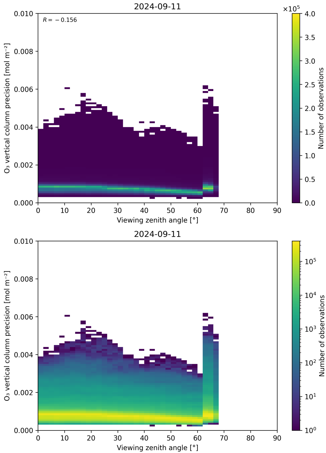
Figure 53: Scatter density plot of “Viewing zenith angle” against “O 3 vertical column precision” for 2024-09-10 to 2024-09-12.
