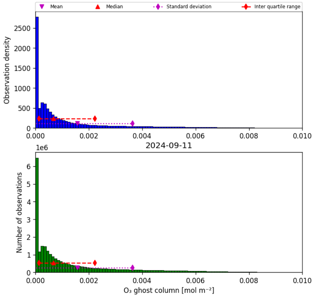
Figure 25: Histogram of "O 3 ghost column" for 2024-09-10 to 2024-09-12
