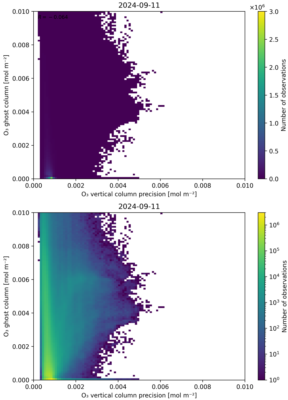
Figure 43: Scatter density plot of “ \text{O}_3 vertical column precision” against “ \text{O}_3 ghost column” for 2024-09-10 to 2024-09-12.
