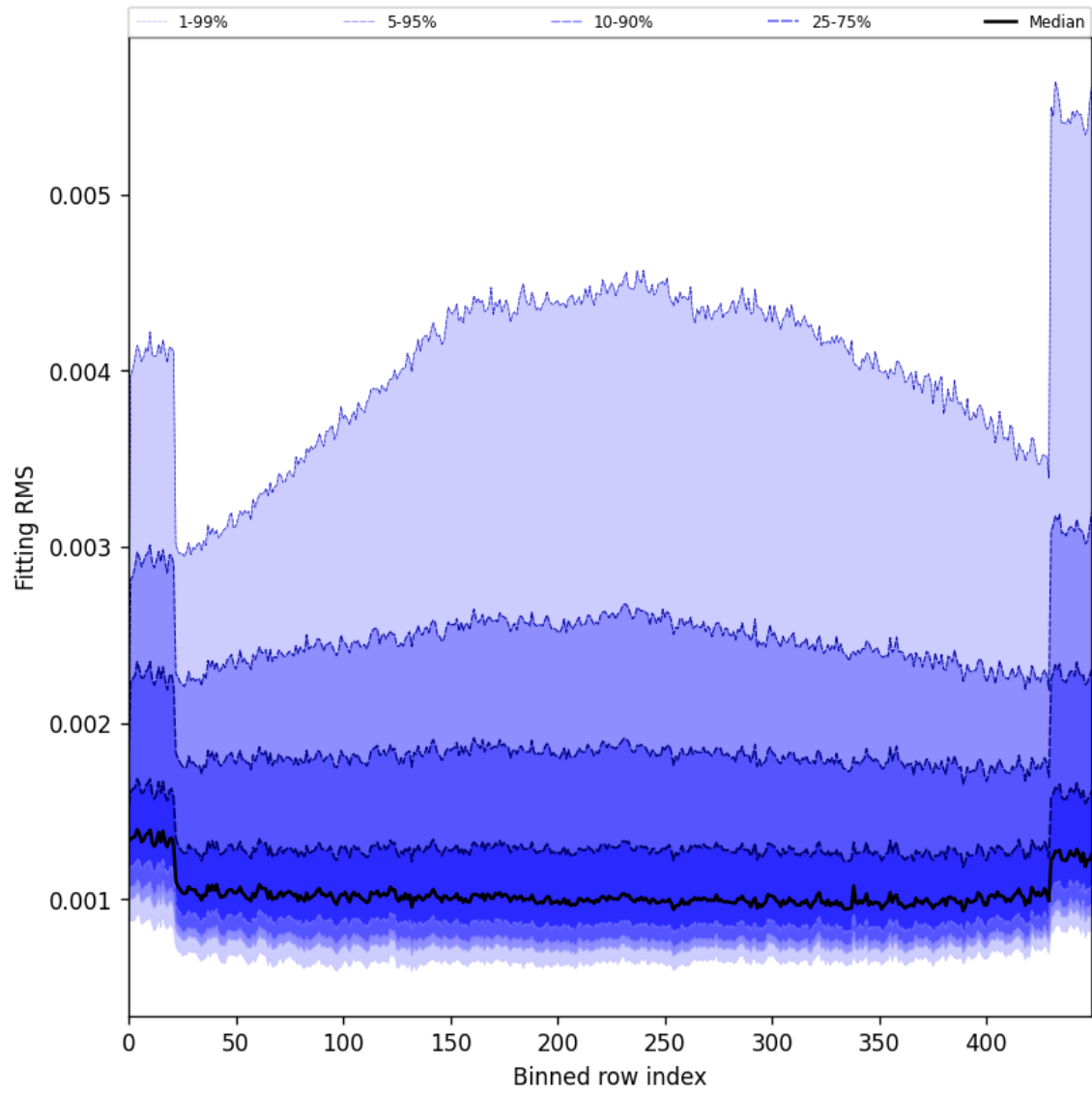
Figure 30: Along track statistics of “Fitting RMS” for 2024-09-10 to 2024-09-12
