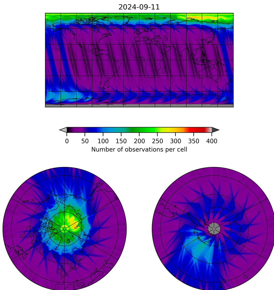
Figure 12: Map of the number of observations for 2024-09-10 to 2024-09-12
