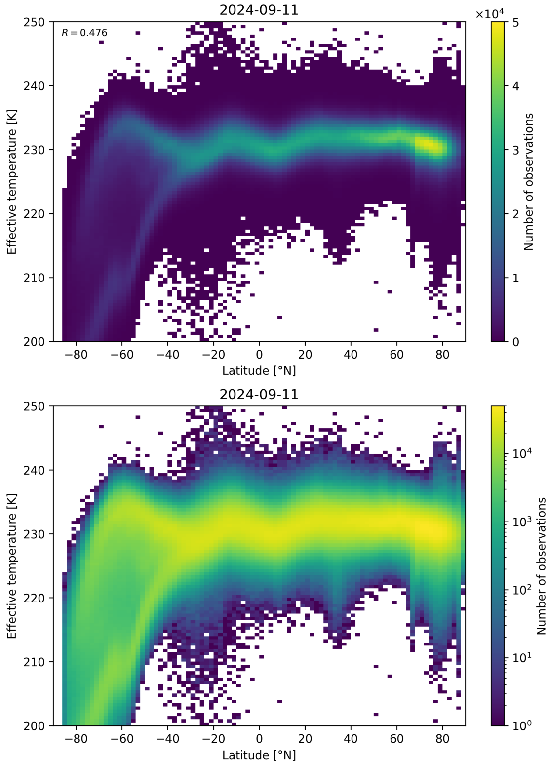
Figure 34: Scatter density plot of “Latitude” against “Effective temperature” for 2024-09-10 to 2024-09-12.
