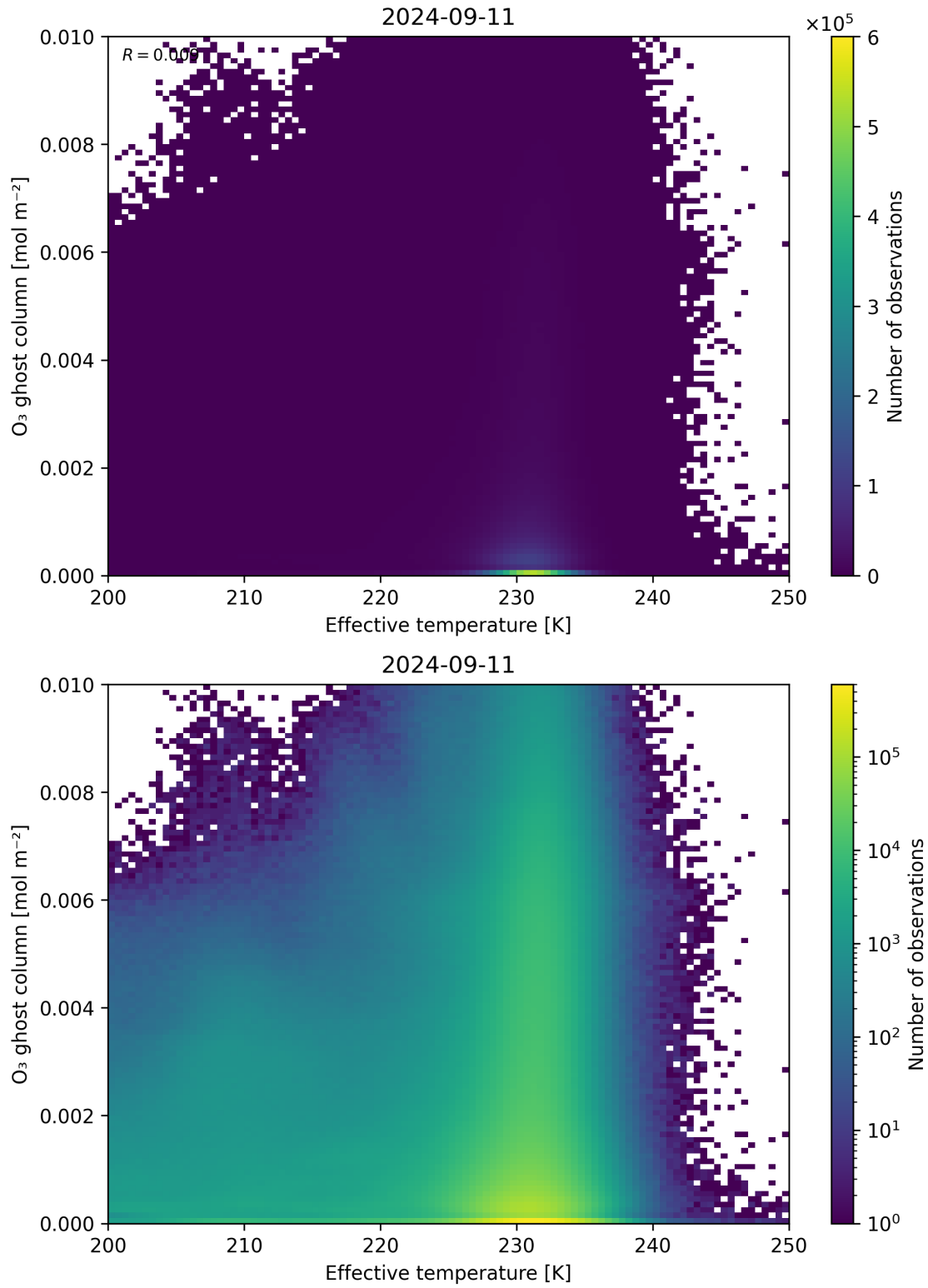
Figure 38: Scatter density plot of “Effective temperature” against “O 3 ghost column” for 2024-09-10 to 2024-09-12.
