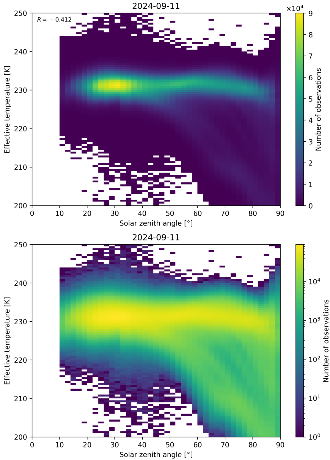
Figure 45: Scatter density plot of “Solar zenith angle” against “Effective temperature” for 2024-09-10 to 2024-09-12.
