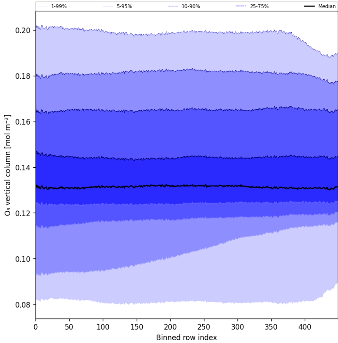
Figure 28: Along track statistics of “O 3 vertical column” for 2024-09-10 to 2024-09-12
