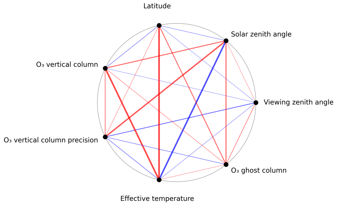
Figure 1: Map of correlation graph for 2024-09-10 to 2024-09-12.
