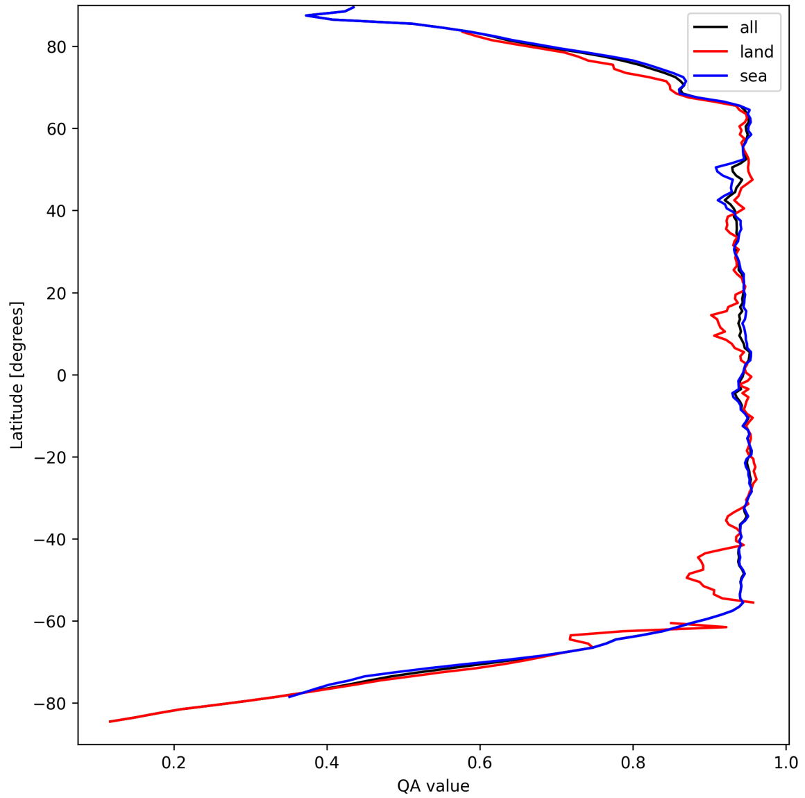
Figure 13: Zonal average of “QA value” for 2024-09-10 to 2024-09-12.
