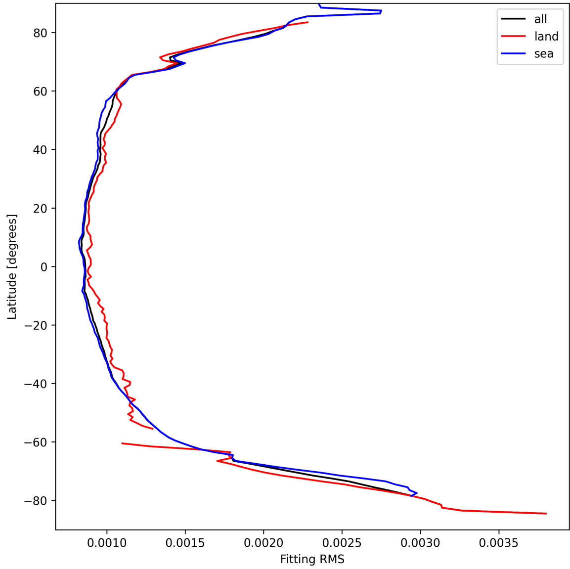
Figure 16: Zonal average of “Fitting RMS” for 2024-09-10 to 2024-09-12.
