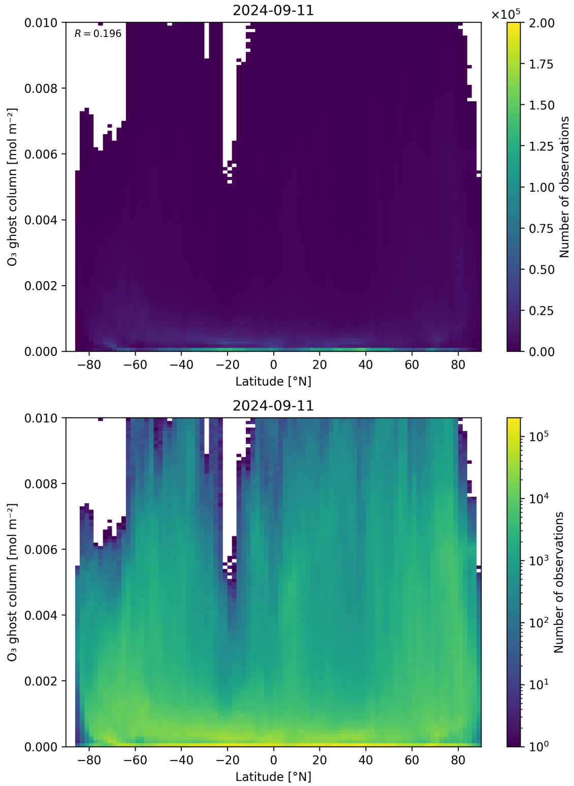
Figure 35: Scatter density plot of “Latitude” against “O 3 ghost column” for 2024-09-10 to 2024-09-12.
