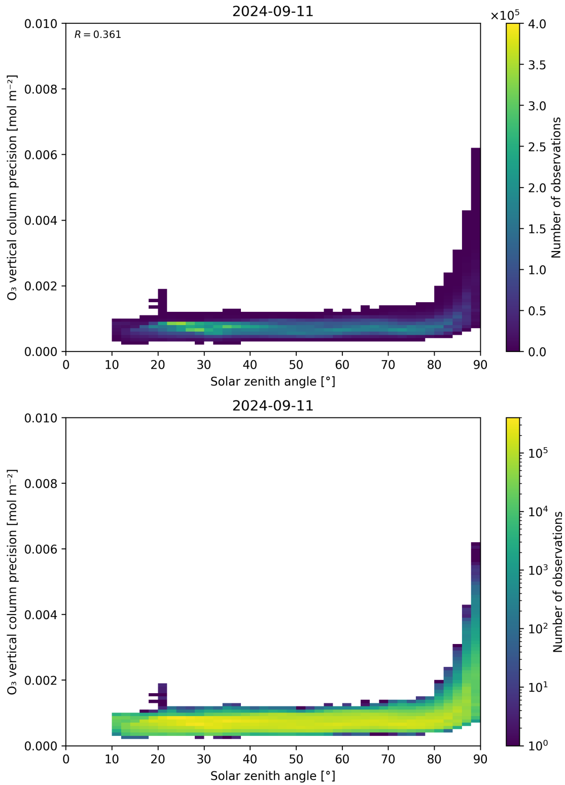
Figure 48: Scatter density plot of “Solar zenith angle” against “O 3 vertical column precision” for 2024-09-10 to 2024-09-12.
