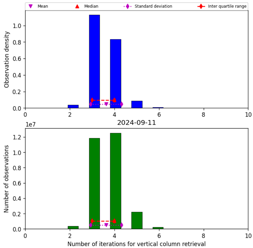
Figure 26: Histogram of “Number of iterations for vertical column retrieval” for 2024-09-10 to 2024-09-12
