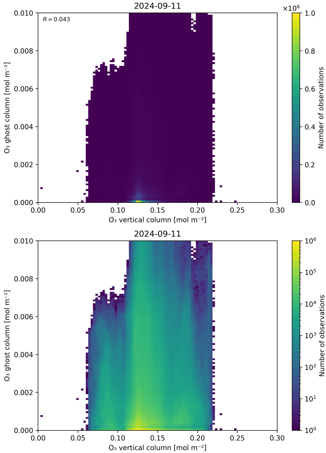
Figure 40: Scatter density plot of “O 3 vertical column” against “O 3 ghost column” for 2024-09-10 to 2024-09-12.
