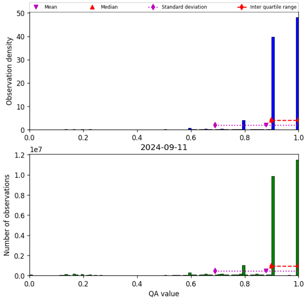
Figure 20: Histogram of “QA value” for 2024-09-10 to 2024-09-12
