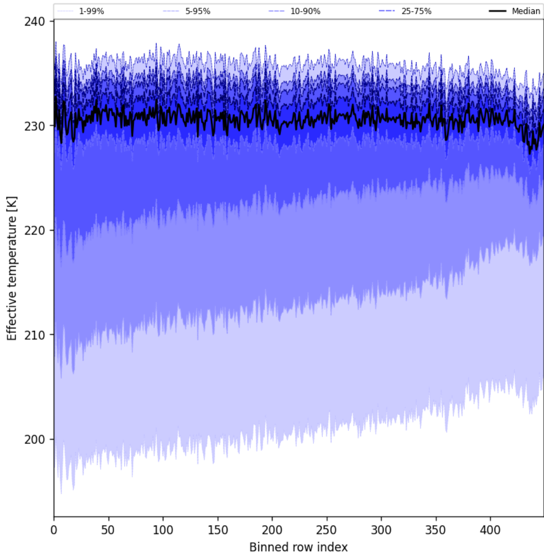
Figure 31: Along track statistics of “Effective temperature” for 2024-09-10 to 2024-09-12
