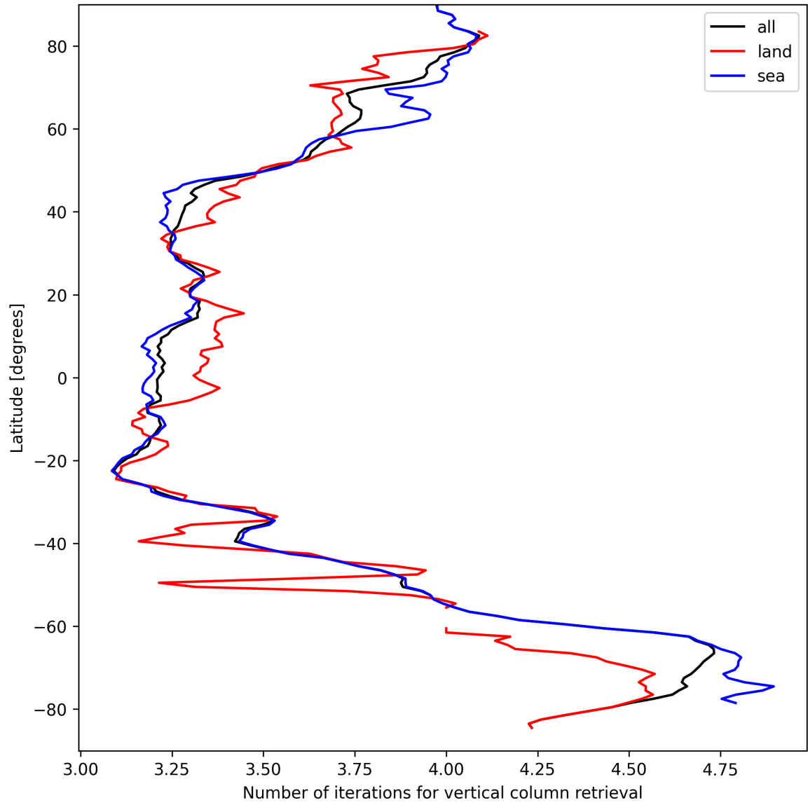
Figure 19: Zonal average of “Number of iterations for vertical column retrieval” for 2024-09-10 to 2024-09-12.
