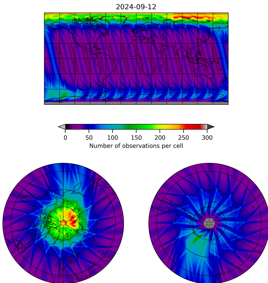
Figure 12: Map of the number of observations for 2024-09-12 to 2024-09-13
