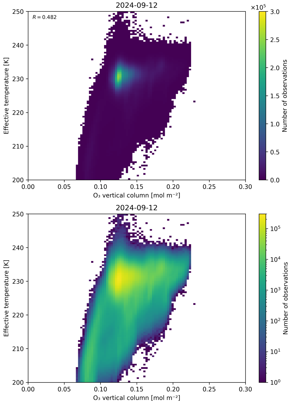
Figure 39: Scatter density plot of “O 3 vertical column” against “Effective temperature” for 2024-09-12 to 2024-09-13.
