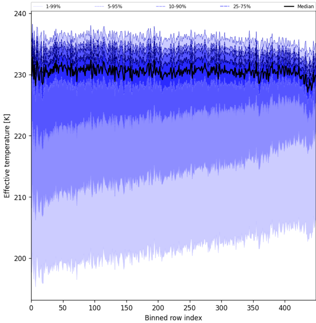
Figure 31: Along track statistics of “Effective temperature” for 2024-09-12 to 2024-09-13
