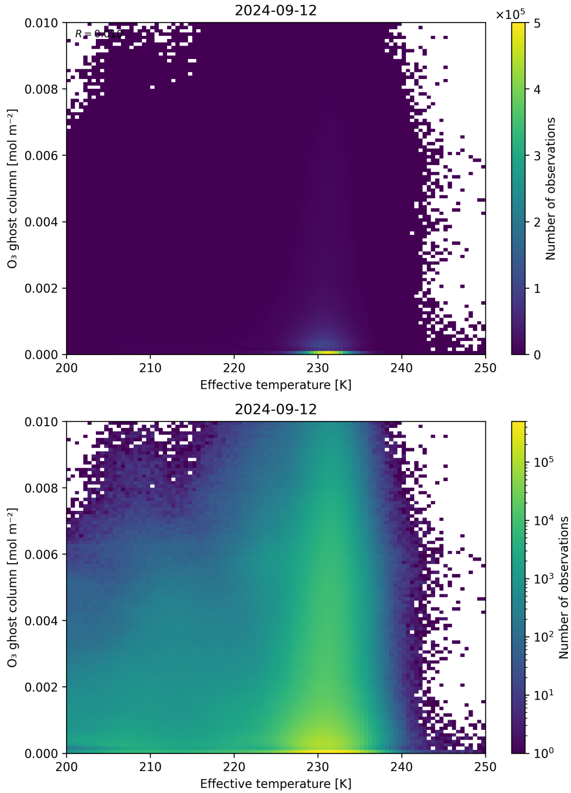
Figure 38: Scatter density plot of “Effective temperature” against “O 3 ghost column” for 2024-09-12 to 2024-09-13.
