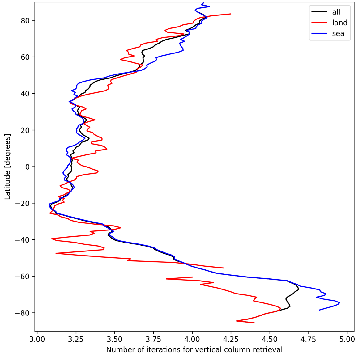
Figure 19: Zonal average of “Number of iterations for vertical column retrieval” for 2024-09-12 to 2024-09-13.
