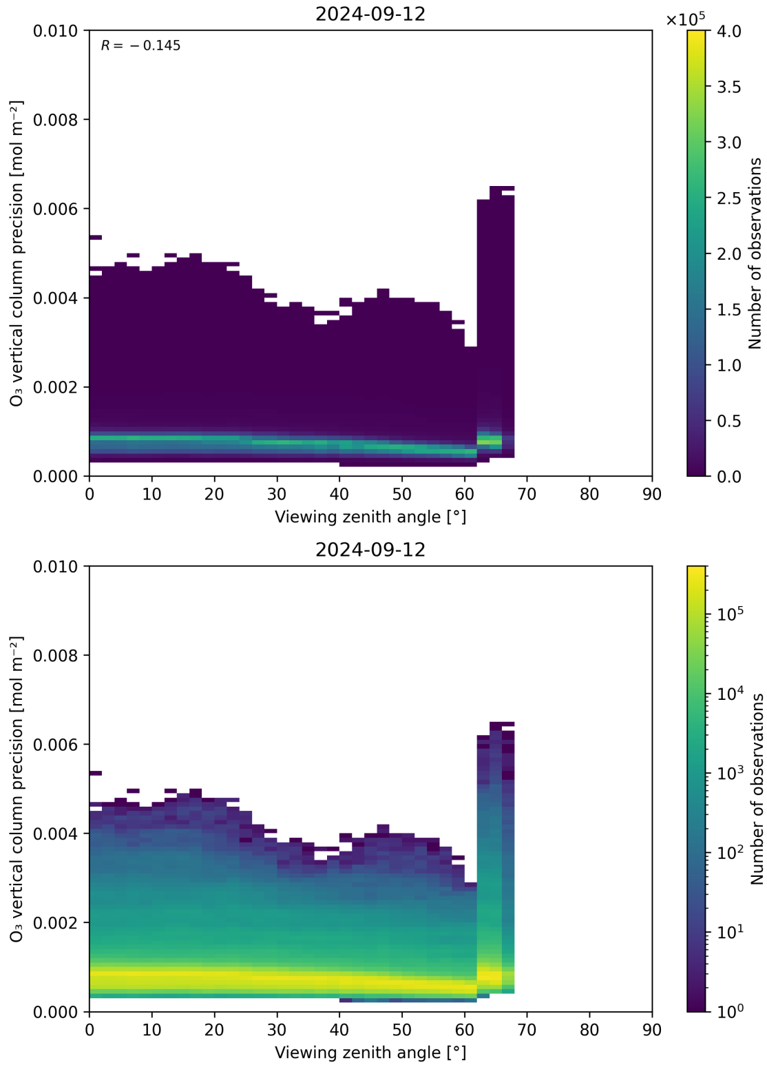
Figure 53: Scatter density plot of “Viewing zenith angle” against “O 3 vertical column precision” for 2024-09-12 to 2024-09-13.
