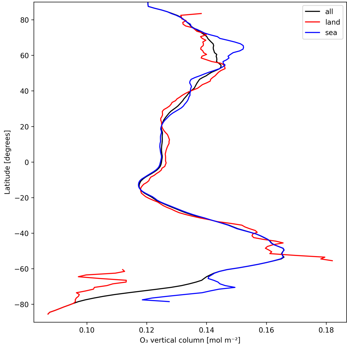
Figure 14: Zonal average of “O 3 vertical column” for 2024-09-12 to 2024-09-13.
