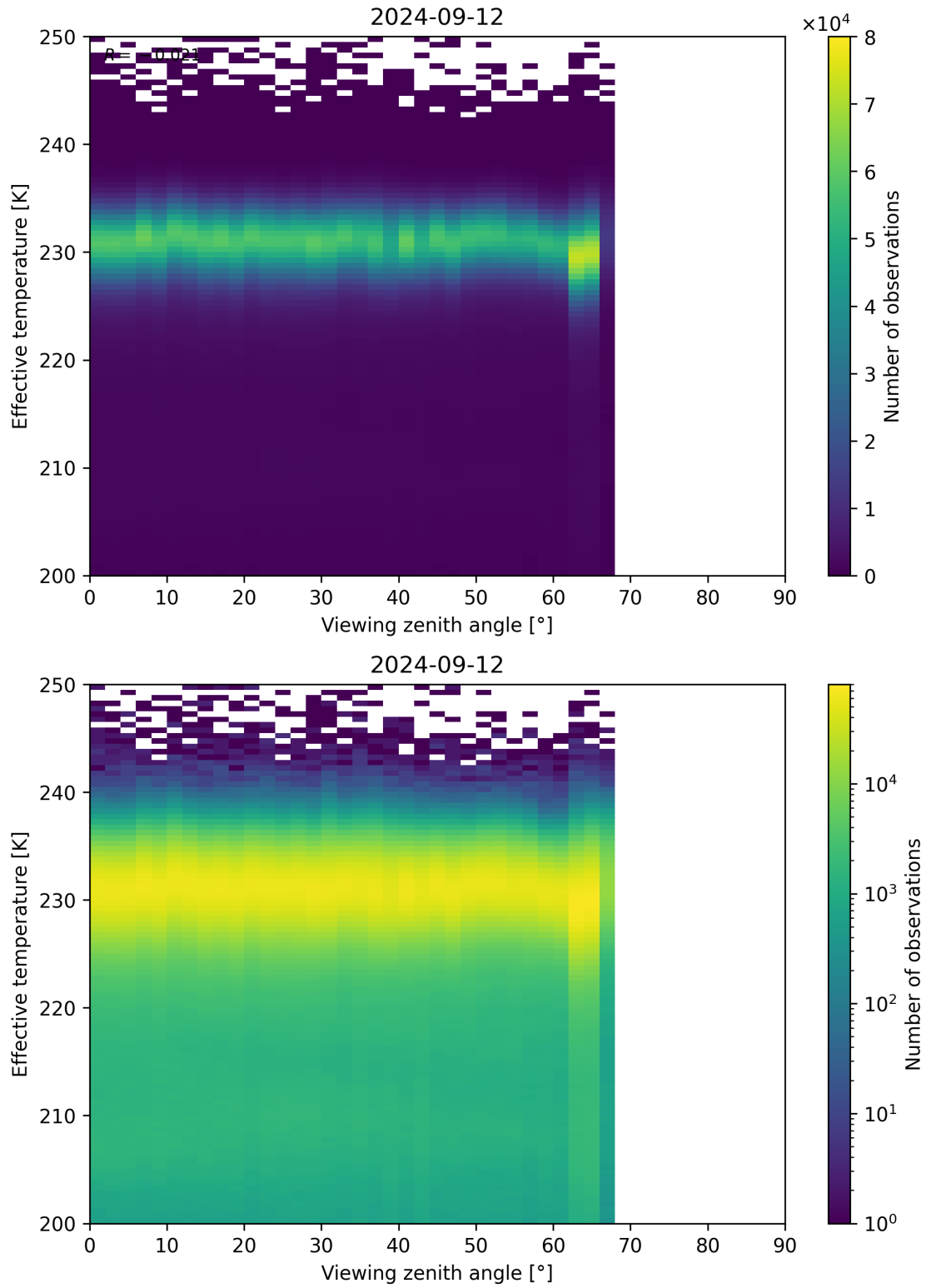
Figure 50: Scatter density plot of “Viewing zenith angle” against “Effective temperature” for 2024-09-12 to 2024-09-13.
