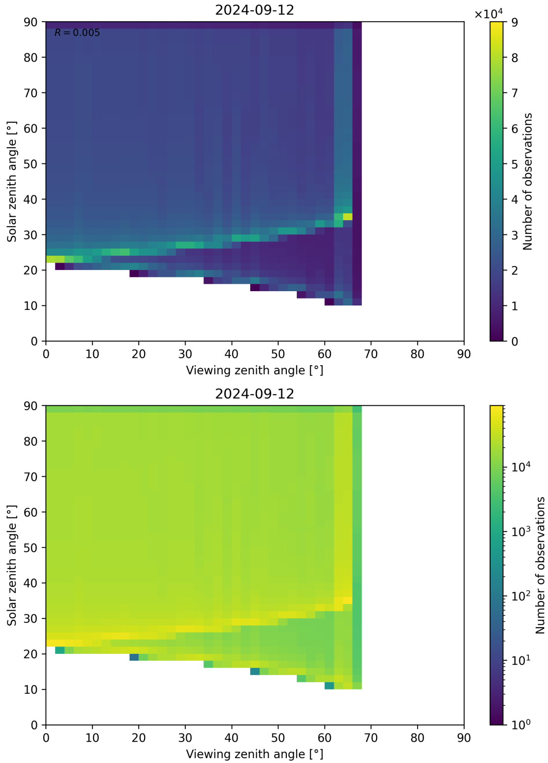
Figure 54: Scatter density plot of “Viewing zenith angle” against “Solar zenith angle” for 2024-09-12 to 2024-09-13.
