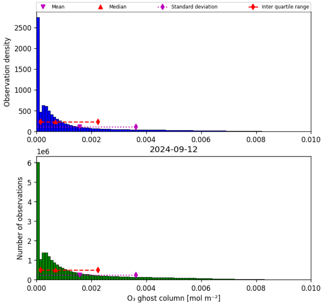
Figure 25: Histogram of “O 3 ghost column” for 2024-09-12 to 2024-09-13
