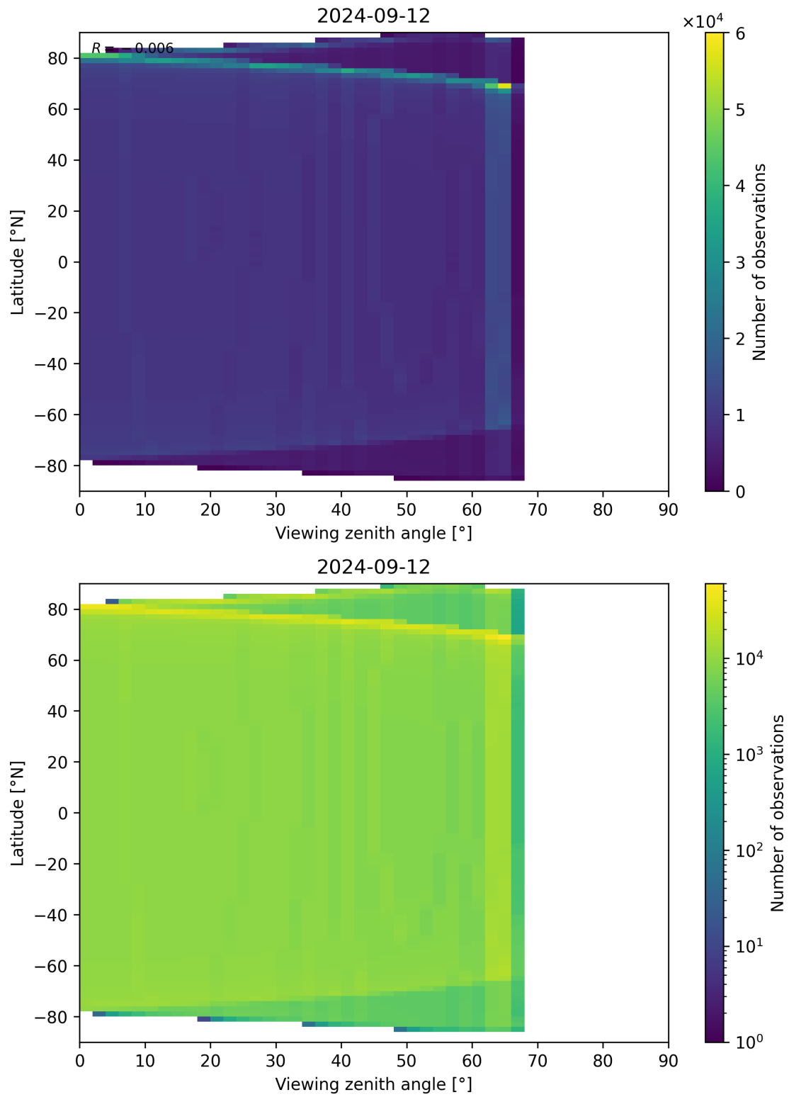
Figure 49: Scatter density plot of “Viewing zenith angle” against “Latitude” for 2024-09-12 to 2024-09-13.
