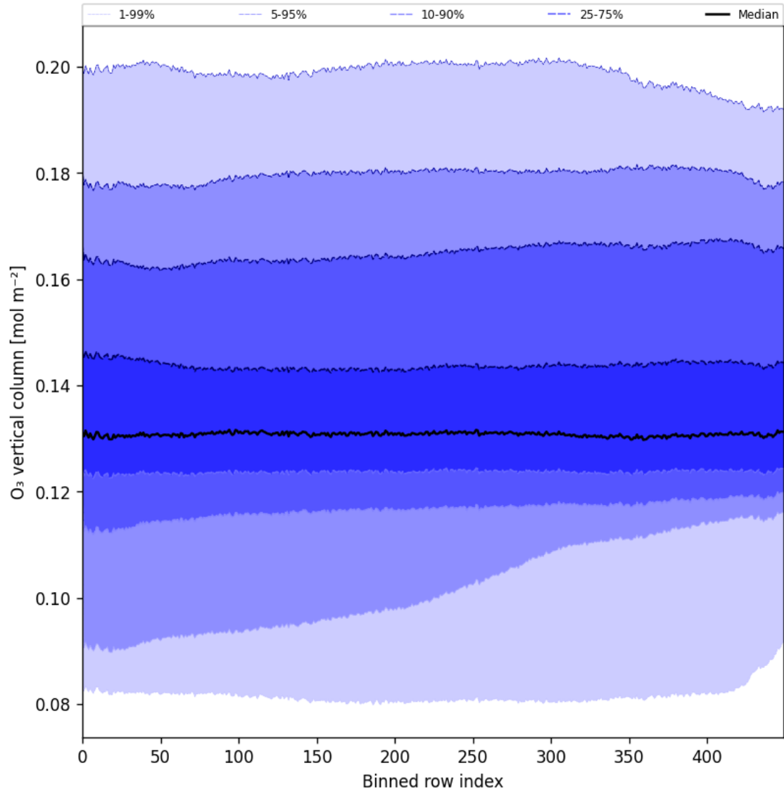
Figure 28: Along track statistics of “O 3 vertical column” for 2024-09-12 to 2024-09-13
