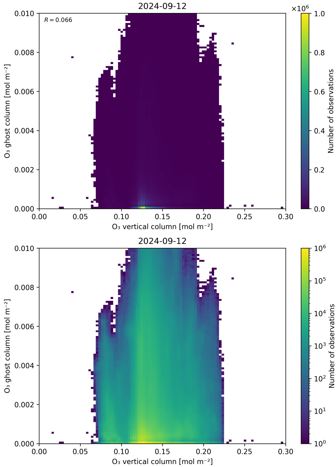
Figure 40: Scatter density plot of “O 3 vertical column” against “O 3 ghost column” for 2024-09-12 to 2024-09-13.
