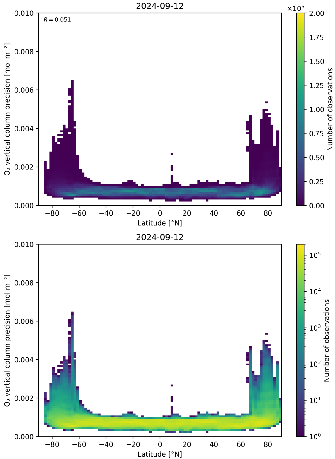
Figure 37: Scatter density plot of “Latitude” against “O 3 vertical column precision” for 2024-09-12 to 2024-09-13.
