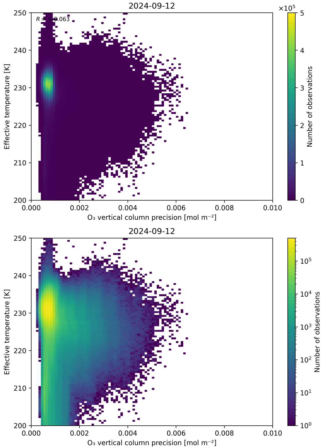
Figure 42: Scatter density plot of “O 3 vertical column precision” against “Effective temperature” for 2024-09-12 to 2024-09-13.
