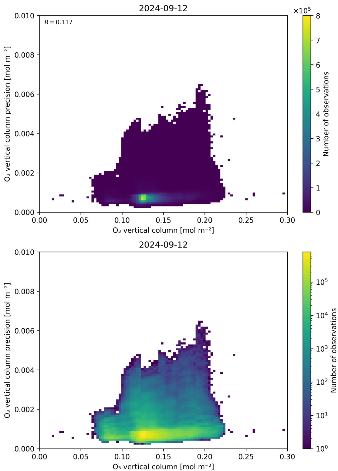
Figure 41: Scatter density plot of “O 3 vertical column” against “O 3 vertical column precision” for 2024-09-12 to 2024-09-13.
