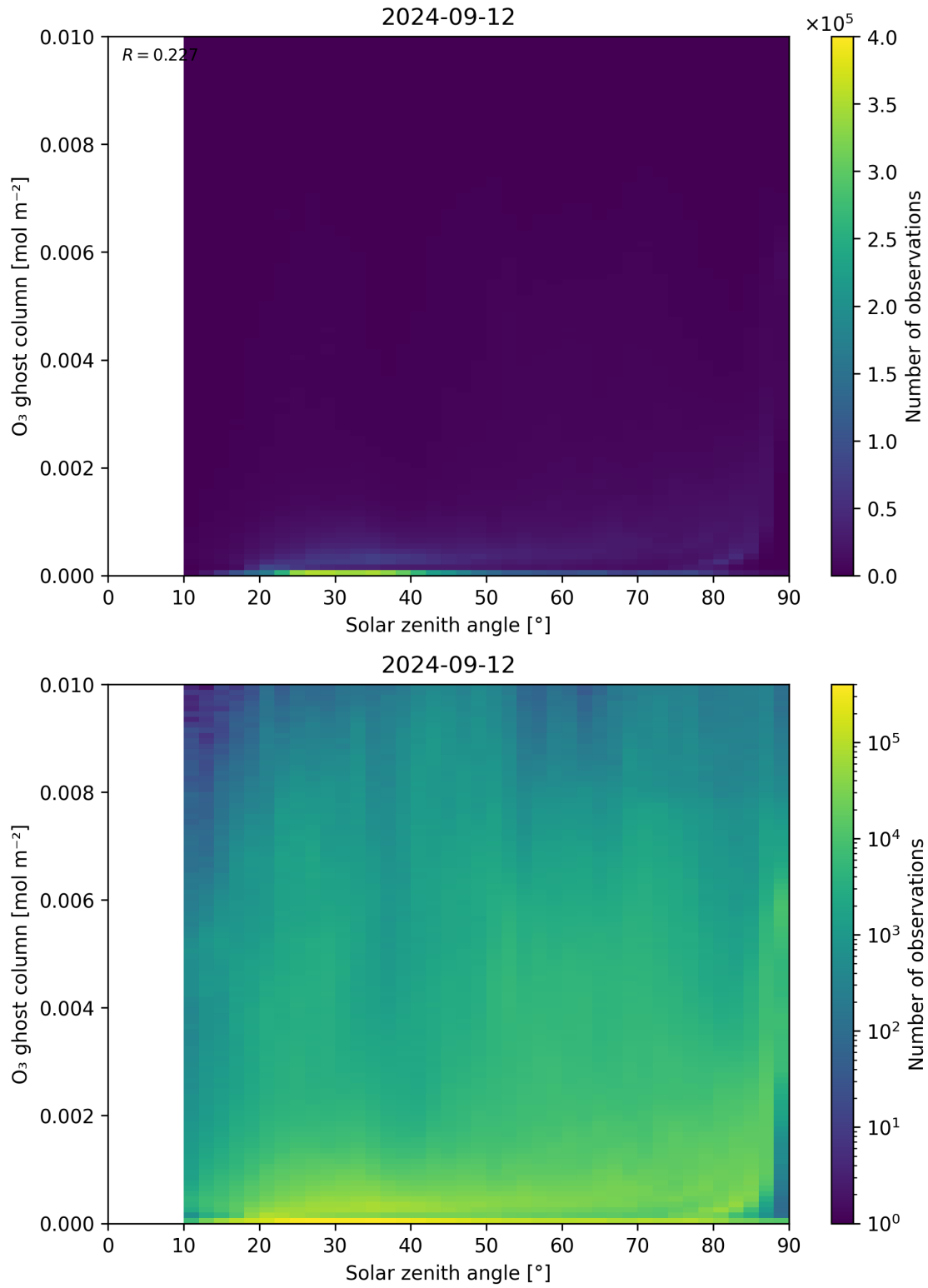
Figure 46: Scatter density plot of “Solar zenith angle” against “O 3 ghost column” for 2024-09-12 to 2024-09-13.
