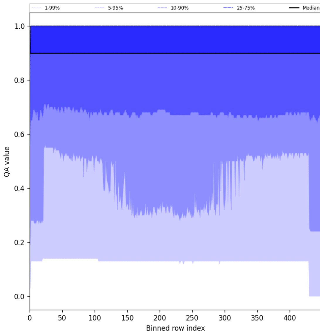
Figure 27: Along track statistics of “QA value” for 2024-09-12 to 2024-09-13
