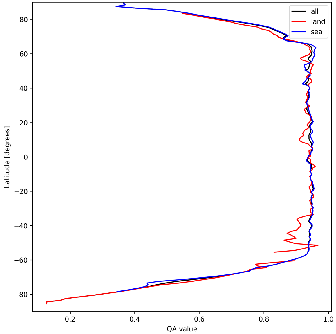
Figure 13: Zonal average of “QA value” for 2024-09-12 to 2024-09-13.
