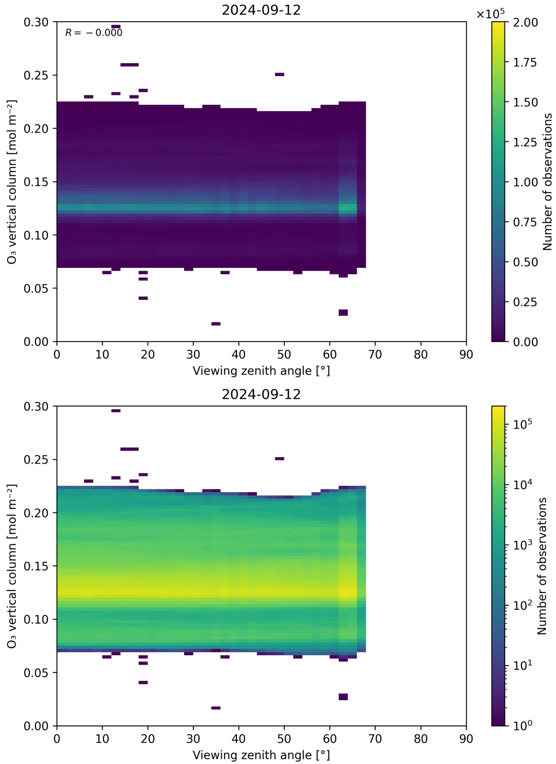
Figure 52: Scatter density plot of “Viewing zenith angle” against “O 3 vertical column” for 2024-09-12 to 2024-09-13.
