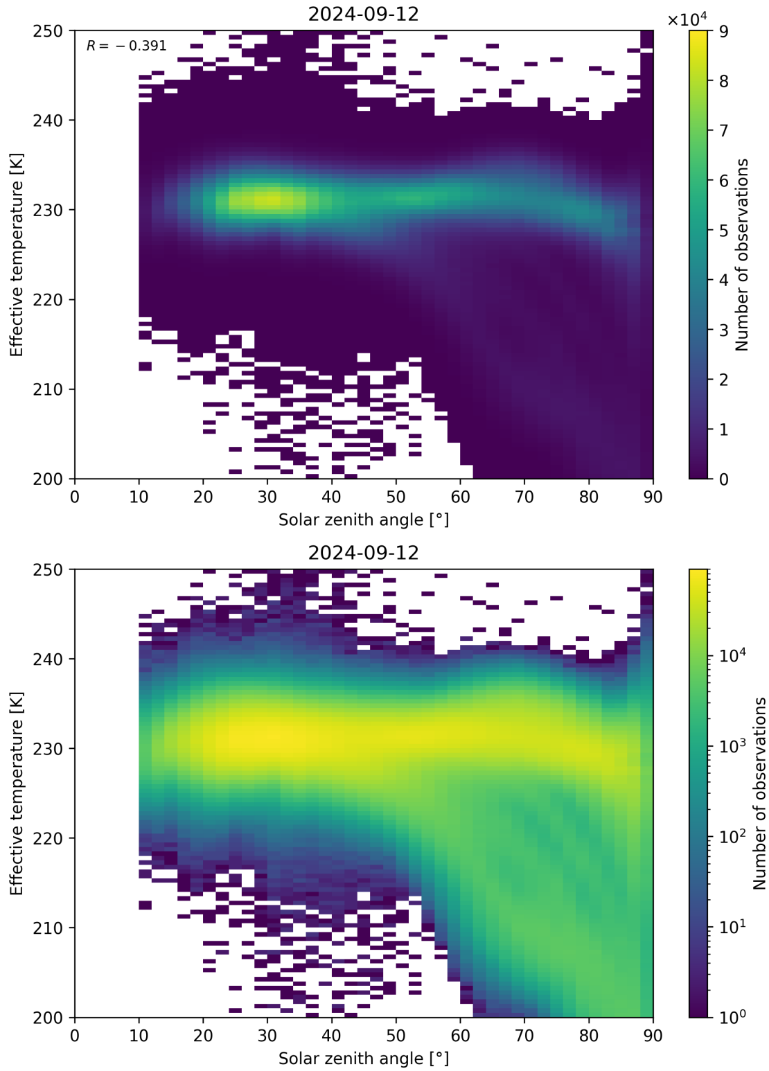
Figure 45: Scatter density plot of “Solar zenith angle” against “Effective temperature” for 2024-09-12 to 2024-09-13.
