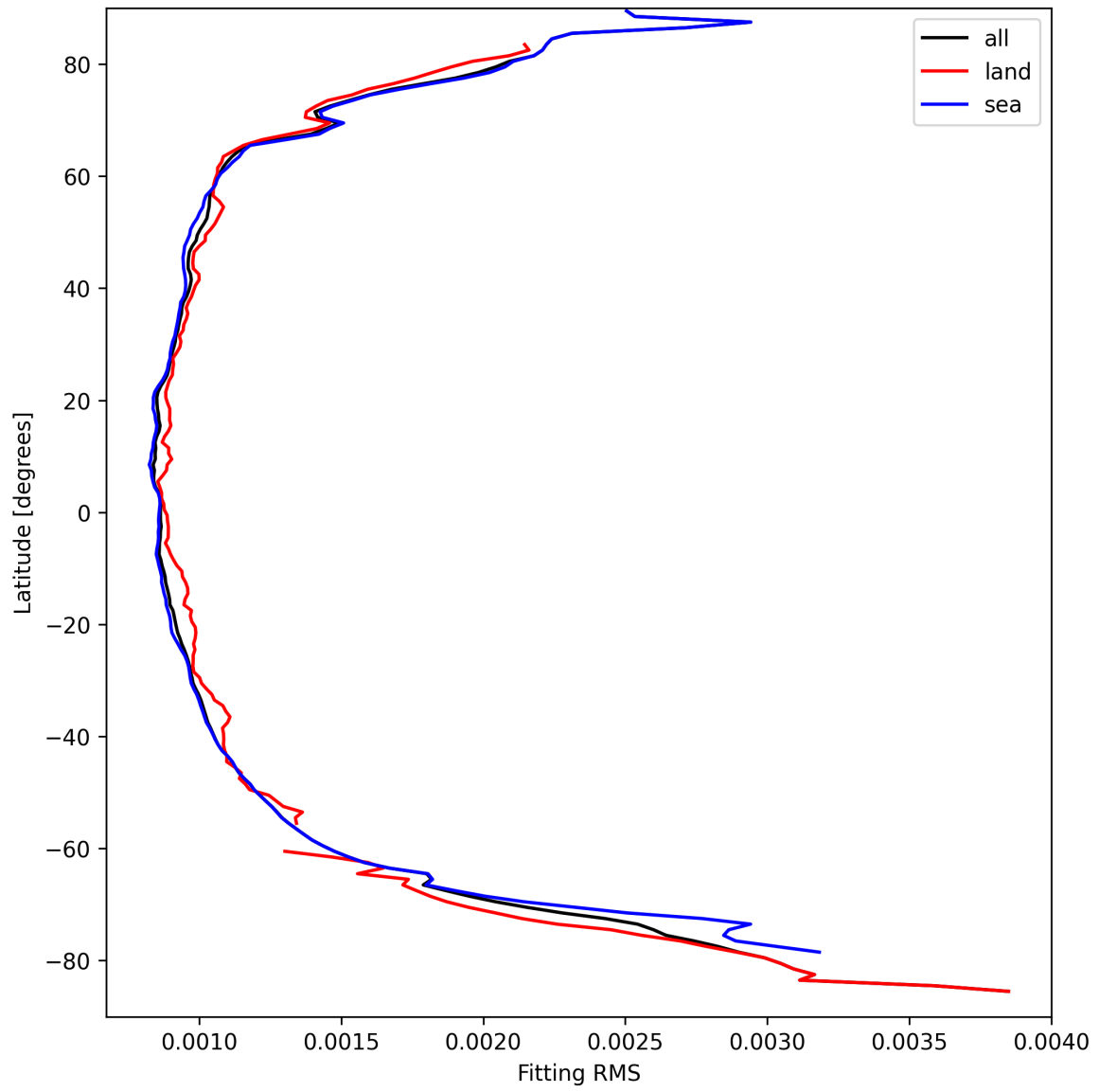
Figure 16: Zonal average of “Fitting RMS” for 2024-09-12 to 2024-09-13.
