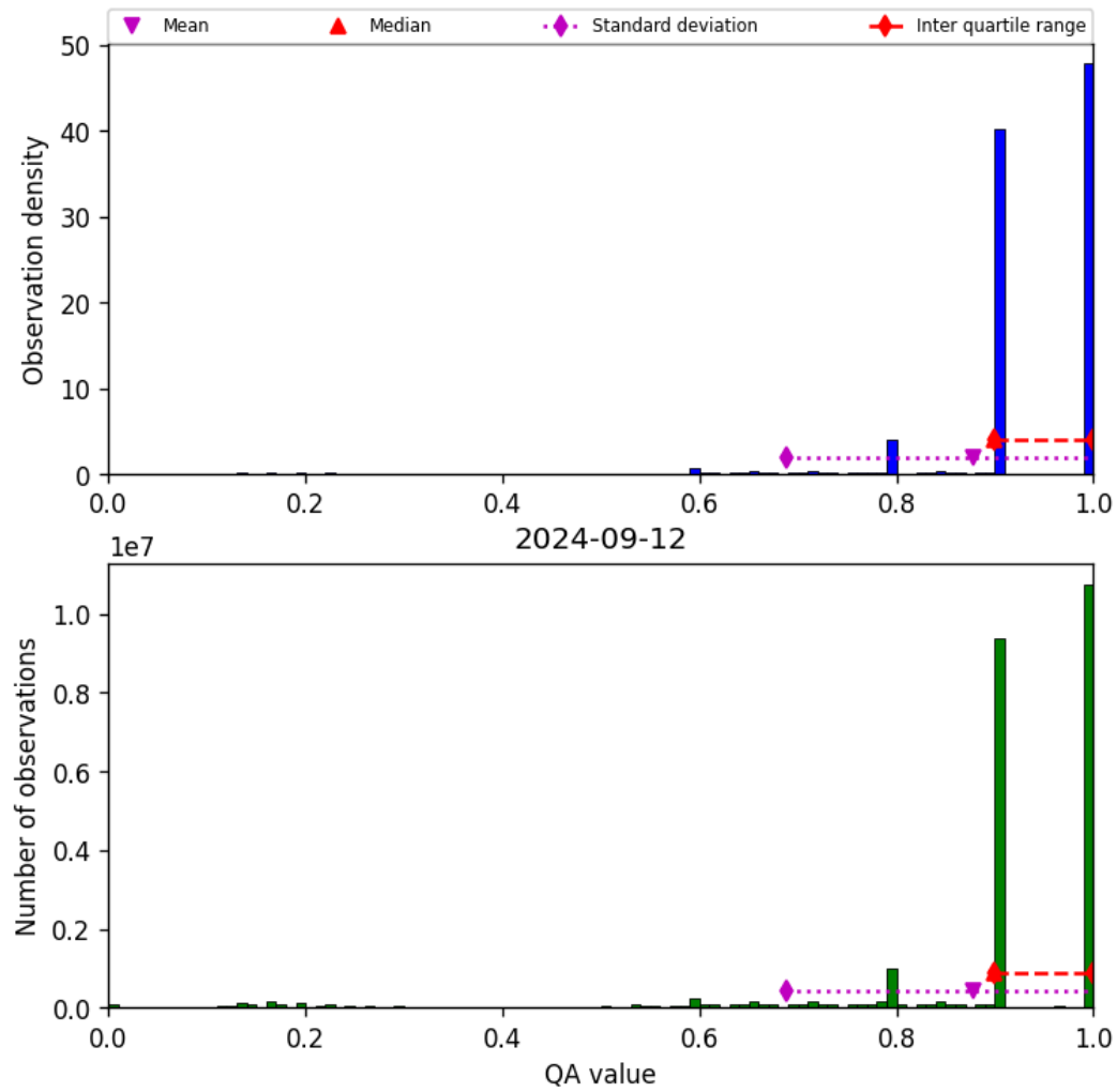
Figure 20: Histogram of “QA value” for 2024-09-12 to 2024-09-13
