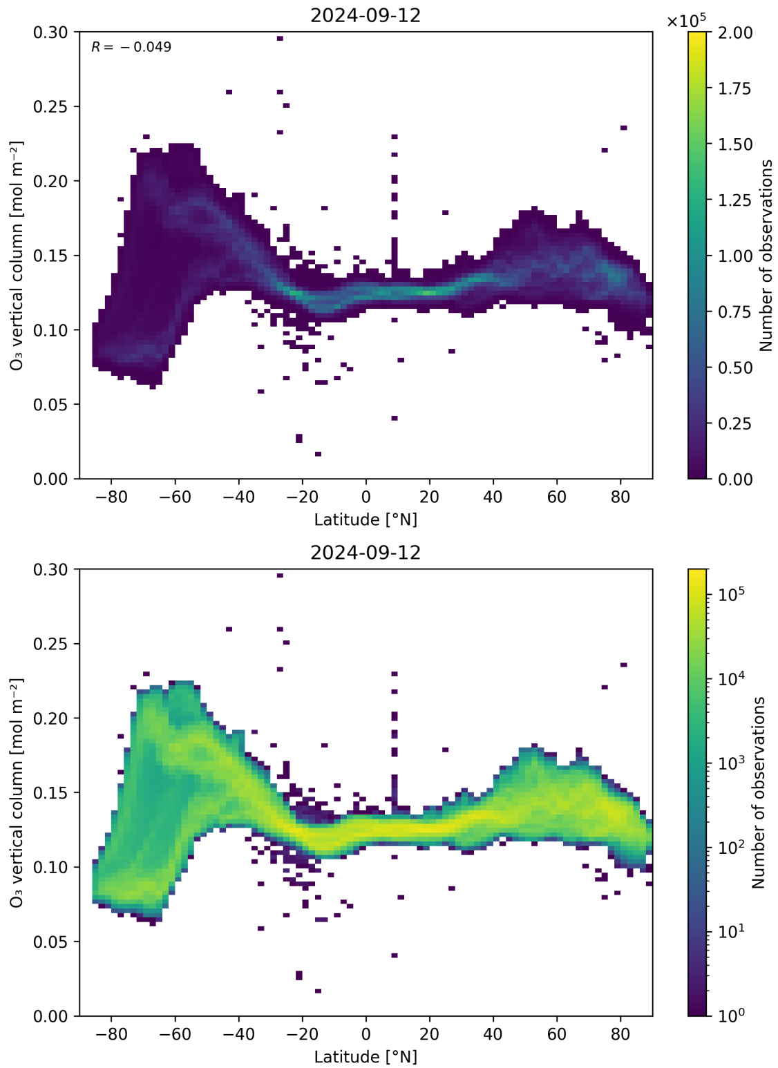
Figure 36: Scatter density plot of “Latitude” against “O 3 vertical column” for 2024-09-12 to 2024-09-13.
