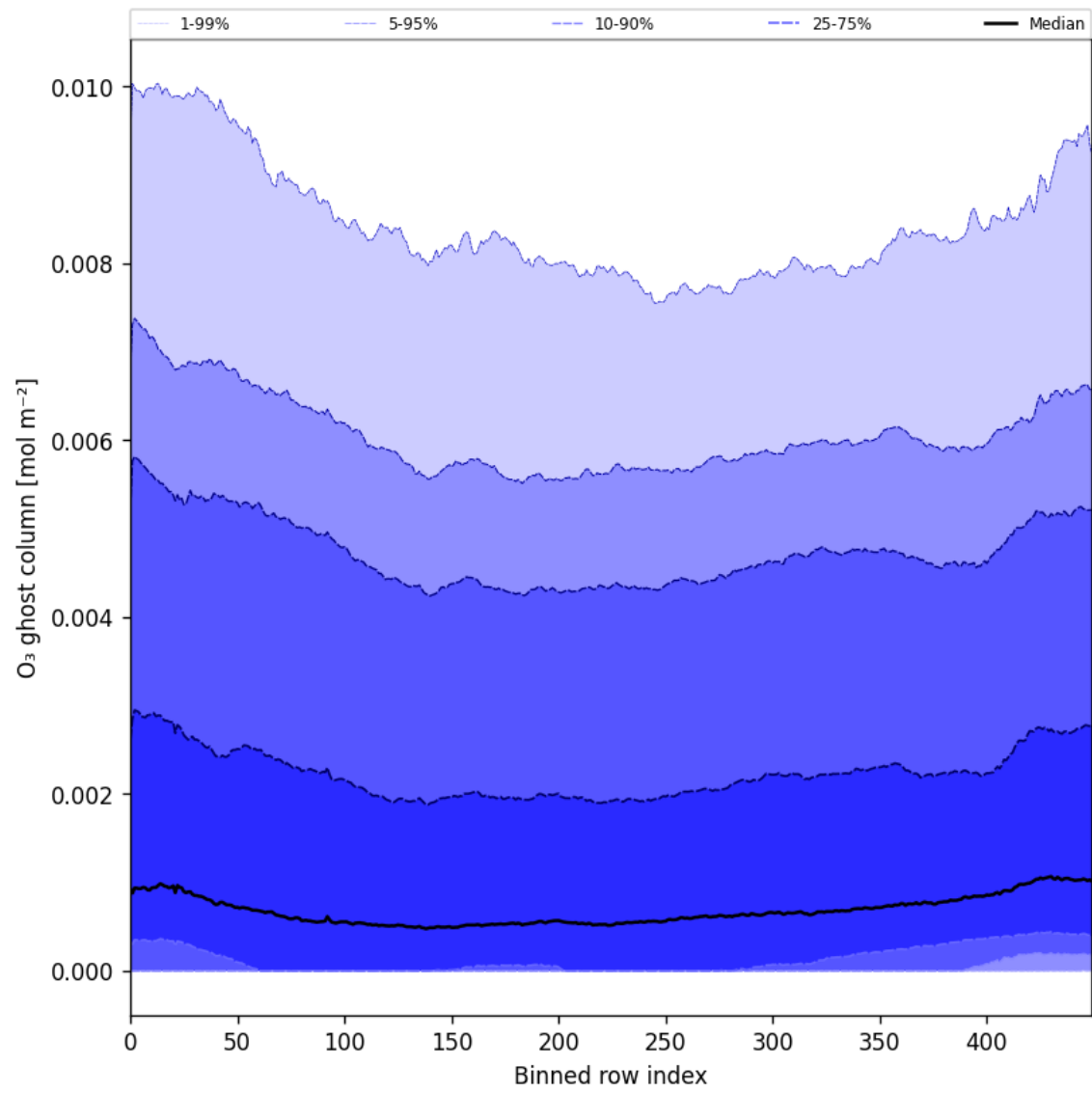
Figure 32: Along track statistics of “O 3 ghost column” for 2024-09-12 to 2024-09-13
