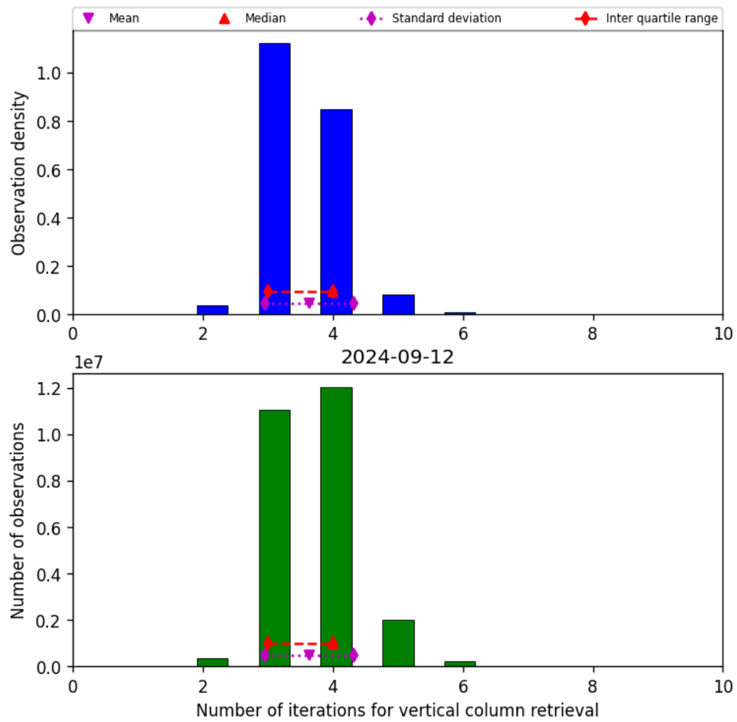
Figure 26: Histogram of “Number of iterations for vertical column retrieval” for 2024-09-12 to 2024-09-13
