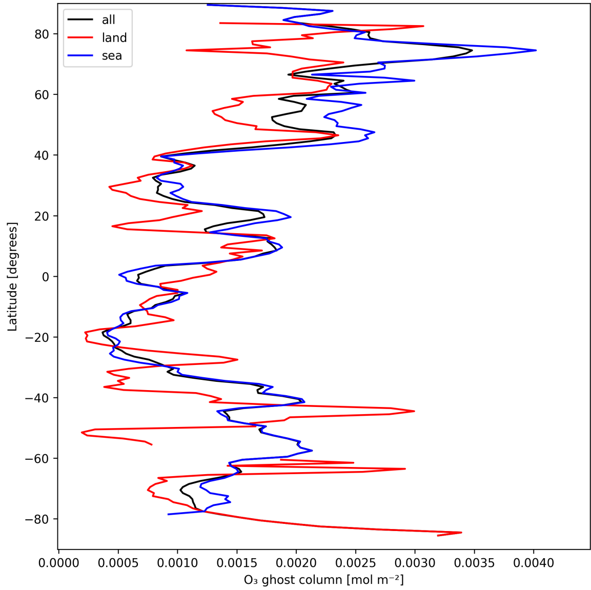
Figure 18: Zonal average of “O 3 ghost column” for 2024-09-12 to 2024-09-13.
