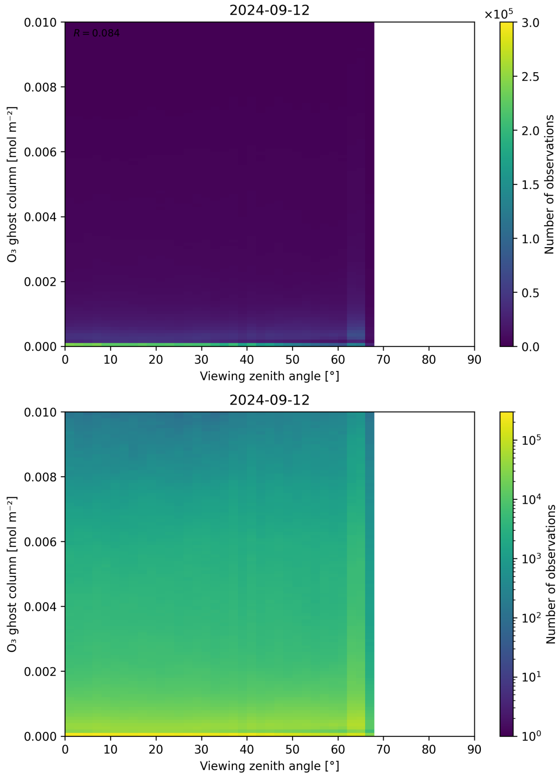
Figure 51: Scatter density plot of “Viewing zenith angle” against “O 3 ghost column” for 2024-09-12 to 2024-09-13.
