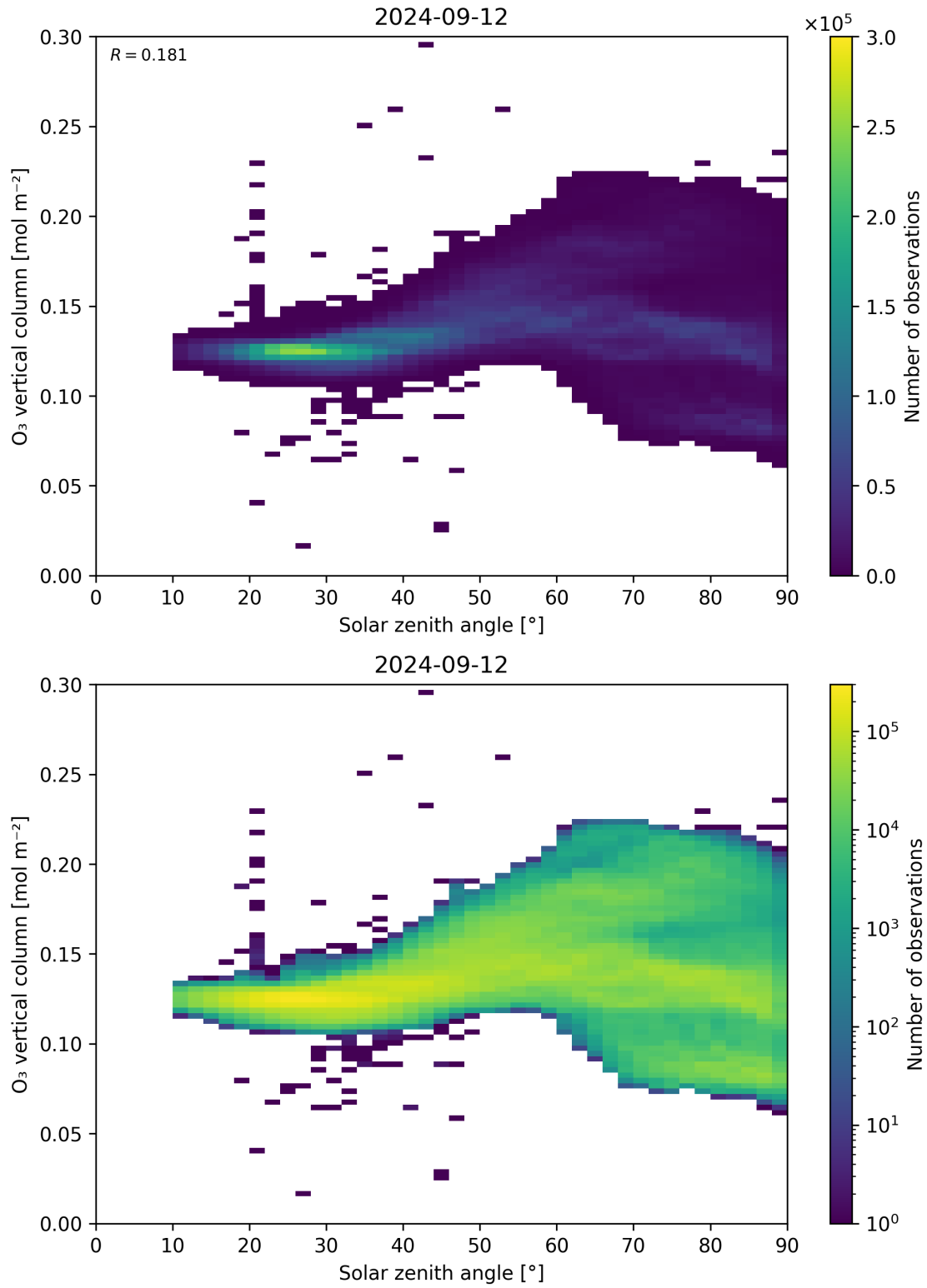
Figure 47: Scatter density plot of “Solar zenith angle” against “O 3 vertical column” for 2024-09-12 to 2024-09-13.
