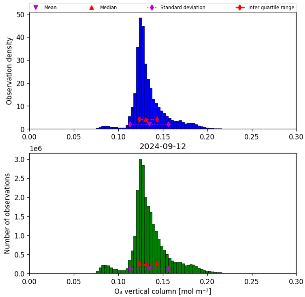
Figure 21: Histogram of “O 3 vertical column” for 2024-09-12 to 2024-09-13
