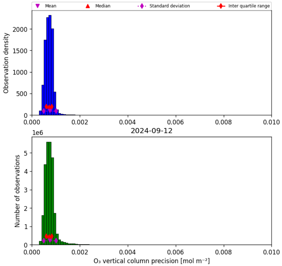
Figure 22: Histogram of “O 3 vertical column precision” for 2024-09-12 to 2024-09-13
