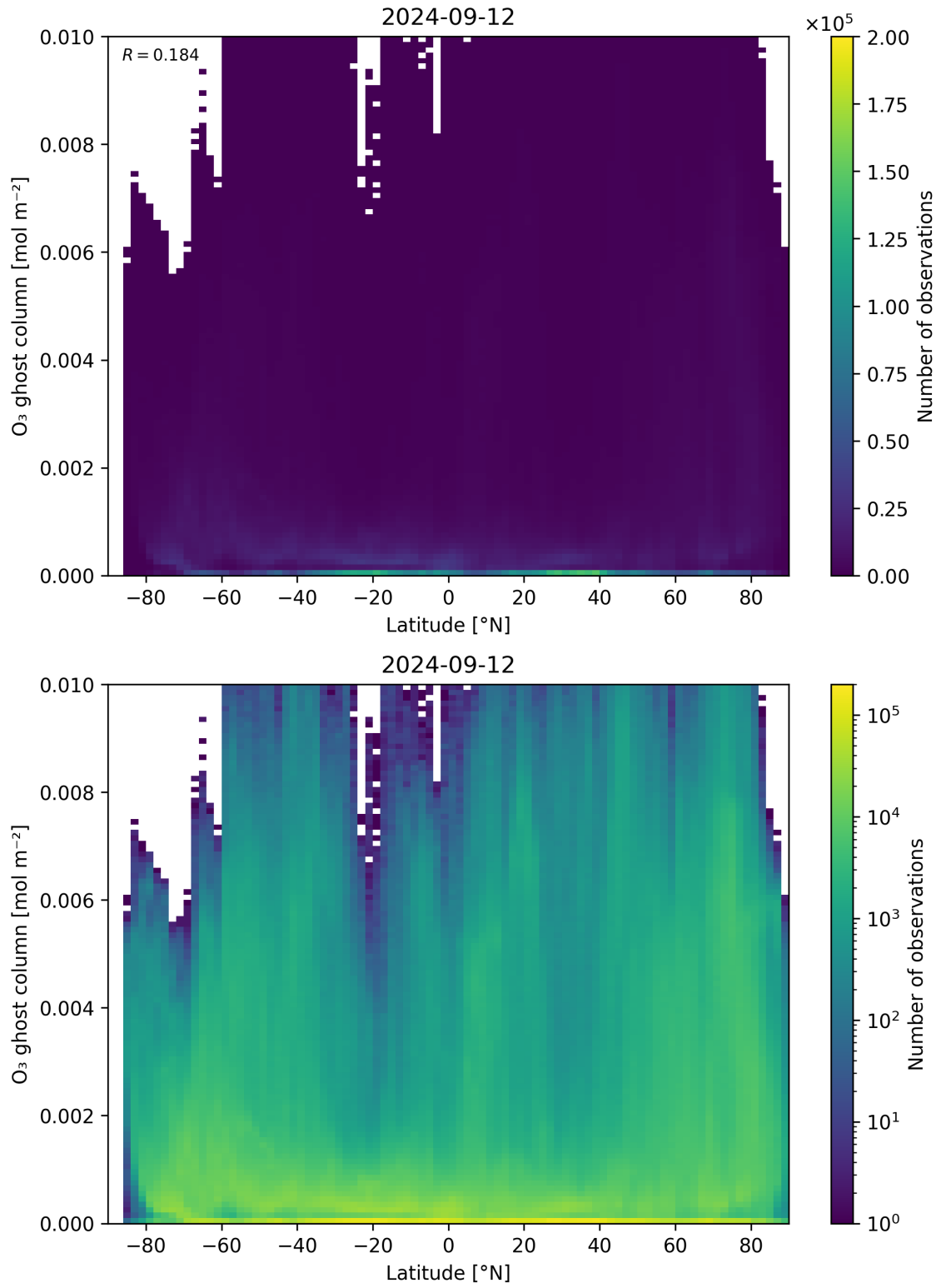
Figure 35: Scatter density plot of “Latitude” against “O 3 ghost column” for 2024-09-12 to 2024-09-13.
