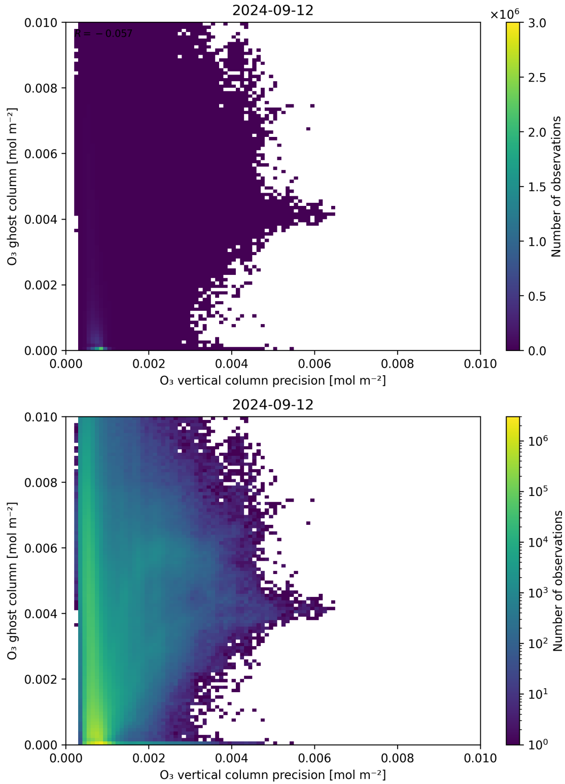
Figure 43: Scatter density plot of “ \text{O}_3 vertical column precision” against “ \text{O}_3 ghost column” for 2024-09-12 to 2024-09-13.
