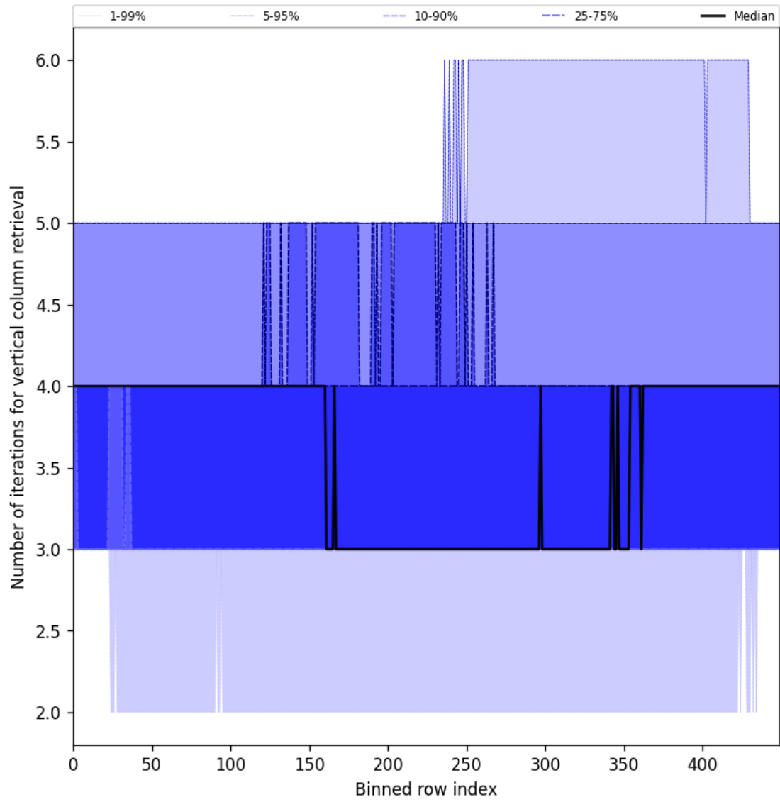
Figure 33: Along track statistics of “Number of iterations for vertical column retrieval” for 2024-09-12 to 2024-09-13
