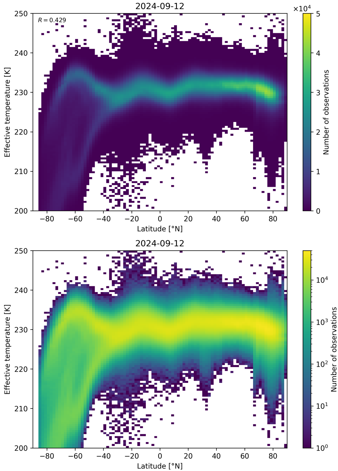
Figure 34: Scatter density plot of “Latitude” against “Effective temperature” for 2024-09-12 to 2024-09-13.
