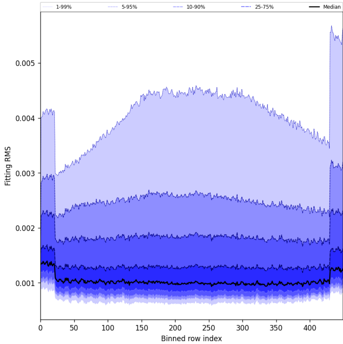
Figure 30: Along track statistics of “Fitting RMS” for 2024-09-12 to 2024-09-13
