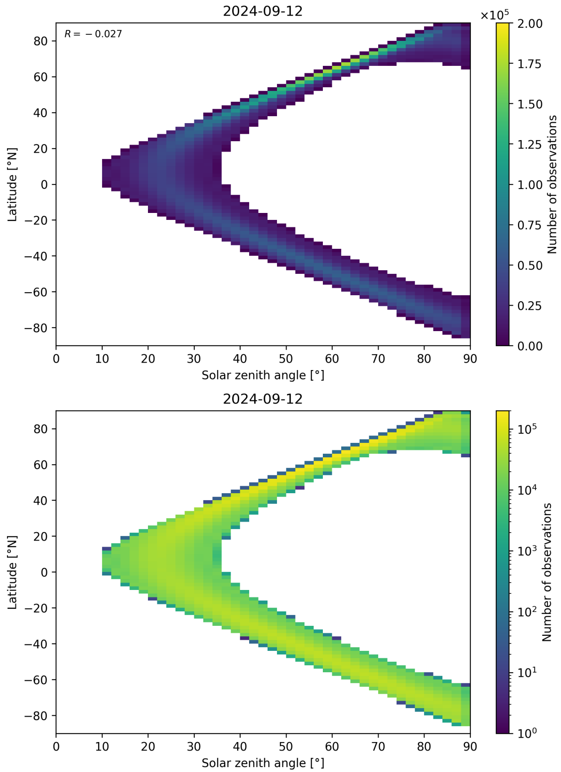
Figure 44: Scatter density plot of “Solar zenith angle” against “Latitude” for 2024-09-12 to 2024-09-13.
