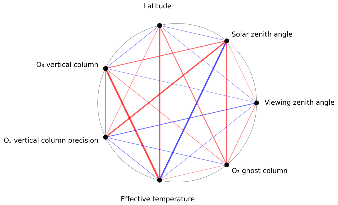
Figure 1: Map of correlation graph for 2024-09-12 to 2024-09-13.
