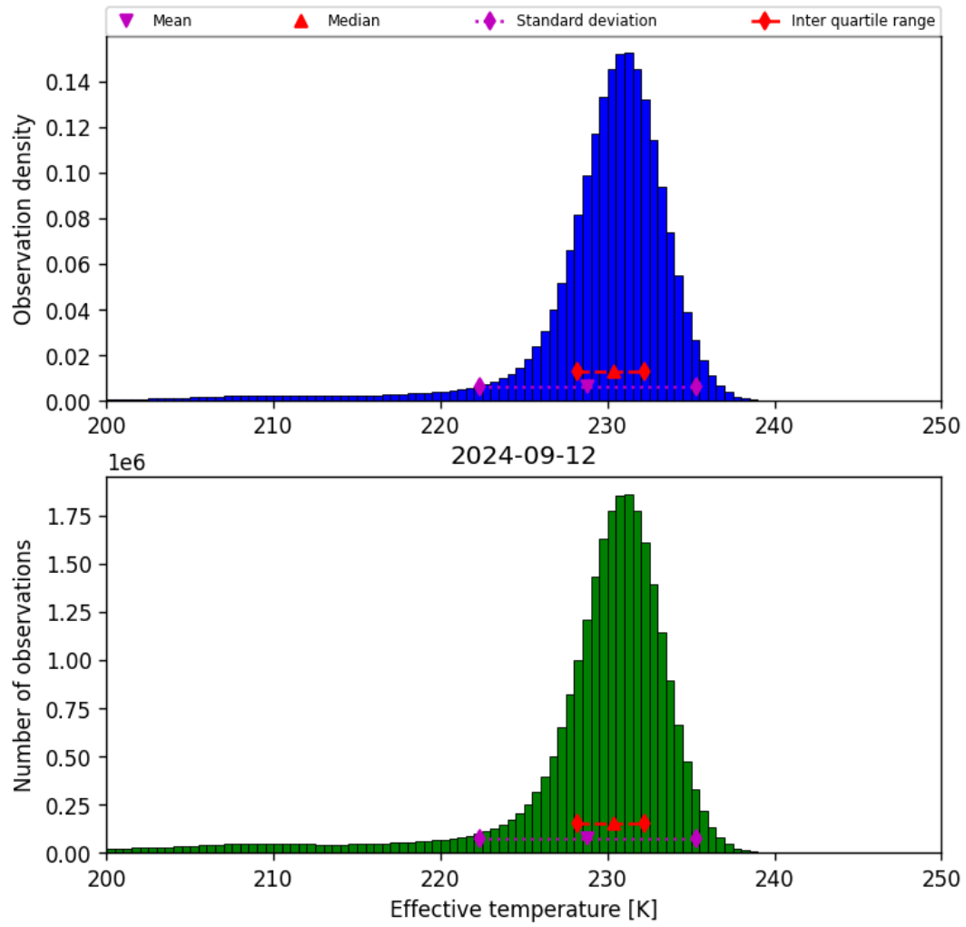
Figure 24: Histogram of “Effective temperature” for 2024-09-12 to 2024-09-13
