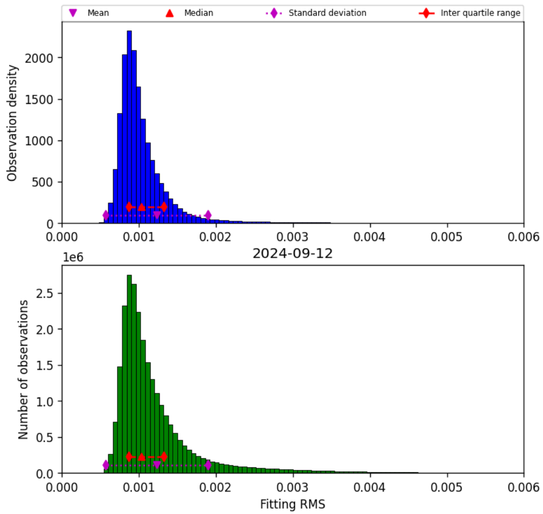
Figure 23: Histogram of “Fitting RMS” for 2024-09-12 to 2024-09-13
