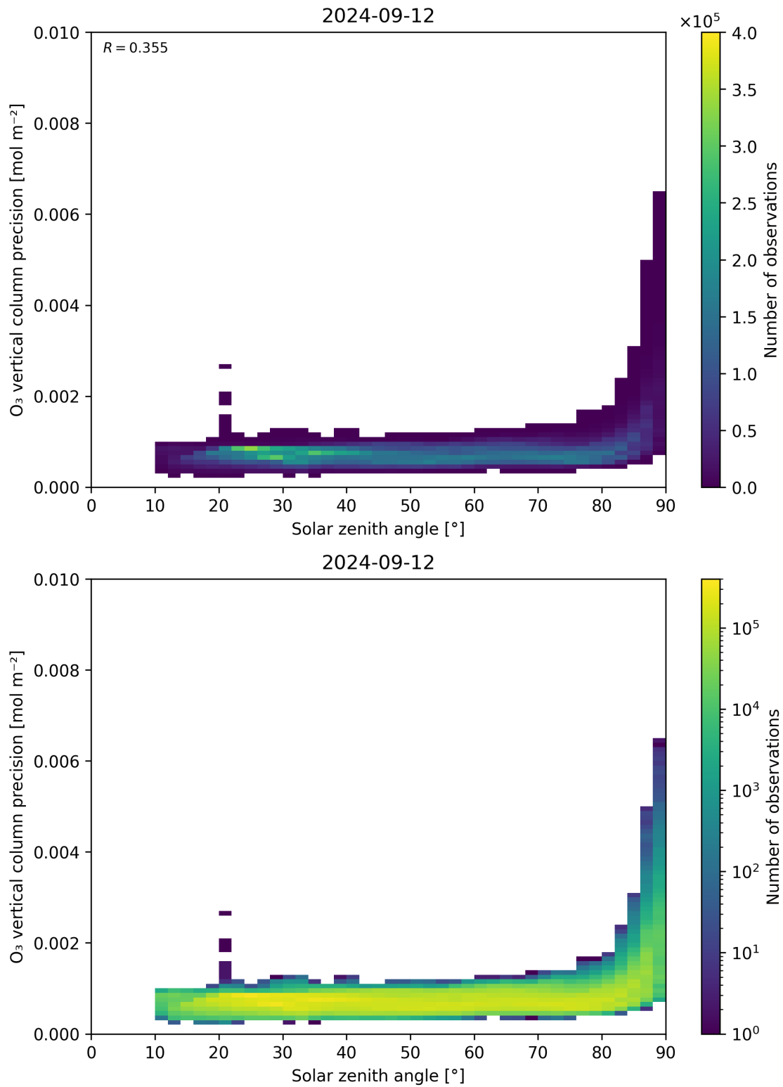
Figure 48: Scatter density plot of “Solar zenith angle” against “O 3 vertical column precision” for 2024-09-12 to 2024-09-13.
