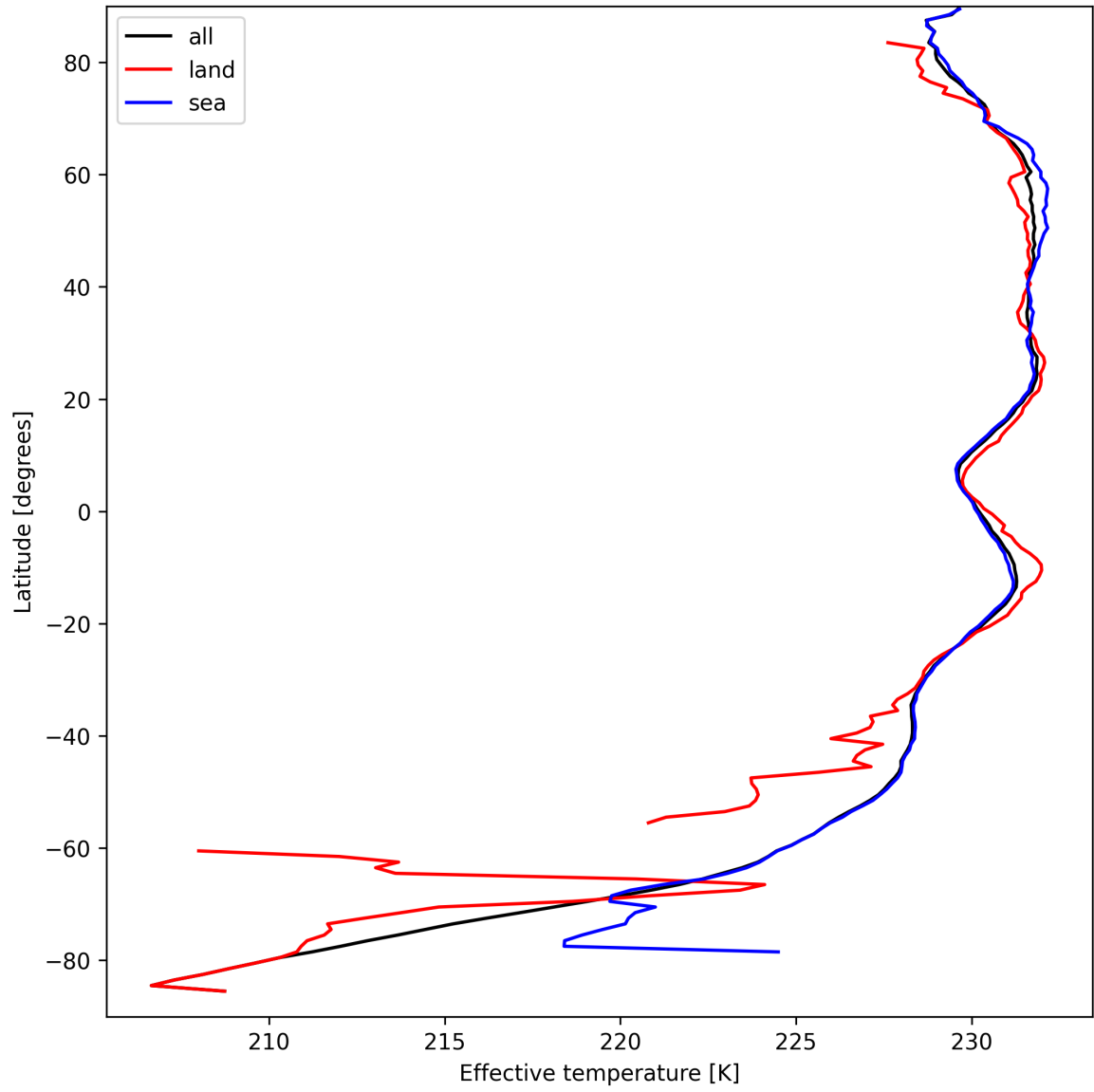
Figure 17: Zonal average of "Effective temperature" for 2024-09-12 to 2024-09-13.
