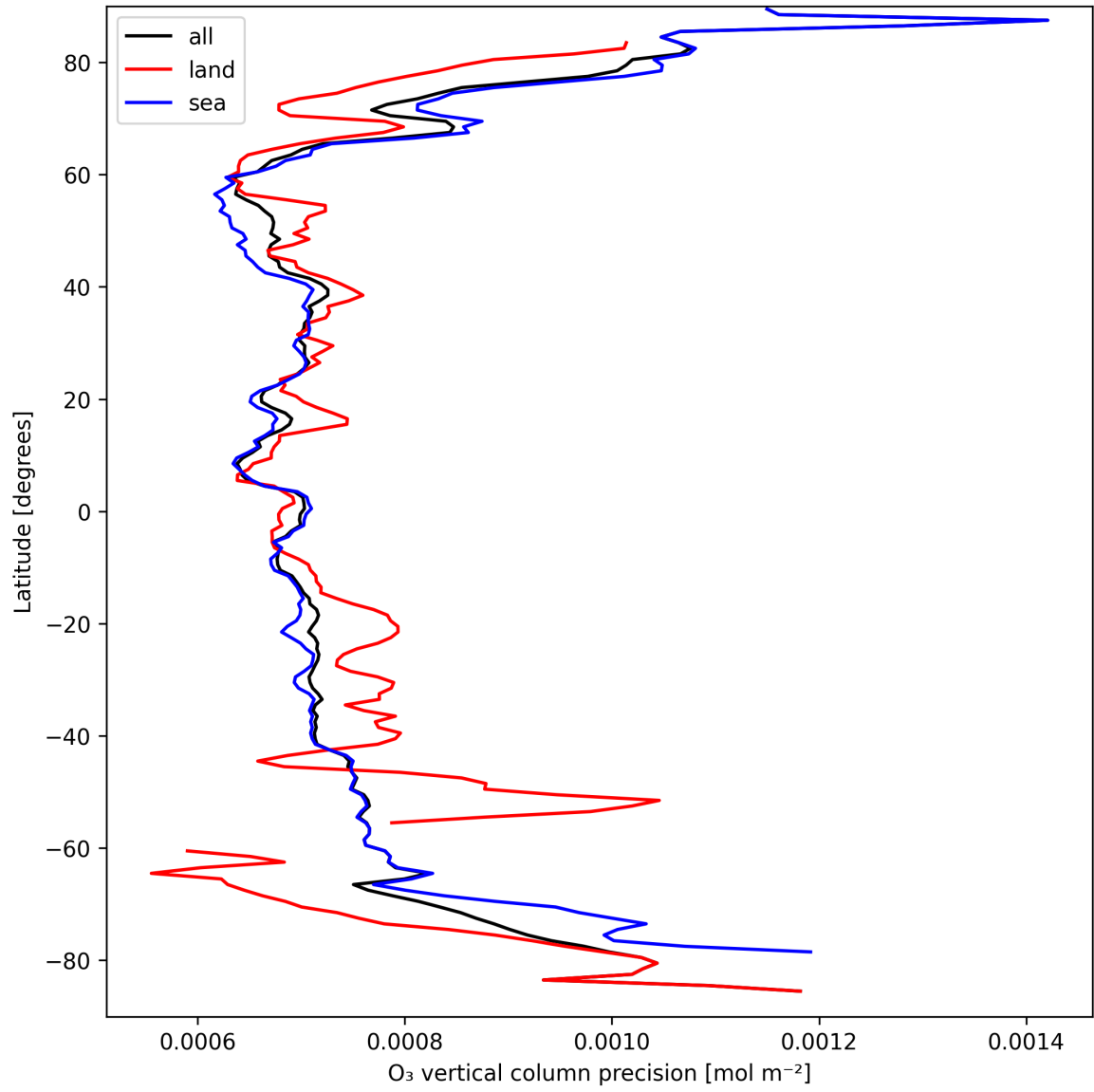
Figure 15: Zonal average of “O 3 vertical column precision” for 2024-09-12 to 2024-09-13.
