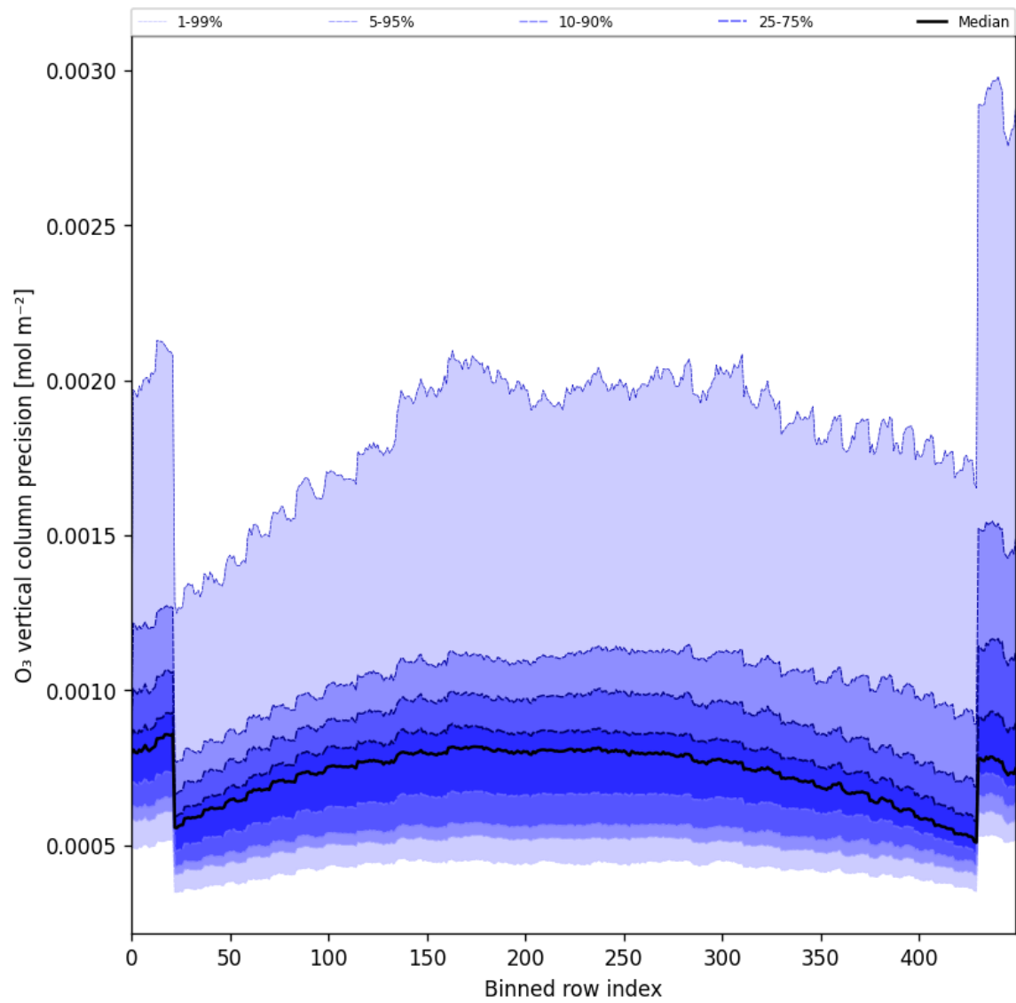
Figure 29: Along track statistics of “O 3 vertical column precision” for 2024-09-12 to 2024-09-13
