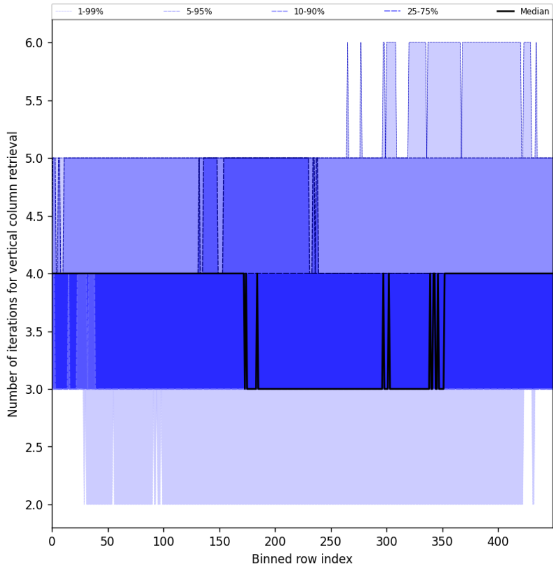
Figure 33: Along track statistics of “Number of iterations for vertical column retrieval” for 2024-09-12 to 2024-09-14
