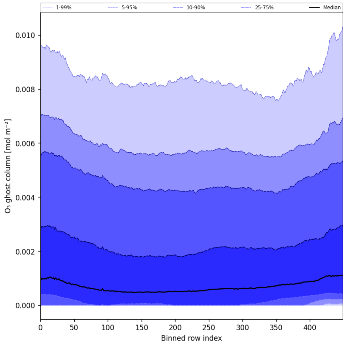
Figure 32: Along track statistics of “O 3 ghost column” for 2024-09-12 to 2024-09-14
