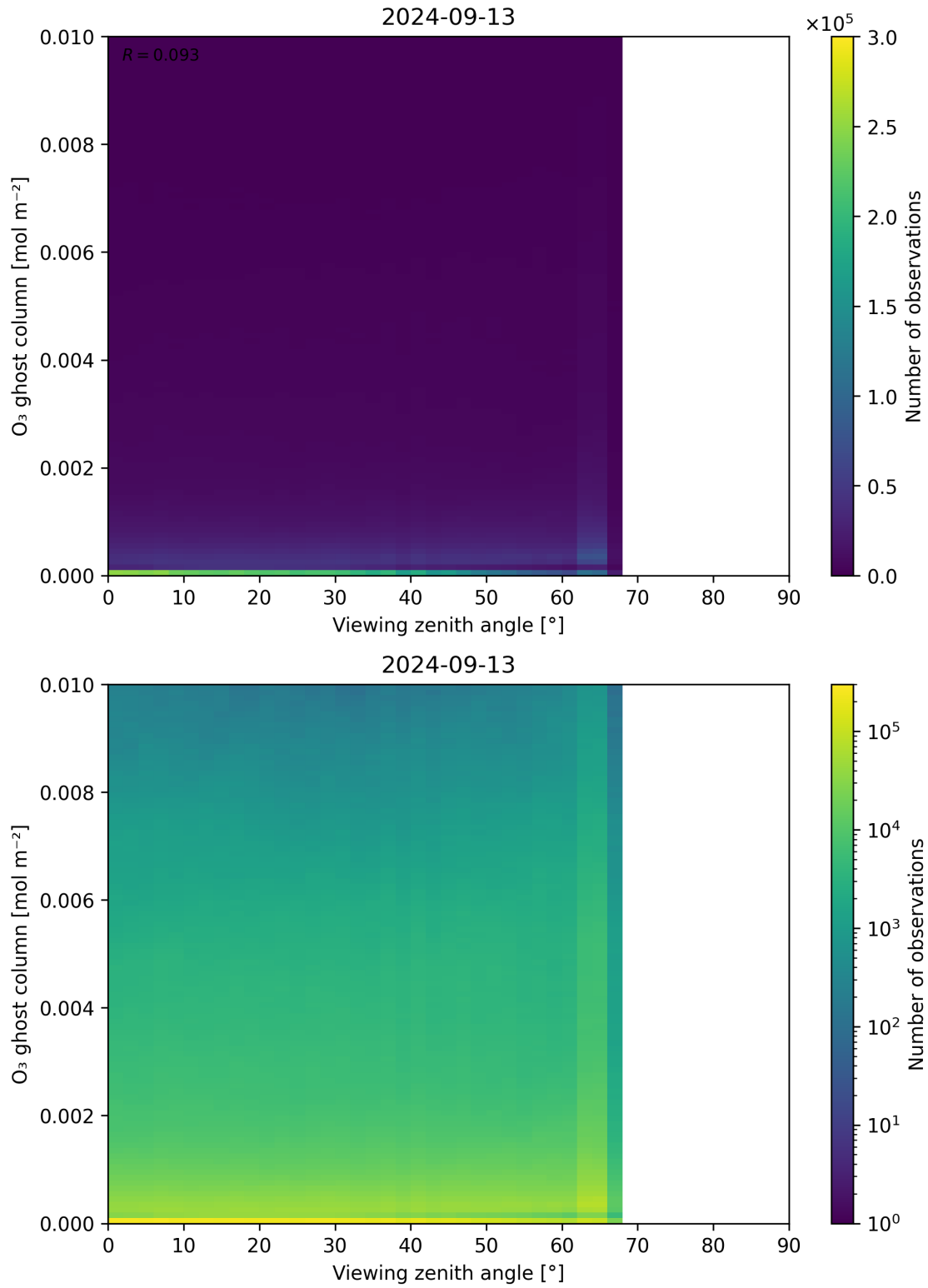
Figure 51: Scatter density plot of “Viewing zenith angle” against “O 3 ghost column” for 2024-09-12 to 2024-09-14.
