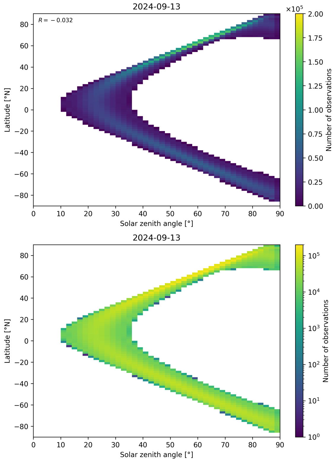
Figure 44: Scatter density plot of “Solar zenith angle” against “Latitude” for 2024-09-12 to 2024-09-14.
