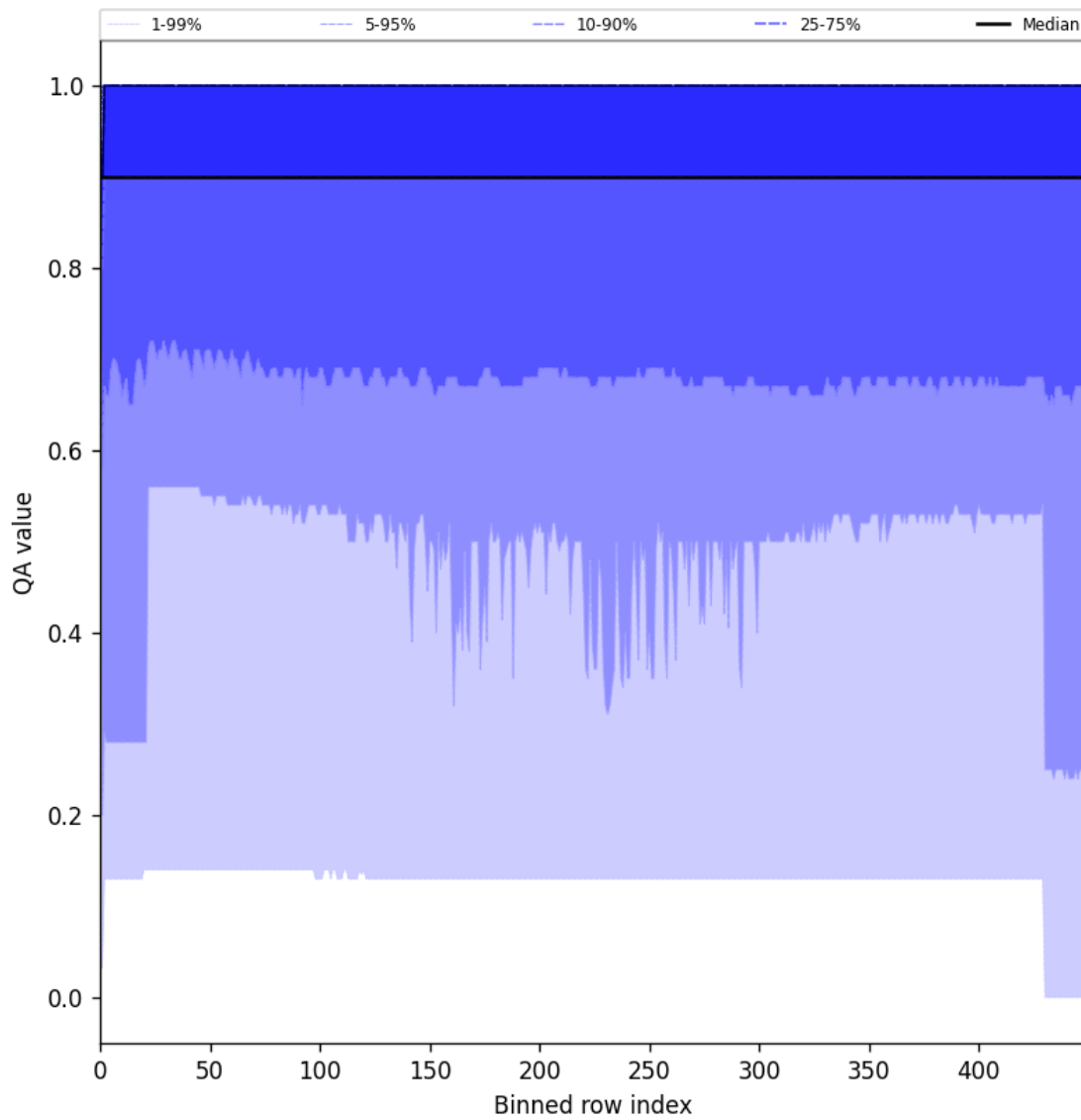
Figure 27: Along track statistics of “QA value” for 2024-09-12 to 2024-09-14
