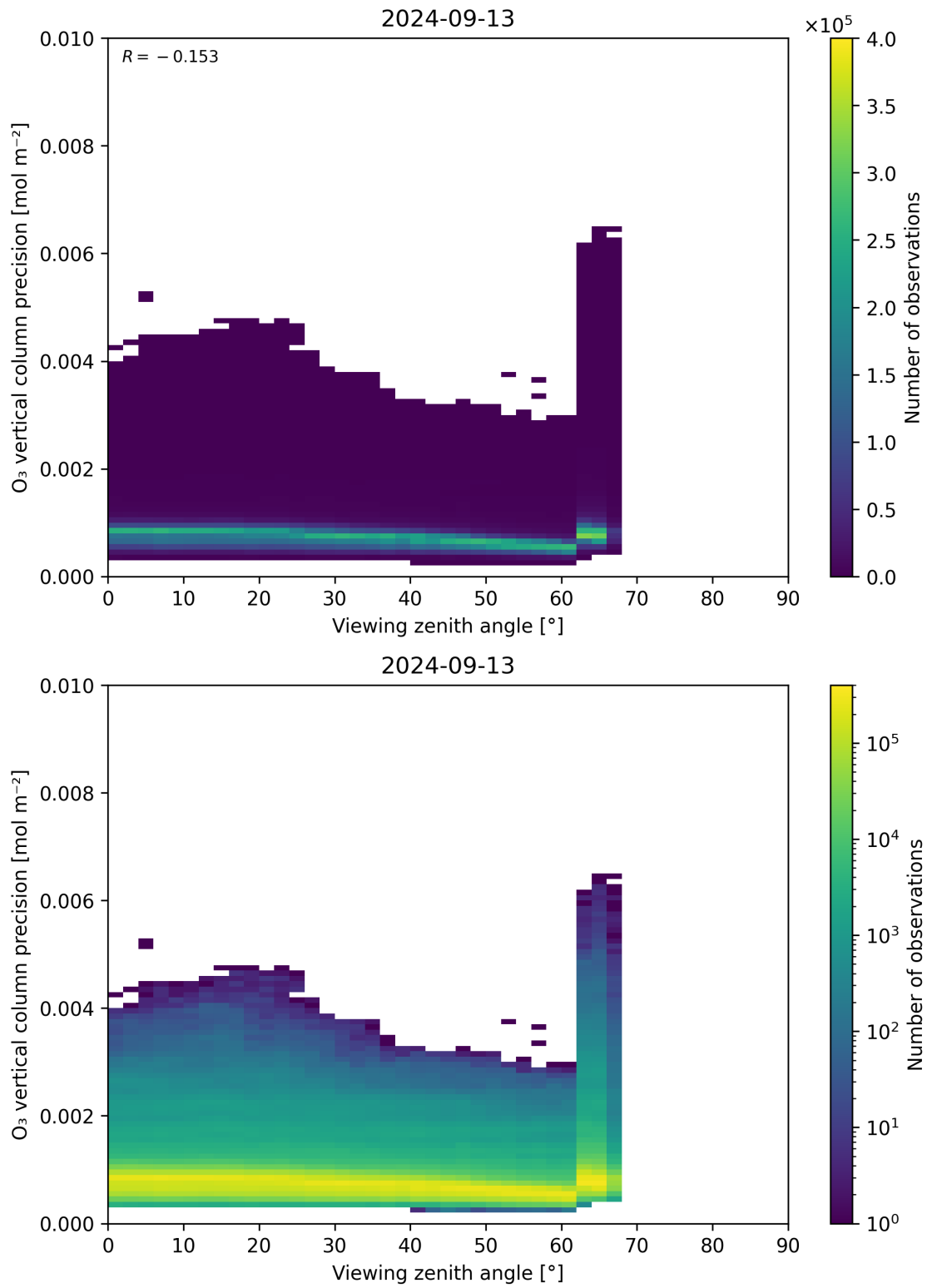
Figure 53: Scatter density plot of “Viewing zenith angle” against “O 3 vertical column precision” for 2024-09-12 to 2024-09-14.
