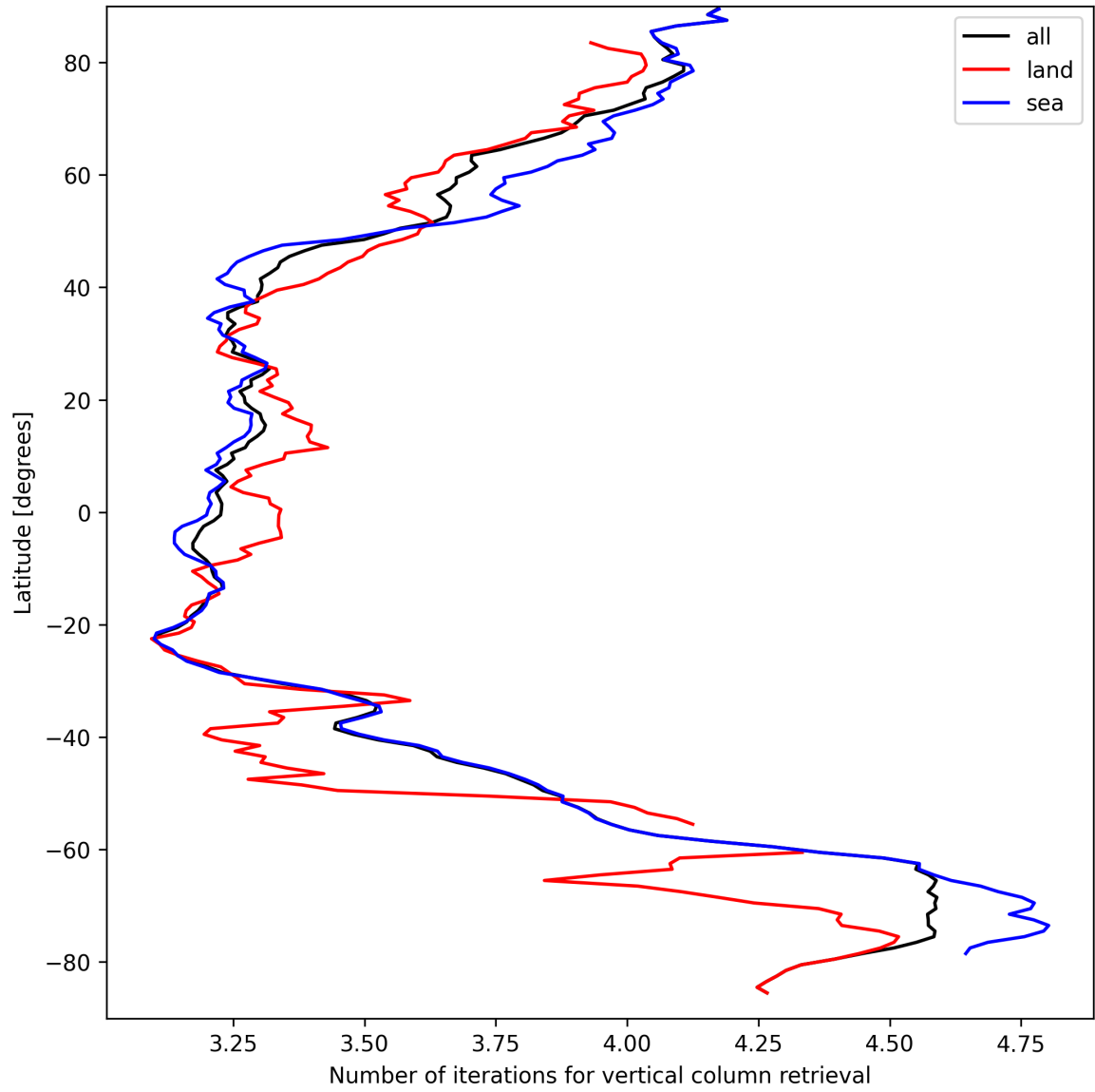
Figure 19: Zonal average of “Number of iterations for vertical column retrieval” for 2024-09-12 to 2024-09-14.
