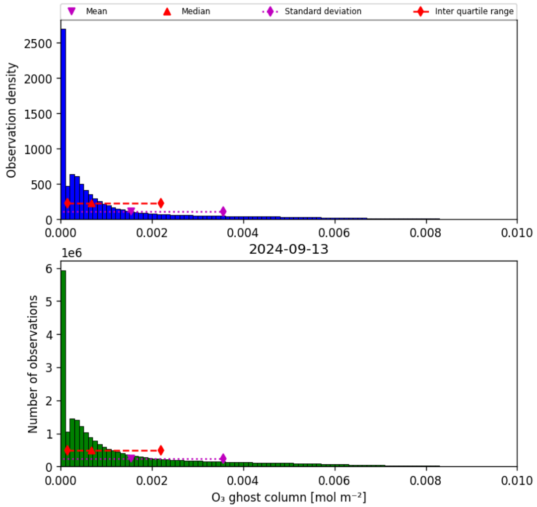
Figure 25: Histogram of "O 3 ghost column" for 2024-09-12 to 2024-09-14
