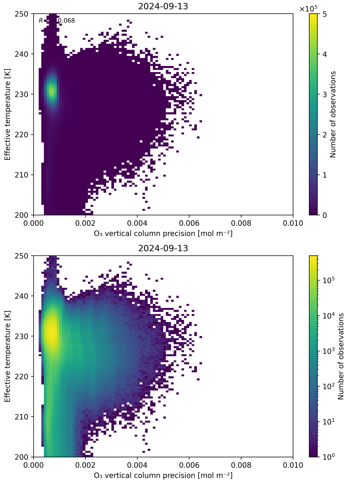
Figure 42: Scatter density plot of “ O_3 vertical column precision” against “Effective temperature” for 2024-09-12 to 2024-09-14.
