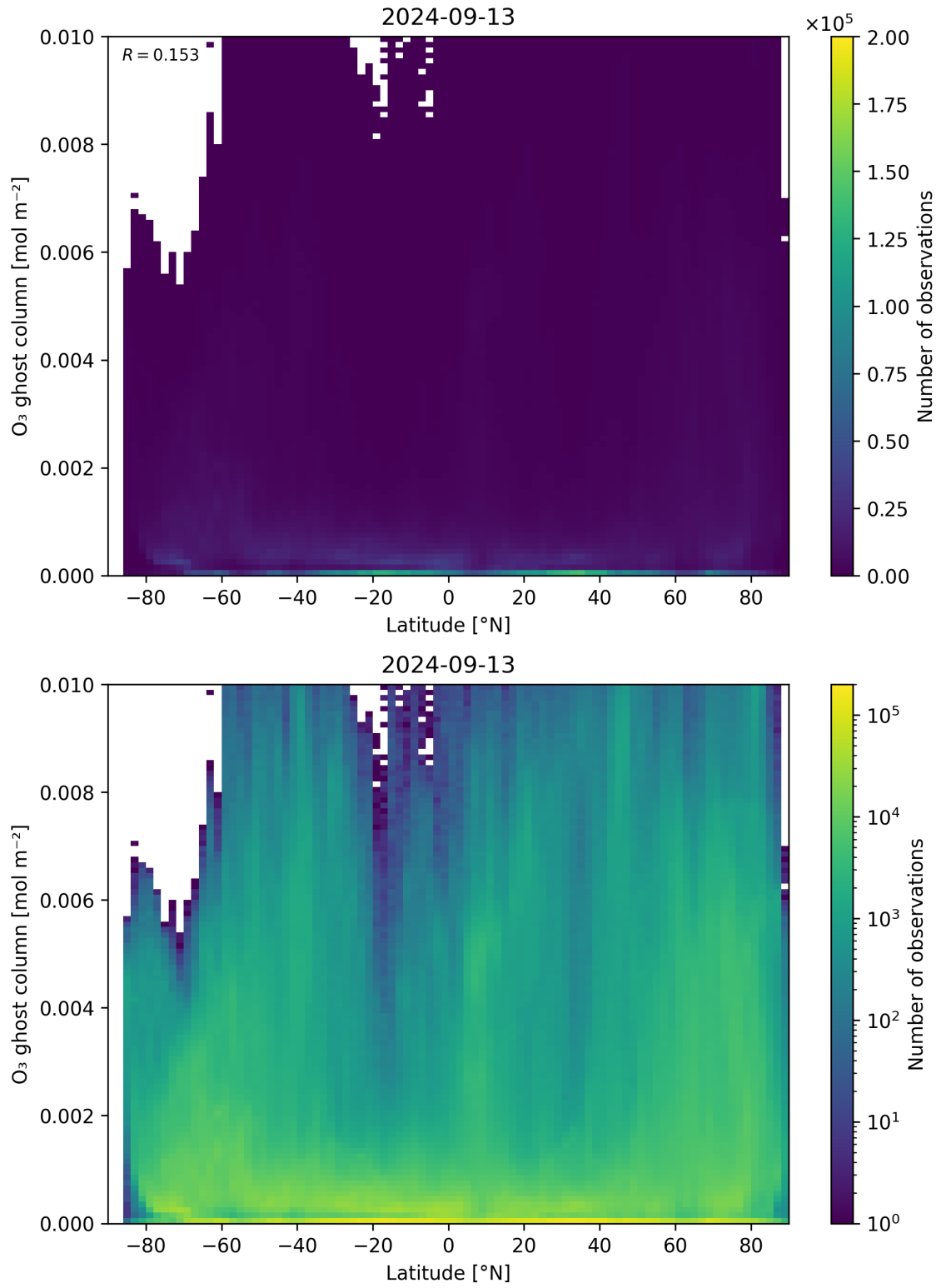
Figure 35: Scatter density plot of “Latitude” against “O 3 ghost column” for 2024-09-12 to 2024-09-14.
