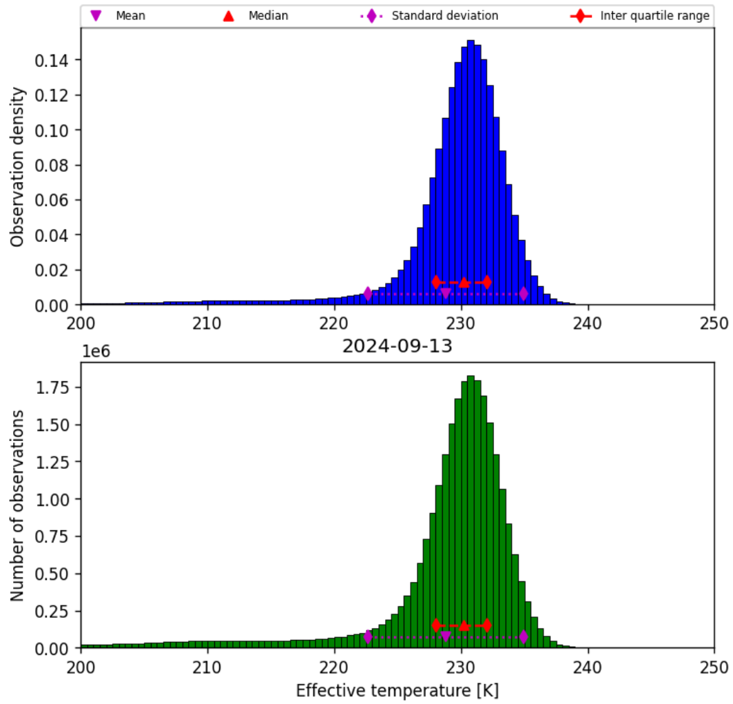
Figure 24: Histogram of “Effective temperature” for 2024-09-12 to 2024-09-14
