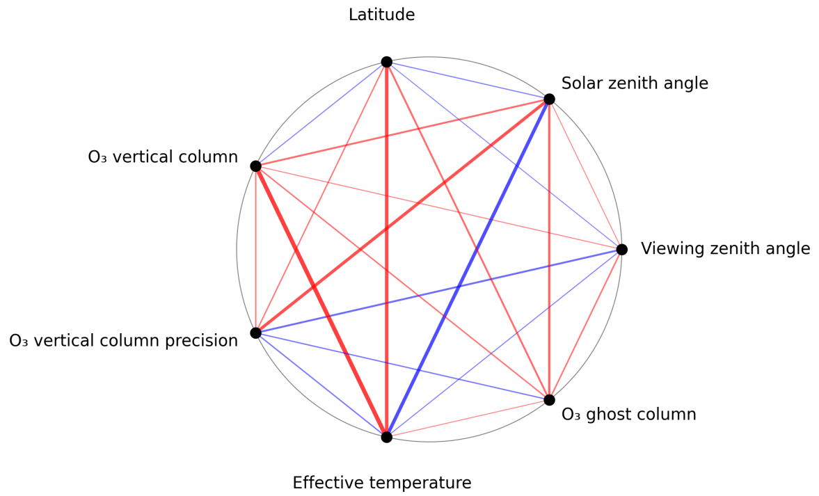
Figure 1: Map of correlation graph for 2024-09-12 to 2024-09-14.
