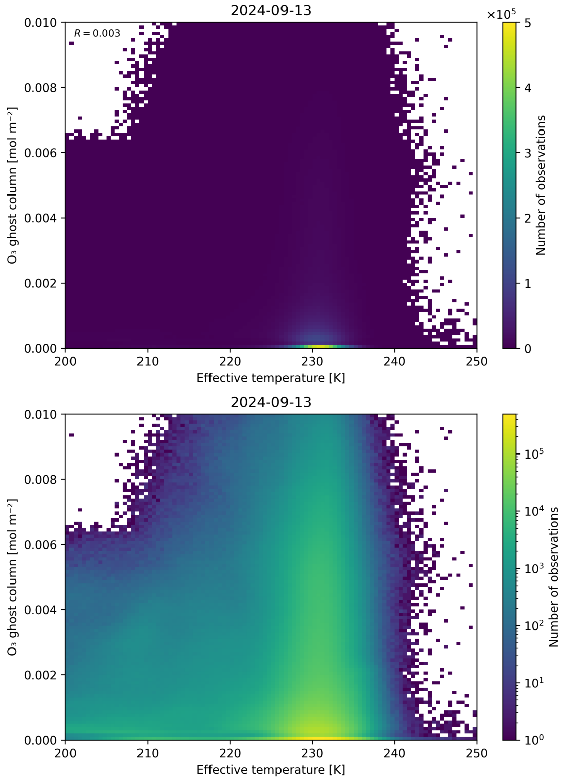
Figure 38: Scatter density plot of “Effective temperature” against “O 3 ghost column” for 2024-09-12 to 2024-09-14.
