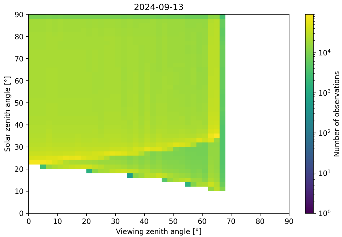
Figure 54: Scatter density plot of “Viewing zenith angle” against “Solar zenith angle” for 2024-09-12 to 2024-09-14.
