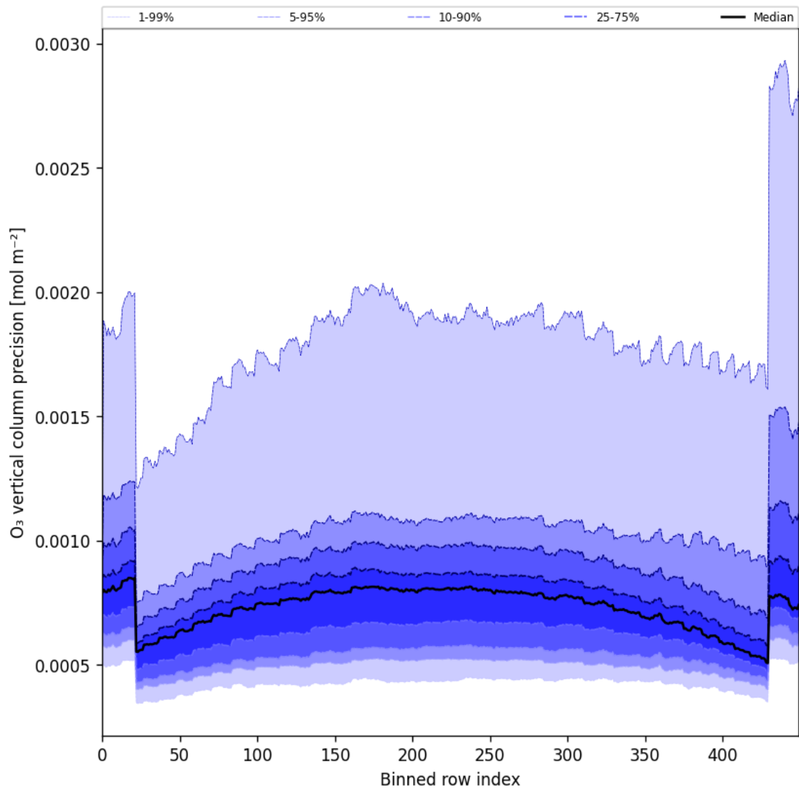
Figure 29: Along track statistics of “O 3 vertical column precision” for 2024-09-12 to 2024-09-14
