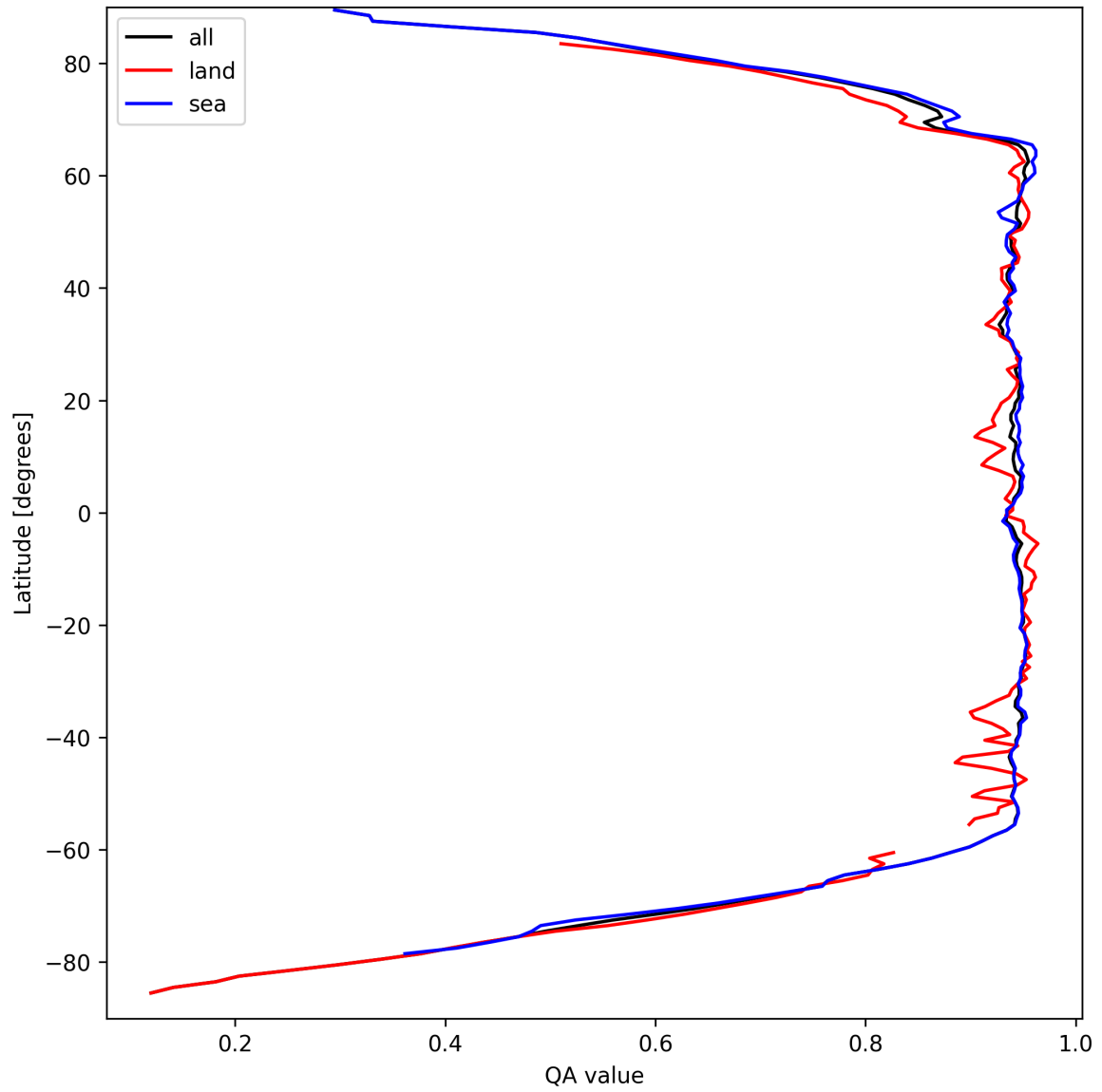
Figure 13: Zonal average of “QA value” for 2024-09-12 to 2024-09-14.
