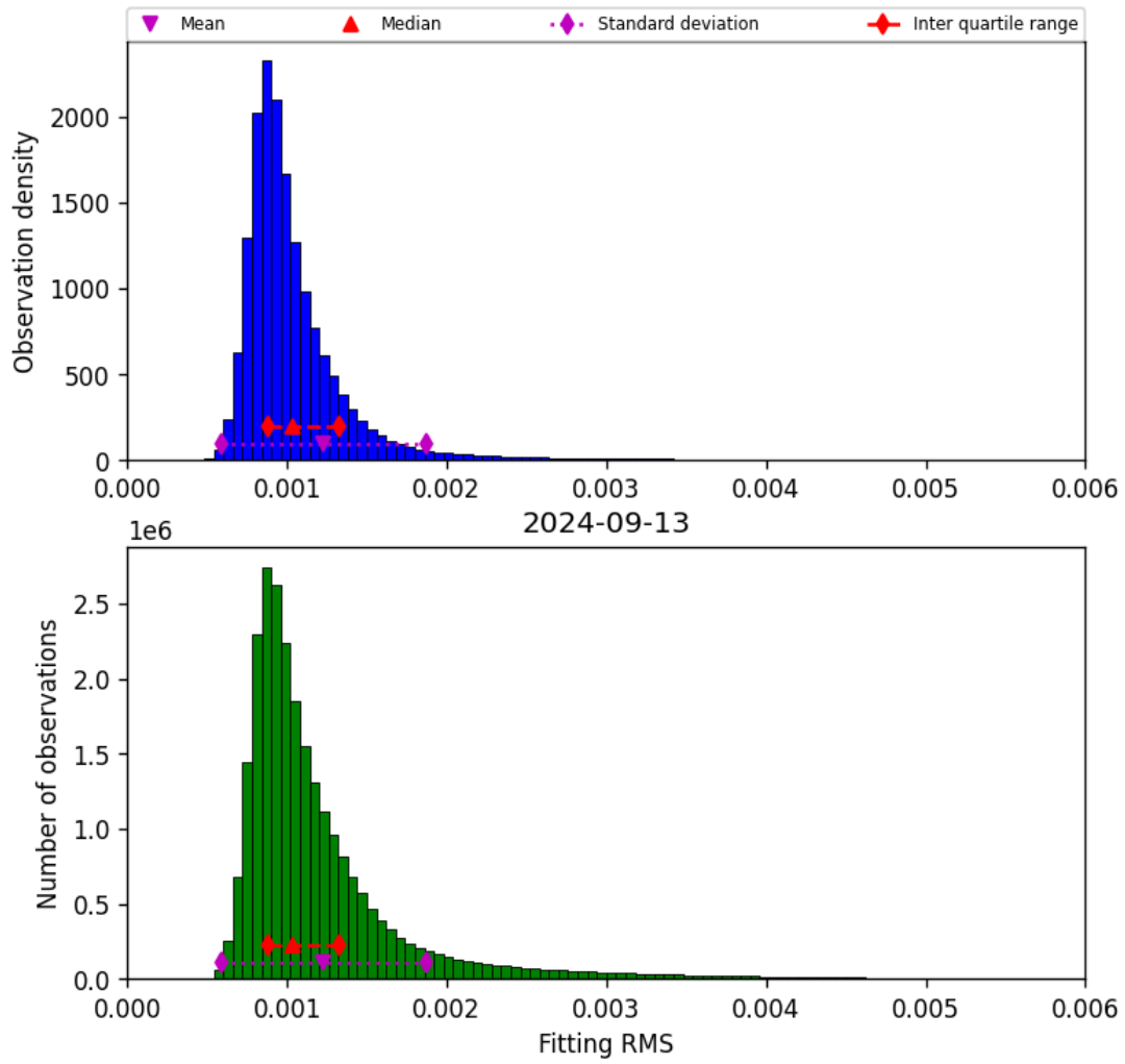
Figure 23: Histogram of “Fitting RMS” for 2024-09-12 to 2024-09-14
