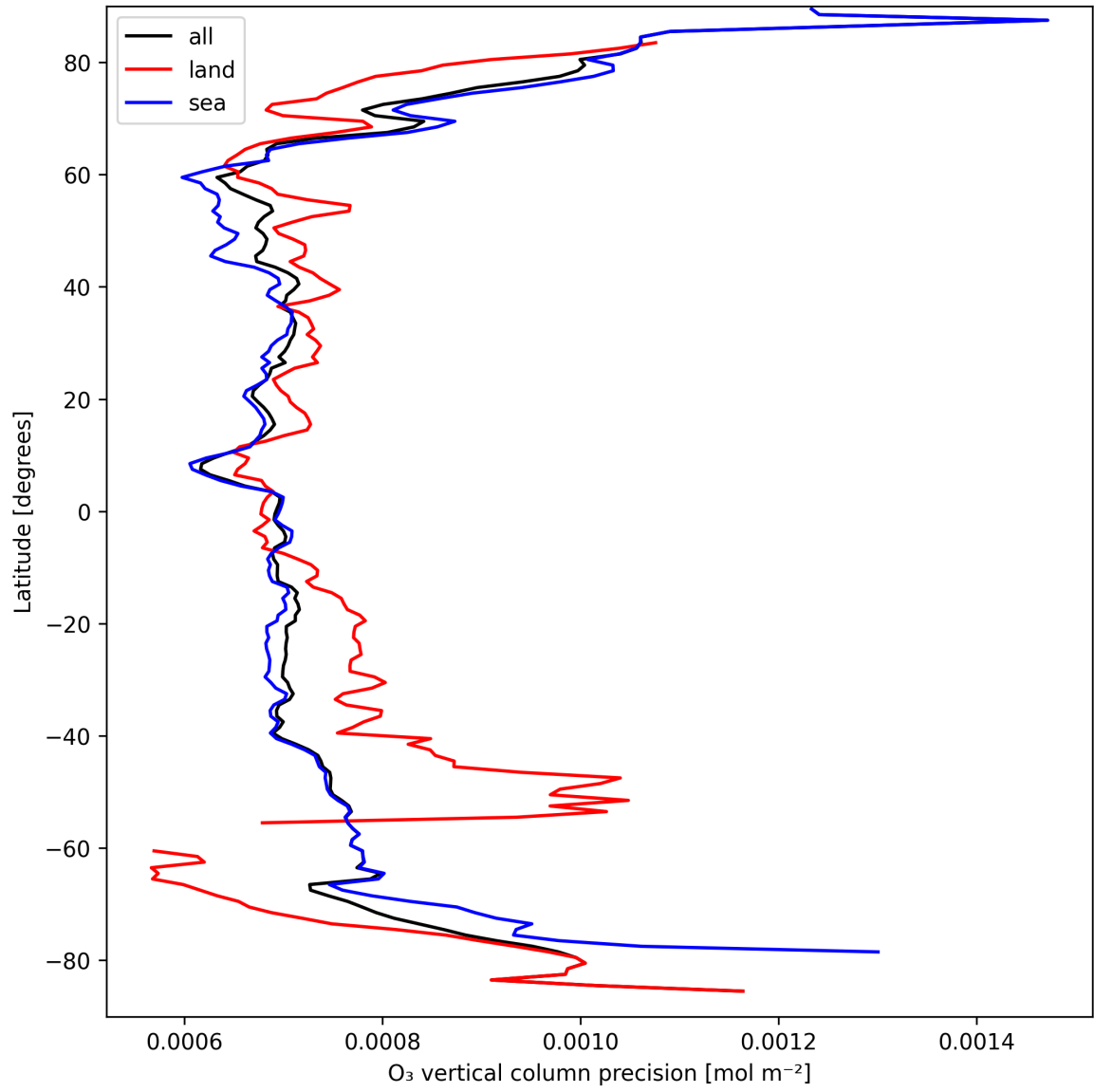
Figure 15: Zonal average of “O 3 vertical column precision” for 2024-09-12 to 2024-09-14.
