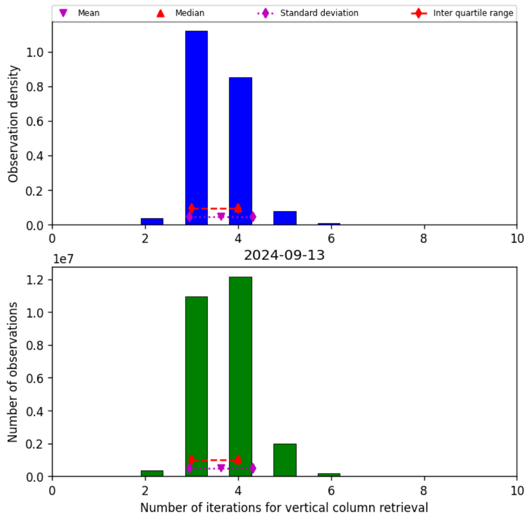
Figure 26: Histogram of “Number of iterations for vertical column retrieval” for 2024-09-12 to 2024-09-14
