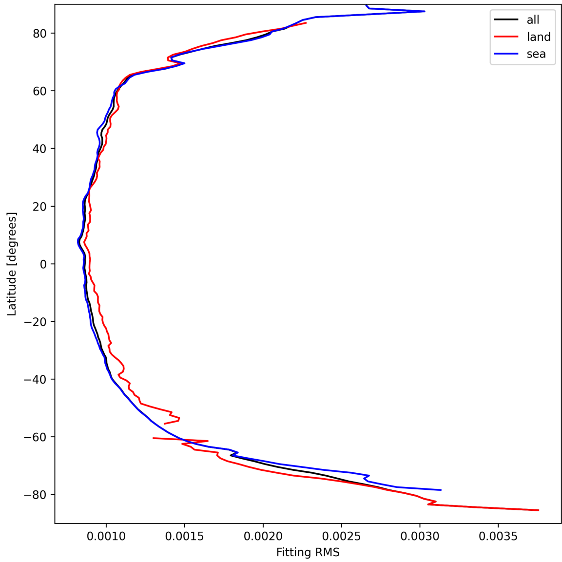
Figure 16: Zonal average of “Fitting RMS” for 2024-09-12 to 2024-09-14.
