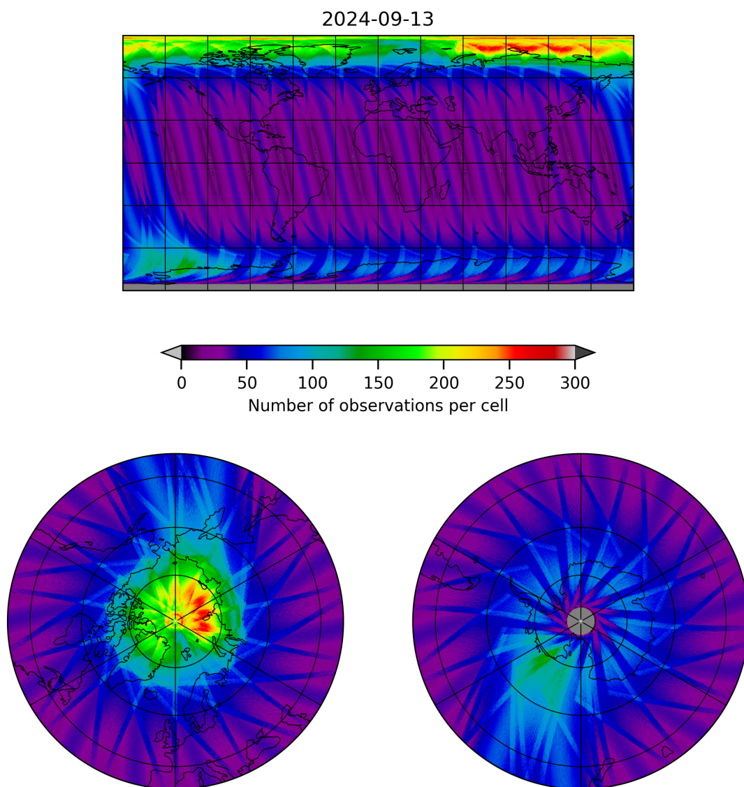
Figure 12: Map of the number of observations for 2024-09-12 to 2024-09-14
