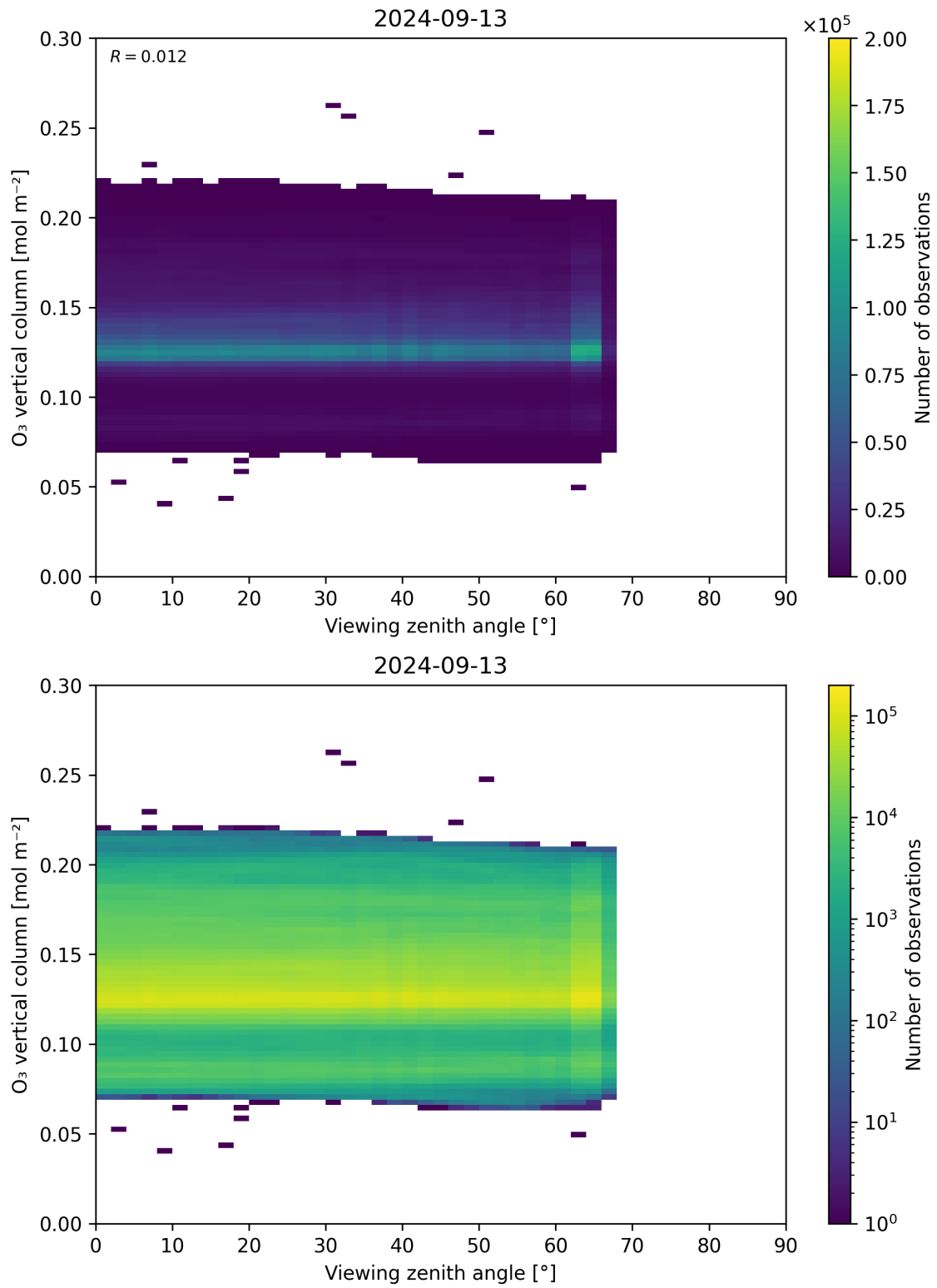
Figure 52: Scatter density plot of “Viewing zenith angle” against “O 3 vertical column” for 2024-09-12 to 2024-09-14.
