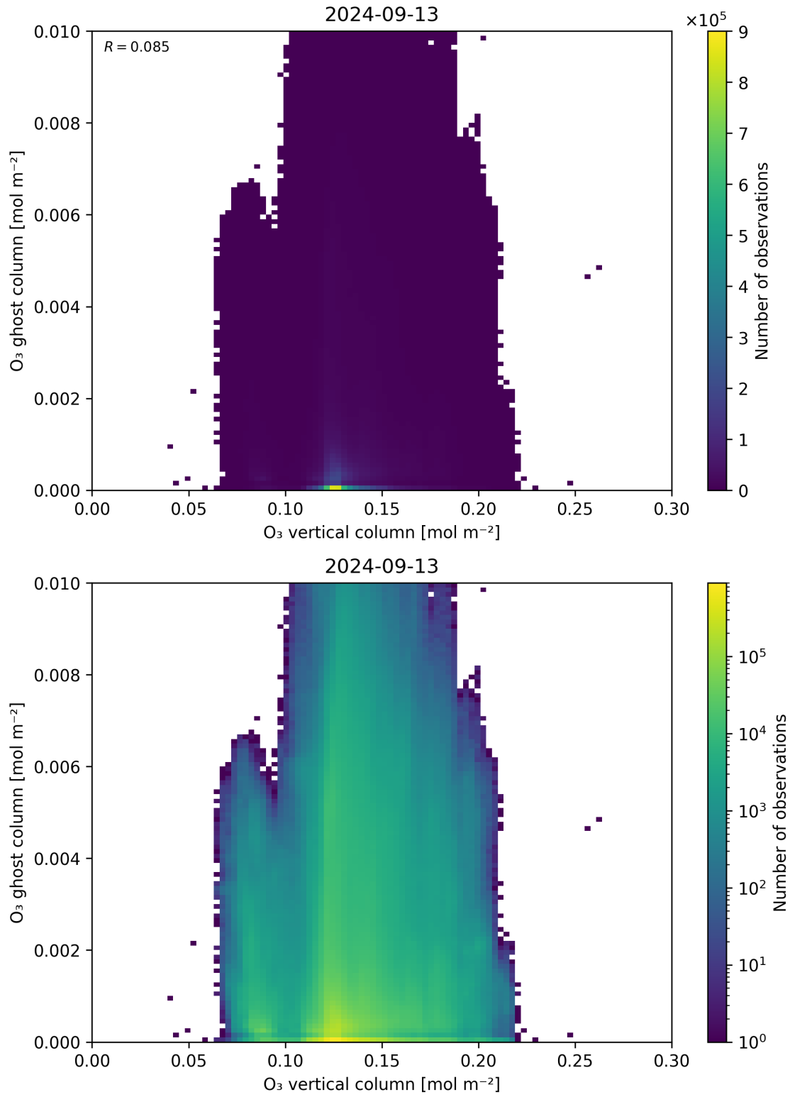
Figure 40: Scatter density plot of “O 3 vertical column” against “O 3 ghost column” for 2024-09-12 to 2024-09-14.
