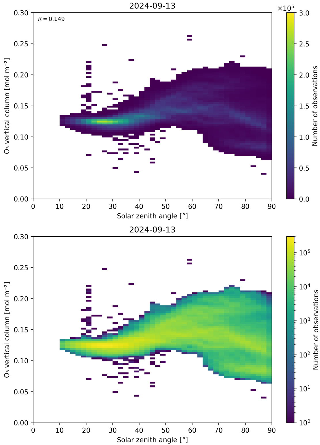
Figure 47: Scatter density plot of “Solar zenith angle” against “O 3 vertical column” for 2024-09-12 to 2024-09-14.
