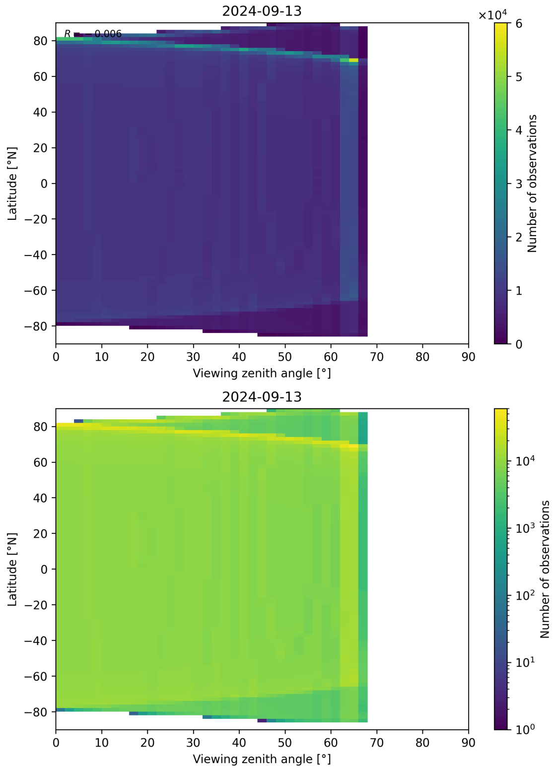
Figure 49: Scatter density plot of “Viewing zenith angle” against “Latitude” for 2024-09-12 to 2024-09-14.
