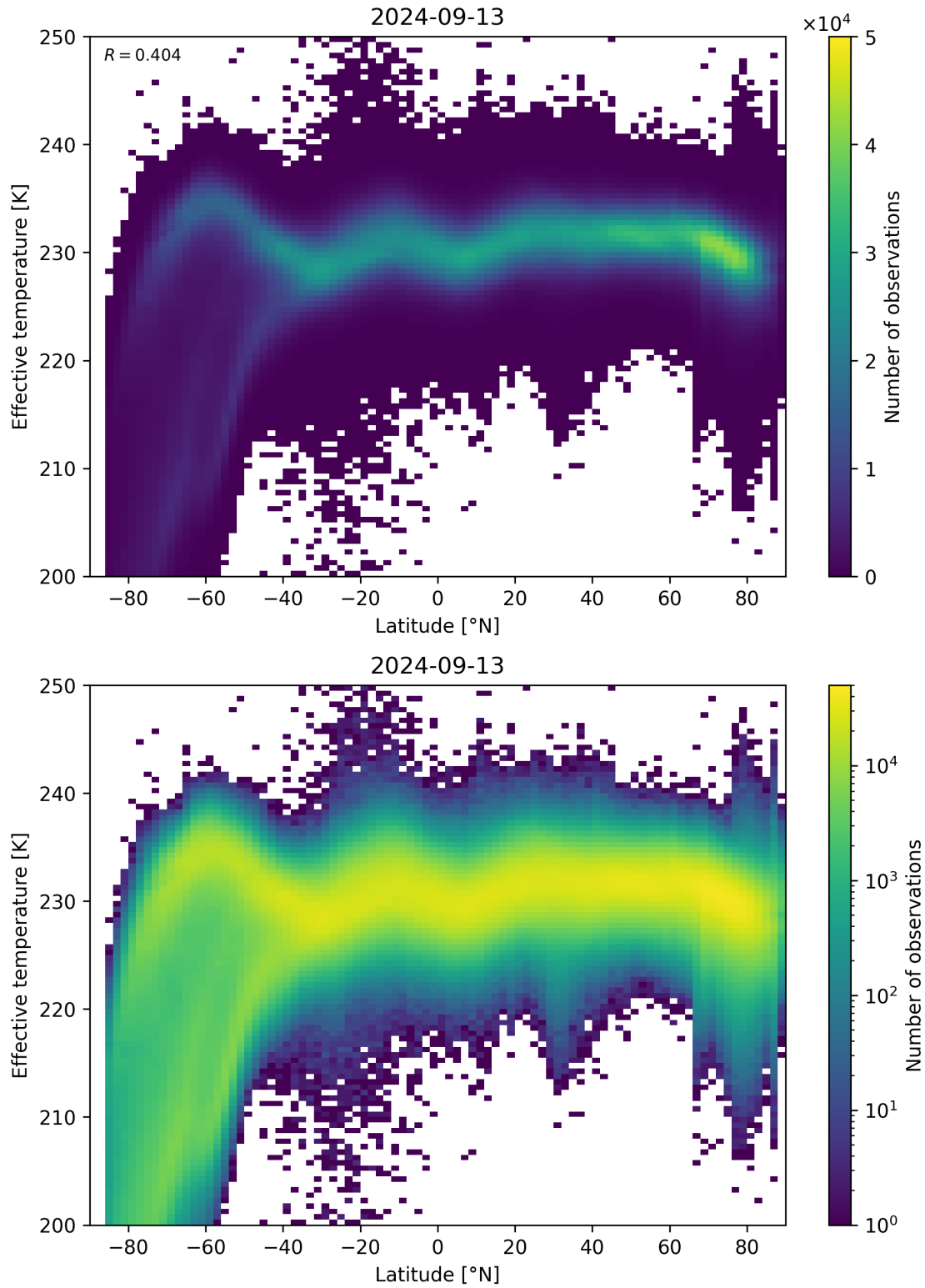
Figure 34: Scatter density plot of “Latitude” against “Effective temperature” for 2024-09-12 to 2024-09-14.
