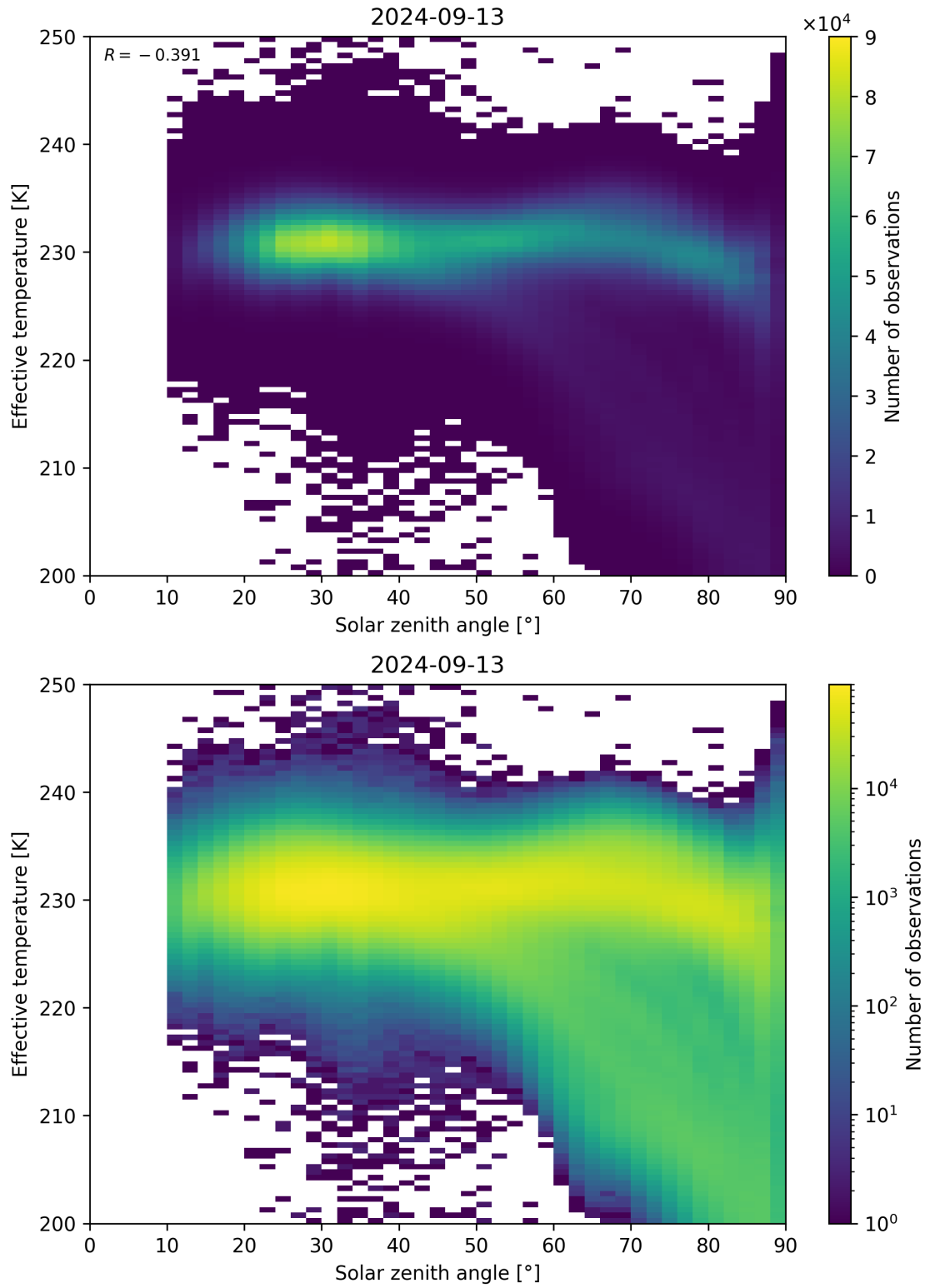
Figure 45: Scatter density plot of “Solar zenith angle” against “Effective temperature” for 2024-09-12 to 2024-09-14.
