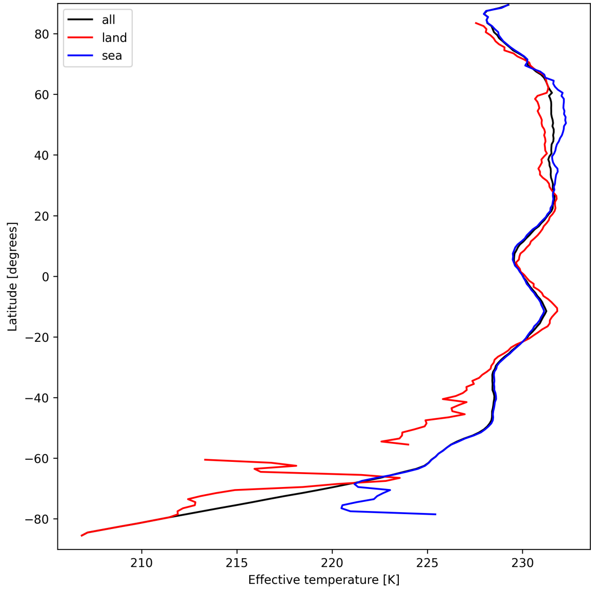
Figure 17: Zonal average of "Effective temperature" for 2024-09-12 to 2024-09-14.
