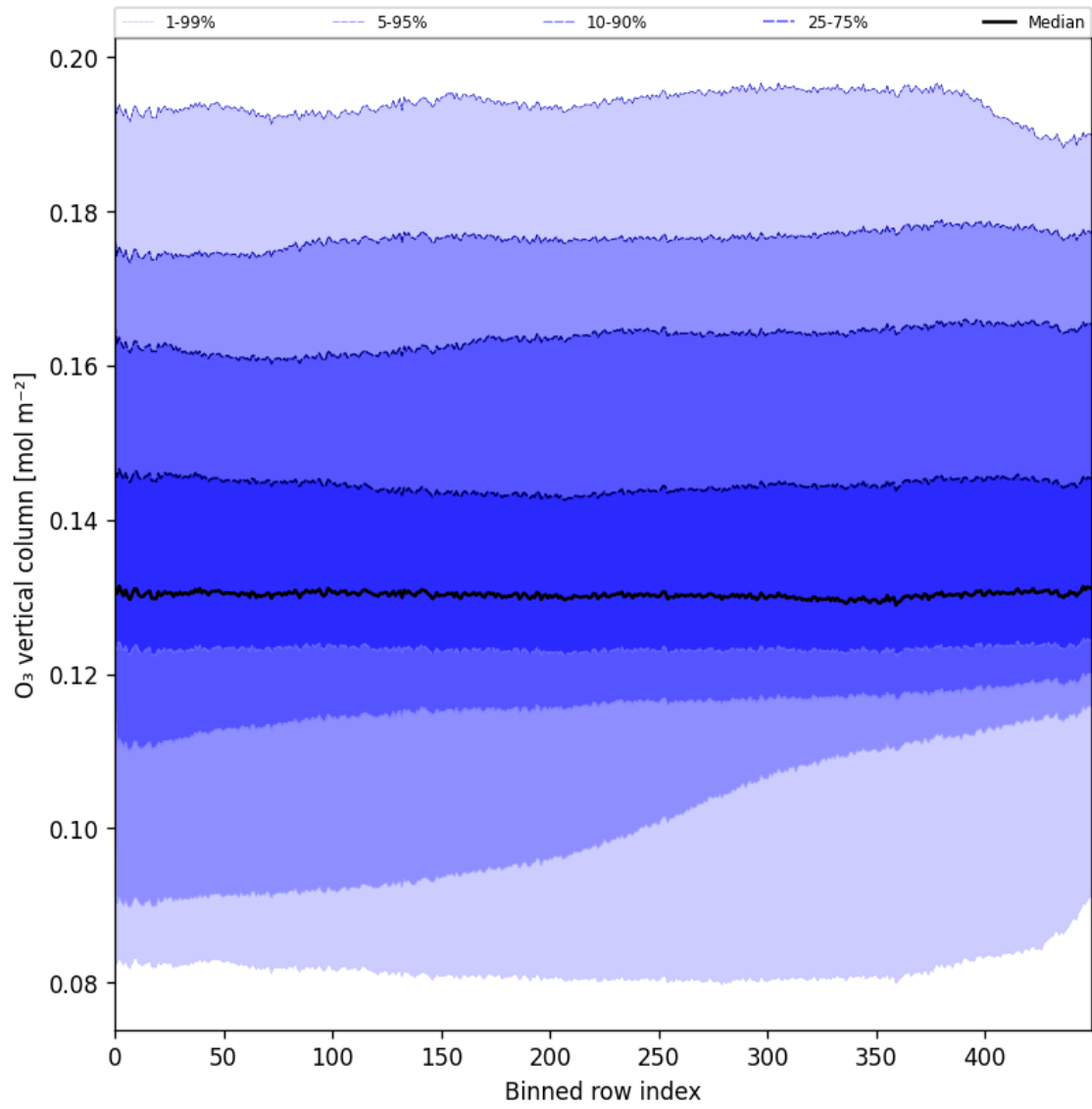
Figure 28: Along track statistics of “O 3 vertical column” for 2024-09-12 to 2024-09-14
