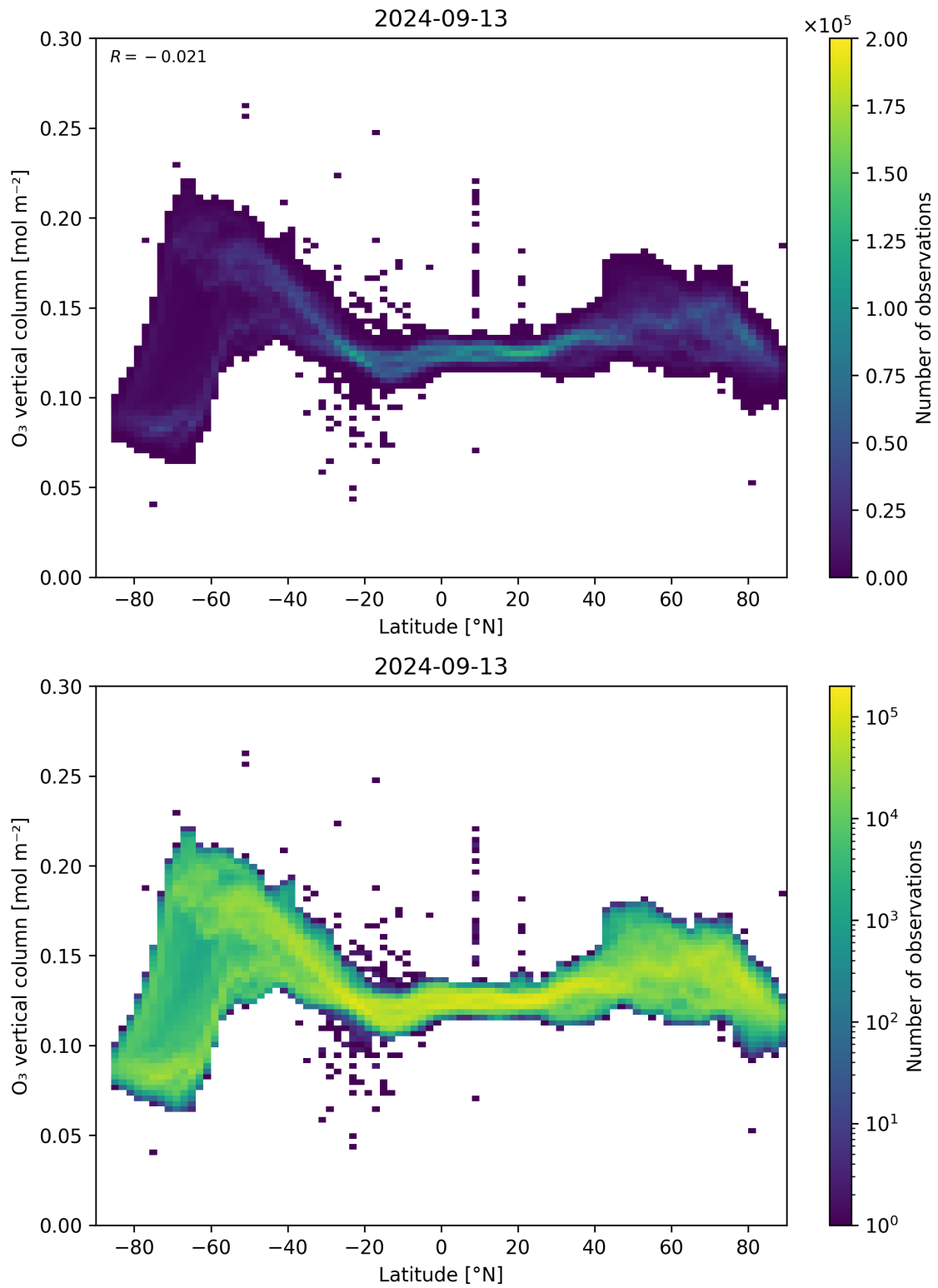
Figure 36: Scatter density plot of “Latitude” against “O 3 vertical column” for 2024-09-12 to 2024-09-14.
