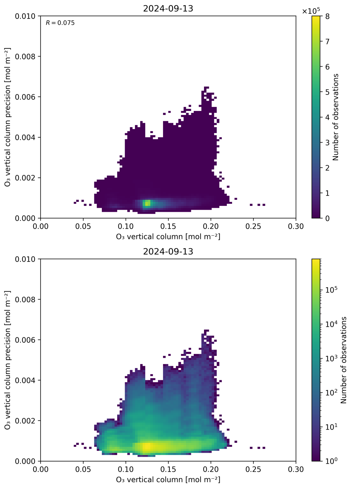
Figure 41: Scatter density plot of “O 3 vertical column” against “O 3 vertical column precision” for 2024-09-12 to 2024-09-14.
