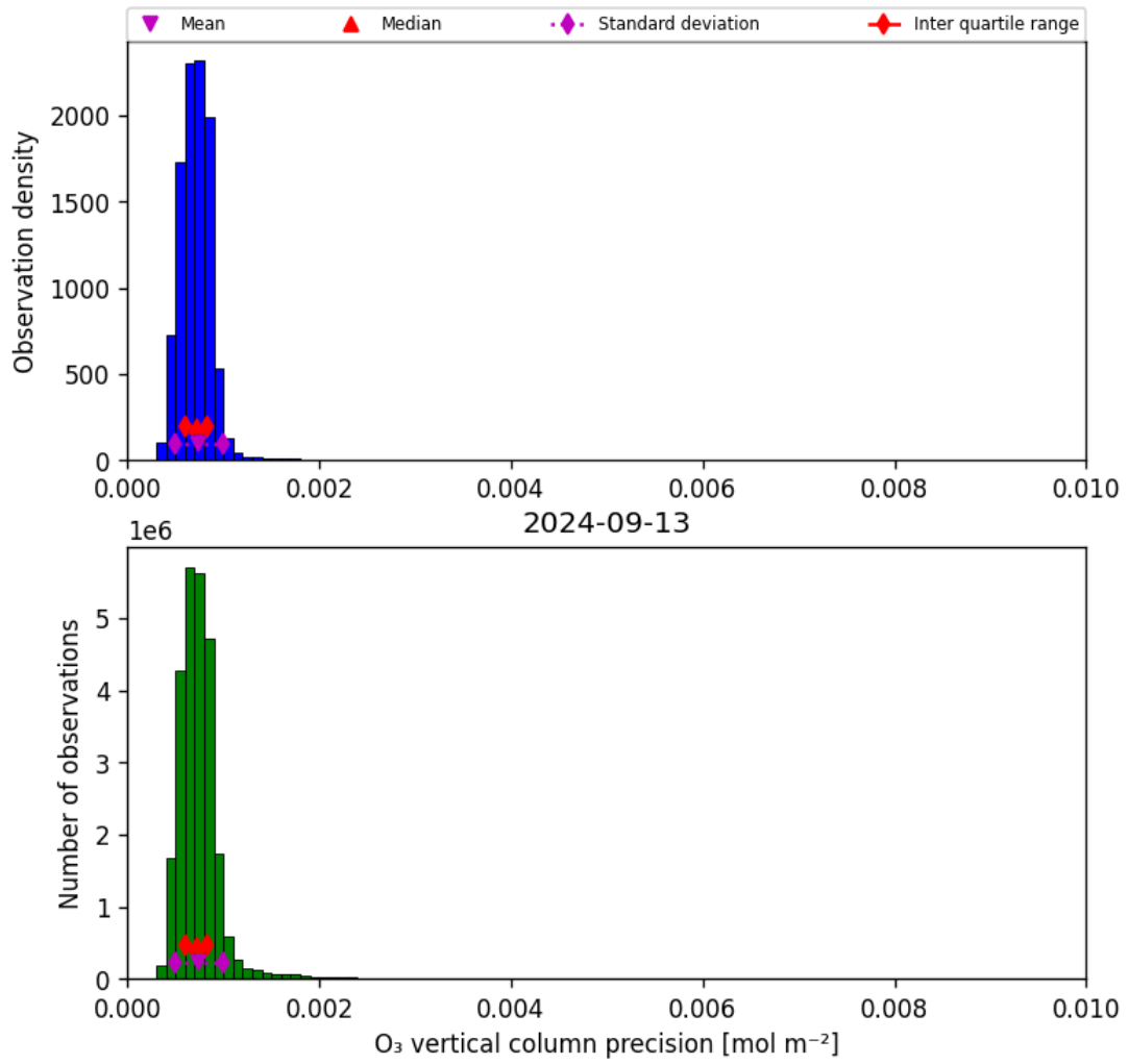
Figure 22: Histogram of “O 3 vertical column precision” for 2024-09-12 to 2024-09-14
