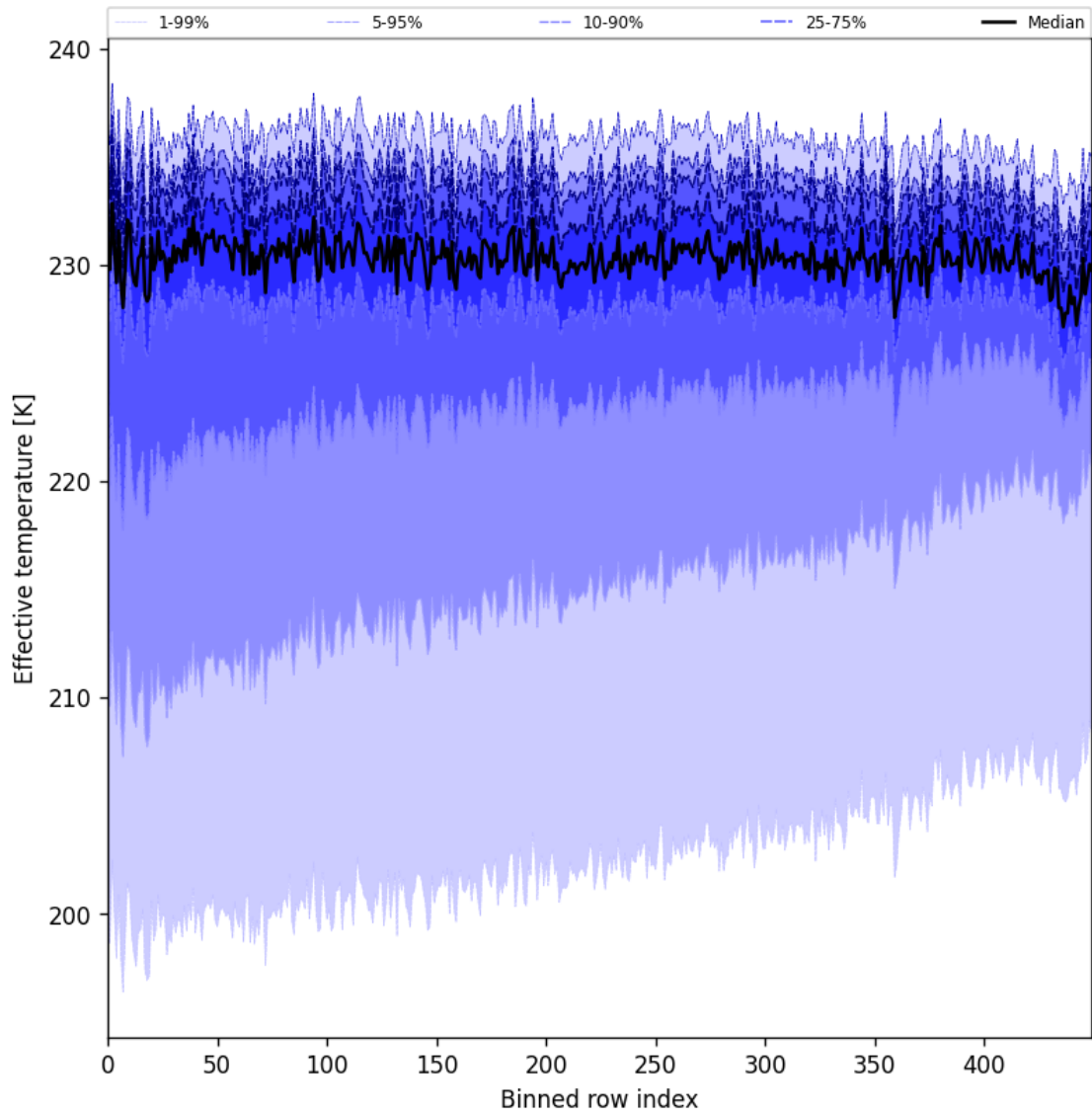
Figure 31: Along track statistics of “Effective temperature” for 2024-09-12 to 2024-09-14
