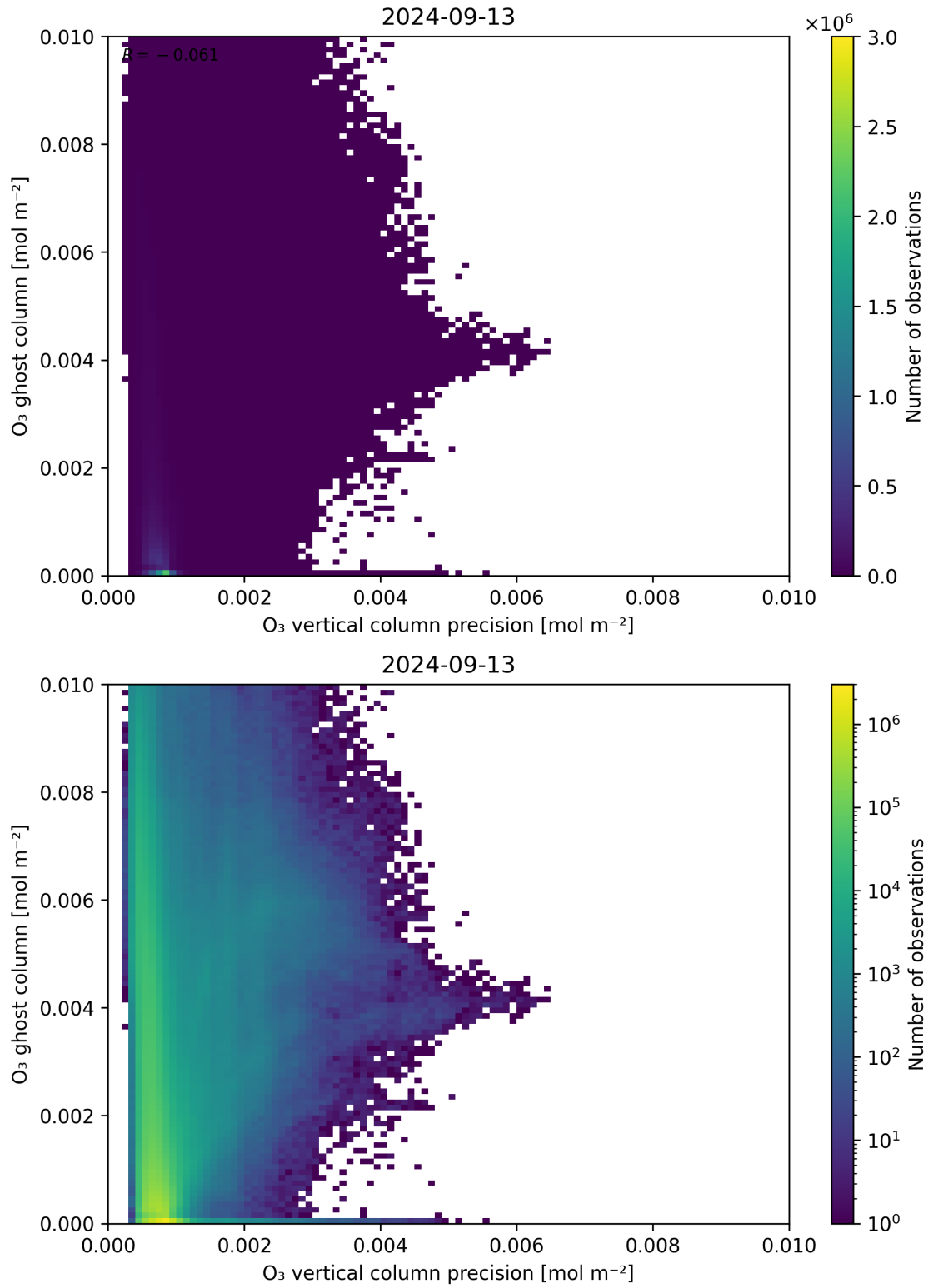
Figure 43: Scatter density plot of “ \text{O}_3 vertical column precision” against “ \text{O}_3 ghost column” for 2024-09-12 to 2024-09-14.
