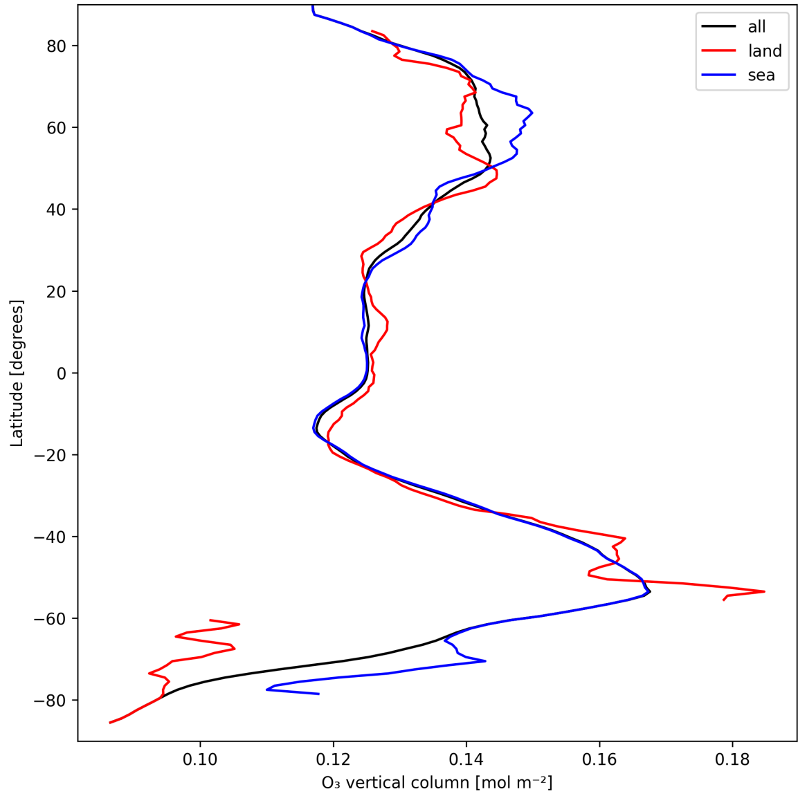
Figure 14: Zonal average of “O 3 vertical column” for 2024-09-12 to 2024-09-14.
