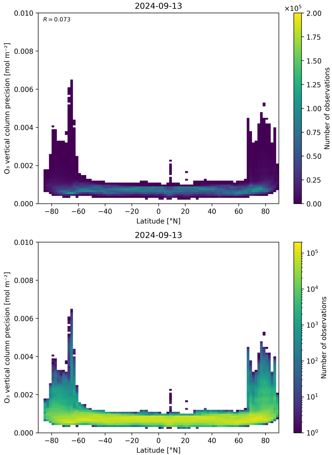
Figure 37: Scatter density plot of “Latitude” against “O 3 vertical column precision” for 2024-09-12 to 2024-09-14.
