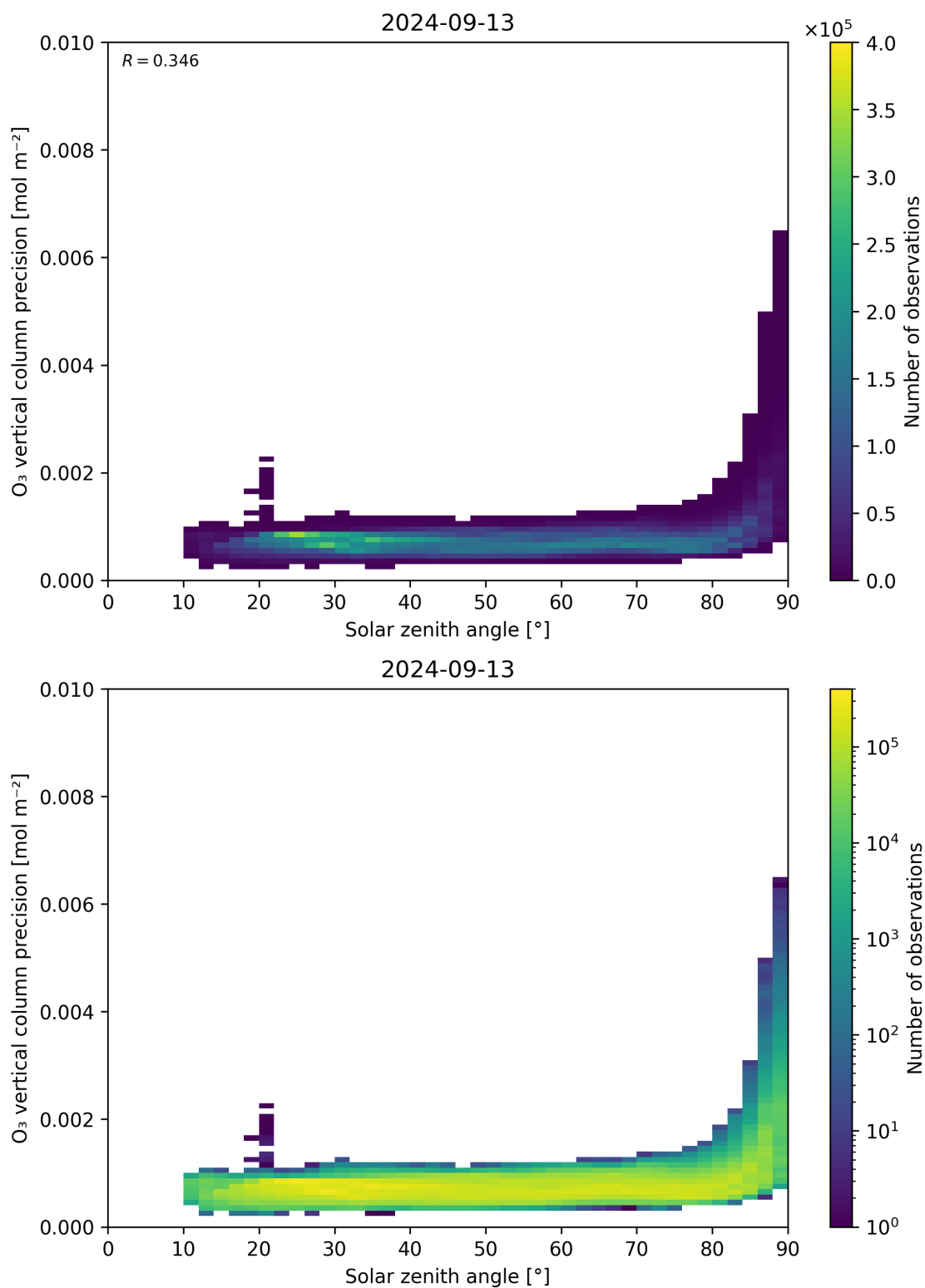
Figure 48: Scatter density plot of “Solar zenith angle” against “O 3 vertical column precision” for 2024-09-12 to 2024-09-14.
