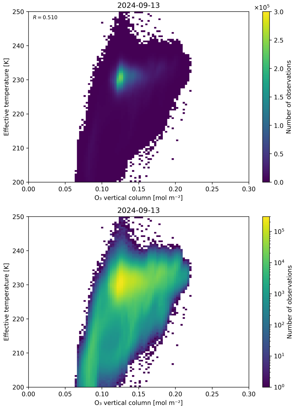
Figure 39: Scatter density plot of “O 3 vertical column” against “Effective temperature” for 2024-09-12 to 2024-09-14.
