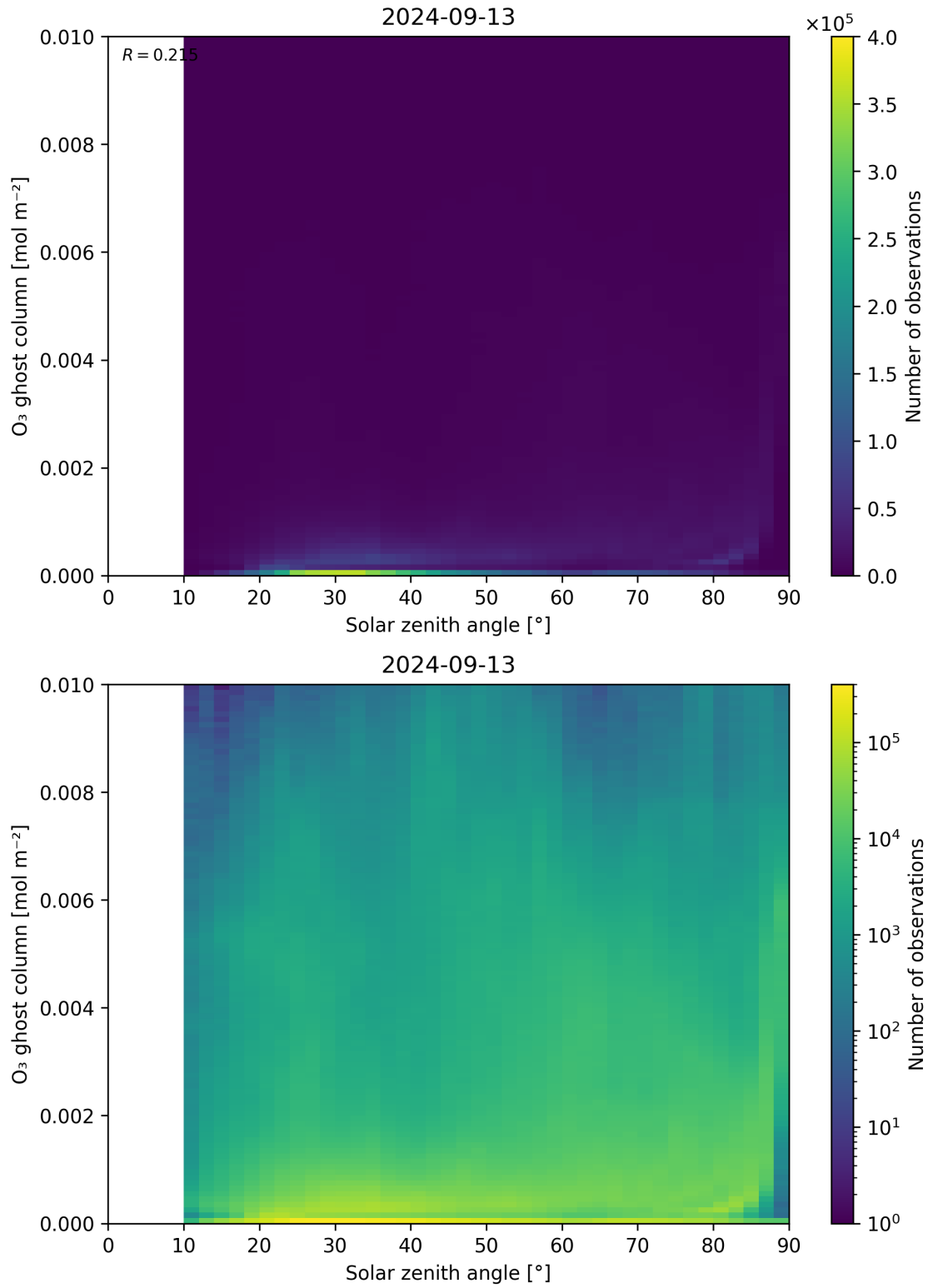
Figure 46: Scatter density plot of “Solar zenith angle” against “O 3 ghost column” for 2024-09-12 to 2024-09-14.
