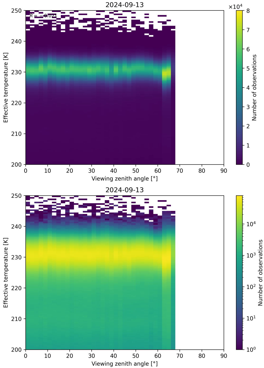
Figure 50: Scatter density plot of “Viewing zenith angle” against “Effective temperature” for 2024-09-12 to 2024-09-14.
