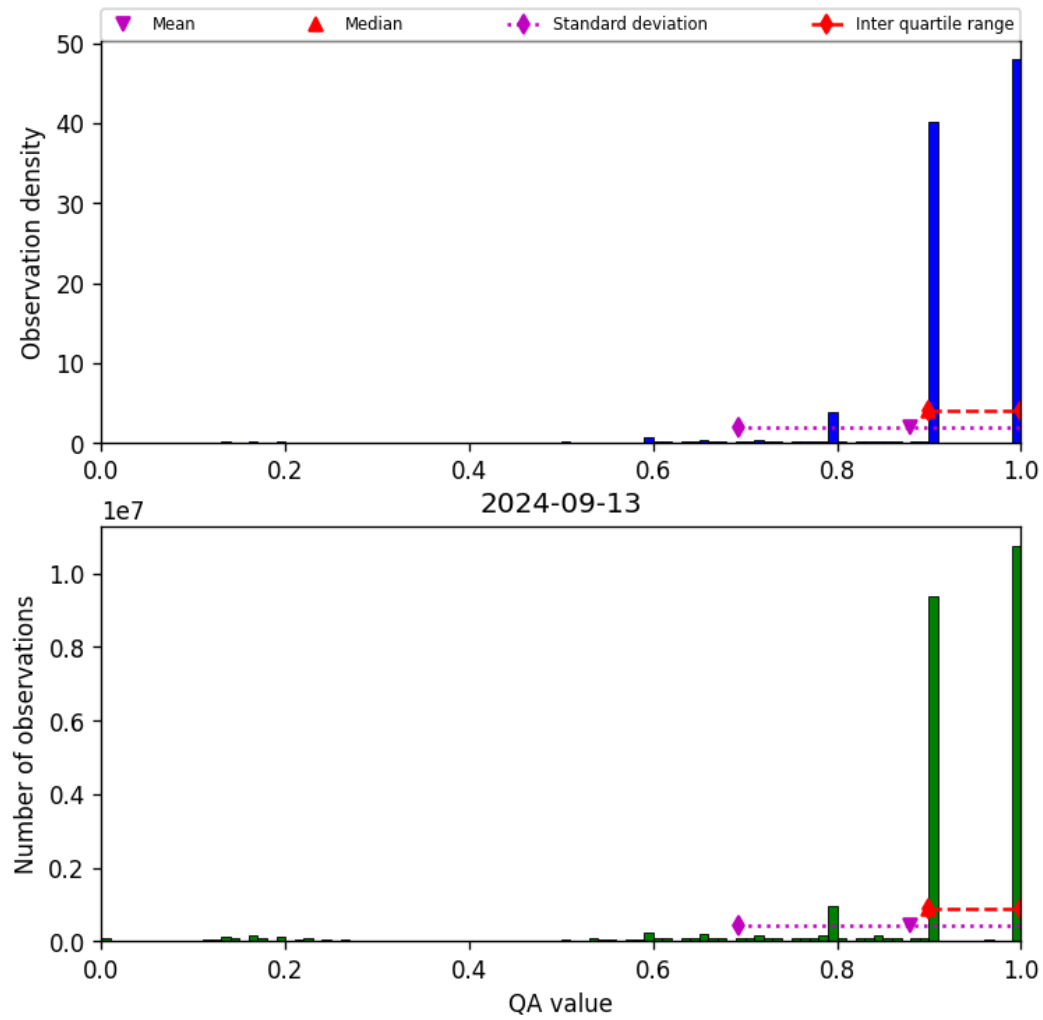
Figure 20: Histogram of “QA value” for 2024-09-12 to 2024-09-14
