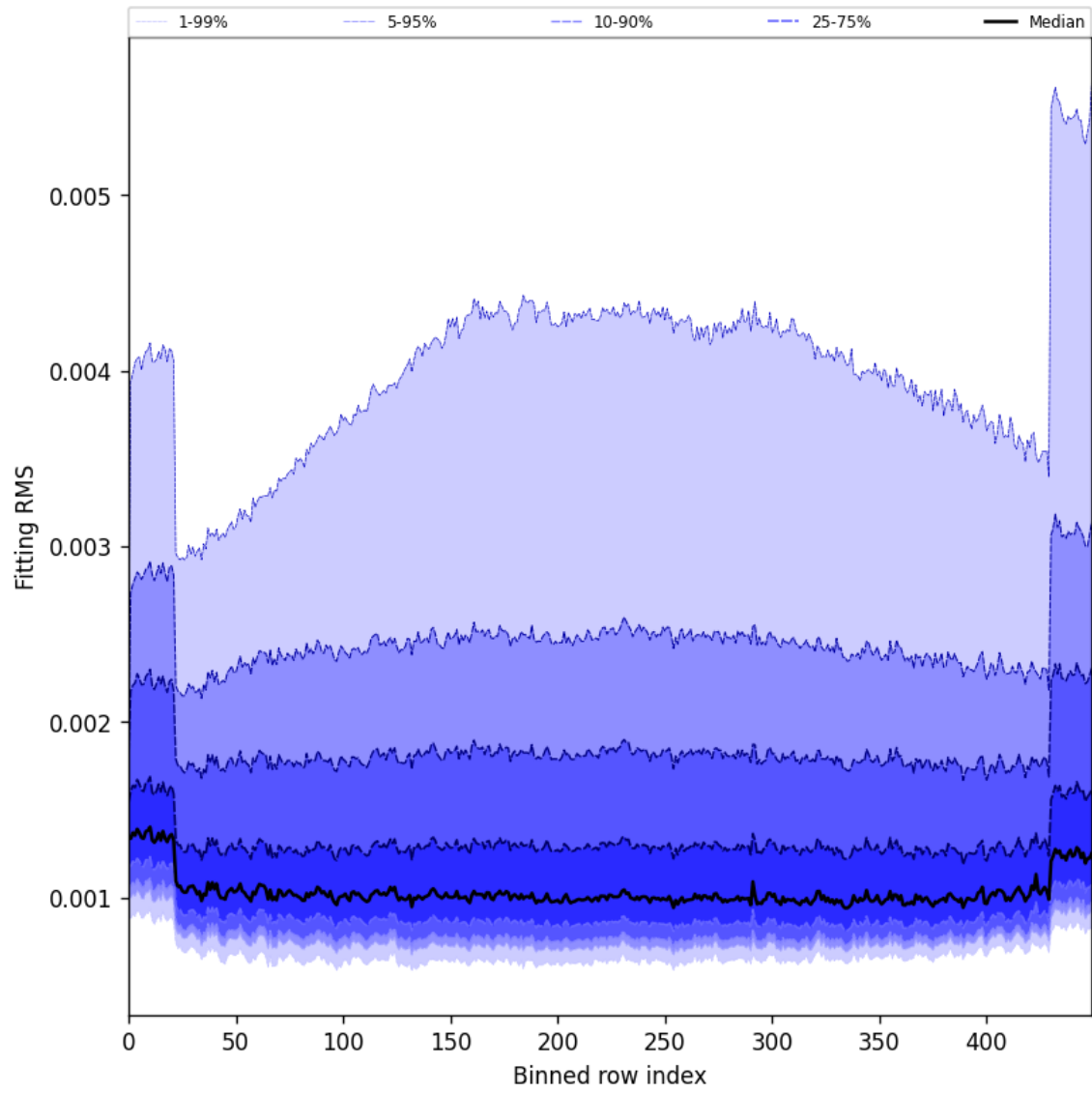
Figure 30: Along track statistics of “Fitting RMS” for 2024-09-12 to 2024-09-14
