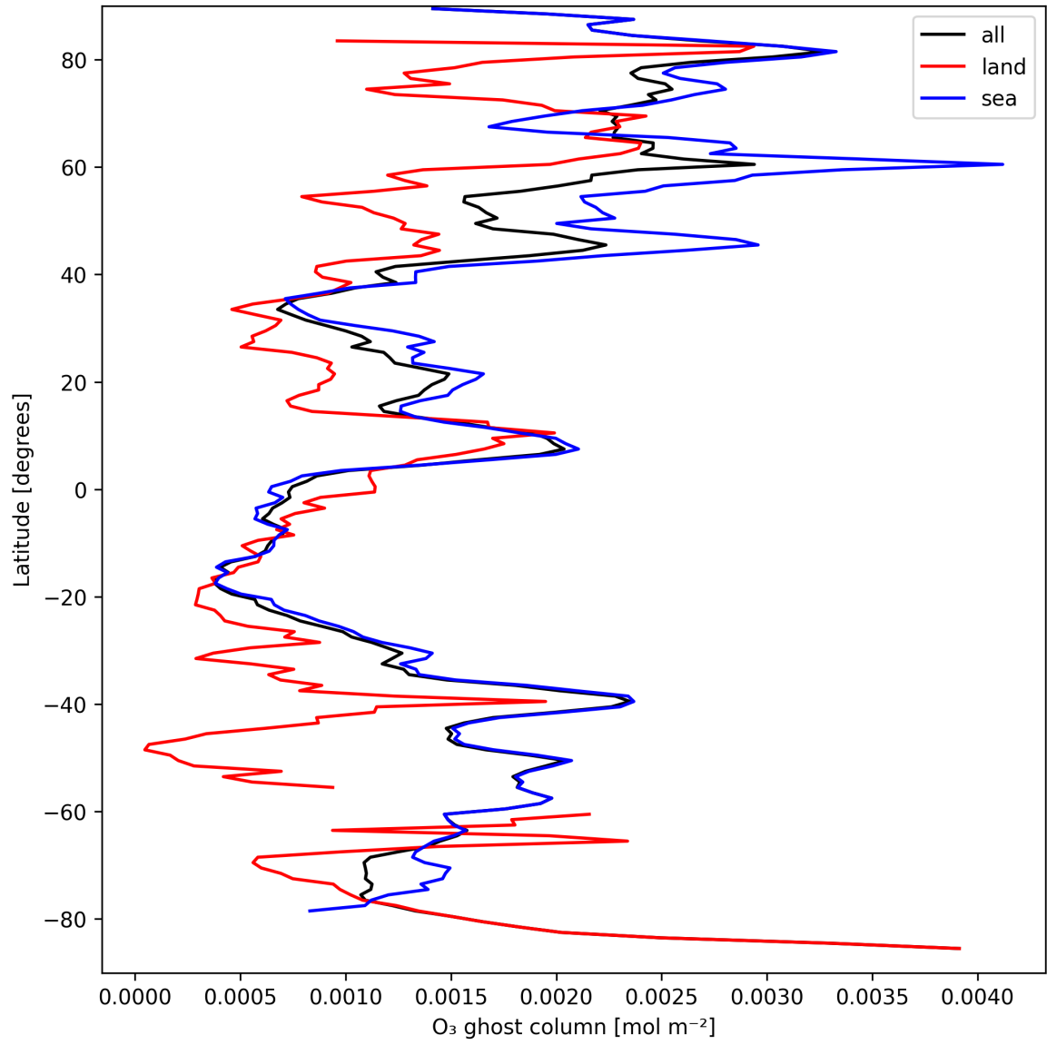
Figure 18: Zonal average of "O 3 ghost column" for 2024-09-12 to 2024-09-14.
