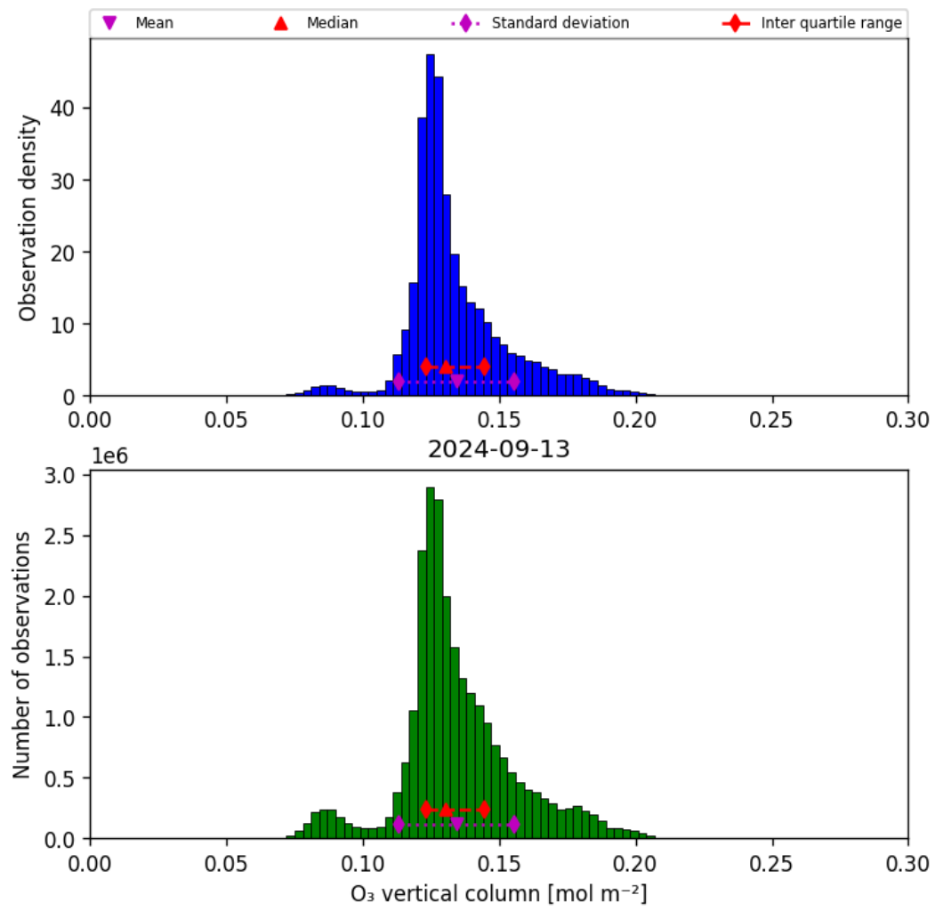
Figure 21: Histogram of “O 3 vertical column” for 2024-09-12 to 2024-09-14
