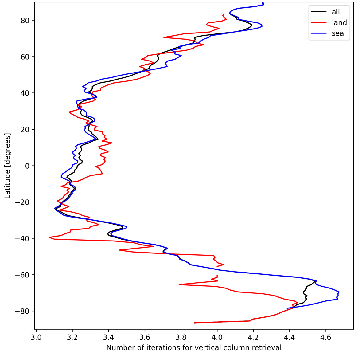
Figure 19: Zonal average of “Number of iterations for vertical column retrieval” for 2024-09-13 to 2024-09-15.
