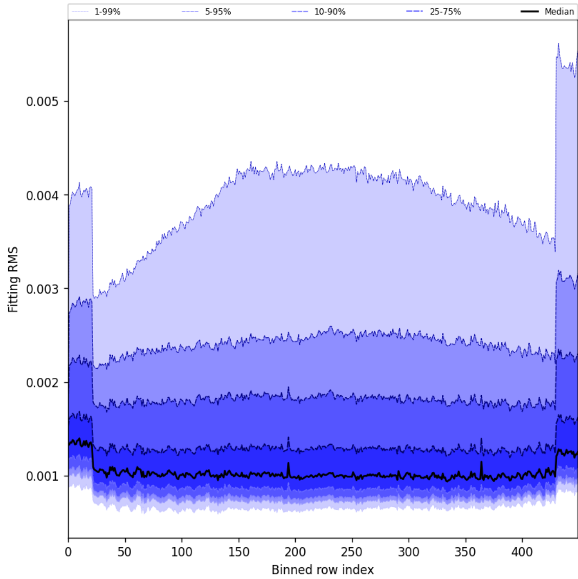
Figure 30: Along track statistics of “Fitting RMS” for 2024-09-13 to 2024-09-15
