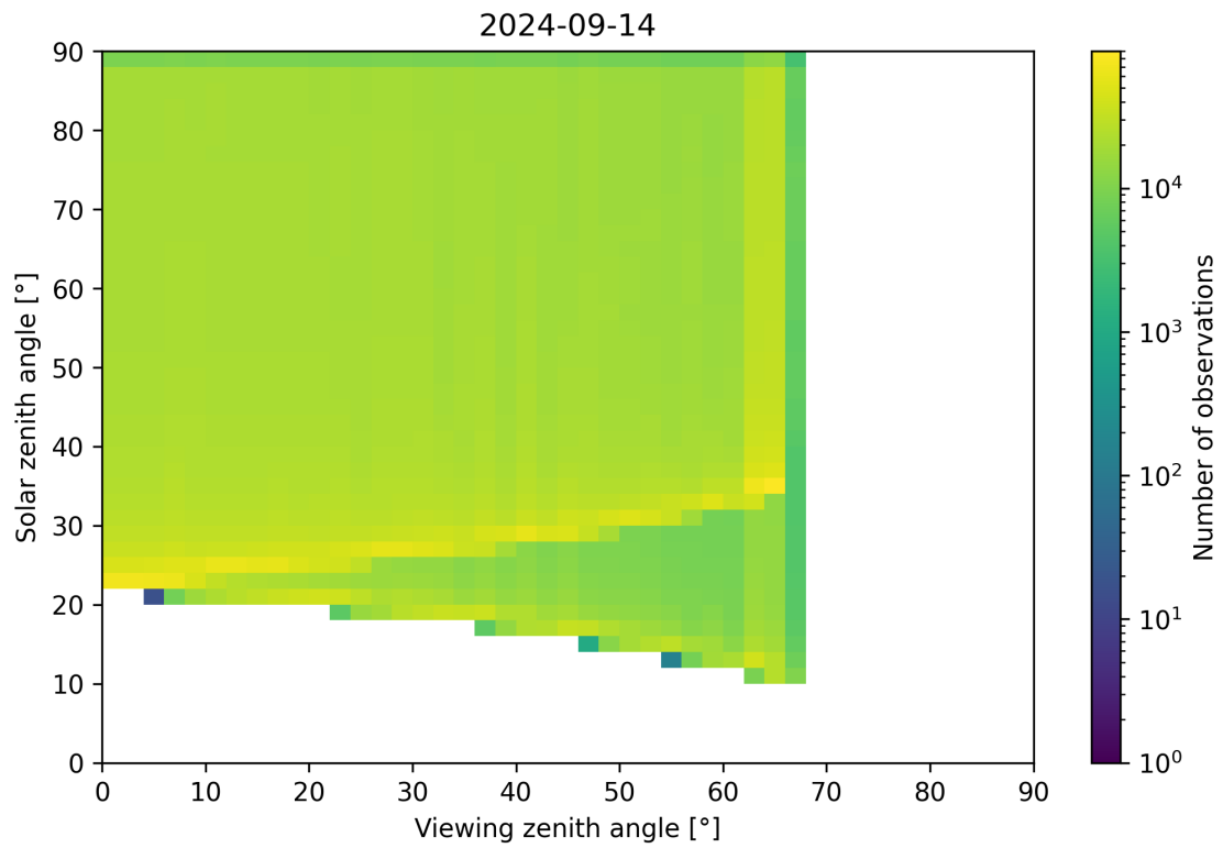
Figure 54: Scatter density plot of “Viewing zenith angle” against “Solar zenith angle” for 2024-09-13 to 2024-09-15.
