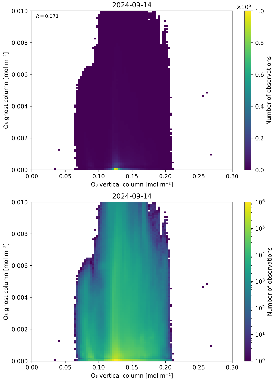
Figure 40: Scatter density plot of “O 3 vertical column” against “O 3 ghost column” for 2024-09-13 to 2024-09-15.
