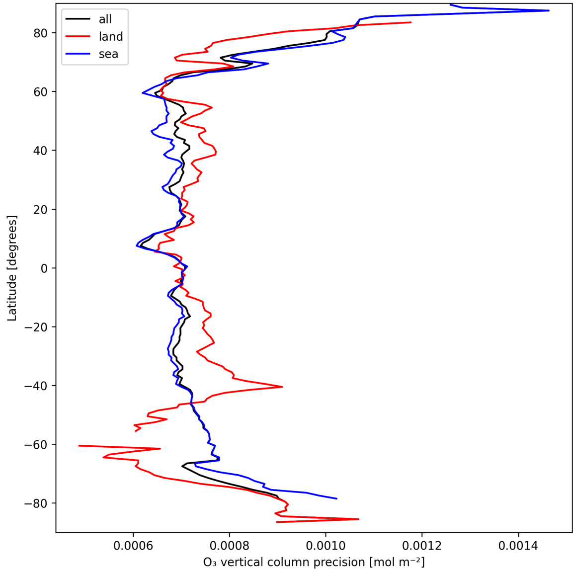
Figure 15: Zonal average of “O 3 vertical column precision” for 2024-09-13 to 2024-09-15.
