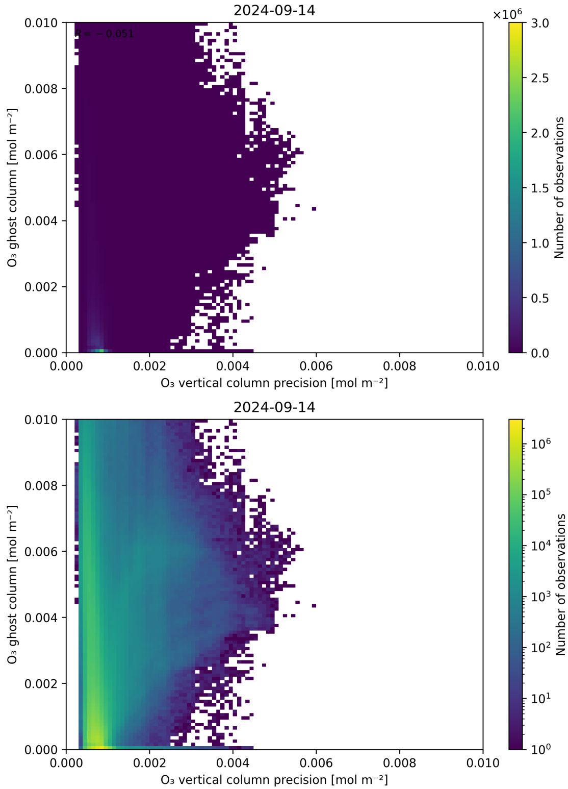
Figure 43: Scatter density plot of “ \text{O}_3 vertical column precision” against “ \text{O}_3 ghost column” for 2024-09-13 to 2024-09-15.
