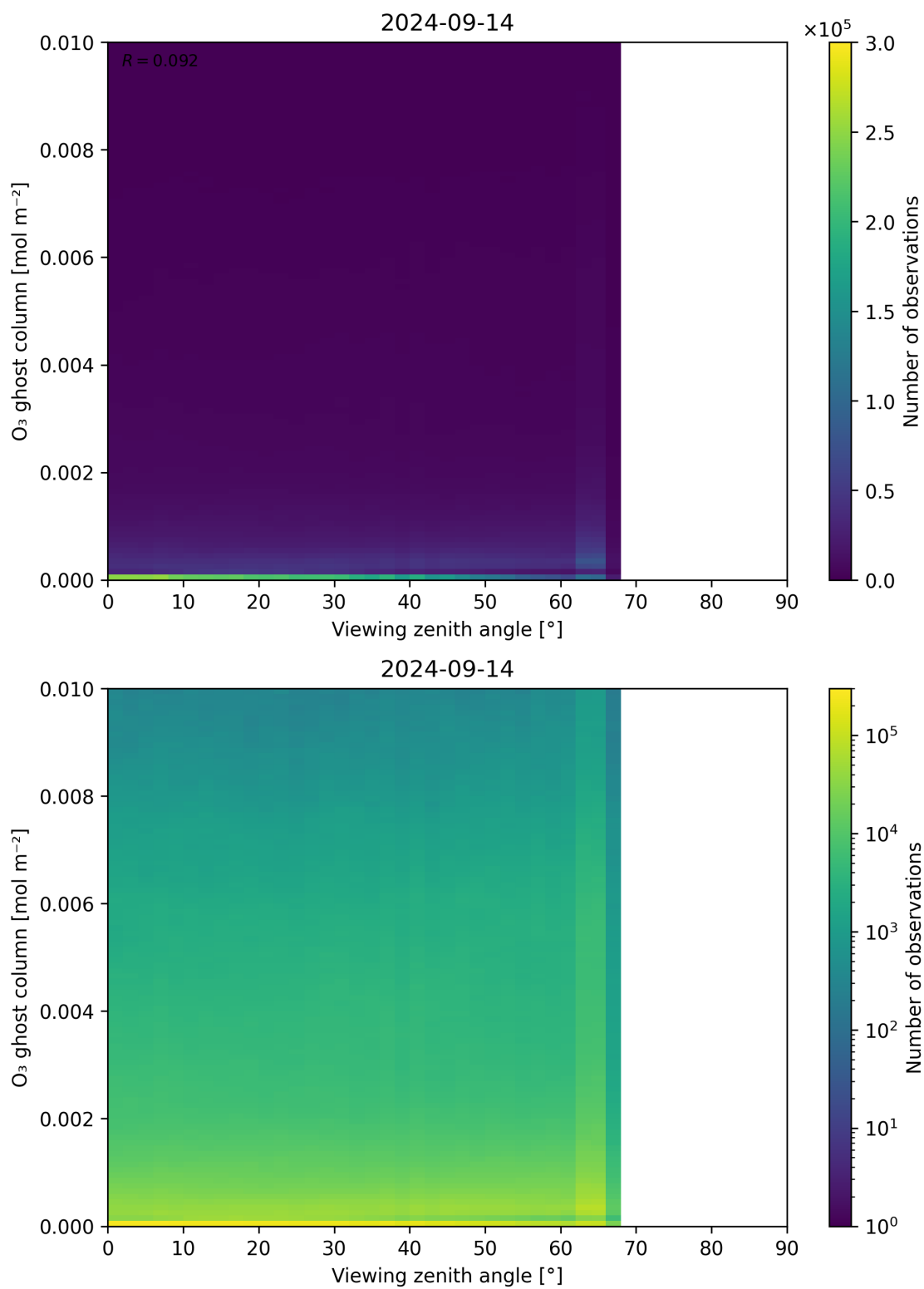
Figure 51: Scatter density plot of “Viewing zenith angle” against “O 3 ghost column” for 2024-09-13 to 2024-09-15.
