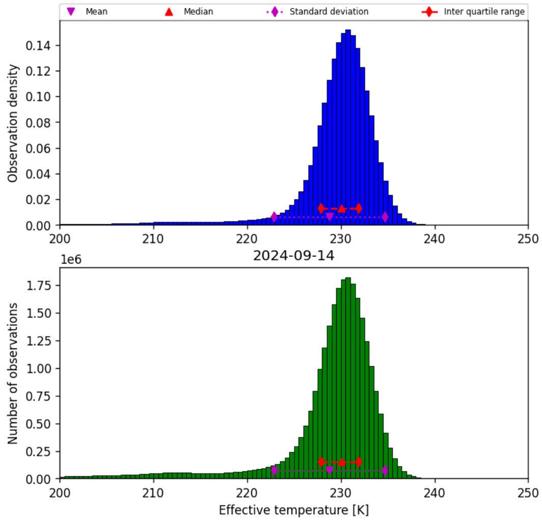
Figure 24: Histogram of “Effective temperature” for 2024-09-13 to 2024-09-15
