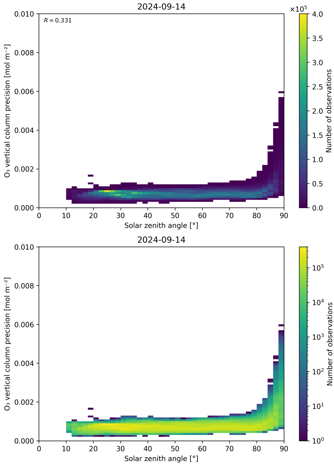
Figure 48: Scatter density plot of “Solar zenith angle” against “O 3 vertical column precision” for 2024-09-13 to 2024-09-15.
