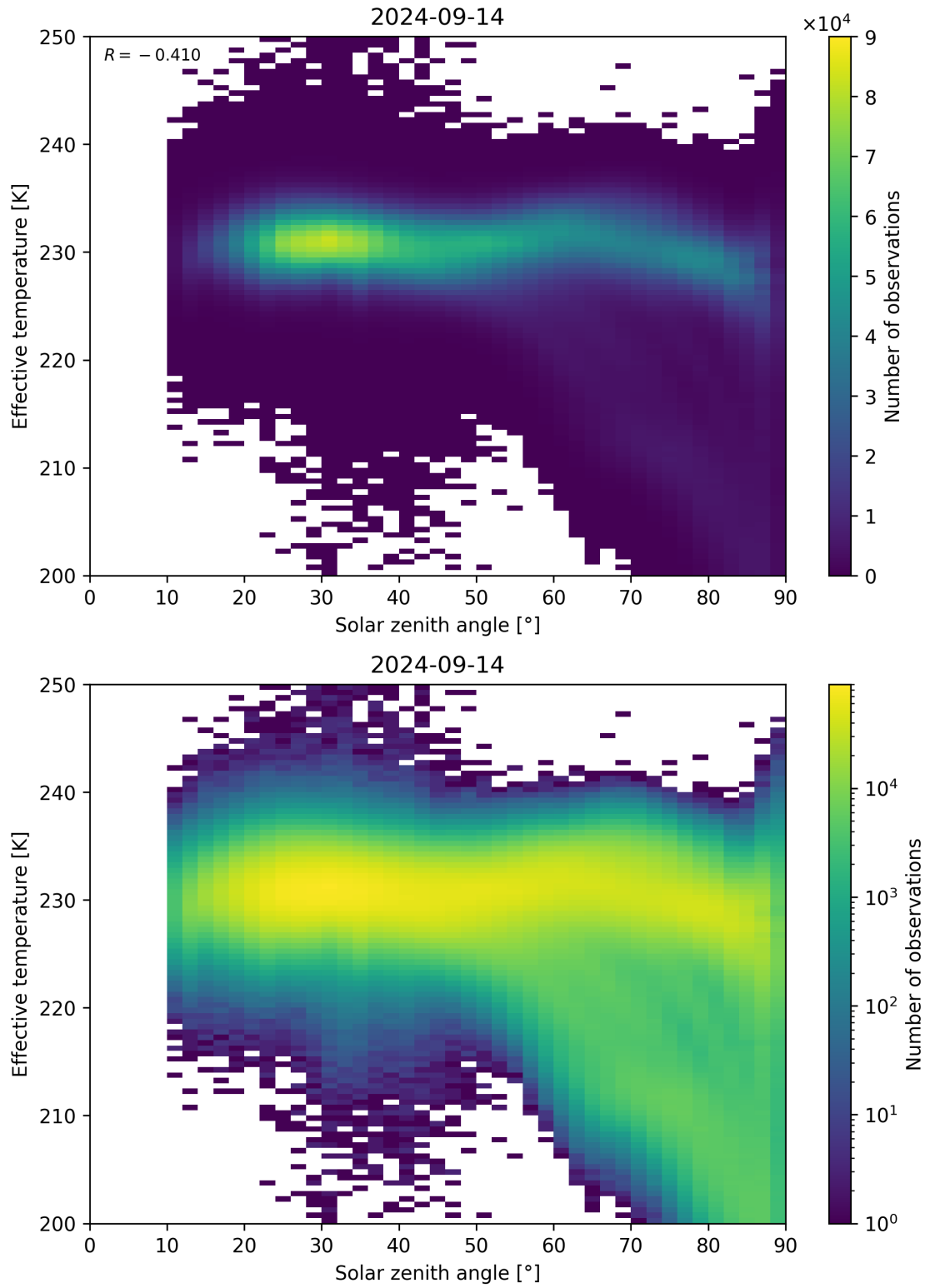
Figure 45: Scatter density plot of “Solar zenith angle” against “Effective temperature” for 2024-09-13 to 2024-09-15.
