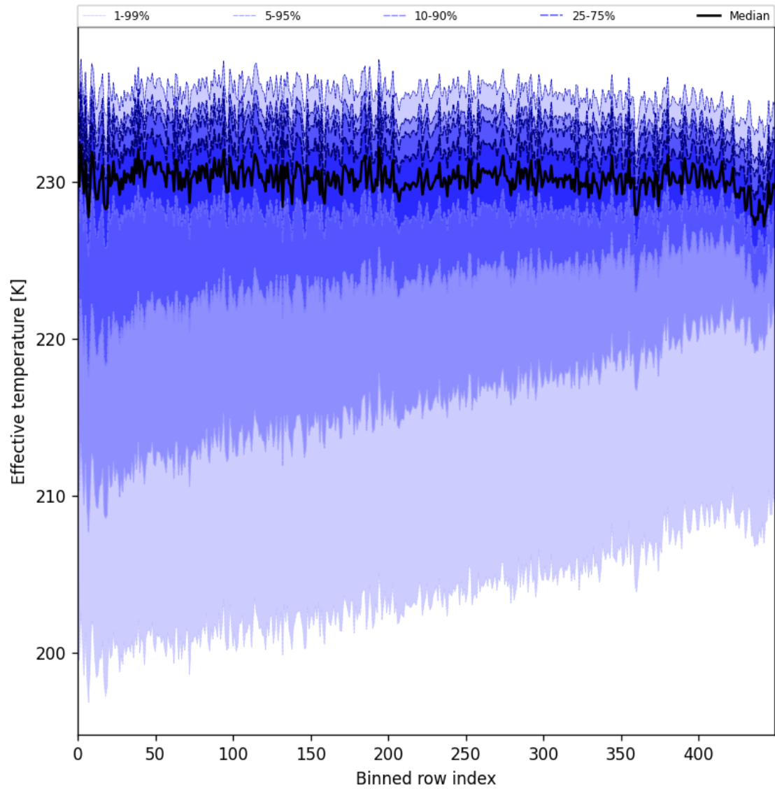
Figure 31: Along track statistics of “Effective temperature” for 2024-09-13 to 2024-09-15
