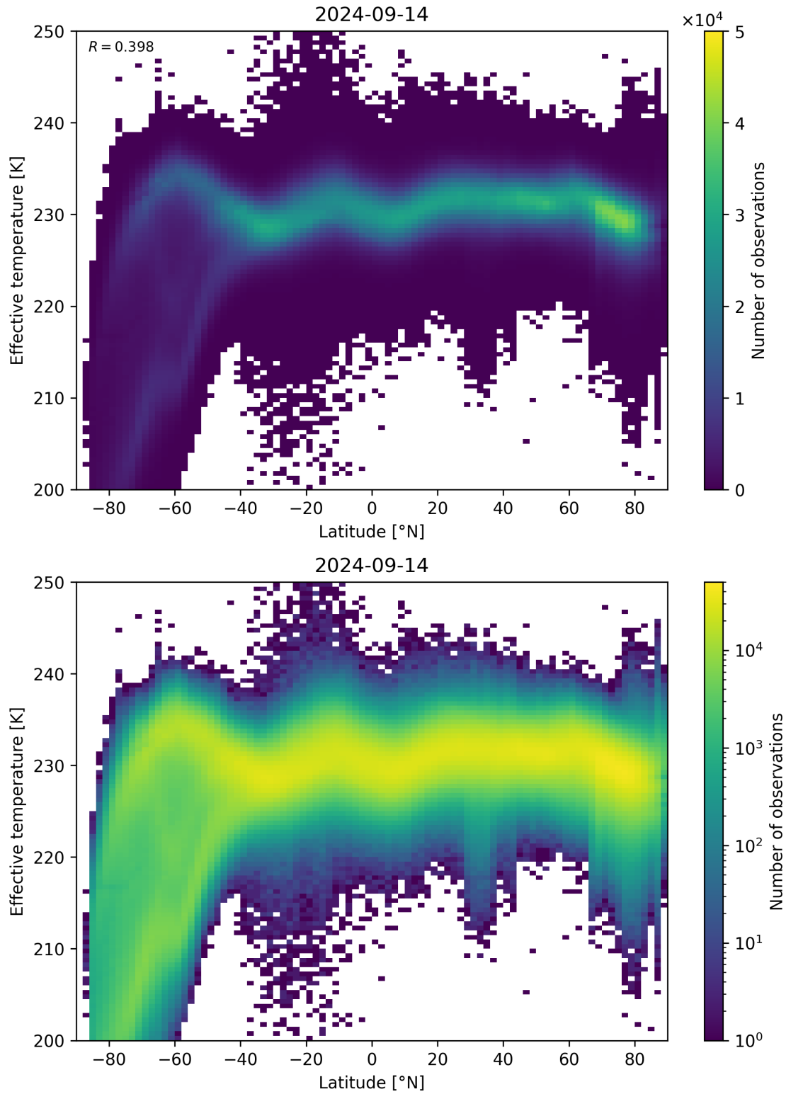
Figure 34: Scatter density plot of “Latitude” against “Effective temperature” for 2024-09-13 to 2024-09-15.
