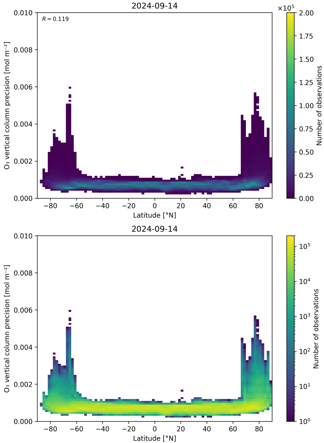
Figure 37: Scatter density plot of “Latitude” against “O 3 vertical column precision” for 2024-09-13 to 2024-09-15.
