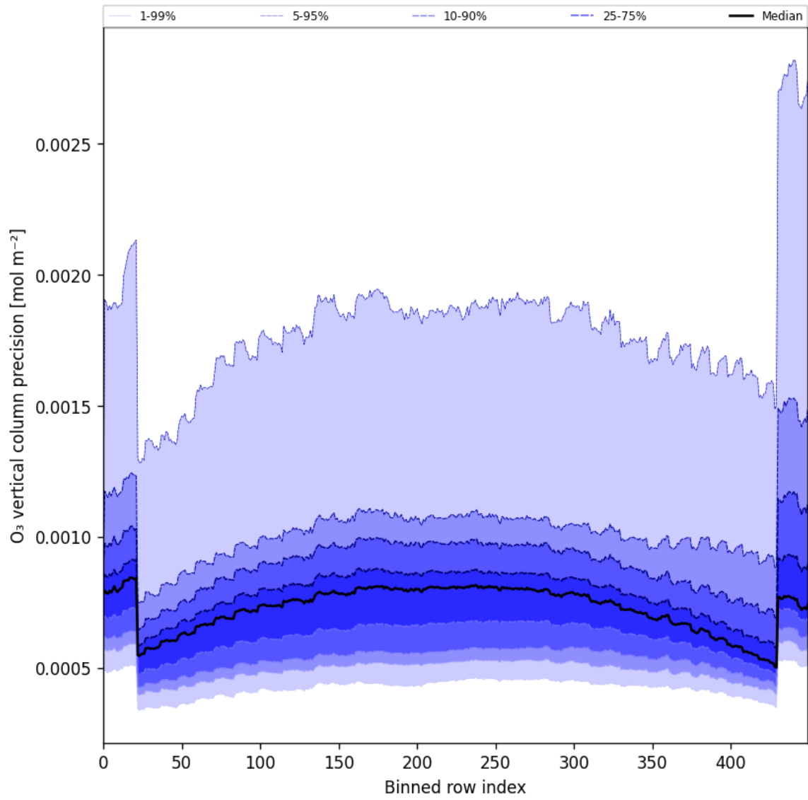
Figure 29: Along track statistics of “O 3 vertical column precision” for 2024-09-13 to 2024-09-15
