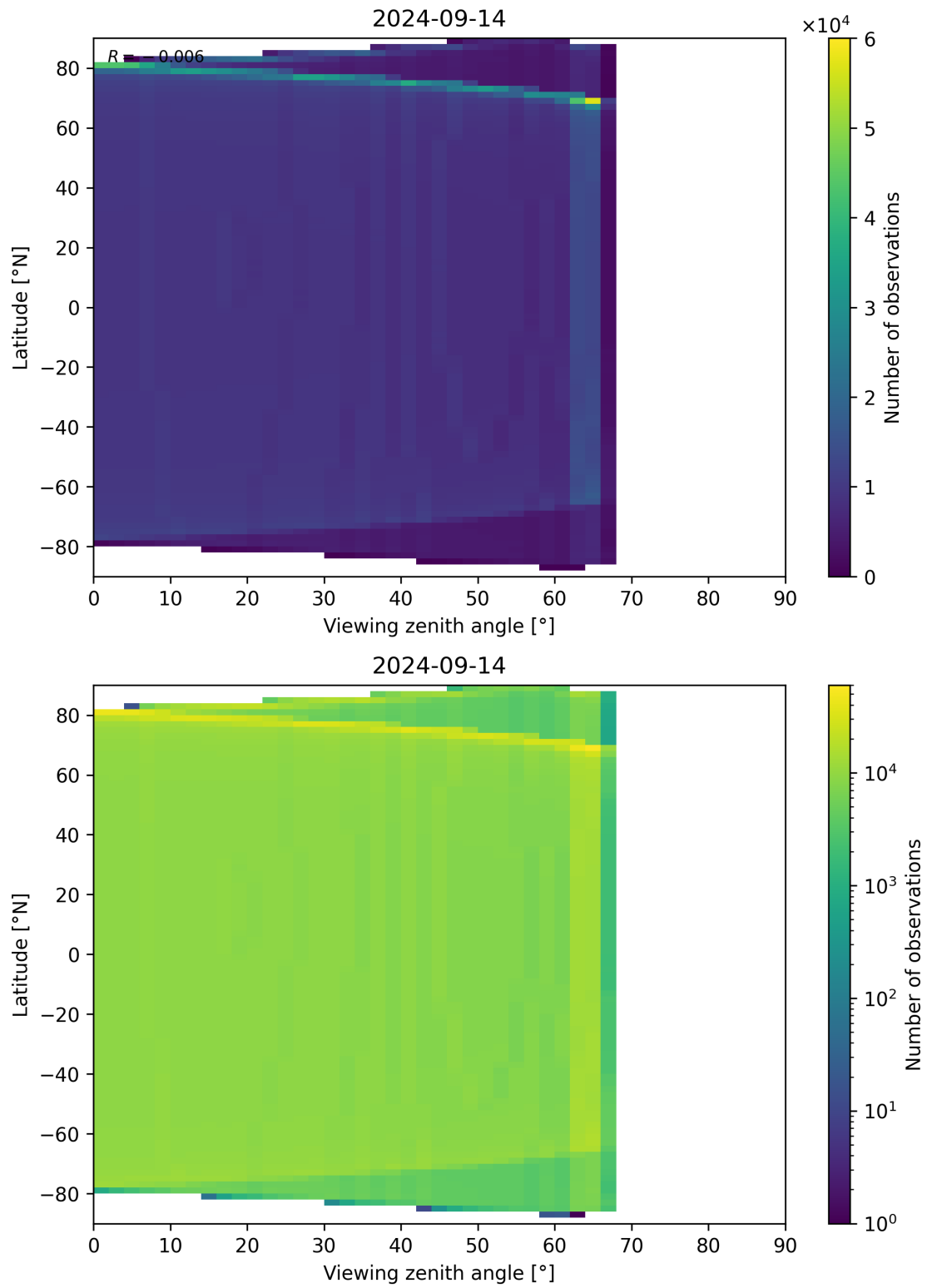
Figure 49: Scatter density plot of “Viewing zenith angle” against “Latitude” for 2024-09-13 to 2024-09-15.
