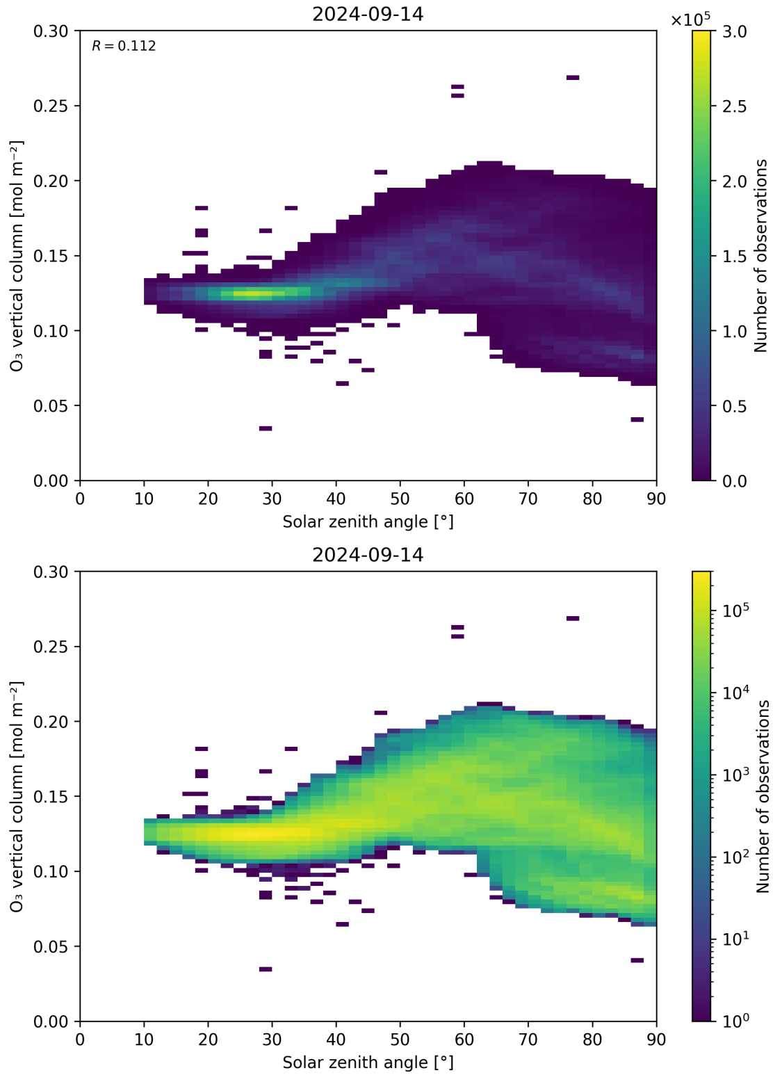
Figure 47: Scatter density plot of “Solar zenith angle” against “O 3 vertical column” for 2024-09-13 to 2024-09-15.
