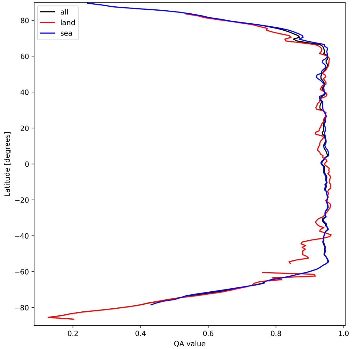
Figure 13: Zonal average of “QA value” for 2024-09-13 to 2024-09-15.
