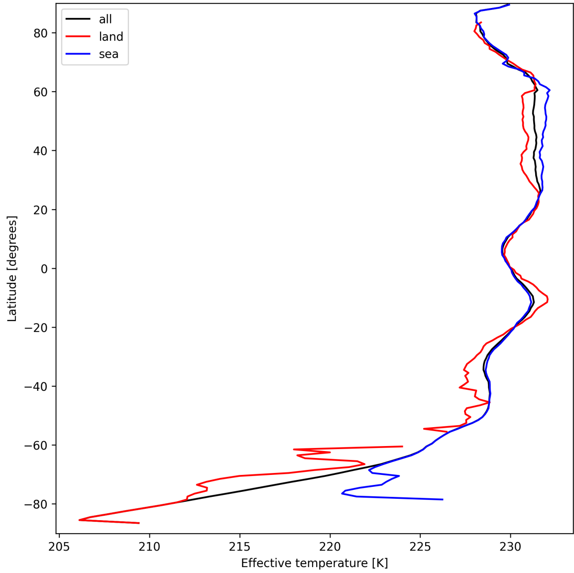
Figure 17: Zonal average of "Effective temperature" for 2024-09-13 to 2024-09-15.
