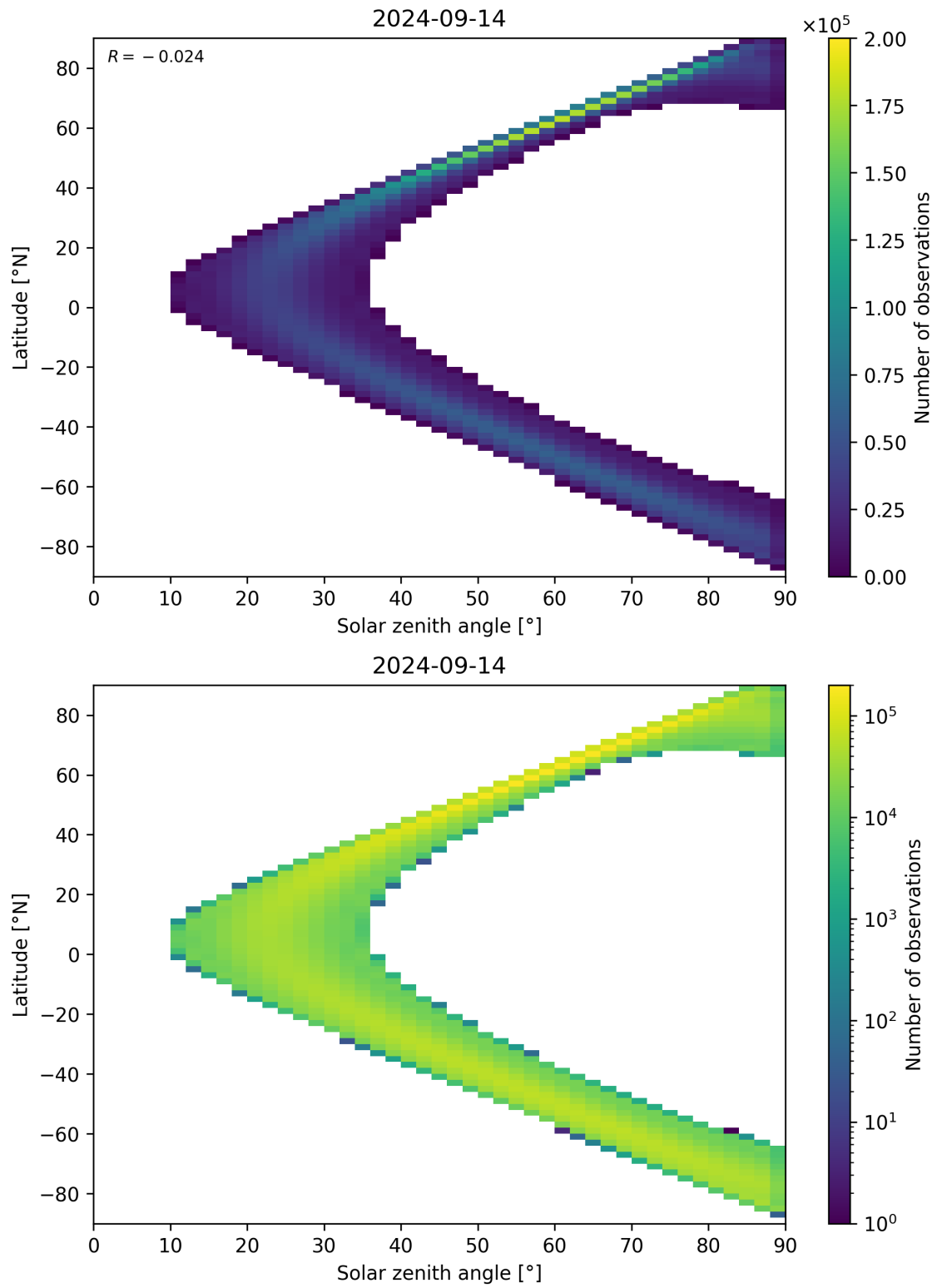
Figure 44: Scatter density plot of “Solar zenith angle” against “Latitude” for 2024-09-13 to 2024-09-15.
