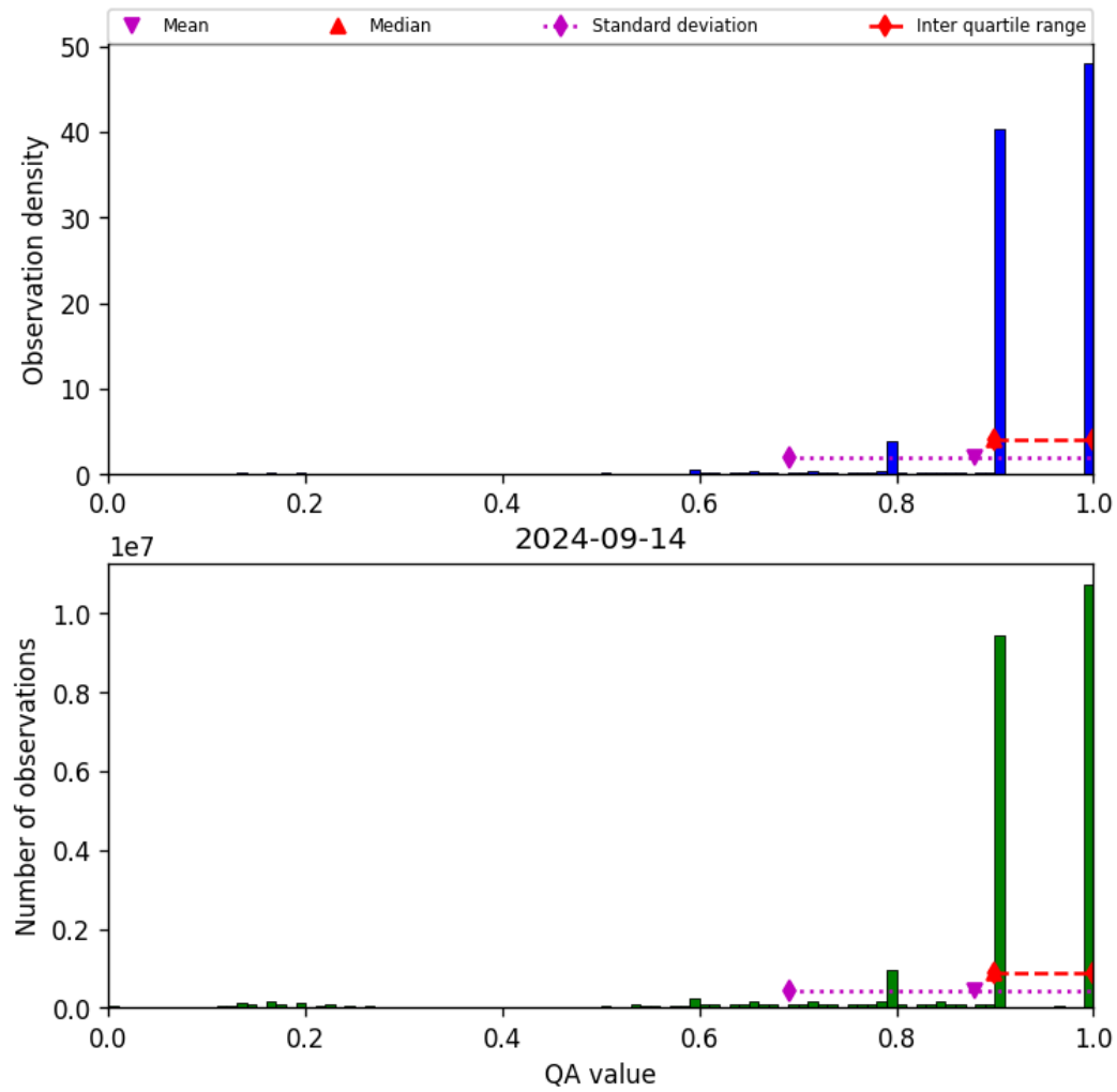
Figure 20: Histogram of “QA value” for 2024-09-13 to 2024-09-15
