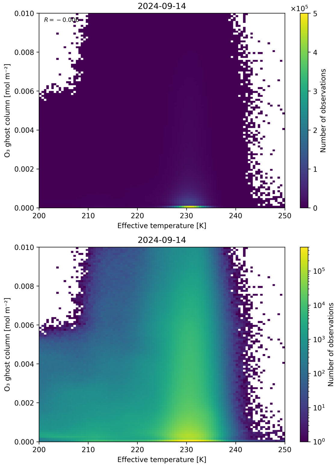
Figure 38: Scatter density plot of “Effective temperature” against “O 3 ghost column” for 2024-09-13 to 2024-09-15.
