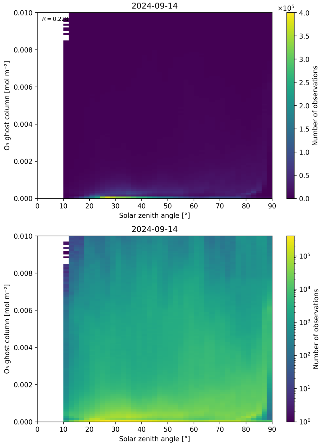
Figure 46: Scatter density plot of “Solar zenith angle” against “O 3 ghost column” for 2024-09-13 to 2024-09-15.
