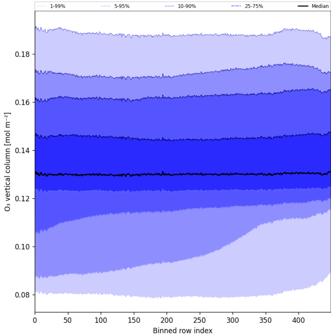
Figure 28: Along track statistics of “O 3 vertical column” for 2024-09-13 to 2024-09-15
