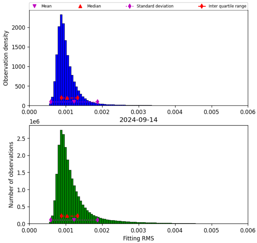
Figure 23: Histogram of “Fitting RMS” for 2024-09-13 to 2024-09-15
