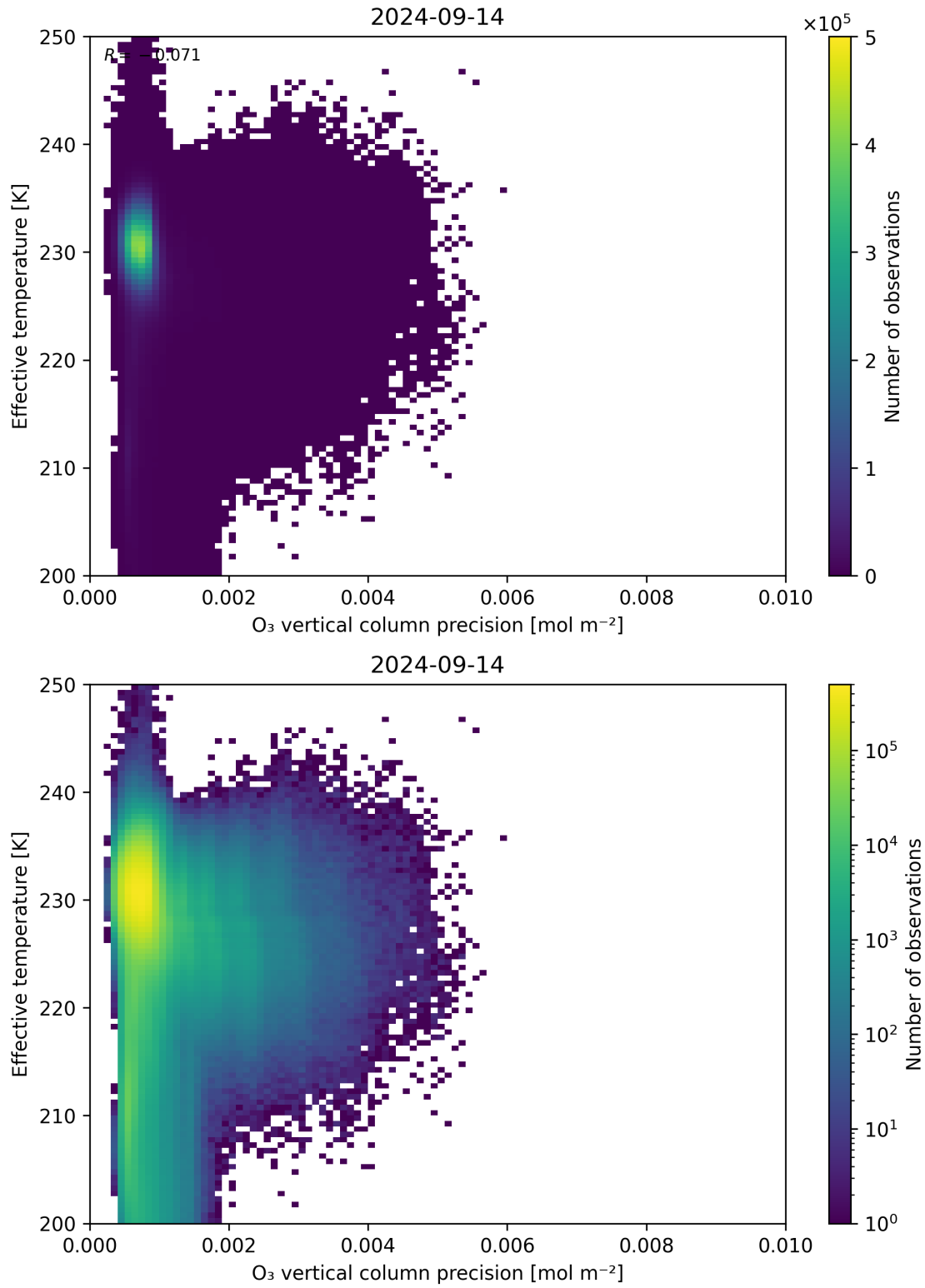
Figure 42: Scatter density plot of “O 3 vertical column precision” against “Effective temperature” for 2024-09-13 to 2024-09-15.
