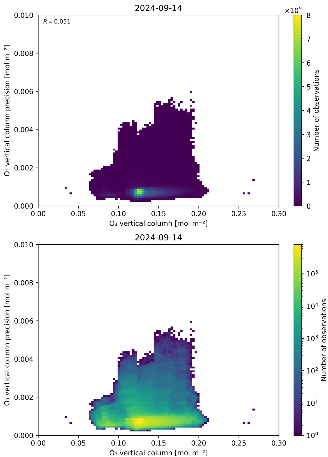
Figure 41: Scatter density plot of “O 3 vertical column” against “O 3 vertical column precision” for 2024-09-13 to 2024-09-15.
