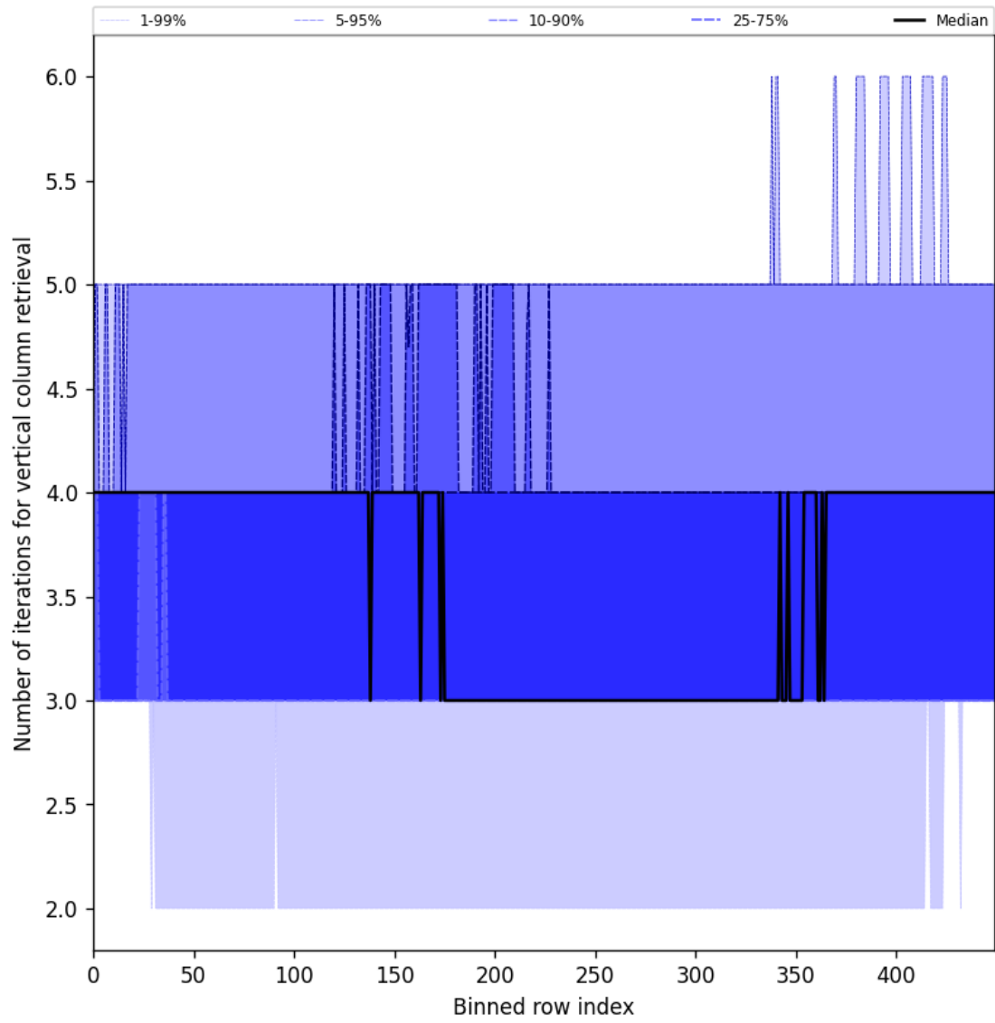
Figure 33: Along track statistics of “Number of iterations for vertical column retrieval” for 2024-09-13 to 2024-09-15
