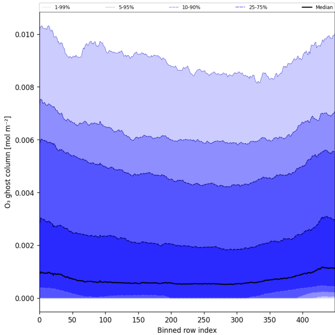
Figure 32: Along track statistics of “O 3 ghost column” for 2024-09-13 to 2024-09-15
