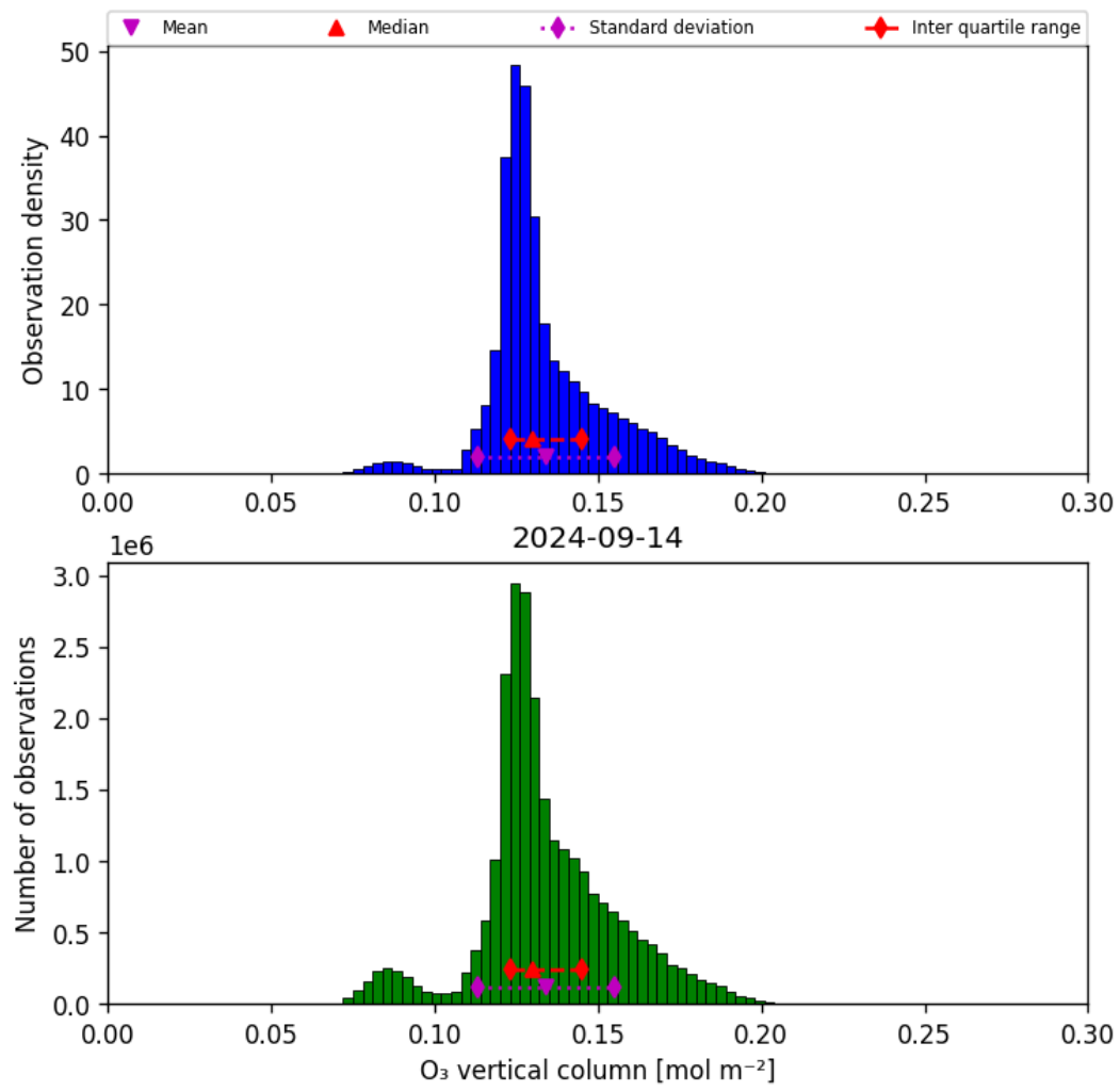
Figure 21: Histogram of “O 3 vertical column” for 2024-09-13 to 2024-09-15
