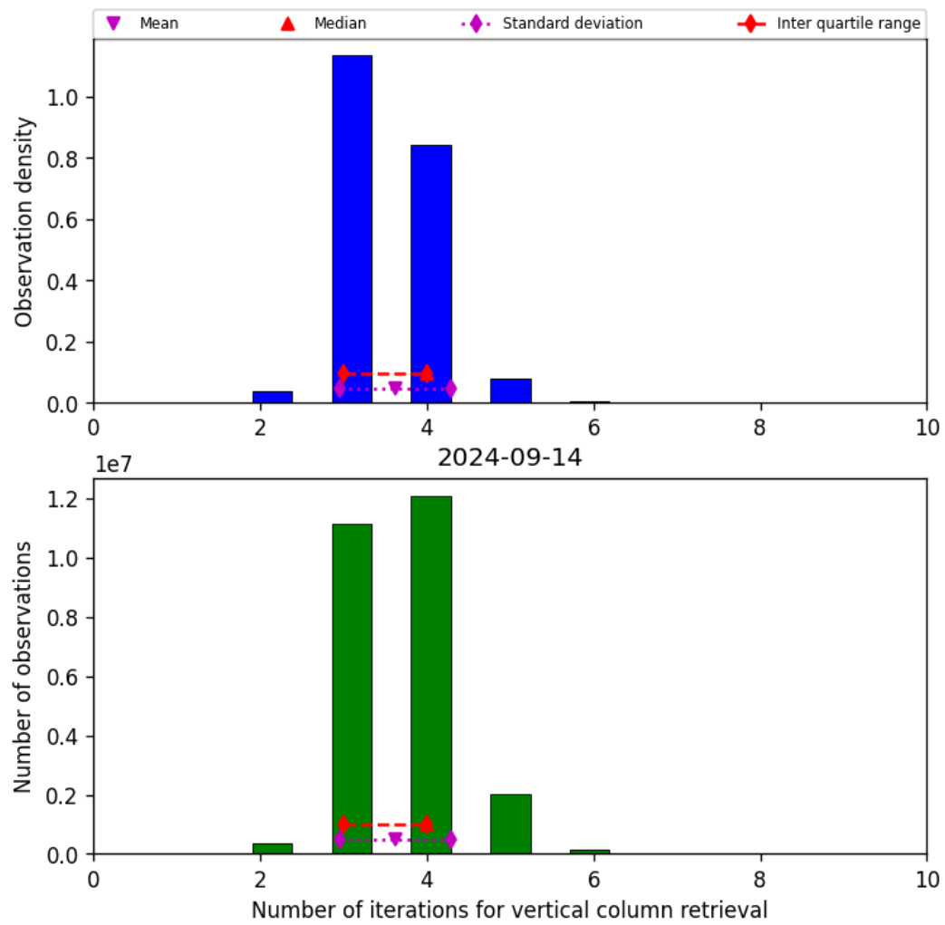
Figure 26: Histogram of “Number of iterations for vertical column retrieval” for 2024-09-13 to 2024-09-15
