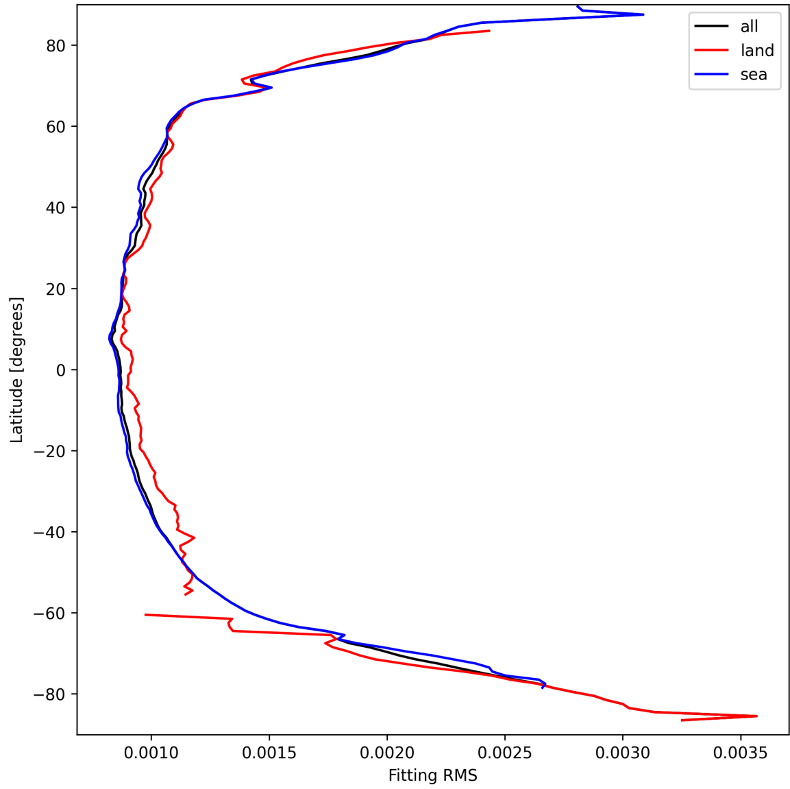
Figure 16: Zonal average of “Fitting RMS” for 2024-09-13 to 2024-09-15.
