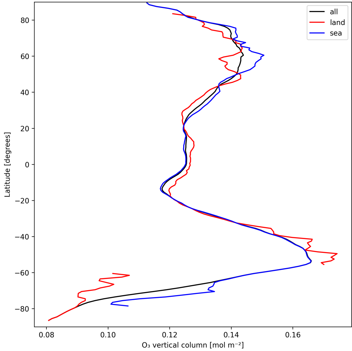
Figure 14: Zonal average of “O 3 vertical column” for 2024-09-13 to 2024-09-15.
