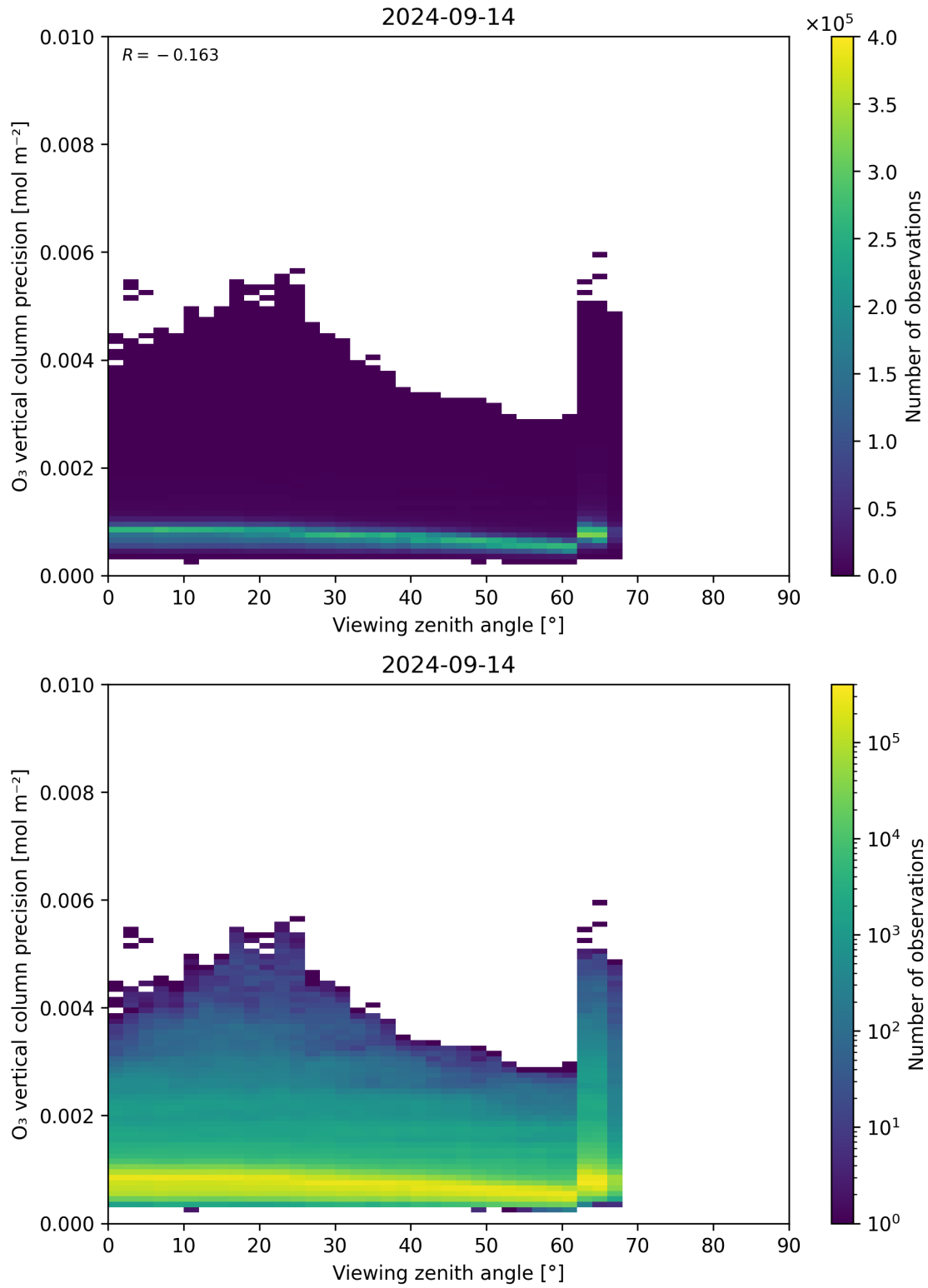
Figure 53: Scatter density plot of “Viewing zenith angle” against “O 3 vertical column precision” for 2024-09-13 to 2024-09-15.
