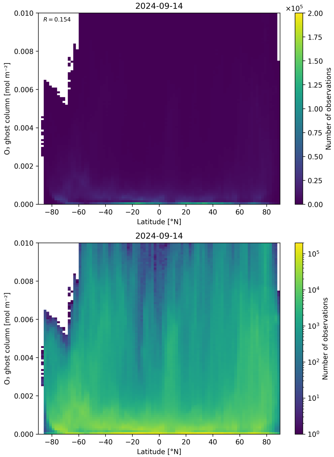
Figure 35: Scatter density plot of “Latitude” against “O 3 ghost column” for 2024-09-13 to 2024-09-15.
