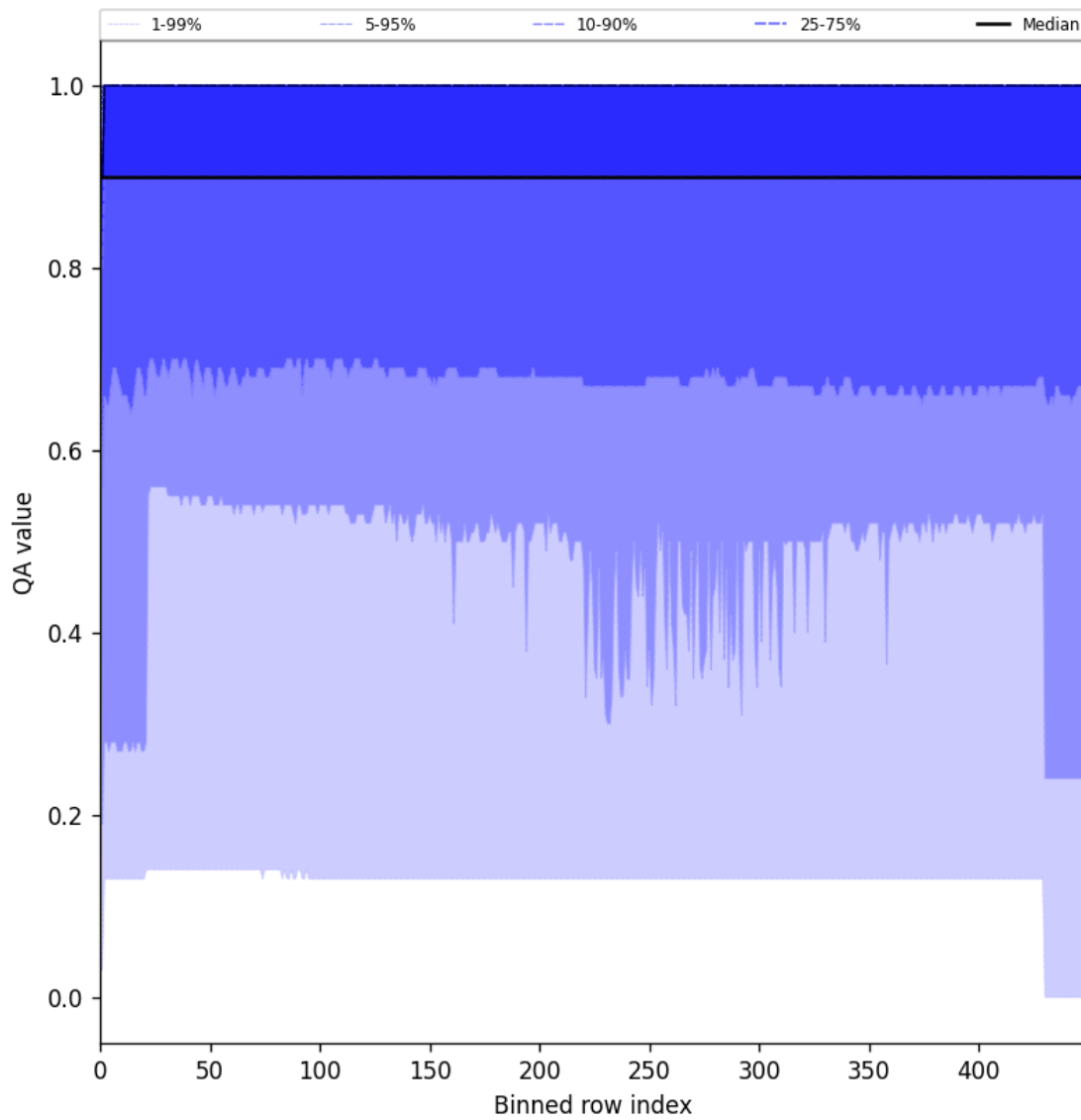
Figure 27: Along track statistics of “QA value” for 2024-09-13 to 2024-09-15
