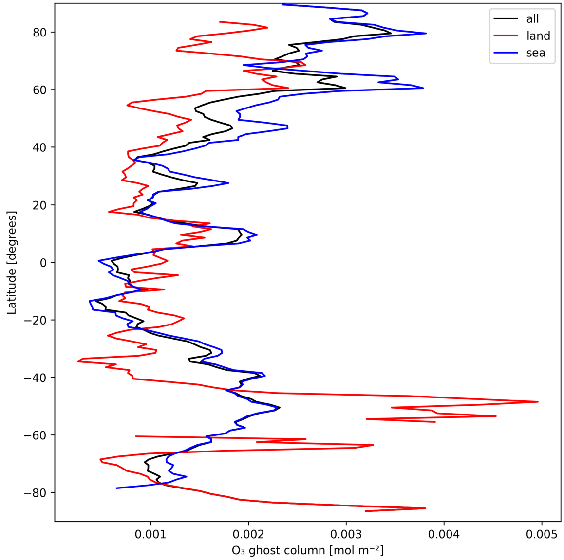
Figure 18: Zonal average of "O 3 ghost column" for 2024-09-13 to 2024-09-15.
