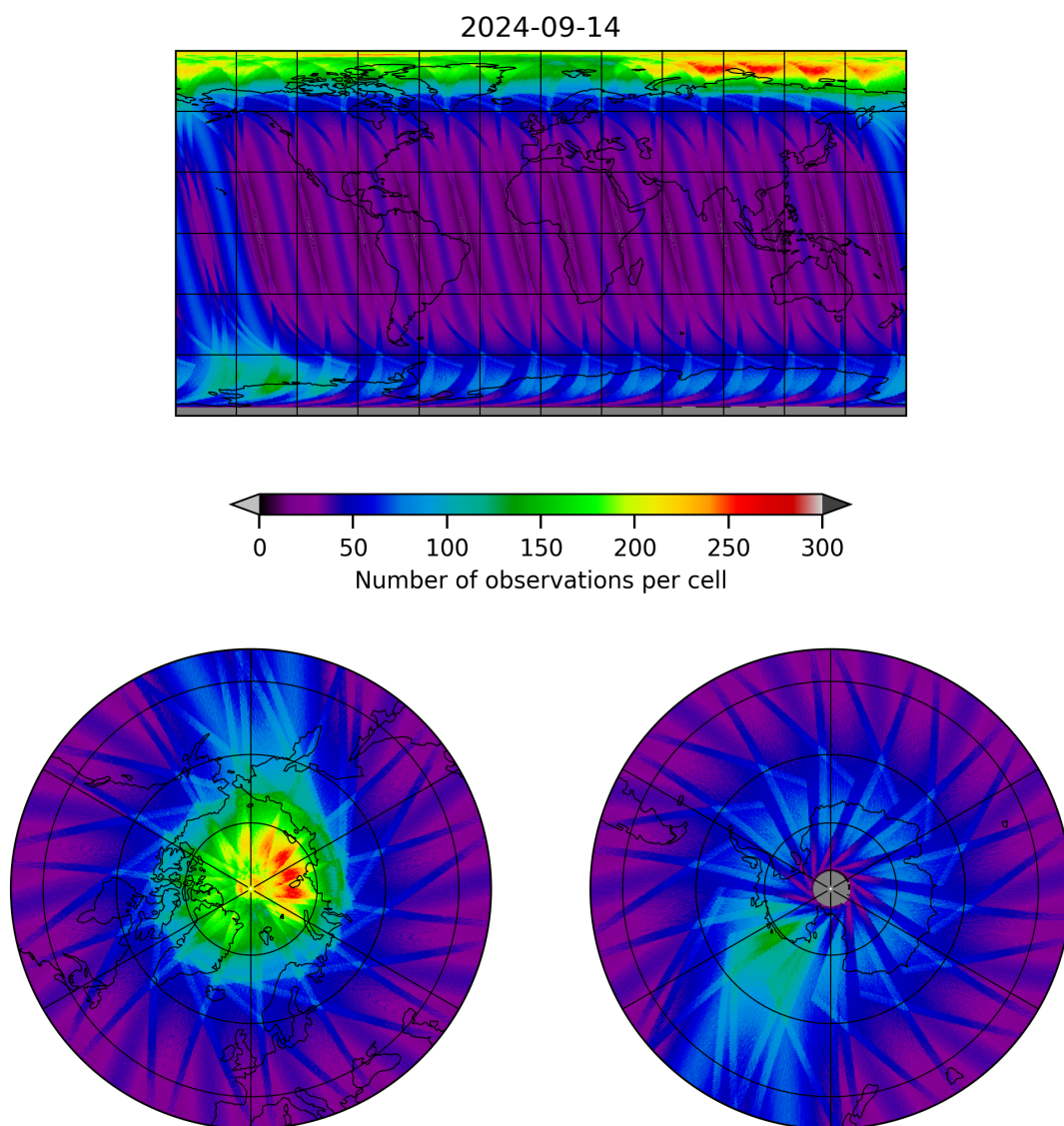
Figure 12: Map of the number of observations for 2024-09-13 to 2024-09-15
