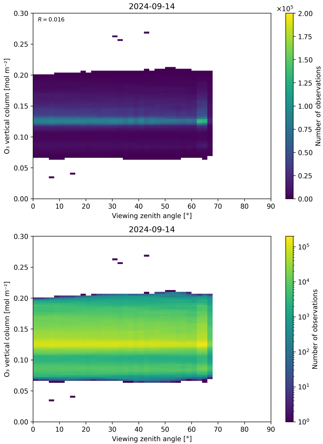
Figure 52: Scatter density plot of “Viewing zenith angle” against “O 3 vertical column” for 2024-09-13 to 2024-09-15.
