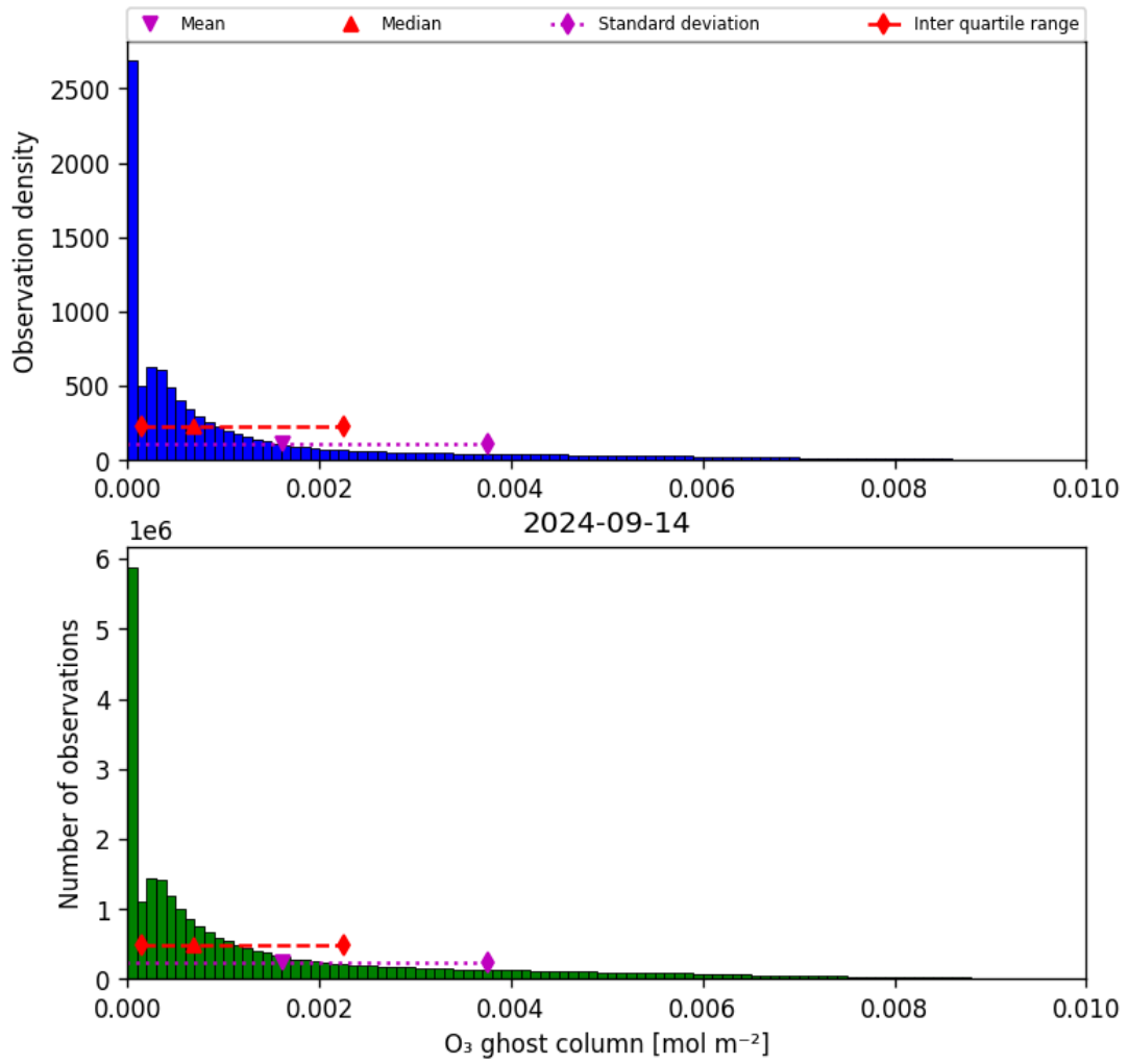
Figure 25: Histogram of “O 3 ghost column” for 2024-09-13 to 2024-09-15
