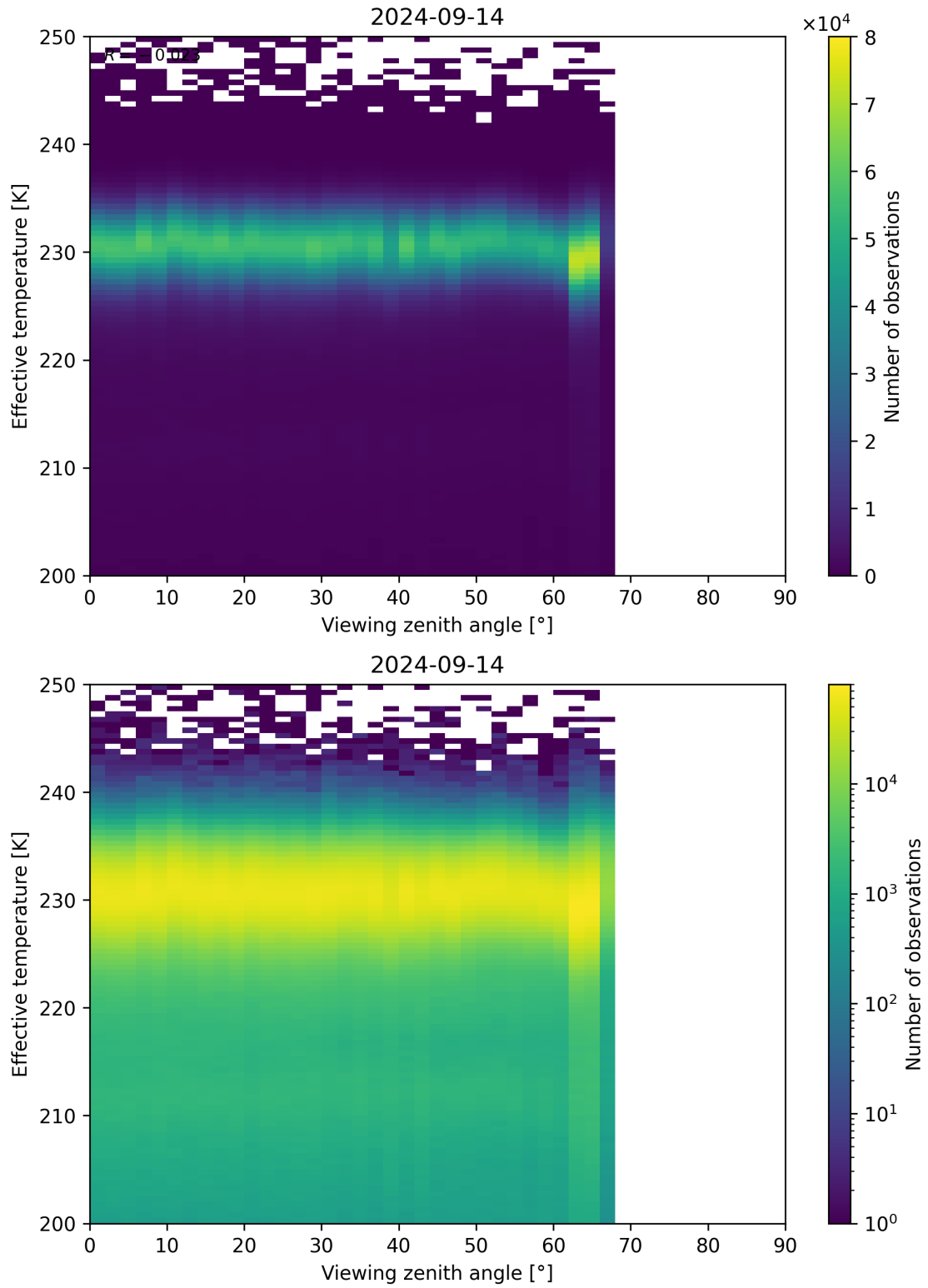
Figure 50: Scatter density plot of “Viewing zenith angle” against “Effective temperature” for 2024-09-13 to 2024-09-15.
