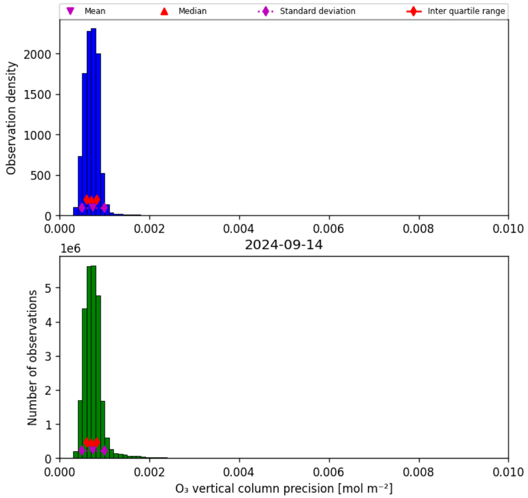
Figure 22: Histogram of “O 3 vertical column precision” for 2024-09-13 to 2024-09-15
