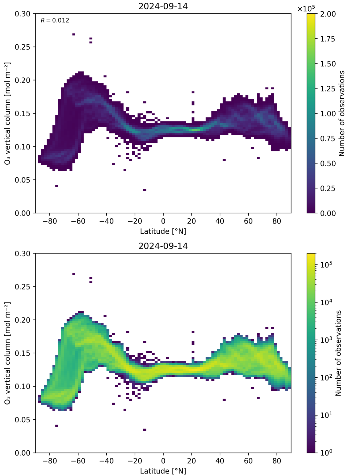
Figure 36: Scatter density plot of “Latitude” against “O 3 vertical column” for 2024-09-13 to 2024-09-15.
