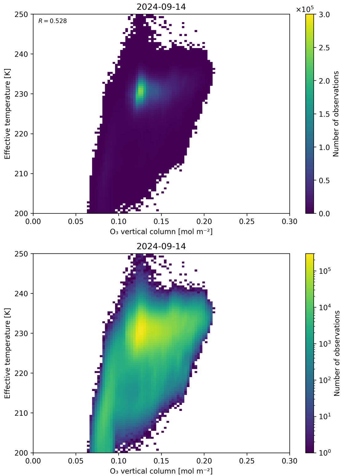
Figure 39: Scatter density plot of “O 3 vertical column” against “Effective temperature” for 2024-09-13 to 2024-09-15.
