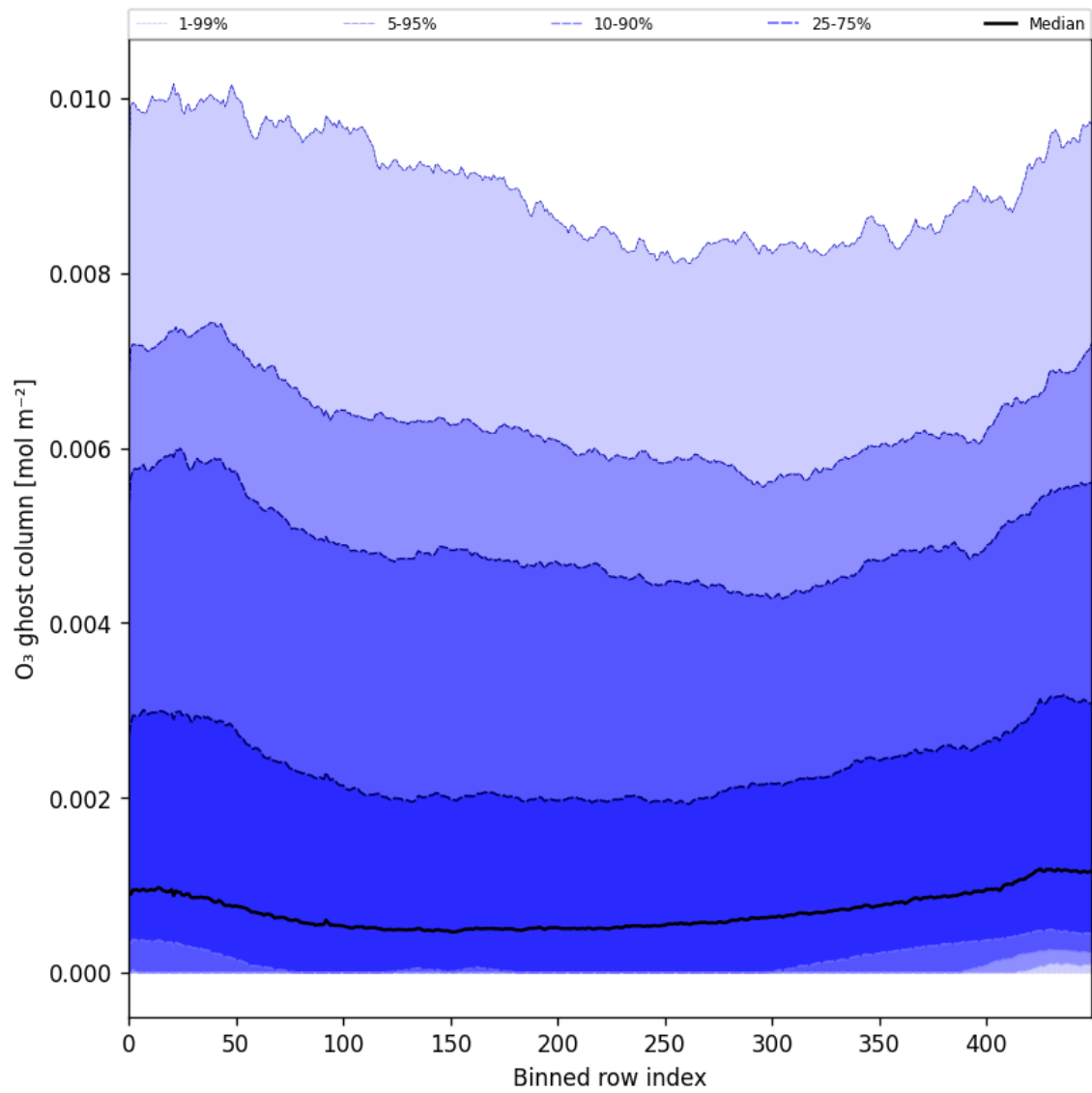
Figure 32: Along track statistics of “O 3 ghost column” for 2024-09-14 to 2024-09-16
