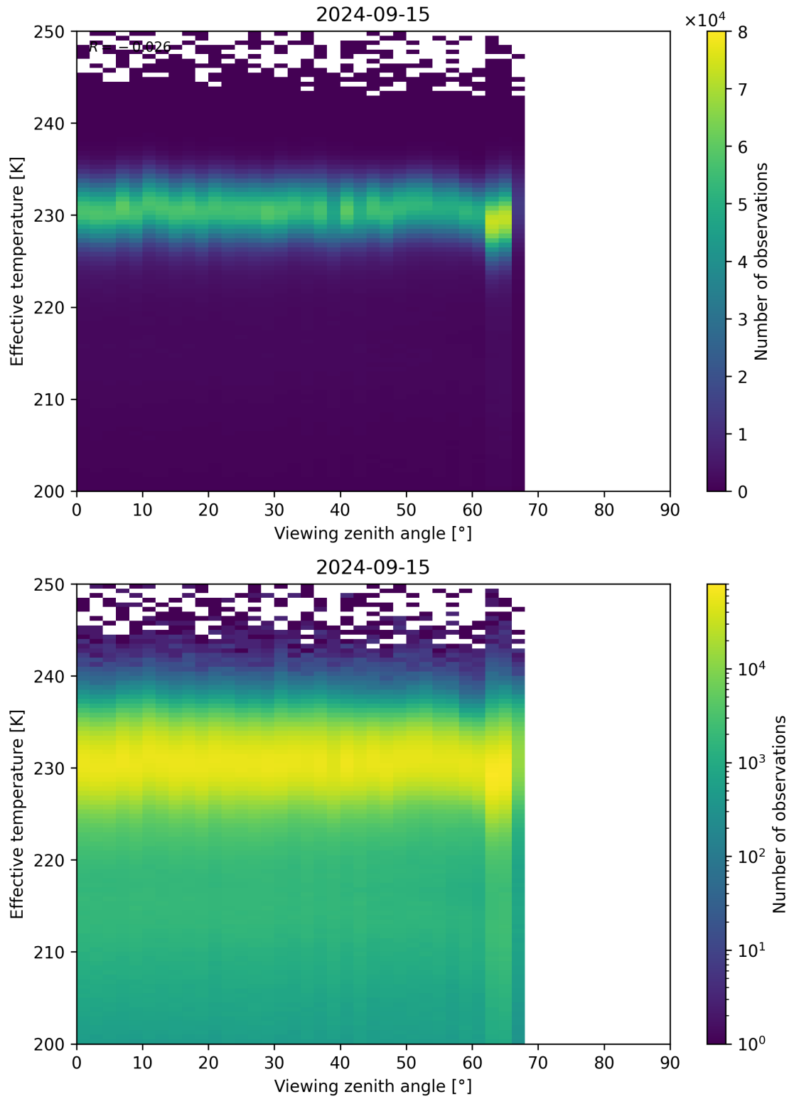
Figure 50: Scatter density plot of “Viewing zenith angle” against “Effective temperature” for 2024-09-14 to 2024-09-16.
