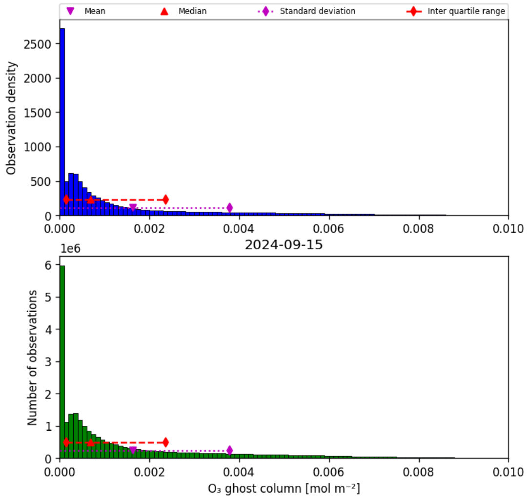
Figure 25: Histogram of “O 3 ghost column” for 2024-09-14 to 2024-09-16
