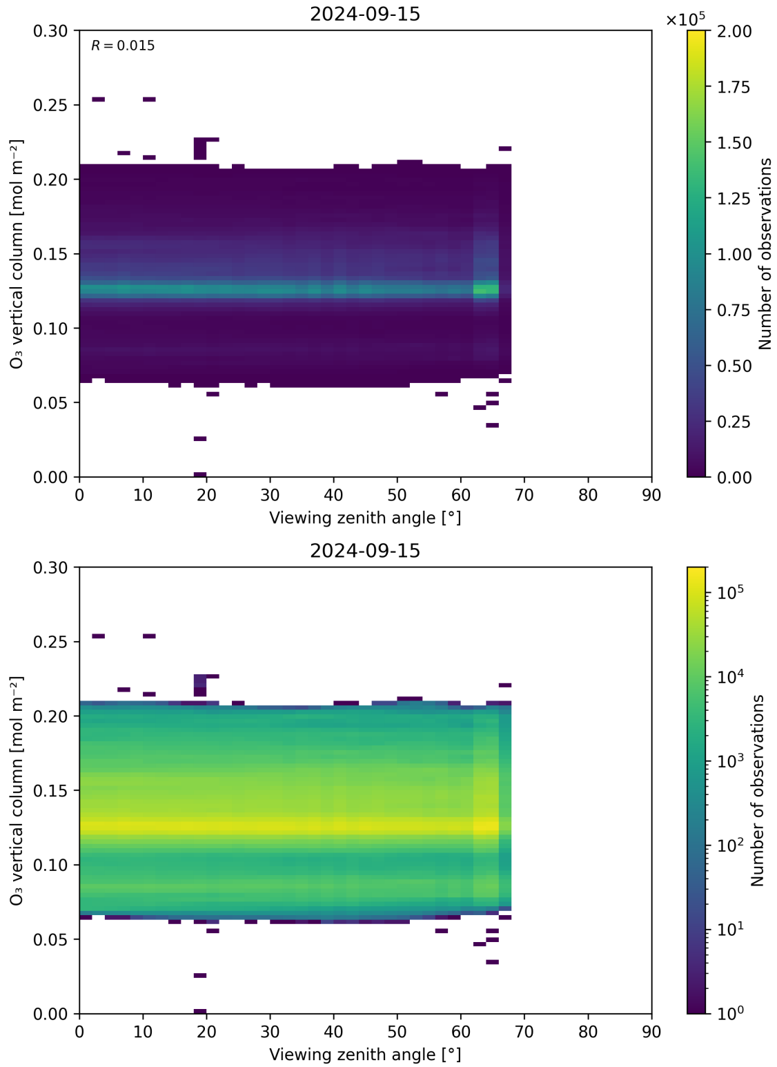
Figure 52: Scatter density plot of “Viewing zenith angle” against “O 3 vertical column” for 2024-09-14 to 2024-09-16.
