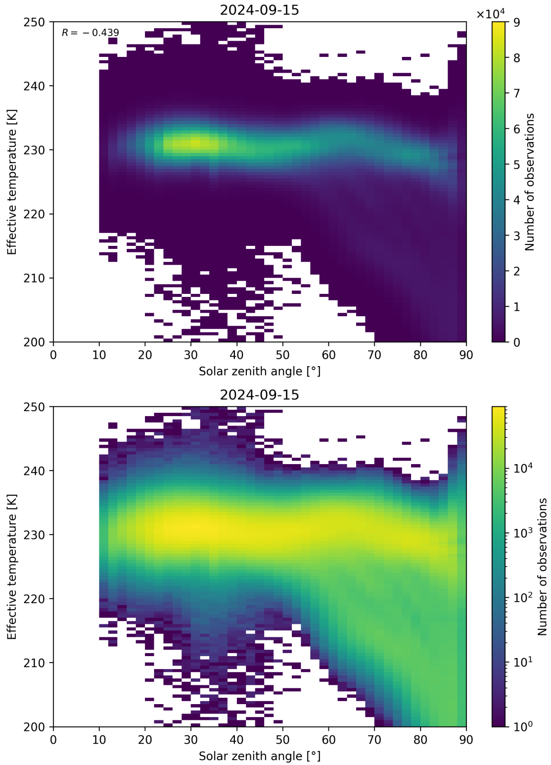
Figure 45: Scatter density plot of “Solar zenith angle” against “Effective temperature” for 2024-09-14 to 2024-09-16.
