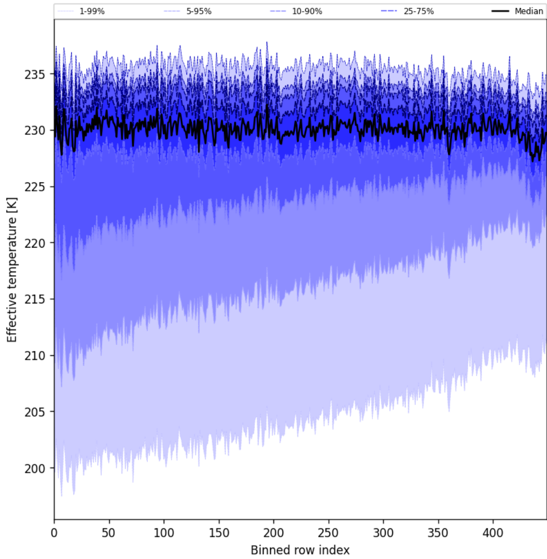
Figure 31: Along track statistics of “Effective temperature” for 2024-09-14 to 2024-09-16
