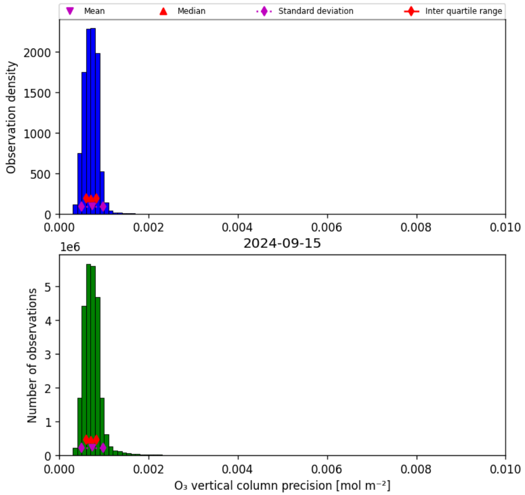
Figure 22: Histogram of “O 3 vertical column precision” for 2024-09-14 to 2024-09-16
