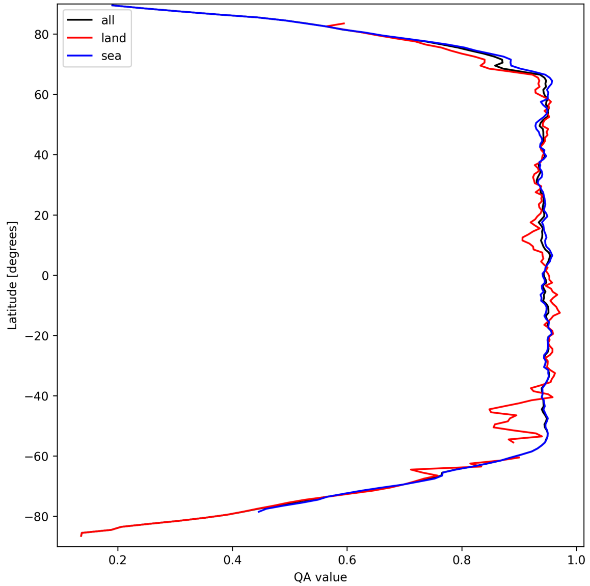
Figure 13: Zonal average of “QA value” for 2024-09-14 to 2024-09-16.
