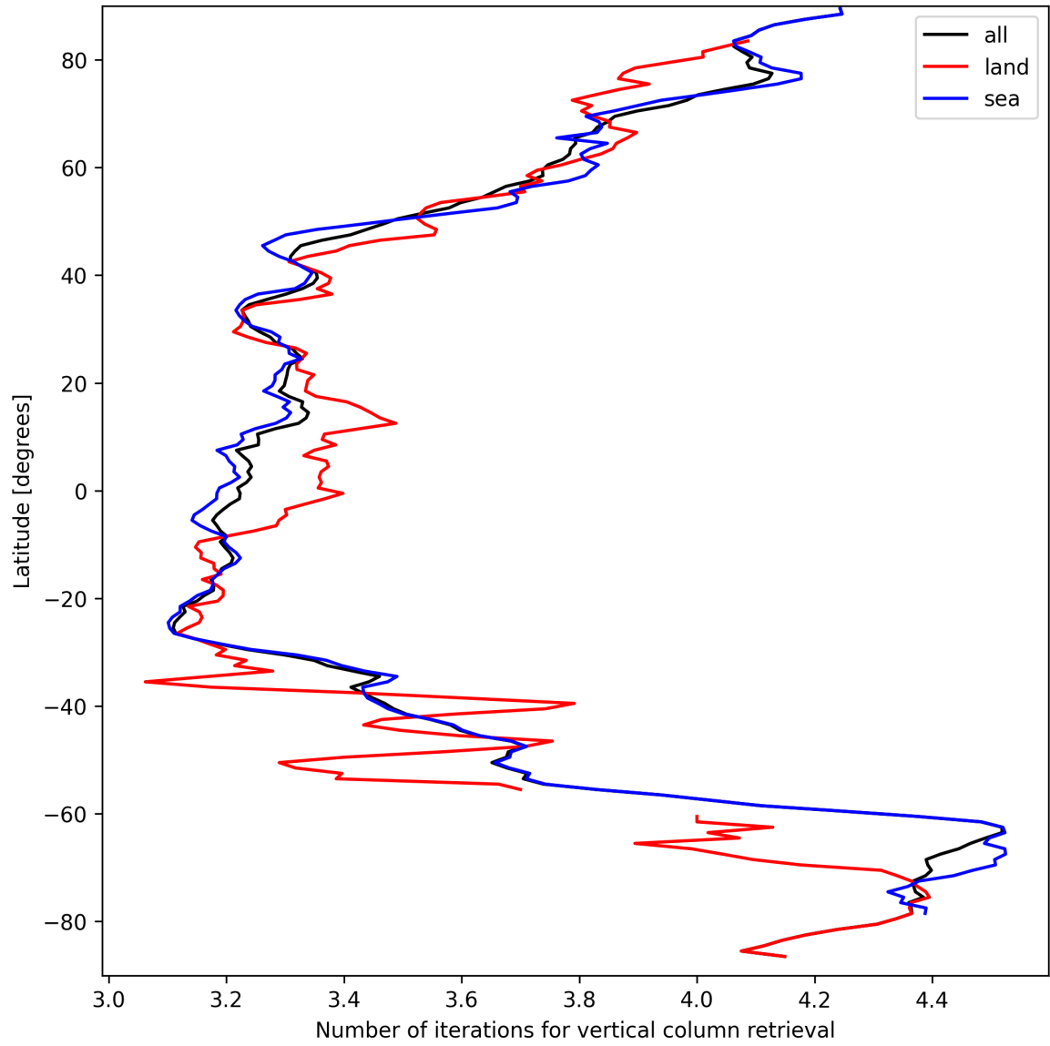
Figure 19: Zonal average of “Number of iterations for vertical column retrieval” for 2024-09-14 to 2024-09-16.
