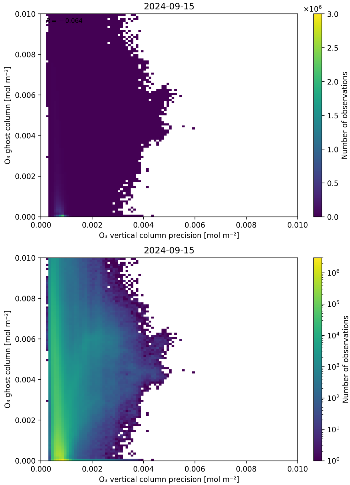
Figure 43: Scatter density plot of “ O_3 vertical column precision” against “ O_3 ghost column” for 2024-09-14 to 2024-09-16.
