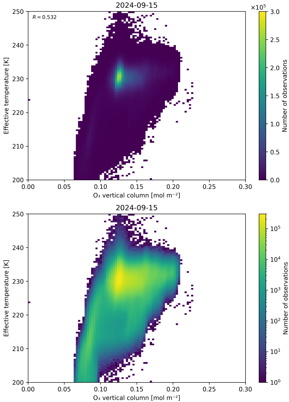
Figure 39: Scatter density plot of “O 3 vertical column” against “Effective temperature” for 2024-09-14 to 2024-09-16.
