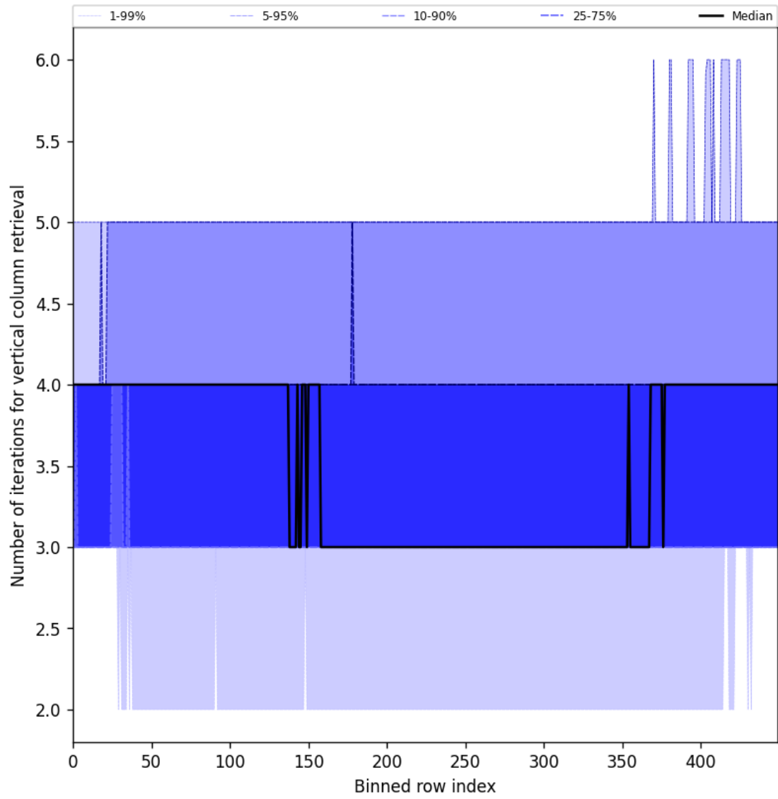
Figure 33: Along track statistics of “Number of iterations for vertical column retrieval” for 2024-09-14 to 2024-09-16
