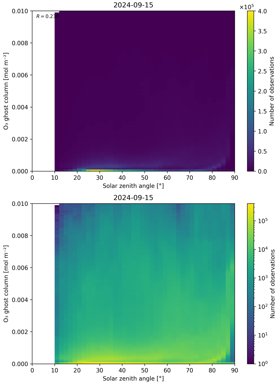
Figure 46: Scatter density plot of “Solar zenith angle” against “O 3 ghost column” for 2024-09-14 to 2024-09-16.
