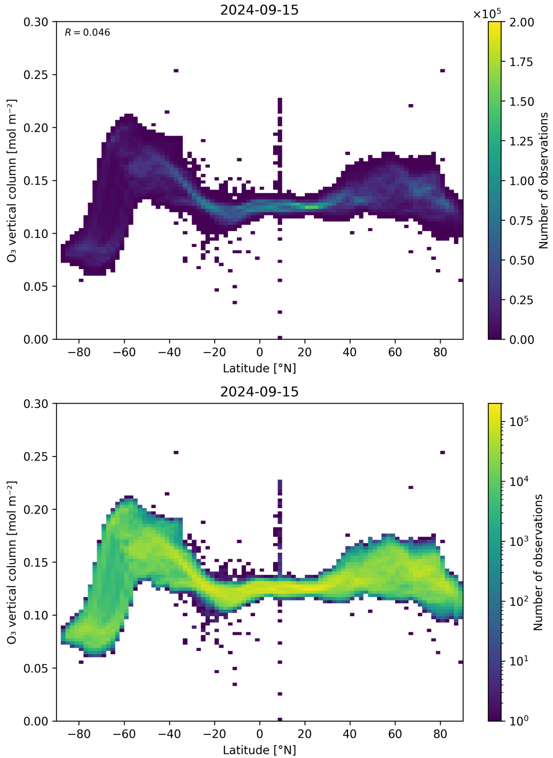
Figure 36: Scatter density plot of “Latitude” against “O 3 vertical column” for 2024-09-14 to 2024-09-16.
