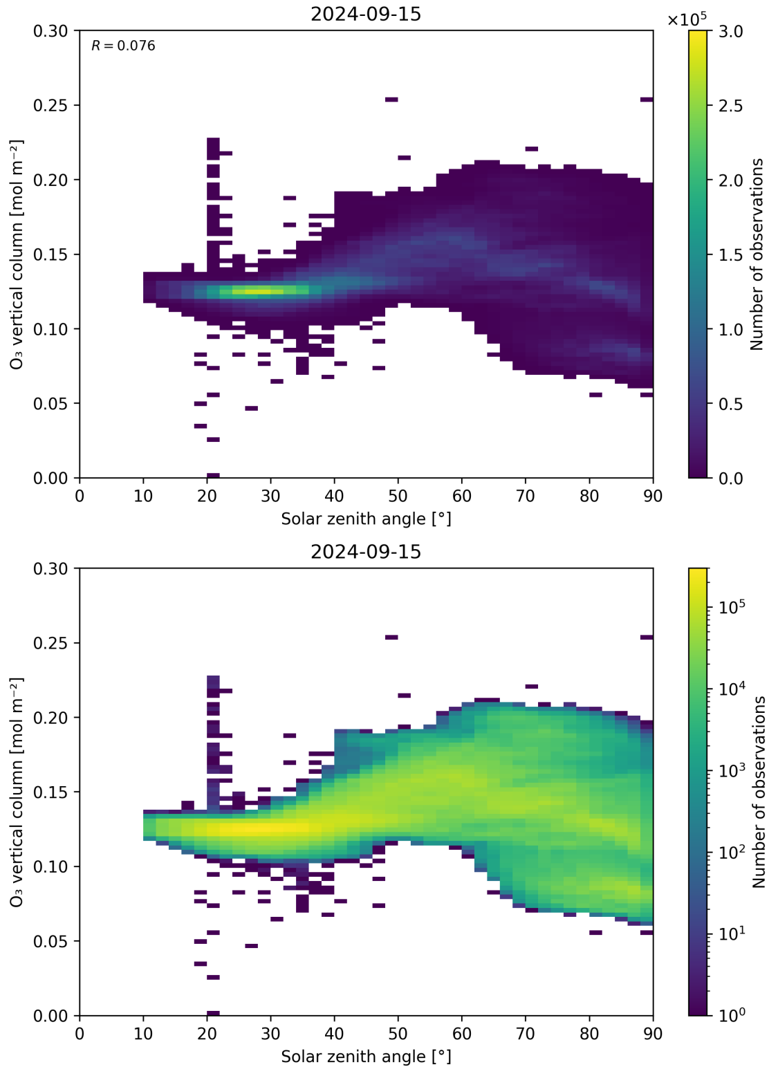
Figure 47: Scatter density plot of “Solar zenith angle” against “O 3 vertical column” for 2024-09-14 to 2024-09-16.
