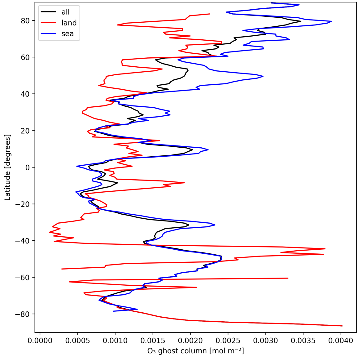
Figure 18: Zonal average of “O 3 ghost column” for 2024-09-14 to 2024-09-16.
