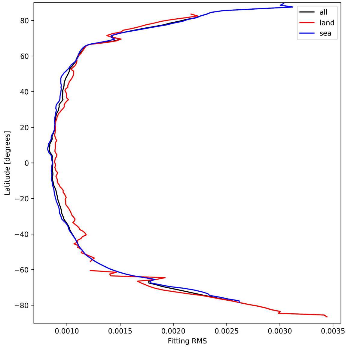
Figure 16: Zonal average of “Fitting RMS” for 2024-09-14 to 2024-09-16.
