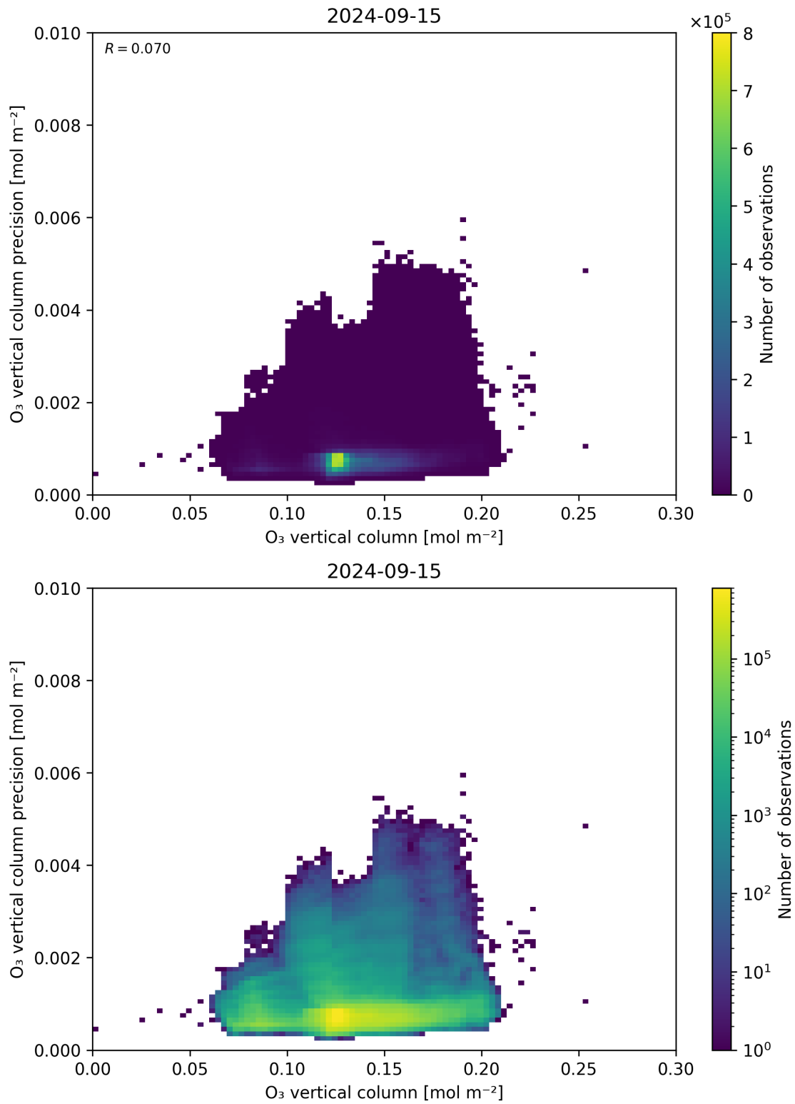
Figure 41: Scatter density plot of “O 3 vertical column” against “O 3 vertical column precision” for 2024-09-14 to 2024-09-16.
