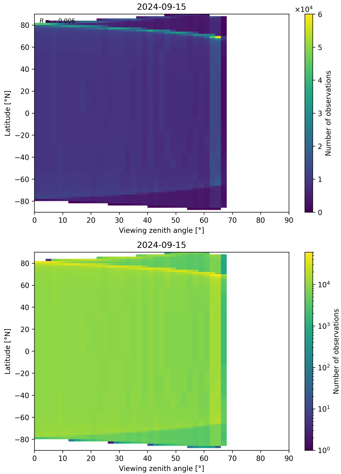
Figure 49: Scatter density plot of “Viewing zenith angle” against “Latitude” for 2024-09-14 to 2024-09-16.
