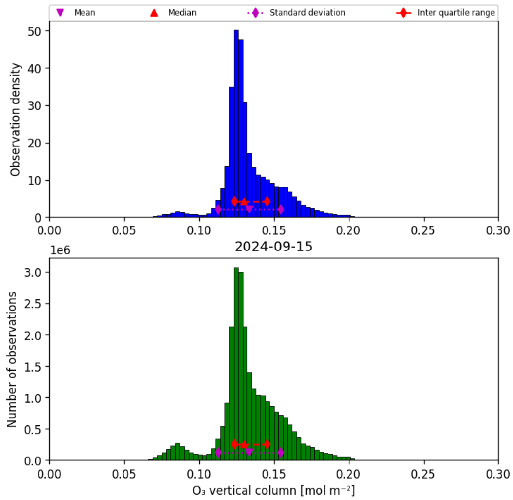
Figure 21: Histogram of “O 3 vertical column” for 2024-09-14 to 2024-09-16
