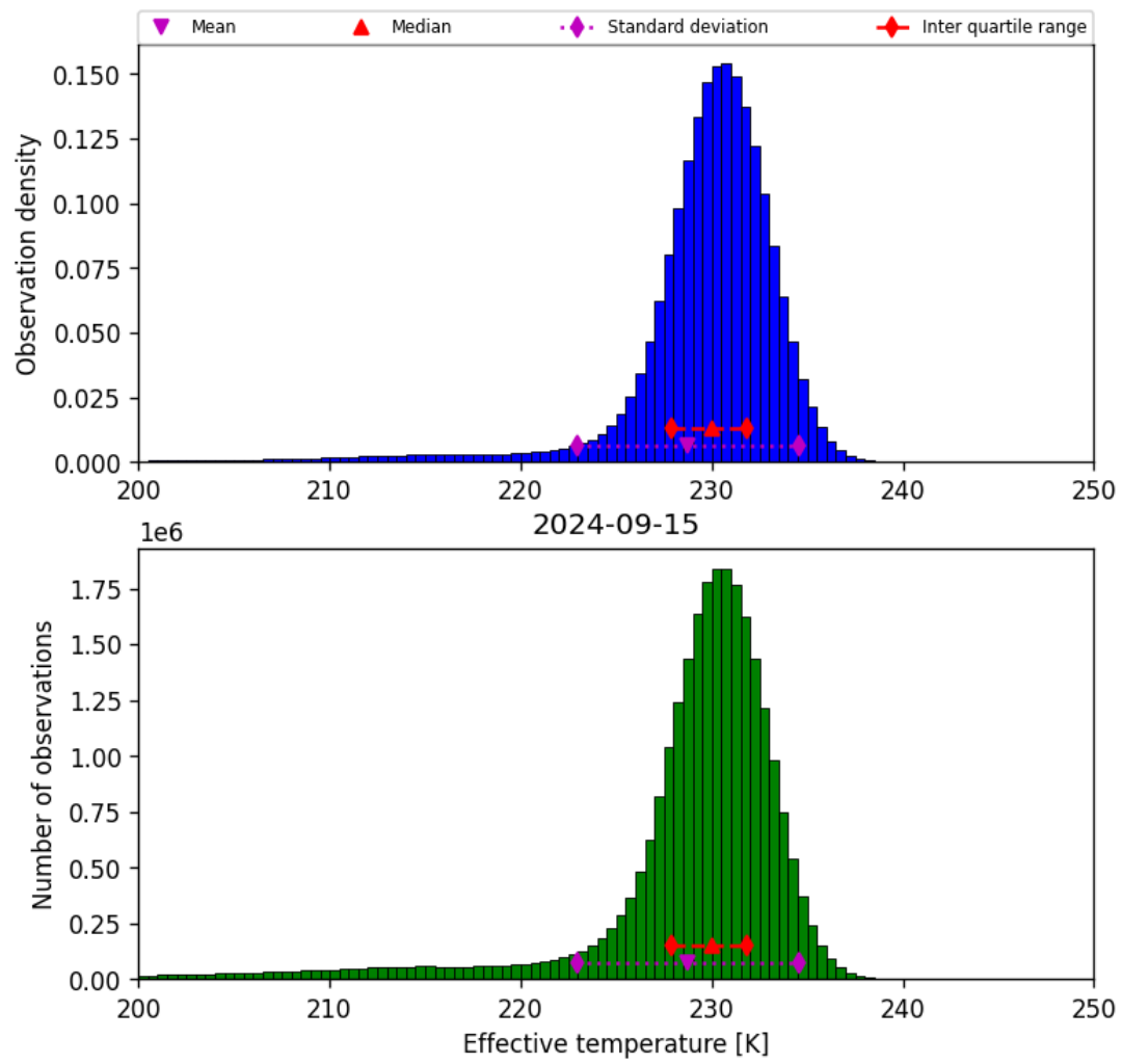
Figure 24: Histogram of “Effective temperature” for 2024-09-14 to 2024-09-16
