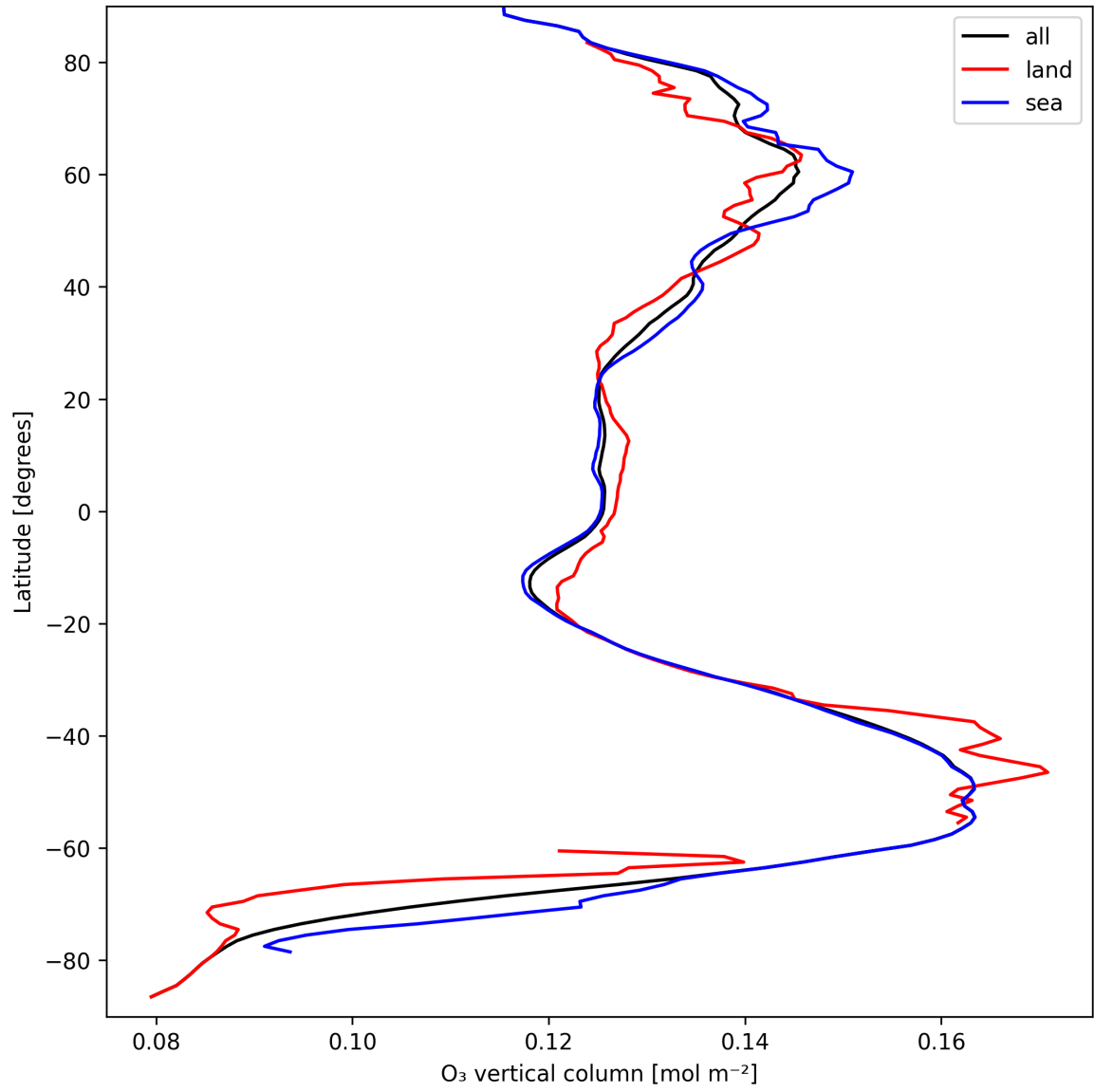
Figure 14: Zonal average of “O 3 vertical column” for 2024-09-14 to 2024-09-16.
