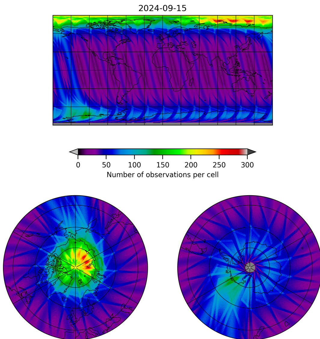
Figure 12: Map of the number of observations for 2024-09-14 to 2024-09-16
