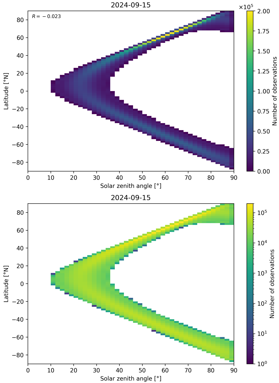
Figure 44: Scatter density plot of “Solar zenith angle” against “Latitude” for 2024-09-14 to 2024-09-16.
