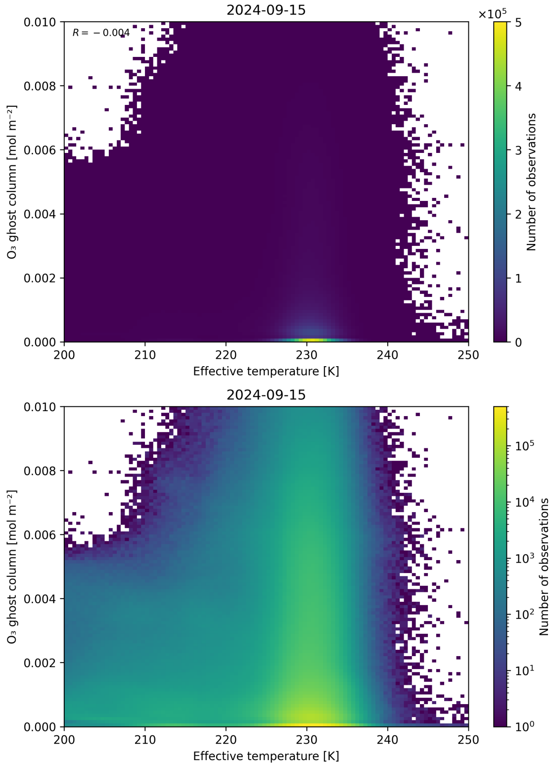
Figure 38: Scatter density plot of “Effective temperature” against “O 3 ghost column” for 2024-09-14 to 2024-09-16.
