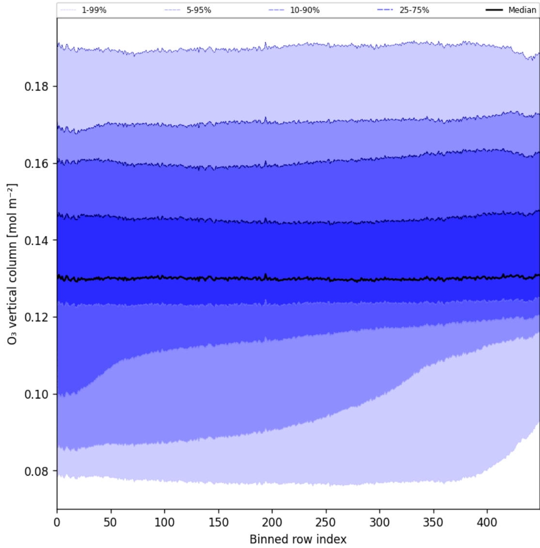
Figure 28: Along track statistics of “O 3 vertical column” for 2024-09-14 to 2024-09-16
