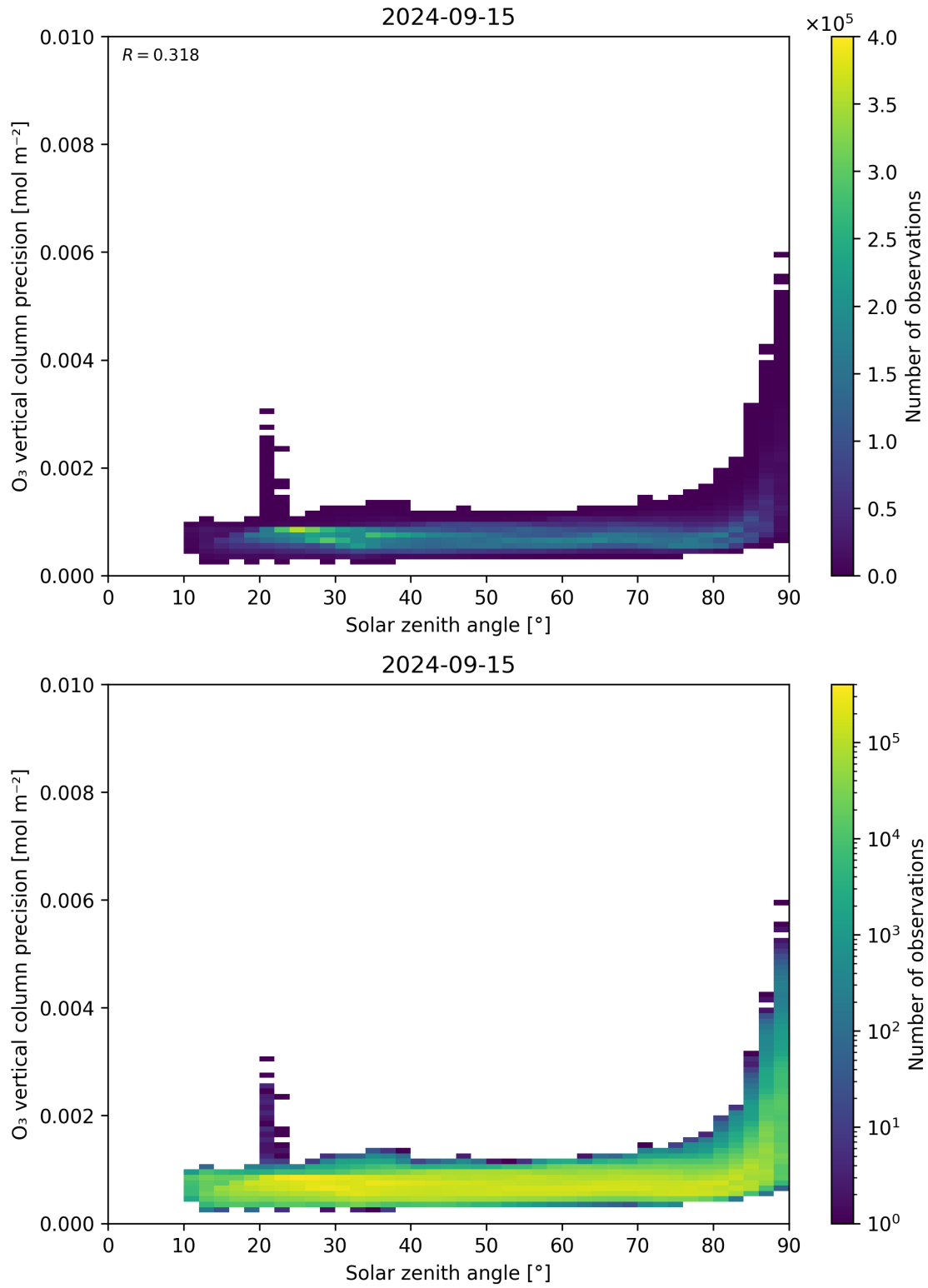
Figure 48: Scatter density plot of “Solar zenith angle” against “O 3 vertical column precision” for 2024-09-14 to 2024-09-16.
