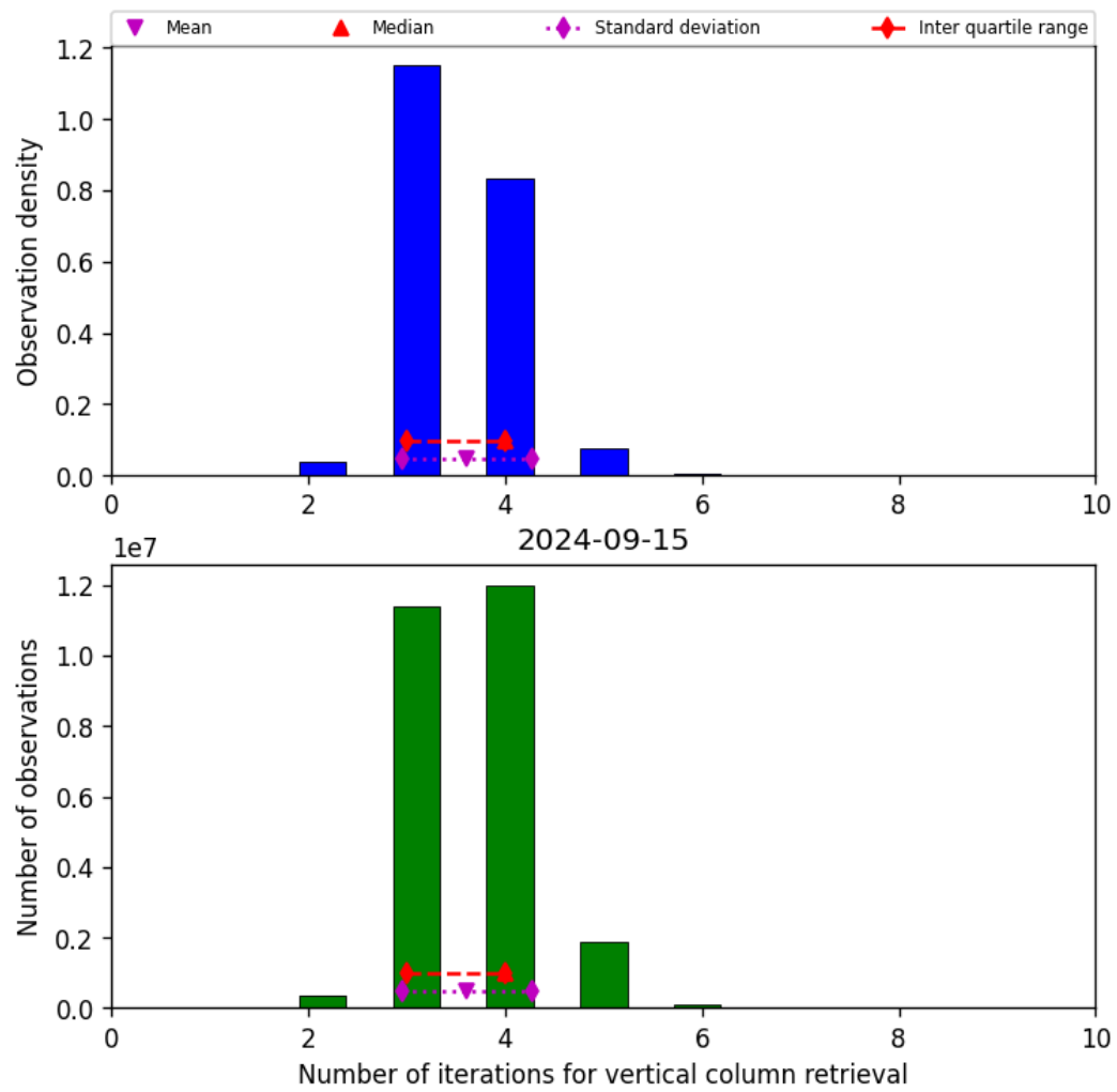
Figure 26: Histogram of “Number of iterations for vertical column retrieval” for 2024-09-14 to 2024-09-16
