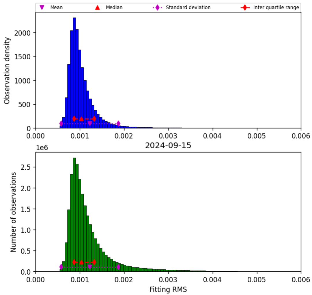
Figure 23: Histogram of “Fitting RMS” for 2024-09-14 to 2024-09-16
