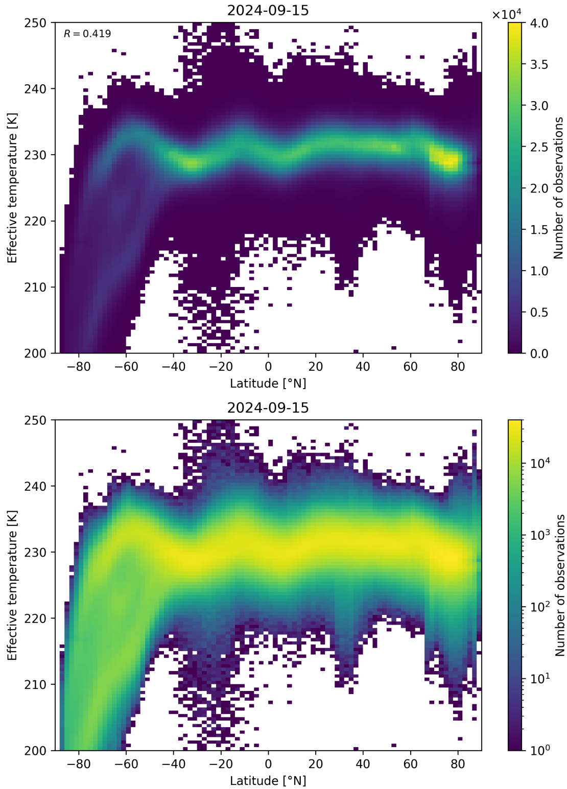
Figure 34: Scatter density plot of “Latitude” against “Effective temperature” for 2024-09-14 to 2024-09-16.
