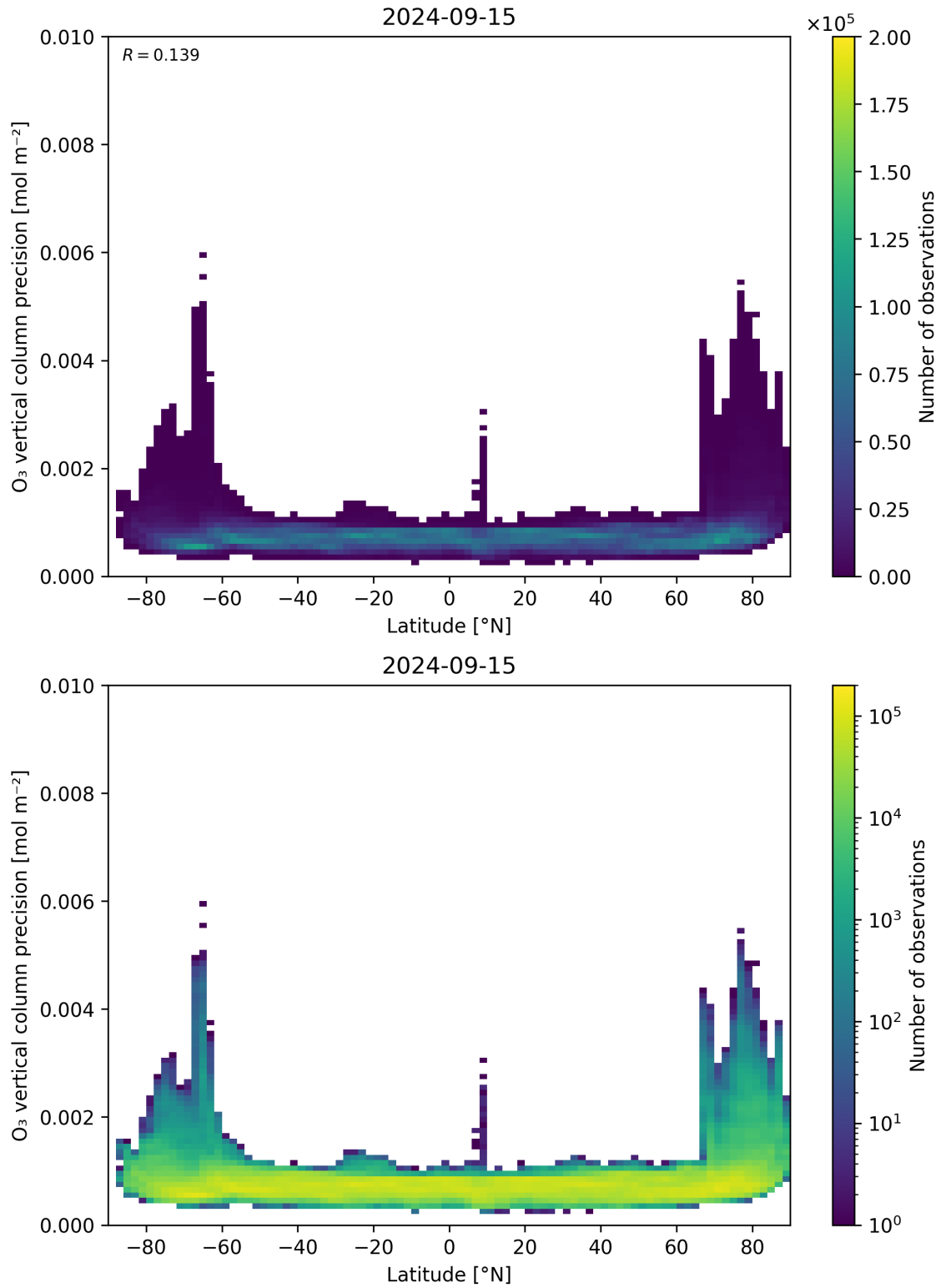
Figure 37: Scatter density plot of “Latitude” against “O 3 vertical column precision” for 2024-09-14 to 2024-09-16.
