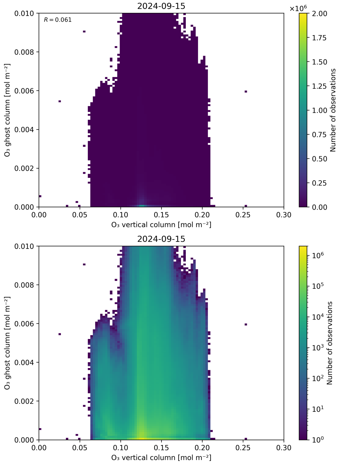
Figure 40: Scatter density plot of “ \text{O}_3 vertical column” against “ \text{O}_3 ghost column” for 2024-09-14 to 2024-09-16.
