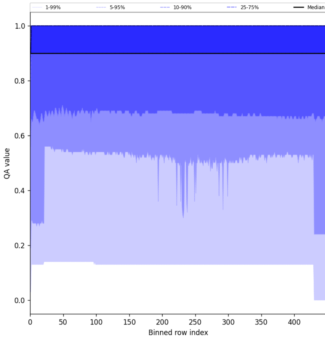
Figure 27: Along track statistics of “QA value” for 2024-09-14 to 2024-09-16
