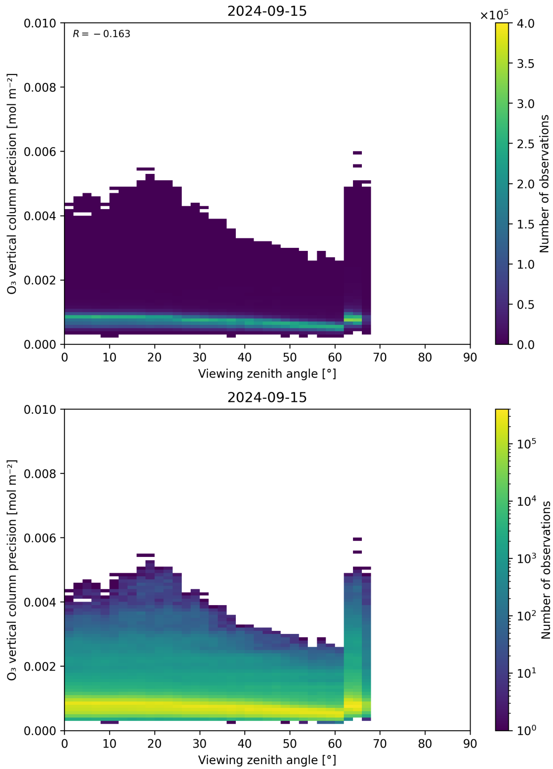
Figure 53: Scatter density plot of “Viewing zenith angle” against “O 3 vertical column precision” for 2024-09-14 to 2024-09-16.
