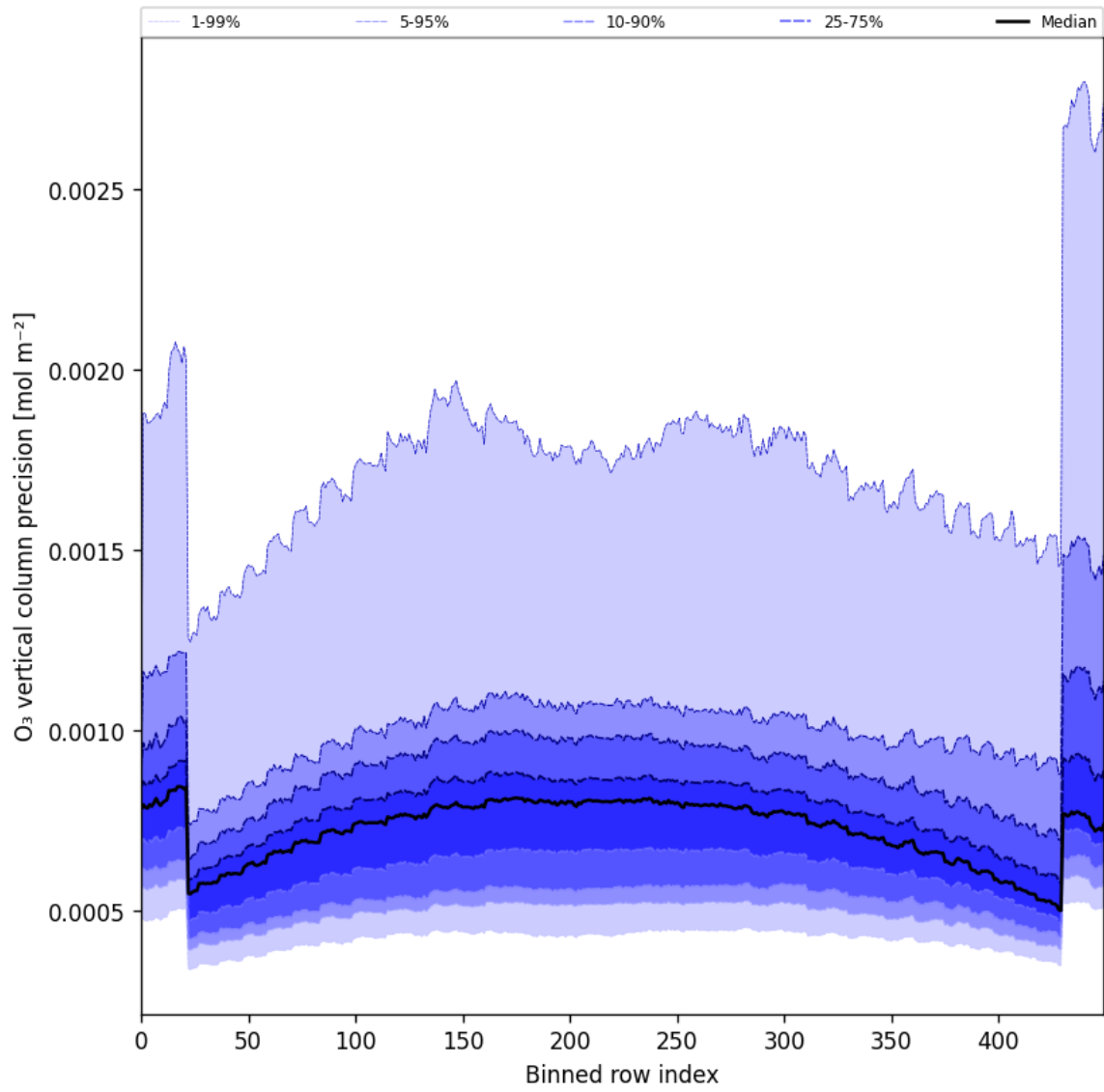
Figure 29: Along track statistics of “O 3 vertical column precision” for 2024-09-14 to 2024-09-16
