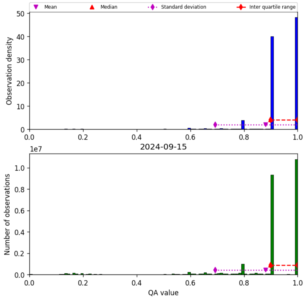
Figure 20: Histogram of “QA value” for 2024-09-14 to 2024-09-16
