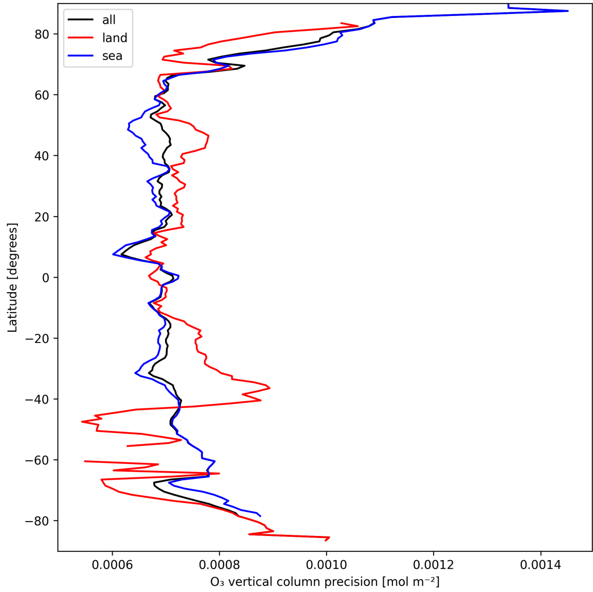
Figure 15: Zonal average of “O 3 vertical column precision” for 2024-09-14 to 2024-09-16.
