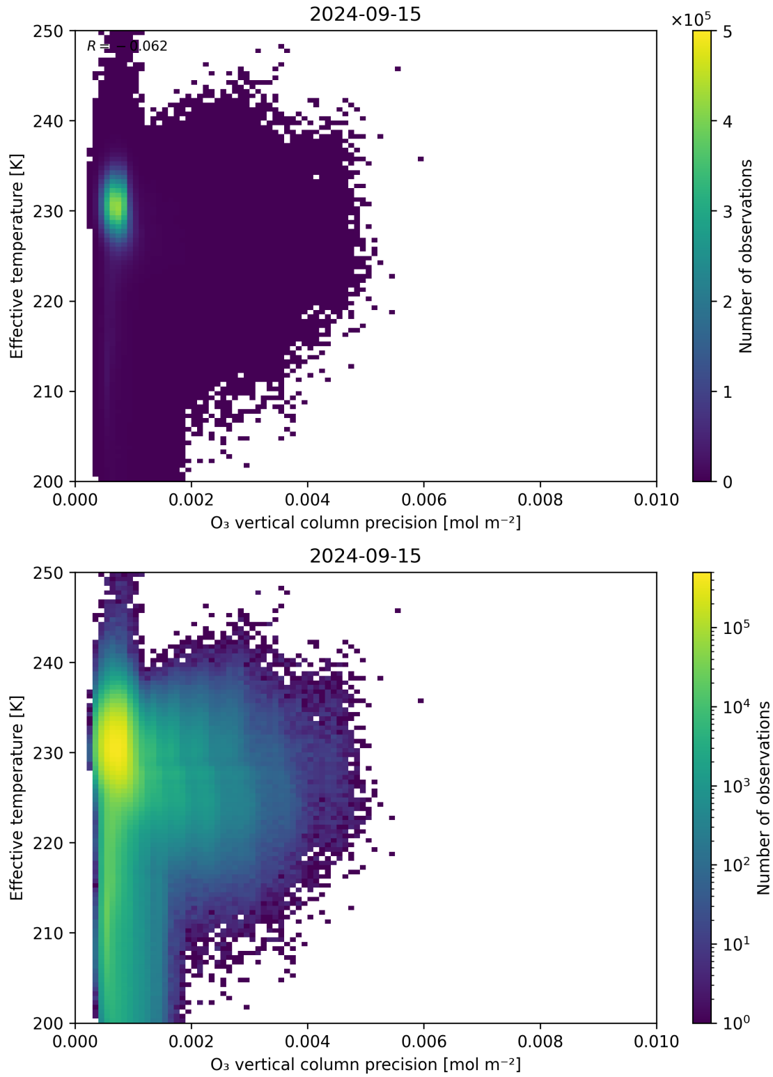
Figure 42: Scatter density plot of “ O_3 vertical column precision” against “Effective temperature” for 2024-09-14 to 2024-09-16.
