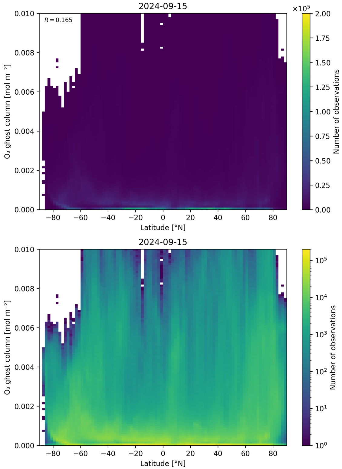
Figure 35: Scatter density plot of “Latitude” against “O 3 ghost column” for 2024-09-14 to 2024-09-16.
