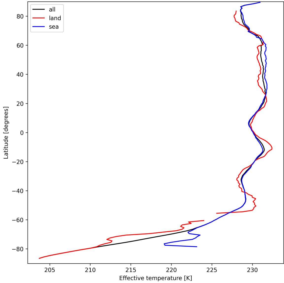
Figure 17: Zonal average of "Effective temperature" for 2024-09-14 to 2024-09-16.
