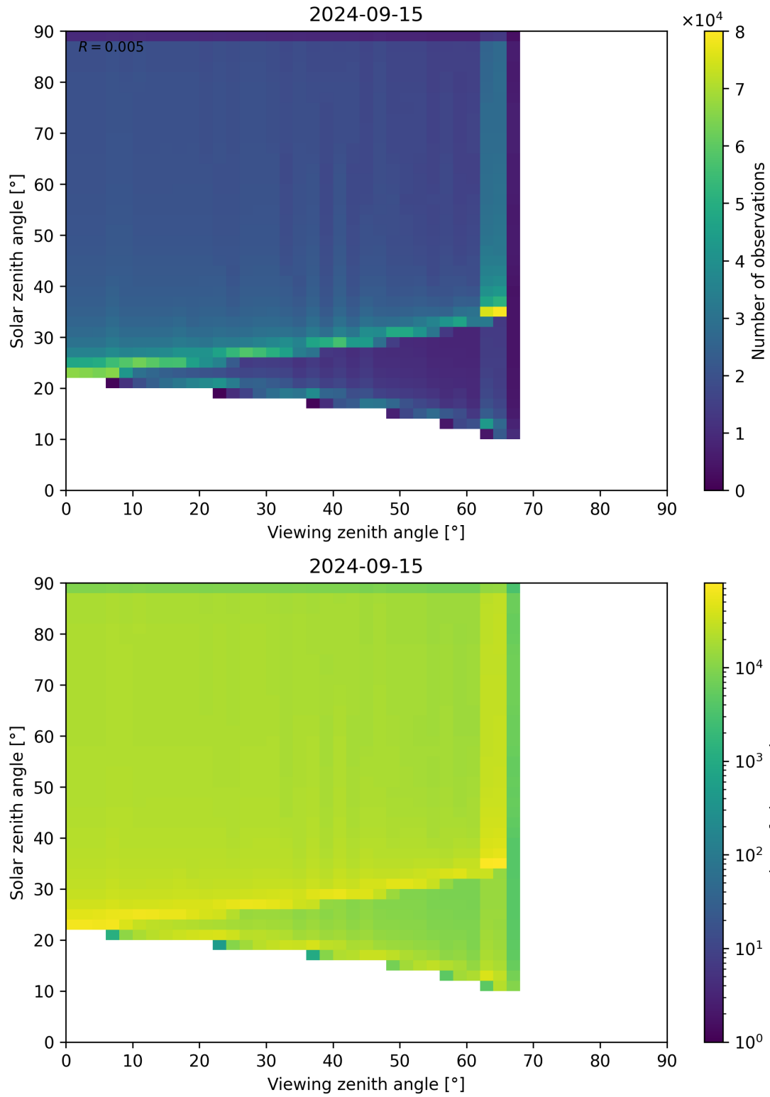
Figure 54: Scatter density plot of “Viewing zenith angle” against “Solar zenith angle” for 2024-09-14 to 2024-09-16.
