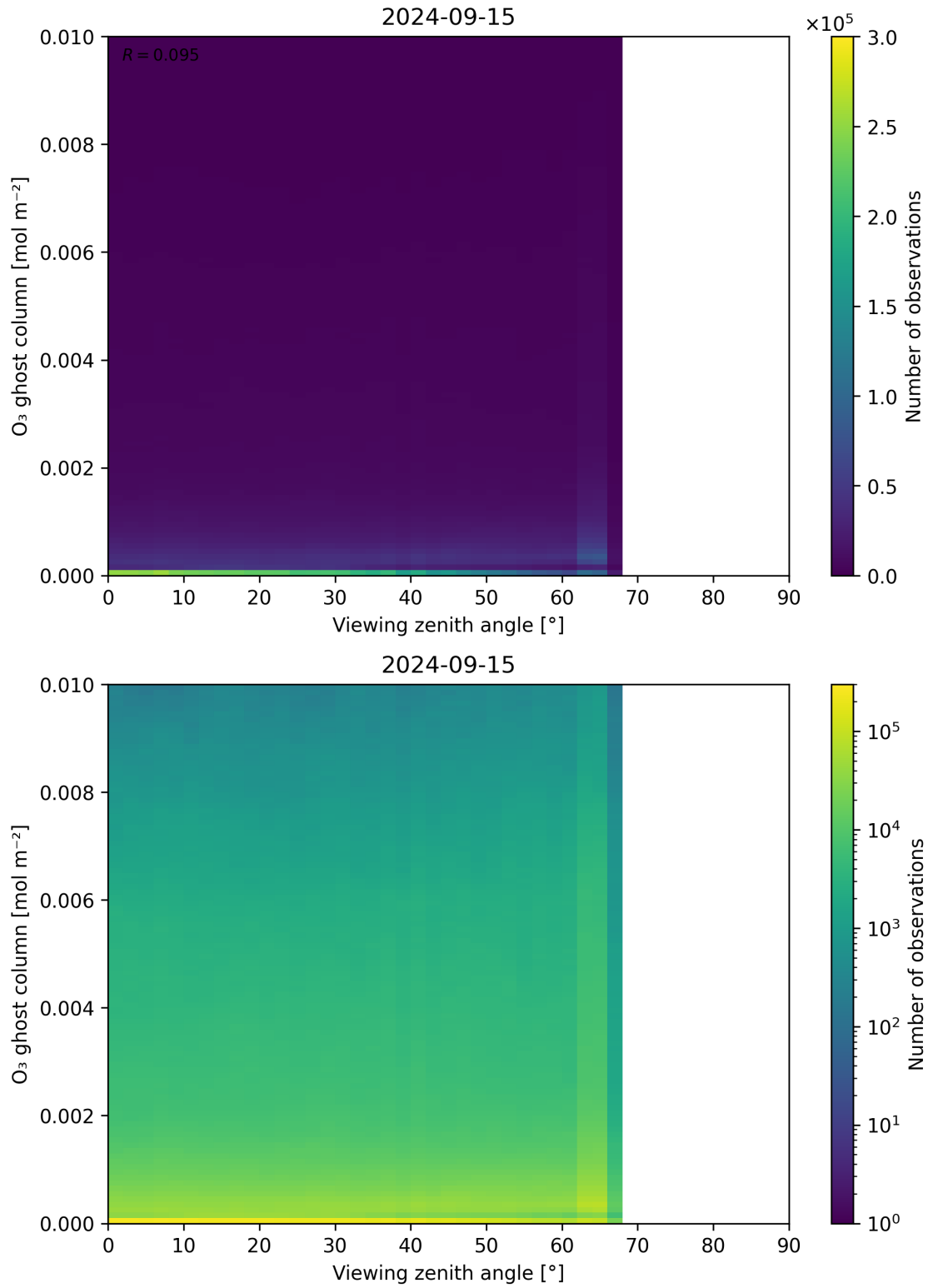
Figure 51: Scatter density plot of “Viewing zenith angle” against “O 3 ghost column” for 2024-09-14 to 2024-09-16.
