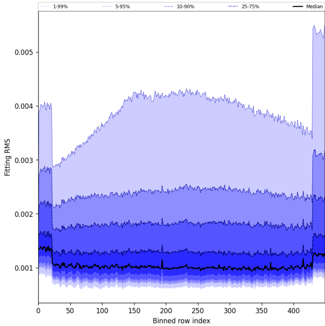
Figure 30: Along track statistics of “Fitting RMS” for 2024-09-14 to 2024-09-16
