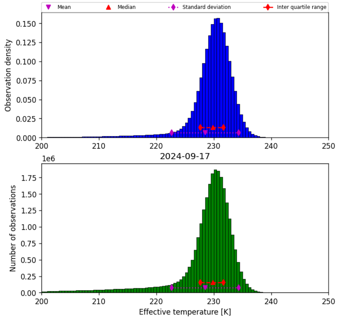
Figure 24: Histogram of “Effective temperature” for 2024-09-17 to 2024-09-18
