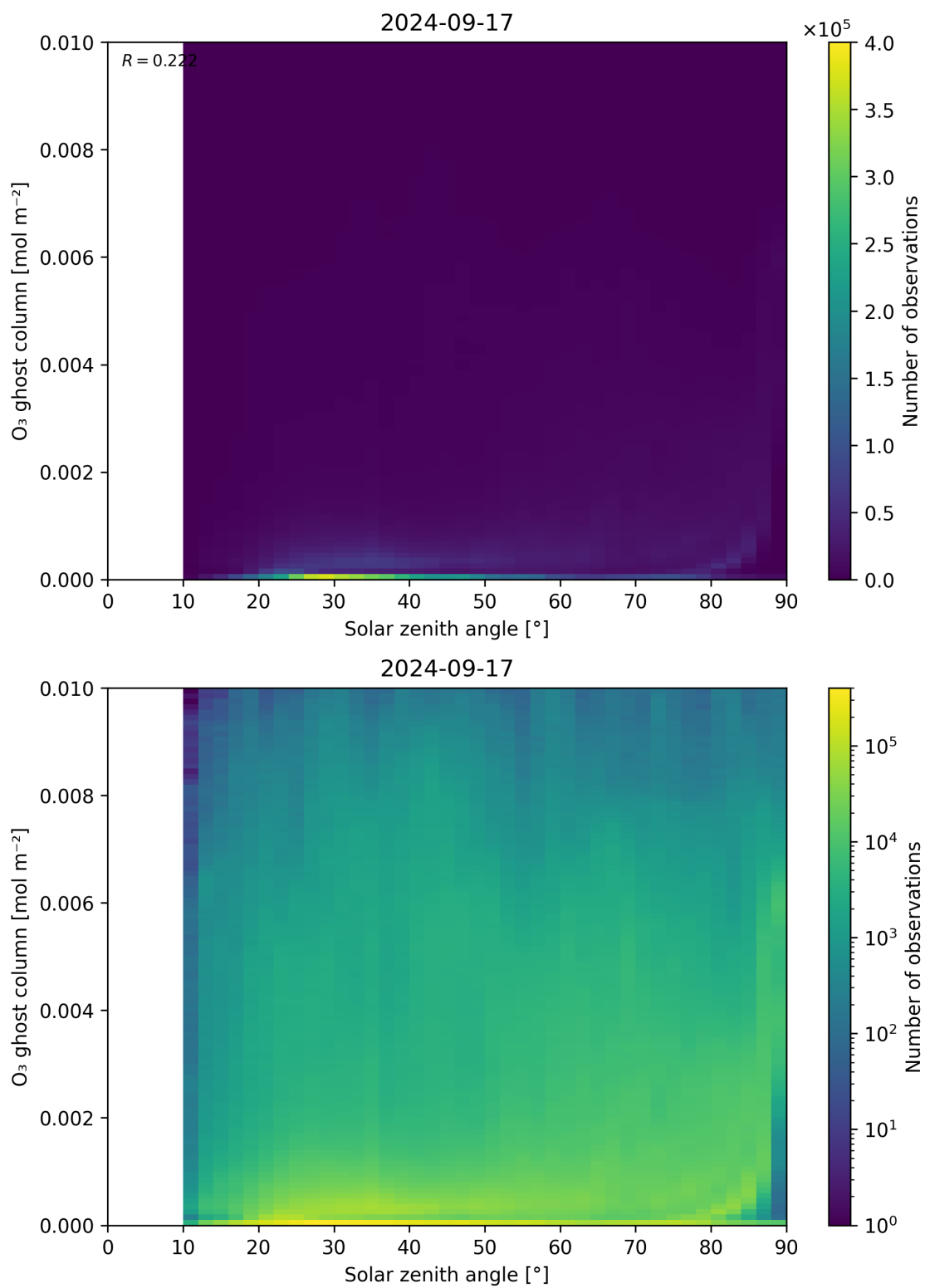
Figure 46: Scatter density plot of “Solar zenith angle” against “O 3 ghost column” for 2024-09-17 to 2024-09-18.
