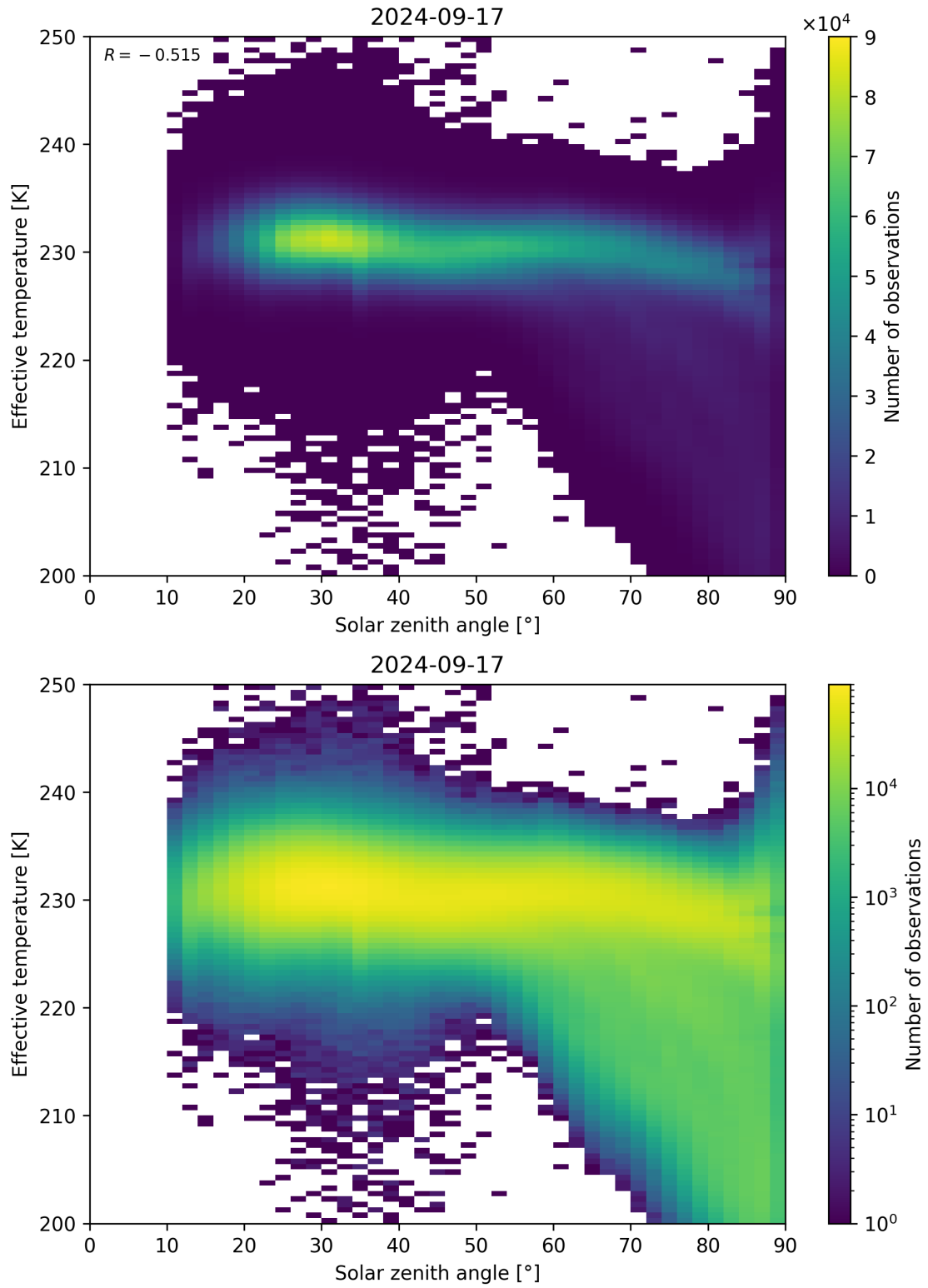
Figure 45: Scatter density plot of “Solar zenith angle” against “Effective temperature” for 2024-09-17 to 2024-09-18.
