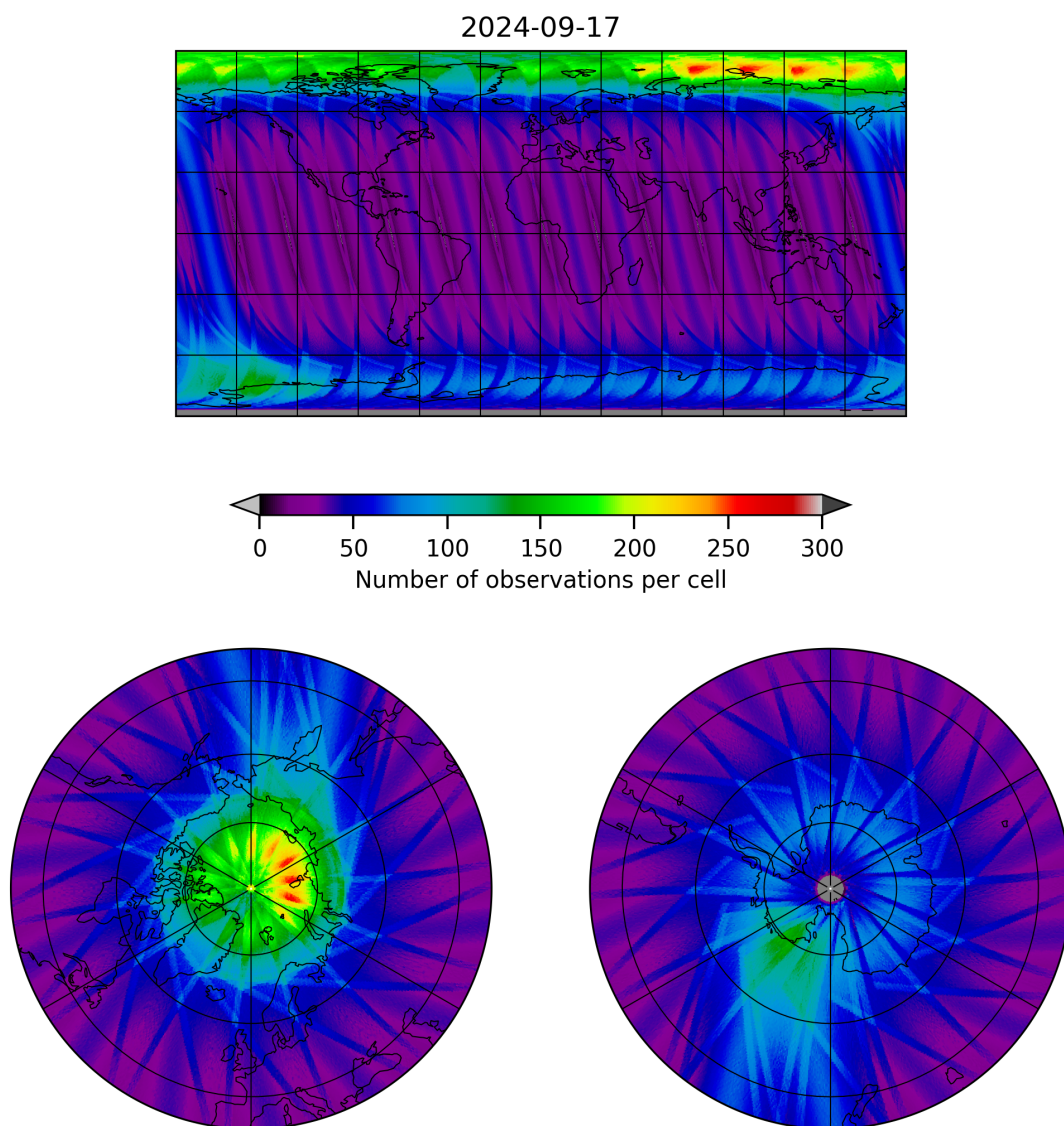
Figure 12: Map of the number of observations for 2024-09-17 to 2024-09-18
