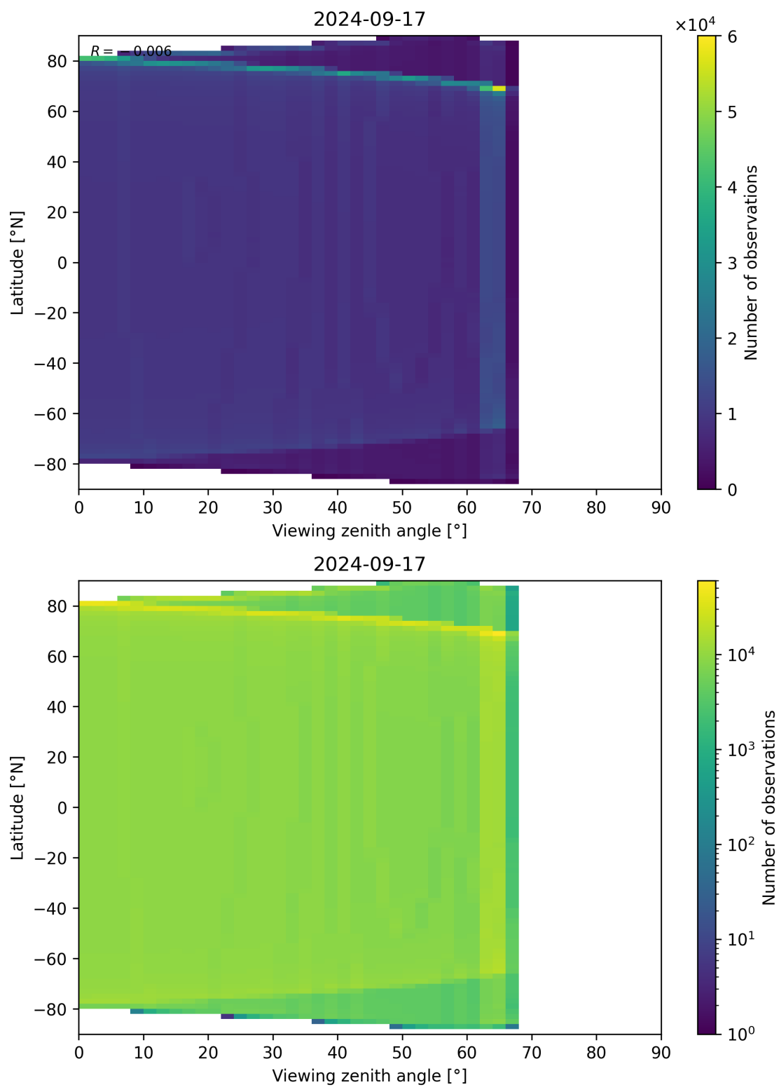
Figure 49: Scatter density plot of “Viewing zenith angle” against “Latitude” for 2024-09-17 to 2024-09-18.
