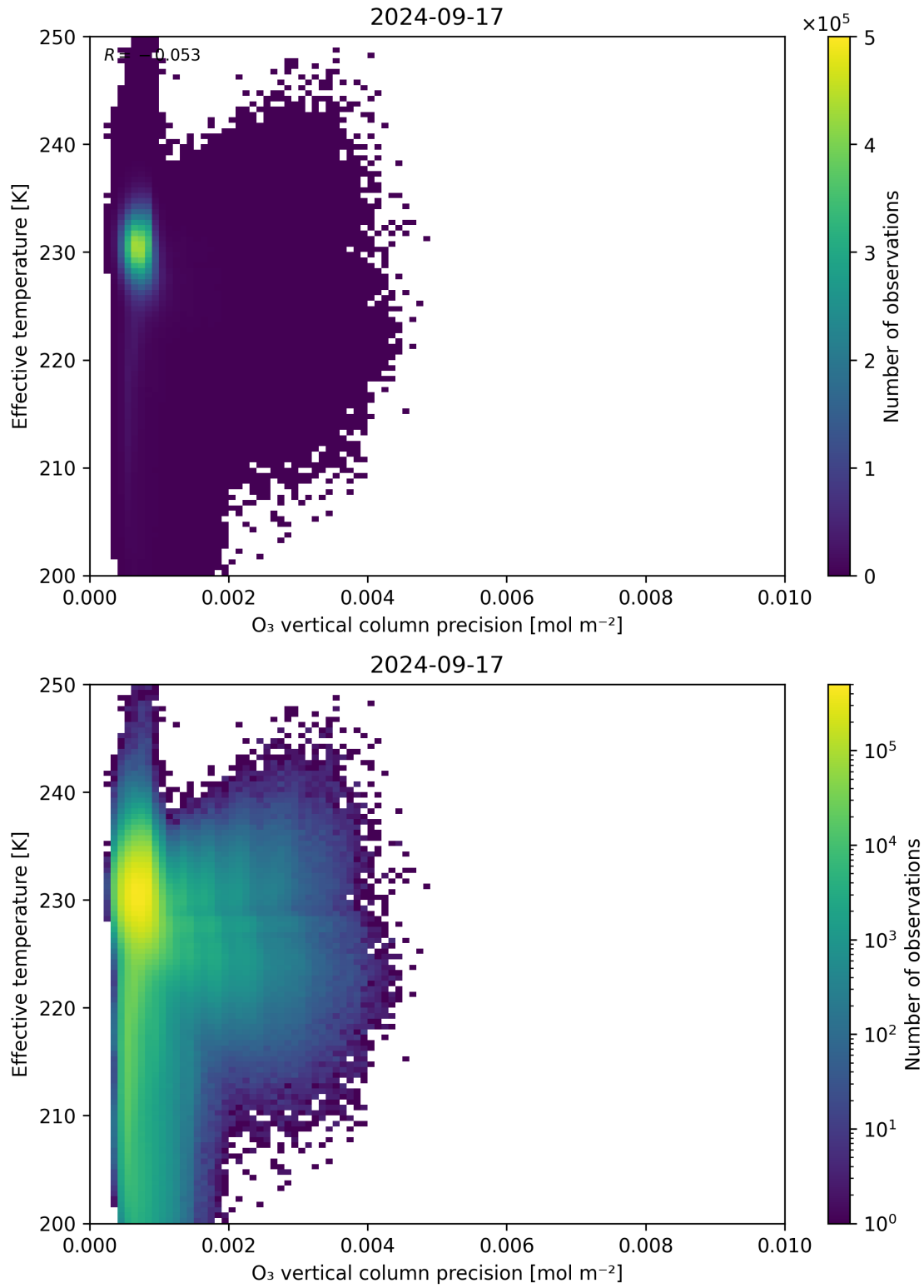
Figure 42: Scatter density plot of “ O_3 vertical column precision” against “Effective temperature” for 2024-09-17 to 2024-09-18.
