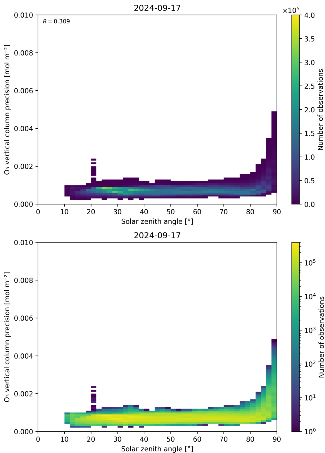
Figure 48: Scatter density plot of “Solar zenith angle” against “O 3 vertical column precision” for 2024-09-17 to 2024-09-18.
