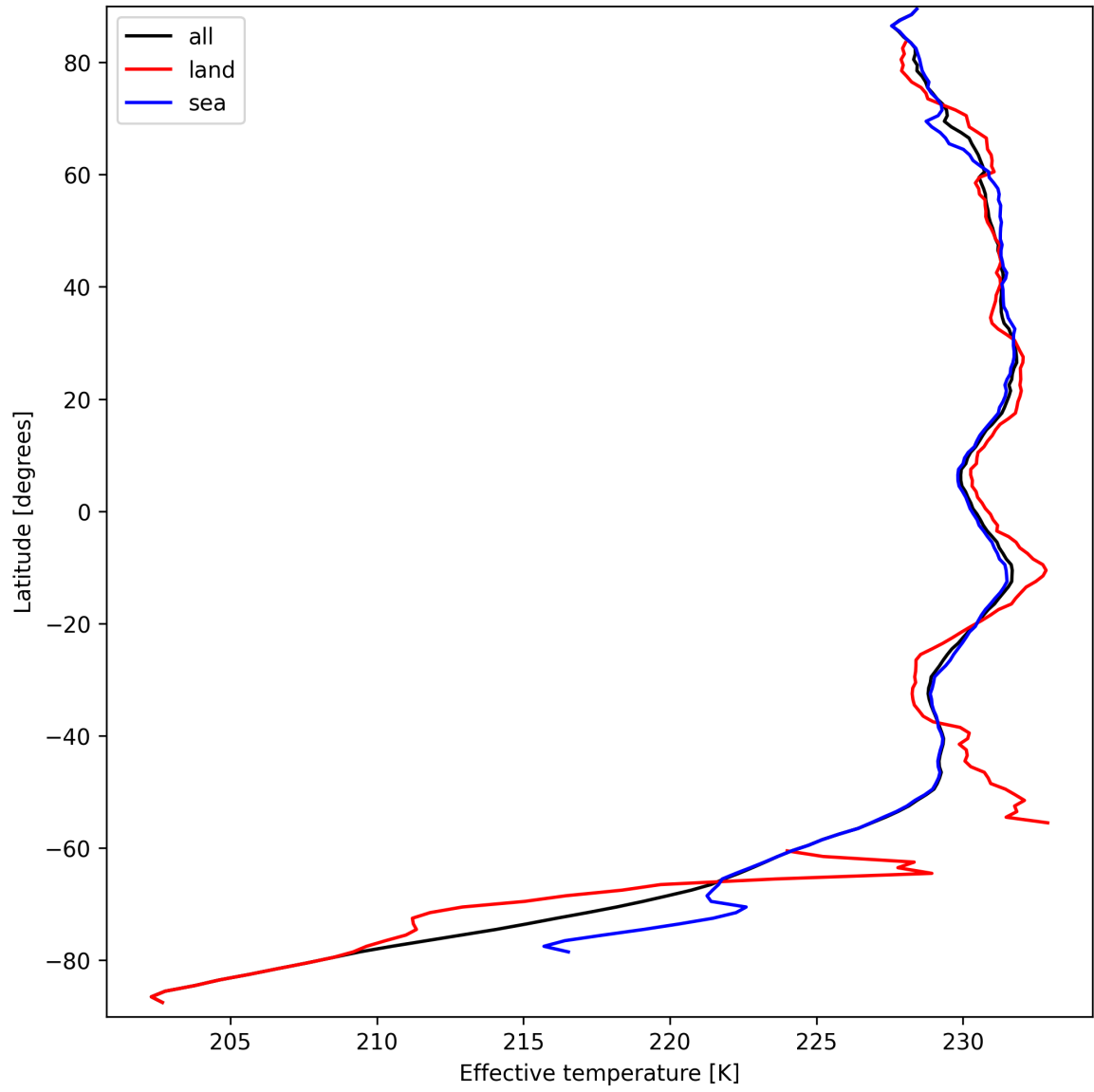
Figure 17: Zonal average of "Effective temperature" for 2024-09-17 to 2024-09-18.
