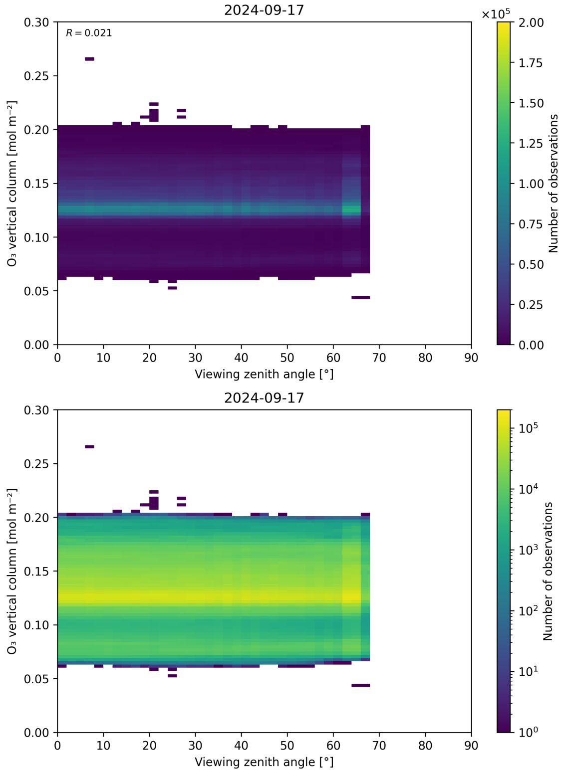
Figure 52: Scatter density plot of “Viewing zenith angle” against “O 3 vertical column” for 2024-09-17 to 2024-09-18.
