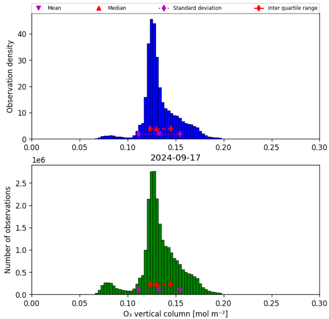
Figure 21: Histogram of “O 3 vertical column” for 2024-09-17 to 2024-09-18
