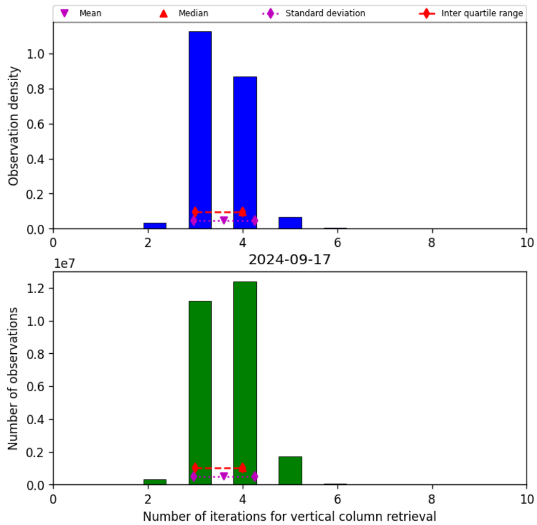
Figure 26: Histogram of “Number of iterations for vertical column retrieval” for 2024-09-17 to 2024-09-18
