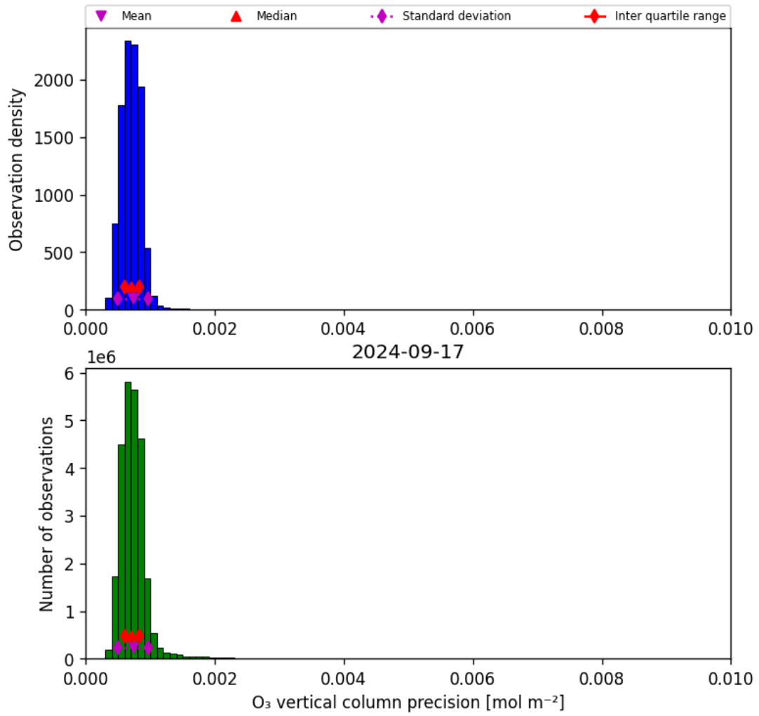
Figure 22: Histogram of “O 3 vertical column precision” for 2024-09-17 to 2024-09-18
