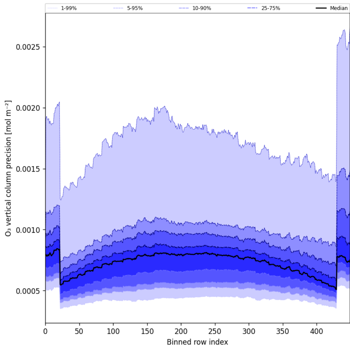
Figure 29: Along track statistics of “O 3 vertical column precision” for 2024-09-17 to 2024-09-18
