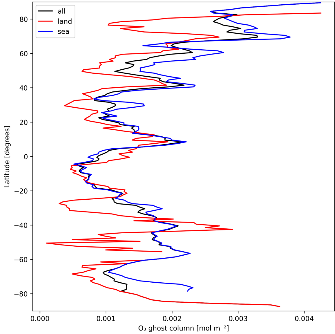
Figure 18: Zonal average of “O 3 ghost column” for 2024-09-17 to 2024-09-18.
