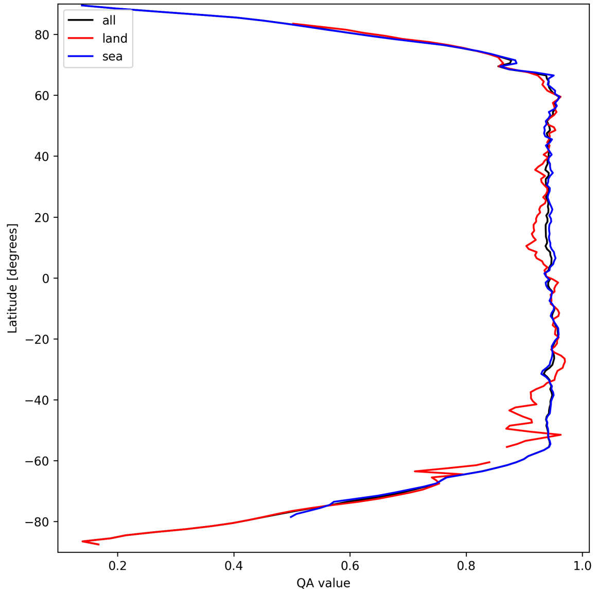
Figure 13: Zonal average of “QA value” for 2024-09-17 to 2024-09-18.
