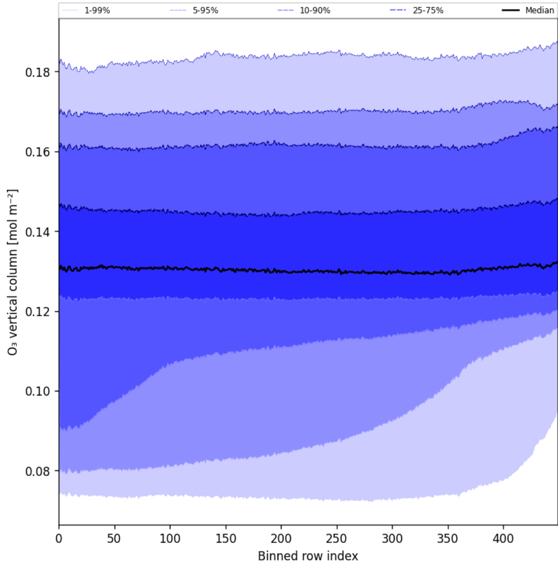
Figure 28: Along track statistics of “O 3 vertical column” for 2024-09-17 to 2024-09-18
