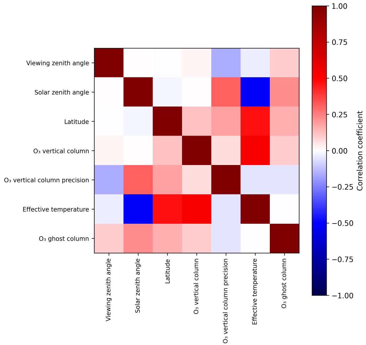
Figure 2: Map of correlation matrix for 2024-09-17 to 2024-09-18.
