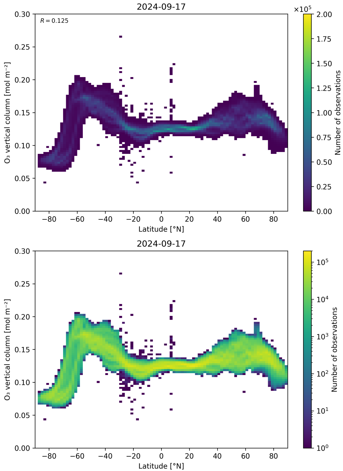
Figure 36: Scatter density plot of “Latitude” against “O 3 vertical column” for 2024-09-17 to 2024-09-18.
