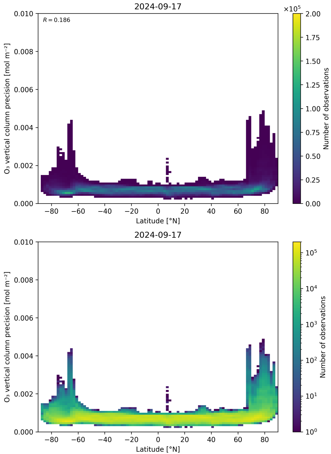
Figure 37: Scatter density plot of “Latitude” against “O 3 vertical column precision” for 2024-09-17 to 2024-09-18.
