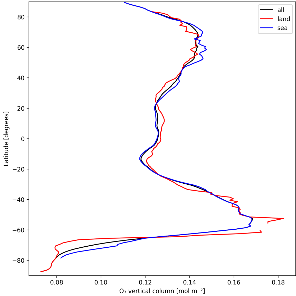
Figure 14: Zonal average of “O 3 vertical column” for 2024-09-17 to 2024-09-18.
