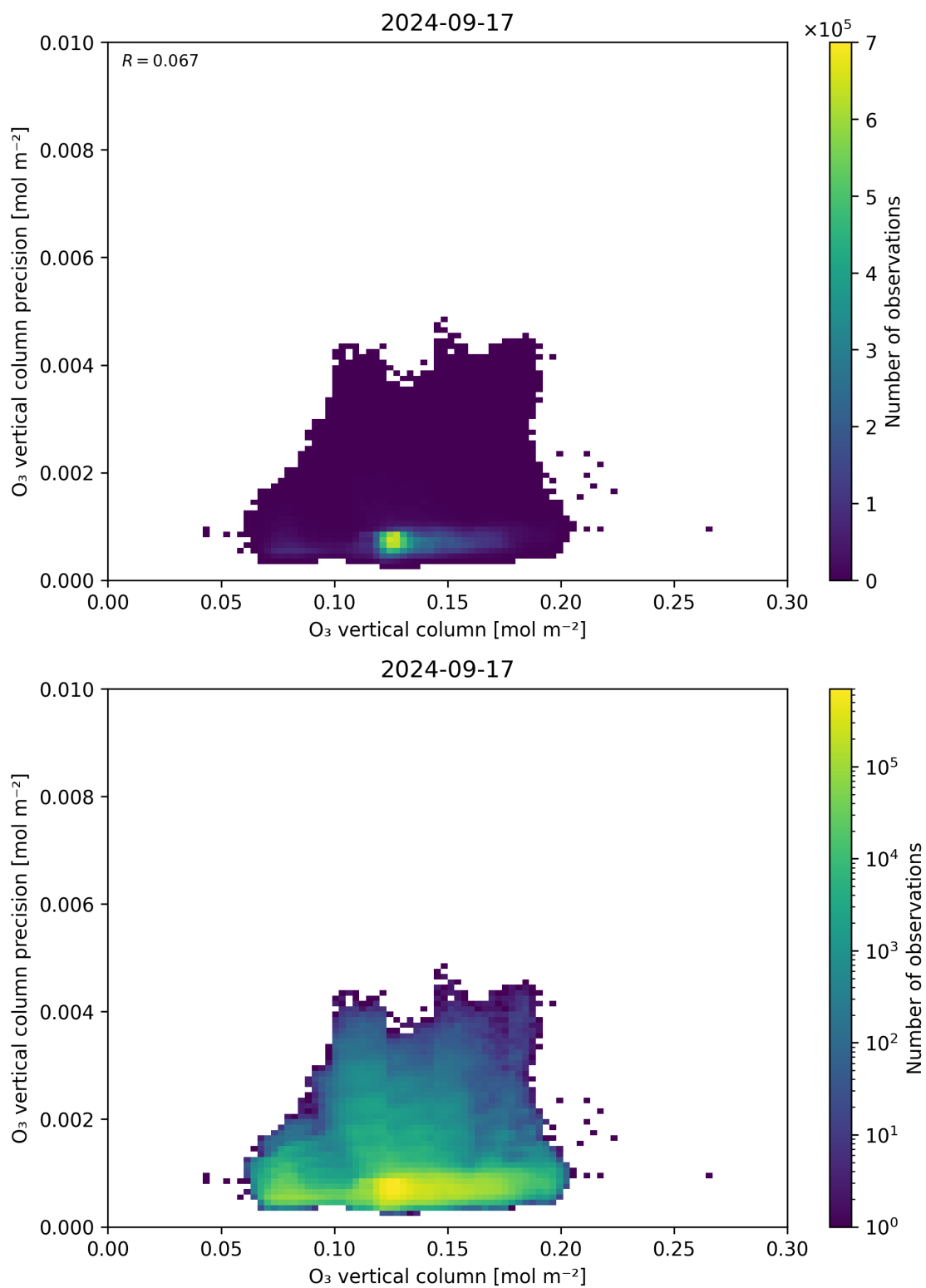
Figure 41: Scatter density plot of “O 3 vertical column” against “O 3 vertical column precision” for 2024-09-17 to 2024-09-18.
