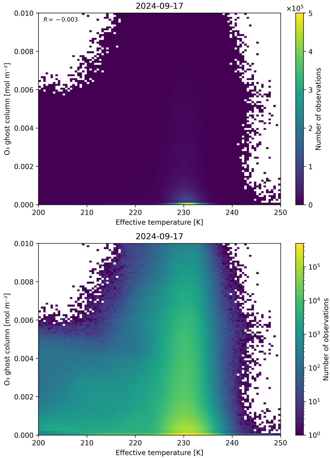
Figure 38: Scatter density plot of “Effective temperature” against “O 3 ghost column” for 2024-09-17 to 2024-09-18.
