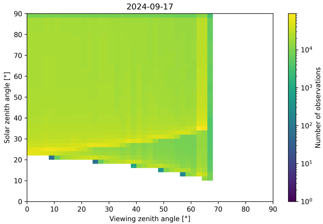
Figure 54: Scatter density plot of “Viewing zenith angle” against “Solar zenith angle” for 2024-09-17 to 2024-09-18.
