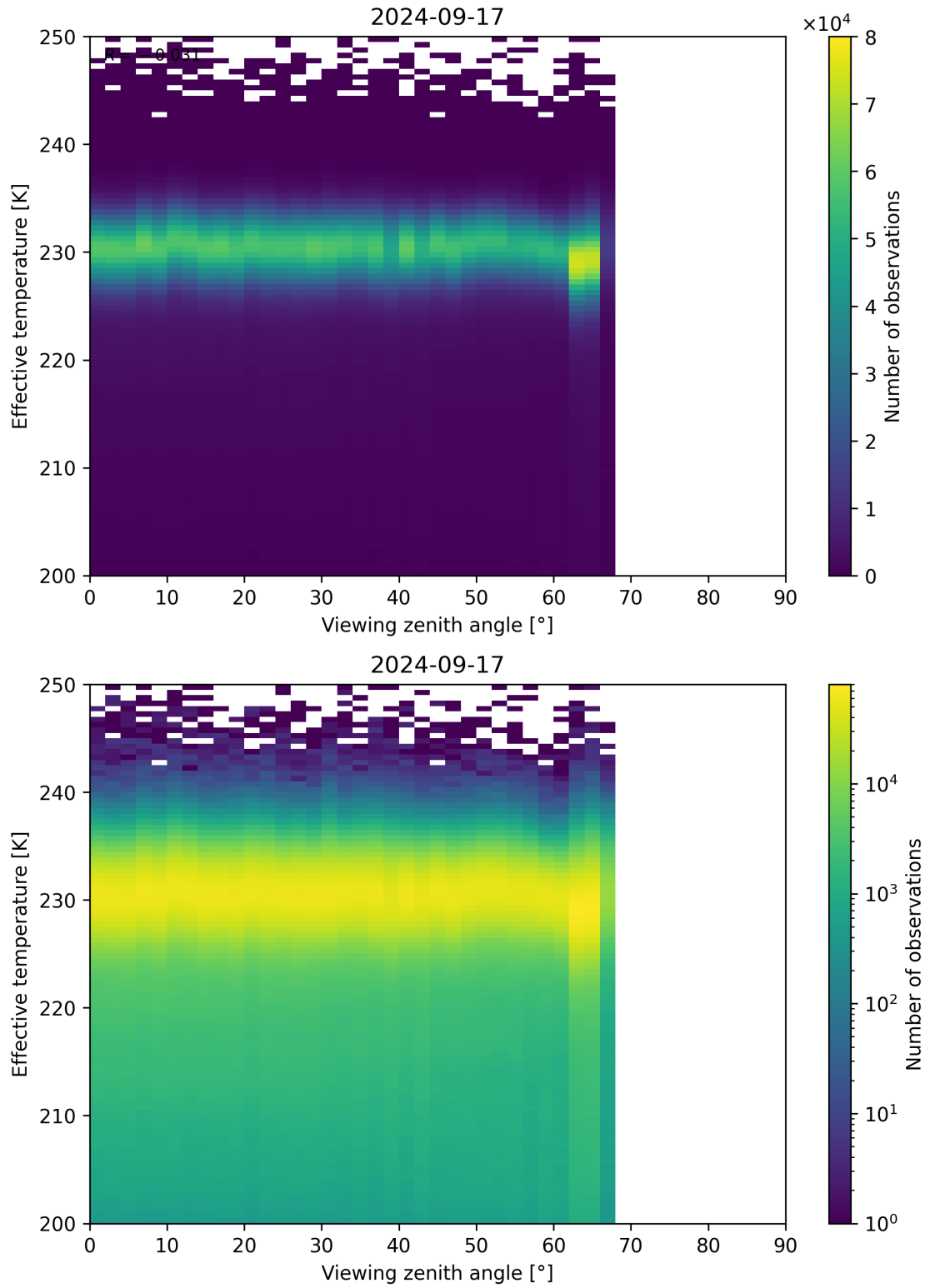
Figure 50: Scatter density plot of “Viewing zenith angle” against “Effective temperature” for 2024-09-17 to 2024-09-18.
