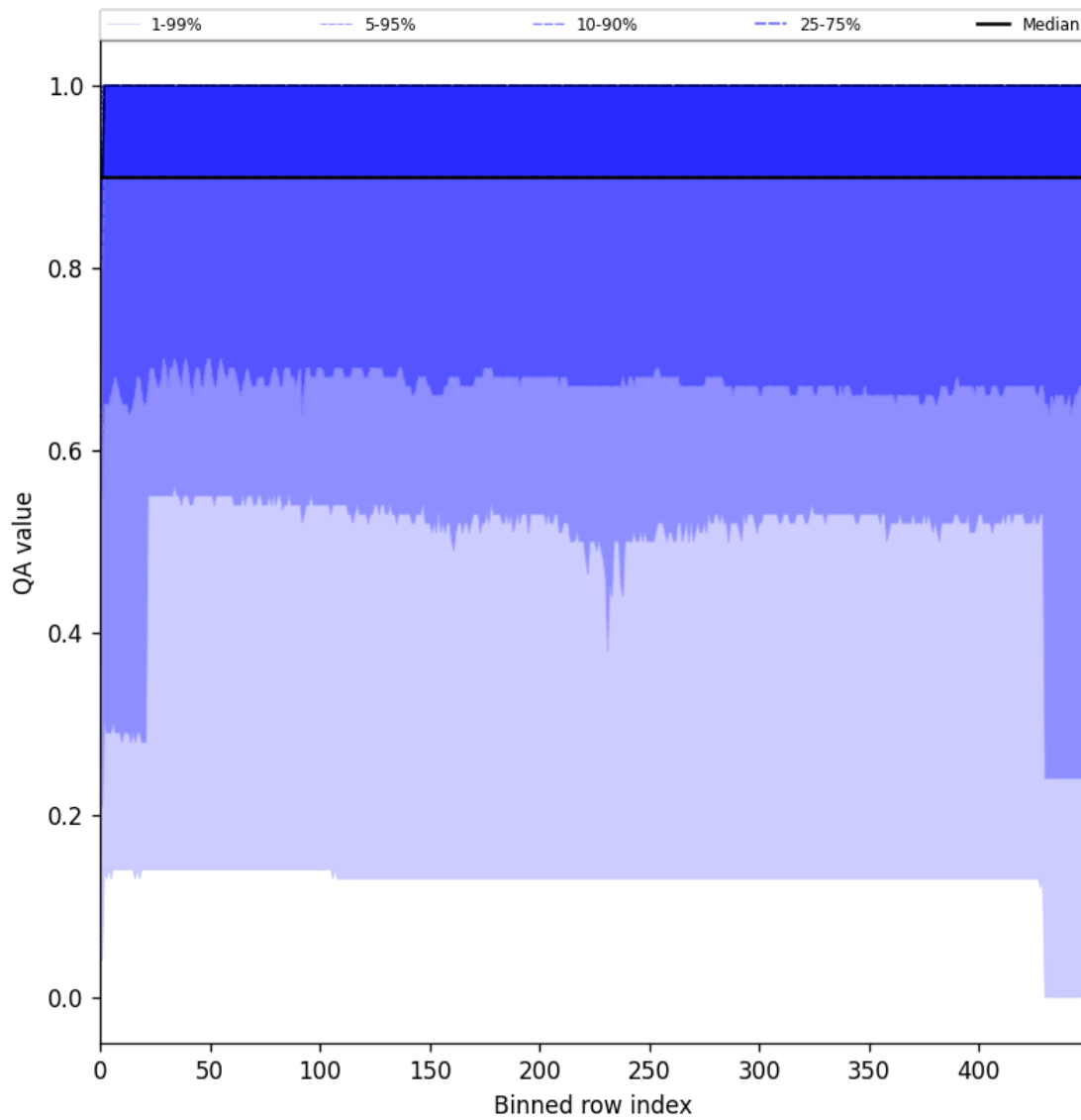
Figure 27: Along track statistics of “QA value” for 2024-09-17 to 2024-09-18
