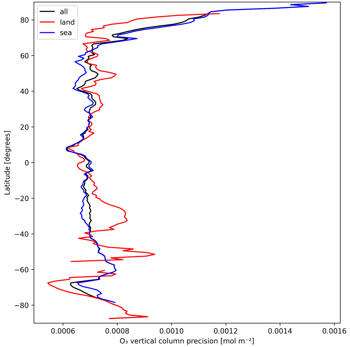
Figure 15: Zonal average of “O 3 vertical column precision” for 2024-09-17 to 2024-09-18.
