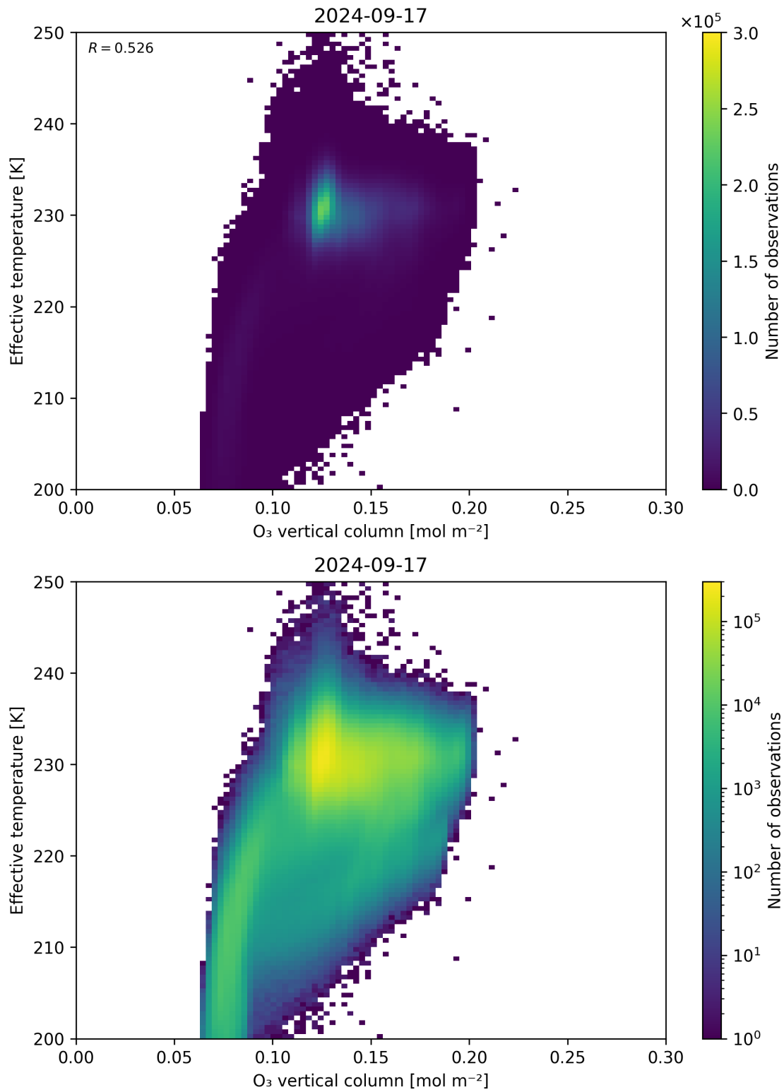
Figure 39: Scatter density plot of “O 3 vertical column” against “Effective temperature” for 2024-09-17 to 2024-09-18.
