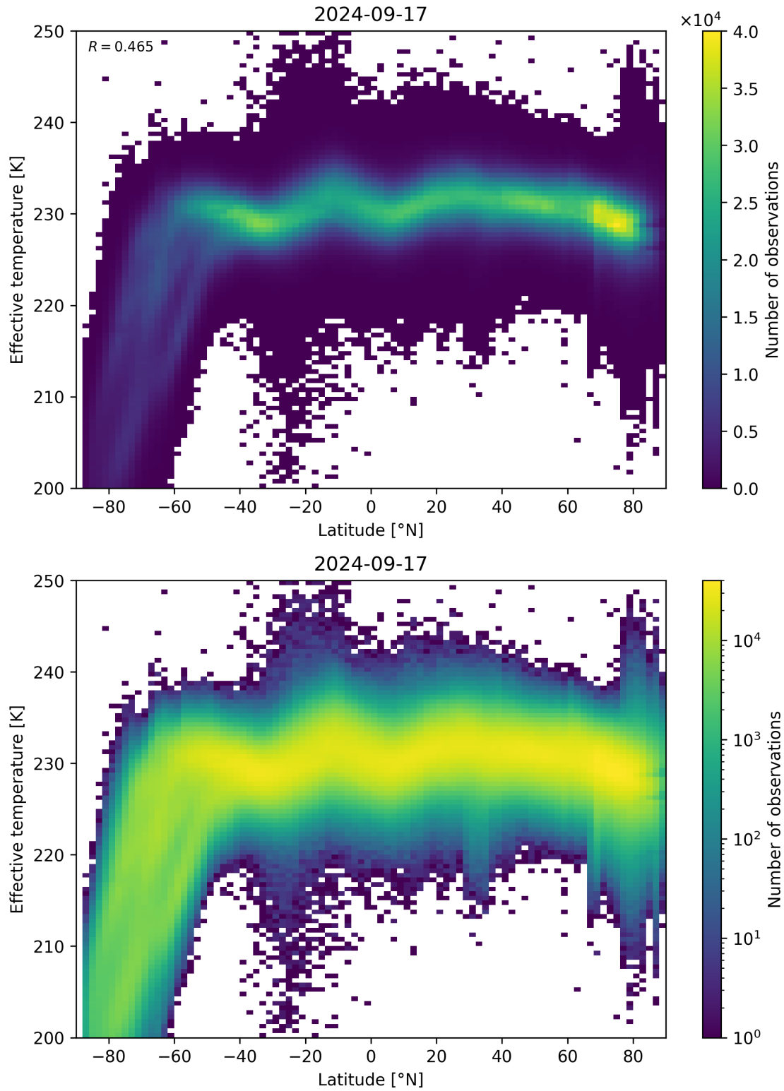
Figure 34: Scatter density plot of “Latitude” against “Effective temperature” for 2024-09-17 to 2024-09-18.
