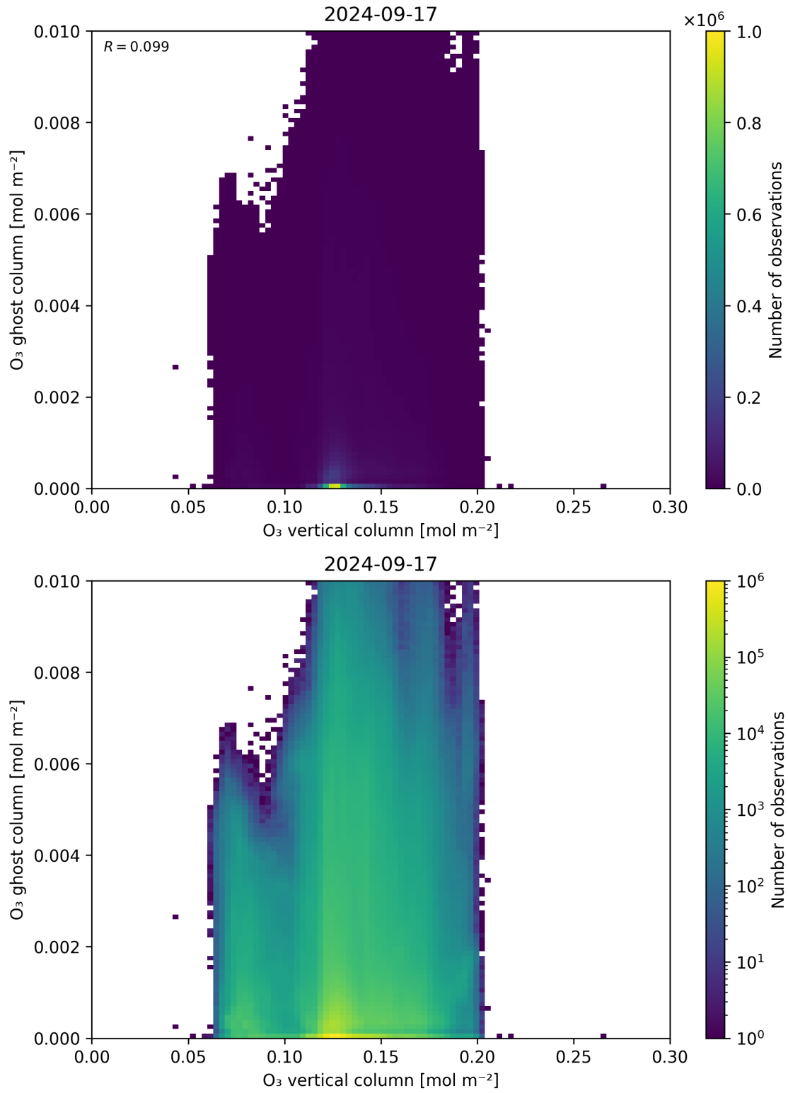
Figure 40: Scatter density plot of “O 3 vertical column” against “O 3 ghost column” for 2024-09-17 to 2024-09-18.
