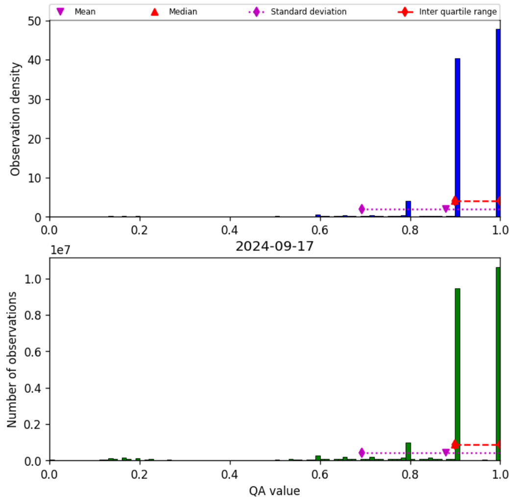
Figure 20: Histogram of “QA value” for 2024-09-17 to 2024-09-18
