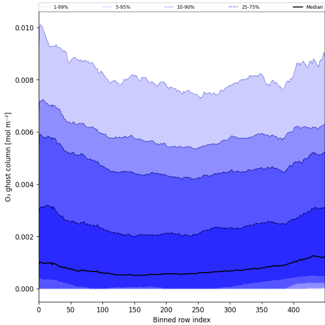
Figure 32: Along track statistics of “O 3 ghost column” for 2024-09-17 to 2024-09-18
