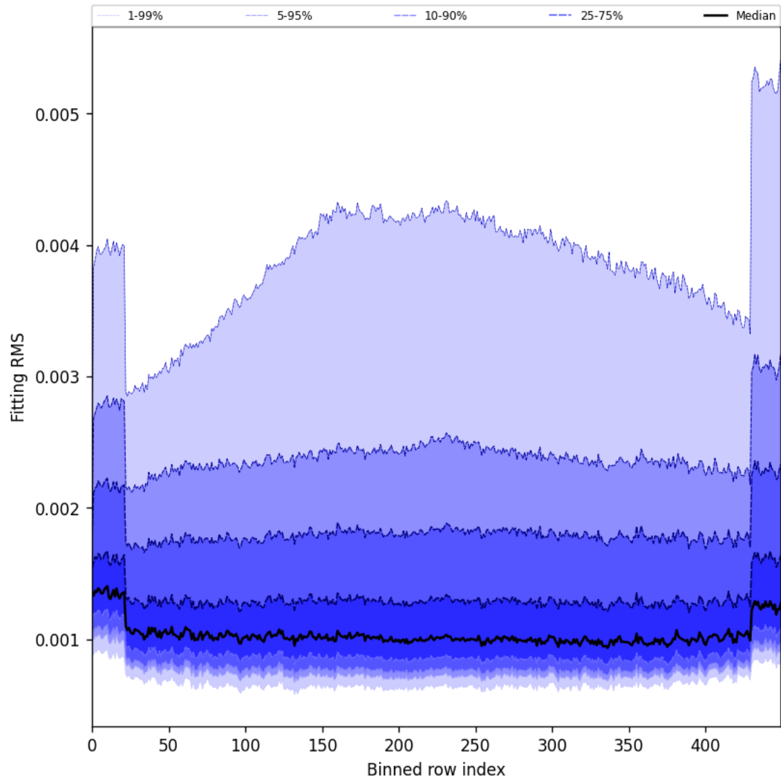
Figure 30: Along track statistics of “Fitting RMS” for 2024-09-17 to 2024-09-18
