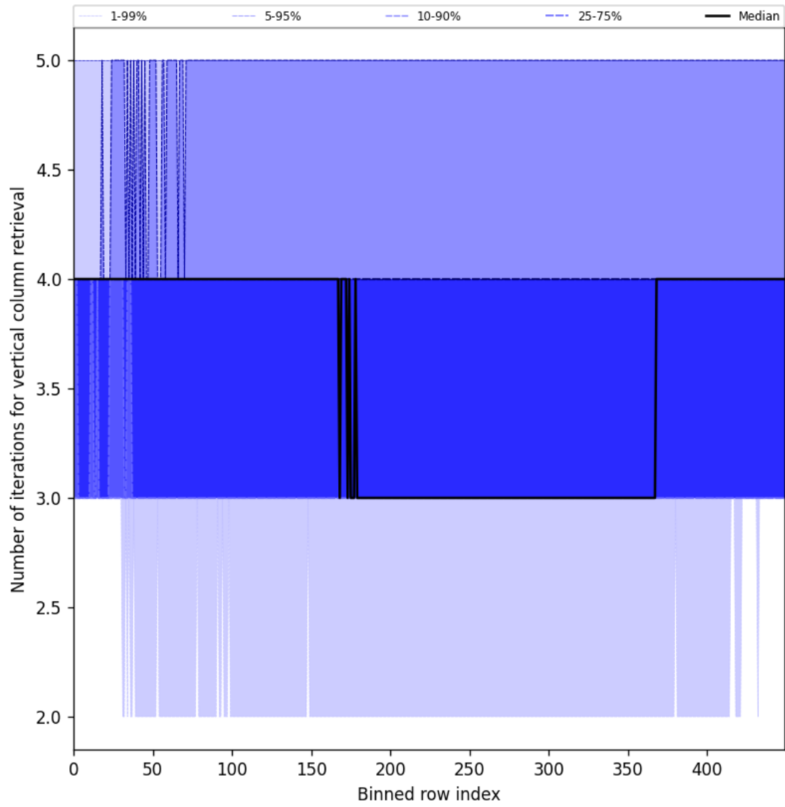
Figure 33: Along track statistics of “Number of iterations for vertical column retrieval” for 2024-09-17 to 2024-09-18
