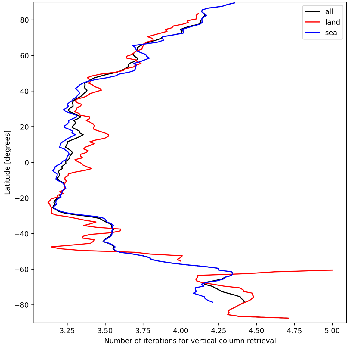
Figure 19: Zonal average of “Number of iterations for vertical column retrieval” for 2024-09-17 to 2024-09-18.
