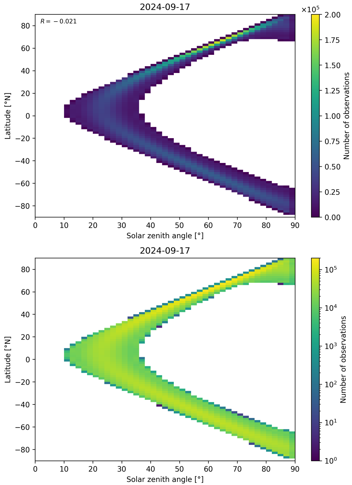
Figure 44: Scatter density plot of “Solar zenith angle” against “Latitude” for 2024-09-17 to 2024-09-18.
