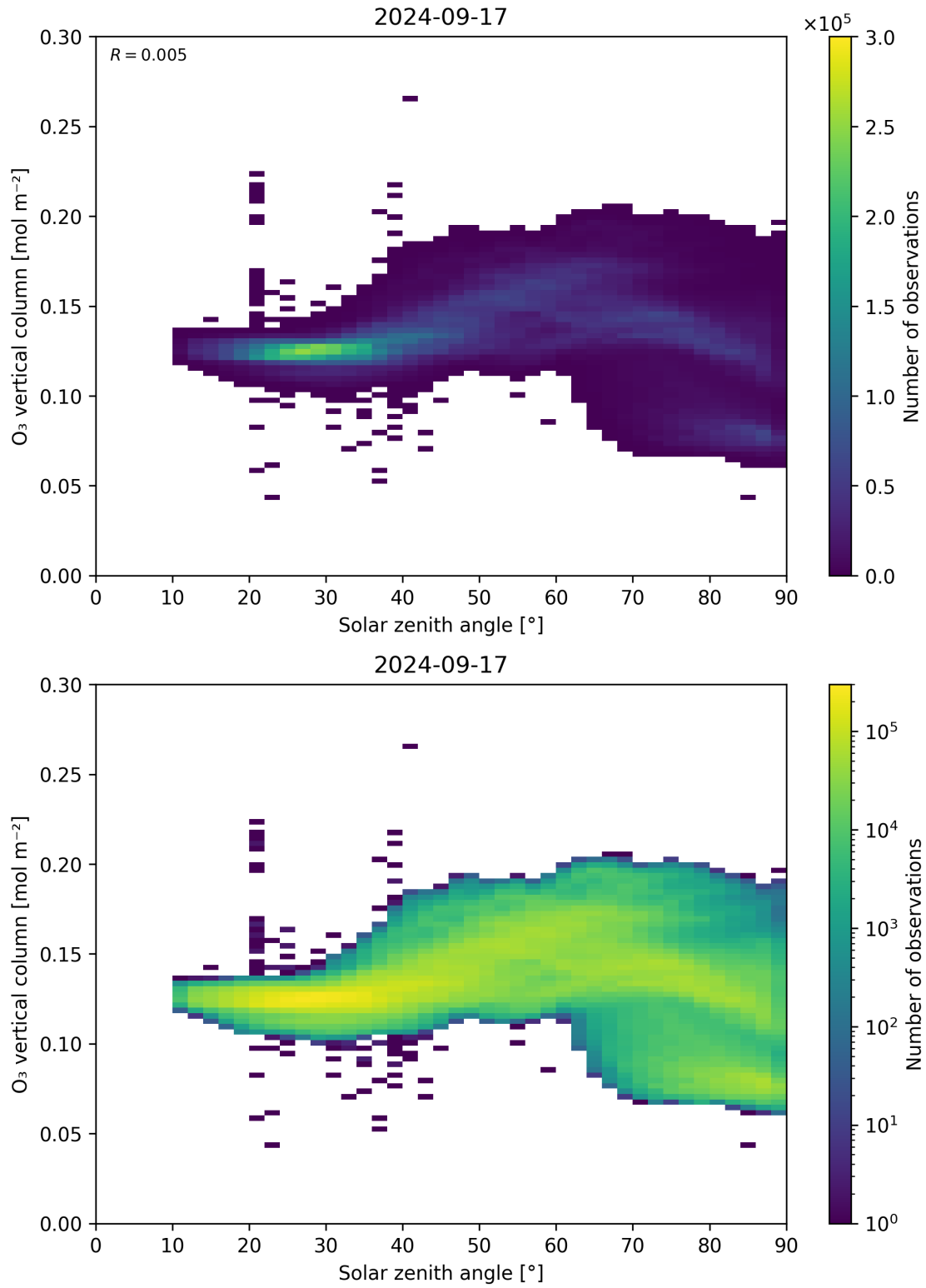
Figure 47: Scatter density plot of “Solar zenith angle” against “O 3 vertical column” for 2024-09-17 to 2024-09-18.
