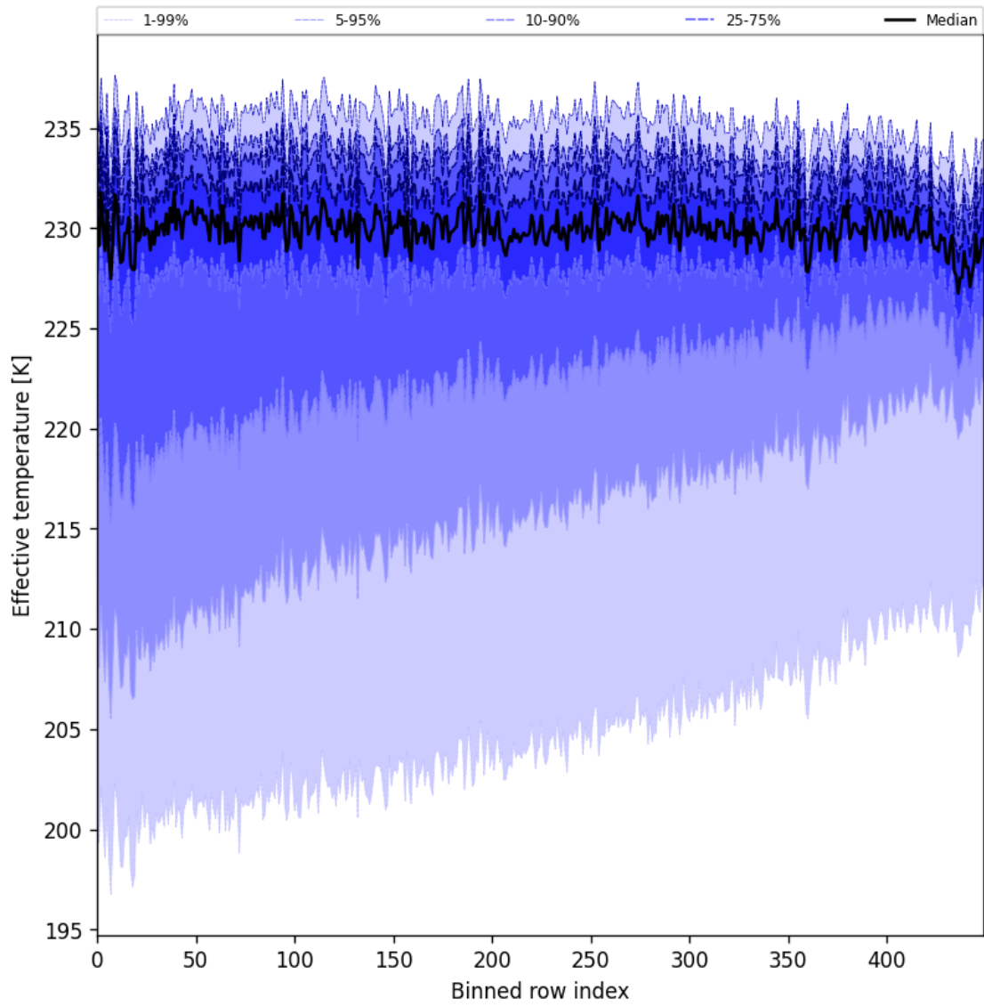
Figure 31: Along track statistics of “Effective temperature” for 2024-09-17 to 2024-09-18
