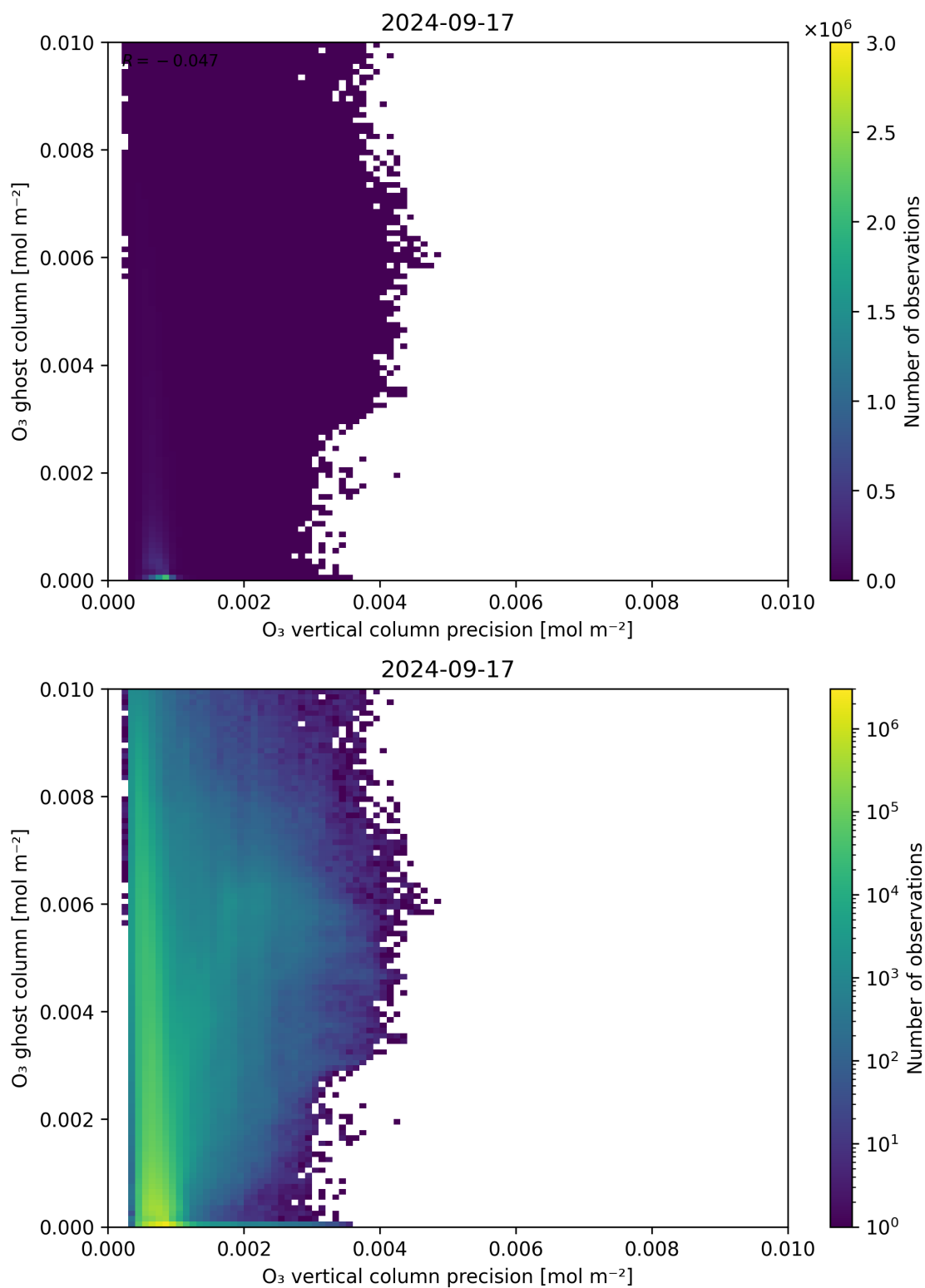
Figure 43: Scatter density plot of “O 3 vertical column precision” against “O 3 ghost column” for 2024-09-17 to 2024-09-18.
