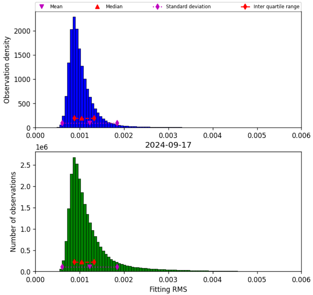
Figure 23: Histogram of “Fitting RMS” for 2024-09-17 to 2024-09-18
