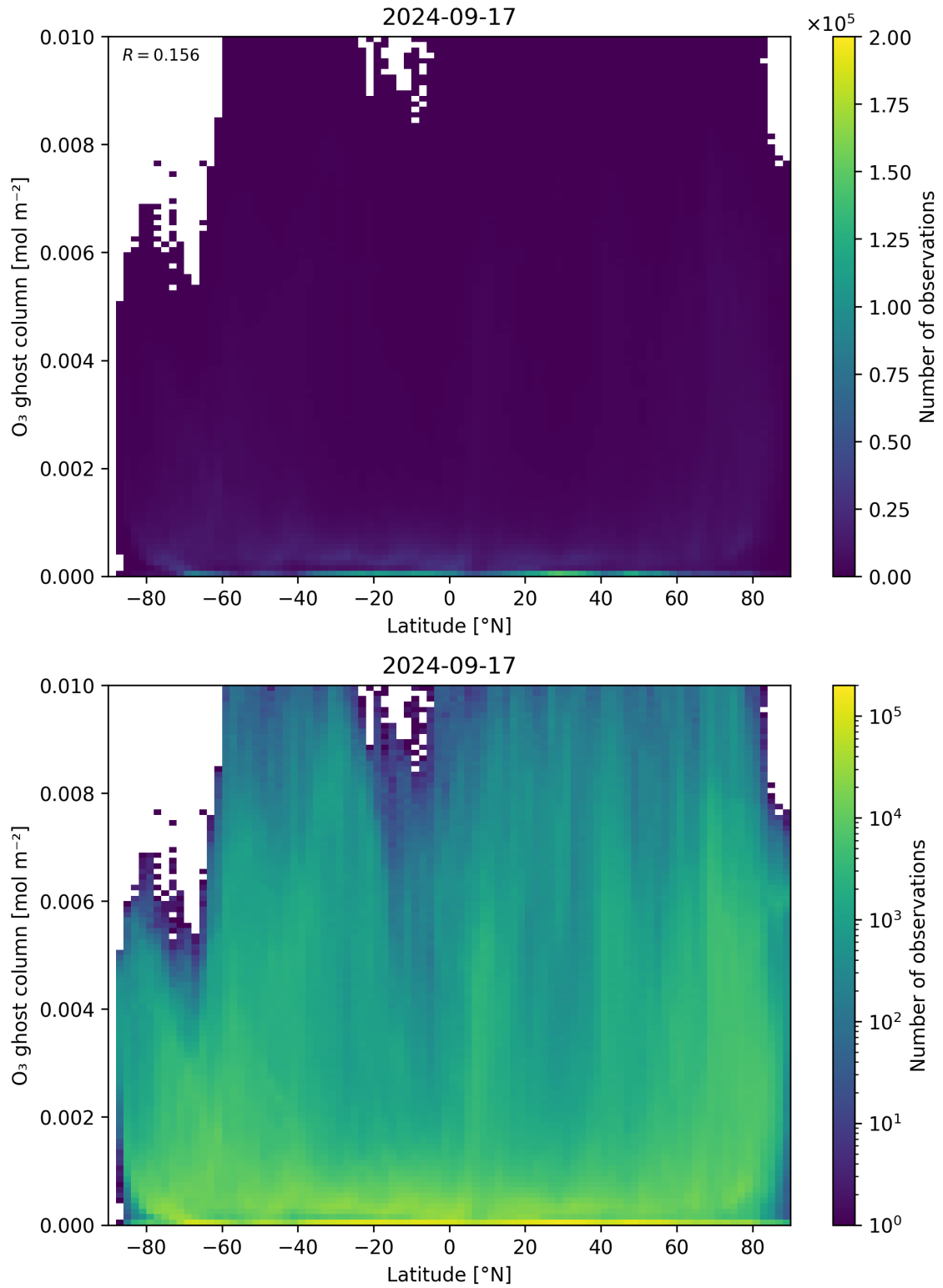
Figure 35: Scatter density plot of “Latitude” against “O 3 ghost column” for 2024-09-17 to 2024-09-18.
