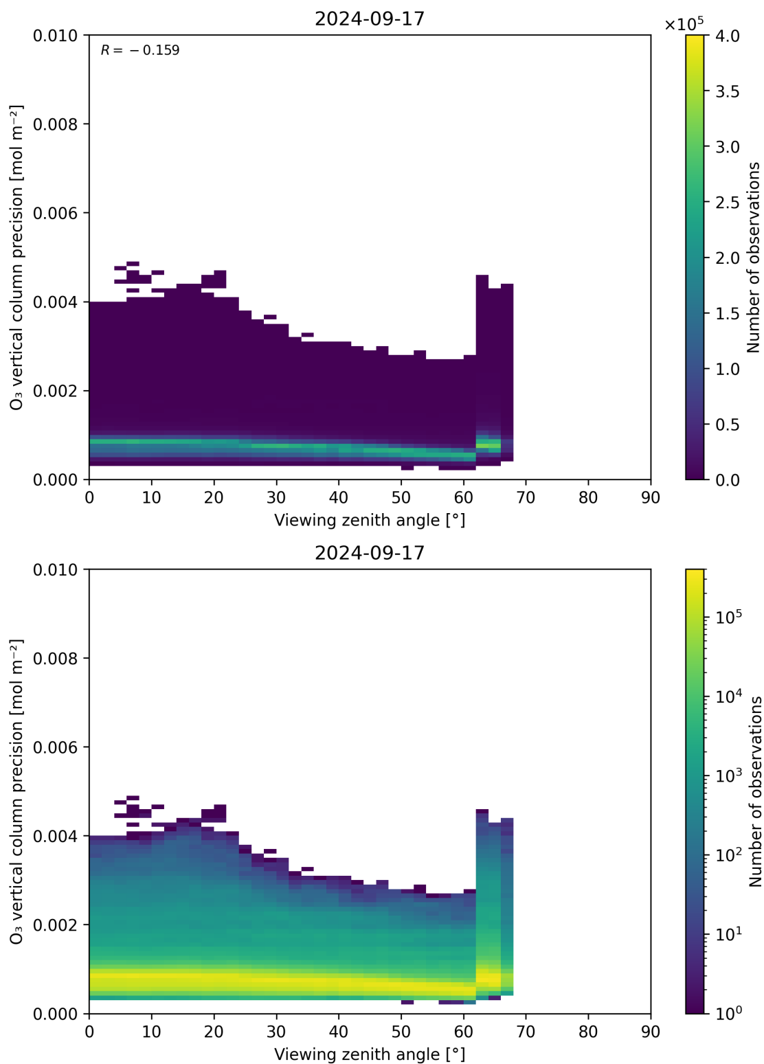
Figure 53: Scatter density plot of “Viewing zenith angle” against “O 3 vertical column precision” for 2024-09-17 to 2024-09-18.
