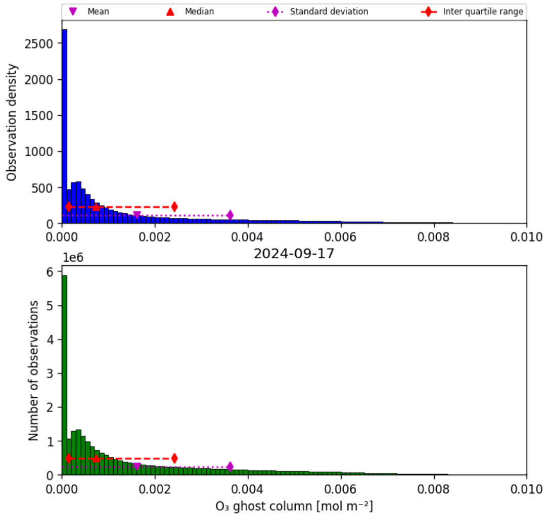
Figure 25: Histogram of “O 3 ghost column” for 2024-09-17 to 2024-09-18
