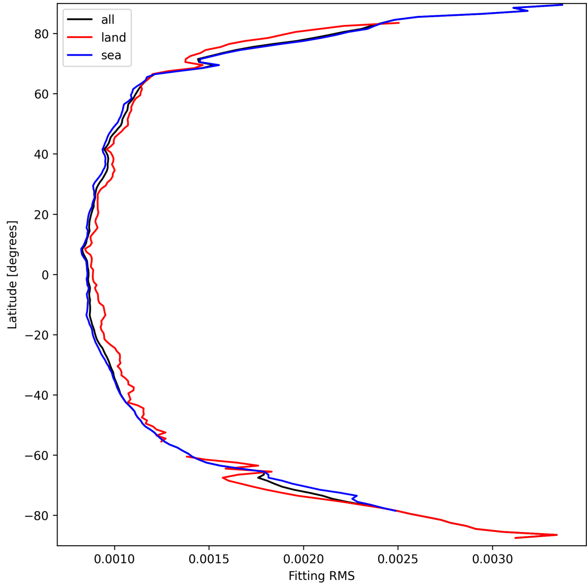
Figure 16: Zonal average of “Fitting RMS” for 2024-09-17 to 2024-09-18.
