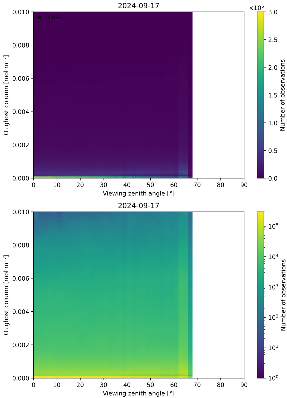
Figure 51: Scatter density plot of “Viewing zenith angle” against “O 3 ghost column” for 2024-09-17 to 2024-09-18.
