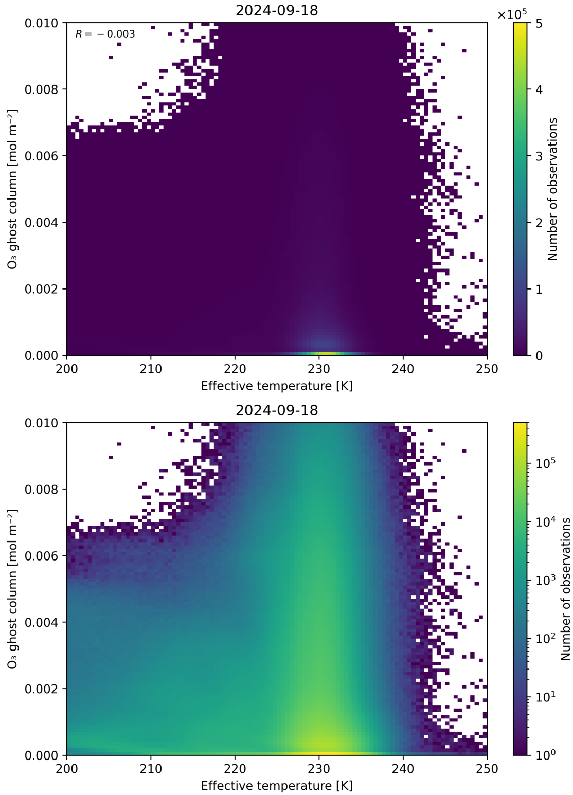
Figure 38: Scatter density plot of “Effective temperature” against “O 3 ghost column” for 2024-09-17 to 2024-09-19.
