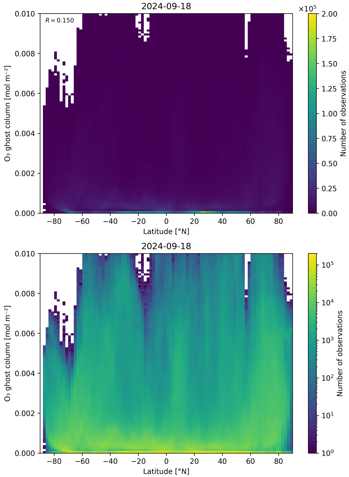
Figure 35: Scatter density plot of “Latitude” against “O 3 ghost column” for 2024-09-17 to 2024-09-19.
