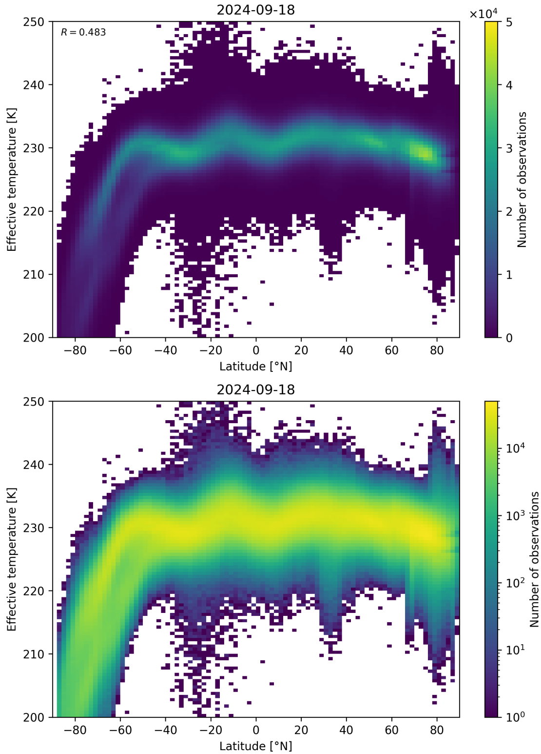
Figure 34: Scatter density plot of “Latitude” against “Effective temperature” for 2024-09-17 to 2024-09-19.
