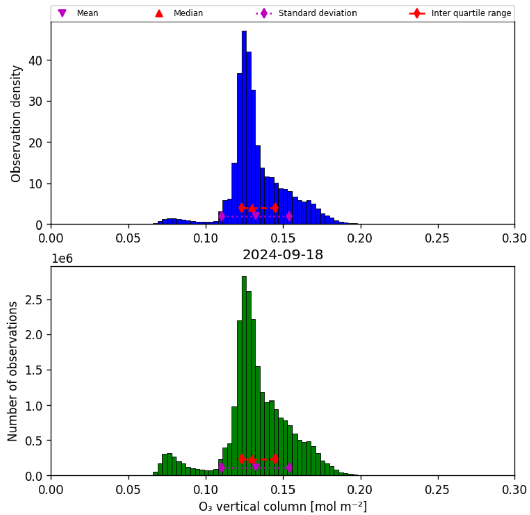
Figure 21: Histogram of “O 3 vertical column” for 2024-09-17 to 2024-09-19
