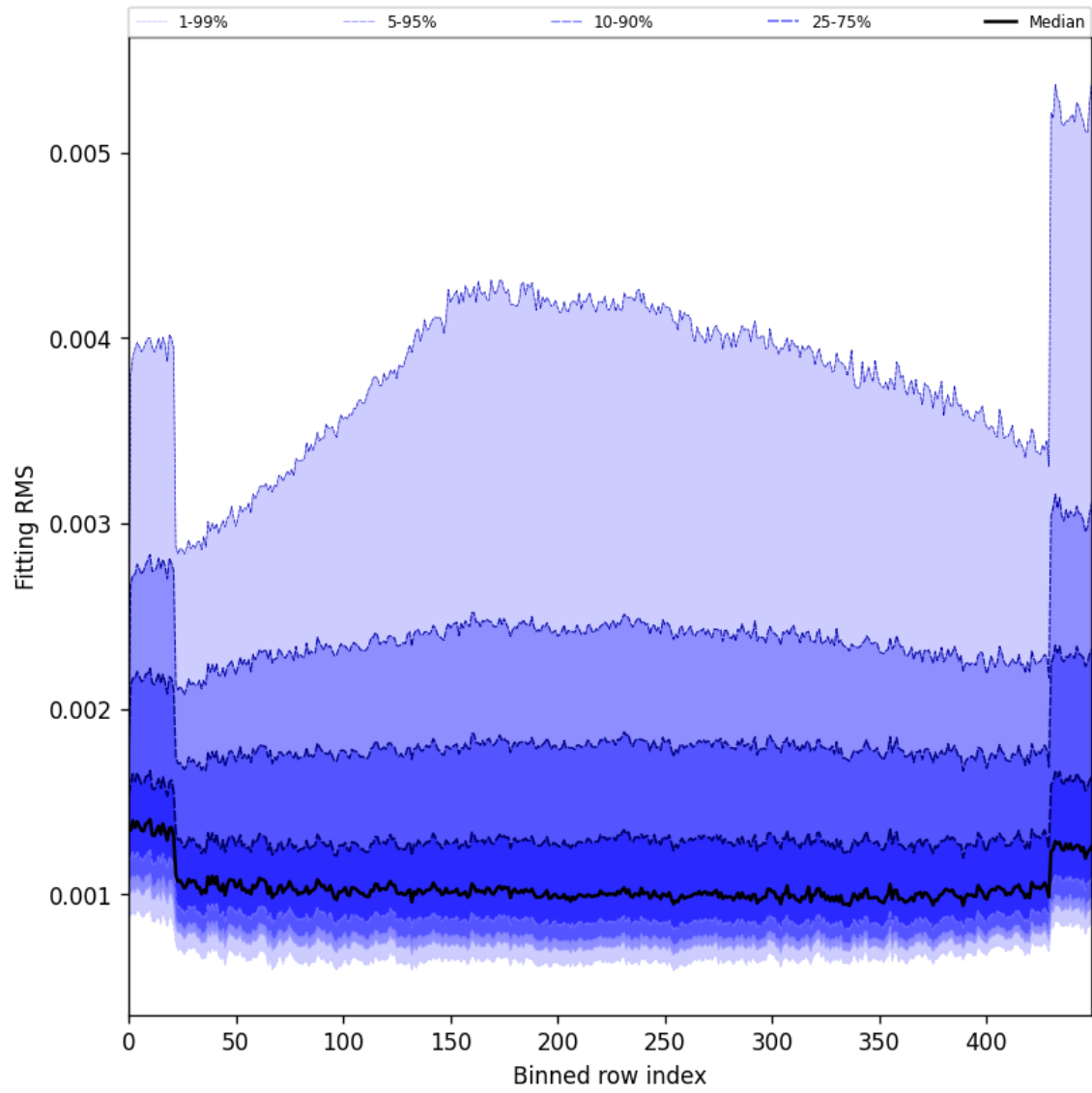
Figure 30: Along track statistics of “Fitting RMS” for 2024-09-17 to 2024-09-19
