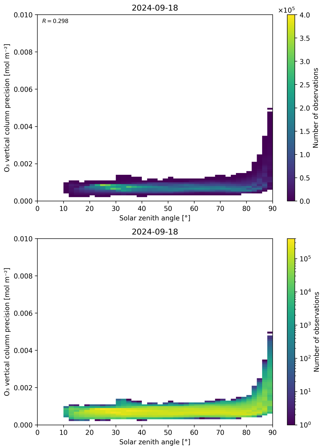
Figure 48: Scatter density plot of “Solar zenith angle” against “O 3 vertical column precision” for 2024-09-17 to 2024-09-19.
