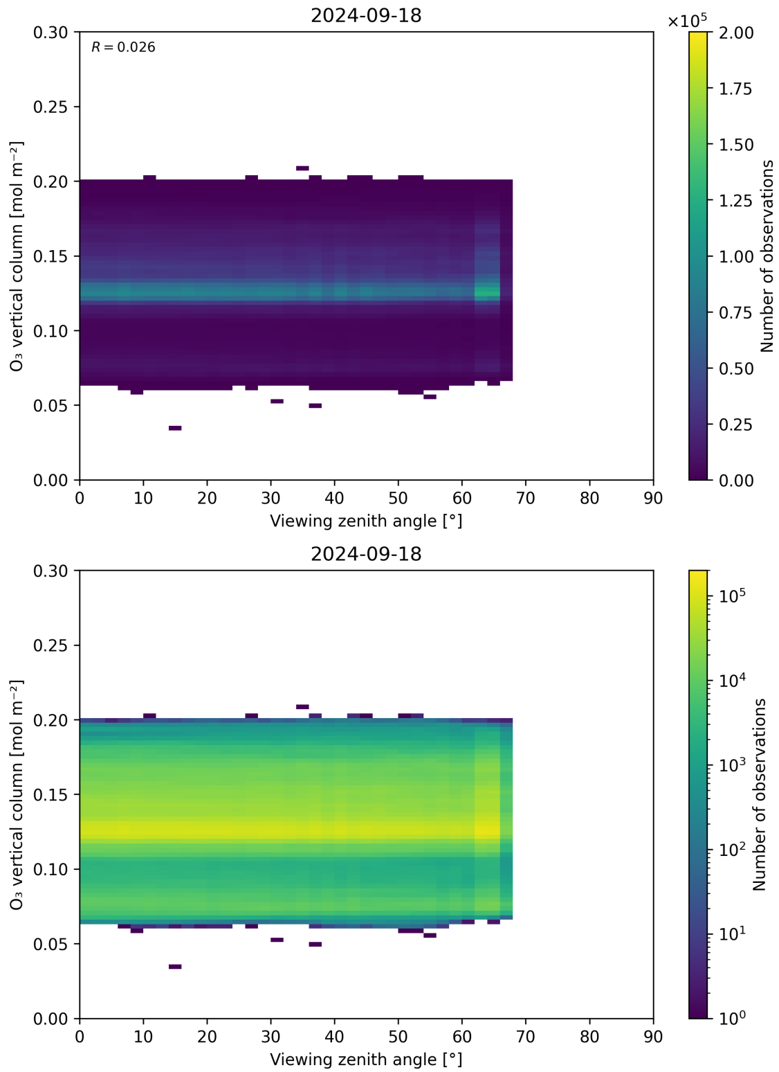
Figure 52: Scatter density plot of “Viewing zenith angle” against “O 3 vertical column” for 2024-09-17 to 2024-09-19.
