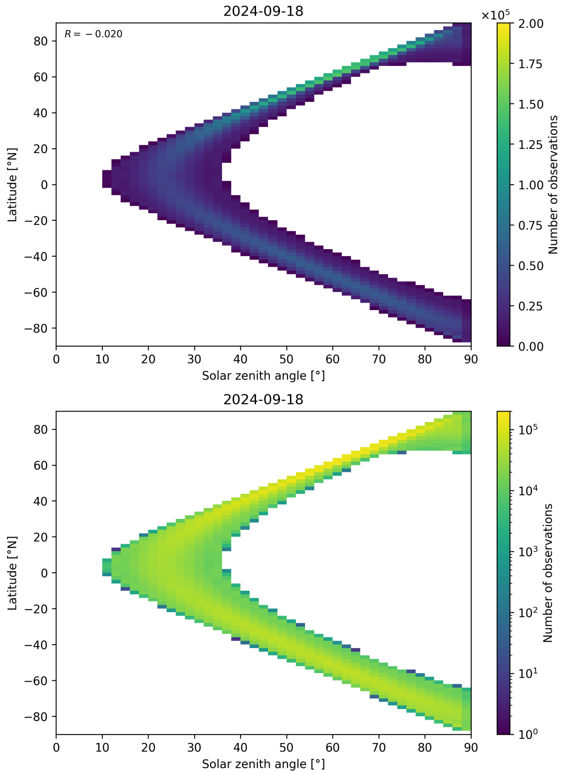
Figure 44: Scatter density plot of “Solar zenith angle” against “Latitude” for 2024-09-17 to 2024-09-19.
