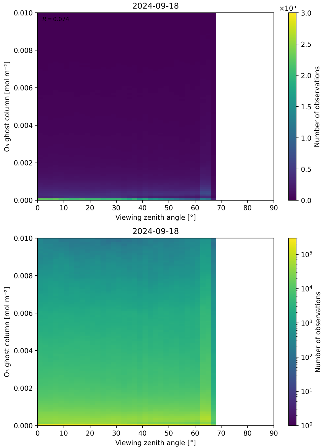
Figure 51: Scatter density plot of “Viewing zenith angle” against “O 3 ghost column” for 2024-09-17 to 2024-09-19.
