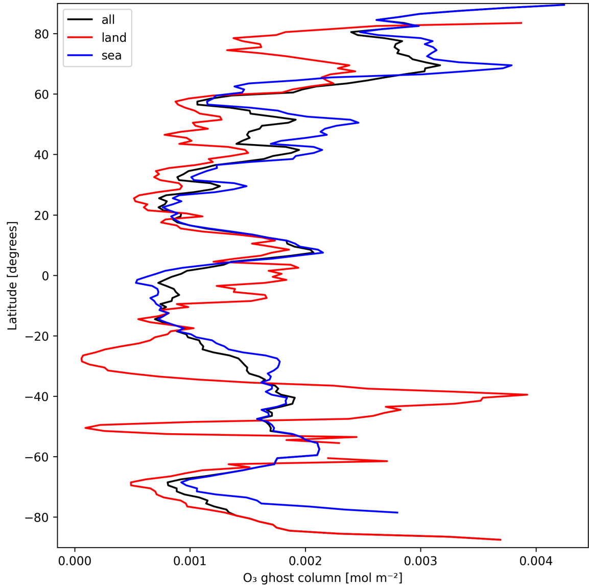
Figure 18: Zonal average of "O 3 ghost column" for 2024-09-17 to 2024-09-19.
