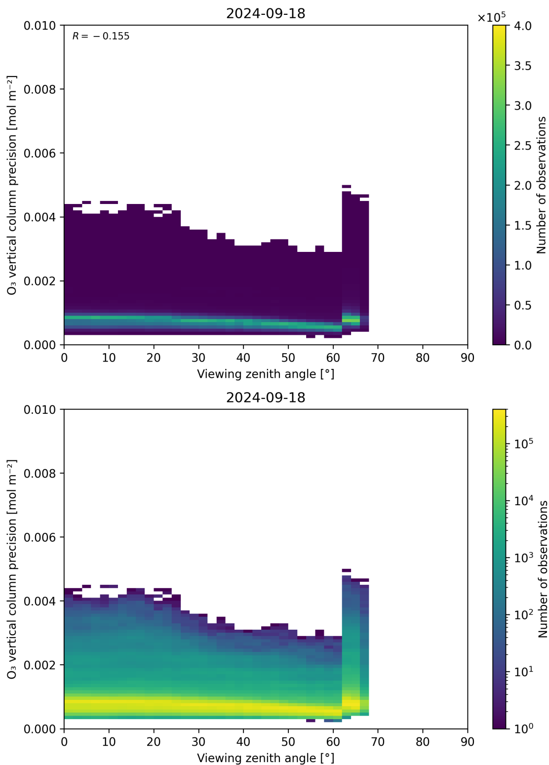
Figure 53: Scatter density plot of “Viewing zenith angle” against “O 3 vertical column precision” for 2024-09-17 to 2024-09-19.
