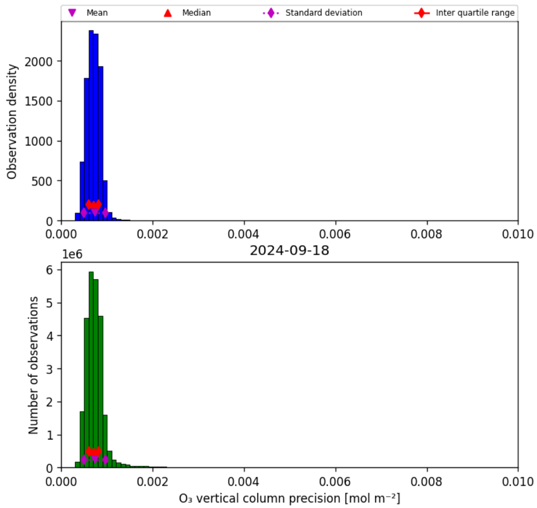
Figure 22: Histogram of “O 3 vertical column precision” for 2024-09-17 to 2024-09-19
