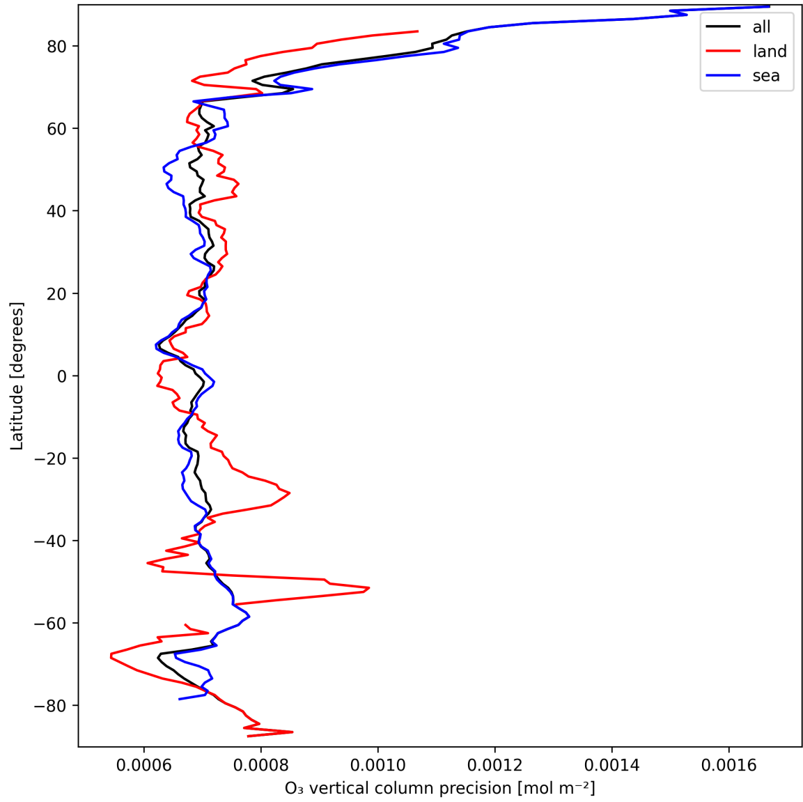
Figure 15: Zonal average of “O 3 vertical column precision” for 2024-09-17 to 2024-09-19.
