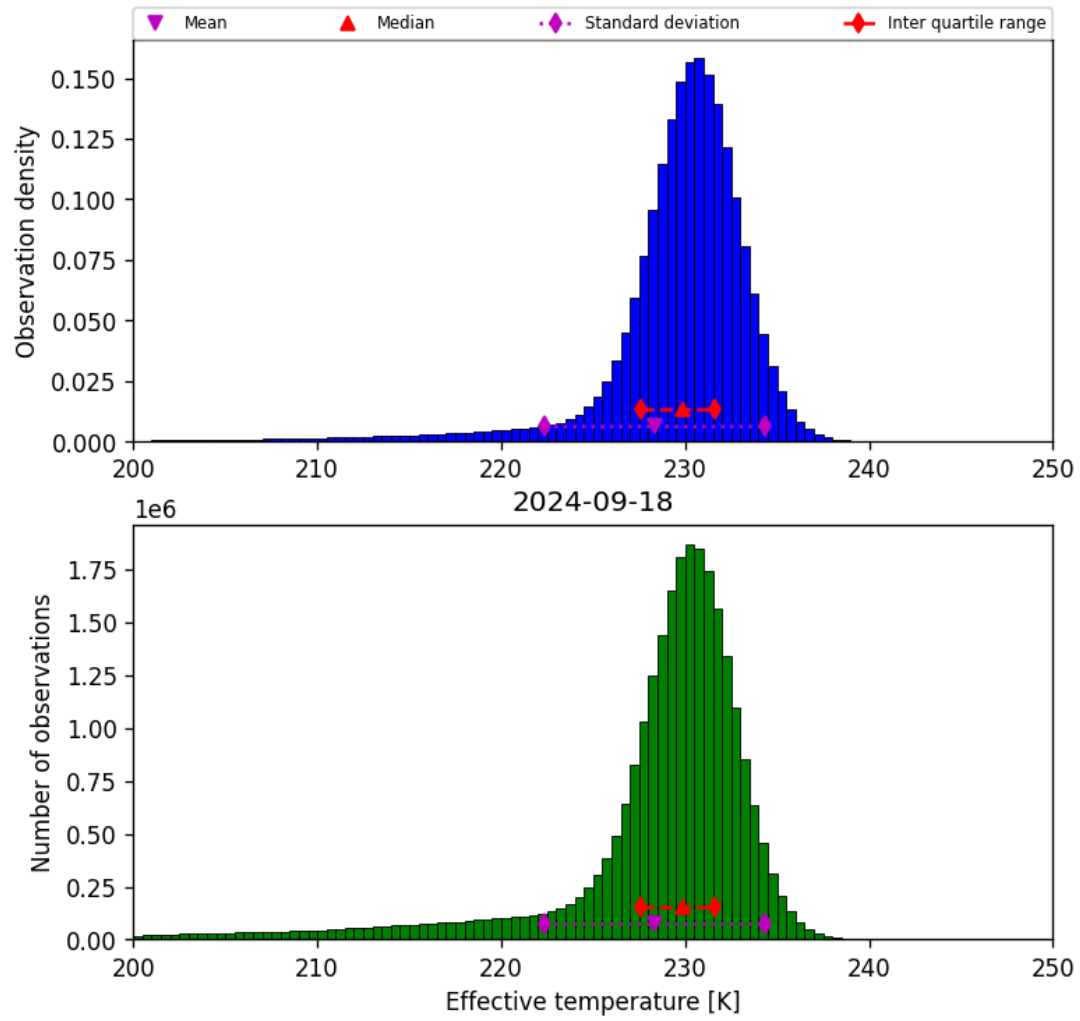
Figure 24: Histogram of “Effective temperature” for 2024-09-17 to 2024-09-19
