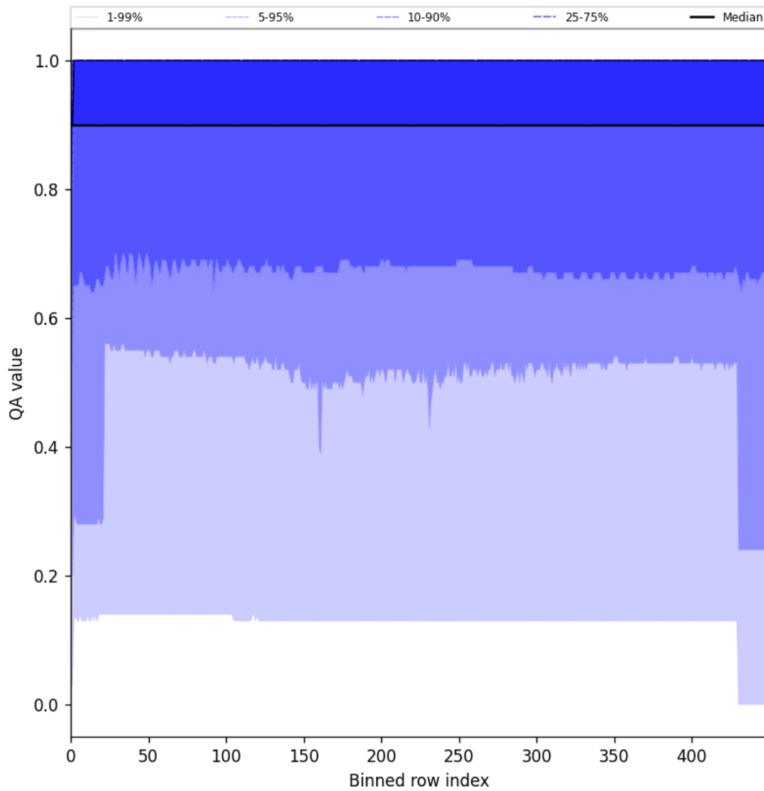
Figure 27: Along track statistics of “QA value” for 2024-09-17 to 2024-09-19
