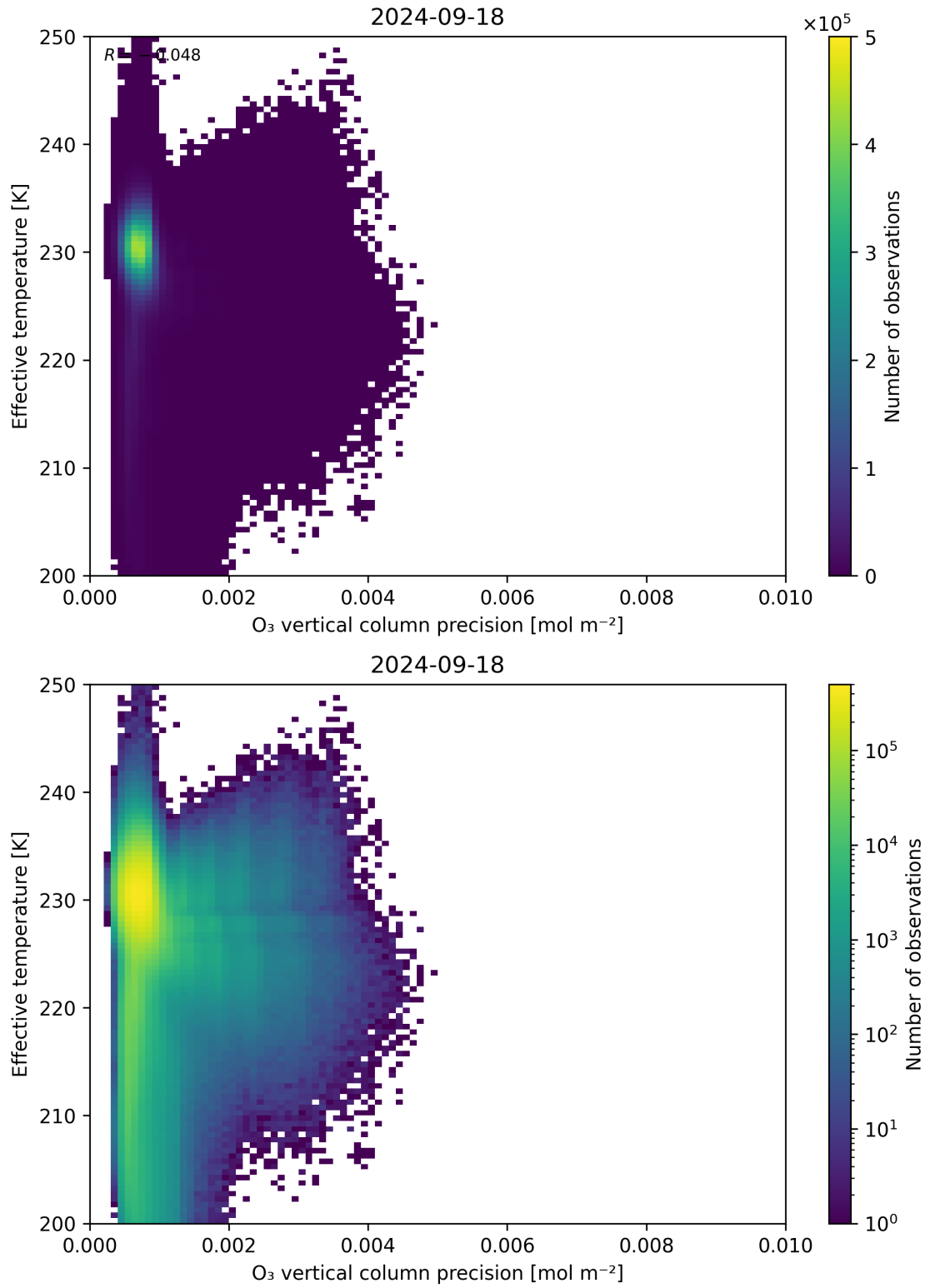
Figure 42: Scatter density plot of “O 3 vertical column precision” against “Effective temperature” for 2024-09-17 to 2024-09-19.
