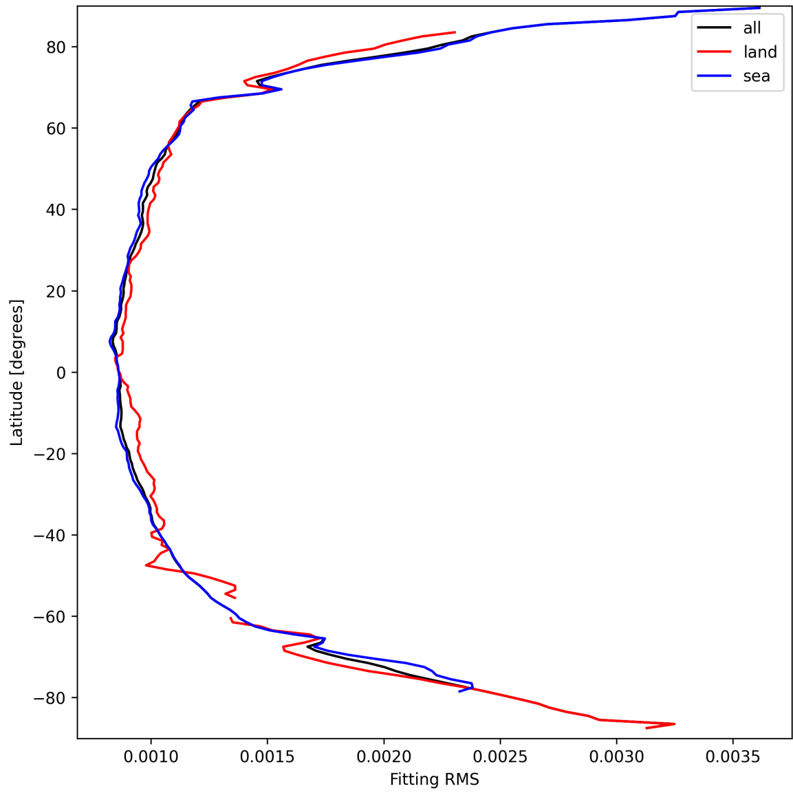
Figure 16: Zonal average of “Fitting RMS” for 2024-09-17 to 2024-09-19.
