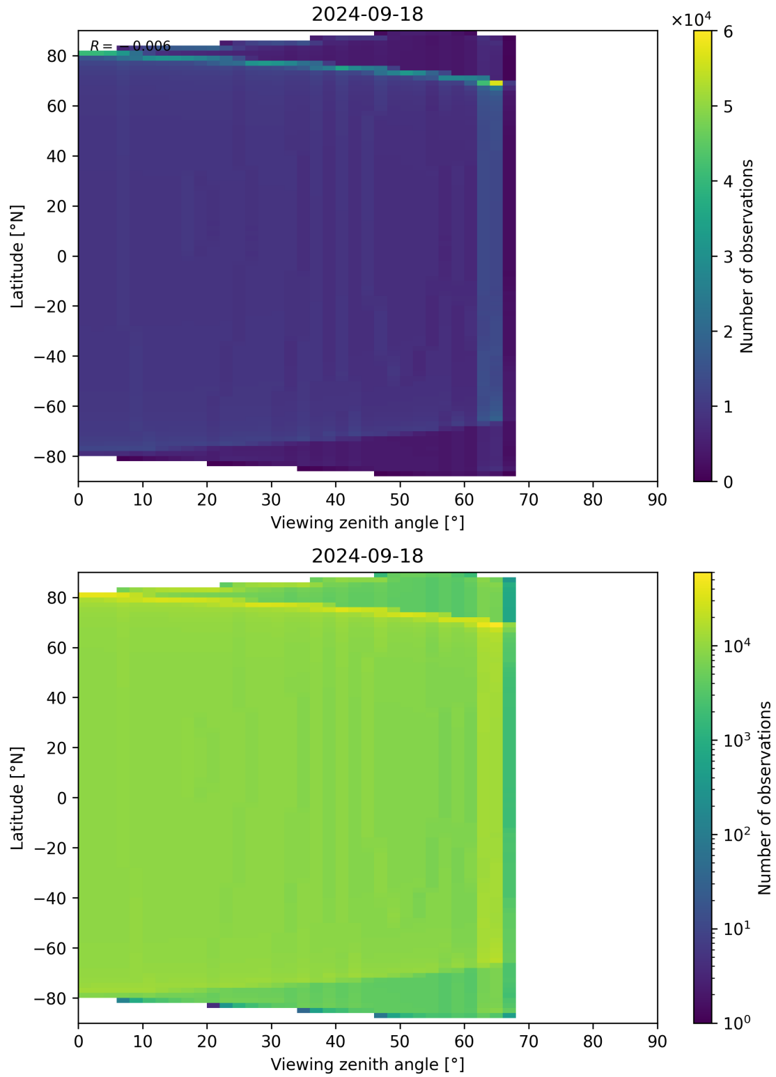
Figure 49: Scatter density plot of “Viewing zenith angle” against “Latitude” for 2024-09-17 to 2024-09-19.
