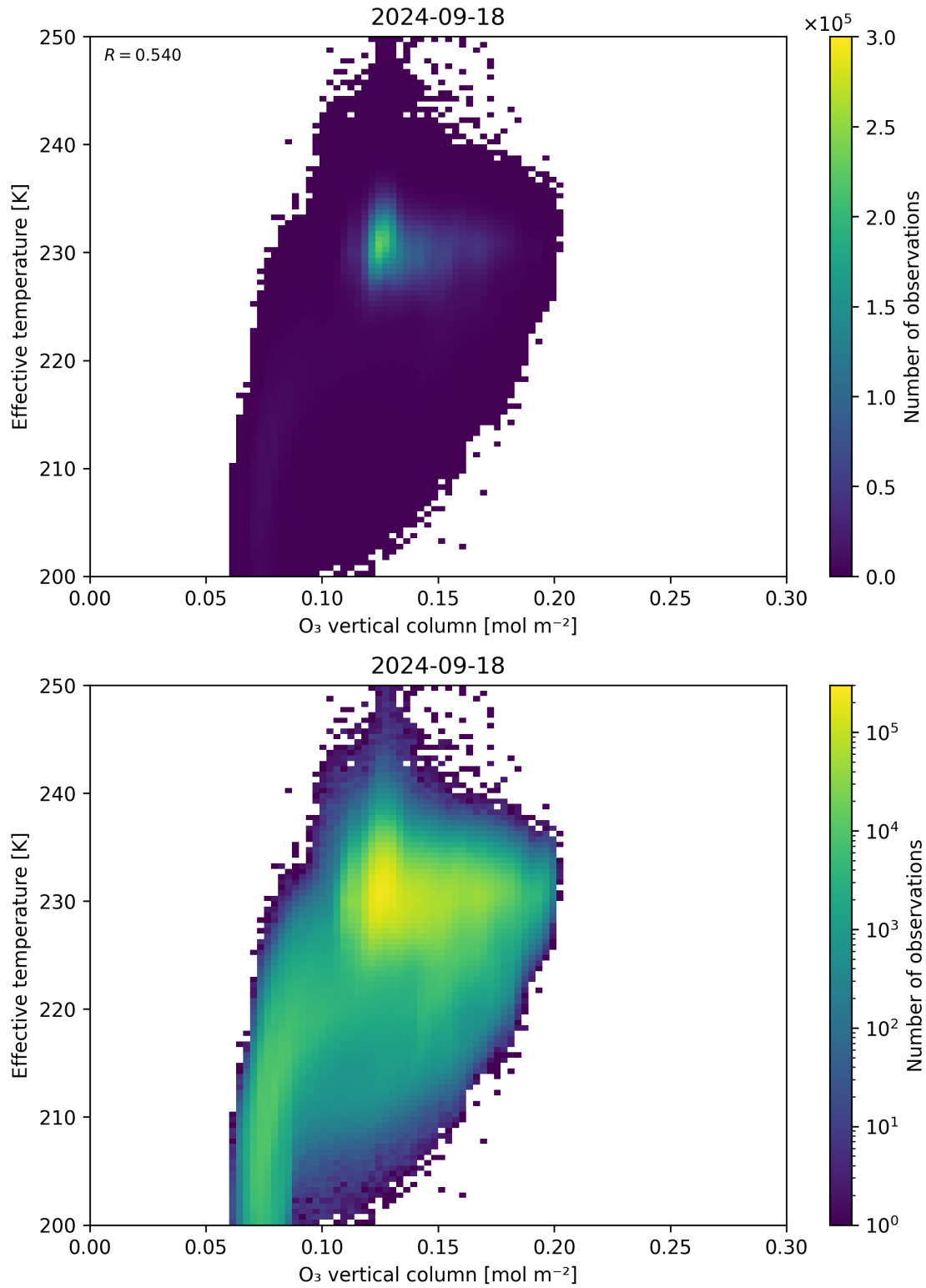
Figure 39: Scatter density plot of “O 3 vertical column” against “Effective temperature” for 2024-09-17 to 2024-09-19.
