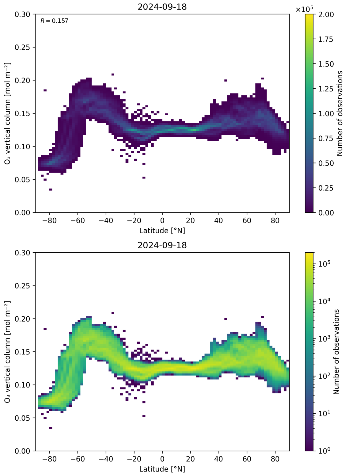
Figure 36: Scatter density plot of “Latitude” against “O 3 vertical column” for 2024-09-17 to 2024-09-19.
