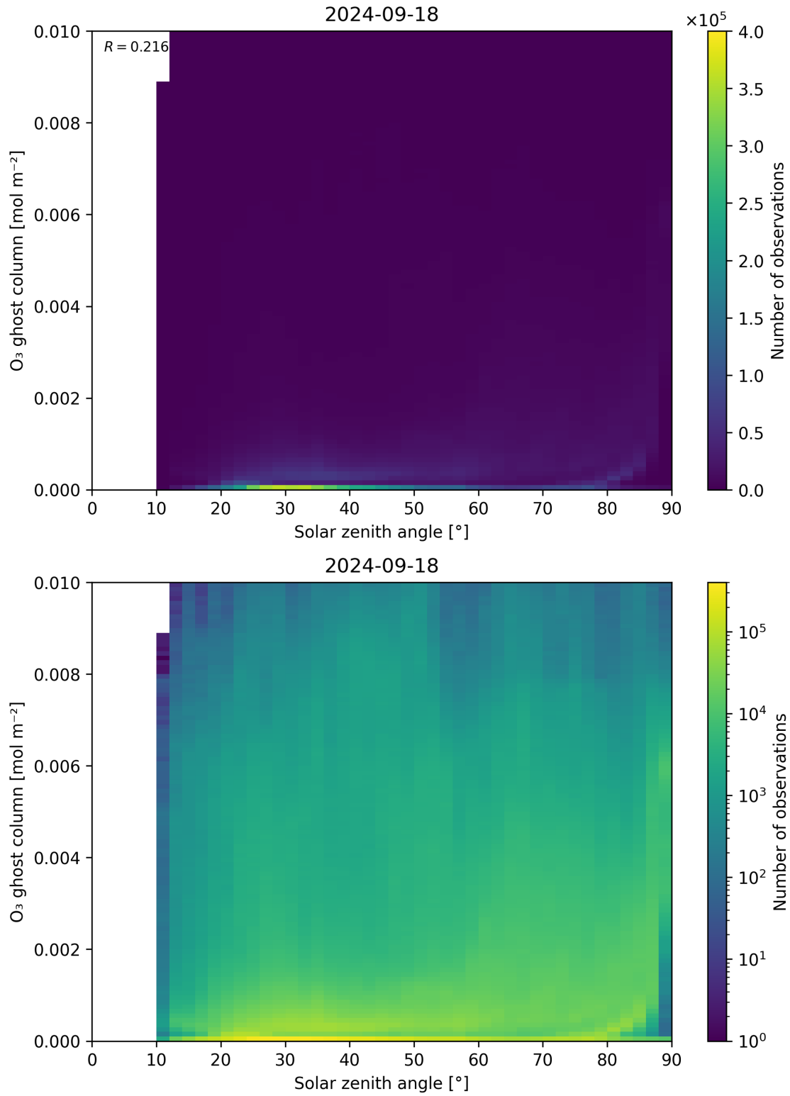
Figure 46: Scatter density plot of “Solar zenith angle” against “O 3 ghost column” for 2024-09-17 to 2024-09-19.
