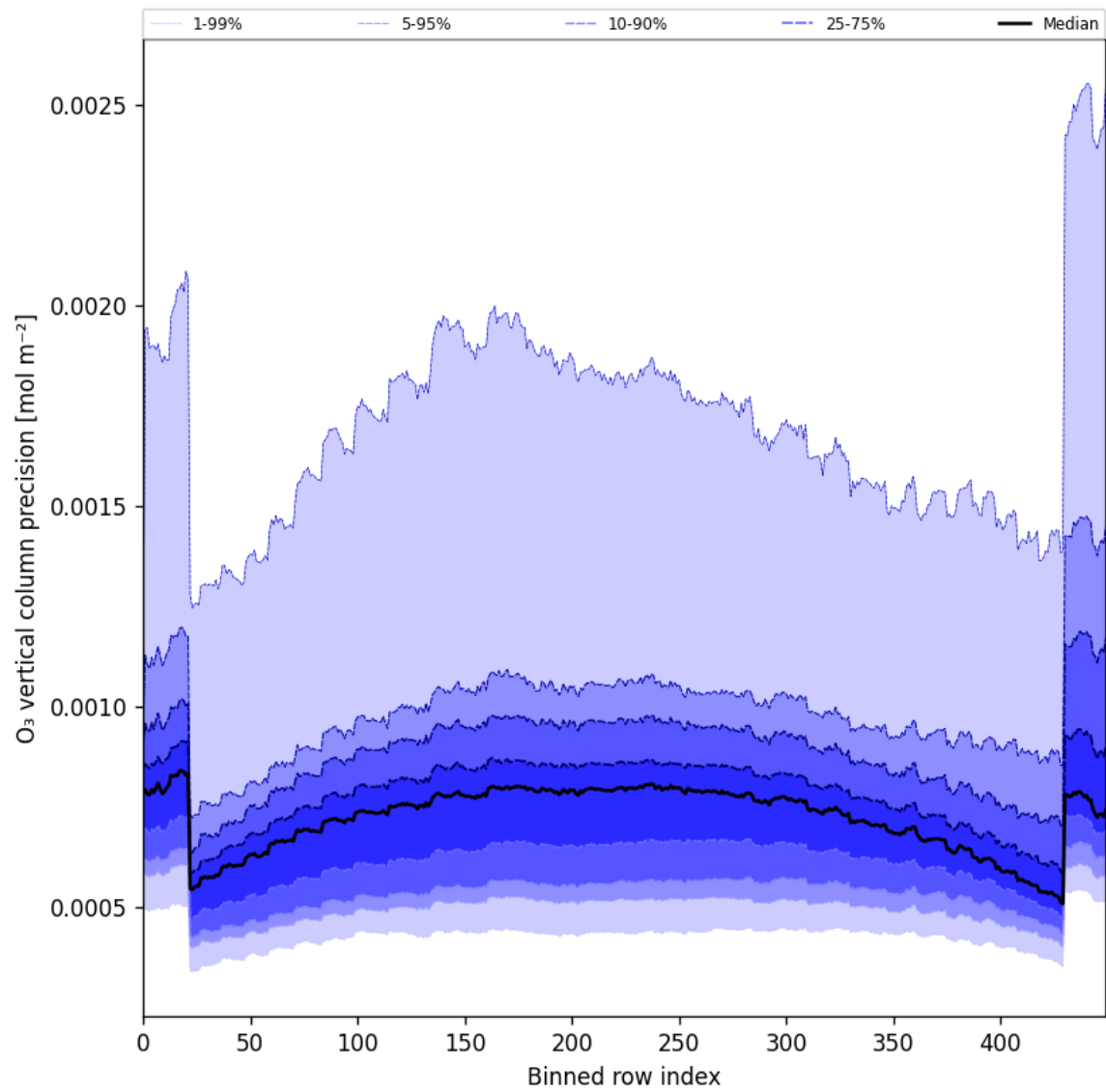
Figure 29: Along track statistics of “O 3 vertical column precision” for 2024-09-17 to 2024-09-19
