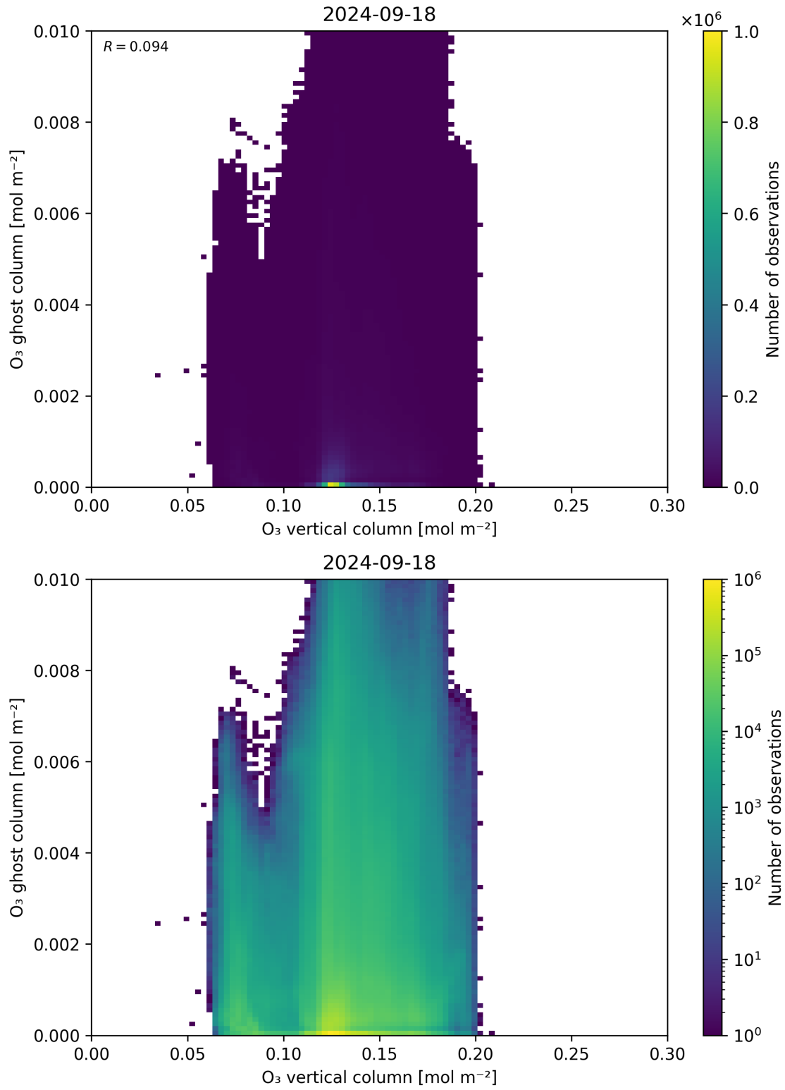
Figure 40: Scatter density plot of “O 3 vertical column” against “O 3 ghost column” for 2024-09-17 to 2024-09-19.
