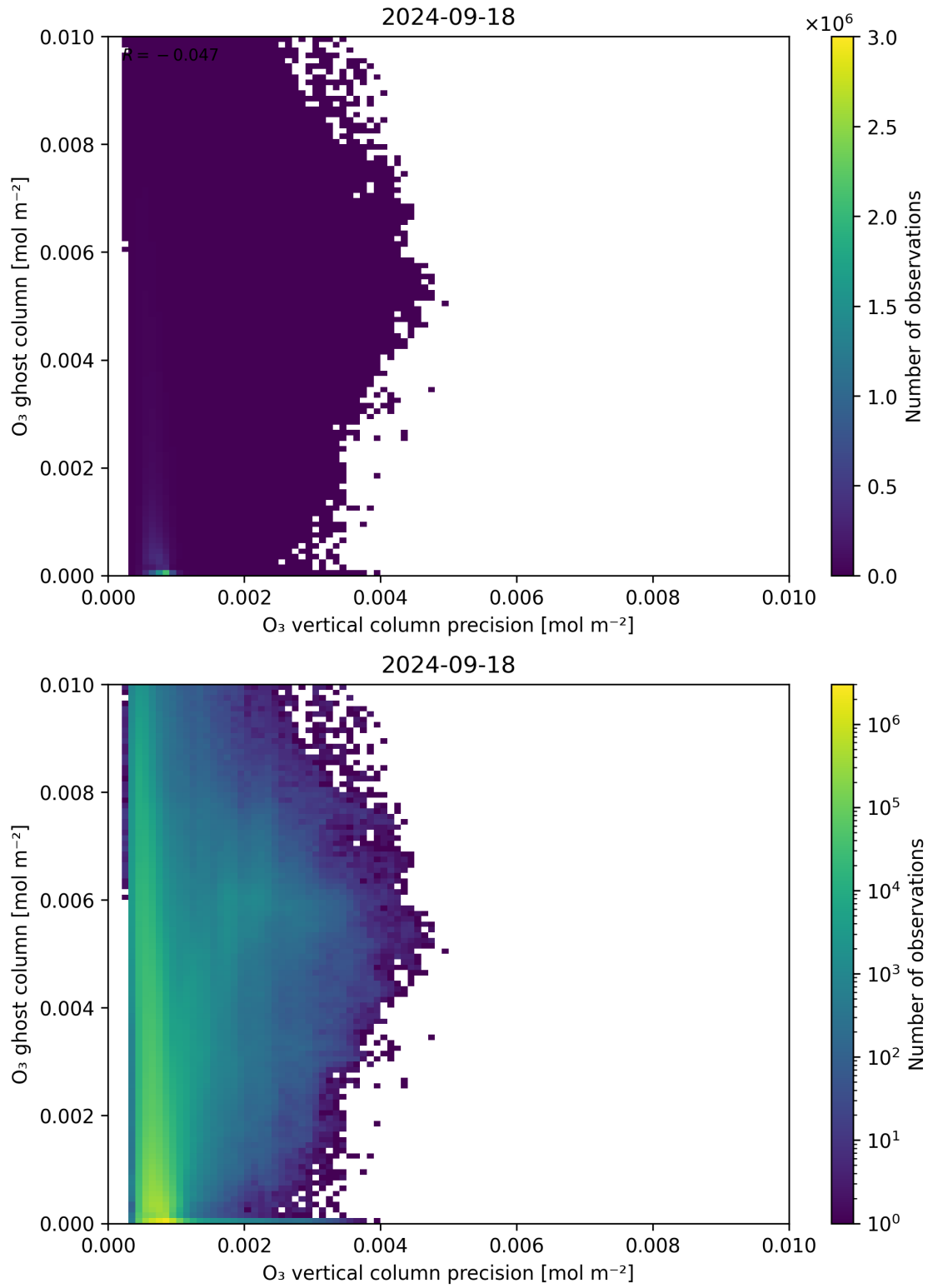
Figure 43: Scatter density plot of “O 3 vertical column precision” against “O 3 ghost column” for 2024-09-17 to 2024-09-19.
