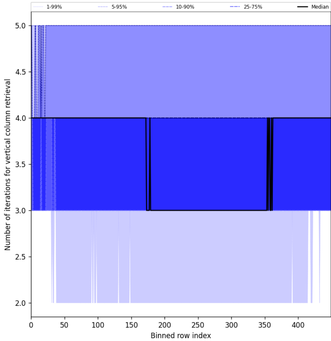
Figure 33: Along track statistics of “Number of iterations for vertical column retrieval” for 2024-09-17 to 2024-09-19
