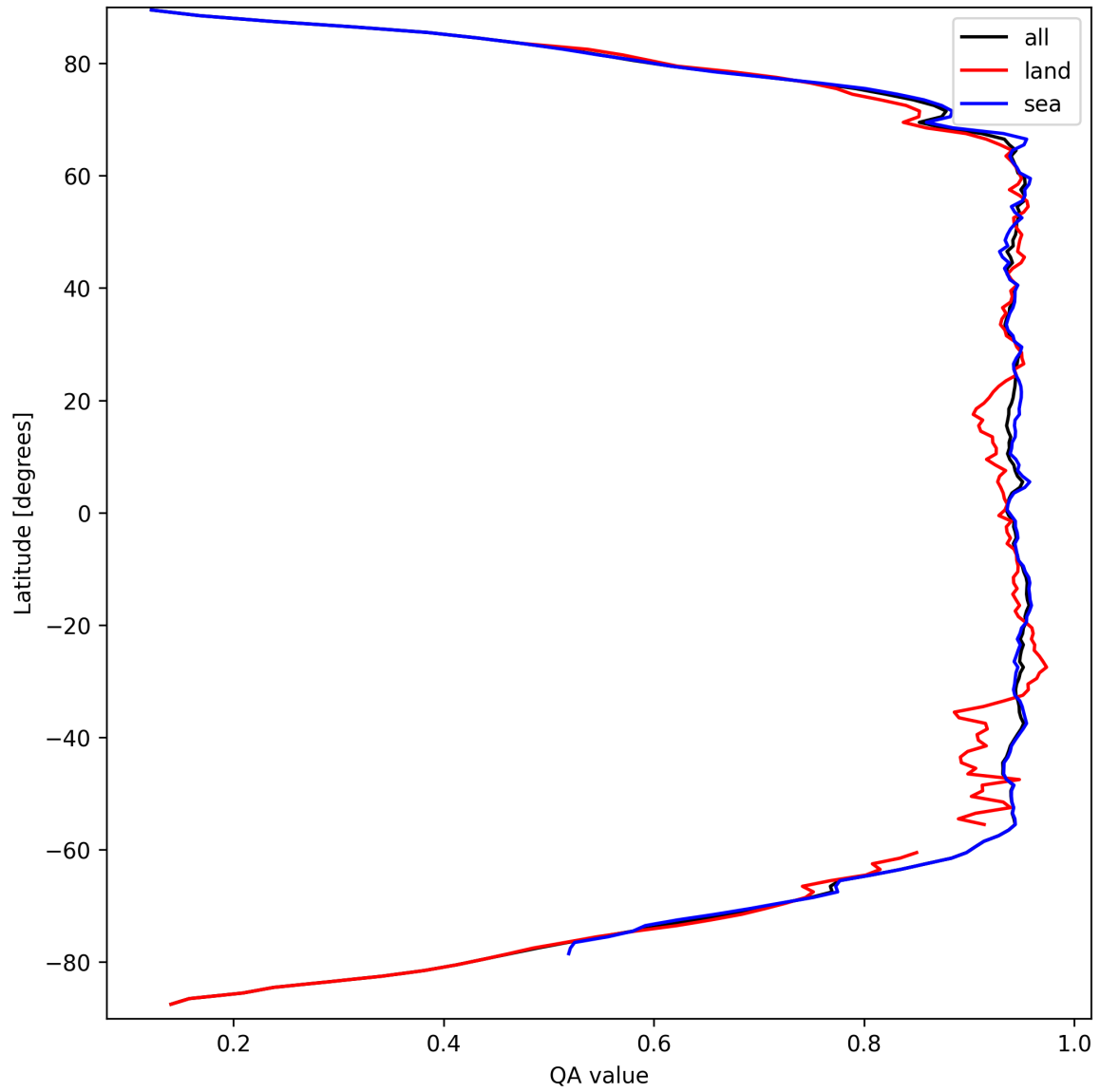
Figure 13: Zonal average of “QA value” for 2024-09-17 to 2024-09-19.
