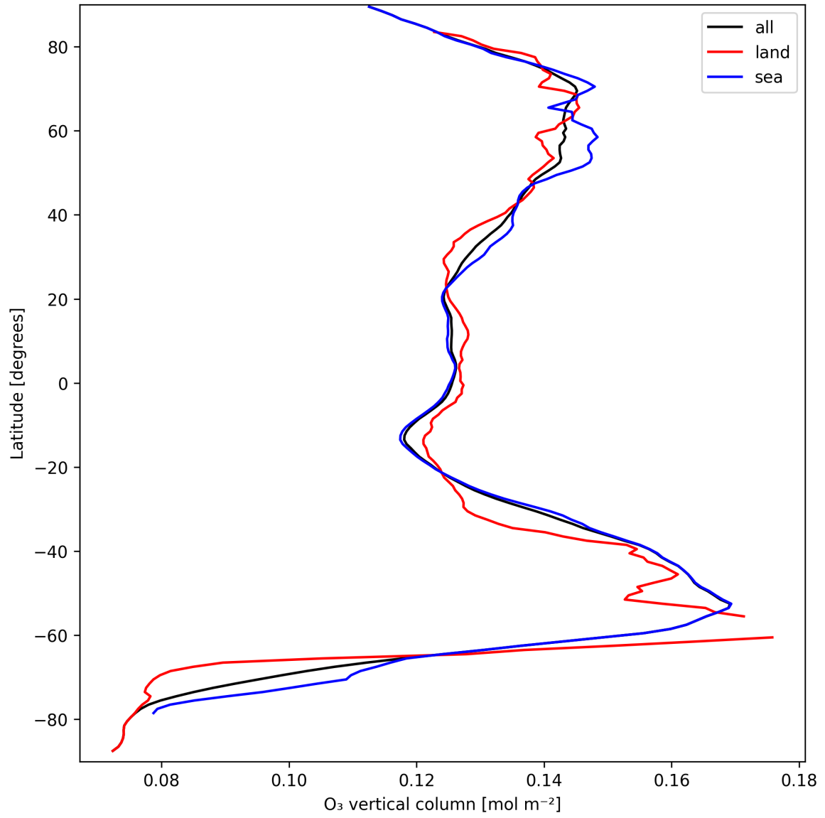
Figure 14: Zonal average of “O 3 vertical column” for 2024-09-17 to 2024-09-19.
