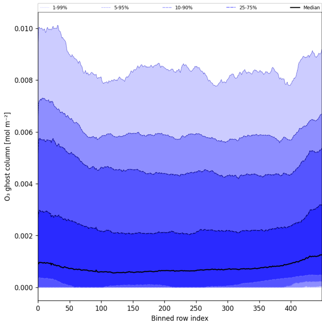
Figure 32: Along track statistics of “O 3 ghost column” for 2024-09-17 to 2024-09-19
