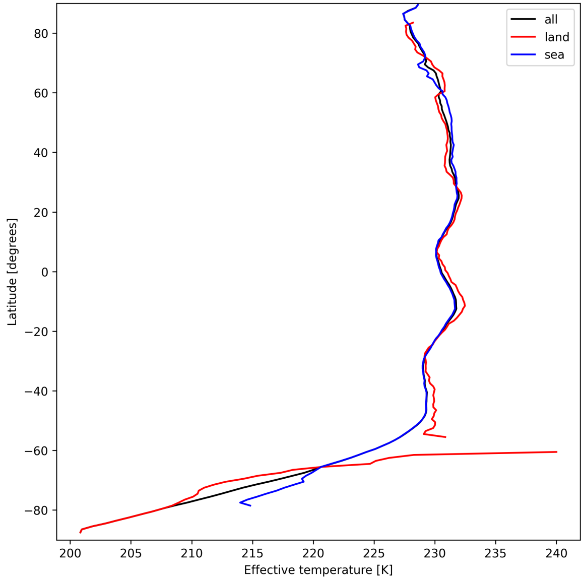
Figure 17: Zonal average of "Effective temperature" for 2024-09-17 to 2024-09-19.
