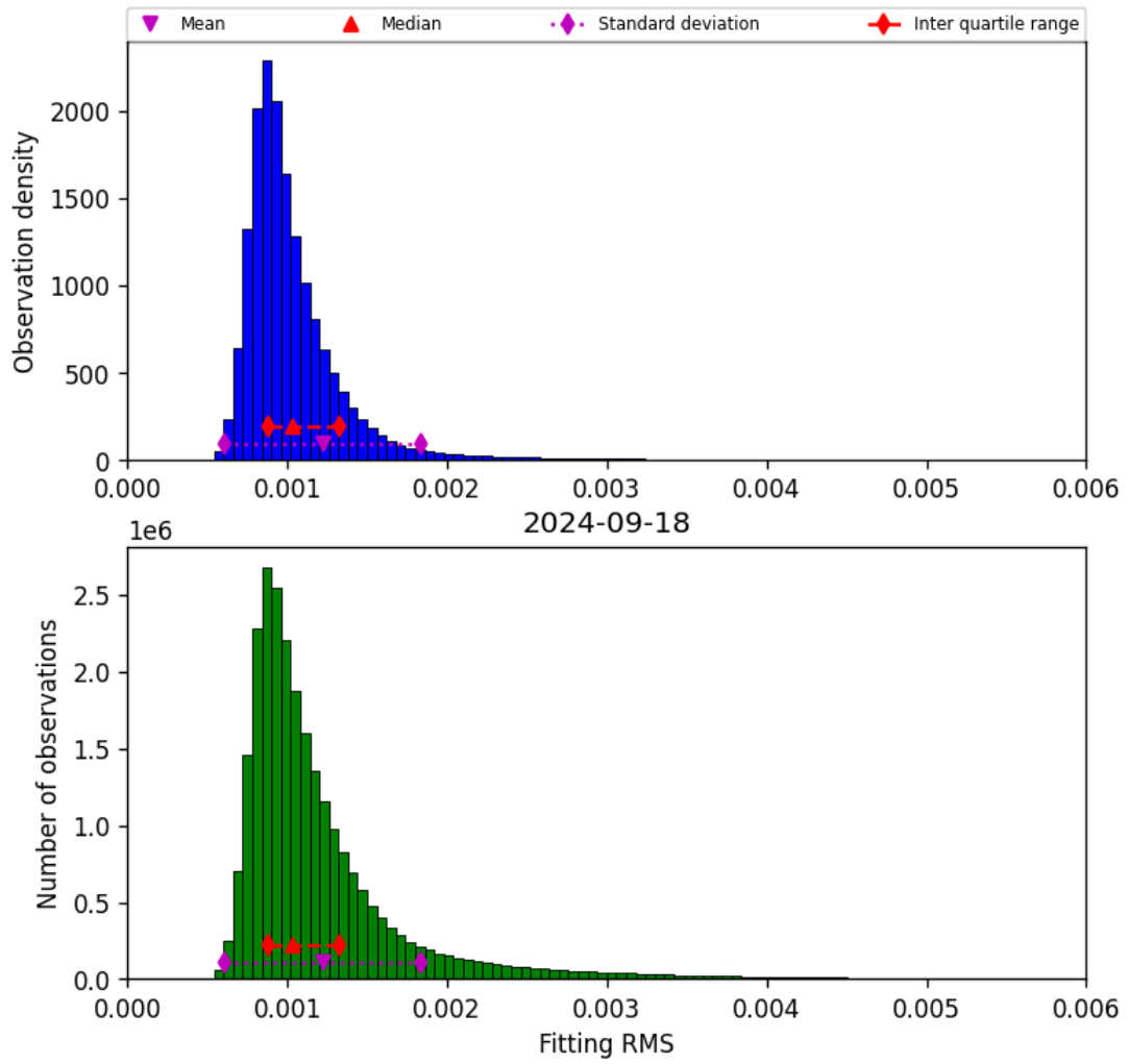
Figure 23: Histogram of “Fitting RMS” for 2024-09-17 to 2024-09-19
