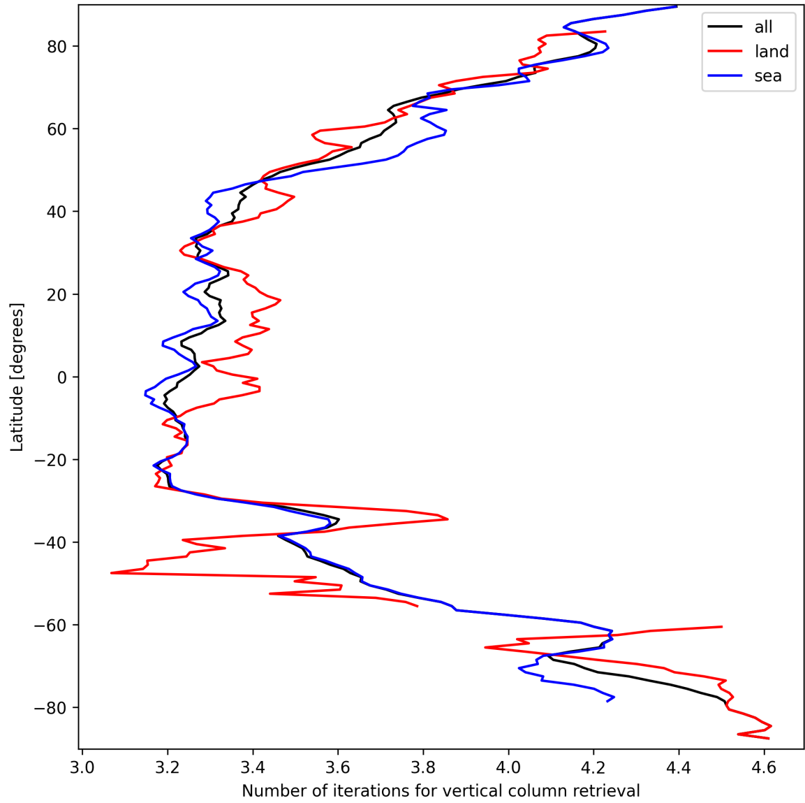
Figure 19: Zonal average of “Number of iterations for vertical column retrieval” for 2024-09-17 to 2024-09-19.
