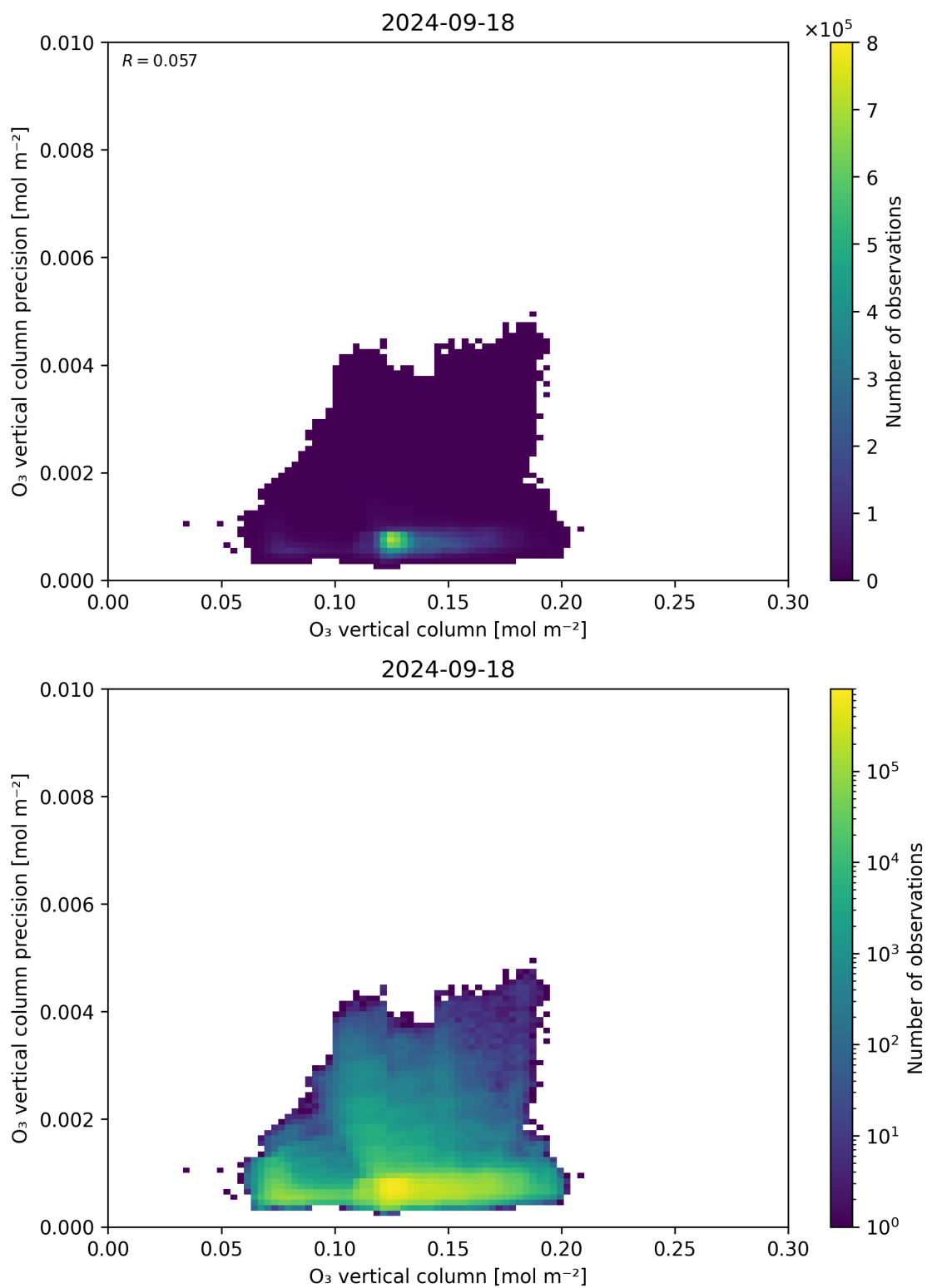
Figure 41: Scatter density plot of “O 3 vertical column” against “O 3 vertical column precision” for 2024-09-17 to 2024-09-19.
