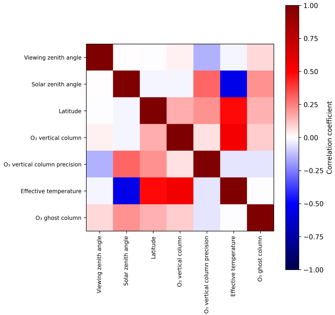
Figure 2: Map of correlation matrix for 2024-09-17 to 2024-09-19.
