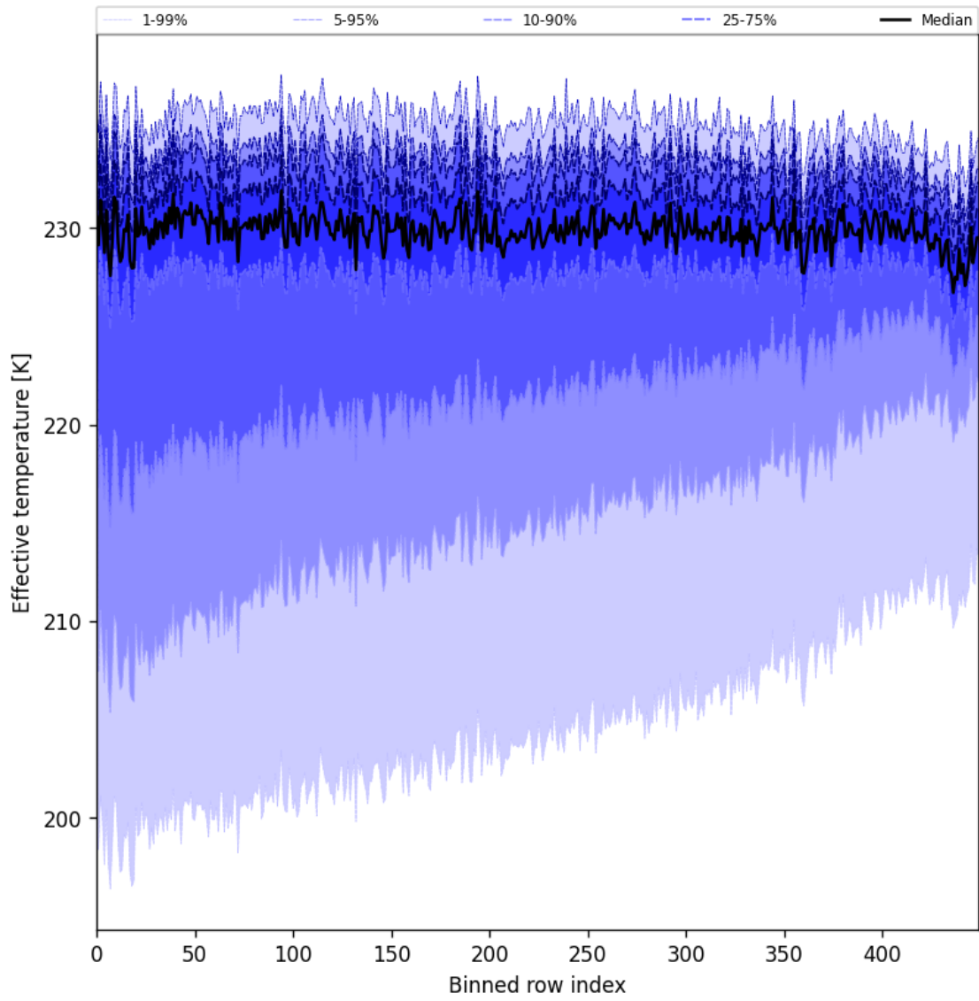
Figure 31: Along track statistics of “Effective temperature” for 2024-09-17 to 2024-09-19
