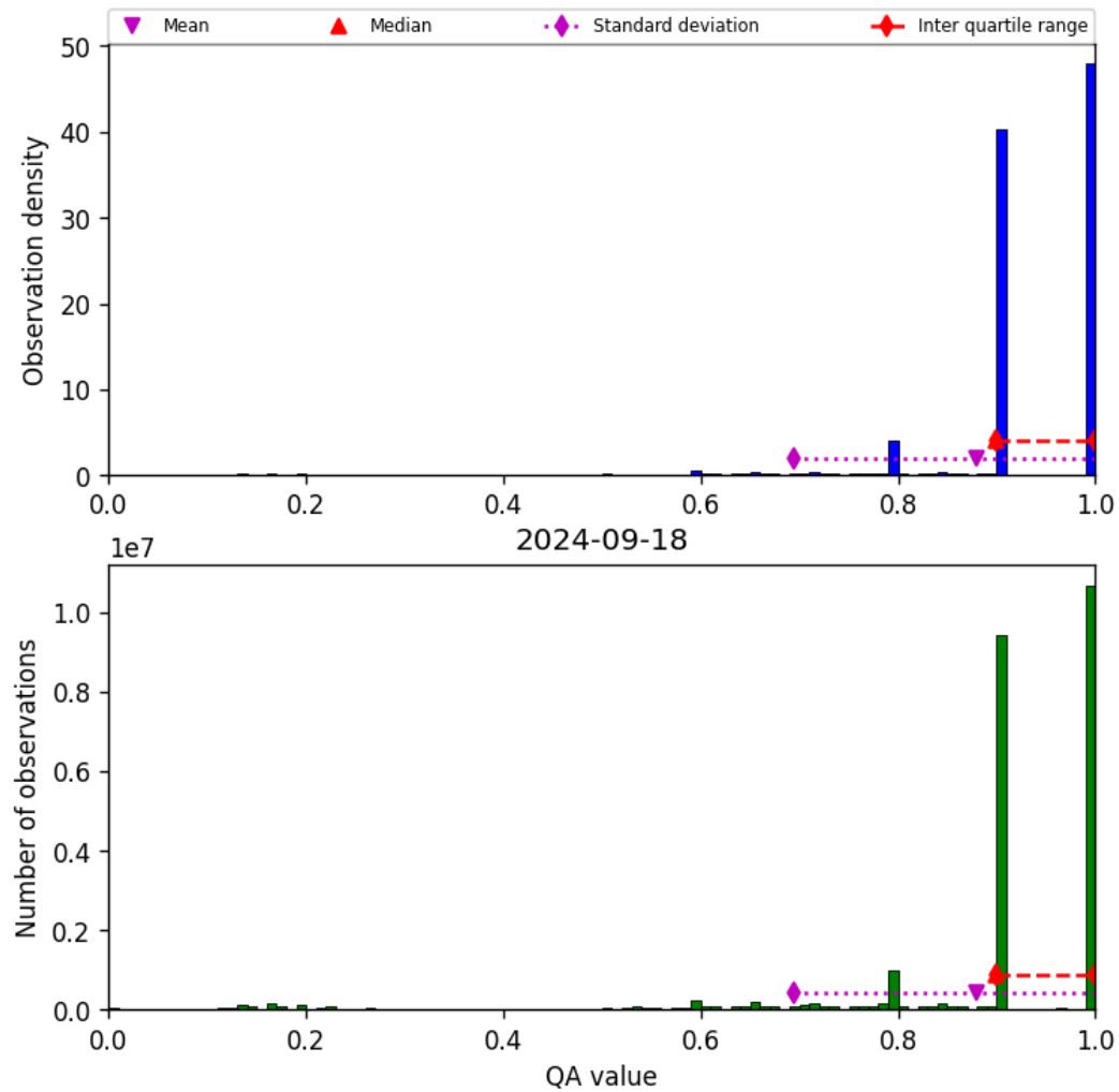
Figure 20: Histogram of “QA value” for 2024-09-17 to 2024-09-19
