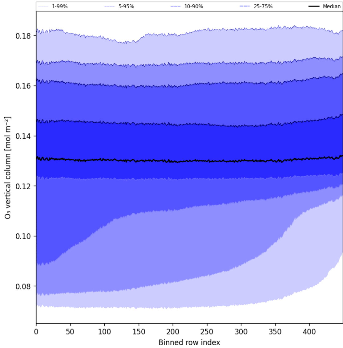
Figure 28: Along track statistics of “O 3 vertical column” for 2024-09-17 to 2024-09-19
