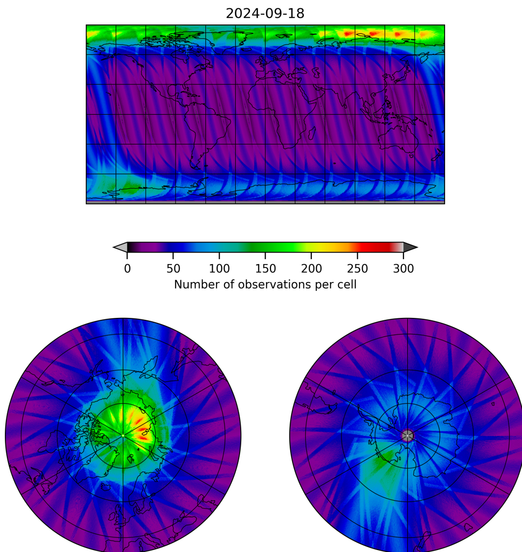
Figure 12: Map of the number of observations for 2024-09-17 to 2024-09-19
