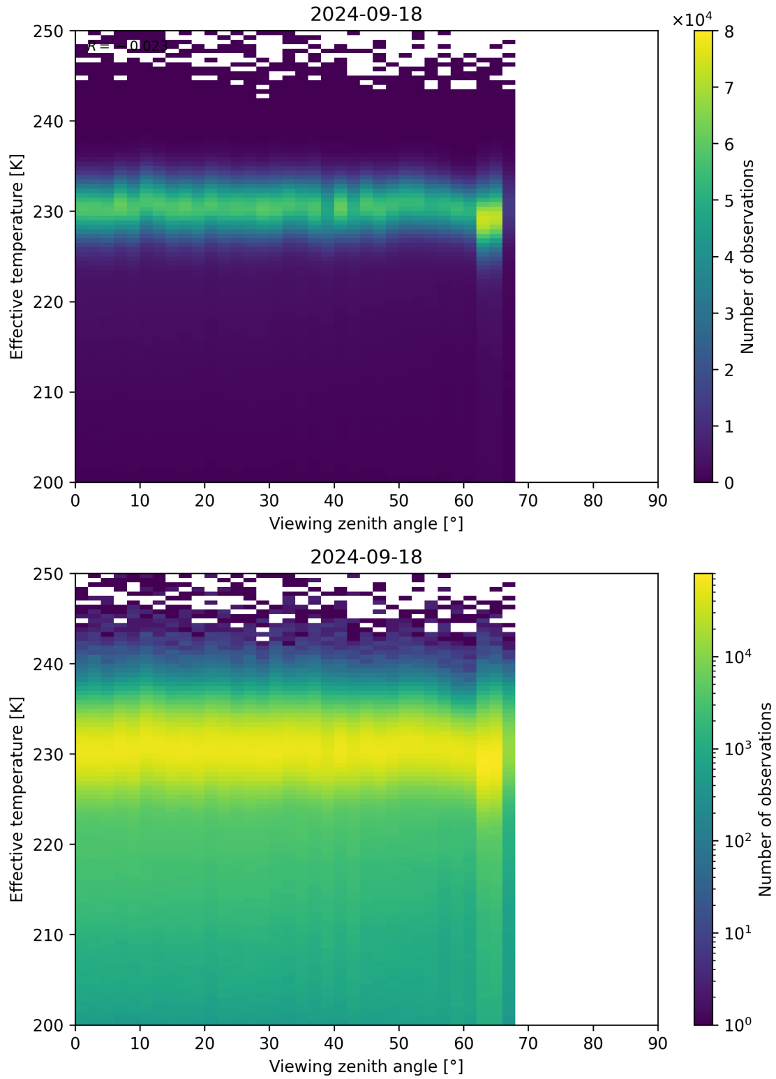
Figure 50: Scatter density plot of “Viewing zenith angle” against “Effective temperature” for 2024-09-17 to 2024-09-19.
