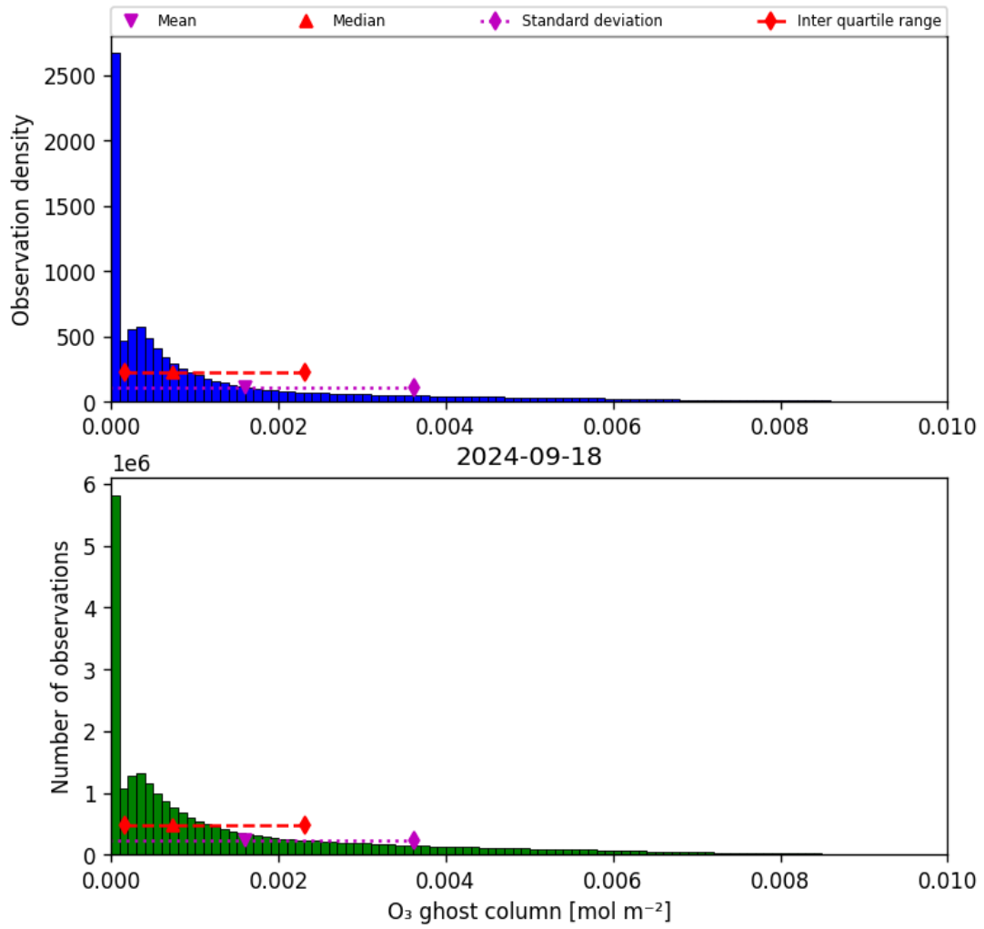
Figure 25: Histogram of "O 3 ghost column" for 2024-09-17 to 2024-09-19
