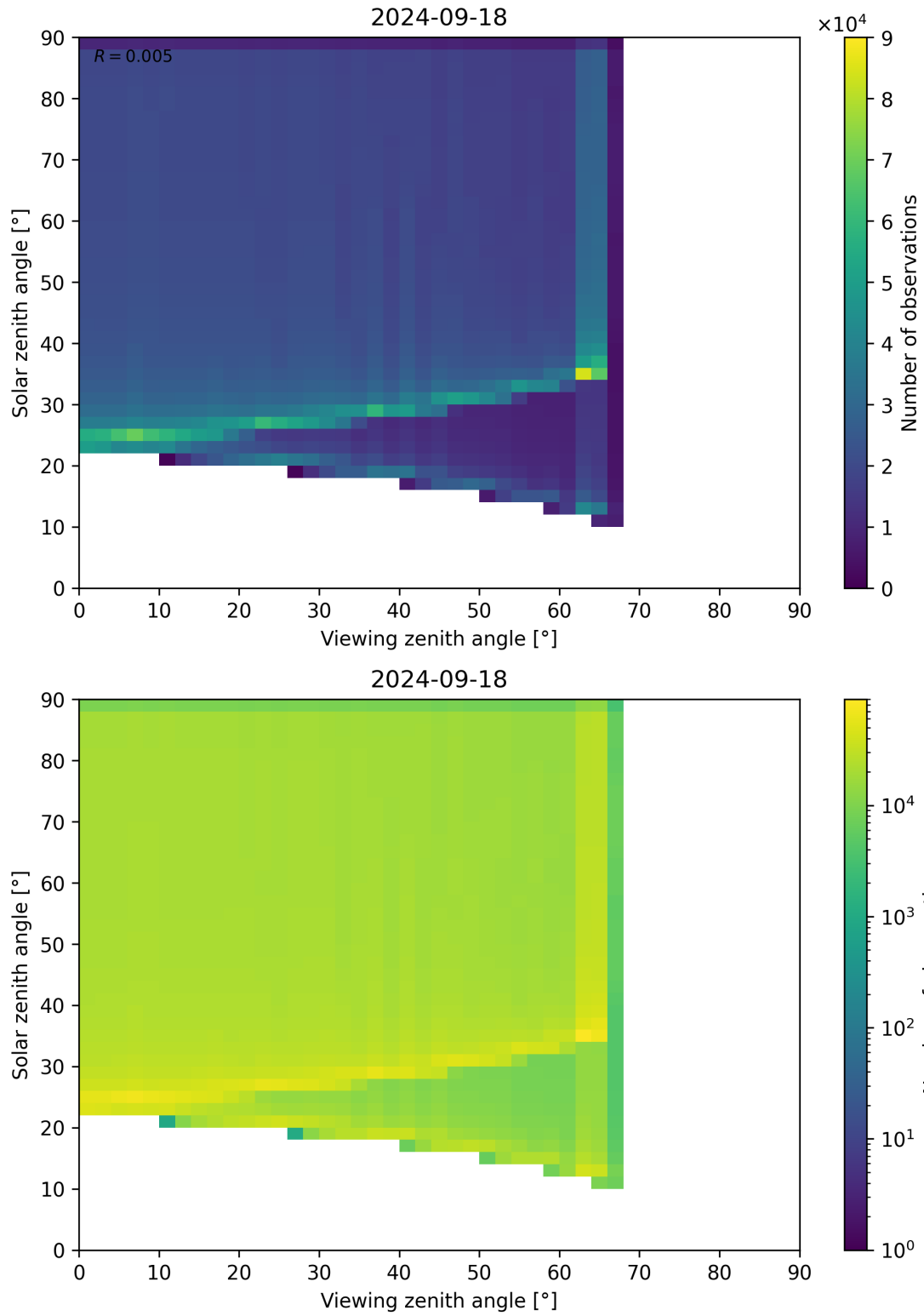
Figure 54: Scatter density plot of “Viewing zenith angle” against “Solar zenith angle” for 2024-09-17 to 2024-09-19.
