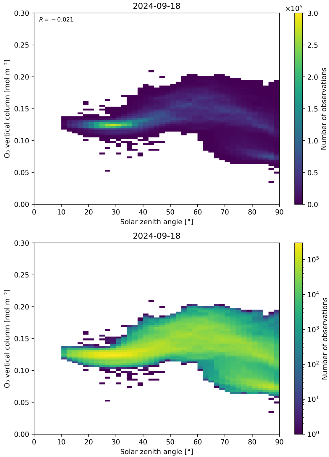
Figure 47: Scatter density plot of “Solar zenith angle” against “O 3 vertical column” for 2024-09-17 to 2024-09-19.
