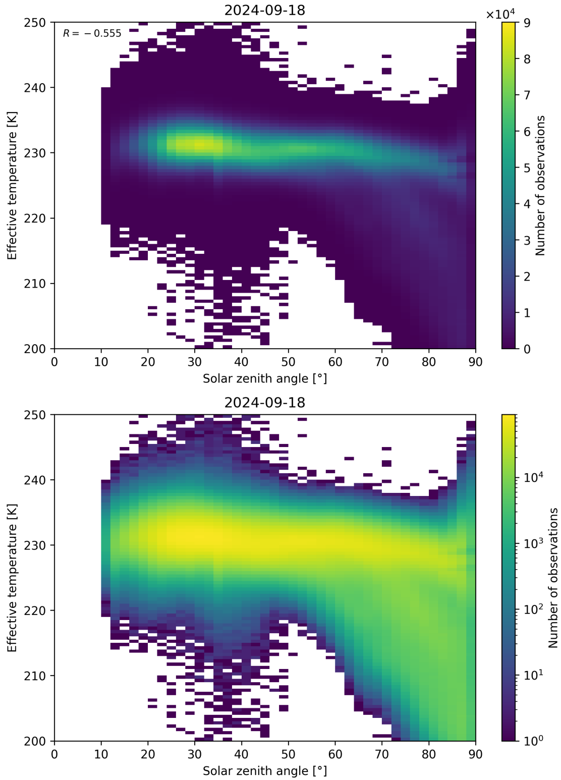
Figure 45: Scatter density plot of “Solar zenith angle” against “Effective temperature” for 2024-09-17 to 2024-09-19.
