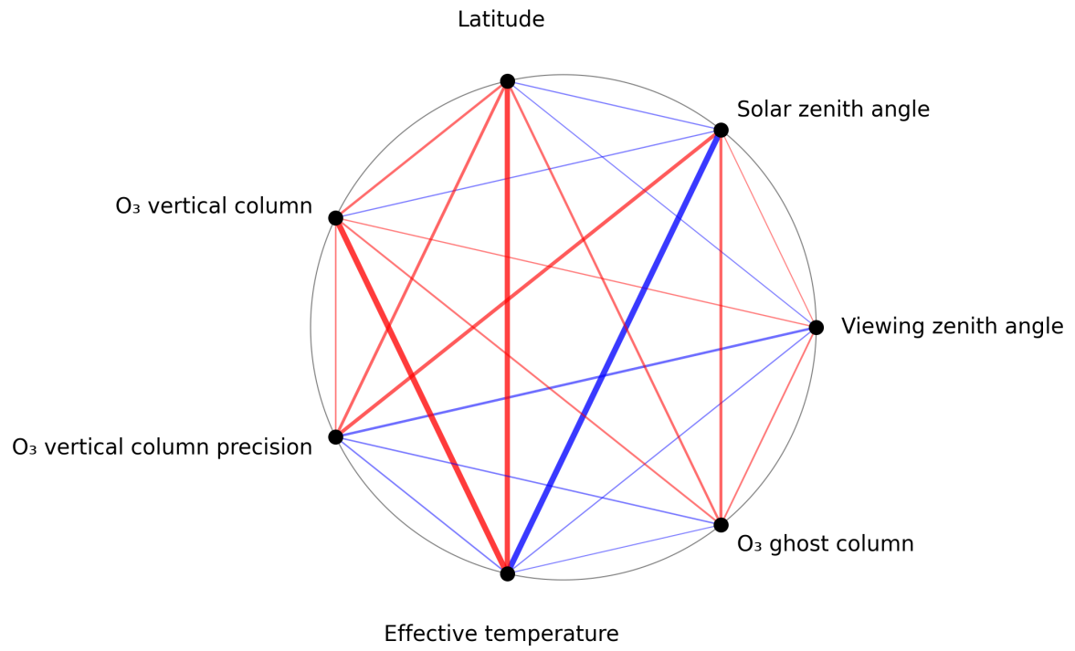
Figure 1: Map of correlation graph for 2024-09-17 to 2024-09-19.
