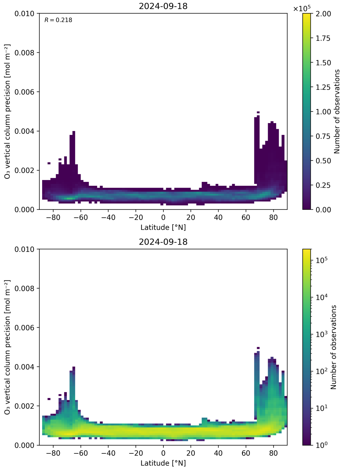
Figure 37: Scatter density plot of “Latitude” against “O 3 vertical column precision” for 2024-09-17 to 2024-09-19.
