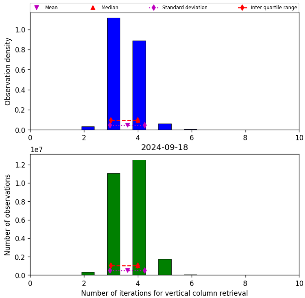
Figure 26: Histogram of “Number of iterations for vertical column retrieval” for 2024-09-17 to 2024-09-19
