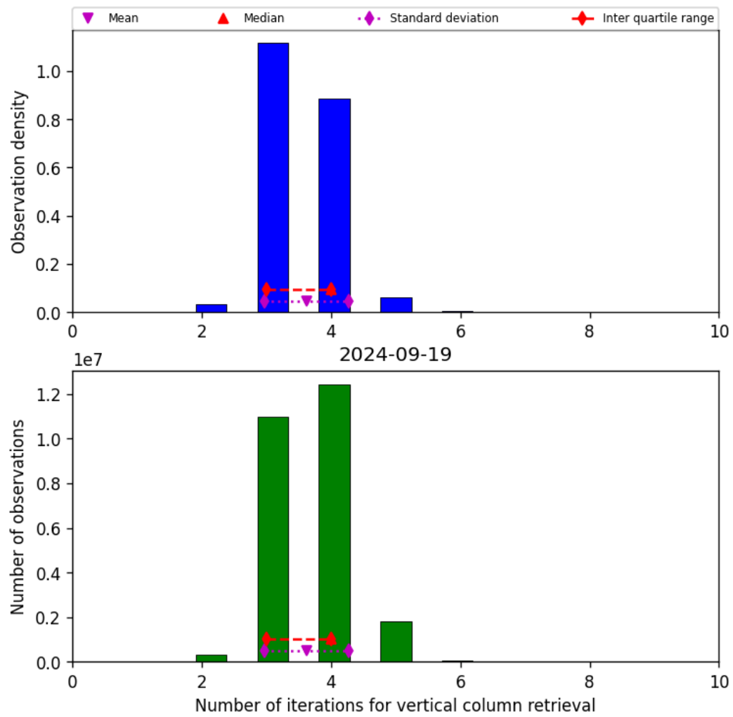
Figure 26: Histogram of “Number of iterations for vertical column retrieval” for 2024-09-18 to 2024-09-20
