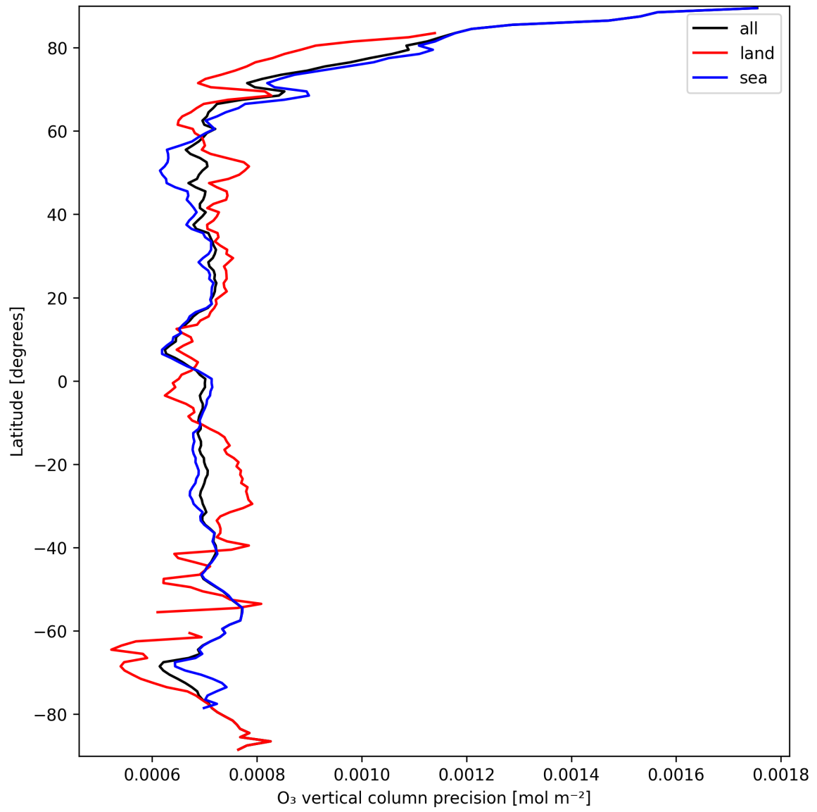
Figure 15: Zonal average of “O 3 vertical column precision” for 2024-09-18 to 2024-09-20.
