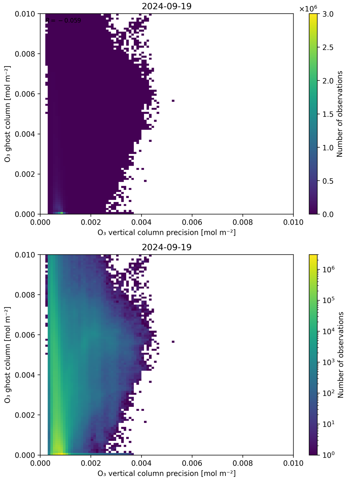
Figure 43: Scatter density plot of “O 3 vertical column precision” against “O 3 ghost column” for 2024-09-18 to 2024-09-20.
