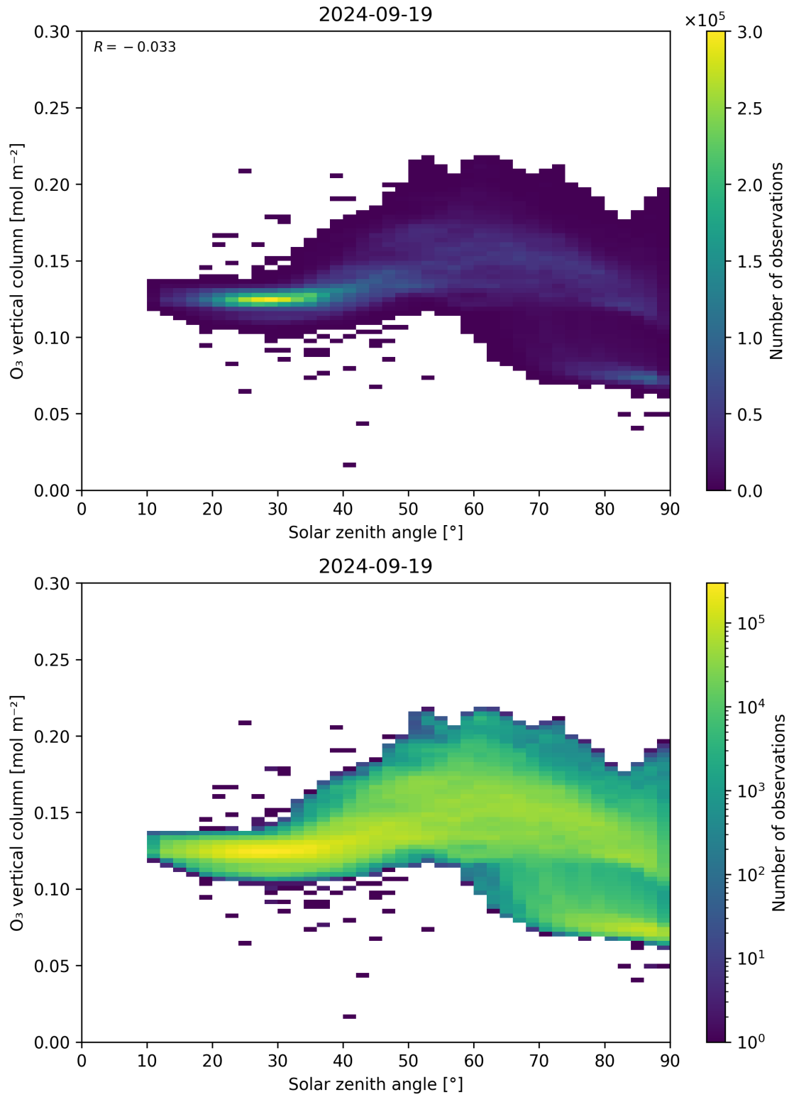
Figure 47: Scatter density plot of “Solar zenith angle” against “O 3 vertical column” for 2024-09-18 to 2024-09-20.
