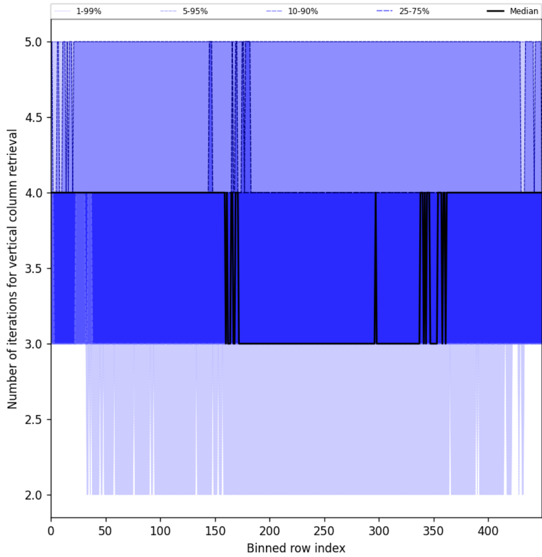
Figure 33: Along track statistics of “Number of iterations for vertical column retrieval” for 2024-09-18 to 2024-09-20
