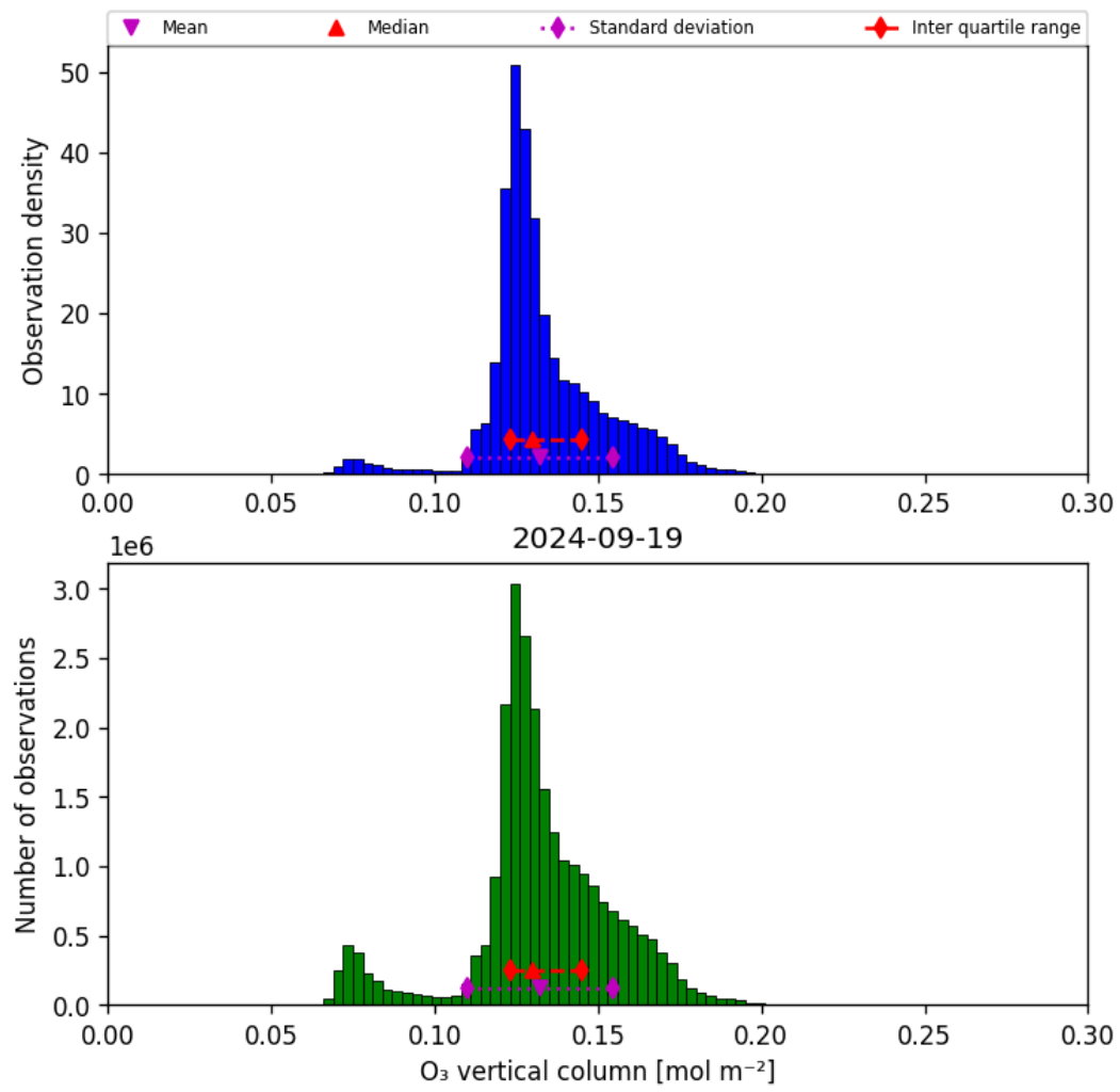
Figure 21: Histogram of “O 3 vertical column” for 2024-09-18 to 2024-09-20
