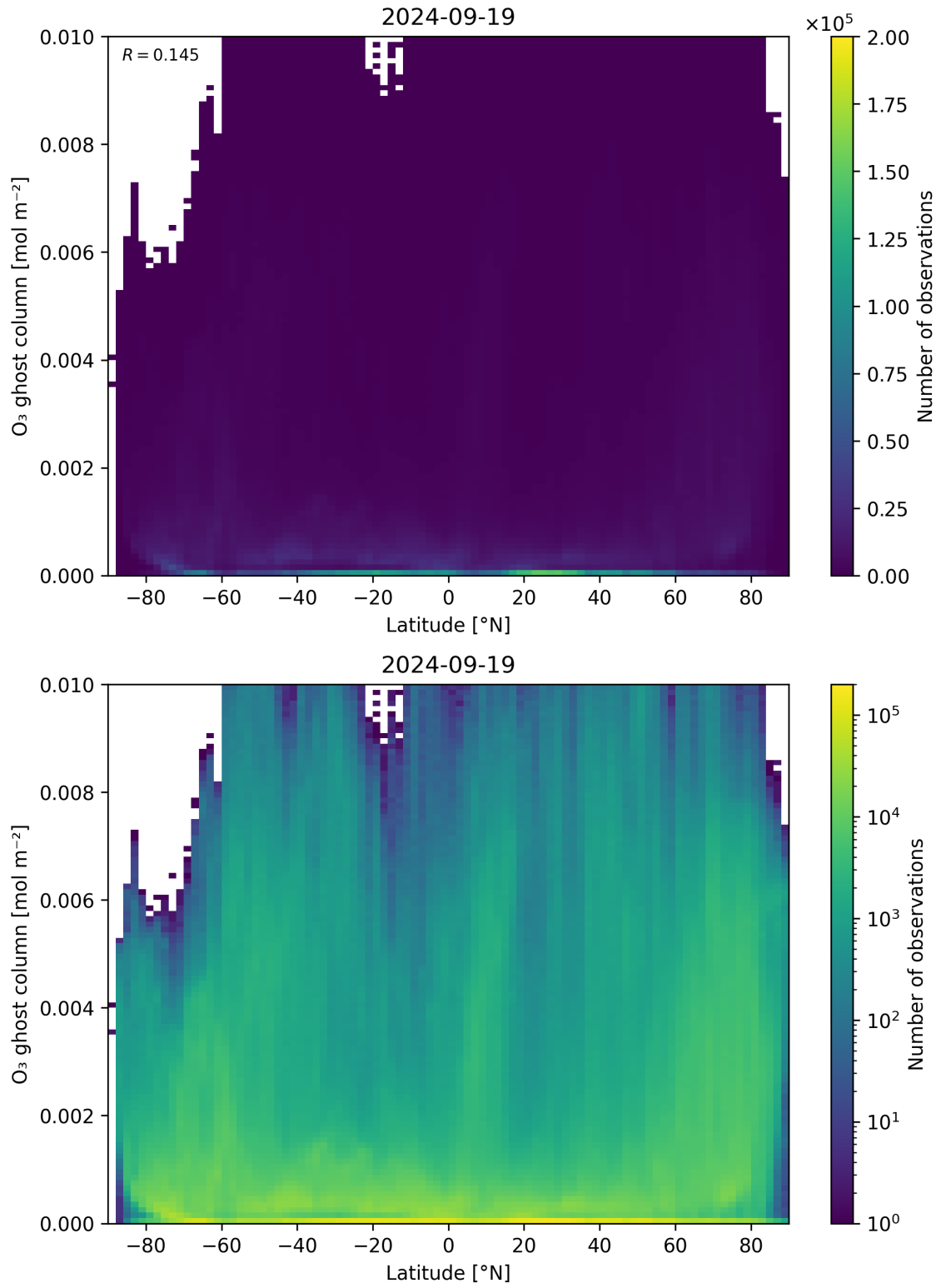
Figure 35: Scatter density plot of “Latitude” against “O 3 ghost column” for 2024-09-18 to 2024-09-20.
