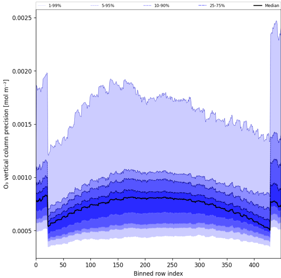
Figure 29: Along track statistics of “O 3 vertical column precision” for 2024-09-18 to 2024-09-20
