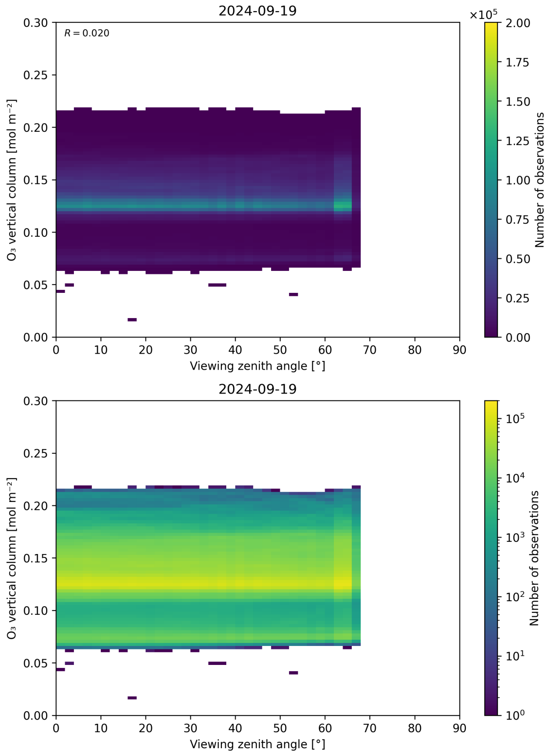
Figure 52: Scatter density plot of “Viewing zenith angle” against “O 3 vertical column” for 2024-09-18 to 2024-09-20.
