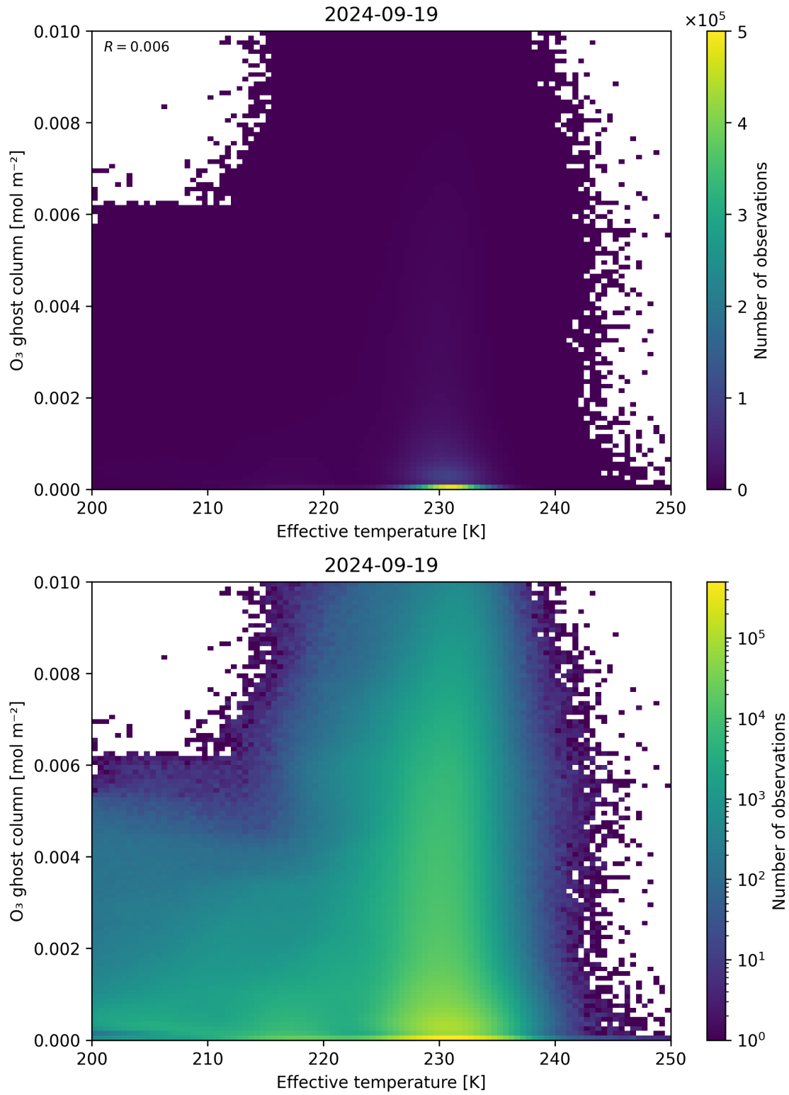
Figure 38: Scatter density plot of “Effective temperature” against “O 3 ghost column” for 2024-09-18 to 2024-09-20.
