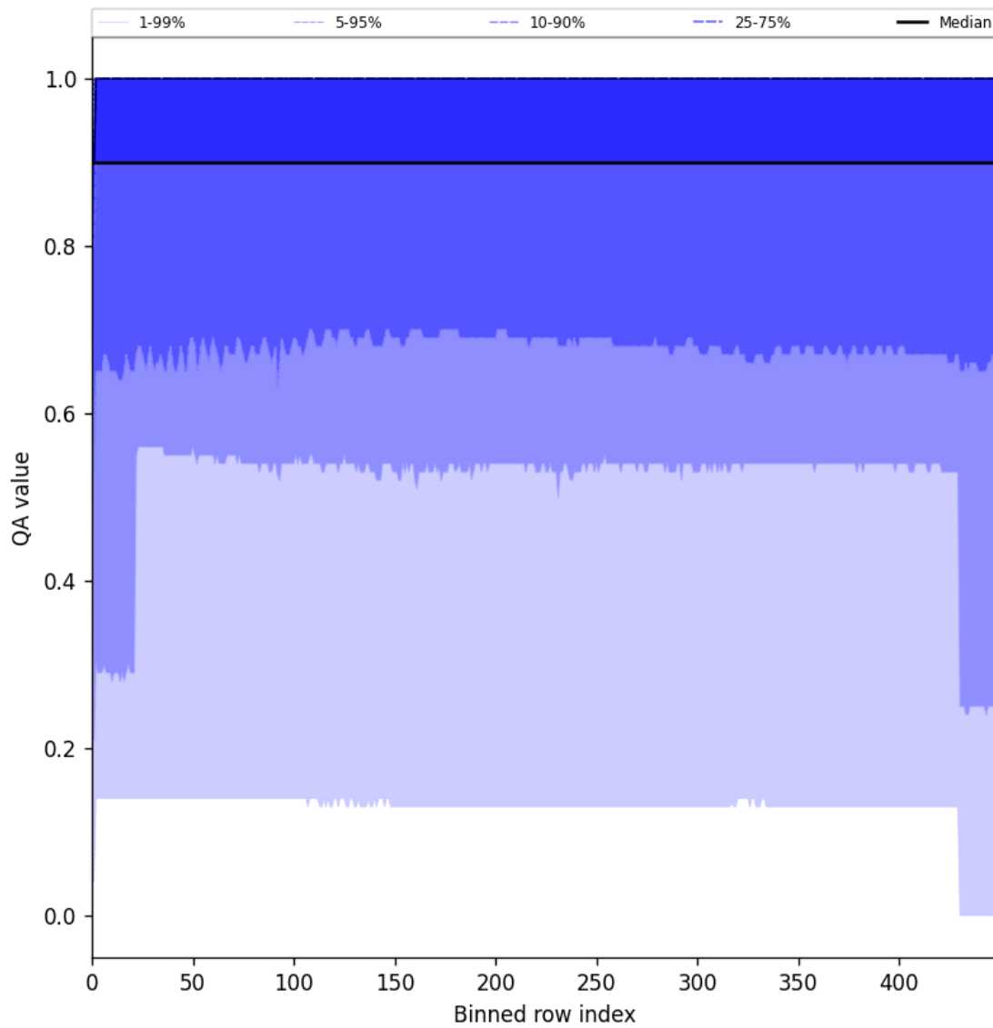
Figure 27: Along track statistics of “QA value” for 2024-09-18 to 2024-09-20
