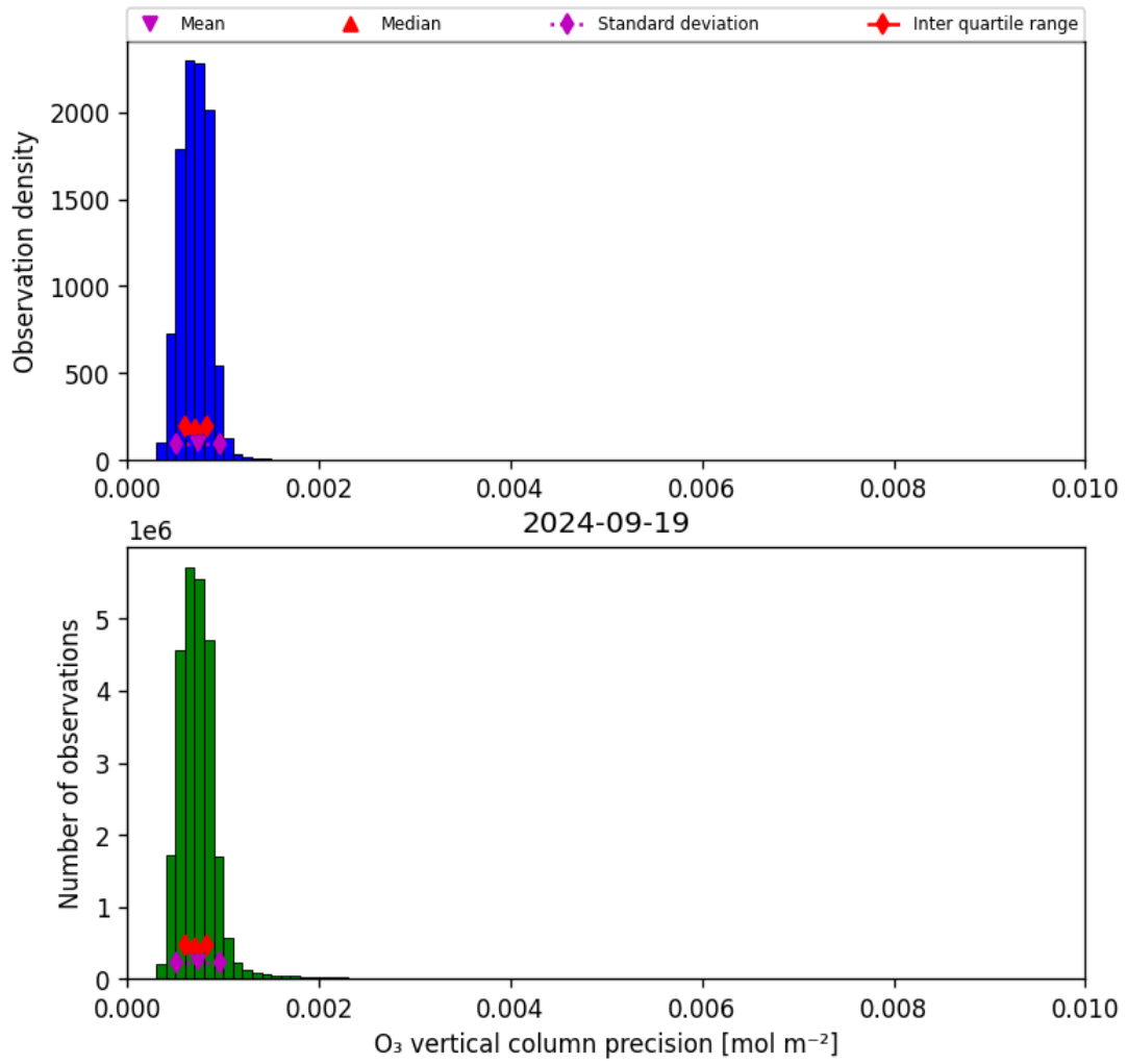
Figure 22: Histogram of “O 3 vertical column precision” for 2024-09-18 to 2024-09-20
