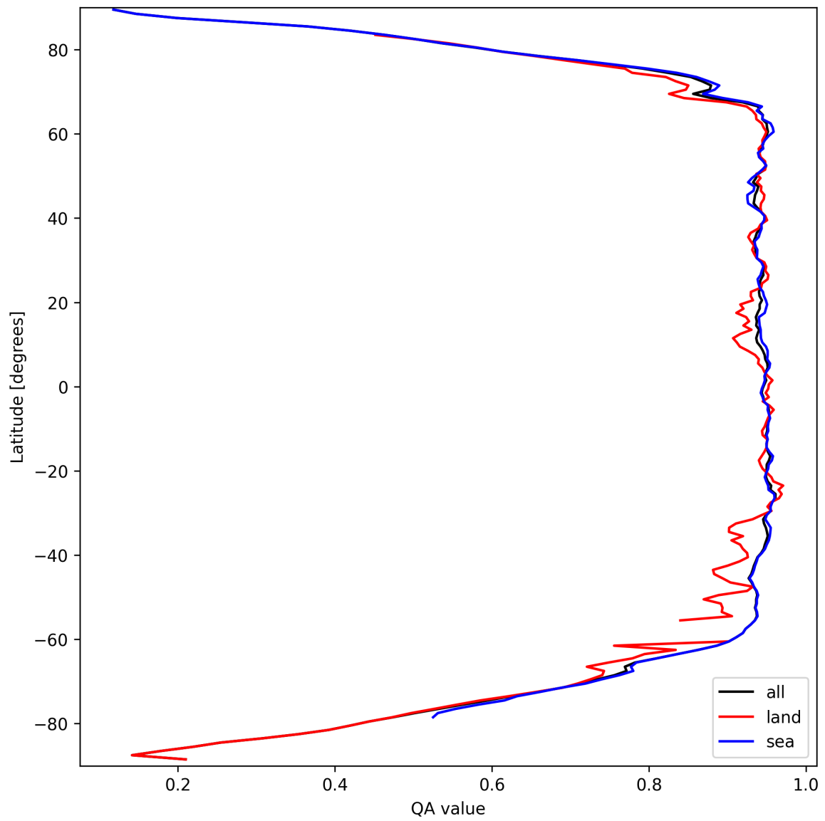
Figure 13: Zonal average of “QA value” for 2024-09-18 to 2024-09-20.
