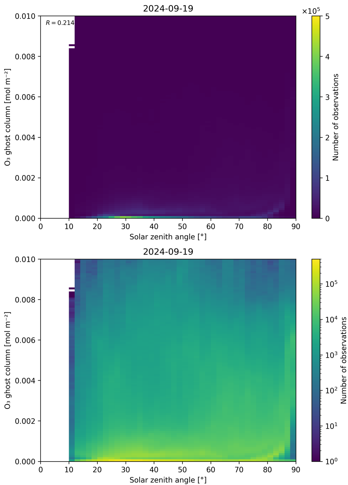
Figure 46: Scatter density plot of “Solar zenith angle” against “O 3 ghost column” for 2024-09-18 to 2024-09-20.
