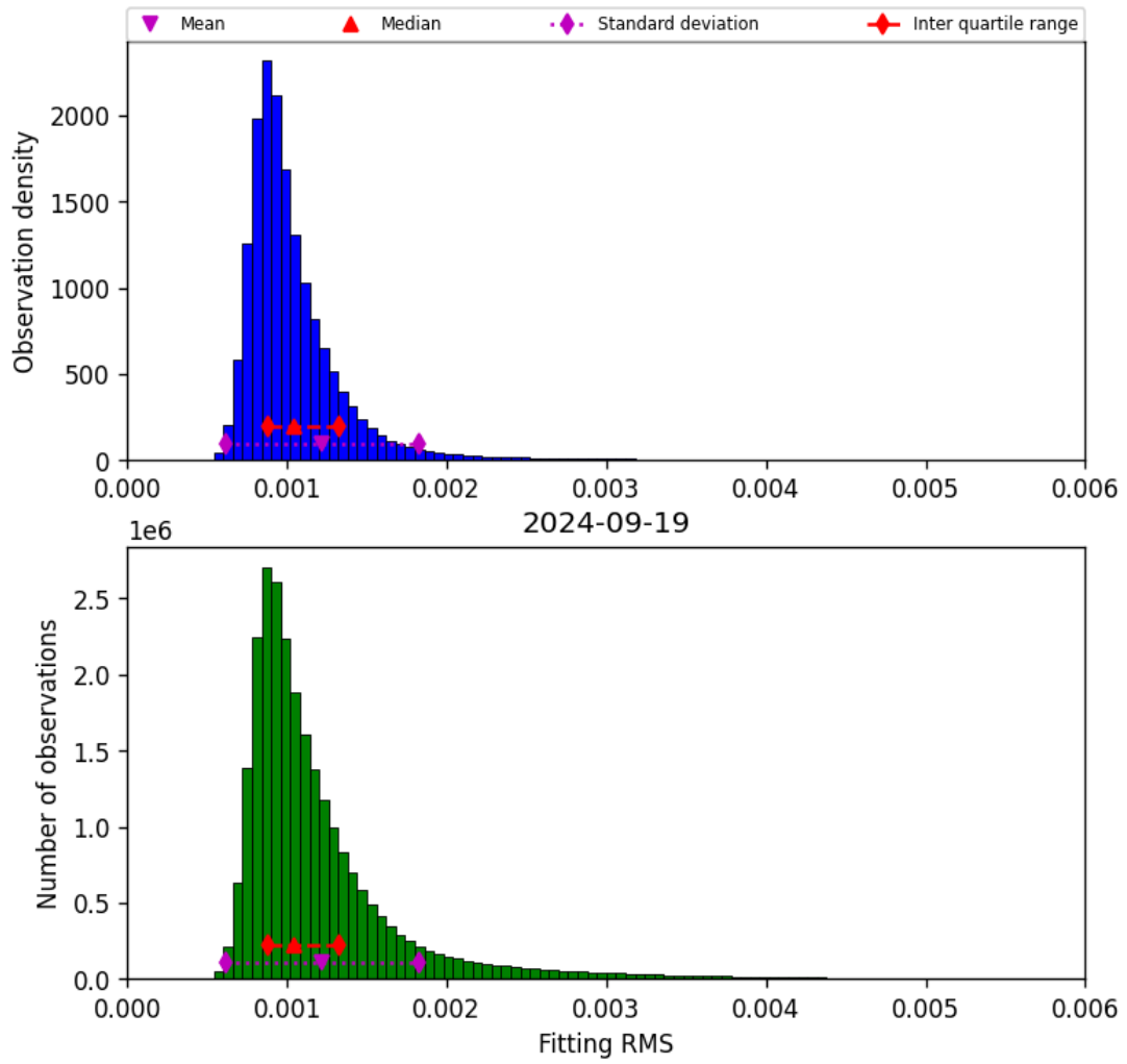
Figure 23: Histogram of “Fitting RMS” for 2024-09-18 to 2024-09-20
