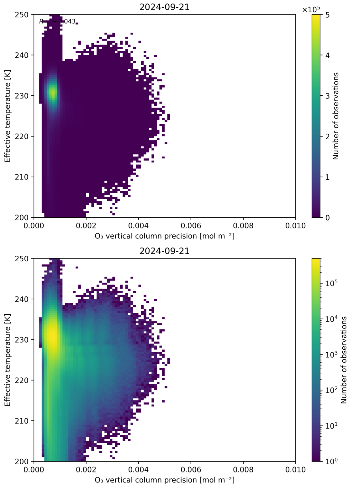
Figure 42: Scatter density plot of “O 3 vertical column precision” against “Effective temperature” for 2024-09-20 to 2024-09-22.
