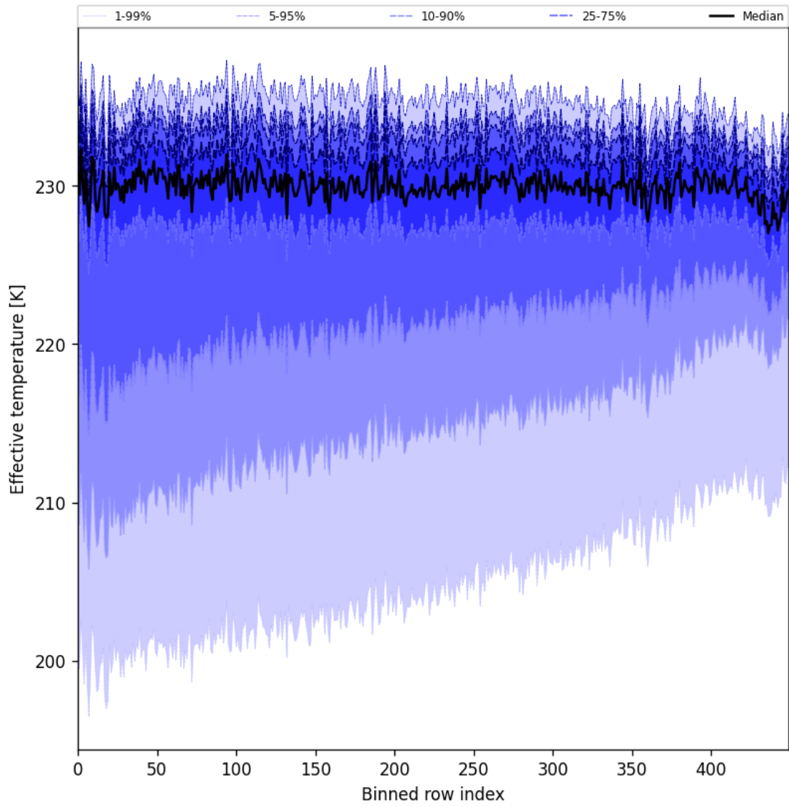
Figure 31: Along track statistics of “Effective temperature” for 2024-09-20 to 2024-09-22
