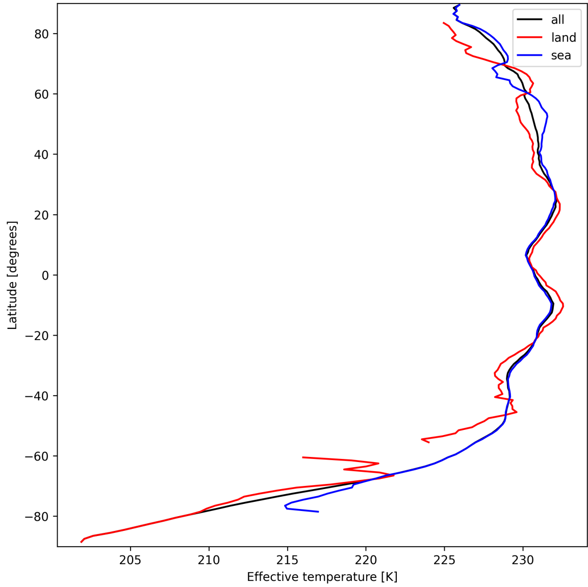
Figure 17: Zonal average of “Effective temperature” for 2024-09-20 to 2024-09-22.
