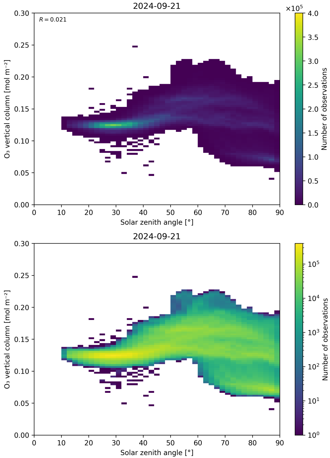
Figure 47: Scatter density plot of “Solar zenith angle” against “O 3 vertical column” for 2024-09-20 to 2024-09-22.
