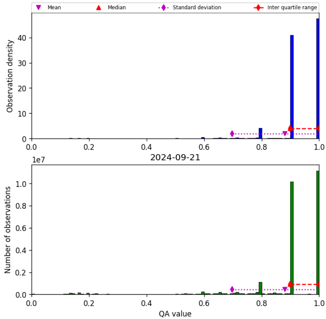
Figure 20: Histogram of “QA value” for 2024-09-20 to 2024-09-22
