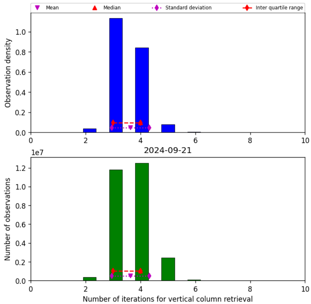
Figure 26: Histogram of “Number of iterations for vertical column retrieval” for 2024-09-20 to 2024-09-22
