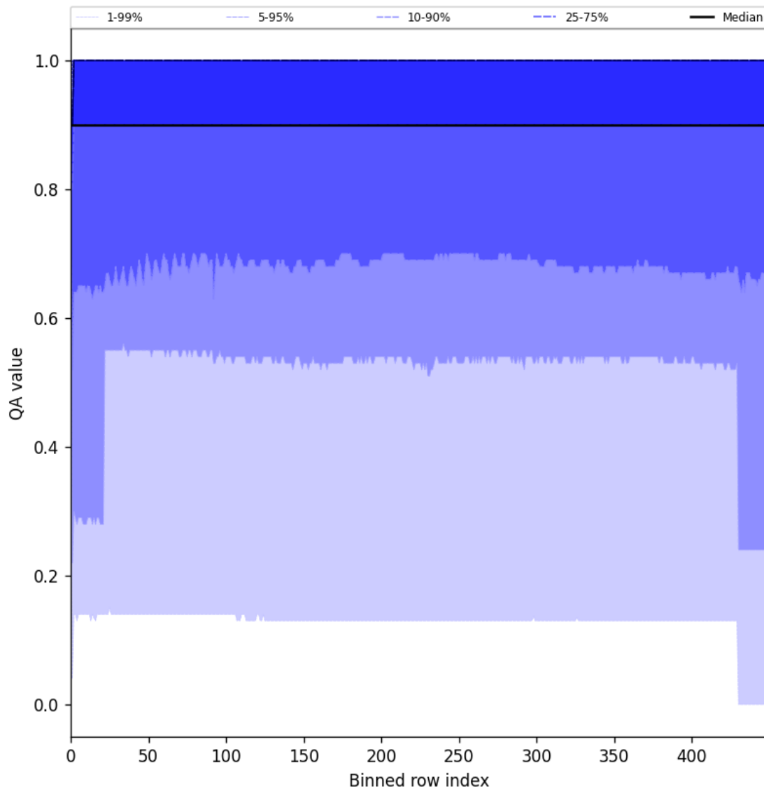
Figure 27: Along track statistics of “QA value” for 2024-09-20 to 2024-09-22
