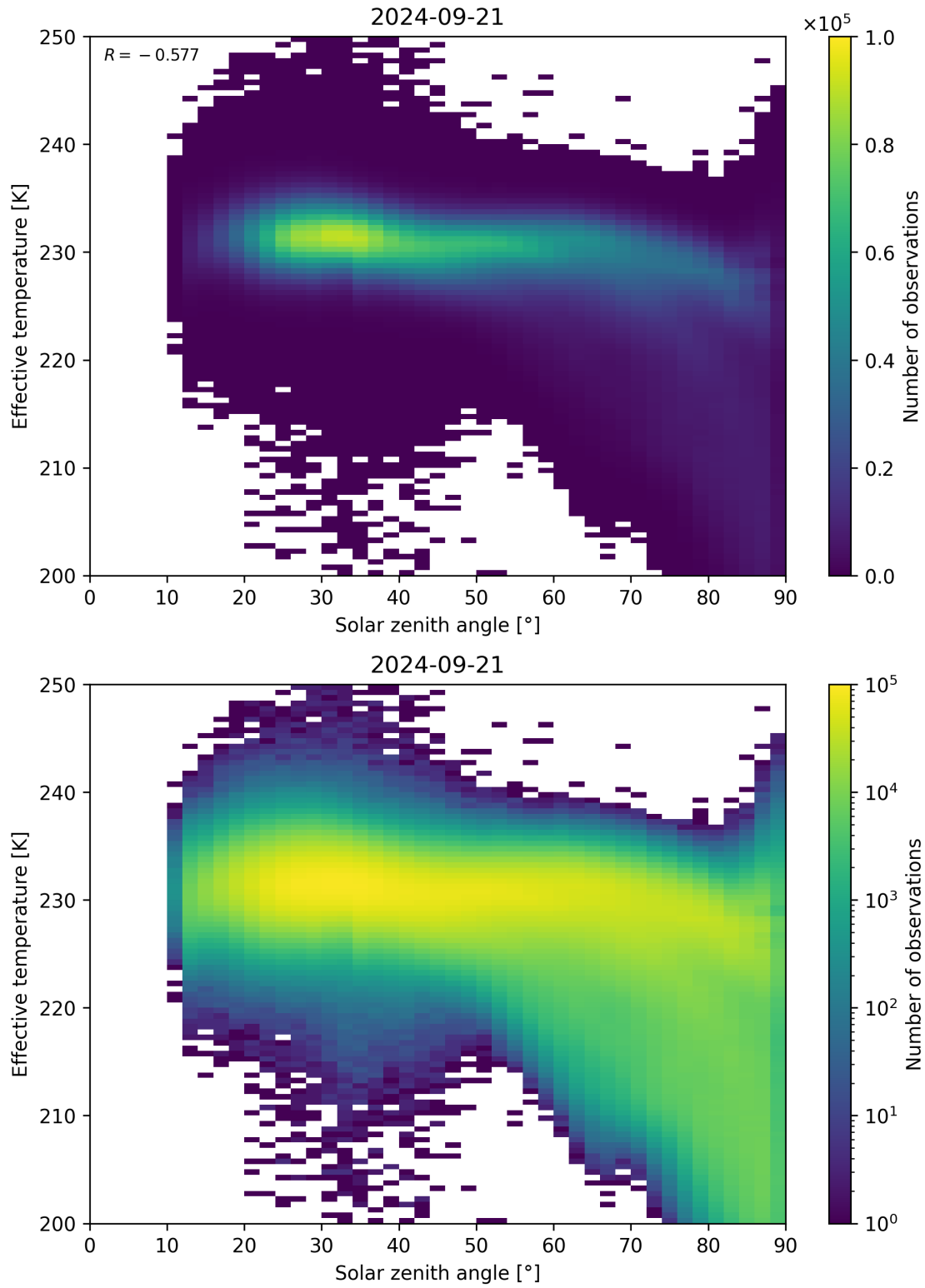
Figure 45: Scatter density plot of “Solar zenith angle” against “Effective temperature” for 2024-09-20 to 2024-09-22.
