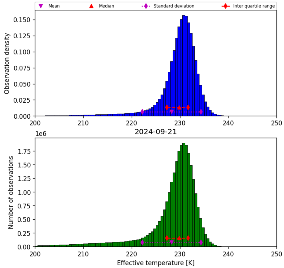
Figure 24: Histogram of “Effective temperature” for 2024-09-20 to 2024-09-22
