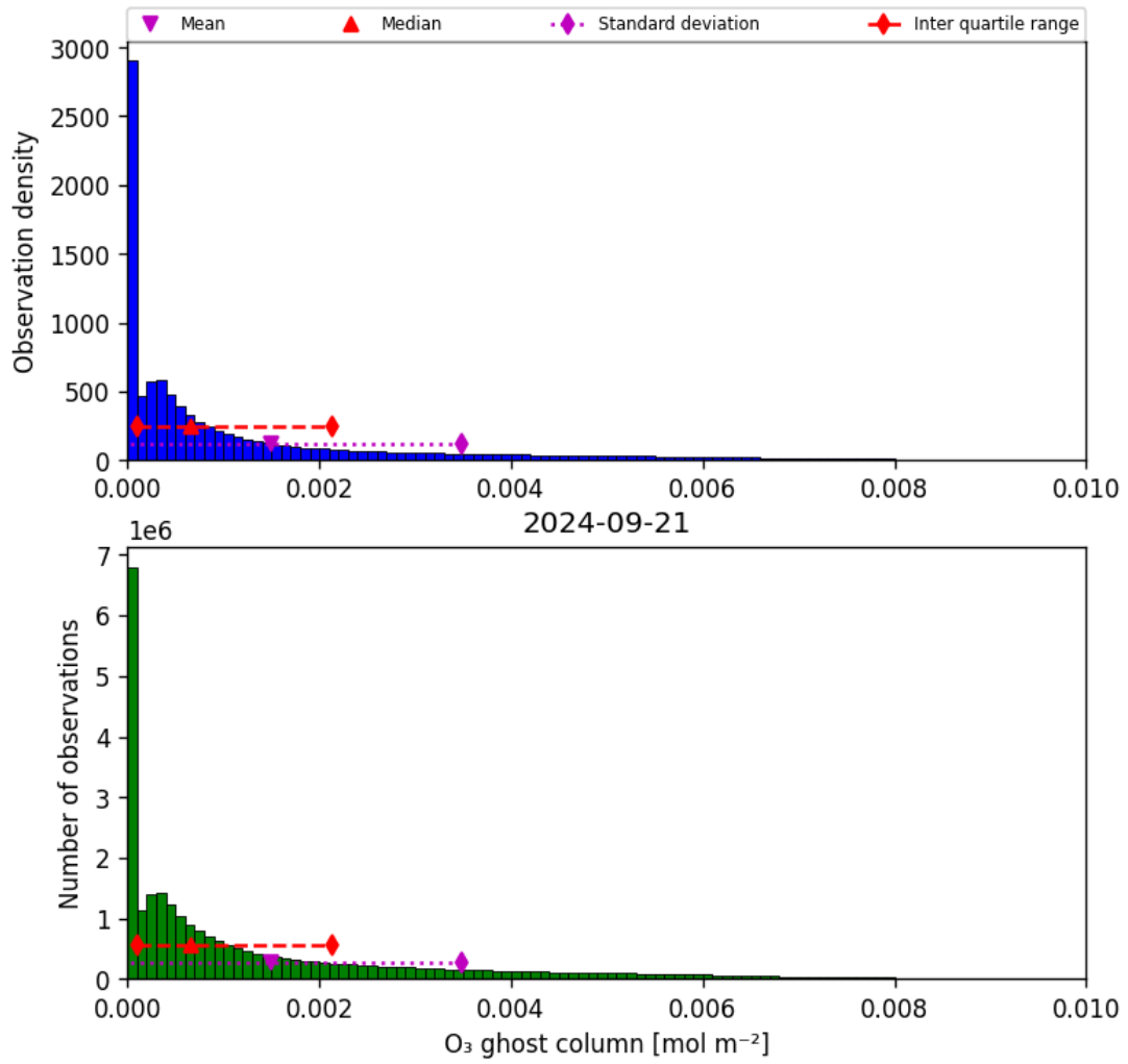
Figure 25: Histogram of “O 3 ghost column” for 2024-09-20 to 2024-09-22
