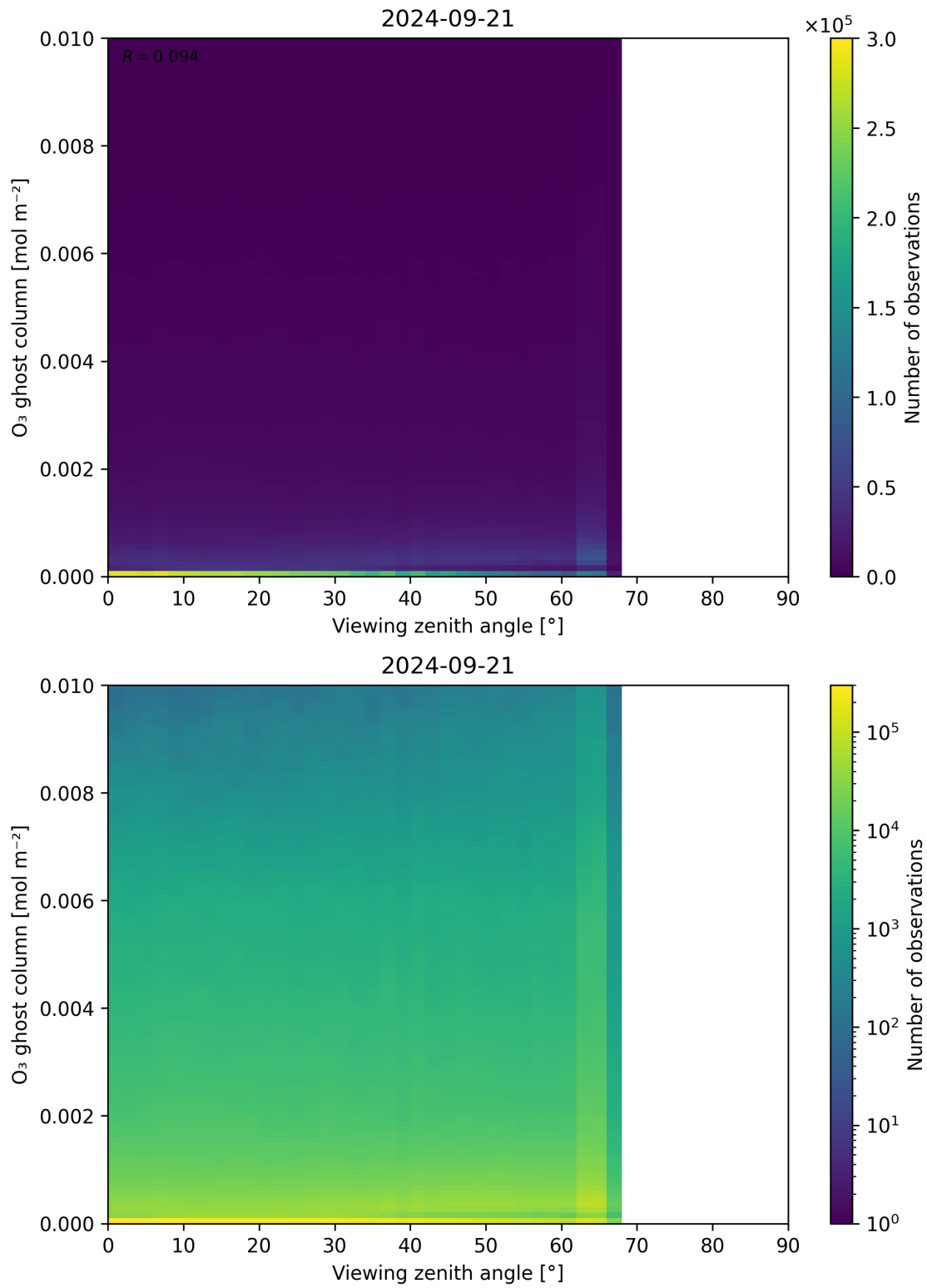
Figure 51: Scatter density plot of “Viewing zenith angle” against “O 3 ghost column” for 2024-09-20 to 2024-09-22.
