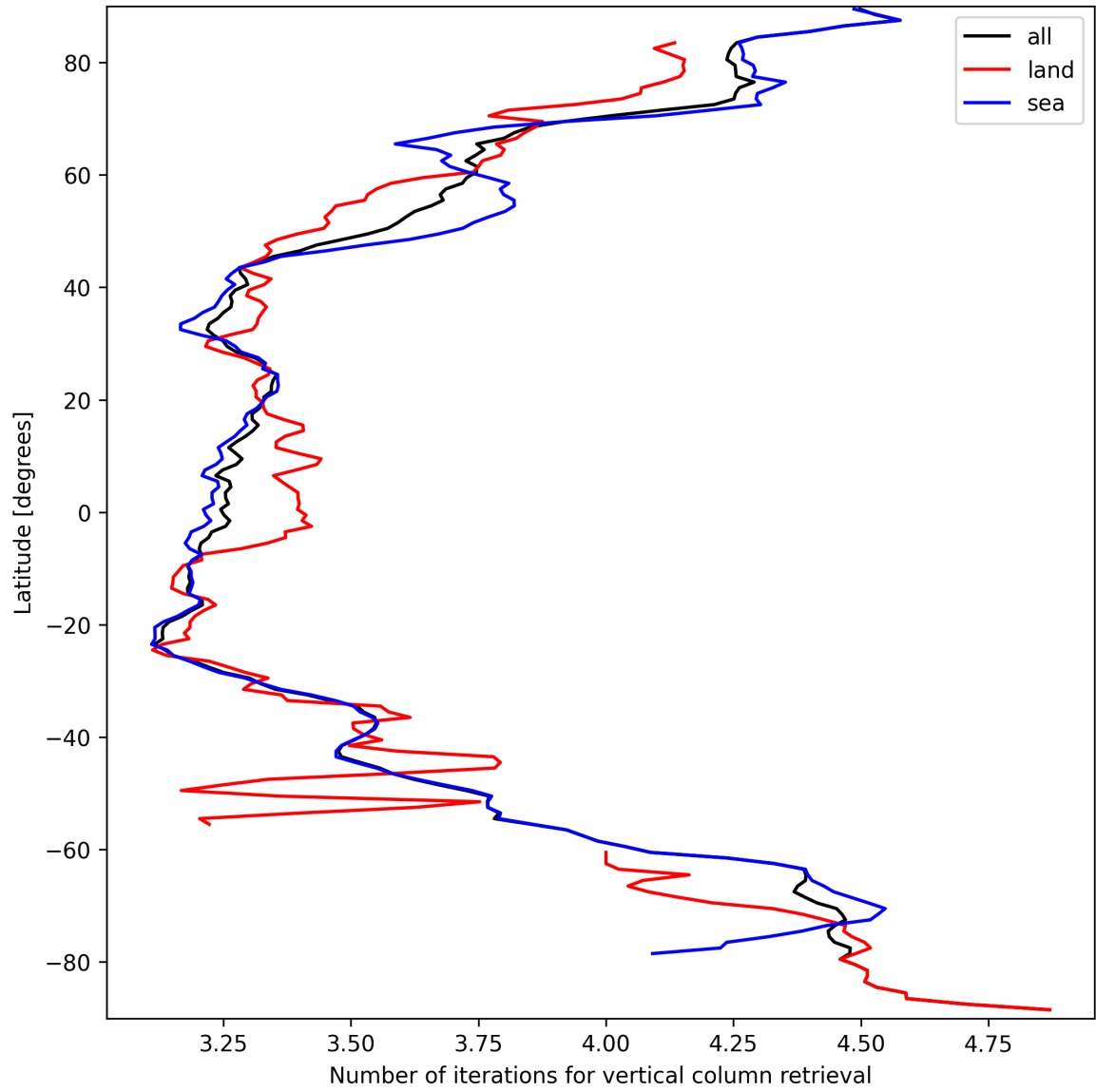
Figure 19: Zonal average of “Number of iterations for vertical column retrieval” for 2024-09-20 to 2024-09-22.
