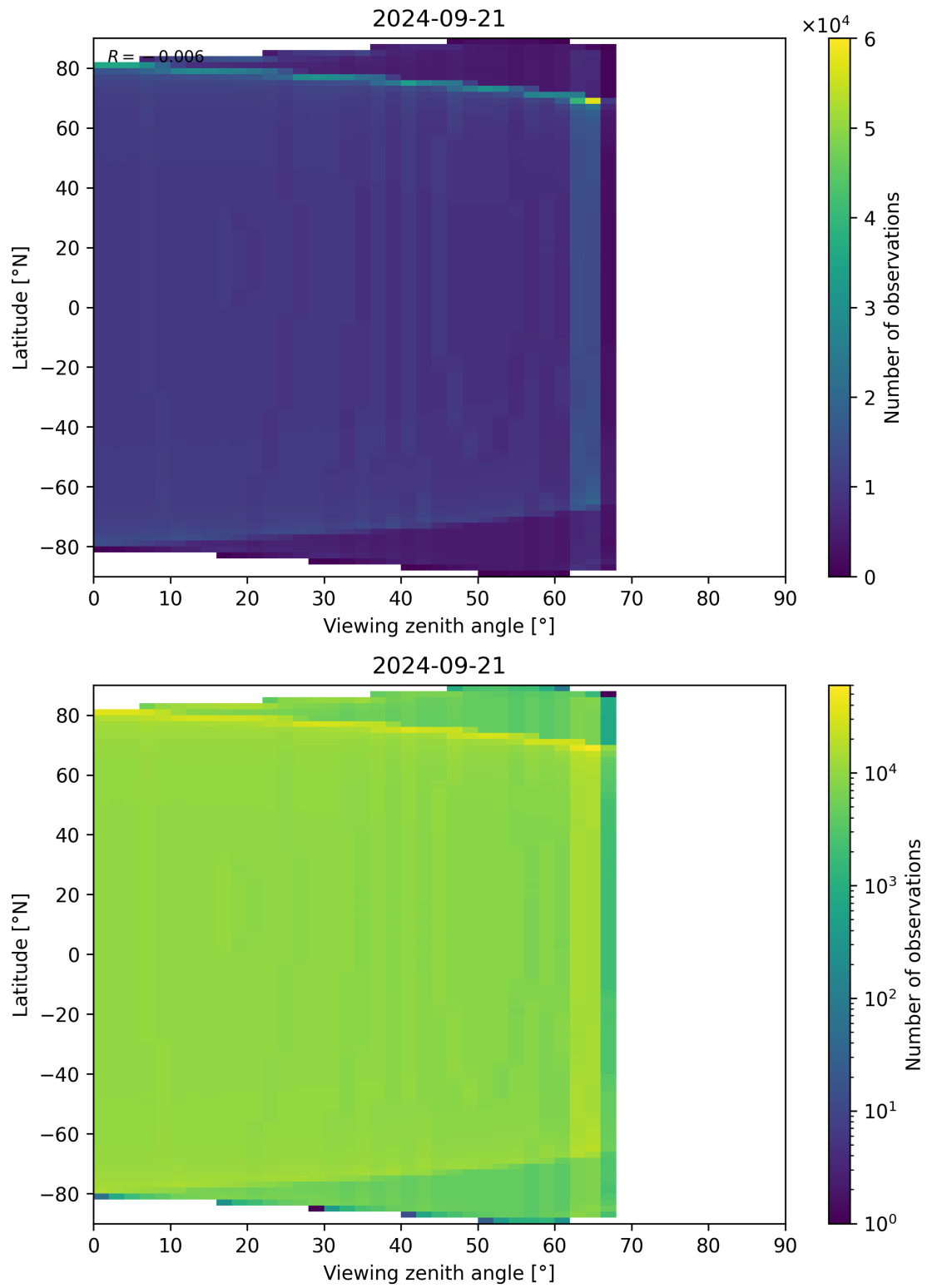
Figure 49: Scatter density plot of “Viewing zenith angle” against “Latitude” for 2024-09-20 to 2024-09-22.
