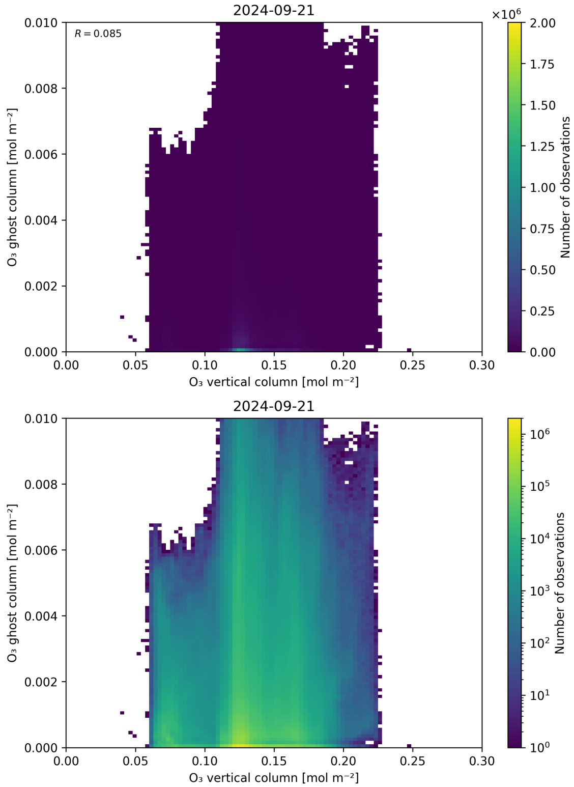
Figure 40: Scatter density plot of “O 3 vertical column” against “O 3 ghost column” for 2024-09-20 to 2024-09-22.
