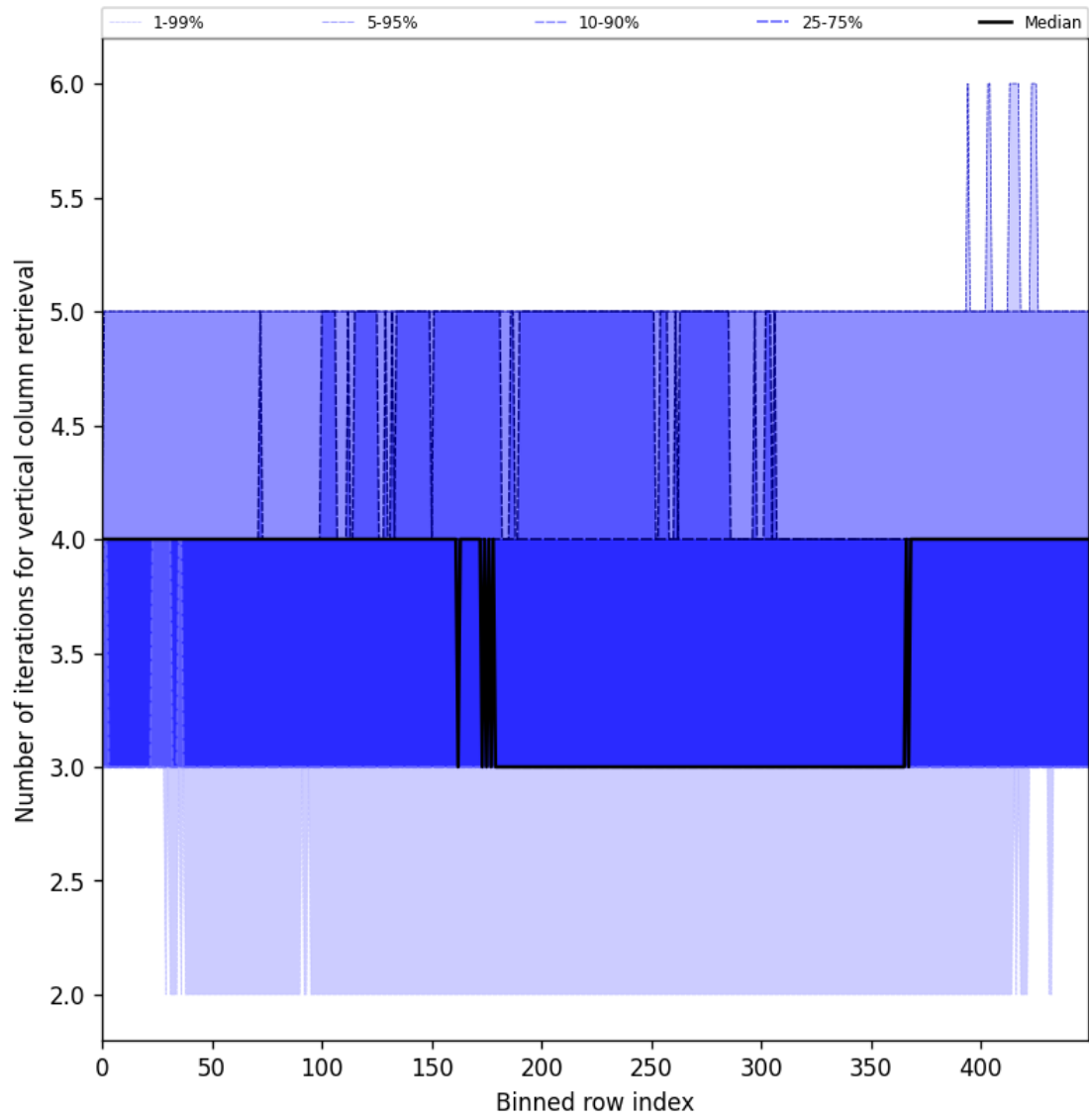
Figure 33: Along track statistics of “Number of iterations for vertical column retrieval” for 2024-09-20 to 2024-09-22
