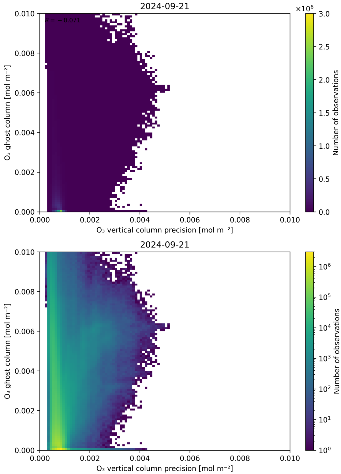
Figure 43: Scatter density plot of “ O_3 vertical column precision” against “ O_3 ghost column” for 2024-09-20 to 2024-09-22.
