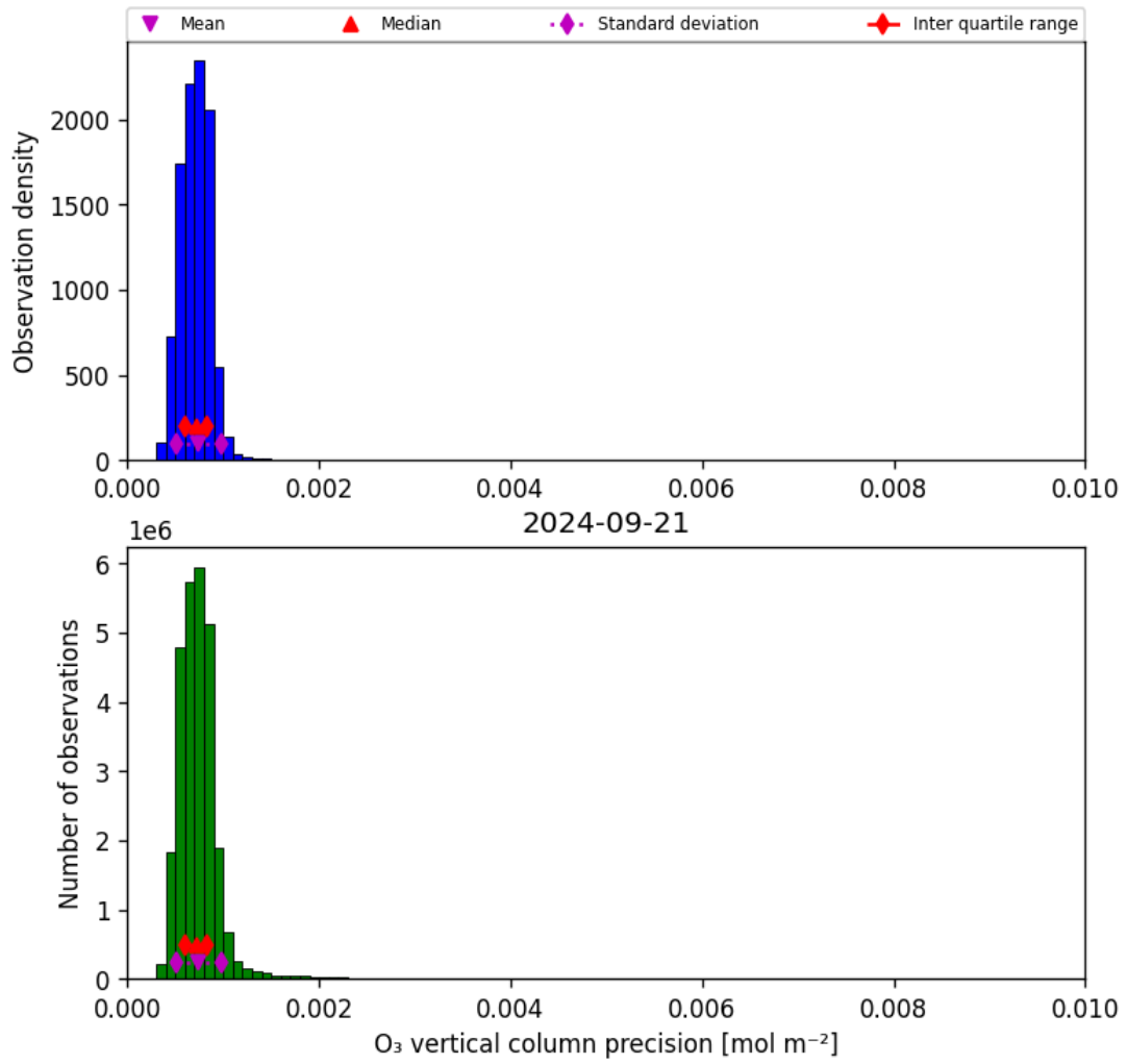
Figure 22: Histogram of “O 3 vertical column precision” for 2024-09-20 to 2024-09-22
