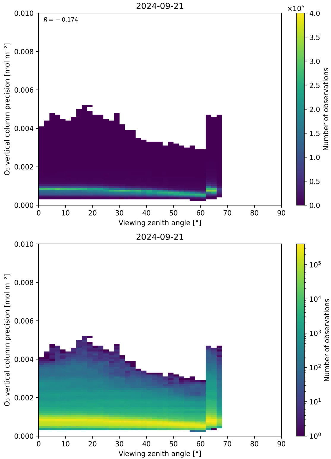
Figure 53: Scatter density plot of “Viewing zenith angle” against “O 3 vertical column precision” for 2024-09-20 to 2024-09-22.
