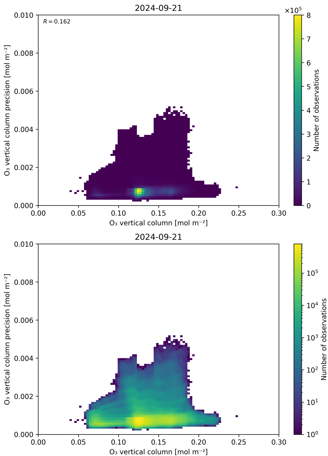
Figure 41: Scatter density plot of “O 3 vertical column” against “O 3 vertical column precision” for 2024-09-20 to 2024-09-22.
