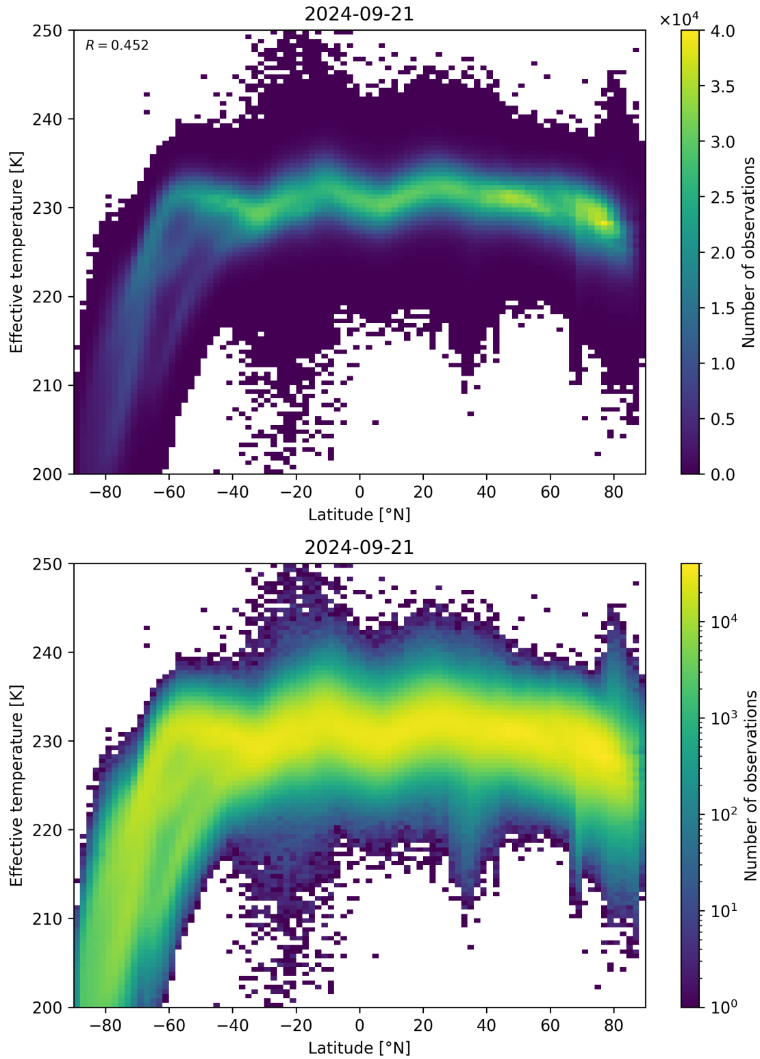
Figure 34: Scatter density plot of “Latitude” against “Effective temperature” for 2024-09-20 to 2024-09-22.
