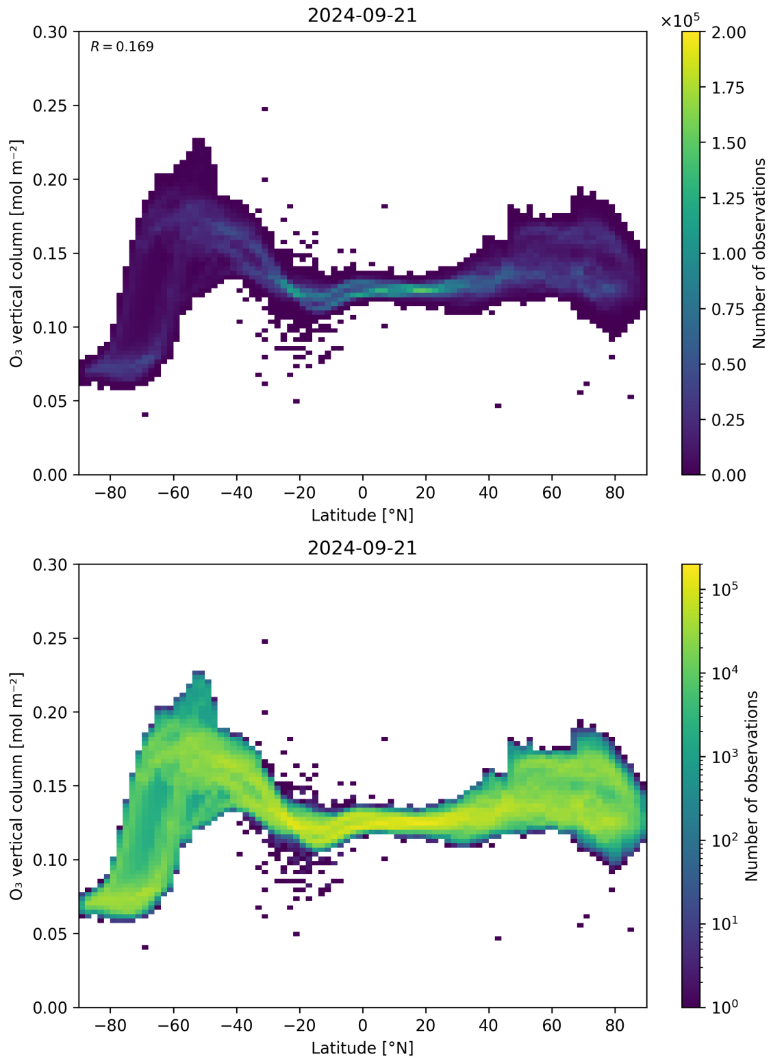
Figure 36: Scatter density plot of “Latitude” against “O 3 vertical column” for 2024-09-20 to 2024-09-22.
