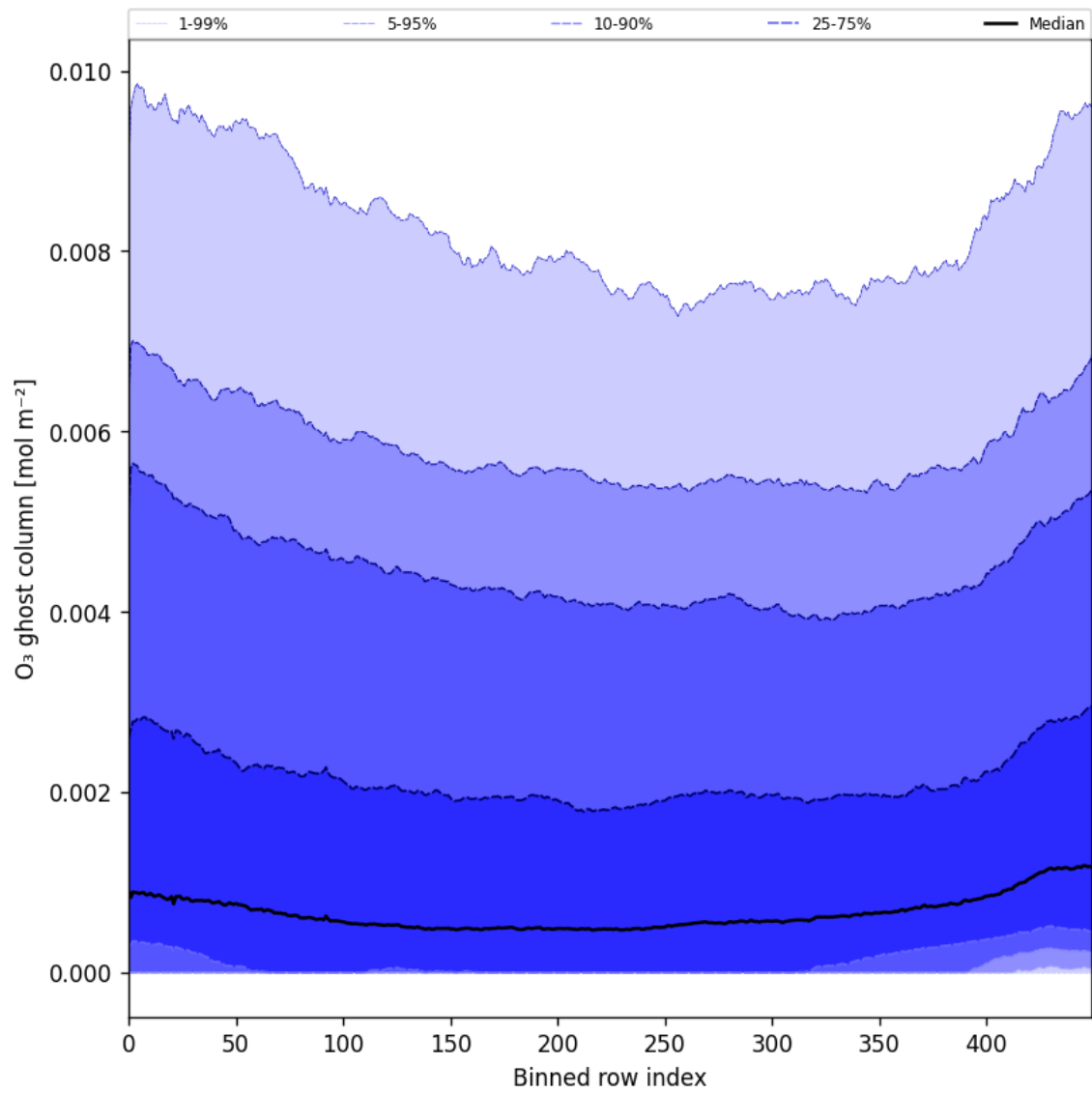
Figure 32: Along track statistics of “O 3 ghost column” for 2024-09-20 to 2024-09-22
