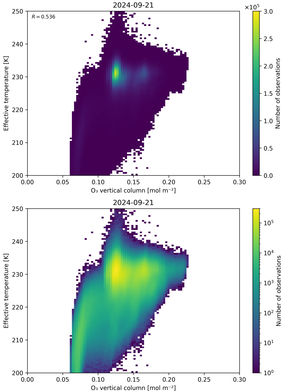
Figure 39: Scatter density plot of “O 3 vertical column” against “Effective temperature” for 2024-09-20 to 2024-09-22.
