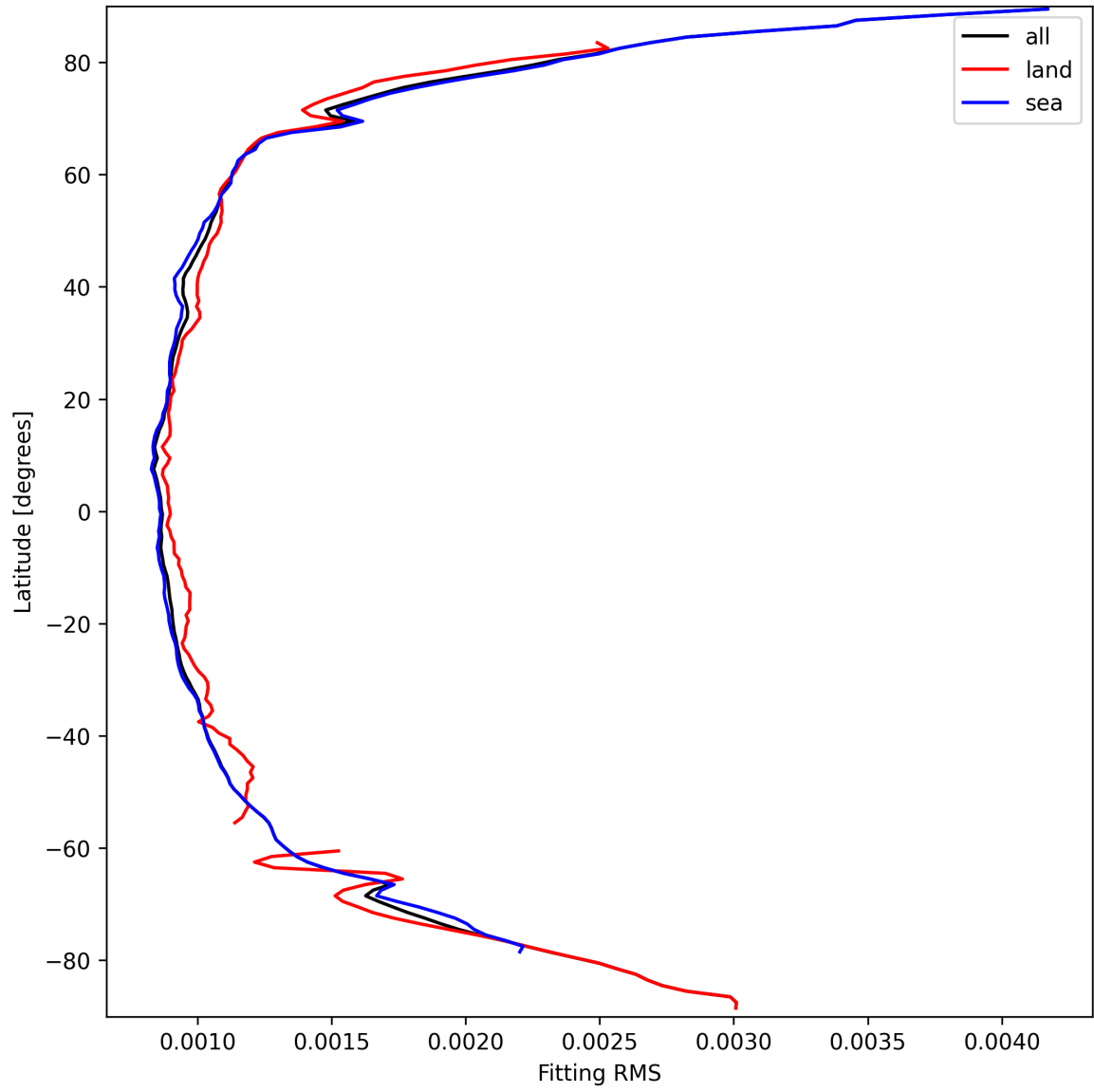
Figure 16: Zonal average of “Fitting RMS” for 2024-09-20 to 2024-09-22.
