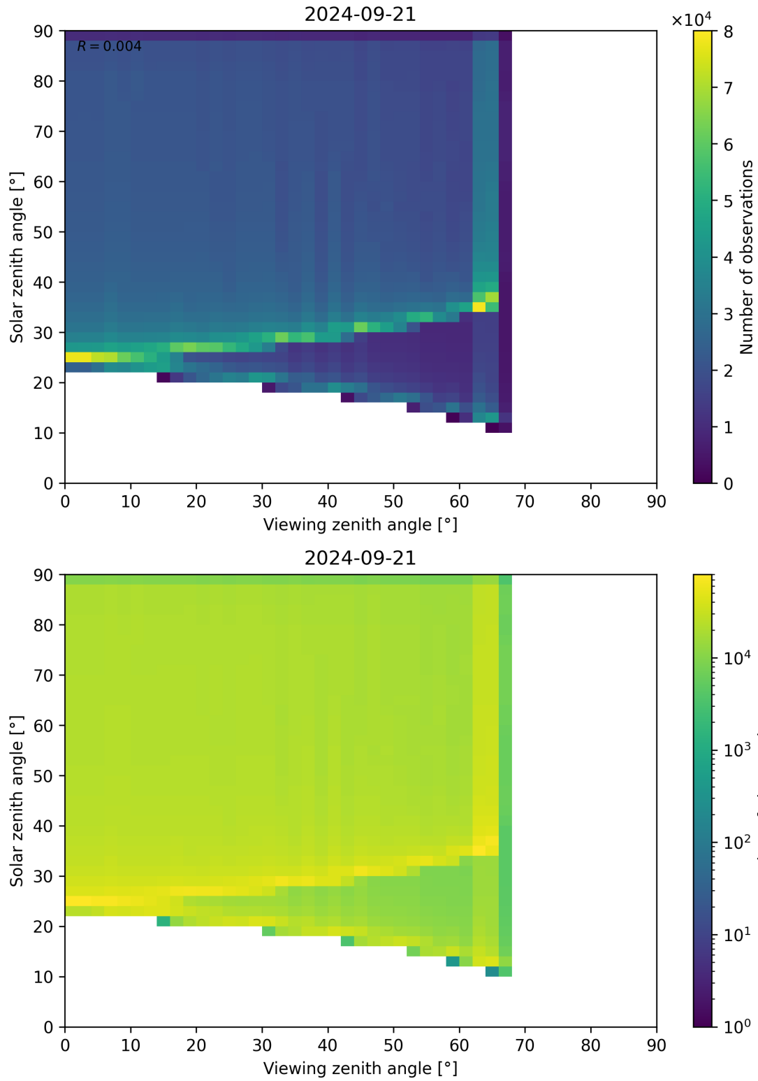
Figure 54: Scatter density plot of “Viewing zenith angle” against “Solar zenith angle” for 2024-09-20 to 2024-09-22.
