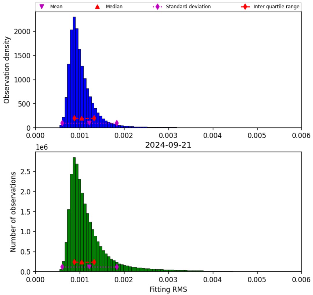
Figure 23: Histogram of “Fitting RMS” for 2024-09-20 to 2024-09-22
