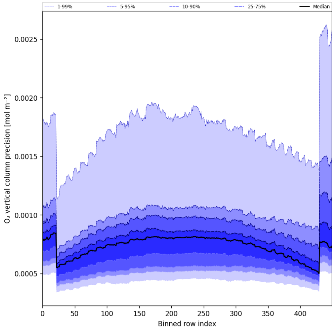
Figure 29: Along track statistics of “O 3 vertical column precision” for 2024-09-20 to 2024-09-22
