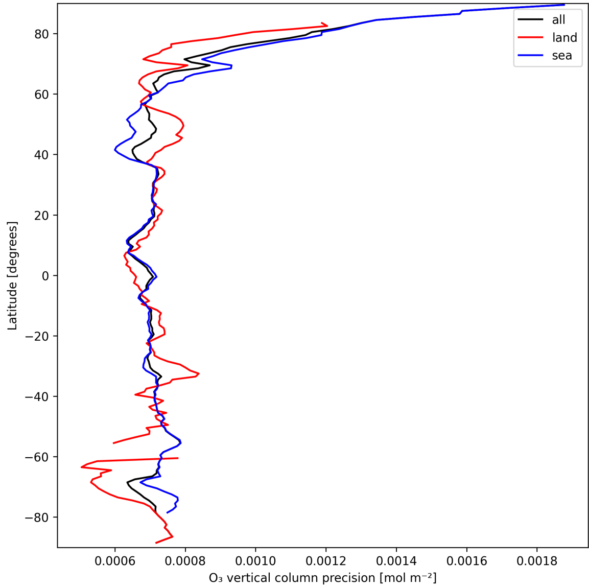
Figure 15: Zonal average of “O 3 vertical column precision” for 2024-09-20 to 2024-09-22.
