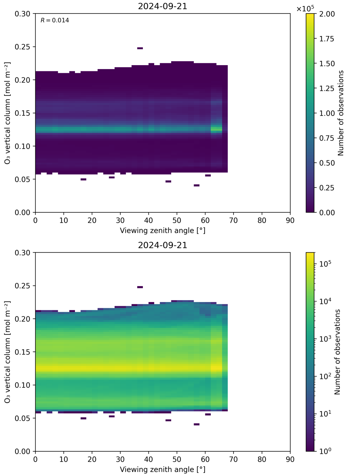
Figure 52: Scatter density plot of “Viewing zenith angle” against “O 3 vertical column” for 2024-09-20 to 2024-09-22.
