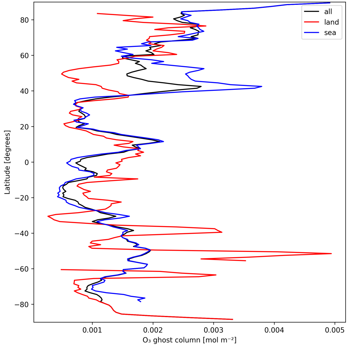
Figure 18: Zonal average of "O 3 ghost column" for 2024-09-20 to 2024-09-22.
