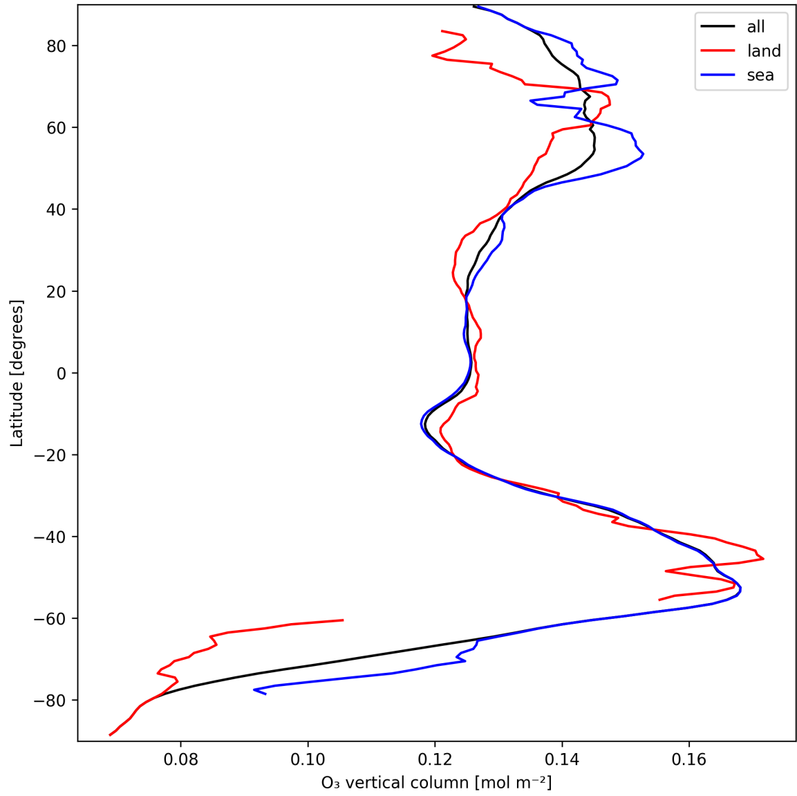
Figure 14: Zonal average of “O 3 vertical column” for 2024-09-20 to 2024-09-22.
