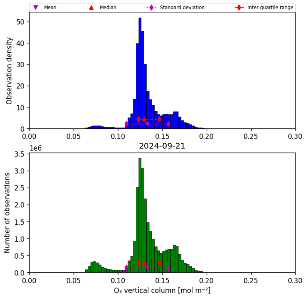
Figure 21: Histogram of “O 3 vertical column” for 2024-09-20 to 2024-09-22
