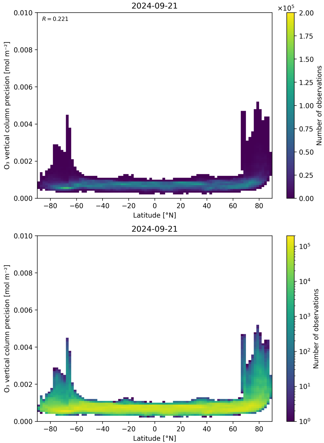
Figure 37: Scatter density plot of “Latitude” against “O 3 vertical column precision” for 2024-09-20 to 2024-09-22.
