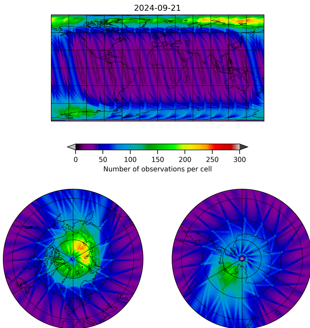
Figure 12: Map of the number of observations for 2024-09-20 to 2024-09-22
