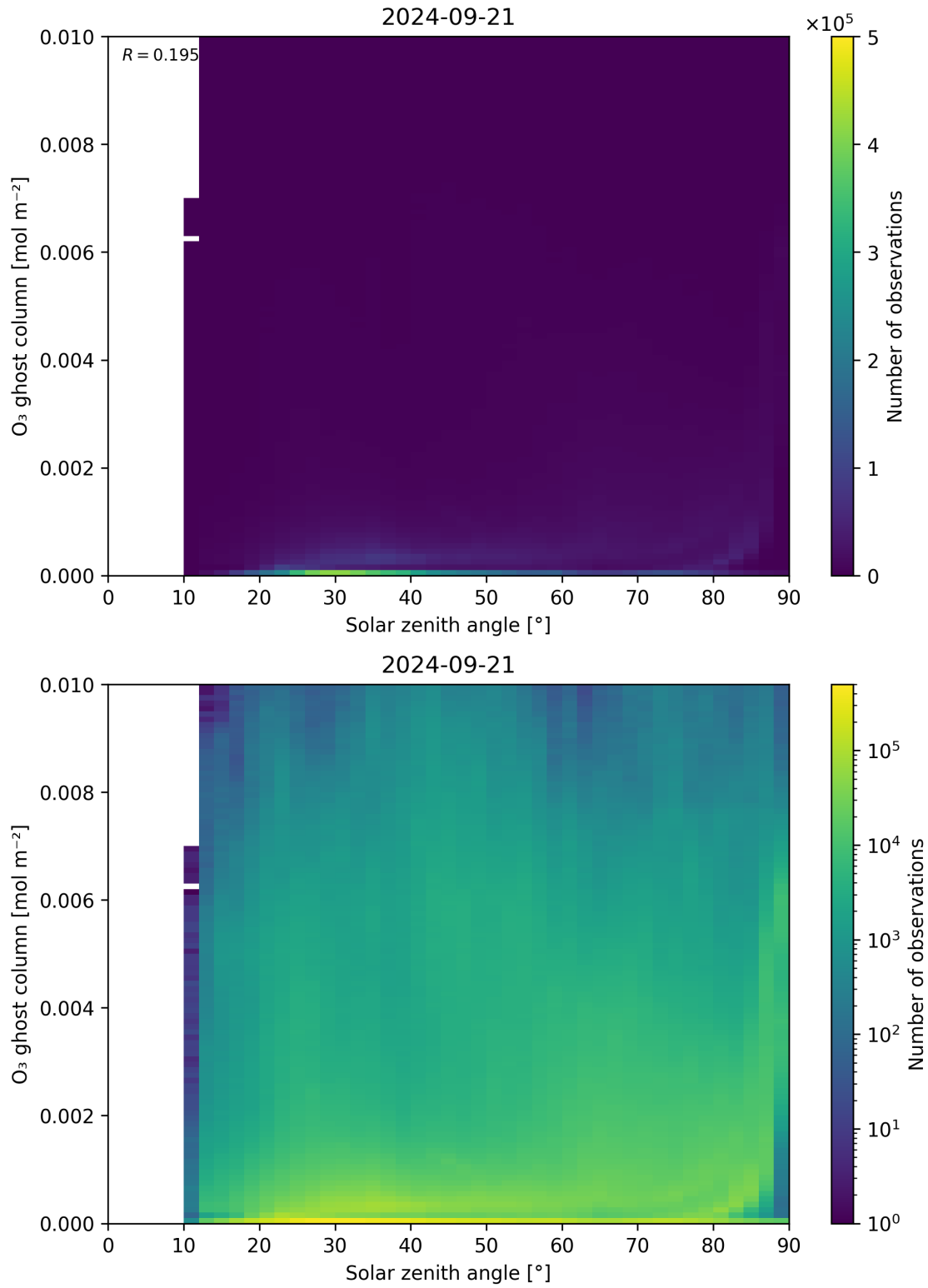
Figure 46: Scatter density plot of “Solar zenith angle” against “O 3 ghost column” for 2024-09-20 to 2024-09-22.
