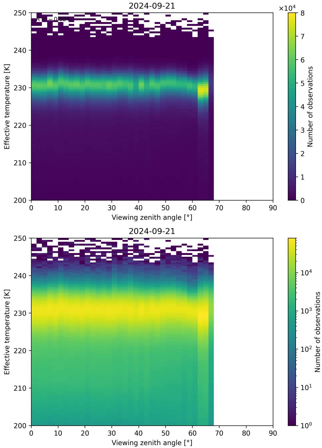
Figure 50: Scatter density plot of “Viewing zenith angle” against “Effective temperature” for 2024-09-20 to 2024-09-22.
