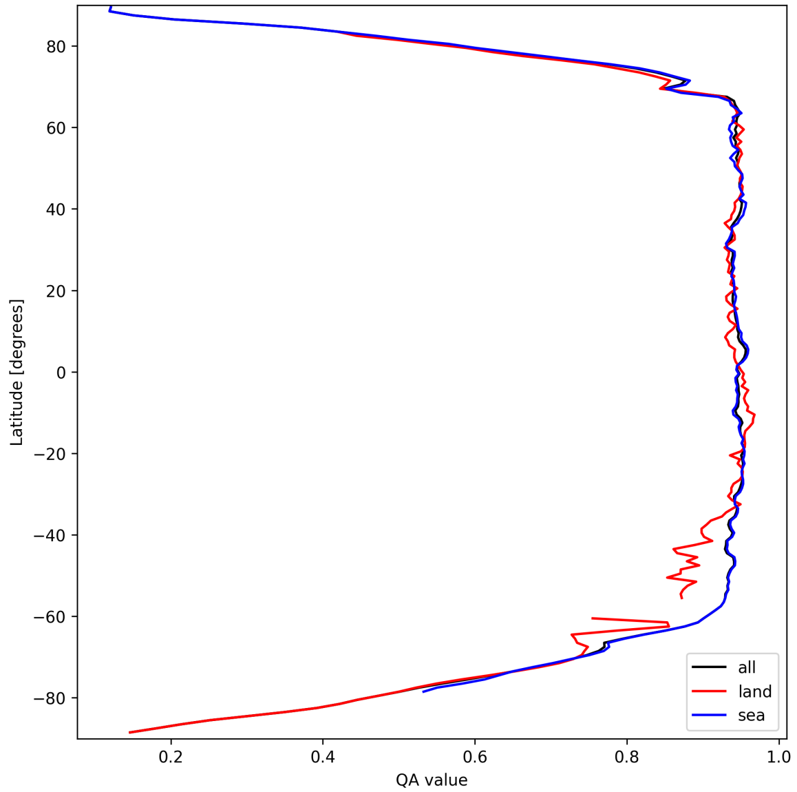
Figure 13: Zonal average of “QA value” for 2024-09-20 to 2024-09-22.
