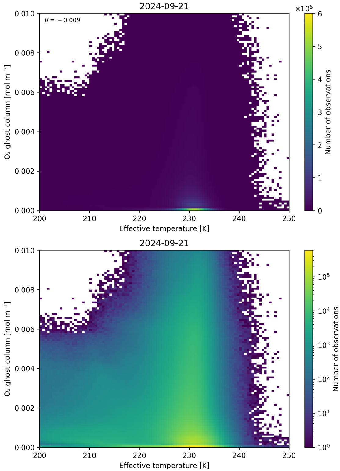
Figure 38: Scatter density plot of “Effective temperature” against “O 3 ghost column” for 2024-09-20 to 2024-09-22.
