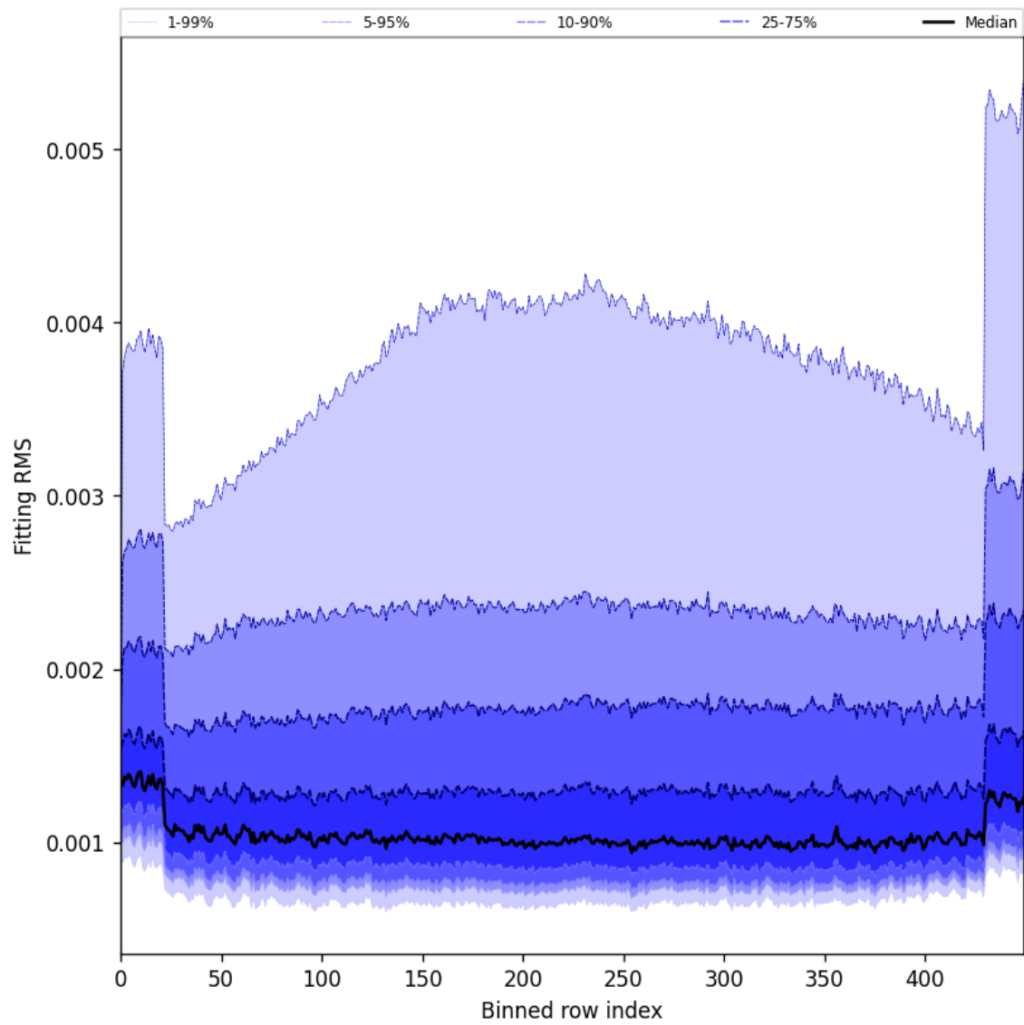
Figure 30: Along track statistics of “Fitting RMS” for 2024-09-20 to 2024-09-22
