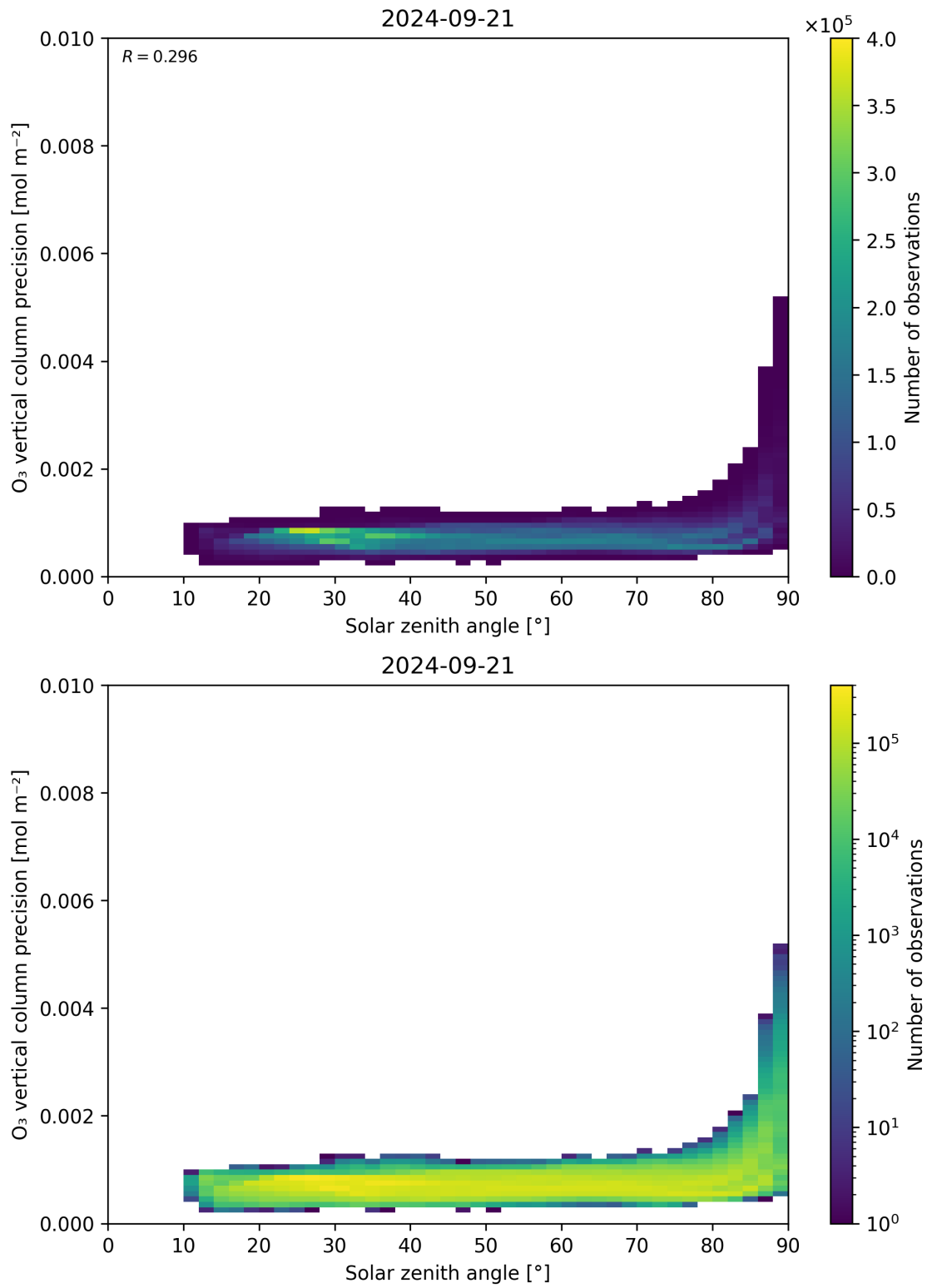
Figure 48: Scatter density plot of “Solar zenith angle” against “O 3 vertical column precision” for 2024-09-20 to 2024-09-22.
