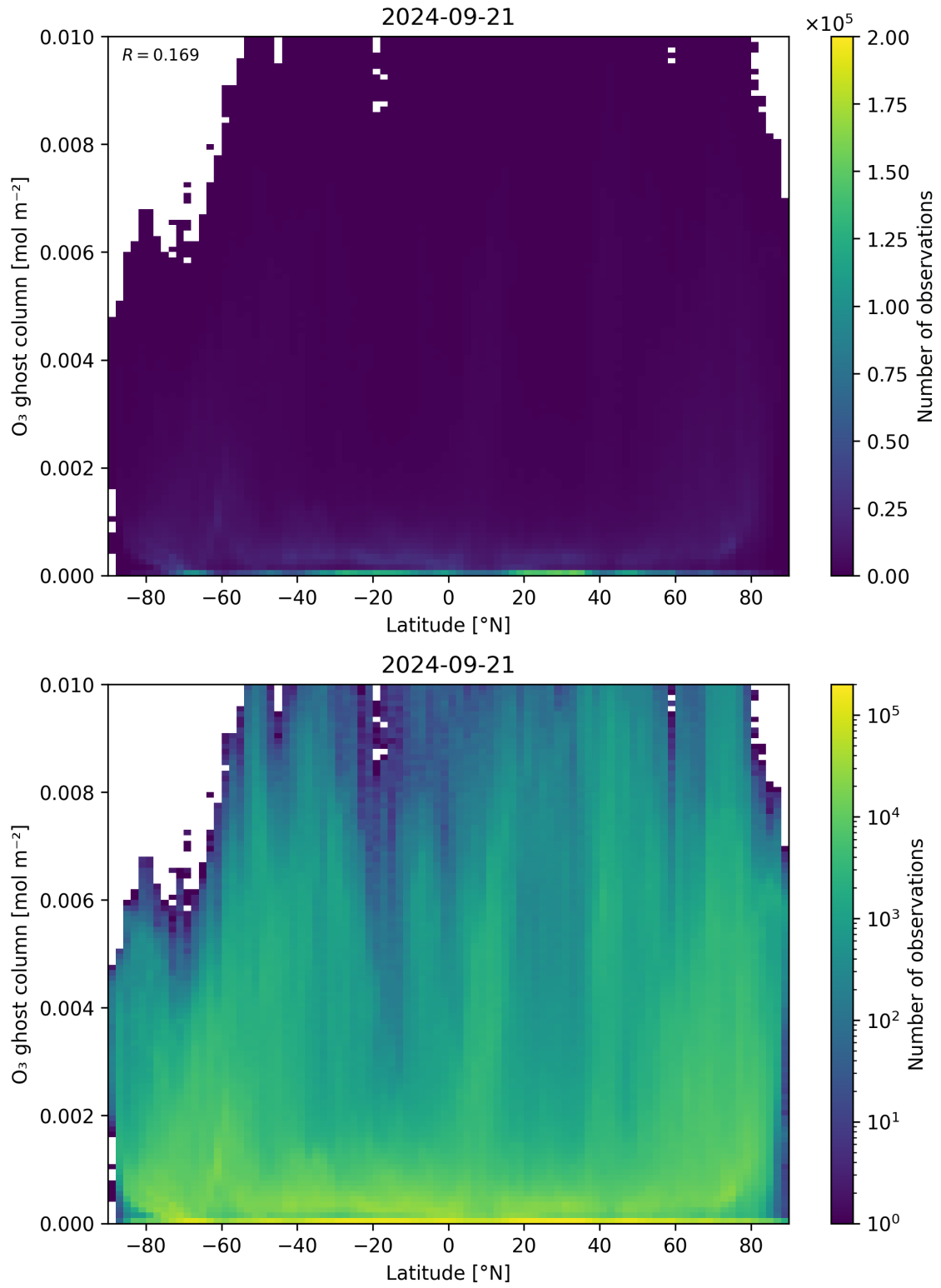
Figure 35: Scatter density plot of “Latitude” against “O 3 ghost column” for 2024-09-20 to 2024-09-22.
