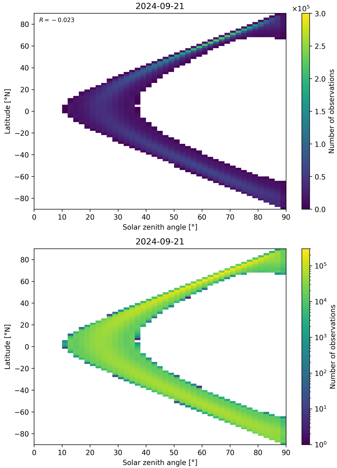
Figure 44: Scatter density plot of “Solar zenith angle” against “Latitude” for 2024-09-20 to 2024-09-22.
