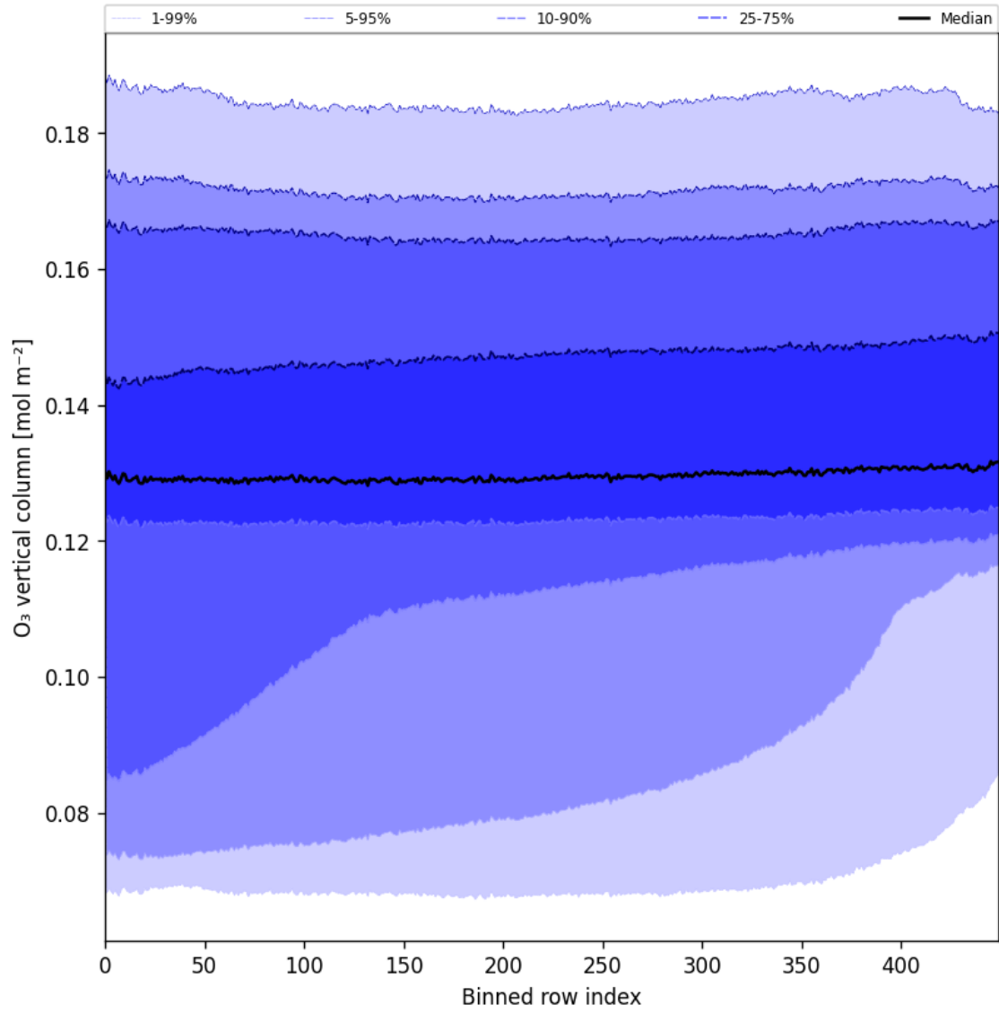
Figure 28: Along track statistics of “O 3 vertical column” for 2024-09-20 to 2024-09-22
