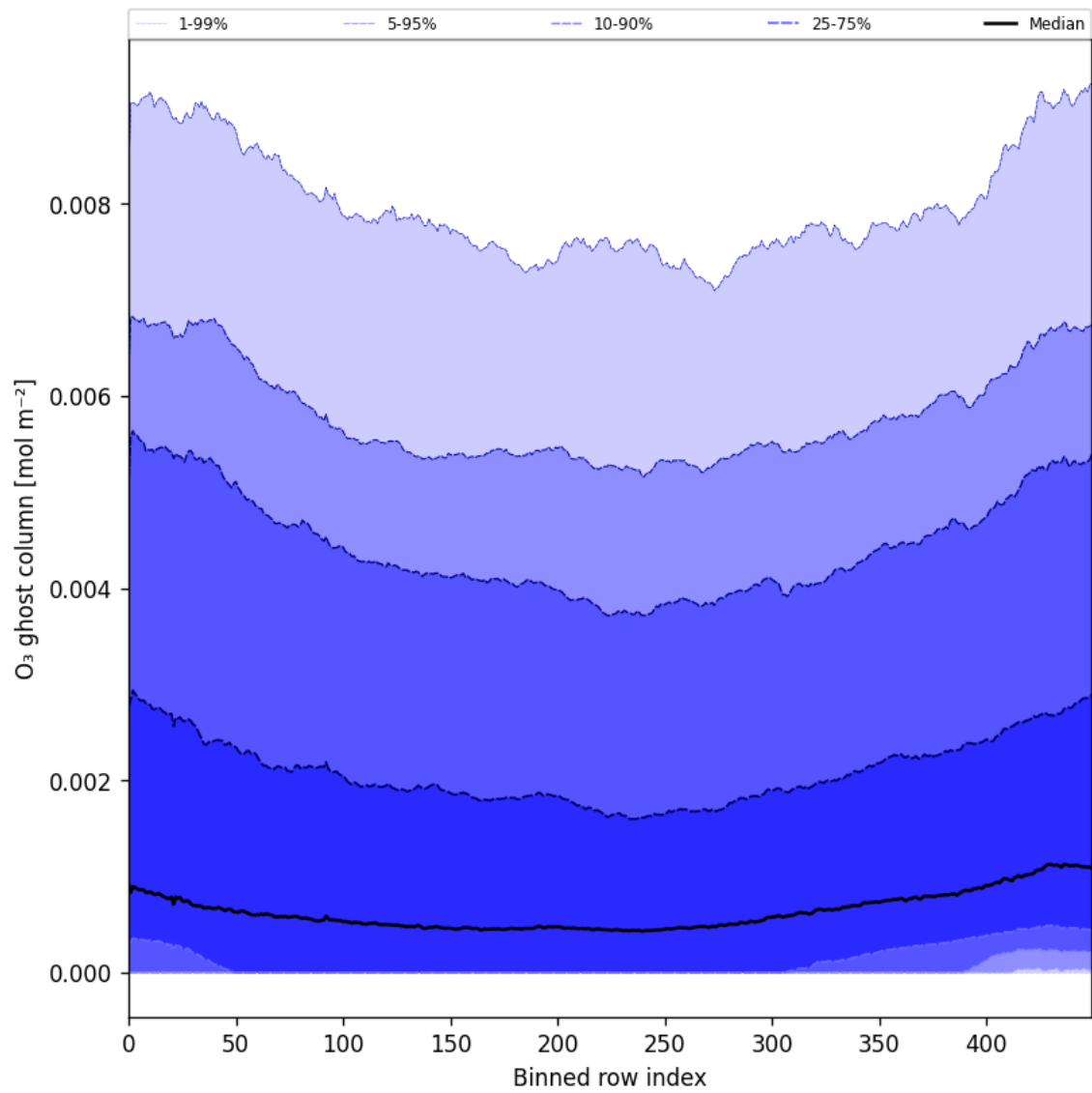
Figure 32: Along track statistics of “O 3 ghost column” for 2024-09-22 to 2024-09-23
