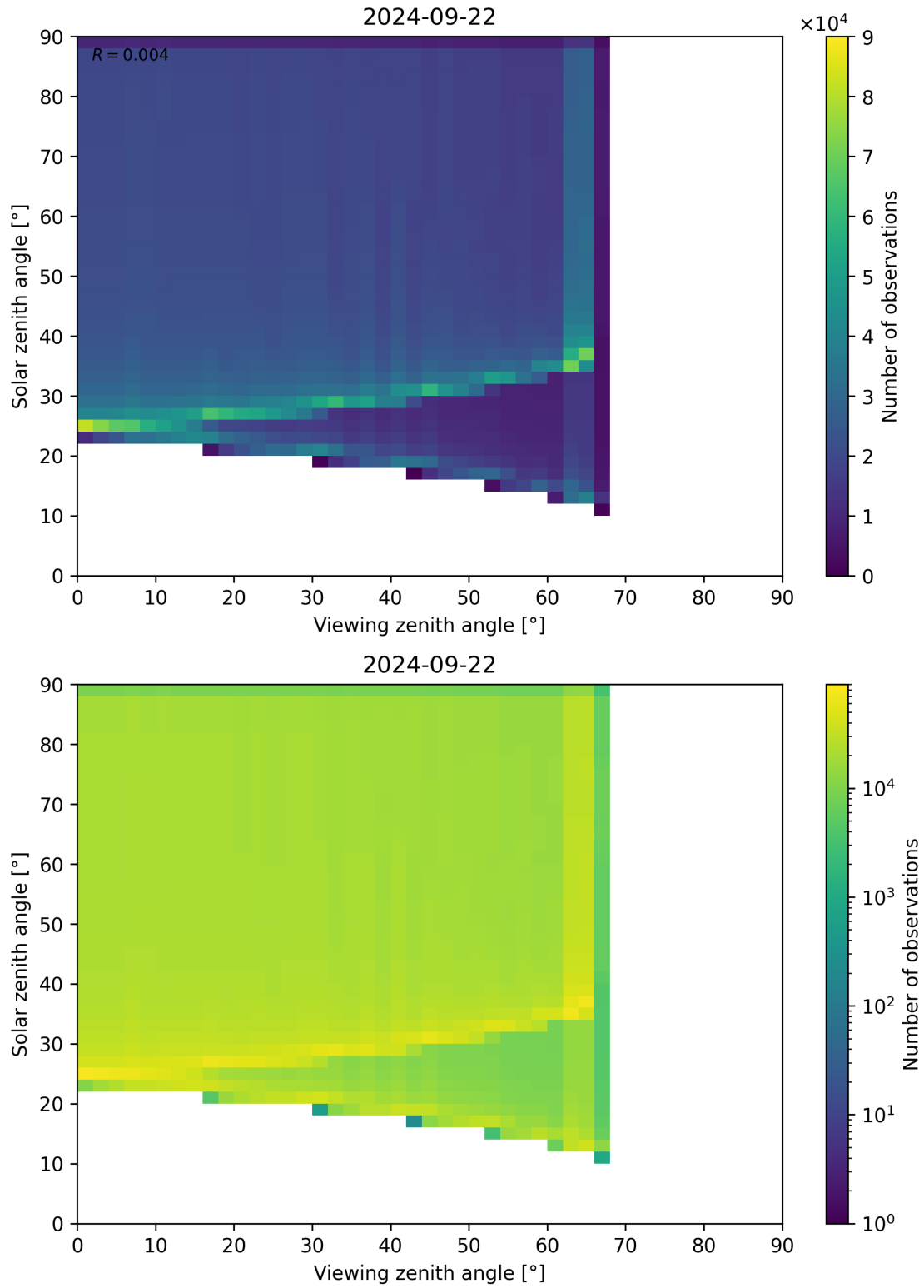
Figure 54: Scatter density plot of “Viewing zenith angle” against “Solar zenith angle” for 2024-09-22 to 2024-09-23.
