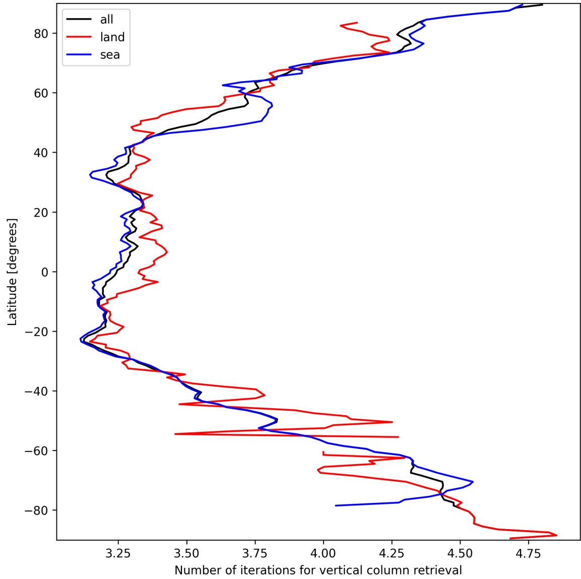
Figure 19: Zonal average of “Number of iterations for vertical column retrieval” for 2024-09-22 to 2024-09-23.
