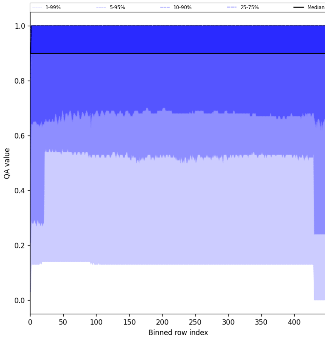
Figure 27: Along track statistics of “QA value” for 2024-09-22 to 2024-09-23
