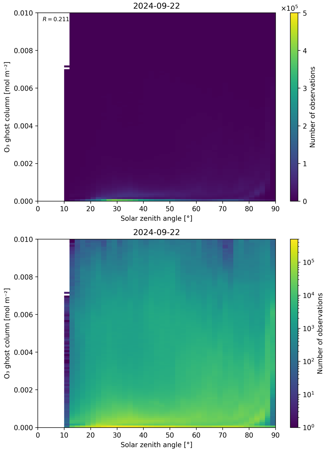
Figure 46: Scatter density plot of “Solar zenith angle” against “O 3 ghost column” for 2024-09-22 to 2024-09-23.
