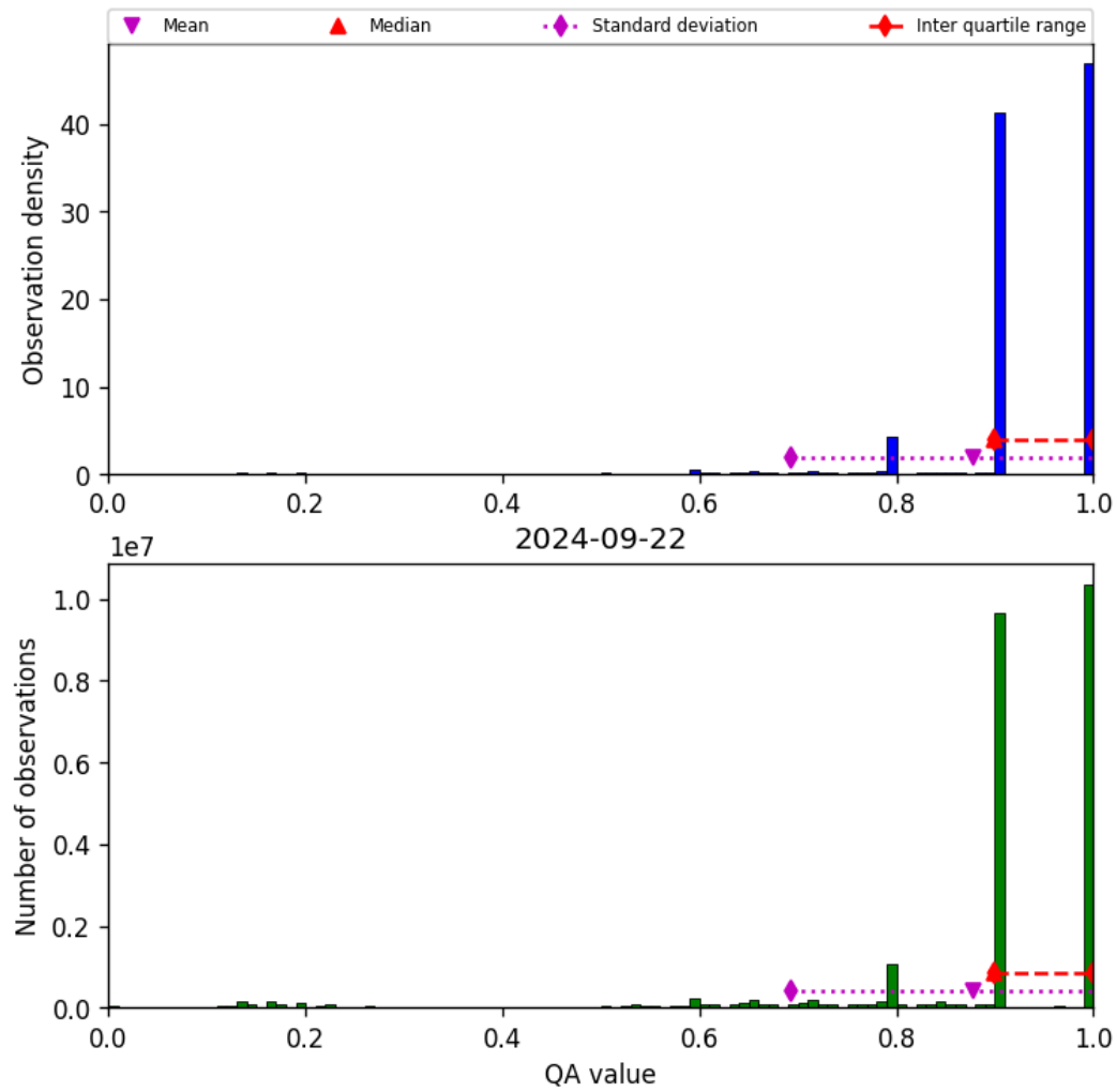
Figure 20: Histogram of “QA value” for 2024-09-22 to 2024-09-23
