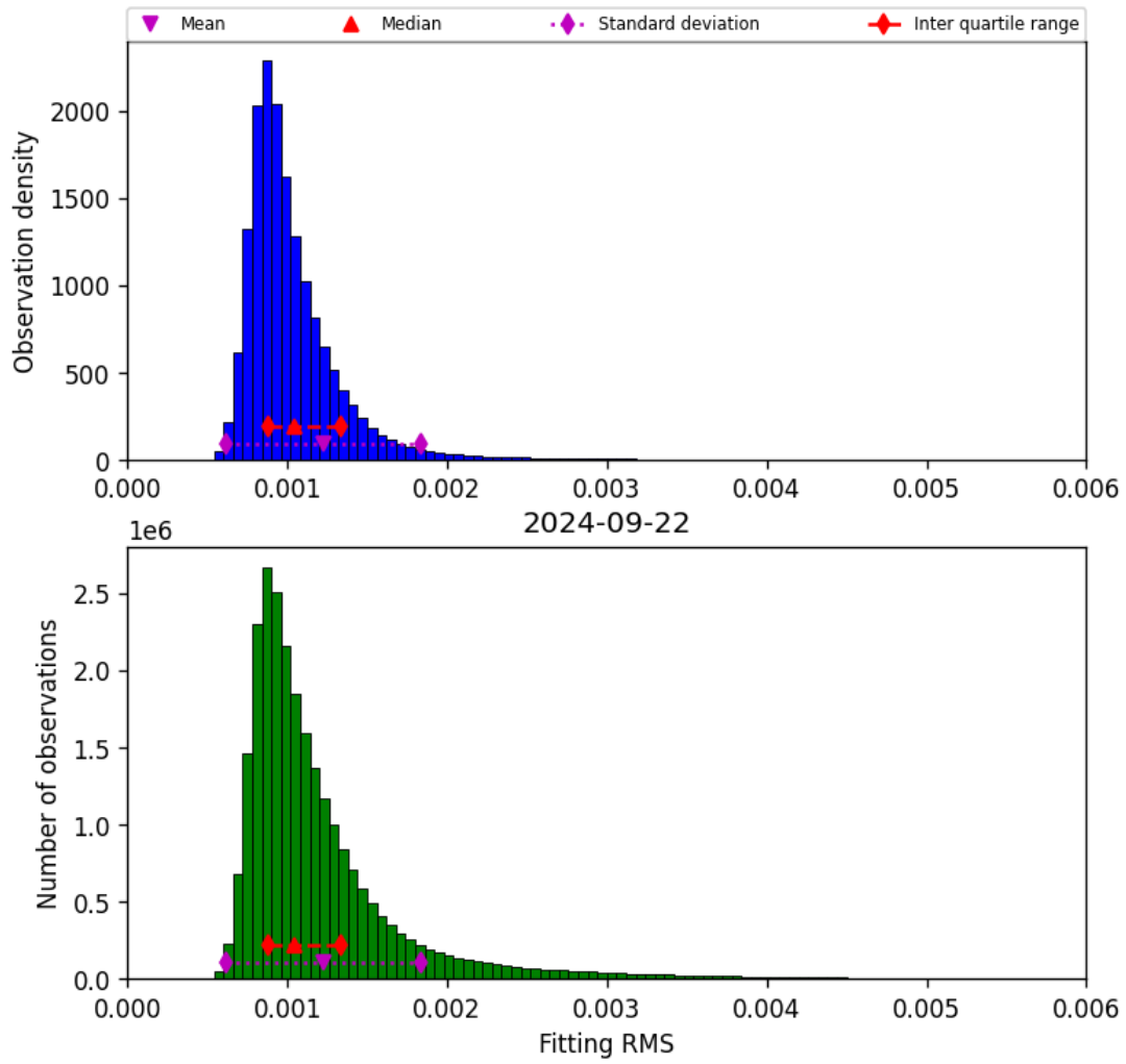
Figure 23: Histogram of “Fitting RMS” for 2024-09-22 to 2024-09-23
