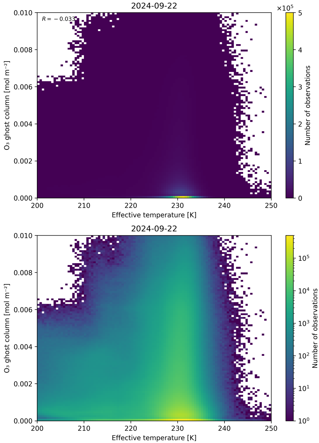
Figure 38: Scatter density plot of “Effective temperature” against “O 3 ghost column” for 2024-09-22 to 2024-09-23.
