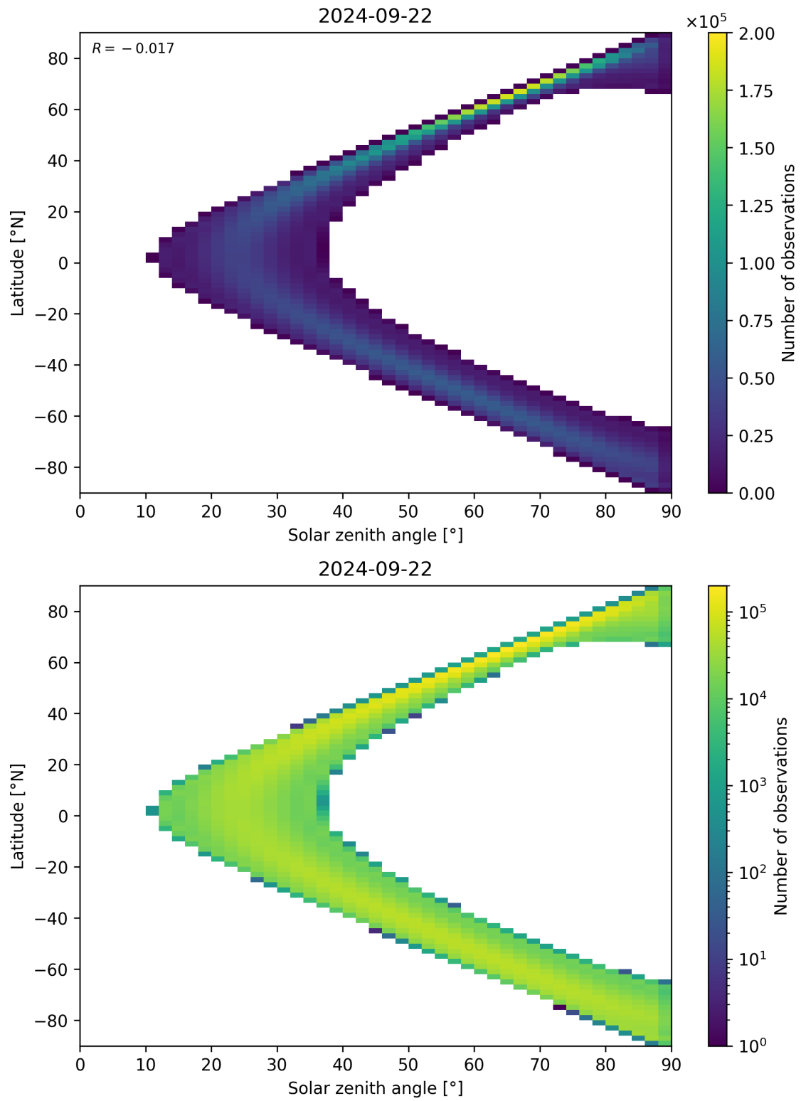
Figure 44: Scatter density plot of “Solar zenith angle” against “Latitude” for 2024-09-22 to 2024-09-23.
