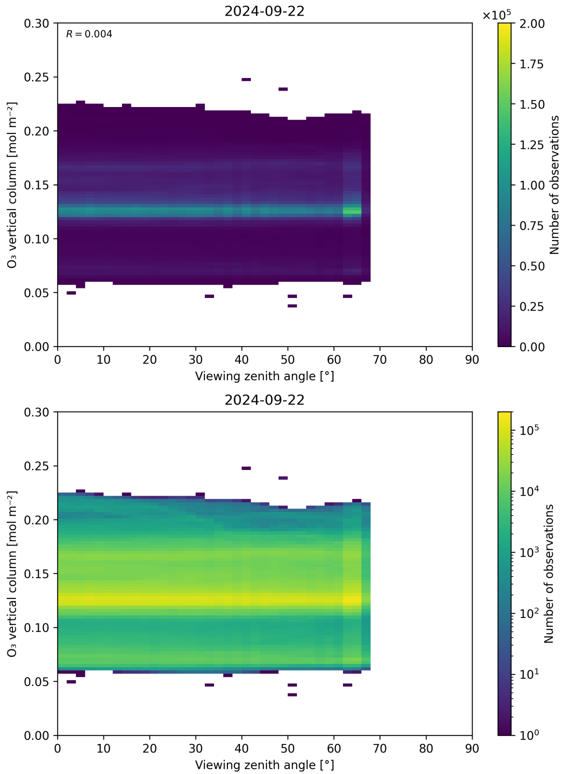
Figure 52: Scatter density plot of “Viewing zenith angle” against “O 3 vertical column” for 2024-09-22 to 2024-09-23.
