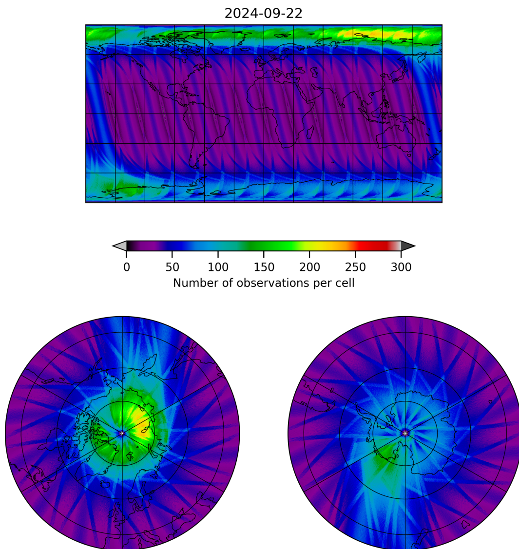
Figure 12: Map of the number of observations for 2024-09-22 to 2024-09-23
