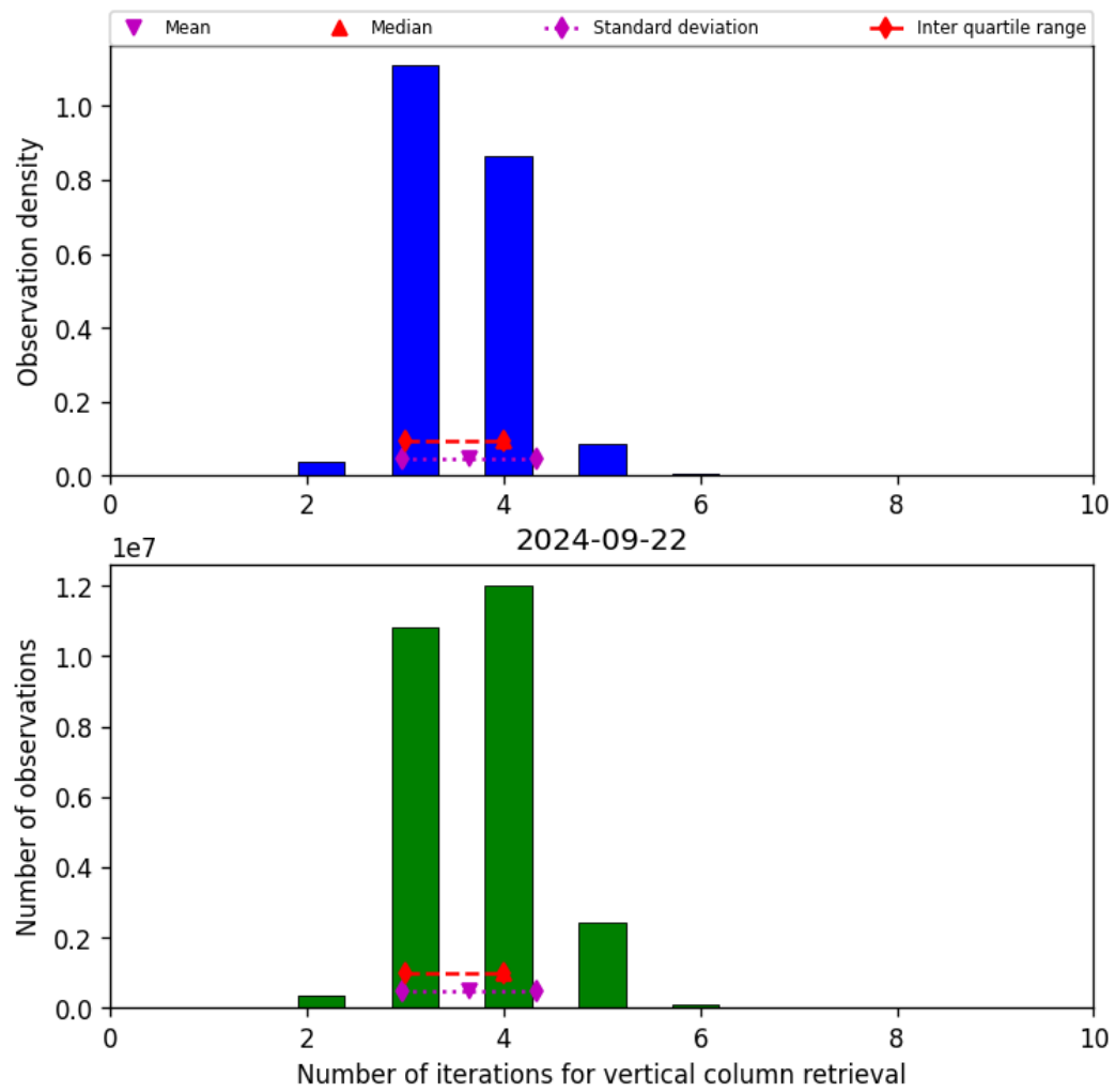
Figure 26: Histogram of “Number of iterations for vertical column retrieval” for 2024-09-22 to 2024-09-23
