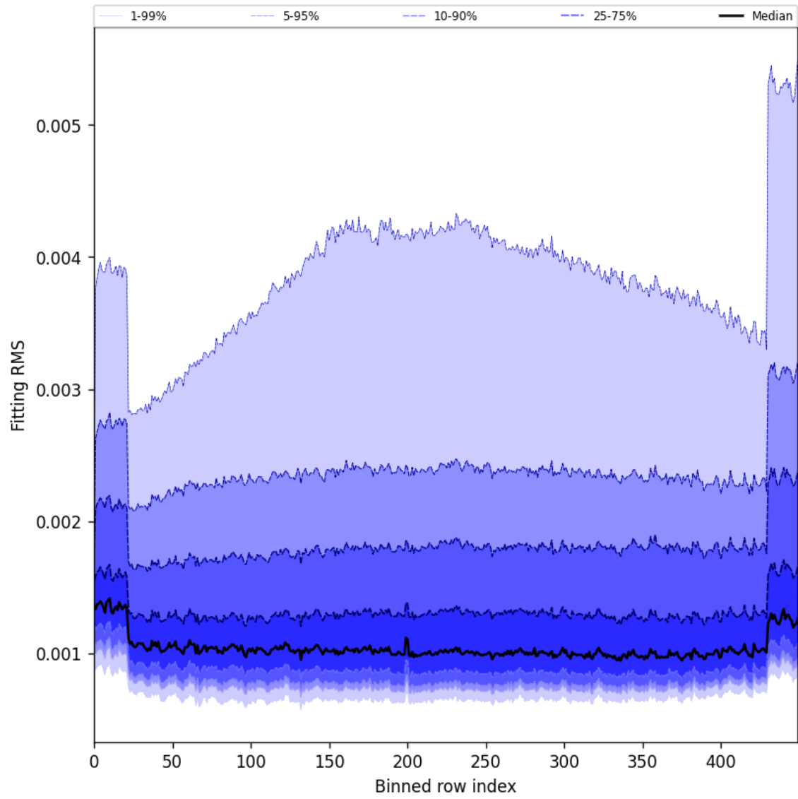
Figure 30: Along track statistics of “Fitting RMS” for 2024-09-22 to 2024-09-23
