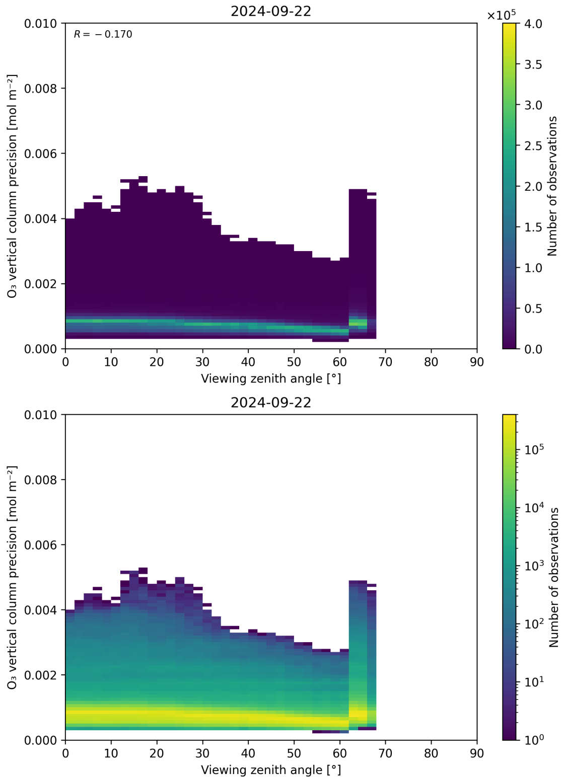
Figure 53: Scatter density plot of “Viewing zenith angle” against “O 3 vertical column precision” for 2024-09-22 to 2024-09-23.
