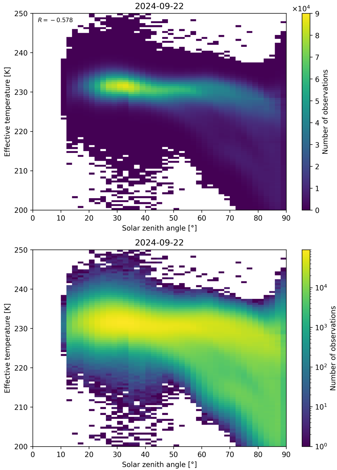
Figure 45: Scatter density plot of “Solar zenith angle” against “Effective temperature” for 2024-09-22 to 2024-09-23.
