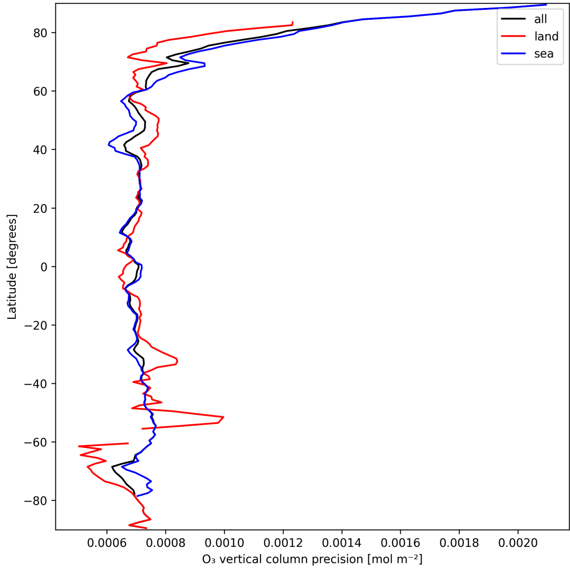
Figure 15: Zonal average of "O 3 vertical column precision" for 2024-09-22 to 2024-09-23.
