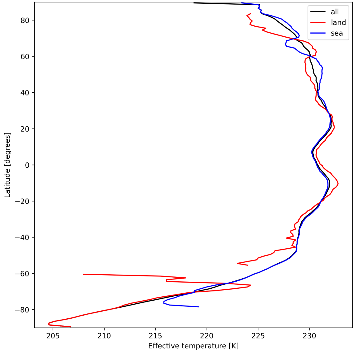
Figure 17: Zonal average of "Effective temperature" for 2024-09-22 to 2024-09-23.
