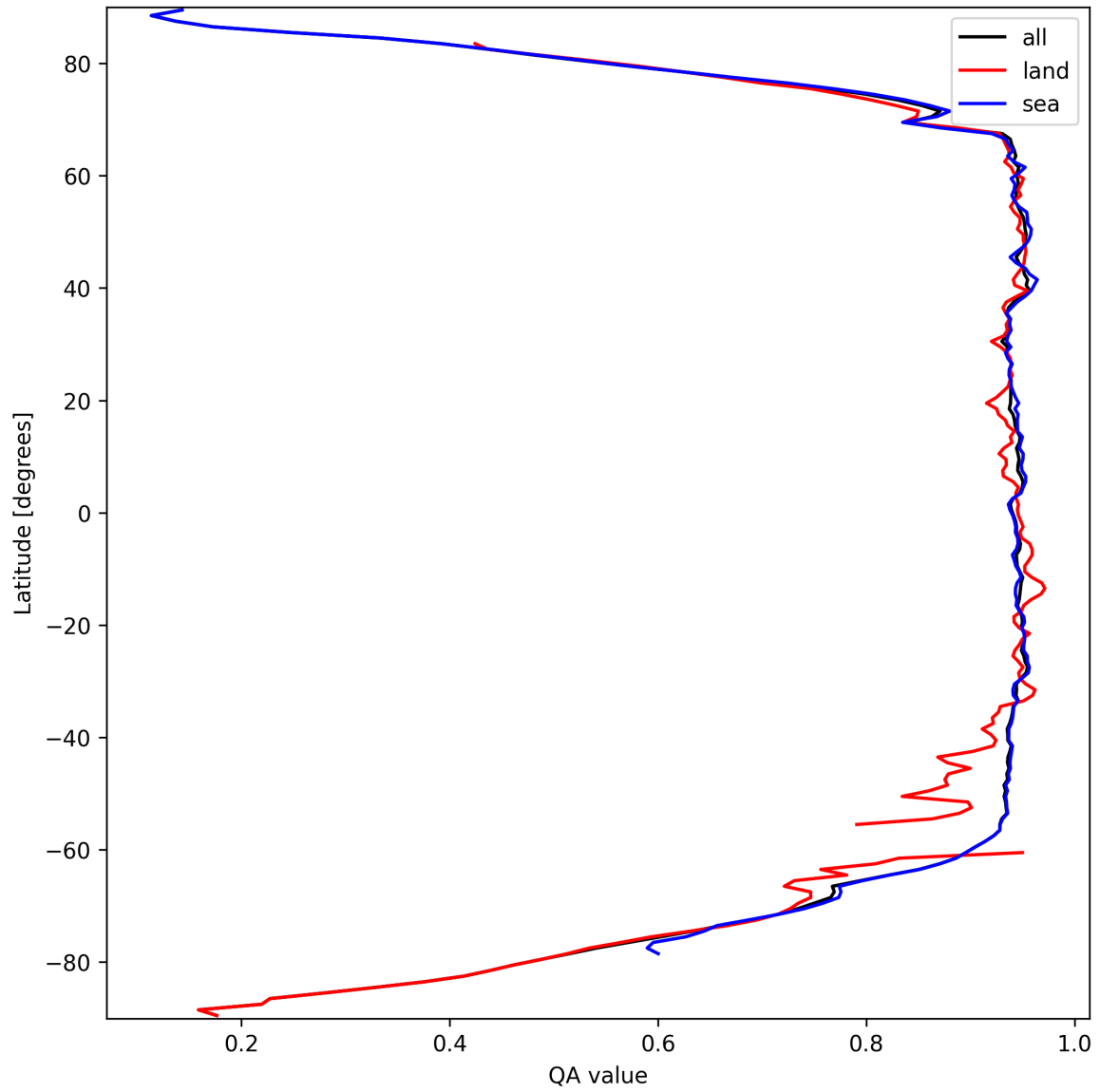
Figure 13: Zonal average of “QA value” for 2024-09-22 to 2024-09-23.
