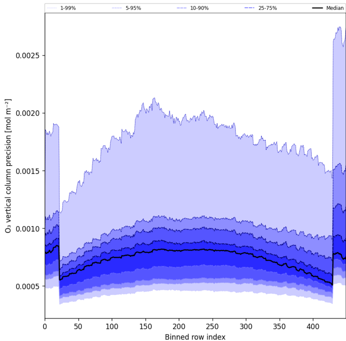
Figure 29: Along track statistics of “O 3 vertical column precision” for 2024-09-22 to 2024-09-23
