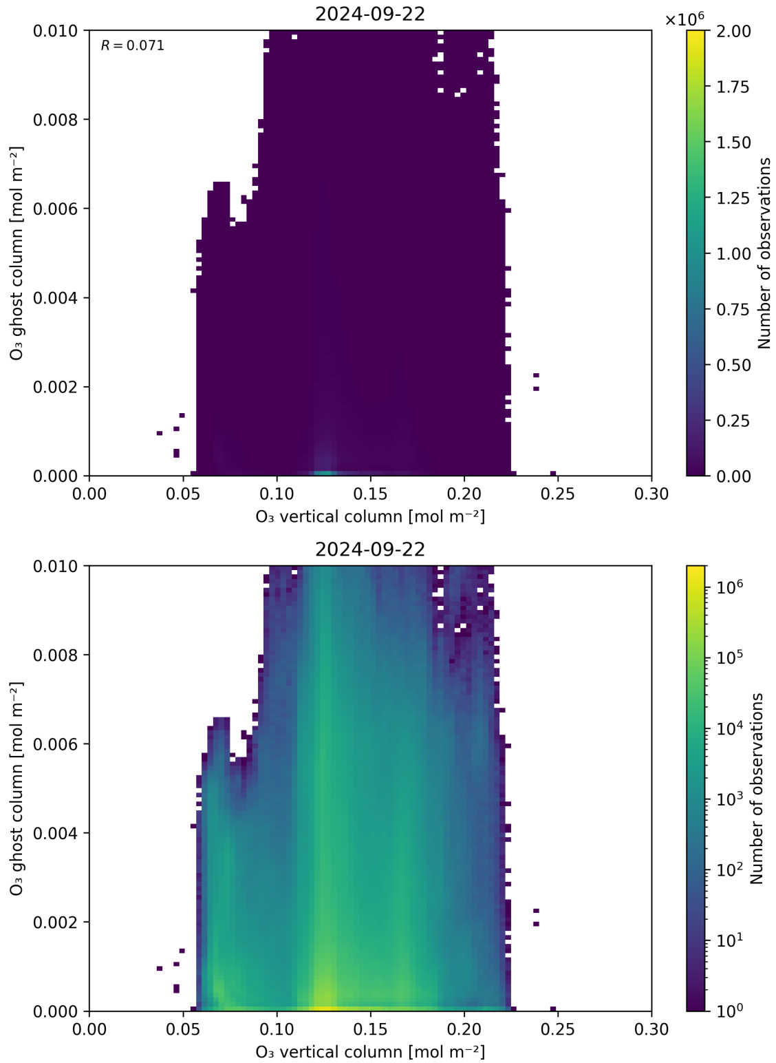
Figure 40: Scatter density plot of “O 3 vertical column” against “O 3 ghost column” for 2024-09-22 to 2024-09-23.
