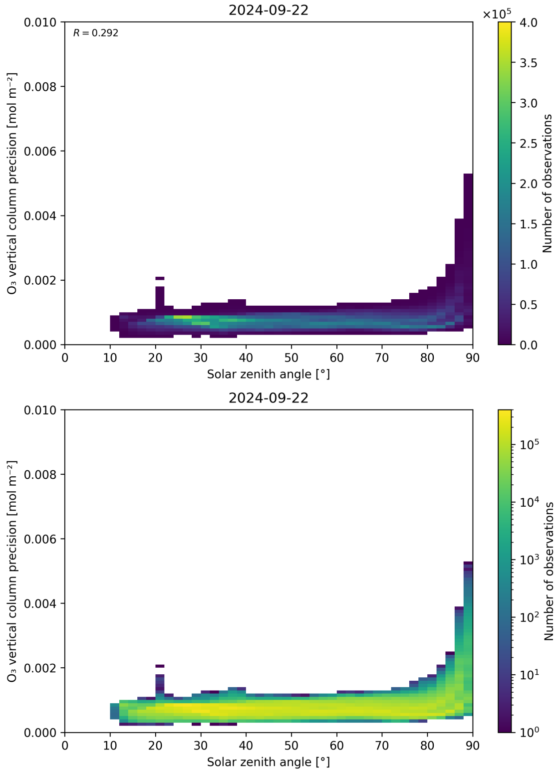
Figure 48: Scatter density plot of “Solar zenith angle” against “O 3 vertical column precision” for 2024-09-22 to 2024-09-23.
