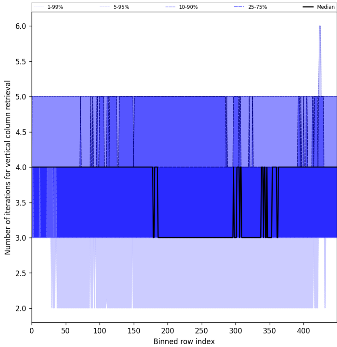
Figure 33: Along track statistics of “Number of iterations for vertical column retrieval” for 2024-09-22 to 2024-09-23
