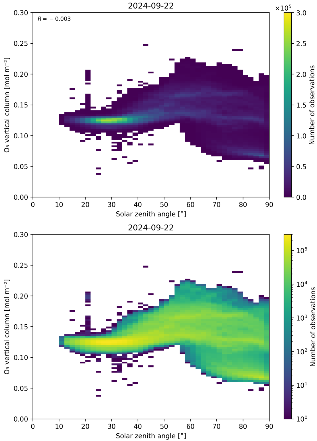
Figure 47: Scatter density plot of “Solar zenith angle” against “O 3 vertical column” for 2024-09-22 to 2024-09-23.
