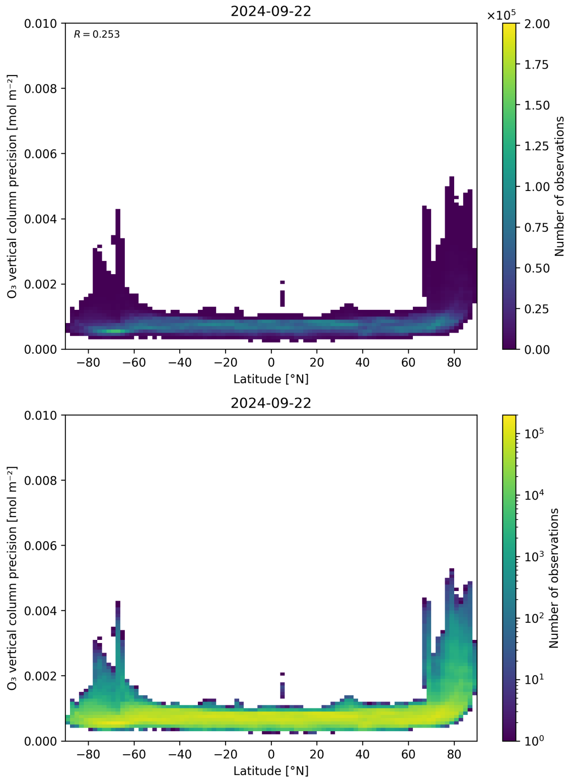
Figure 37: Scatter density plot of “Latitude” against “O 3 vertical column precision” for 2024-09-22 to 2024-09-23.
