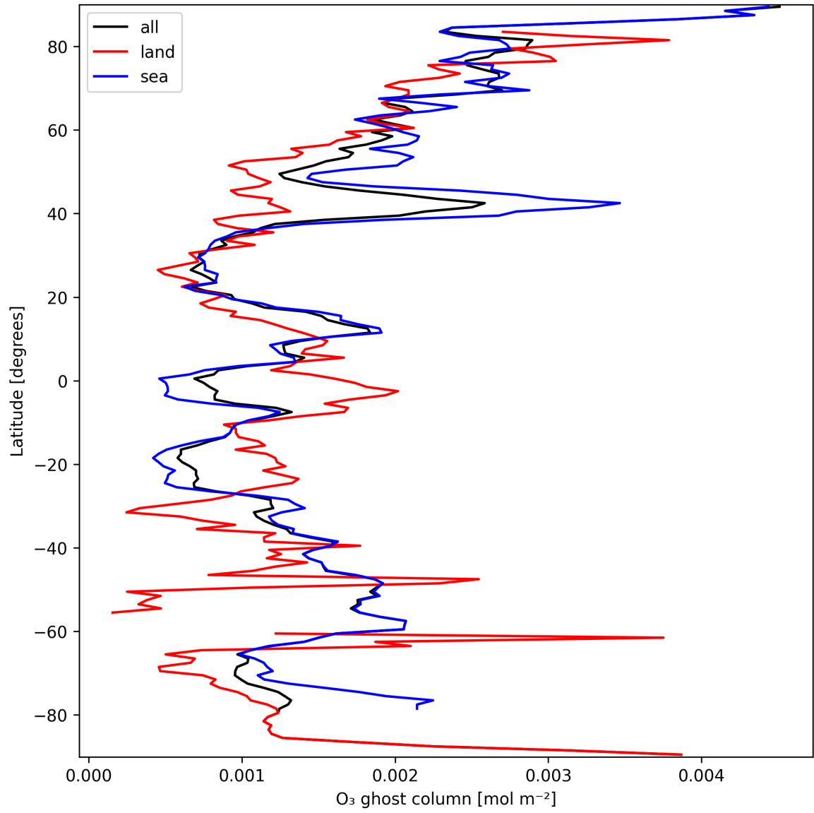
Figure 18: Zonal average of "O 3 ghost column" for 2024-09-22 to 2024-09-23.
