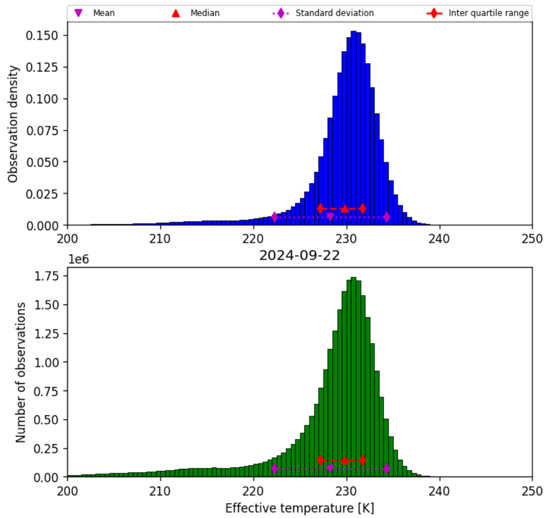
Figure 24: Histogram of “Effective temperature” for 2024-09-22 to 2024-09-23
