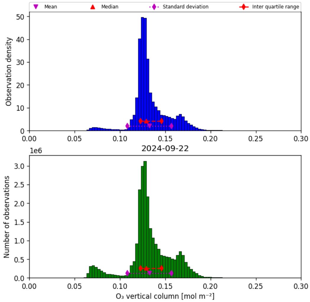
Figure 21: Histogram of “O 3 vertical column” for 2024-09-22 to 2024-09-23
