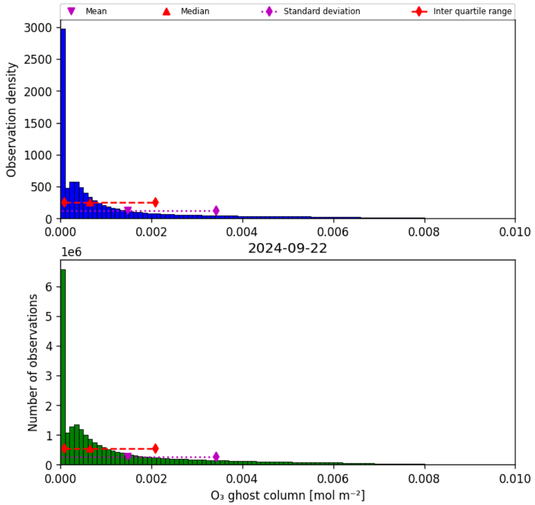
Figure 25: Histogram of “O 3 ghost column” for 2024-09-22 to 2024-09-23
