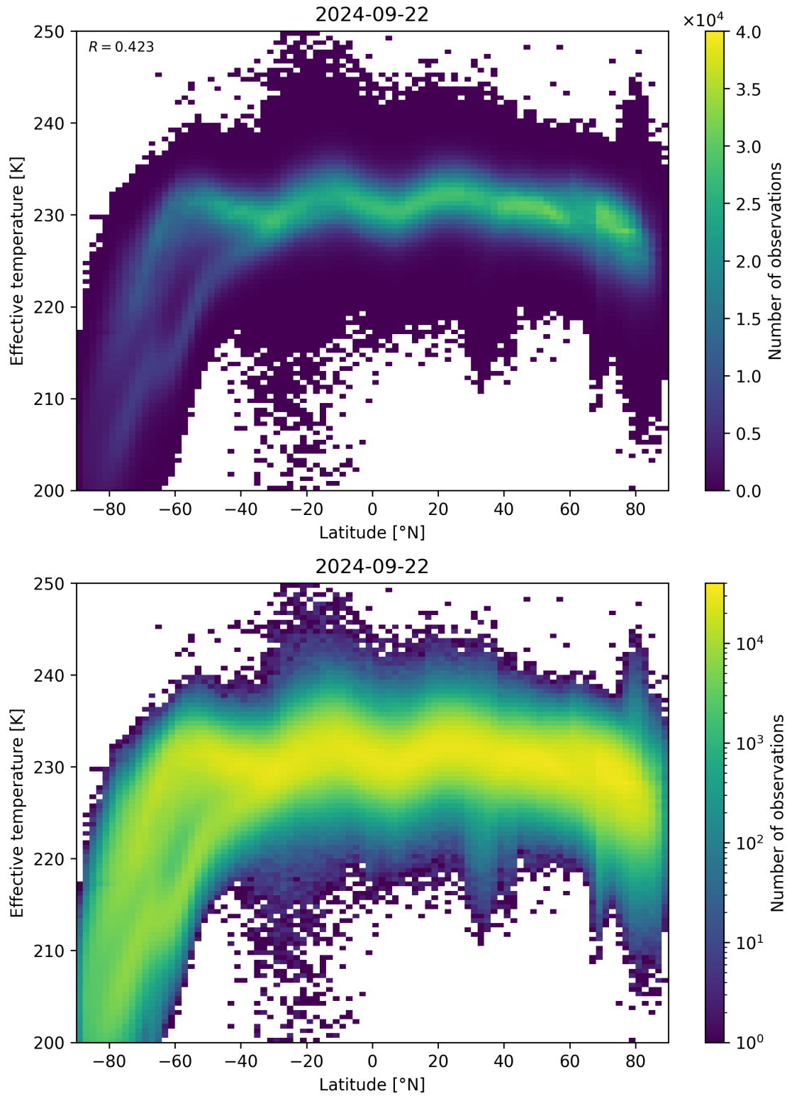
Figure 34: Scatter density plot of “Latitude” against “Effective temperature” for 2024-09-22 to 2024-09-23.
