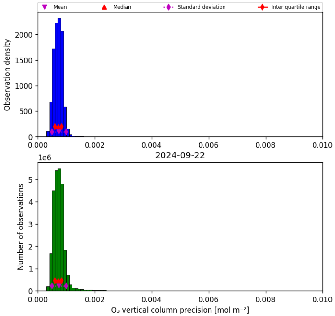
Figure 22: Histogram of “O 3 vertical column precision” for 2024-09-22 to 2024-09-23
