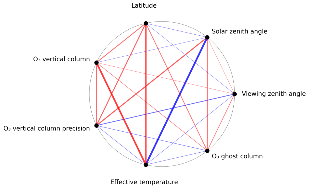
Figure 1: Map of correlation graph for 2024-09-22 to 2024-09-23.
