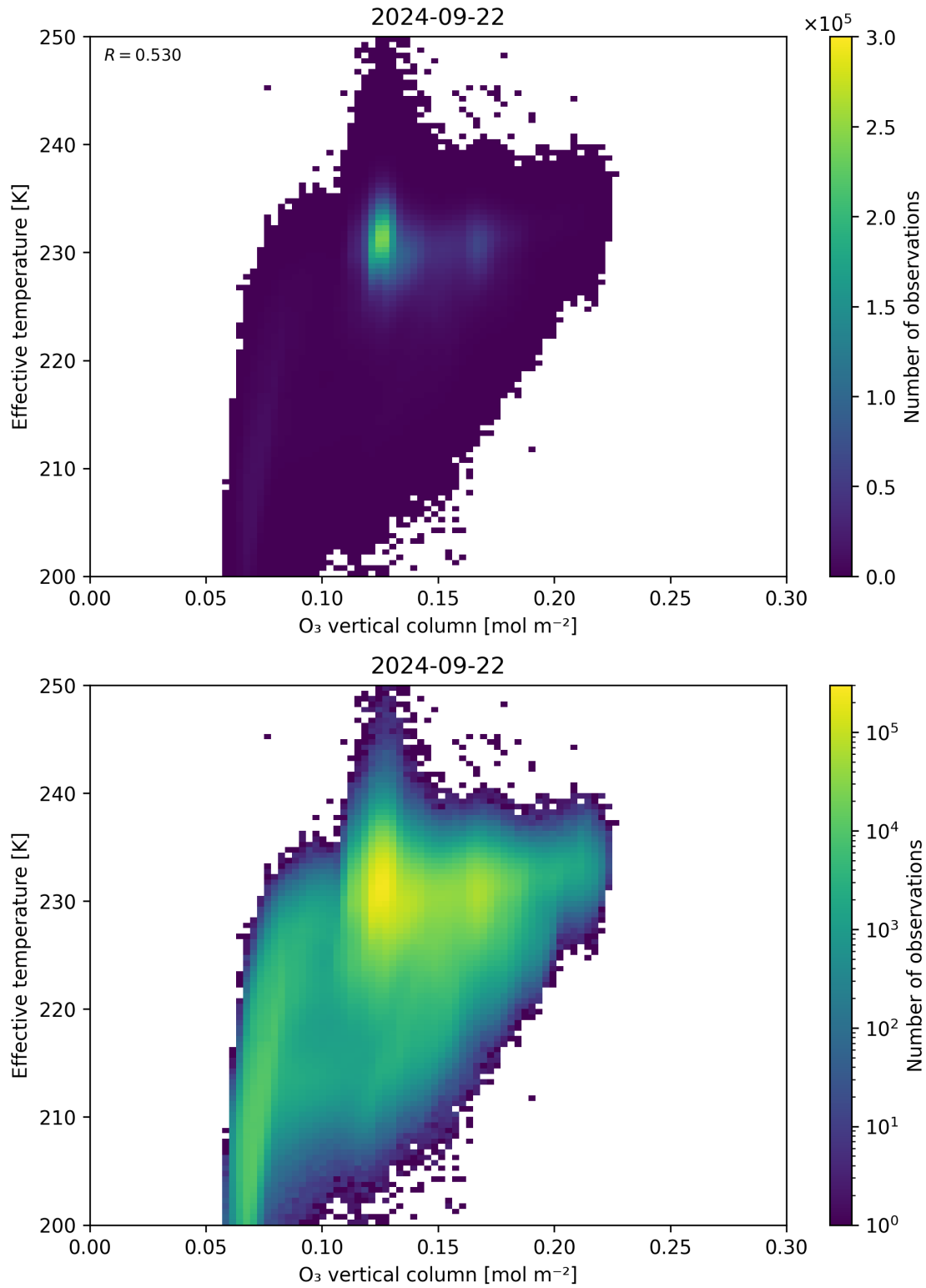
Figure 39: Scatter density plot of “O 3 vertical column” against “Effective temperature” for 2024-09-22 to 2024-09-23.
