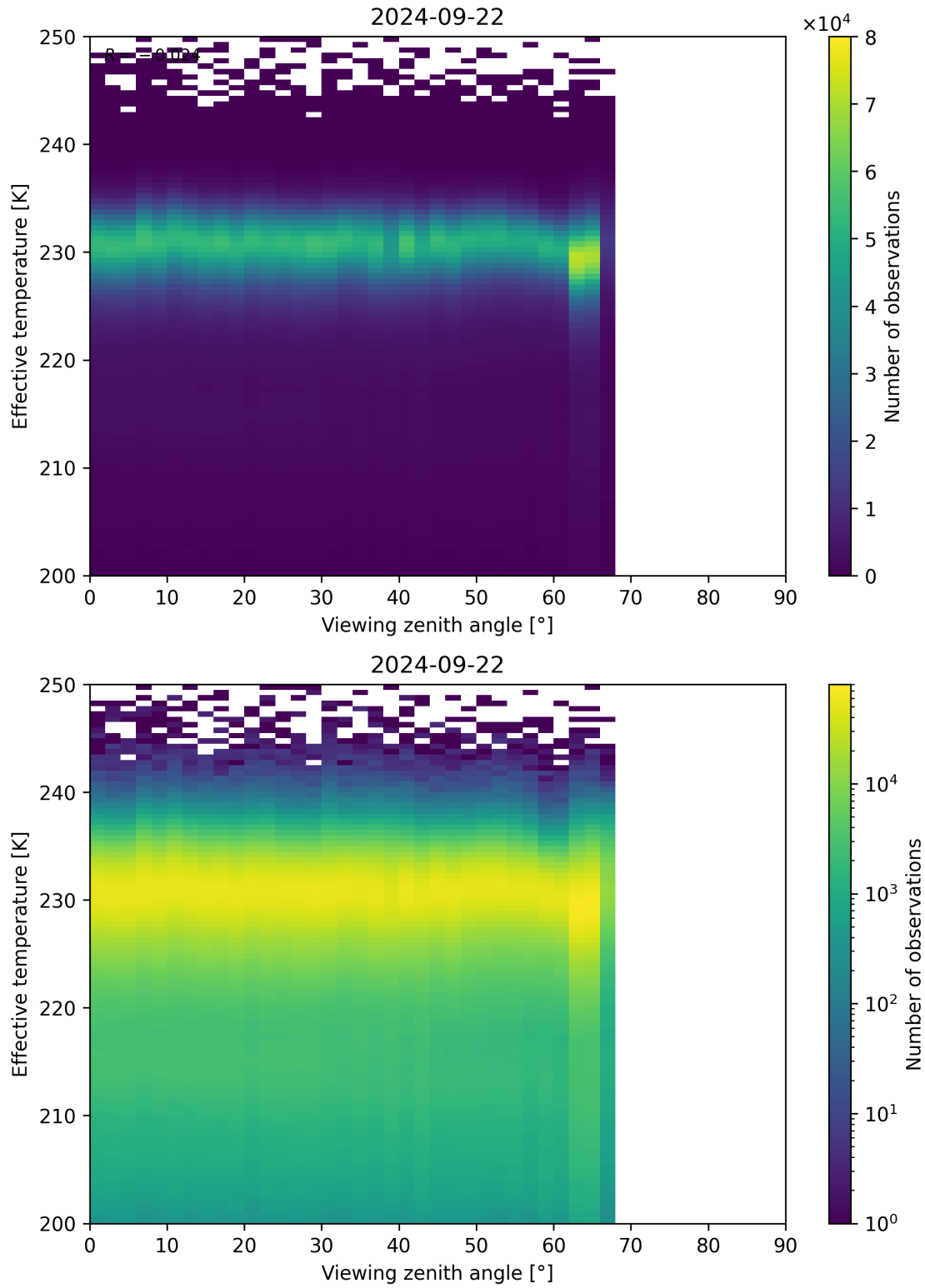
Figure 50: Scatter density plot of “Viewing zenith angle” against “Effective temperature” for 2024-09-22 to 2024-09-23.
