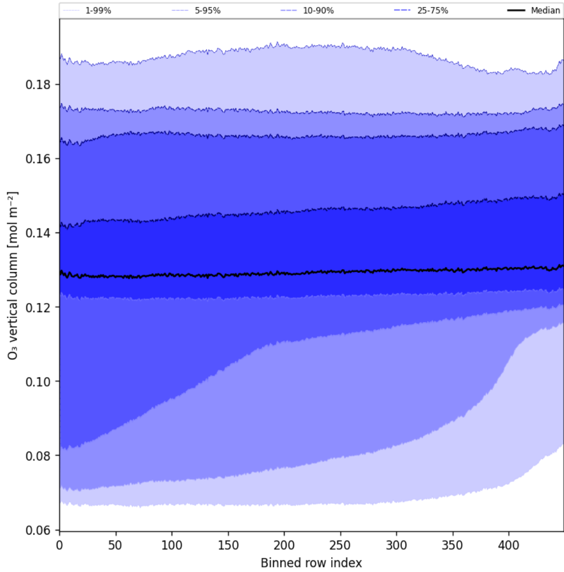
Figure 28: Along track statistics of “O 3 vertical column” for 2024-09-22 to 2024-09-23
