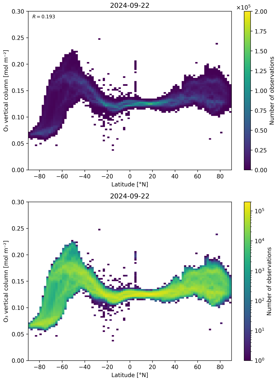
Figure 36: Scatter density plot of “Latitude” against “O 3 vertical column” for 2024-09-22 to 2024-09-23.
