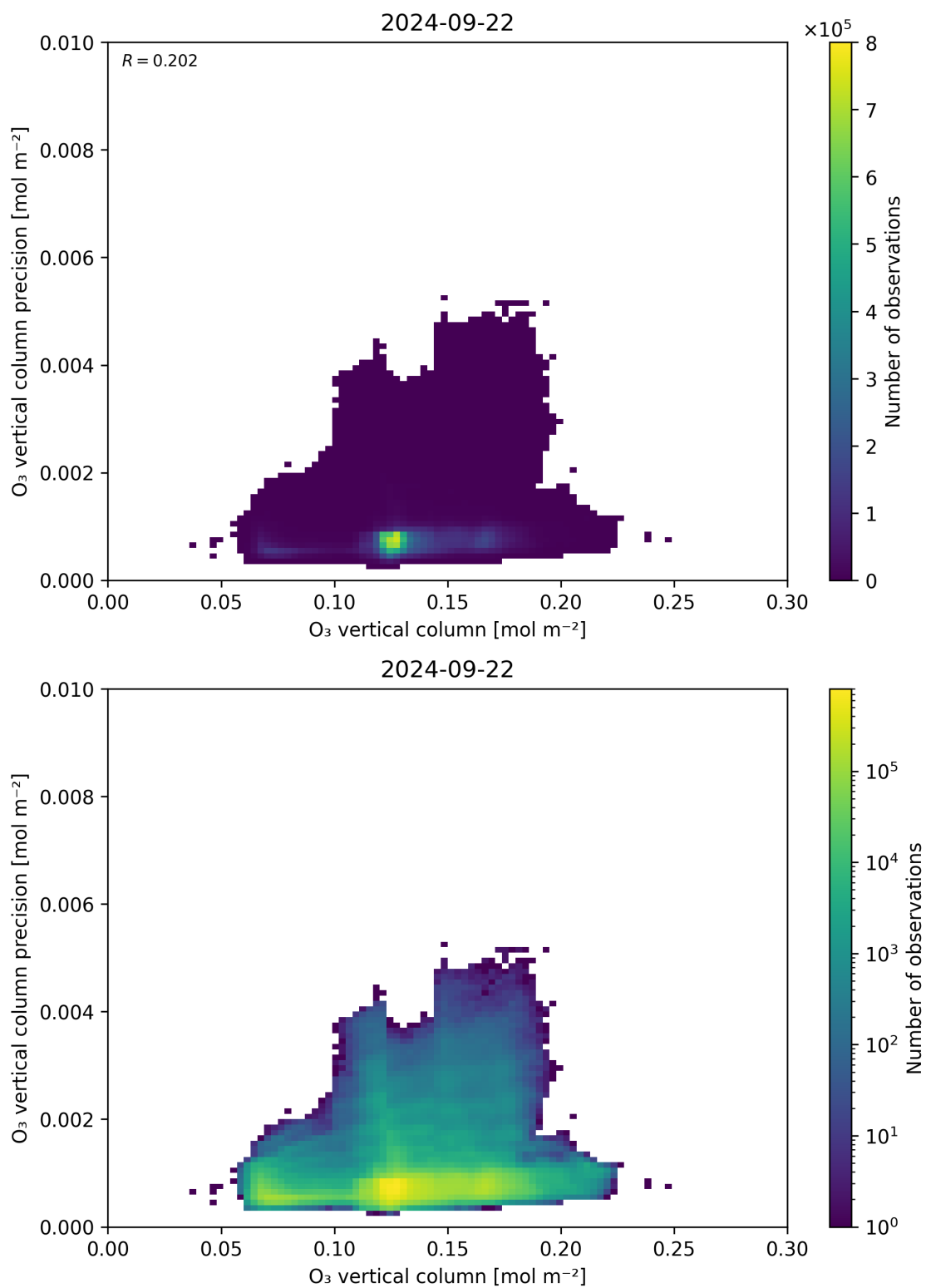
Figure 41: Scatter density plot of “O 3 vertical column” against “O 3 vertical column precision” for 2024-09-22 to 2024-09-23.
