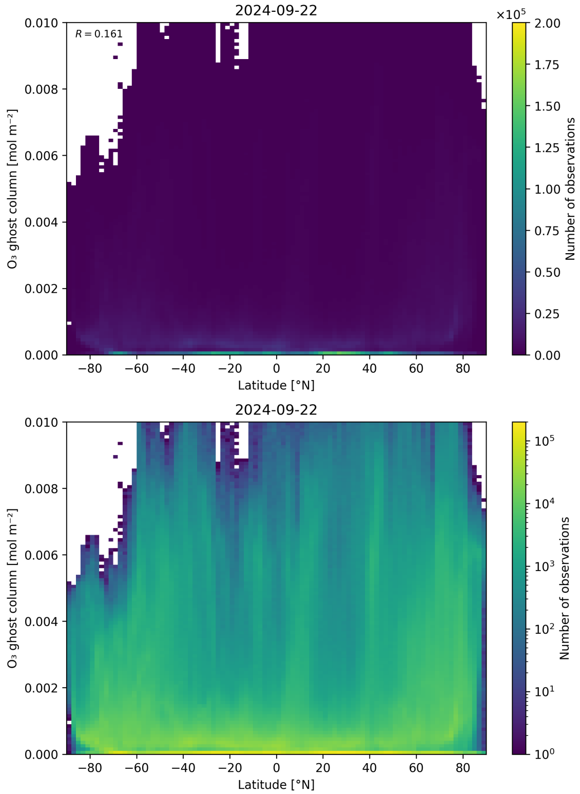
Figure 35: Scatter density plot of “Latitude” against “O 3 ghost column” for 2024-09-22 to 2024-09-23.
