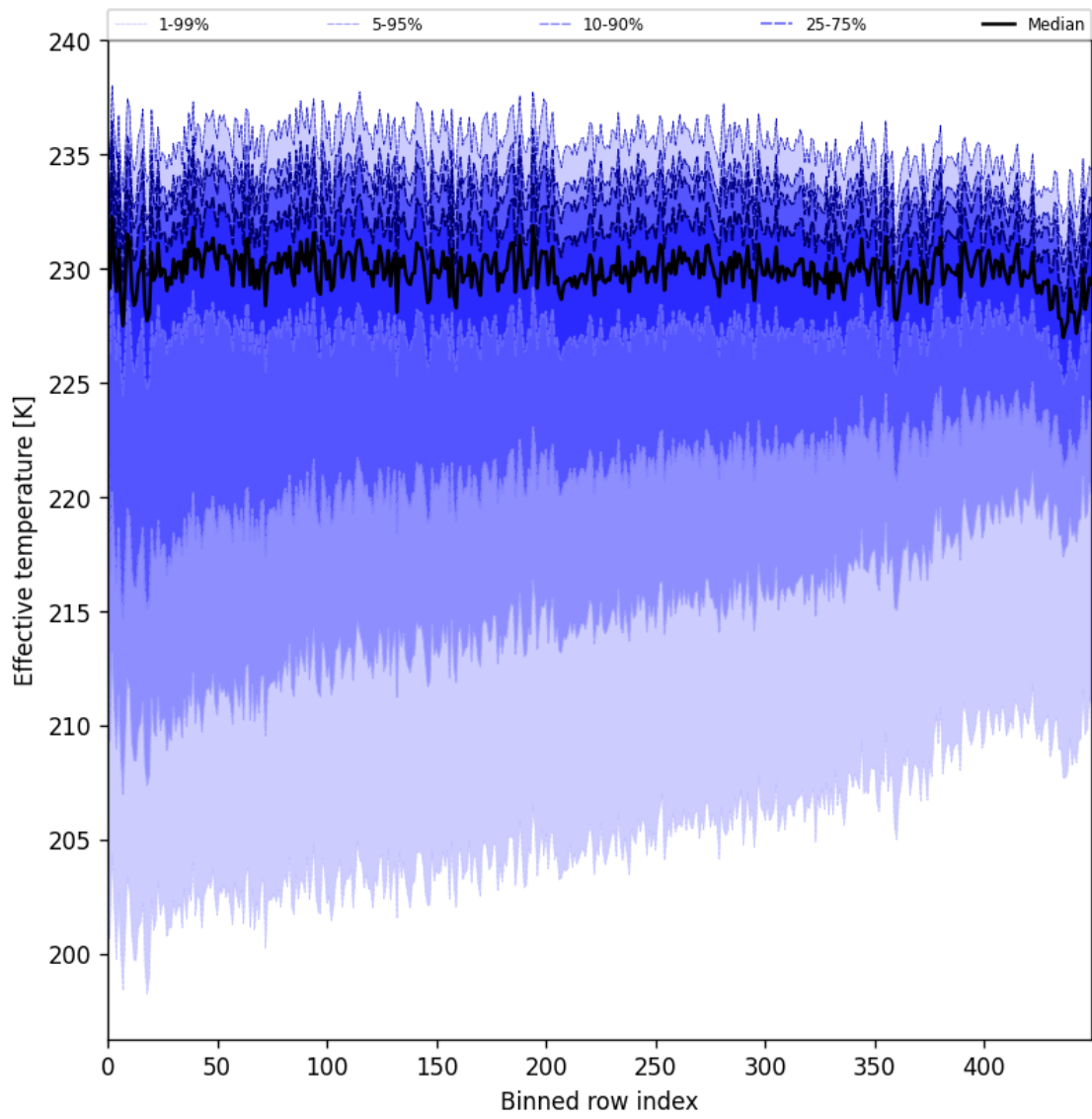
Figure 31: Along track statistics of “Effective temperature” for 2024-09-22 to 2024-09-23
