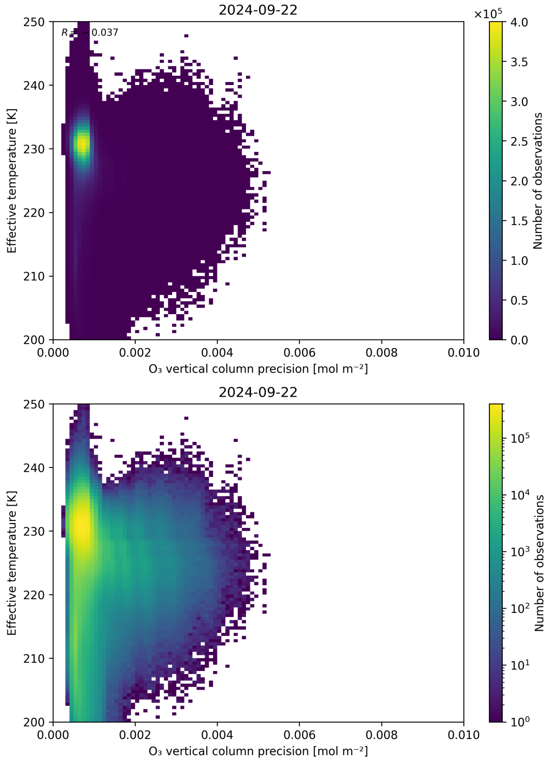
Figure 42: Scatter density plot of “ O_3 vertical column precision” against “Effective temperature” for 2024-09-22 to 2024-09-23.
