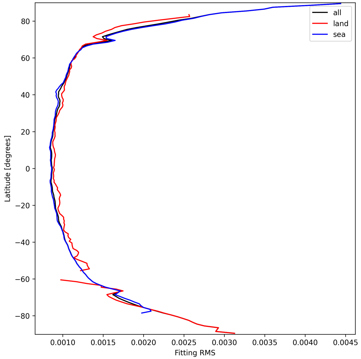
Figure 16: Zonal average of “Fitting RMS” for 2024-09-22 to 2024-09-23.
