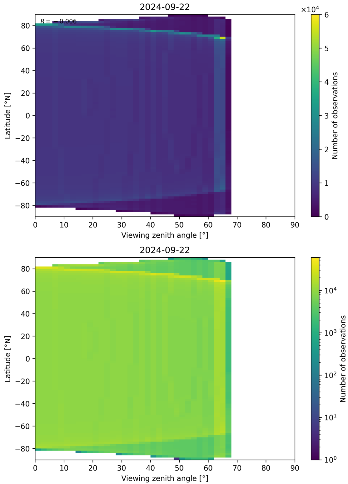
Figure 49: Scatter density plot of “Viewing zenith angle” against “Latitude” for 2024-09-22 to 2024-09-23.
