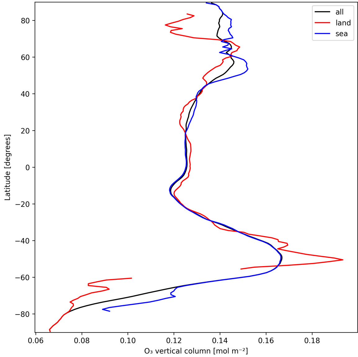
Figure 14: Zonal average of “O 3 vertical column” for 2024-09-22 to 2024-09-23.
