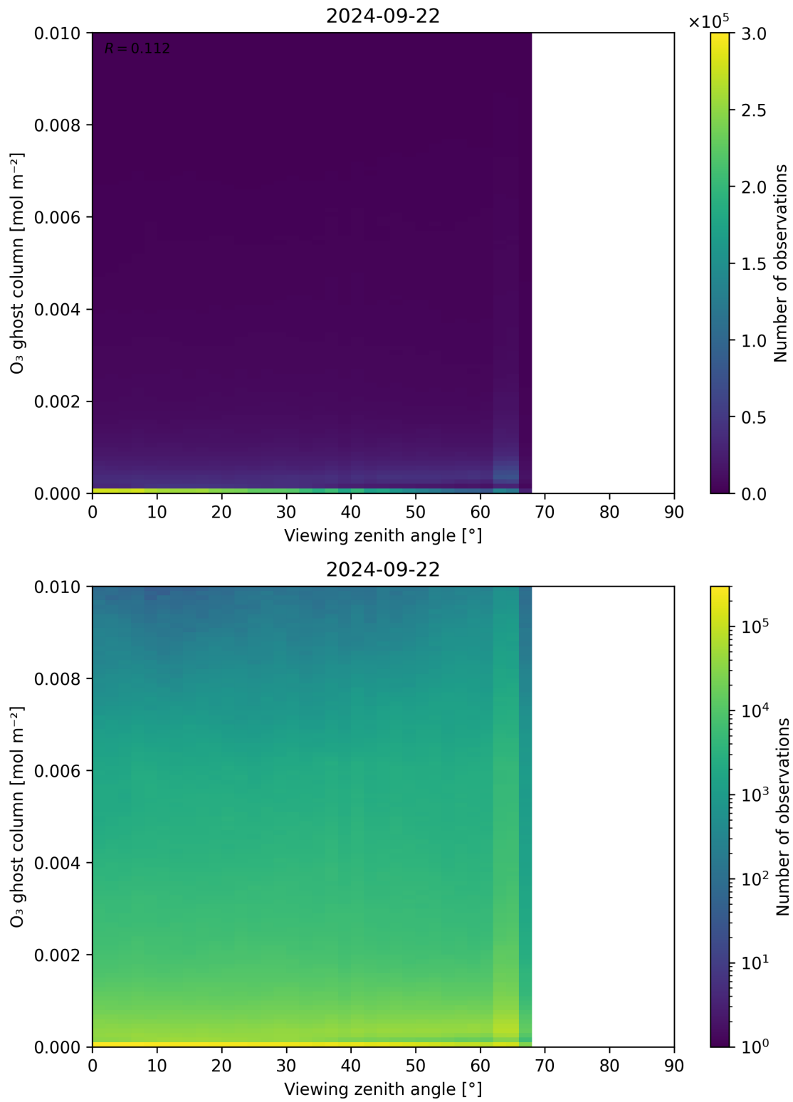
Figure 51: Scatter density plot of “Viewing zenith angle” against “O 3 ghost column” for 2024-09-22 to 2024-09-23.
