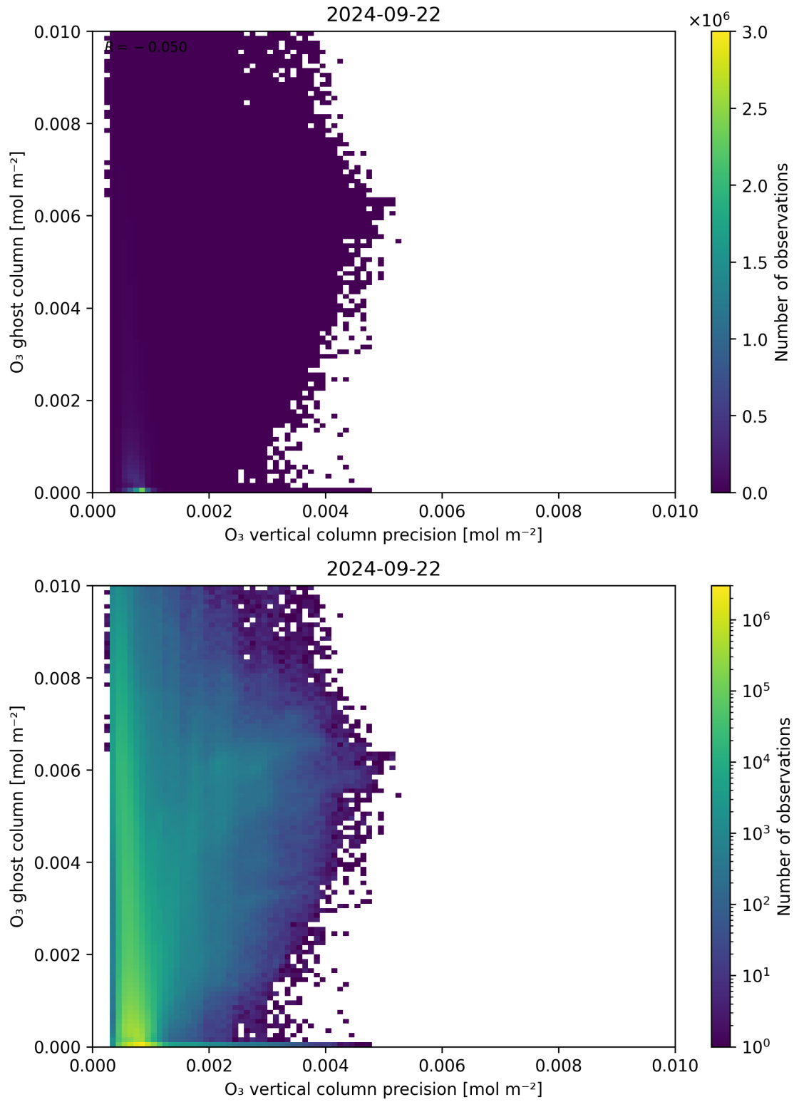
Figure 43: Scatter density plot of “O 3 vertical column precision” against “O 3 ghost column” for 2024-09-22 to 2024-09-23.
