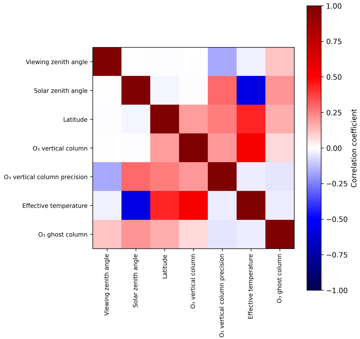
Figure 2: Map of correlation matrix for 2024-09-22 to 2024-09-23.
