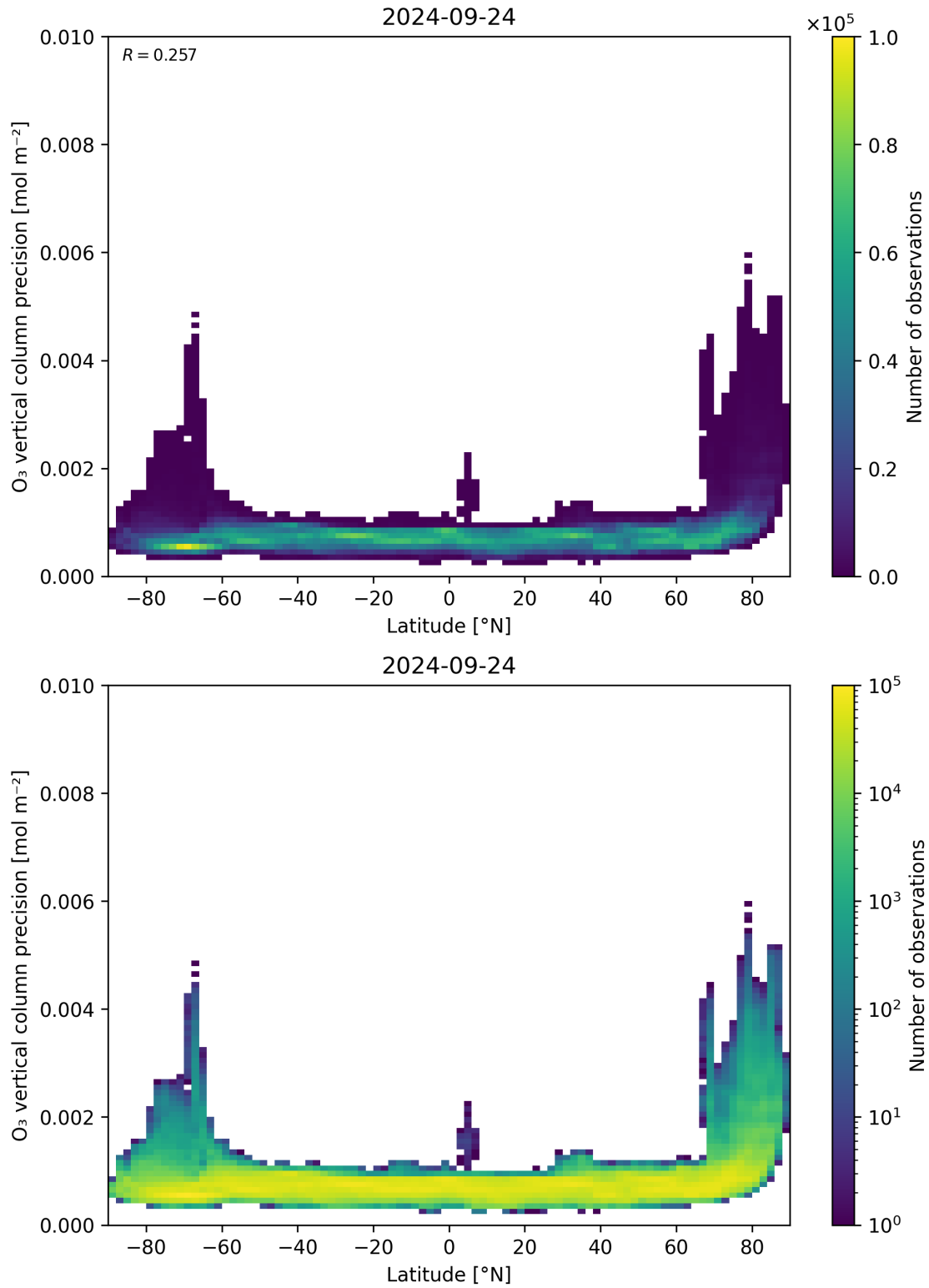
Figure 37: Scatter density plot of “Latitude” against “O 3 vertical column precision” for 2024-09-23 to 2024-09-25.
