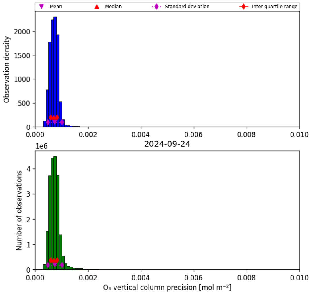
Figure 22: Histogram of “O 3 vertical column precision” for 2024-09-23 to 2024-09-25
