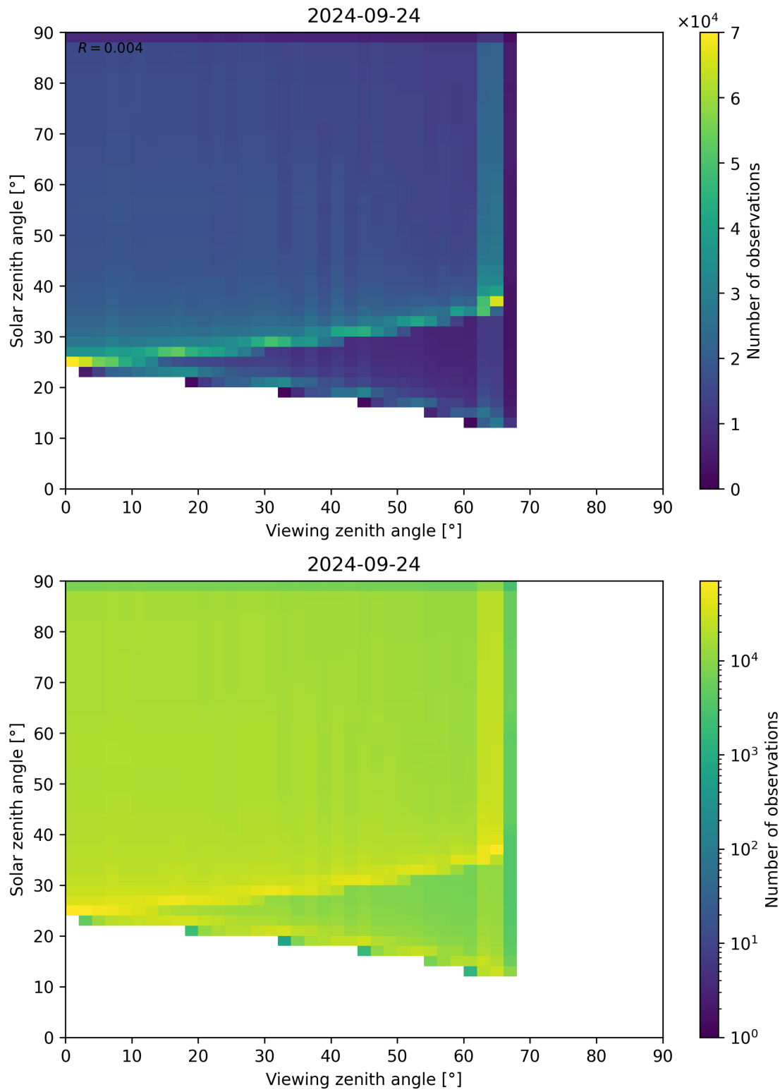
Figure 54: Scatter density plot of “Viewing zenith angle” against “Solar zenith angle” for 2024-09-23 to 2024-09-25.
