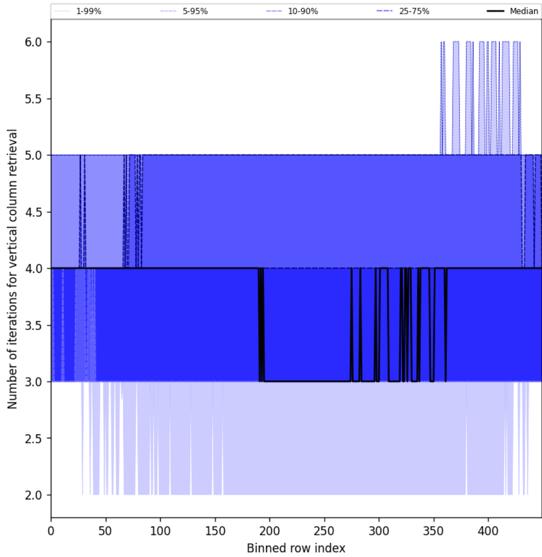
Figure 33: Along track statistics of “Number of iterations for vertical column retrieval” for 2024-09-23 to 2024-09-25
