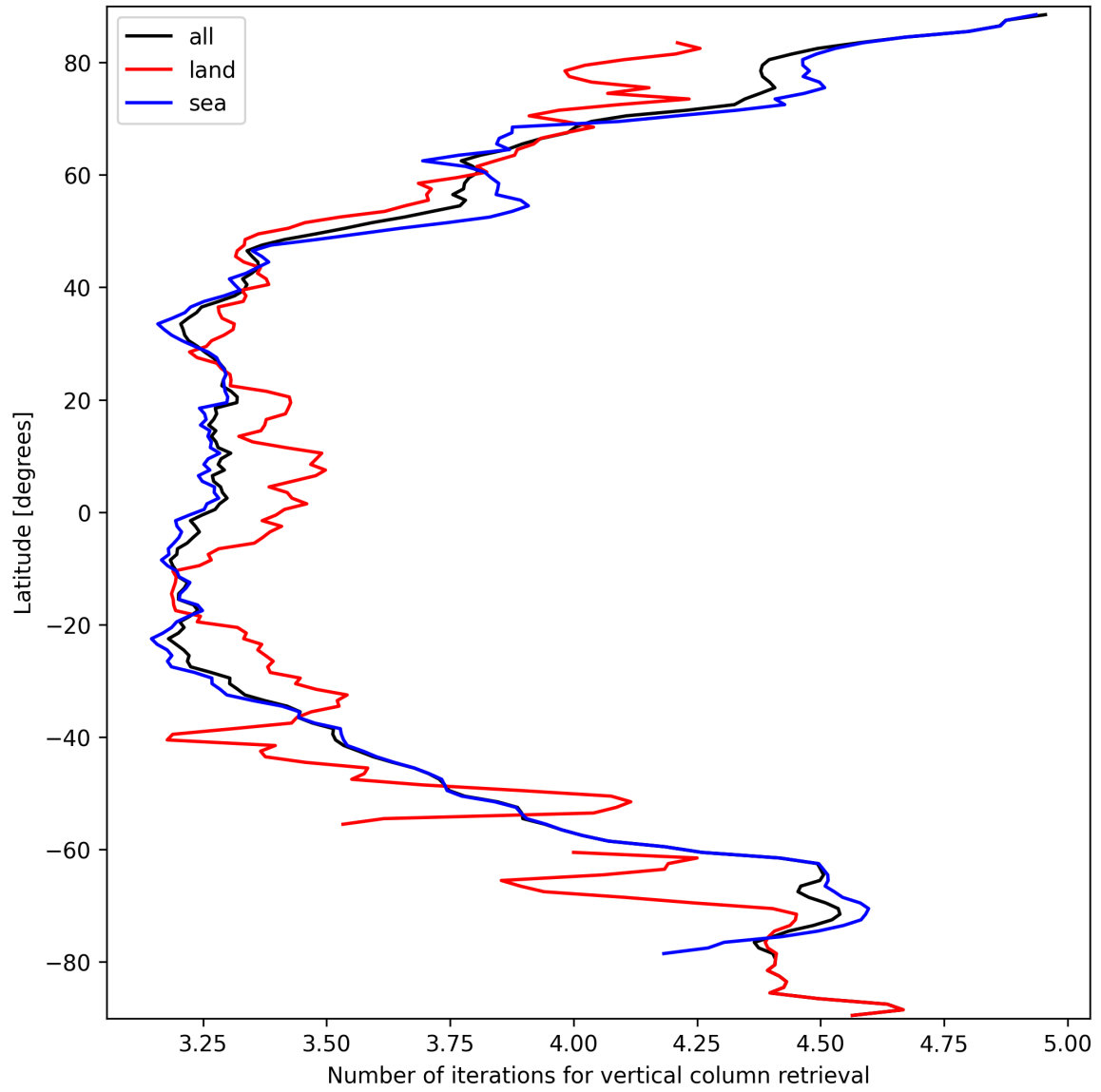
Figure 19: Zonal average of “Number of iterations for vertical column retrieval” for 2024-09-23 to 2024-09-25.
