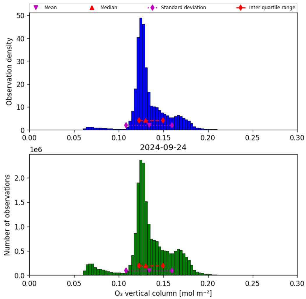
Figure 21: Histogram of “O 3 vertical column” for 2024-09-23 to 2024-09-25
