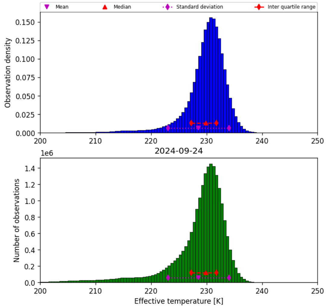
Figure 24: Histogram of “Effective temperature” for 2024-09-23 to 2024-09-25
