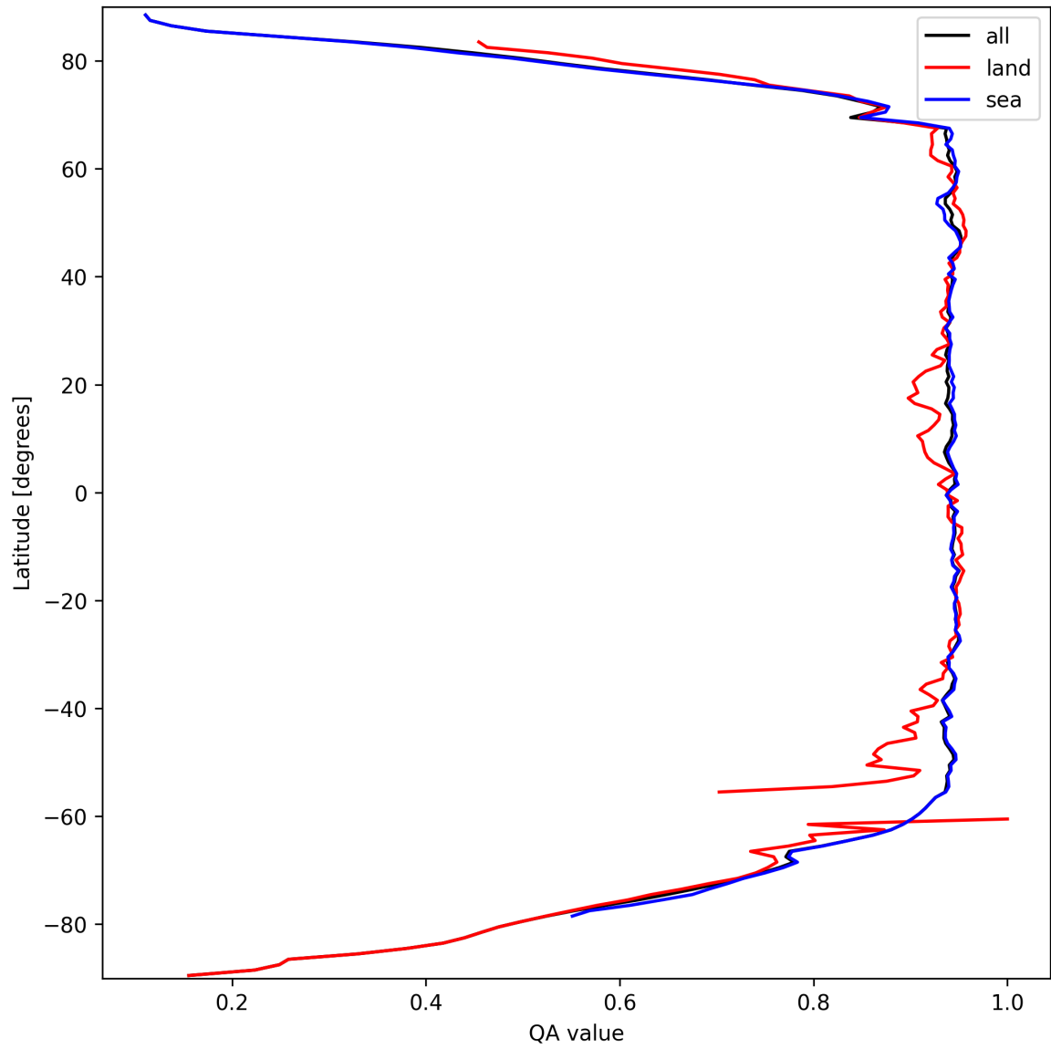
Figure 13: Zonal average of “QA value” for 2024-09-23 to 2024-09-25.
