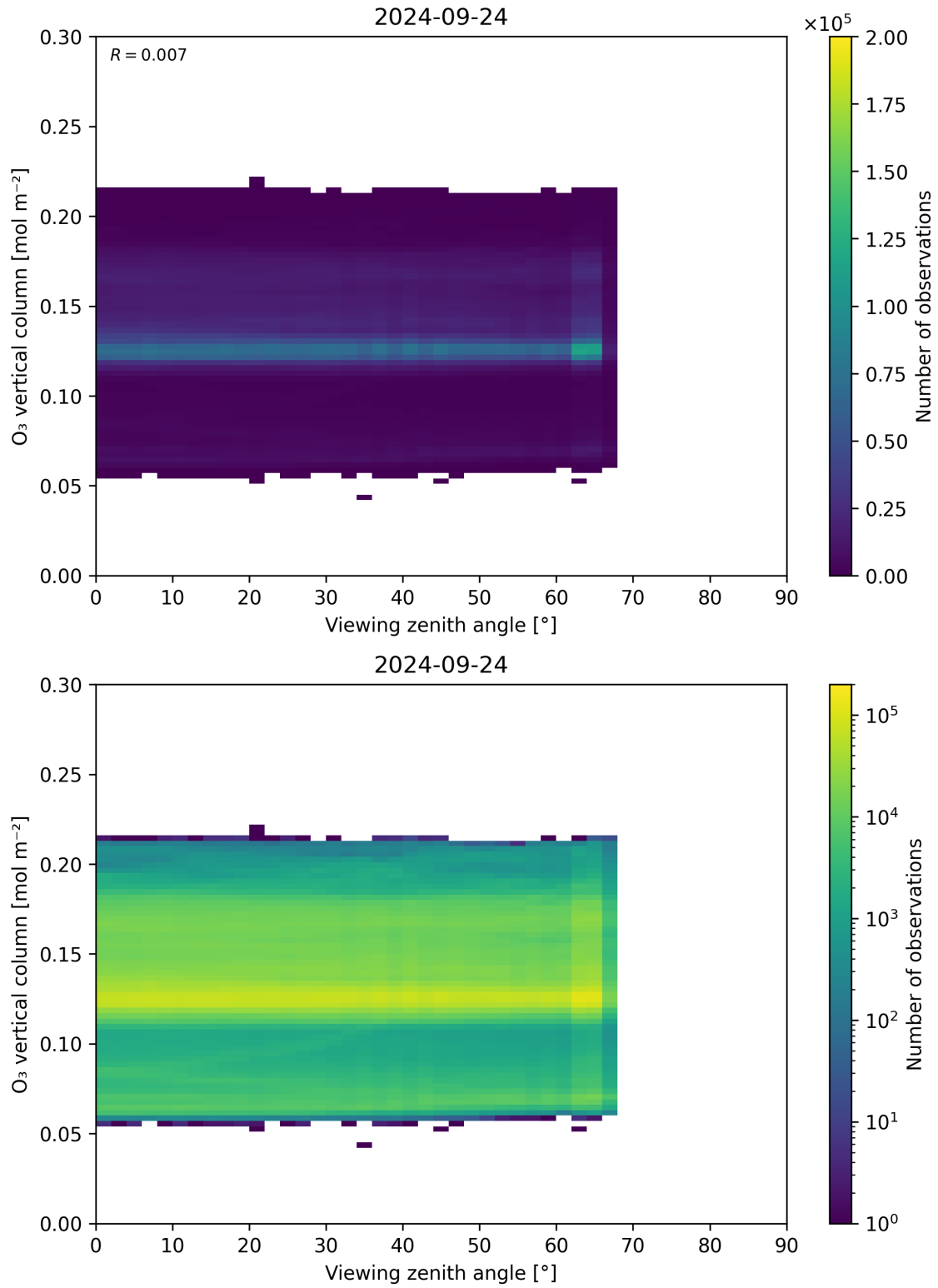
Figure 52: Scatter density plot of “Viewing zenith angle” against “O 3 vertical column” for 2024-09-23 to 2024-09-25.
