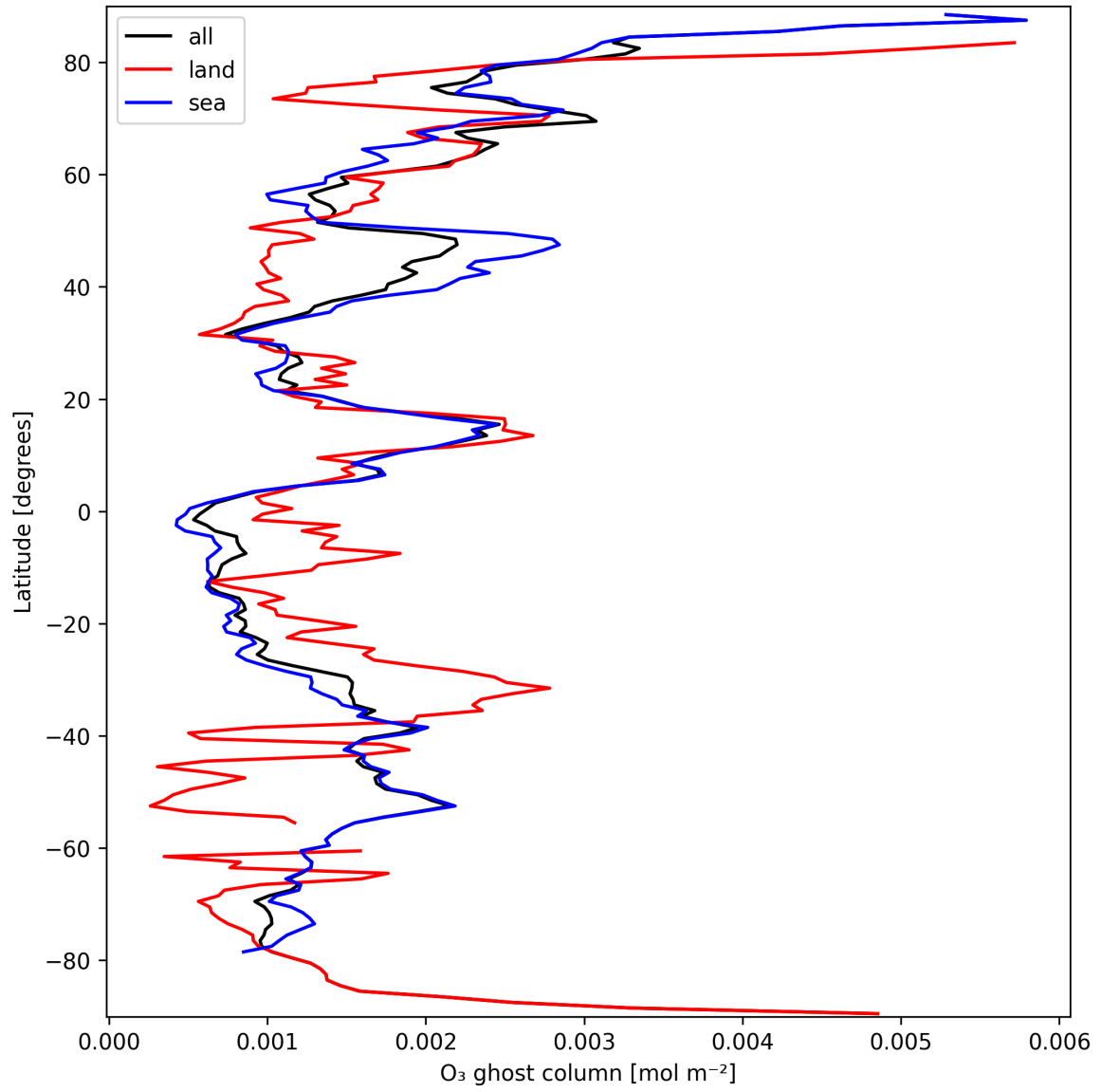
Figure 18: Zonal average of “O 3 ghost column” for 2024-09-23 to 2024-09-25.
