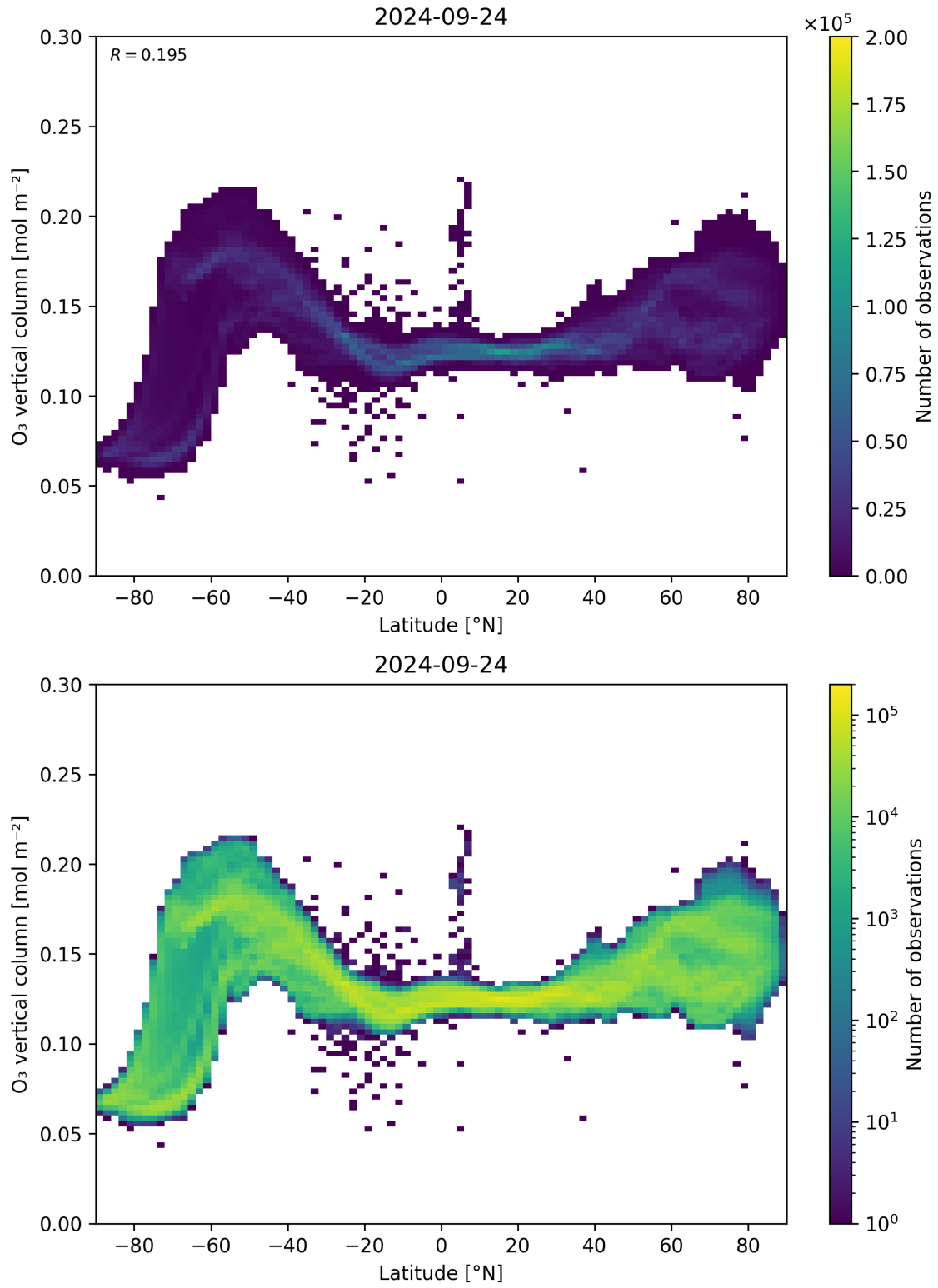
Figure 36: Scatter density plot of “Latitude” against “O 3 vertical column” for 2024-09-23 to 2024-09-25.
