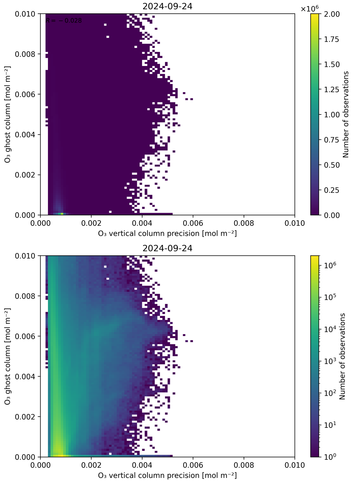
Figure 43: Scatter density plot of “ \text{O}_3 vertical column precision” against “ \text{O}_3 ghost column” for 2024-09-23 to 2024-09-25.
