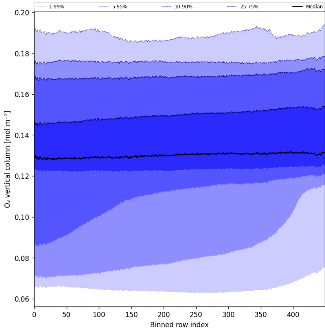
Figure 28: Along track statistics of “O 3 vertical column” for 2024-09-23 to 2024-09-25
