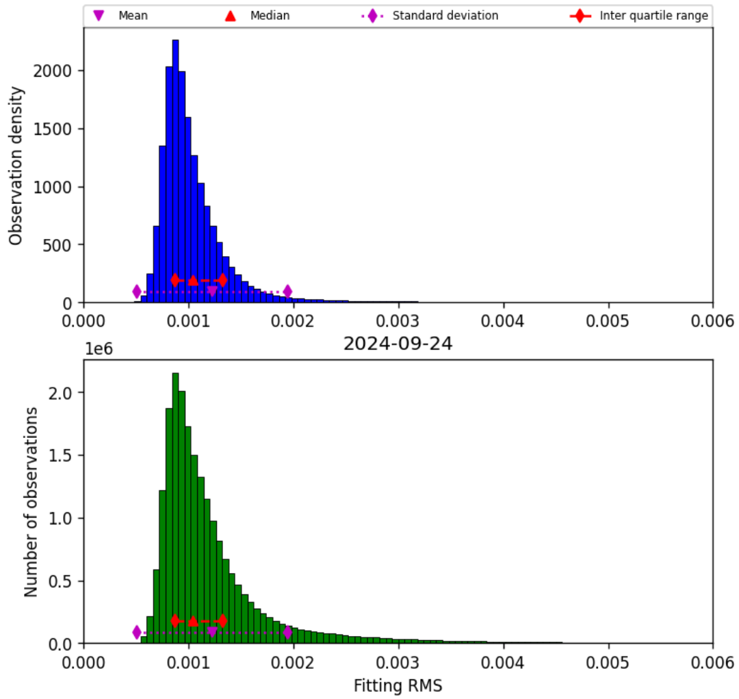
Figure 23: Histogram of “Fitting RMS” for 2024-09-23 to 2024-09-25
