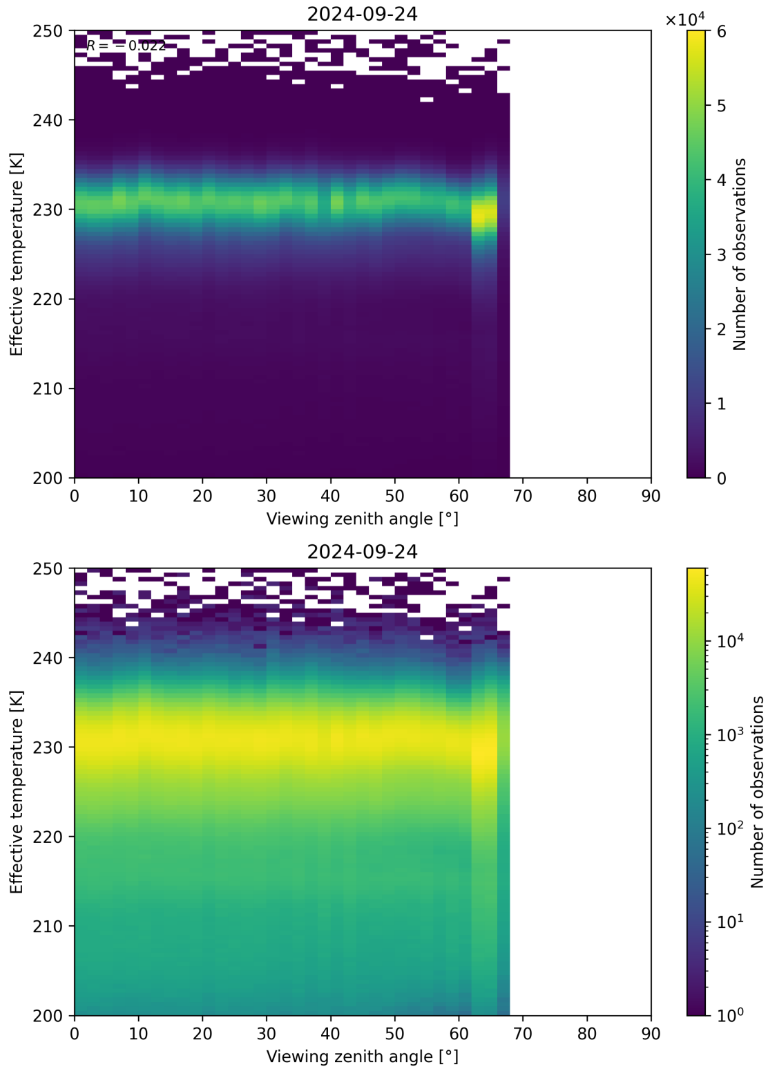
Figure 50: Scatter density plot of “Viewing zenith angle” against “Effective temperature” for 2024-09-23 to 2024-09-25.
