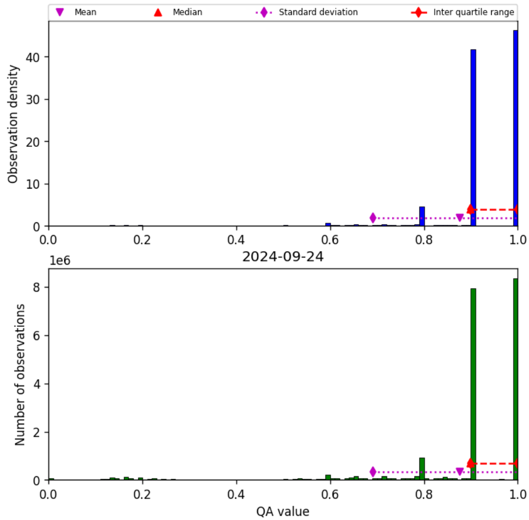
Figure 20: Histogram of “QA value” for 2024-09-23 to 2024-09-25
