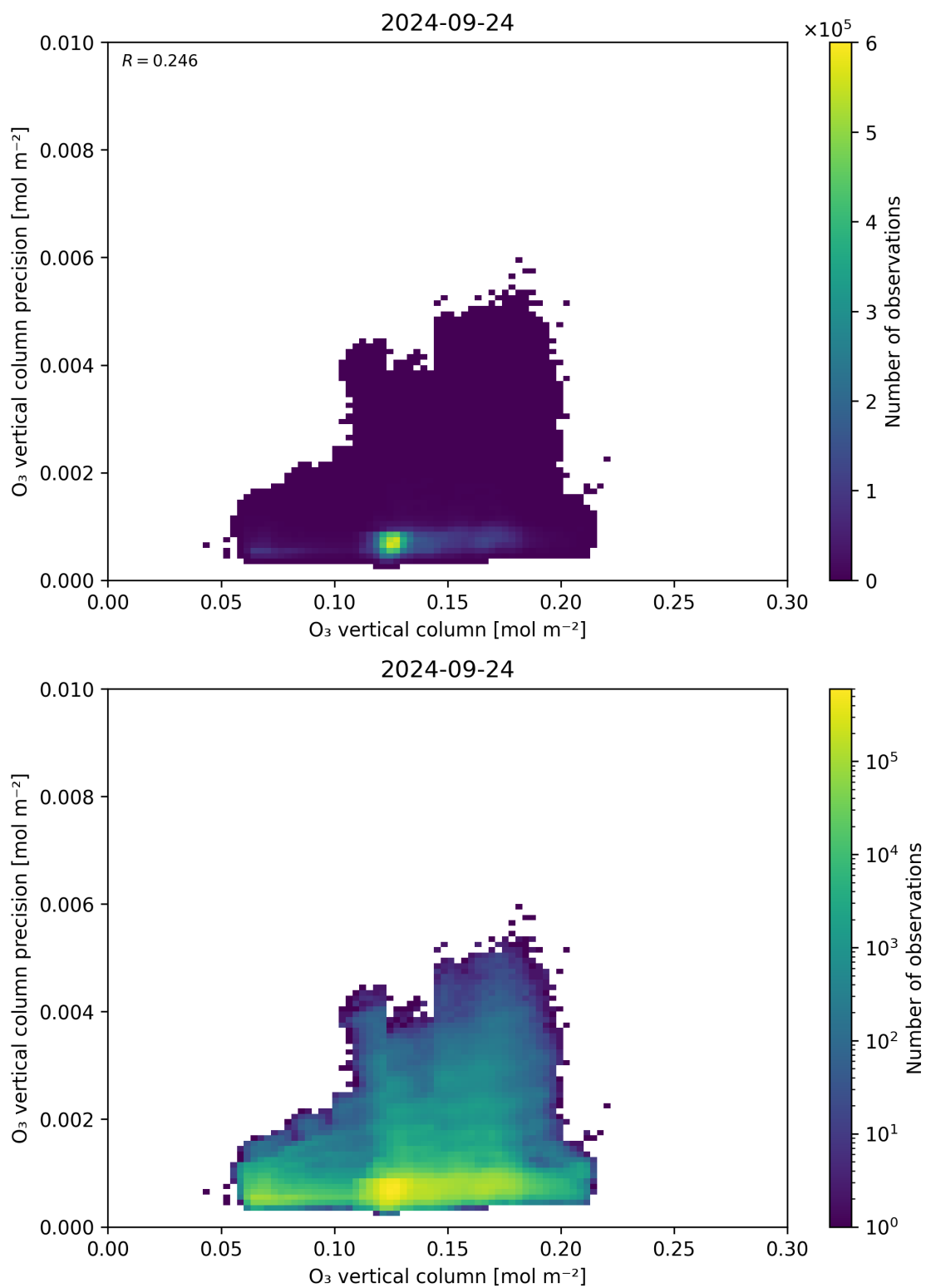
Figure 41: Scatter density plot of “O 3 vertical column” against “O 3 vertical column precision” for 2024-09-23 to 2024-09-25.
