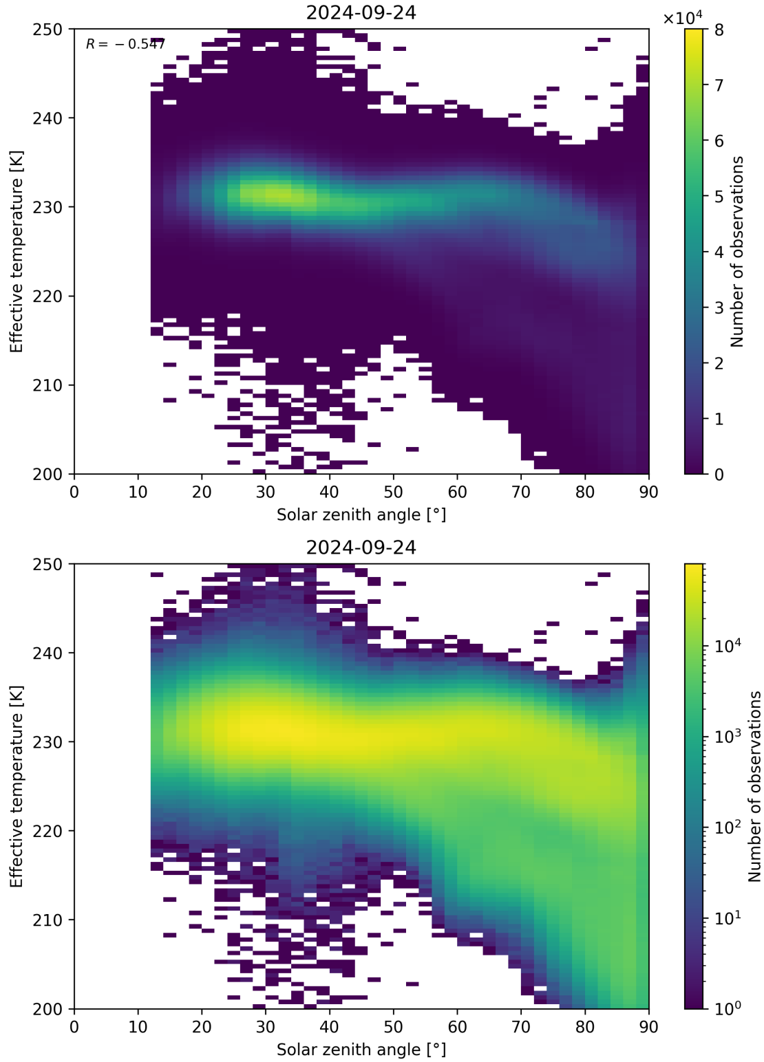
Figure 45: Scatter density plot of “Solar zenith angle” against “Effective temperature” for 2024-09-23 to 2024-09-25.
