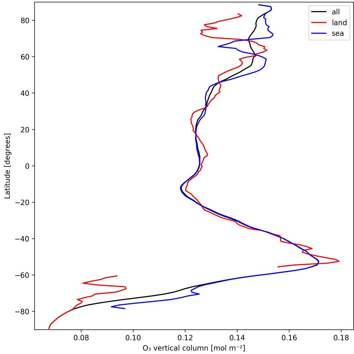
Figure 14: Zonal average of “O 3 vertical column” for 2024-09-23 to 2024-09-25.
