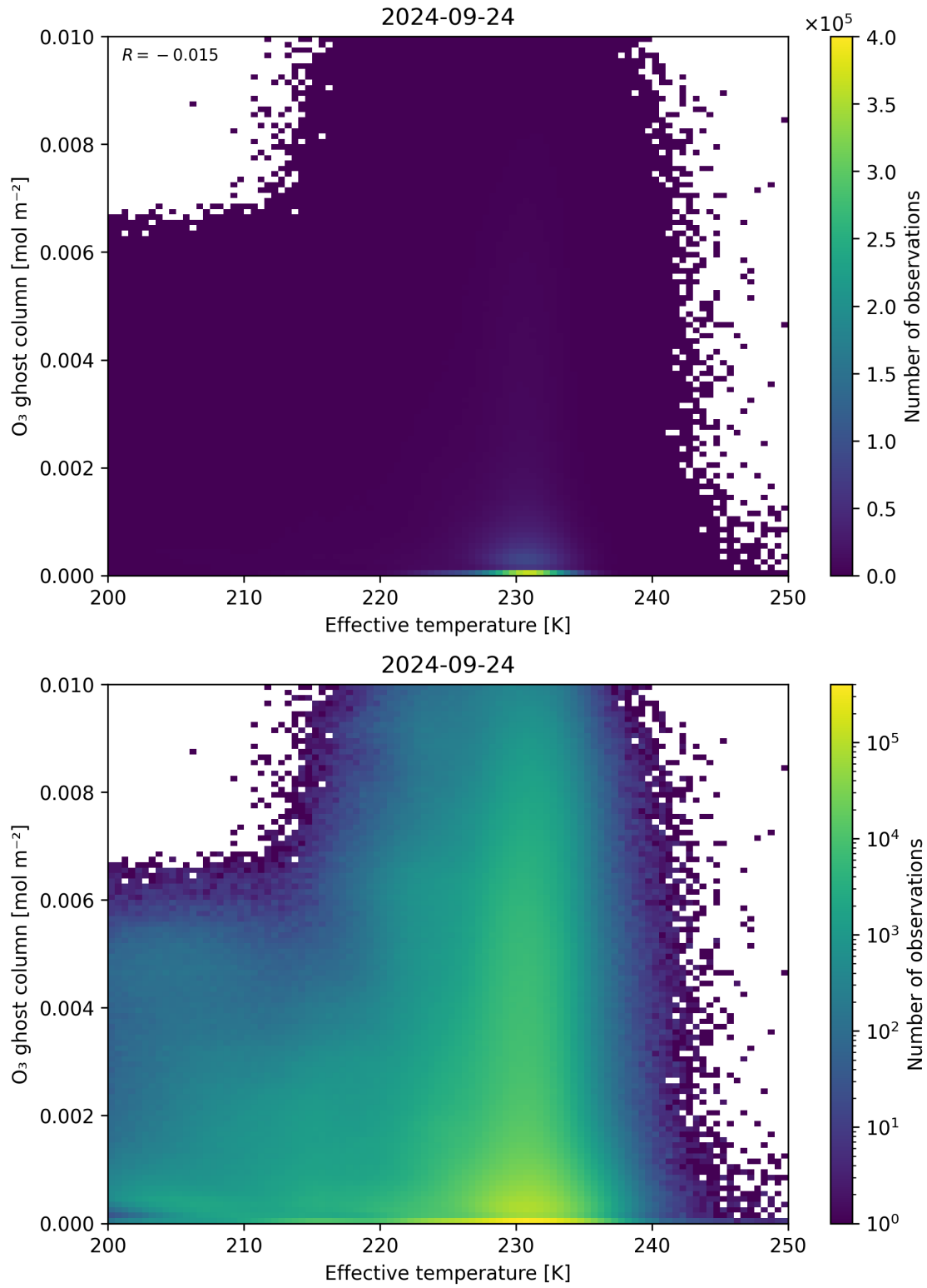
Figure 38: Scatter density plot of “Effective temperature” against “O 3 ghost column” for 2024-09-23 to 2024-09-25.
