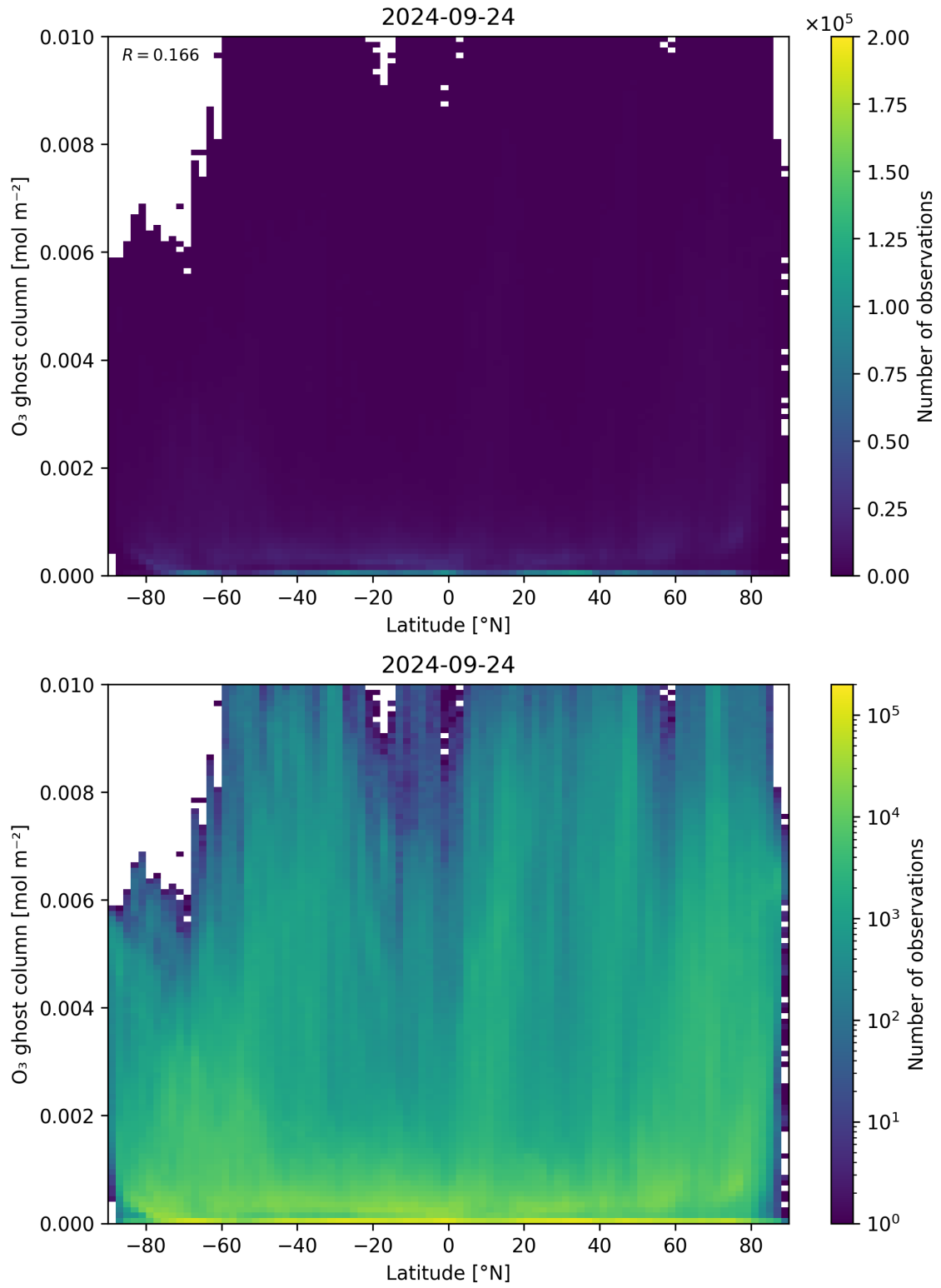
Figure 35: Scatter density plot of “Latitude” against “O 3 ghost column” for 2024-09-23 to 2024-09-25.
