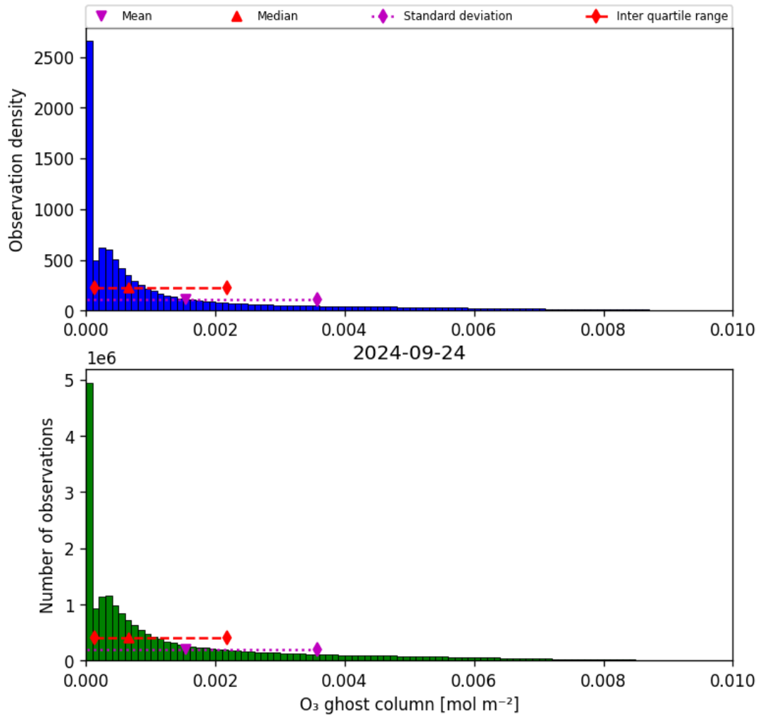
Figure 25: Histogram of "O 3 ghost column" for 2024-09-23 to 2024-09-25
