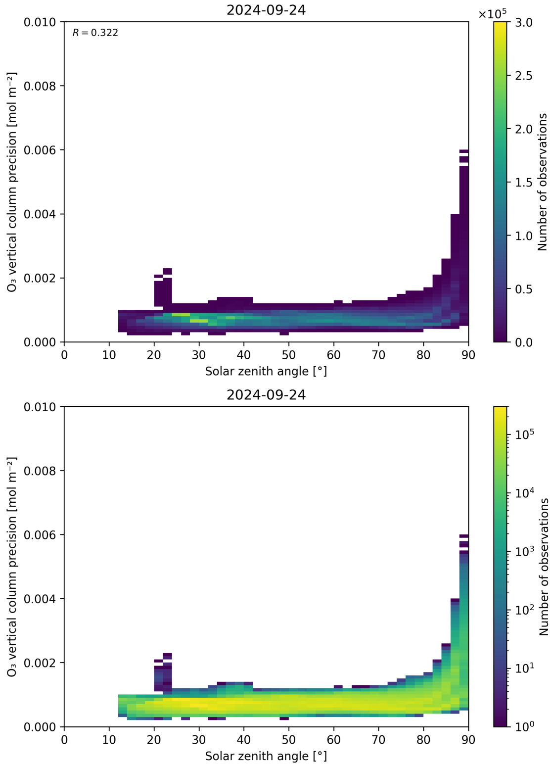
Figure 48: Scatter density plot of “Solar zenith angle” against “O 3 vertical column precision” for 2024-09-23 to 2024-09-25.
