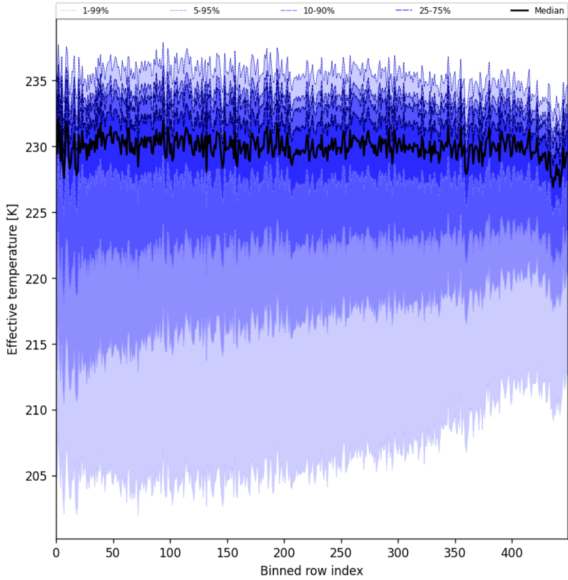
Figure 31: Along track statistics of “Effective temperature” for 2024-09-23 to 2024-09-25
