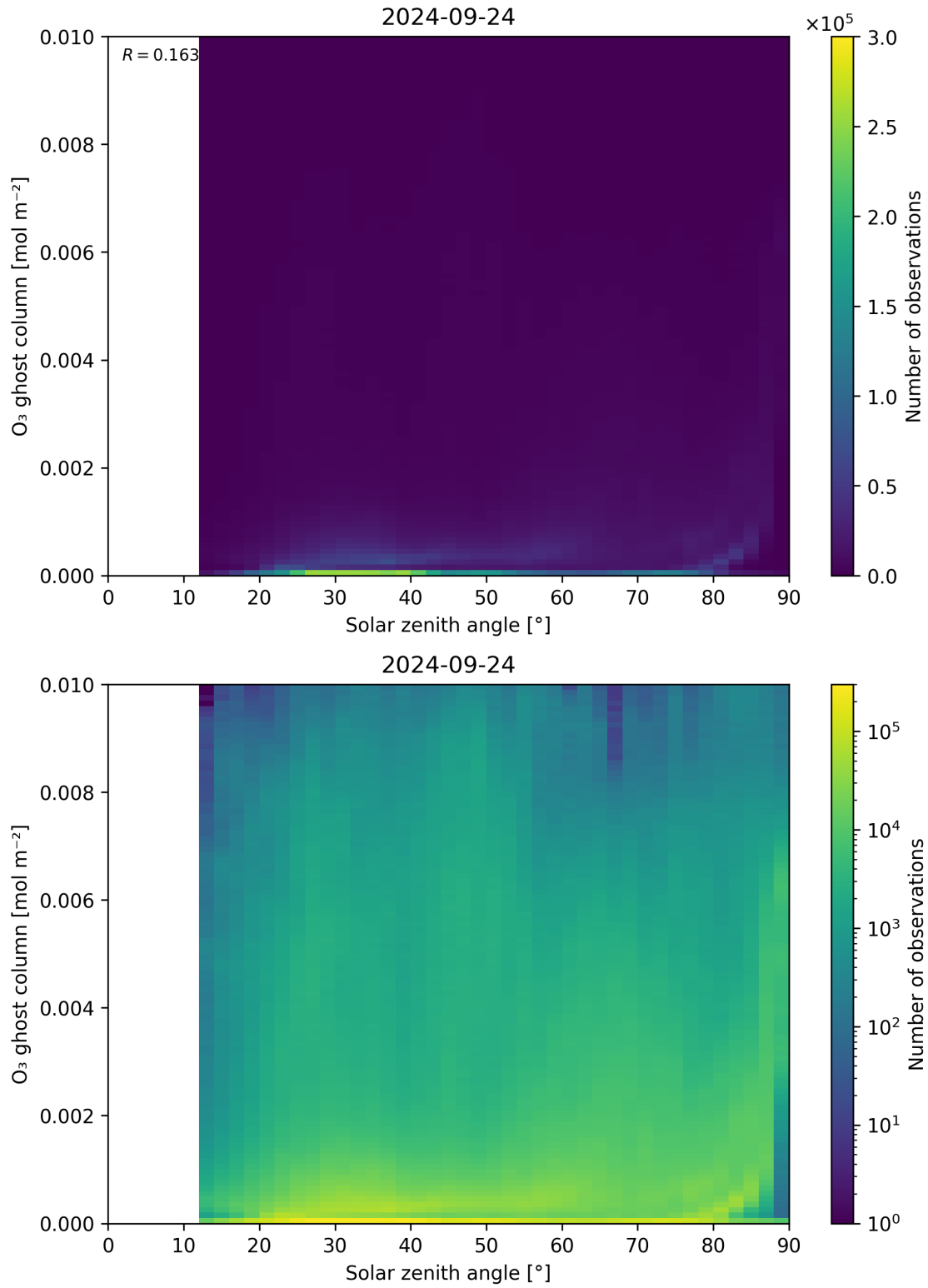
Figure 46: Scatter density plot of “Solar zenith angle” against “O 3 ghost column” for 2024-09-23 to 2024-09-25.
