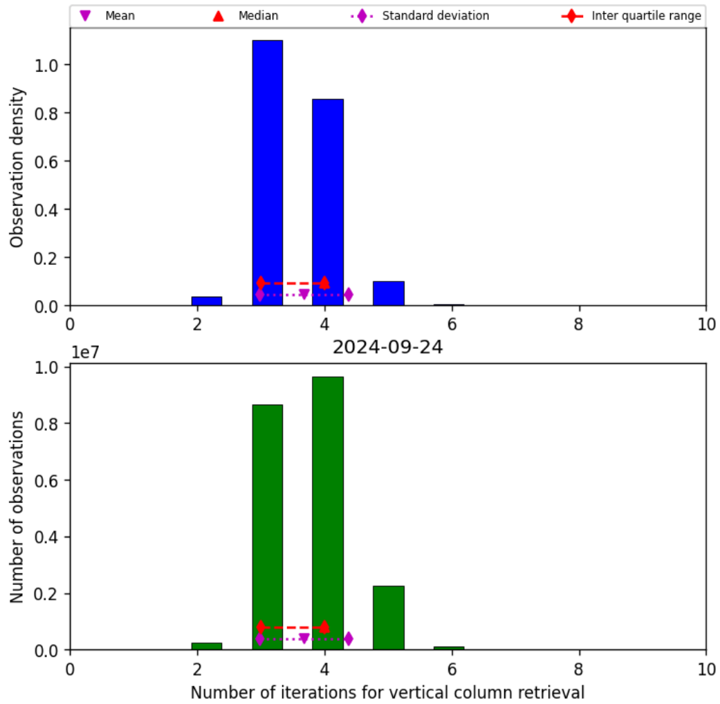
Figure 26: Histogram of “Number of iterations for vertical column retrieval” for 2024-09-23 to 2024-09-25
