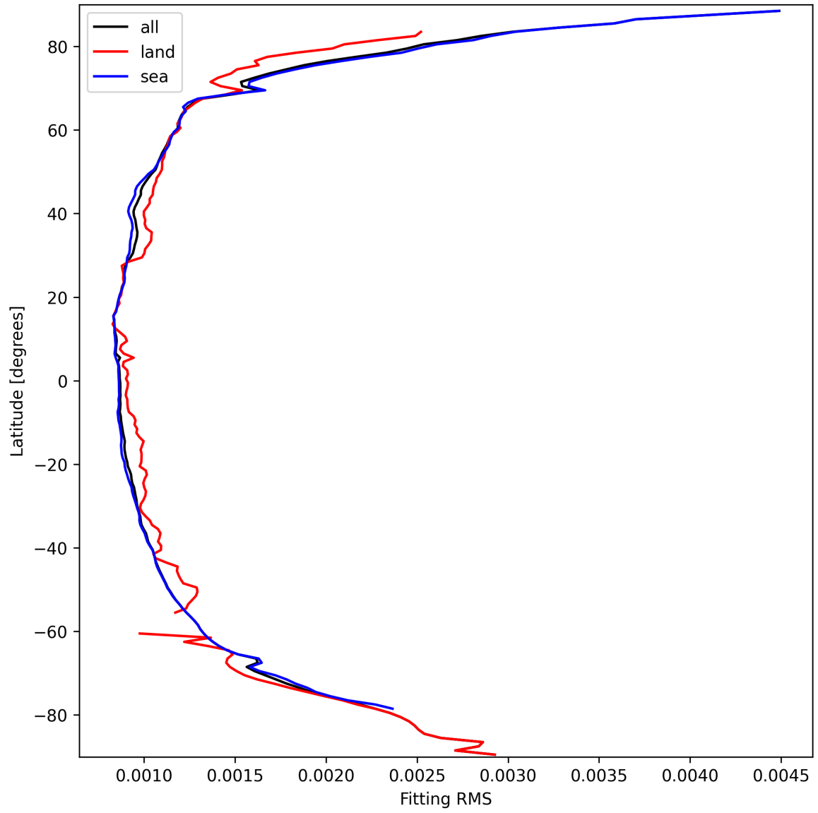
Figure 16: Zonal average of “Fitting RMS” for 2024-09-23 to 2024-09-25.
