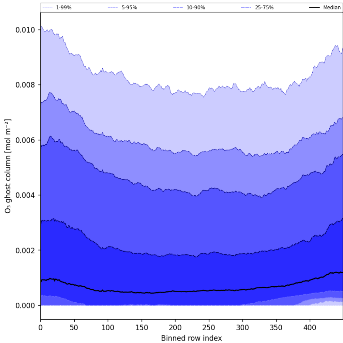
Figure 32: Along track statistics of “O 3 ghost column” for 2024-09-23 to 2024-09-25
