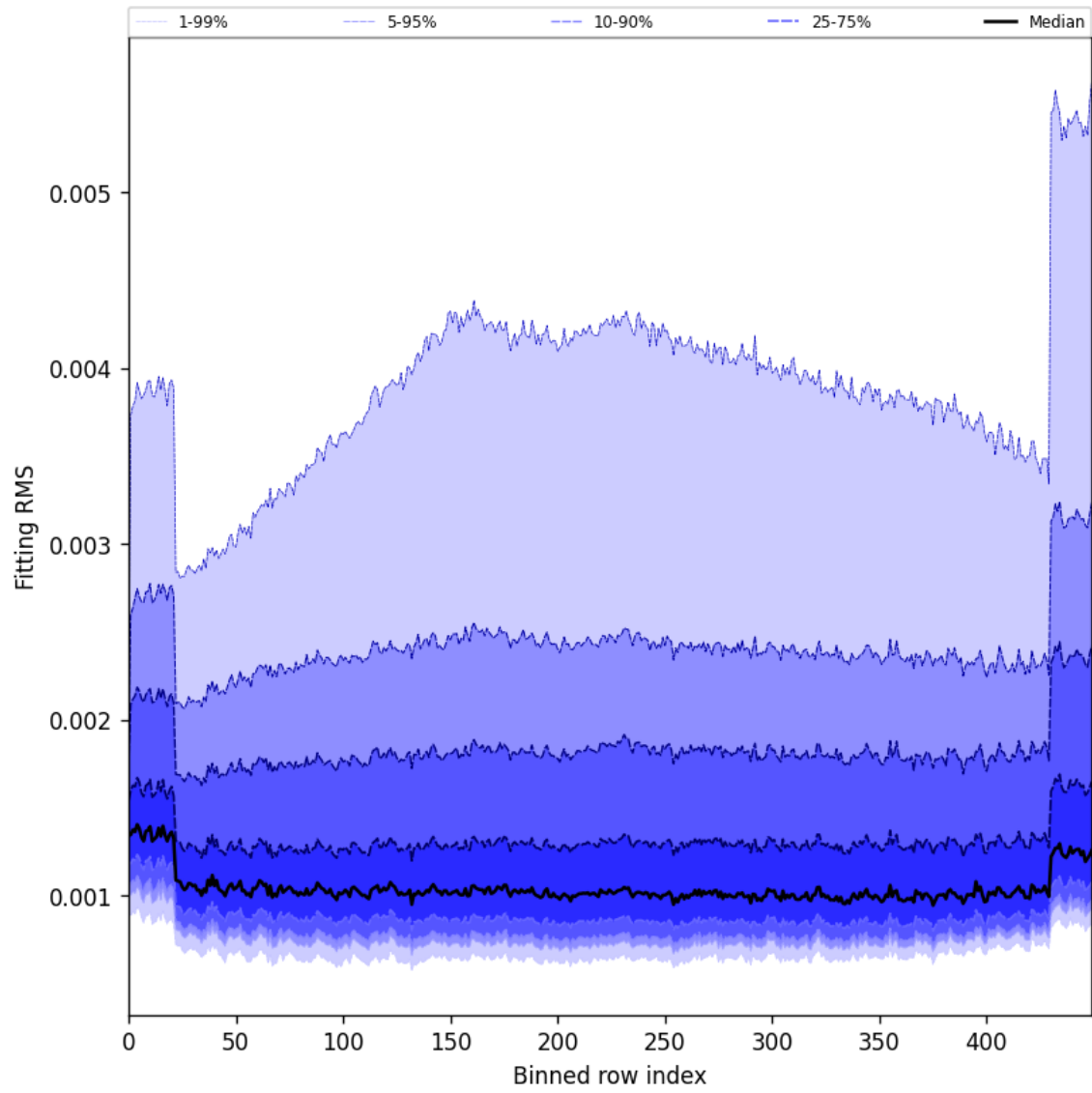
Figure 30: Along track statistics of “Fitting RMS” for 2024-09-23 to 2024-09-25
