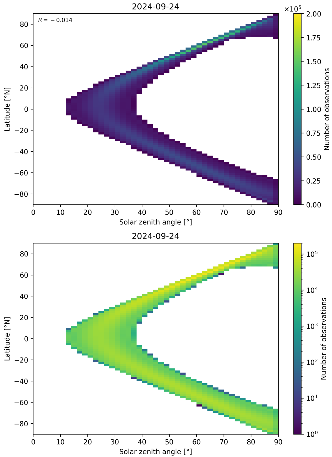
Figure 44: Scatter density plot of “Solar zenith angle” against “Latitude” for 2024-09-23 to 2024-09-25.
