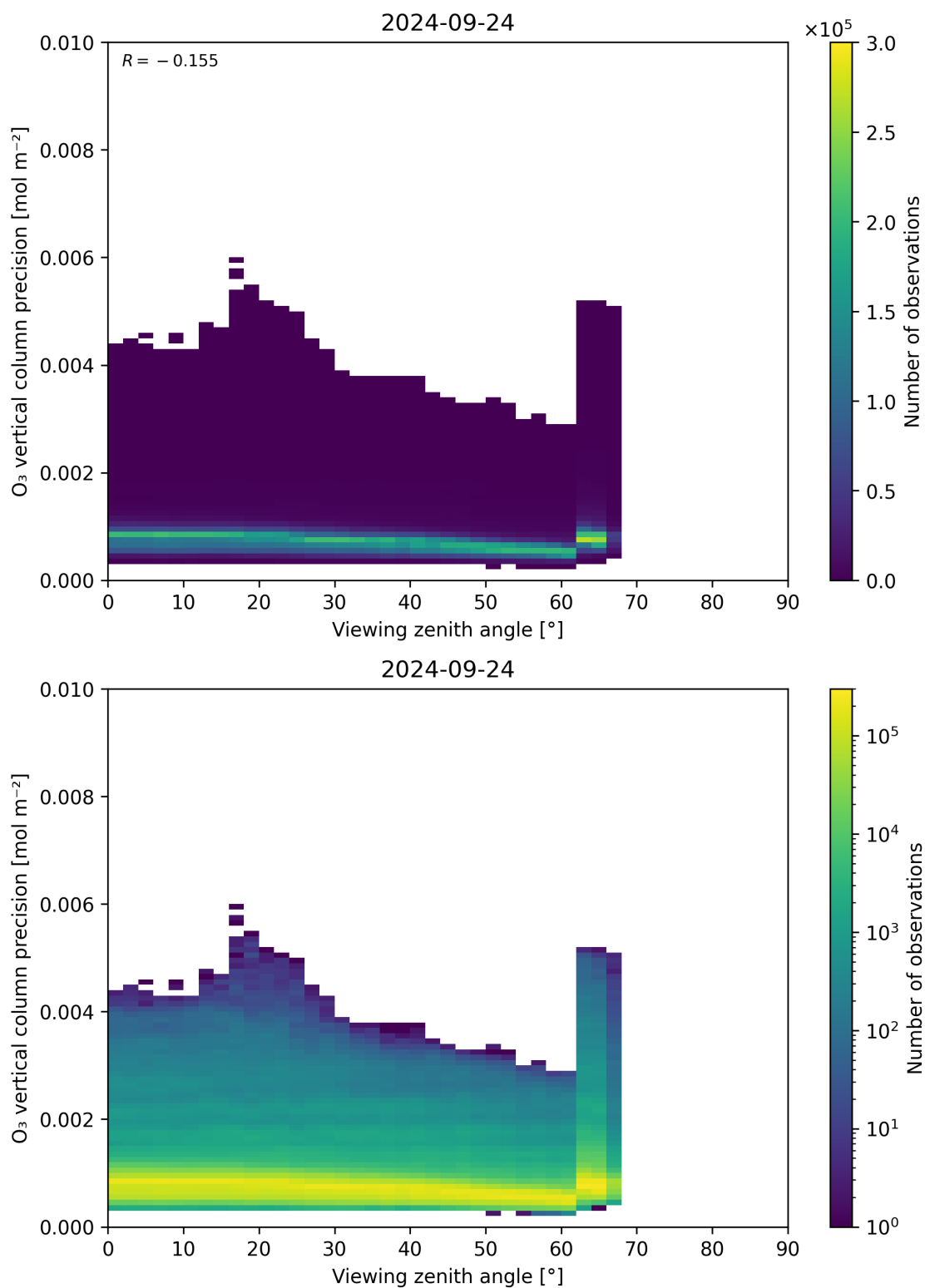
Figure 53: Scatter density plot of “Viewing zenith angle” against “O 3 vertical column precision” for 2024-09-23 to 2024-09-25.
