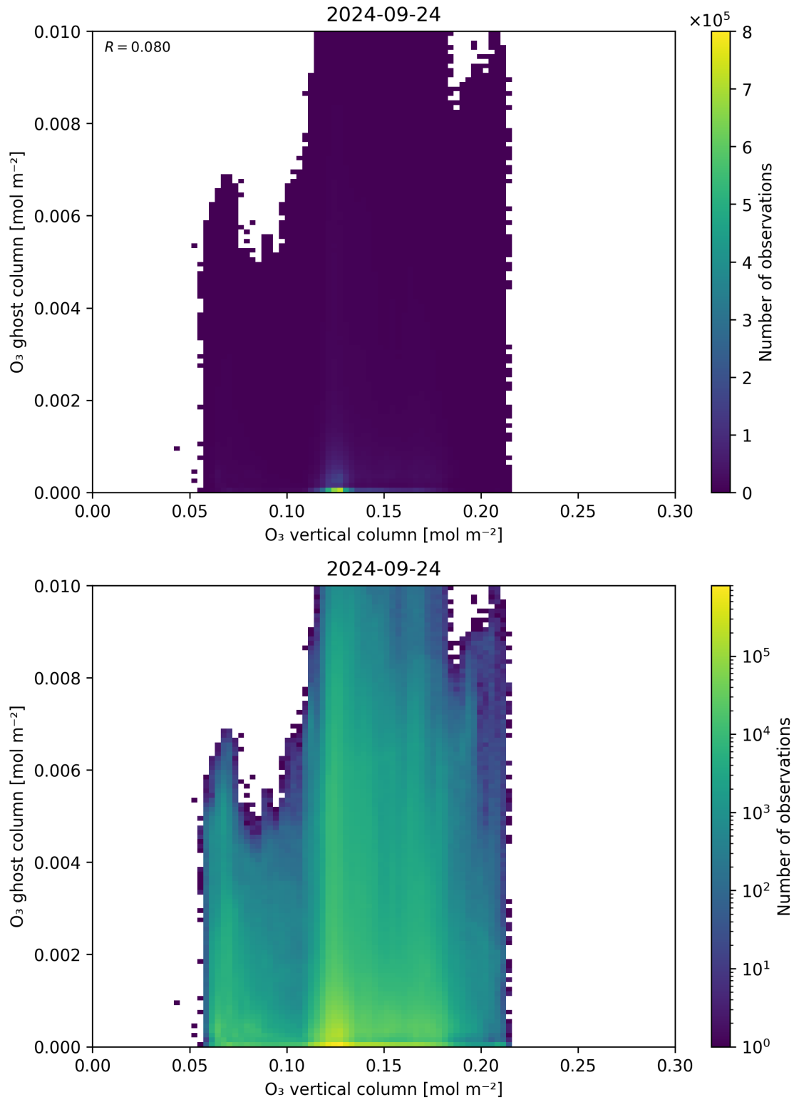
Figure 40: Scatter density plot of “O 3 vertical column” against “O 3 ghost column” for 2024-09-23 to 2024-09-25.
