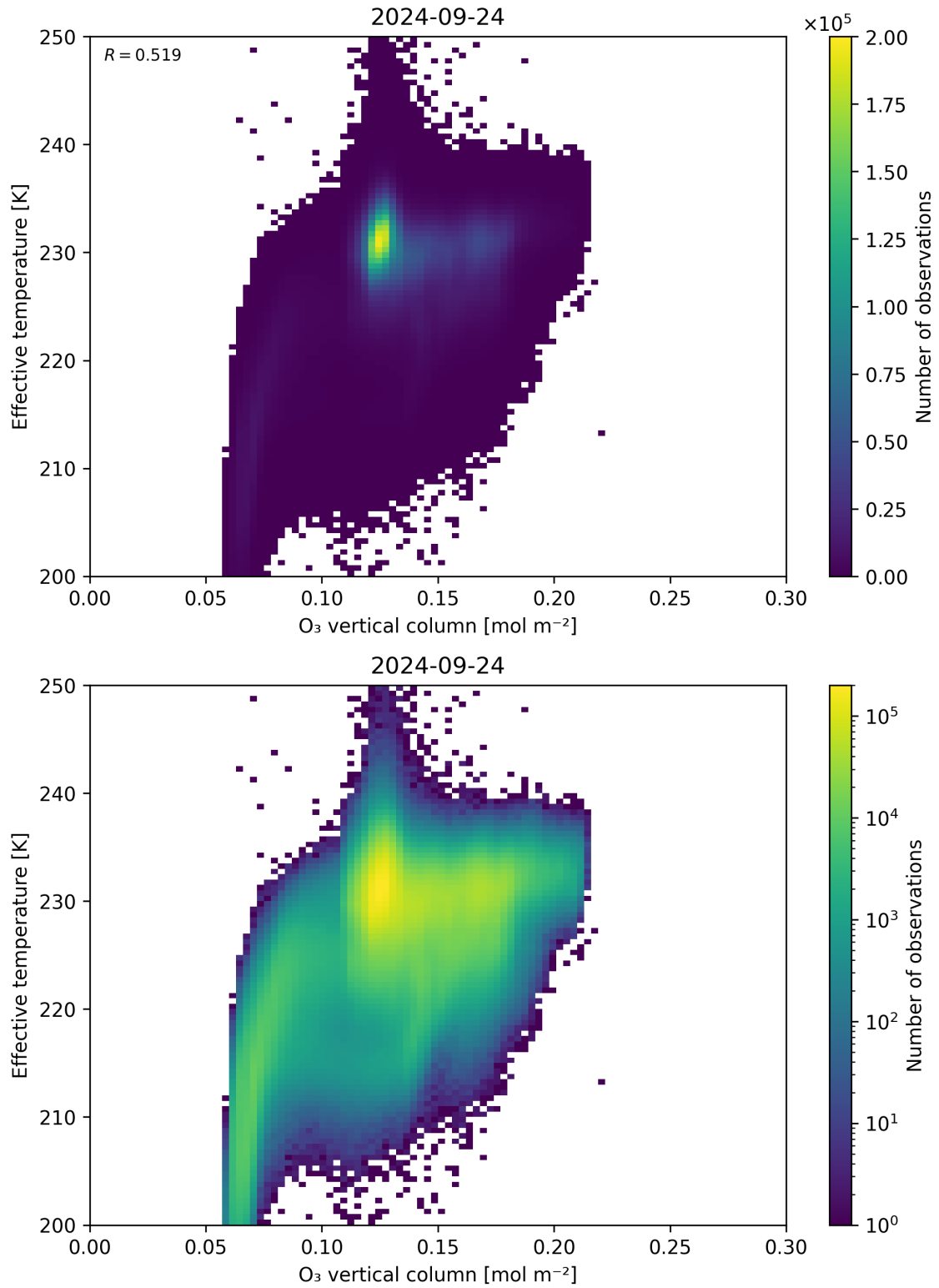
Figure 39: Scatter density plot of “O 3 vertical column” against “Effective temperature” for 2024-09-23 to 2024-09-25.
