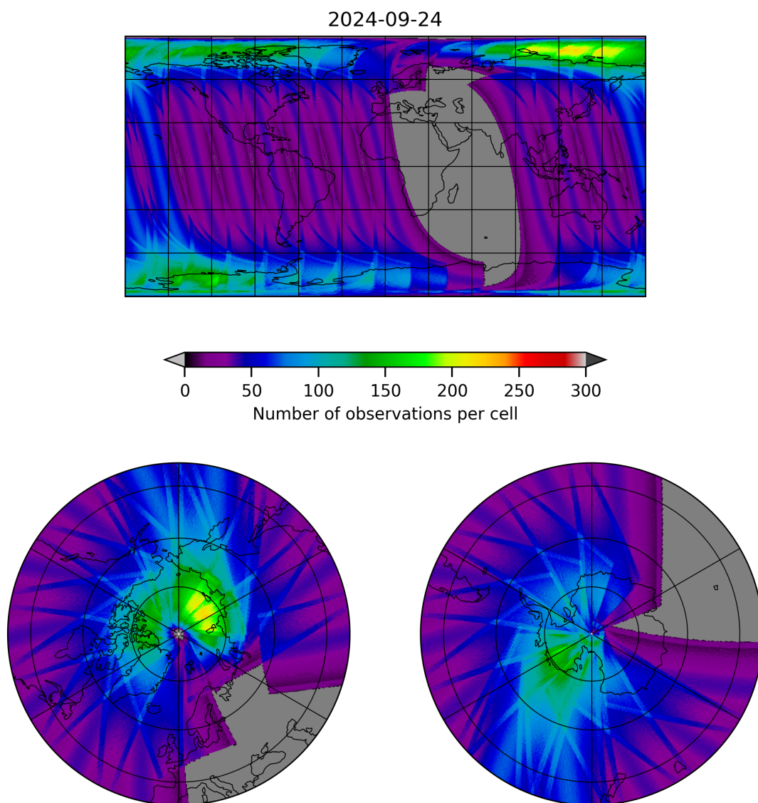
Figure 12: Map of the number of observations for 2024-09-23 to 2024-09-25
