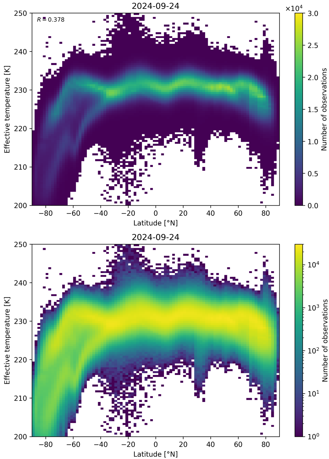
Figure 34: Scatter density plot of “Latitude” against “Effective temperature” for 2024-09-23 to 2024-09-25.
