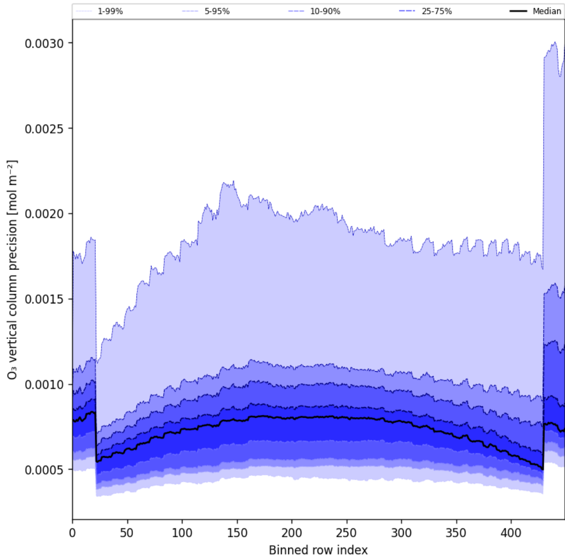
Figure 29: Along track statistics of “O 3 vertical column precision” for 2024-09-23 to 2024-09-25
