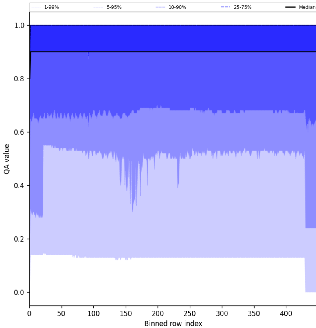
Figure 27: Along track statistics of “QA value” for 2024-09-23 to 2024-09-25
