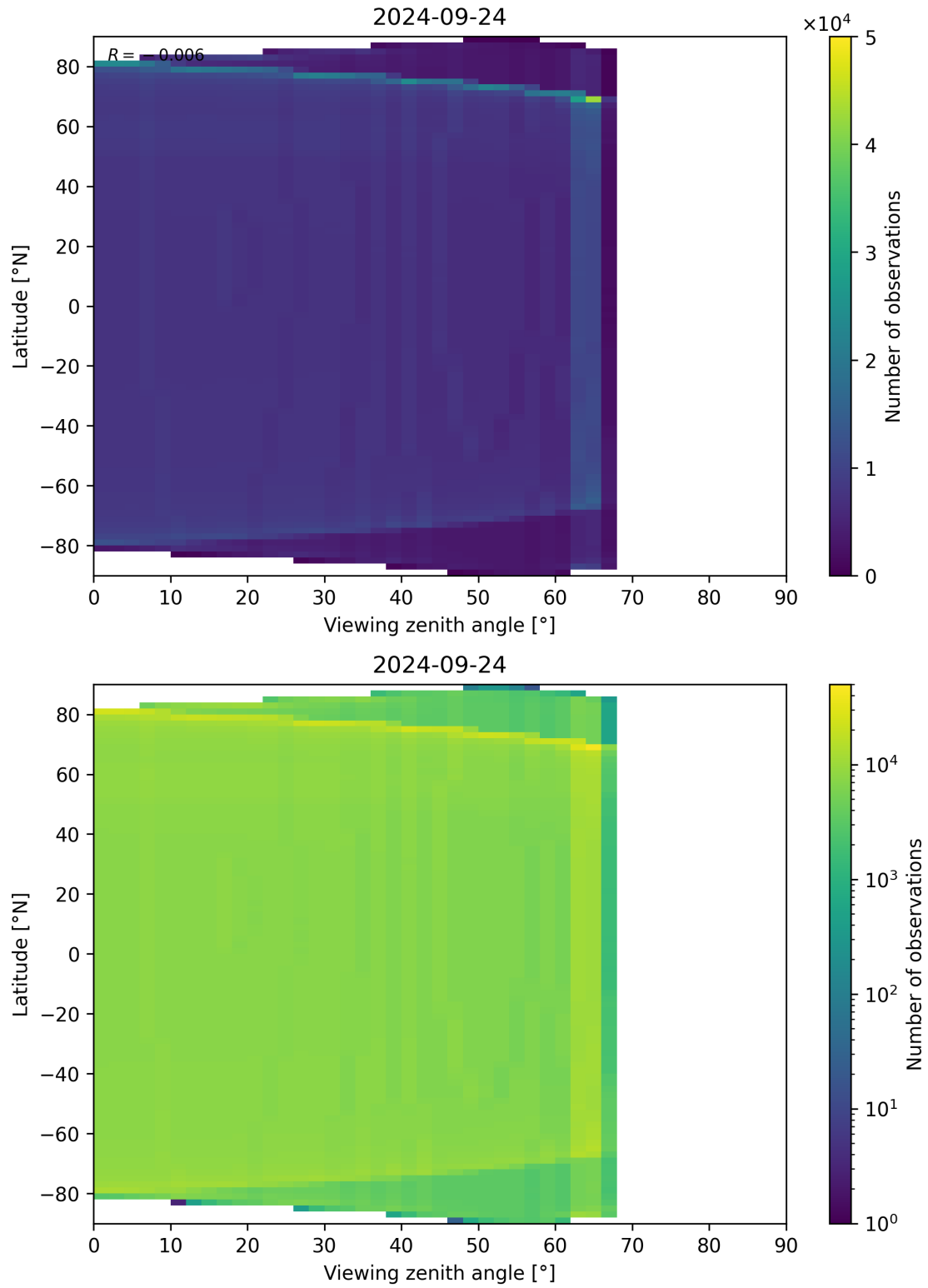
Figure 49: Scatter density plot of “Viewing zenith angle” against “Latitude” for 2024-09-23 to 2024-09-25.
