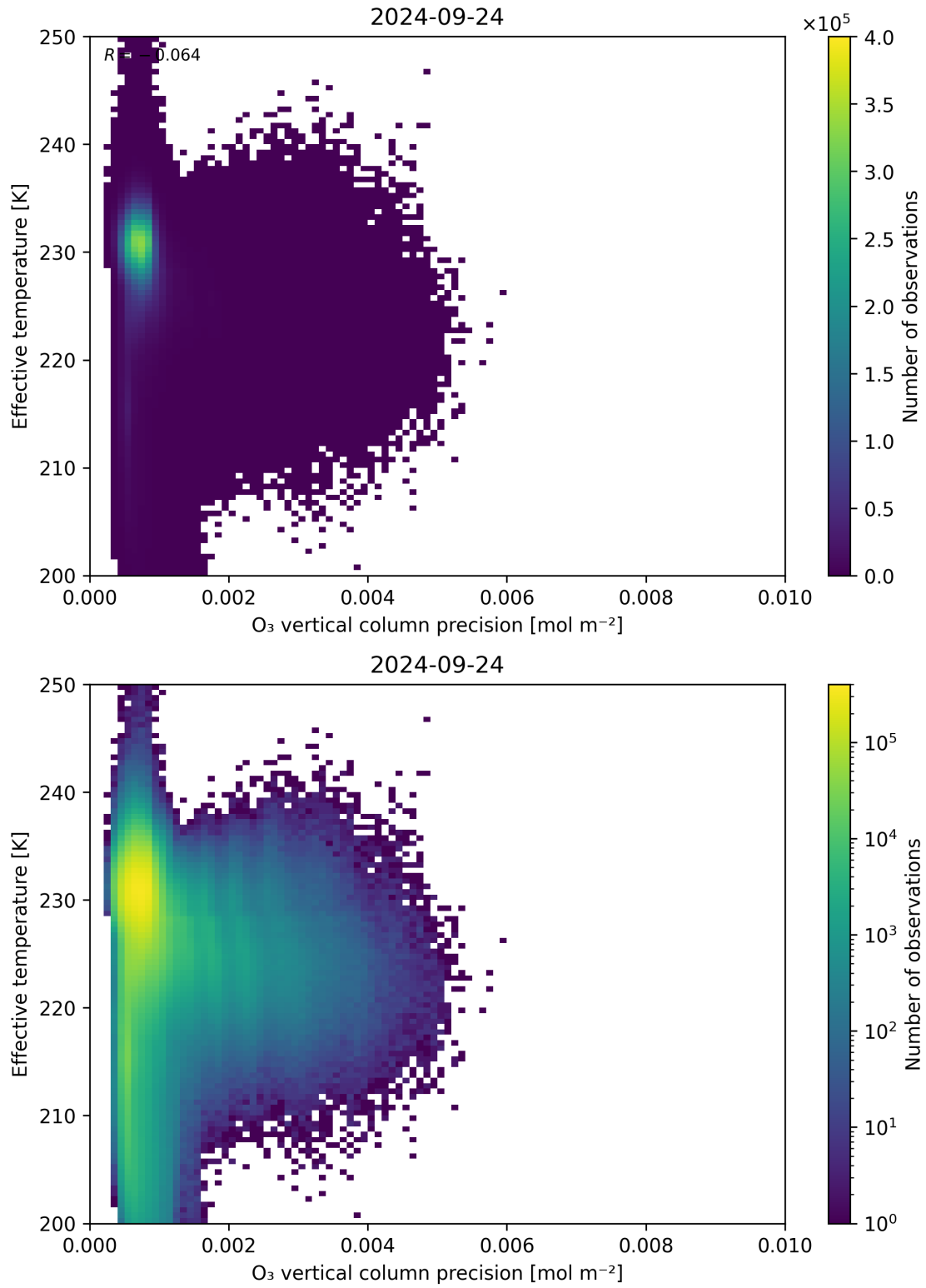
Figure 42: Scatter density plot of “O 3 vertical column precision” against “Effective temperature” for 2024-09-23 to 2024-09-25.
