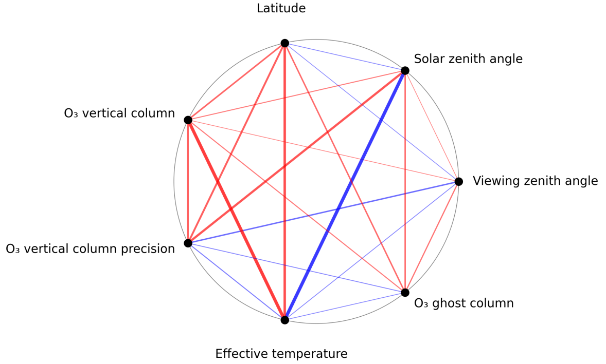
Figure 1: Map of correlation graph for 2024-09-23 to 2024-09-25.
