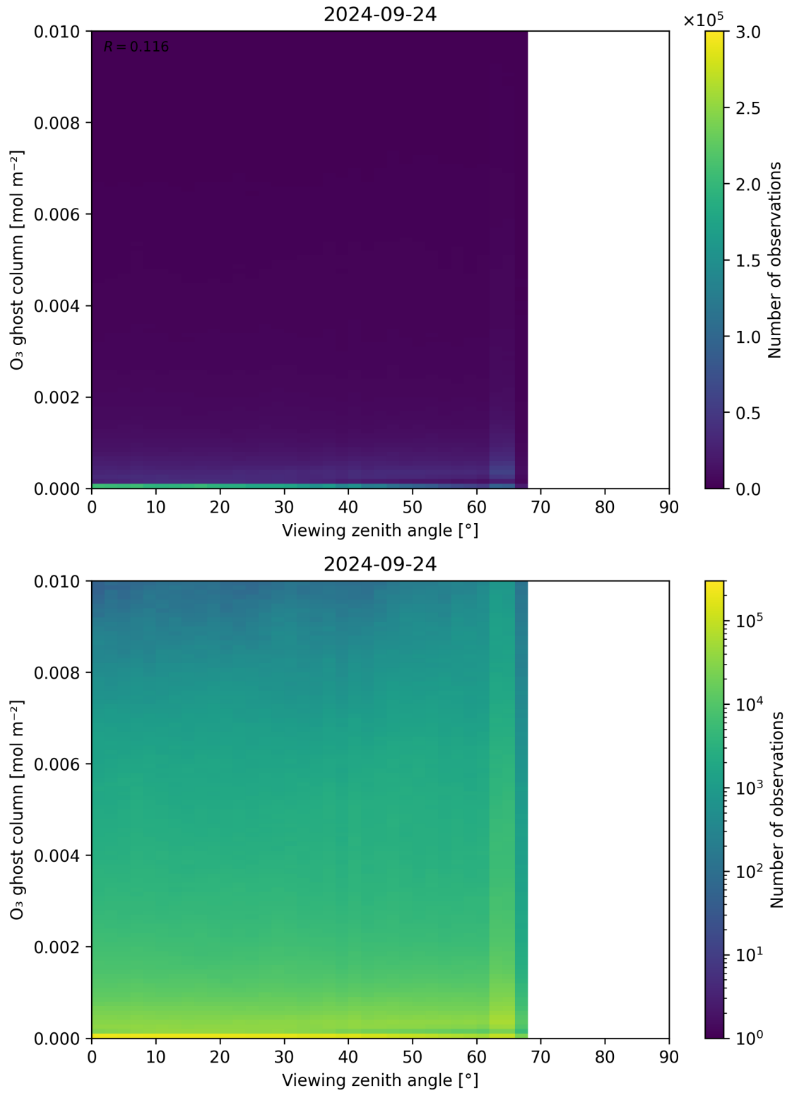
Figure 51: Scatter density plot of “Viewing zenith angle” against “O 3 ghost column” for 2024-09-23 to 2024-09-25.
