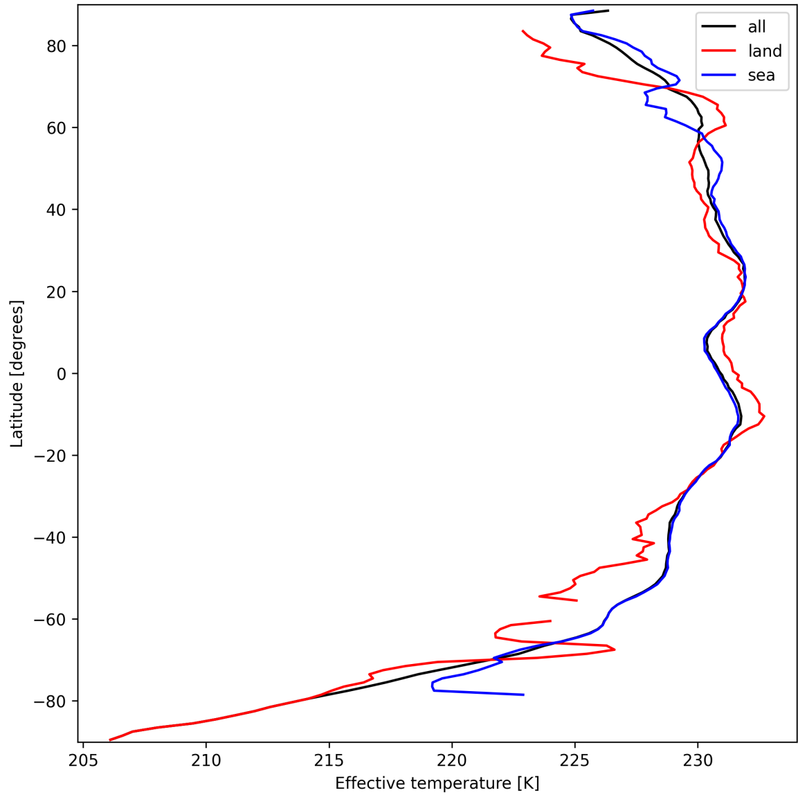
Figure 17: Zonal average of "Effective temperature" for 2024-09-23 to 2024-09-25.
