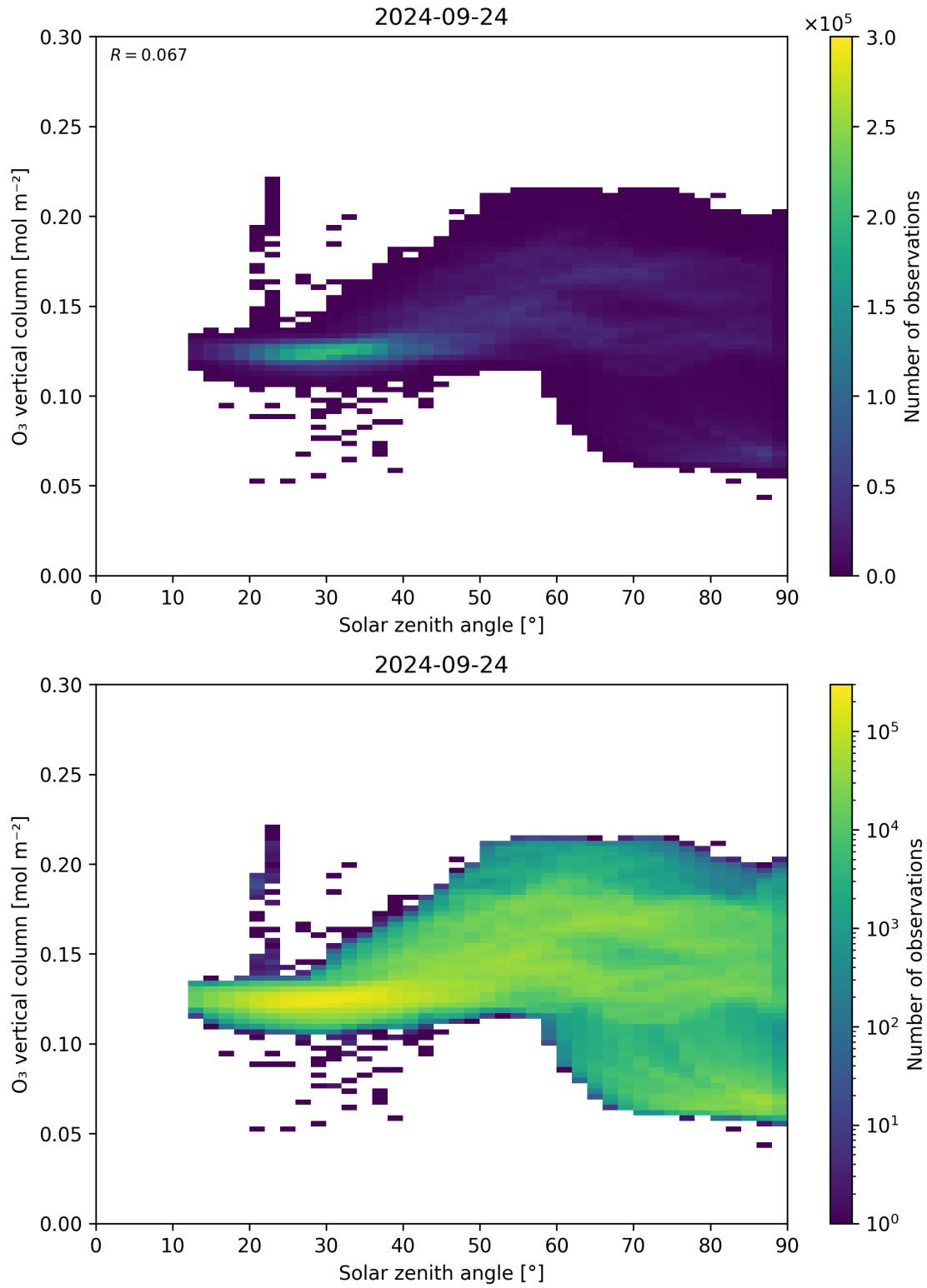
Figure 47: Scatter density plot of “Solar zenith angle” against “O 3 vertical column” for 2024-09-23 to 2024-09-25.
