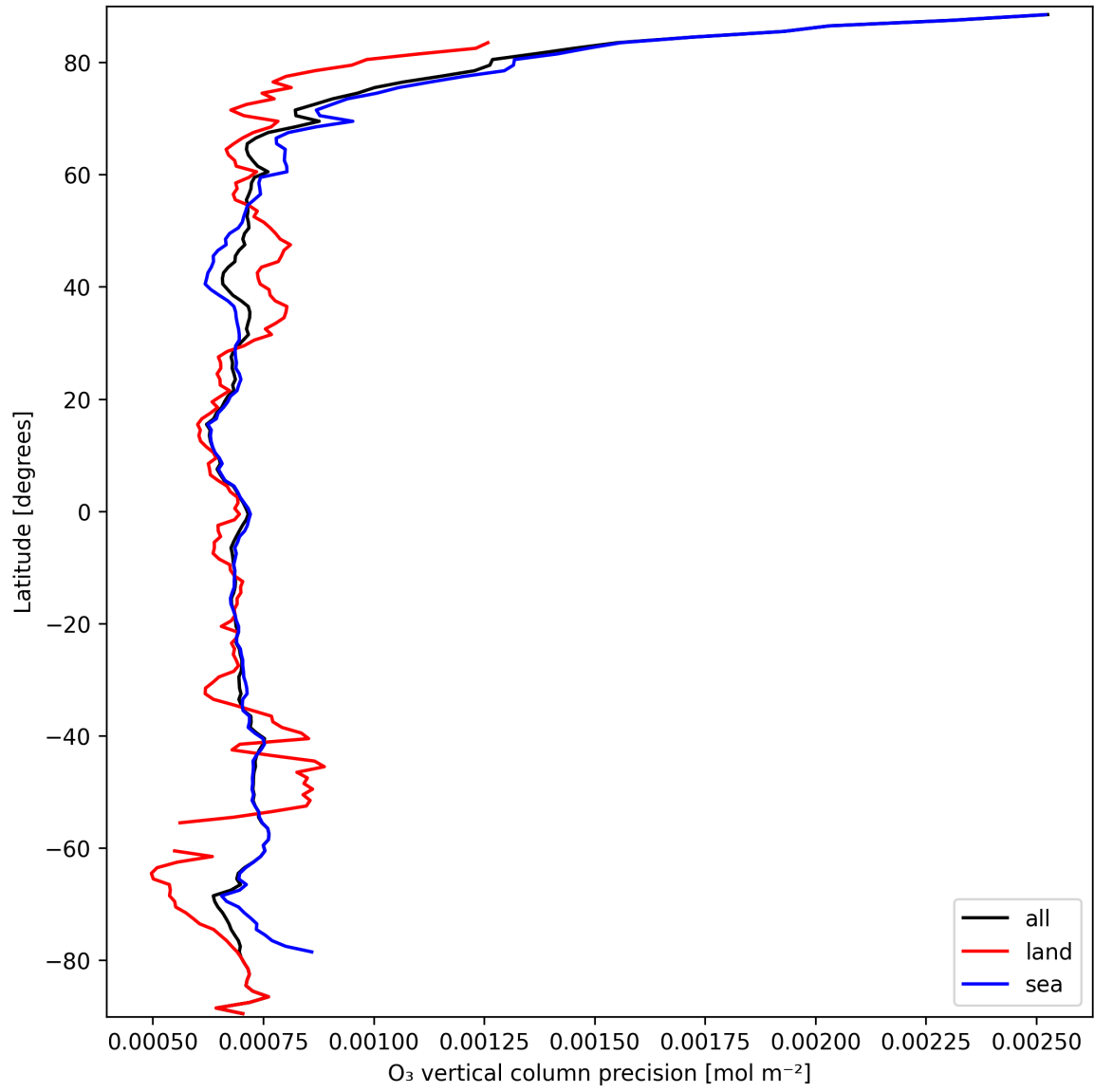
Figure 15: Zonal average of “O 3 vertical column precision” for 2024-09-23 to 2024-09-25.
