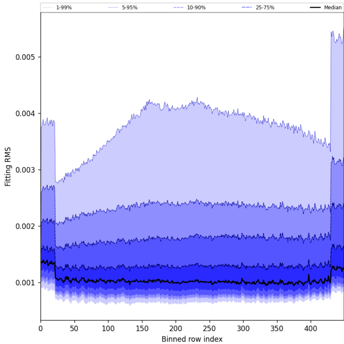
Figure 30: Along track statistics of “Fitting RMS” for 2024-09-24 to 2024-09-26
