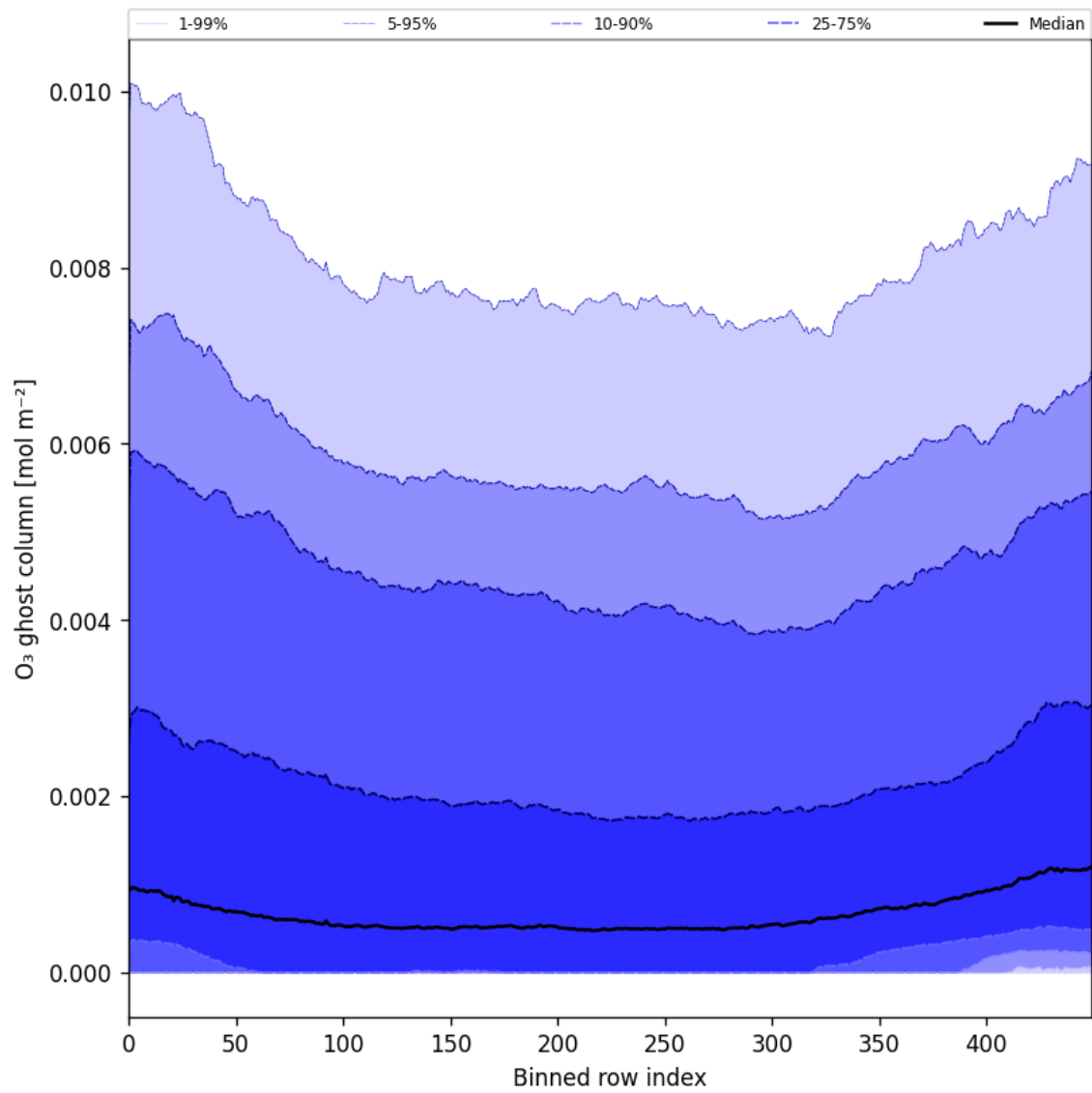
Figure 32: Along track statistics of “O 3 ghost column” for 2024-09-24 to 2024-09-26
