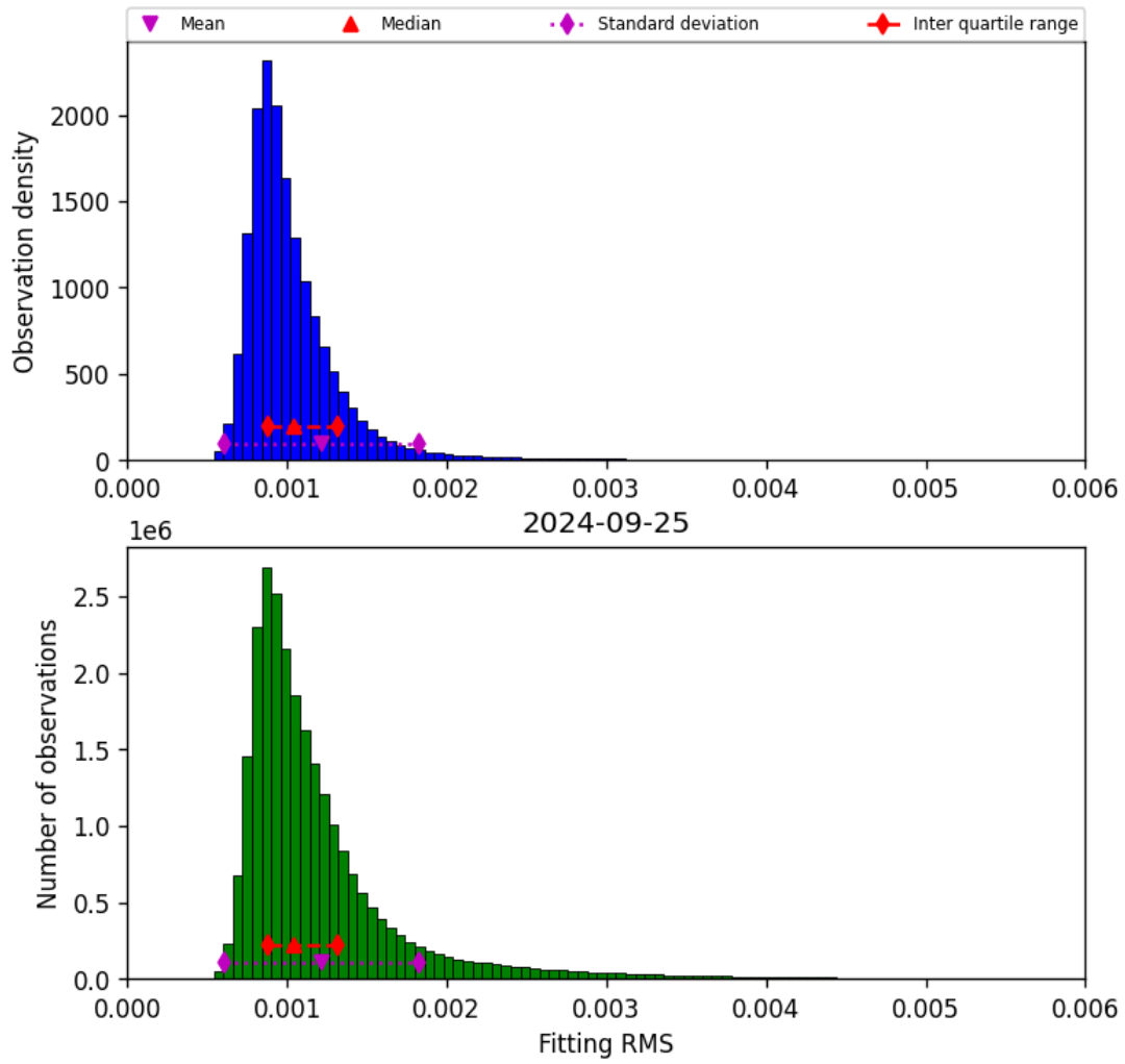
Figure 23: Histogram of “Fitting RMS” for 2024-09-24 to 2024-09-26
