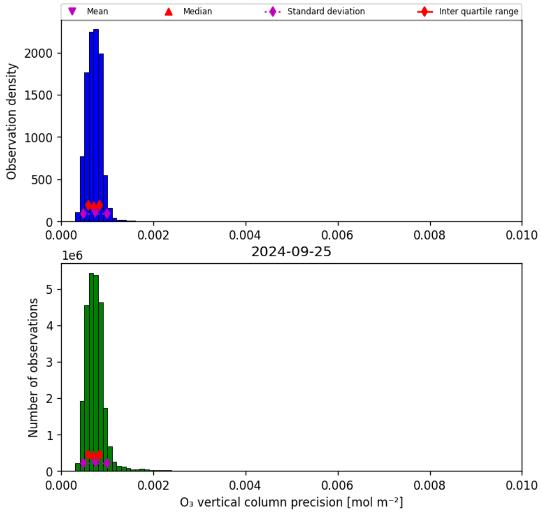
Figure 22: Histogram of “O 3 vertical column precision” for 2024-09-24 to 2024-09-26
