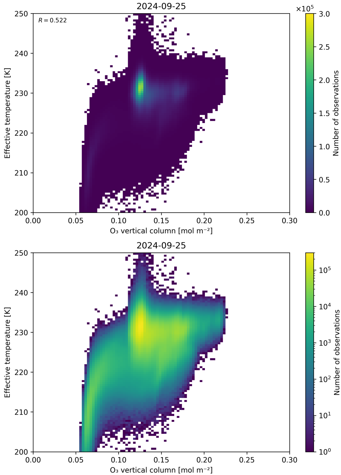
Figure 39: Scatter density plot of “O 3 vertical column” against “Effective temperature” for 2024-09-24 to 2024-09-26.
