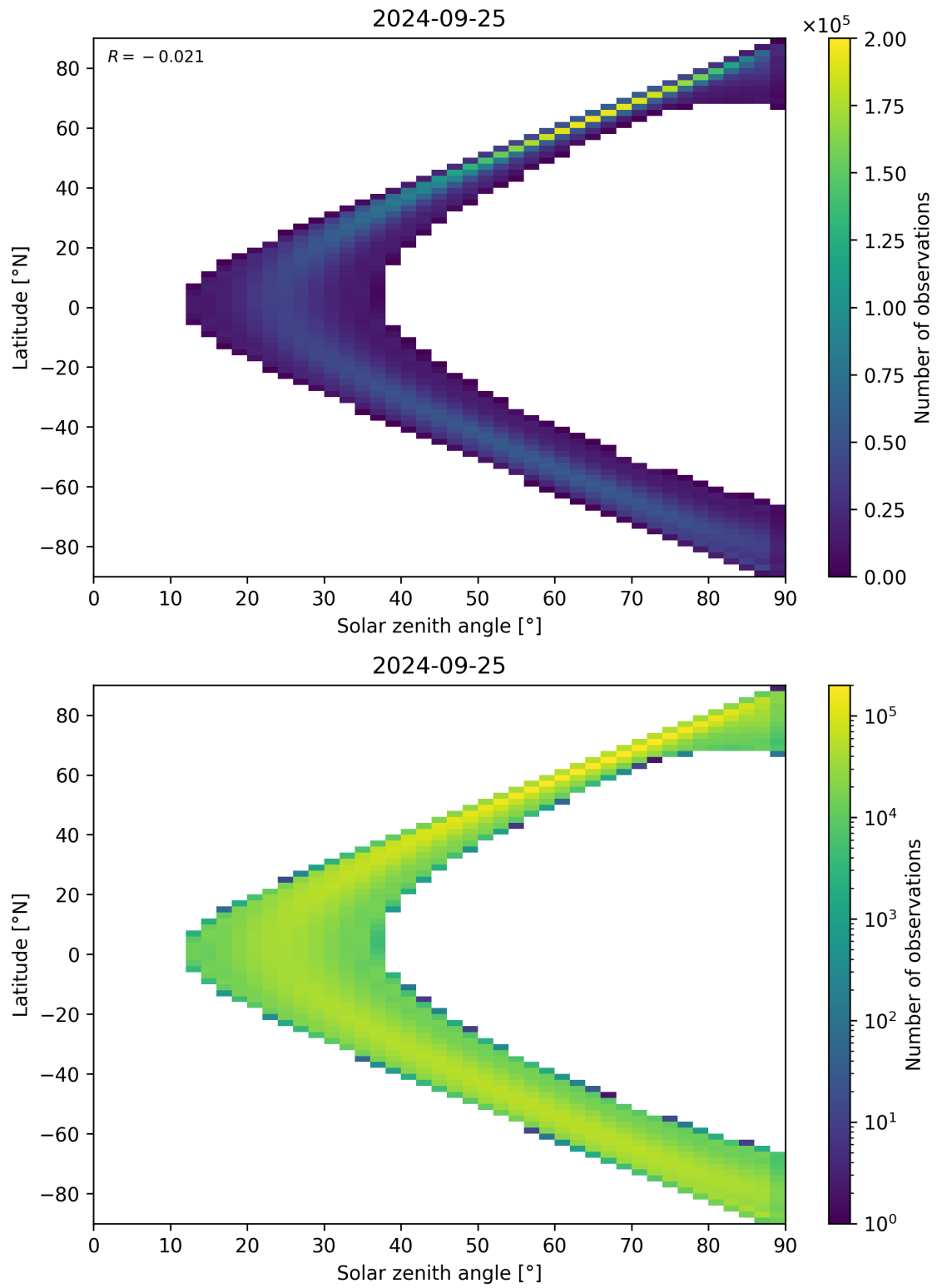
Figure 44: Scatter density plot of “Solar zenith angle” against “Latitude” for 2024-09-24 to 2024-09-26.
