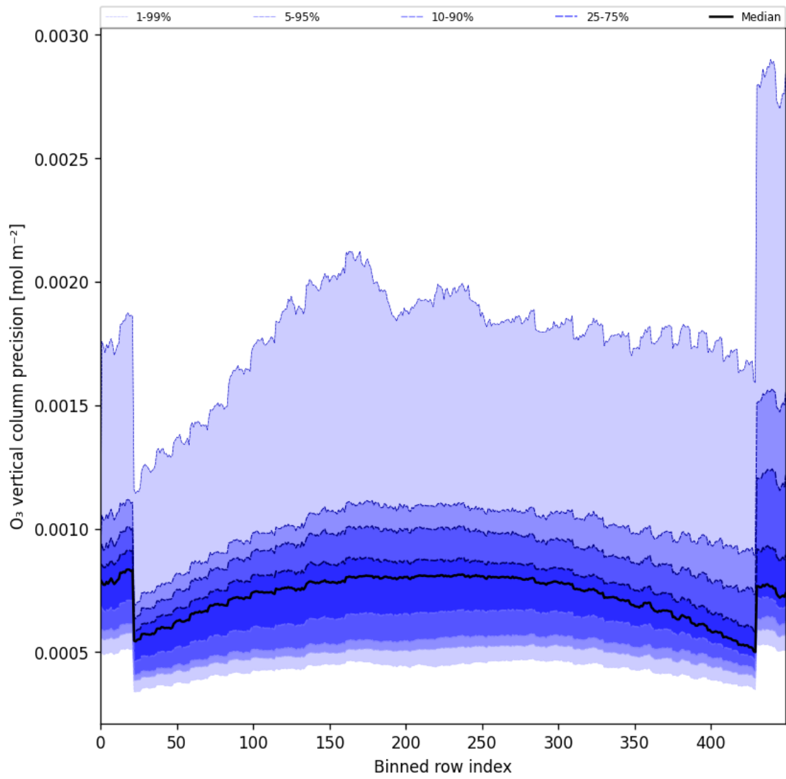
Figure 29: Along track statistics of “O 3 vertical column precision” for 2024-09-24 to 2024-09-26
