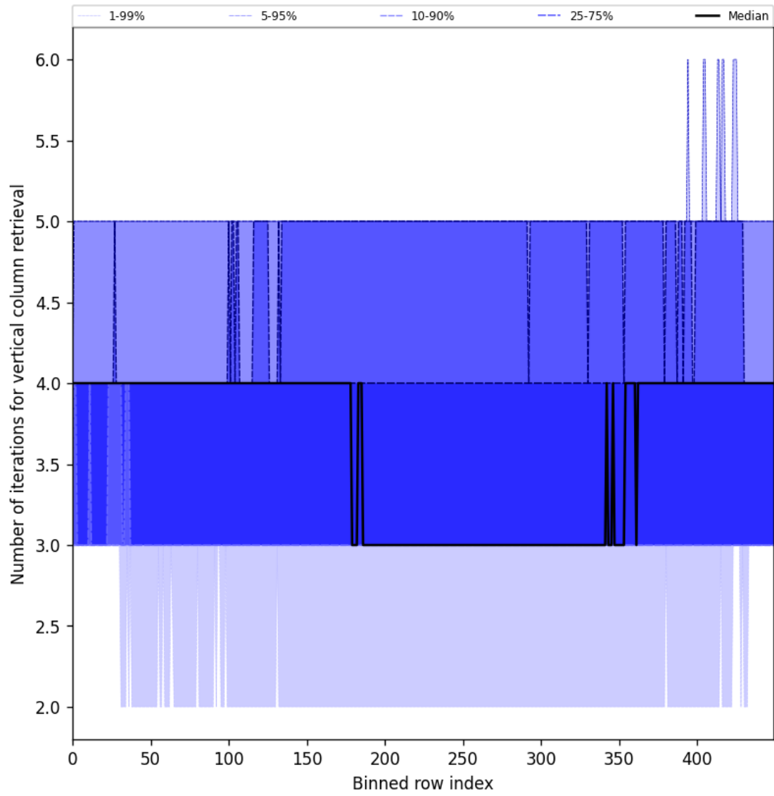
Figure 33: Along track statistics of “Number of iterations for vertical column retrieval” for 2024-09-24 to 2024-09-26
