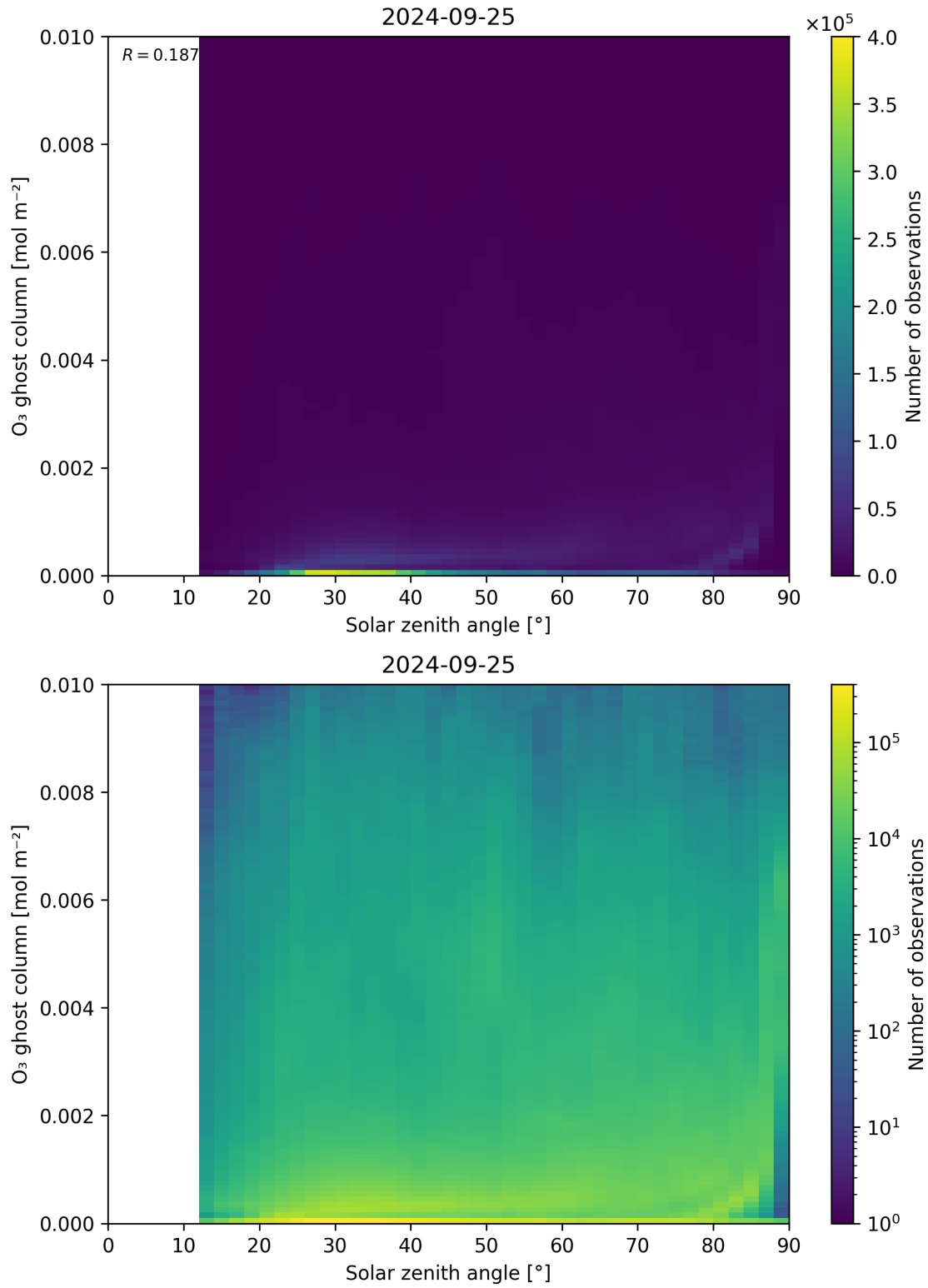
Figure 46: Scatter density plot of “Solar zenith angle” against “O 3 ghost column” for 2024-09-24 to 2024-09-26.
