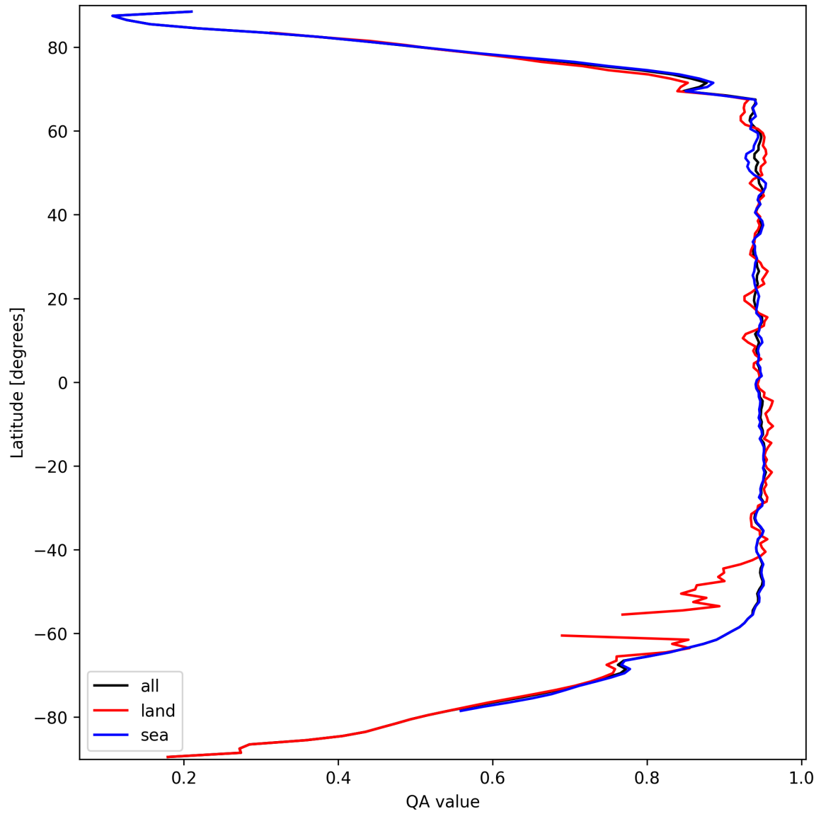
Figure 13: Zonal average of “QA value” for 2024-09-24 to 2024-09-26.
