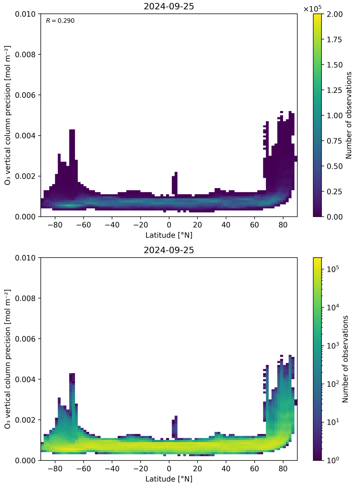
Figure 37: Scatter density plot of “Latitude” against “O 3 vertical column precision” for 2024-09-24 to 2024-09-26.
