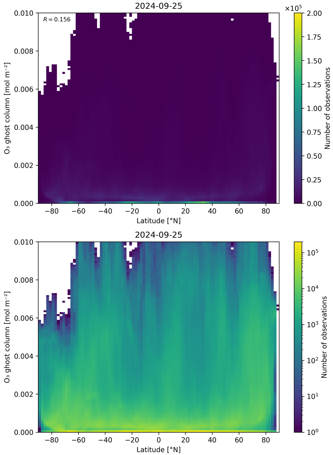
Figure 35: Scatter density plot of “Latitude” against “O 3 ghost column” for 2024-09-24 to 2024-09-26.
