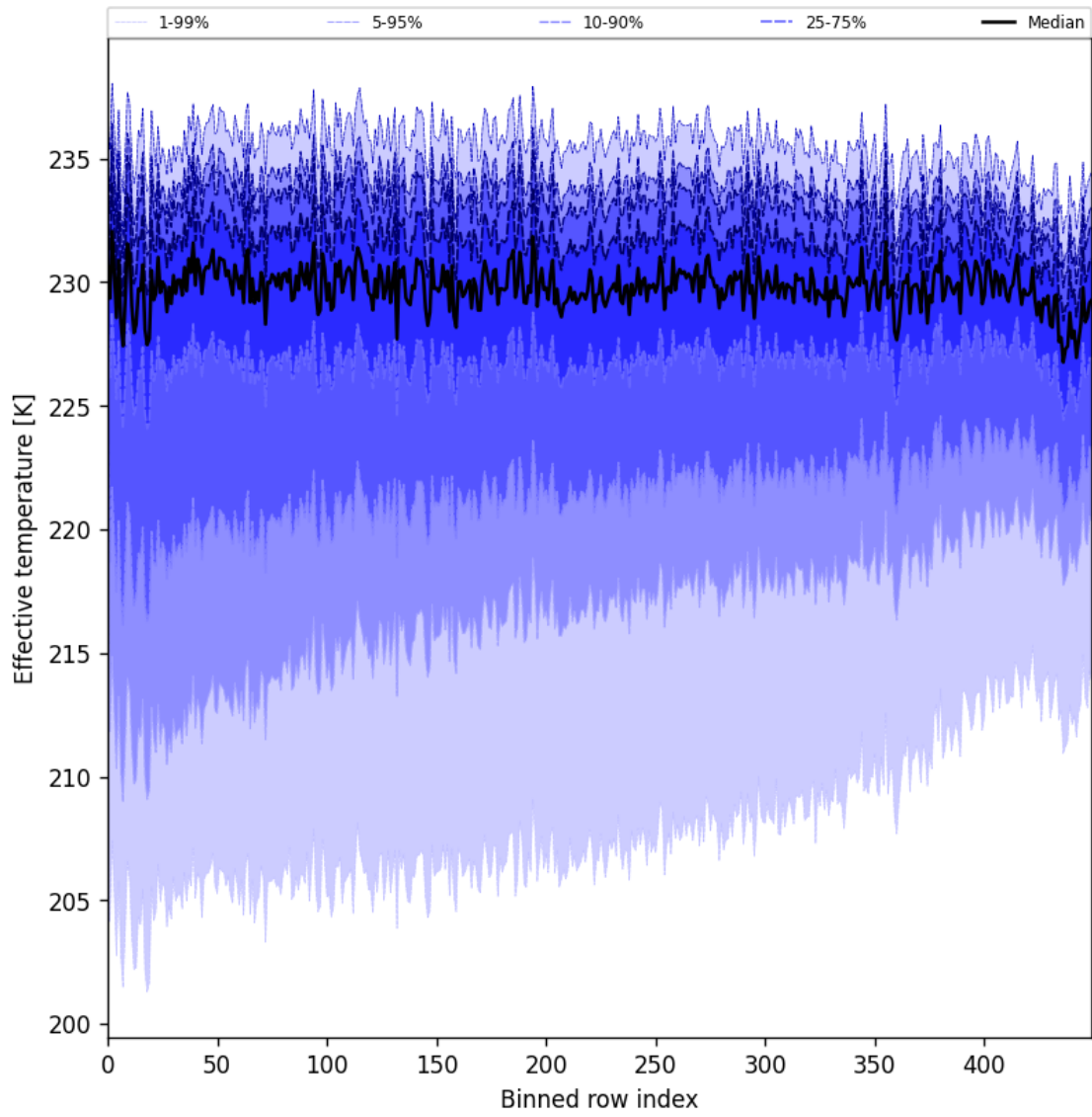
Figure 31: Along track statistics of “Effective temperature” for 2024-09-24 to 2024-09-26
