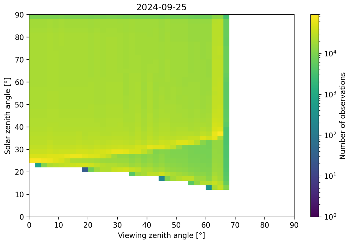
Figure 54: Scatter density plot of “Viewing zenith angle” against “Solar zenith angle” for 2024-09-24 to 2024-09-26.
