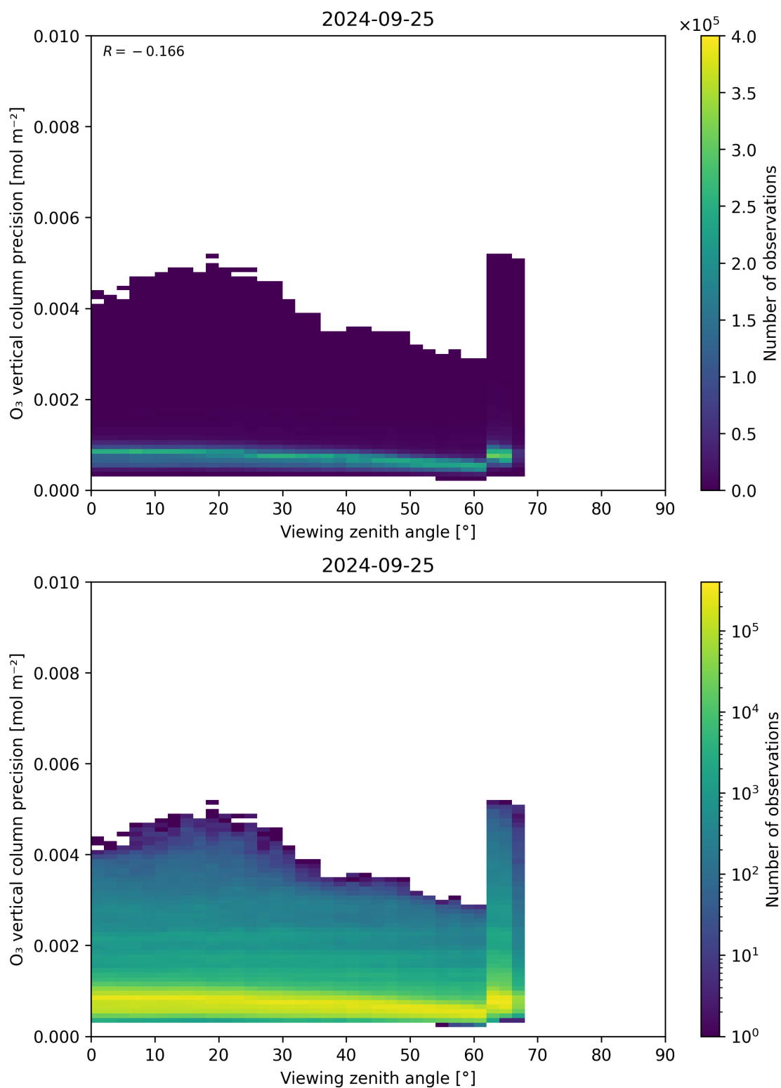
Figure 53: Scatter density plot of “Viewing zenith angle” against “O 3 vertical column precision” for 2024-09-24 to 2024-09-26.
