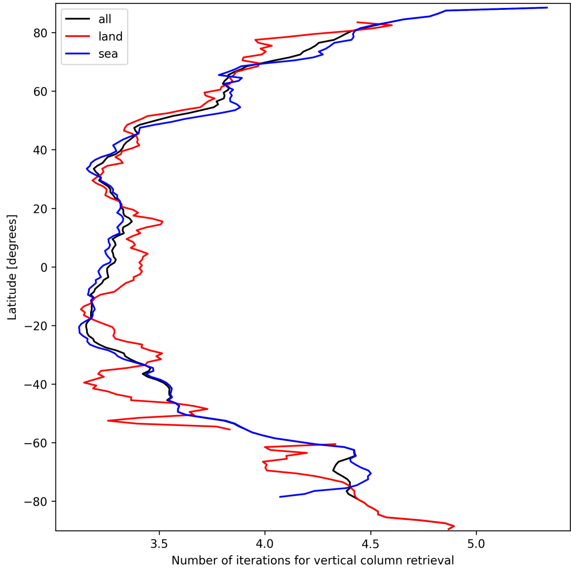
Figure 19: Zonal average of “Number of iterations for vertical column retrieval” for 2024-09-24 to 2024-09-26.
