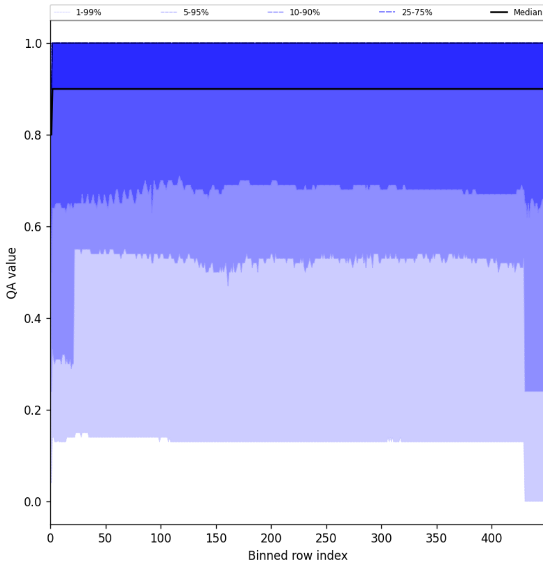
Figure 27: Along track statistics of “QA value” for 2024-09-24 to 2024-09-26
