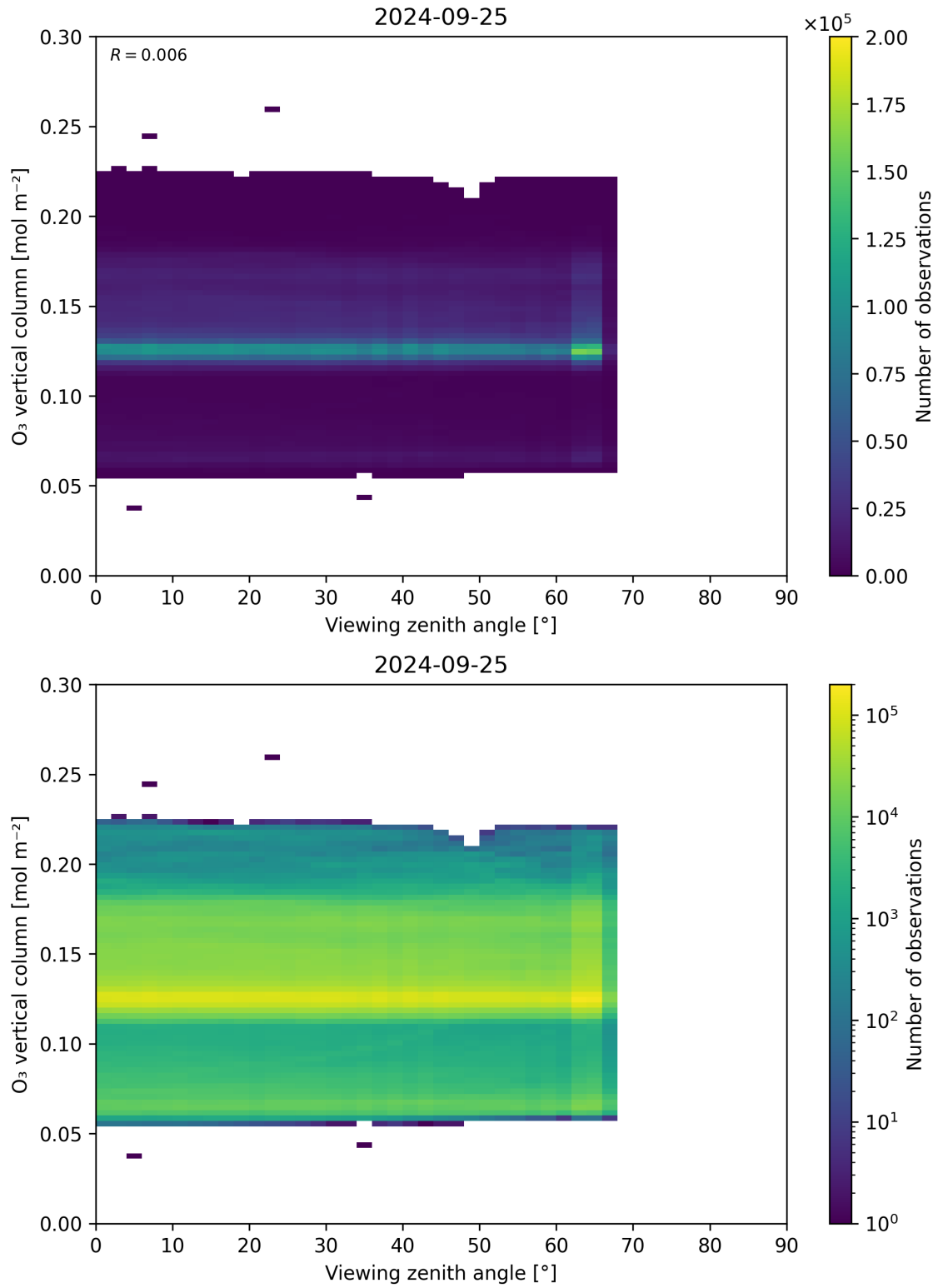
Figure 52: Scatter density plot of “Viewing zenith angle” against “O 3 vertical column” for 2024-09-24 to 2024-09-26.
