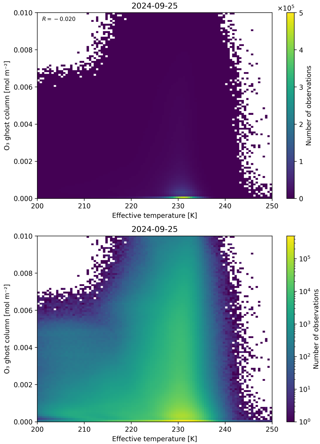
Figure 38: Scatter density plot of “Effective temperature” against “O 3 ghost column” for 2024-09-24 to 2024-09-26.
