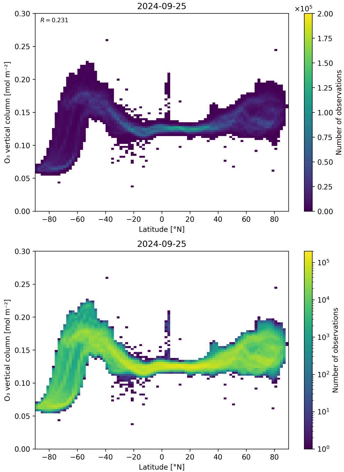
Figure 36: Scatter density plot of “Latitude” against “O 3 vertical column” for 2024-09-24 to 2024-09-26.
