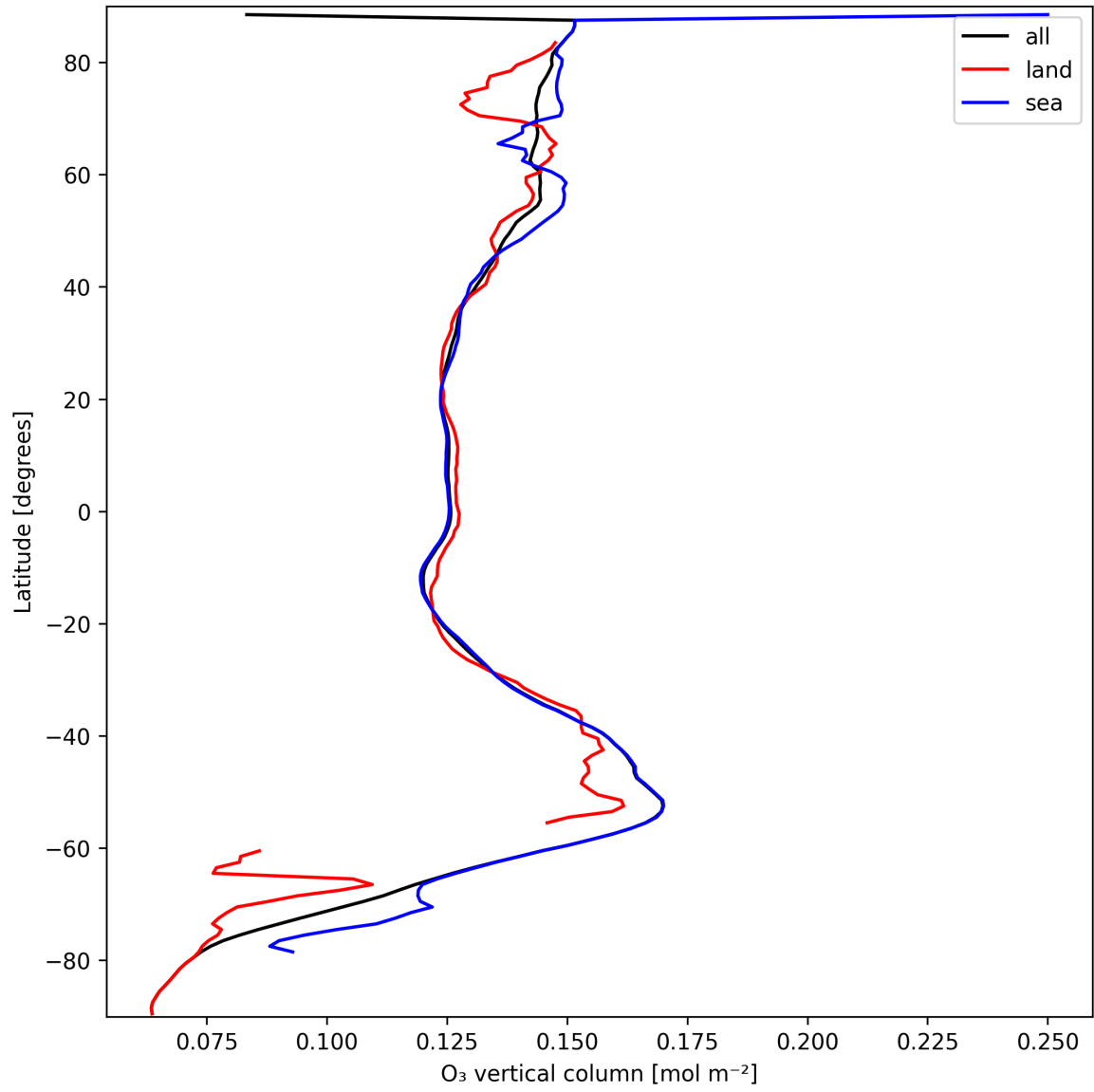
Figure 14: Zonal average of “O 3 vertical column” for 2024-09-24 to 2024-09-26.
