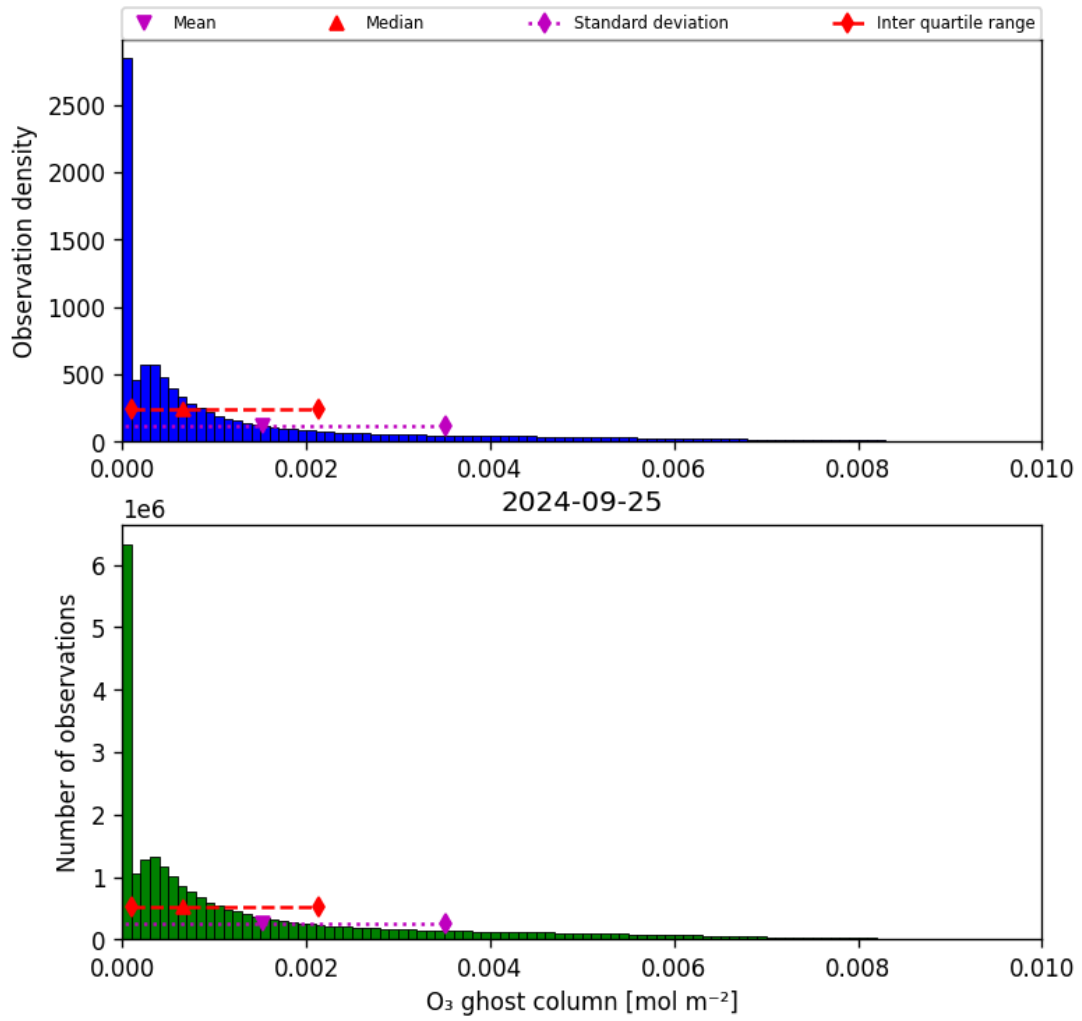
Figure 25: Histogram of “O 3 ghost column” for 2024-09-24 to 2024-09-26
