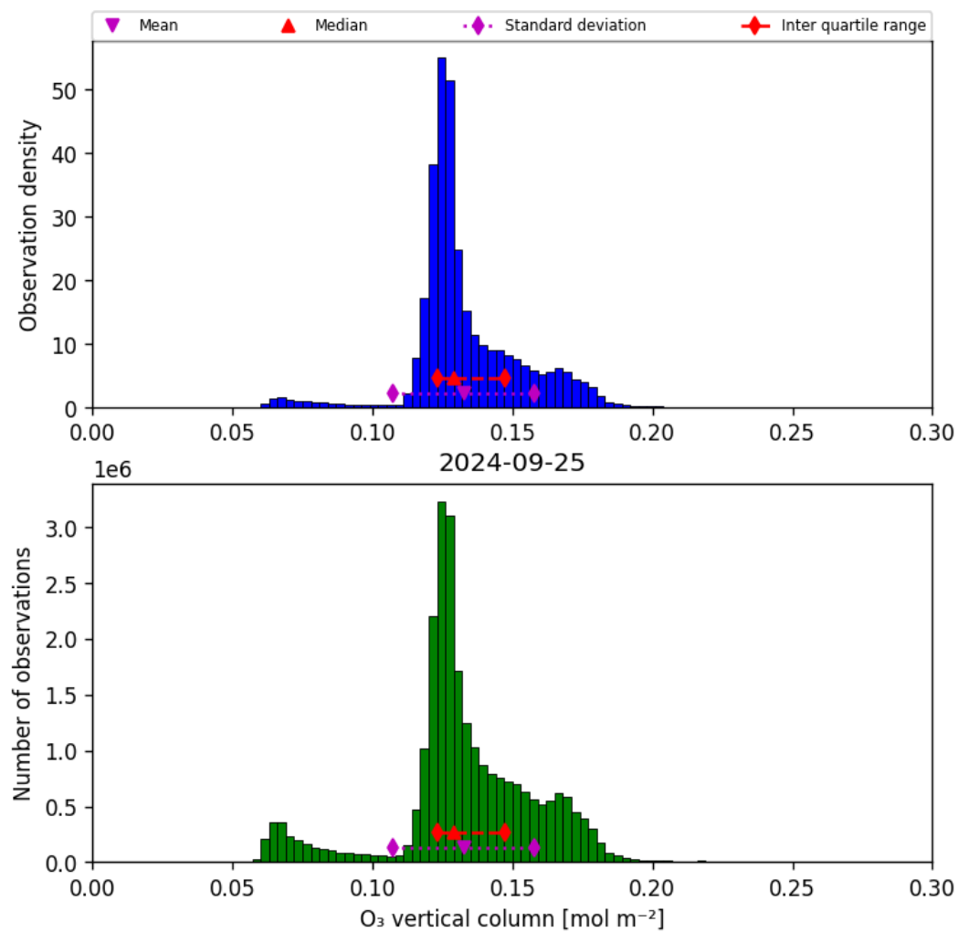
Figure 21: Histogram of “O 3 vertical column” for 2024-09-24 to 2024-09-26
