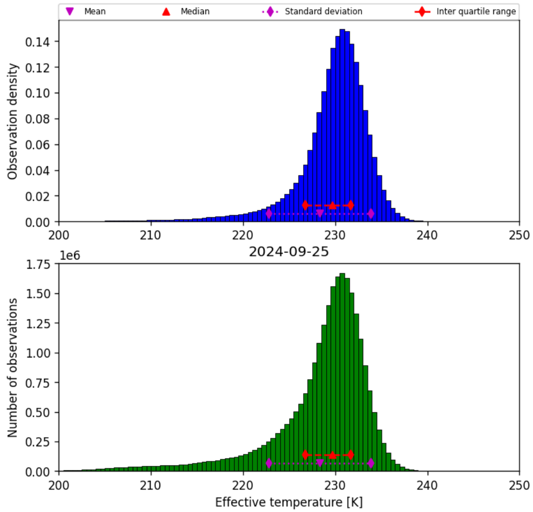
Figure 24: Histogram of “Effective temperature” for 2024-09-24 to 2024-09-26
