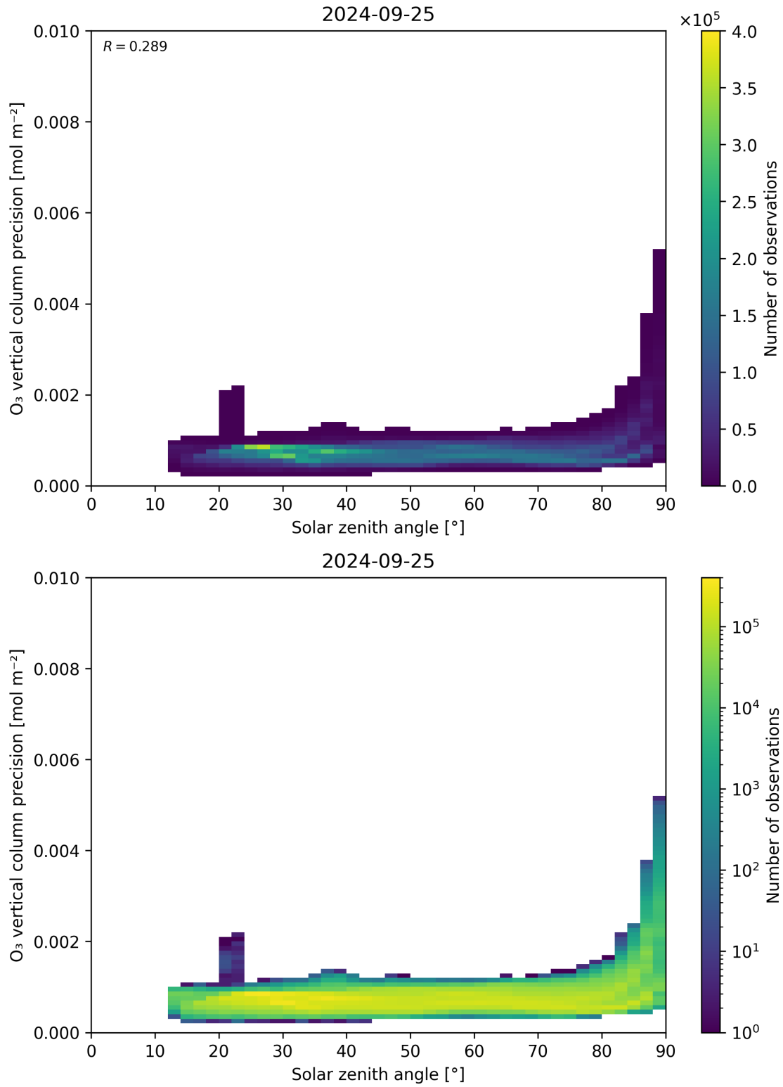
Figure 48: Scatter density plot of “Solar zenith angle” against “O 3 vertical column precision” for 2024-09-24 to 2024-09-26.
