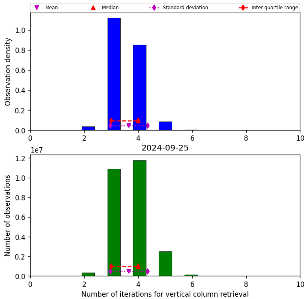
Figure 26: Histogram of “Number of iterations for vertical column retrieval” for 2024-09-24 to 2024-09-26
