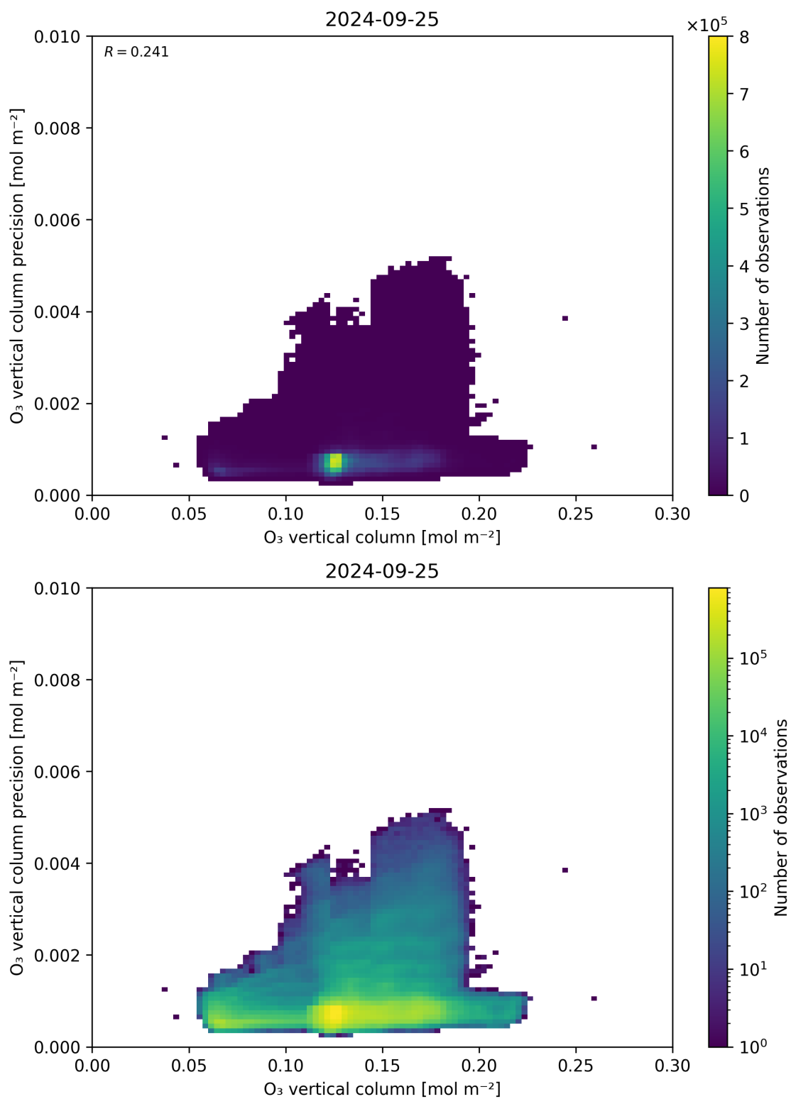
Figure 41: Scatter density plot of “O 3 vertical column” against “O 3 vertical column precision” for 2024-09-24 to 2024-09-26.
