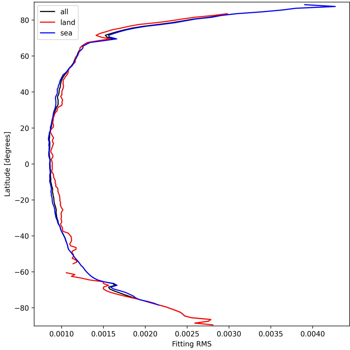
Figure 16: Zonal average of “Fitting RMS” for 2024-09-24 to 2024-09-26.
