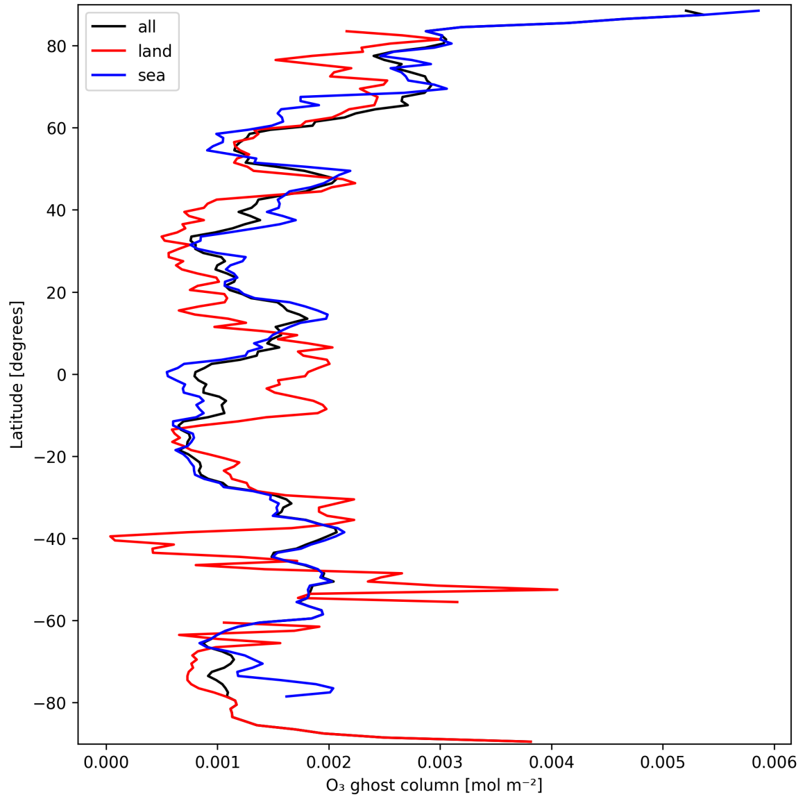
Figure 18: Zonal average of "O 3 ghost column" for 2024-09-24 to 2024-09-26.
