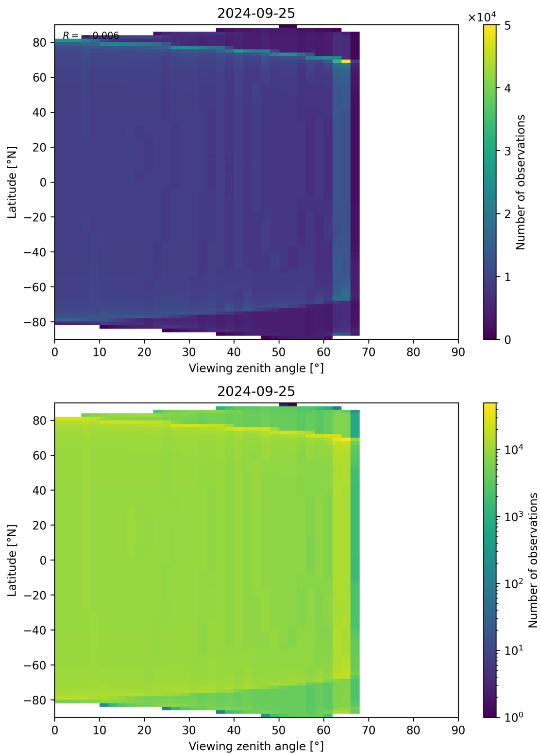
Figure 49: Scatter density plot of “Viewing zenith angle” against “Latitude” for 2024-09-24 to 2024-09-26.
