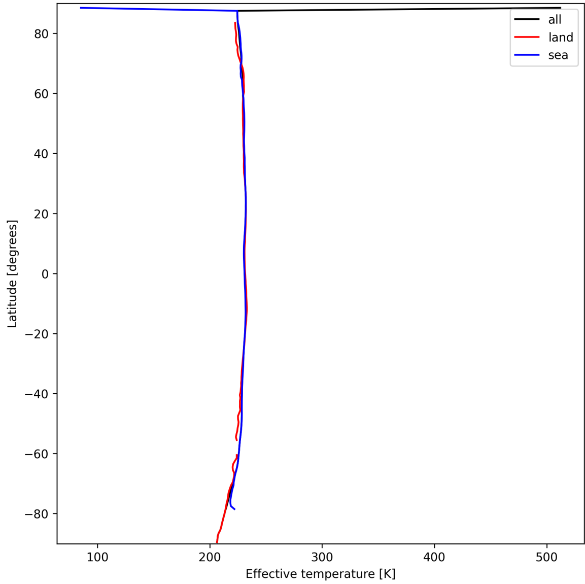
Figure 17: Zonal average of "Effective temperature" for 2024-09-24 to 2024-09-26.
