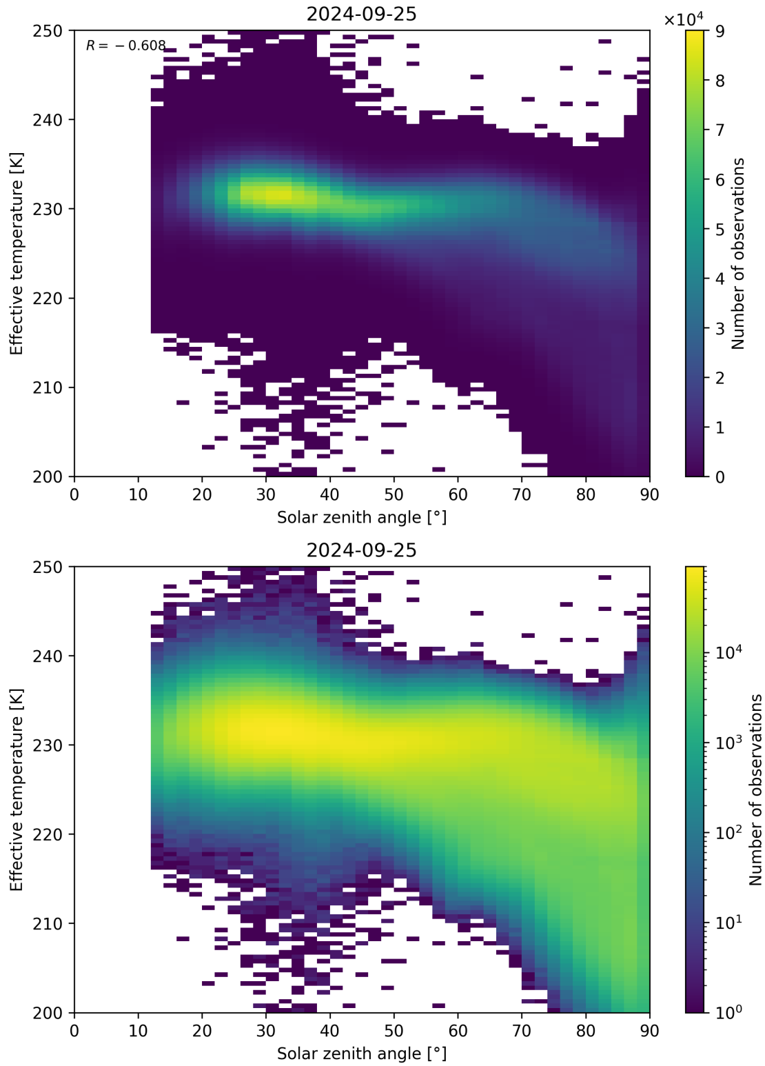
Figure 45: Scatter density plot of “Solar zenith angle” against “Effective temperature” for 2024-09-24 to 2024-09-26.
