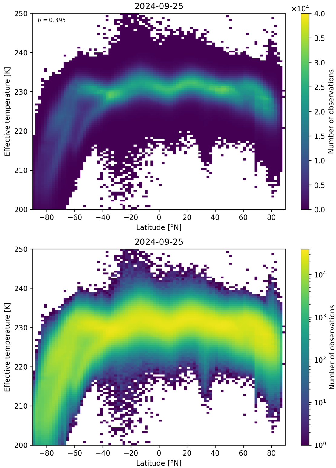
Figure 34: Scatter density plot of “Latitude” against “Effective temperature” for 2024-09-24 to 2024-09-26.
