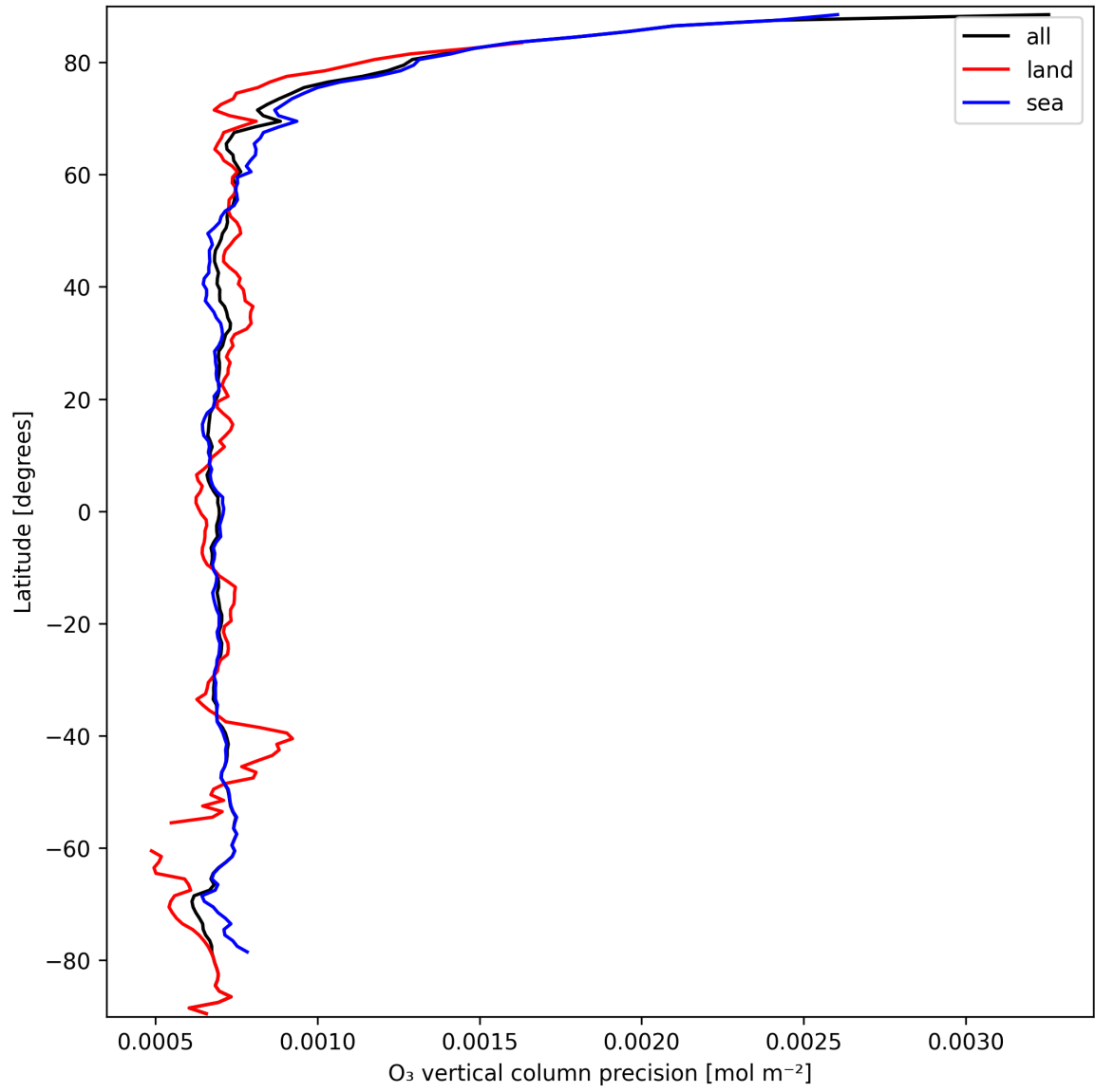
Figure 15: Zonal average of “O 3 vertical column precision” for 2024-09-24 to 2024-09-26.
