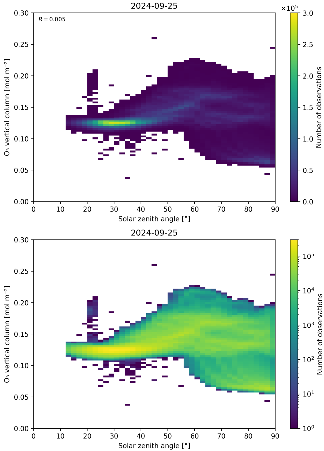
Figure 47: Scatter density plot of “Solar zenith angle” against “O 3 vertical column” for 2024-09-24 to 2024-09-26.
