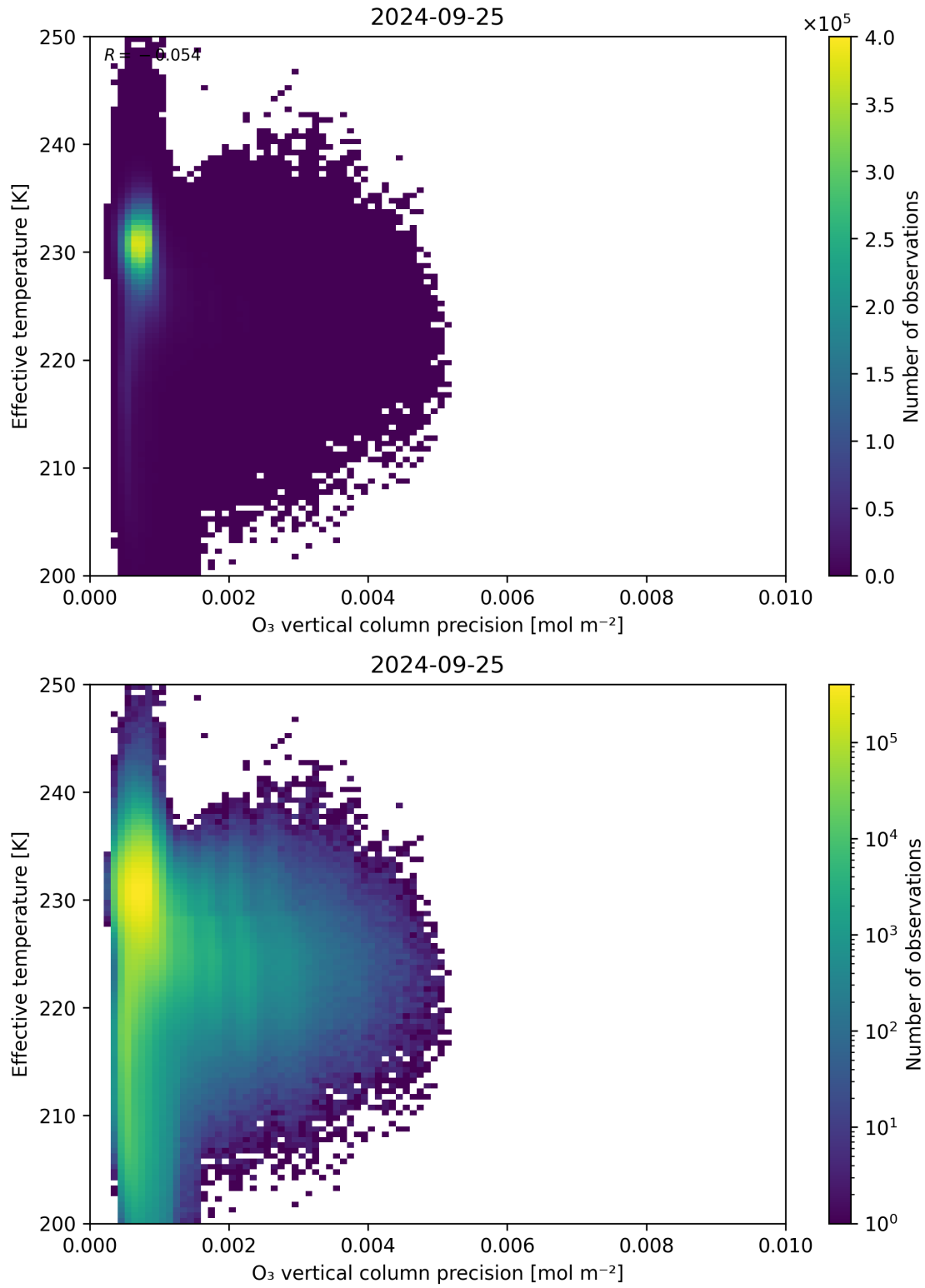
Figure 42: Scatter density plot of “O 3 vertical column precision” against “Effective temperature” for 2024-09-24 to 2024-09-26.
