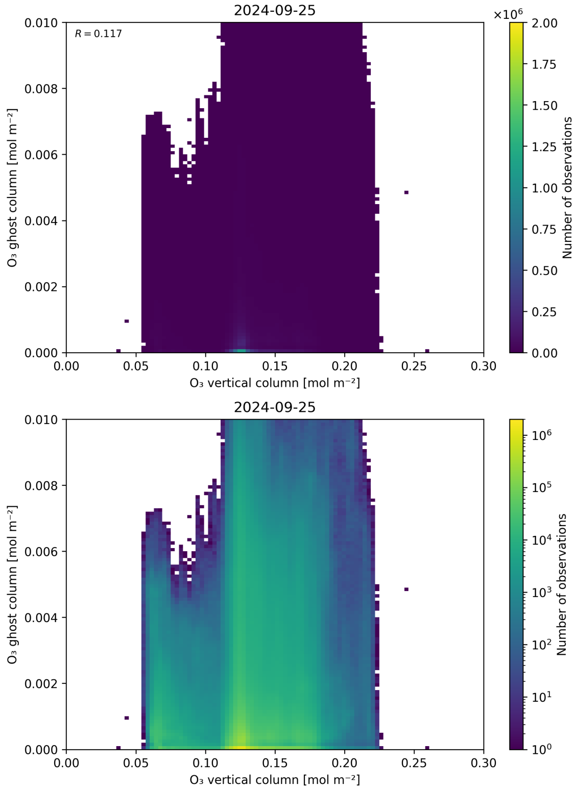
Figure 40: Scatter density plot of “O 3 vertical column” against “O 3 ghost column” for 2024-09-24 to 2024-09-26.
