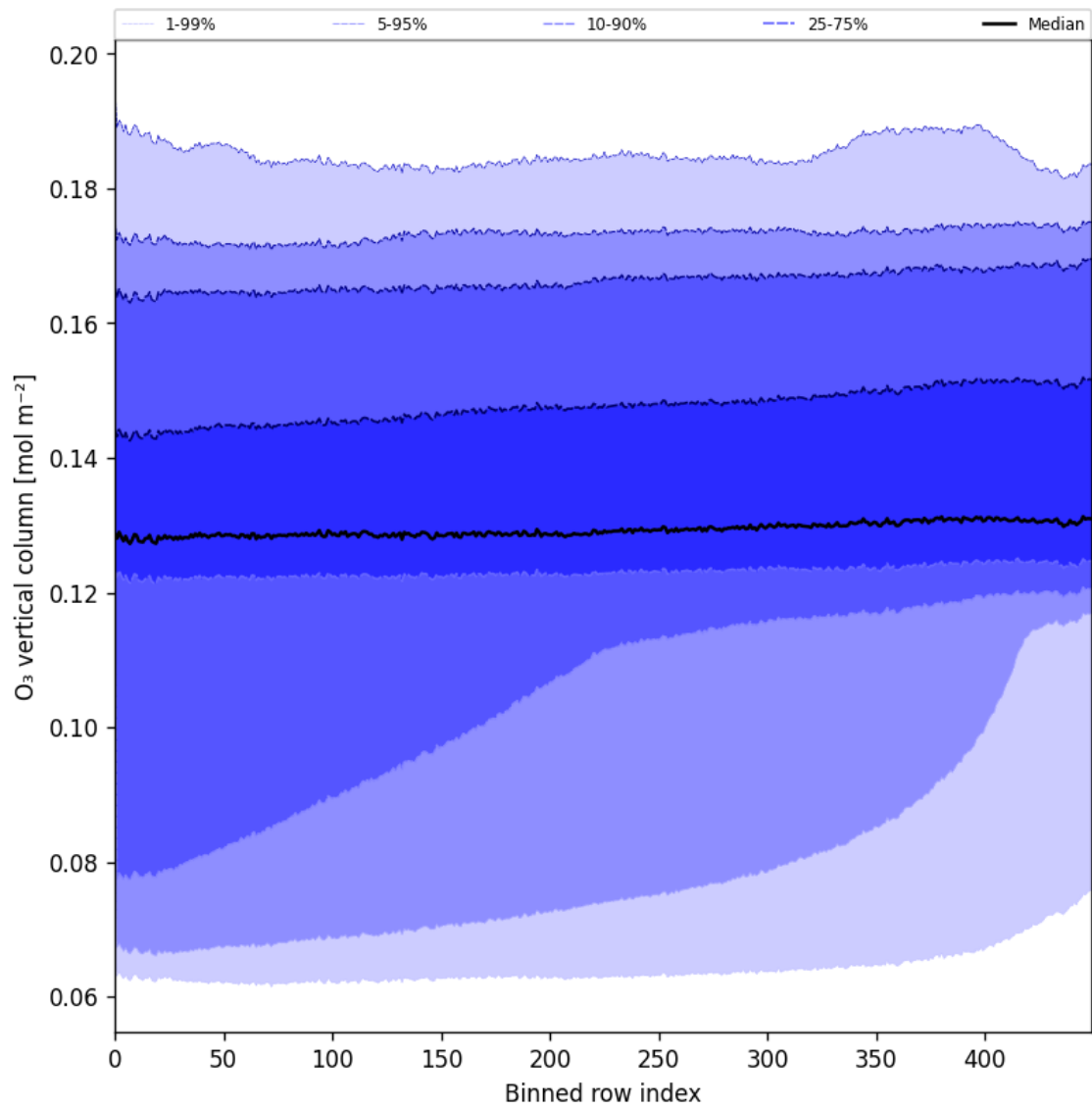
Figure 28: Along track statistics of “O 3 vertical column” for 2024-09-24 to 2024-09-26
