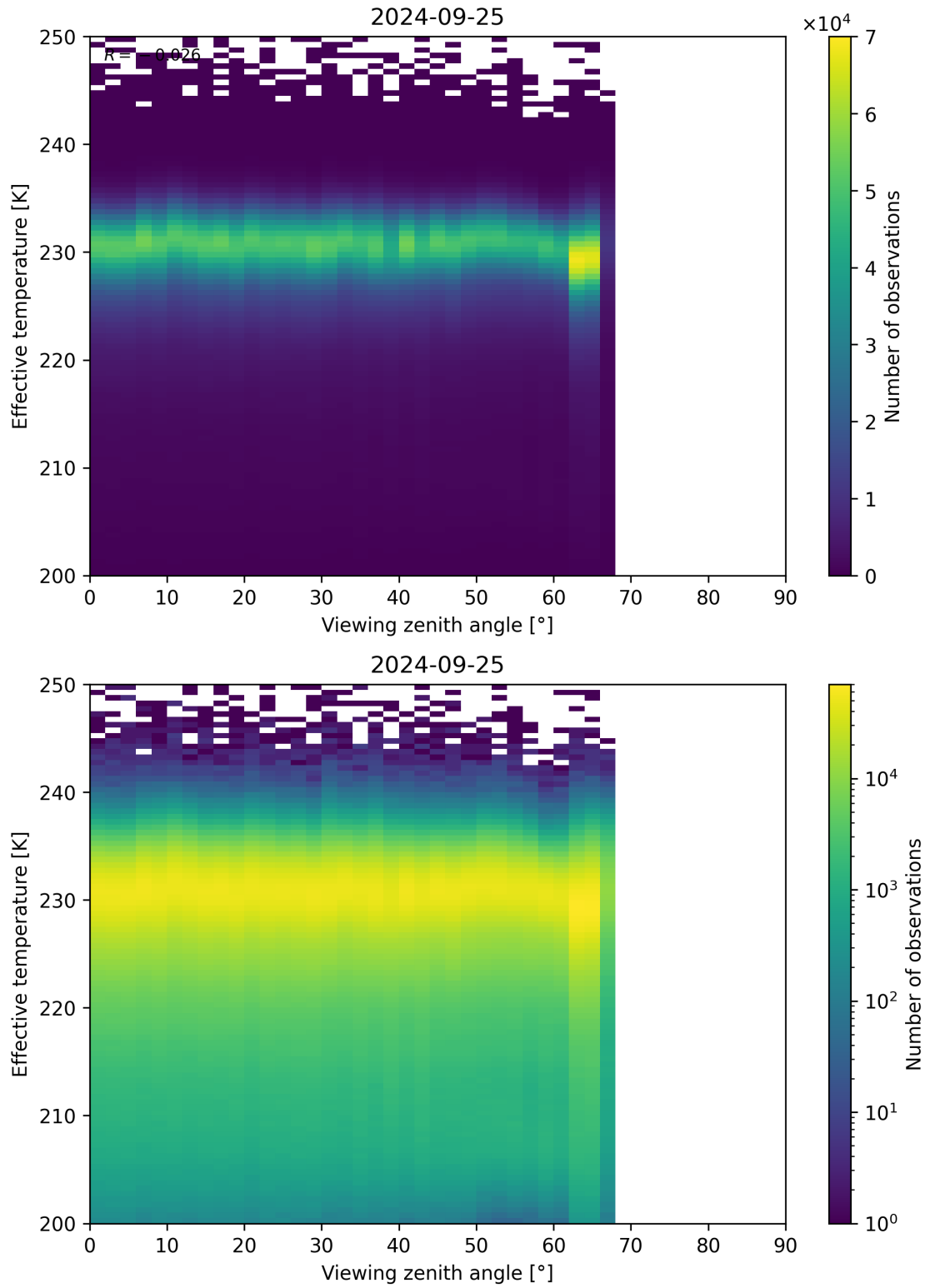
Figure 50: Scatter density plot of “Viewing zenith angle” against “Effective temperature” for 2024-09-24 to 2024-09-26.
