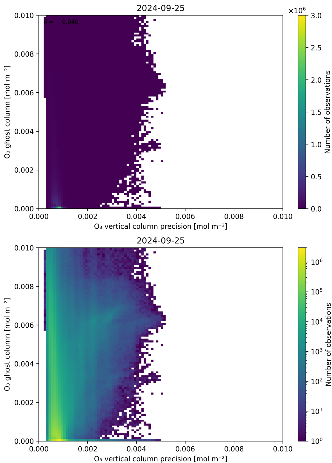
Figure 43: Scatter density plot of “ \text{O}_3 vertical column precision” against “ \text{O}_3 ghost column” for 2024-09-24 to 2024-09-26.
