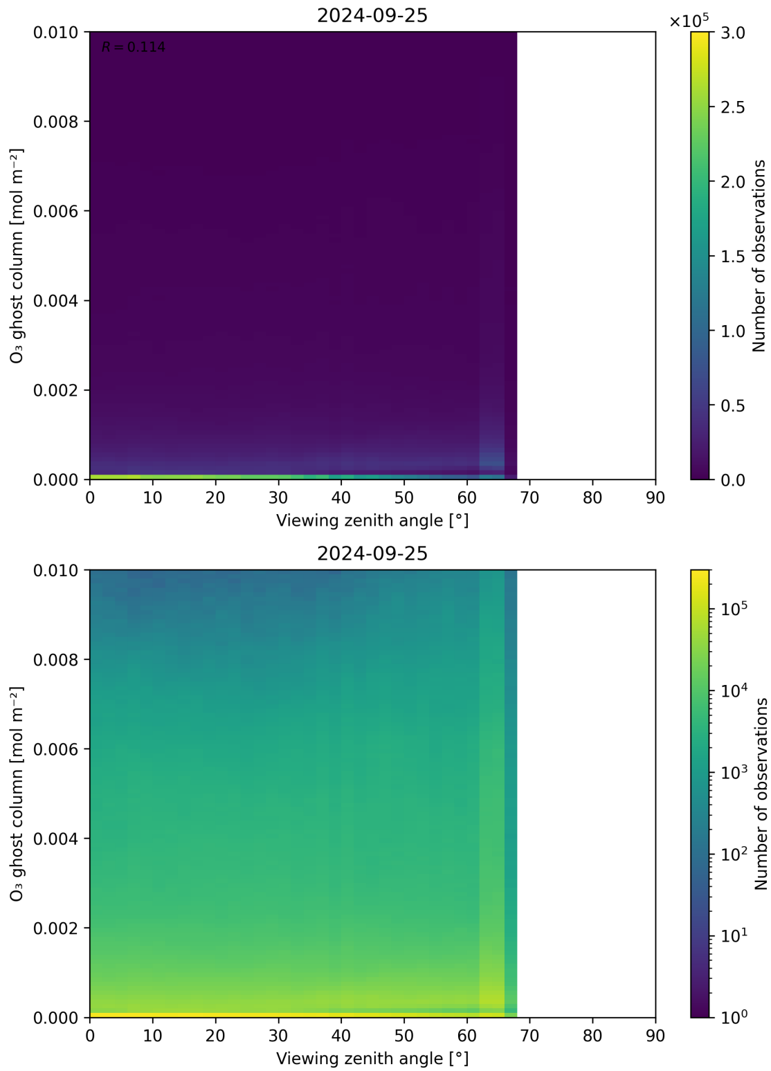
Figure 51: Scatter density plot of “Viewing zenith angle” against “O 3 ghost column” for 2024-09-24 to 2024-09-26.
