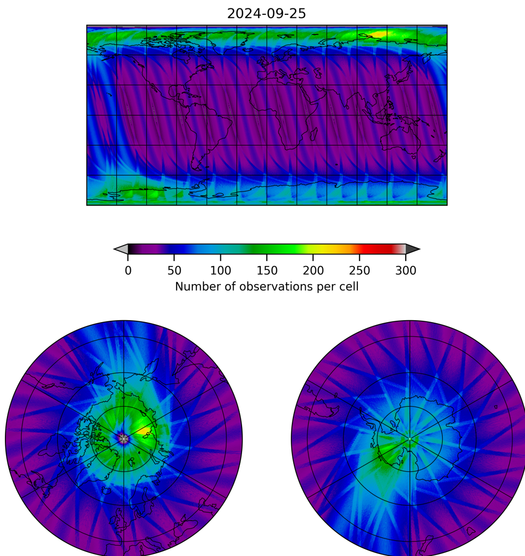
Figure 12: Map of the number of observations for 2024-09-24 to 2024-09-26
