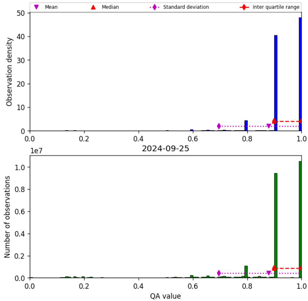
Figure 20: Histogram of “QA value” for 2024-09-24 to 2024-09-26
