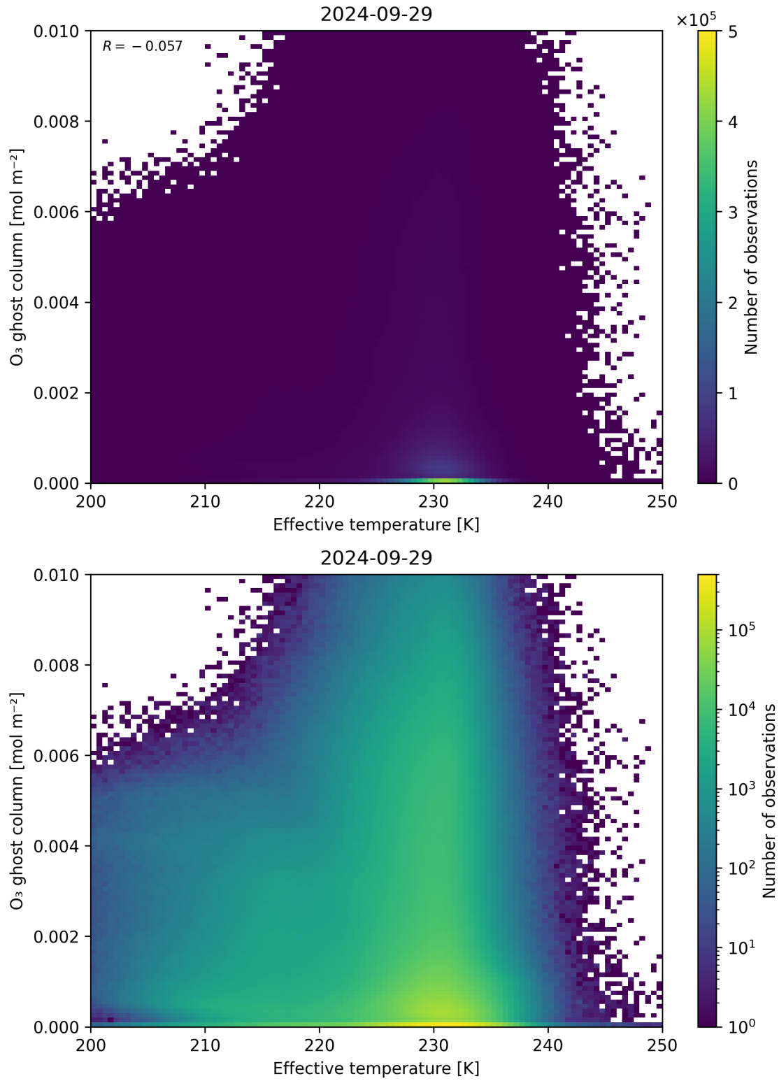
Figure 38: Scatter density plot of “Effective temperature” against “O 3 ghost column” for 2024-09-28 to 2024-09-30.
