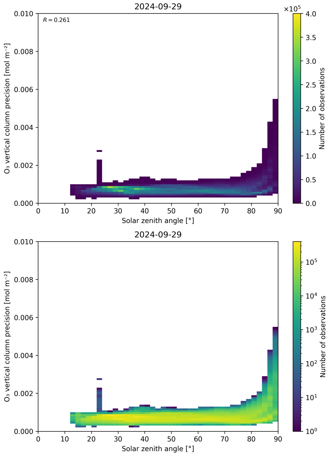
Figure 48: Scatter density plot of “Solar zenith angle” against “O 3 vertical column precision” for 2024-09-28 to 2024-09-30.
