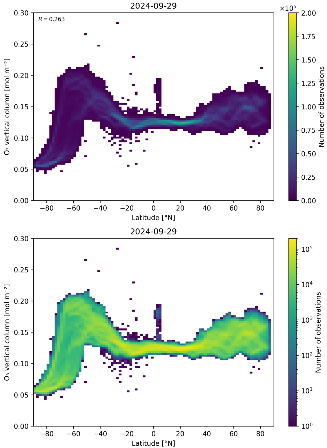
Figure 36: Scatter density plot of “Latitude” against “O 3 vertical column” for 2024-09-28 to 2024-09-30.
