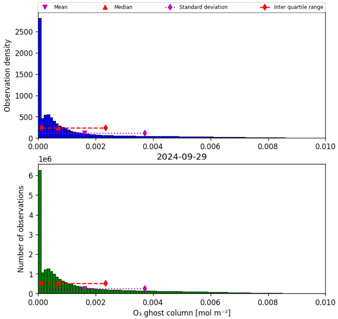
Figure 25: Histogram of “O 3 ghost column” for 2024-09-28 to 2024-09-30
