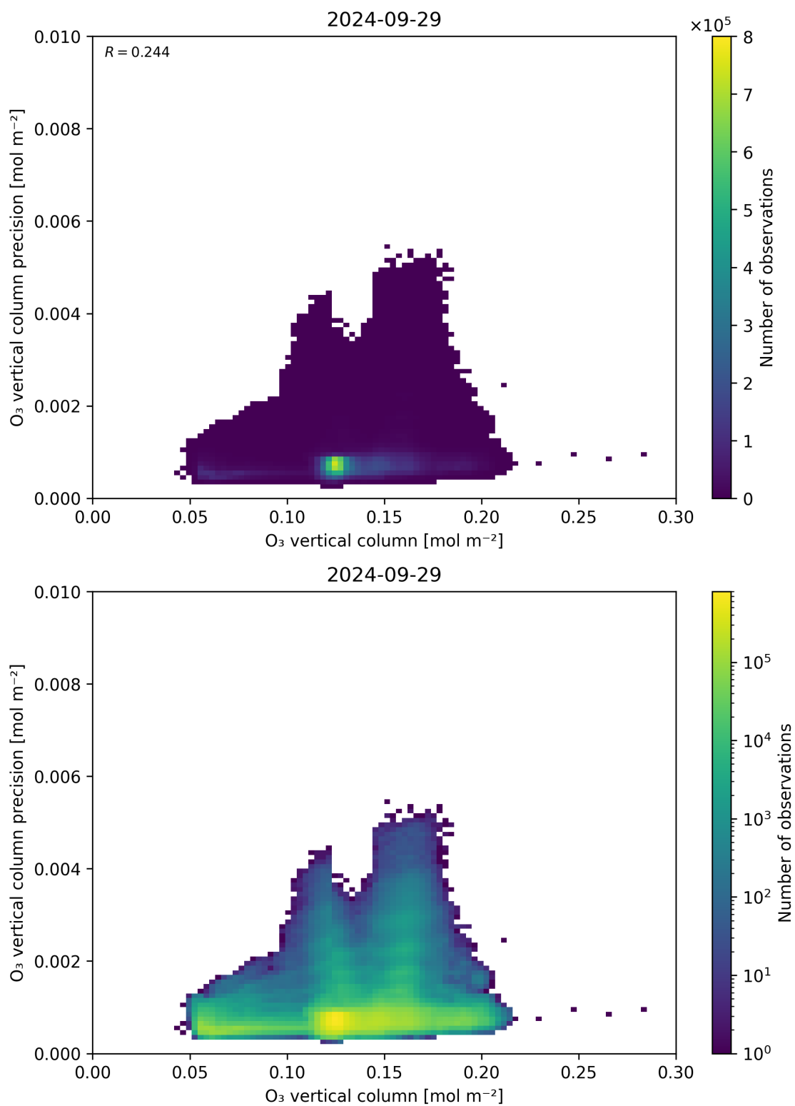
Figure 41: Scatter density plot of “O 3 vertical column” against “O 3 vertical column precision” for 2024-09-28 to 2024-09-30.
