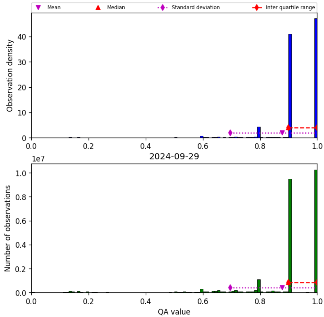
Figure 20: Histogram of “QA value” for 2024-09-28 to 2024-09-30
