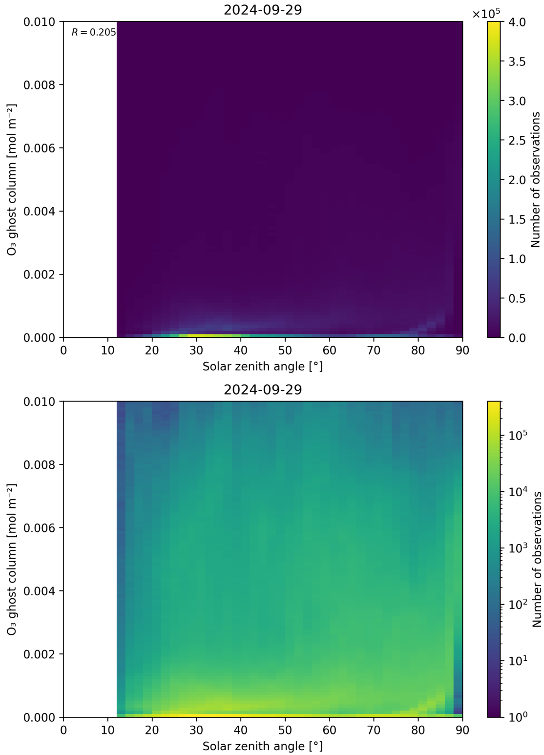
Figure 46: Scatter density plot of “Solar zenith angle” against “O 3 ghost column” for 2024-09-28 to 2024-09-30.
