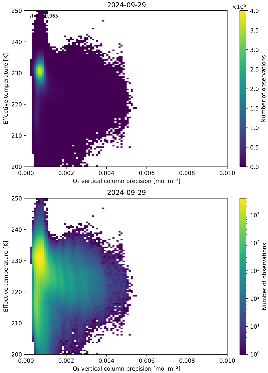
Figure 42: Scatter density plot of “O 3 vertical column precision” against “Effective temperature” for 2024-09-28 to 2024-09-30.
