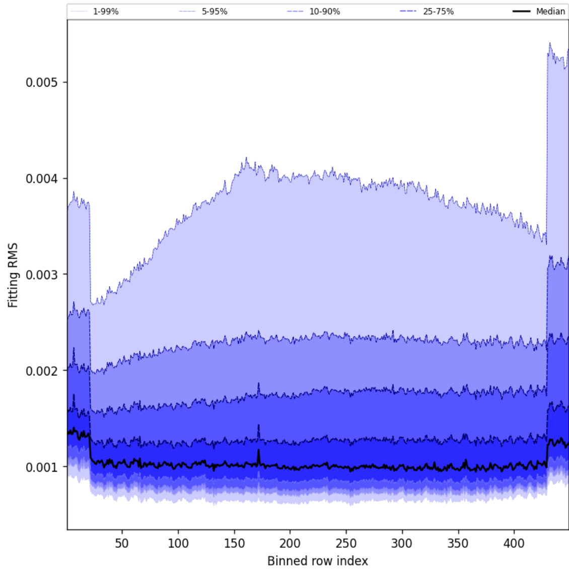
Figure 30: Along track statistics of “Fitting RMS” for 2024-09-28 to 2024-09-30
