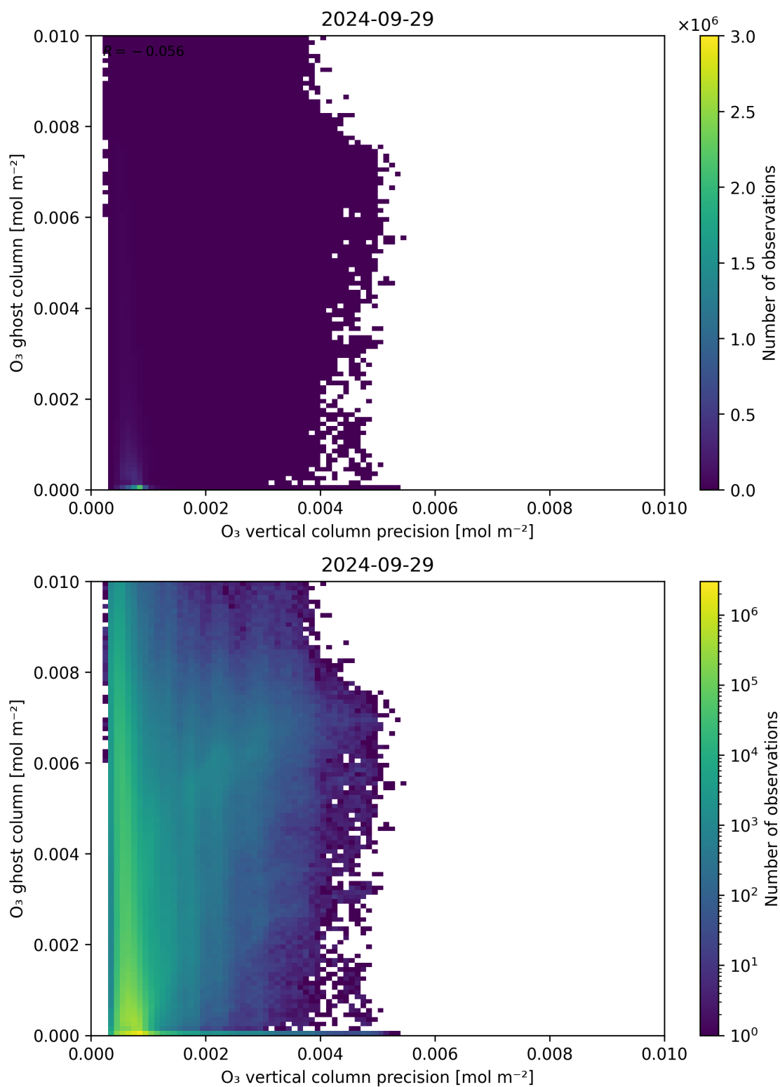
Figure 43: Scatter density plot of “ \text{O}_3 vertical column precision” against “ \text{O}_3 ghost column” for 2024-09-28 to 2024-09-30.
