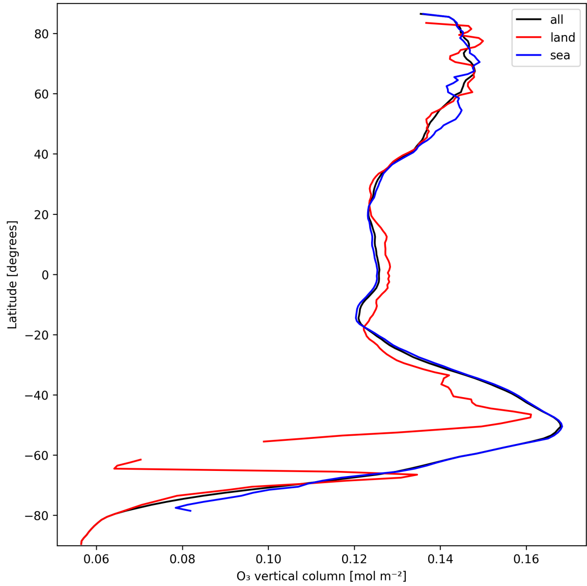
Figure 14: Zonal average of “O 3 vertical column” for 2024-09-28 to 2024-09-30.
