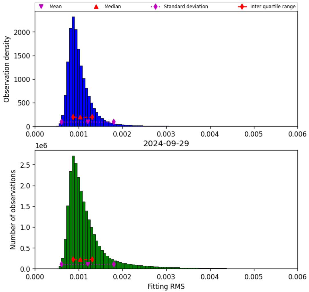
Figure 23: Histogram of “Fitting RMS” for 2024-09-28 to 2024-09-30
