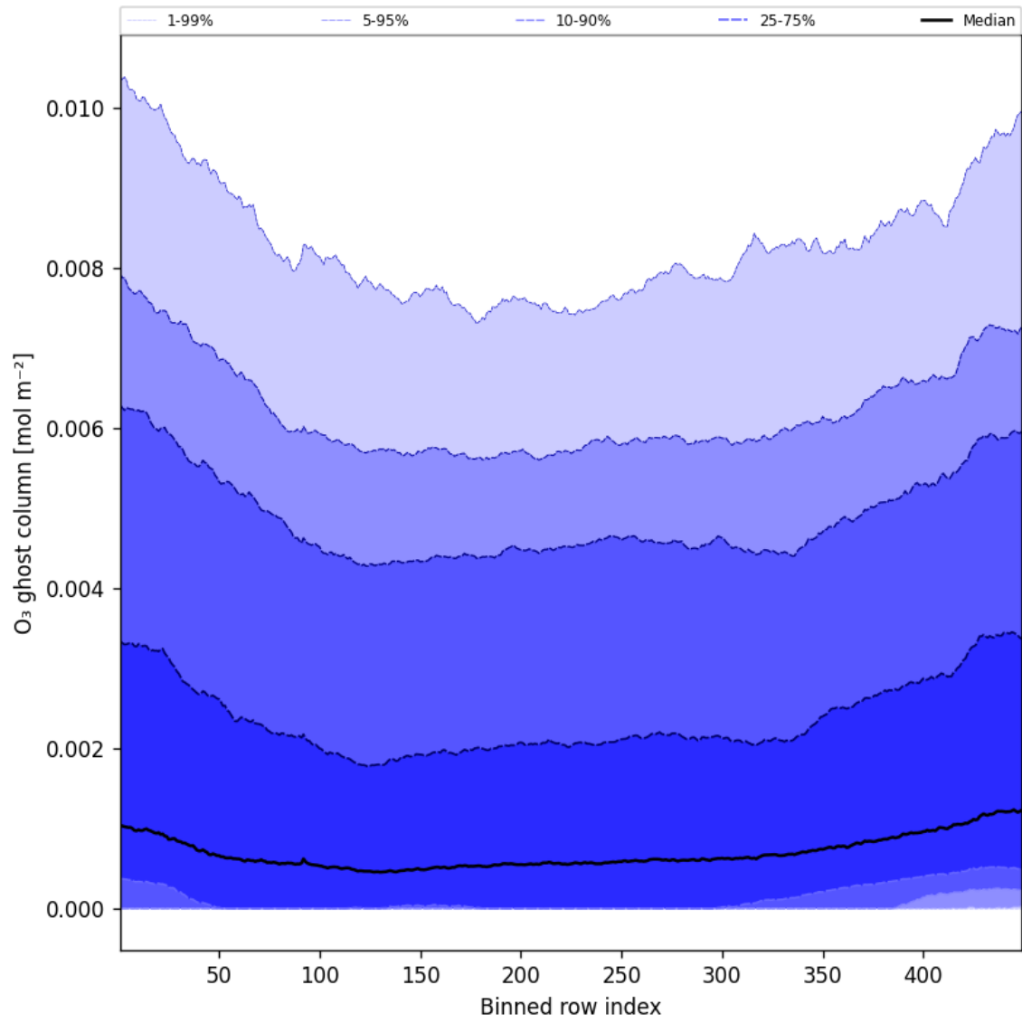
Figure 32: Along track statistics of “O 3 ghost column” for 2024-09-28 to 2024-09-30
