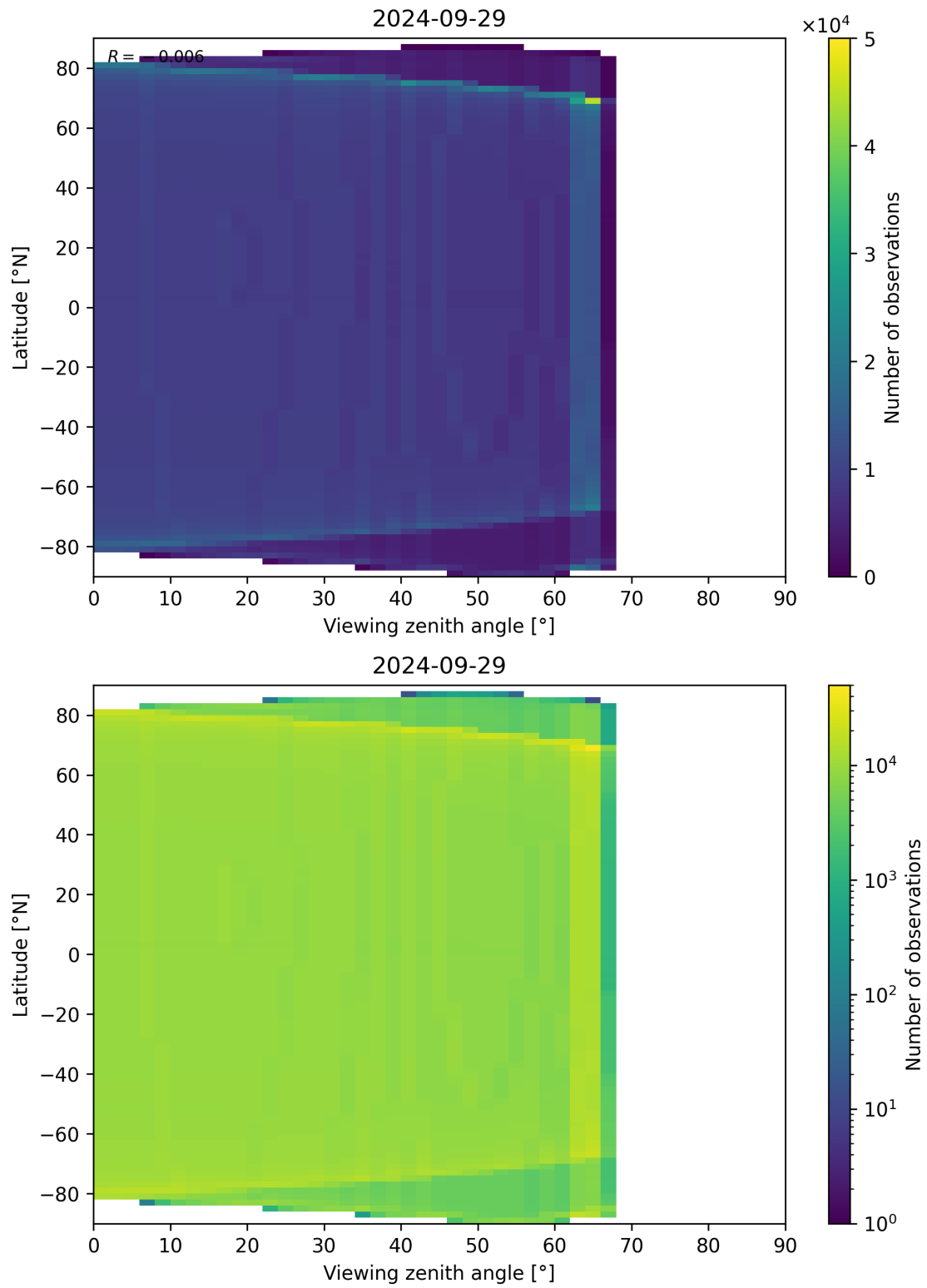
Figure 49: Scatter density plot of “Viewing zenith angle” against “Latitude” for 2024-09-28 to 2024-09-30.
