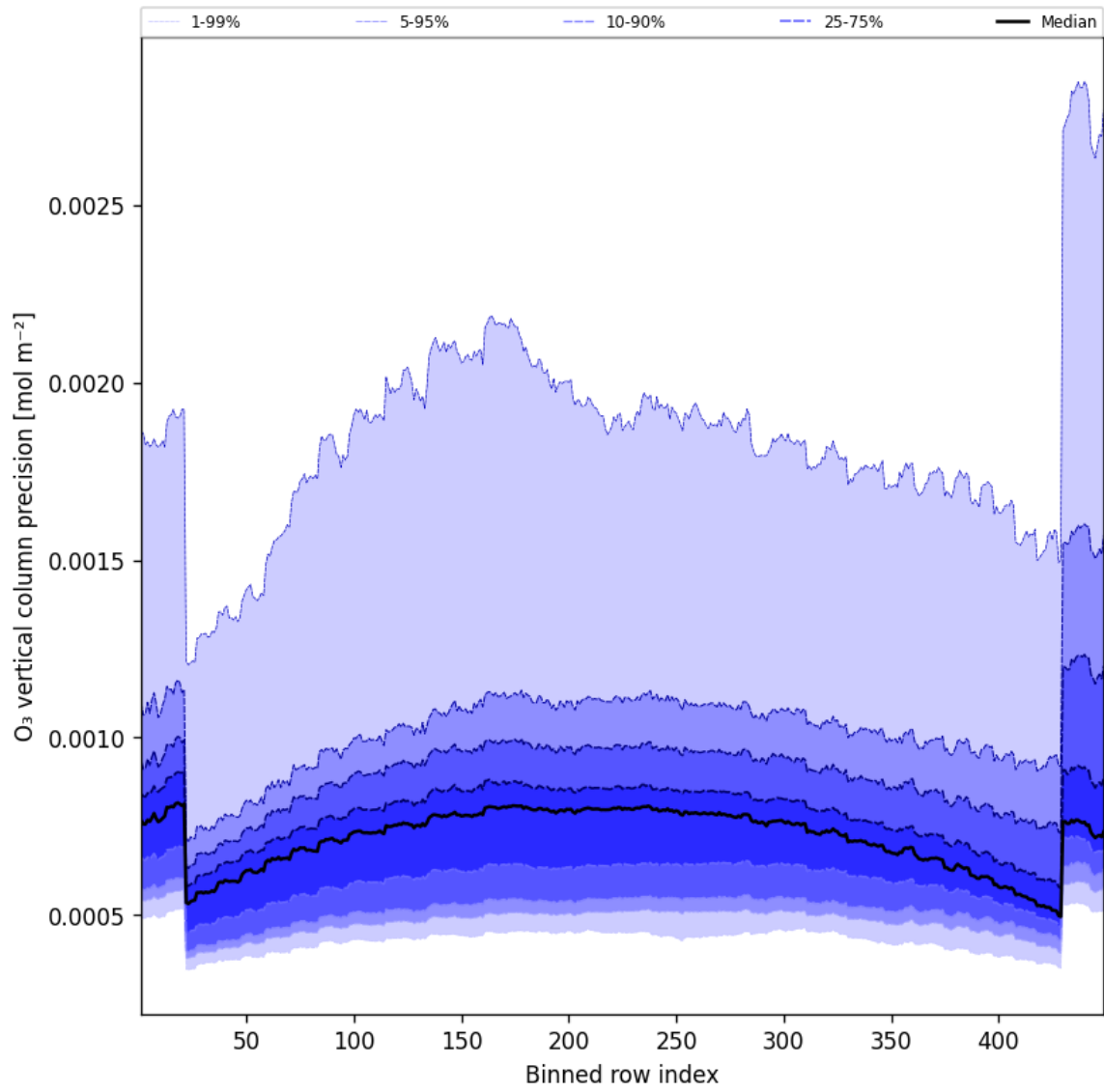
Figure 29: Along track statistics of “O 3 vertical column precision” for 2024-09-28 to 2024-09-30
