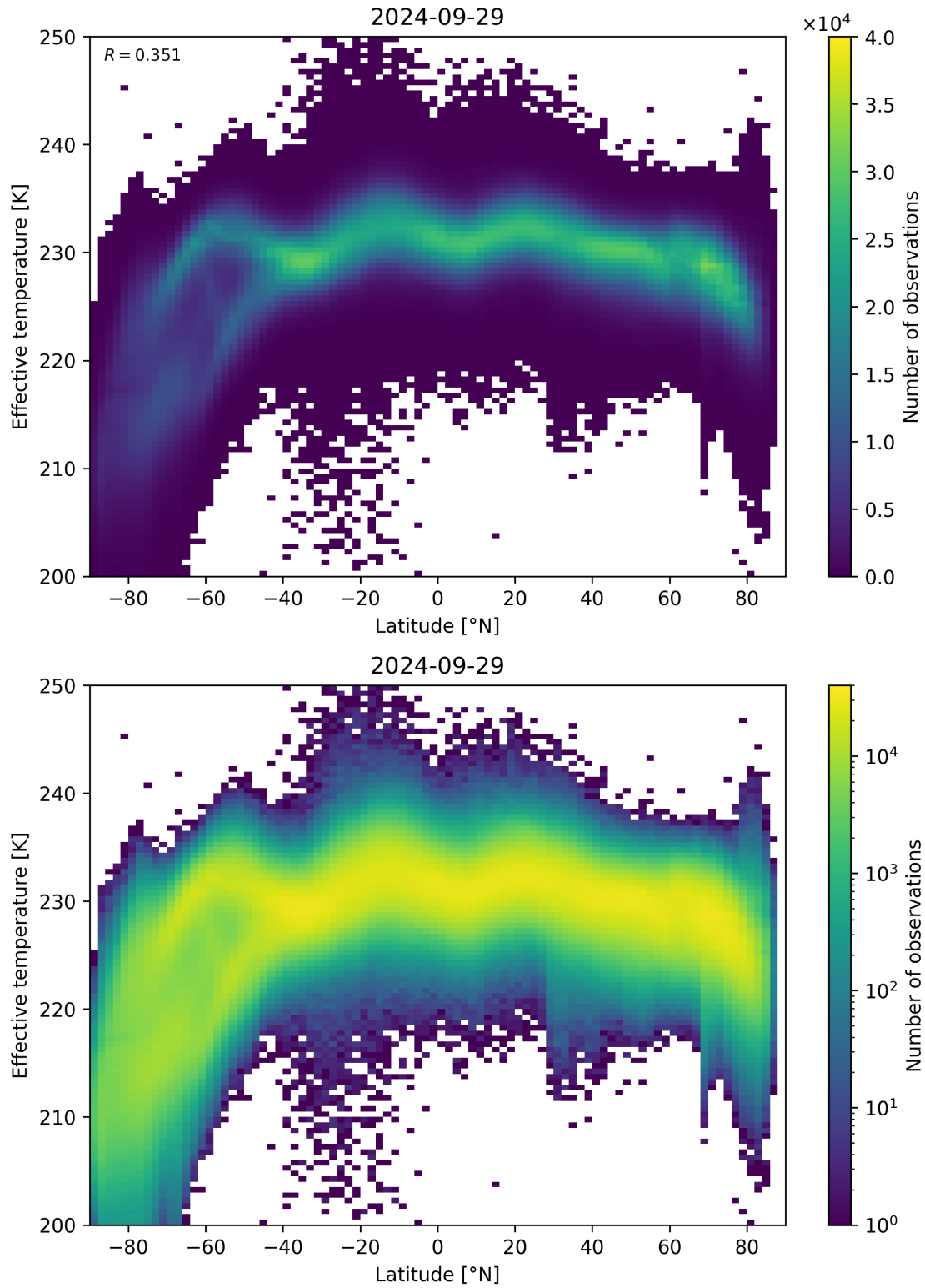
Figure 34: Scatter density plot of “Latitude” against “Effective temperature” for 2024-09-28 to 2024-09-30.
