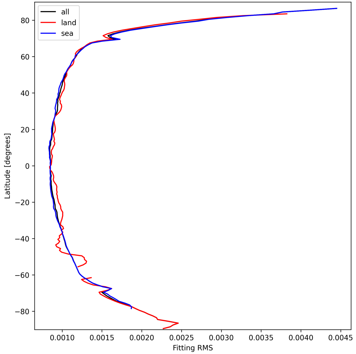
Figure 16: Zonal average of “Fitting RMS” for 2024-09-28 to 2024-09-30.
