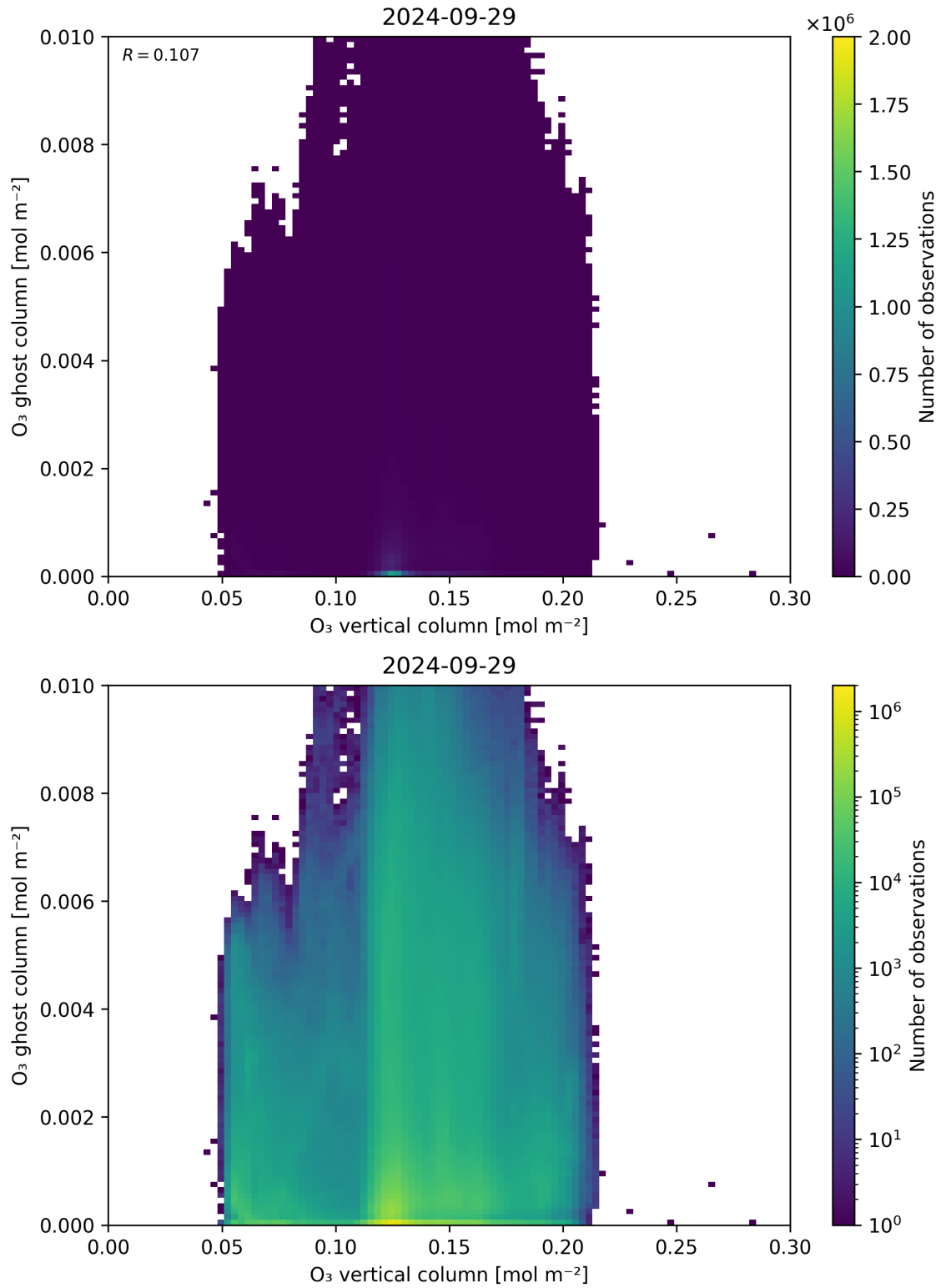
Figure 40: Scatter density plot of “O 3 vertical column” against “O 3 ghost column” for 2024-09-28 to 2024-09-30.
