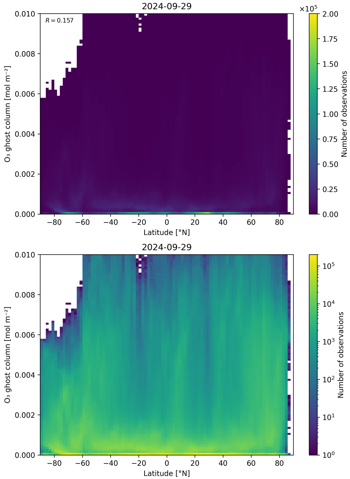
Figure 35: Scatter density plot of “Latitude” against “O 3 ghost column” for 2024-09-28 to 2024-09-30.
