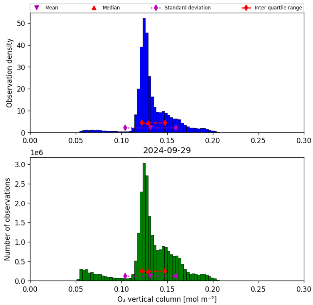
Figure 21: Histogram of “O 3 vertical column” for 2024-09-28 to 2024-09-30
