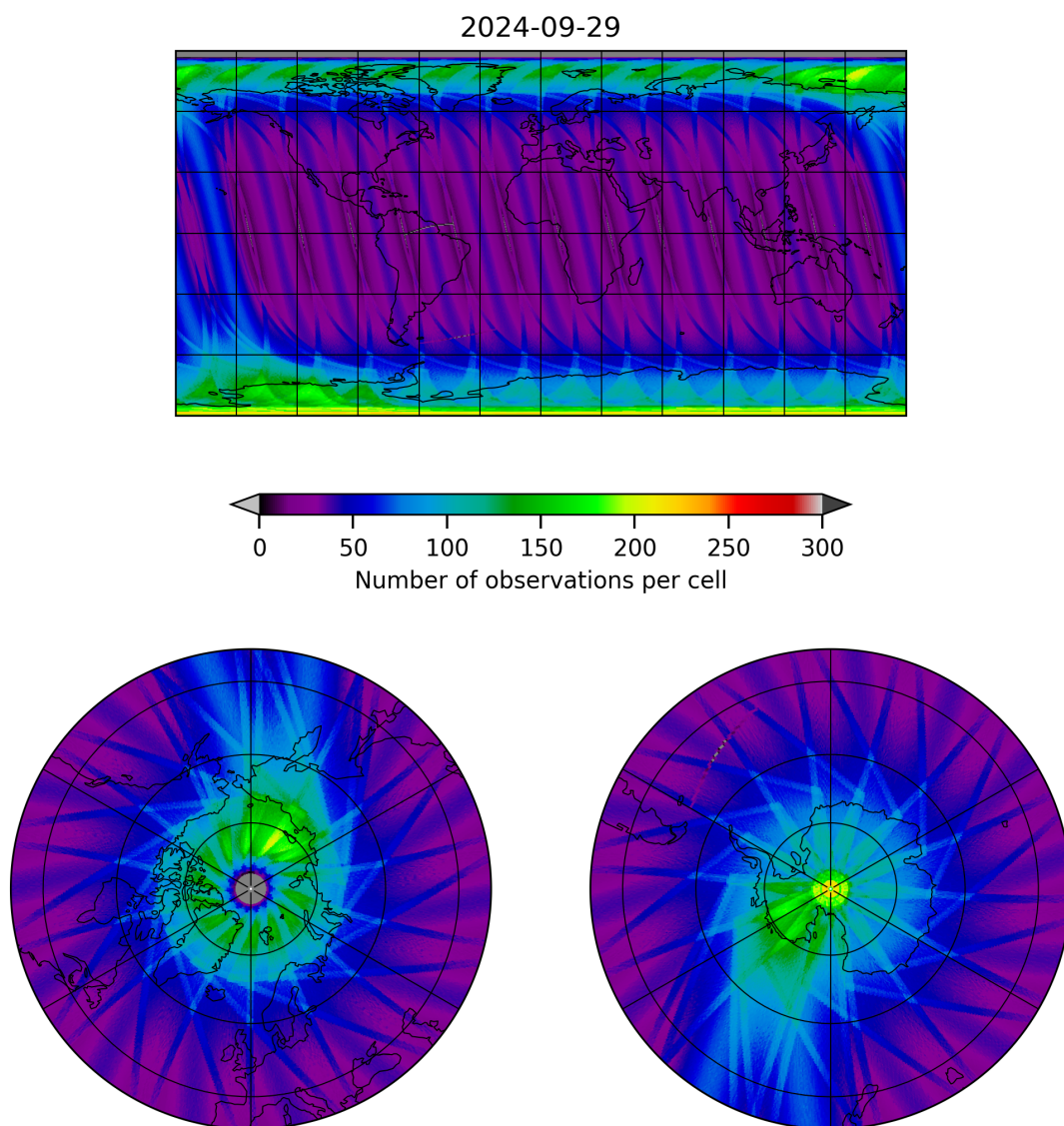
Figure 12: Map of the number of observations for 2024-09-28 to 2024-09-30
