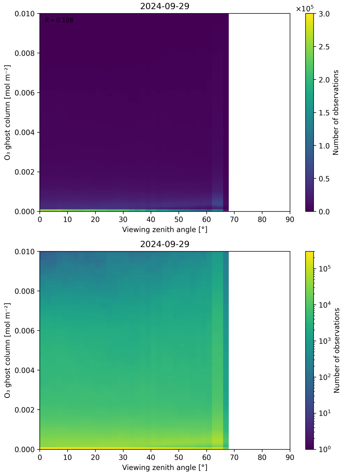
Figure 51: Scatter density plot of “Viewing zenith angle” against “O 3 ghost column” for 2024-09-28 to 2024-09-30.
