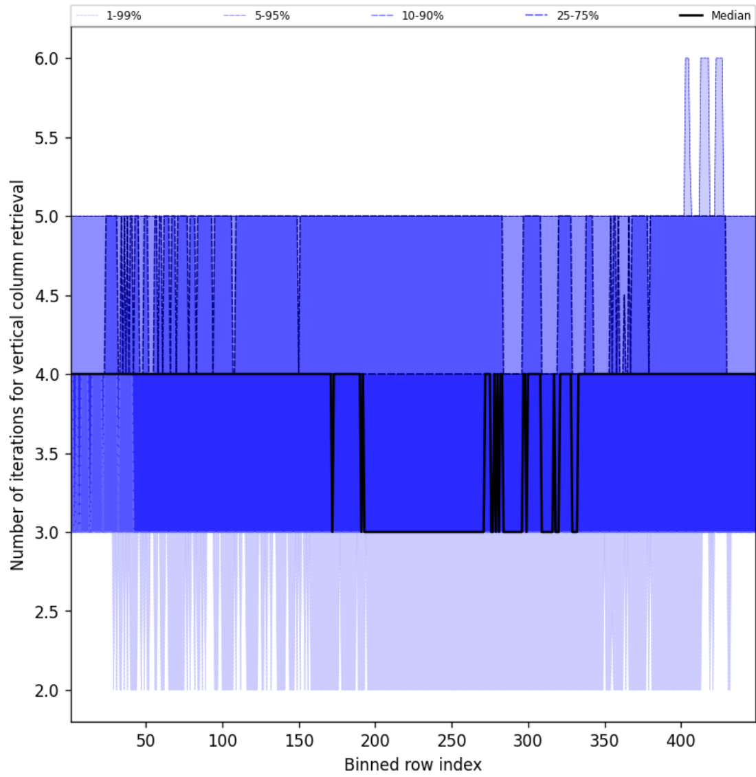
Figure 33: Along track statistics of “Number of iterations for vertical column retrieval” for 2024-09-28 to 2024-09-30
