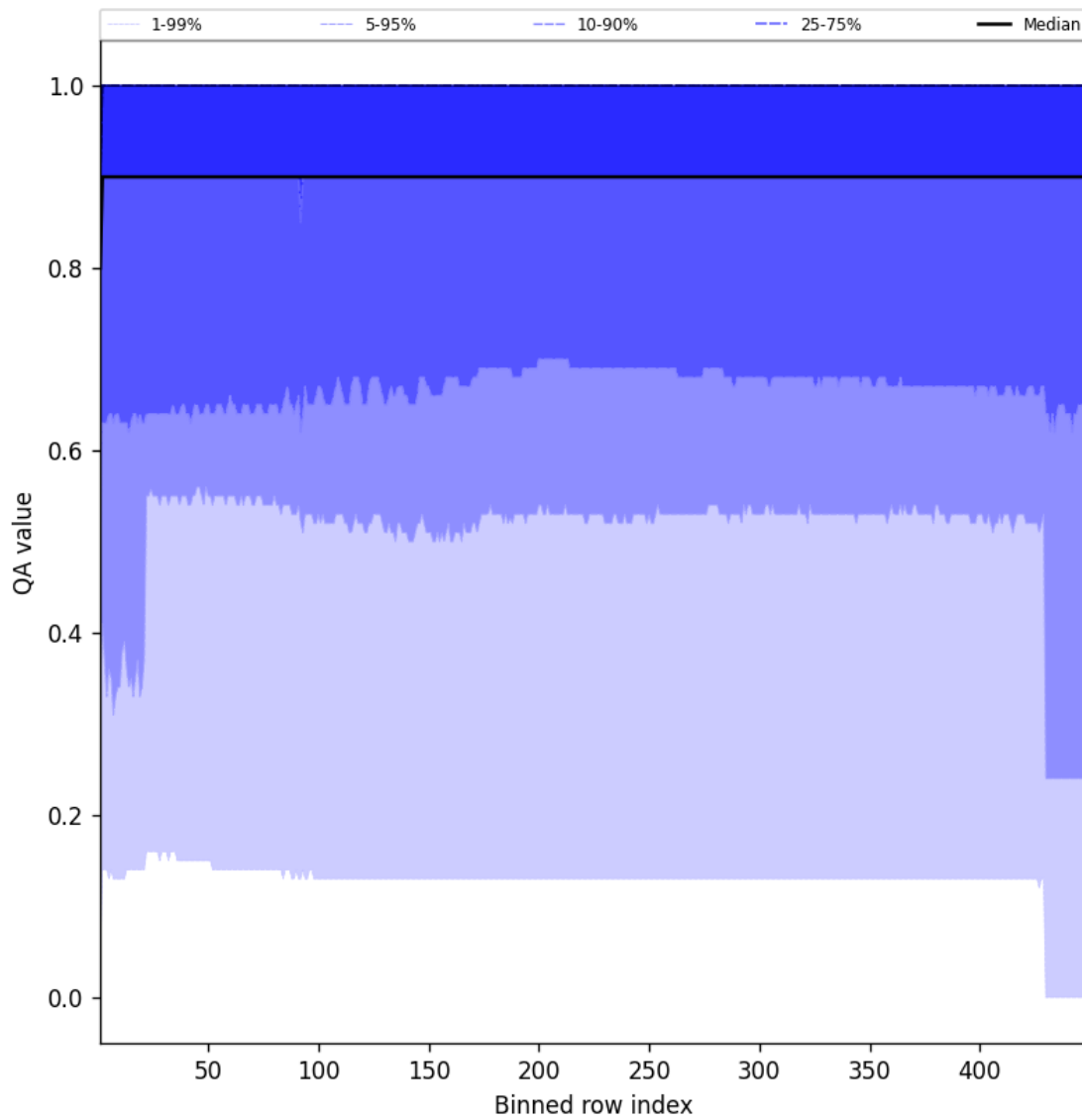
Figure 27: Along track statistics of “QA value” for 2024-09-28 to 2024-09-30
