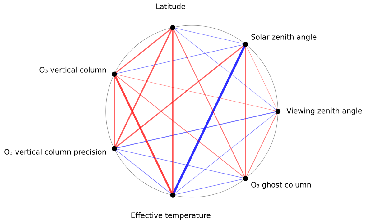
Figure 1: Map of correlation graph for 2024-09-28 to 2024-09-30.
