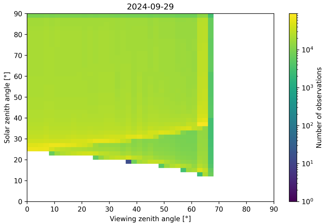
Figure 54: Scatter density plot of “Viewing zenith angle” against “Solar zenith angle” for 2024-09-28 to 2024-09-30.
