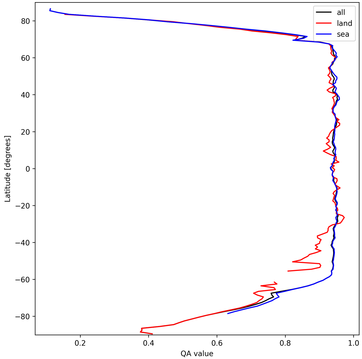
Figure 13: Zonal average of “QA value” for 2024-09-28 to 2024-09-30.
