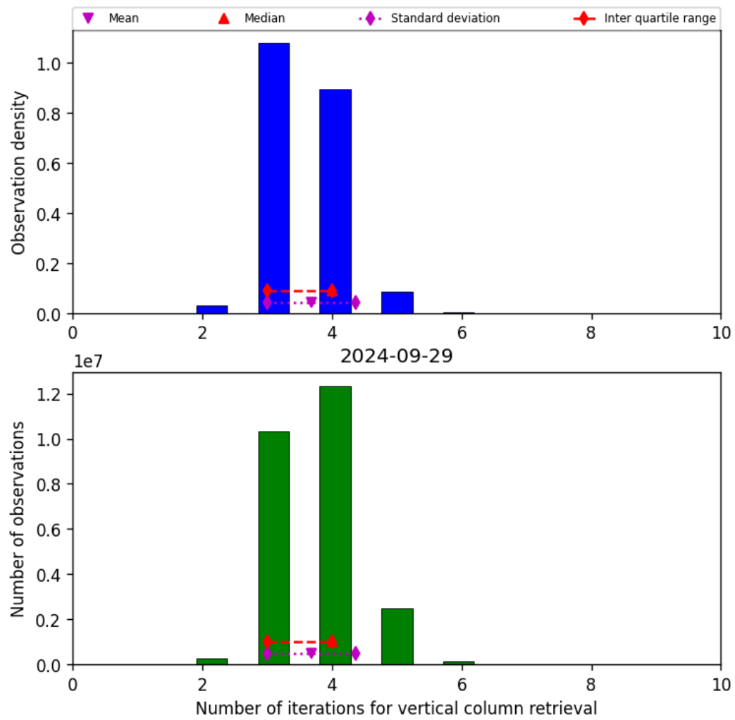
Figure 26: Histogram of “Number of iterations for vertical column retrieval” for 2024-09-28 to 2024-09-30
