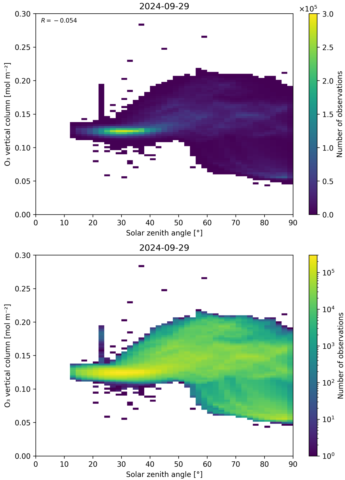
Figure 47: Scatter density plot of “Solar zenith angle” against “O 3 vertical column” for 2024-09-28 to 2024-09-30.
