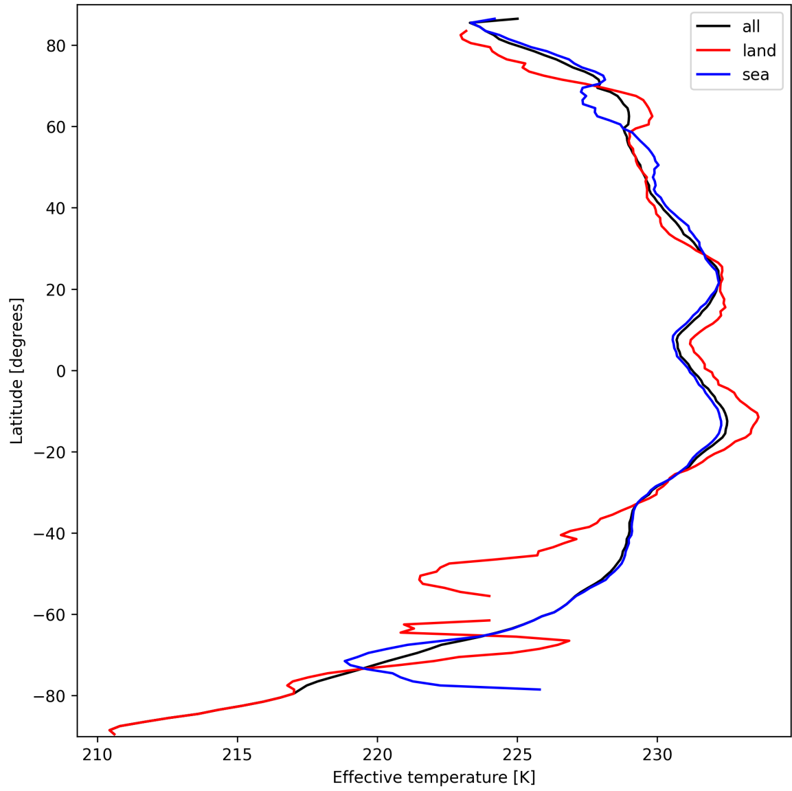
Figure 17: Zonal average of "Effective temperature" for 2024-09-28 to 2024-09-30.
