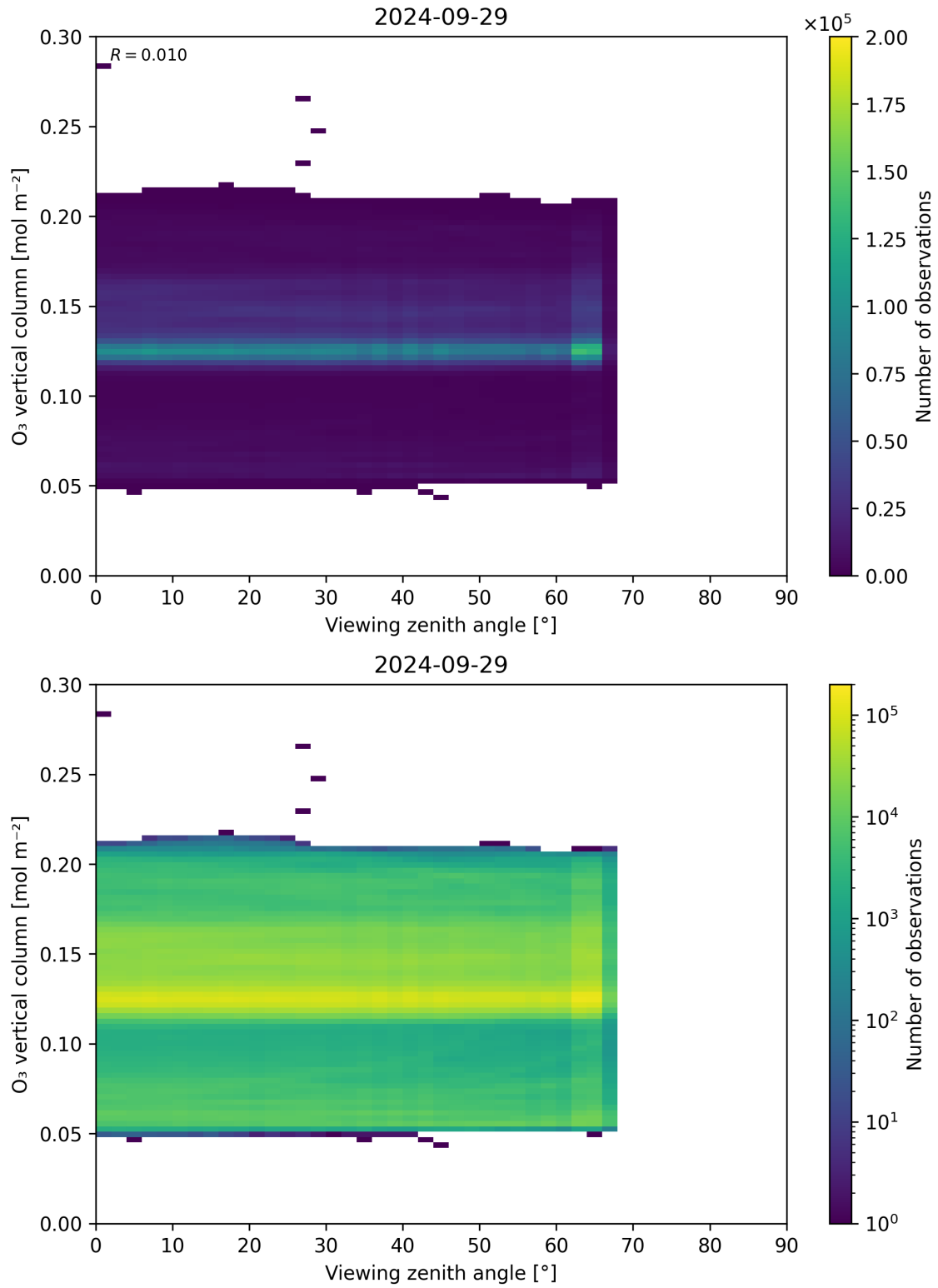
Figure 52: Scatter density plot of “Viewing zenith angle” against “O 3 vertical column” for 2024-09-28 to 2024-09-30.
