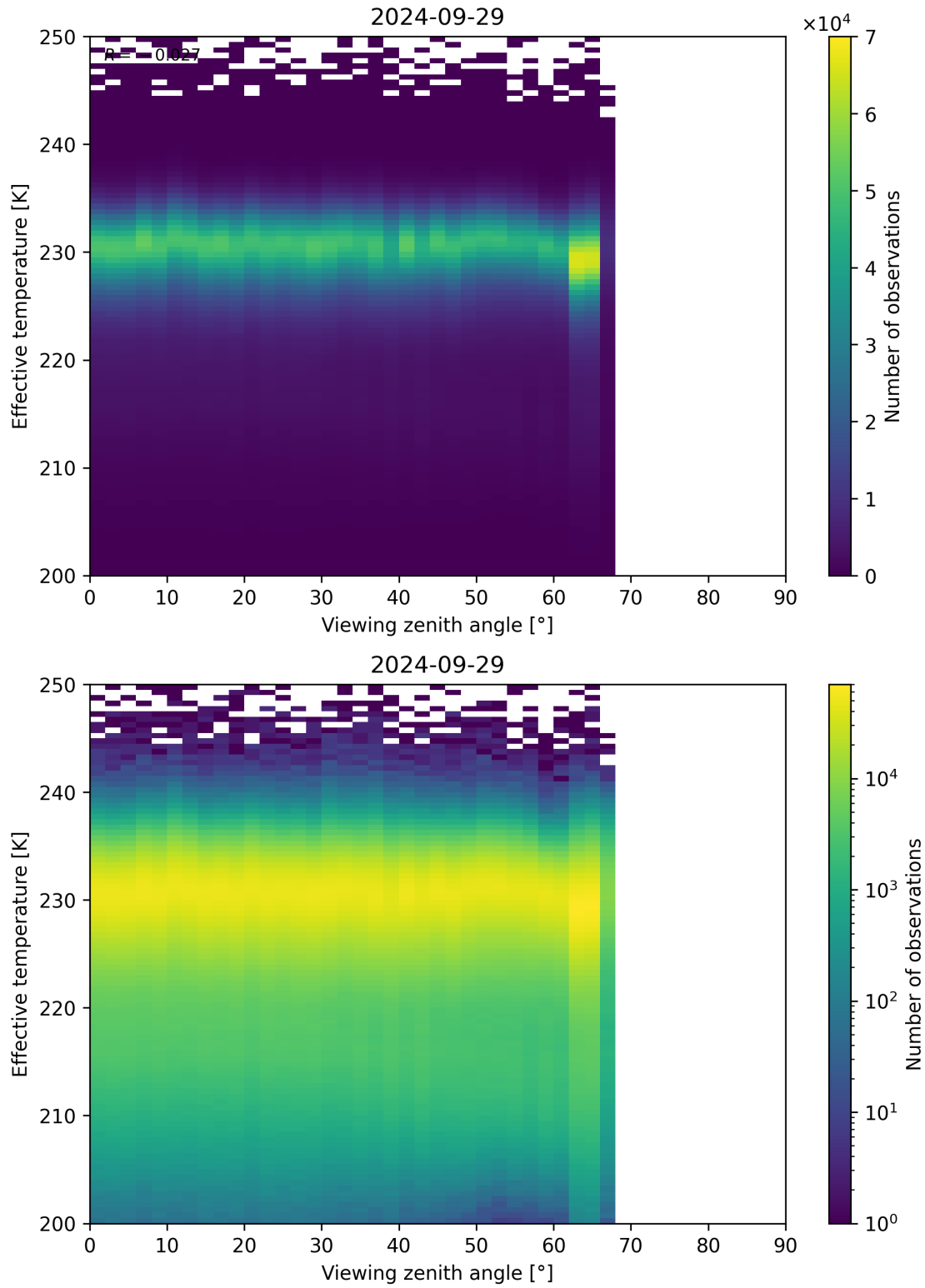
Figure 50: Scatter density plot of “Viewing zenith angle” against “Effective temperature” for 2024-09-28 to 2024-09-30.
