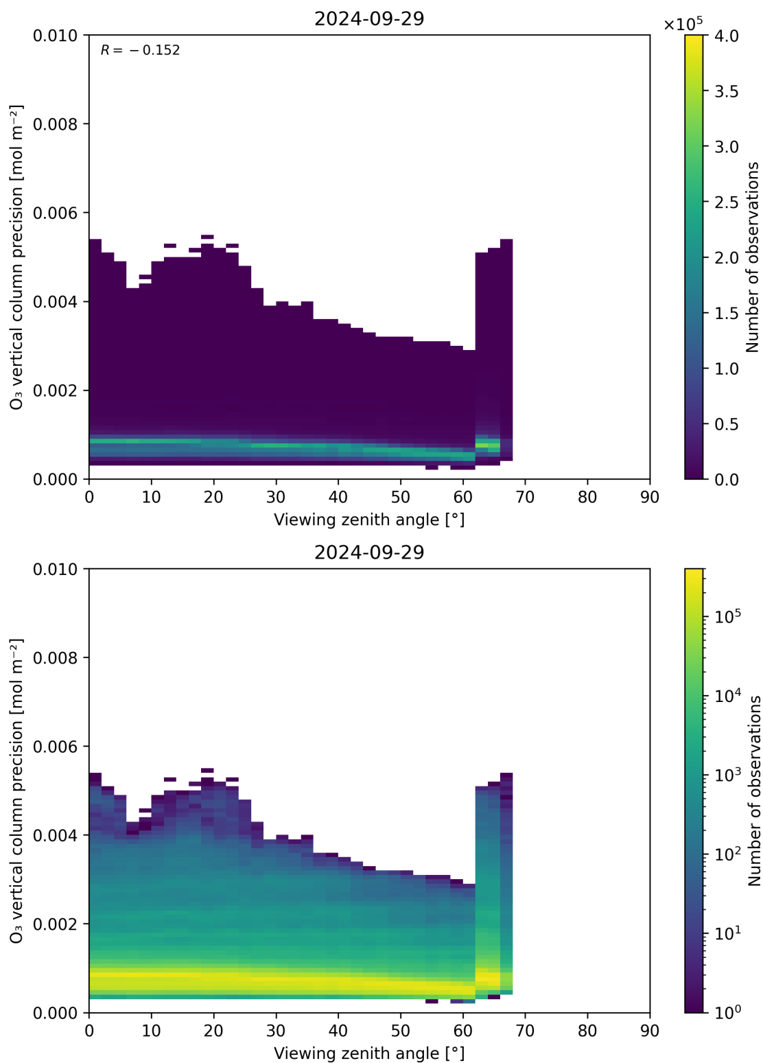
Figure 53: Scatter density plot of “Viewing zenith angle” against “O 3 vertical column precision” for 2024-09-28 to 2024-09-30.
