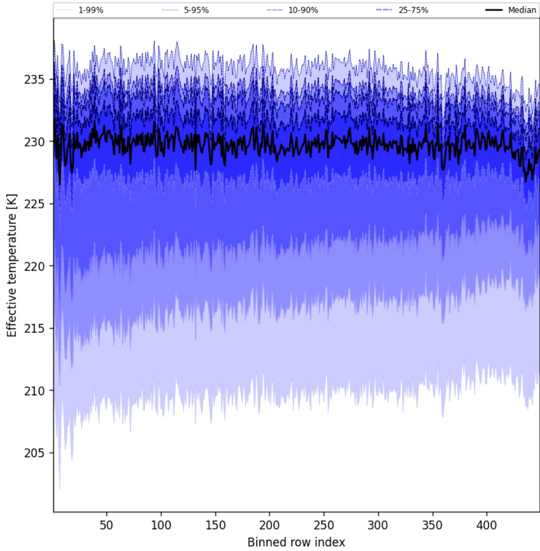
Figure 31: Along track statistics of “Effective temperature” for 2024-09-28 to 2024-09-30
