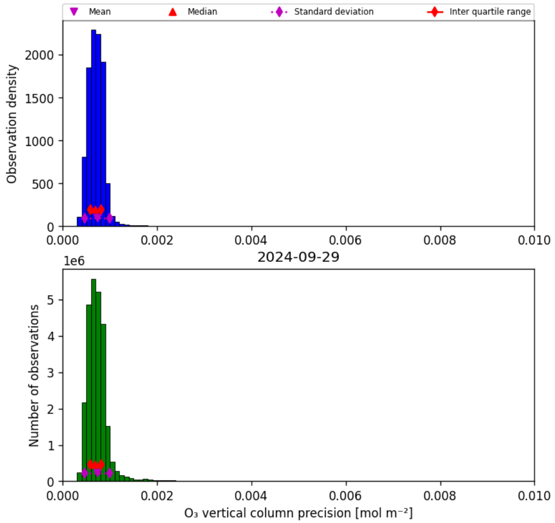
Figure 22: Histogram of "O 3 vertical column precision" for 2024-09-28 to 2024-09-30
