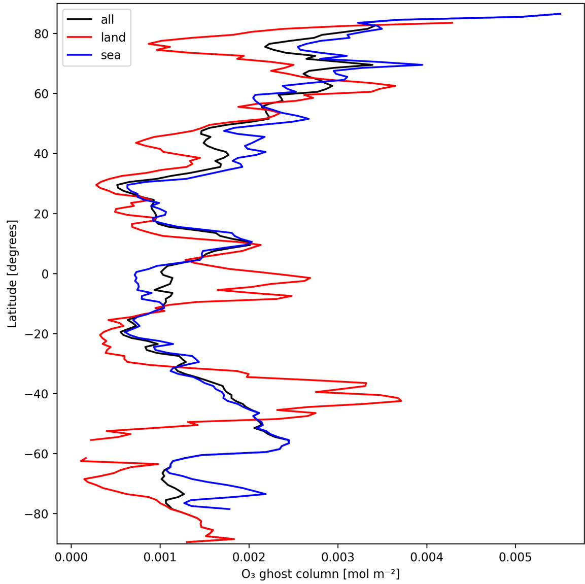
Figure 18: Zonal average of “O 3 ghost column” for 2024-09-28 to 2024-09-30.
