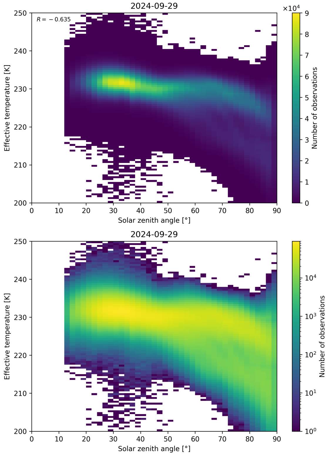
Figure 45: Scatter density plot of “Solar zenith angle” against “Effective temperature” for 2024-09-28 to 2024-09-30.
