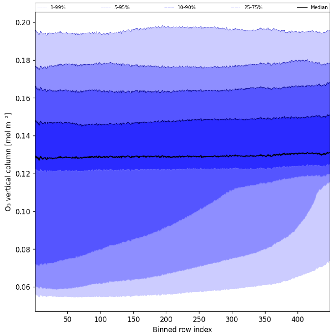
Figure 28: Along track statistics of “O 3 vertical column” for 2024-09-28 to 2024-09-30
