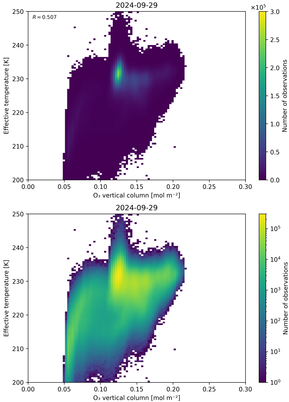
Figure 39: Scatter density plot of “O 3 vertical column” against “Effective temperature” for 2024-09-28 to 2024-09-30.
