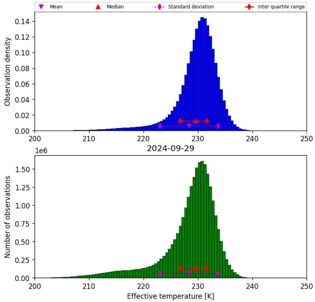
Figure 24: Histogram of “Effective temperature” for 2024-09-28 to 2024-09-30
