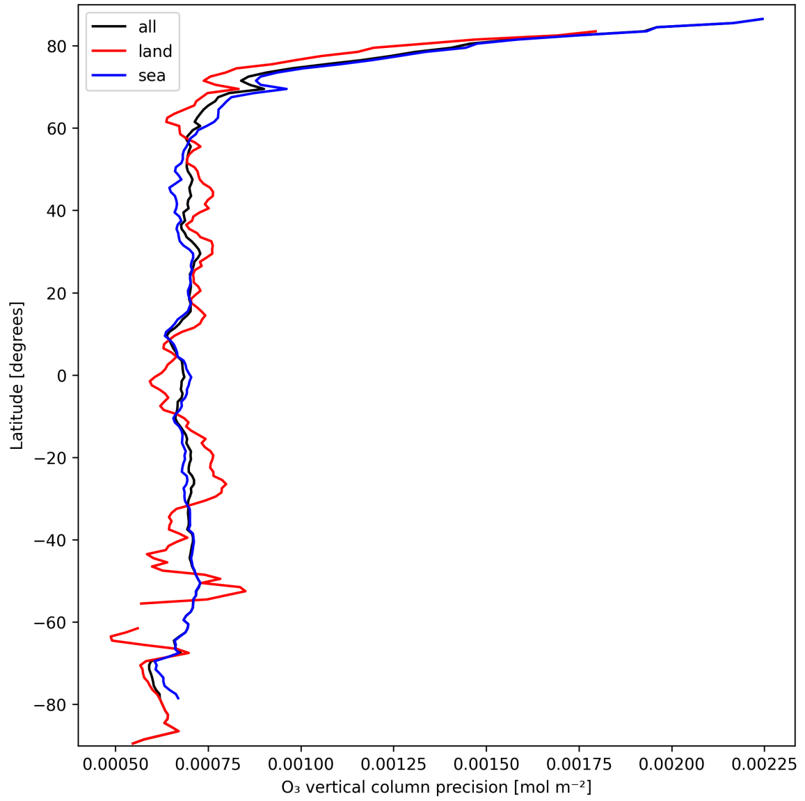
Figure 15: Zonal average of "O 3 vertical column precision" for 2024-09-28 to 2024-09-30.
