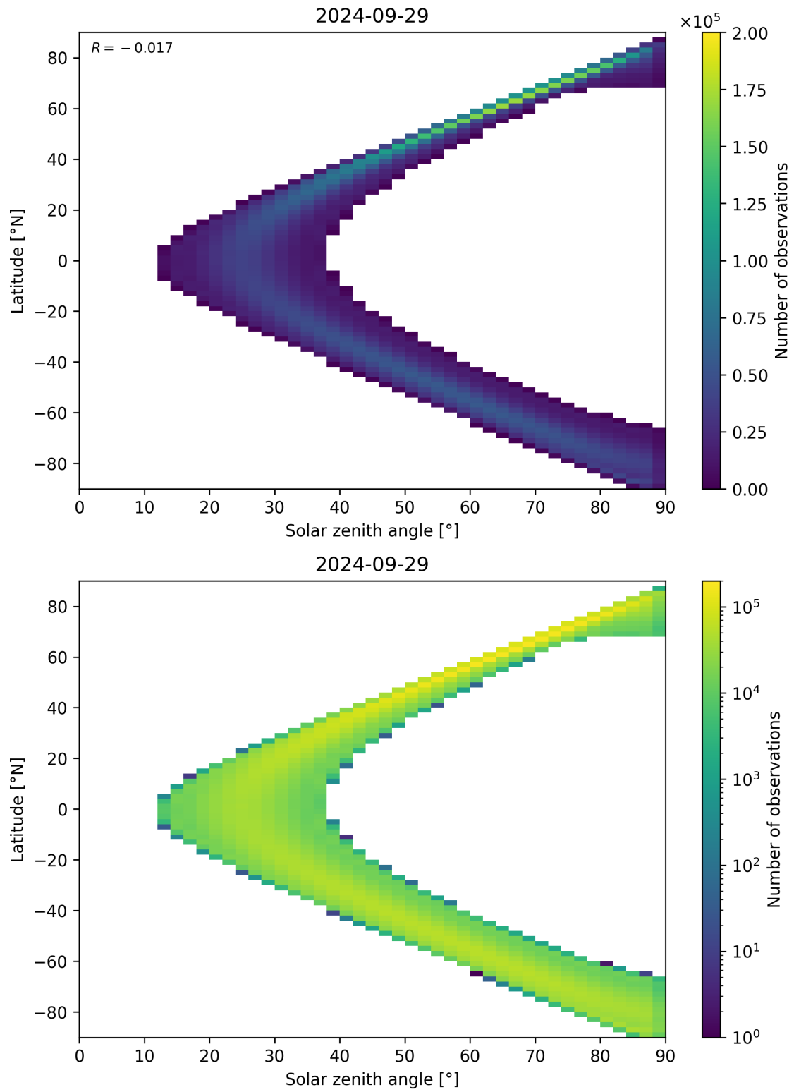
Figure 44: Scatter density plot of “Solar zenith angle” against “Latitude” for 2024-09-28 to 2024-09-30.
