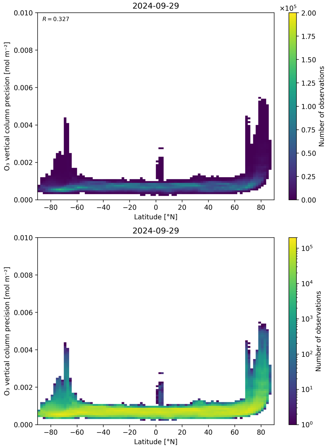
Figure 37: Scatter density plot of “Latitude” against “O 3 vertical column precision” for 2024-09-28 to 2024-09-30.
