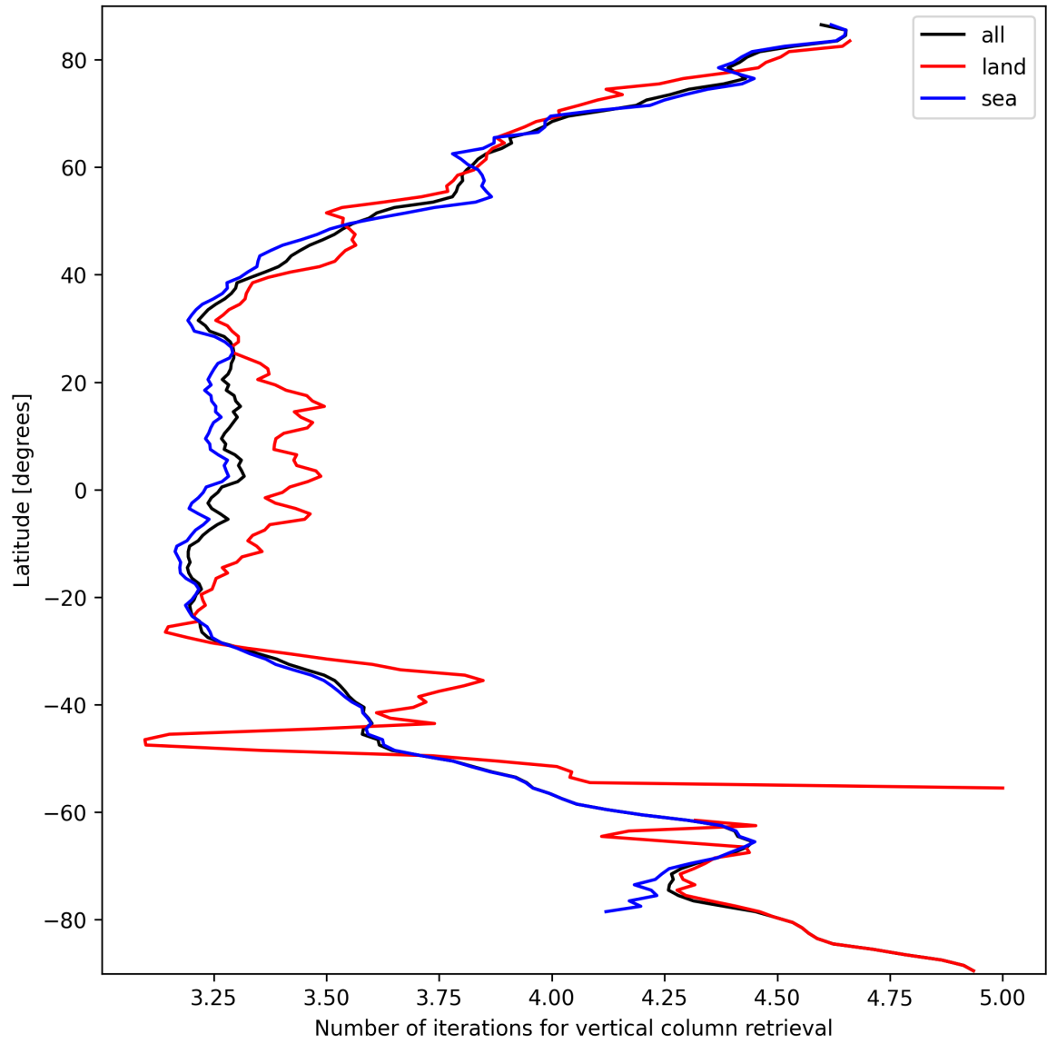
Figure 19: Zonal average of “Number of iterations for vertical column retrieval” for 2024-09-28 to 2024-09-30.
