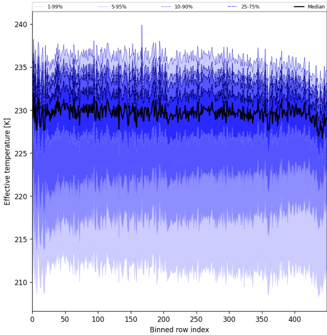
Figure 31: Along track statistics of “Effective temperature” for 2024-09-29 to 2024-10-01
