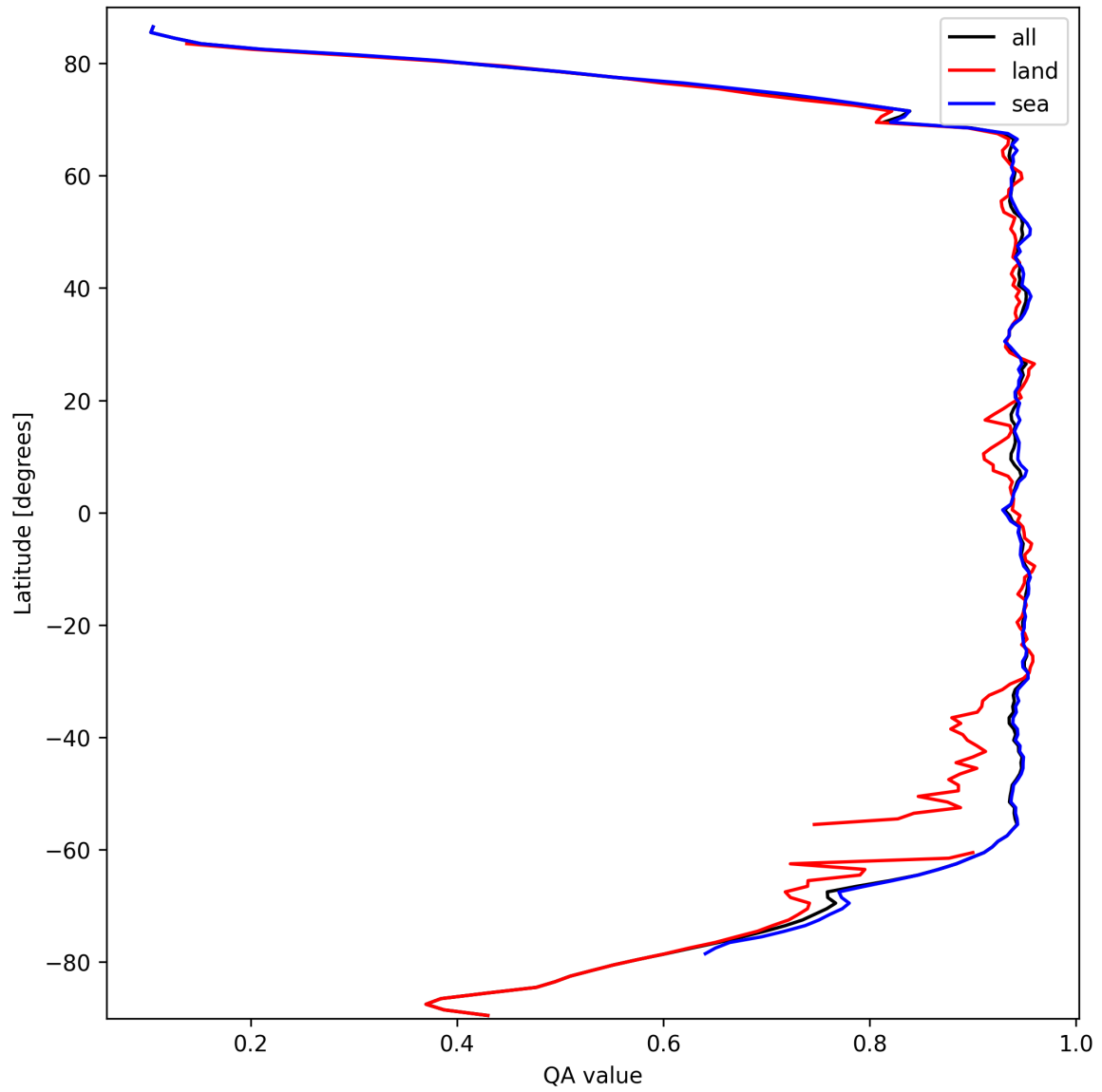
Figure 13: Zonal average of “QA value” for 2024-09-29 to 2024-10-01.
