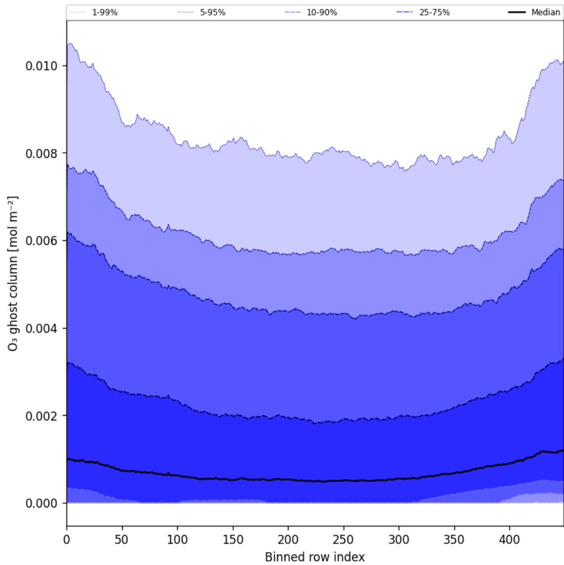
Figure 32: Along track statistics of “O 3 ghost column” for 2024-09-29 to 2024-10-01
