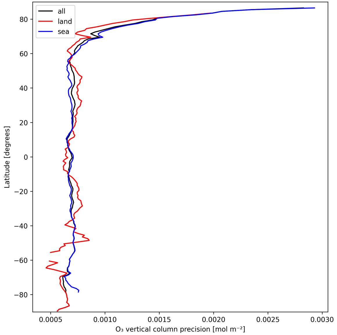
Figure 15: Zonal average of “O 3 vertical column precision” for 2024-09-29 to 2024-10-01.
