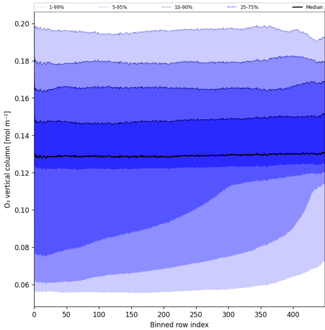
Figure 28: Along track statistics of “O 3 vertical column” for 2024-09-29 to 2024-10-01
