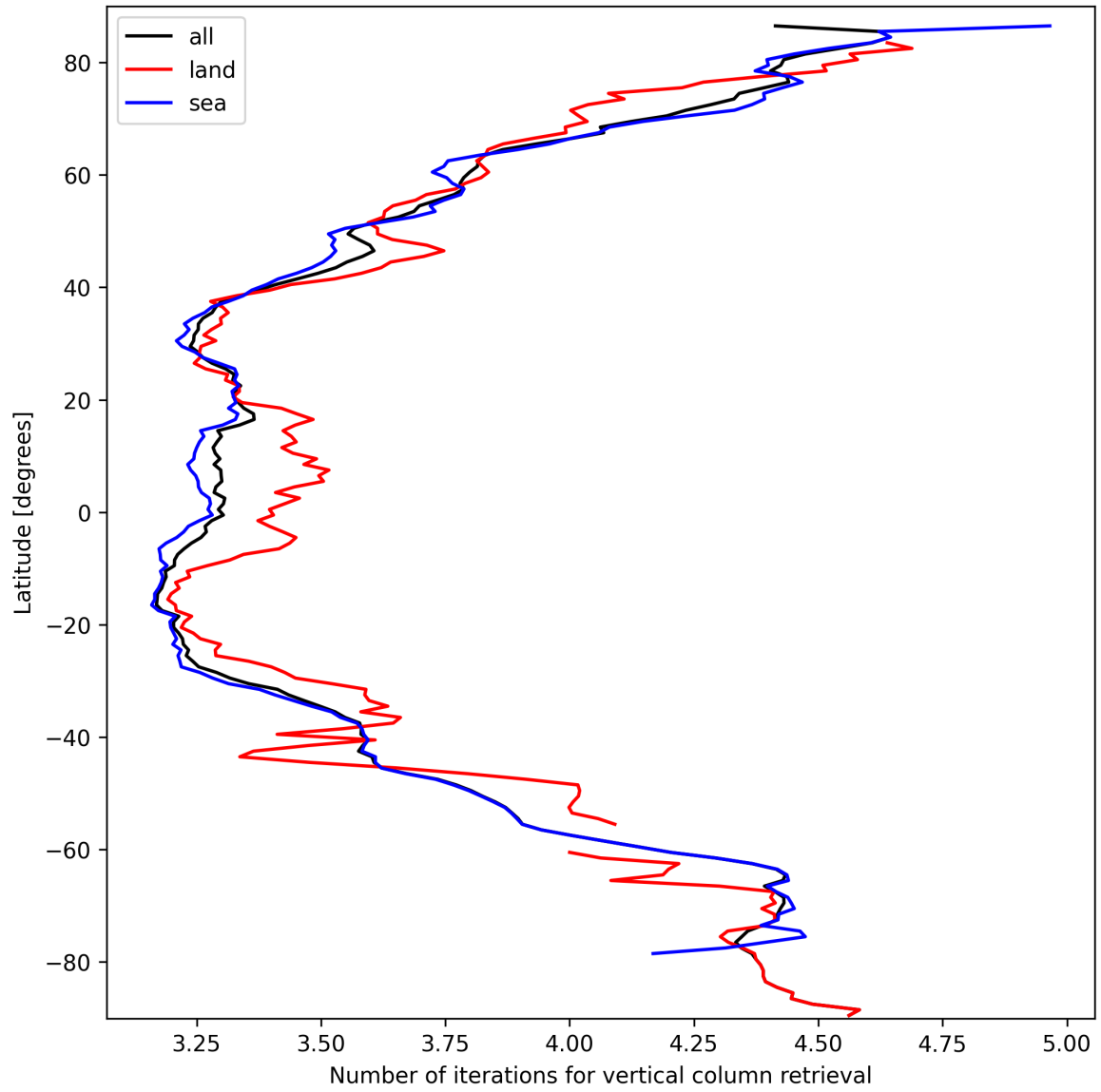
Figure 19: Zonal average of “Number of iterations for vertical column retrieval” for 2024-09-29 to 2024-10-01.
