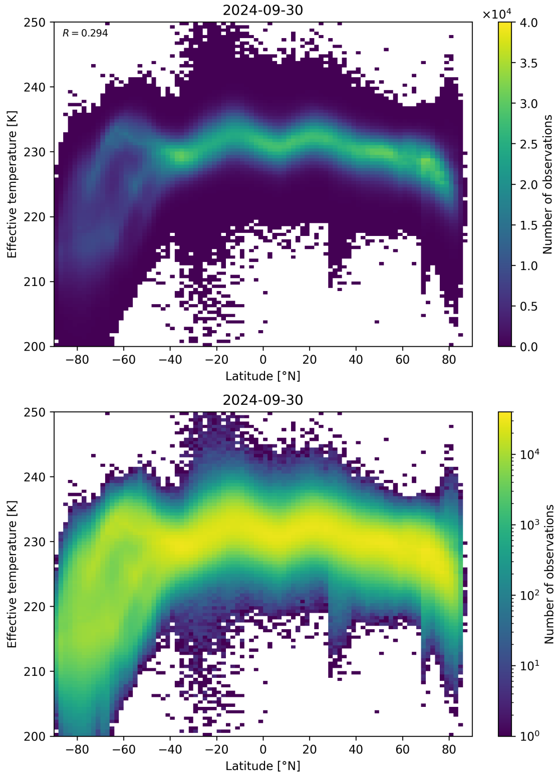
Figure 34: Scatter density plot of “Latitude” against “Effective temperature” for 2024-09-29 to 2024-10-01.
