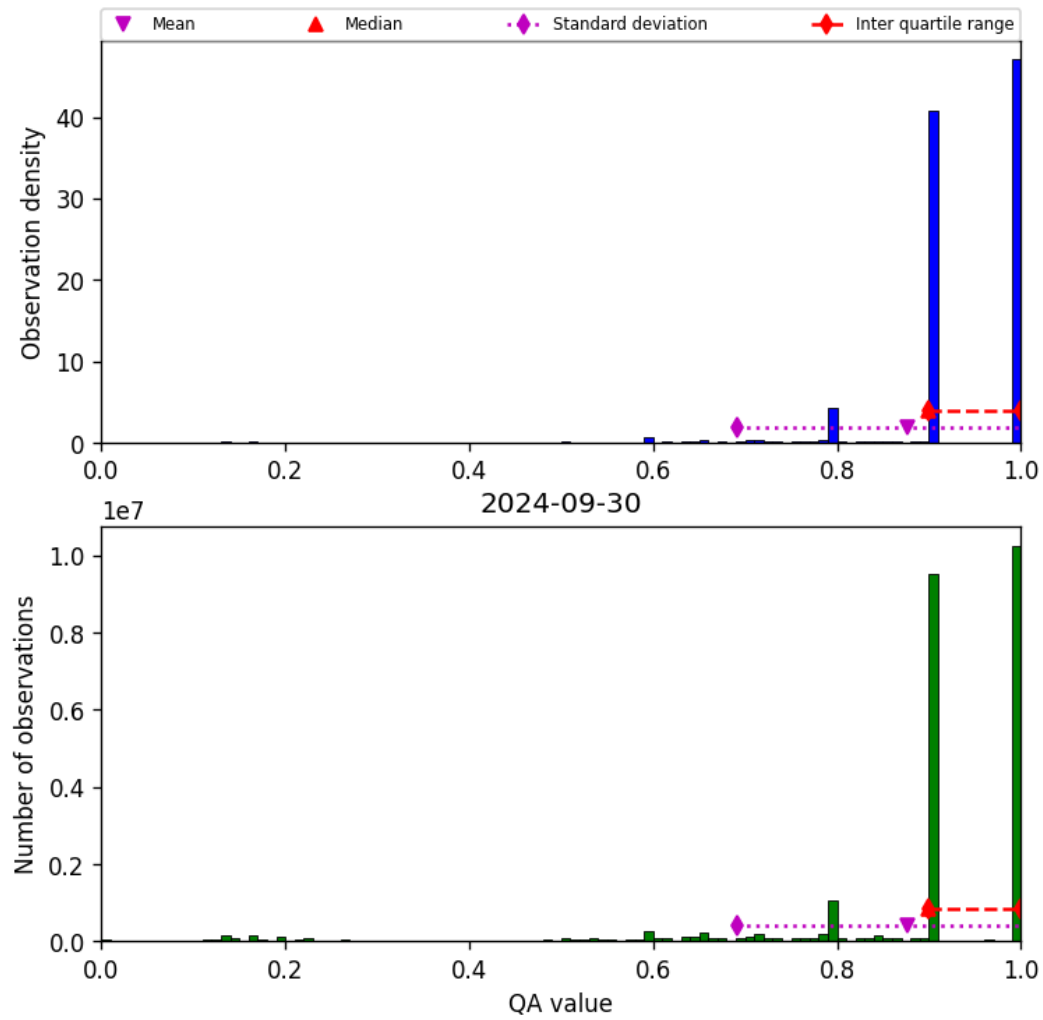
Figure 20: Histogram of “QA value” for 2024-09-29 to 2024-10-01
