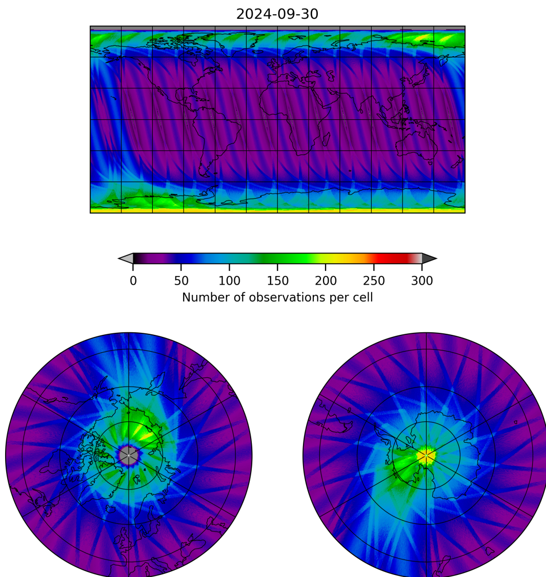
Figure 12: Map of the number of observations for 2024-09-29 to 2024-10-01
