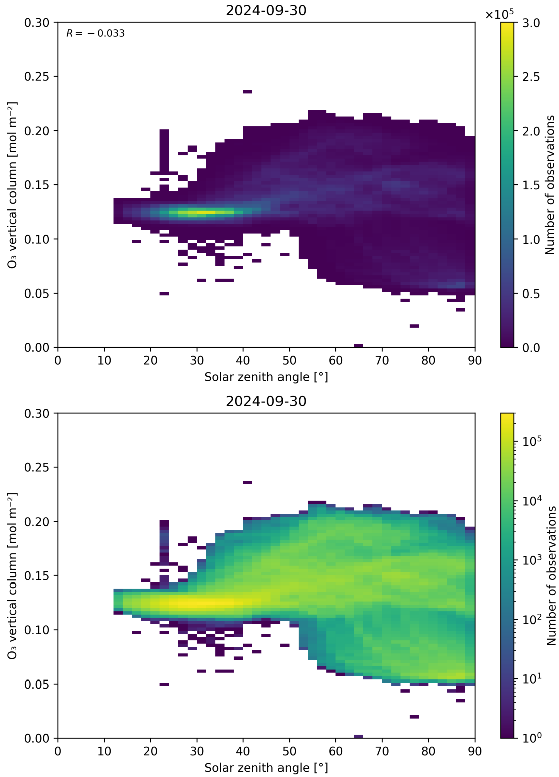
Figure 47: Scatter density plot of “Solar zenith angle” against “O 3 vertical column” for 2024-09-29 to 2024-10-01.
