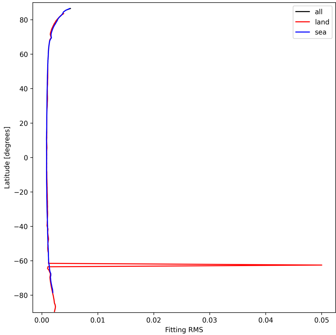
Figure 16: Zonal average of “Fitting RMS” for 2024-09-29 to 2024-10-01.
