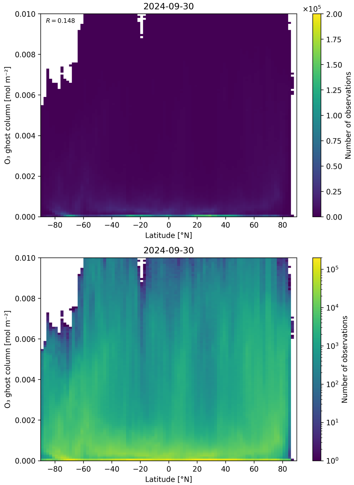
Figure 35: Scatter density plot of “Latitude” against “O 3 ghost column” for 2024-09-29 to 2024-10-01.
