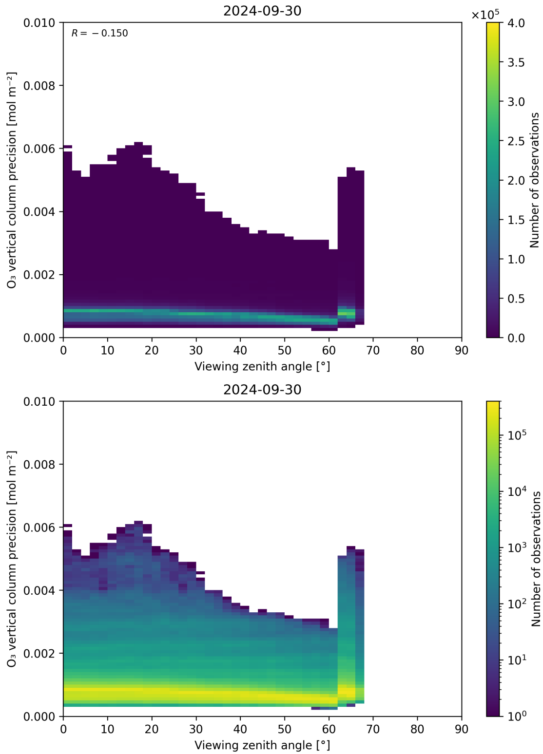
Figure 53: Scatter density plot of “Viewing zenith angle” against “O 3 vertical column precision” for 2024-09-29 to 2024-10-01.
