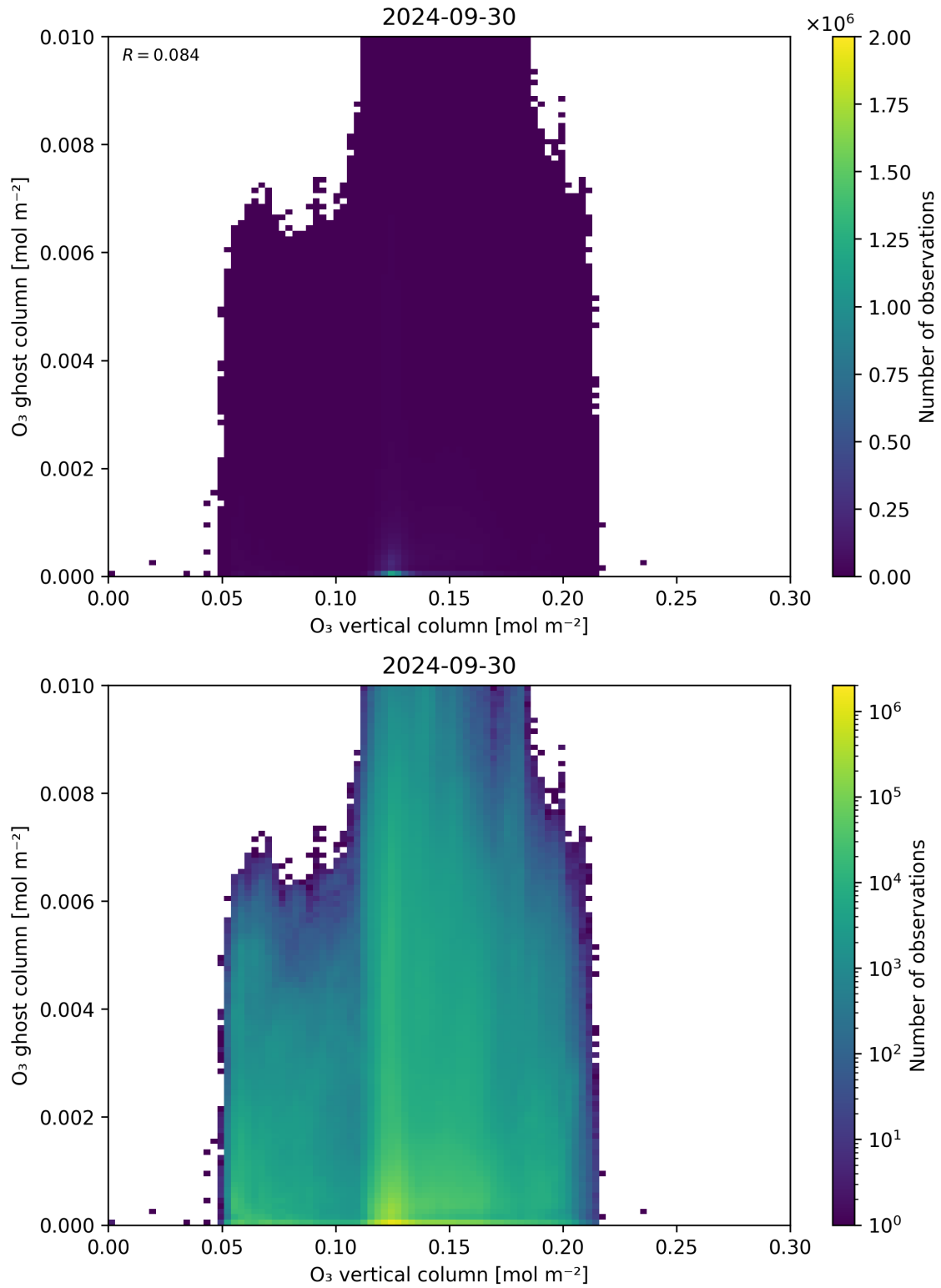
Figure 40: Scatter density plot of “O 3 vertical column” against “O 3 ghost column” for 2024-09-29 to 2024-10-01.
