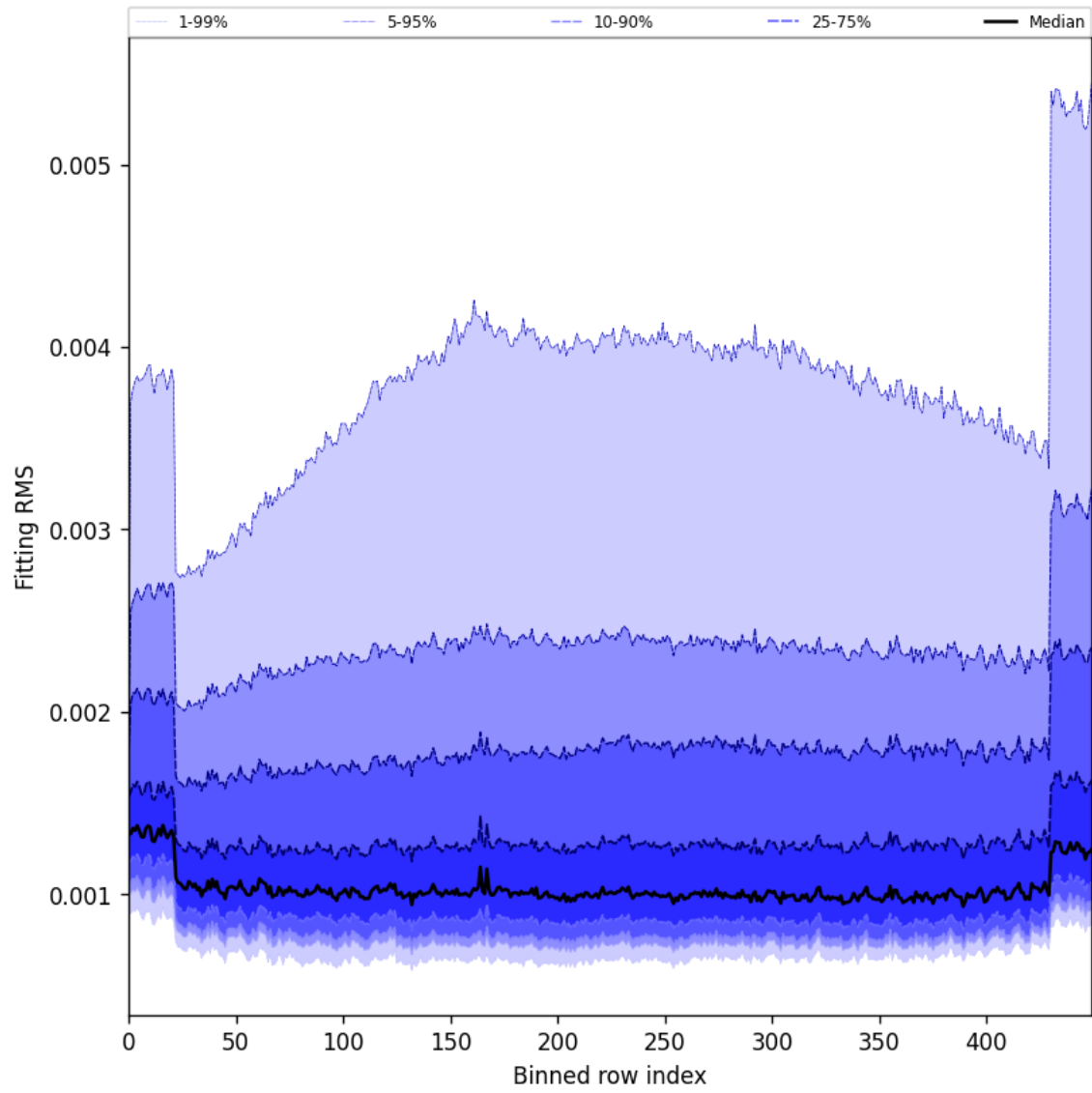
Figure 30: Along track statistics of “Fitting RMS” for 2024-09-29 to 2024-10-01
