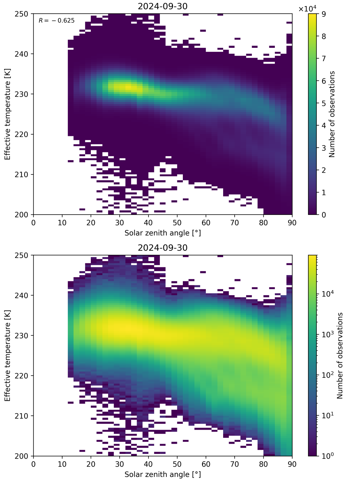
Figure 45: Scatter density plot of “Solar zenith angle” against “Effective temperature” for 2024-09-29 to 2024-10-01.
