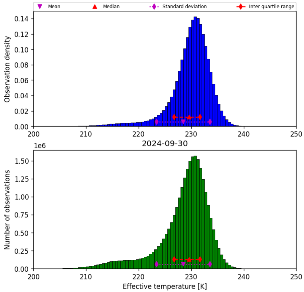
Figure 24: Histogram of “Effective temperature” for 2024-09-29 to 2024-10-01
