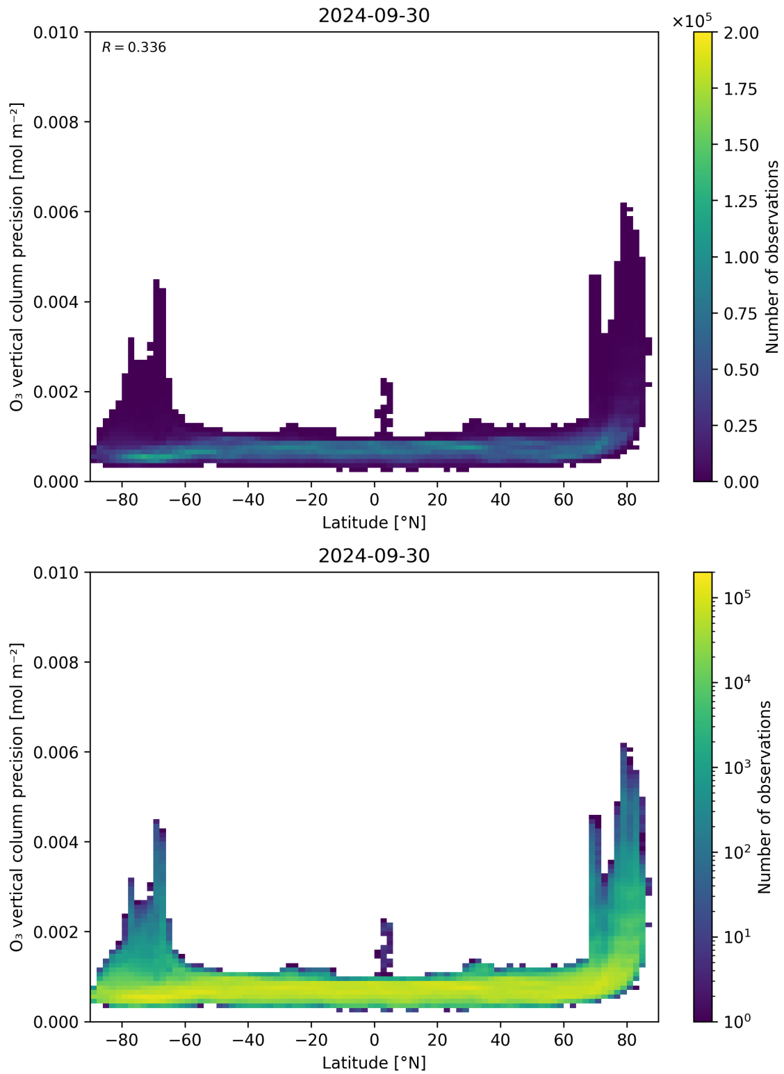
Figure 37: Scatter density plot of “Latitude” against “O 3 vertical column precision” for 2024-09-29 to 2024-10-01.
