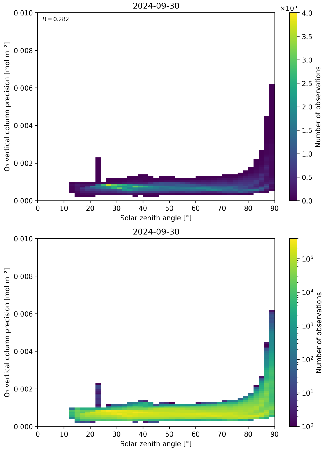
Figure 48: Scatter density plot of “Solar zenith angle” against “O 3 vertical column precision” for 2024-09-29 to 2024-10-01.
