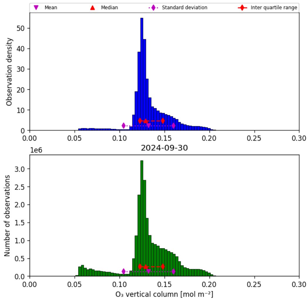
Figure 21: Histogram of “O 3 vertical column” for 2024-09-29 to 2024-10-01
