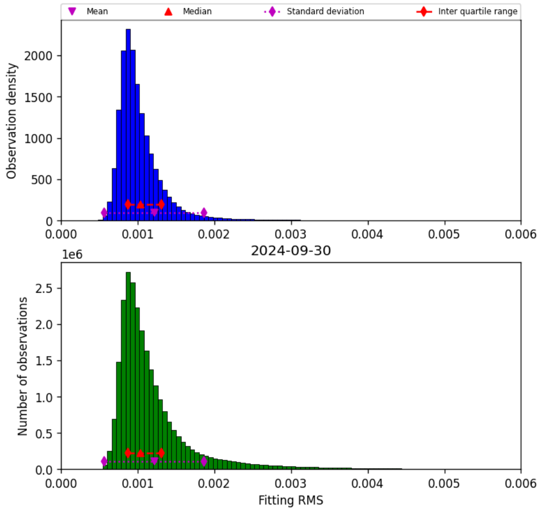
Figure 23: Histogram of “Fitting RMS” for 2024-09-29 to 2024-10-01
