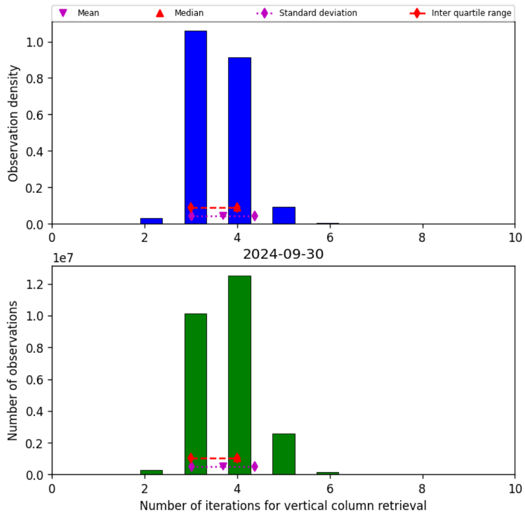
Figure 26: Histogram of “Number of iterations for vertical column retrieval” for 2024-09-29 to 2024-10-01
