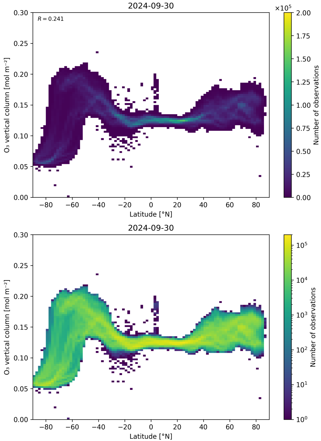
Figure 36: Scatter density plot of “Latitude” against “O 3 vertical column” for 2024-09-29 to 2024-10-01.
