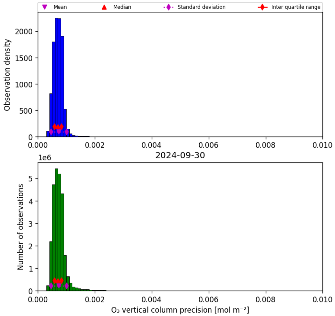
Figure 22: Histogram of “O 3 vertical column precision” for 2024-09-29 to 2024-10-01
