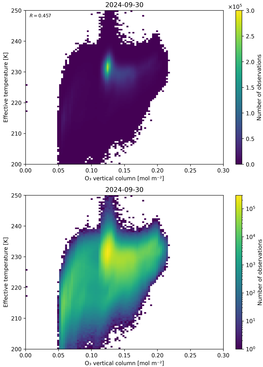
Figure 39: Scatter density plot of “O 3 vertical column” against “Effective temperature” for 2024-09-29 to 2024-10-01.
