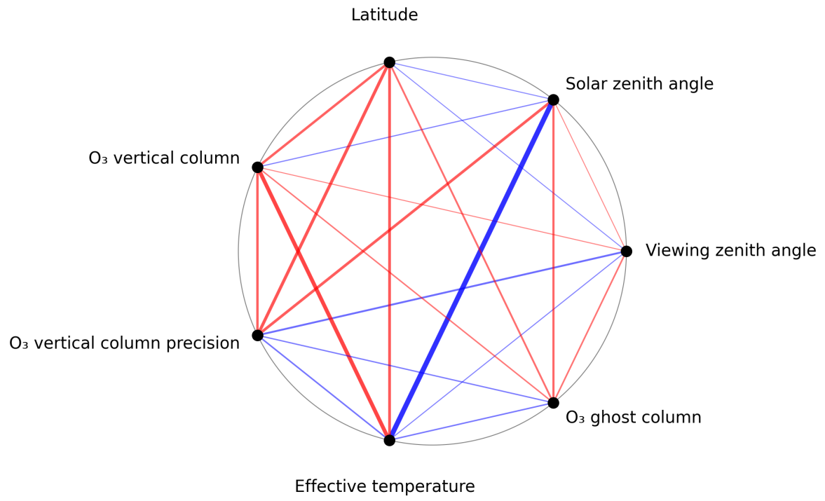
Figure 1: Map of correlation graph for 2024-09-29 to 2024-10-01.
