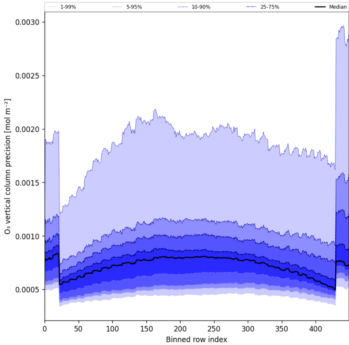
Figure 29: Along track statistics of “O 3 vertical column precision” for 2024-09-29 to 2024-10-01
