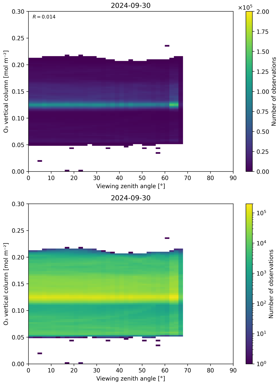
Figure 52: Scatter density plot of “Viewing zenith angle” against “O 3 vertical column” for 2024-09-29 to 2024-10-01.
