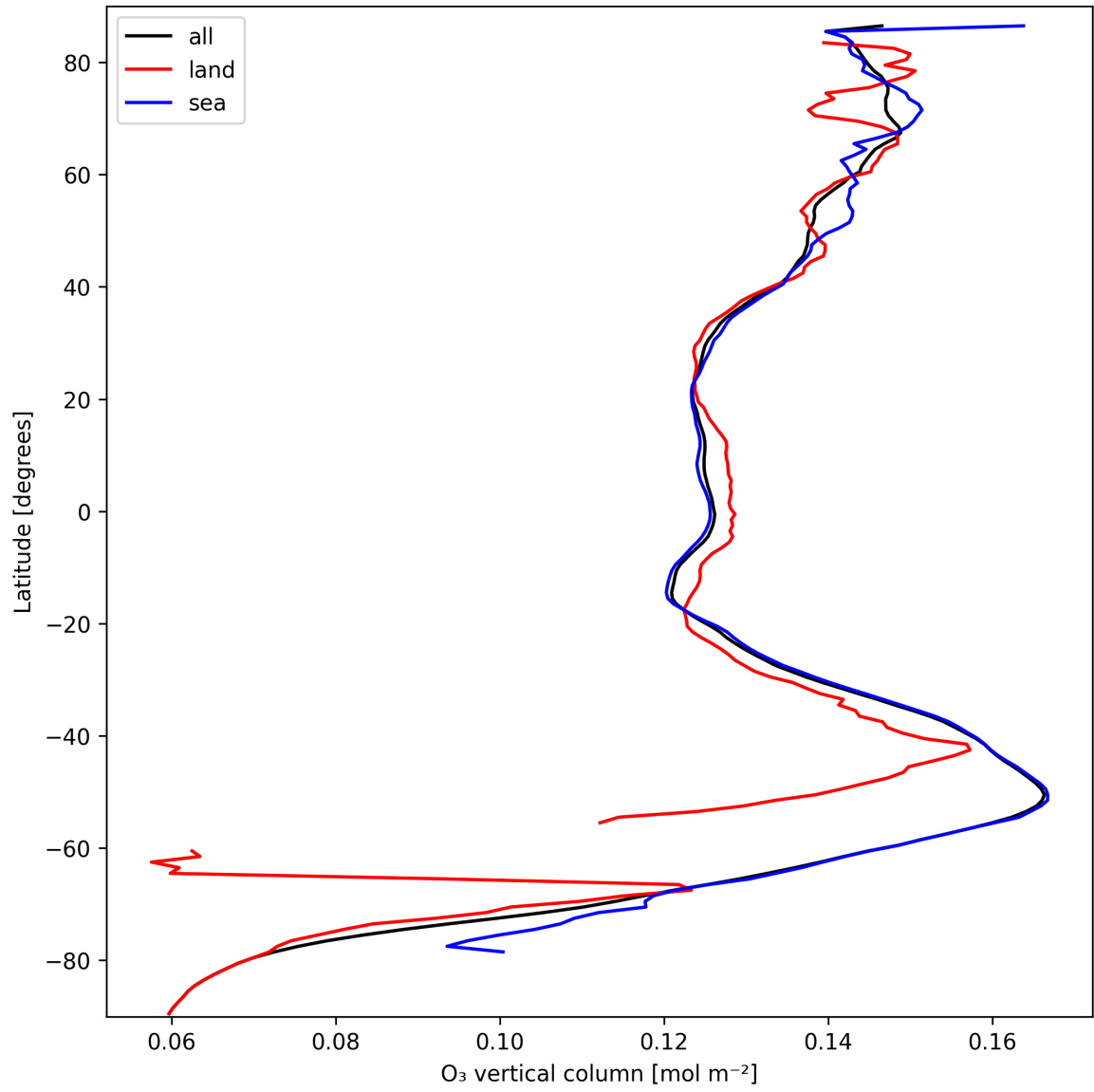
Figure 14: Zonal average of “O 3 vertical column” for 2024-09-29 to 2024-10-01.
