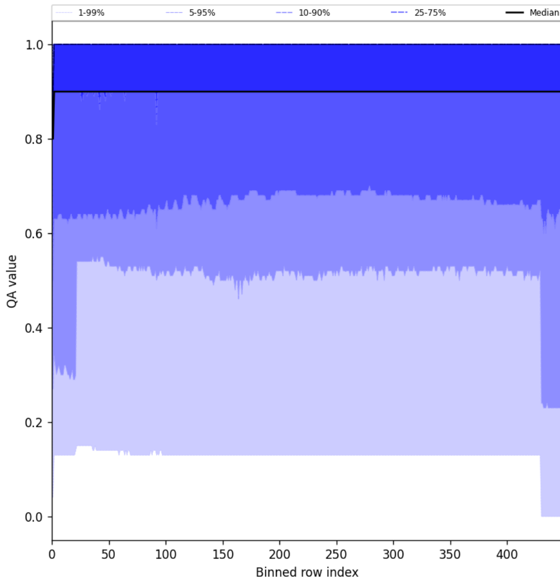
Figure 27: Along track statistics of “QA value” for 2024-09-29 to 2024-10-01
