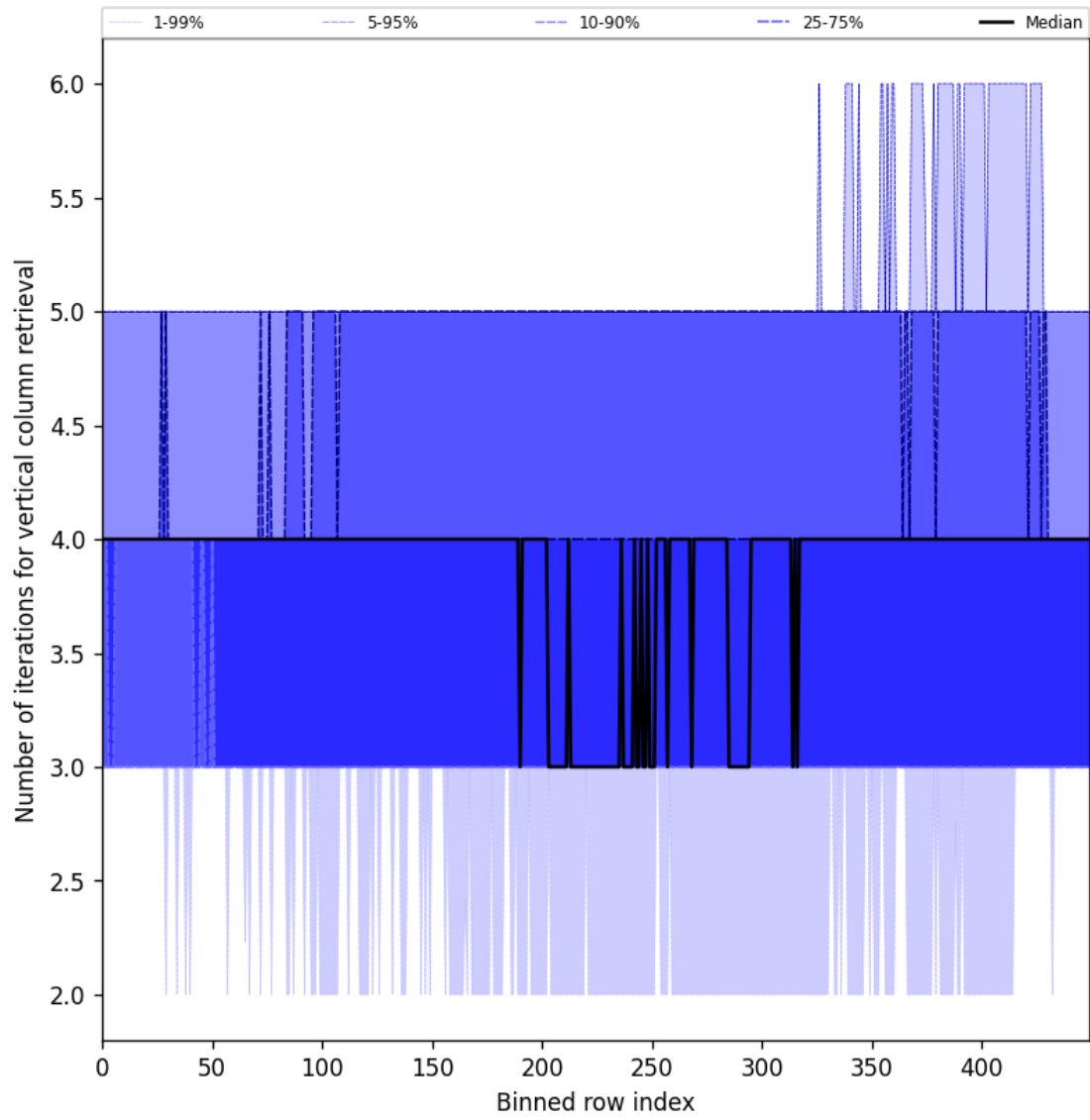
Figure 33: Along track statistics of “Number of iterations for vertical column retrieval” for 2024-09-29 to 2024-10-01
