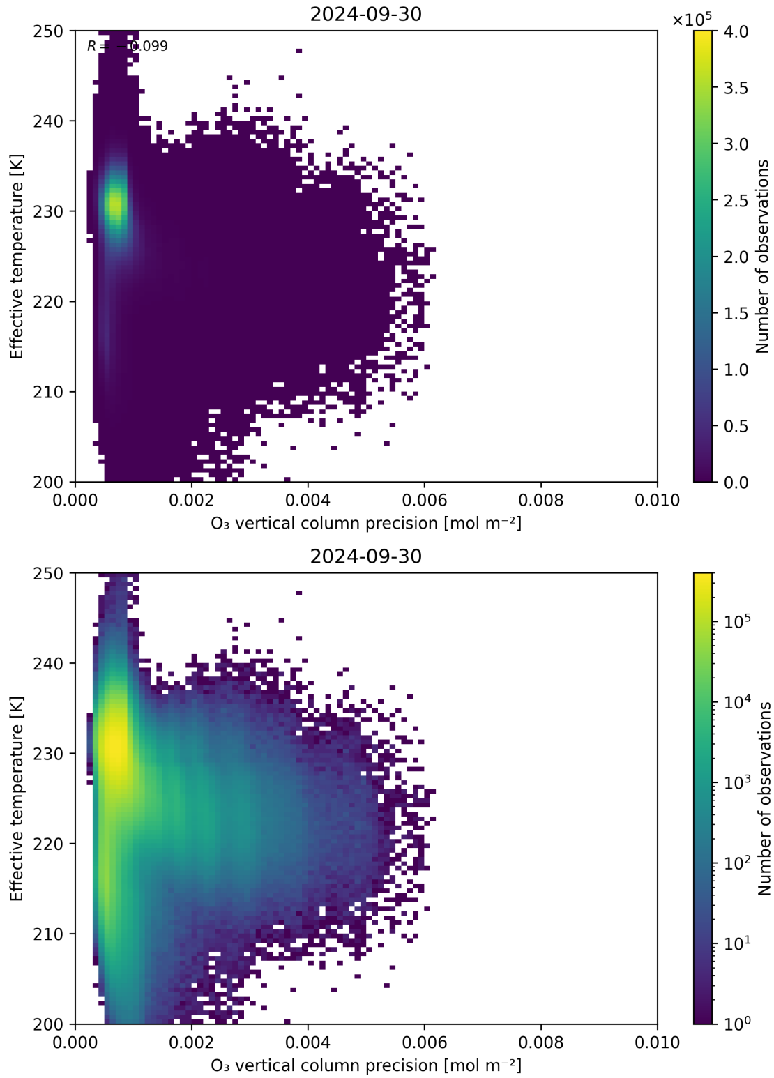
Figure 42: Scatter density plot of “O 3 vertical column precision” against “Effective temperature” for 2024-09-29 to 2024-10-01.
