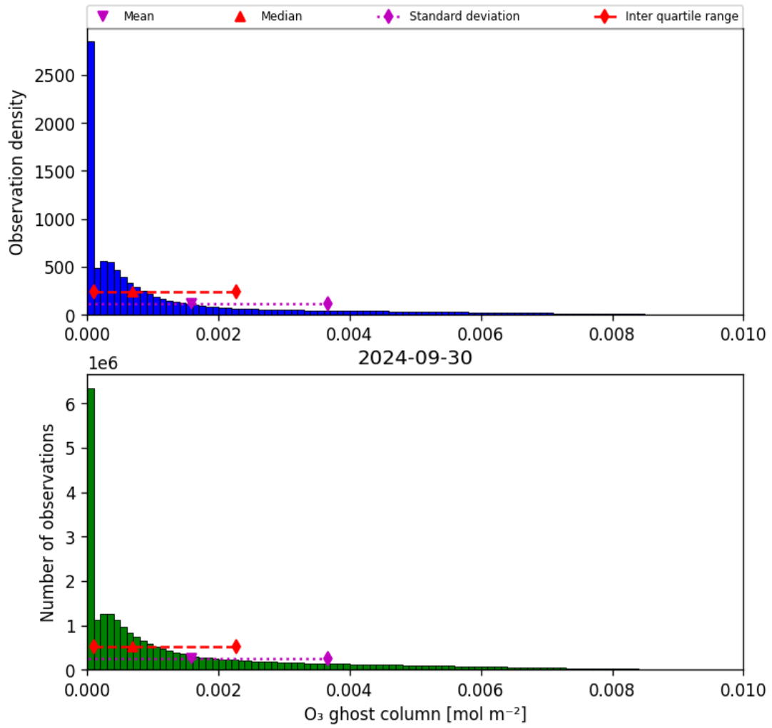
Figure 25: Histogram of “O 3 ghost column” for 2024-09-29 to 2024-10-01
