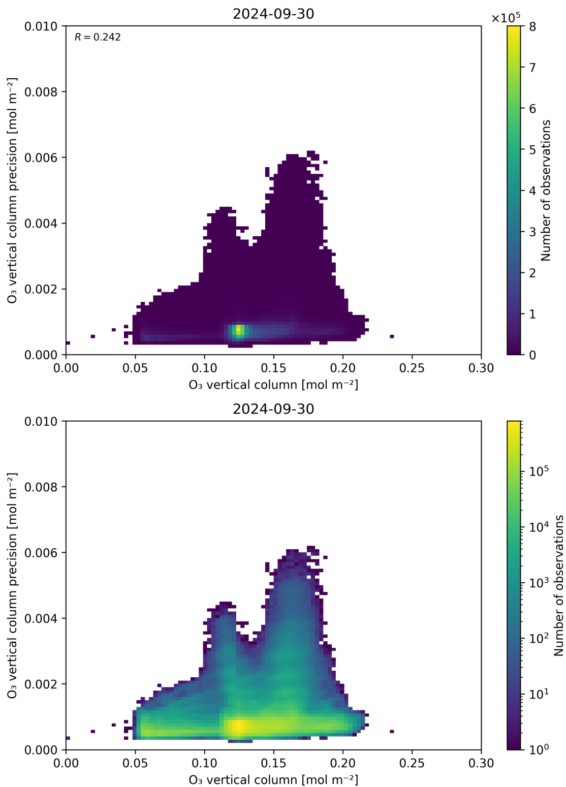
Figure 41: Scatter density plot of “O 3 vertical column” against “O 3 vertical column precision” for 2024-09-29 to 2024-10-01.
