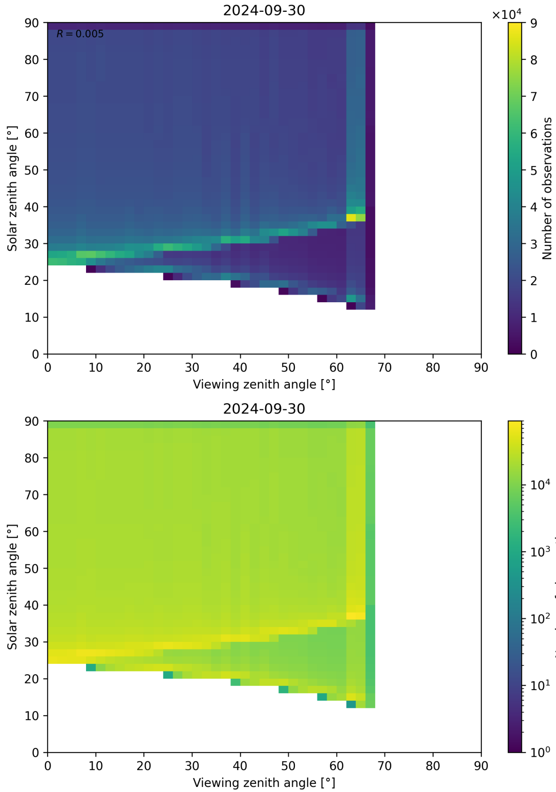
Figure 54: Scatter density plot of “Viewing zenith angle” against “Solar zenith angle” for 2024-09-29 to 2024-10-01.
