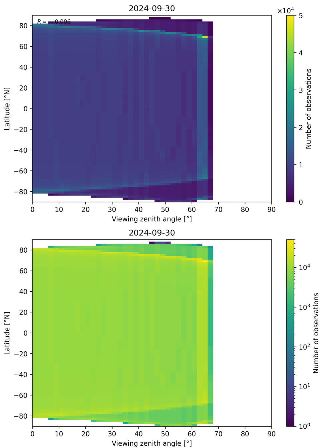
Figure 49: Scatter density plot of “Viewing zenith angle” against “Latitude” for 2024-09-29 to 2024-10-01.
