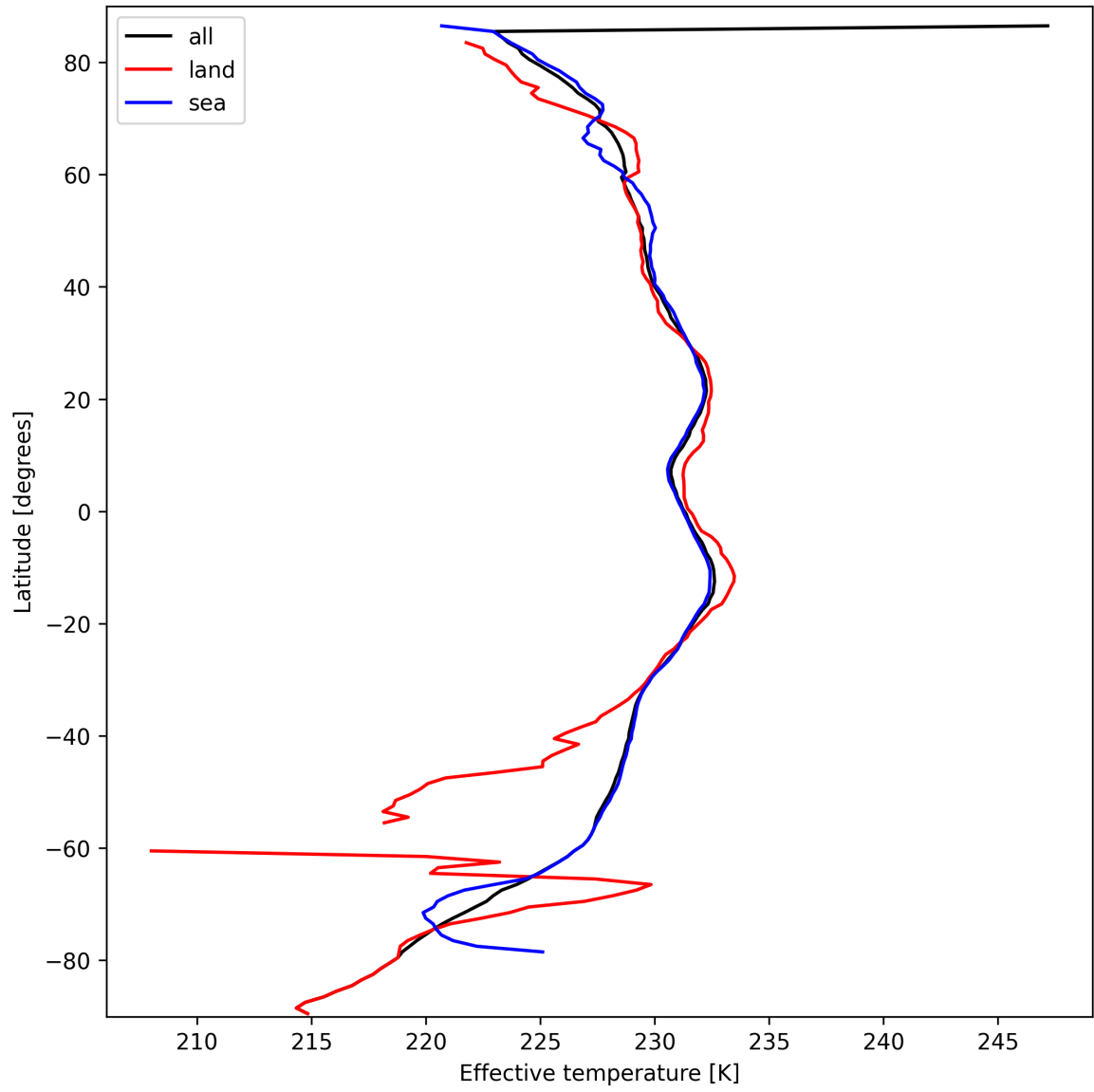
Figure 17: Zonal average of “Effective temperature” for 2024-09-29 to 2024-10-01.
