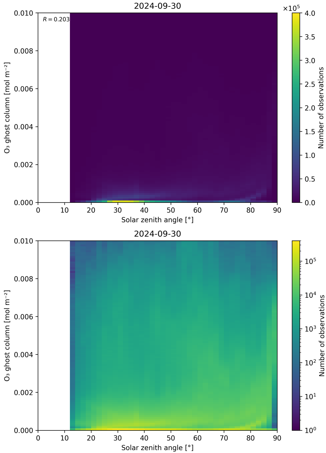
Figure 46: Scatter density plot of “Solar zenith angle” against “O 3 ghost column” for 2024-09-29 to 2024-10-01.
