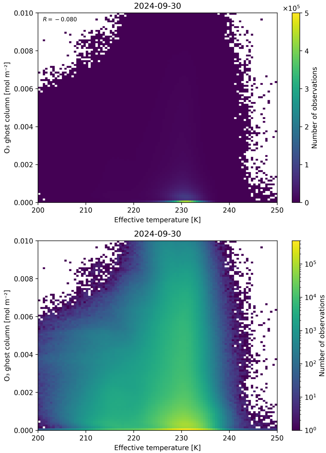
Figure 38: Scatter density plot of “Effective temperature” against “O 3 ghost column” for 2024-09-29 to 2024-10-01.
