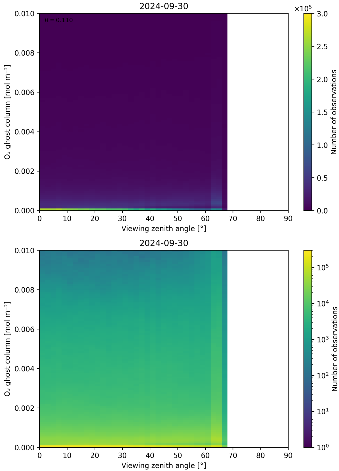
Figure 51: Scatter density plot of “Viewing zenith angle” against “O 3 ghost column” for 2024-09-29 to 2024-10-01.
