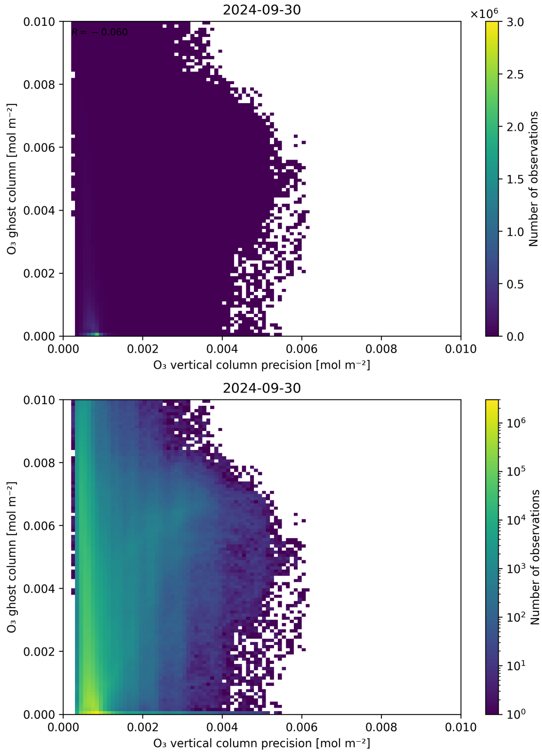
Figure 43: Scatter density plot of “ \text{O}_3 vertical column precision” against “ \text{O}_3 ghost column” for 2024-09-29 to 2024-10-01.
