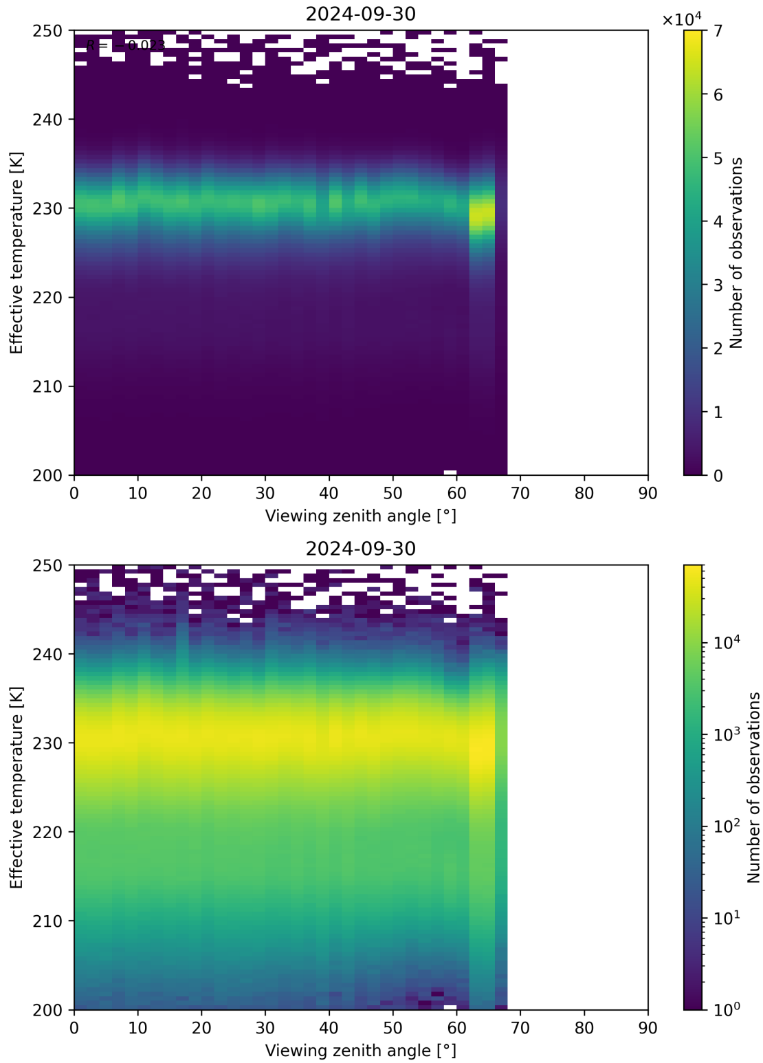
Figure 50: Scatter density plot of “Viewing zenith angle” against “Effective temperature” for 2024-09-29 to 2024-10-01.
