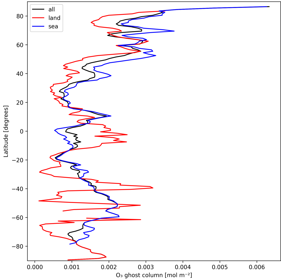
Figure 18: Zonal average of “O 3 ghost column” for 2024-09-29 to 2024-10-01.
