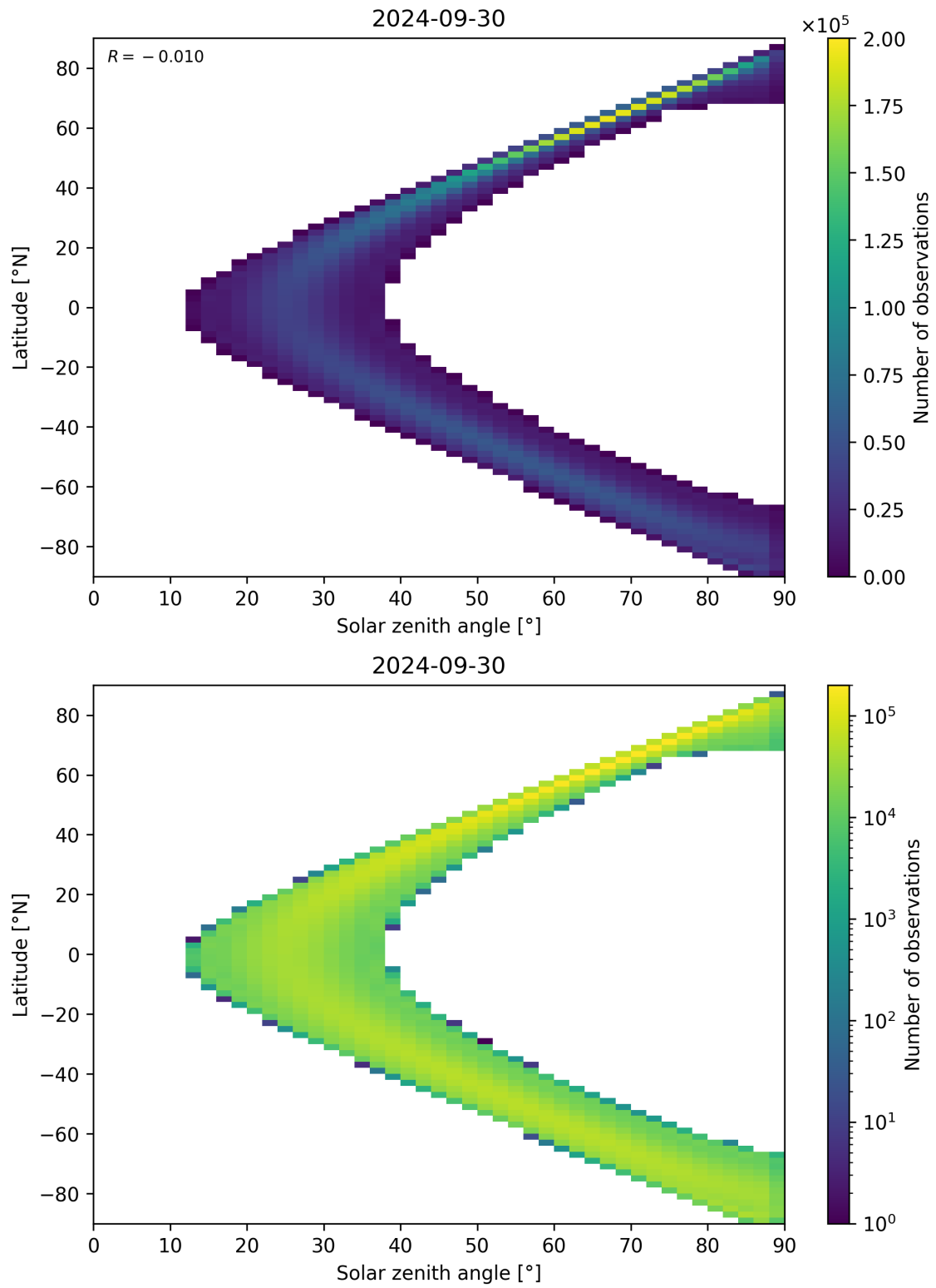
Figure 44: Scatter density plot of “Solar zenith angle” against “Latitude” for 2024-09-29 to 2024-10-01.
