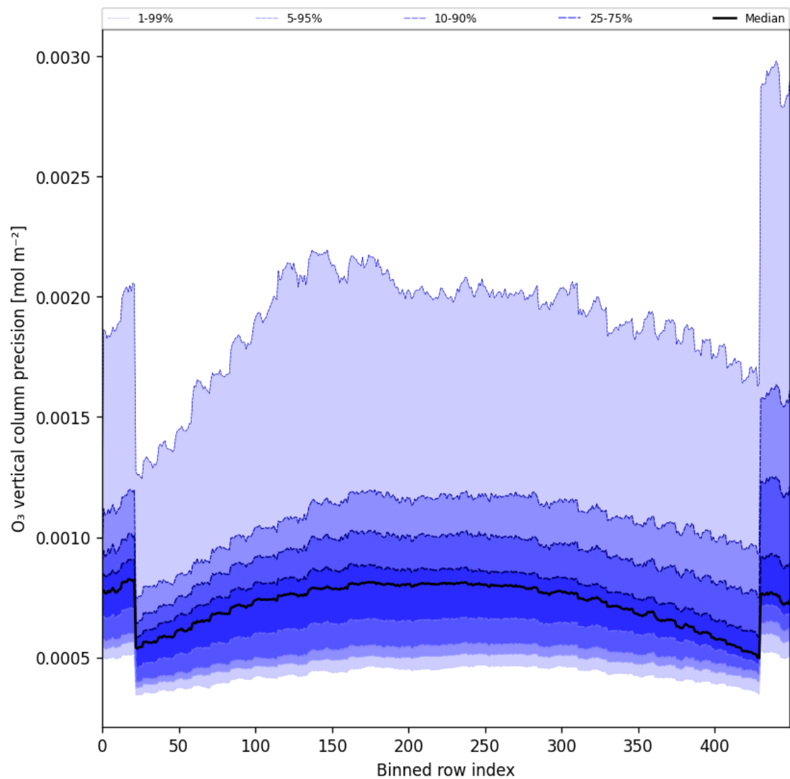
Figure 29: Along track statistics of “O 3 vertical column precision” for 2024-09-30 to 2024-10-02
