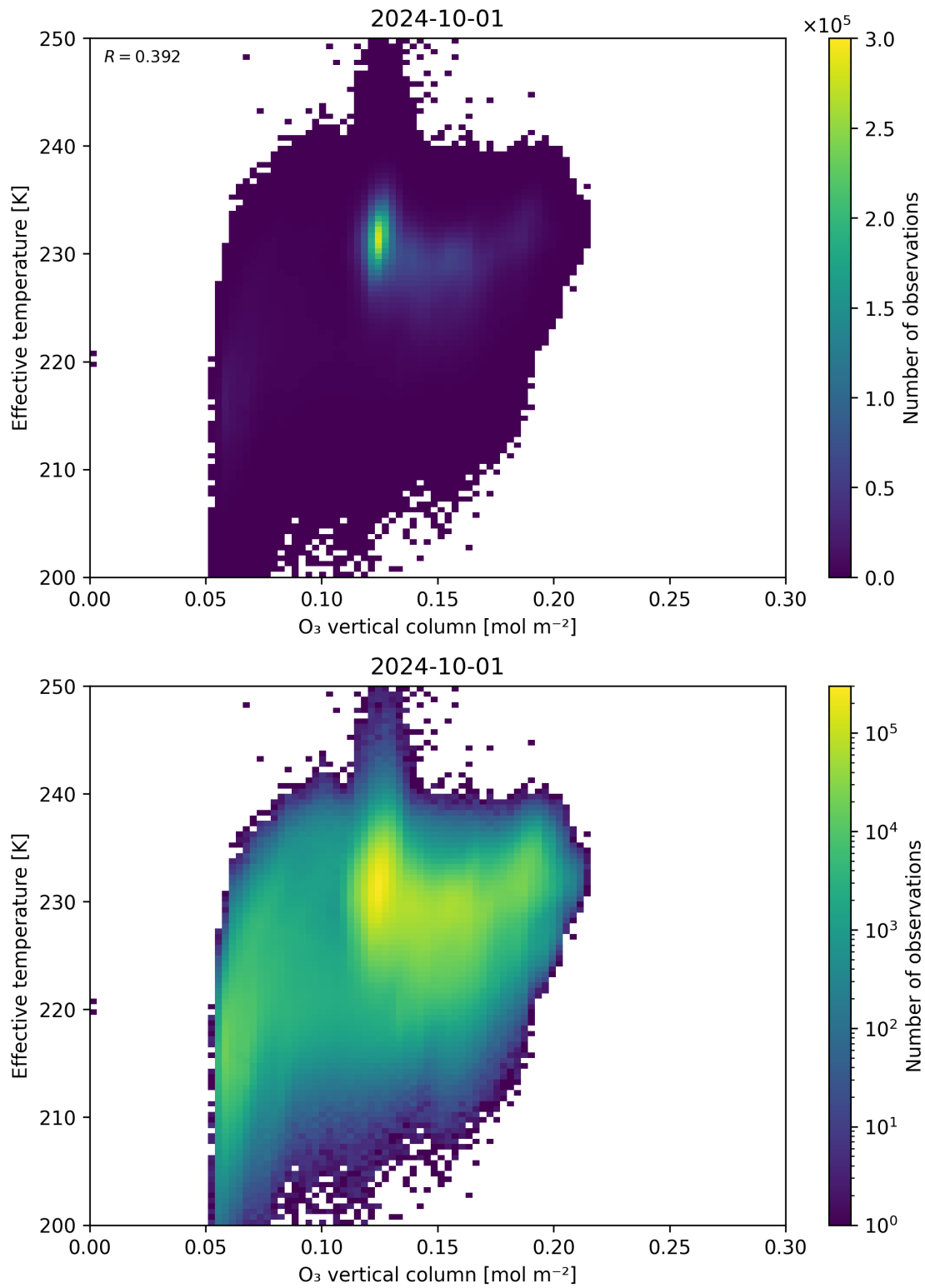
Figure 39: Scatter density plot of “O 3 vertical column” against “Effective temperature” for 2024-09-30 to 2024-10-02.
