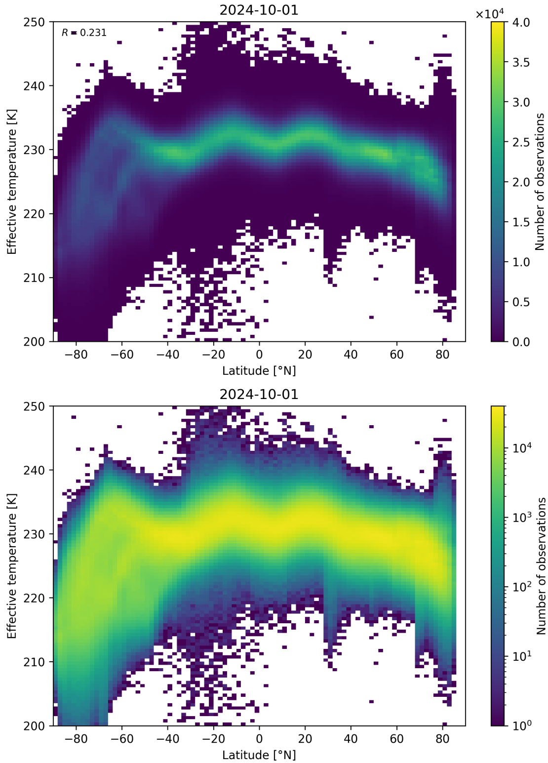
Figure 34: Scatter density plot of “Latitude” against “Effective temperature” for 2024-09-30 to 2024-10-02.
