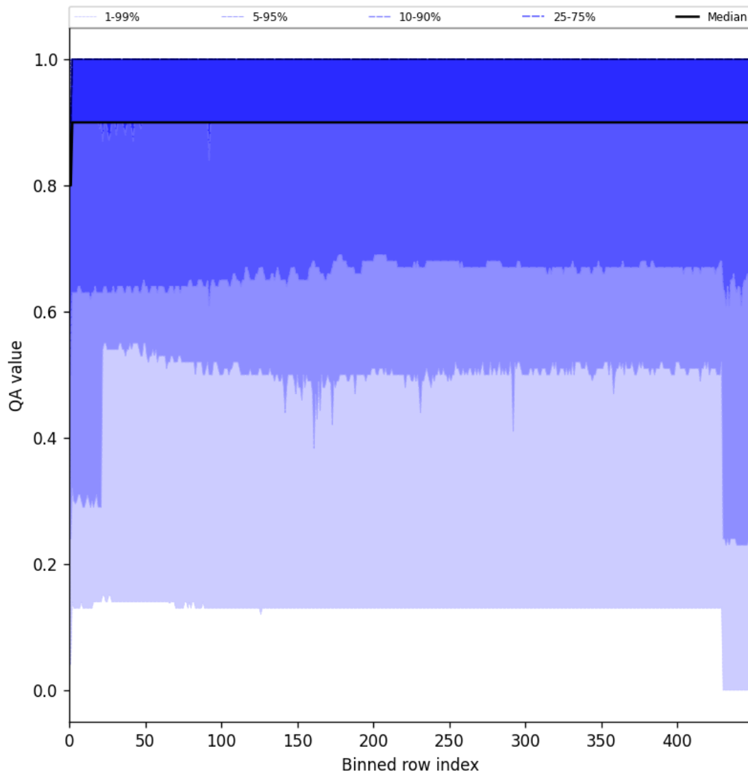
Figure 27: Along track statistics of “QA value” for 2024-09-30 to 2024-10-02
