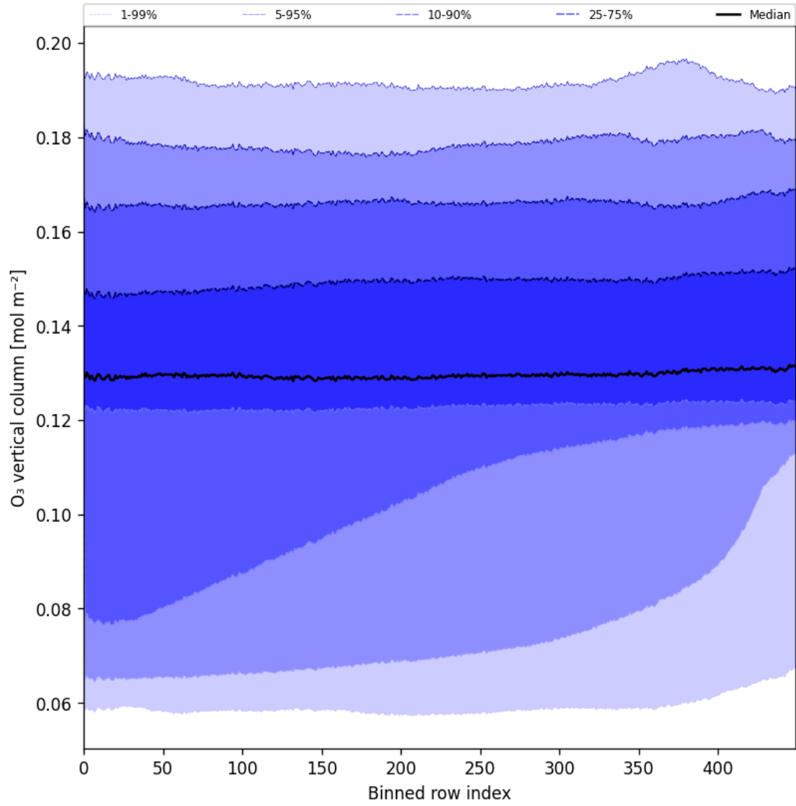
Figure 28: Along track statistics of "O 3 vertical column" for 2024-09-30 to 2024-10-02
