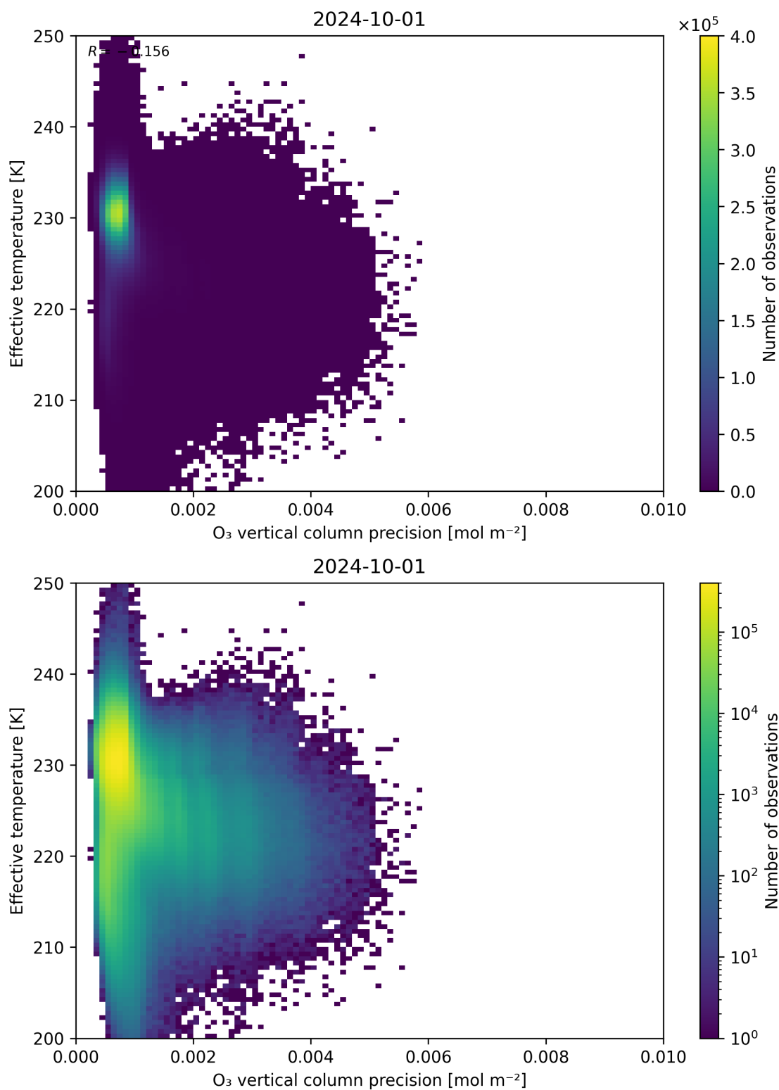
Figure 42: Scatter density plot of “O 3 vertical column precision” against “Effective temperature” for 2024-09-30 to 2024-10-02.
