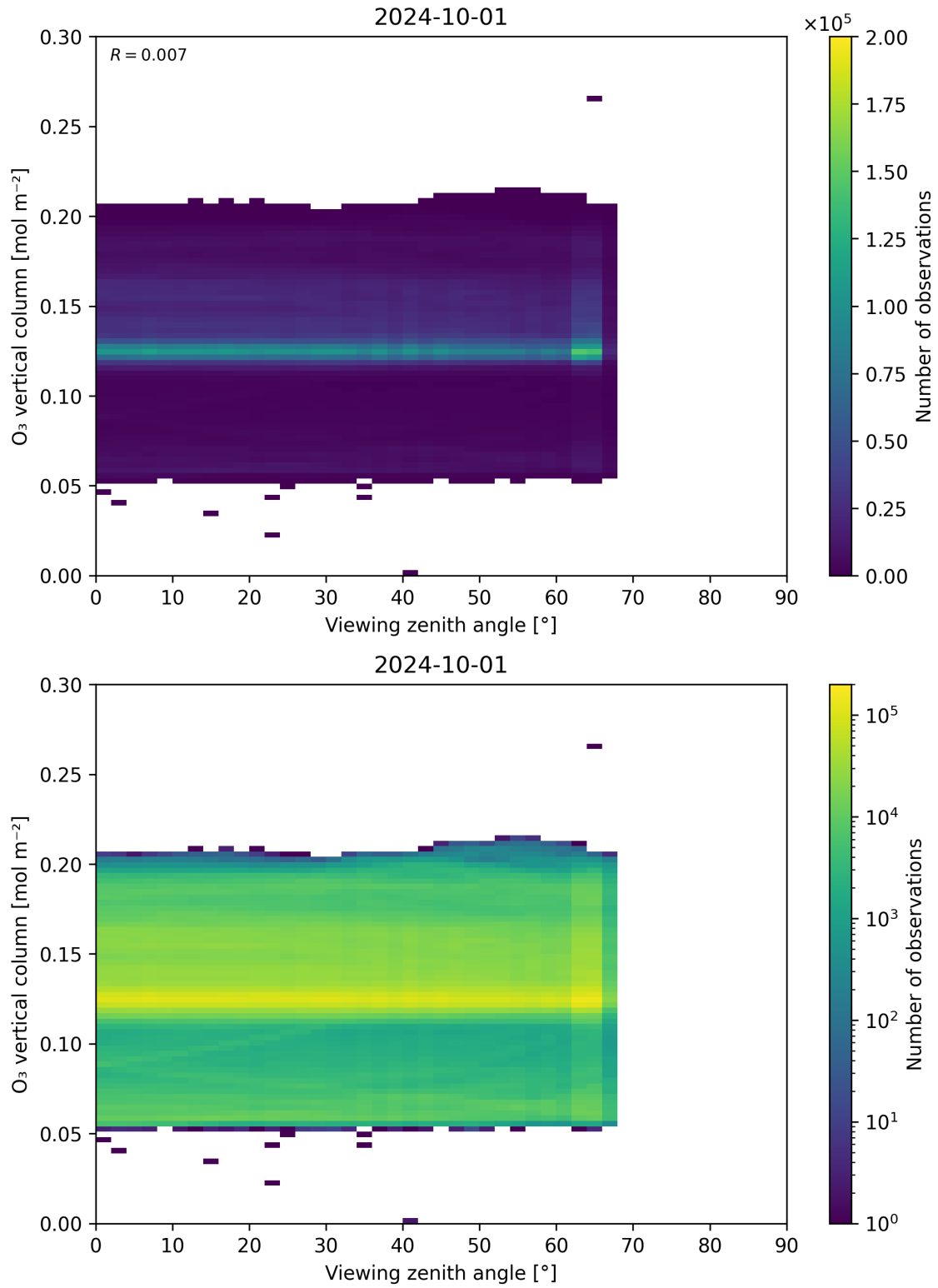
Figure 52: Scatter density plot of “Viewing zenith angle” against “O 3 vertical column” for 2024-09-30 to 2024-10-02.
