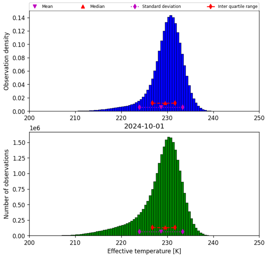
Figure 24: Histogram of “Effective temperature” for 2024-09-30 to 2024-10-02
