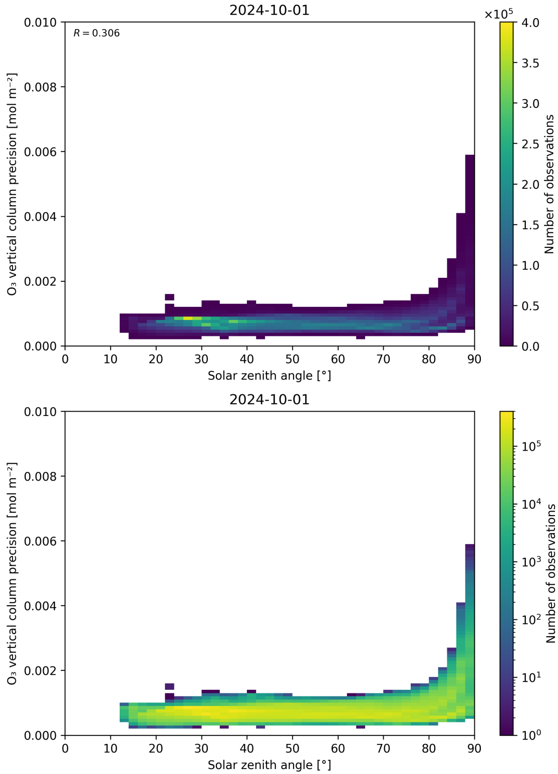
Figure 48: Scatter density plot of “Solar zenith angle” against “O 3 vertical column precision” for 2024-09-30 to 2024-10-02.
