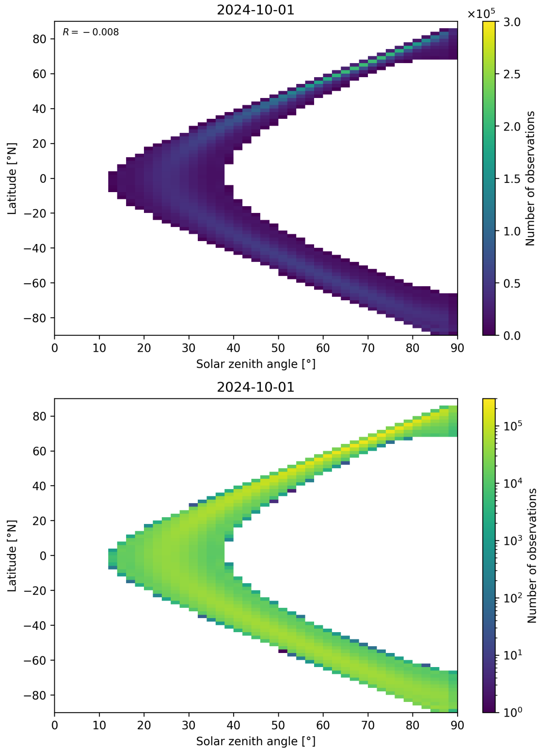
Figure 44: Scatter density plot of “Solar zenith angle” against “Latitude” for 2024-09-30 to 2024-10-02.
