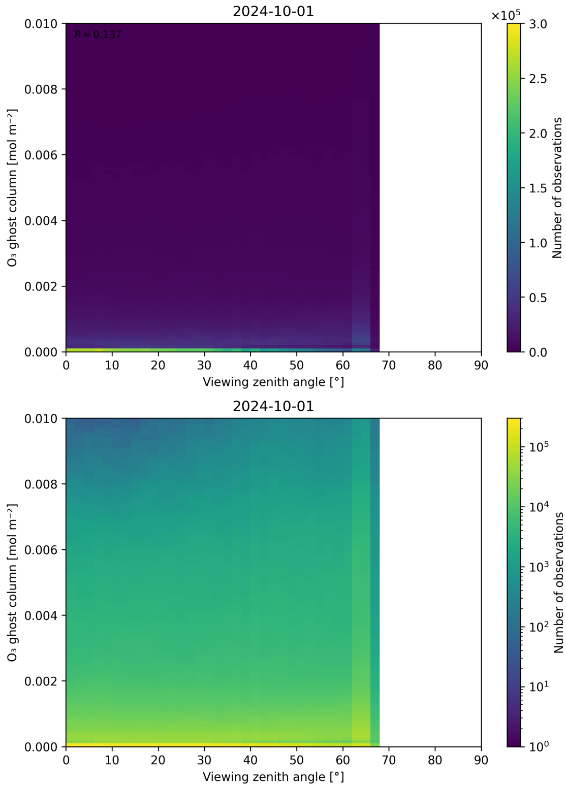
Figure 51: Scatter density plot of “Viewing zenith angle” against “O 3 ghost column” for 2024-09-30 to 2024-10-02.
