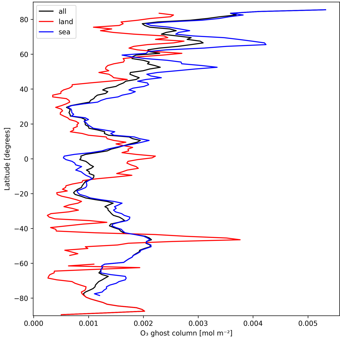
Figure 18: Zonal average of “O 3 ghost column” for 2024-09-30 to 2024-10-02.
