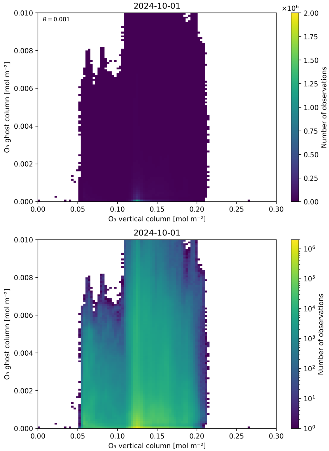
Figure 40: Scatter density plot of “O 3 vertical column” against “O 3 ghost column” for 2024-09-30 to 2024-10-02.
