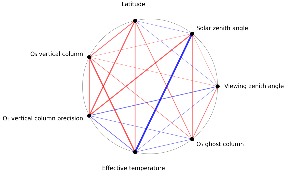
Figure 1: Map of correlation graph for 2024-09-30 to 2024-10-02.
