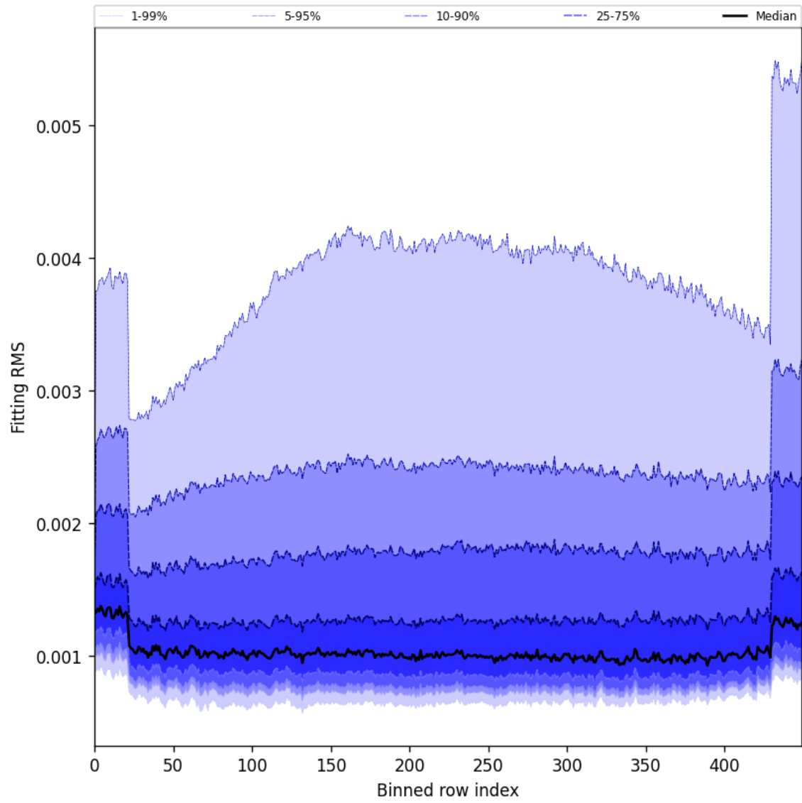
Figure 30: Along track statistics of “Fitting RMS” for 2024-09-30 to 2024-10-02
