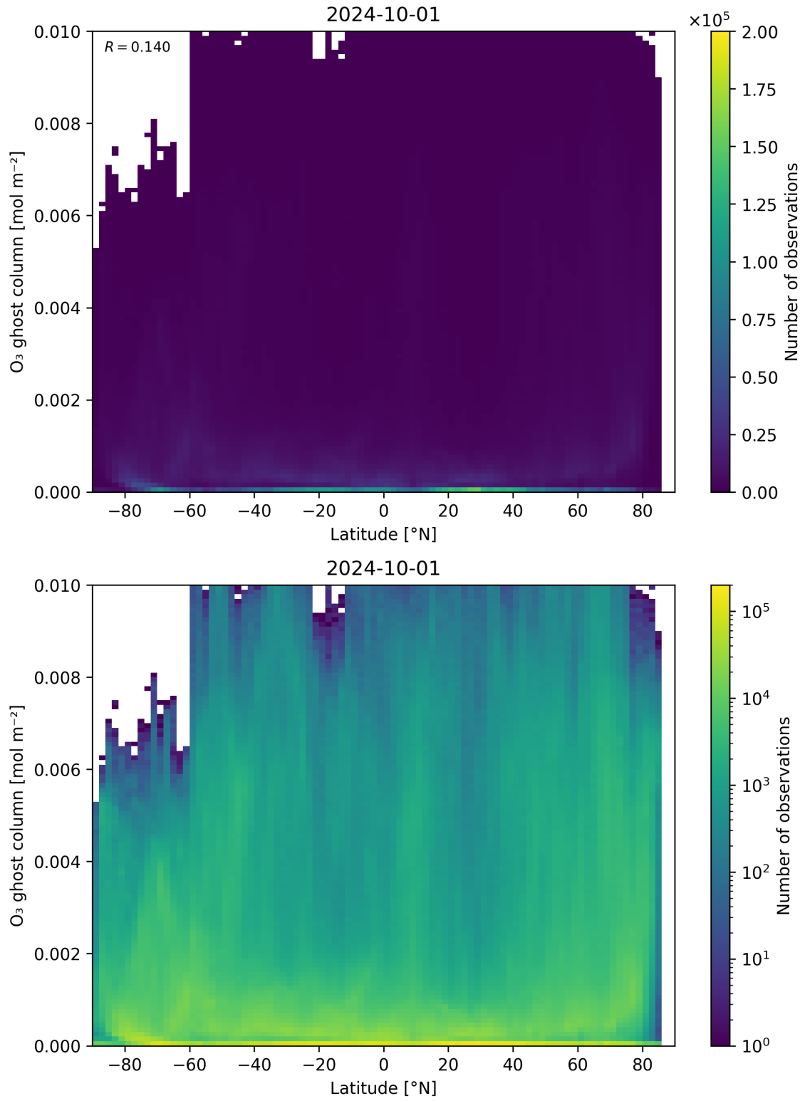
Figure 35: Scatter density plot of “Latitude” against “O 3 ghost column” for 2024-09-30 to 2024-10-02.
