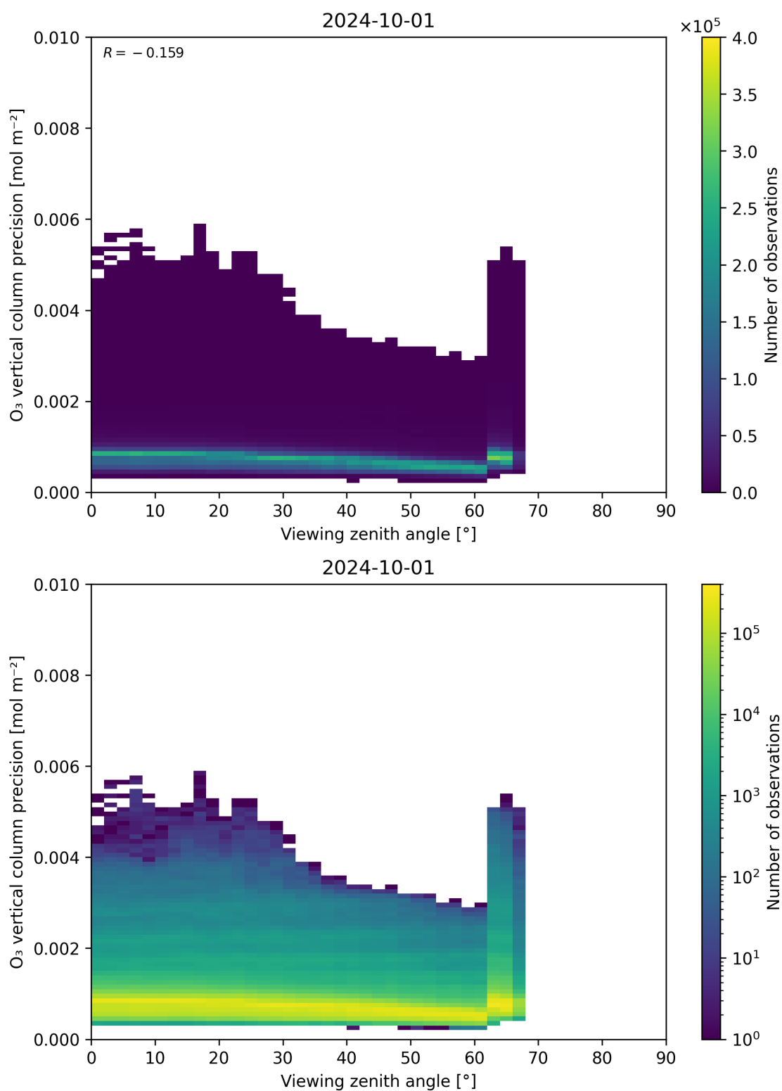
Figure 53: Scatter density plot of “Viewing zenith angle” against “O 3 vertical column precision” for 2024-09-30 to 2024-10-02.
