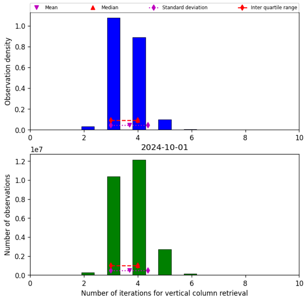
Figure 26: Histogram of “Number of iterations for vertical column retrieval” for 2024-09-30 to 2024-10-02
