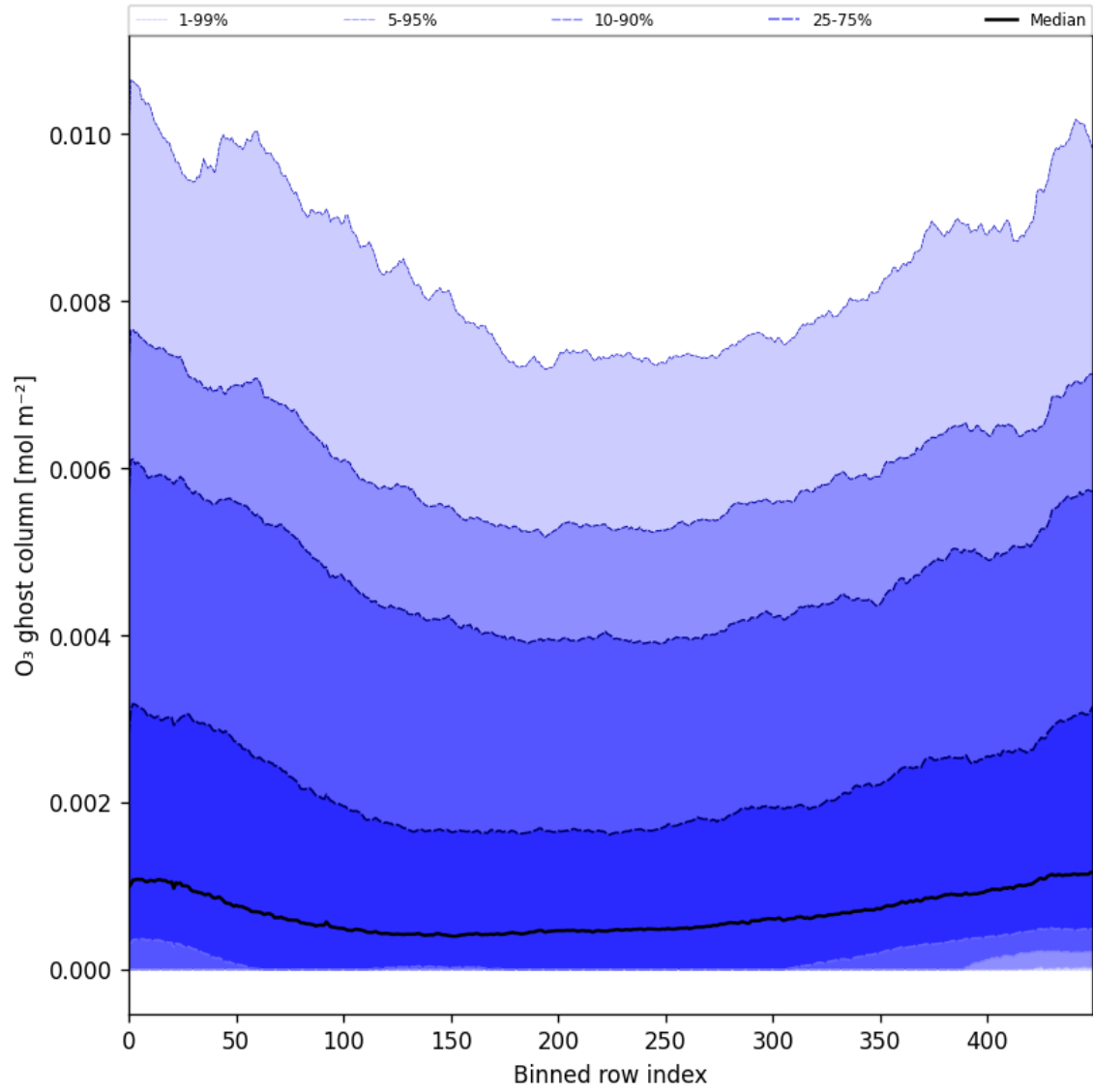
Figure 32: Along track statistics of “O 3 ghost column” for 2024-09-30 to 2024-10-02
