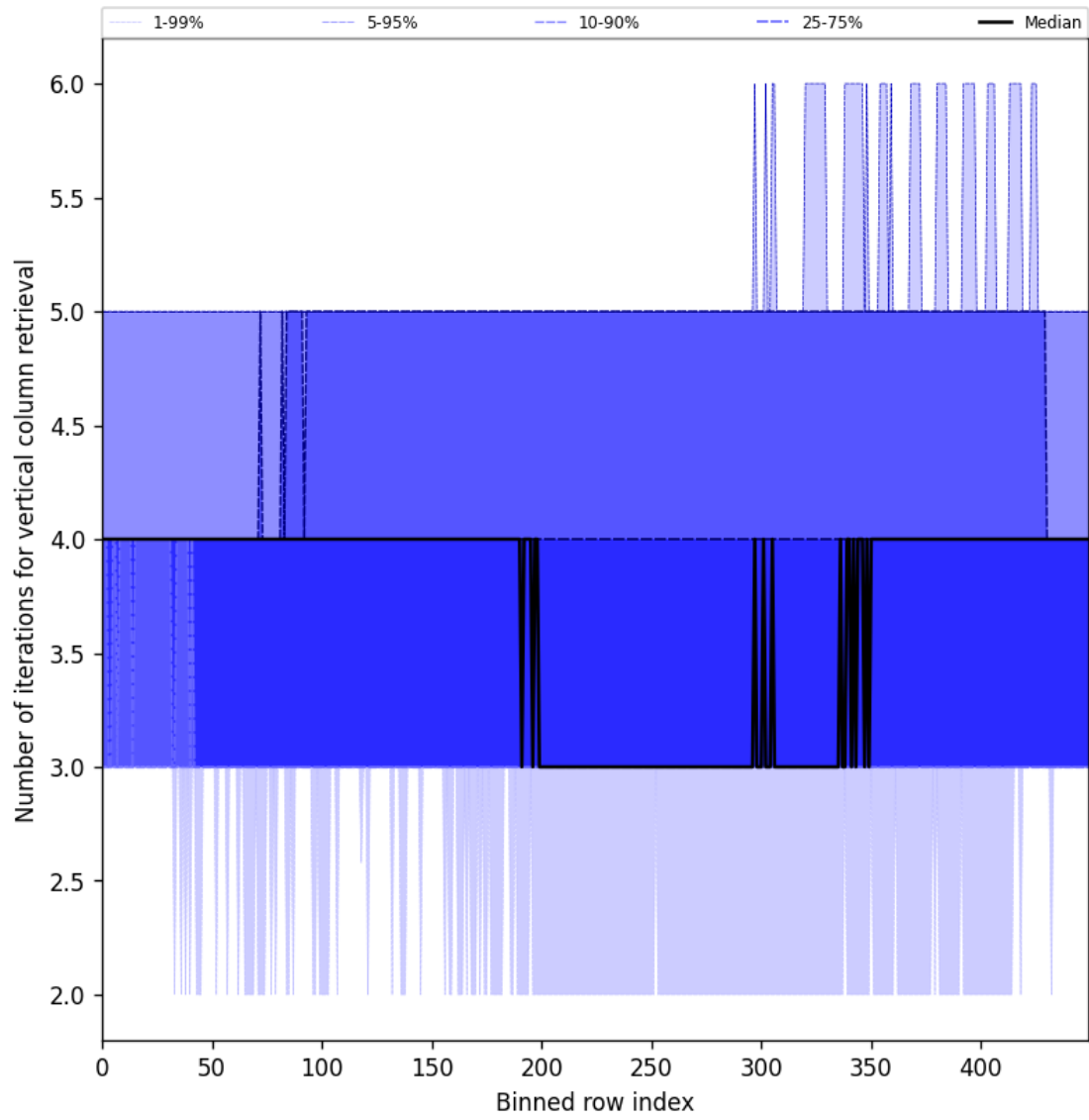
Figure 33: Along track statistics of “Number of iterations for vertical column retrieval” for 2024-09-30 to 2024-10-02
