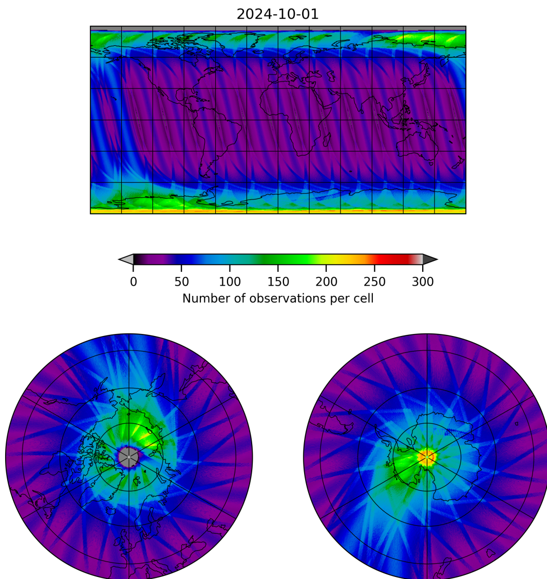
Figure 12: Map of the number of observations for 2024-09-30 to 2024-10-02
