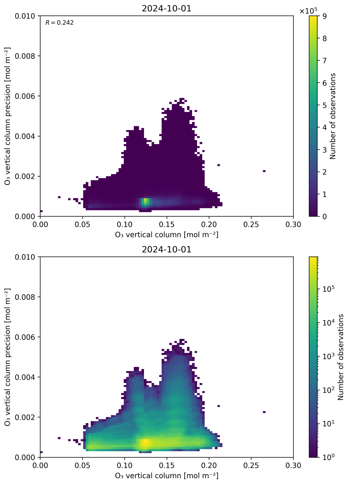
Figure 41: Scatter density plot of “O 3 vertical column” against “O 3 vertical column precision” for 2024-09-30 to 2024-10-02.
