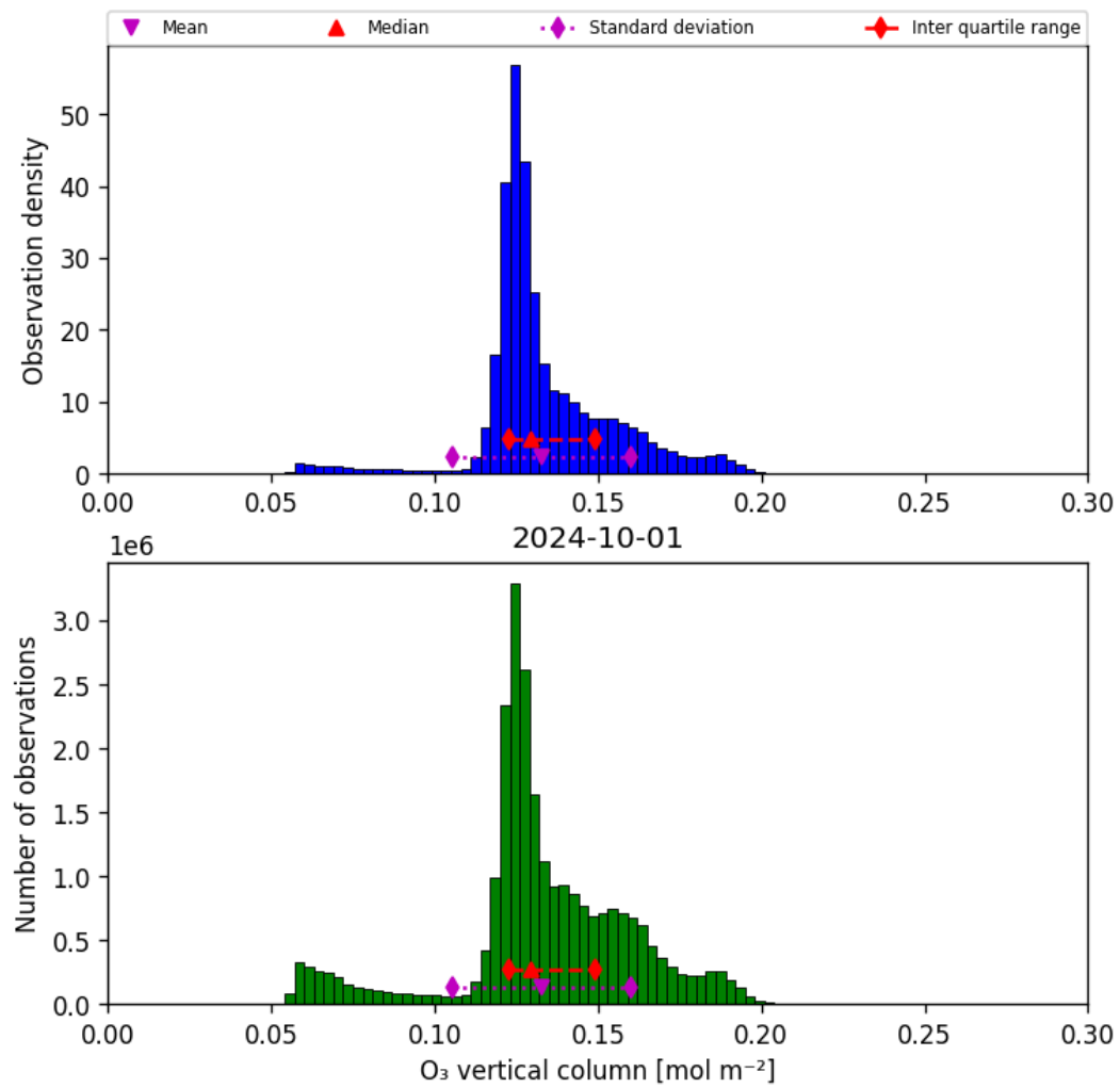
Figure 21: Histogram of “O 3 vertical column” for 2024-09-30 to 2024-10-02
