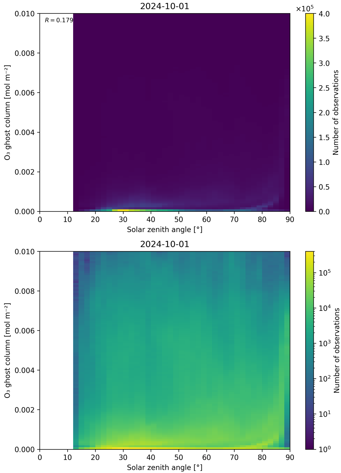
Figure 46: Scatter density plot of “Solar zenith angle” against “O 3 ghost column” for 2024-09-30 to 2024-10-02.
