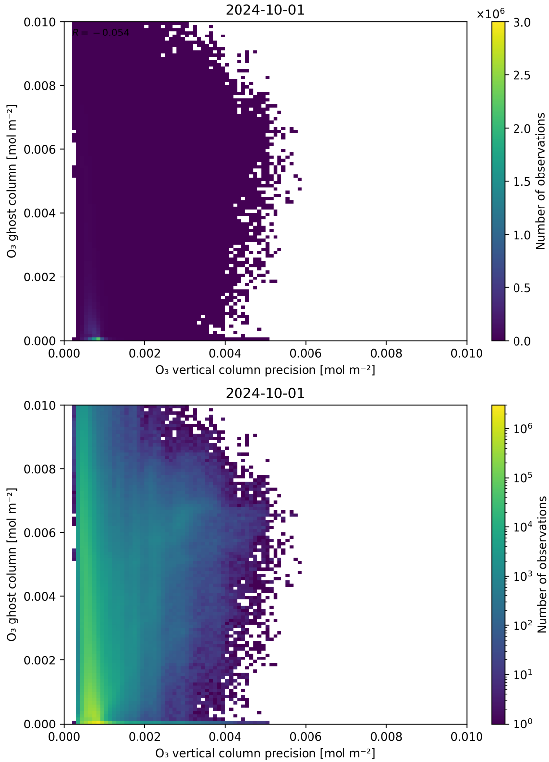
Figure 43: Scatter density plot of “O 3 vertical column precision” against “O 3 ghost column” for 2024-09-30 to 2024-10-02.
