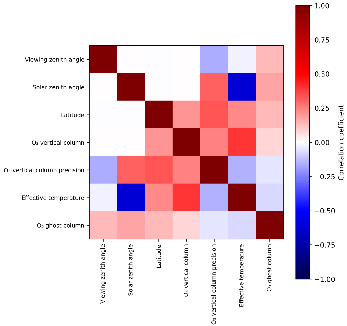
Figure 2: Map of correlation matrix for 2024-09-30 to 2024-10-02.
