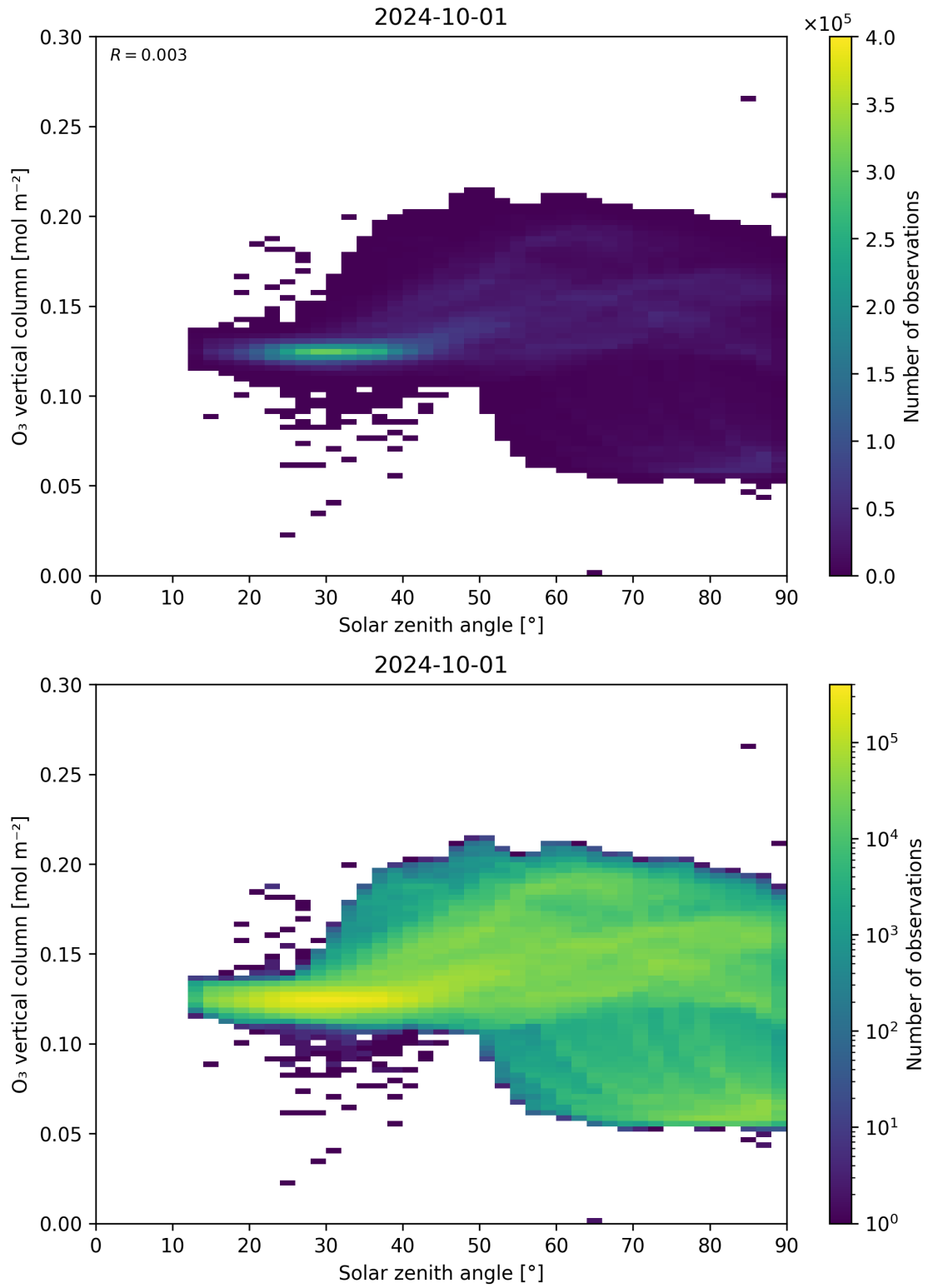
Figure 47: Scatter density plot of “Solar zenith angle” against “O 3 vertical column” for 2024-09-30 to 2024-10-02.
