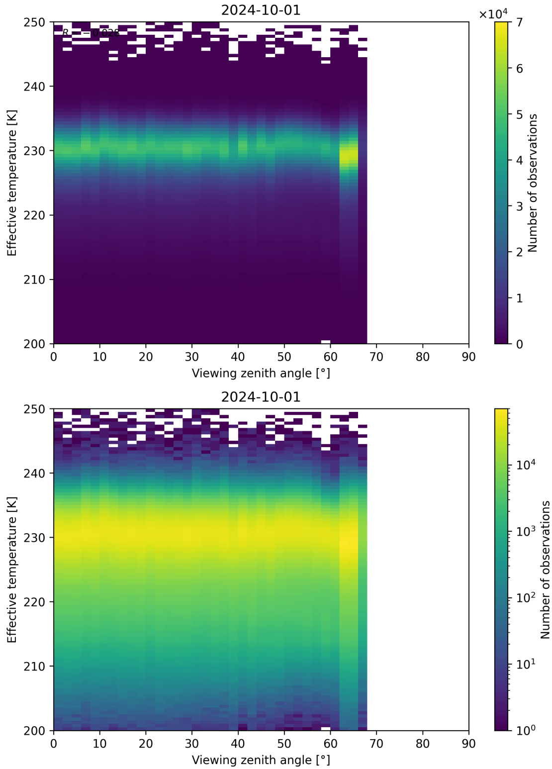
Figure 50: Scatter density plot of “Viewing zenith angle” against “Effective temperature” for 2024-09-30 to 2024-10-02.
