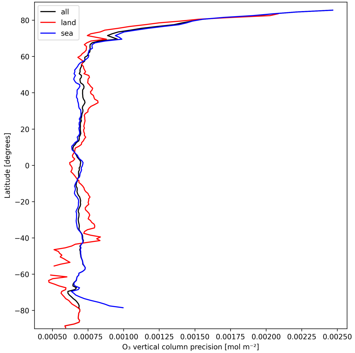
Figure 15: Zonal average of “O 3 vertical column precision” for 2024-09-30 to 2024-10-02.
