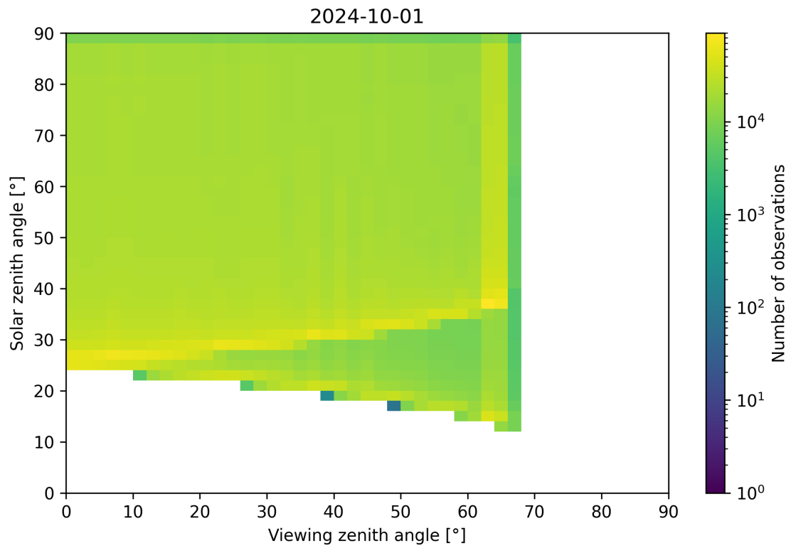
Figure 54: Scatter density plot of “Viewing zenith angle” against “Solar zenith angle” for 2024-09-30 to 2024-10-02.
