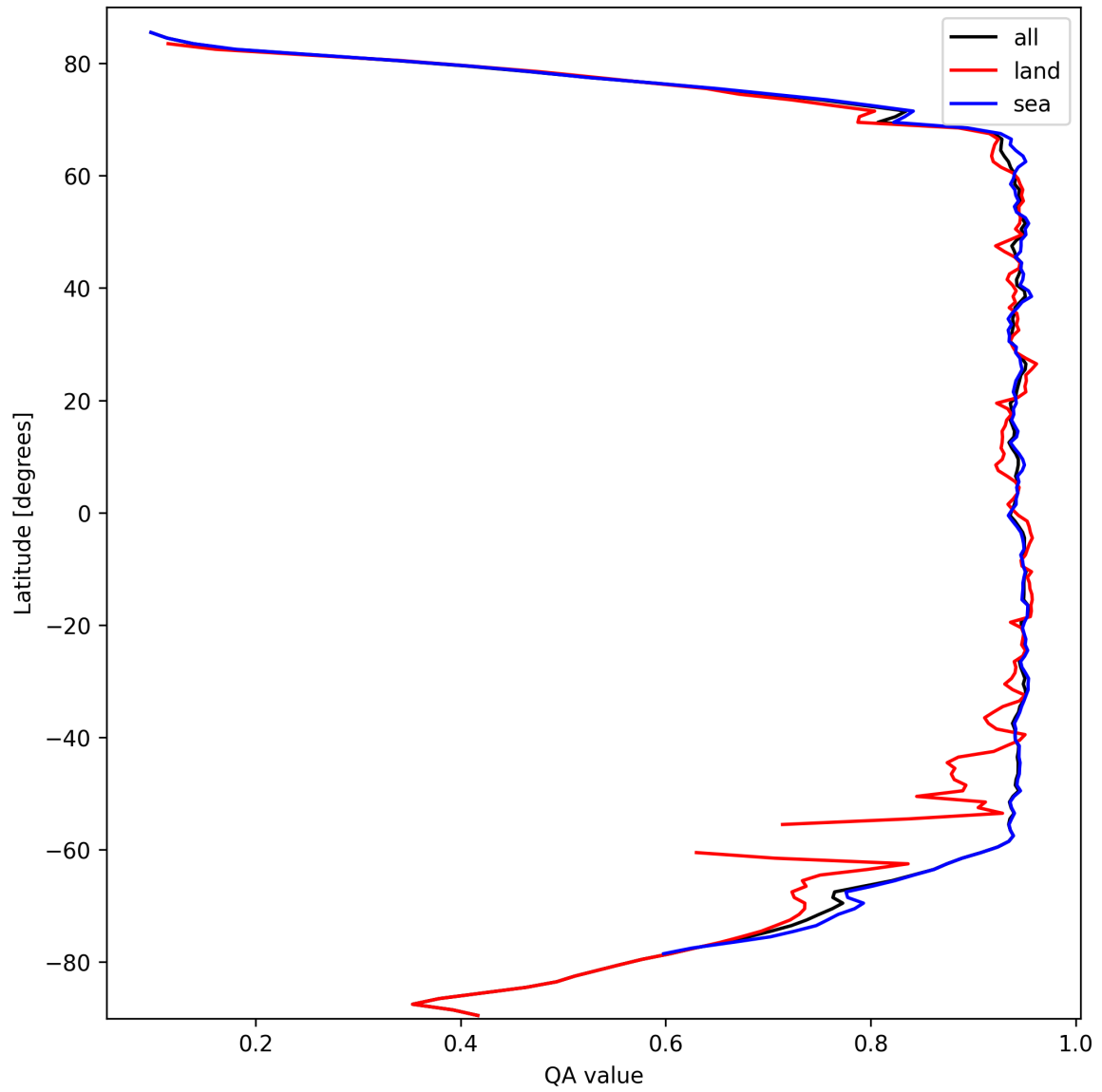
Figure 13: Zonal average of “QA value” for 2024-09-30 to 2024-10-02.
