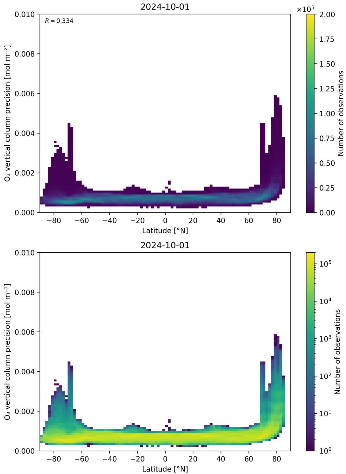
Figure 37: Scatter density plot of “Latitude” against “O 3 vertical column precision” for 2024-09-30 to 2024-10-02.
