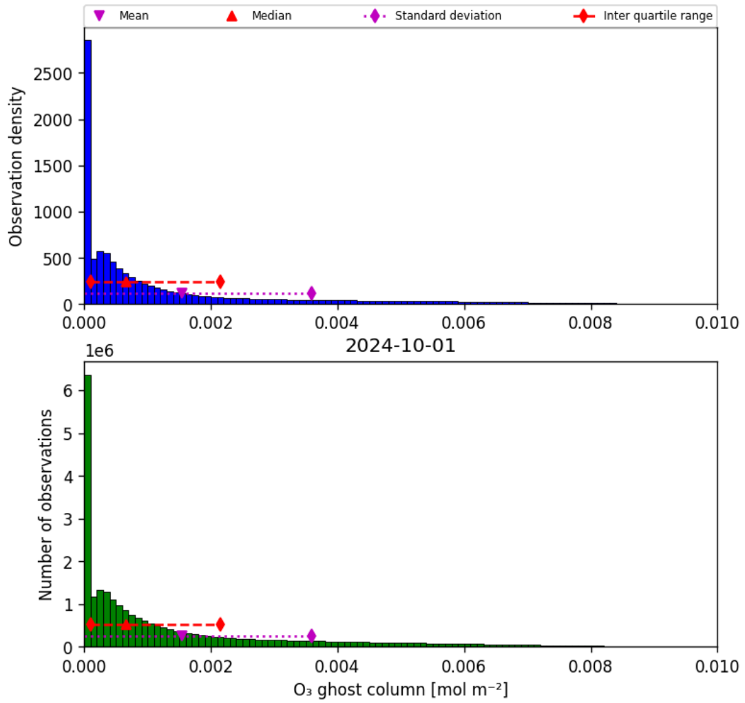
Figure 25: Histogram of “O 3 ghost column” for 2024-09-30 to 2024-10-02
