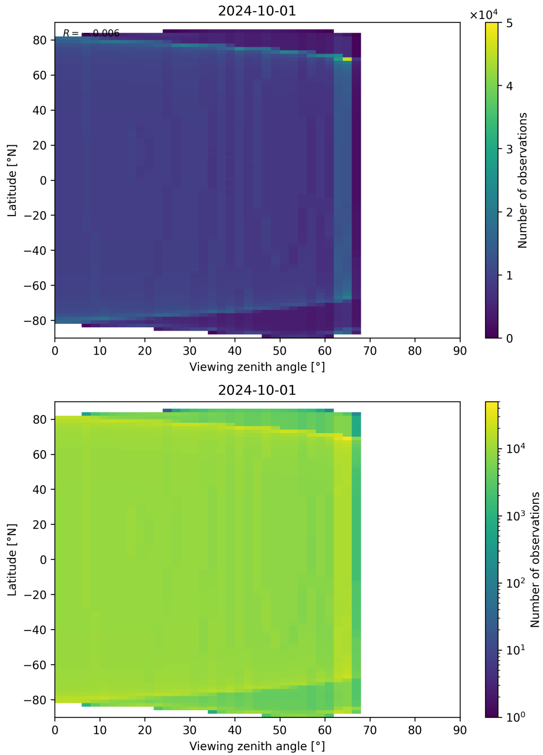
Figure 49: Scatter density plot of “Viewing zenith angle” against “Latitude” for 2024-09-30 to 2024-10-02.
