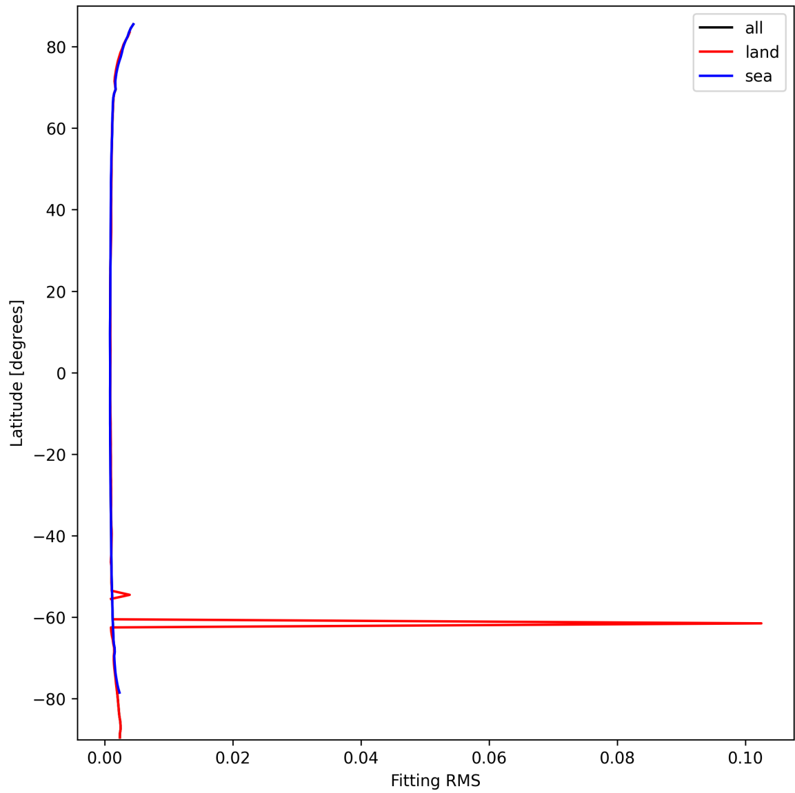
Figure 16: Zonal average of “Fitting RMS” for 2024-09-30 to 2024-10-02.
