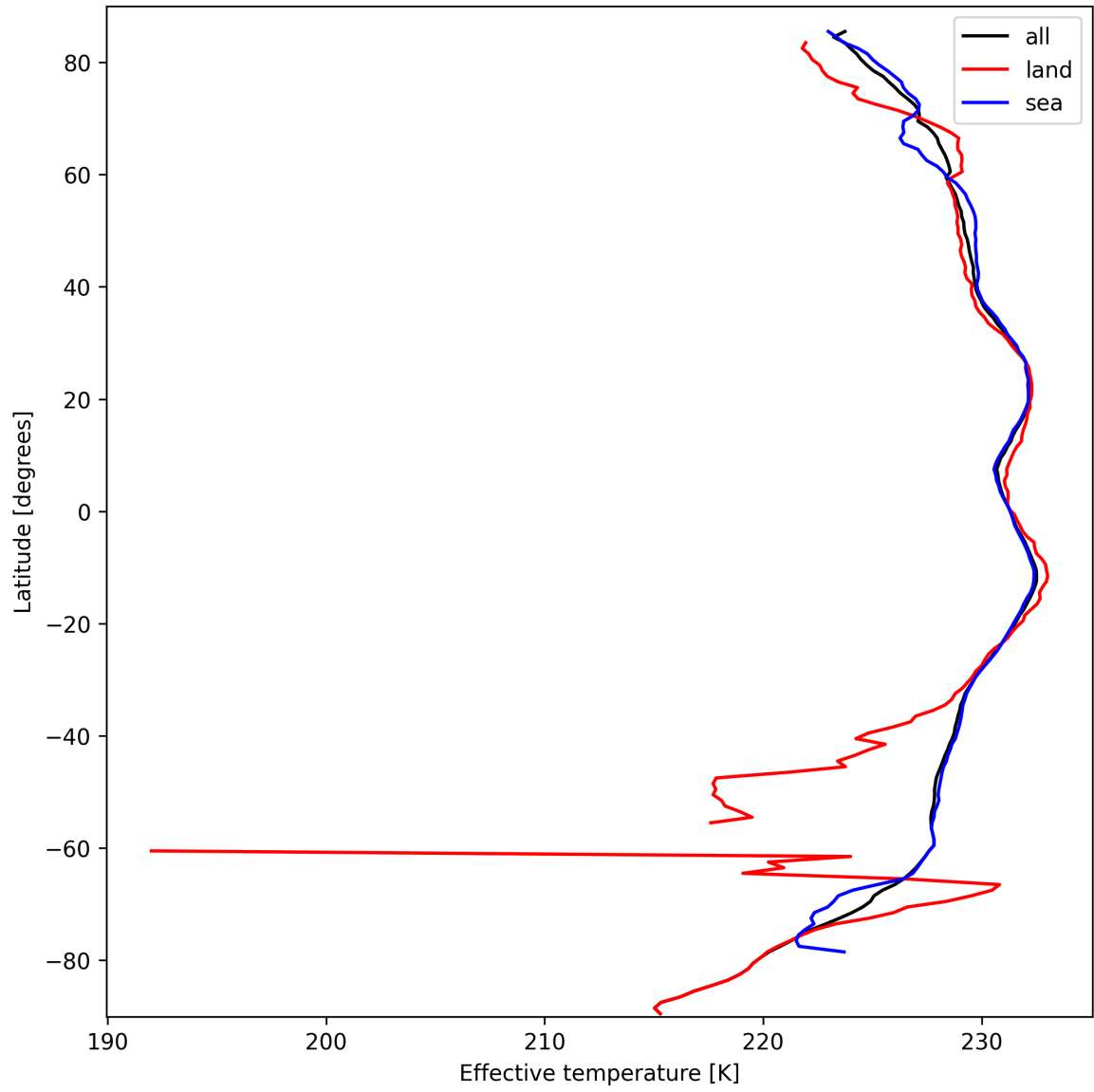
Figure 17: Zonal average of “Effective temperature” for 2024-09-30 to 2024-10-02.
