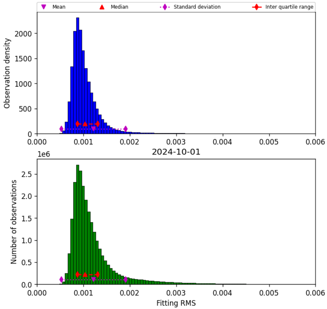
Figure 23: Histogram of “Fitting RMS” for 2024-09-30 to 2024-10-02
