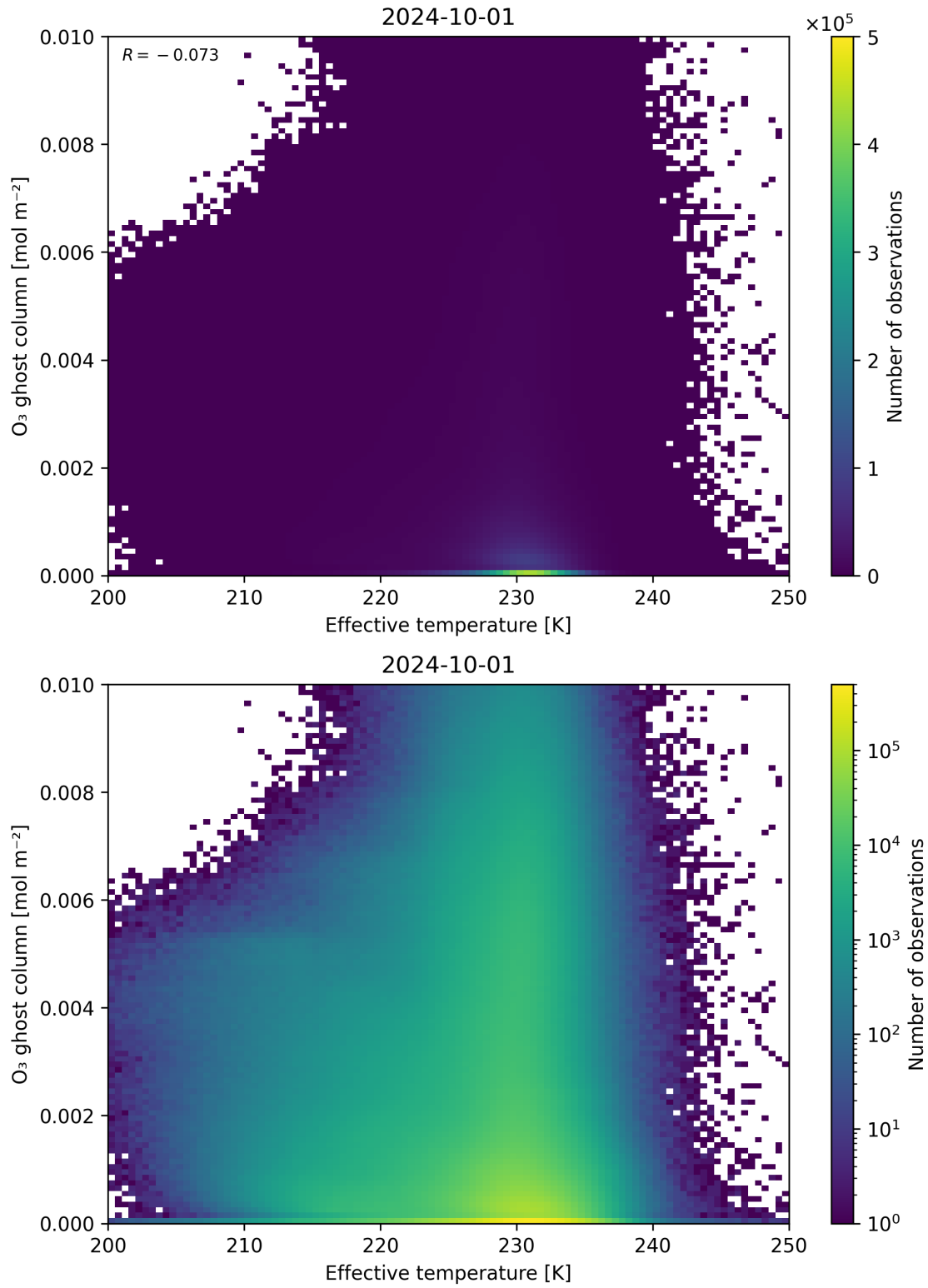
Figure 38: Scatter density plot of “Effective temperature” against “O 3 ghost column” for 2024-09-30 to 2024-10-02.
