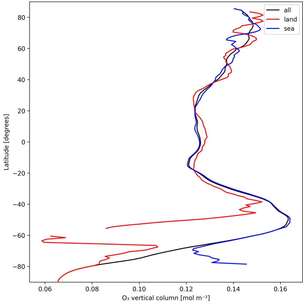
Figure 14: Zonal average of “O 3 vertical column” for 2024-09-30 to 2024-10-02.
