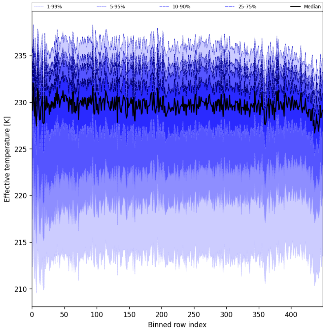
Figure 31: Along track statistics of “Effective temperature” for 2024-09-30 to 2024-10-02
