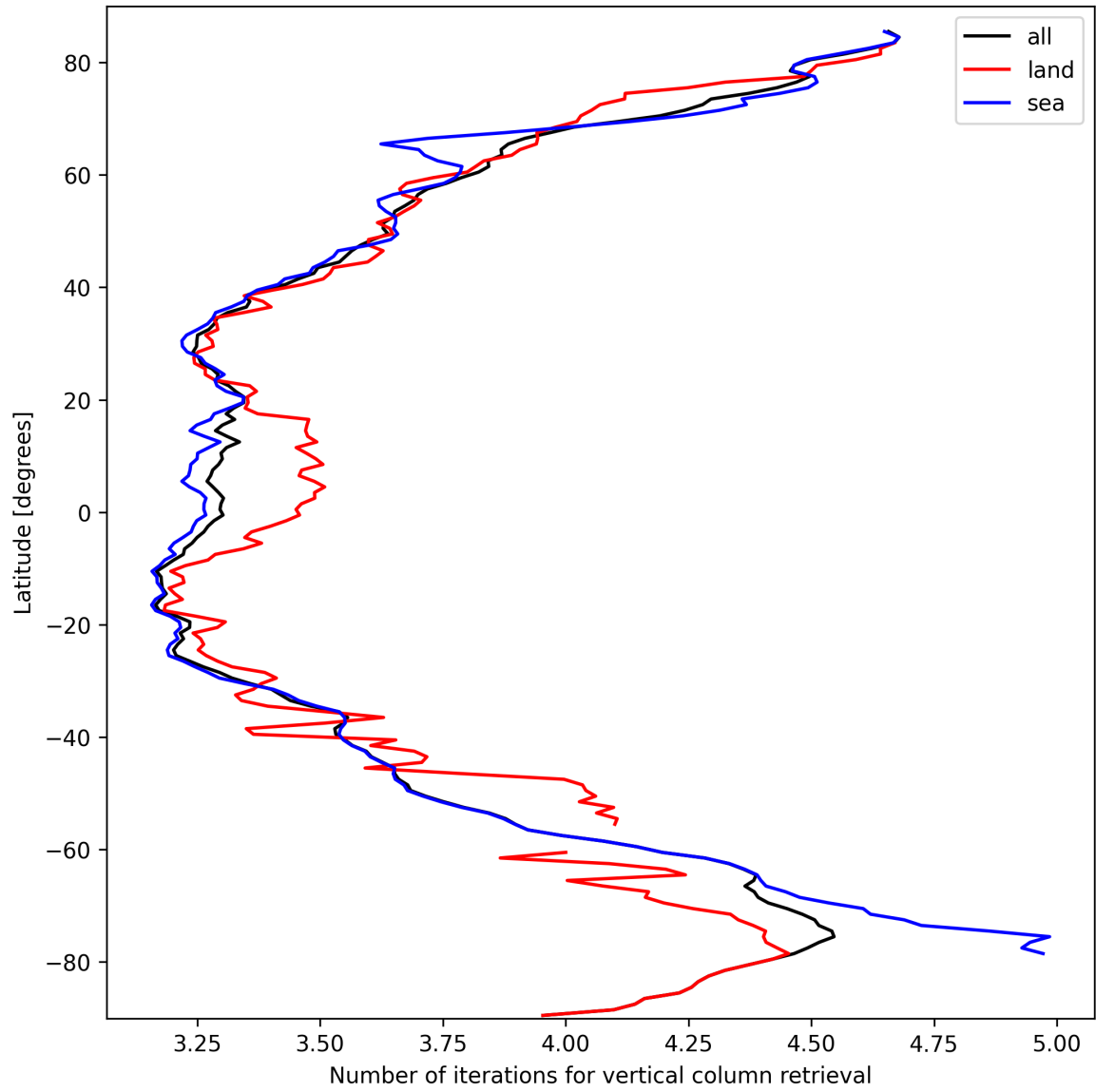
Figure 19: Zonal average of “Number of iterations for vertical column retrieval” for 2024-09-30 to 2024-10-02.
