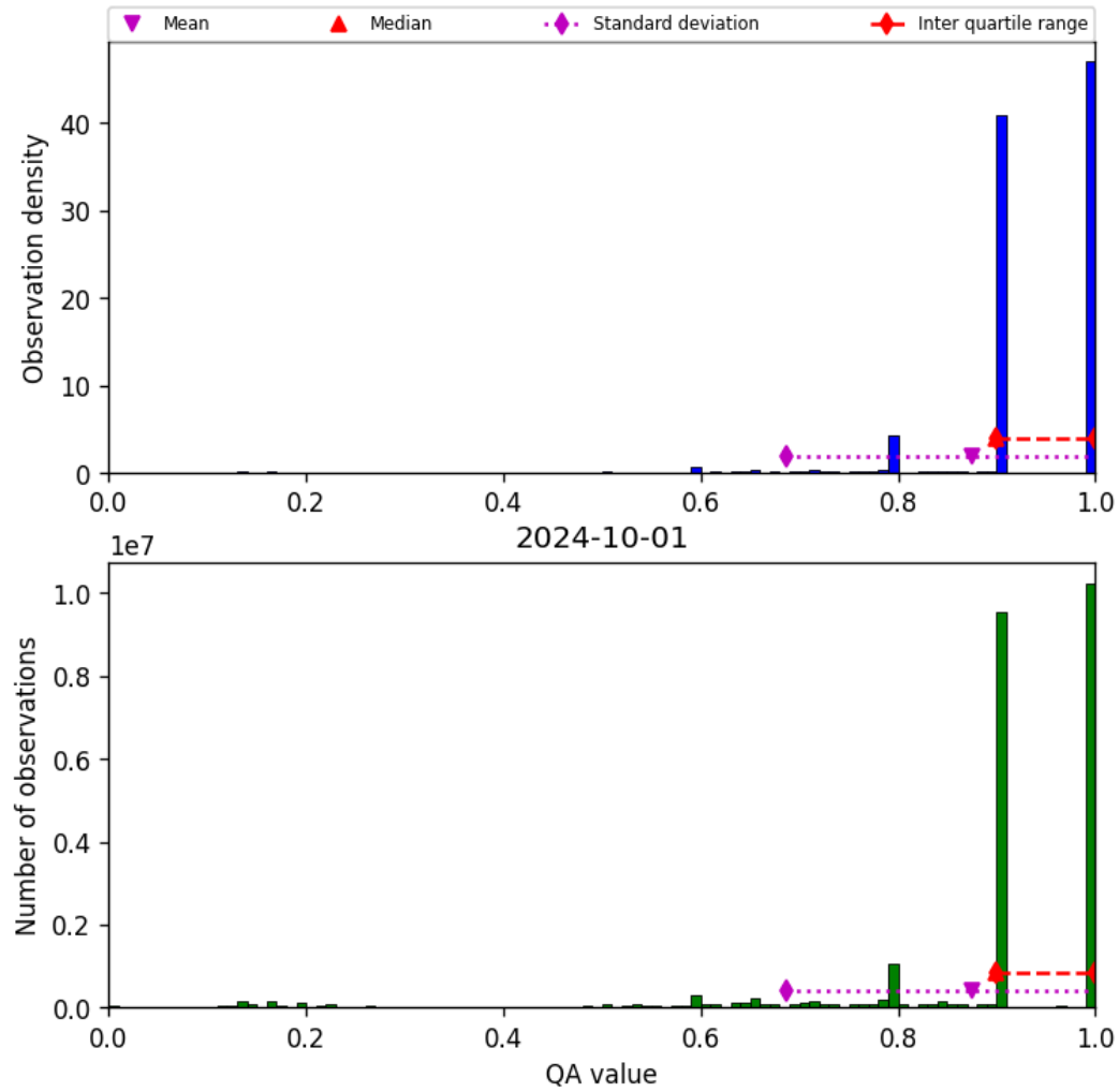
Figure 20: Histogram of “QA value” for 2024-09-30 to 2024-10-02
