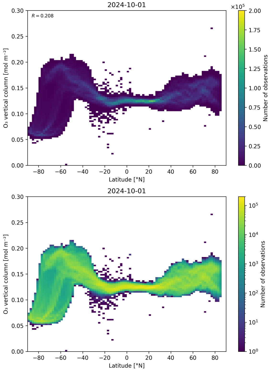
Figure 36: Scatter density plot of “Latitude” against “O 3 vertical column” for 2024-09-30 to 2024-10-02.
