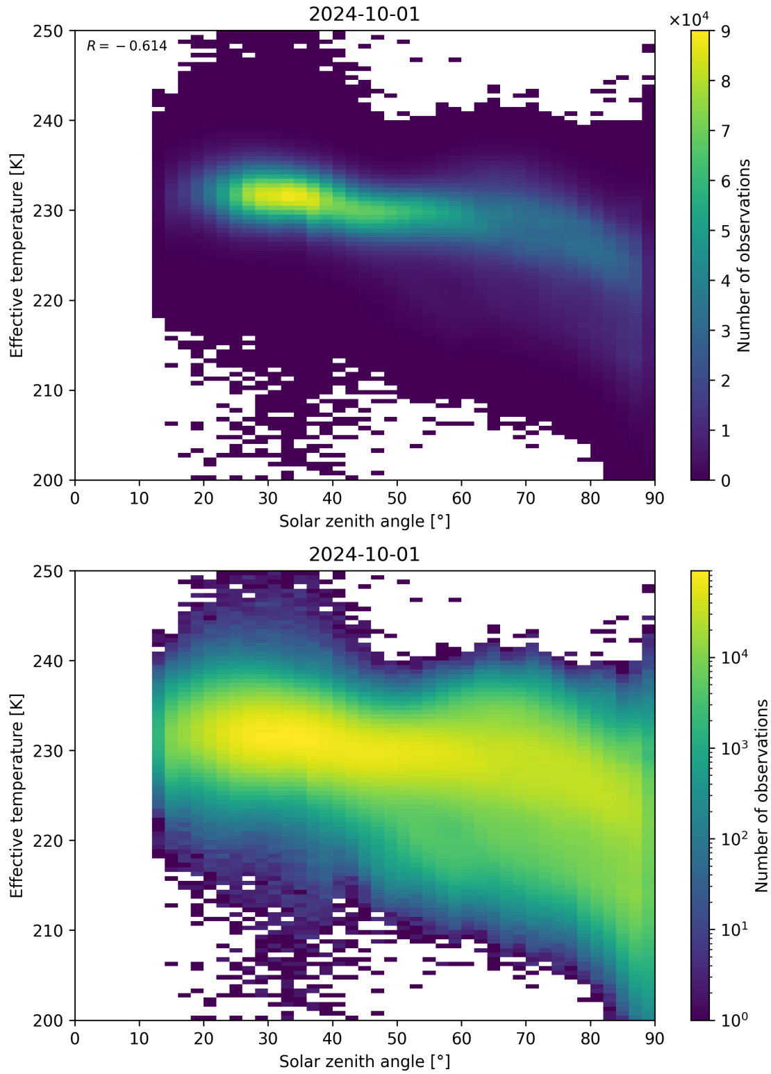
Figure 45: Scatter density plot of “Solar zenith angle” against “Effective temperature” for 2024-09-30 to 2024-10-02.
