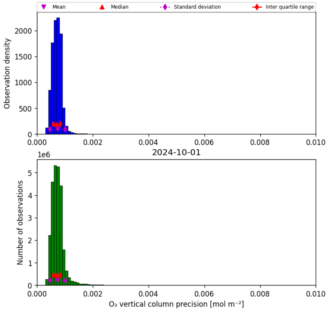
Figure 22: Histogram of “O 3 vertical column precision” for 2024-09-30 to 2024-10-02
