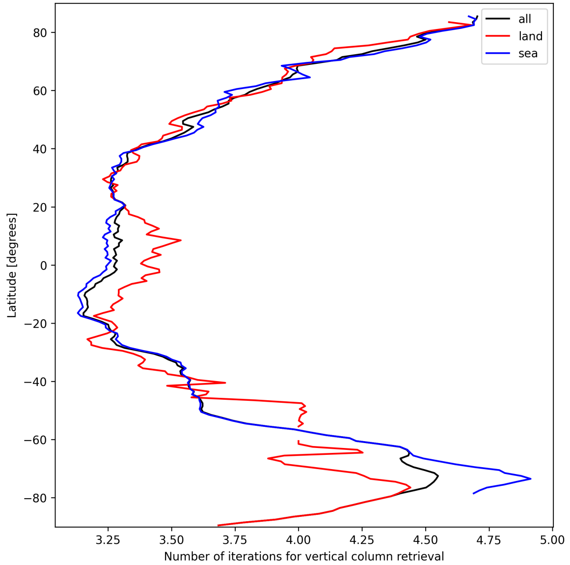
Figure 19: Zonal average of “Number of iterations for vertical column retrieval” for 2024-10-01 to 2024-10-03.
