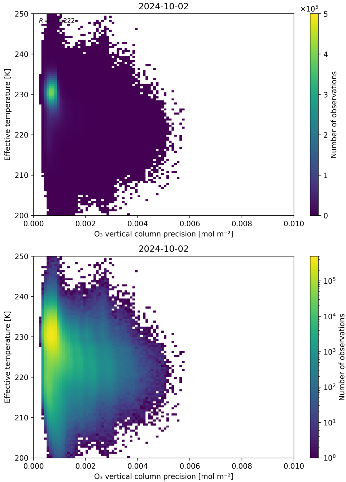
Figure 42: Scatter density plot of “O 3 vertical column precision” against “Effective temperature” for 2024-10-01 to 2024-10-03.
