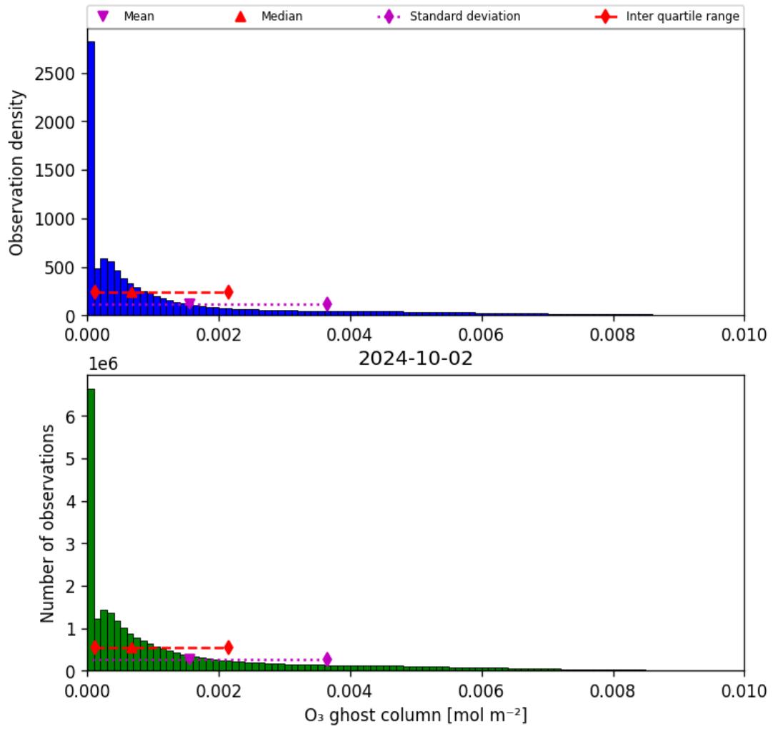
Figure 25: Histogram of “O 3 ghost column” for 2024-10-01 to 2024-10-03
