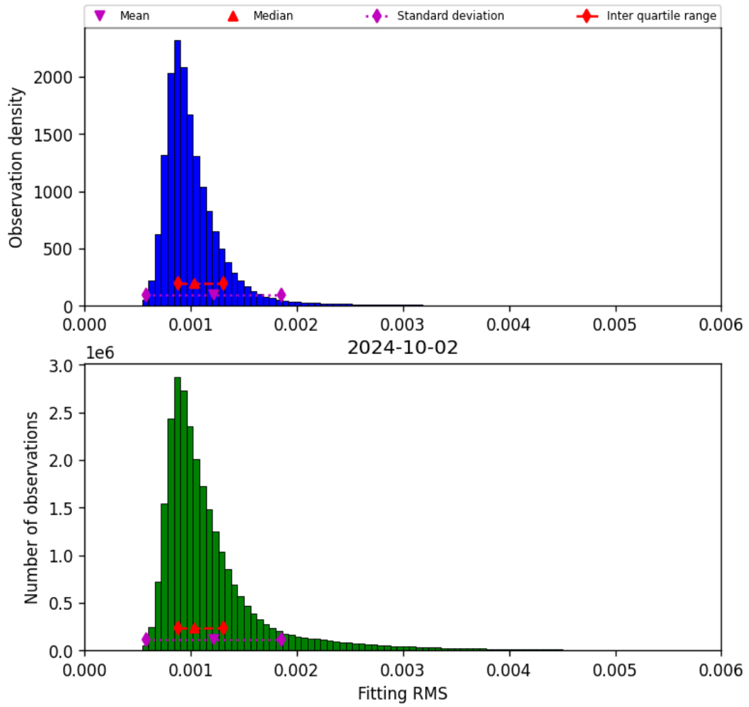
Figure 23: Histogram of “Fitting RMS” for 2024-10-01 to 2024-10-03
