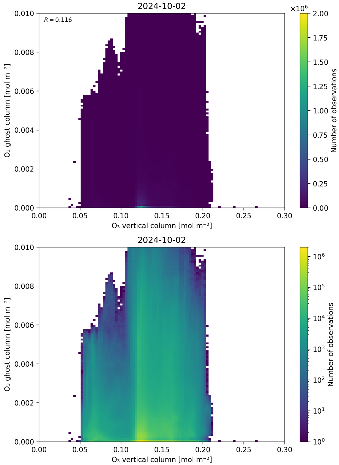
Figure 40: Scatter density plot of “O 3 vertical column” against “O 3 ghost column” for 2024-10-01 to 2024-10-03.
