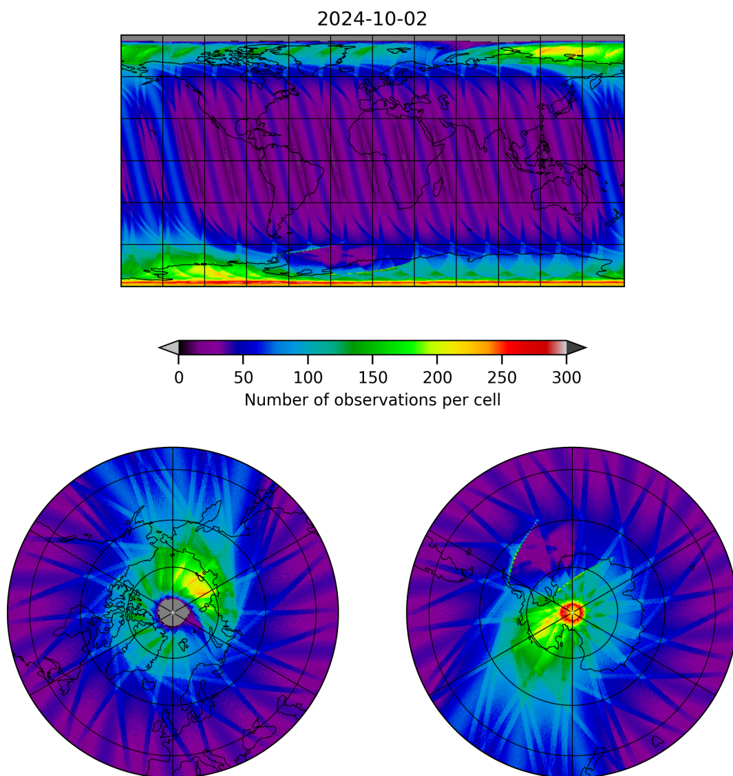
Figure 12: Map of the number of observations for 2024-10-01 to 2024-10-03
