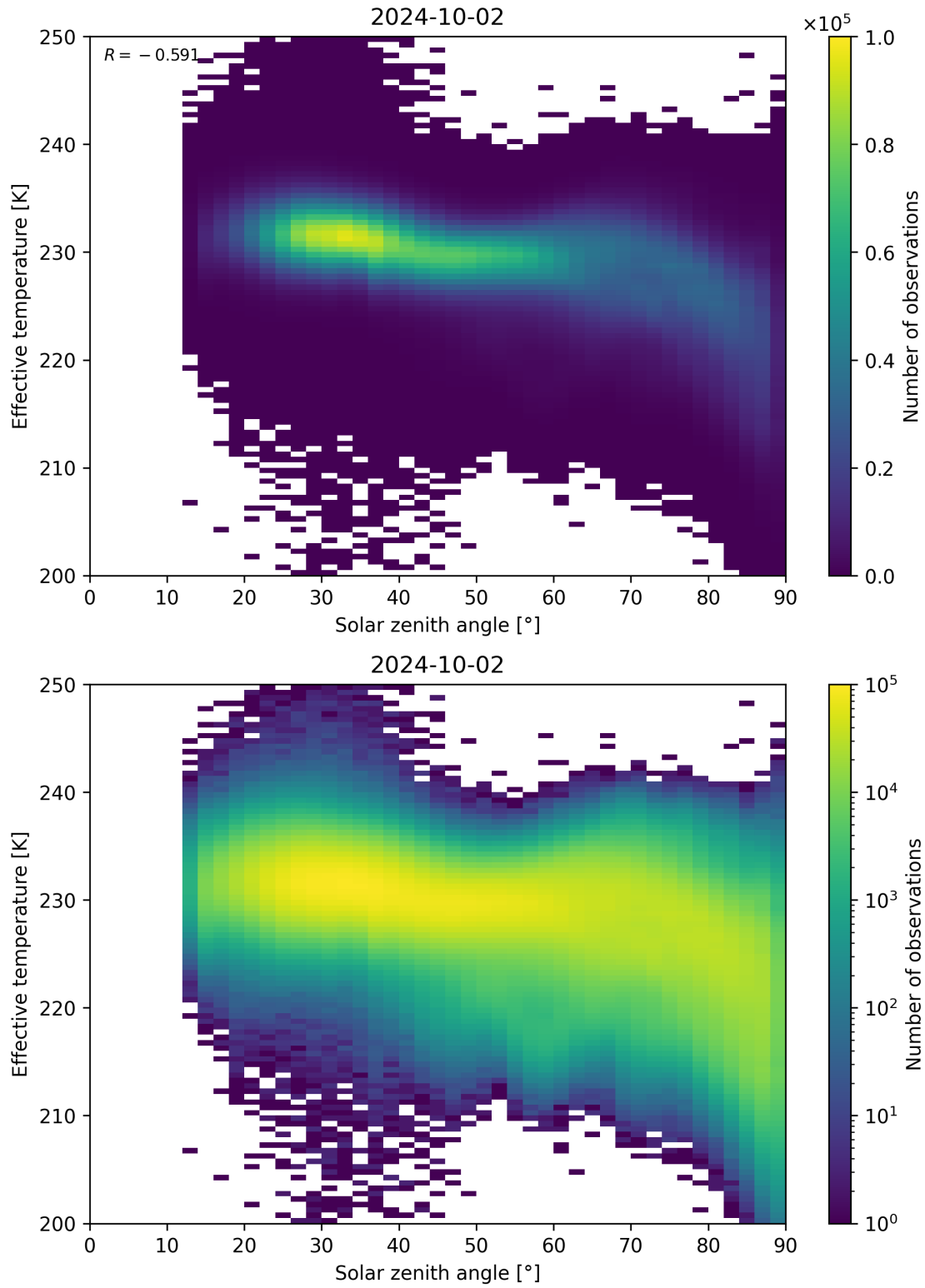
Figure 45: Scatter density plot of “Solar zenith angle” against “Effective temperature” for 2024-10-01 to 2024-10-03.
