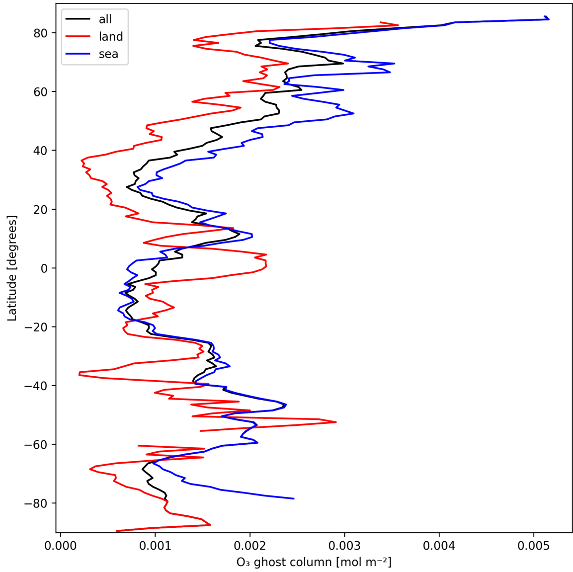
Figure 18: Zonal average of “O 3 ghost column” for 2024-10-01 to 2024-10-03.
