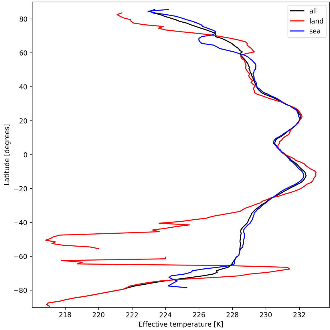
Figure 17: Zonal average of “Effective temperature” for 2024-10-01 to 2024-10-03.
