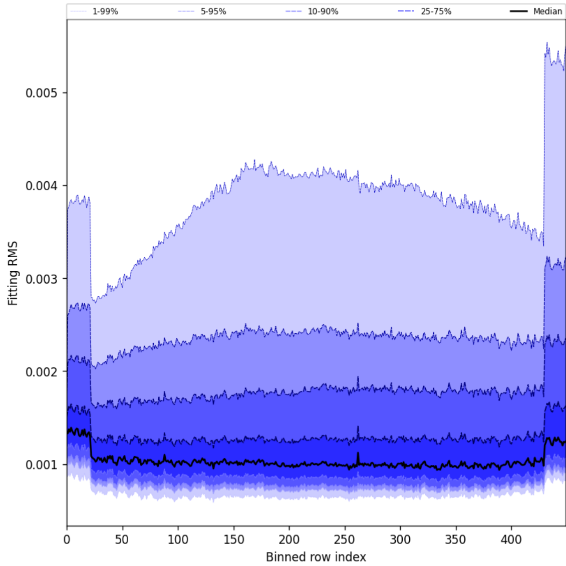
Figure 30: Along track statistics of “Fitting RMS” for 2024-10-01 to 2024-10-03
