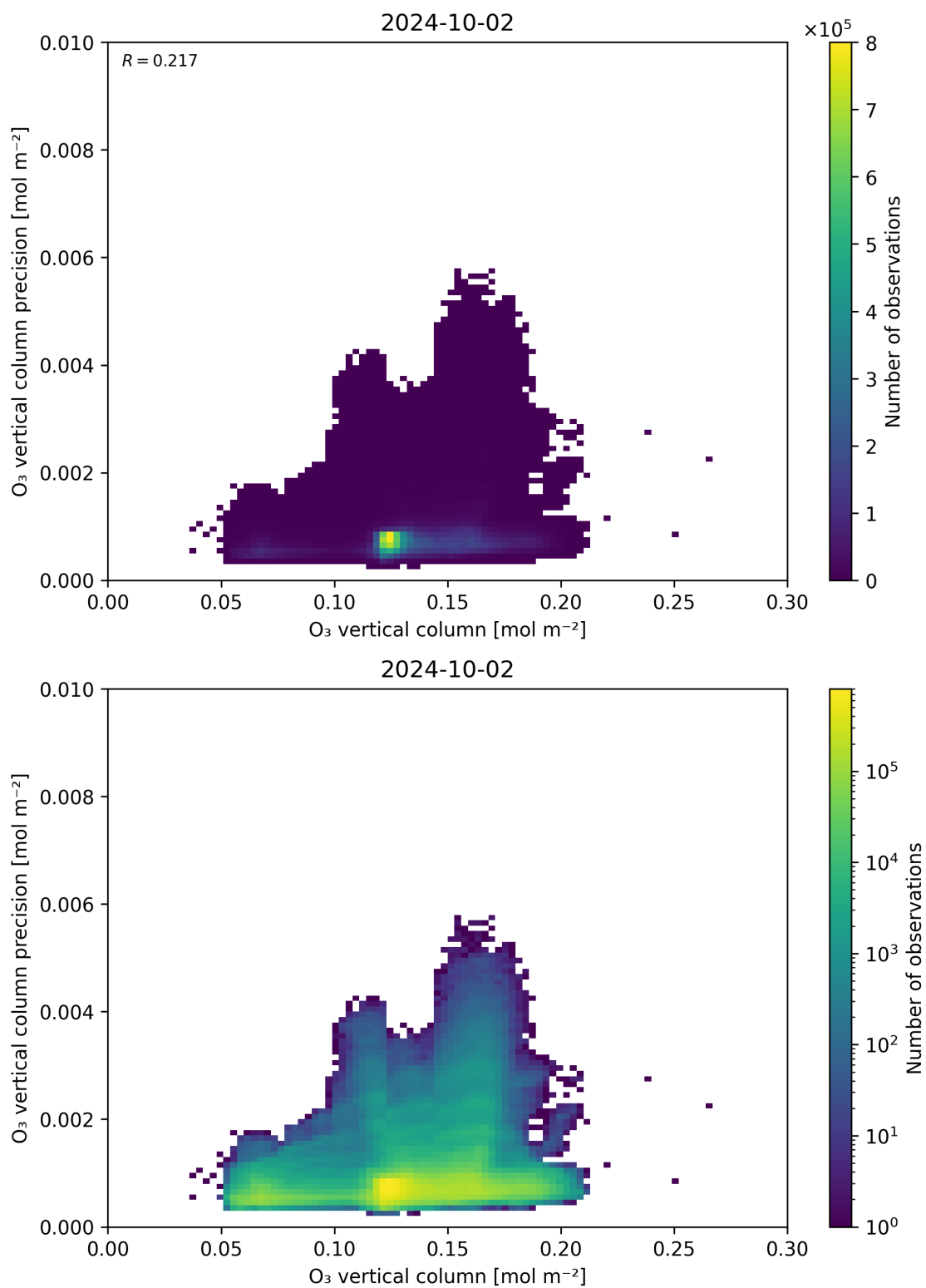
Figure 41: Scatter density plot of “O 3 vertical column” against “O 3 vertical column precision” for 2024-10-01 to 2024-10-03.
