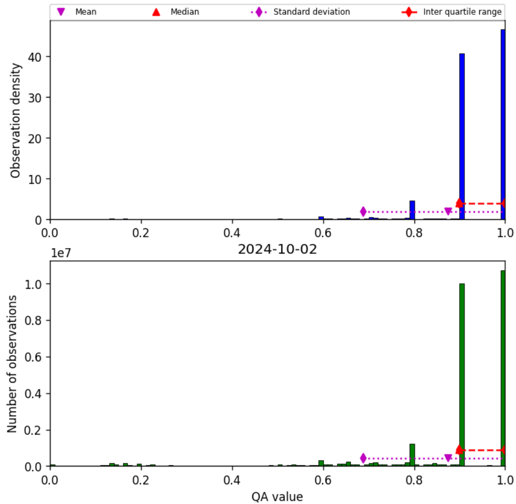
Figure 20: Histogram of “QA value” for 2024-10-01 to 2024-10-03
