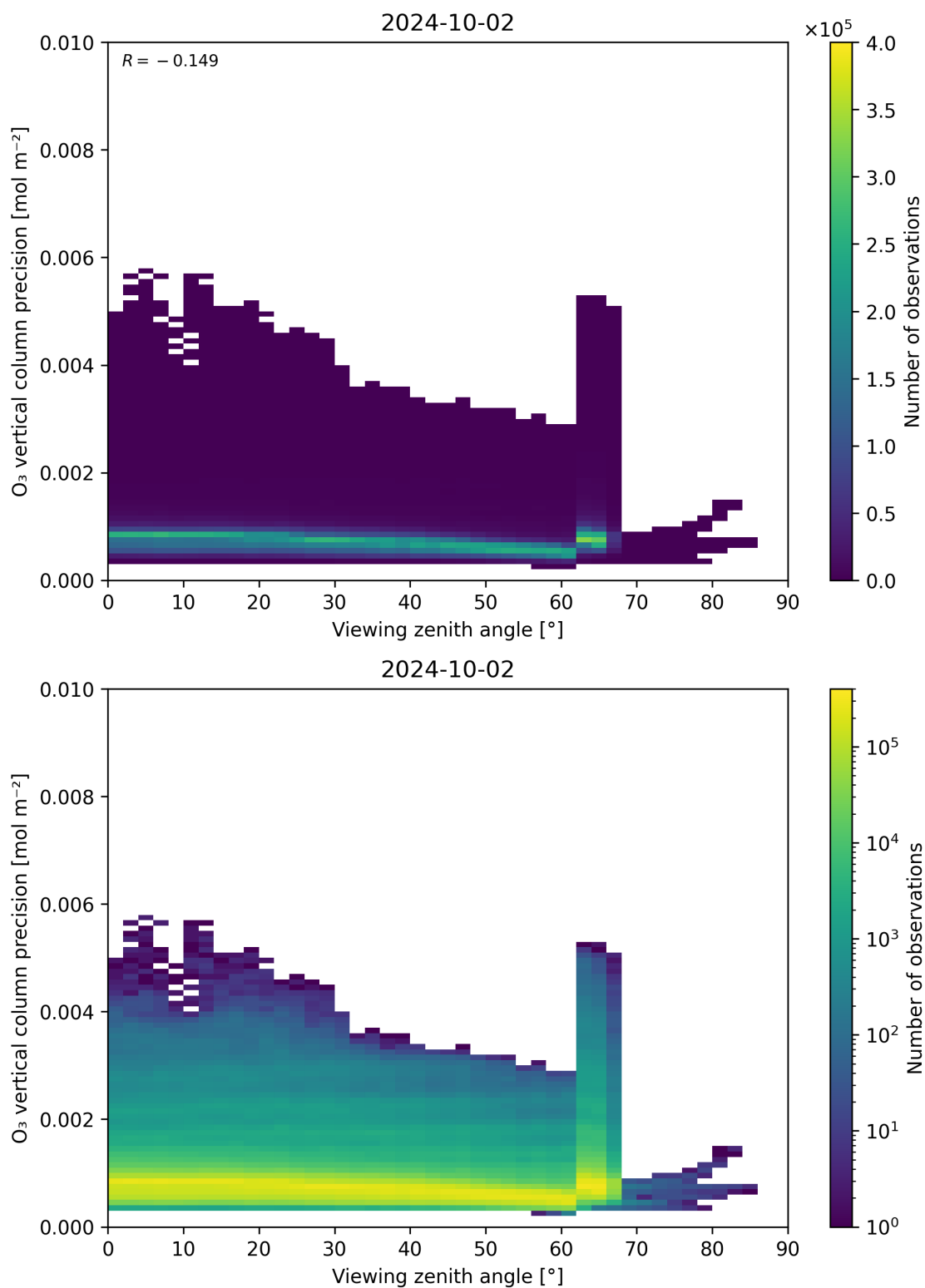
Figure 53: Scatter density plot of “Viewing zenith angle” against “O 3 vertical column precision” for 2024-10-01 to 2024-10-03.
