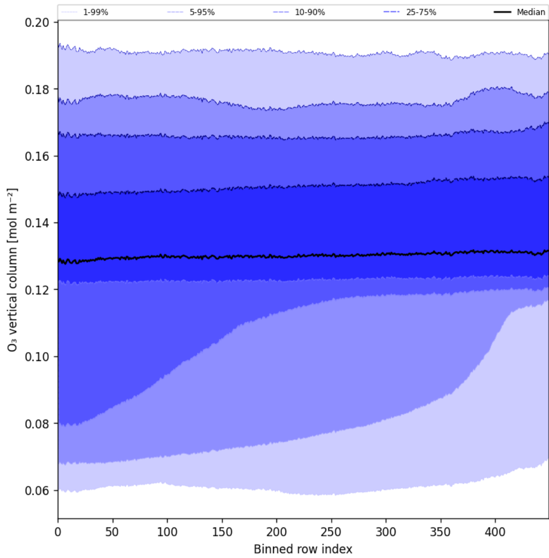
Figure 28: Along track statistics of “O 3 vertical column” for 2024-10-01 to 2024-10-03
