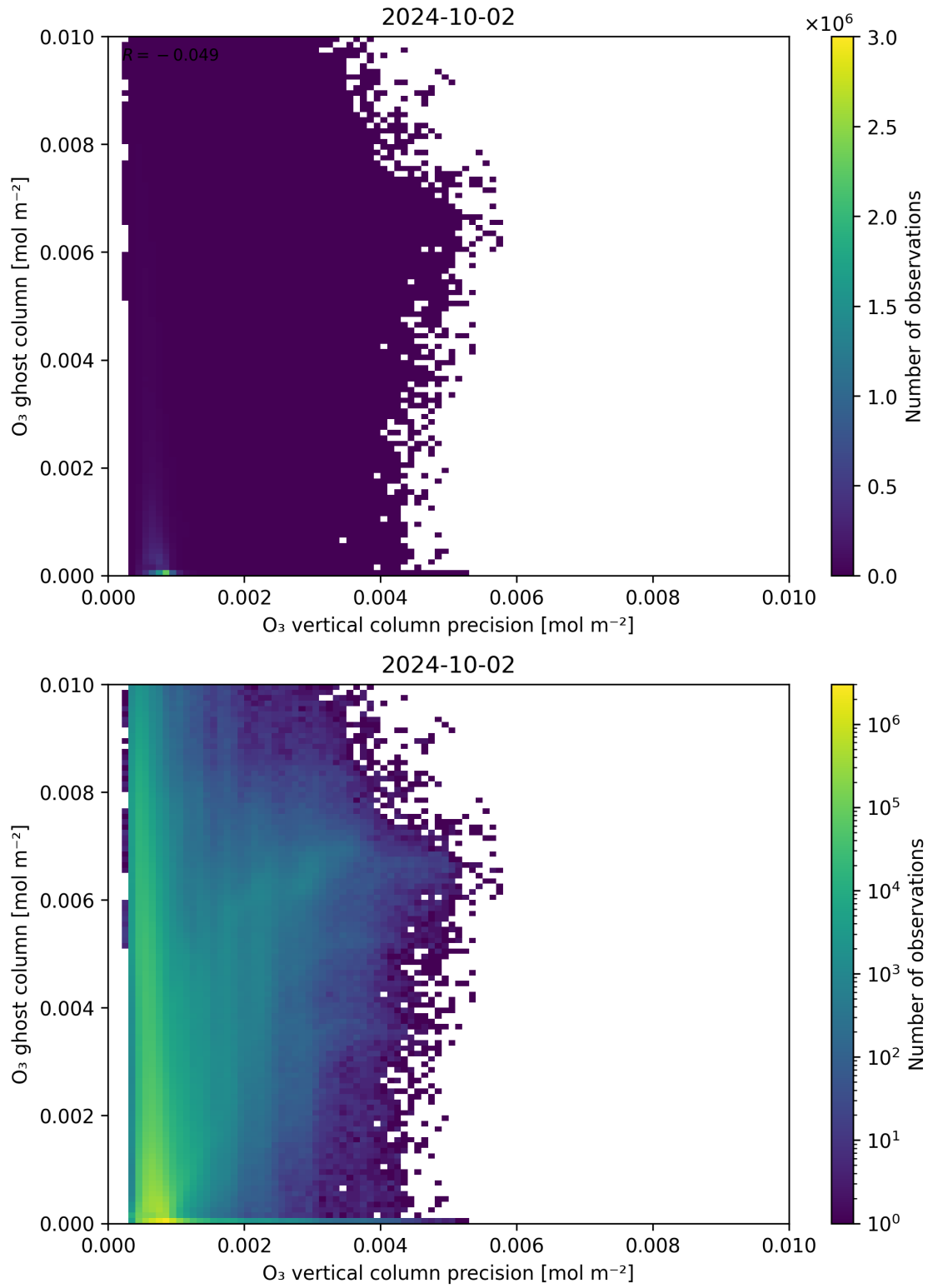
Figure 43: Scatter density plot of “ \text{O}_3 vertical column precision” against “ \text{O}_3 ghost column” for 2024-10-01 to 2024-10-03.
