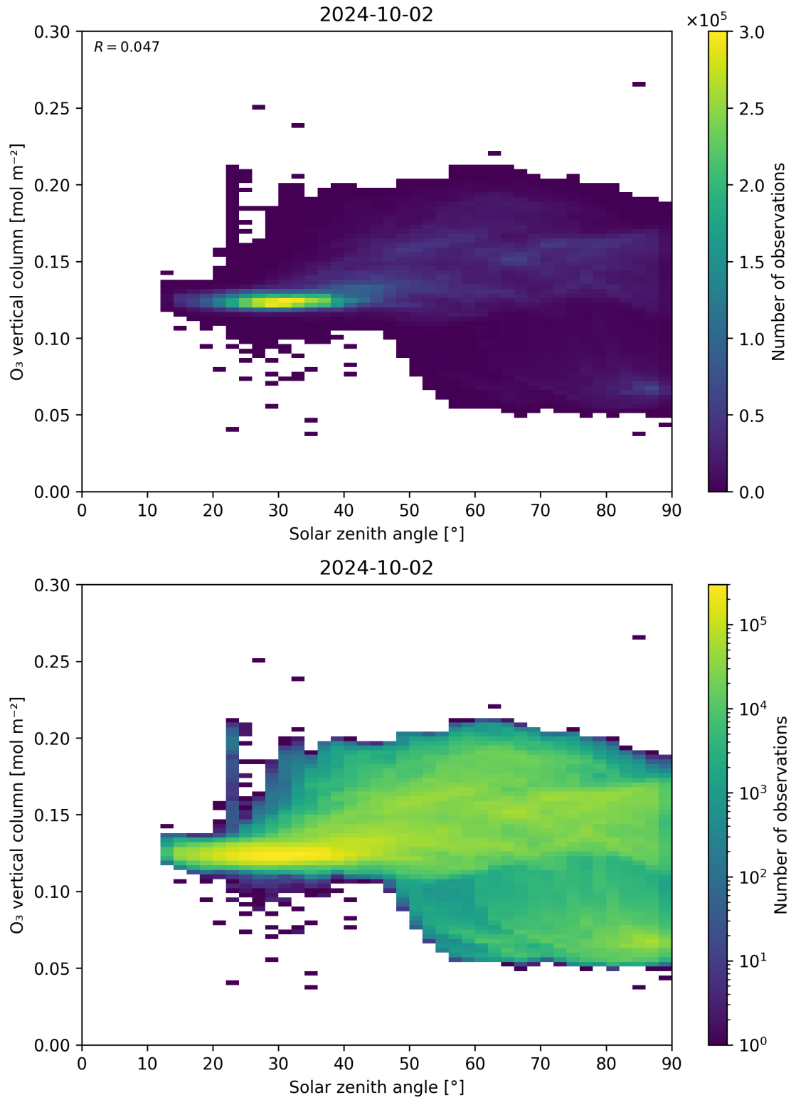
Figure 47: Scatter density plot of “Solar zenith angle” against “O 3 vertical column” for 2024-10-01 to 2024-10-03.
