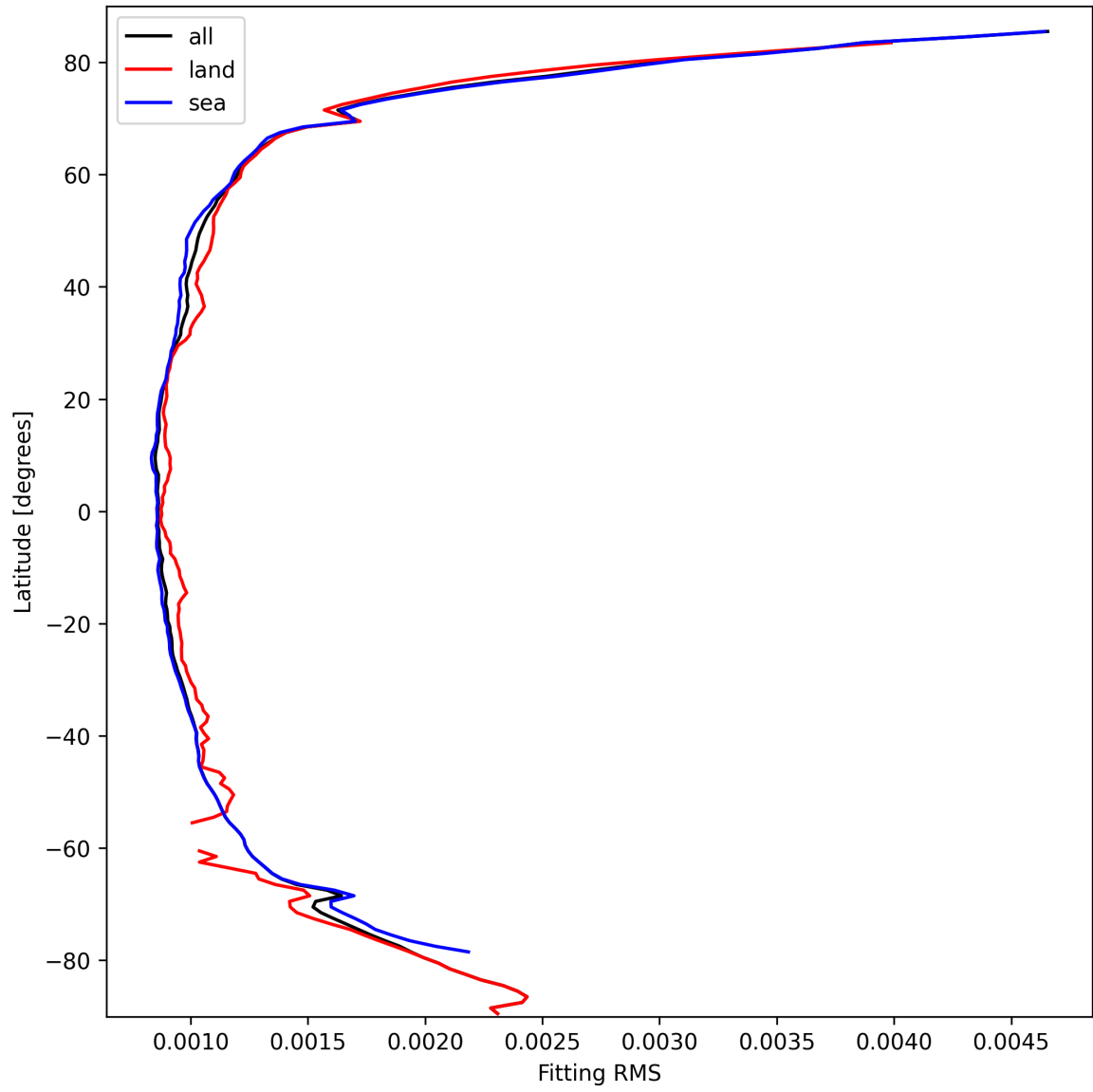
Figure 16: Zonal average of “Fitting RMS” for 2024-10-01 to 2024-10-03.
