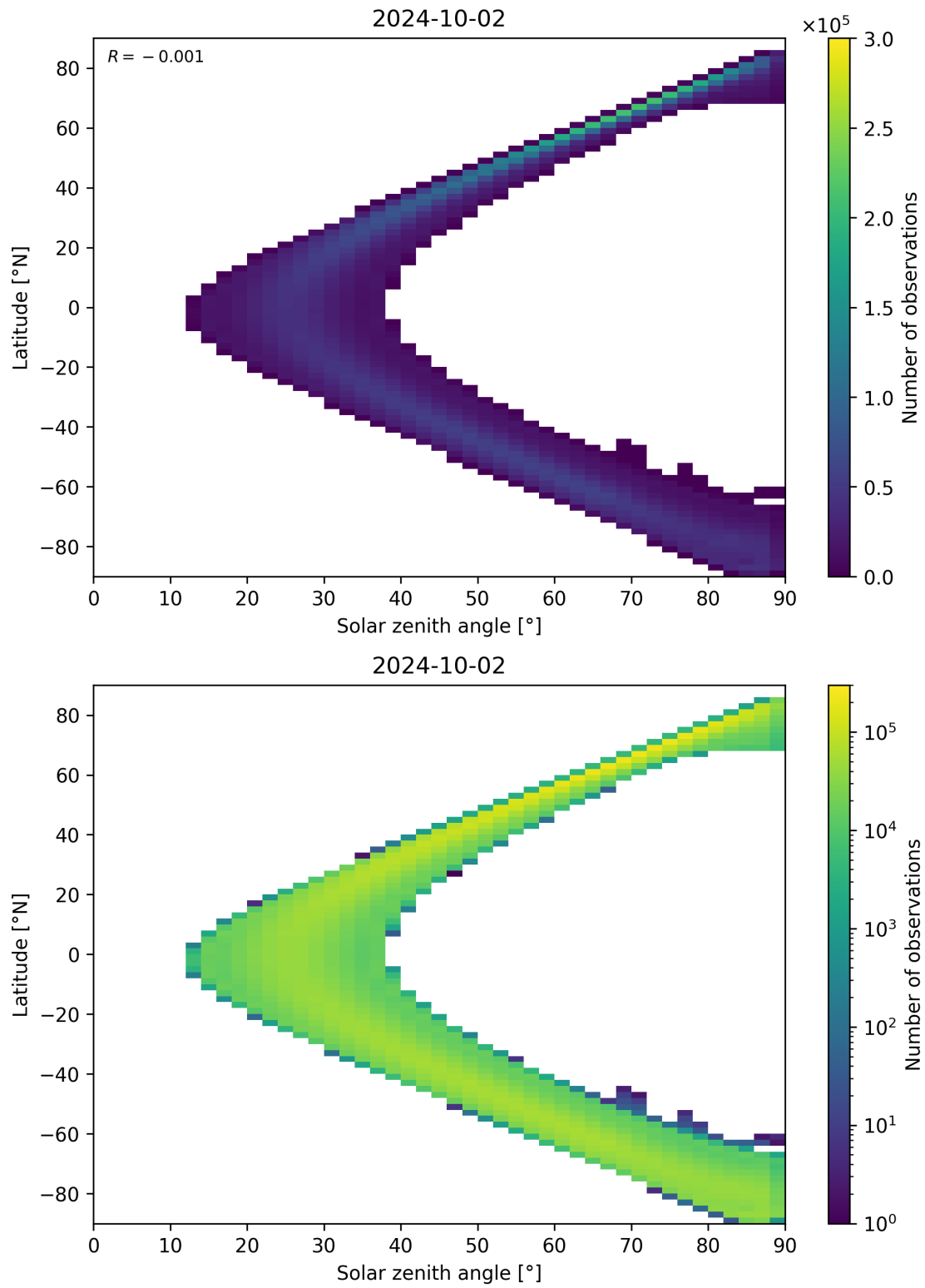
Figure 44: Scatter density plot of “Solar zenith angle” against “Latitude” for 2024-10-01 to 2024-10-03.
