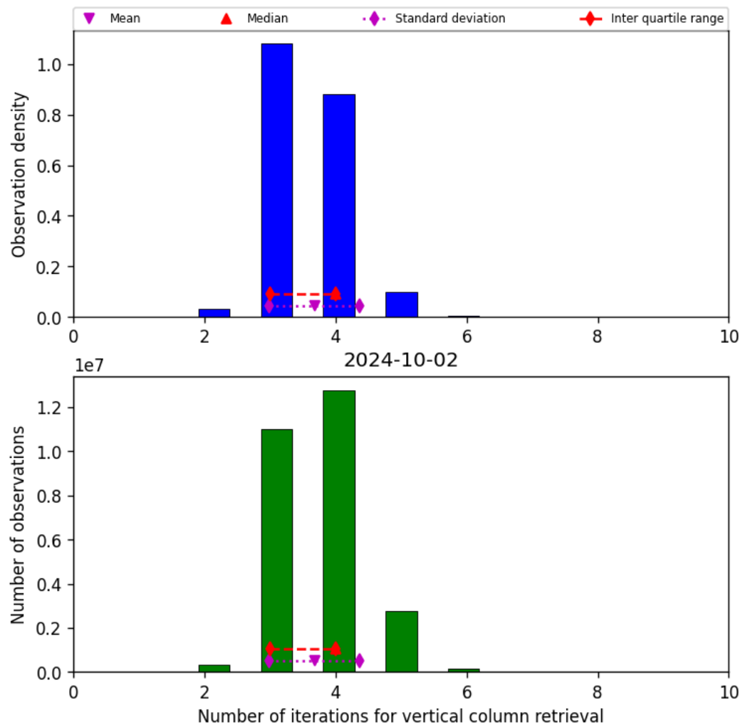
Figure 26: Histogram of “Number of iterations for vertical column retrieval” for 2024-10-01 to 2024-10-03
