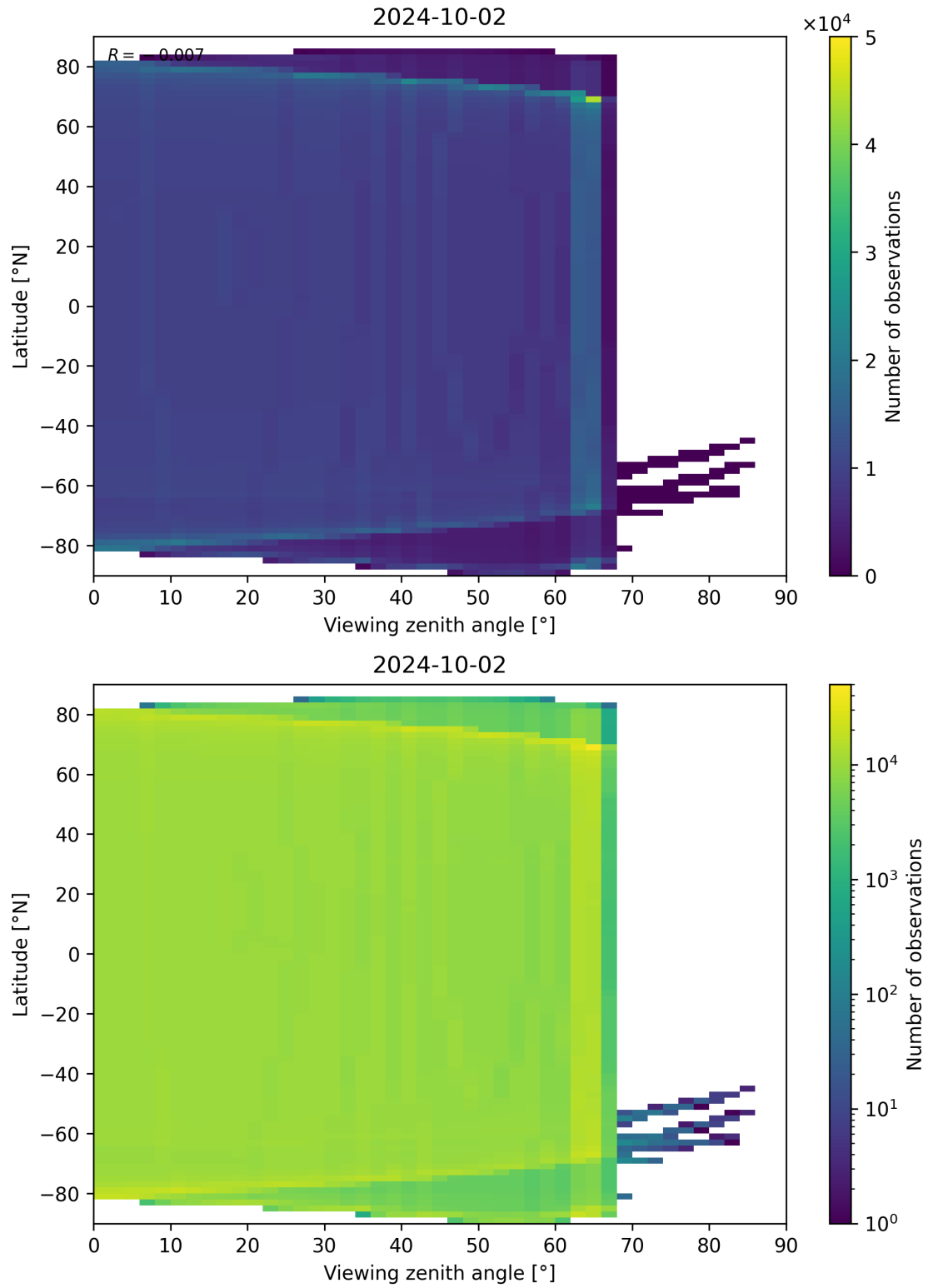
Figure 49: Scatter density plot of “Viewing zenith angle” against “Latitude” for 2024-10-01 to 2024-10-03.
