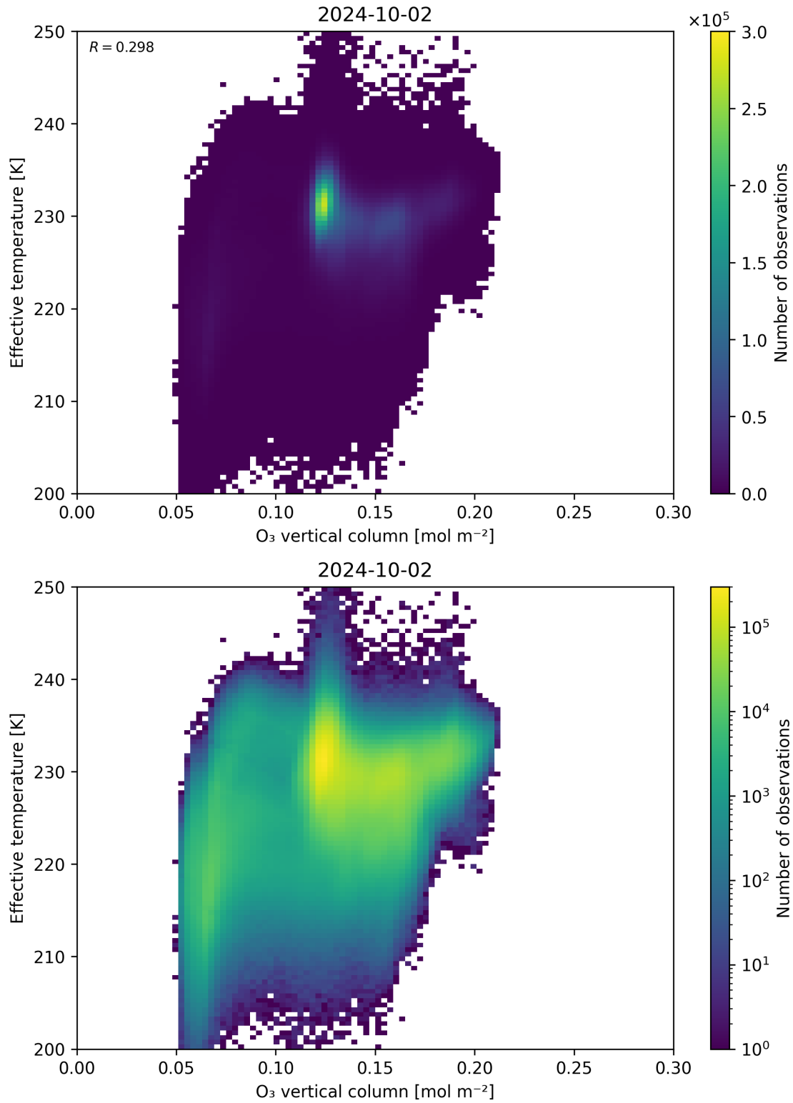
Figure 39: Scatter density plot of “O 3 vertical column” against “Effective temperature” for 2024-10-01 to 2024-10-03.
