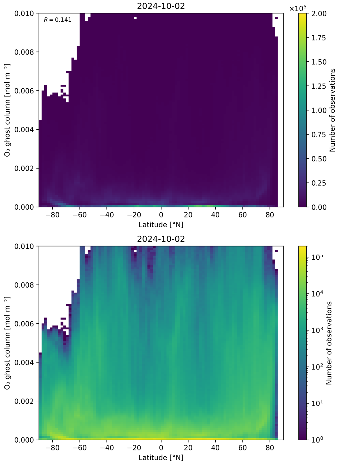
Figure 35: Scatter density plot of “Latitude” against “O 3 ghost column” for 2024-10-01 to 2024-10-03.
