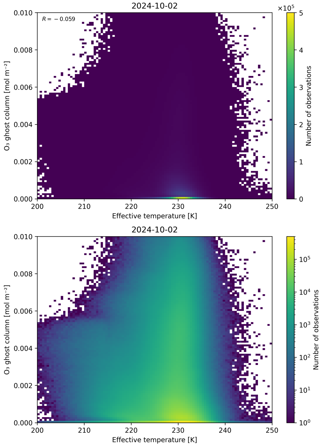
Figure 38: Scatter density plot of “Effective temperature” against “O 3 ghost column” for 2024-10-01 to 2024-10-03.
