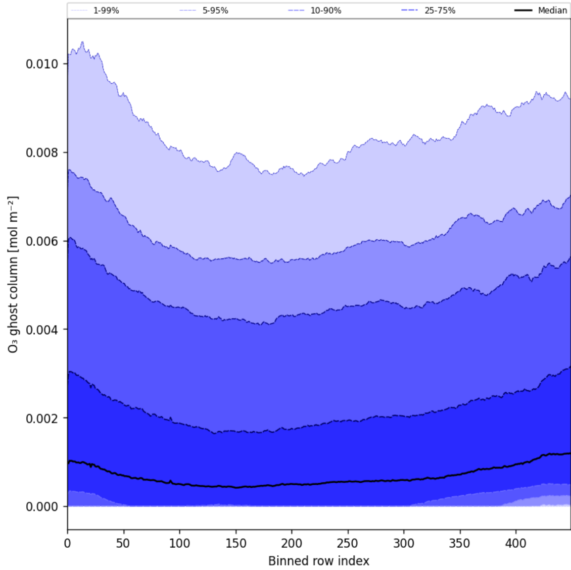
Figure 32: Along track statistics of “O 3 ghost column” for 2024-10-01 to 2024-10-03
