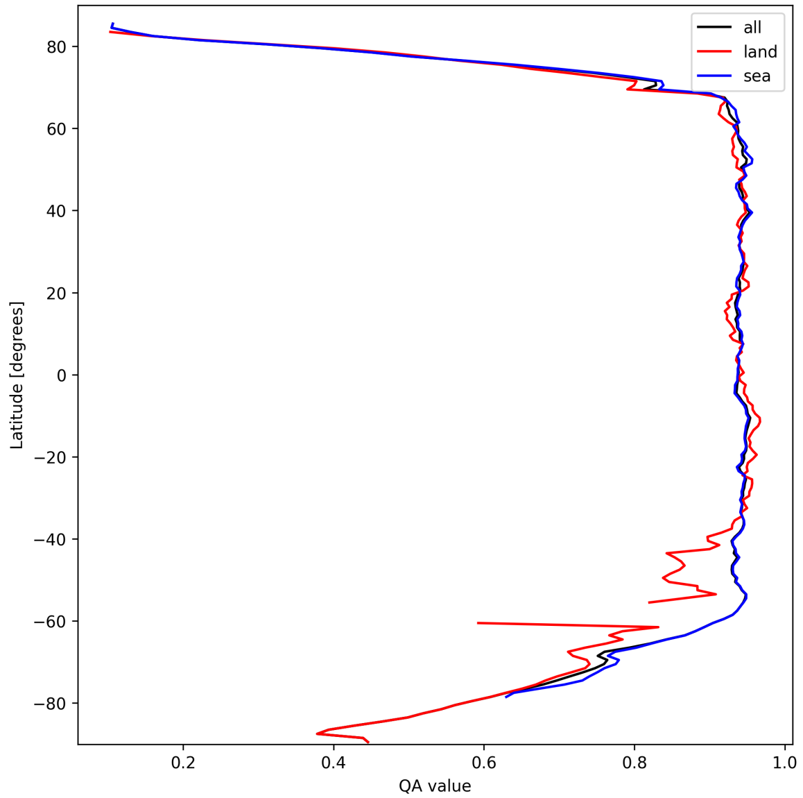
Figure 13: Zonal average of “QA value” for 2024-10-01 to 2024-10-03.
