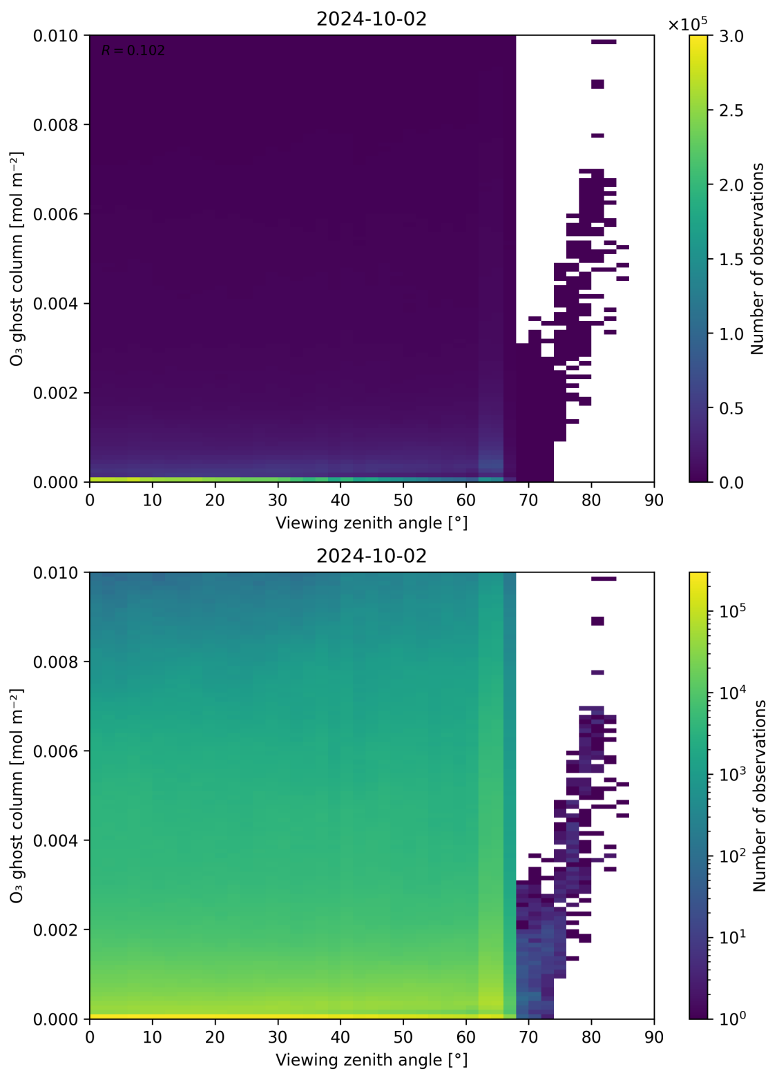
Figure 51: Scatter density plot of “Viewing zenith angle” against “O 3 ghost column” for 2024-10-01 to 2024-10-03.
