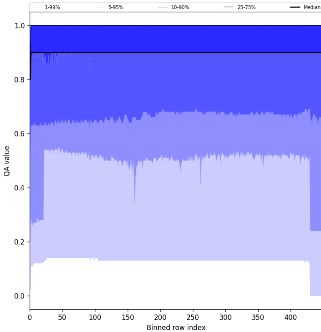
Figure 27: Along track statistics of “QA value” for 2024-10-01 to 2024-10-03
