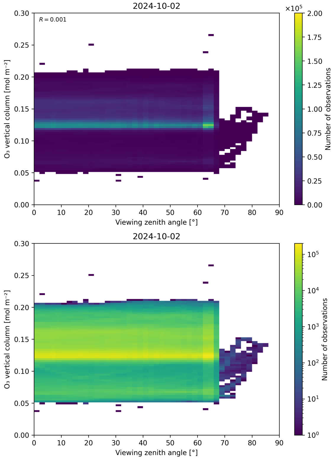
Figure 52: Scatter density plot of “Viewing zenith angle” against “O 3 vertical column” for 2024-10-01 to 2024-10-03.
