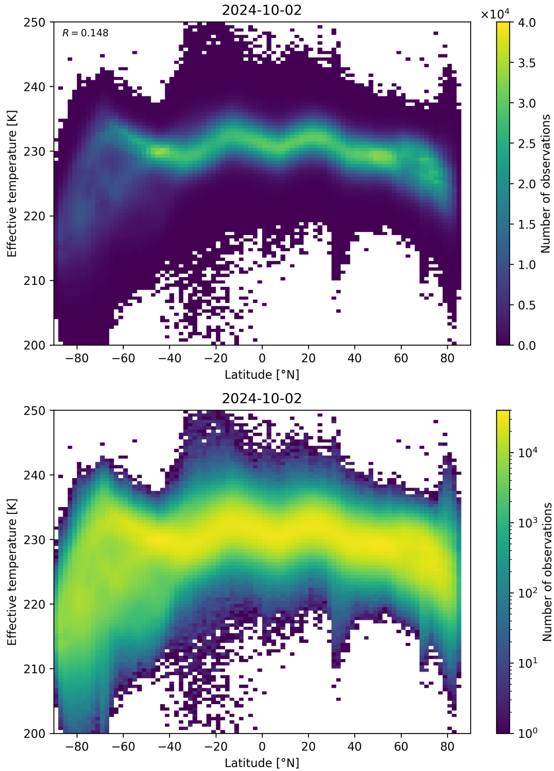
Figure 34: Scatter density plot of “Latitude” against “Effective temperature” for 2024-10-01 to 2024-10-03.
