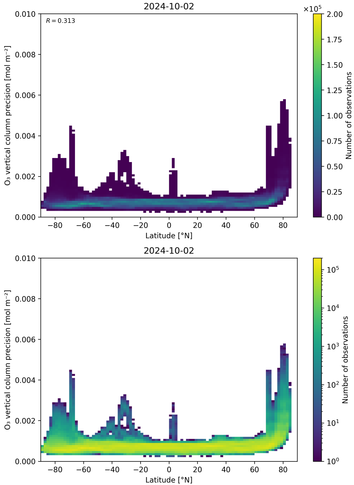
Figure 37: Scatter density plot of “Latitude” against “O 3 vertical column precision” for 2024-10-01 to 2024-10-03.
