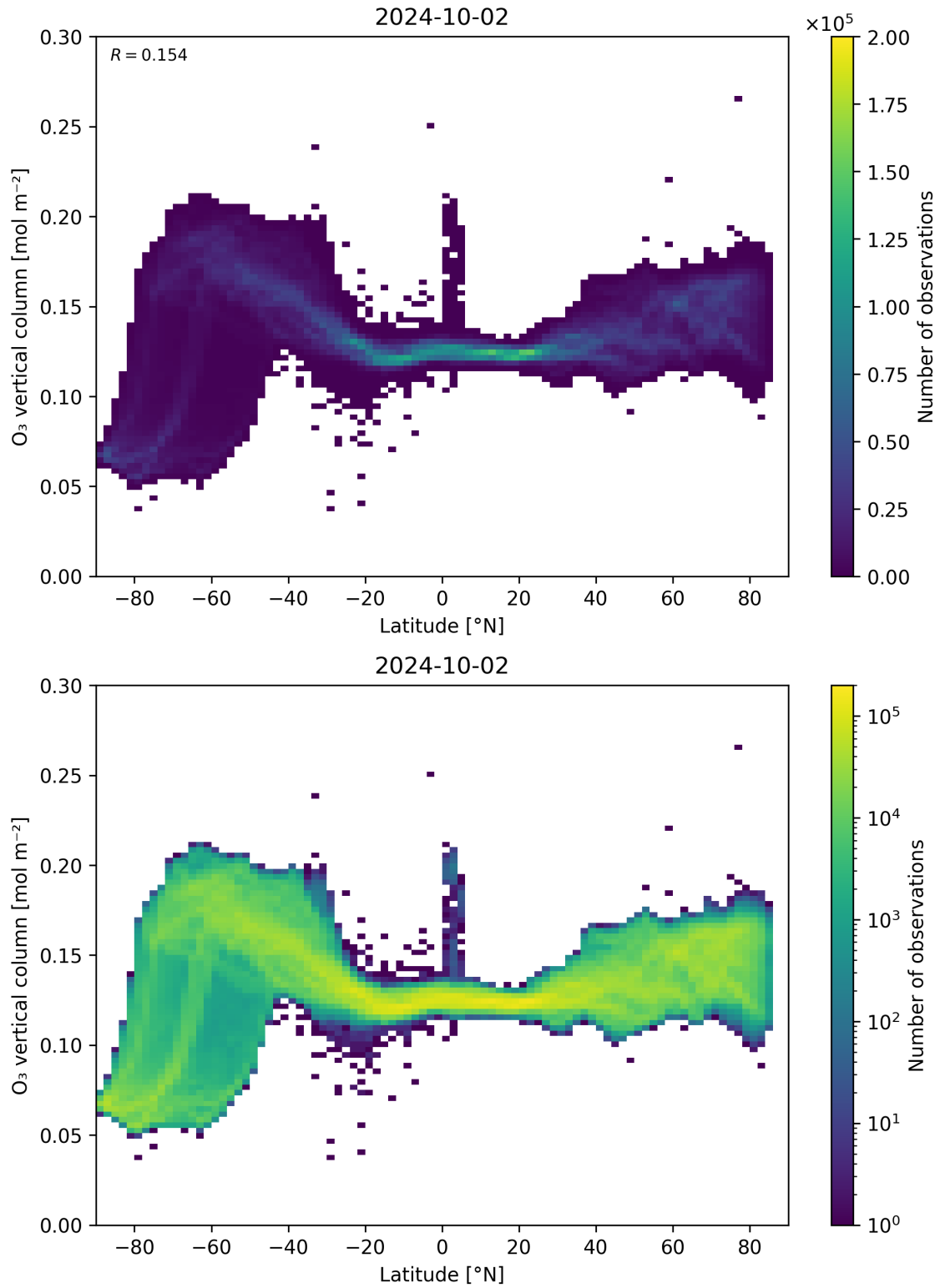
Figure 36: Scatter density plot of “Latitude” against “O 3 vertical column” for 2024-10-01 to 2024-10-03.
