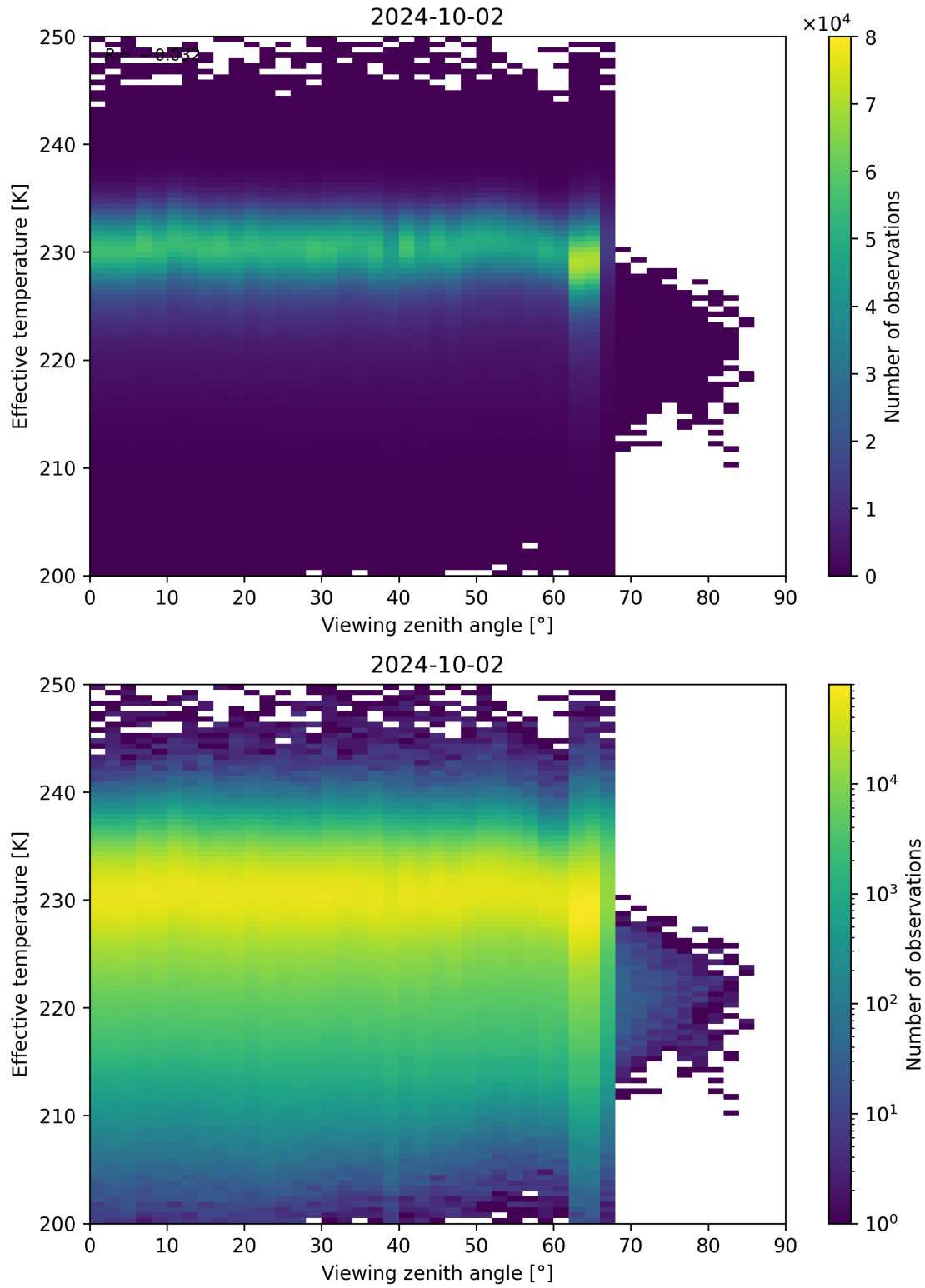
Figure 50: Scatter density plot of “Viewing zenith angle” against “Effective temperature” for 2024-10-01 to 2024-10-03.
