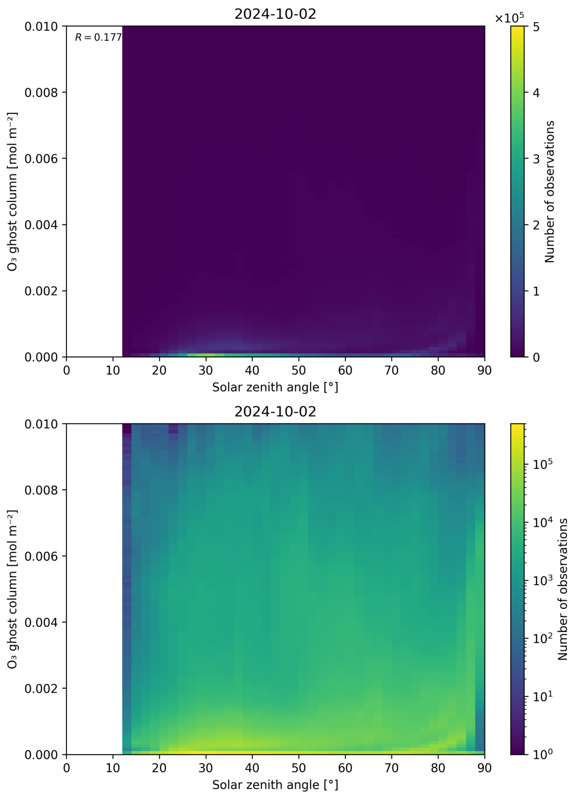
Figure 46: Scatter density plot of “Solar zenith angle” against “O 3 ghost column” for 2024-10-01 to 2024-10-03.
