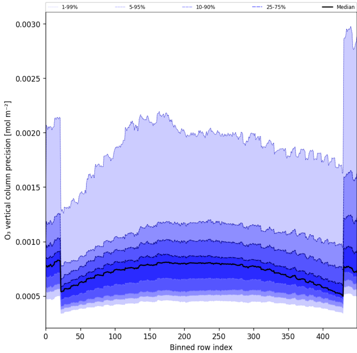
Figure 29: Along track statistics of “O 3 vertical column precision” for 2024-10-01 to 2024-10-03
