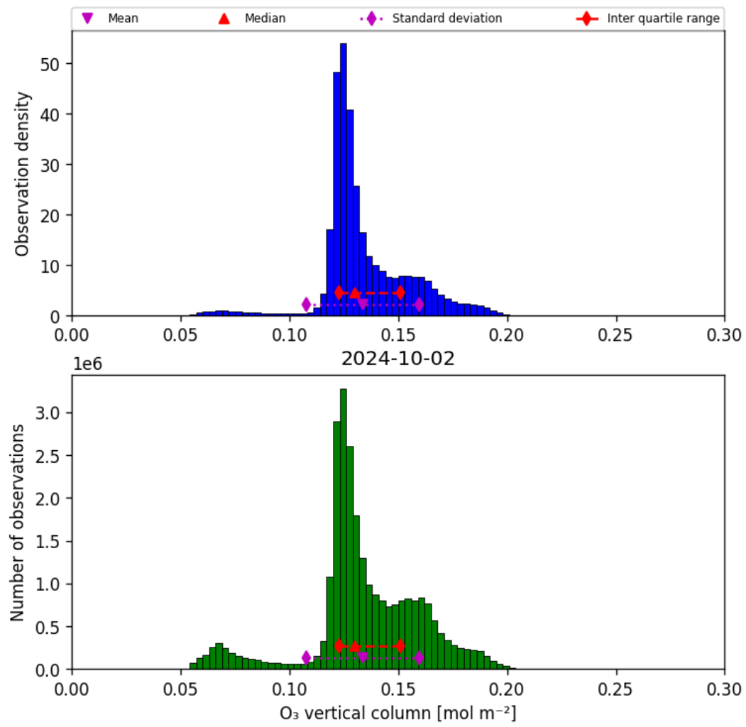
Figure 21: Histogram of “O 3 vertical column” for 2024-10-01 to 2024-10-03
