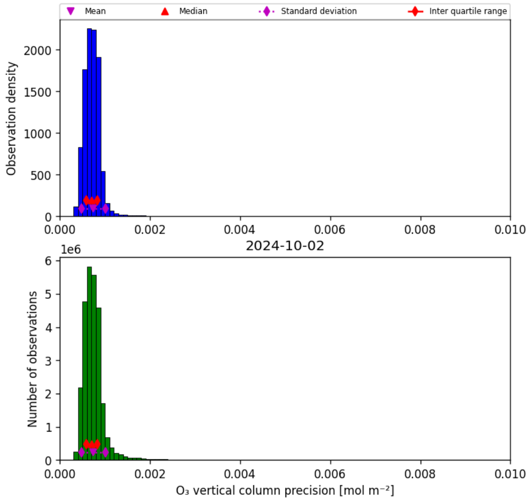
Figure 22: Histogram of “O 3 vertical column precision” for 2024-10-01 to 2024-10-03
