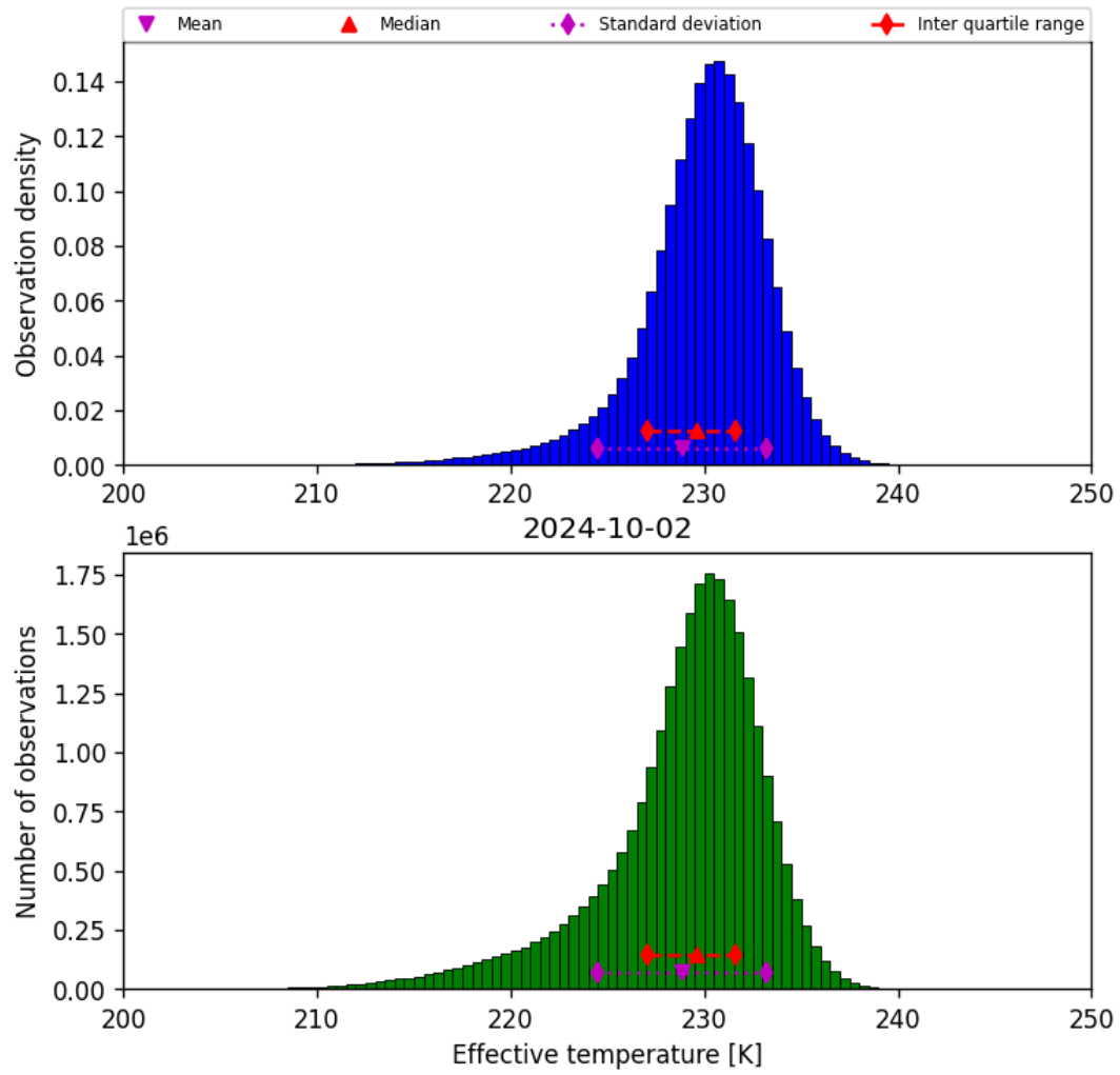
Figure 24: Histogram of “Effective temperature” for 2024-10-01 to 2024-10-03
