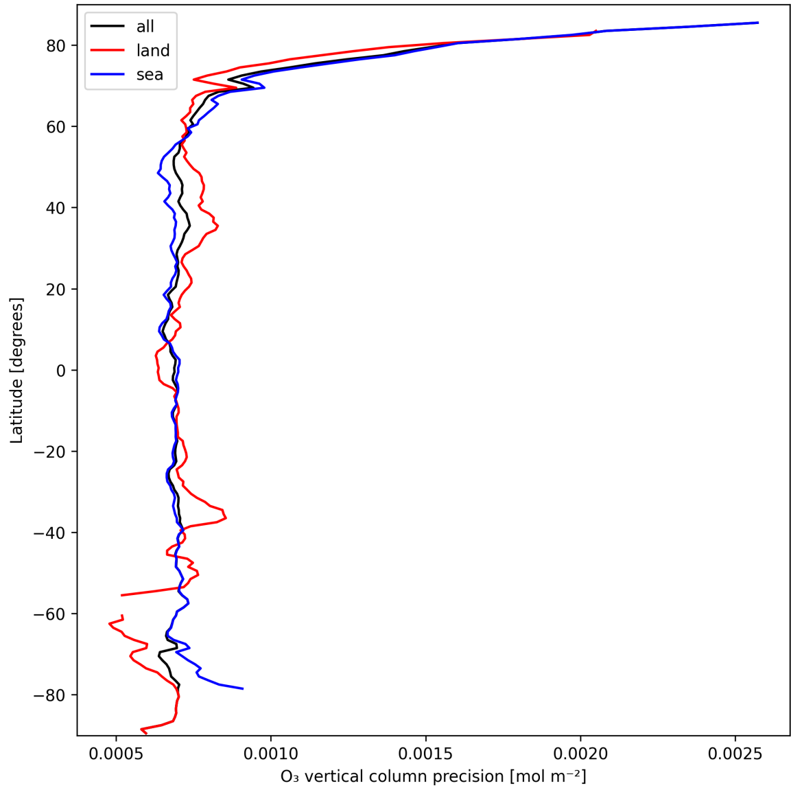
Figure 15: Zonal average of “O 3 vertical column precision” for 2024-10-01 to 2024-10-03.
