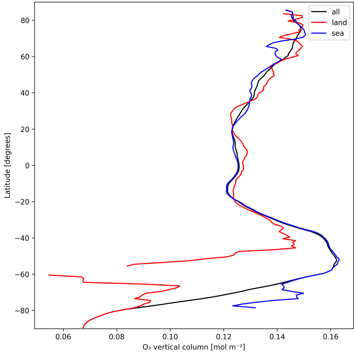
Figure 14: Zonal average of “O 3 vertical column” for 2024-10-01 to 2024-10-03.
