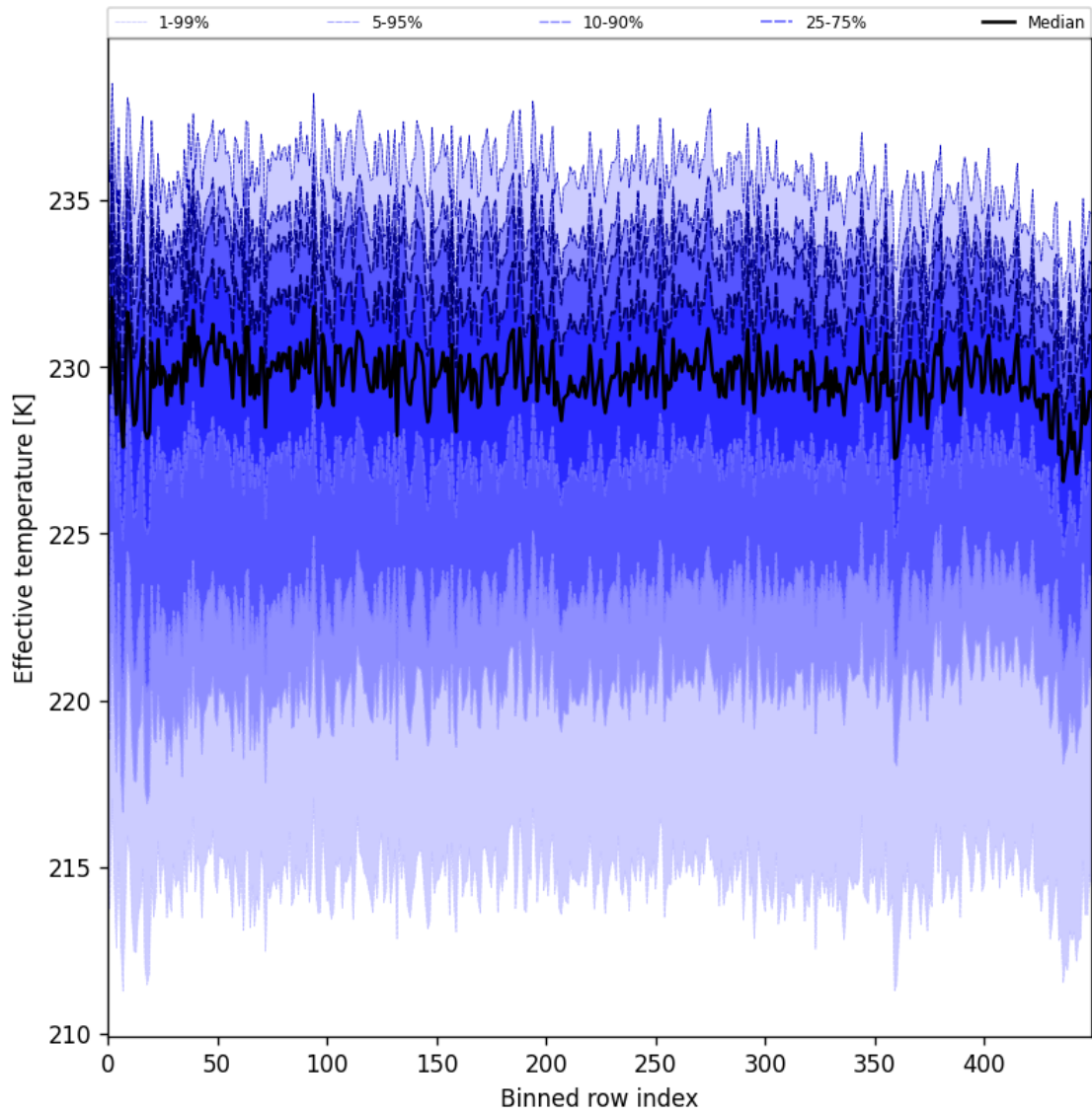
Figure 31: Along track statistics of “Effective temperature” for 2024-10-01 to 2024-10-03
