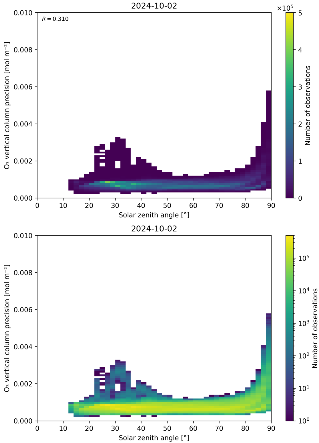
Figure 48: Scatter density plot of “Solar zenith angle” against “O 3 vertical column precision” for 2024-10-01 to 2024-10-03.
