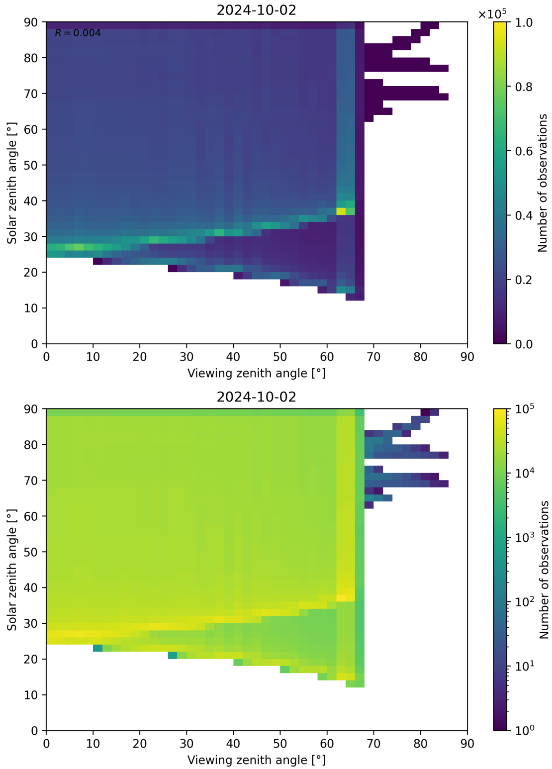
Figure 54: Scatter density plot of “Viewing zenith angle” against “Solar zenith angle” for 2024-10-01 to 2024-10-03.
