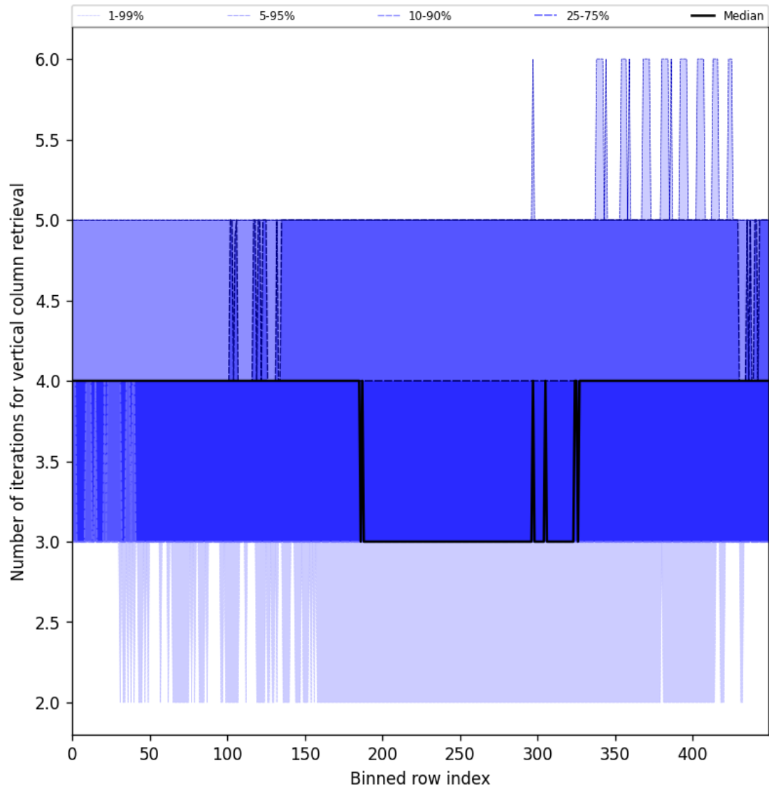
Figure 33: Along track statistics of “Number of iterations for vertical column retrieval” for 2024-10-01 to 2024-10-03
