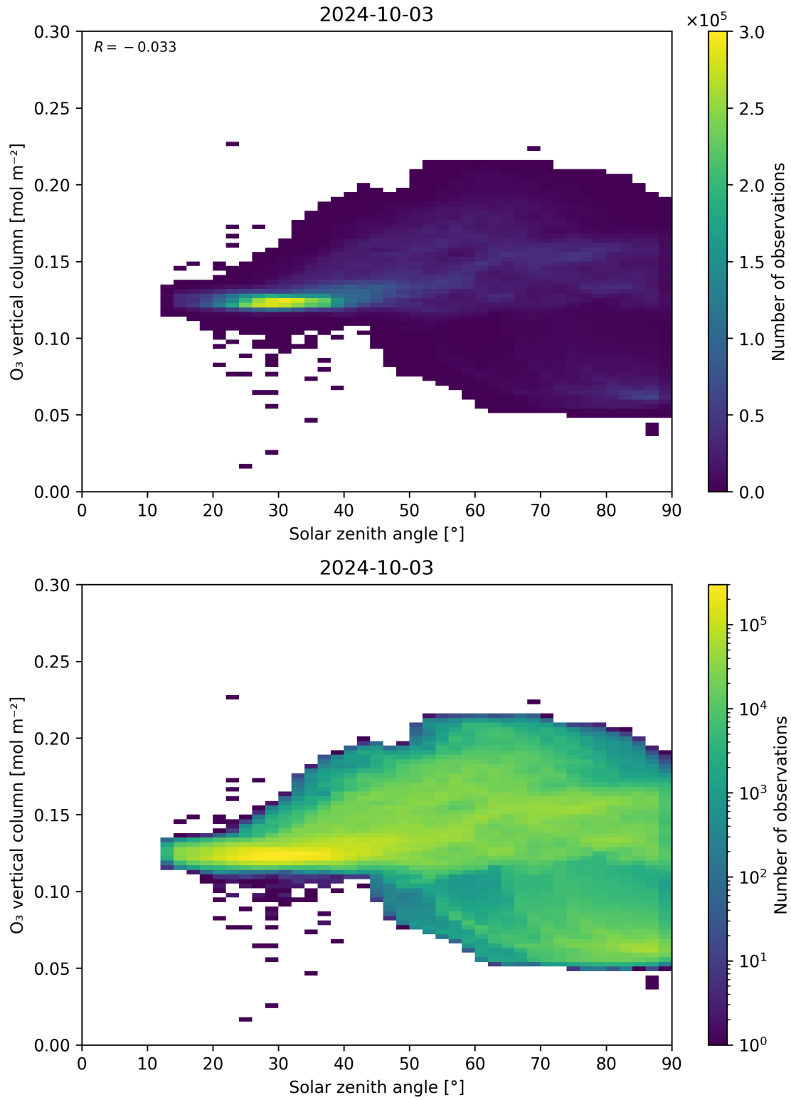
Figure 47: Scatter density plot of “Solar zenith angle” against “O 3 vertical column” for 2024-10-03 to 2024-10-04.
