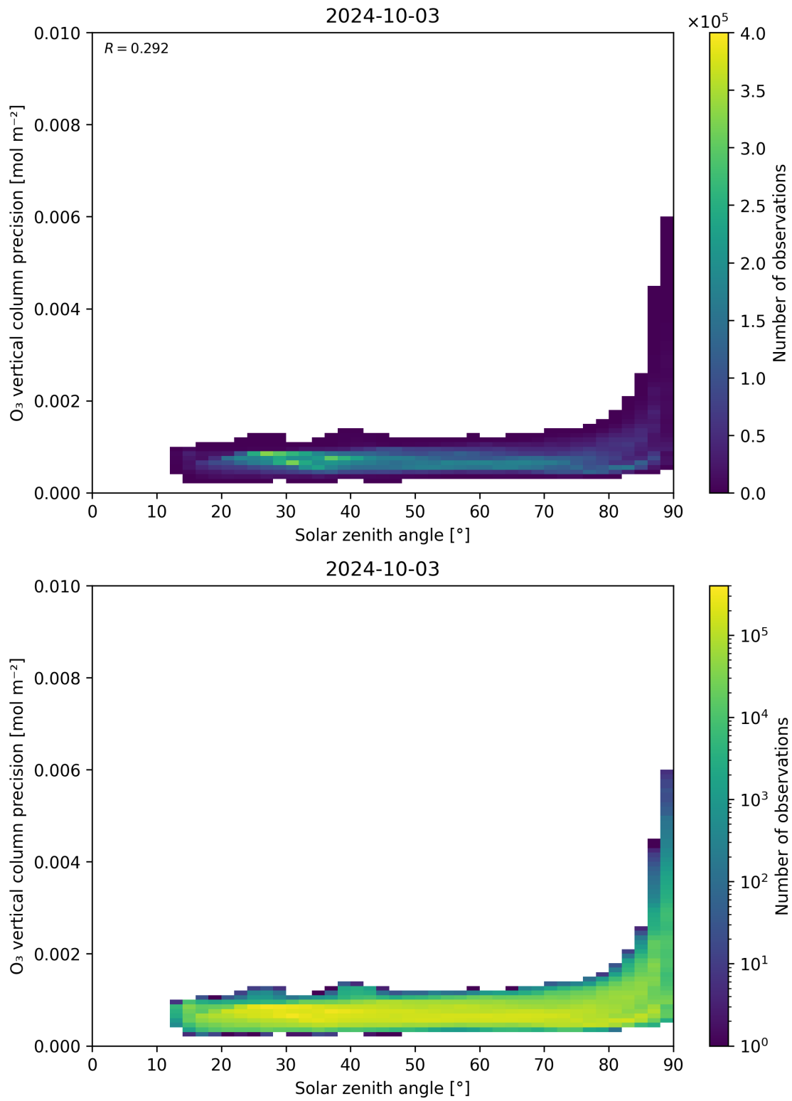
Figure 48: Scatter density plot of “Solar zenith angle” against “O 3 vertical column precision” for 2024-10-03 to 2024-10-04.
