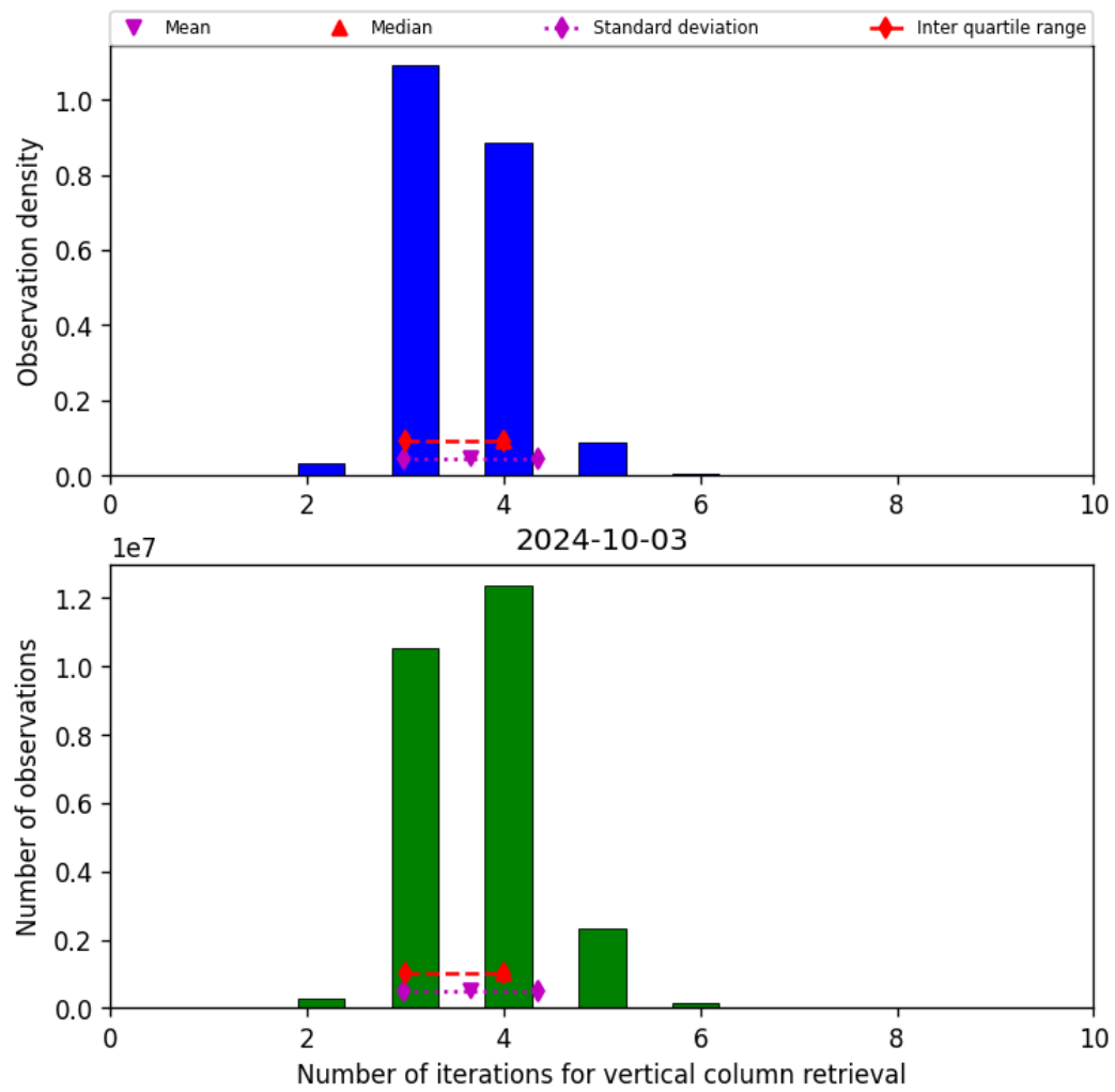
Figure 26: Histogram of "Number of iterations for vertical column retrieval" for 2024-10-03 to 2024-10-04
