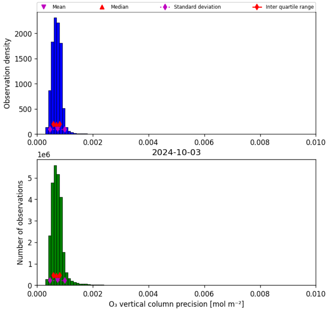
Figure 22: Histogram of “O 3 vertical column precision” for 2024-10-03 to 2024-10-04
