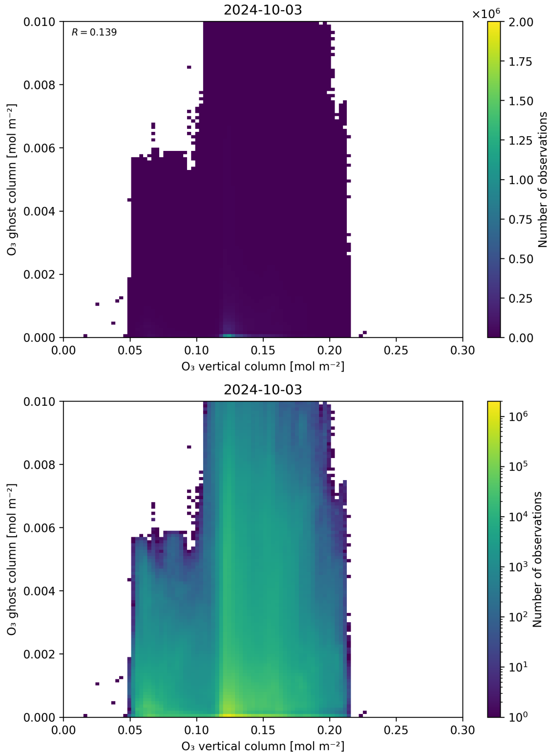
Figure 40: Scatter density plot of “O 3 vertical column” against “O 3 ghost column” for 2024-10-03 to 2024-10-04.
