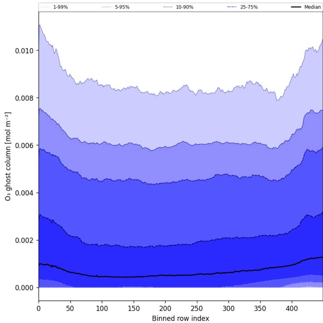
Figure 32: Along track statistics of “O 3 ghost column” for 2024-10-03 to 2024-10-04
