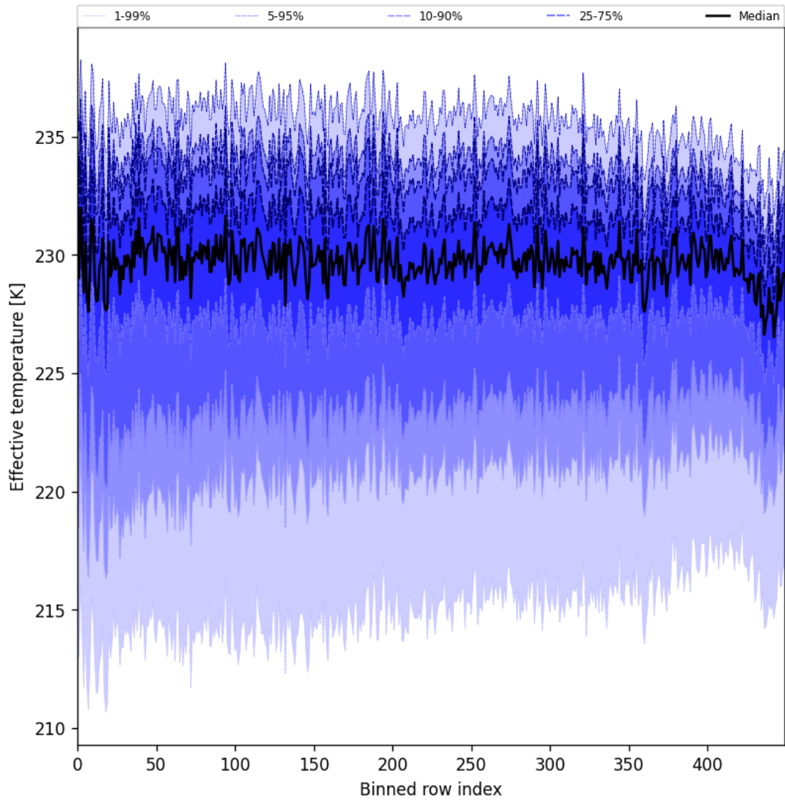
Figure 31: Along track statistics of “Effective temperature” for 2024-10-03 to 2024-10-04
