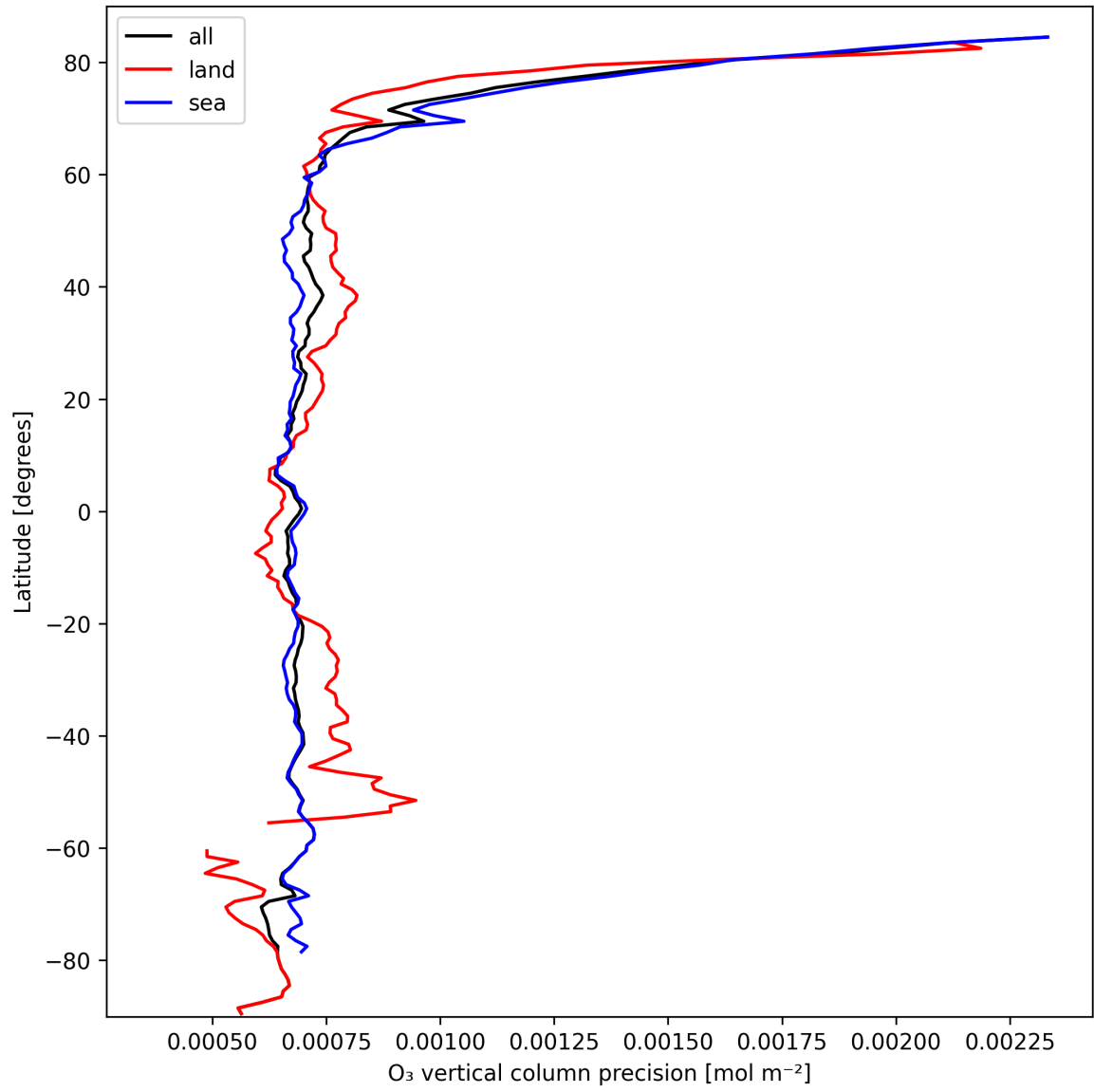
Figure 15: Zonal average of "O 3 vertical column precision" for 2024-10-03 to 2024-10-04.
