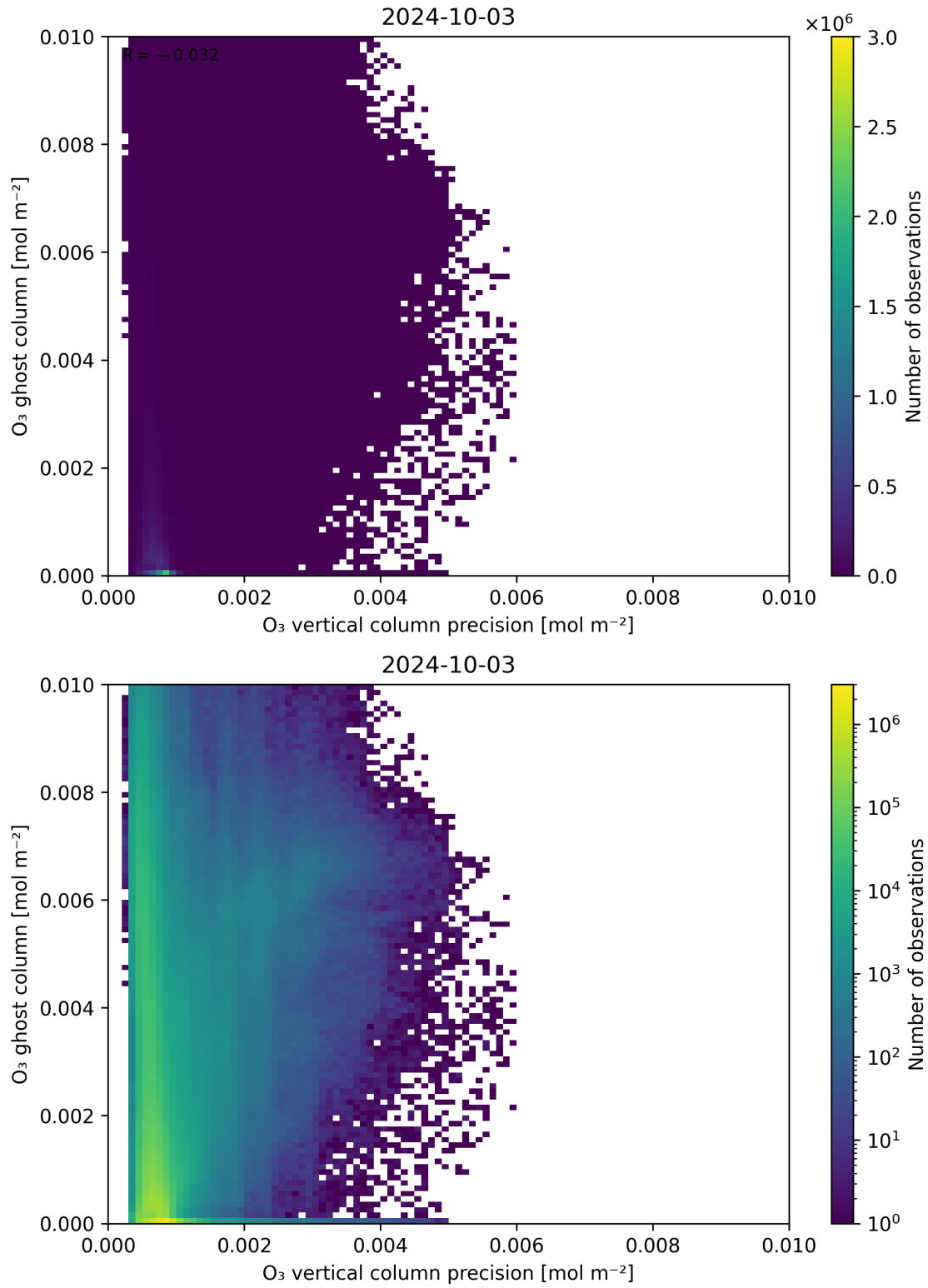
Figure 43: Scatter density plot of “ \text{O}_3 vertical column precision” against “ \text{O}_3 ghost column” for 2024-10-03 to 2024-10-04.
