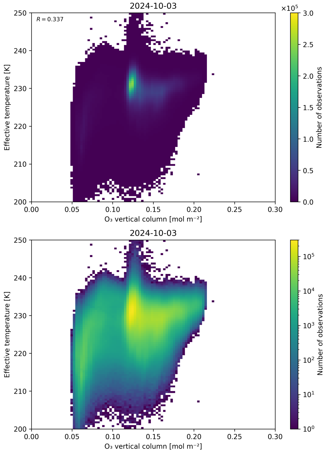
Figure 39: Scatter density plot of “O 3 vertical column” against “Effective temperature” for 2024-10-03 to 2024-10-04.
