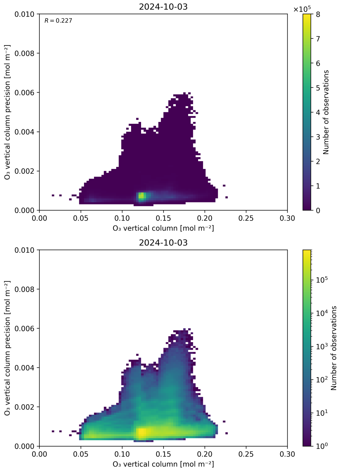
Figure 41: Scatter density plot of “O 3 vertical column” against “O 3 vertical column precision” for 2024-10-03 to 2024-10-04.
