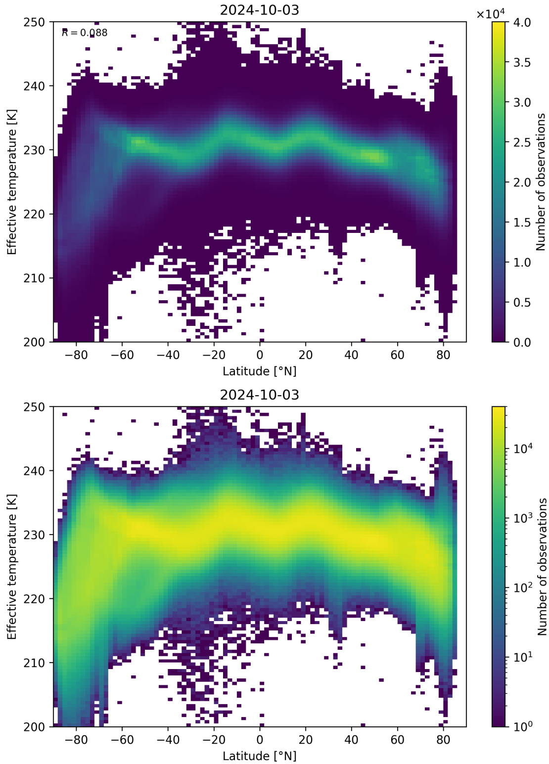
Figure 34: Scatter density plot of “Latitude” against “Effective temperature” for 2024-10-03 to 2024-10-04.
