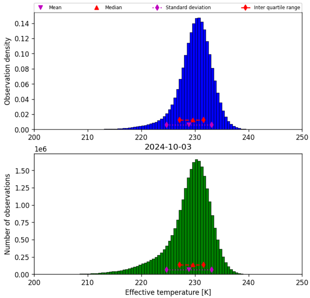
Figure 24: Histogram of “Effective temperature” for 2024-10-03 to 2024-10-04
