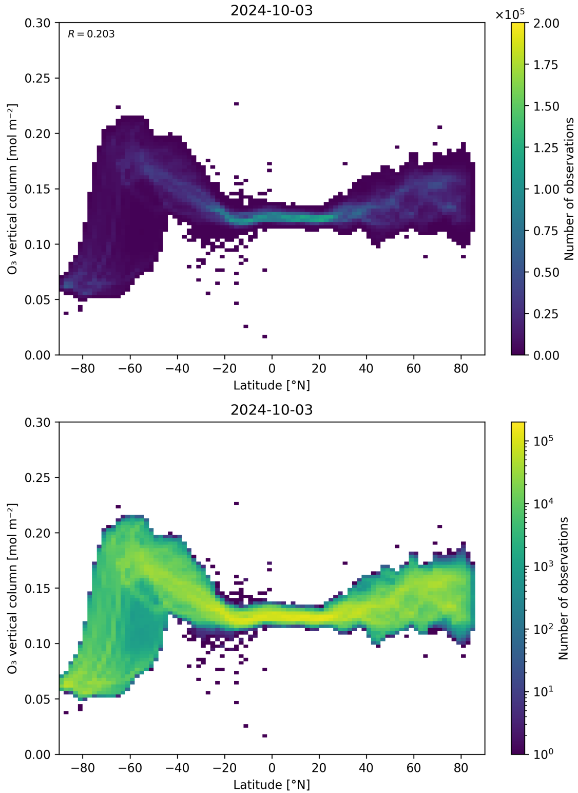
Figure 36: Scatter density plot of “Latitude” against “O 3 vertical column” for 2024-10-03 to 2024-10-04.
