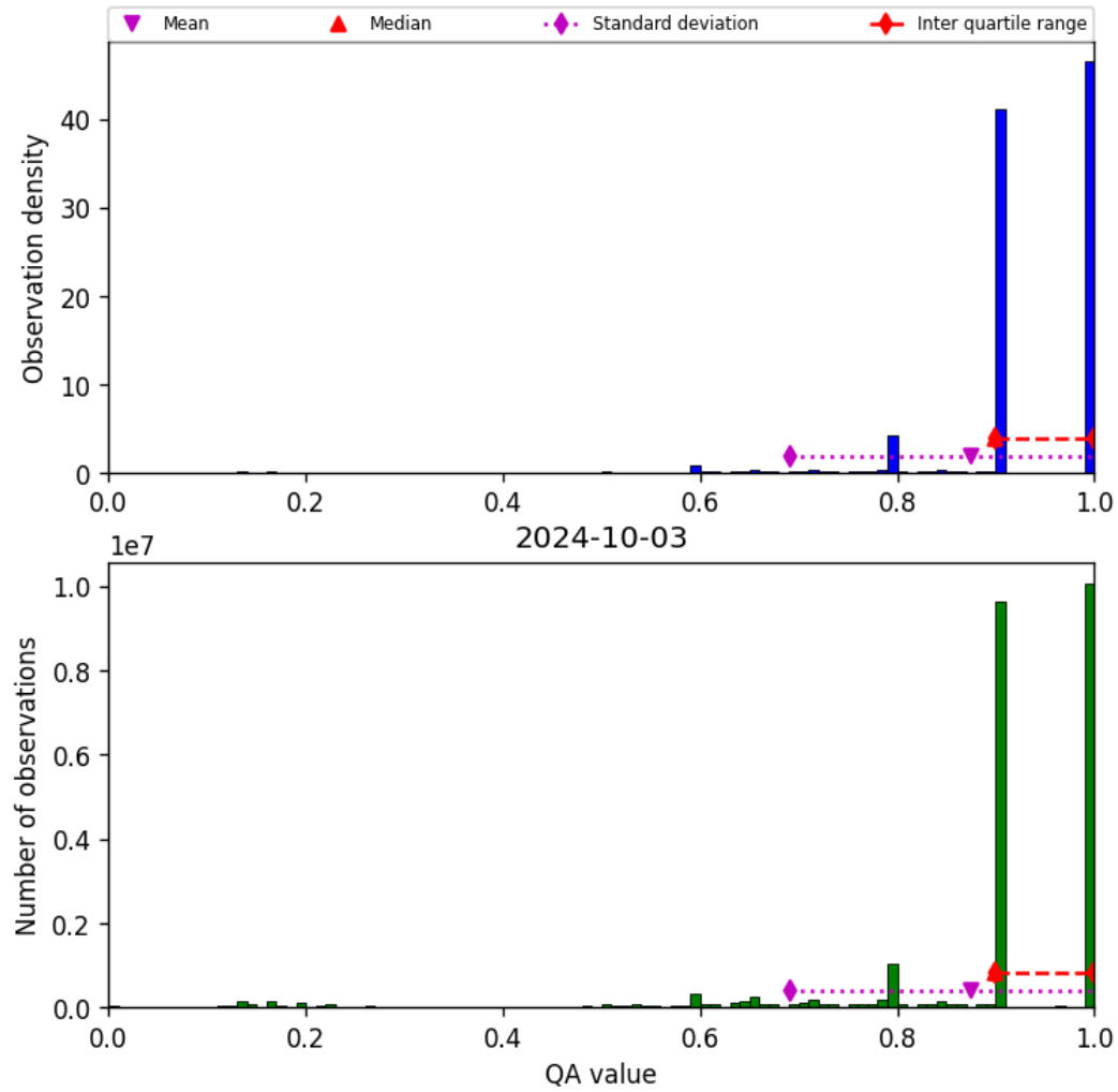
Figure 20: Histogram of “QA value” for 2024-10-03 to 2024-10-04
