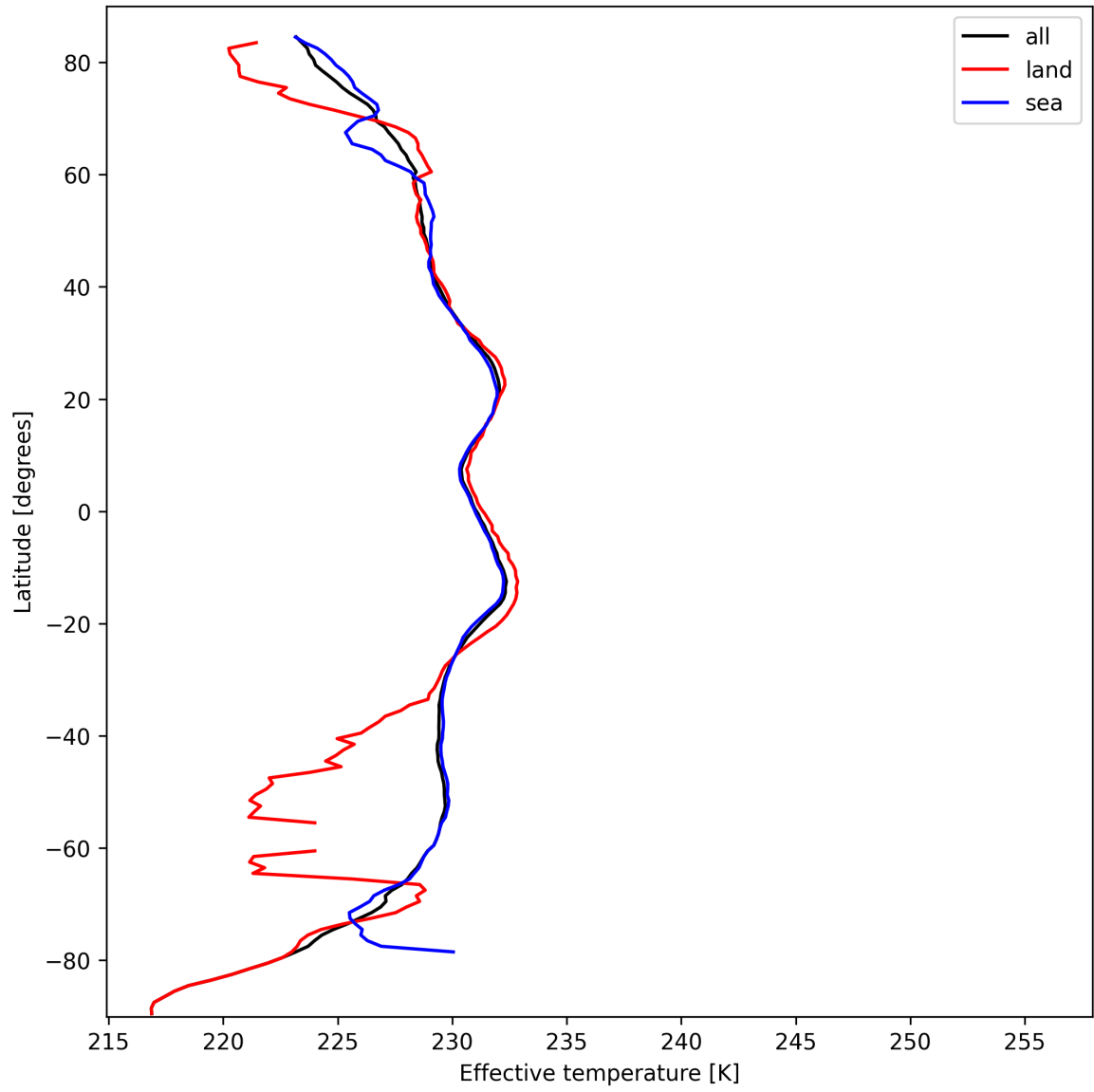
Figure 17: Zonal average of "Effective temperature" for 2024-10-03 to 2024-10-04.
