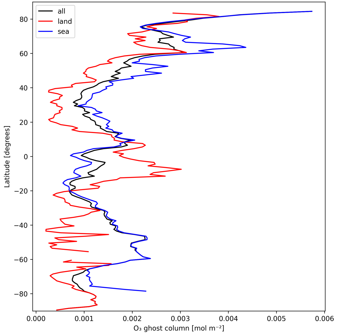
Figure 18: Zonal average of "O 3 ghost column" for 2024-10-03 to 2024-10-04.
