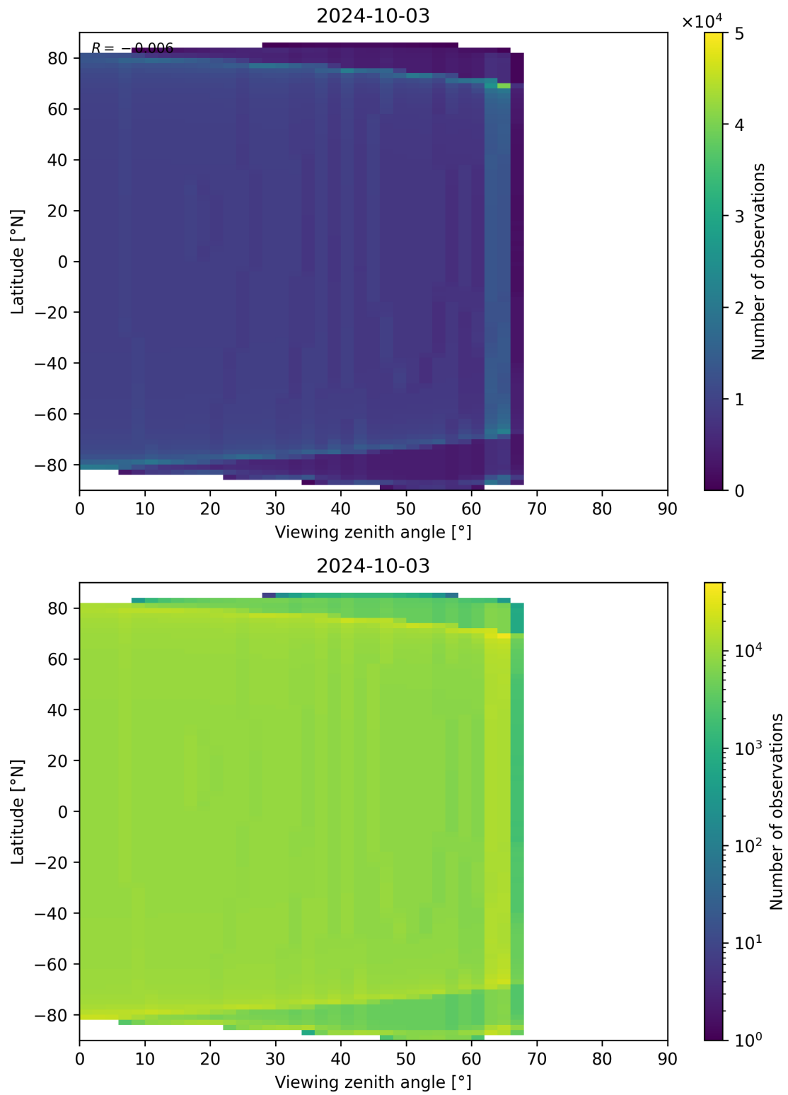
Figure 49: Scatter density plot of “Viewing zenith angle” against “Latitude” for 2024-10-03 to 2024-10-04.
