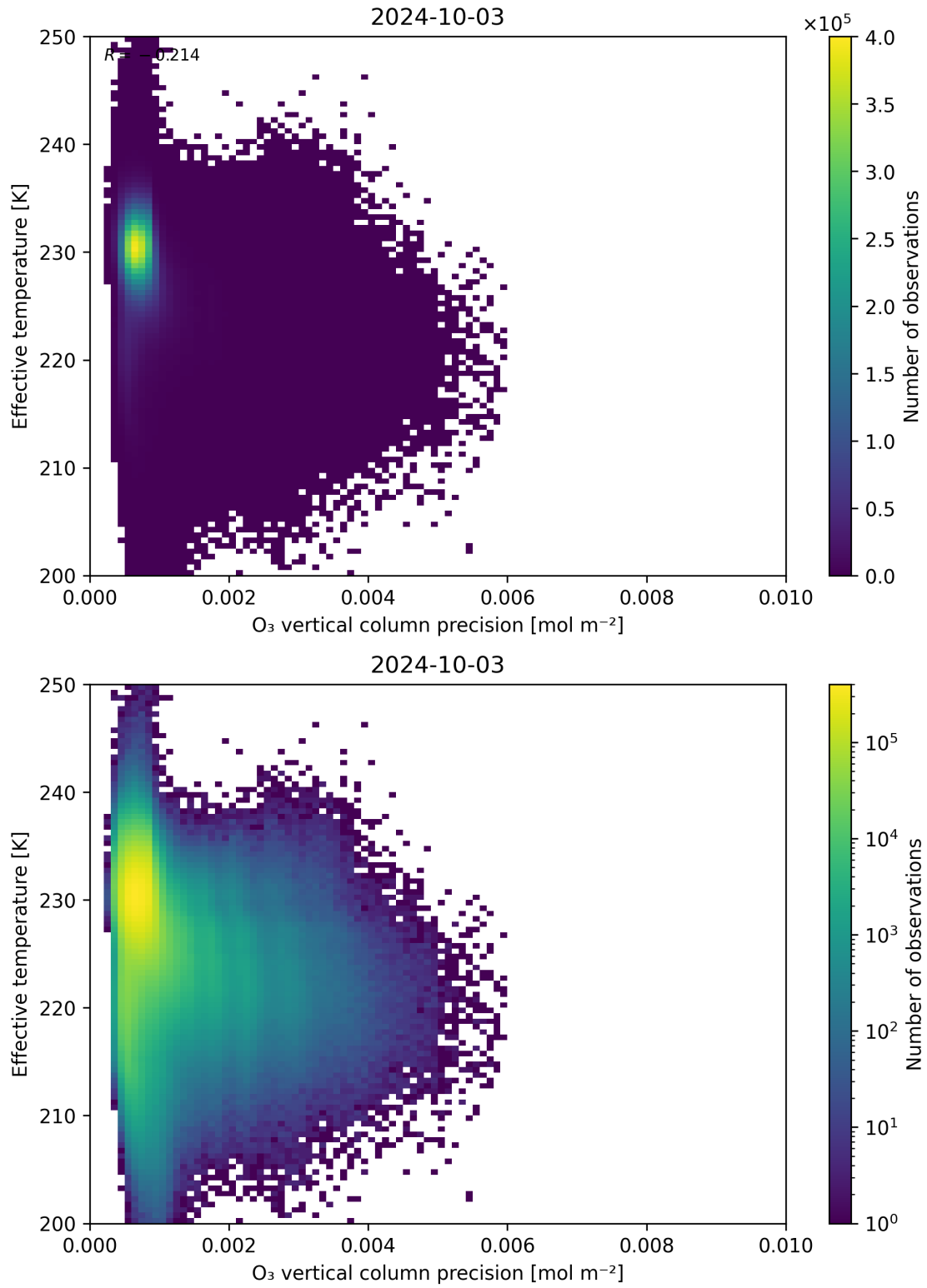
Figure 42: Scatter density plot of “O 3 vertical column precision” against “Effective temperature” for 2024-10-03 to 2024-10-04.
