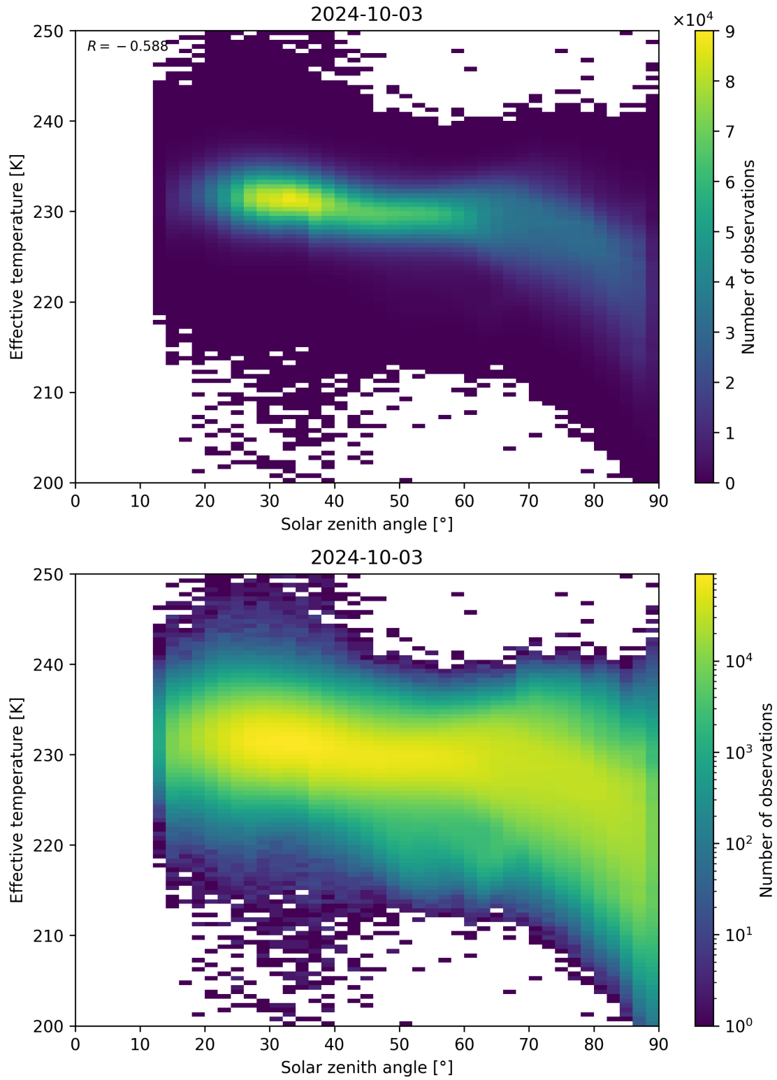
Figure 45: Scatter density plot of “Solar zenith angle” against “Effective temperature” for 2024-10-03 to 2024-10-04.
