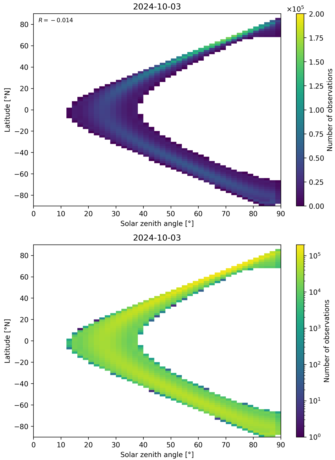
Figure 44: Scatter density plot of “Solar zenith angle” against “Latitude” for 2024-10-03 to 2024-10-04.
