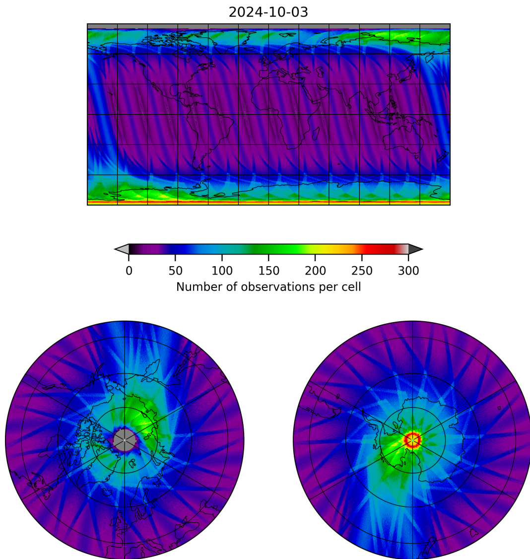
Figure 12: Map of the number of observations for 2024-10-03 to 2024-10-04
