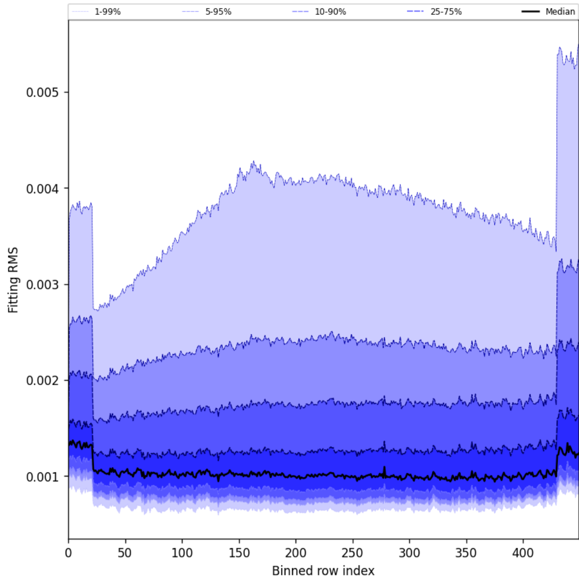
Figure 30: Along track statistics of “Fitting RMS” for 2024-10-03 to 2024-10-05
