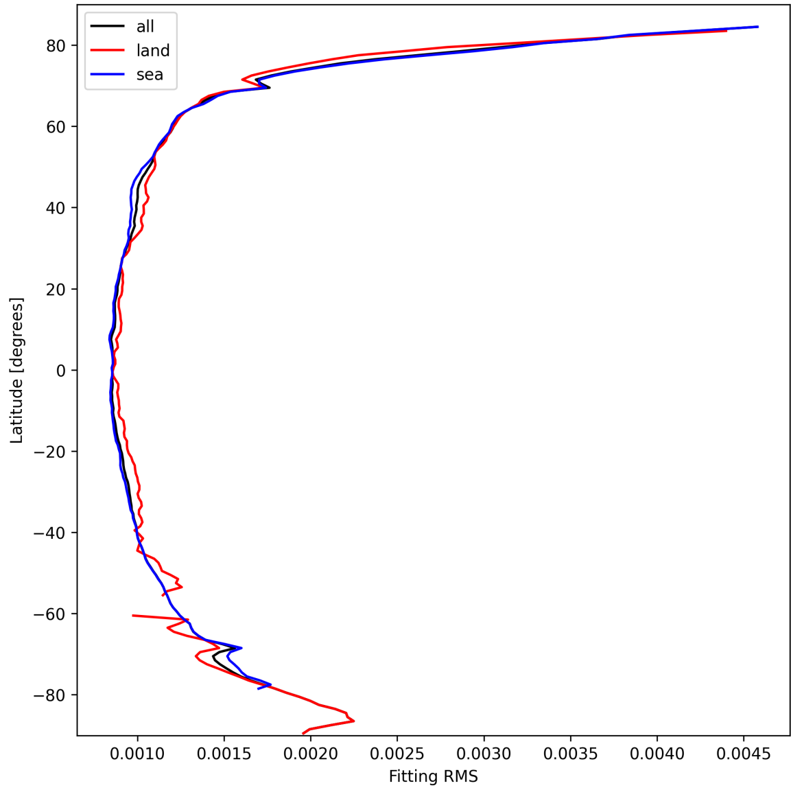
Figure 16: Zonal average of “Fitting RMS” for 2024-10-03 to 2024-10-05.
