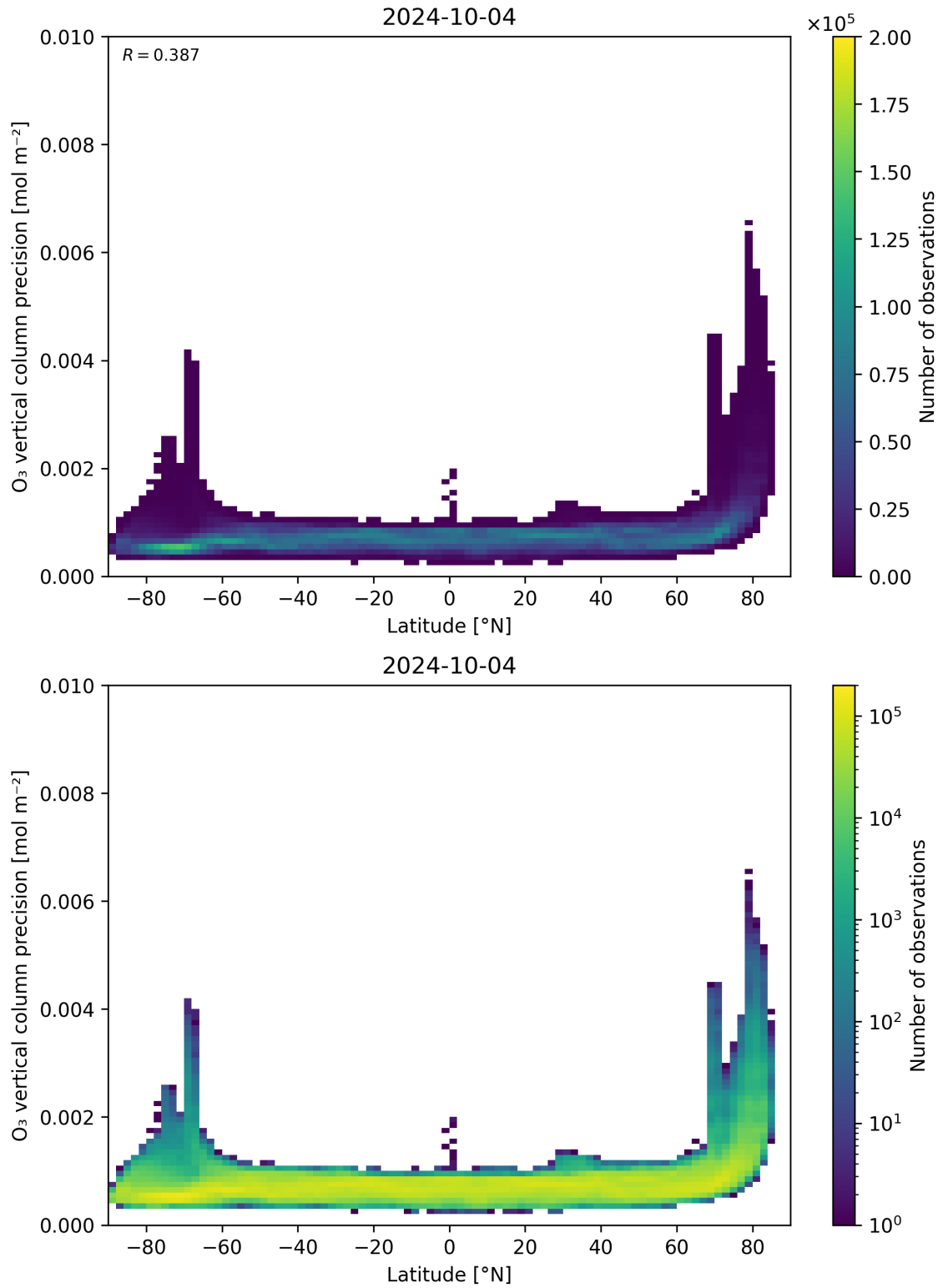
Figure 37: Scatter density plot of “Latitude” against “O 3 vertical column precision” for 2024-10-03 to 2024-10-05.
