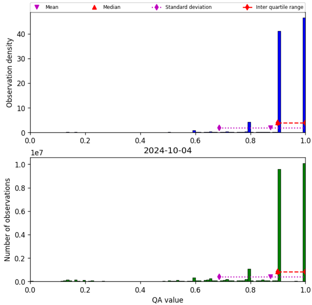
Figure 20: Histogram of “QA value” for 2024-10-03 to 2024-10-05
