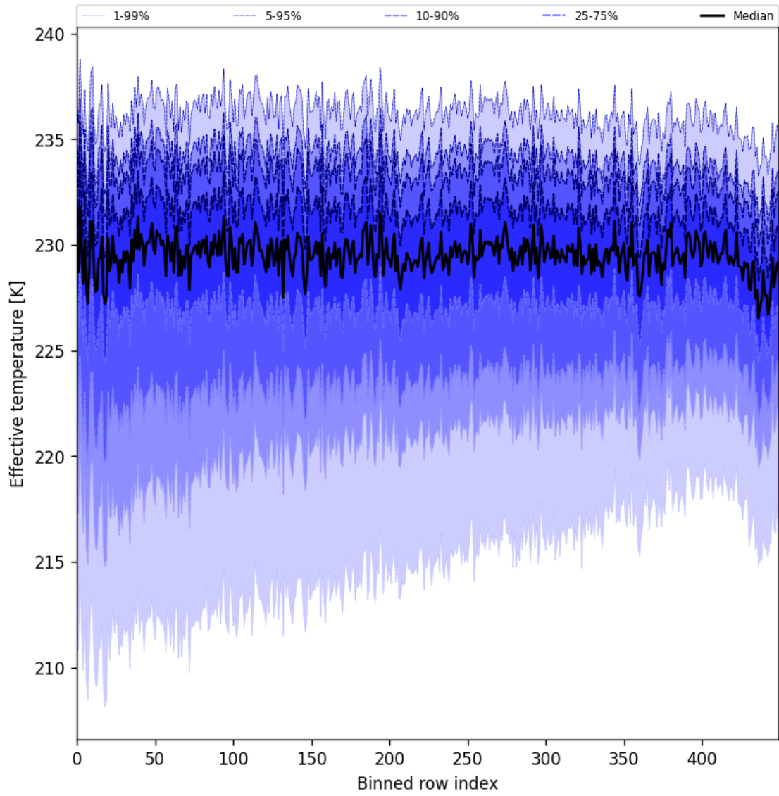
Figure 31: Along track statistics of “Effective temperature” for 2024-10-03 to 2024-10-05
