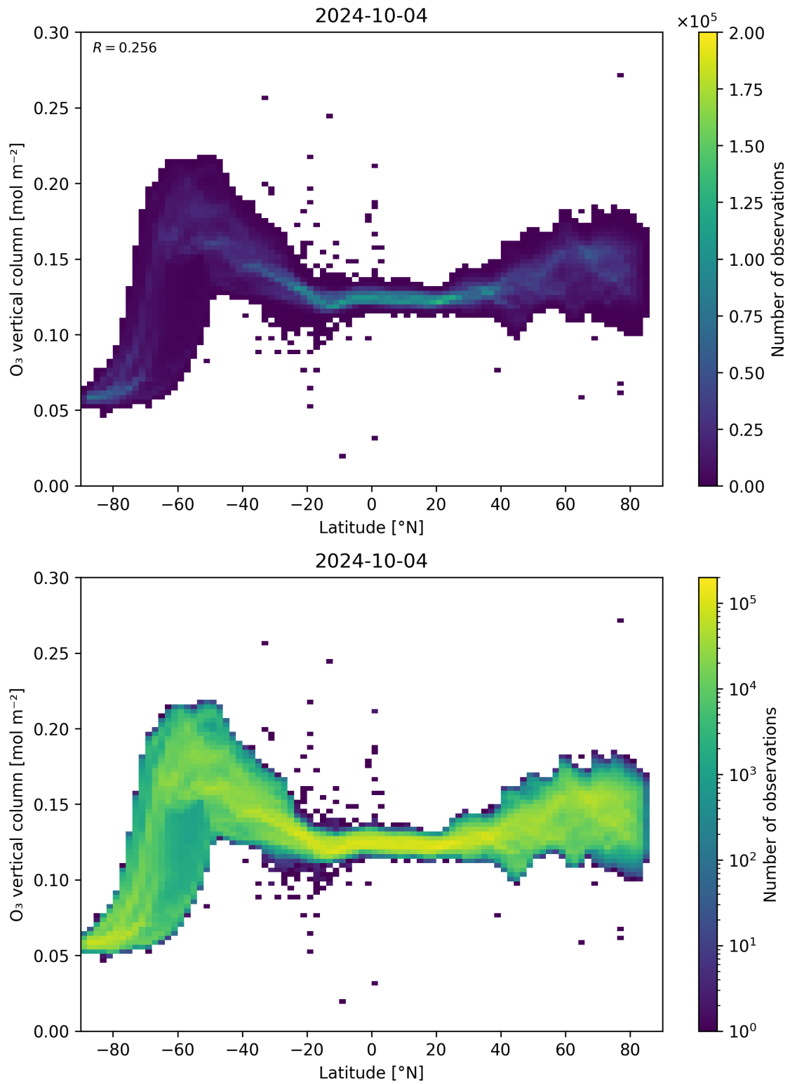
Figure 36: Scatter density plot of “Latitude” against “O 3 vertical column” for 2024-10-03 to 2024-10-05.
