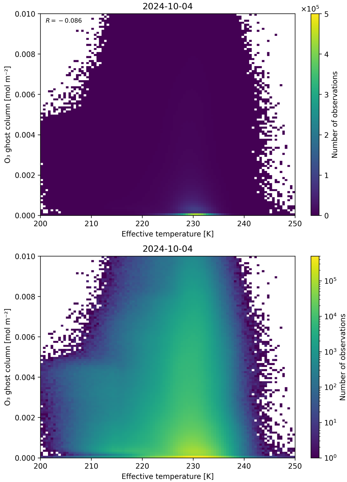
Figure 38: Scatter density plot of “Effective temperature” against “O 3 ghost column” for 2024-10-03 to 2024-10-05.
