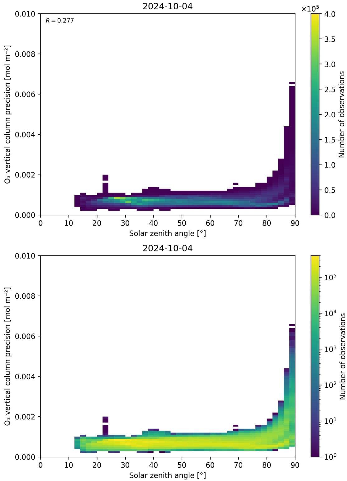
Figure 48: Scatter density plot of “Solar zenith angle” against “O 3 vertical column precision” for 2024-10-03 to 2024-10-05.
