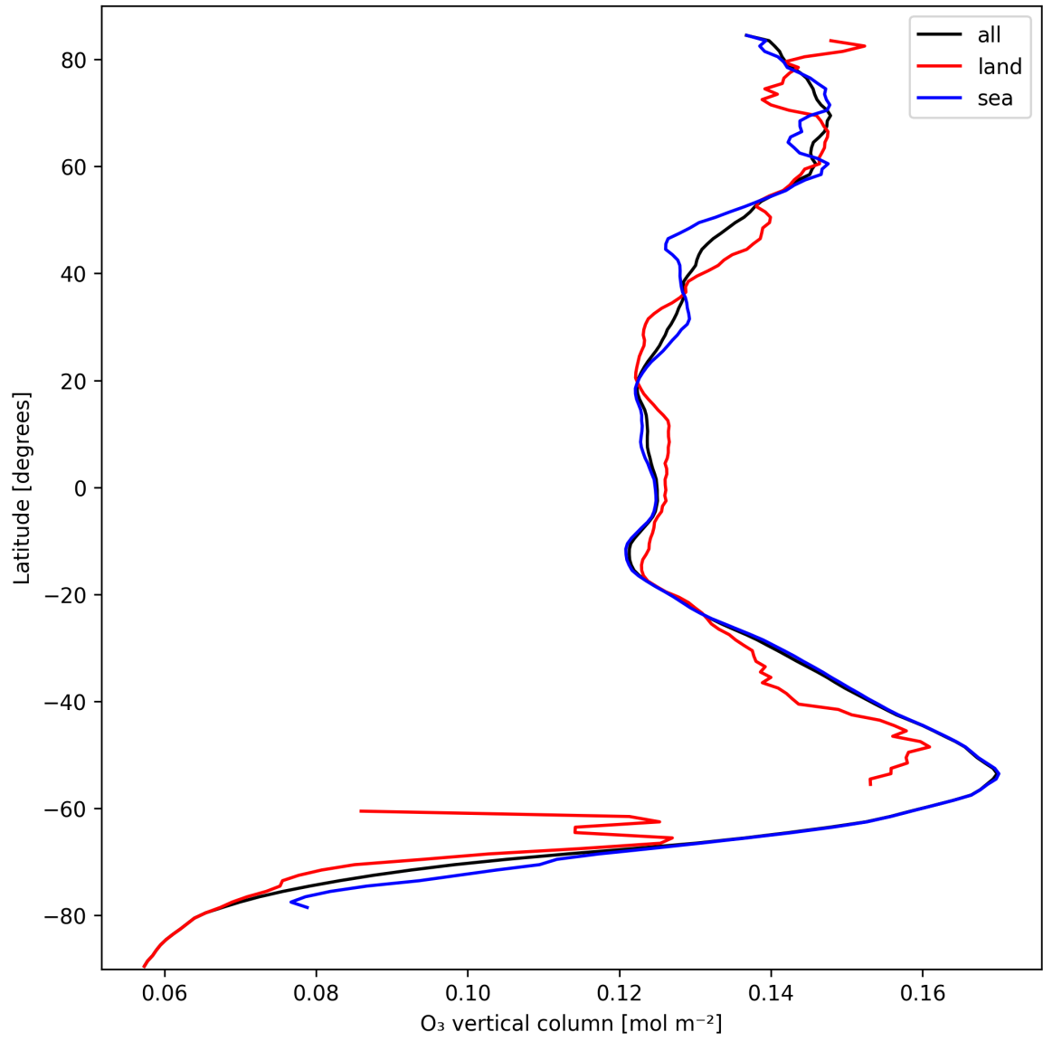
Figure 14: Zonal average of “O 3 vertical column” for 2024-10-03 to 2024-10-05.
