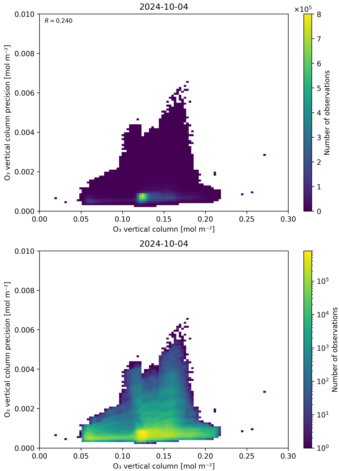
Figure 41: Scatter density plot of “O 3 vertical column” against “O 3 vertical column precision” for 2024-10-03 to 2024-10-05.
