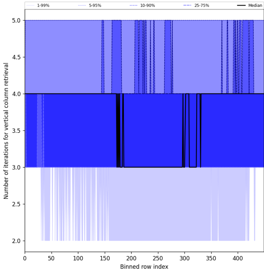
Figure 33: Along track statistics of “Number of iterations for vertical column retrieval” for 2024-10-03 to 2024-10-05
