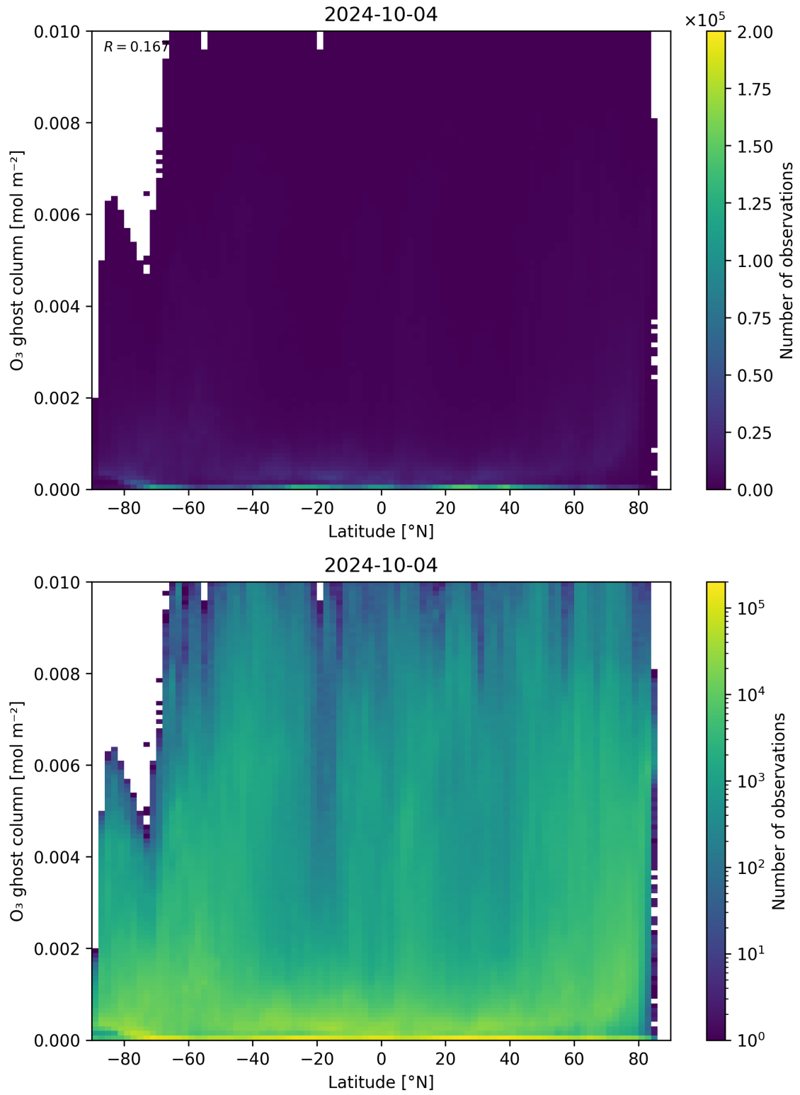
Figure 35: Scatter density plot of “Latitude” against “O 3 ghost column” for 2024-10-03 to 2024-10-05.
