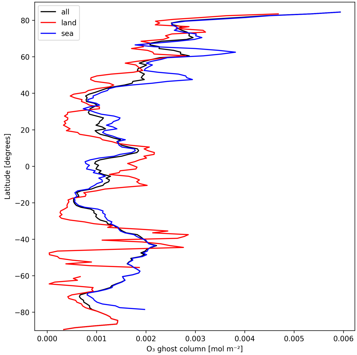
Figure 18: Zonal average of “O 3 ghost column” for 2024-10-03 to 2024-10-05.
