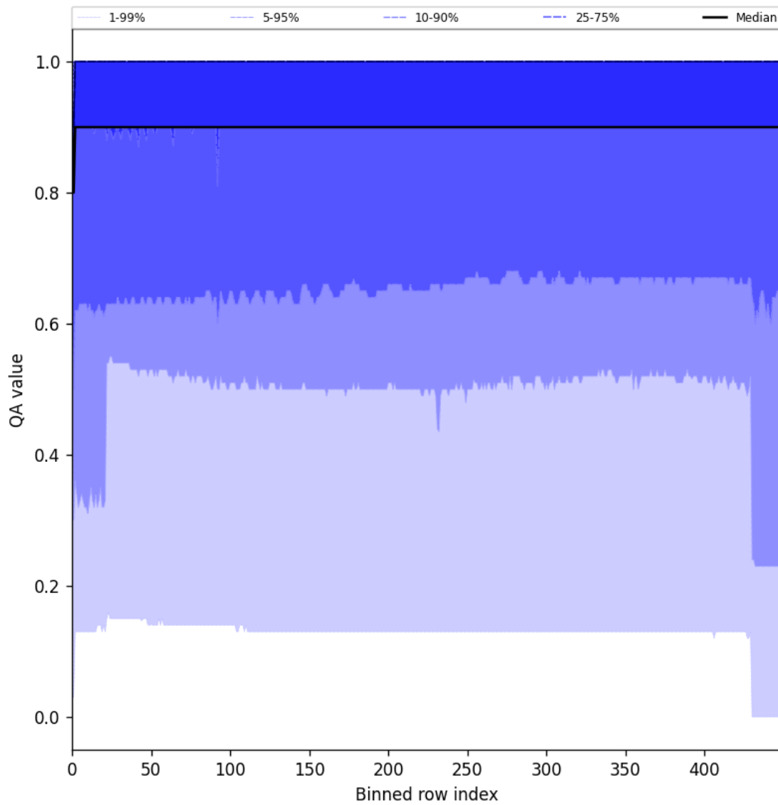
Figure 27: Along track statistics of “QA value” for 2024-10-03 to 2024-10-05
