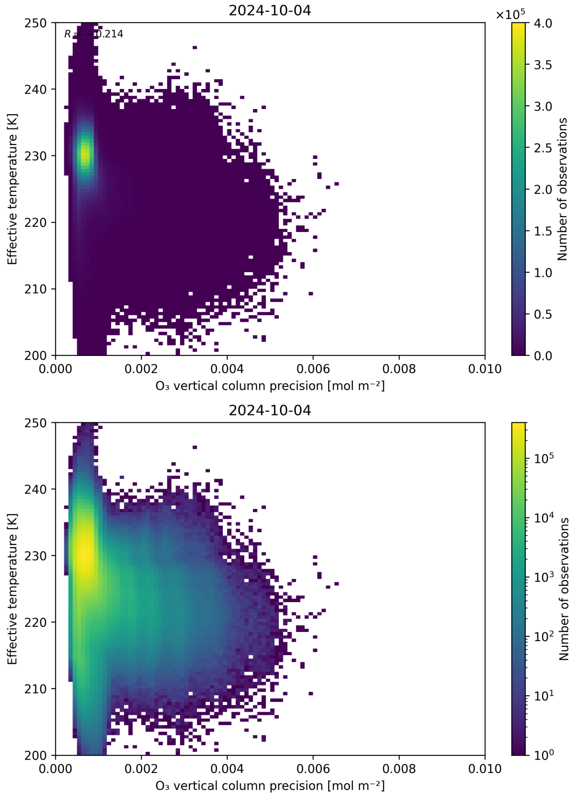
Figure 42: Scatter density plot of “O 3 vertical column precision” against “Effective temperature” for 2024-10-03 to 2024-10-05.
