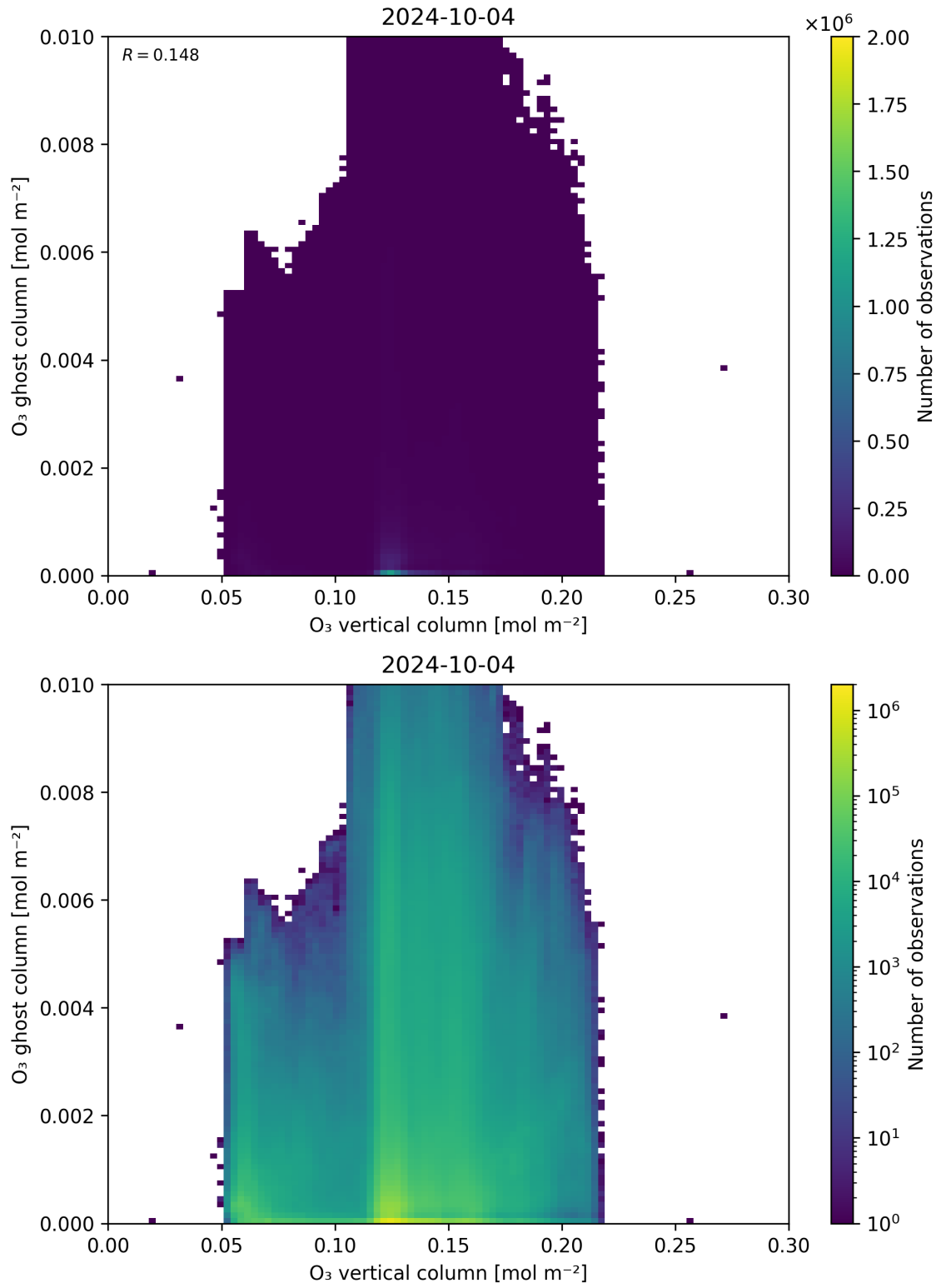
Figure 40: Scatter density plot of “O 3 vertical column” against “O 3 ghost column” for 2024-10-03 to 2024-10-05.
