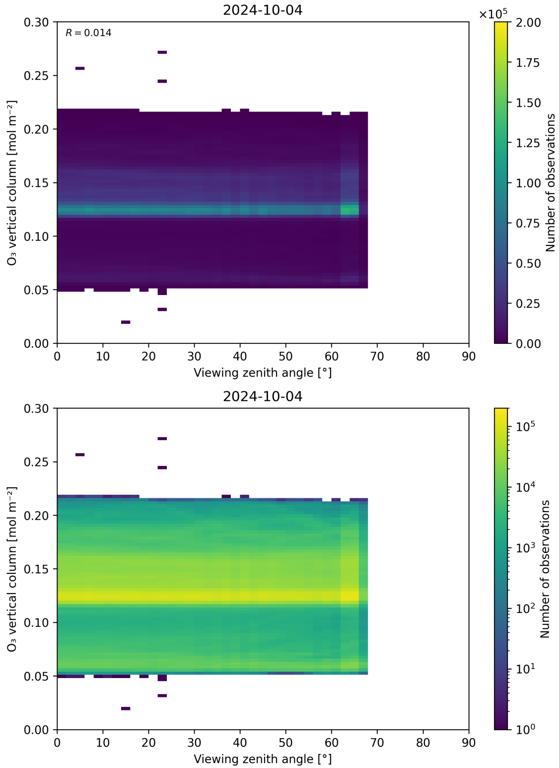
Figure 52: Scatter density plot of “Viewing zenith angle” against “O 3 vertical column” for 2024-10-03 to 2024-10-05.
