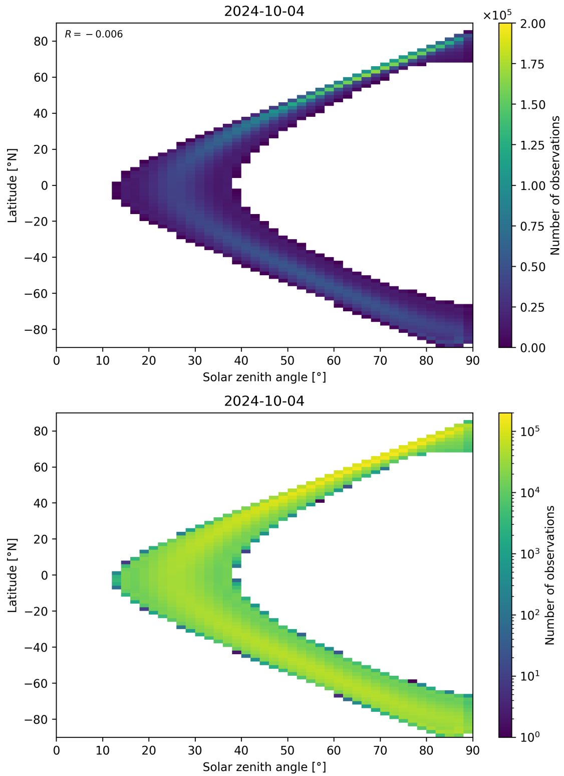
Figure 44: Scatter density plot of “Solar zenith angle” against “Latitude” for 2024-10-03 to 2024-10-05.
