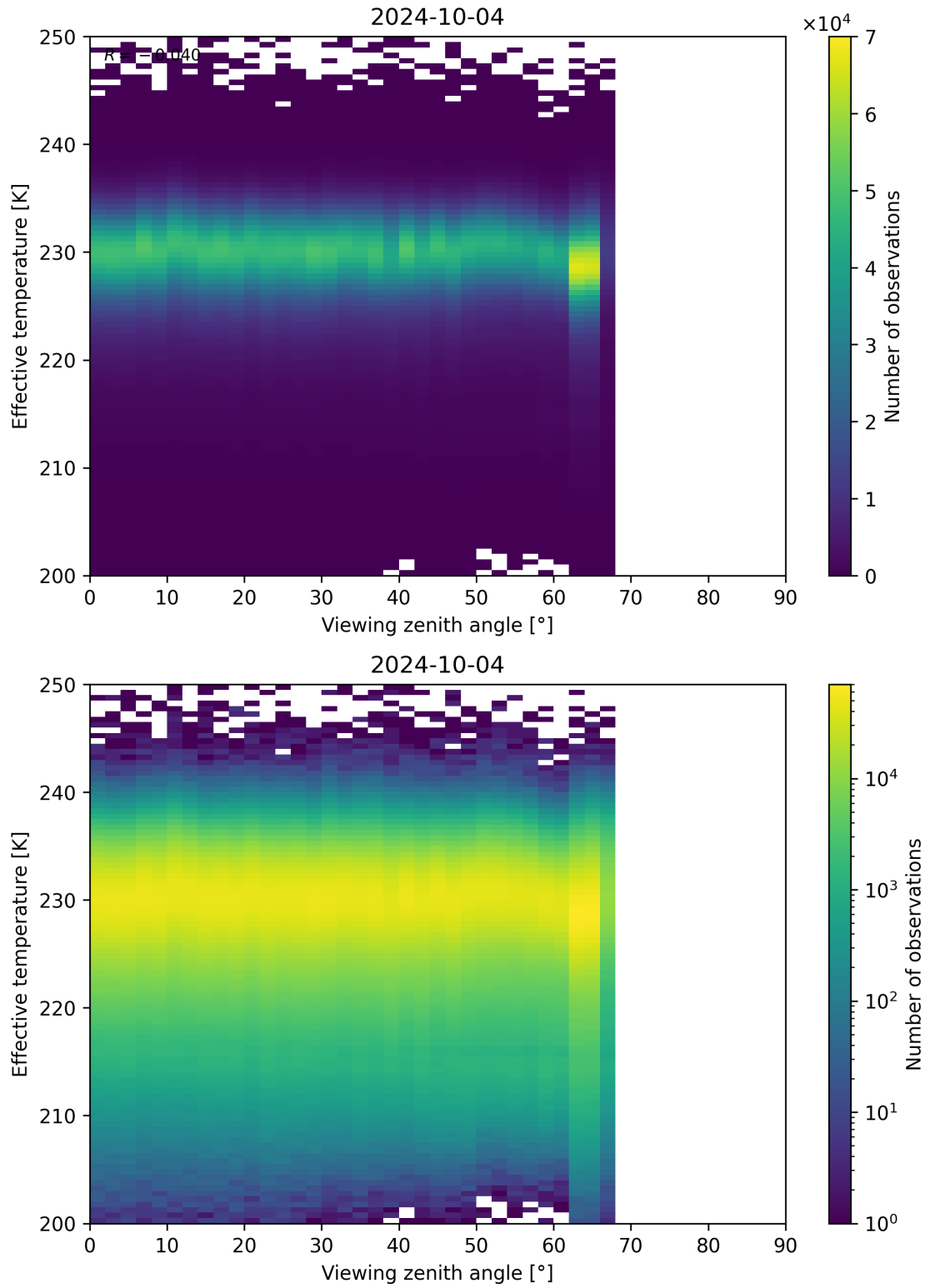
Figure 50: Scatter density plot of “Viewing zenith angle” against “Effective temperature” for 2024-10-03 to 2024-10-05.
