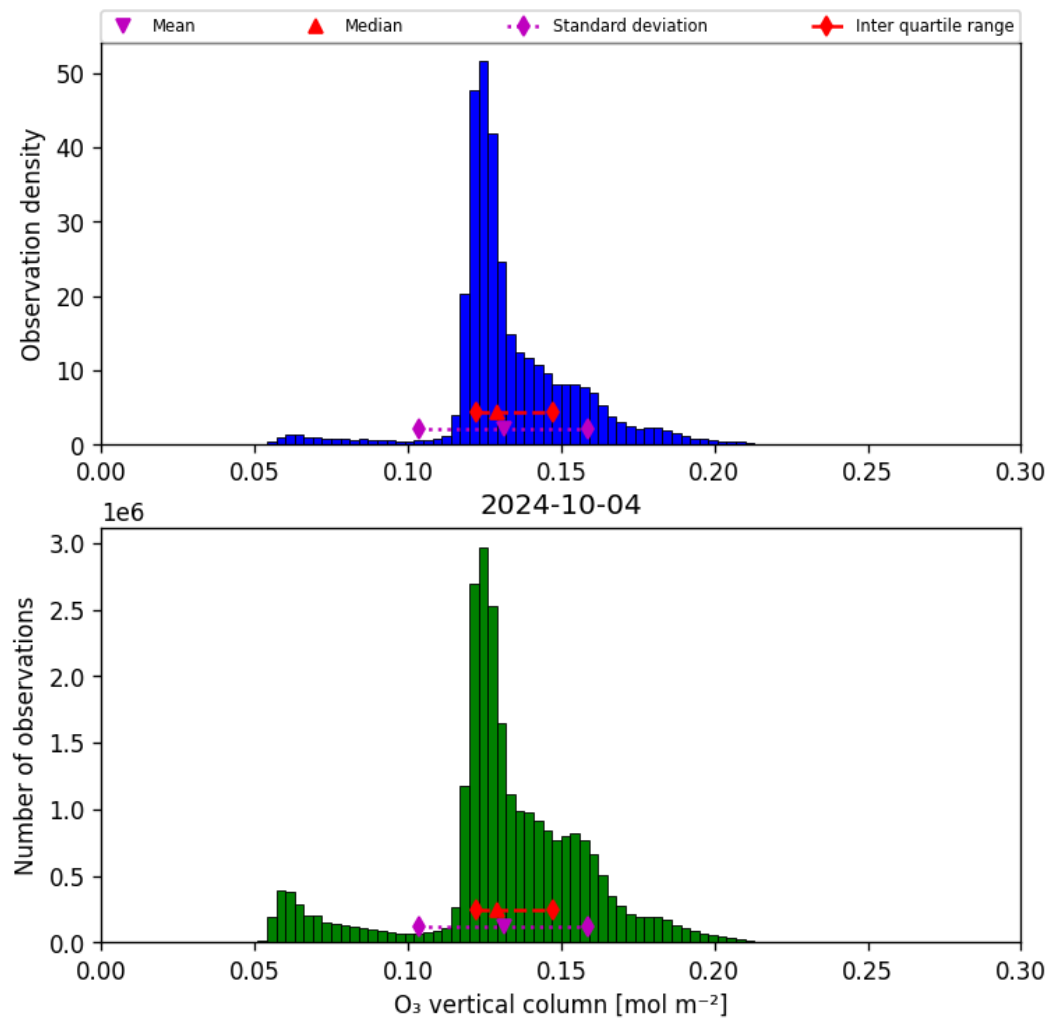
Figure 21: Histogram of “O 3 vertical column” for 2024-10-03 to 2024-10-05
