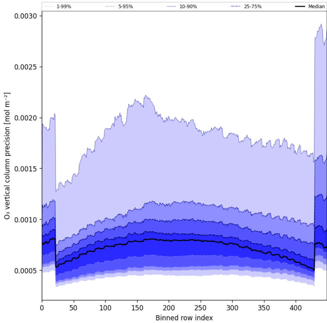
Figure 29: Along track statistics of “O 3 vertical column precision” for 2024-10-03 to 2024-10-05
