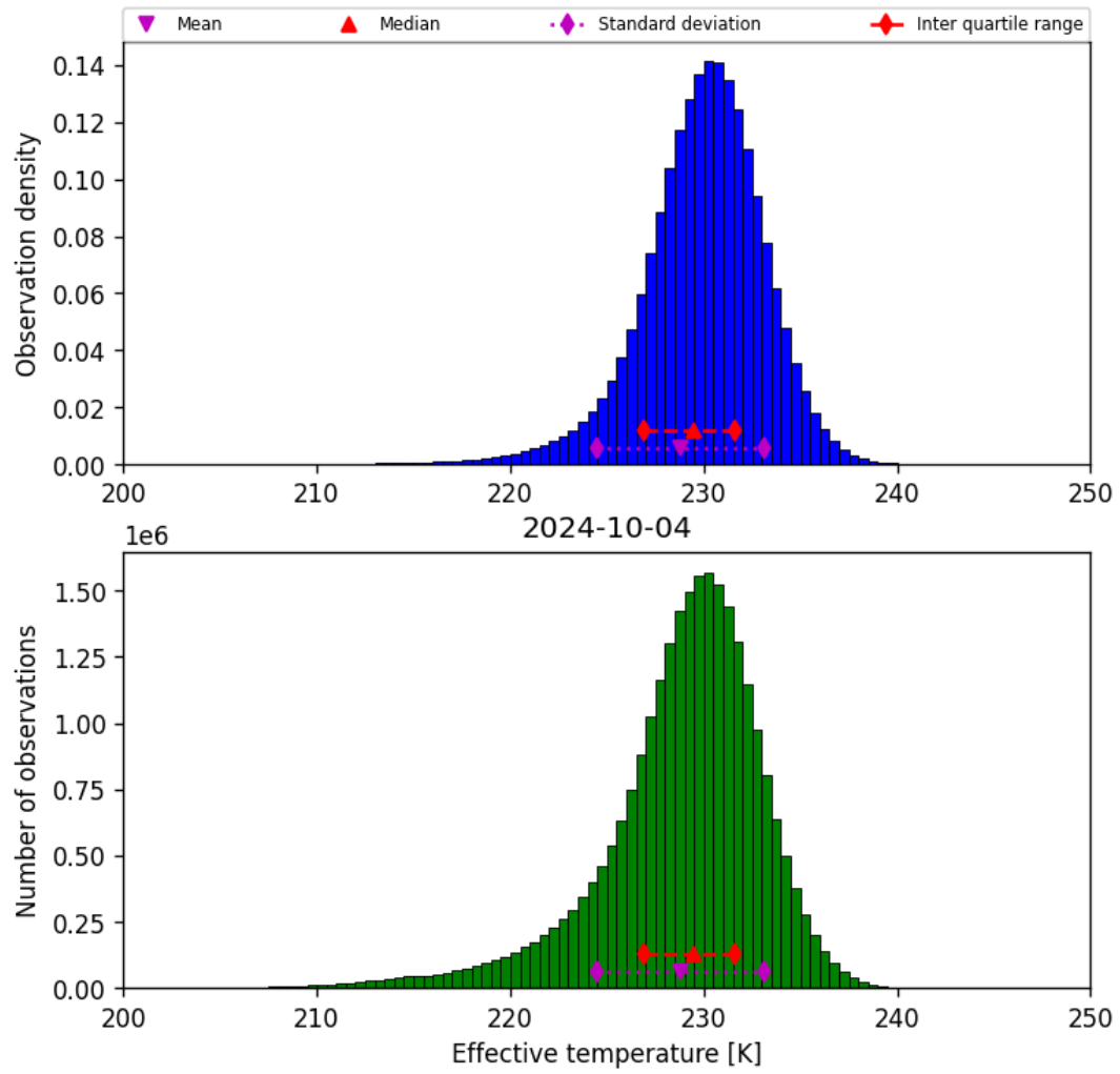
Figure 24: Histogram of “Effective temperature” for 2024-10-03 to 2024-10-05
