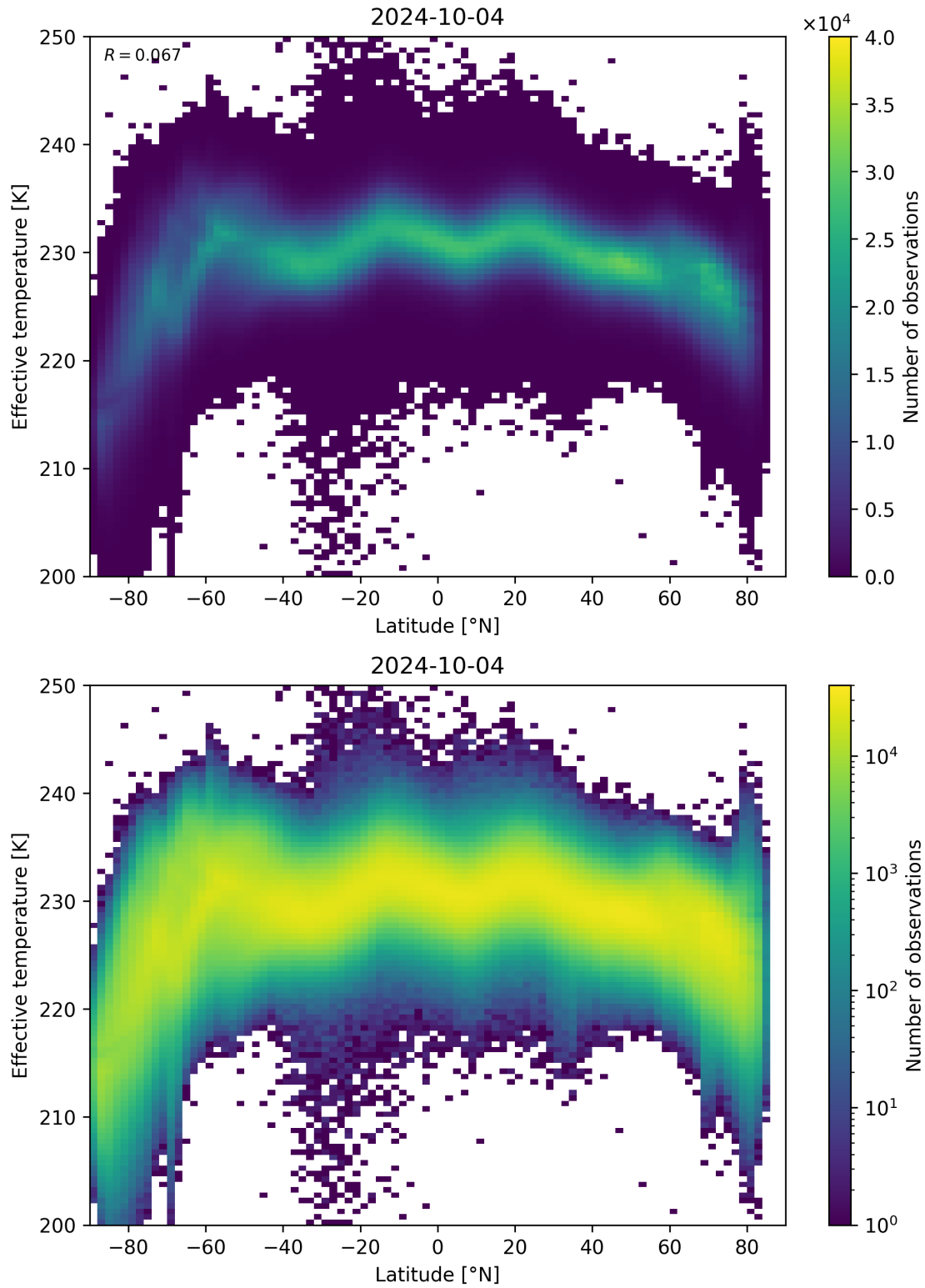
Figure 34: Scatter density plot of “Latitude” against “Effective temperature” for 2024-10-03 to 2024-10-05.
