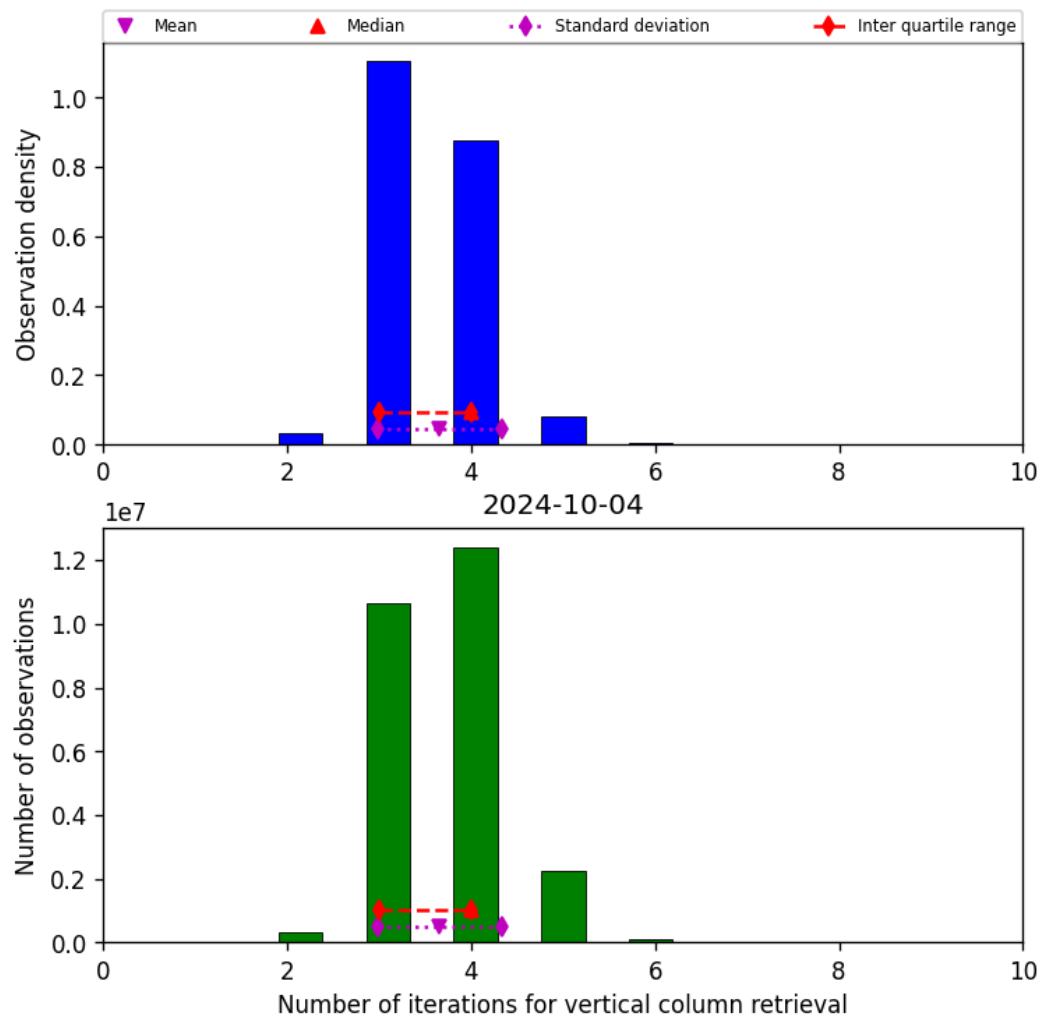
Figure 26: Histogram of “Number of iterations for vertical column retrieval” for 2024-10-03 to 2024-10-05
