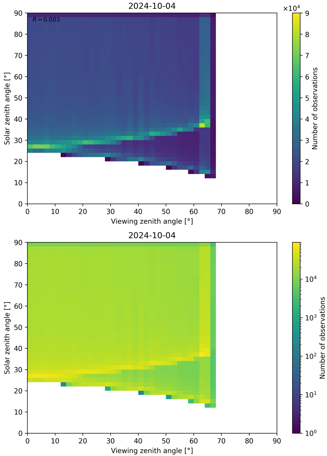
Figure 54: Scatter density plot of “Viewing zenith angle” against “Solar zenith angle” for 2024-10-03 to 2024-10-05.
