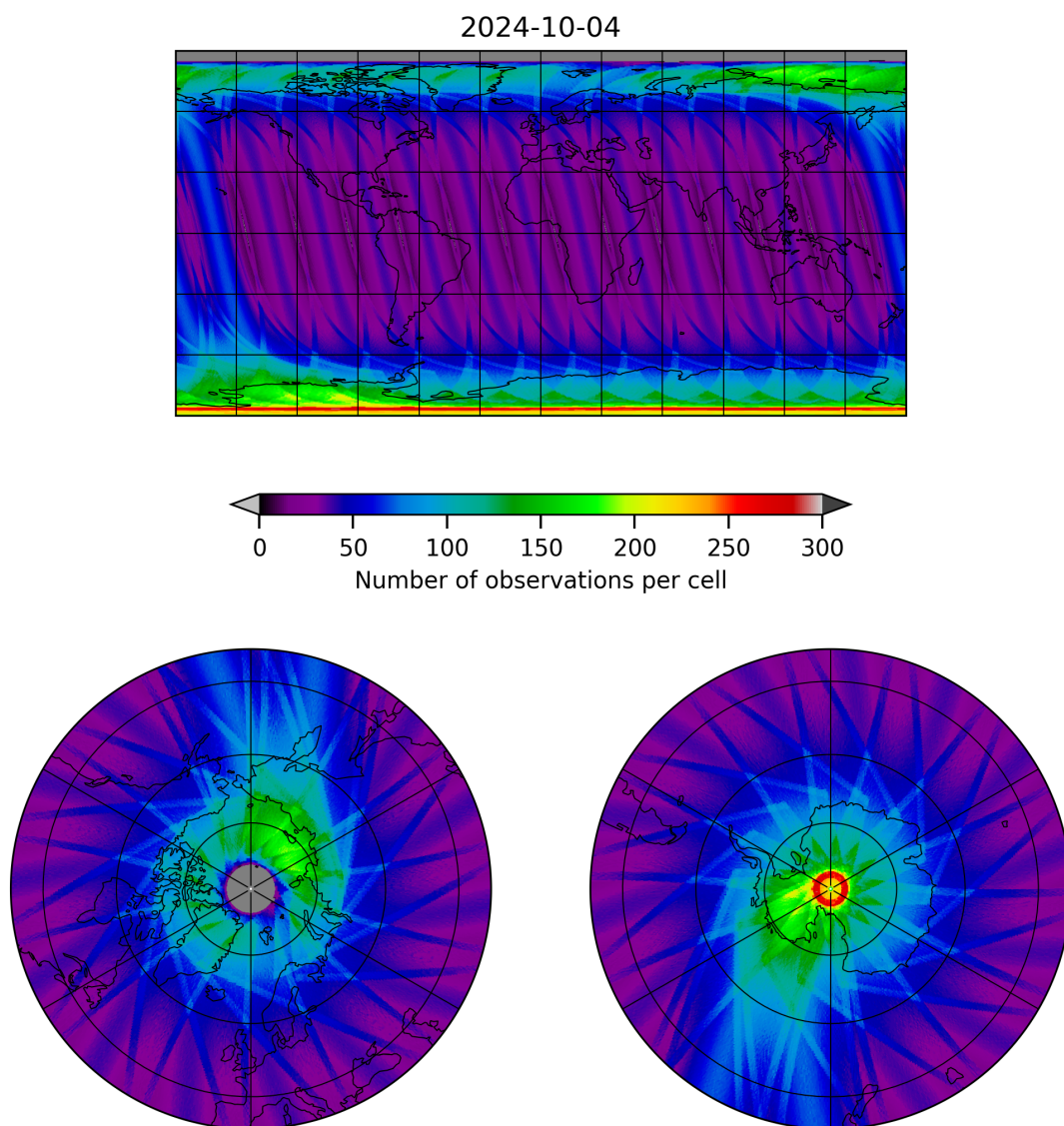
Figure 12: Map of the number of observations for 2024-10-03 to 2024-10-05
