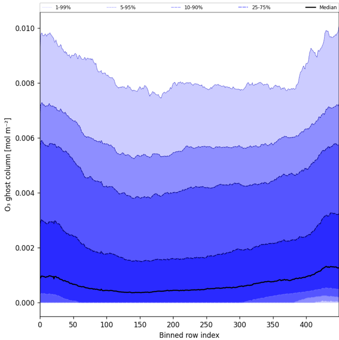
Figure 32: Along track statistics of “O 3 ghost column” for 2024-10-03 to 2024-10-05
