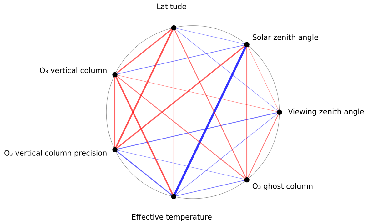
Figure 1: Map of correlation graph for 2024-10-03 to 2024-10-05.
