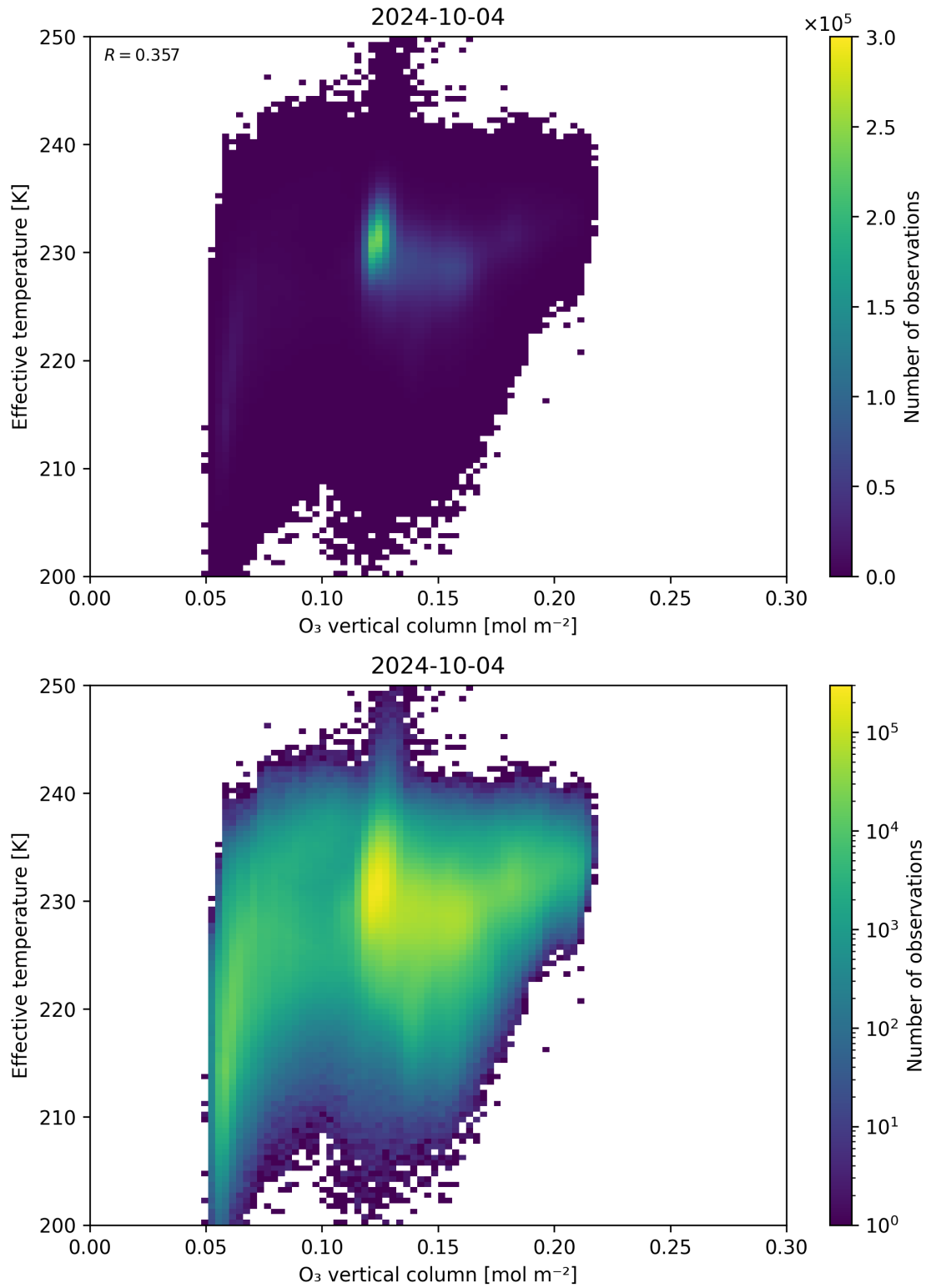
Figure 39: Scatter density plot of “O 3 vertical column” against “Effective temperature” for 2024-10-03 to 2024-10-05.
