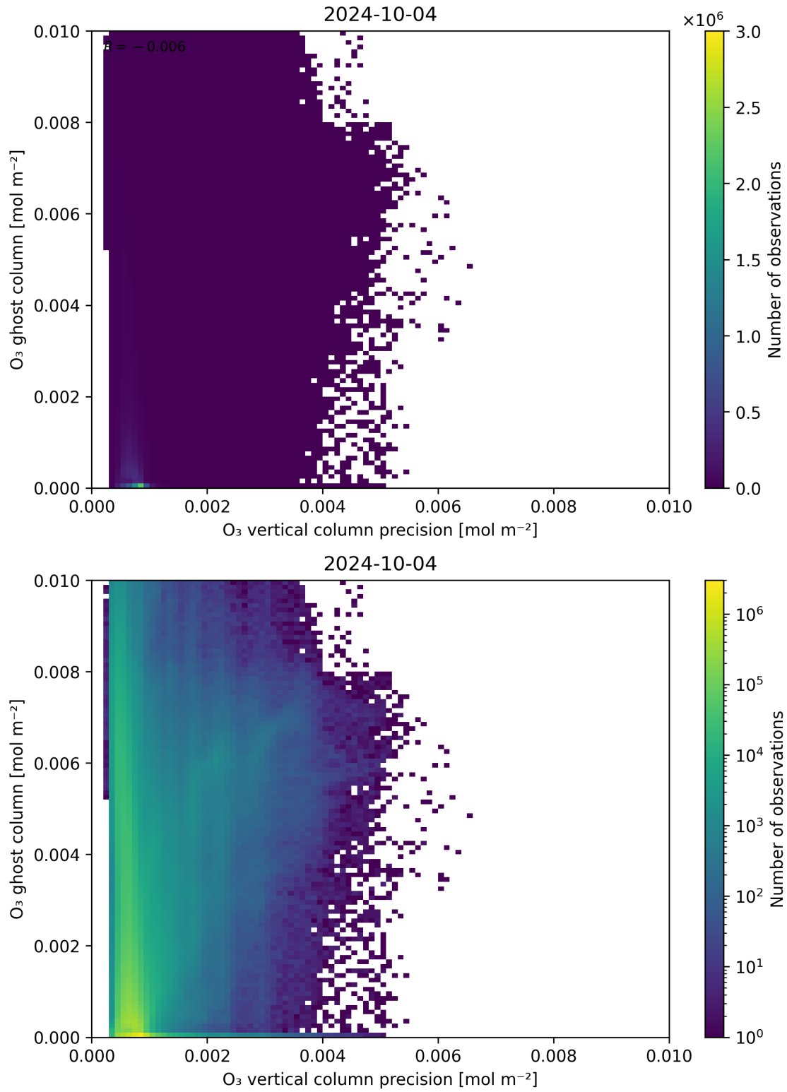
Figure 43: Scatter density plot of “O 3 vertical column precision” against “O 3 ghost column” for 2024-10-03 to 2024-10-05.
