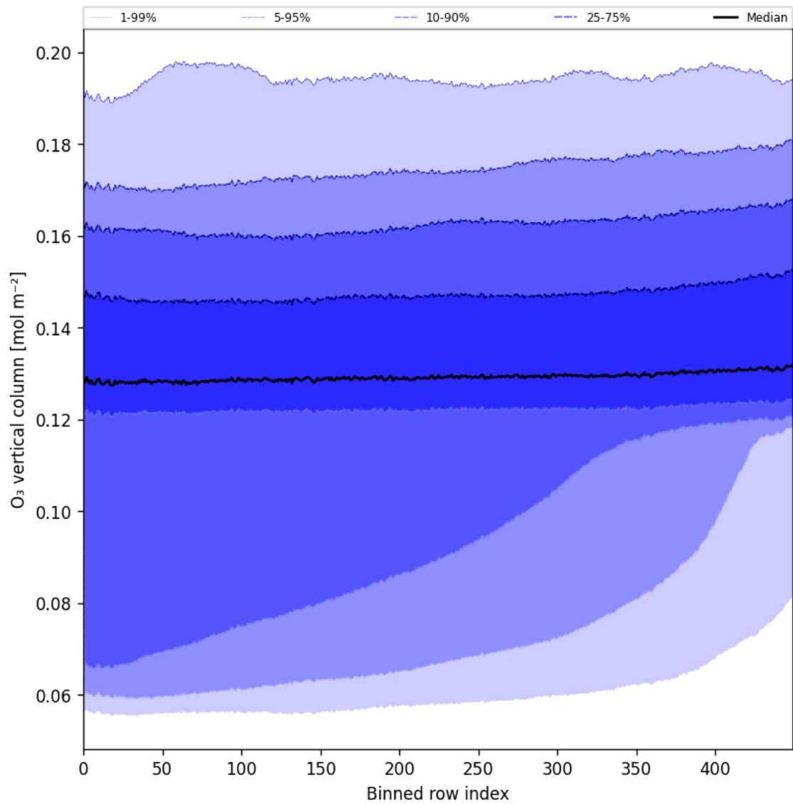
Figure 28: Along track statistics of “O 3 vertical column” for 2024-10-03 to 2024-10-05
