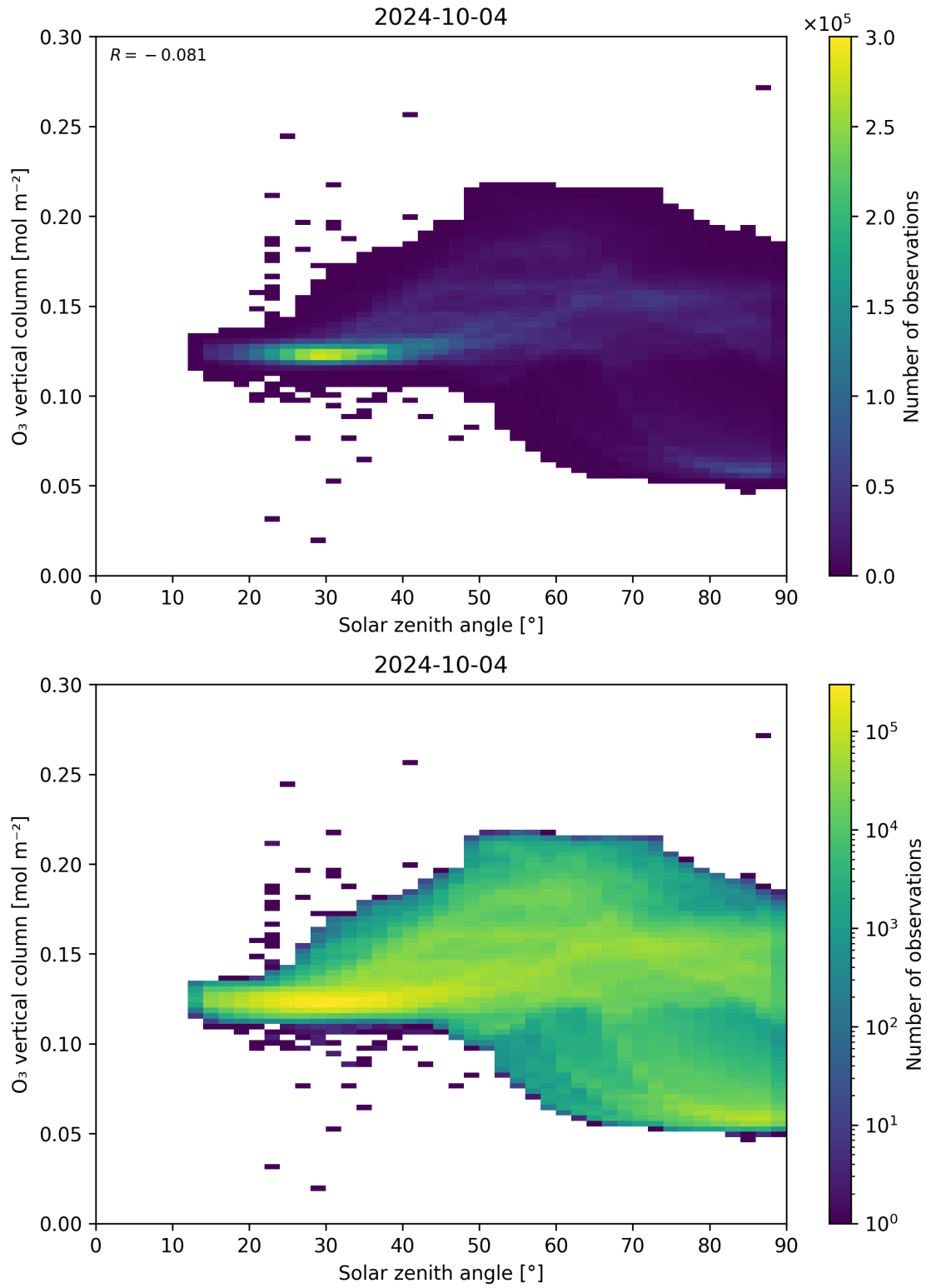
Figure 47: Scatter density plot of “Solar zenith angle” against “O 3 vertical column” for 2024-10-03 to 2024-10-05.
