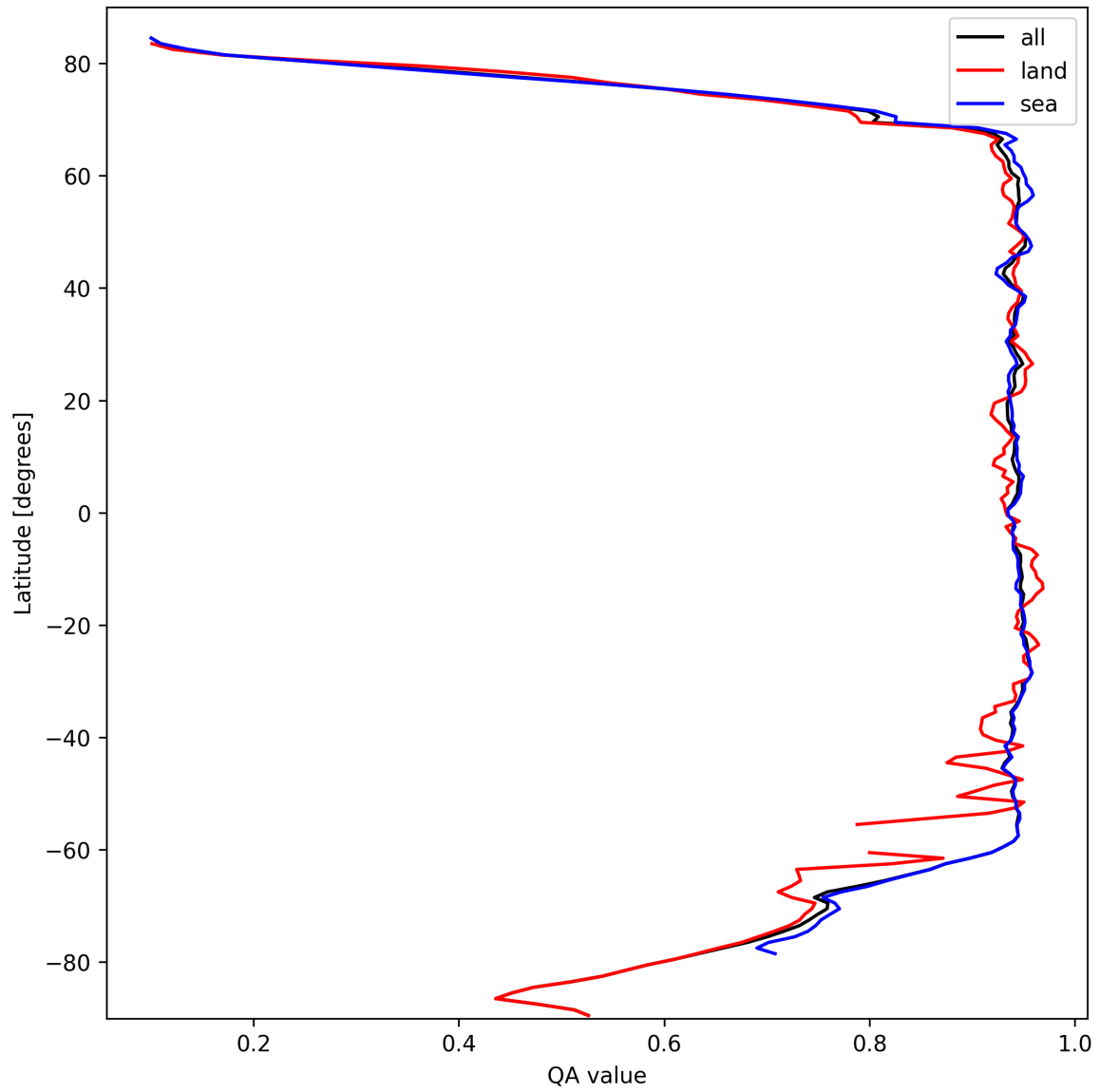
Figure 13: Zonal average of “QA value” for 2024-10-03 to 2024-10-05.
