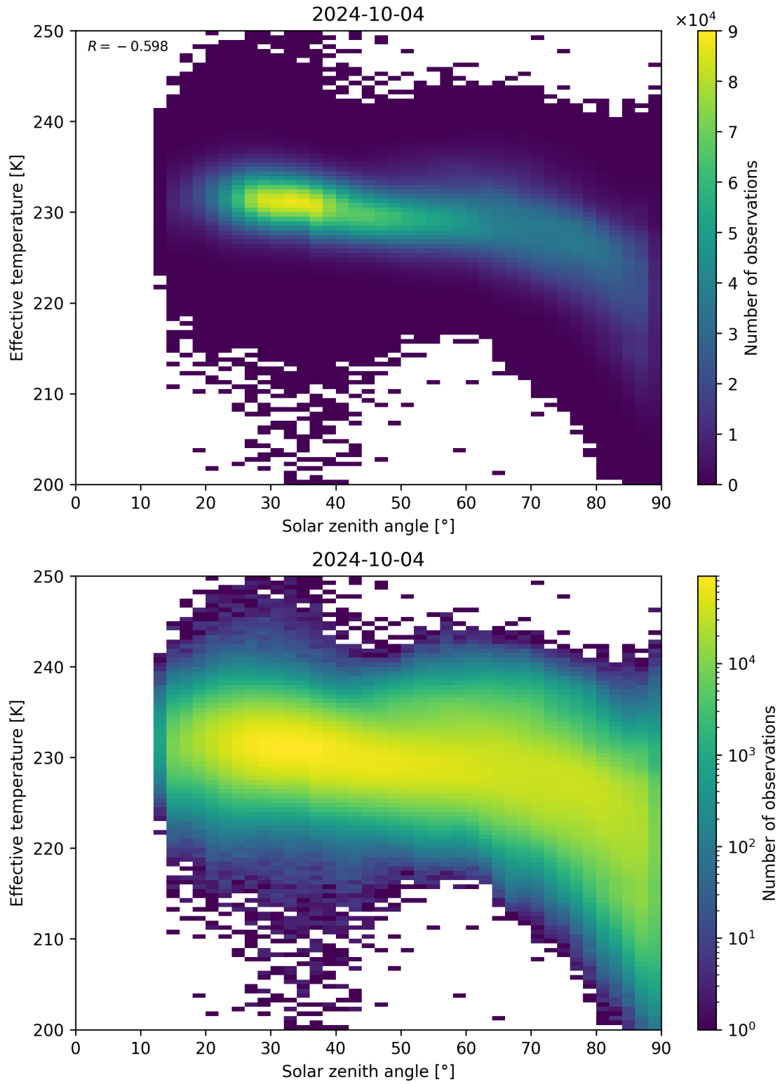
Figure 45: Scatter density plot of “Solar zenith angle” against “Effective temperature” for 2024-10-03 to 2024-10-05.
