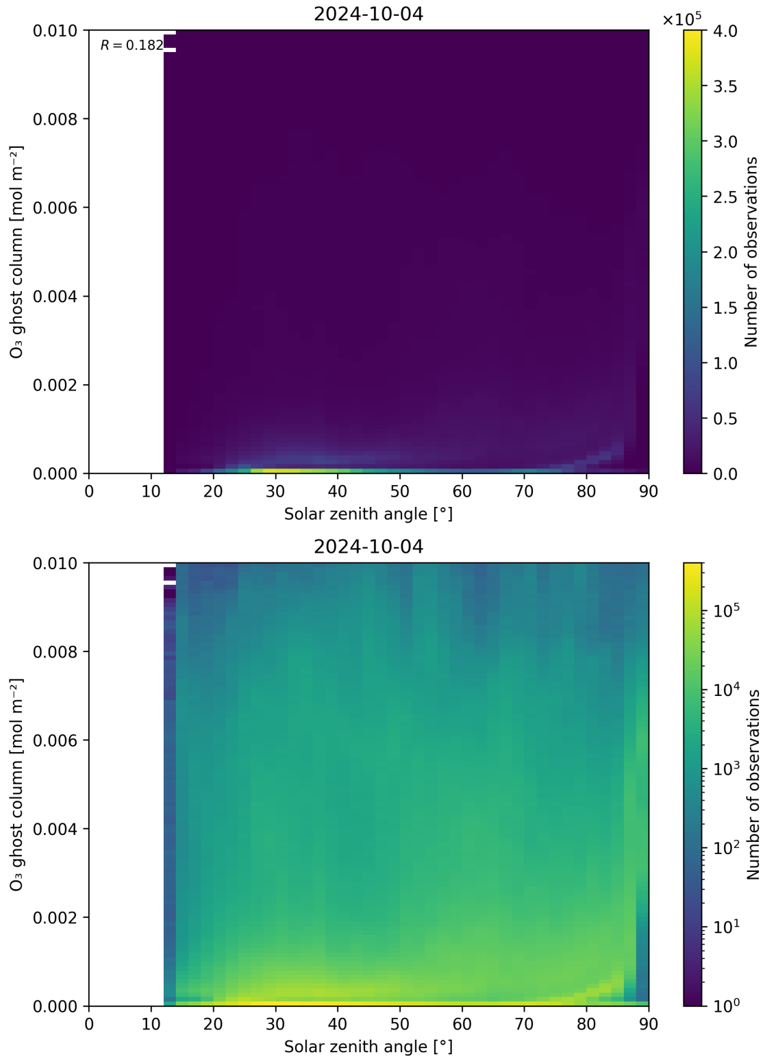
Figure 46: Scatter density plot of “Solar zenith angle” against “O 3 ghost column” for 2024-10-03 to 2024-10-05.
