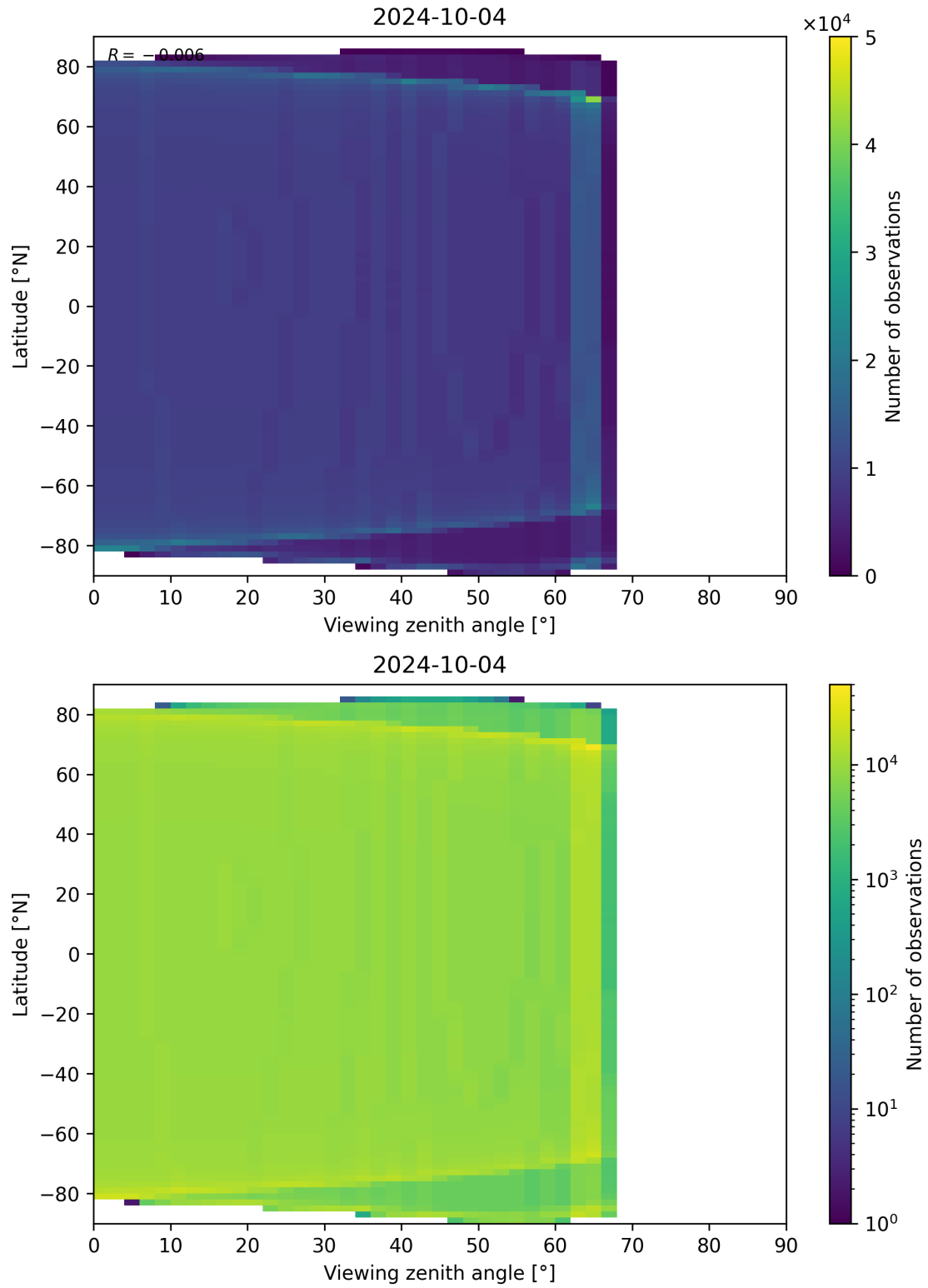
Figure 49: Scatter density plot of “Viewing zenith angle” against “Latitude” for 2024-10-03 to 2024-10-05.
