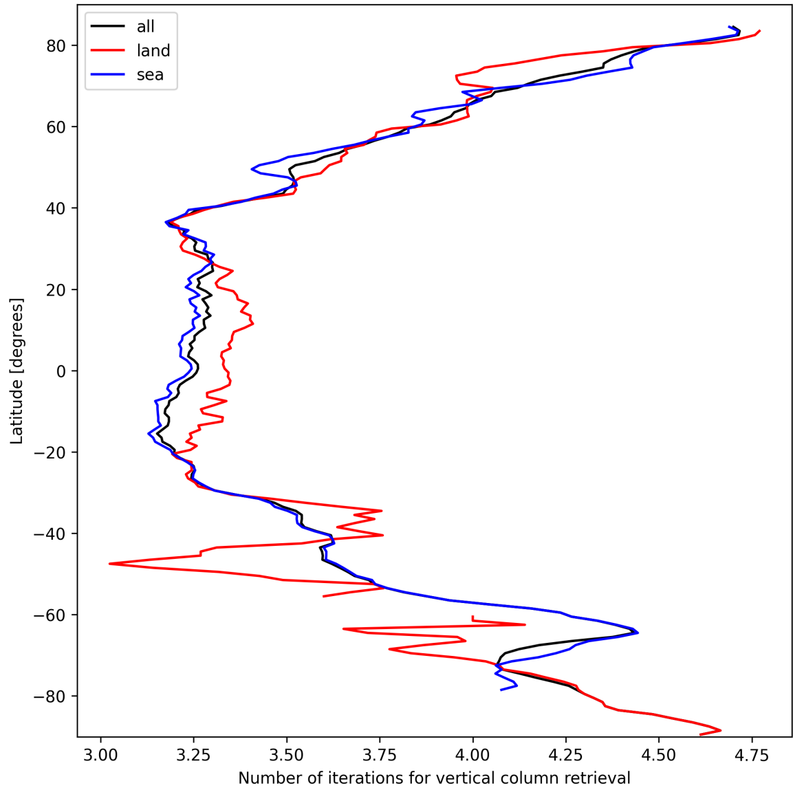
Figure 19: Zonal average of “Number of iterations for vertical column retrieval” for 2024-10-03 to 2024-10-05.
