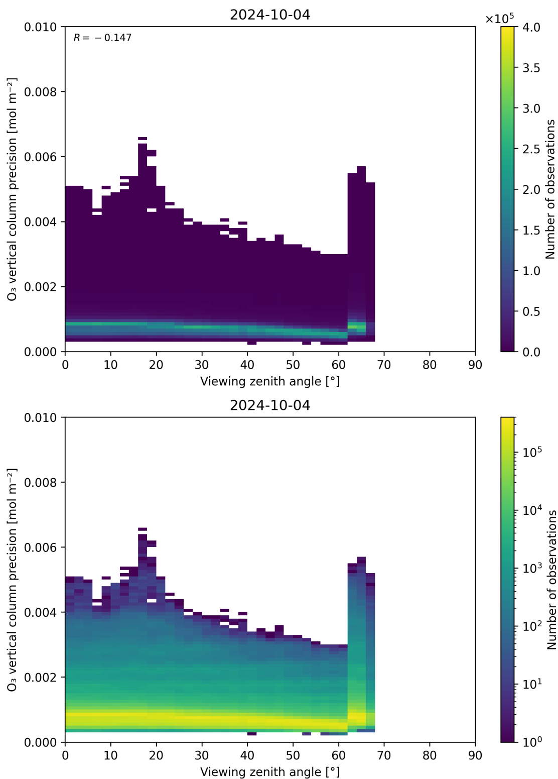
Figure 53: Scatter density plot of “Viewing zenith angle” against “O 3 vertical column precision” for 2024-10-03 to 2024-10-05.
