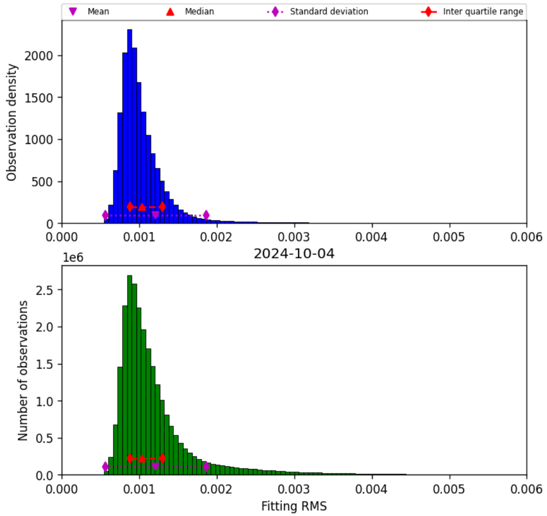
Figure 23: Histogram of “Fitting RMS” for 2024-10-03 to 2024-10-05
