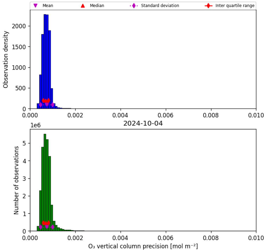
Figure 22: Histogram of “O 3 vertical column precision” for 2024-10-03 to 2024-10-05
