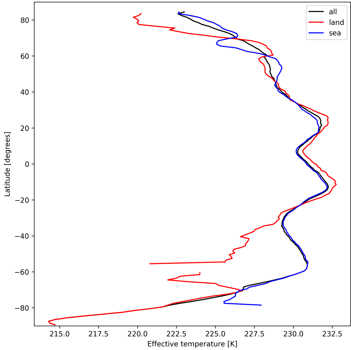
Figure 17: Zonal average of "Effective temperature" for 2024-10-03 to 2024-10-05.
