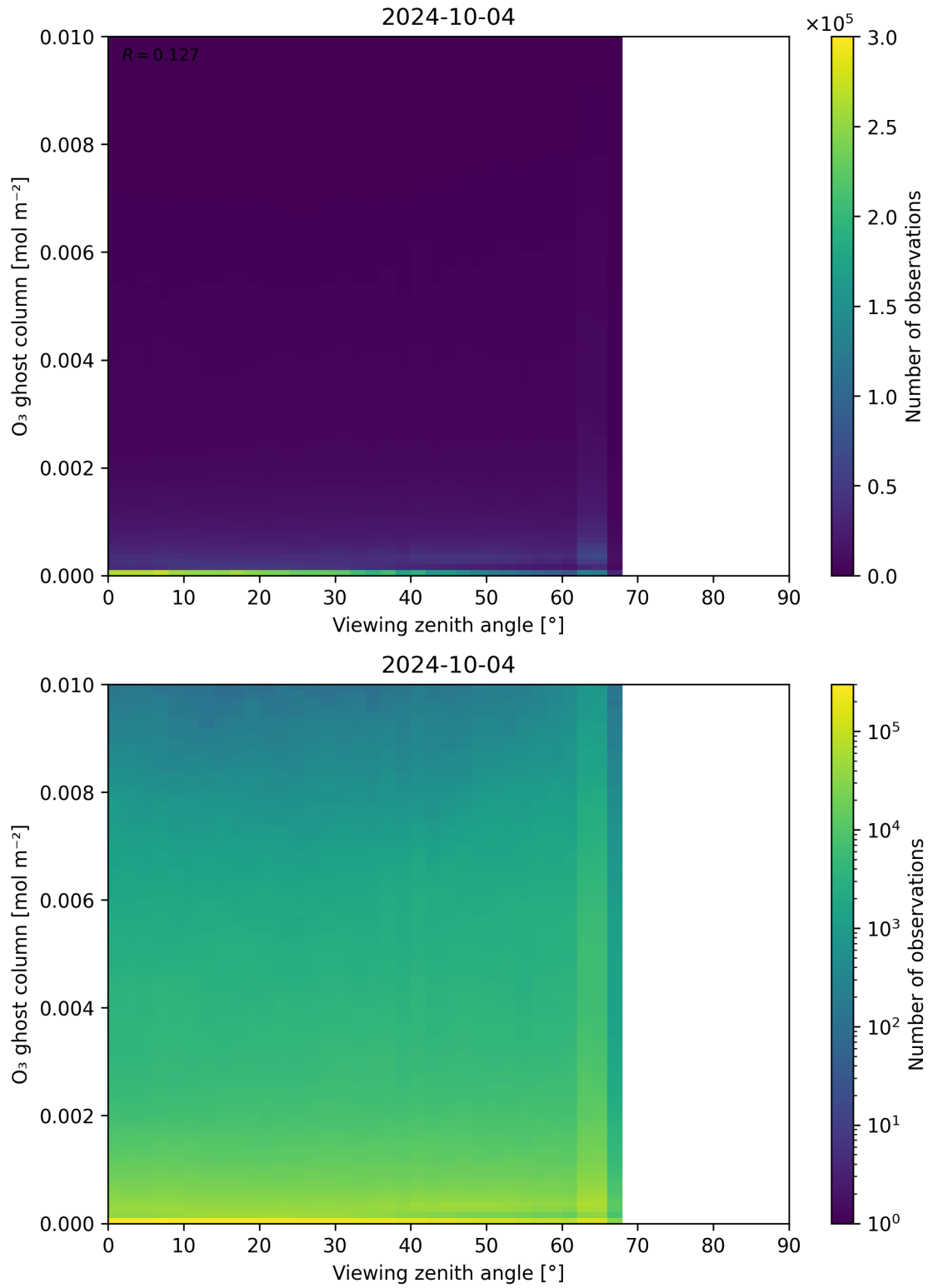
Figure 51: Scatter density plot of “Viewing zenith angle” against “O 3 ghost column” for 2024-10-03 to 2024-10-05.
