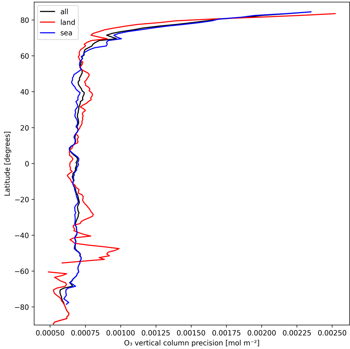
Figure 15: Zonal average of “O 3 vertical column precision” for 2024-10-03 to 2024-10-05.
