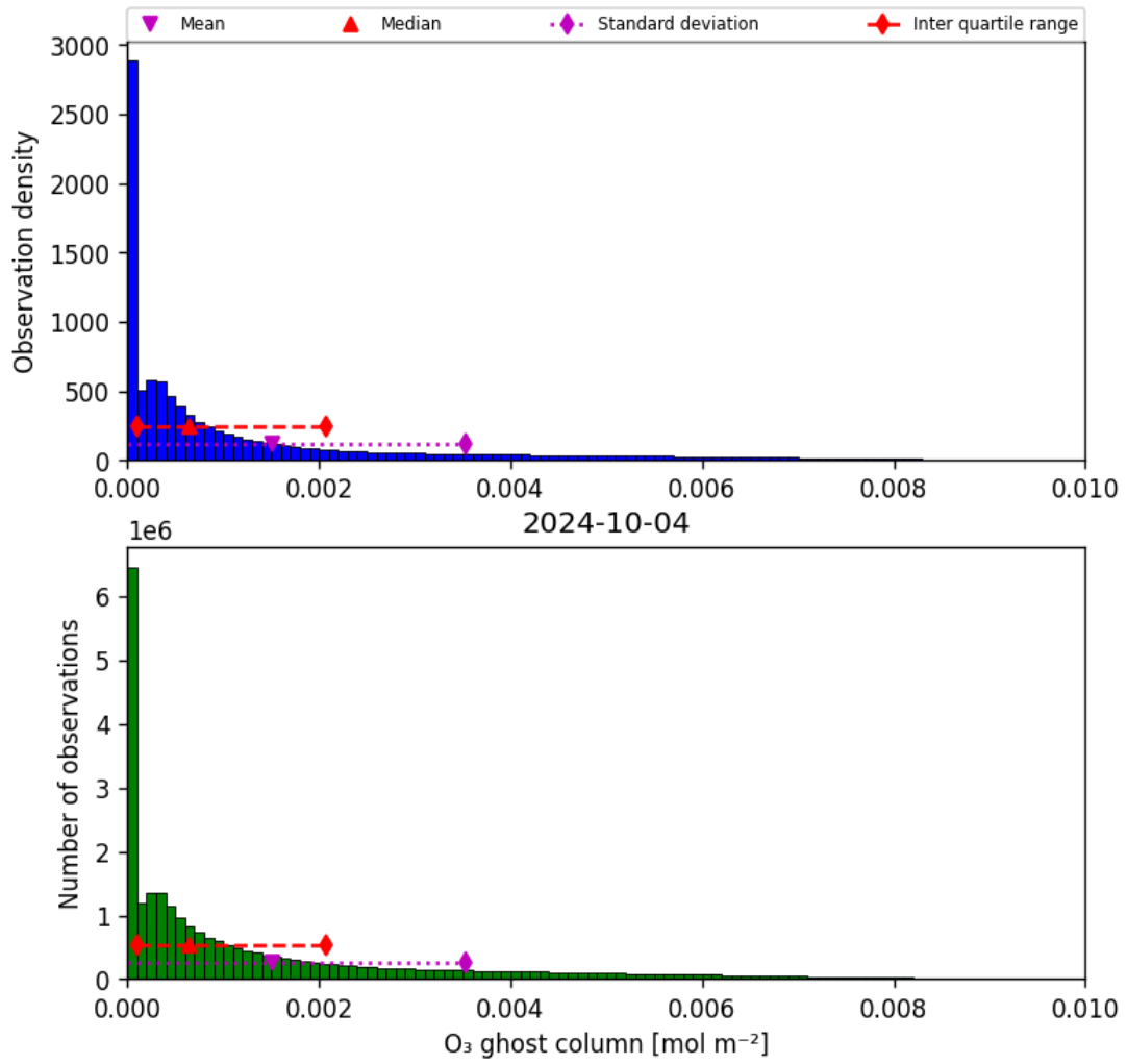
Figure 25: Histogram of “O 3 ghost column” for 2024-10-03 to 2024-10-05
