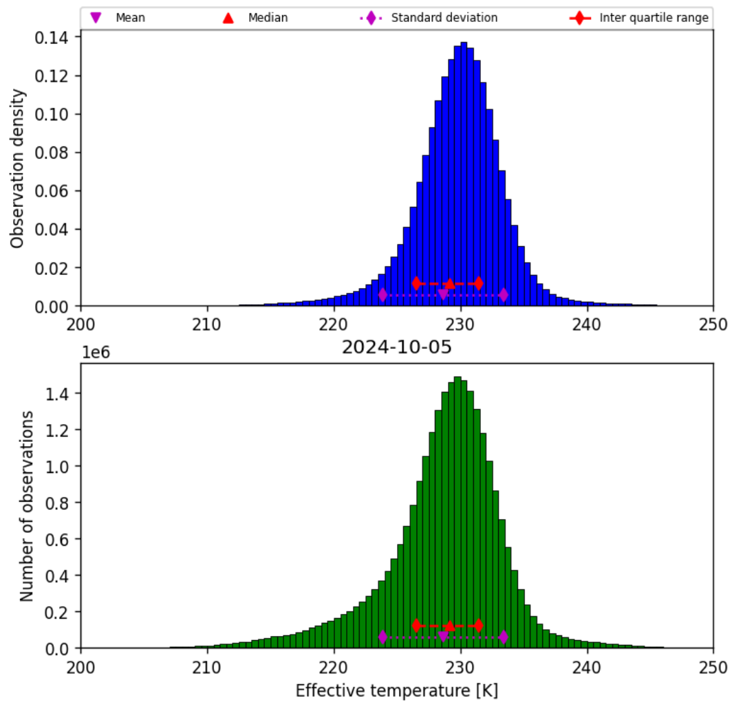
Figure 24: Histogram of “Effective temperature” for 2024-10-04 to 2024-10-06
