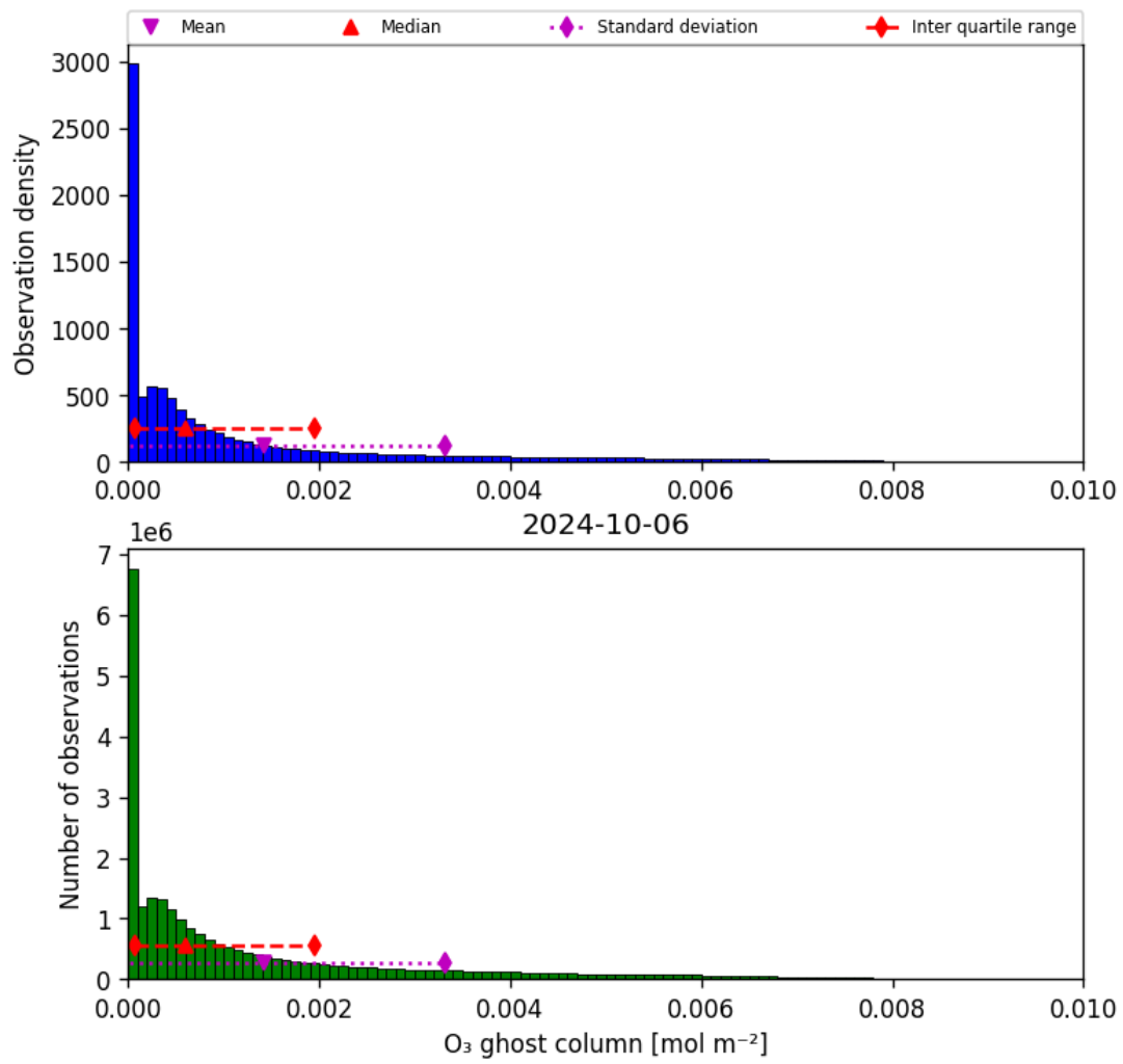
Figure 25: Histogram of “O 3 ghost column” for 2024-10-05 to 2024-10-07
