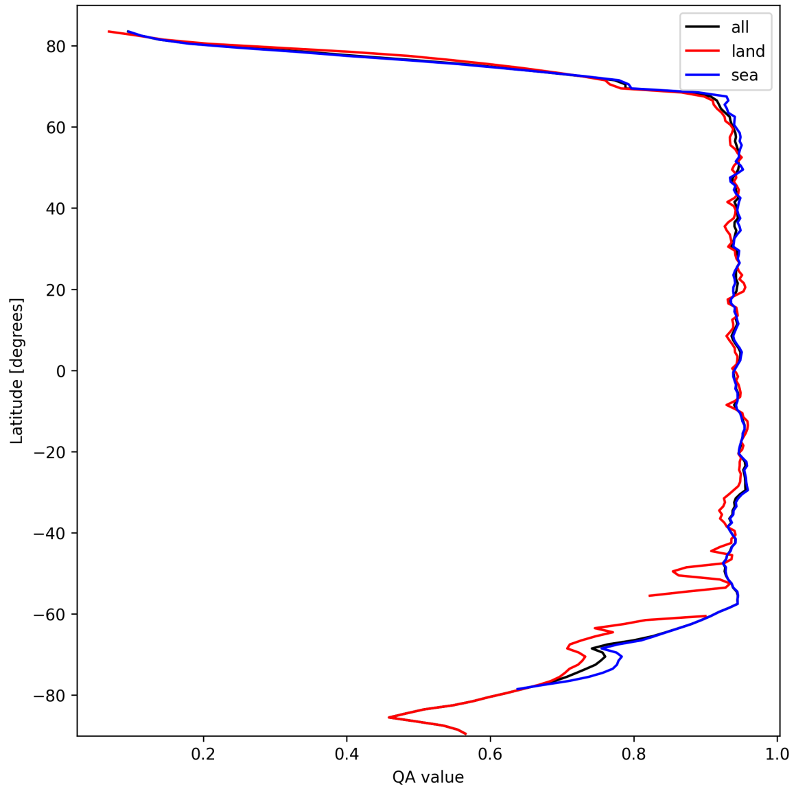
Figure 13: Zonal average of “QA value” for 2024-10-05 to 2024-10-07.
