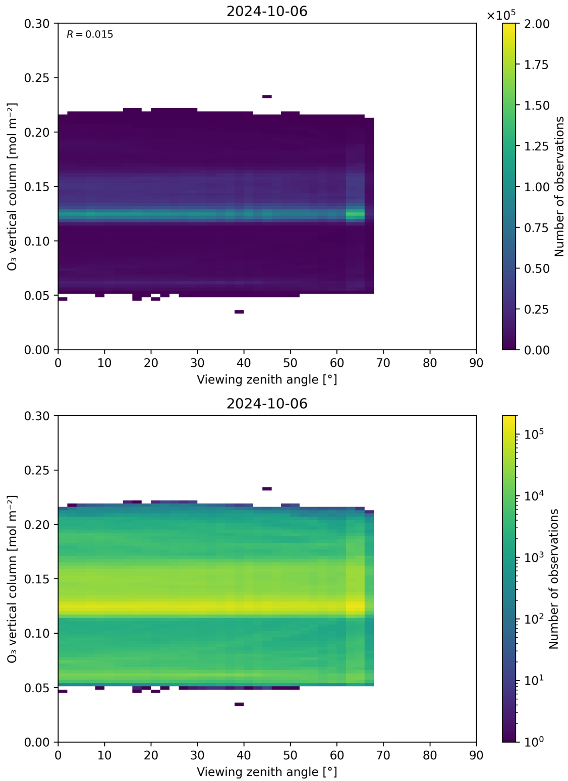
Figure 52: Scatter density plot of “Viewing zenith angle” against “O 3 vertical column” for 2024-10-05 to 2024-10-07.
