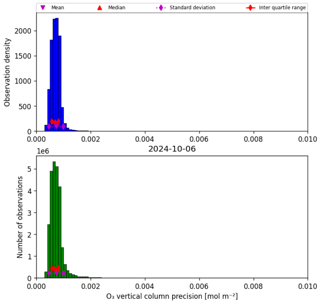
Figure 22: Histogram of "O 3 vertical column precision" for 2024-10-05 to 2024-10-07
