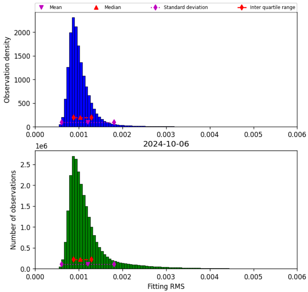
Figure 23: Histogram of “Fitting RMS” for 2024-10-05 to 2024-10-07
