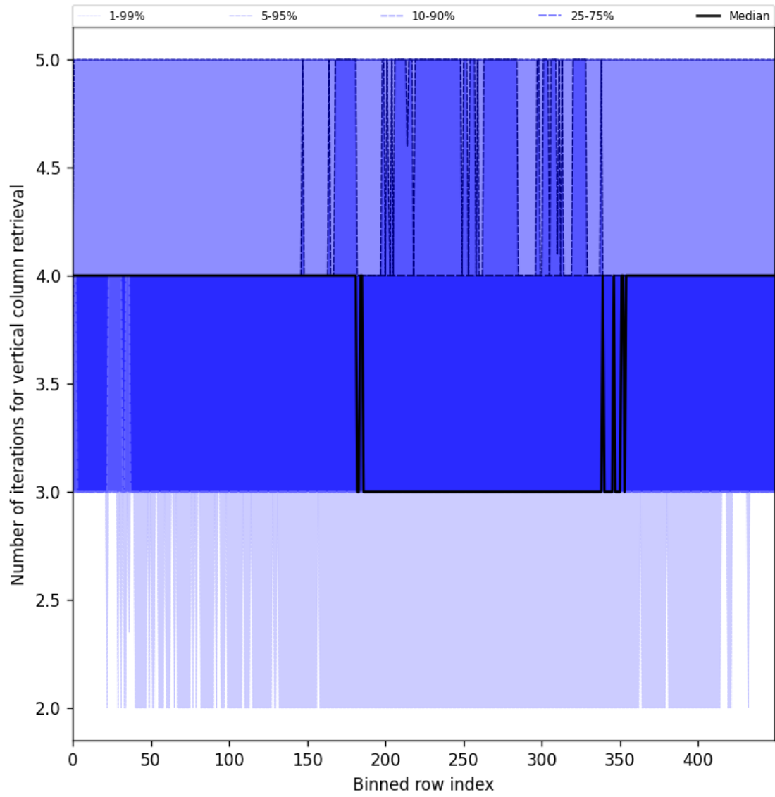
Figure 33: Along track statistics of “Number of iterations for vertical column retrieval” for 2024-10-05 to 2024-10-07
