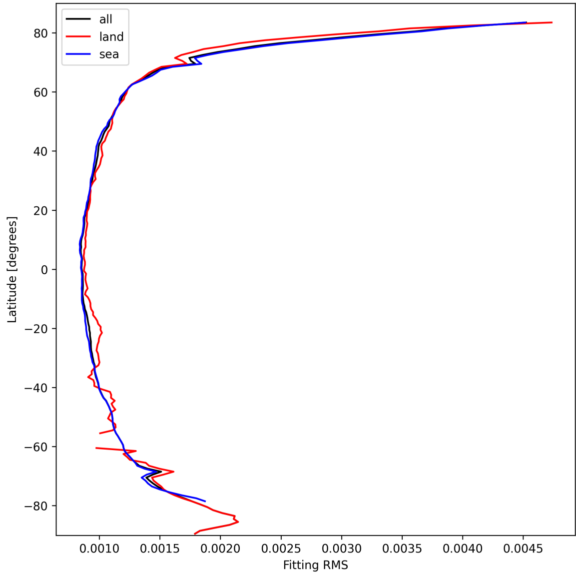
Figure 16: Zonal average of “Fitting RMS” for 2024-10-05 to 2024-10-07.
