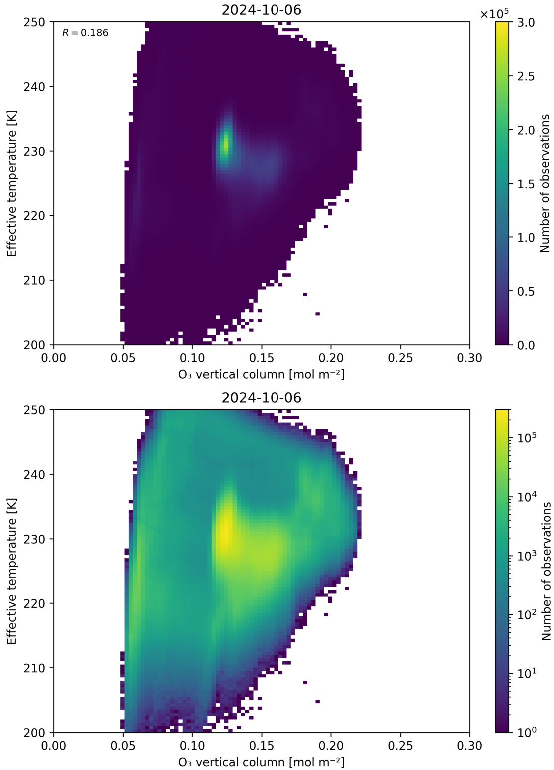
Figure 39: Scatter density plot of “O 3 vertical column” against “Effective temperature” for 2024-10-05 to 2024-10-07.
