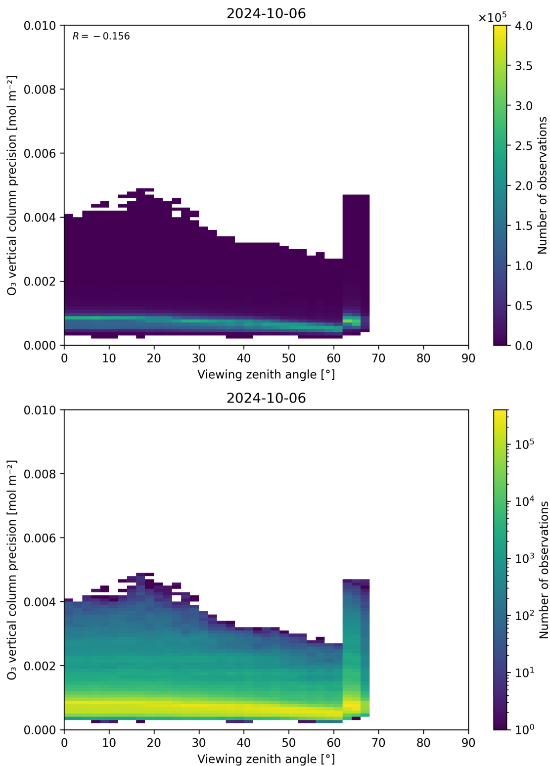
Figure 53: Scatter density plot of “Viewing zenith angle” against “O 3 vertical column precision” for 2024-10-05 to 2024-10-07.
