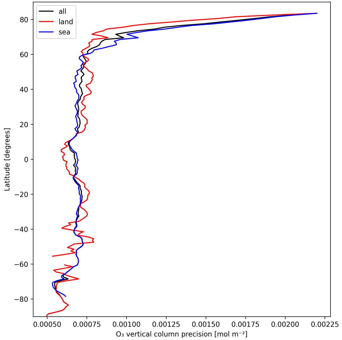
Figure 15: Zonal average of “O 3 vertical column precision” for 2024-10-05 to 2024-10-07.
