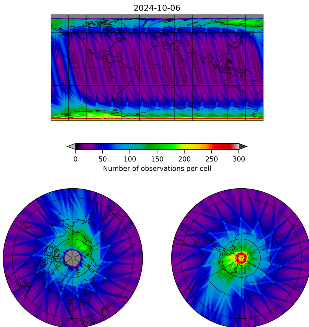
Figure 12: Map of the number of observations for 2024-10-05 to 2024-10-07
