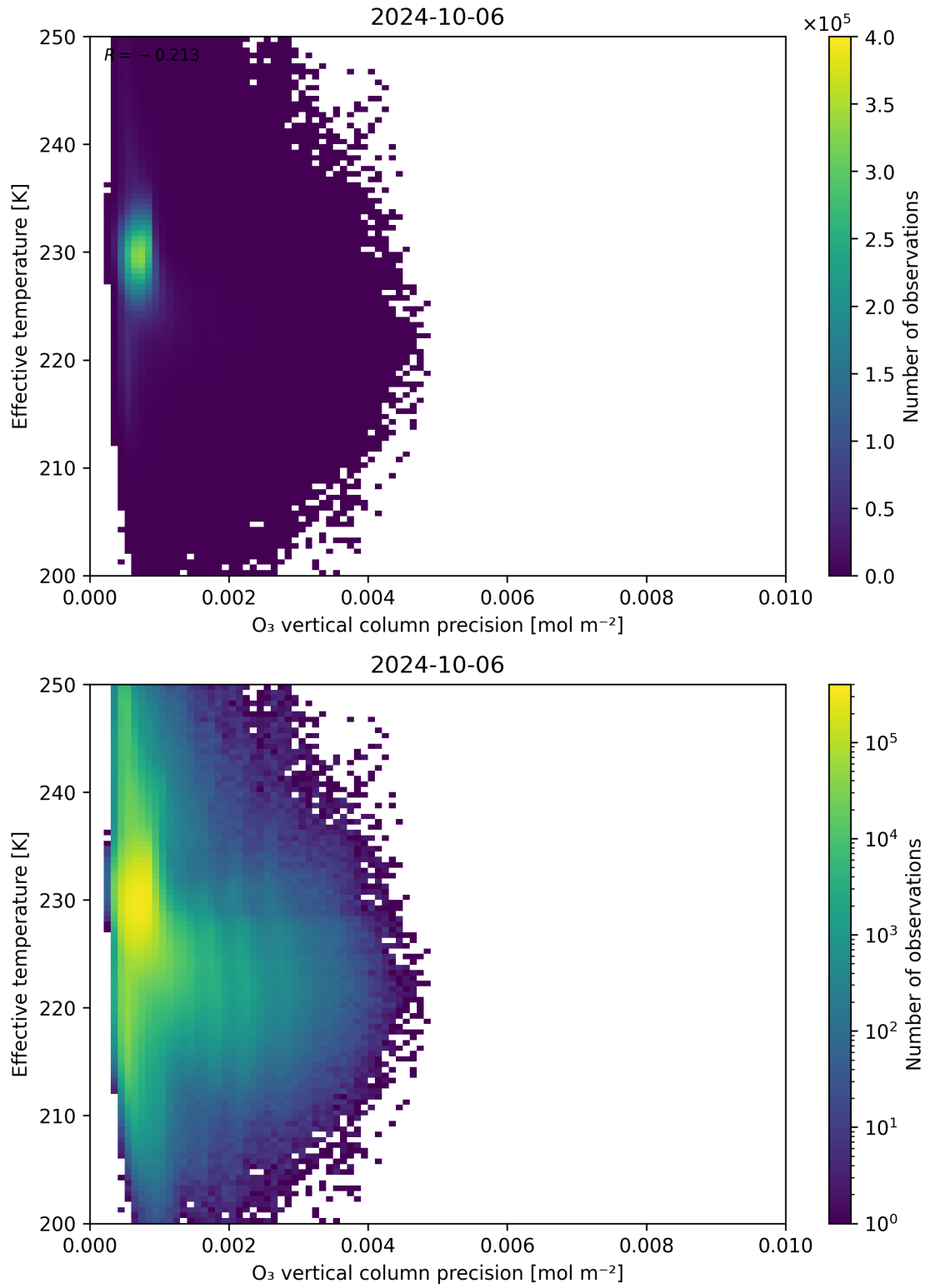
Figure 42: Scatter density plot of “O 3 vertical column precision” against “Effective temperature” for 2024-10-05 to 2024-10-07.
