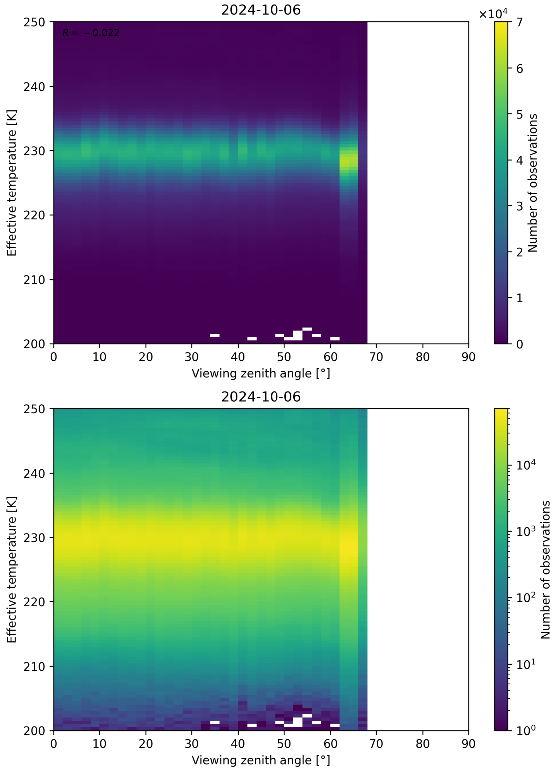
Figure 50: Scatter density plot of “Viewing zenith angle” against “Effective temperature” for 2024-10-05 to 2024-10-07.
