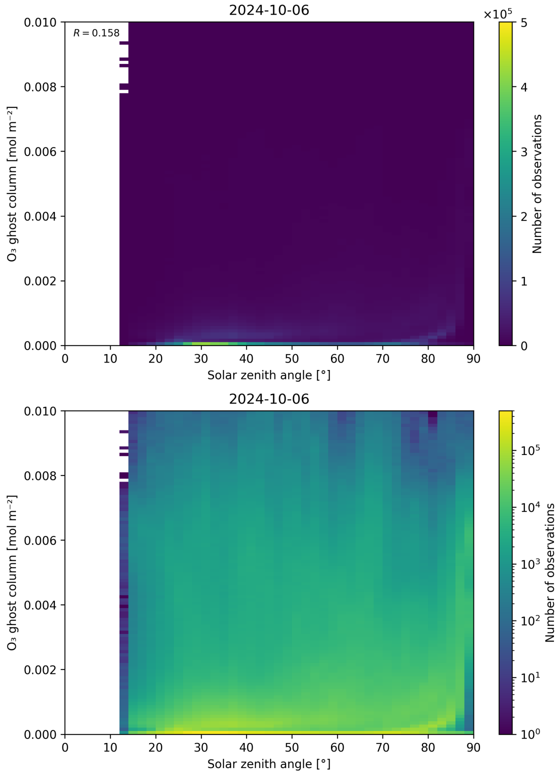
Figure 46: Scatter density plot of “Solar zenith angle” against “O 3 ghost column” for 2024-10-05 to 2024-10-07.
