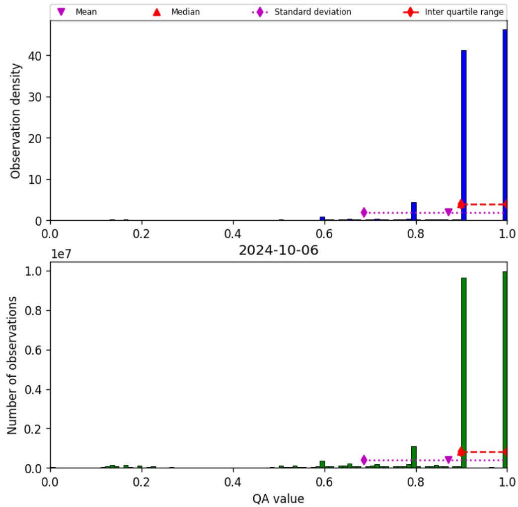
Figure 20: Histogram of “QA value” for 2024-10-05 to 2024-10-07
