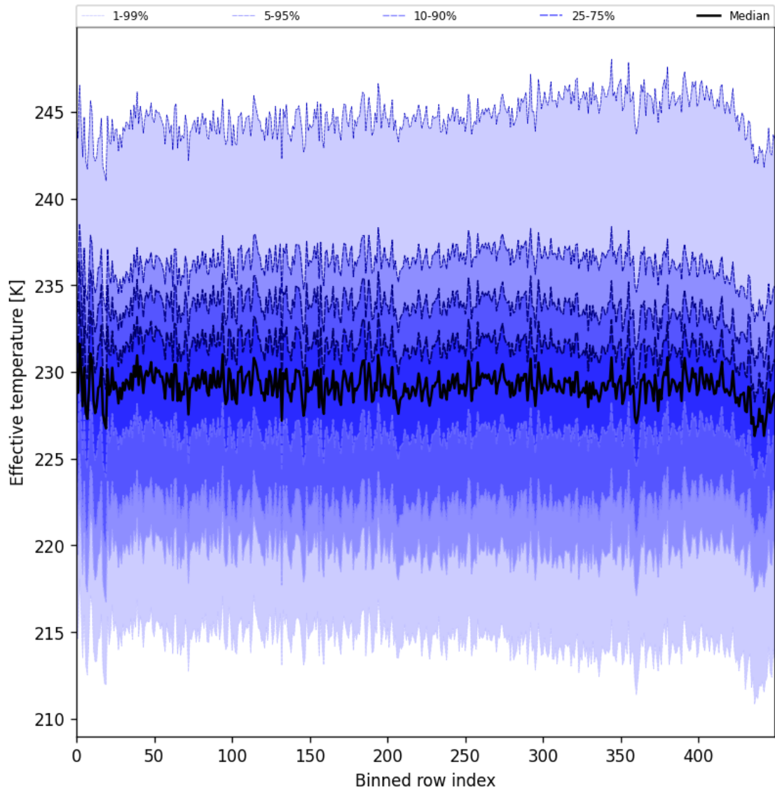
Figure 31: Along track statistics of “Effective temperature” for 2024-10-05 to 2024-10-07
