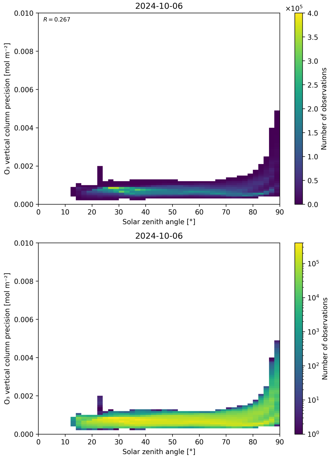
Figure 48: Scatter density plot of “Solar zenith angle” against “O 3 vertical column precision” for 2024-10-05 to 2024-10-07.
