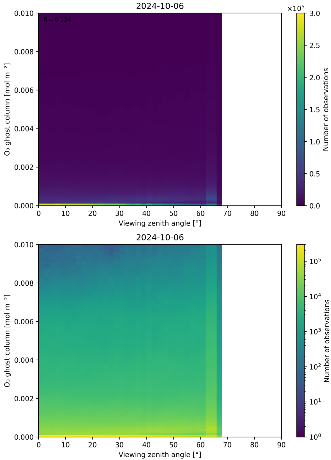
Figure 51: Scatter density plot of “Viewing zenith angle” against “O 3 ghost column” for 2024-10-05 to 2024-10-07.
