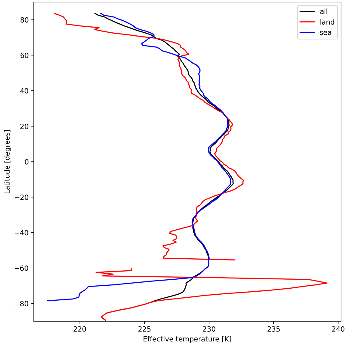
Figure 17: Zonal average of “Effective temperature” for 2024-10-05 to 2024-10-07.
