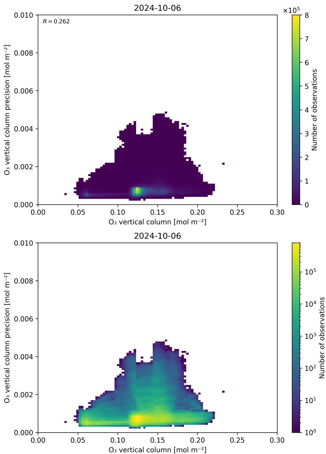
Figure 41: Scatter density plot of “O 3 vertical column” against “O 3 vertical column precision” for 2024-10-05 to 2024-10-07.
