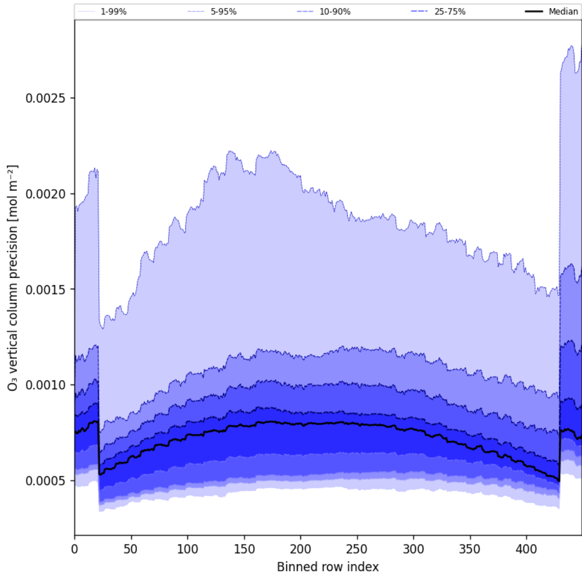
Figure 29: Along track statistics of “O 3 vertical column precision” for 2024-10-05 to 2024-10-07
