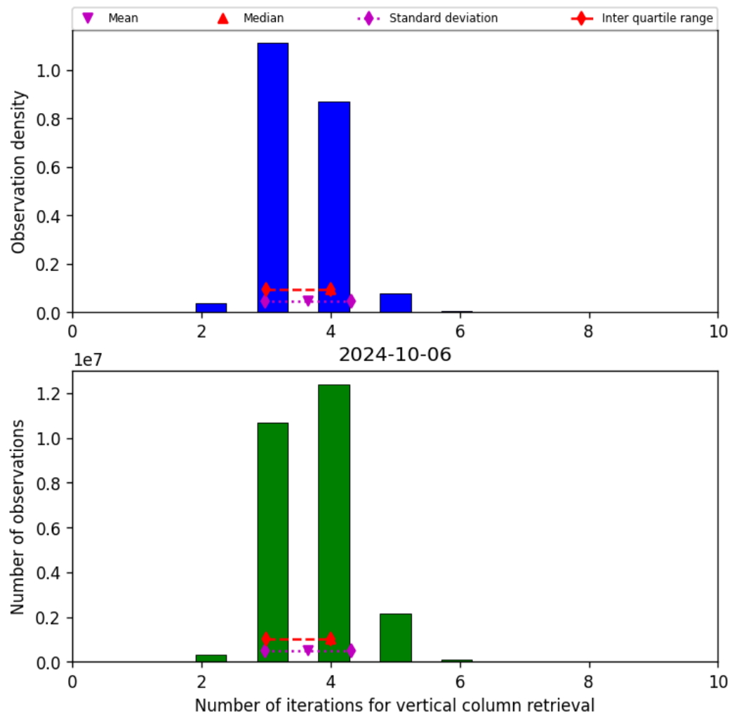
Figure 26: Histogram of “Number of iterations for vertical column retrieval” for 2024-10-05 to 2024-10-07
