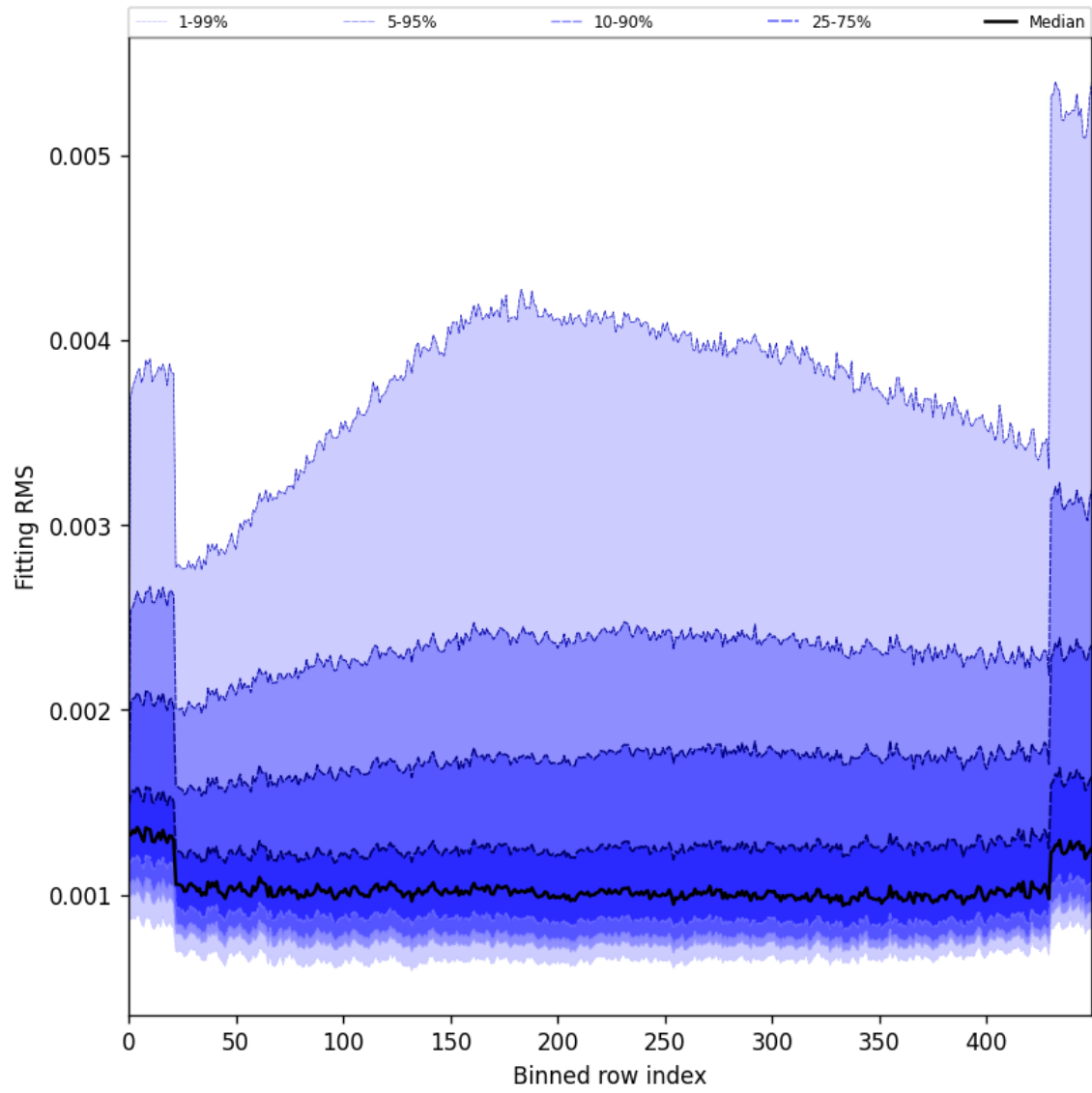
Figure 30: Along track statistics of “Fitting RMS” for 2024-10-05 to 2024-10-07
