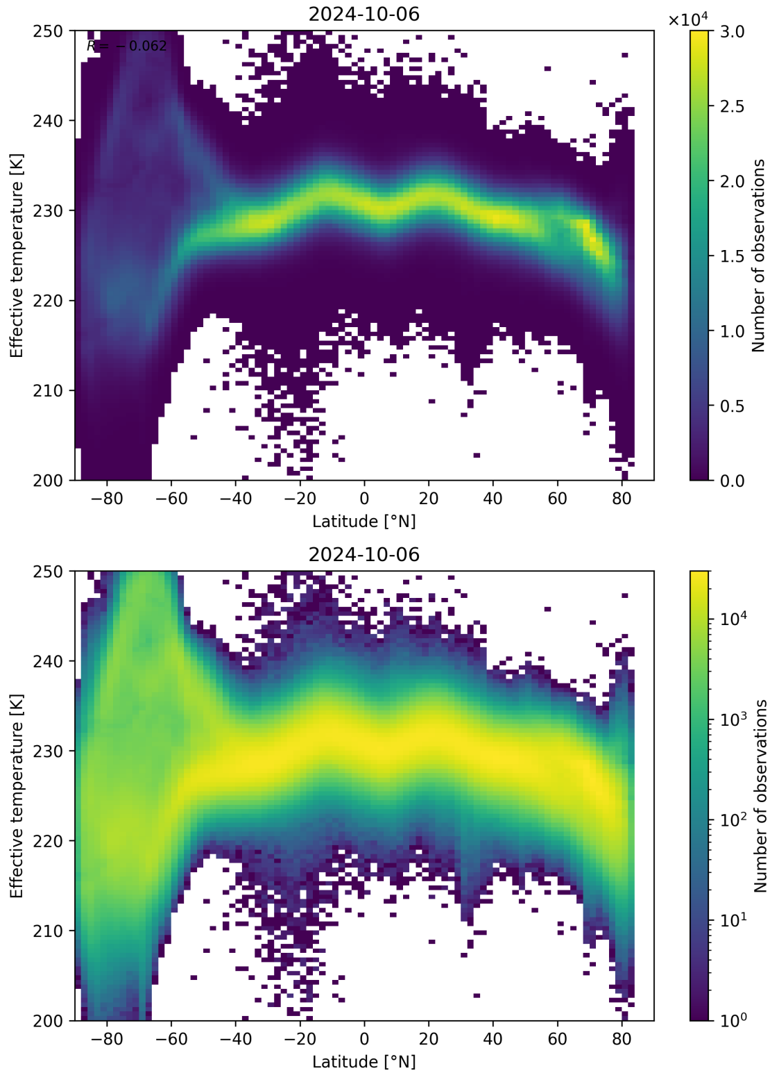
Figure 34: Scatter density plot of “Latitude” against “Effective temperature” for 2024-10-05 to 2024-10-07.
