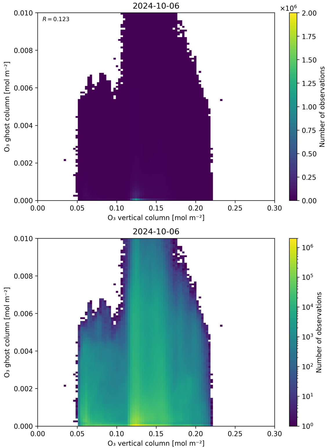
Figure 40: Scatter density plot of “O 3 vertical column” against “O 3 ghost column” for 2024-10-05 to 2024-10-07.
