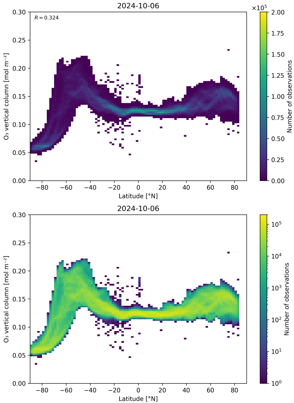
Figure 36: Scatter density plot of “Latitude” against “O 3 vertical column” for 2024-10-05 to 2024-10-07.
