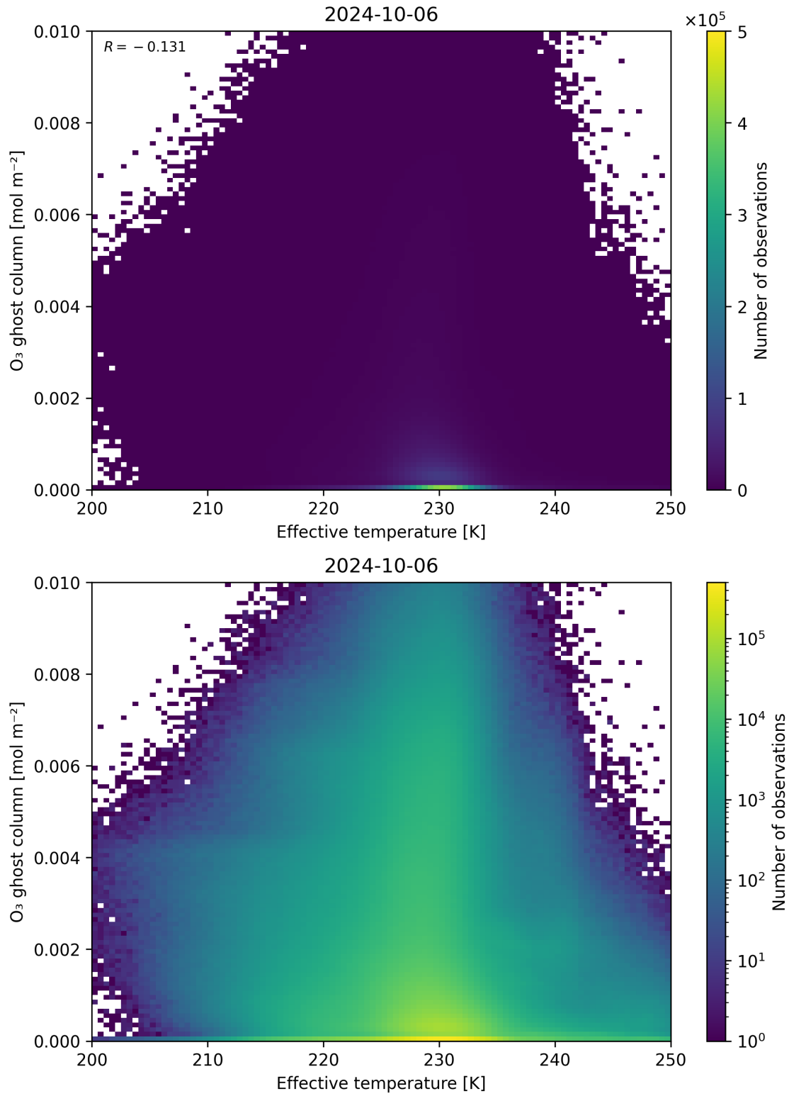
Figure 38: Scatter density plot of “Effective temperature” against “O 3 ghost column” for 2024-10-05 to 2024-10-07.
