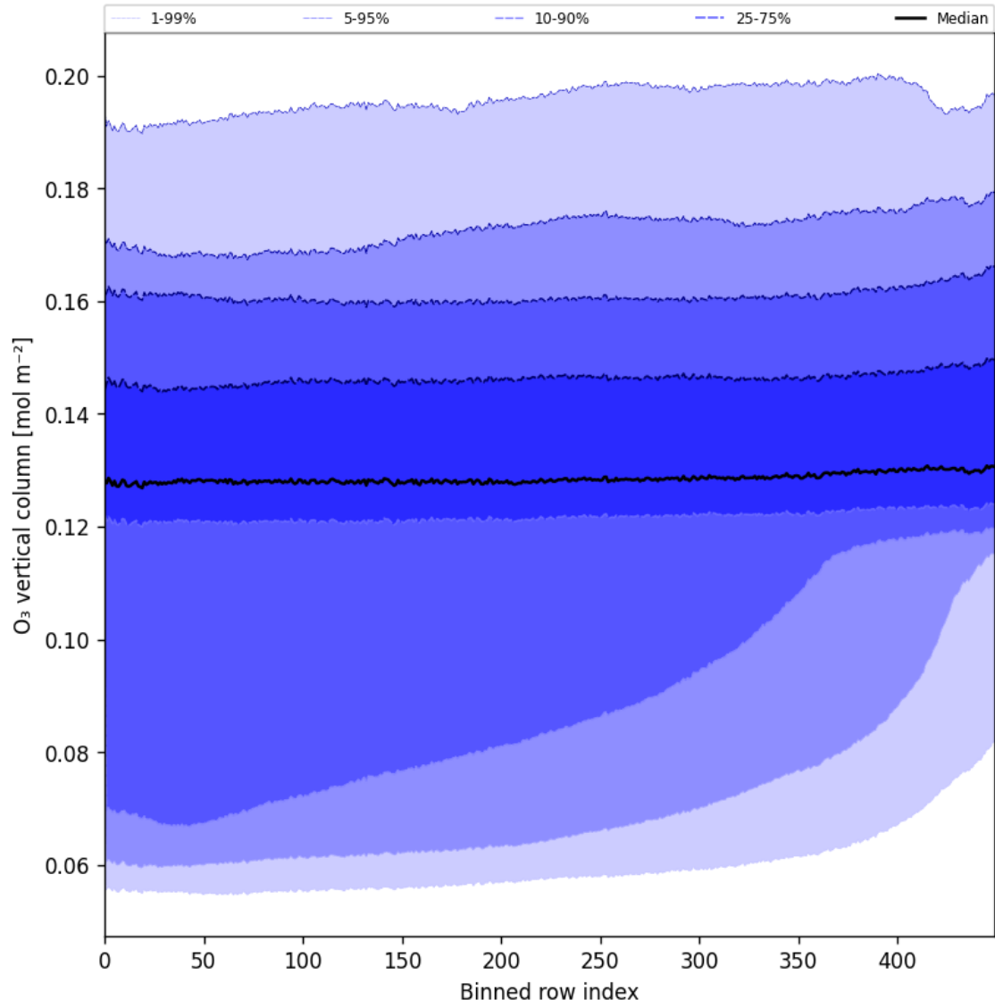
Figure 28: Along track statistics of “O 3 vertical column” for 2024-10-05 to 2024-10-07
