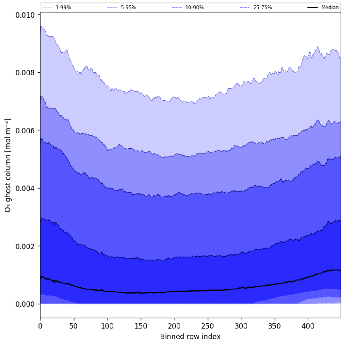
Figure 32: Along track statistics of “O 3 ghost column” for 2024-10-05 to 2024-10-07
