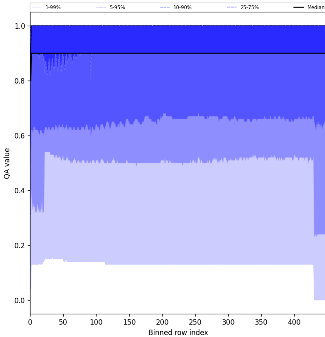
Figure 27: Along track statistics of “QA value” for 2024-10-05 to 2024-10-07
