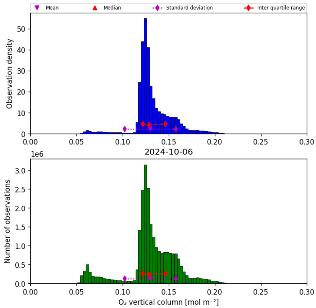
Figure 21: Histogram of “O 3 vertical column” for 2024-10-05 to 2024-10-07
