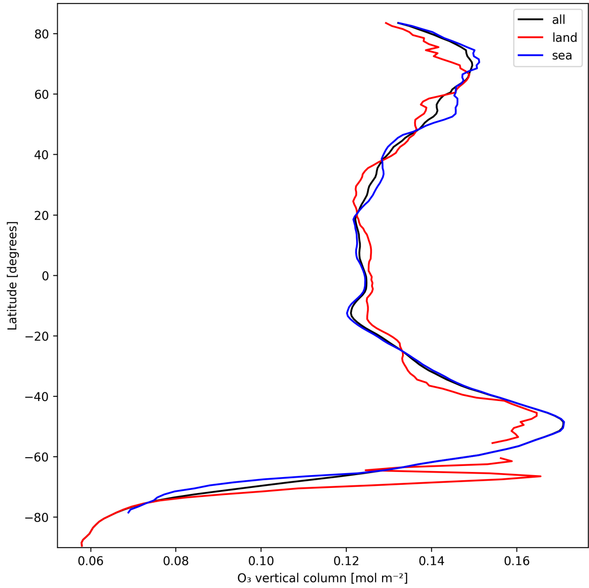
Figure 14: Zonal average of “O 3 vertical column” for 2024-10-05 to 2024-10-07.
