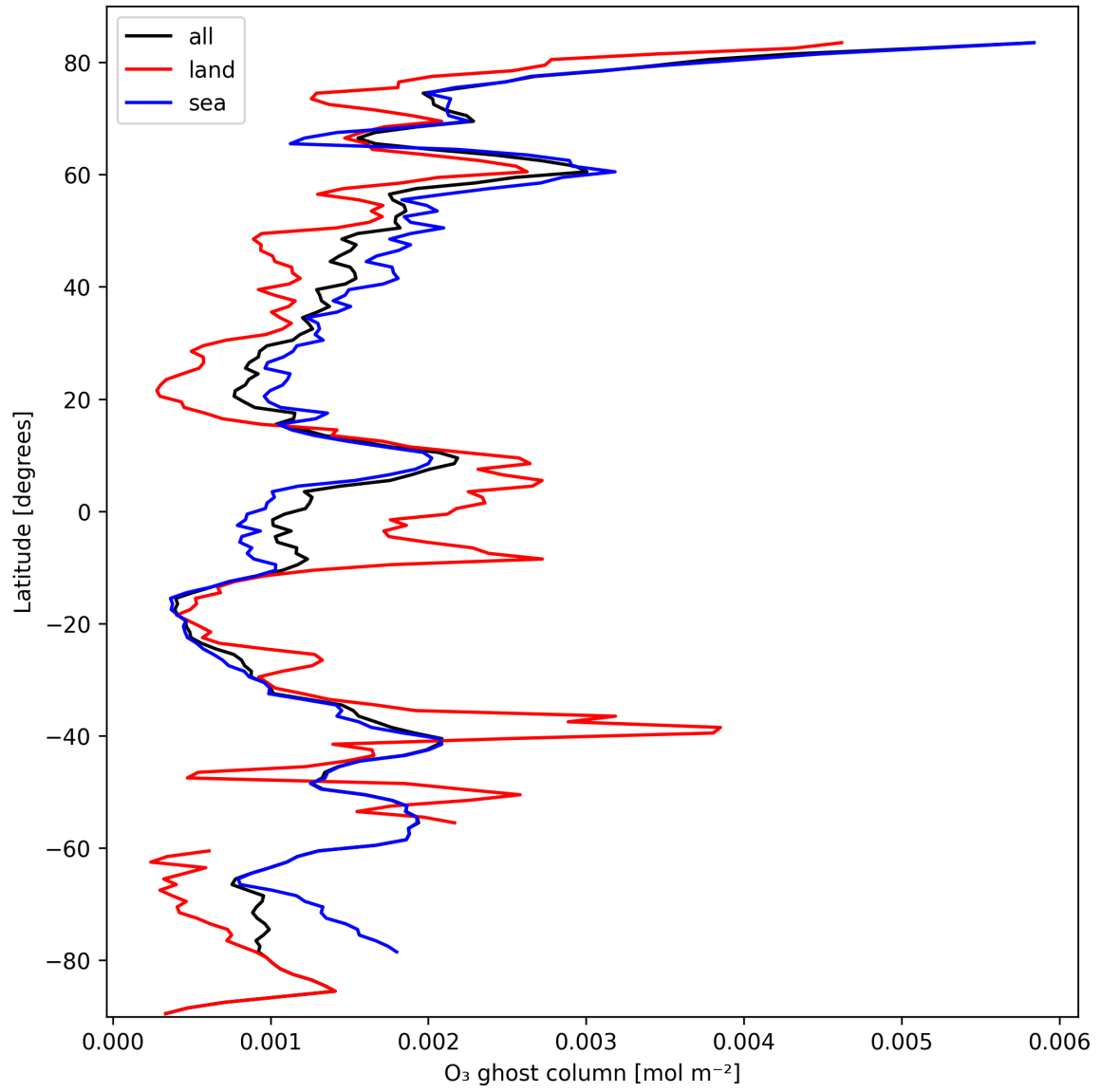
Figure 18: Zonal average of "O 3 ghost column" for 2024-10-05 to 2024-10-07.
