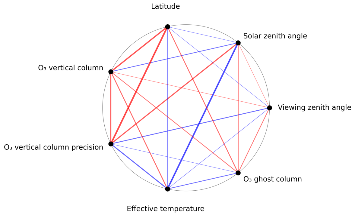
Figure 1: Map of correlation graph for 2024-10-05 to 2024-10-07.
