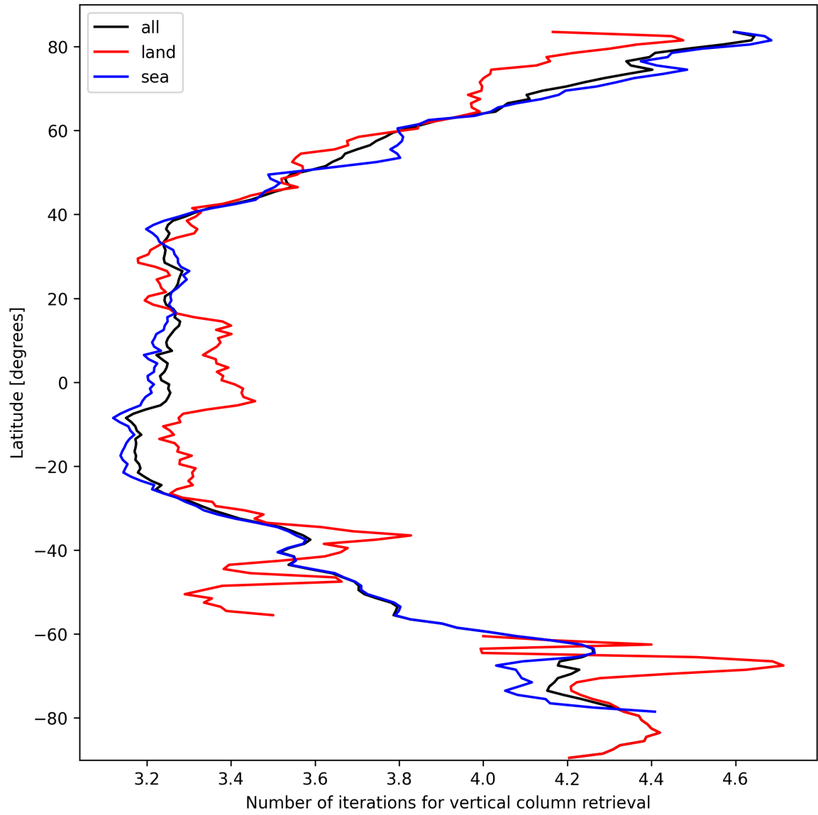
Figure 19: Zonal average of “Number of iterations for vertical column retrieval” for 2024-10-05 to 2024-10-07.
