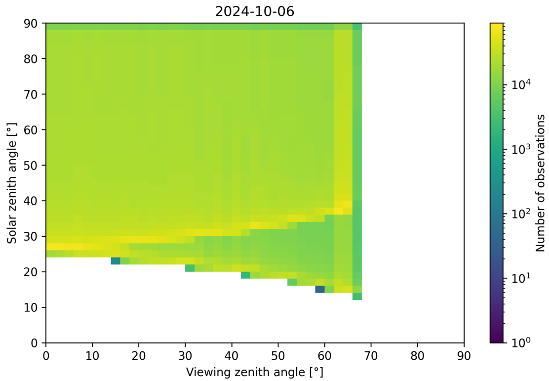
Figure 54: Scatter density plot of “Viewing zenith angle” against “Solar zenith angle” for 2024-10-05 to 2024-10-07.
