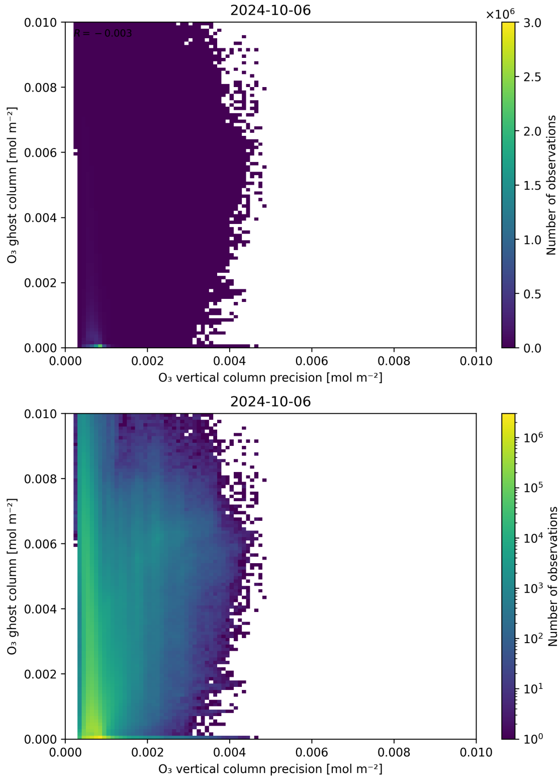
Figure 43: Scatter density plot of “O 3 vertical column precision” against “O 3 ghost column” for 2024-10-05 to 2024-10-07.
