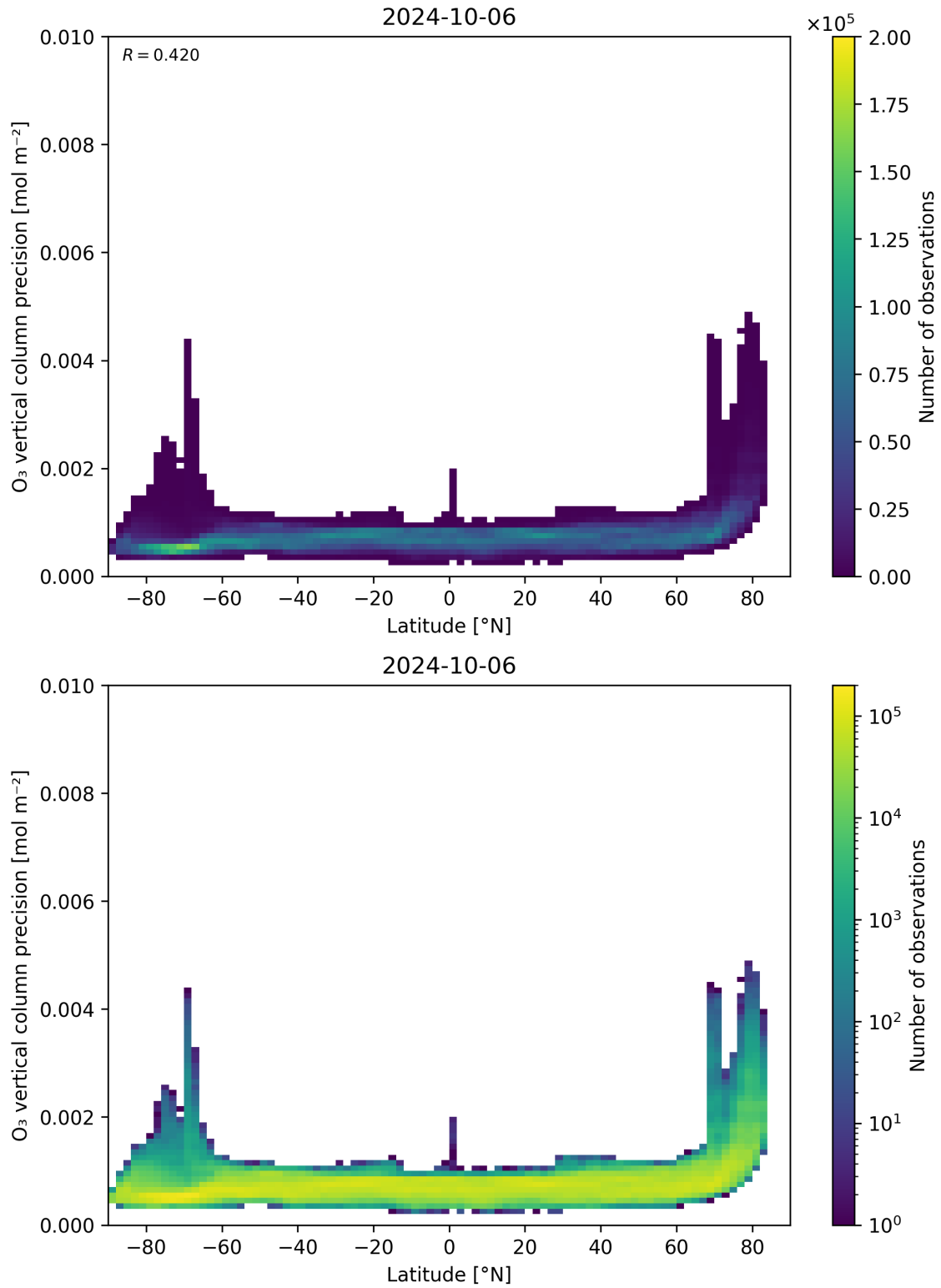
Figure 37: Scatter density plot of “Latitude” against “O 3 vertical column precision” for 2024-10-05 to 2024-10-07.
