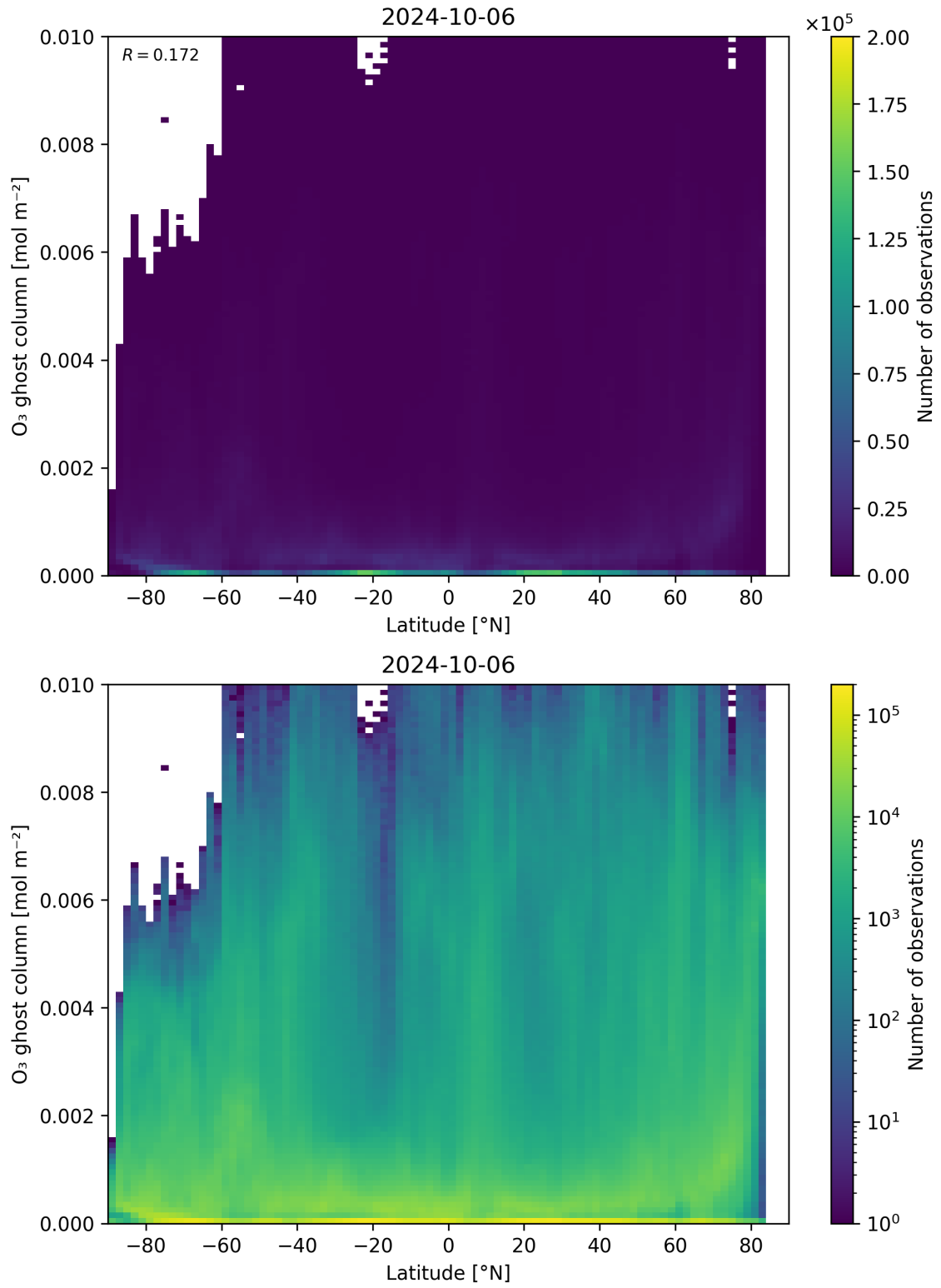
Figure 35: Scatter density plot of “Latitude” against “O 3 ghost column” for 2024-10-05 to 2024-10-07.
