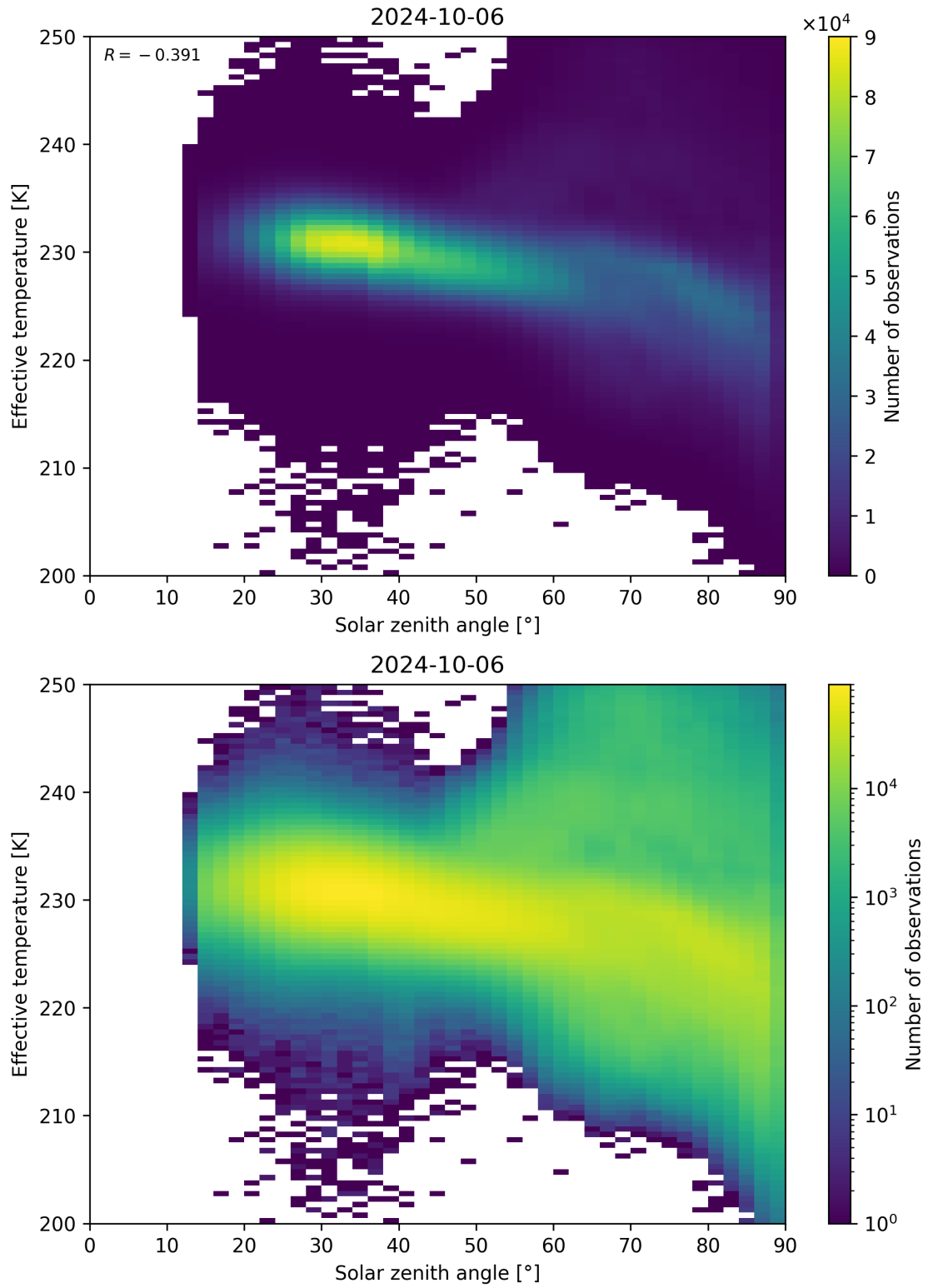
Figure 45: Scatter density plot of “Solar zenith angle” against “Effective temperature” for 2024-10-05 to 2024-10-07.
