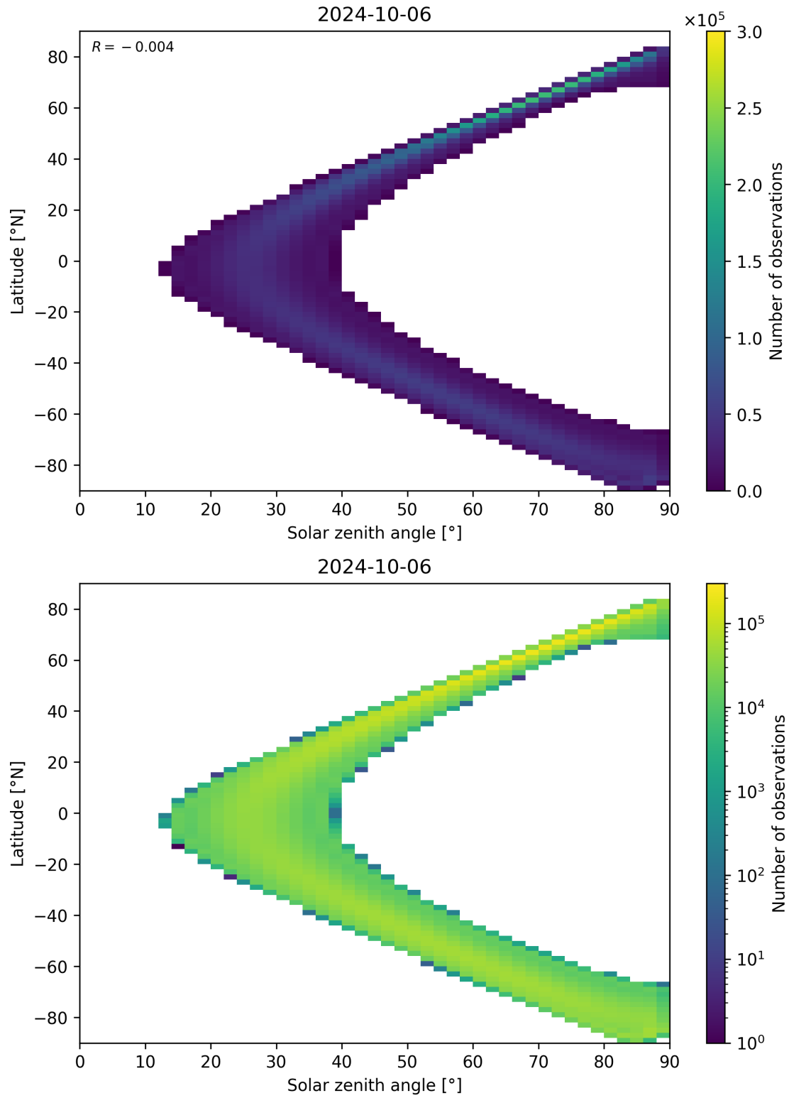
Figure 44: Scatter density plot of “Solar zenith angle” against “Latitude” for 2024-10-05 to 2024-10-07.
