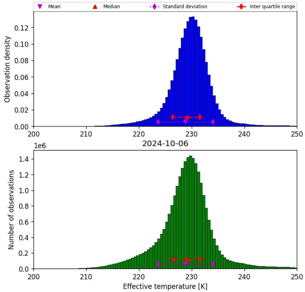
Figure 24: Histogram of “Effective temperature” for 2024-10-05 to 2024-10-07
