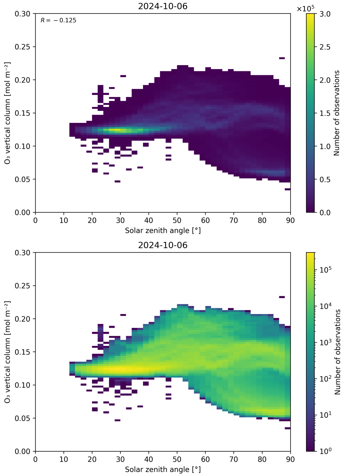
Figure 47: Scatter density plot of “Solar zenith angle” against “O 3 vertical column” for 2024-10-05 to 2024-10-07.
