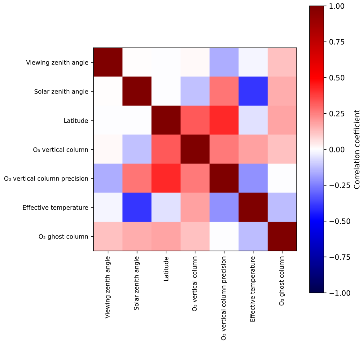
Figure 2: Map of correlation matrix for 2024-10-05 to 2024-10-07.
