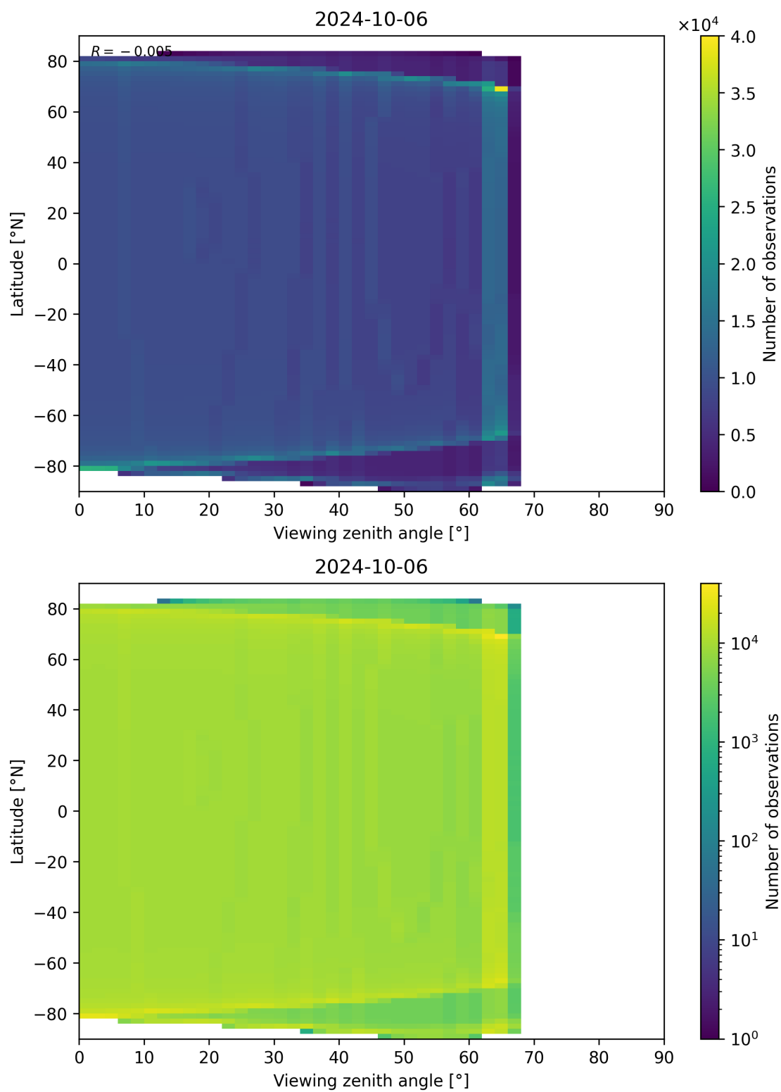
Figure 49: Scatter density plot of “Viewing zenith angle” against “Latitude” for 2024-10-05 to 2024-10-07.
