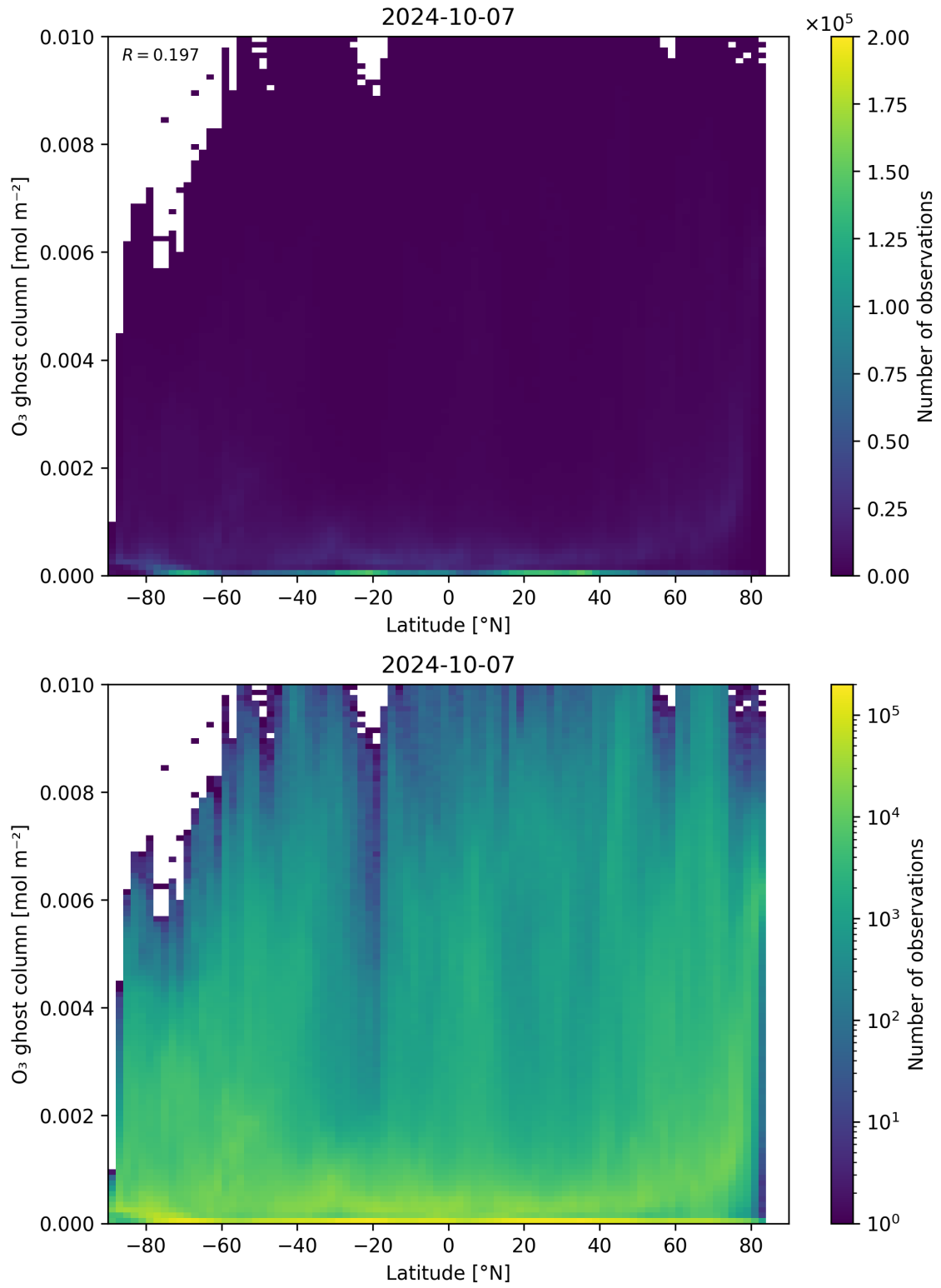
Figure 35: Scatter density plot of “Latitude” against “O 3 ghost column” for 2024-10-06 to 2024-10-08.
