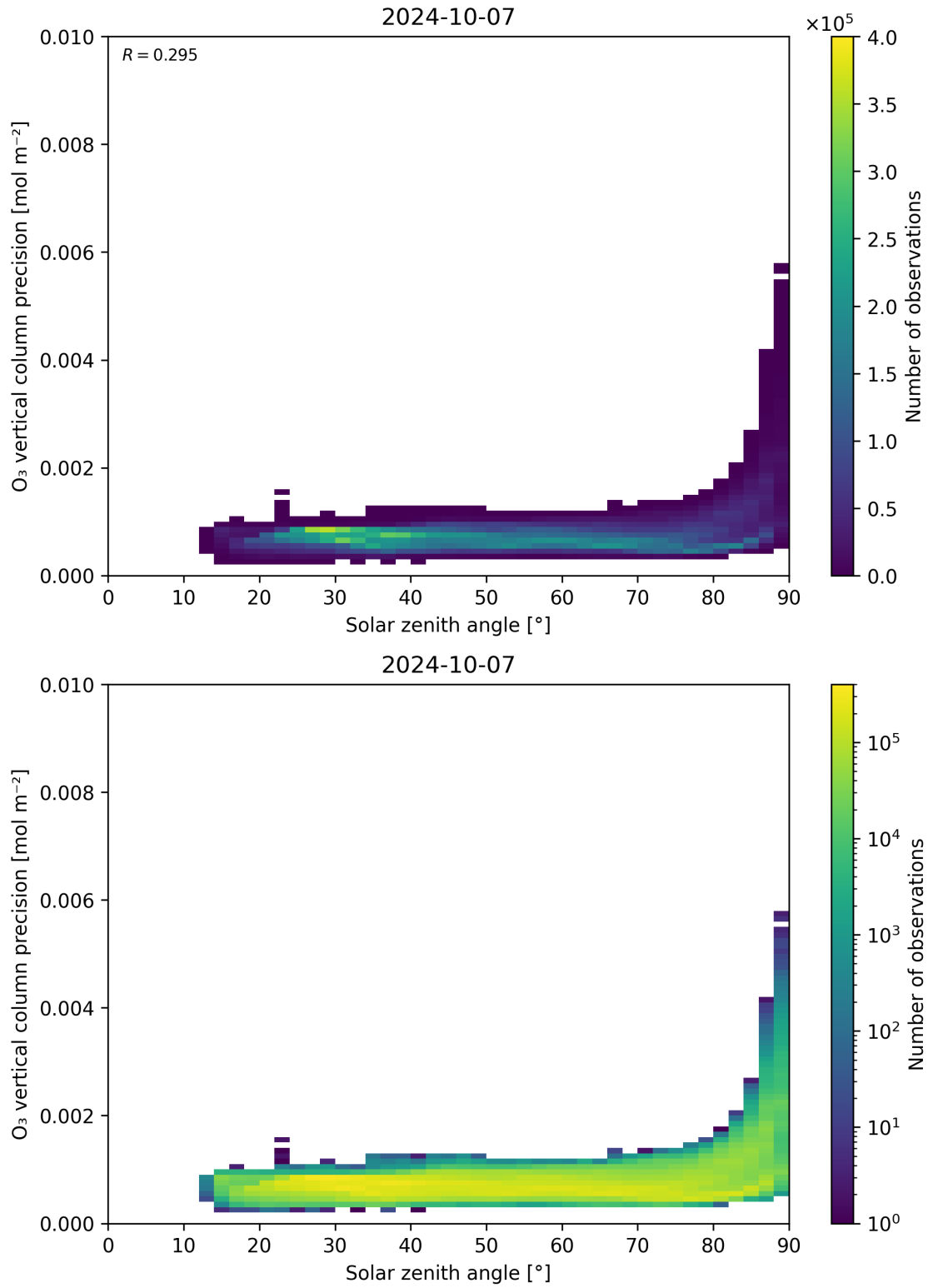
Figure 48: Scatter density plot of “Solar zenith angle” against “O 3 vertical column precision” for 2024-10-06 to 2024-10-08.
