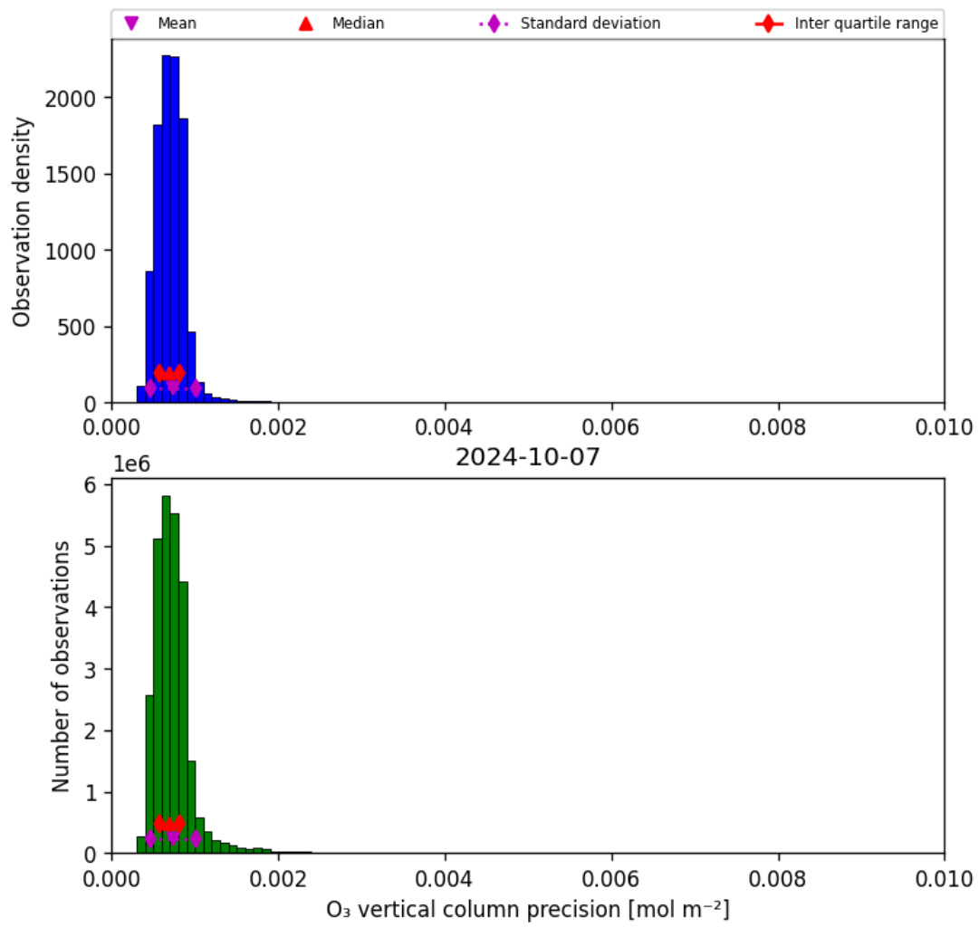
Figure 22: Histogram of “O 3 vertical column precision” for 2024-10-06 to 2024-10-08
