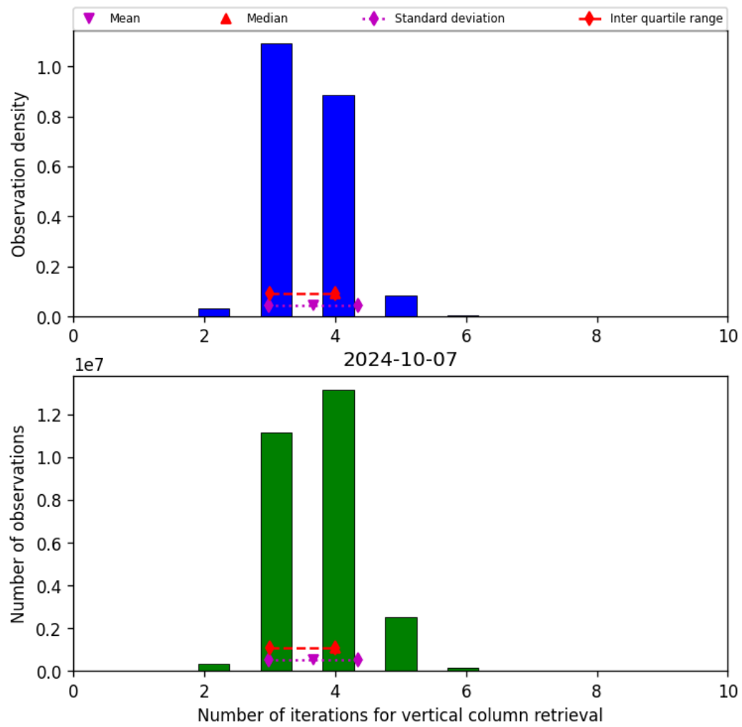
Figure 26: Histogram of “Number of iterations for vertical column retrieval” for 2024-10-06 to 2024-10-08
