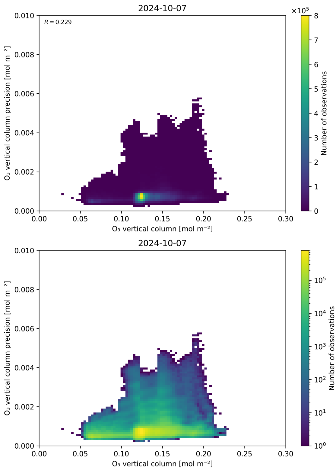
Figure 41: Scatter density plot of “O 3 vertical column” against “O 3 vertical column precision” for 2024-10-06 to 2024-10-08.
