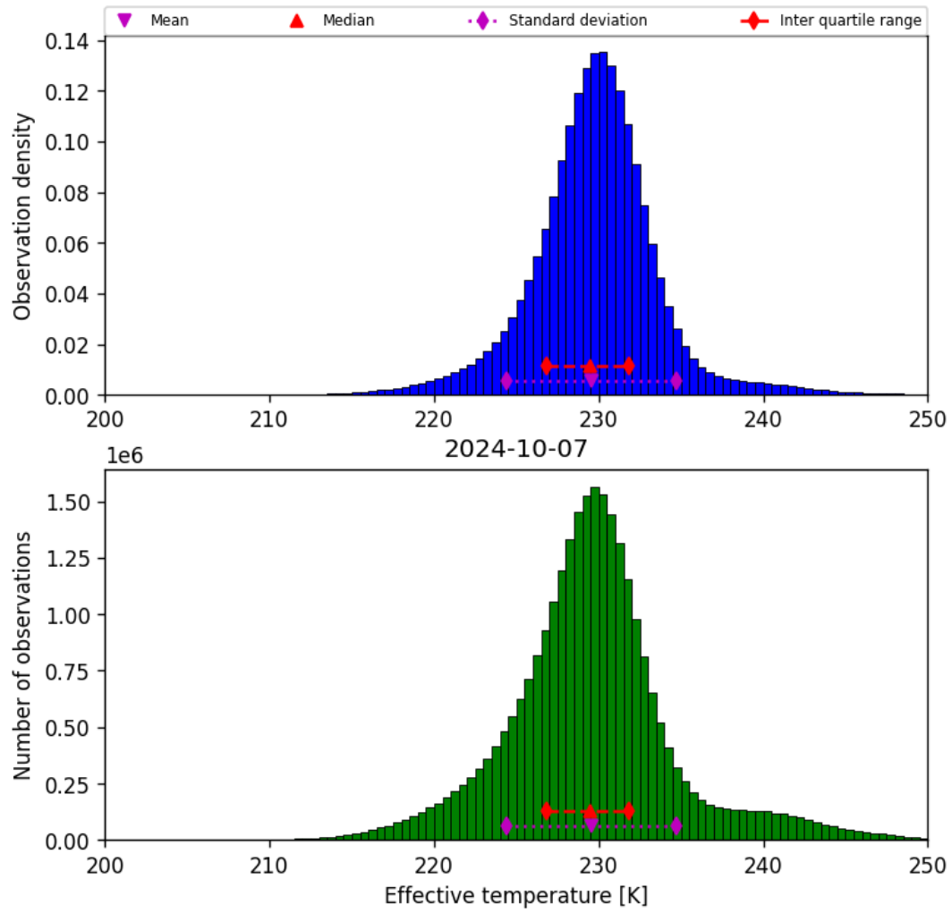
Figure 24: Histogram of “Effective temperature” for 2024-10-06 to 2024-10-08
