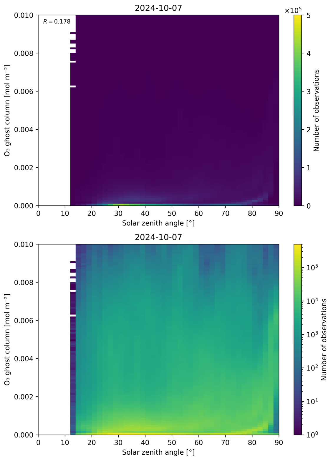
Figure 46: Scatter density plot of “Solar zenith angle” against “O 3 ghost column” for 2024-10-06 to 2024-10-08.
