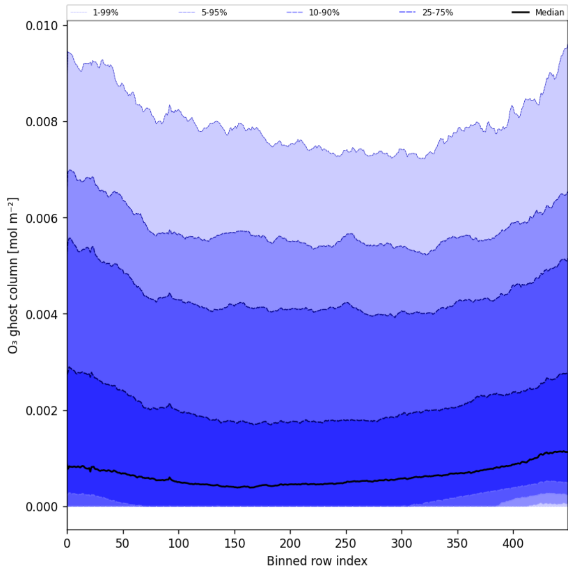
Figure 32: Along track statistics of “O 3 ghost column” for 2024-10-06 to 2024-10-08
