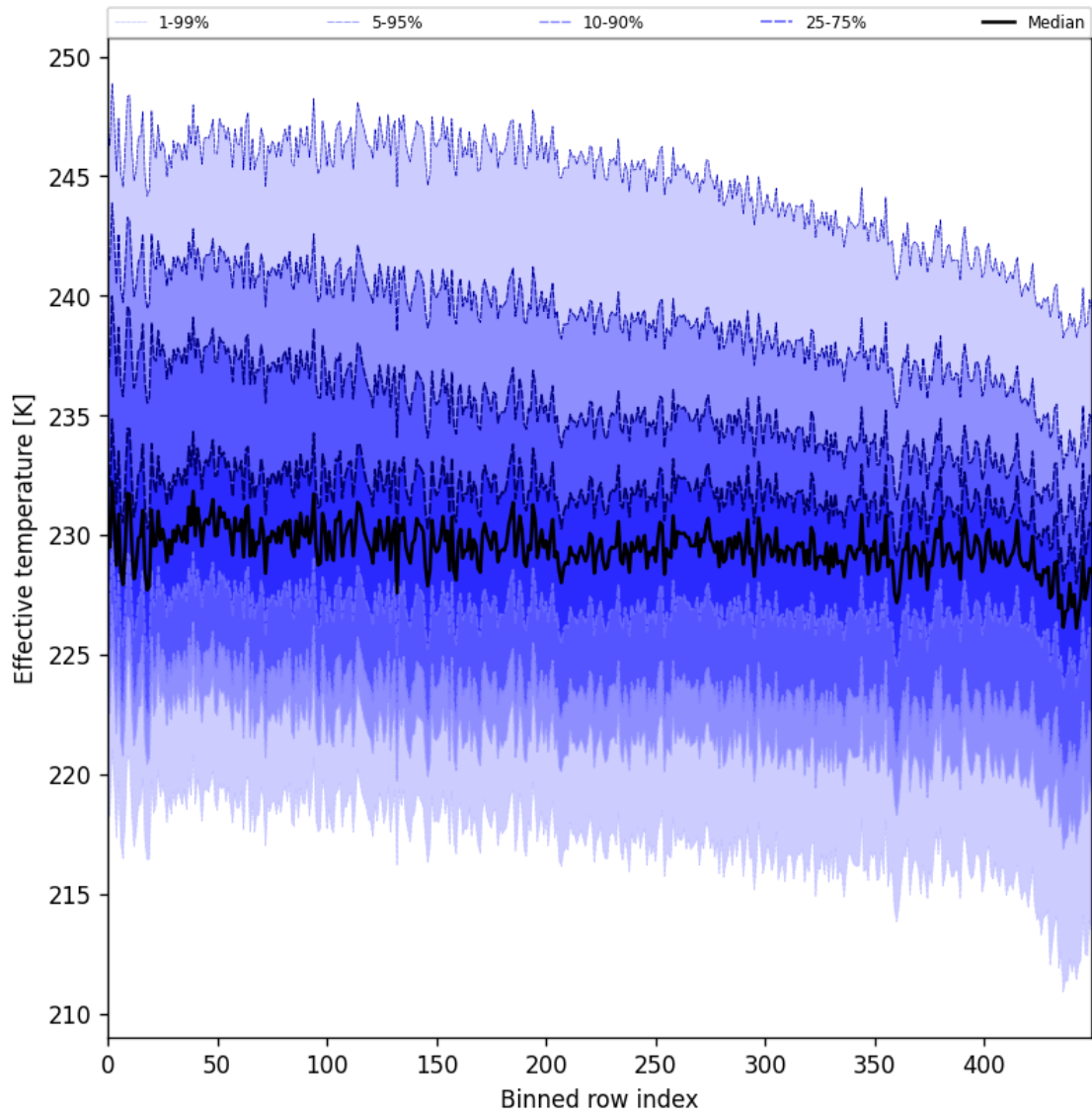
Figure 31: Along track statistics of “Effective temperature” for 2024-10-06 to 2024-10-08
