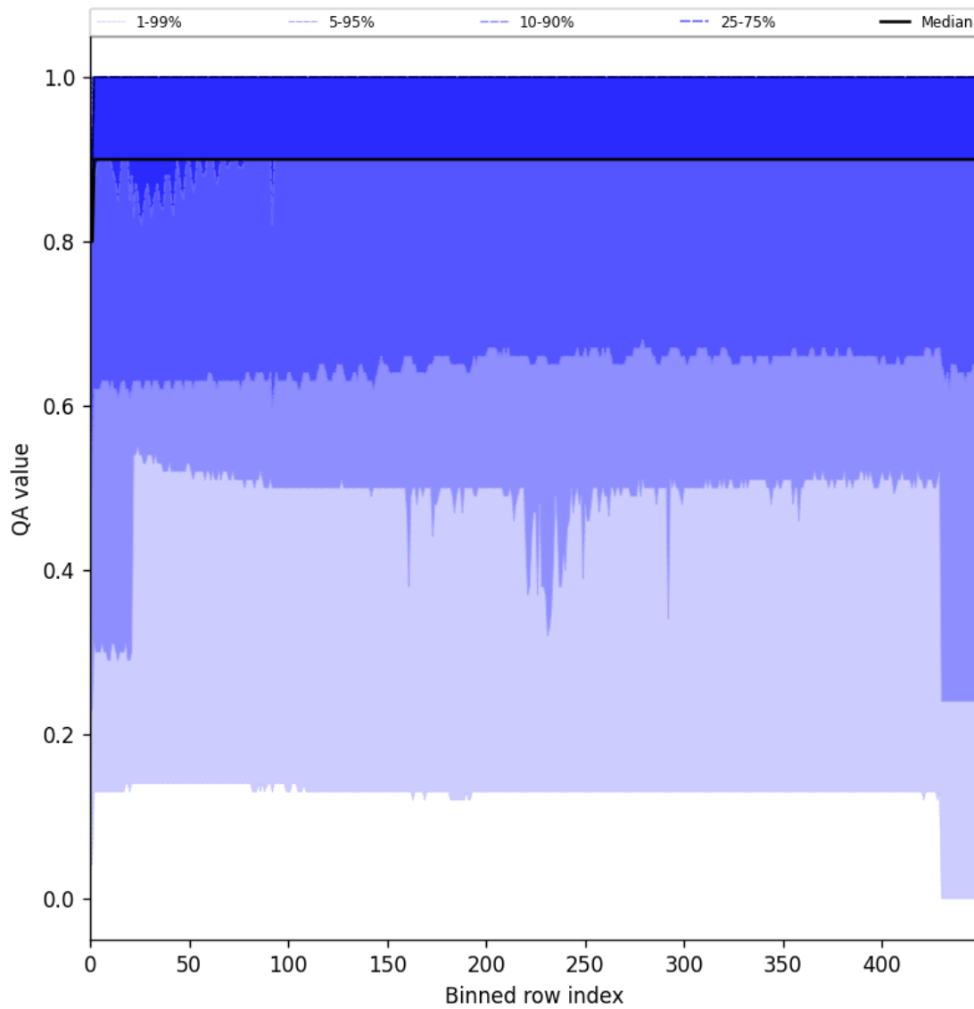
Figure 27: Along track statistics of “QA value” for 2024-10-06 to 2024-10-08
