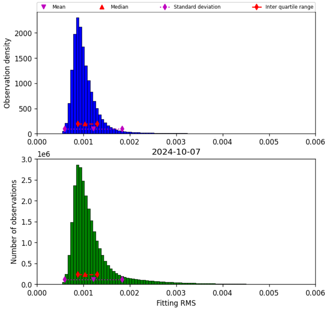
Figure 23: Histogram of “Fitting RMS” for 2024-10-06 to 2024-10-08
