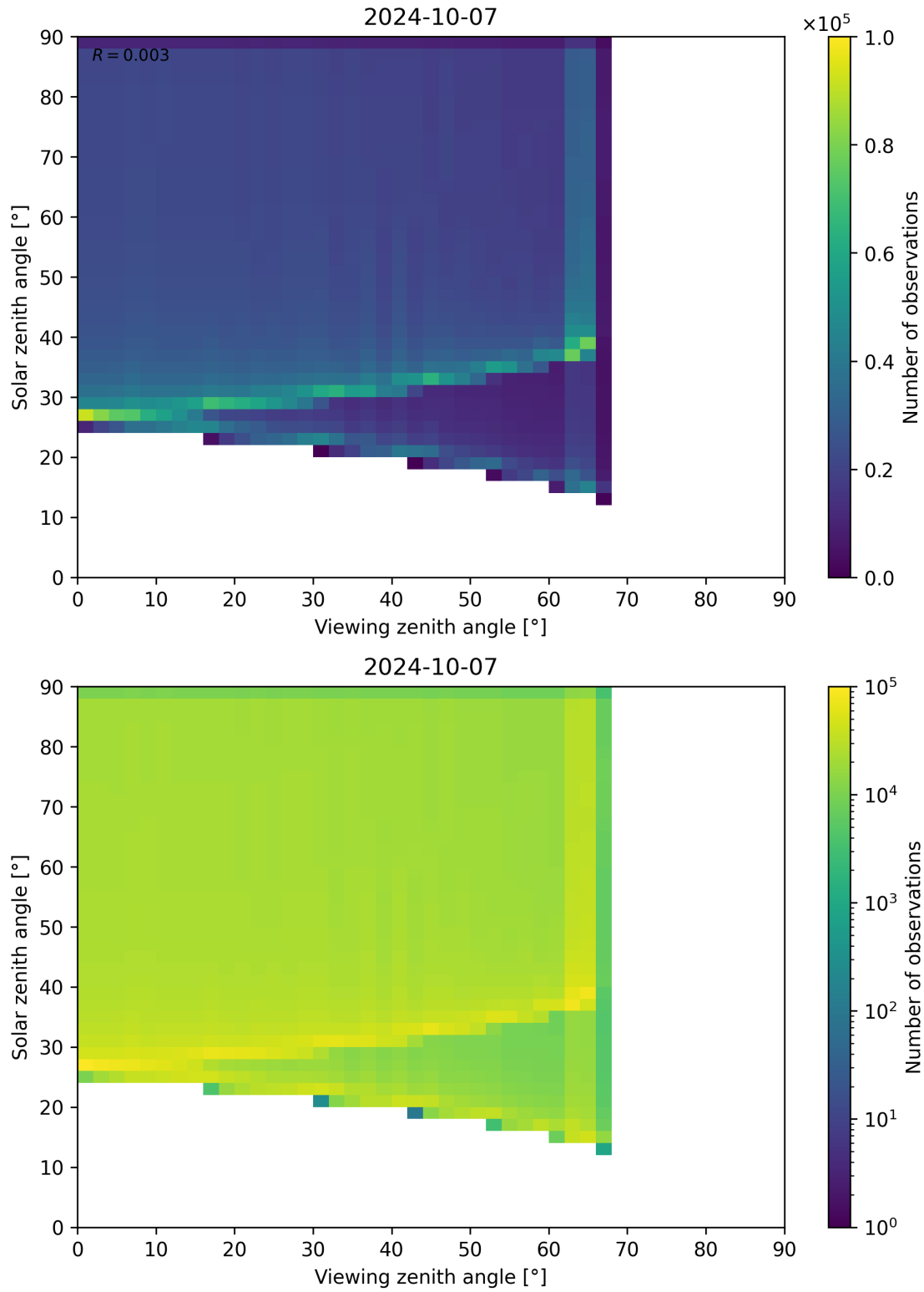
Figure 54: Scatter density plot of “Viewing zenith angle” against “Solar zenith angle” for 2024-10-06 to 2024-10-08.
