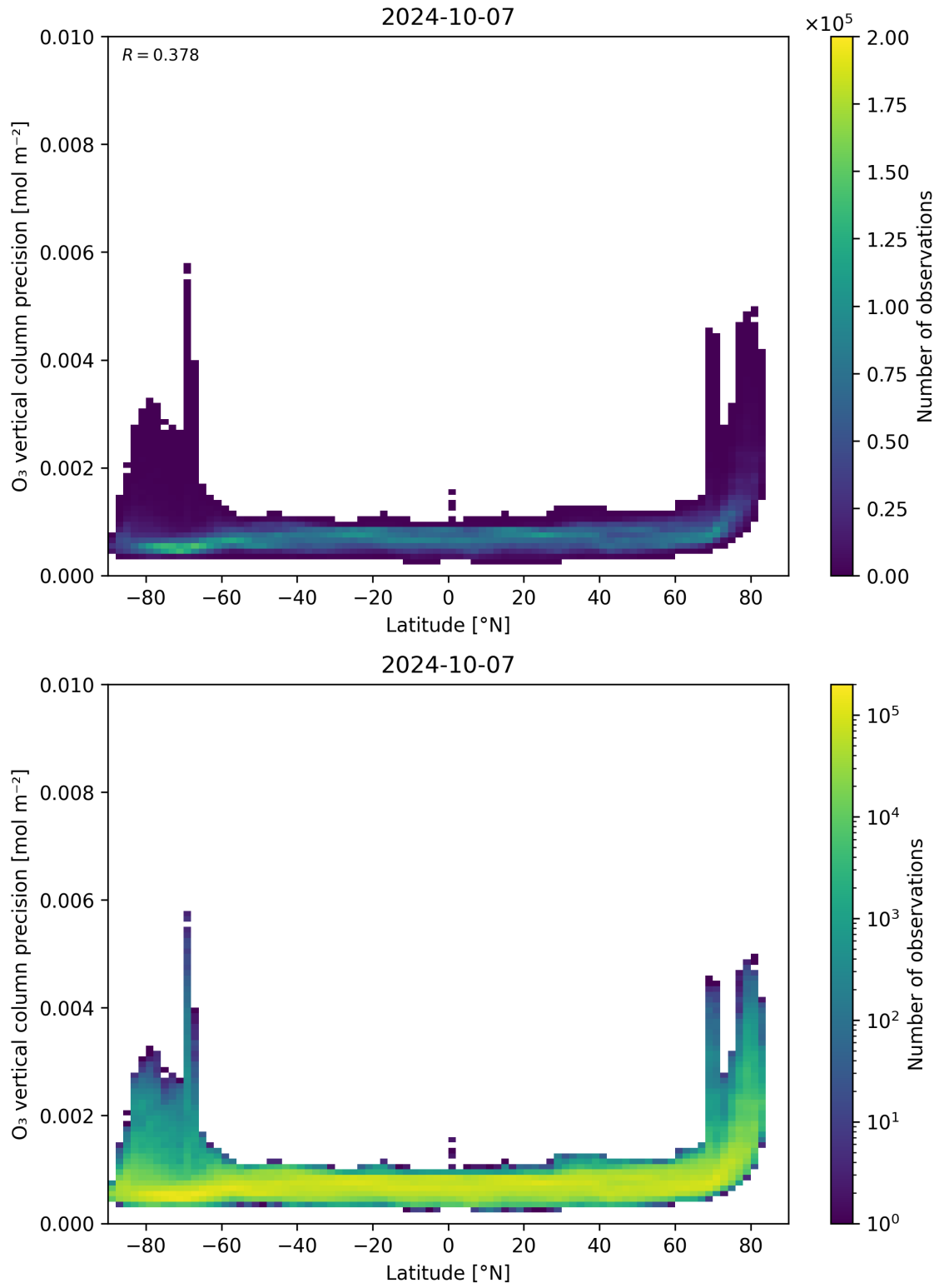
Figure 37: Scatter density plot of “Latitude” against “O 3 vertical column precision” for 2024-10-06 to 2024-10-08.
