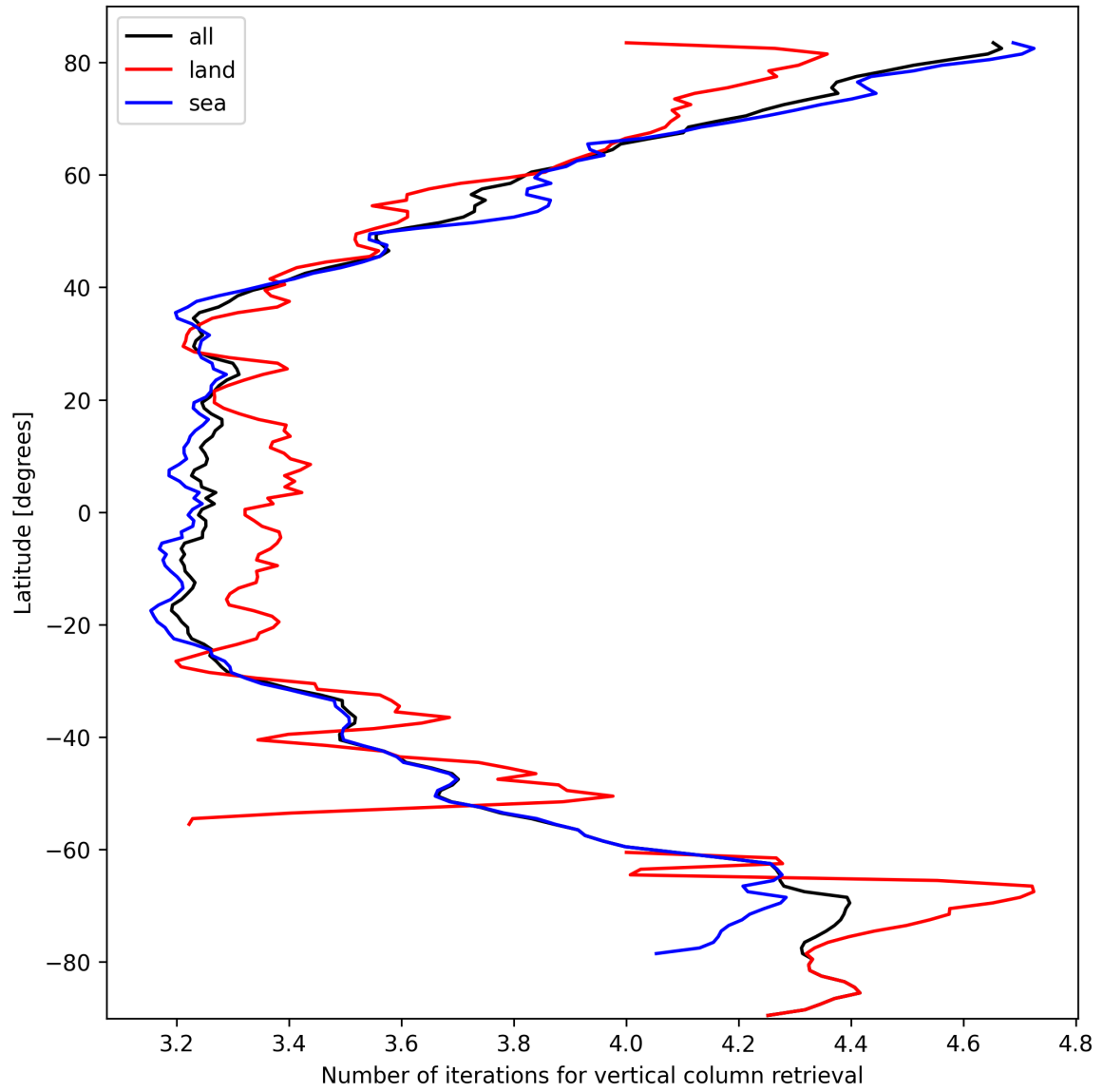
Figure 19: Zonal average of “Number of iterations for vertical column retrieval” for 2024-10-06 to 2024-10-08.
