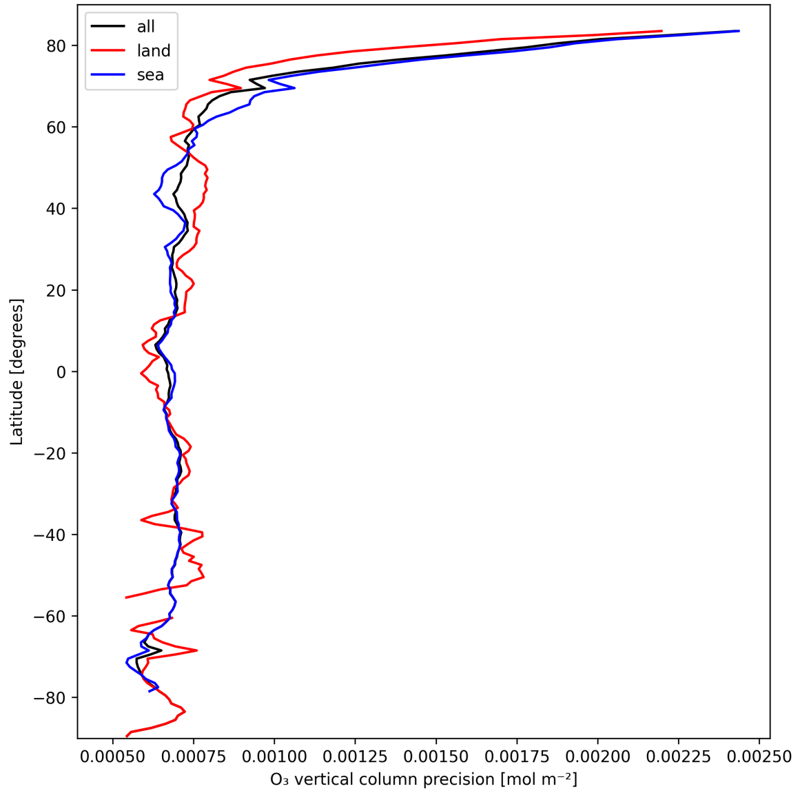
Figure 15: Zonal average of “O 3 vertical column precision” for 2024-10-06 to 2024-10-08.
