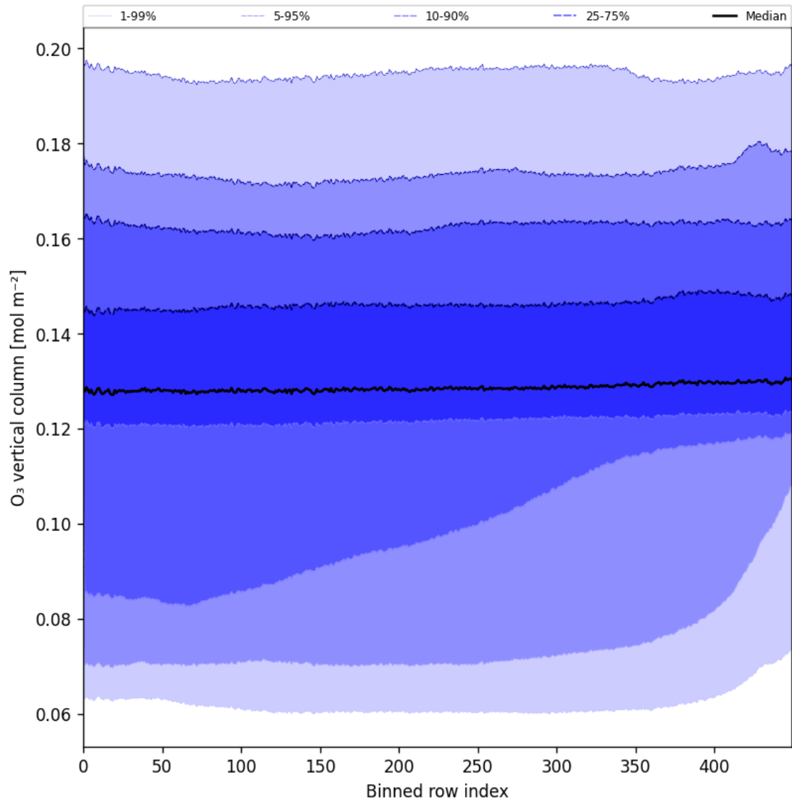
Figure 28: Along track statistics of “O 3 vertical column” for 2024-10-06 to 2024-10-08
