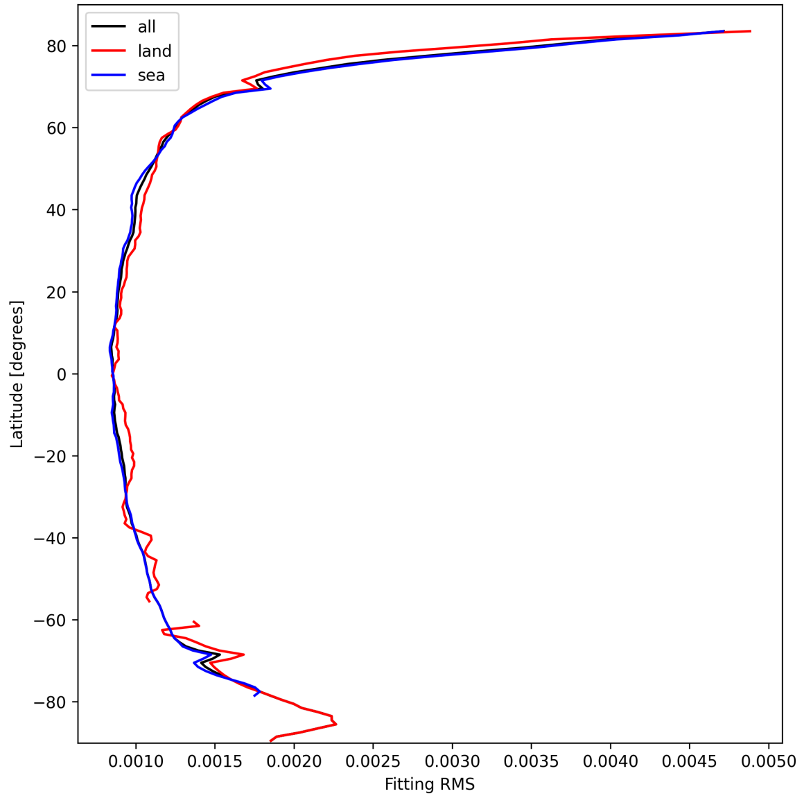
Figure 16: Zonal average of “Fitting RMS” for 2024-10-06 to 2024-10-08.
