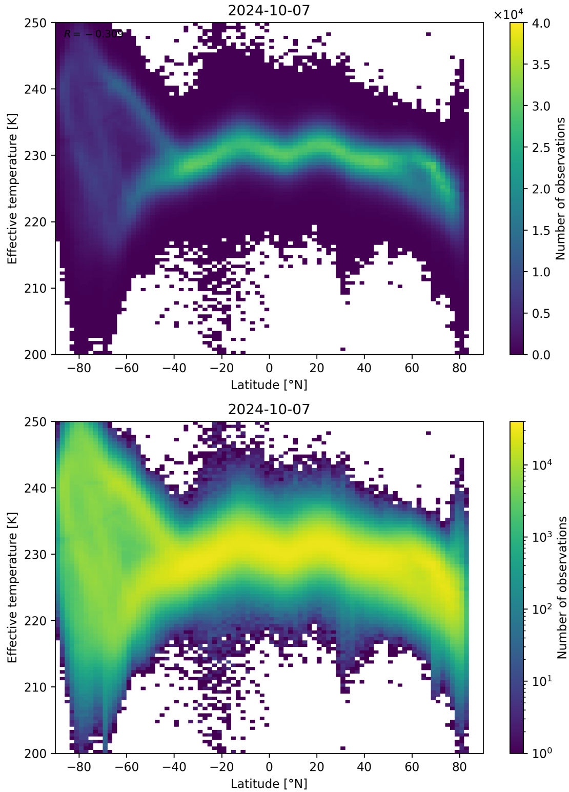
Figure 34: Scatter density plot of “Latitude” against “Effective temperature” for 2024-10-06 to 2024-10-08.
