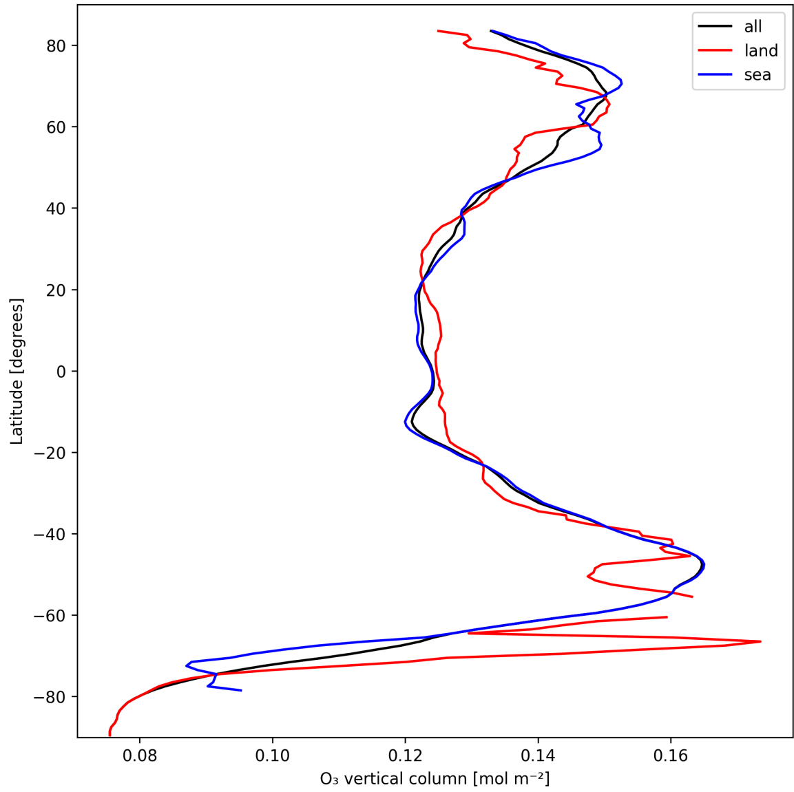
Figure 14: Zonal average of “O 3 vertical column” for 2024-10-06 to 2024-10-08.
