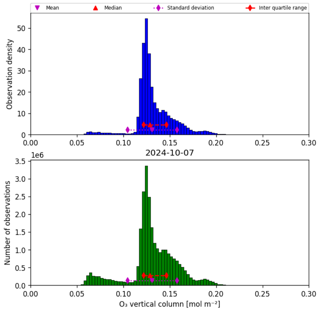
Figure 21: Histogram of “O 3 vertical column” for 2024-10-06 to 2024-10-08
