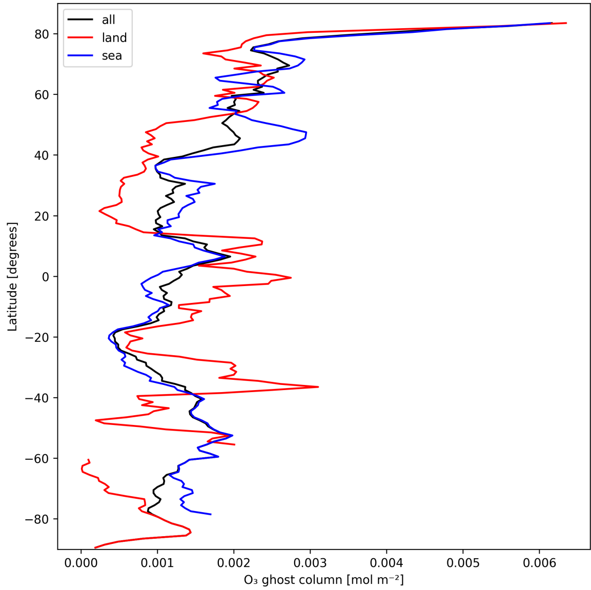
Figure 18: Zonal average of "O 3 ghost column" for 2024-10-06 to 2024-10-08.
