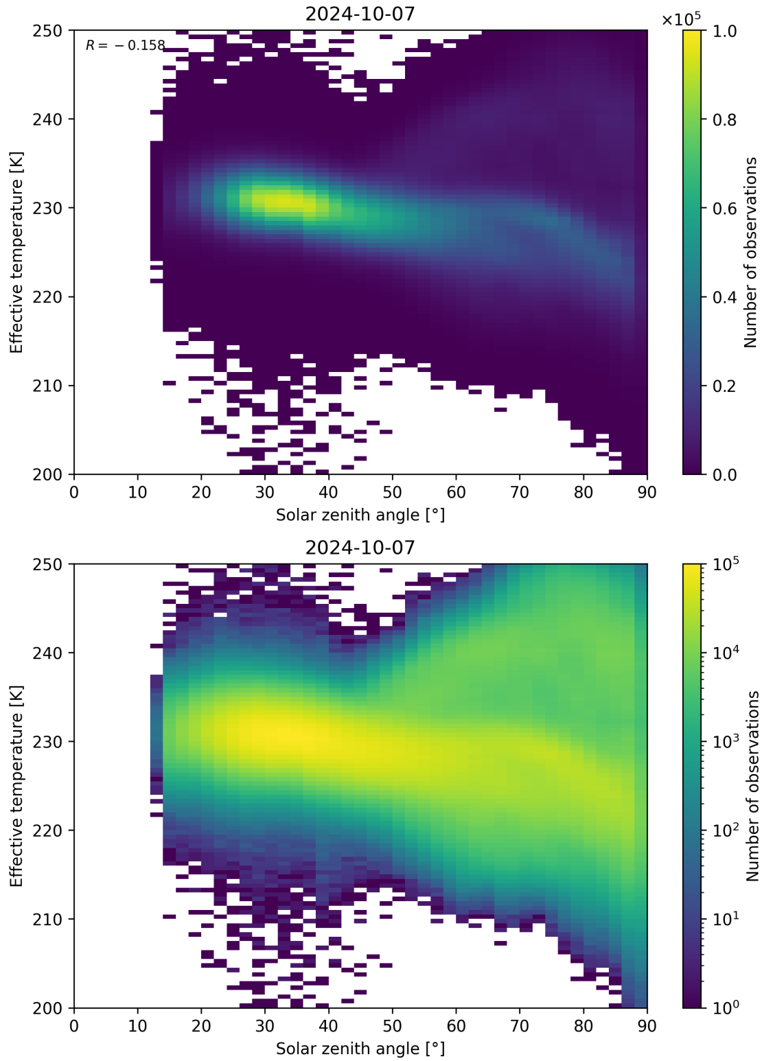
Figure 45: Scatter density plot of “Solar zenith angle” against “Effective temperature” for 2024-10-06 to 2024-10-08.
