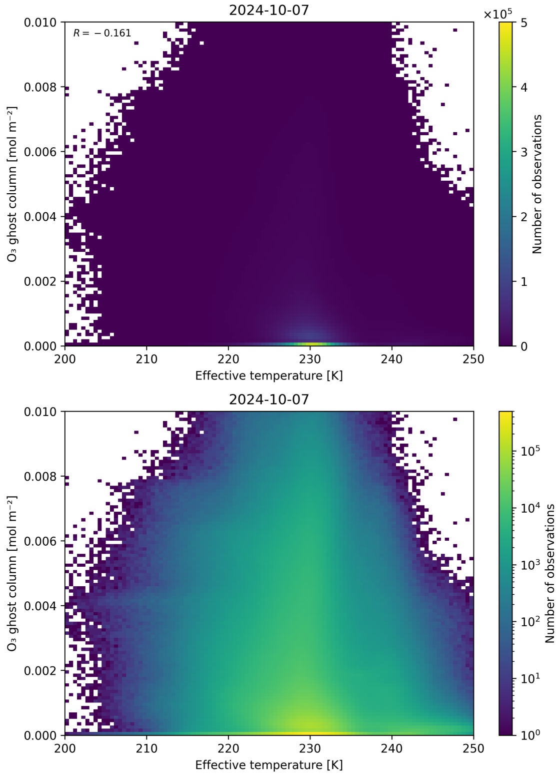
Figure 38: Scatter density plot of “Effective temperature” against “O 3 ghost column” for 2024-10-06 to 2024-10-08.
