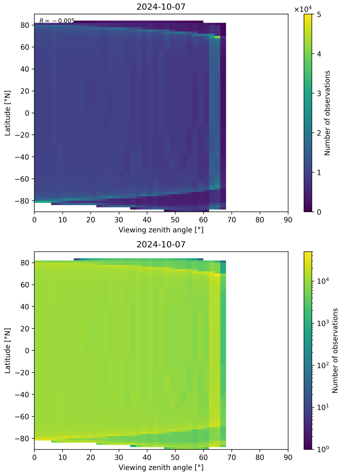
Figure 49: Scatter density plot of “Viewing zenith angle” against “Latitude” for 2024-10-06 to 2024-10-08.
