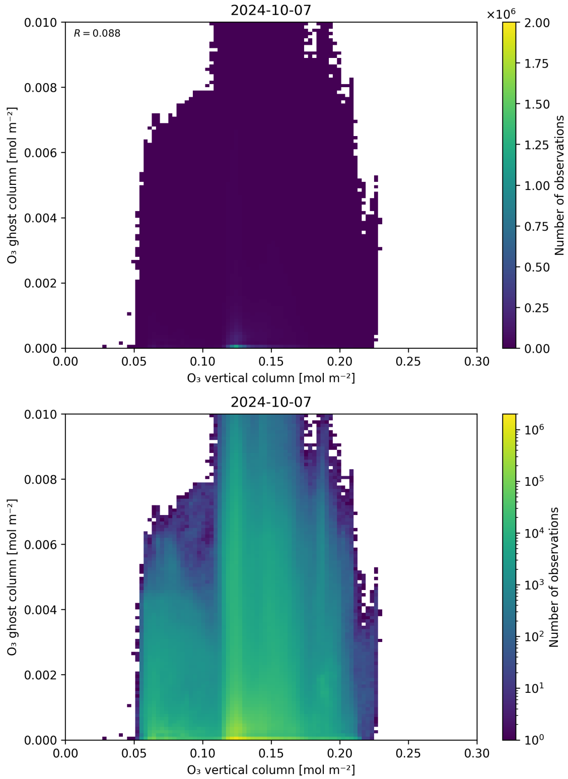
Figure 40: Scatter density plot of “O 3 vertical column” against “O 3 ghost column” for 2024-10-06 to 2024-10-08.
