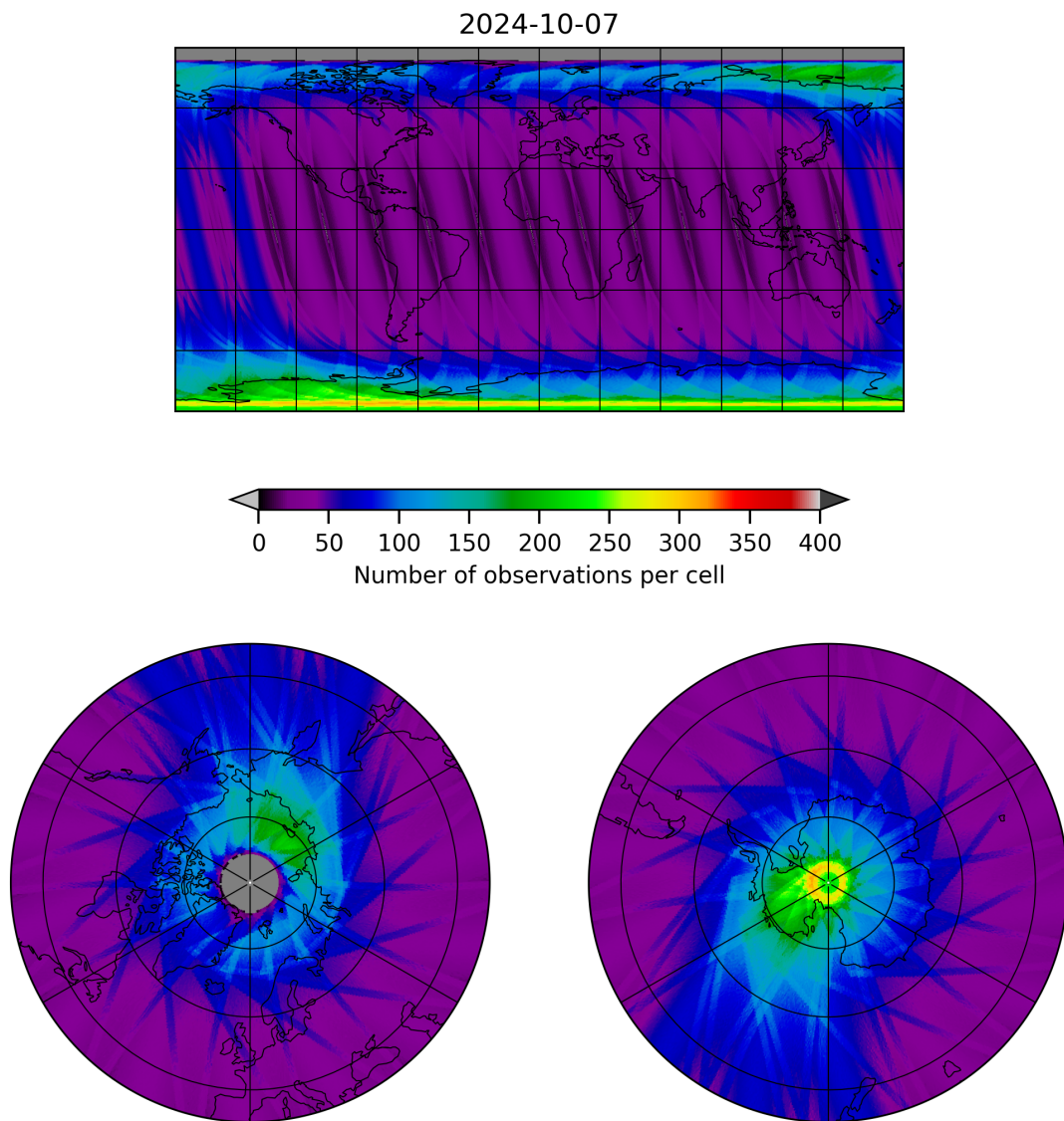
Figure 12: Map of the number of observations for 2024-10-06 to 2024-10-08
