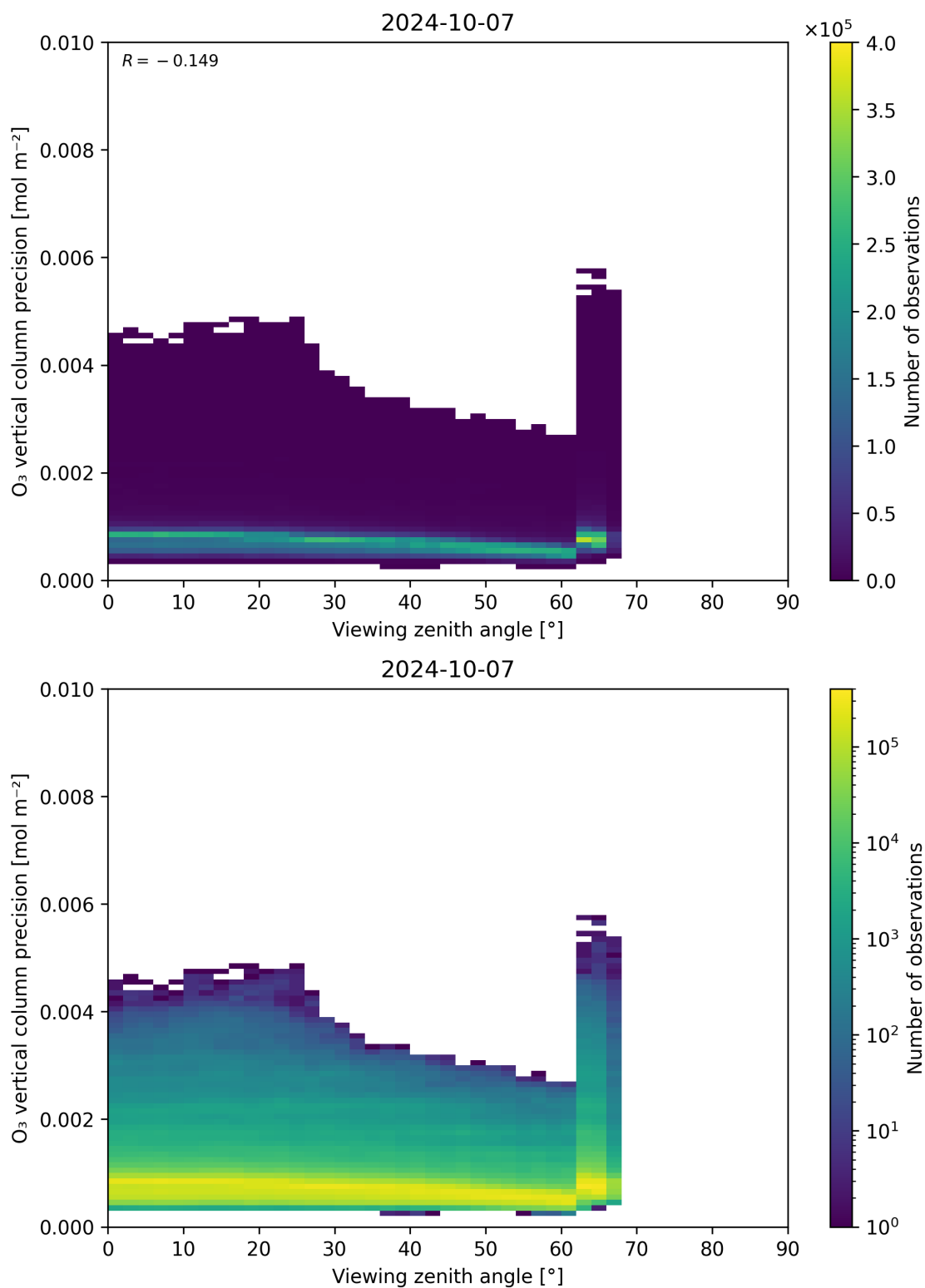
Figure 53: Scatter density plot of “Viewing zenith angle” against “O 3 vertical column precision” for 2024-10-06 to 2024-10-08.
