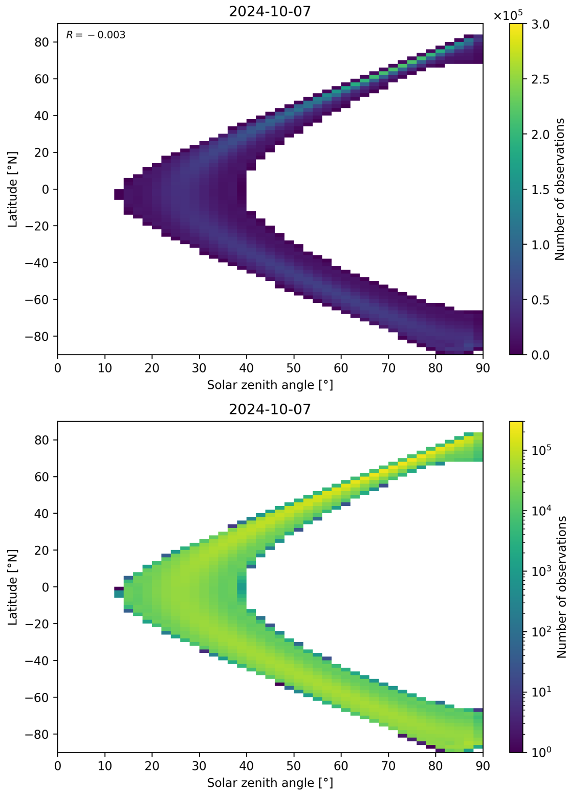
Figure 44: Scatter density plot of “Solar zenith angle” against “Latitude” for 2024-10-06 to 2024-10-08.
