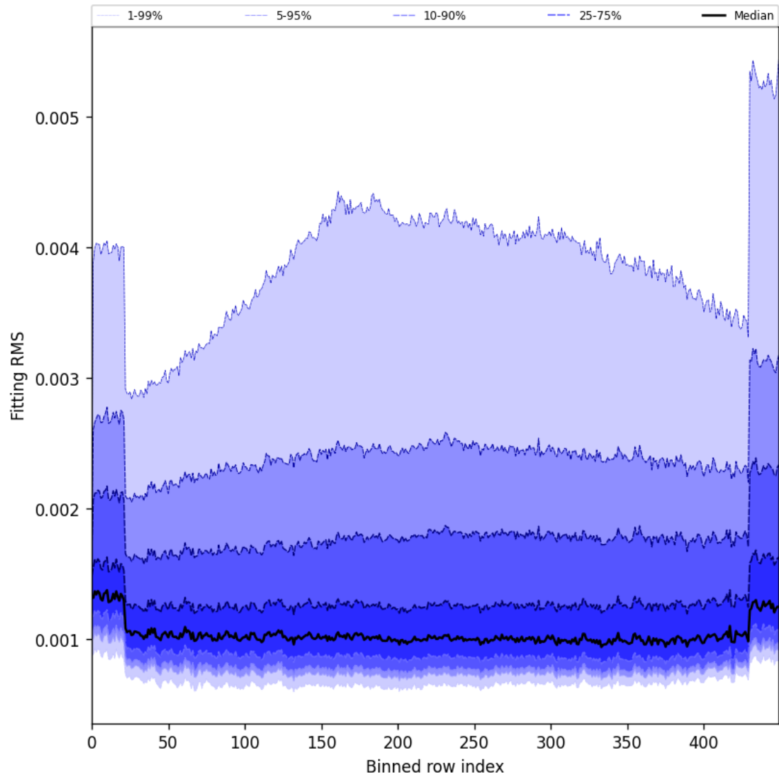
Figure 30: Along track statistics of “Fitting RMS” for 2024-10-06 to 2024-10-08
