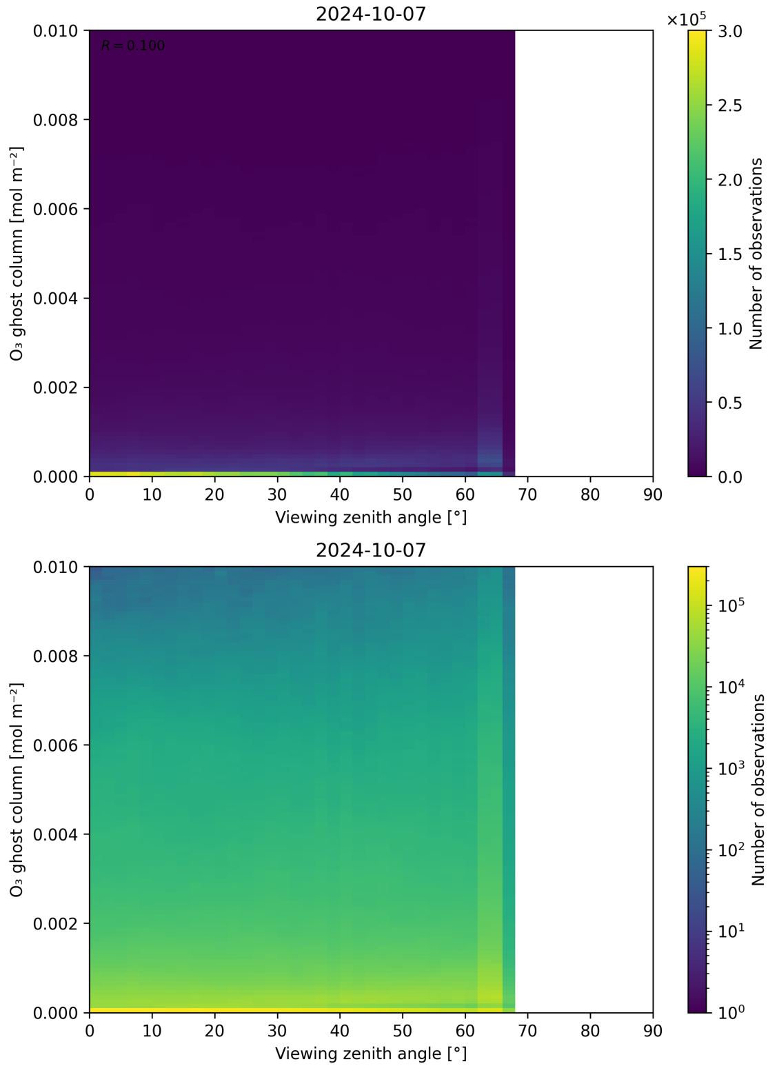
Figure 51: Scatter density plot of “Viewing zenith angle” against “O 3 ghost column” for 2024-10-06 to 2024-10-08.
