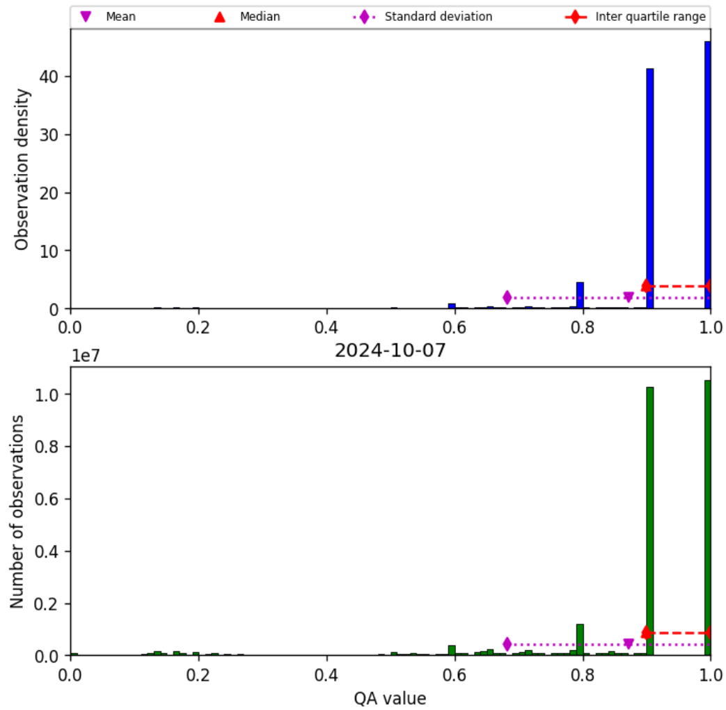
Figure 20: Histogram of “QA value” for 2024-10-06 to 2024-10-08
