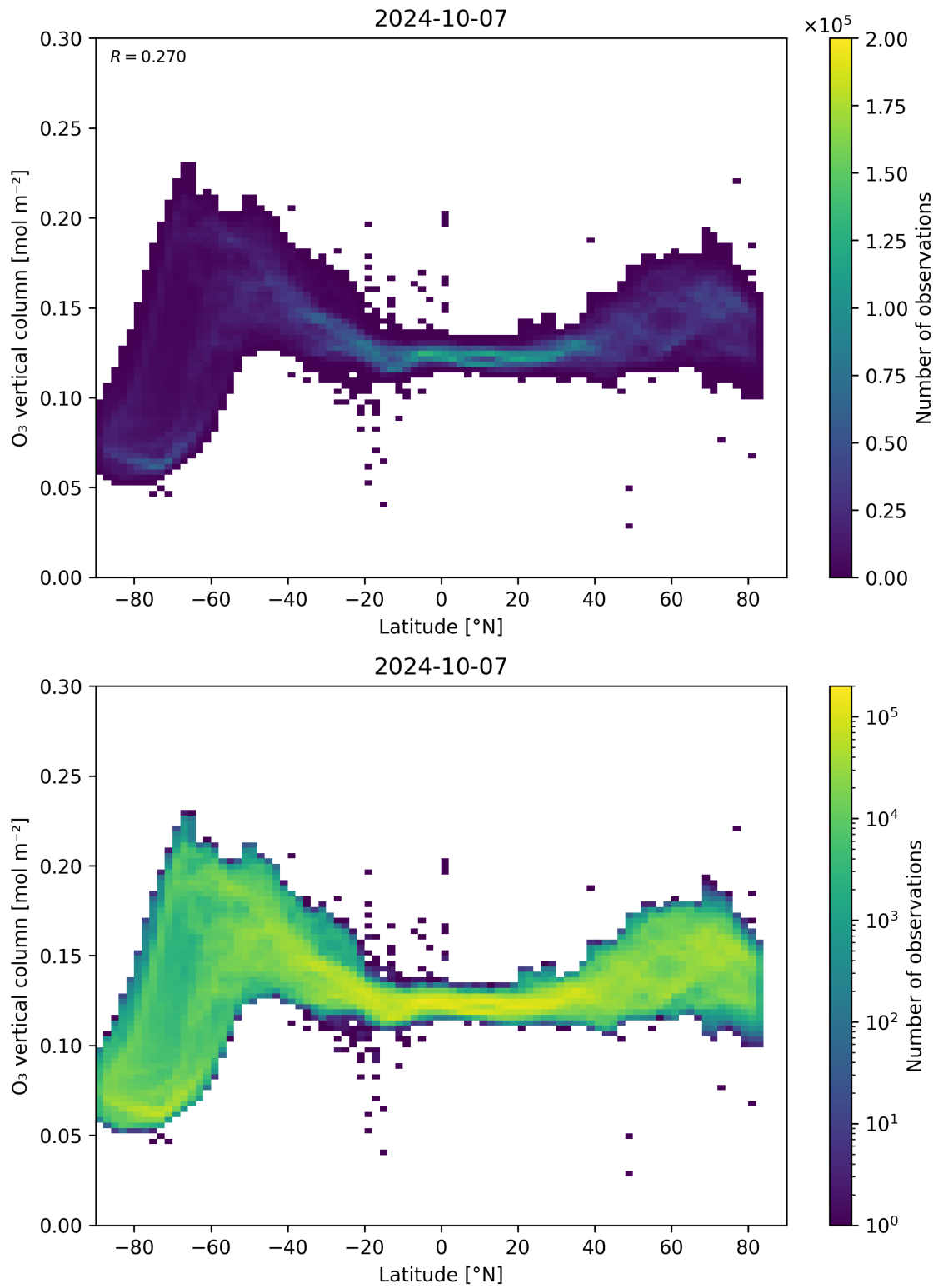
Figure 36: Scatter density plot of “Latitude” against “O 3 vertical column” for 2024-10-06 to 2024-10-08.
