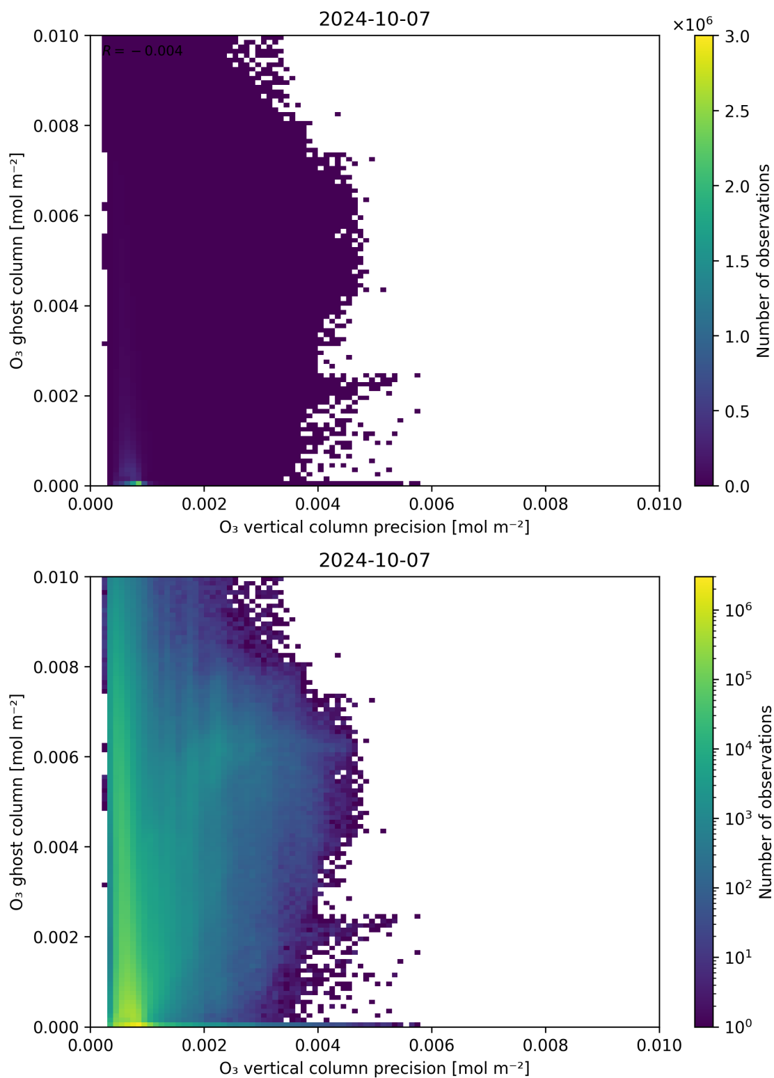
Figure 43: Scatter density plot of “ \text{O}_3 vertical column precision” against “ \text{O}_3 ghost column” for 2024-10-06 to 2024-10-08.
