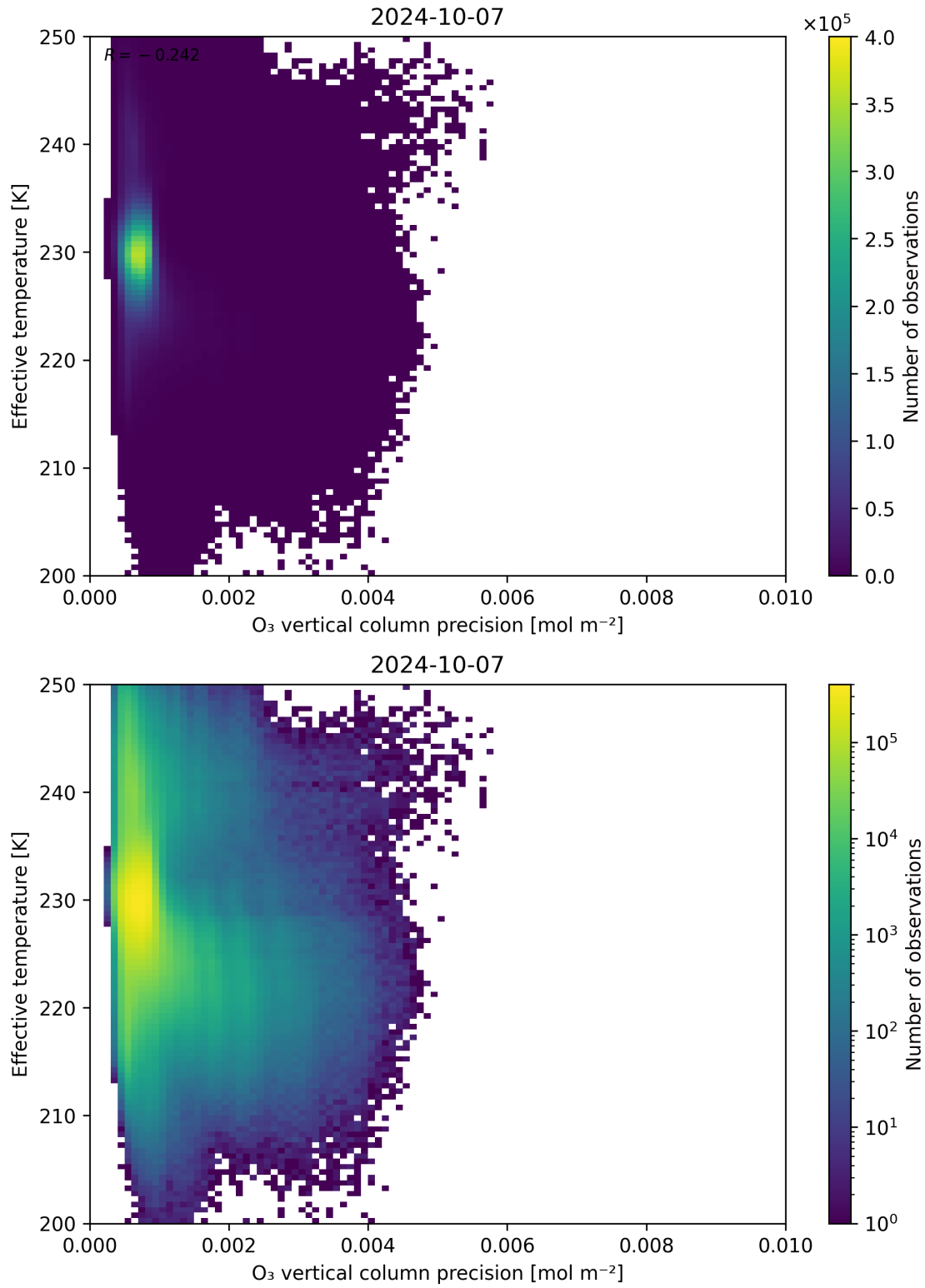
Figure 42: Scatter density plot of “O 3 vertical column precision” against “Effective temperature” for 2024-10-06 to 2024-10-08.
