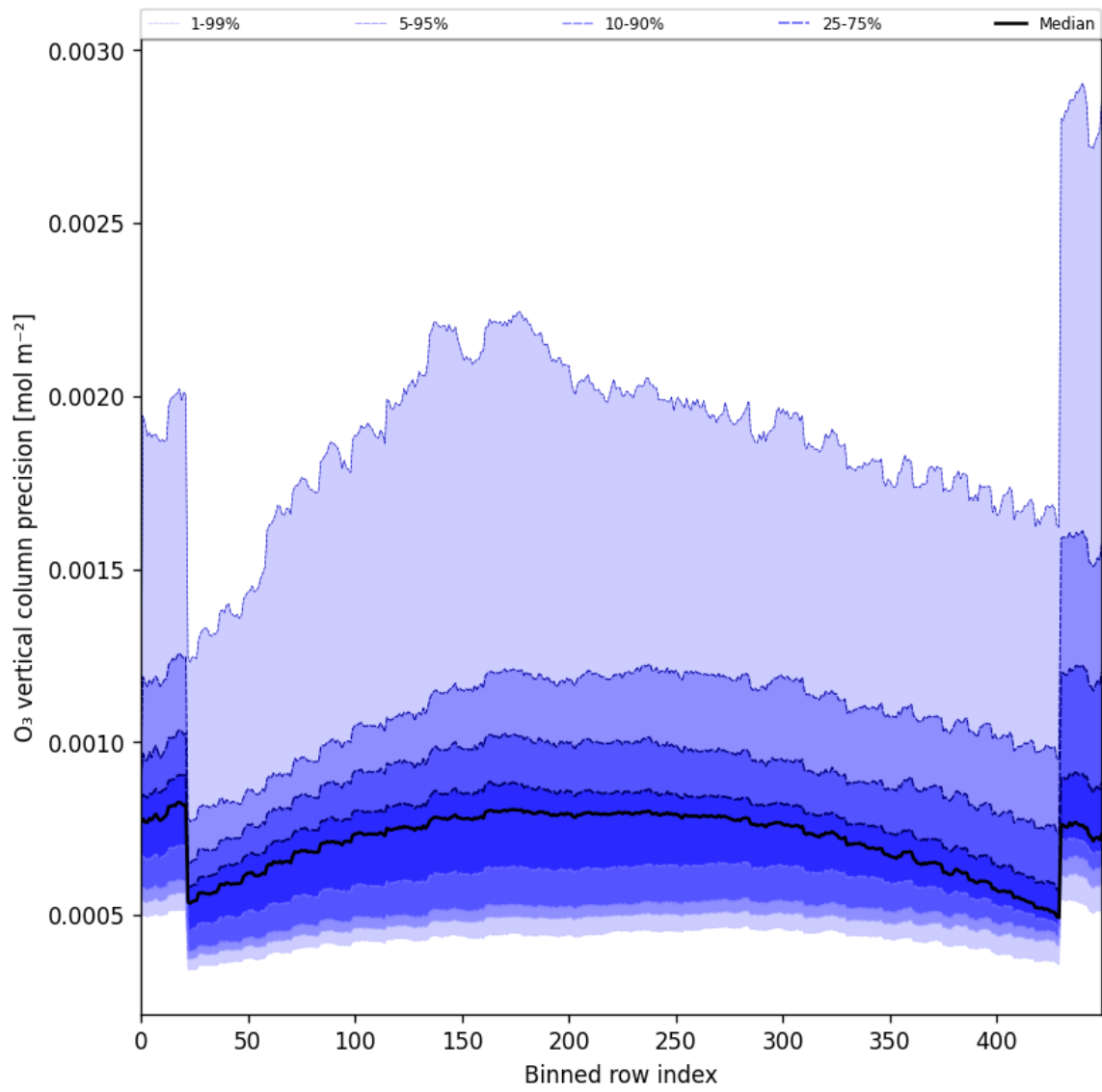
Figure 29: Along track statistics of “O 3 vertical column precision” for 2024-10-06 to 2024-10-08
