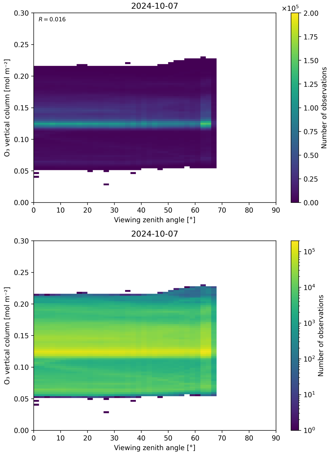
Figure 52: Scatter density plot of “Viewing zenith angle” against “O 3 vertical column” for 2024-10-06 to 2024-10-08.
