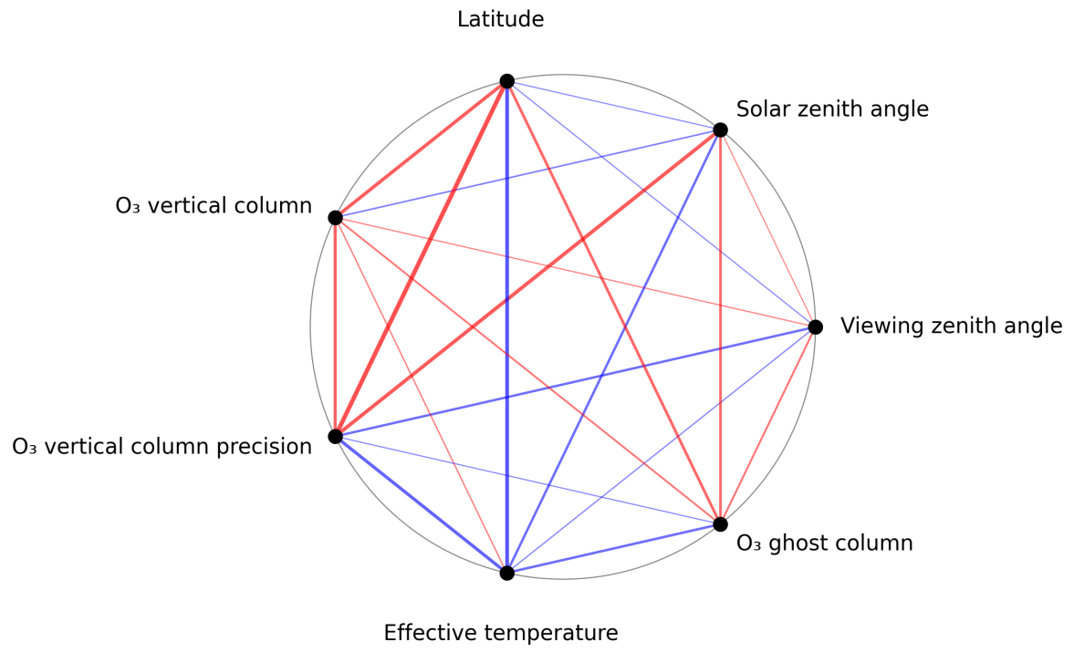
Figure 1: Map of correlation graph for 2024-10-06 to 2024-10-08.
