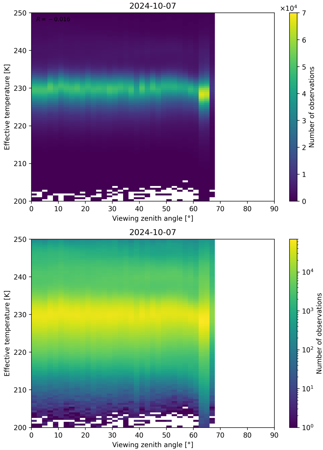
Figure 50: Scatter density plot of “Viewing zenith angle” against “Effective temperature” for 2024-10-06 to 2024-10-08.
