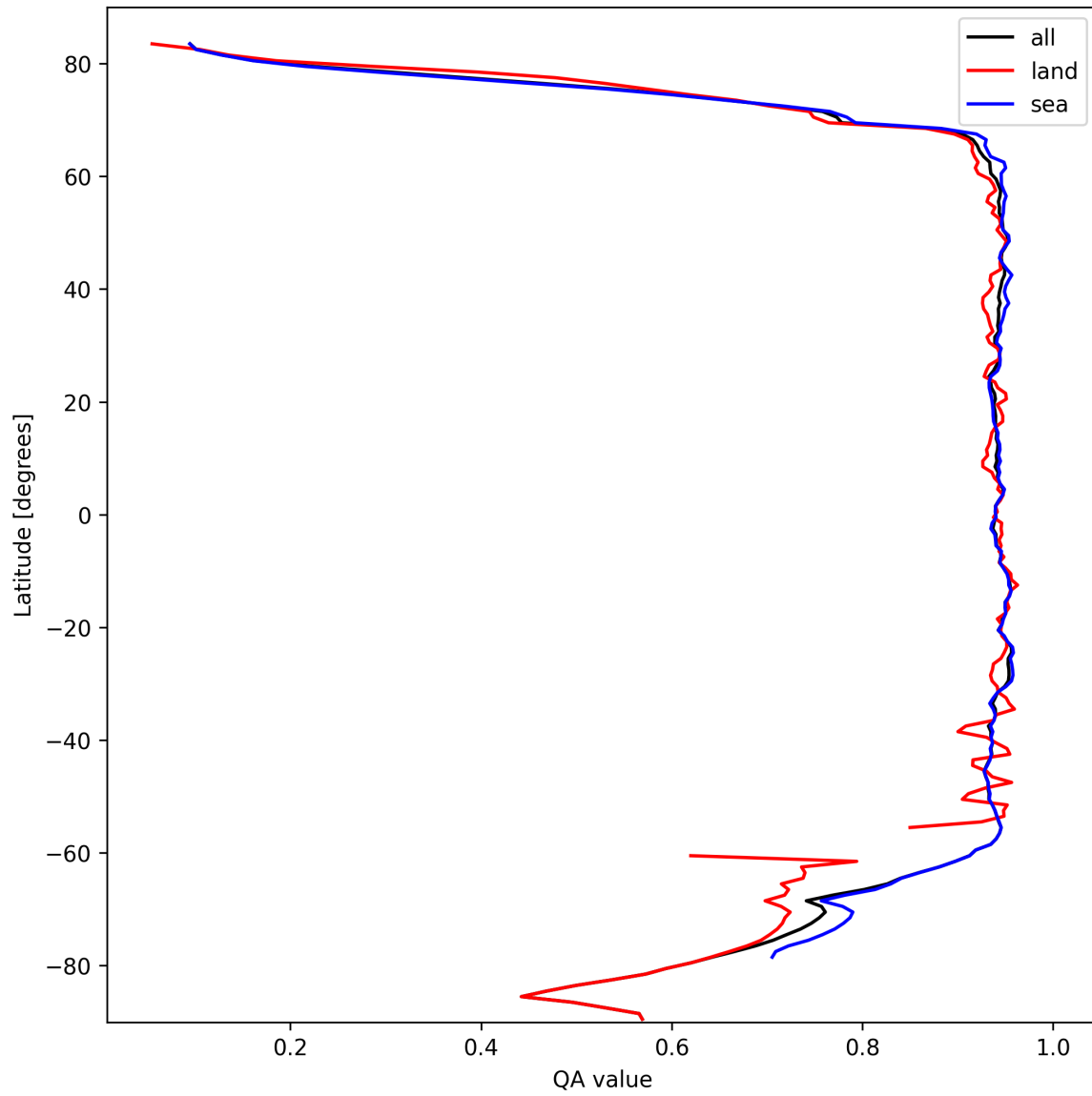
Figure 13: Zonal average of “QA value” for 2024-10-06 to 2024-10-08.
