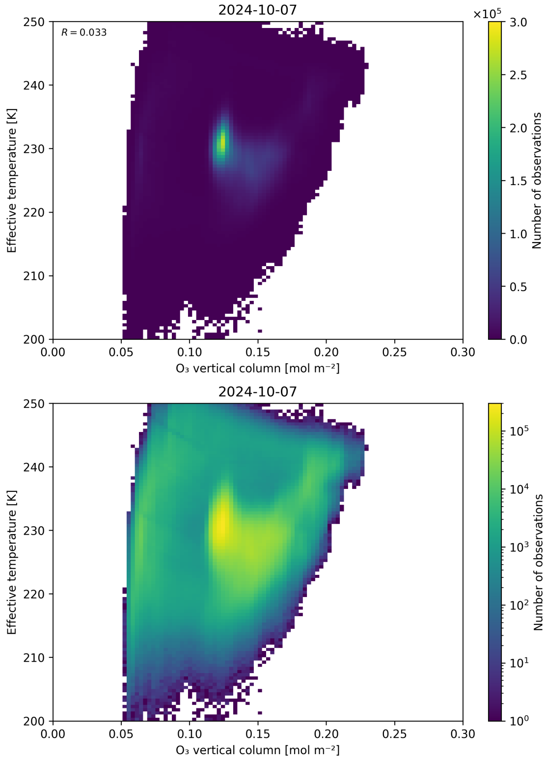
Figure 39: Scatter density plot of “O 3 vertical column” against “Effective temperature” for 2024-10-06 to 2024-10-08.
