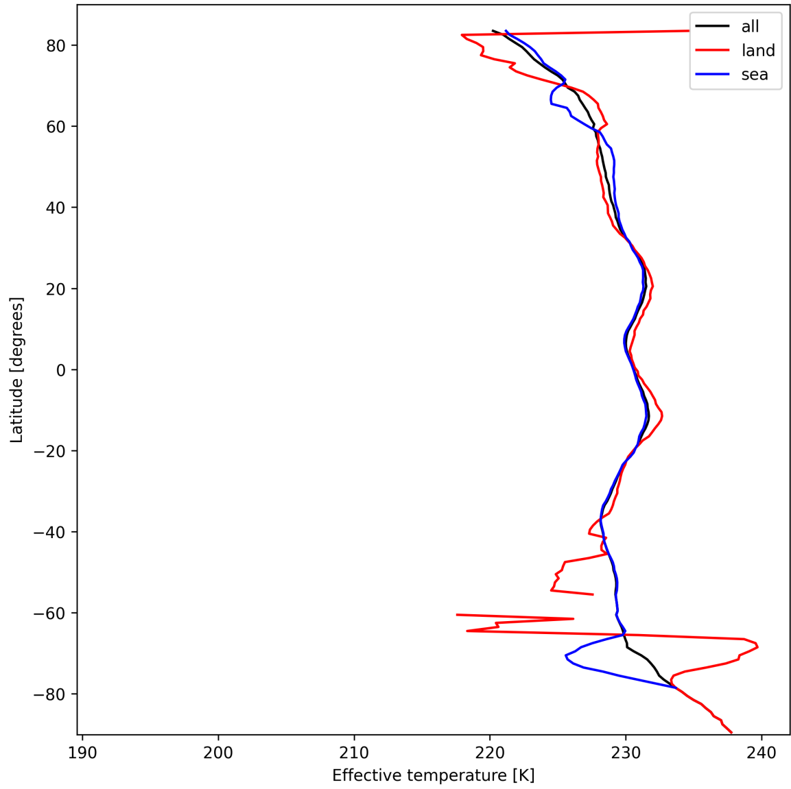
Figure 17: Zonal average of "Effective temperature" for 2024-10-06 to 2024-10-08.
