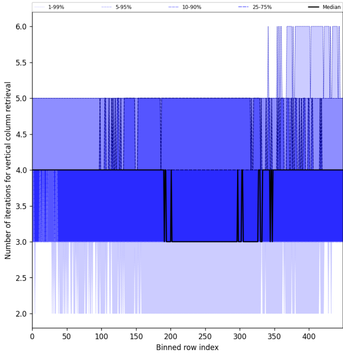
Figure 33: Along track statistics of “Number of iterations for vertical column retrieval” for 2024-10-06 to 2024-10-08
