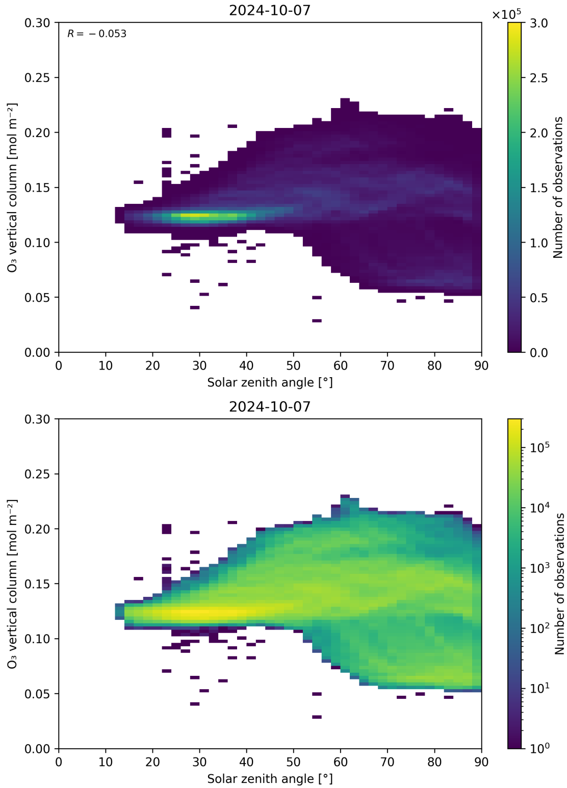
Figure 47: Scatter density plot of “Solar zenith angle” against “O 3 vertical column” for 2024-10-06 to 2024-10-08.
