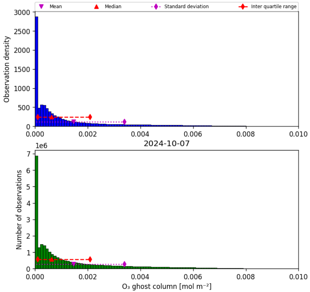
Figure 25: Histogram of “O 3 ghost column” for 2024-10-06 to 2024-10-08
