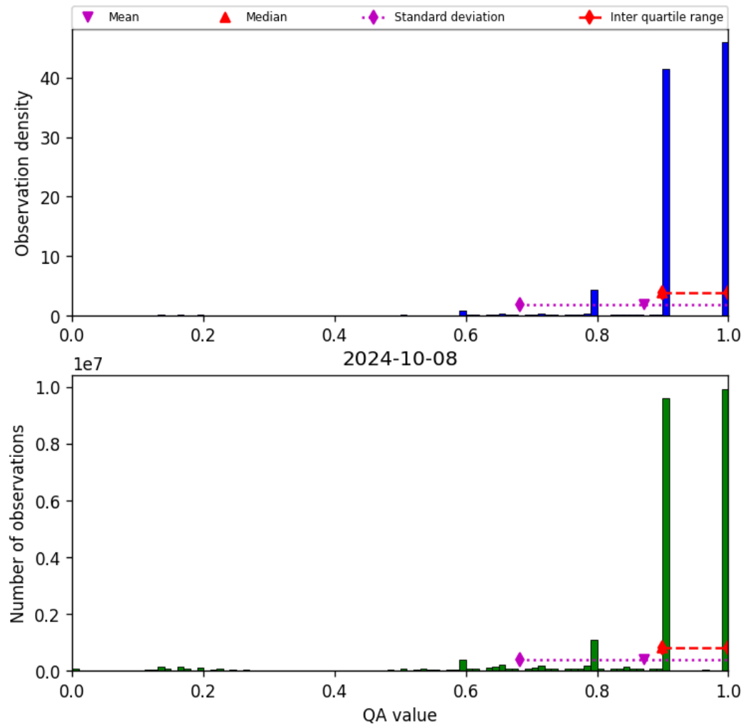
Figure 20: Histogram of “QA value” for 2024-10-08 to 2024-10-09
