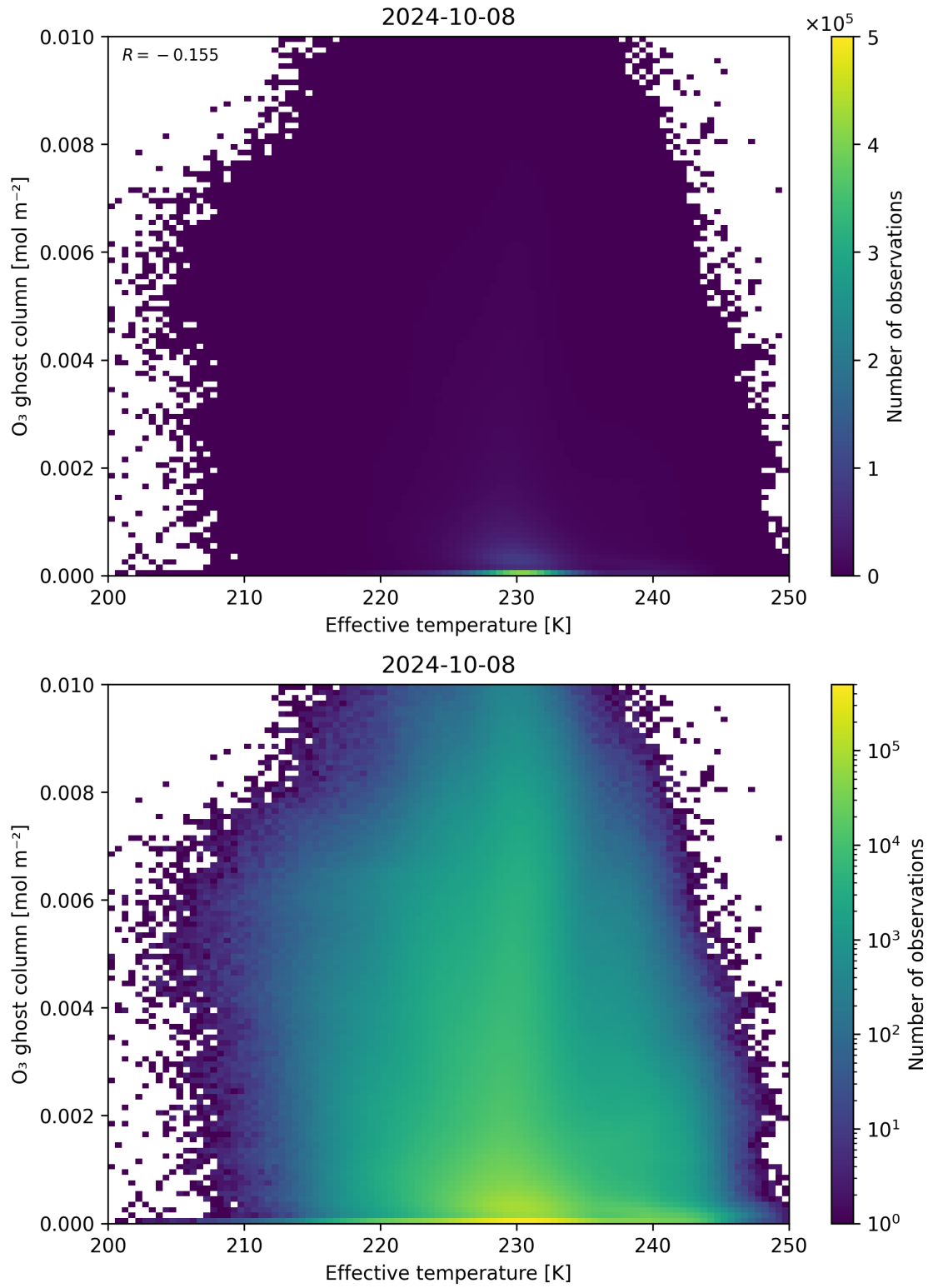
Figure 38: Scatter density plot of “Effective temperature” against “O 3 ghost column” for 2024-10-08 to 2024-10-09.
