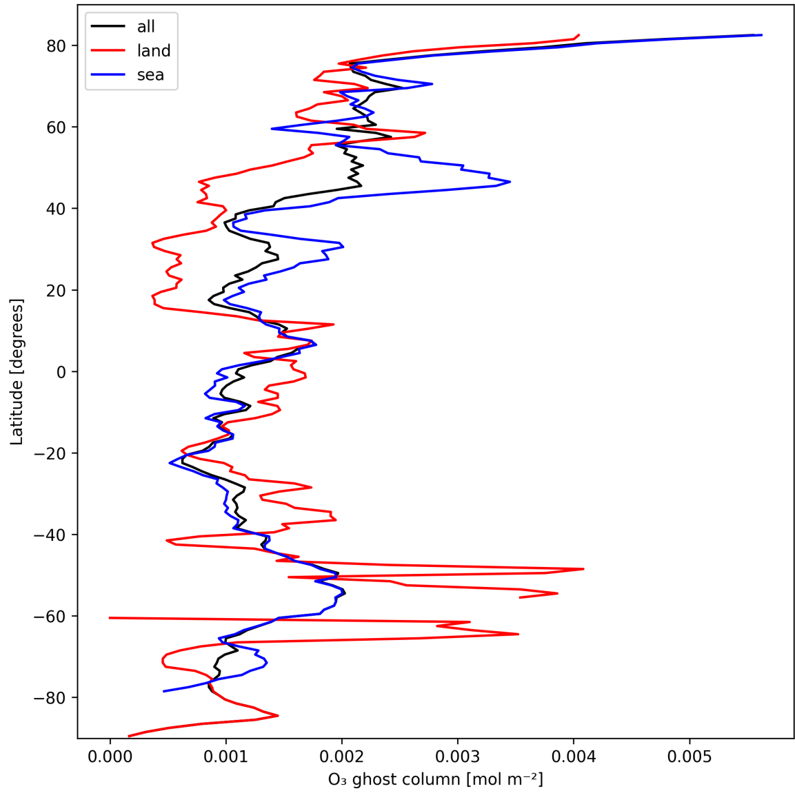
Figure 18: Zonal average of "O 3 ghost column" for 2024-10-08 to 2024-10-09.
