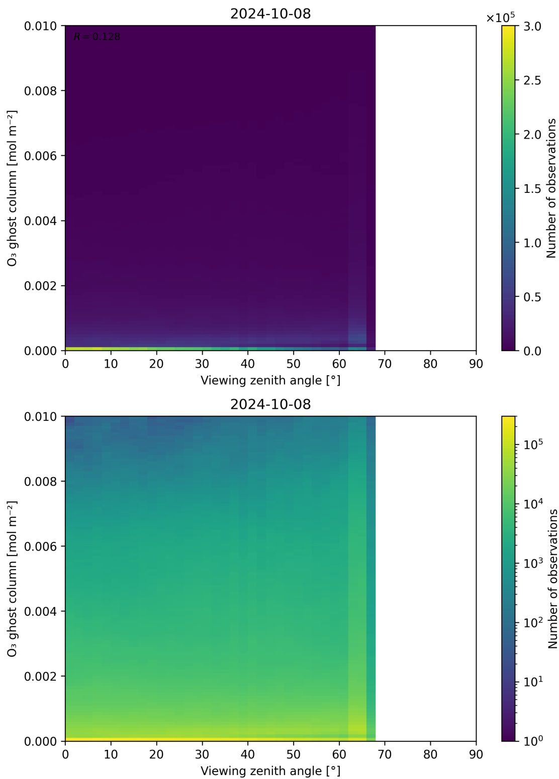
Figure 51: Scatter density plot of “Viewing zenith angle” against “O 3 ghost column” for 2024-10-08 to 2024-10-09.
