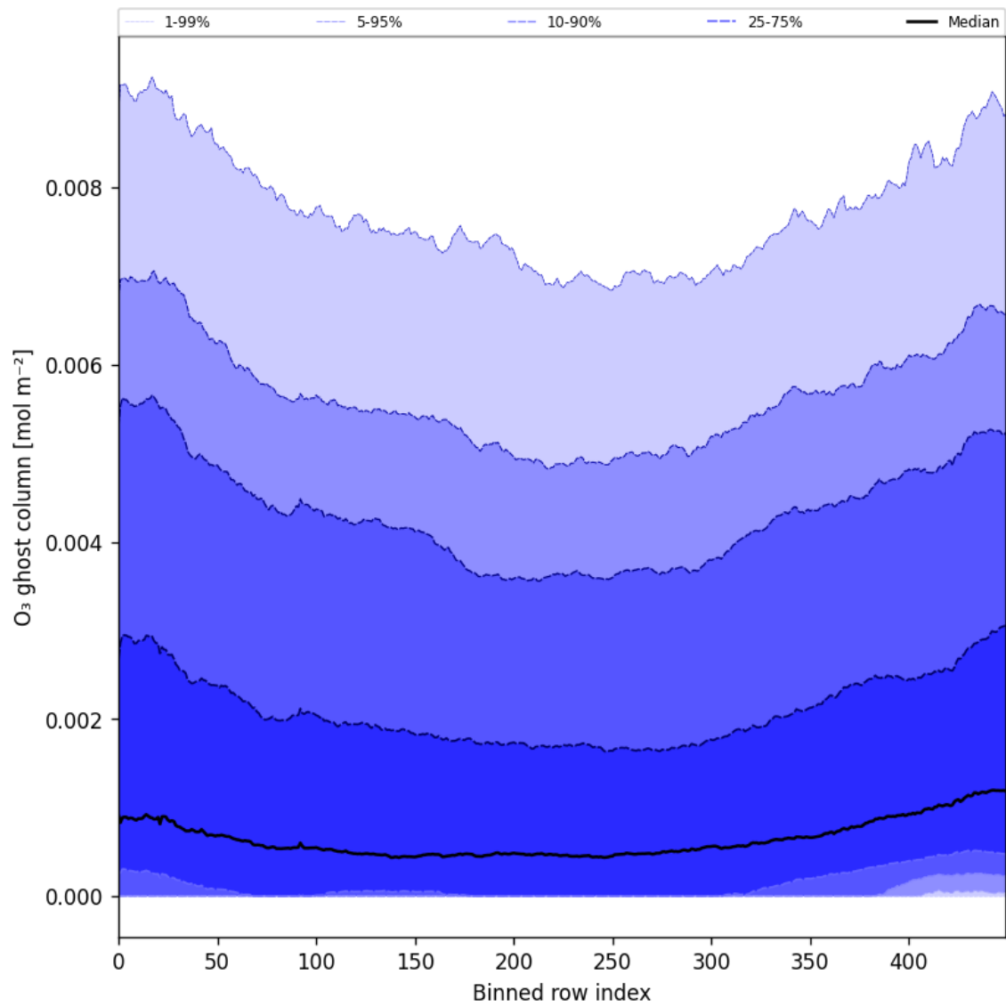
Figure 32: Along track statistics of “O 3 ghost column” for 2024-10-08 to 2024-10-09
