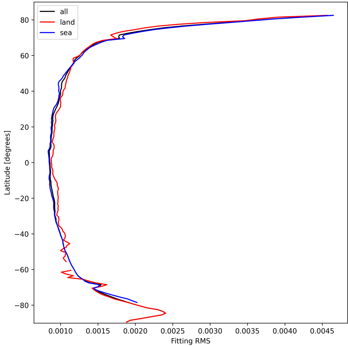
Figure 16: Zonal average of “Fitting RMS” for 2024-10-08 to 2024-10-09.
