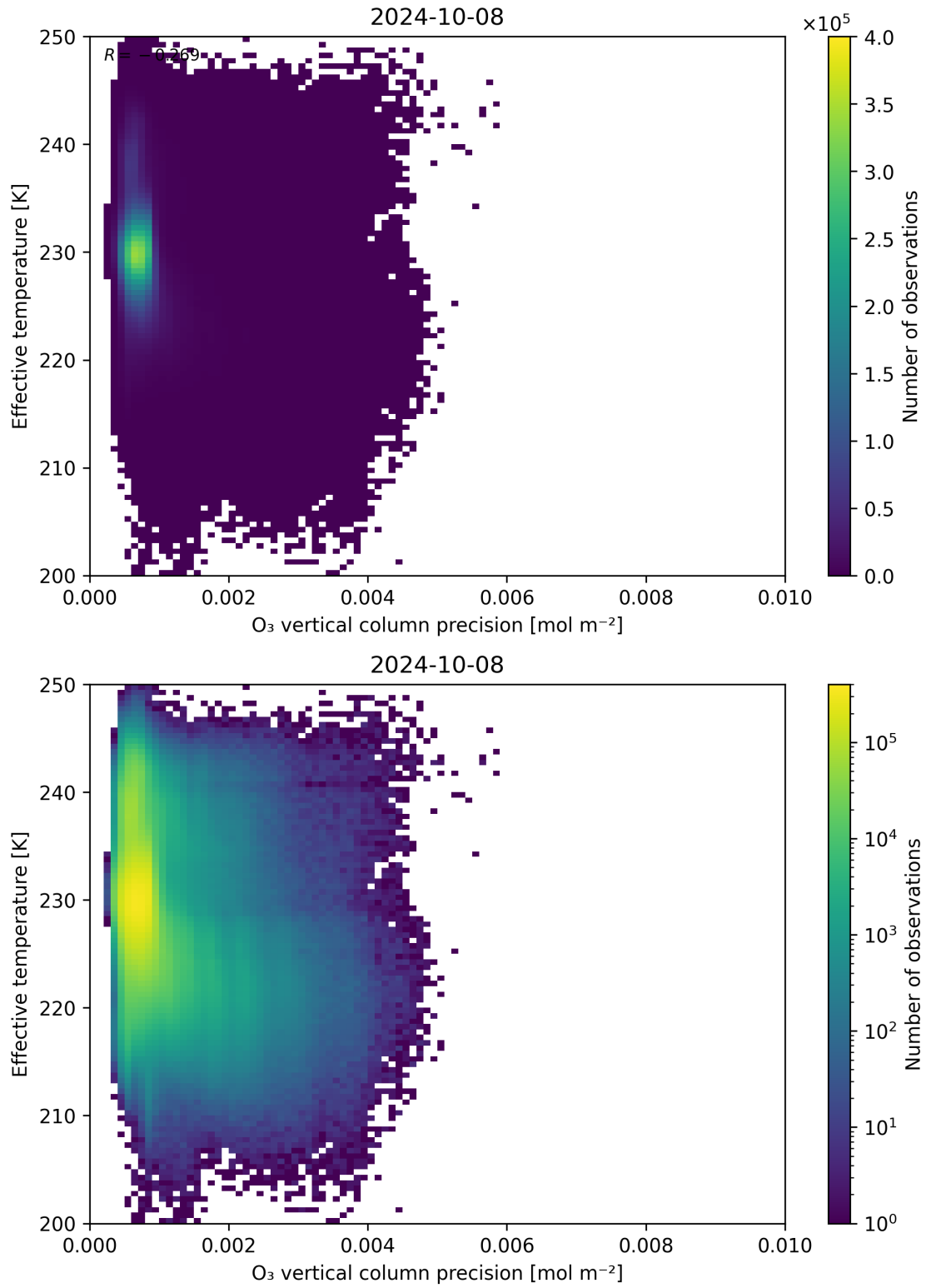
Figure 42: Scatter density plot of “ O_3 vertical column precision” against “Effective temperature” for 2024-10-08 to 2024-10-09.
