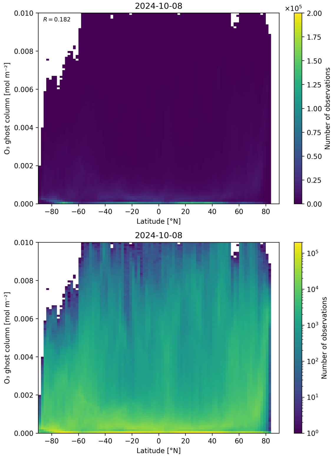
Figure 35: Scatter density plot of “Latitude” against “O 3 ghost column” for 2024-10-08 to 2024-10-09.
