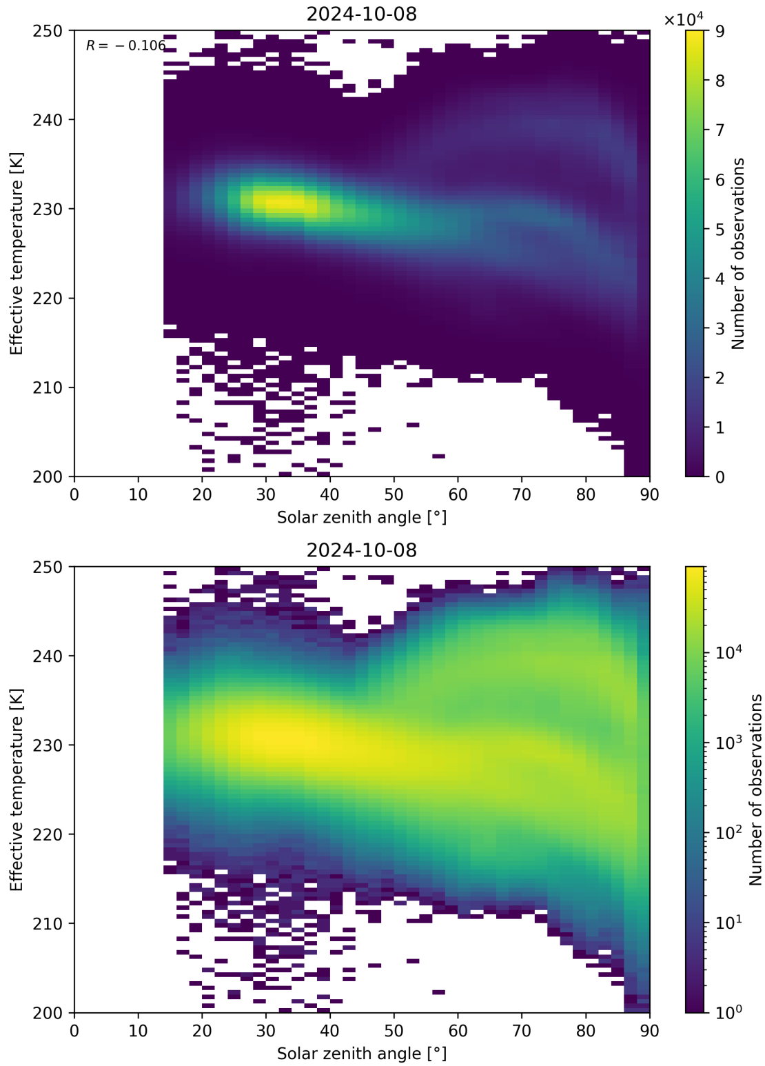
Figure 45: Scatter density plot of “Solar zenith angle” against “Effective temperature” for 2024-10-08 to 2024-10-09.
