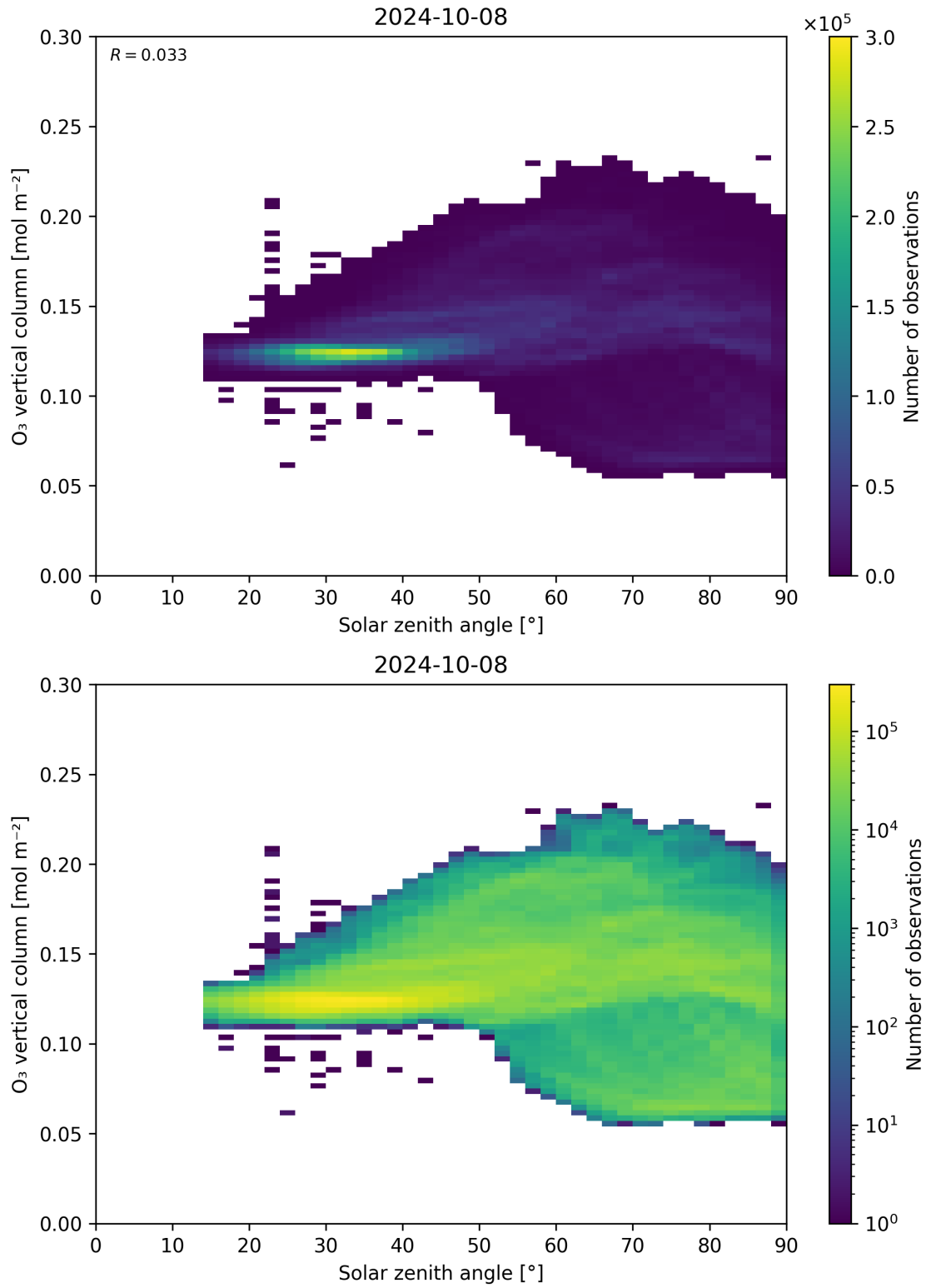
Figure 47: Scatter density plot of “Solar zenith angle” against “O 3 vertical column” for 2024-10-08 to 2024-10-09.
