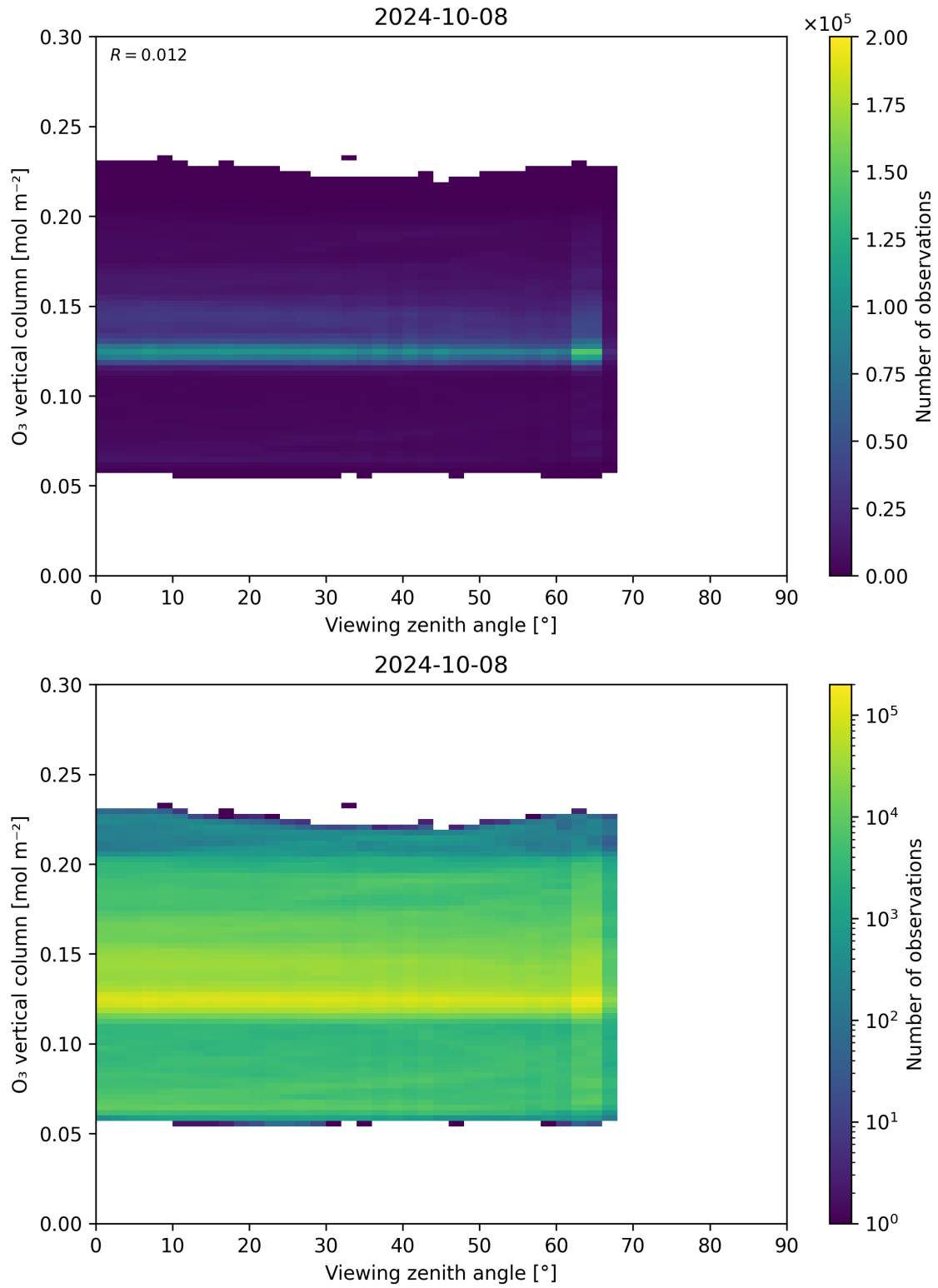
Figure 52: Scatter density plot of “Viewing zenith angle” against “O 3 vertical column” for 2024-10-08 to 2024-10-09.
