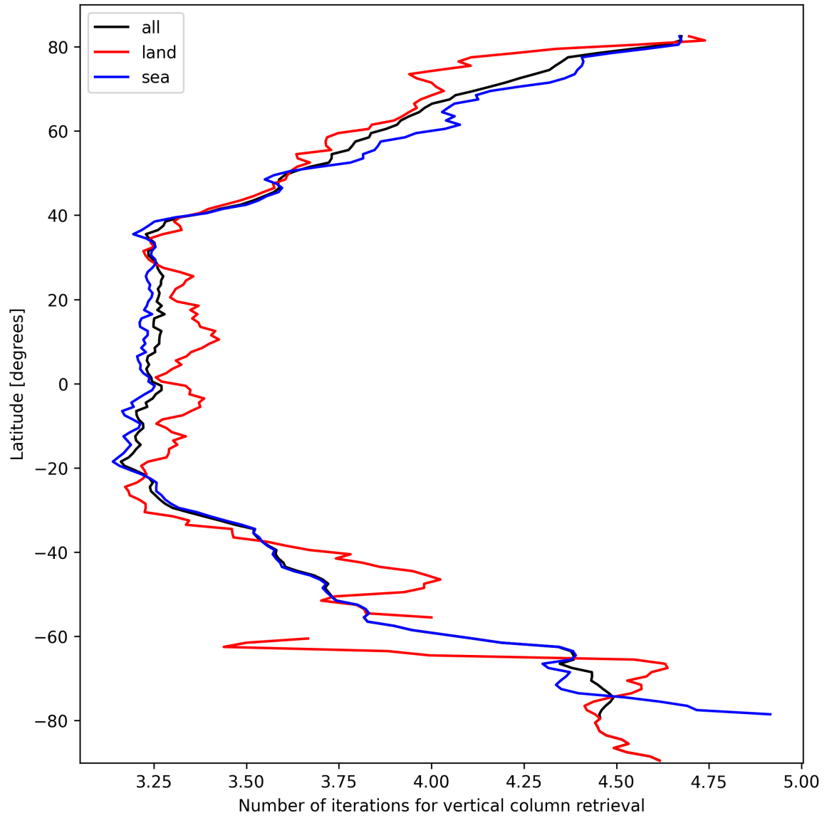
Figure 19: Zonal average of “Number of iterations for vertical column retrieval” for 2024-10-08 to 2024-10-09.
