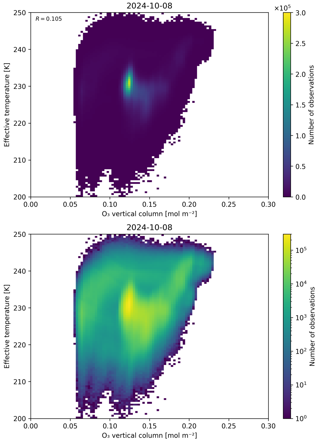
Figure 39: Scatter density plot of “O 3 vertical column” against “Effective temperature” for 2024-10-08 to 2024-10-09.
