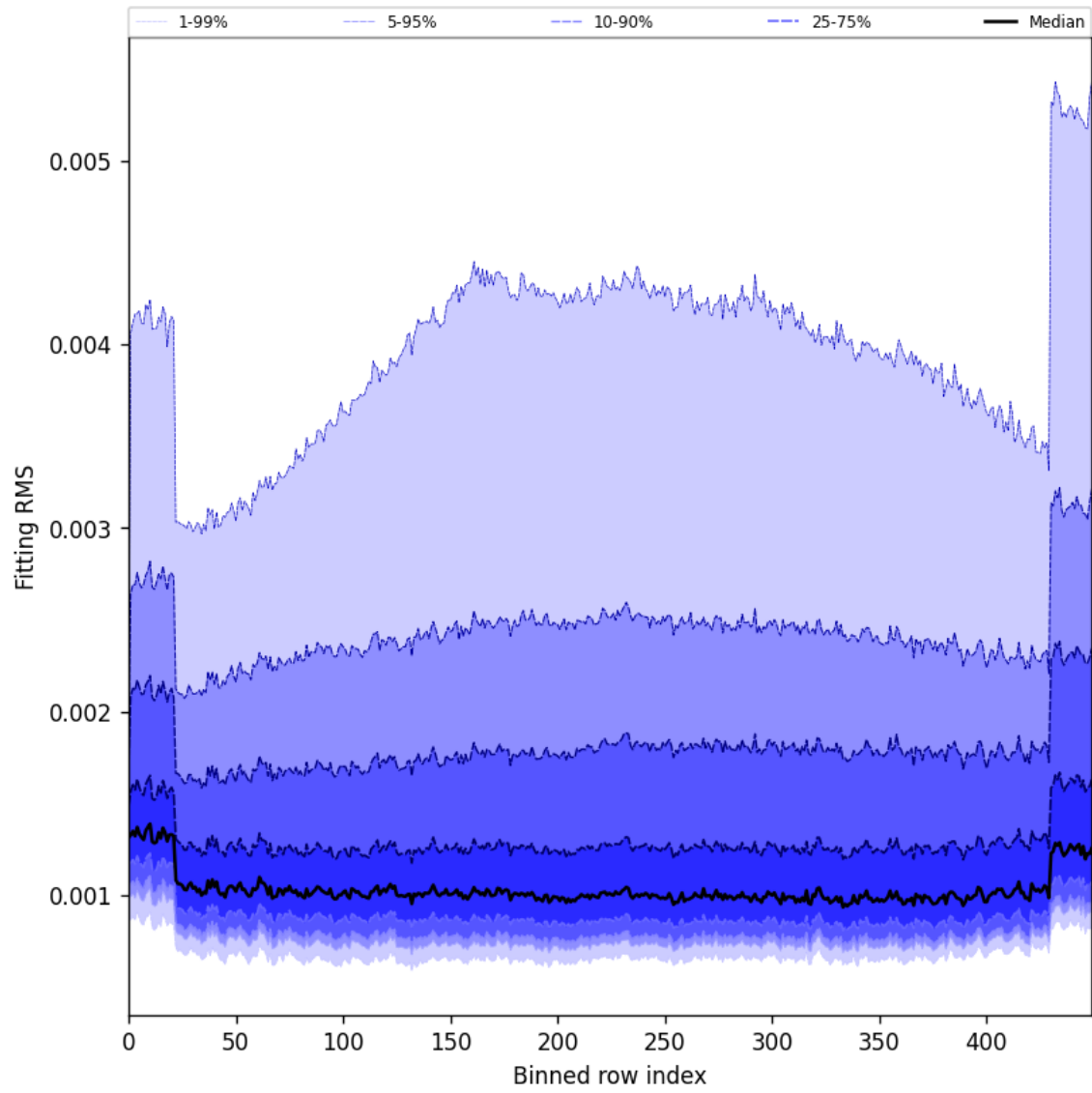
Figure 30: Along track statistics of “Fitting RMS” for 2024-10-08 to 2024-10-09
