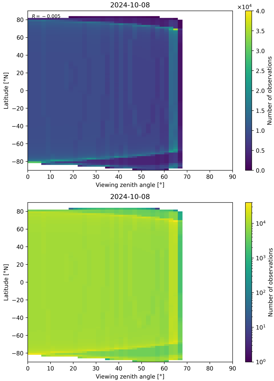
Figure 49: Scatter density plot of “Viewing zenith angle” against “Latitude” for 2024-10-08 to 2024-10-09.
