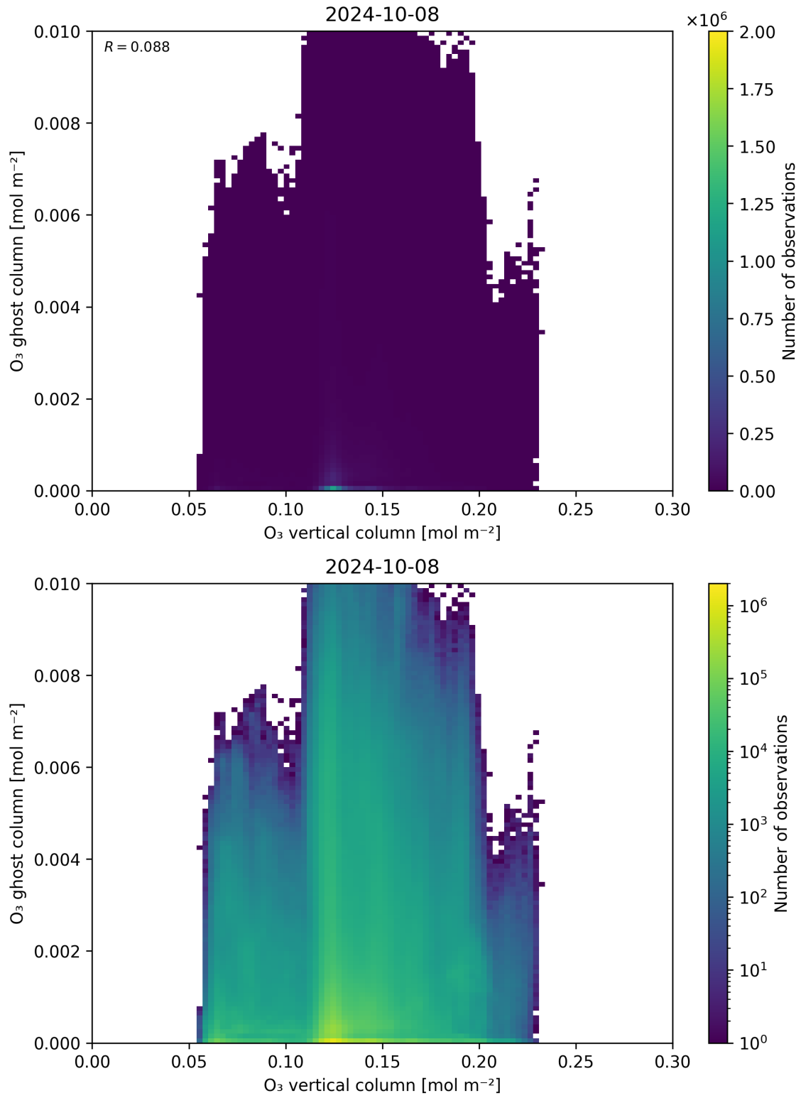
Figure 40: Scatter density plot of “O 3 vertical column” against “O 3 ghost column” for 2024-10-08 to 2024-10-09.
