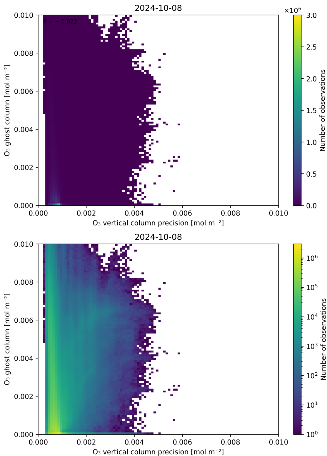
Figure 43: Scatter density plot of “O 3 vertical column precision” against “O 3 ghost column” for 2024-10-08 to 2024-10-09.
