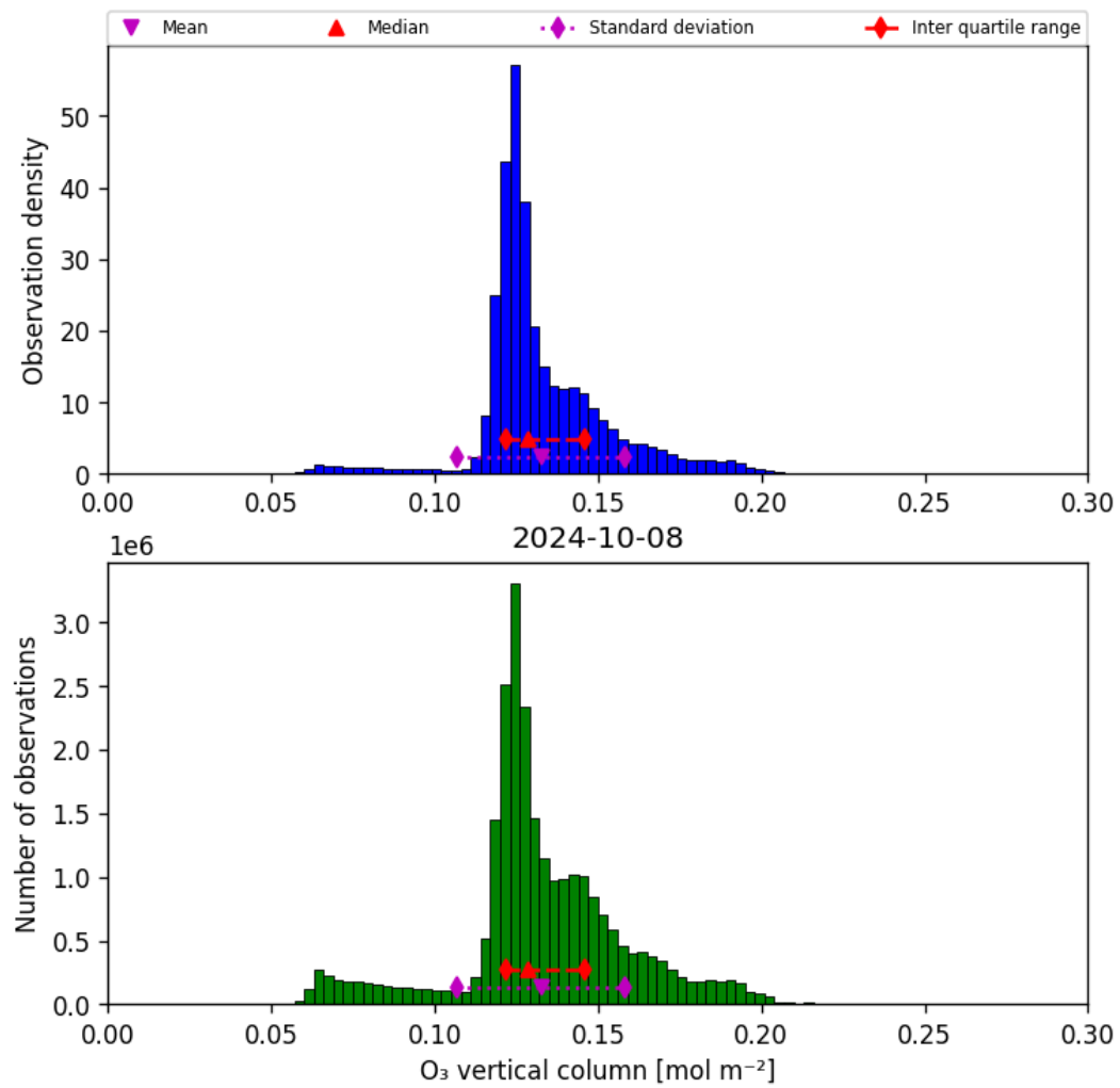
Figure 21: Histogram of “O 3 vertical column” for 2024-10-08 to 2024-10-09
