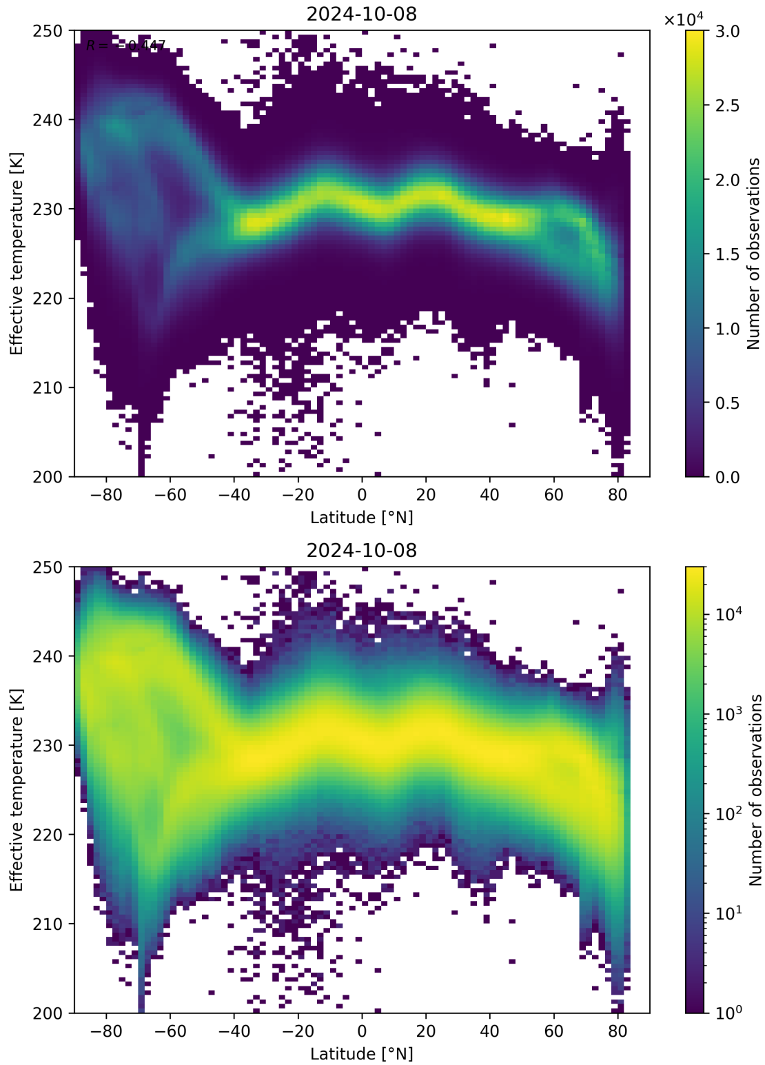
Figure 34: Scatter density plot of “Latitude” against “Effective temperature” for 2024-10-08 to 2024-10-09.
