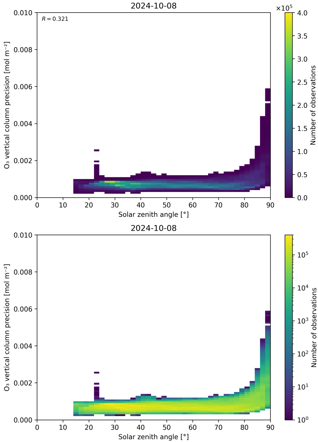
Figure 48: Scatter density plot of “Solar zenith angle” against “O 3 vertical column precision” for 2024-10-08 to 2024-10-09.
