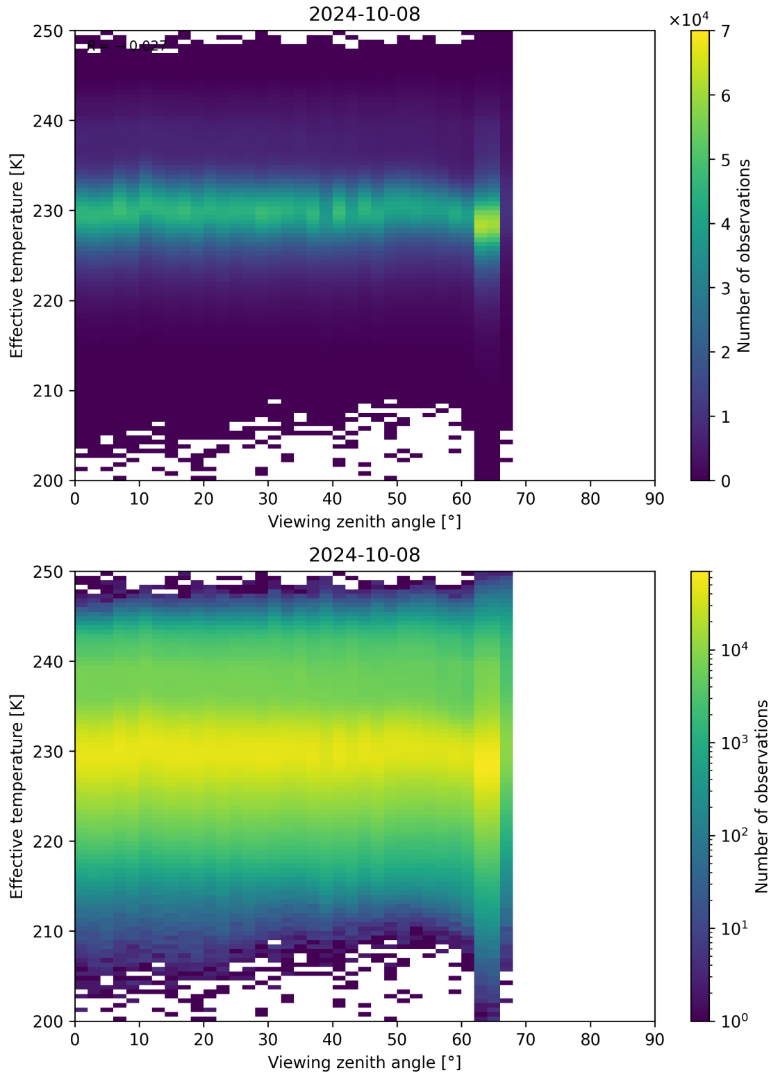
Figure 50: Scatter density plot of “Viewing zenith angle” against “Effective temperature” for 2024-10-08 to 2024-10-09.
