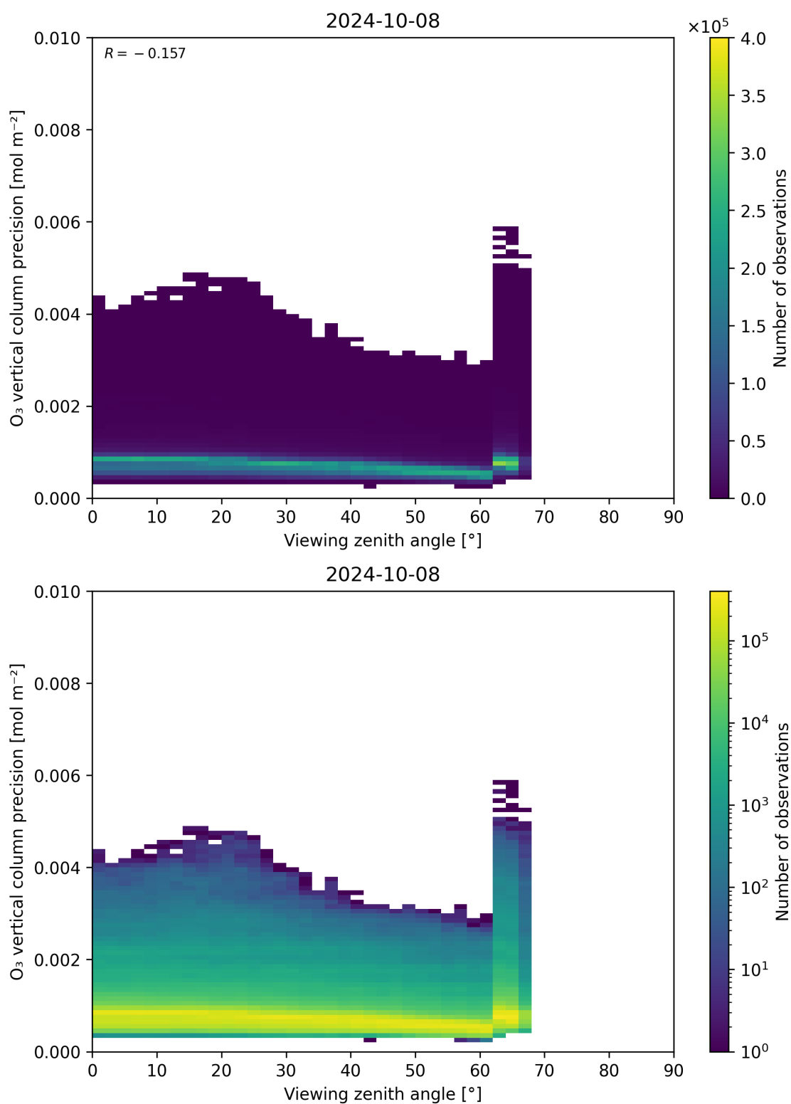
Figure 53: Scatter density plot of “Viewing zenith angle” against “O 3 vertical column precision” for 2024-10-08 to 2024-10-09.
