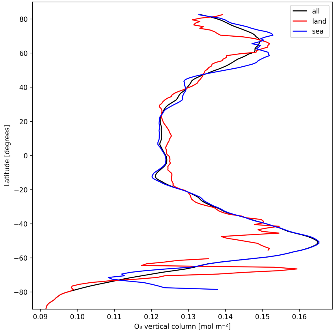
Figure 14: Zonal average of “O 3 vertical column” for 2024-10-08 to 2024-10-09.
