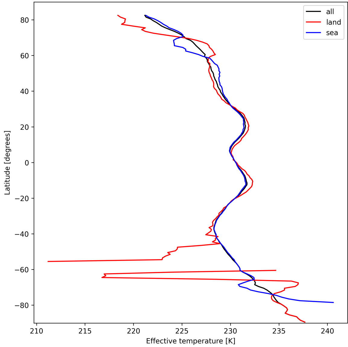
Figure 17: Zonal average of “Effective temperature” for 2024-10-08 to 2024-10-09.
