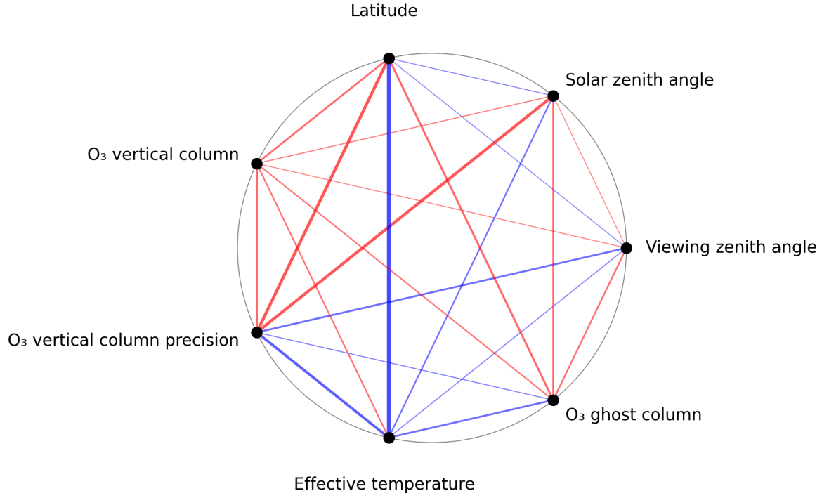
Figure 1: Map of correlation graph for 2024-10-08 to 2024-10-09.
