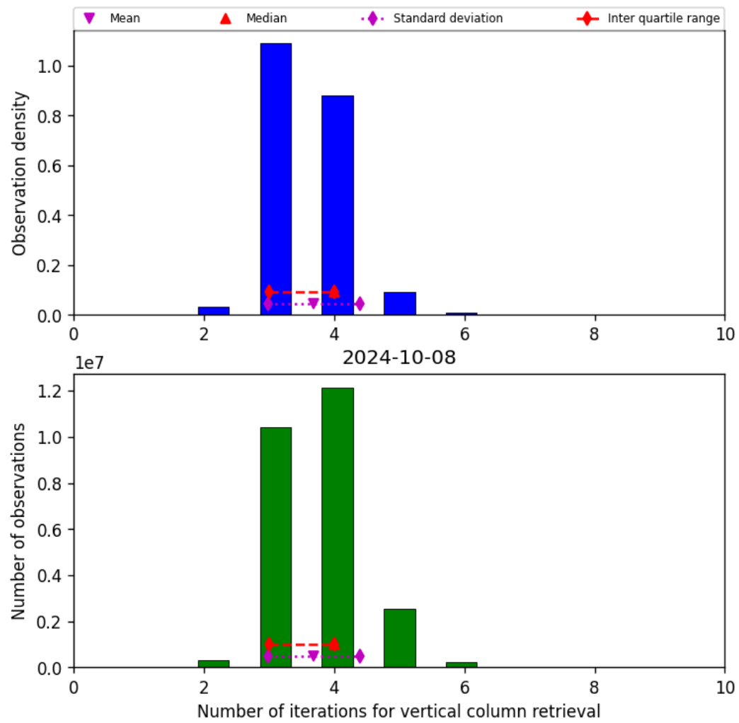
Figure 26: Histogram of “Number of iterations for vertical column retrieval” for 2024-10-08 to 2024-10-09
