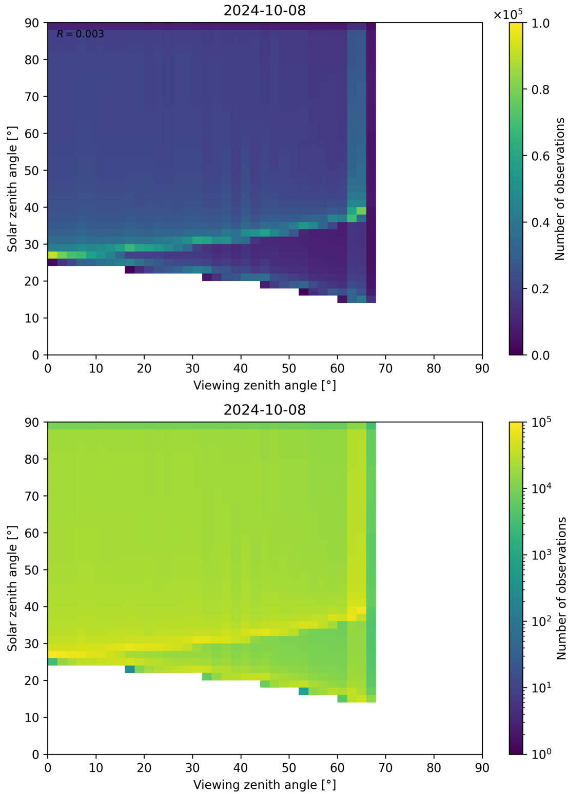
Figure 54: Scatter density plot of “Viewing zenith angle” against “Solar zenith angle” for 2024-10-08 to 2024-10-09.
