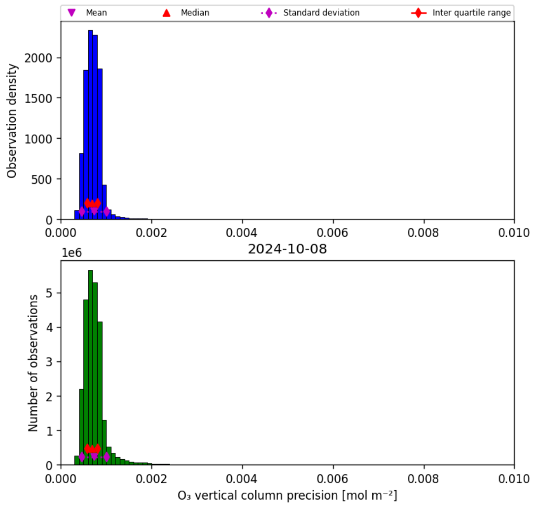
Figure 22: Histogram of “O 3 vertical column precision” for 2024-10-08 to 2024-10-09
