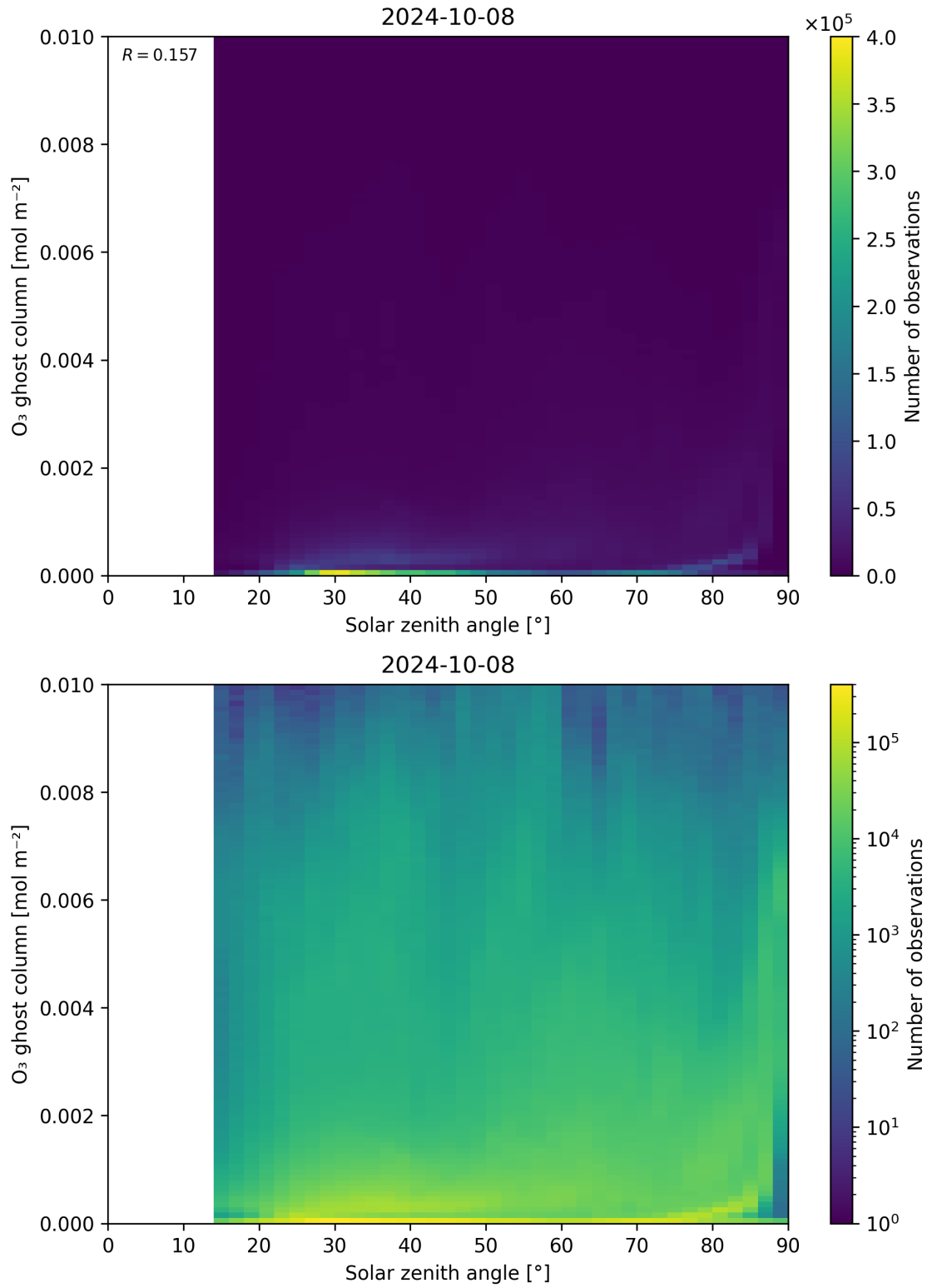
Figure 46: Scatter density plot of “Solar zenith angle” against “O 3 ghost column” for 2024-10-08 to 2024-10-09.
