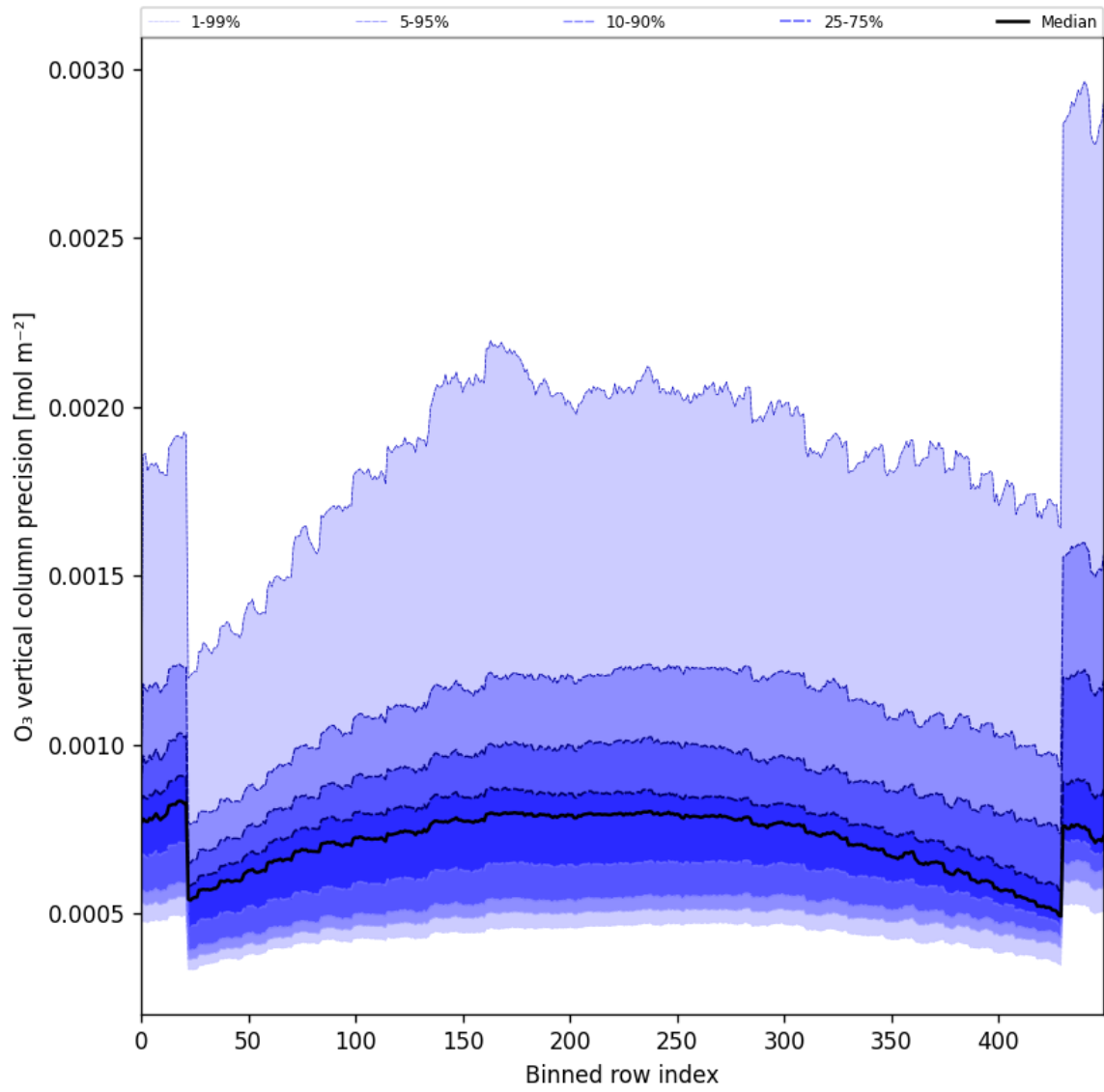
Figure 29: Along track statistics of “O 3 vertical column precision” for 2024-10-08 to 2024-10-09
