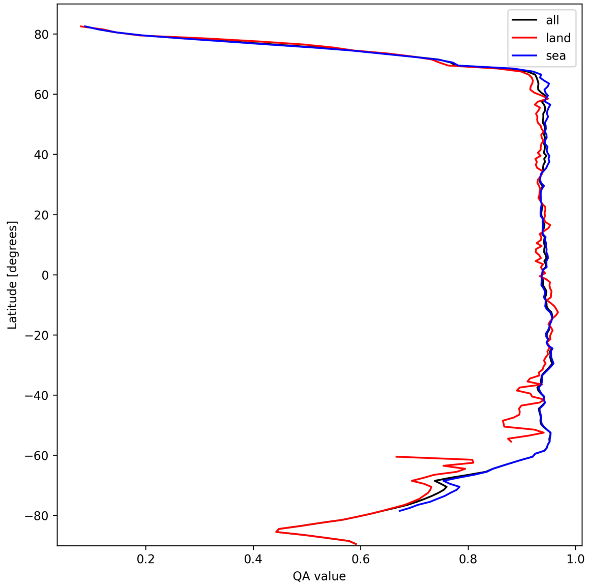
Figure 13: Zonal average of “QA value” for 2024-10-08 to 2024-10-09.
