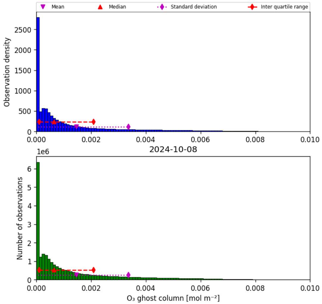
Figure 25: Histogram of “O 3 ghost column” for 2024-10-08 to 2024-10-09
