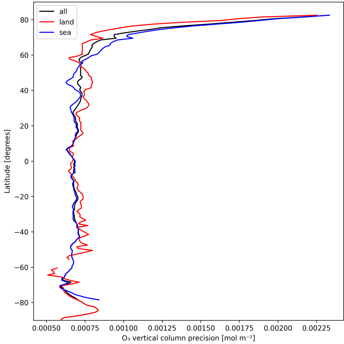
Figure 15: Zonal average of “O 3 vertical column precision” for 2024-10-08 to 2024-10-09.
