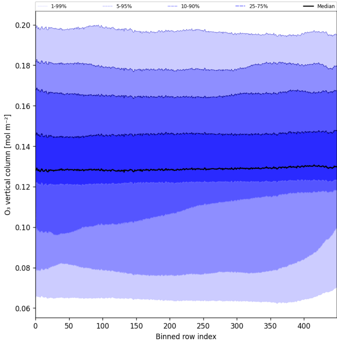
Figure 28: Along track statistics of “O 3 vertical column” for 2024-10-08 to 2024-10-09
