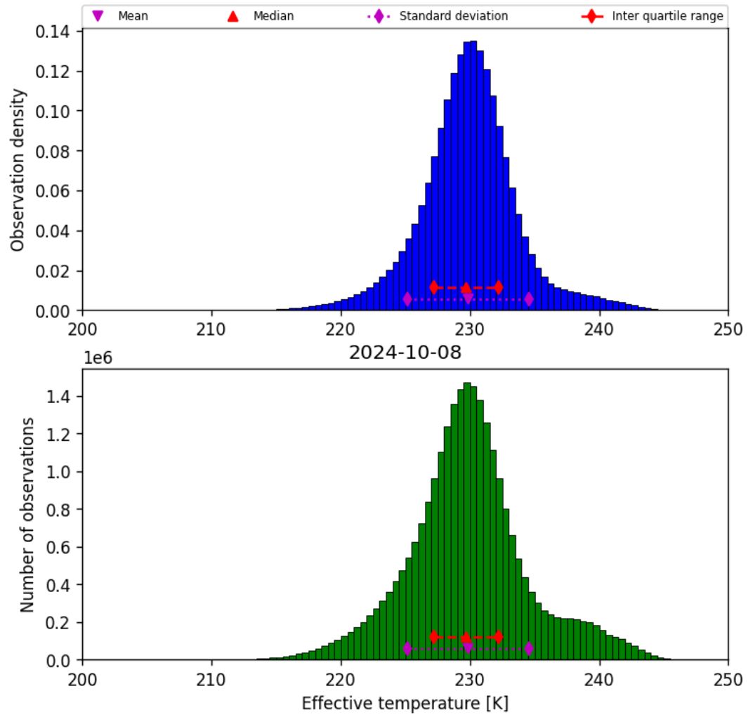
Figure 24: Histogram of “Effective temperature” for 2024-10-08 to 2024-10-09
