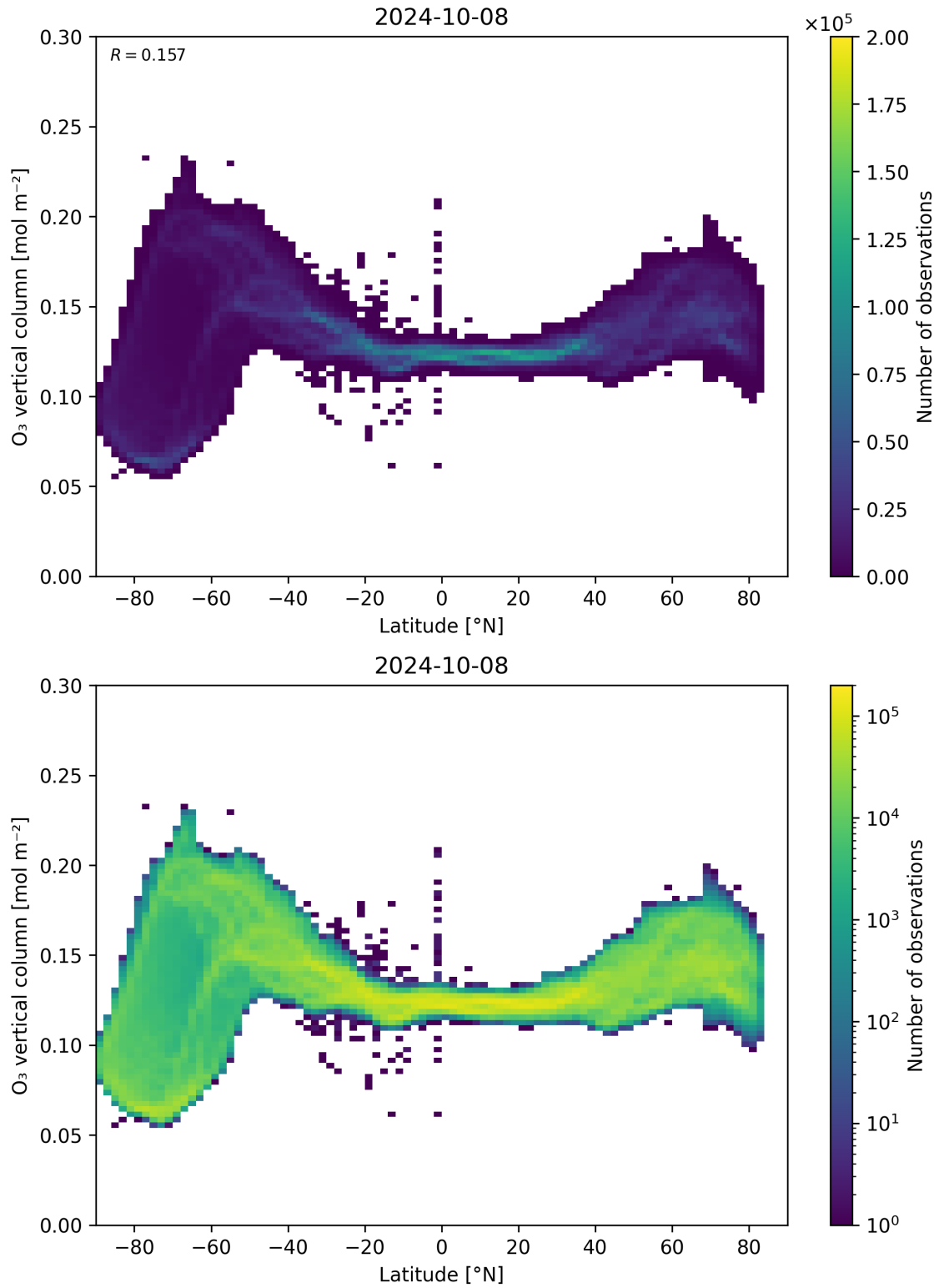
Figure 36: Scatter density plot of “Latitude” against “O 3 vertical column” for 2024-10-08 to 2024-10-09.
