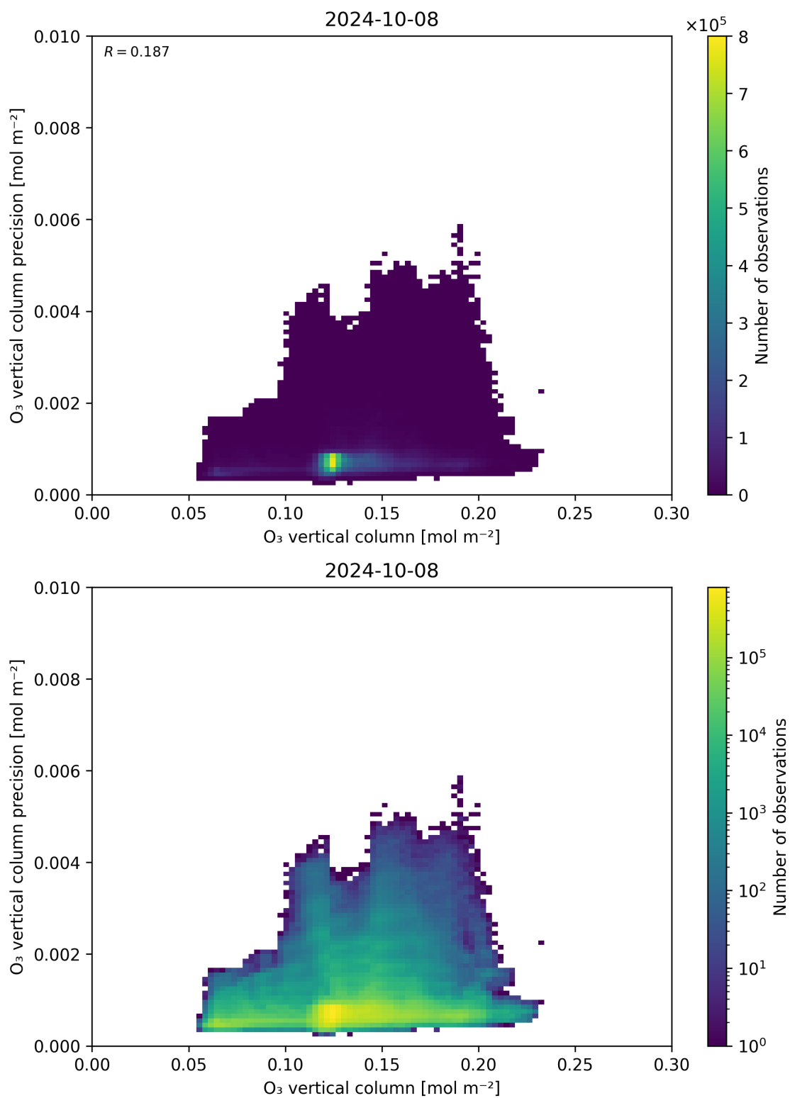
Figure 41: Scatter density plot of “O 3 vertical column” against “O 3 vertical column precision” for 2024-10-08 to 2024-10-09.
