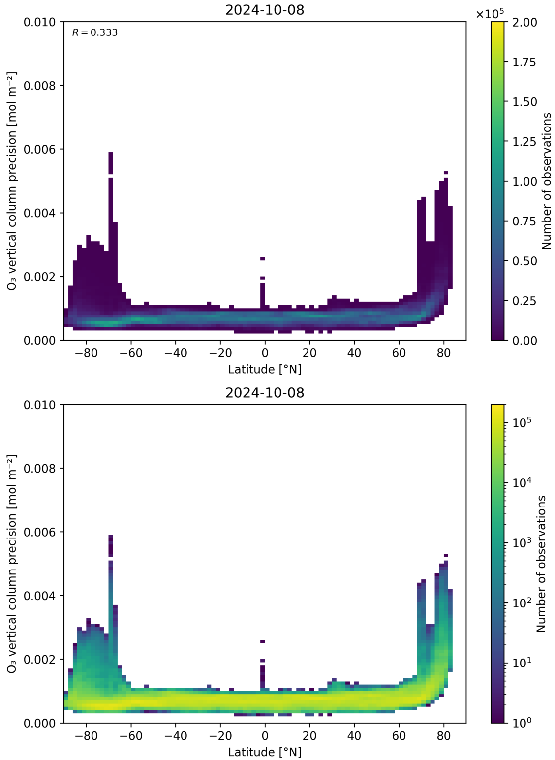
Figure 37: Scatter density plot of “Latitude” against “O 3 vertical column precision” for 2024-10-08 to 2024-10-09.
