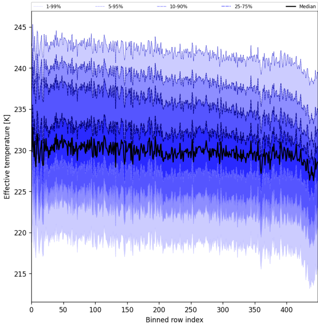
Figure 31: Along track statistics of “Effective temperature” for 2024-10-08 to 2024-10-09
