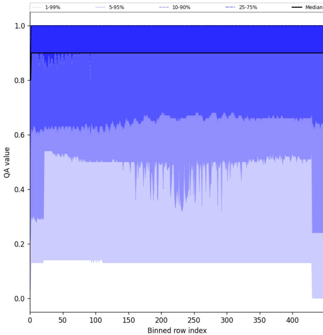
Figure 27: Along track statistics of “QA value” for 2024-10-08 to 2024-10-09
