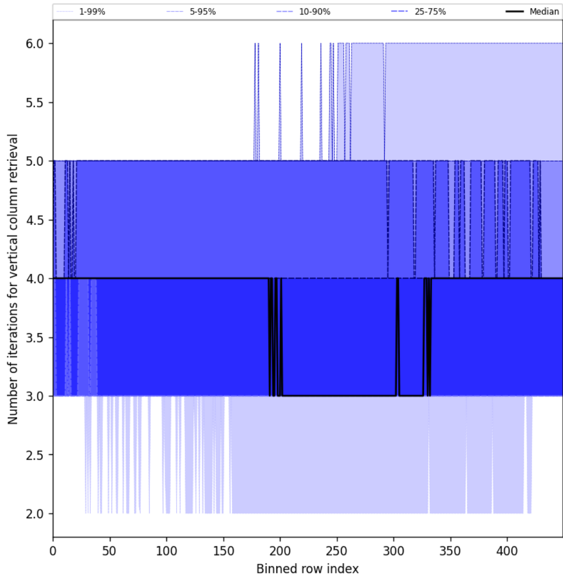
Figure 33: Along track statistics of “Number of iterations for vertical column retrieval” for 2024-10-08 to 2024-10-09
