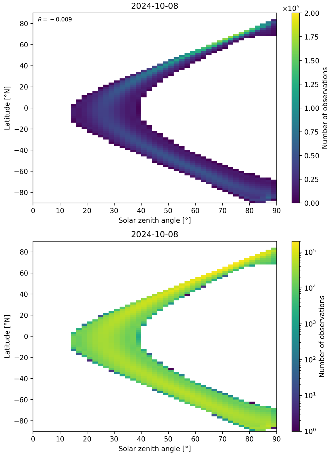
Figure 44: Scatter density plot of “Solar zenith angle” against “Latitude” for 2024-10-08 to 2024-10-09.
