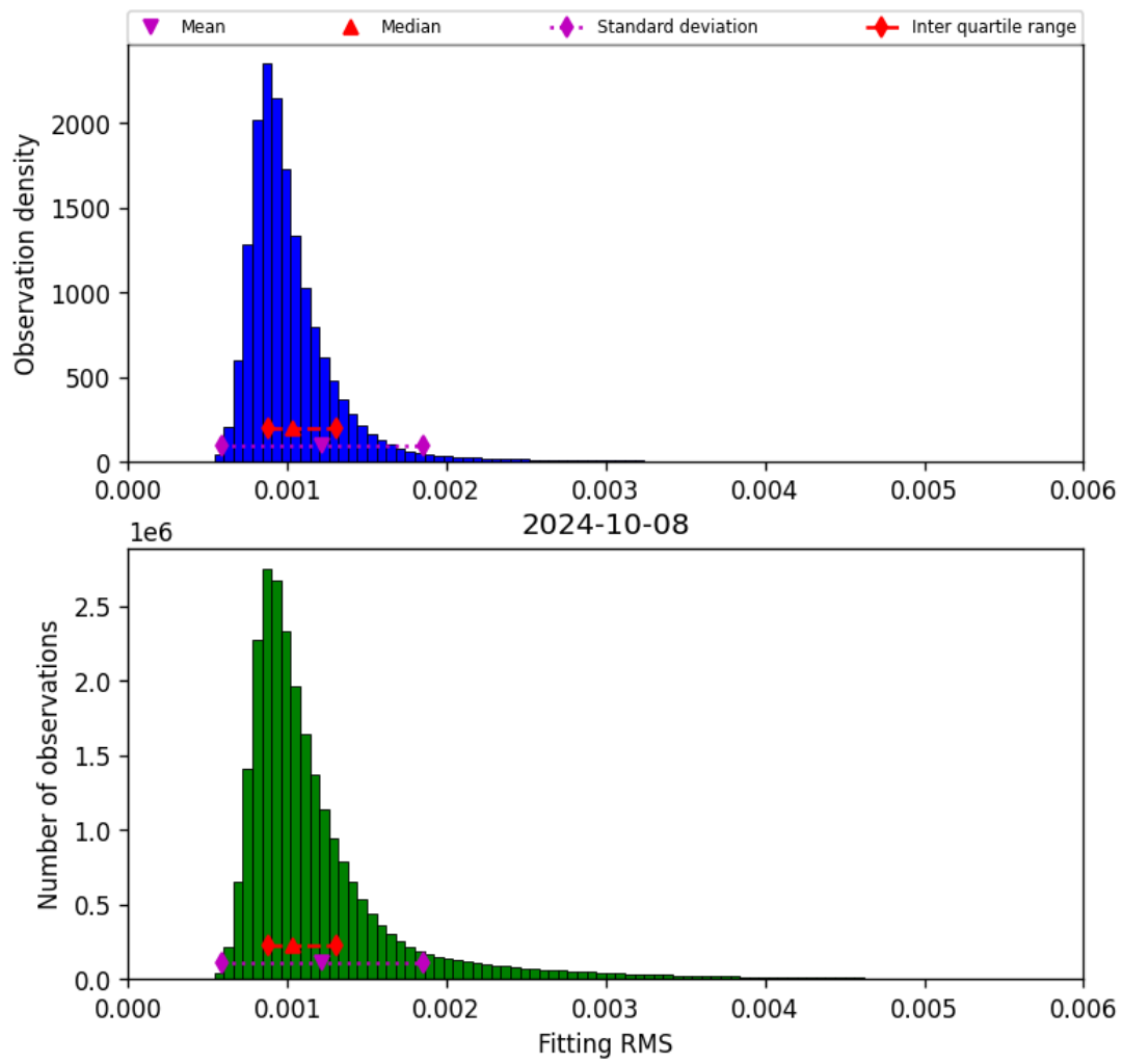
Figure 23: Histogram of “Fitting RMS” for 2024-10-08 to 2024-10-09
