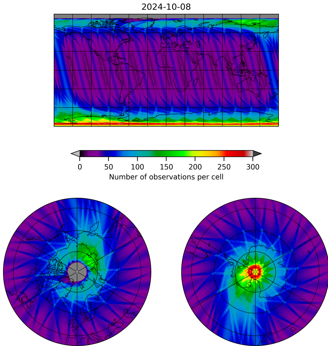
Figure 12: Map of the number of observations for 2024-10-08 to 2024-10-09
