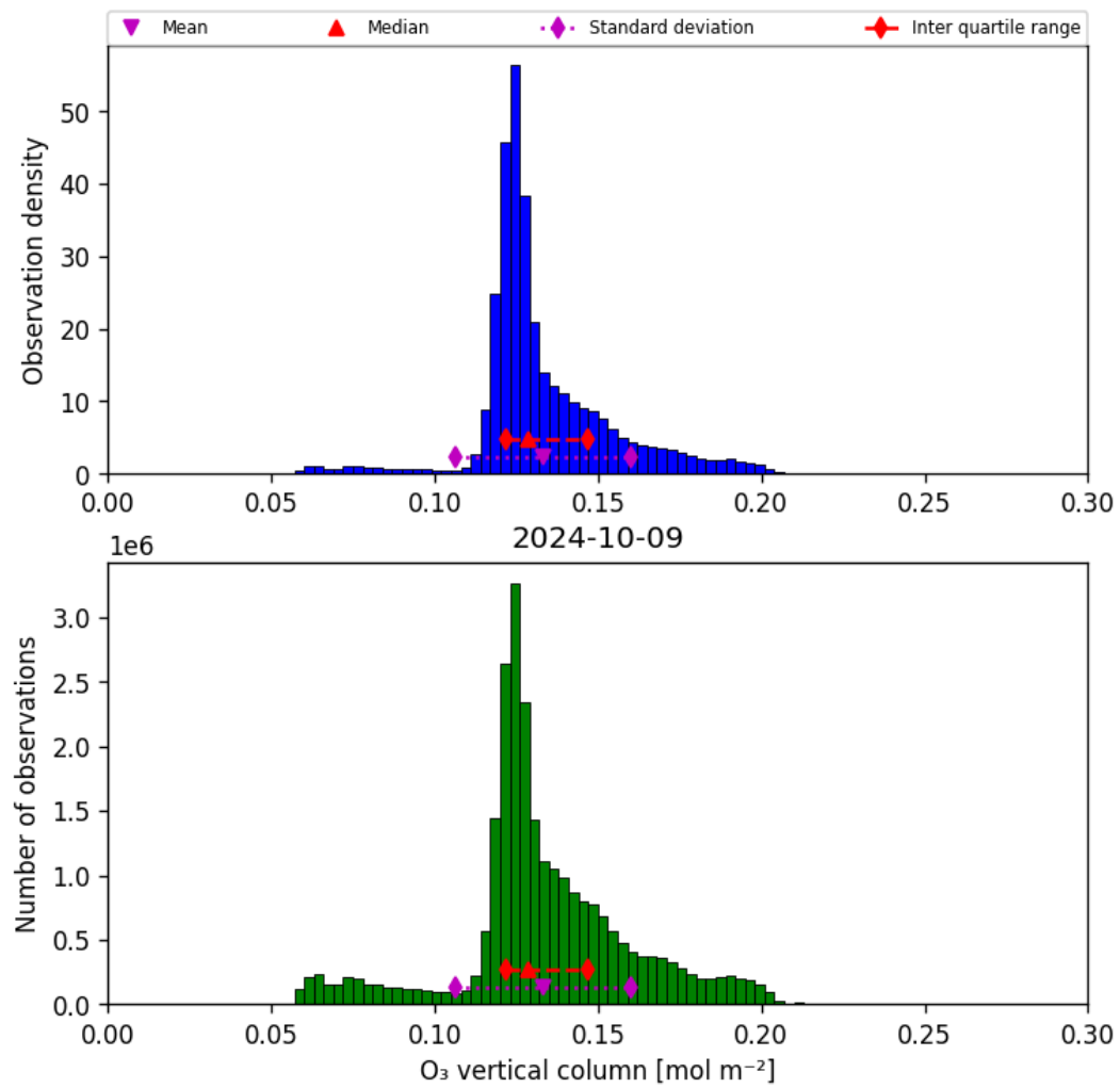
Figure 21: Histogram of “O 3 vertical column” for 2024-10-08 to 2024-10-10
