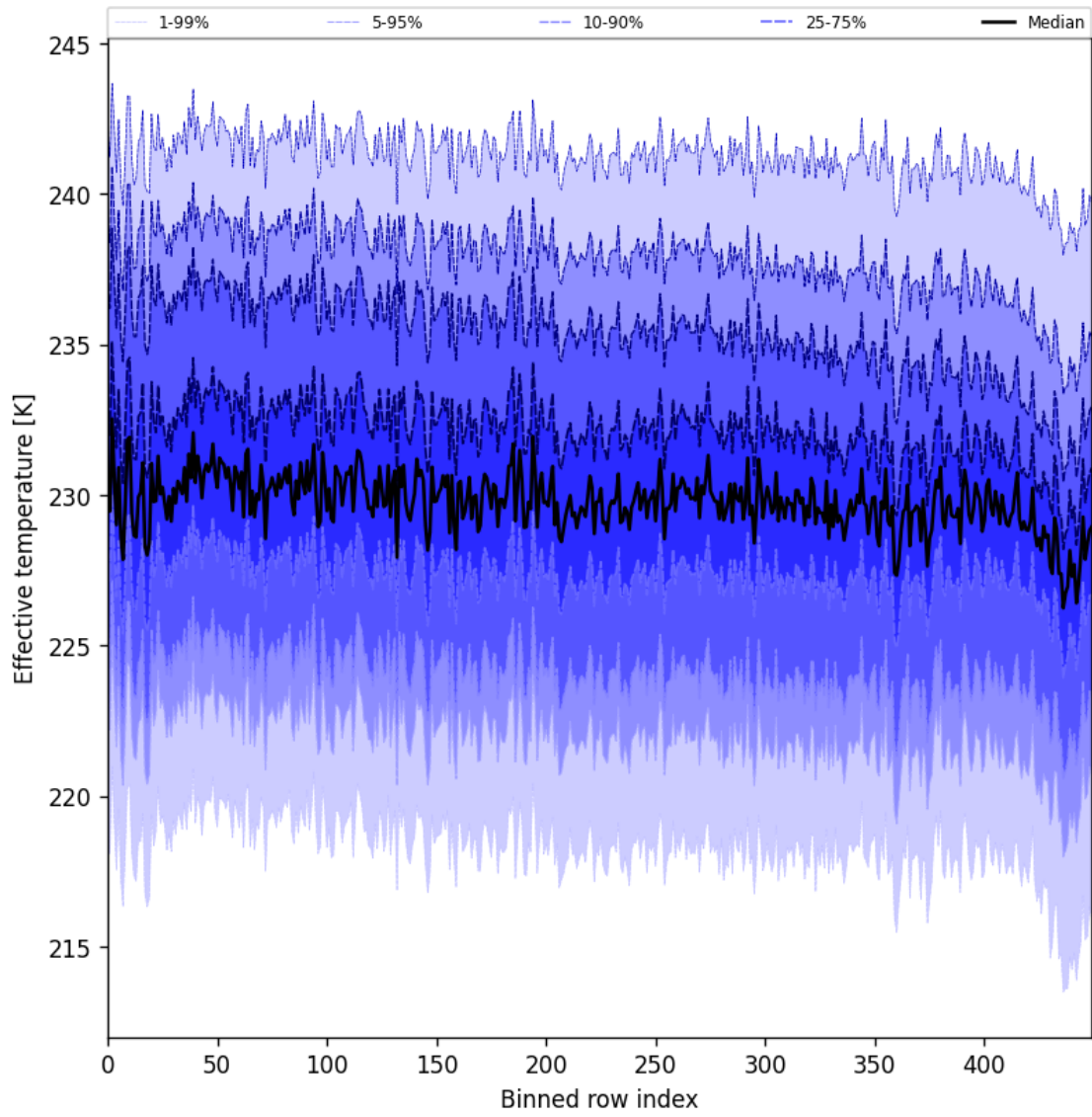
Figure 31: Along track statistics of “Effective temperature” for 2024-10-08 to 2024-10-10
