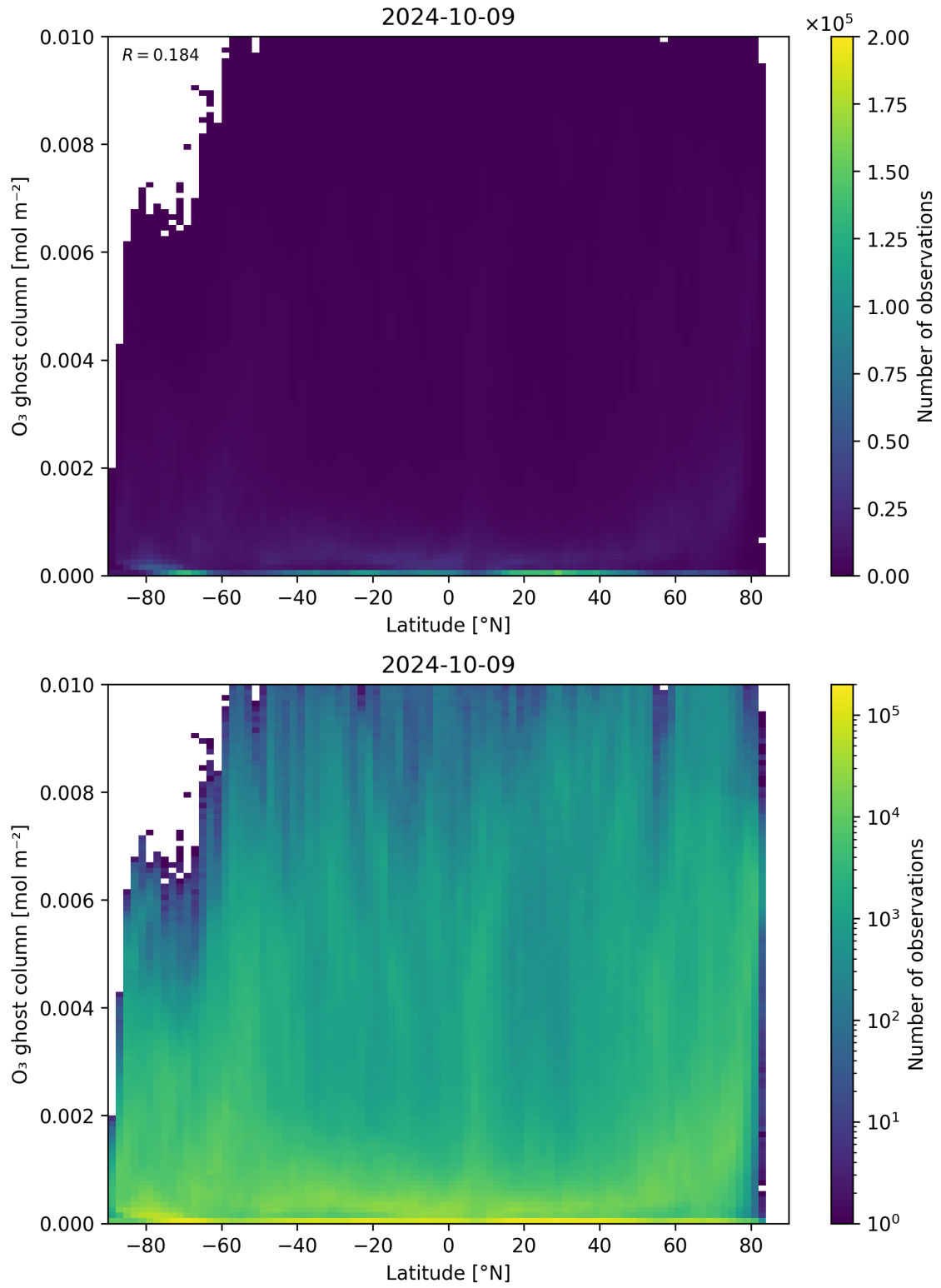
Figure 35: Scatter density plot of “Latitude” against “O 3 ghost column” for 2024-10-08 to 2024-10-10.
