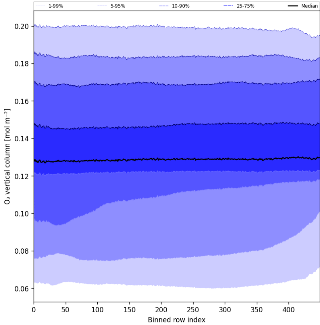
Figure 28: Along track statistics of “O 3 vertical column” for 2024-10-08 to 2024-10-10
