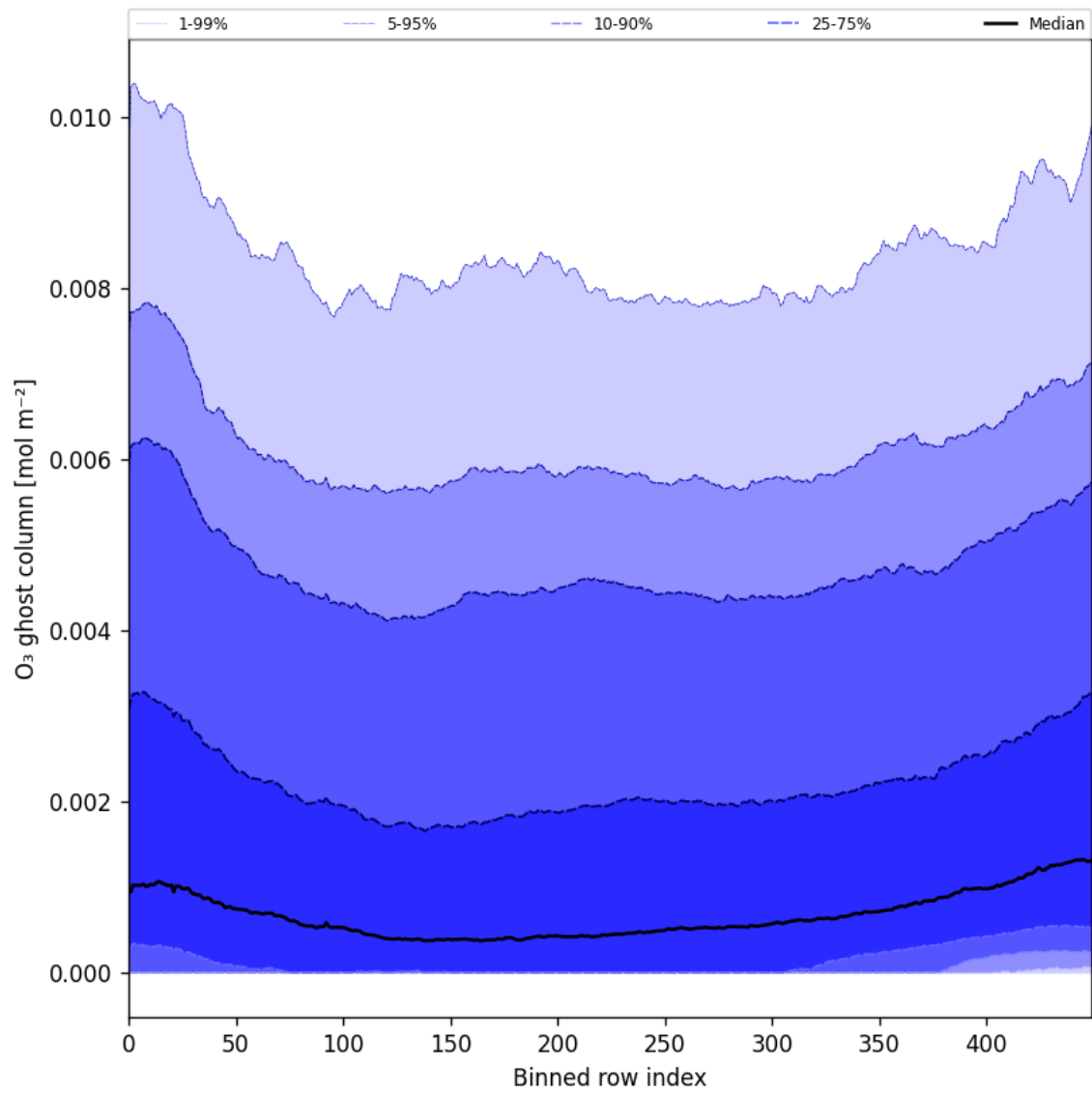
Figure 32: Along track statistics of “O 3 ghost column” for 2024-10-08 to 2024-10-10
