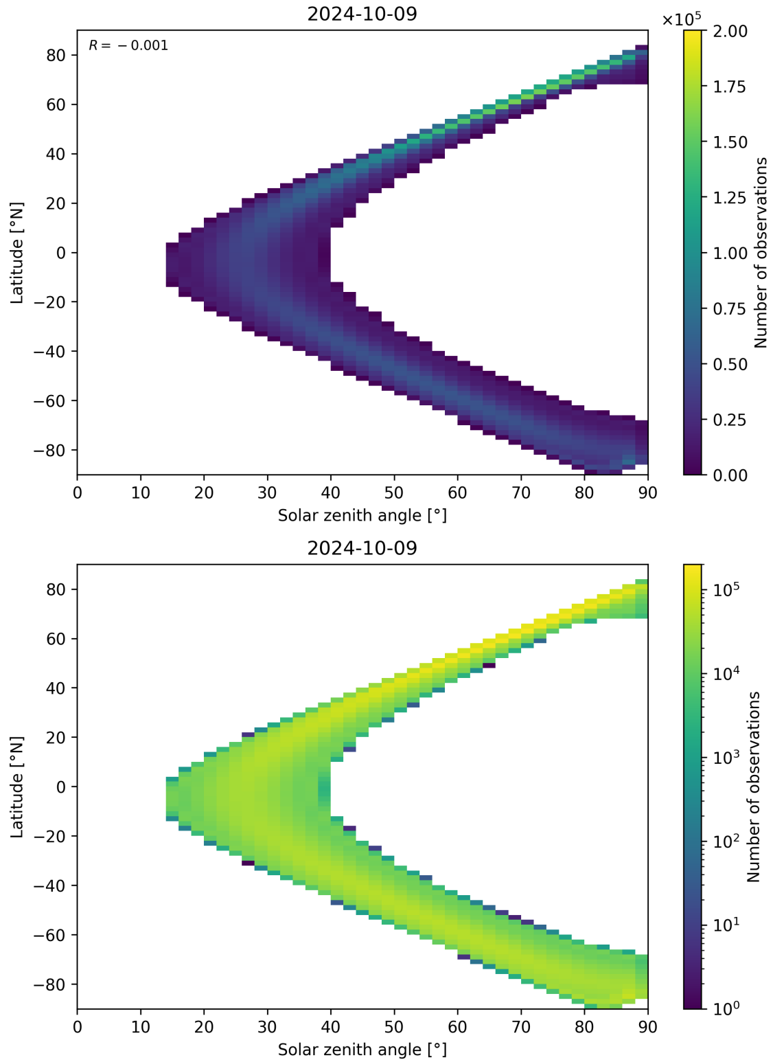
Figure 44: Scatter density plot of “Solar zenith angle” against “Latitude” for 2024-10-08 to 2024-10-10.
