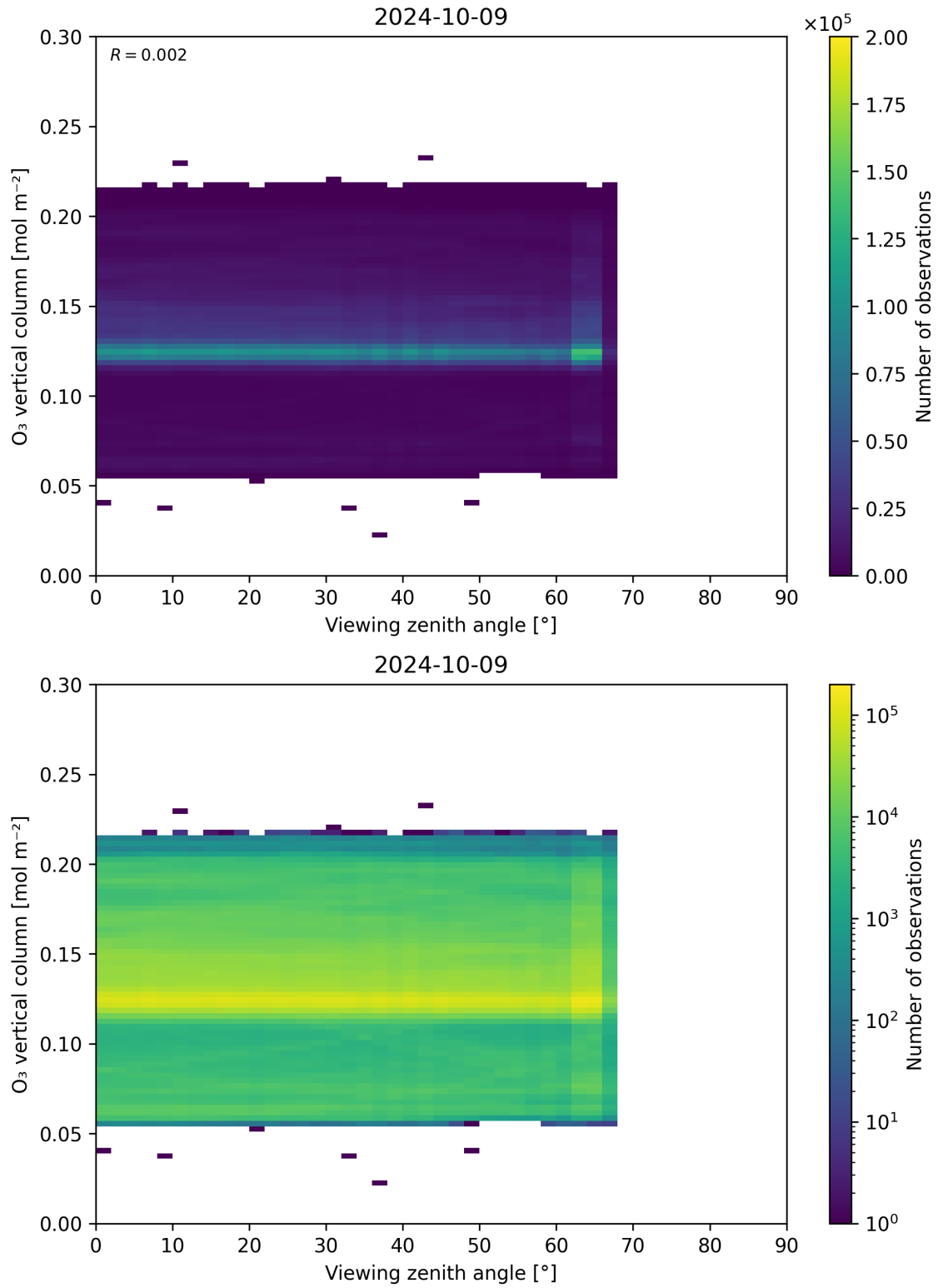
Figure 52: Scatter density plot of “Viewing zenith angle” against “O 3 vertical column” for 2024-10-08 to 2024-10-10.
