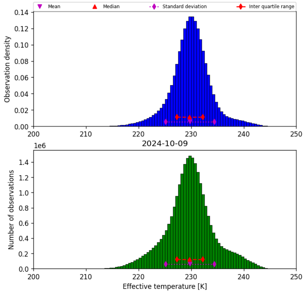
Figure 24: Histogram of “Effective temperature” for 2024-10-08 to 2024-10-10
