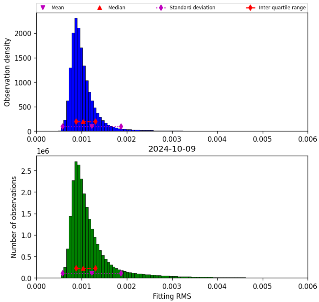
Figure 23: Histogram of “Fitting RMS” for 2024-10-08 to 2024-10-10
