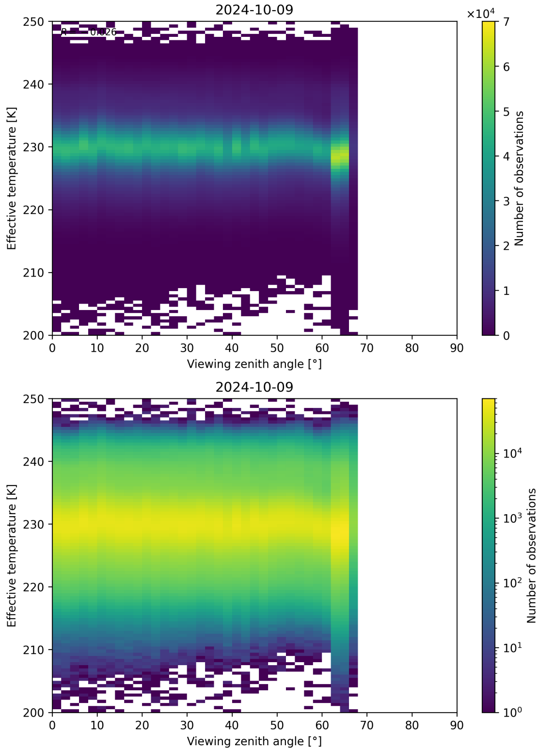
Figure 50: Scatter density plot of “Viewing zenith angle” against “Effective temperature” for 2024-10-08 to 2024-10-10.
