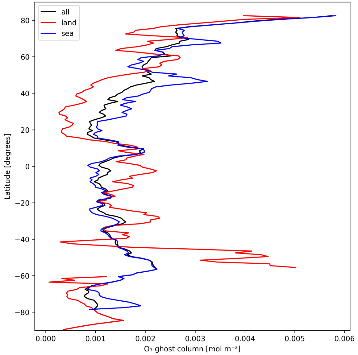
Figure 18: Zonal average of "O 3 ghost column" for 2024-10-08 to 2024-10-10.
