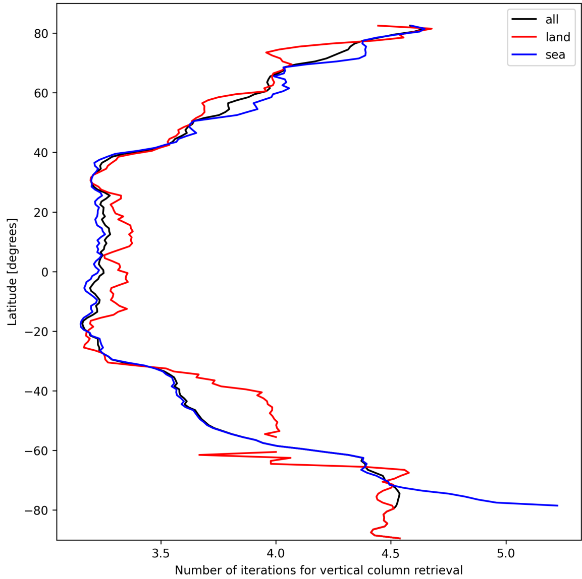
Figure 19: Zonal average of “Number of iterations for vertical column retrieval” for 2024-10-08 to 2024-10-10.
