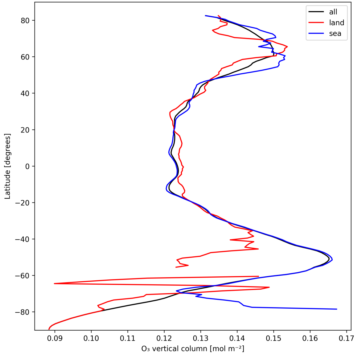
Figure 14: Zonal average of “O 3 vertical column” for 2024-10-08 to 2024-10-10.
