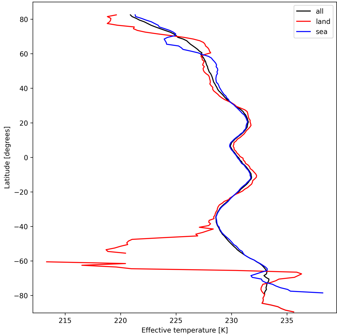
Figure 17: Zonal average of “Effective temperature” for 2024-10-08 to 2024-10-10.
