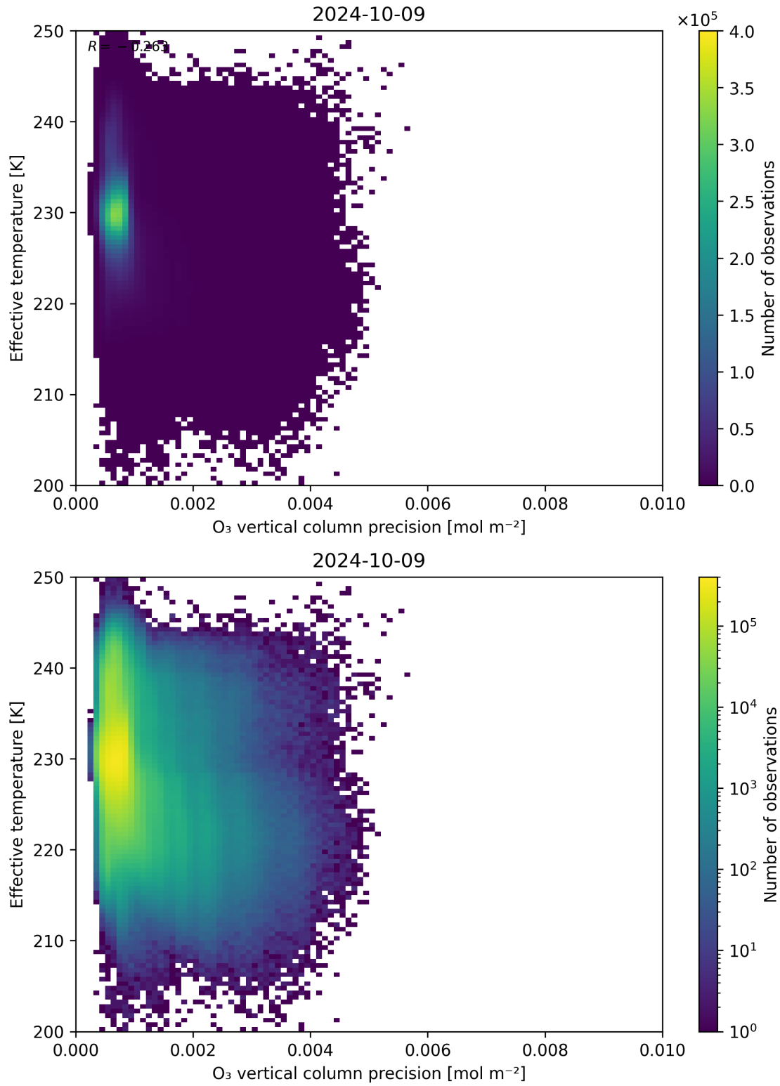
Figure 42: Scatter density plot of “O 3 vertical column precision” against “Effective temperature” for 2024-10-08 to 2024-10-10.
