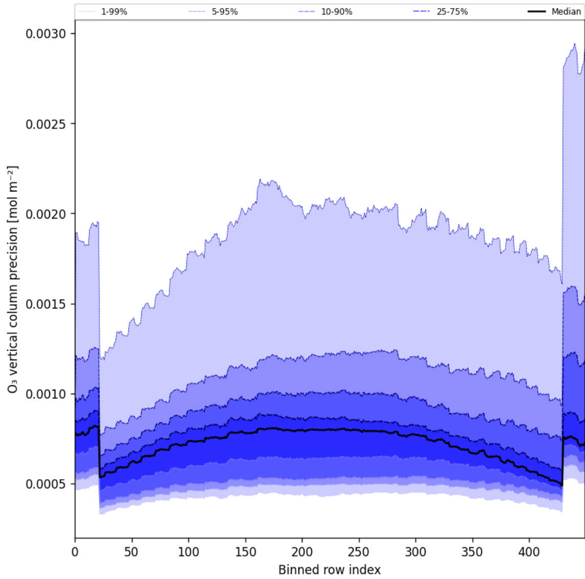
Figure 29: Along track statistics of “O 3 vertical column precision” for 2024-10-08 to 2024-10-10
