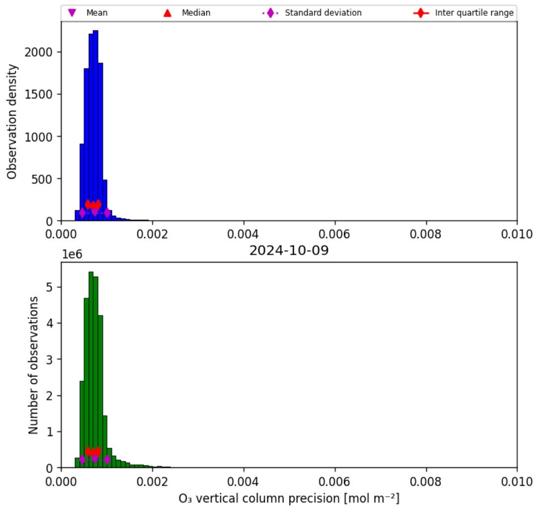
Figure 22: Histogram of “O 3 vertical column precision” for 2024-10-08 to 2024-10-10
