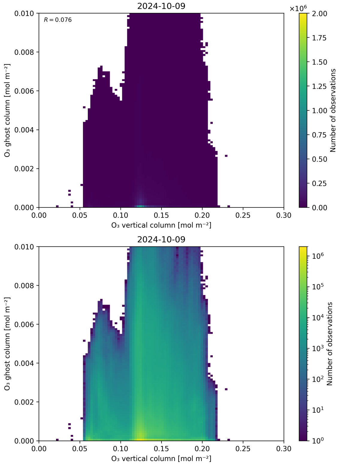
Figure 40: Scatter density plot of “O 3 vertical column” against “O 3 ghost column” for 2024-10-08 to 2024-10-10.
