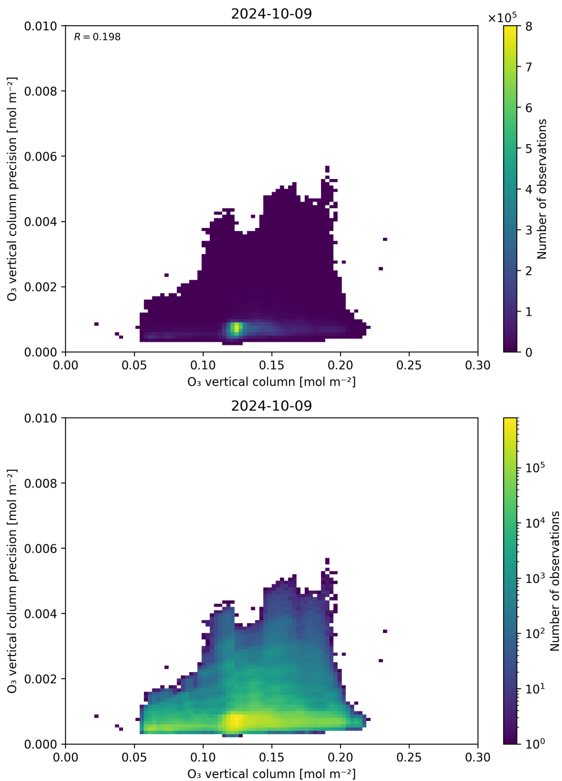
Figure 41: Scatter density plot of “O 3 vertical column” against “O 3 vertical column precision” for 2024-10-08 to 2024-10-10.
