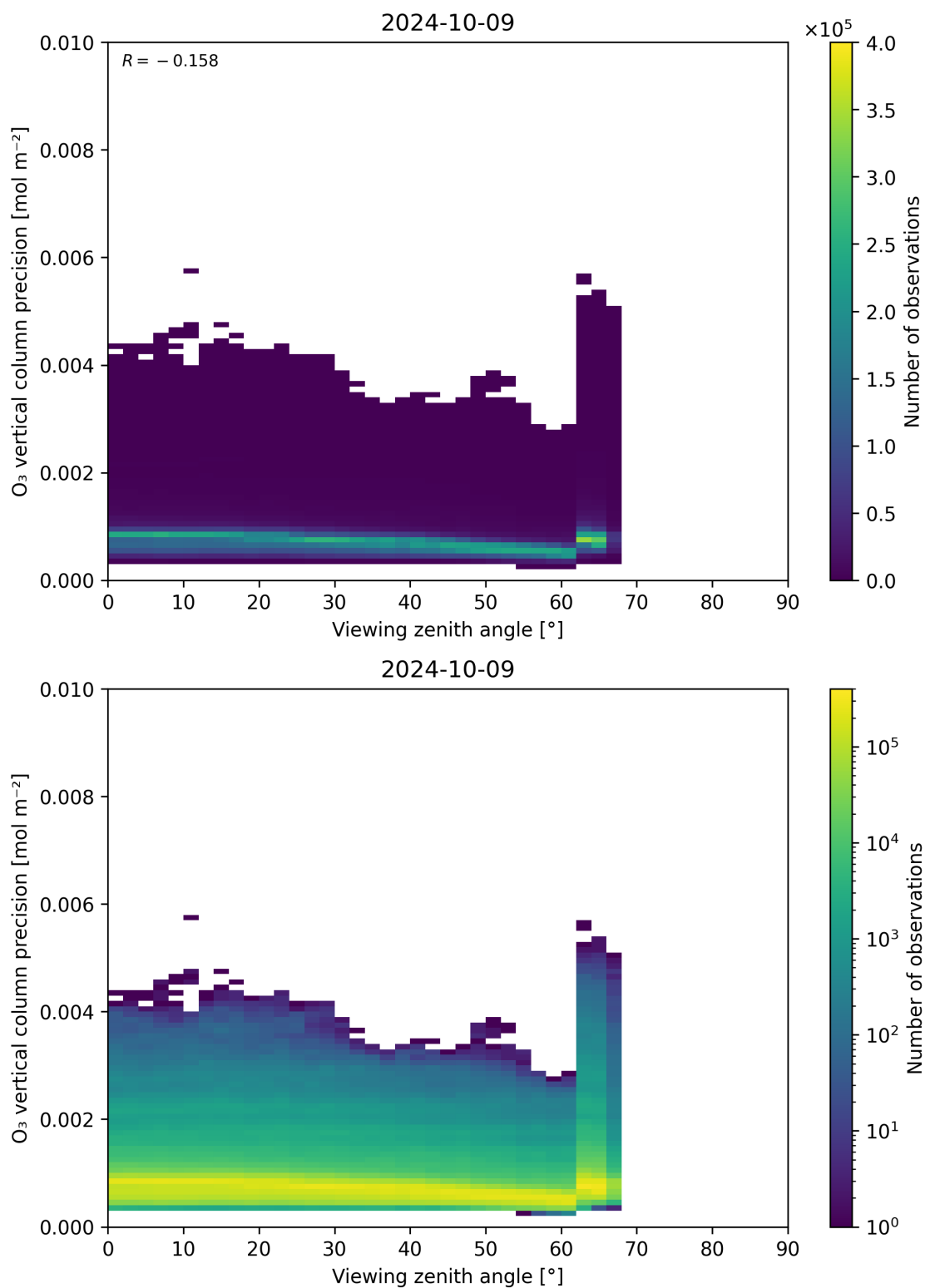
Figure 53: Scatter density plot of “Viewing zenith angle” against “O 3 vertical column precision” for 2024-10-08 to 2024-10-10.
