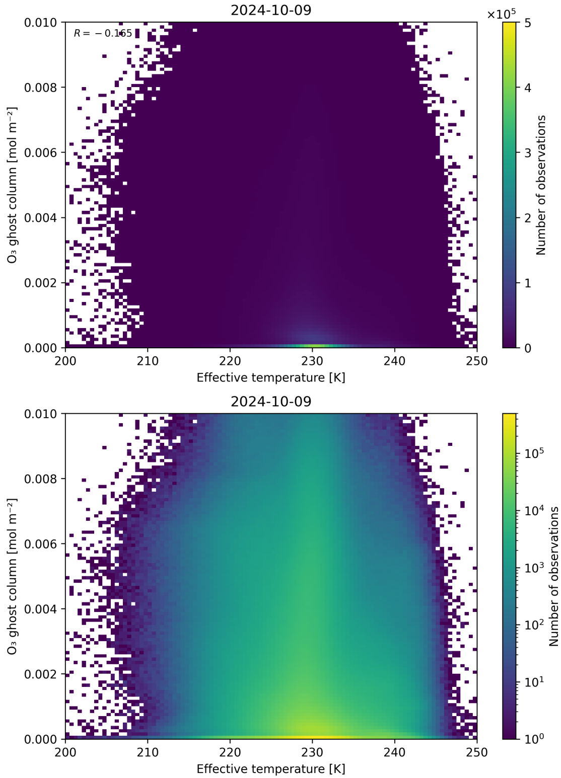
Figure 38: Scatter density plot of “Effective temperature” against “O 3 ghost column” for 2024-10-08 to 2024-10-10.
