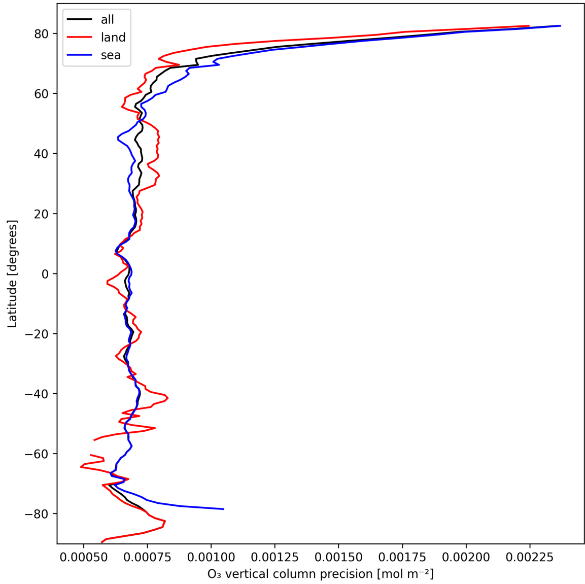
Figure 15: Zonal average of “O 3 vertical column precision” for 2024-10-08 to 2024-10-10.
