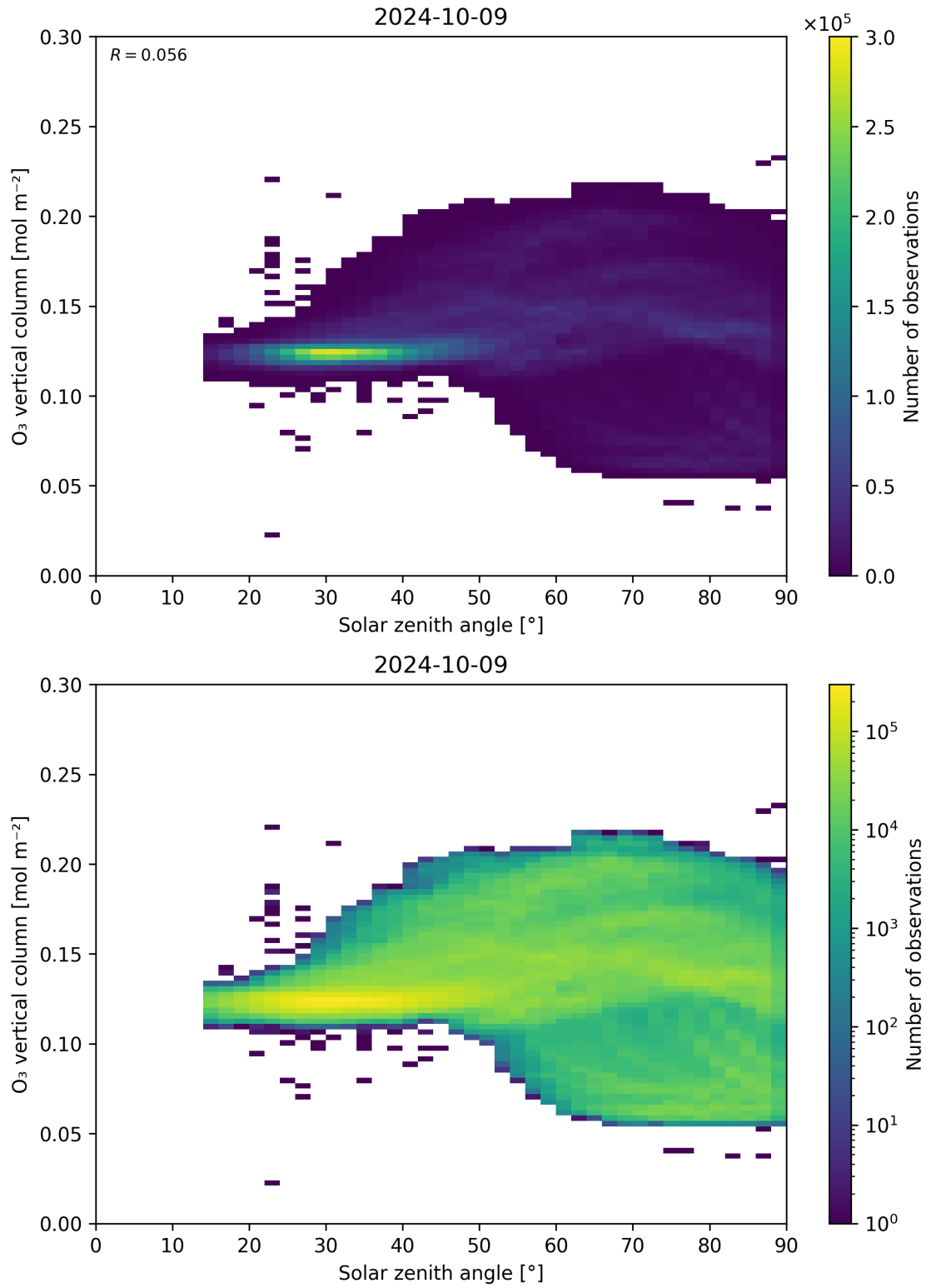
Figure 47: Scatter density plot of “Solar zenith angle” against “O 3 vertical column” for 2024-10-08 to 2024-10-10.
