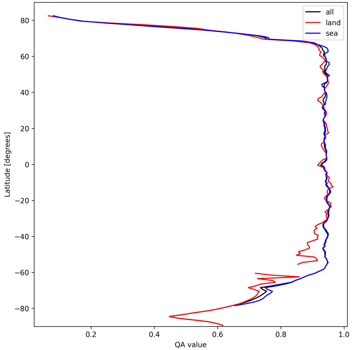
Figure 13: Zonal average of “QA value” for 2024-10-08 to 2024-10-10.
