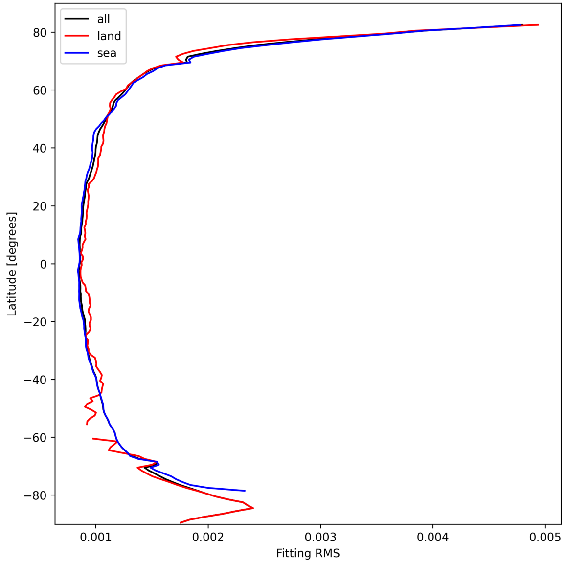
Figure 16: Zonal average of “Fitting RMS” for 2024-10-08 to 2024-10-10.
