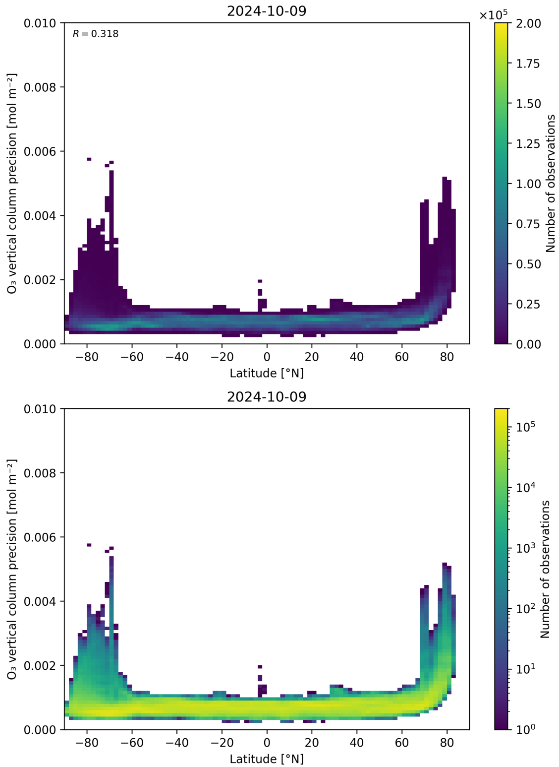
Figure 37: Scatter density plot of “Latitude” against “O 3 vertical column precision” for 2024-10-08 to 2024-10-10.
