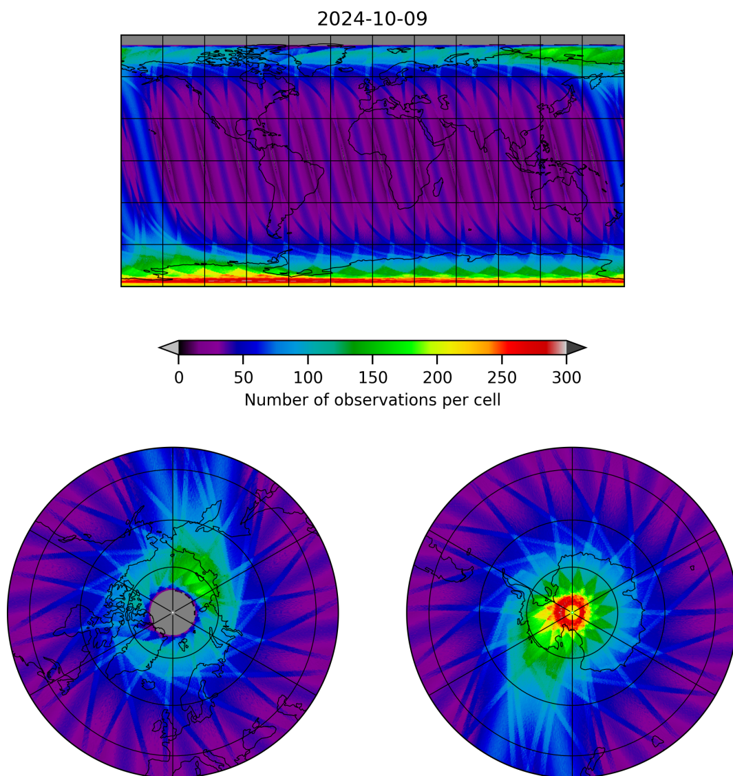
Figure 12: Map of the number of observations for 2024-10-08 to 2024-10-10
