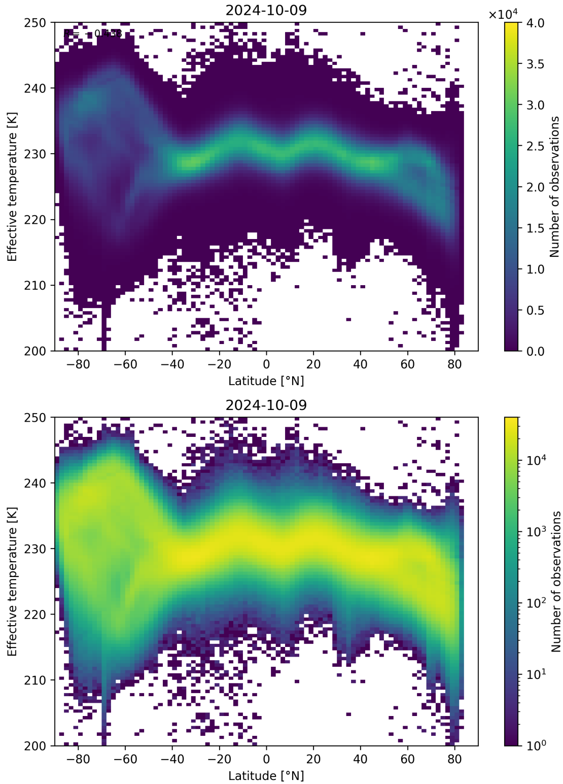
Figure 34: Scatter density plot of “Latitude” against “Effective temperature” for 2024-10-08 to 2024-10-10.
