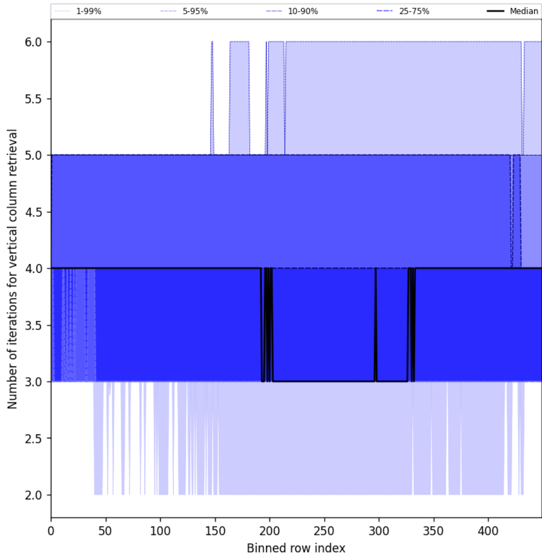
Figure 33: Along track statistics of “Number of iterations for vertical column retrieval” for 2024-10-08 to 2024-10-10
