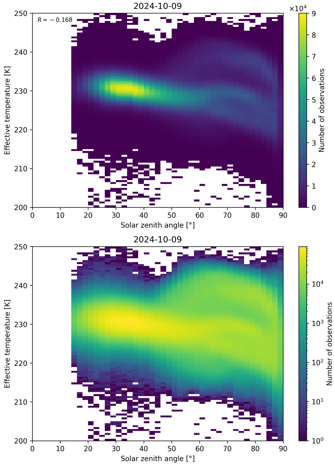
Figure 45: Scatter density plot of “Solar zenith angle” against “Effective temperature” for 2024-10-08 to 2024-10-10.
