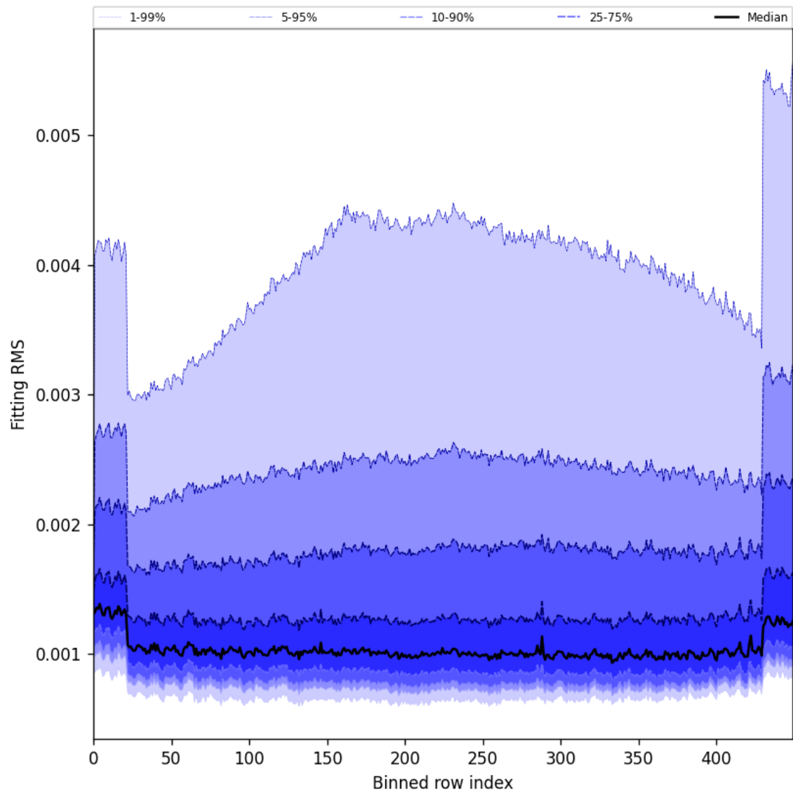
Figure 30: Along track statistics of “Fitting RMS” for 2024-10-08 to 2024-10-10
