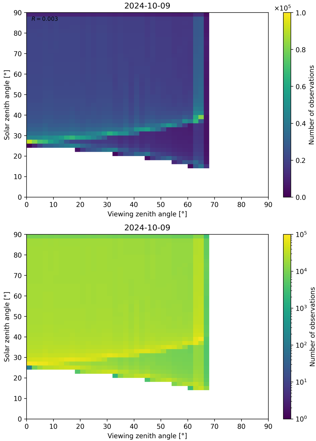
Figure 54: Scatter density plot of “Viewing zenith angle” against “Solar zenith angle” for 2024-10-08 to 2024-10-10.
