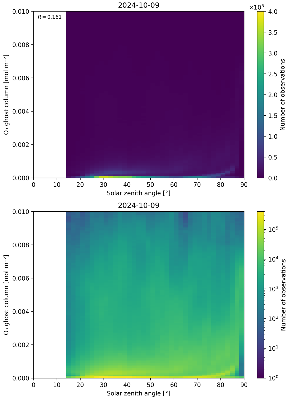
Figure 46: Scatter density plot of “Solar zenith angle” against “O 3 ghost column” for 2024-10-08 to 2024-10-10.
