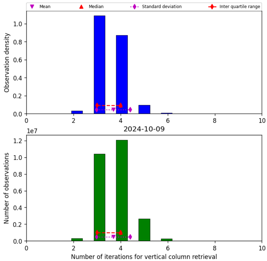
Figure 26: Histogram of “Number of iterations for vertical column retrieval” for 2024-10-08 to 2024-10-10
