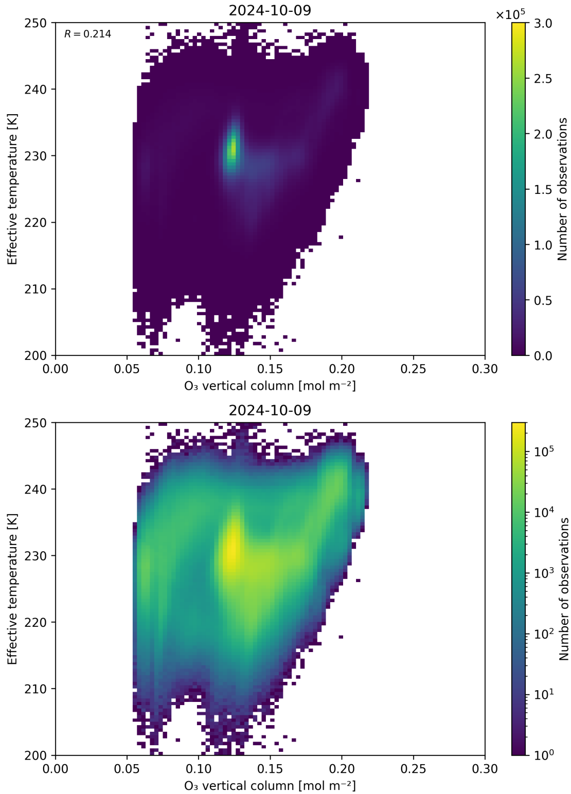
Figure 39: Scatter density plot of “O 3 vertical column” against “Effective temperature” for 2024-10-08 to 2024-10-10.
