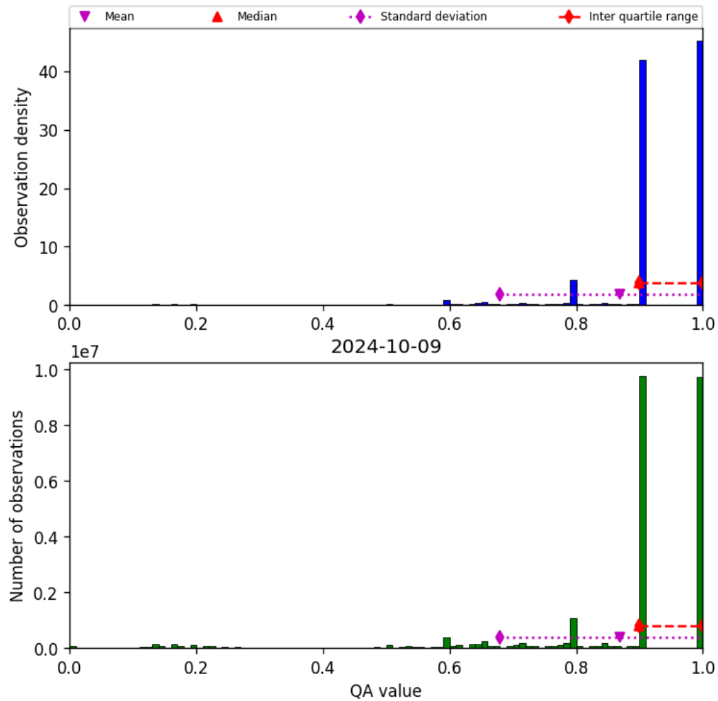
Figure 20: Histogram of “QA value” for 2024-10-08 to 2024-10-10
