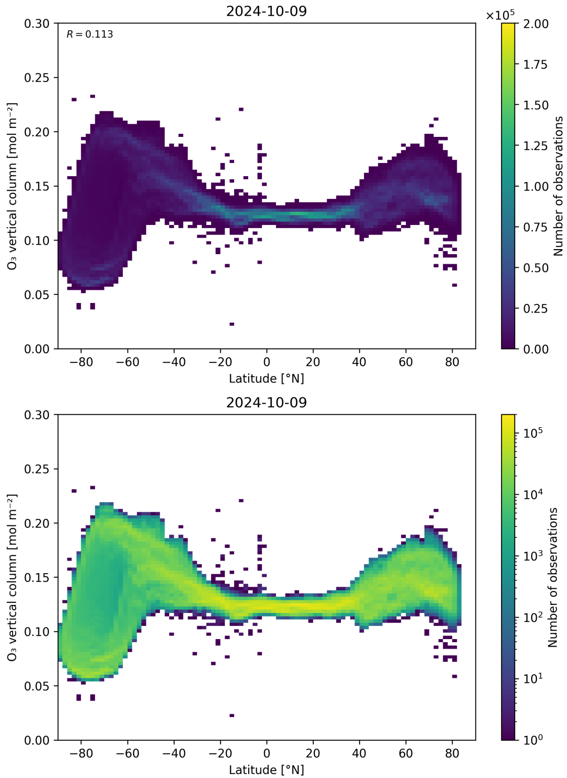
Figure 36: Scatter density plot of “Latitude” against “O 3 vertical column” for 2024-10-08 to 2024-10-10.
