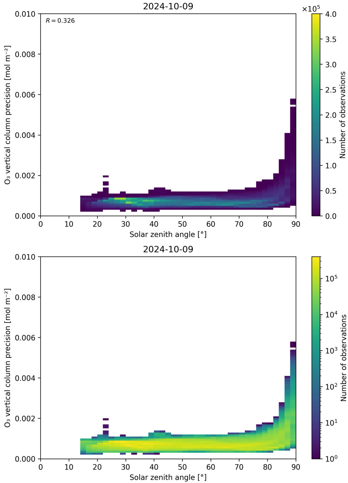
Figure 48: Scatter density plot of “Solar zenith angle” against “O 3 vertical column precision” for 2024-10-08 to 2024-10-10.
