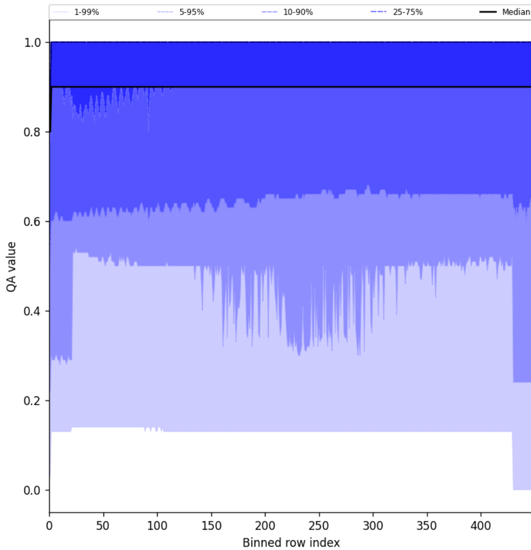
Figure 27: Along track statistics of “QA value” for 2024-10-08 to 2024-10-10
