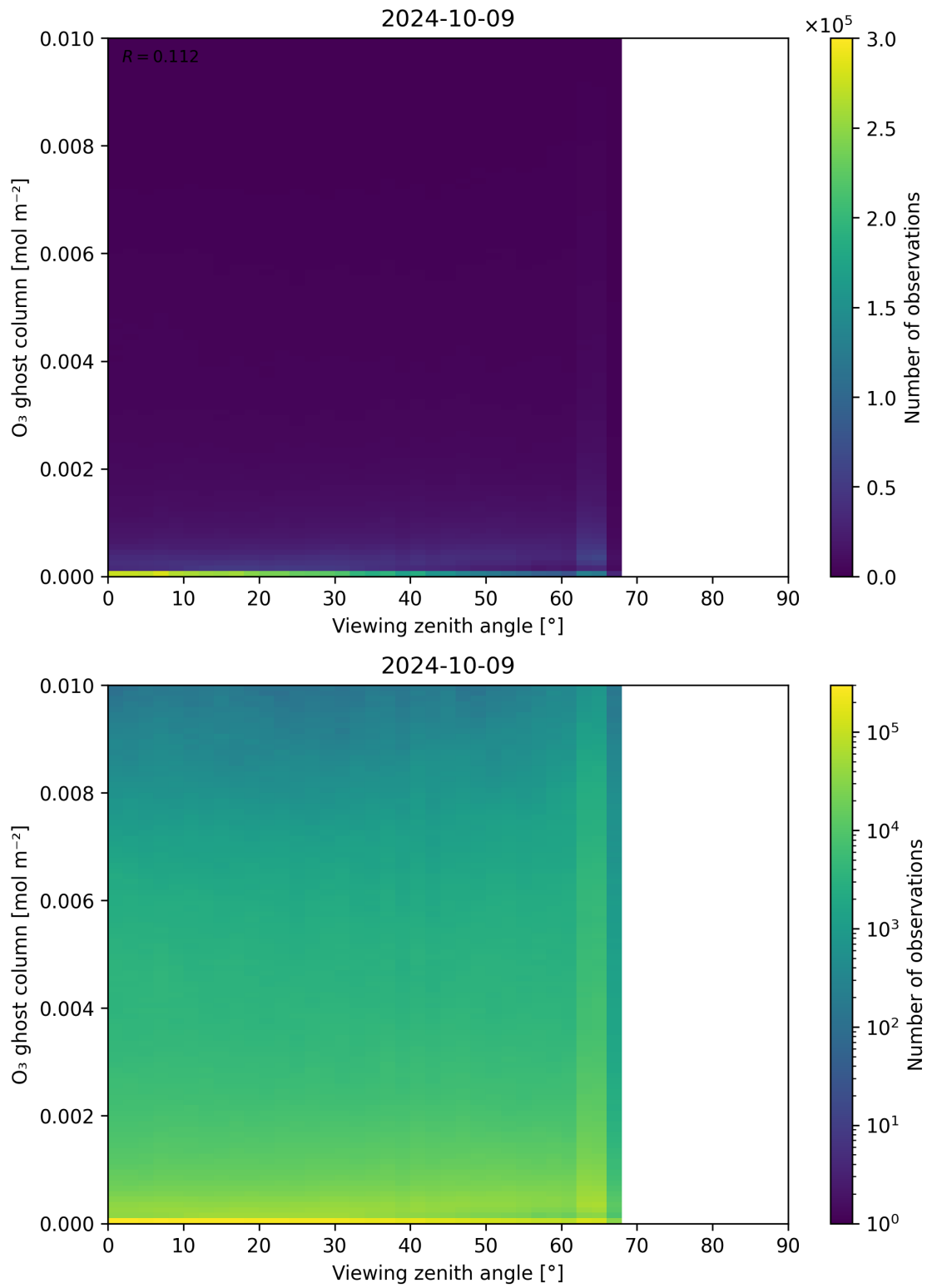
Figure 51: Scatter density plot of “Viewing zenith angle” against “O 3 ghost column” for 2024-10-08 to 2024-10-10.
