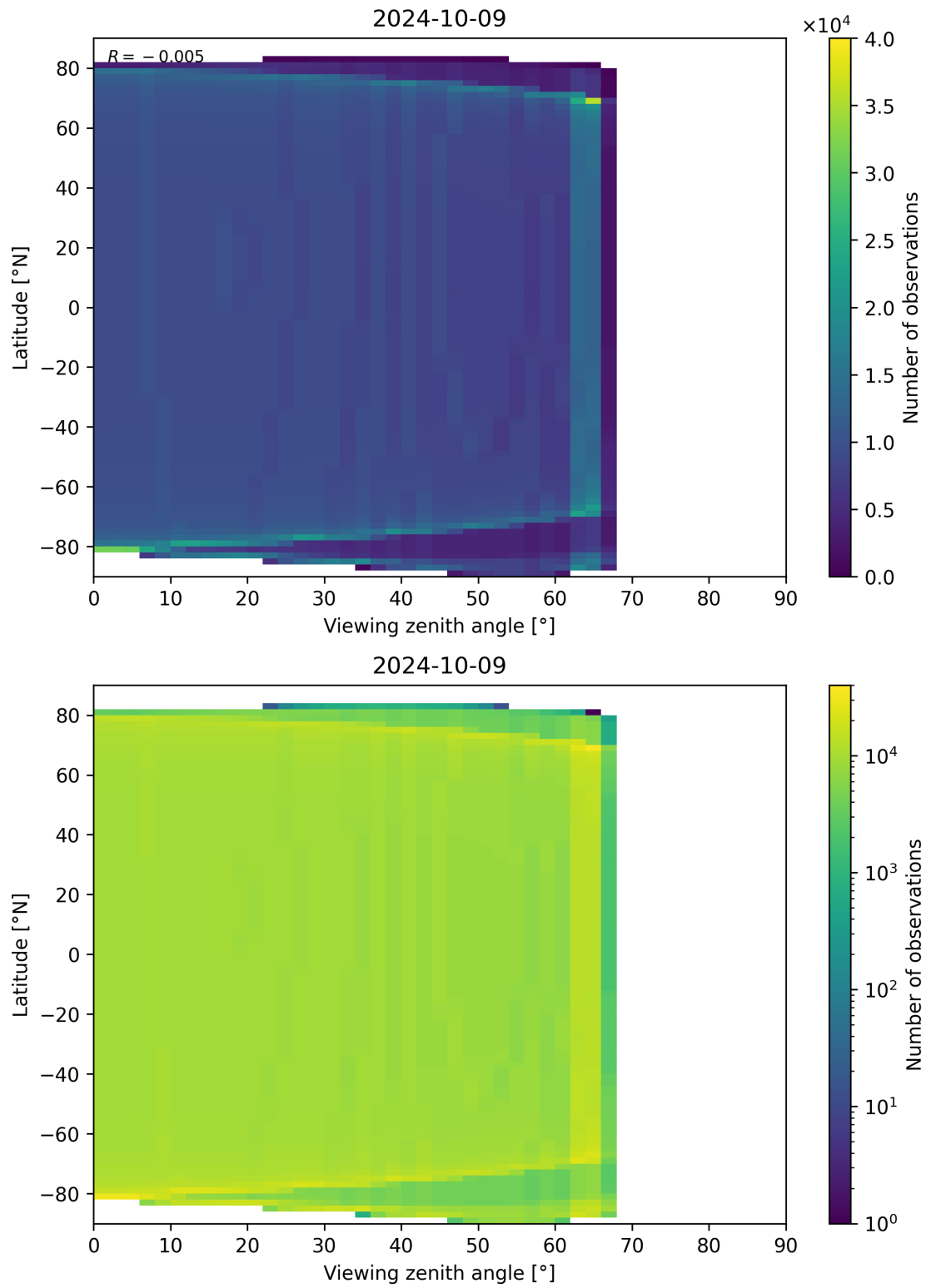
Figure 49: Scatter density plot of “Viewing zenith angle” against “Latitude” for 2024-10-08 to 2024-10-10.
