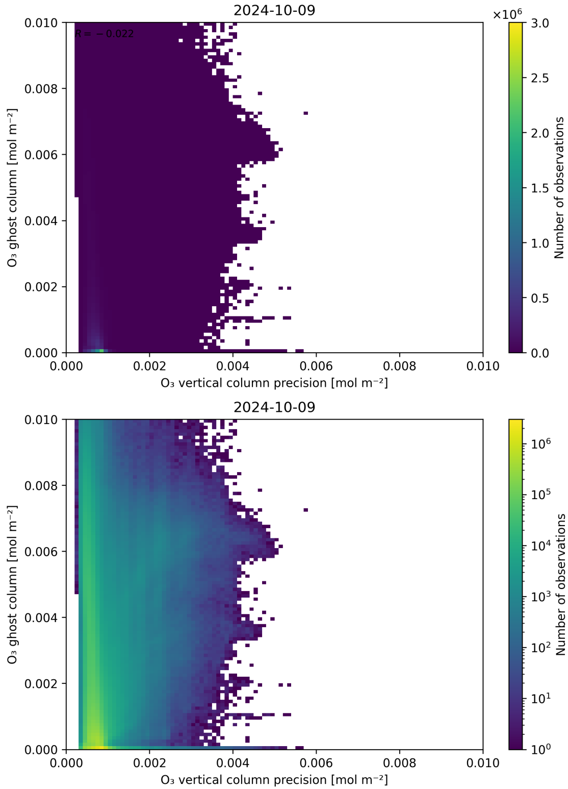
Figure 43: Scatter density plot of “ O_3 vertical column precision” against “ O_3 ghost column” for 2024-10-08 to 2024-10-10.
