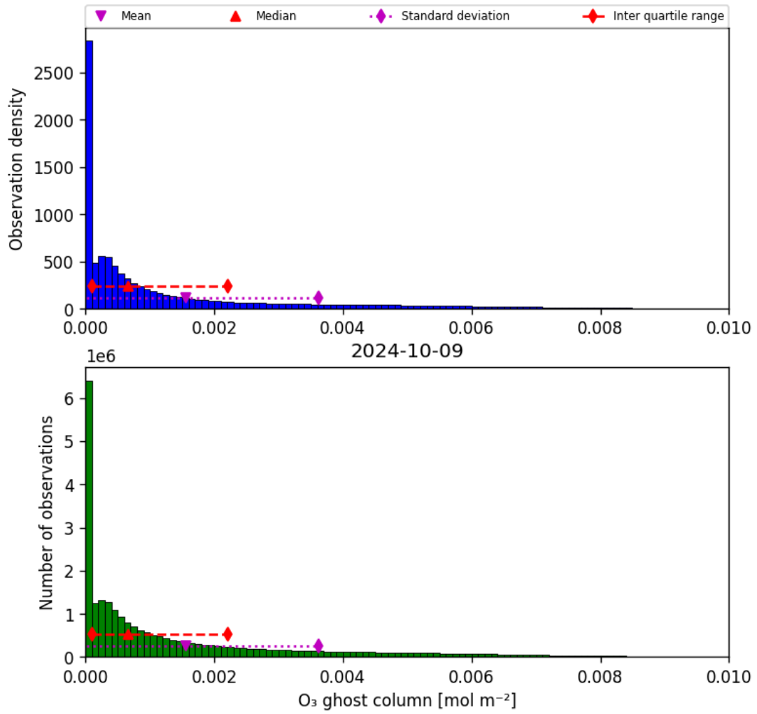
Figure 25: Histogram of “O 3 ghost column” for 2024-10-08 to 2024-10-10
