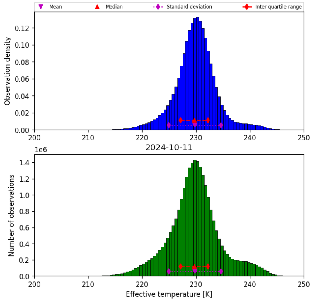
Figure 24: Histogram of “Effective temperature” for 2024-10-10 to 2024-10-12
