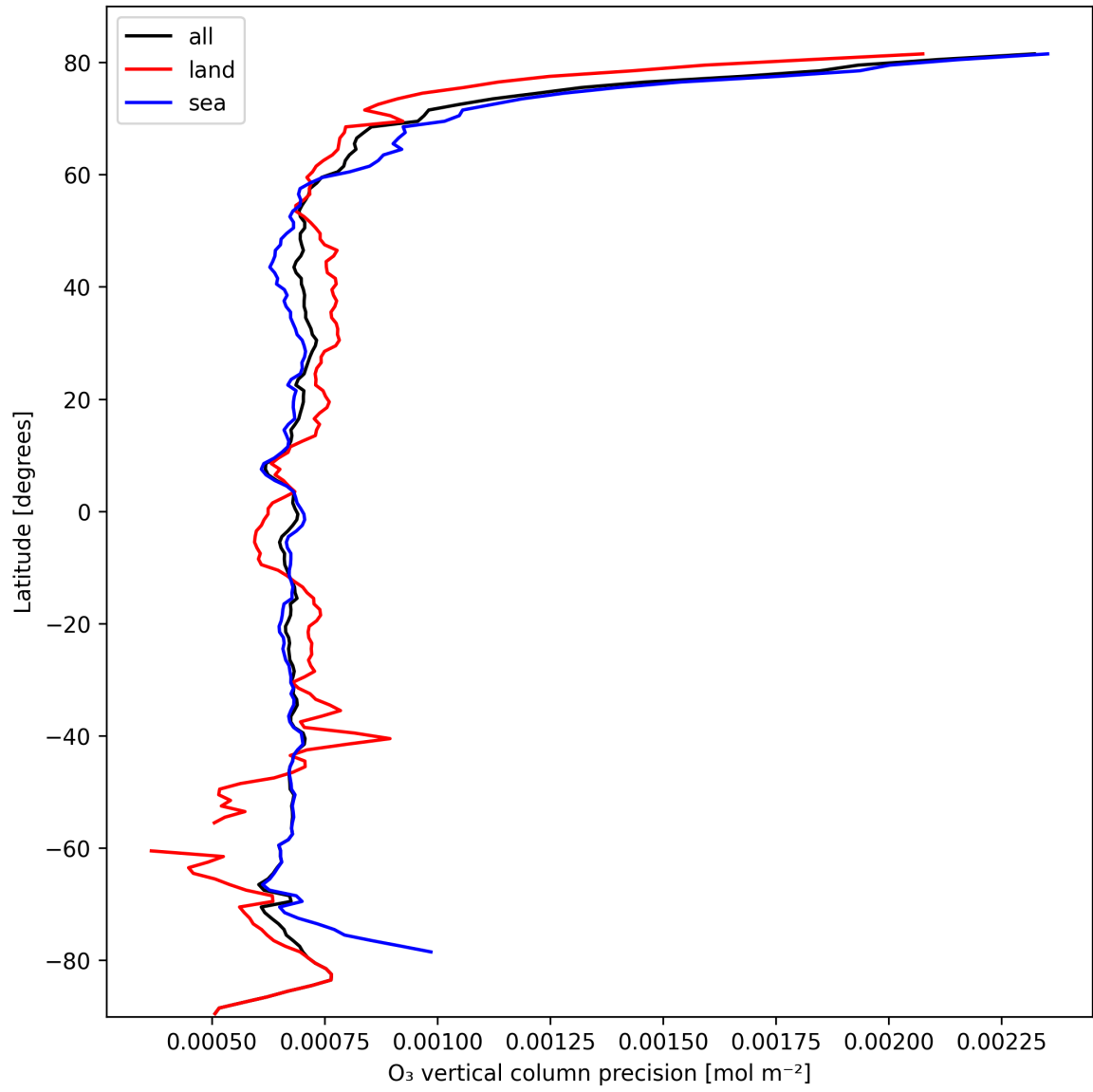
Figure 15: Zonal average of “O 3 vertical column precision” for 2024-10-10 to 2024-10-12.
