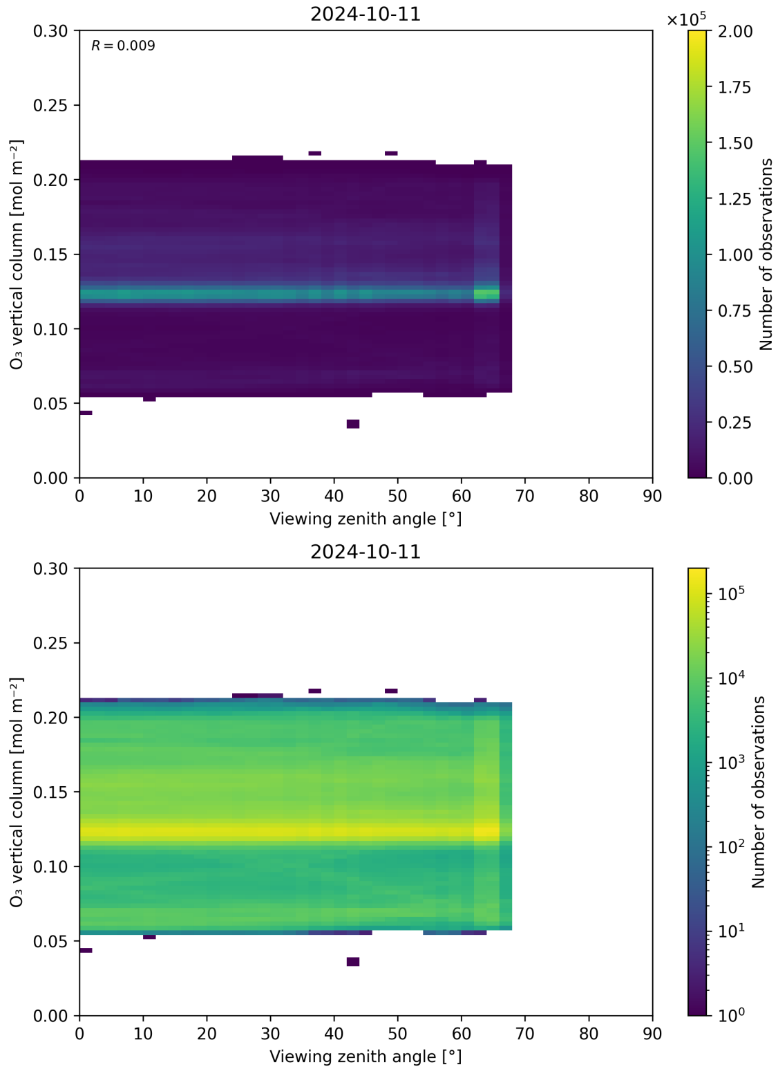
Figure 52: Scatter density plot of “Viewing zenith angle” against “O 3 vertical column” for 2024-10-10 to 2024-10-12.
