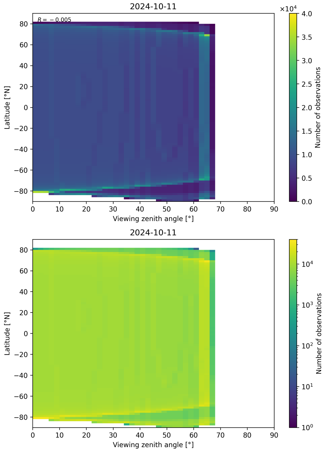
Figure 49: Scatter density plot of “Viewing zenith angle” against “Latitude” for 2024-10-10 to 2024-10-12.
