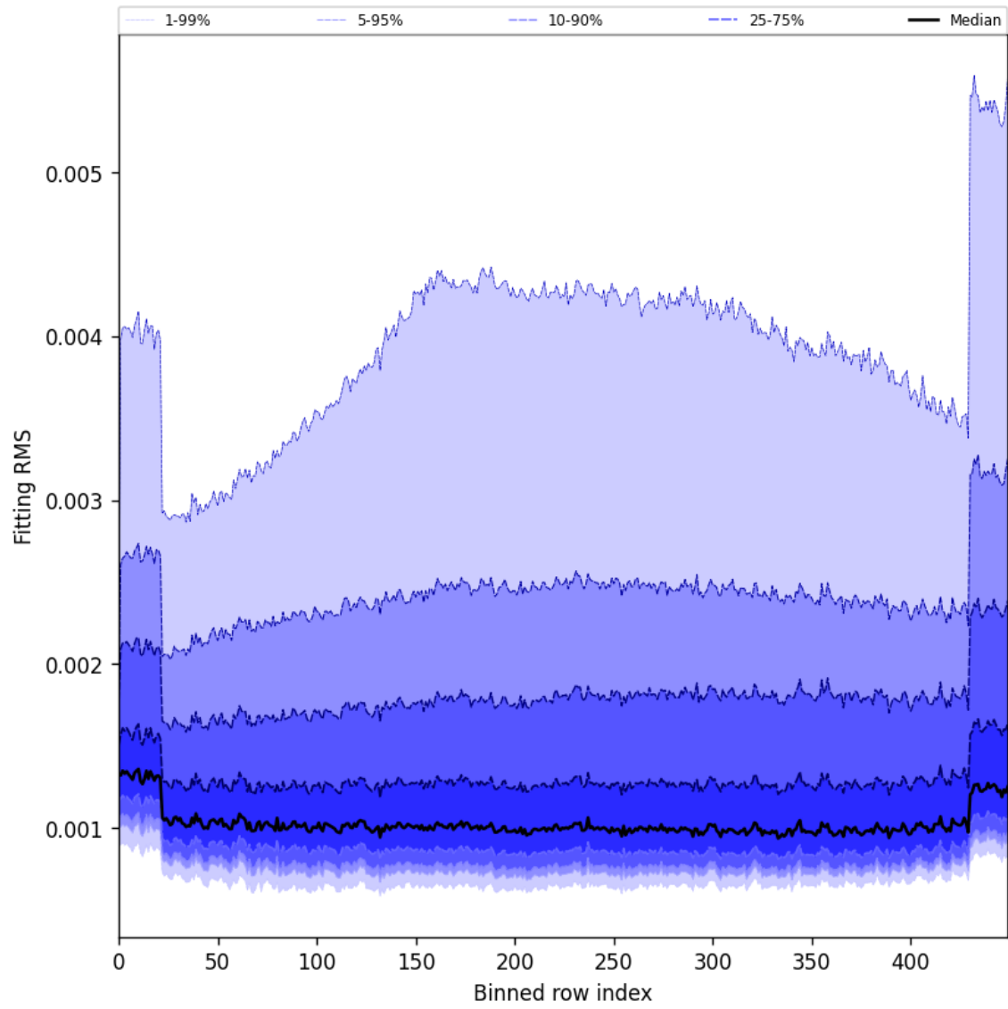
Figure 30: Along track statistics of “Fitting RMS” for 2024-10-10 to 2024-10-12
