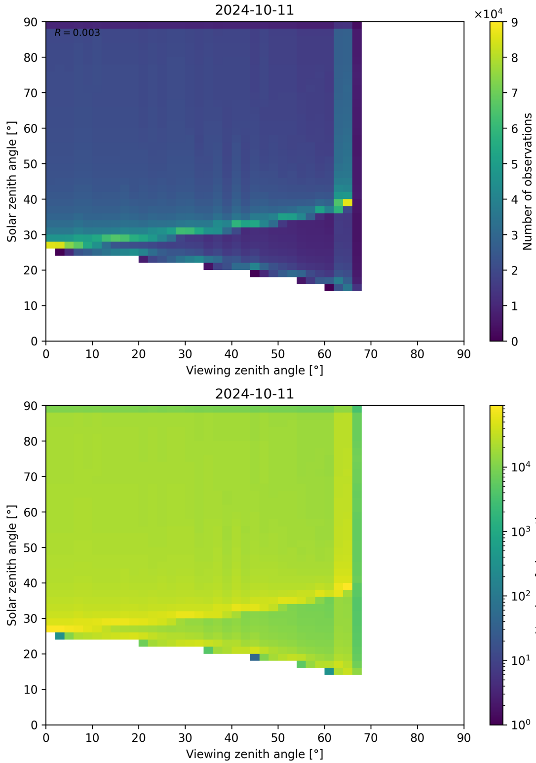
Figure 54: Scatter density plot of “Viewing zenith angle” against “Solar zenith angle” for 2024-10-10 to 2024-10-12.
