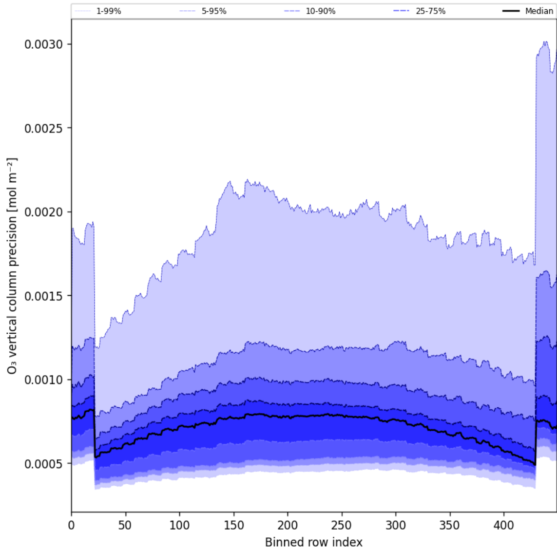
Figure 29: Along track statistics of “O 3 vertical column precision” for 2024-10-10 to 2024-10-12
