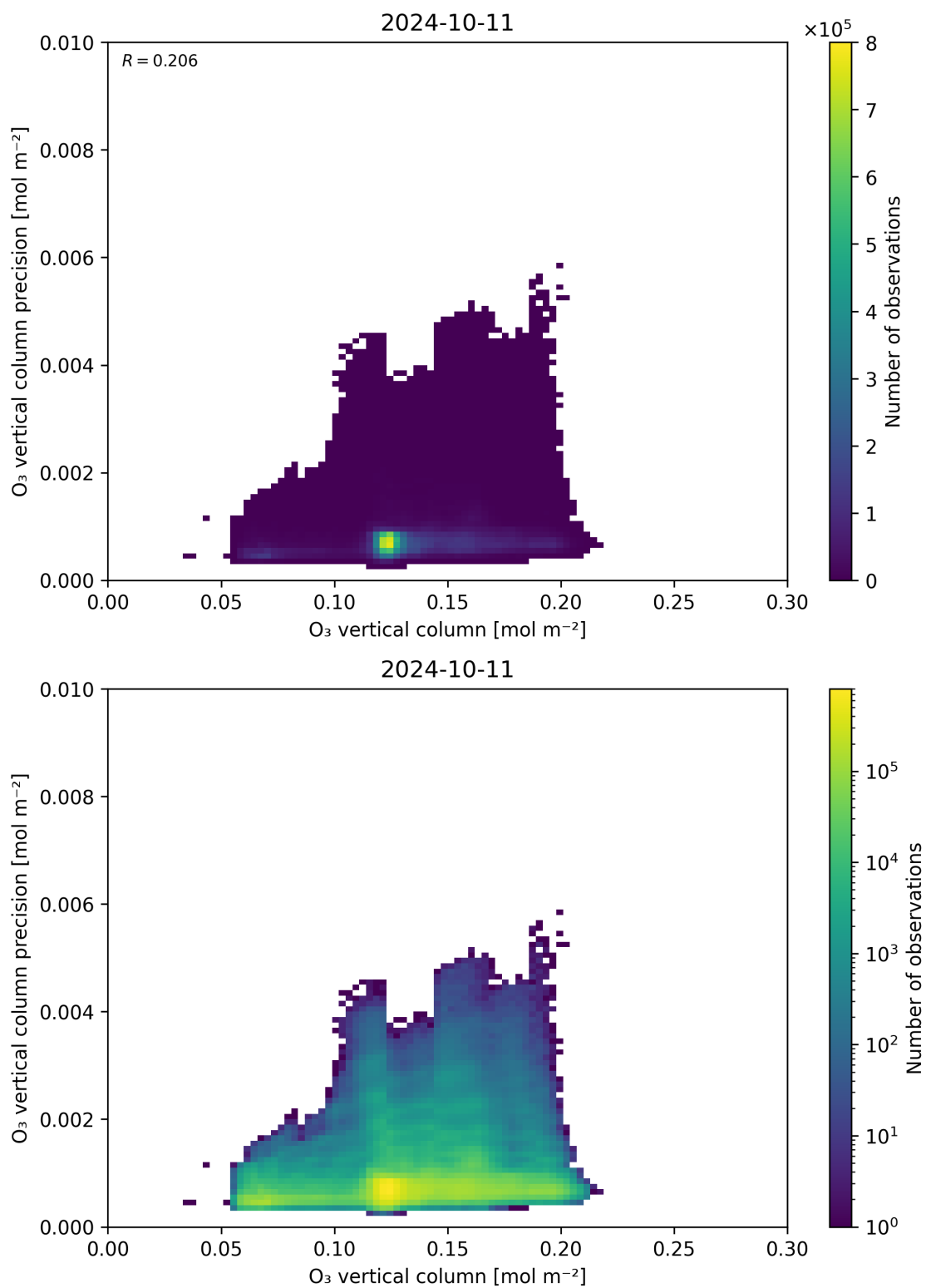
Figure 41: Scatter density plot of “O 3 vertical column” against “O 3 vertical column precision” for 2024-10-10 to 2024-10-12.
