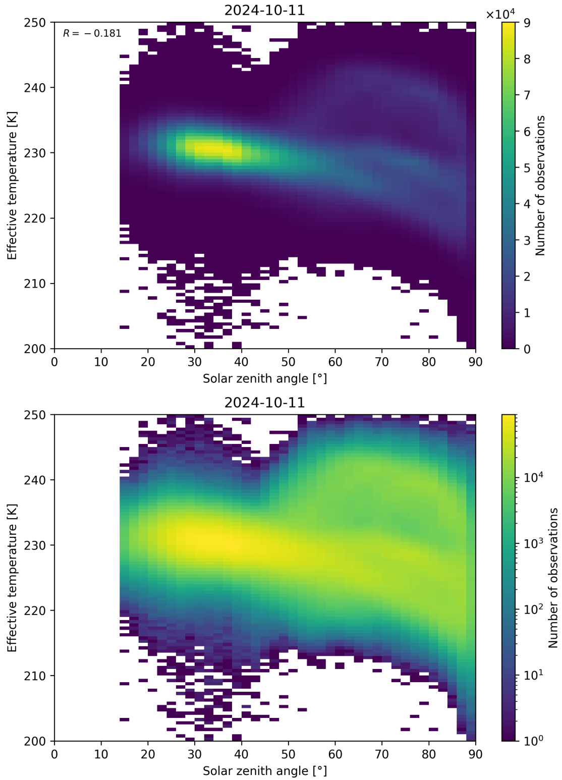
Figure 45: Scatter density plot of “Solar zenith angle” against “Effective temperature” for 2024-10-10 to 2024-10-12.
