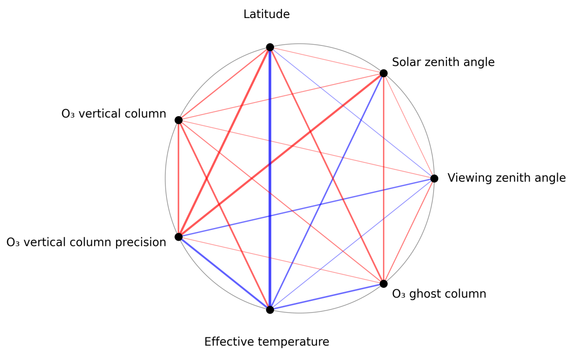
Figure 1: Map of correlation graph for 2024-10-10 to 2024-10-12.
