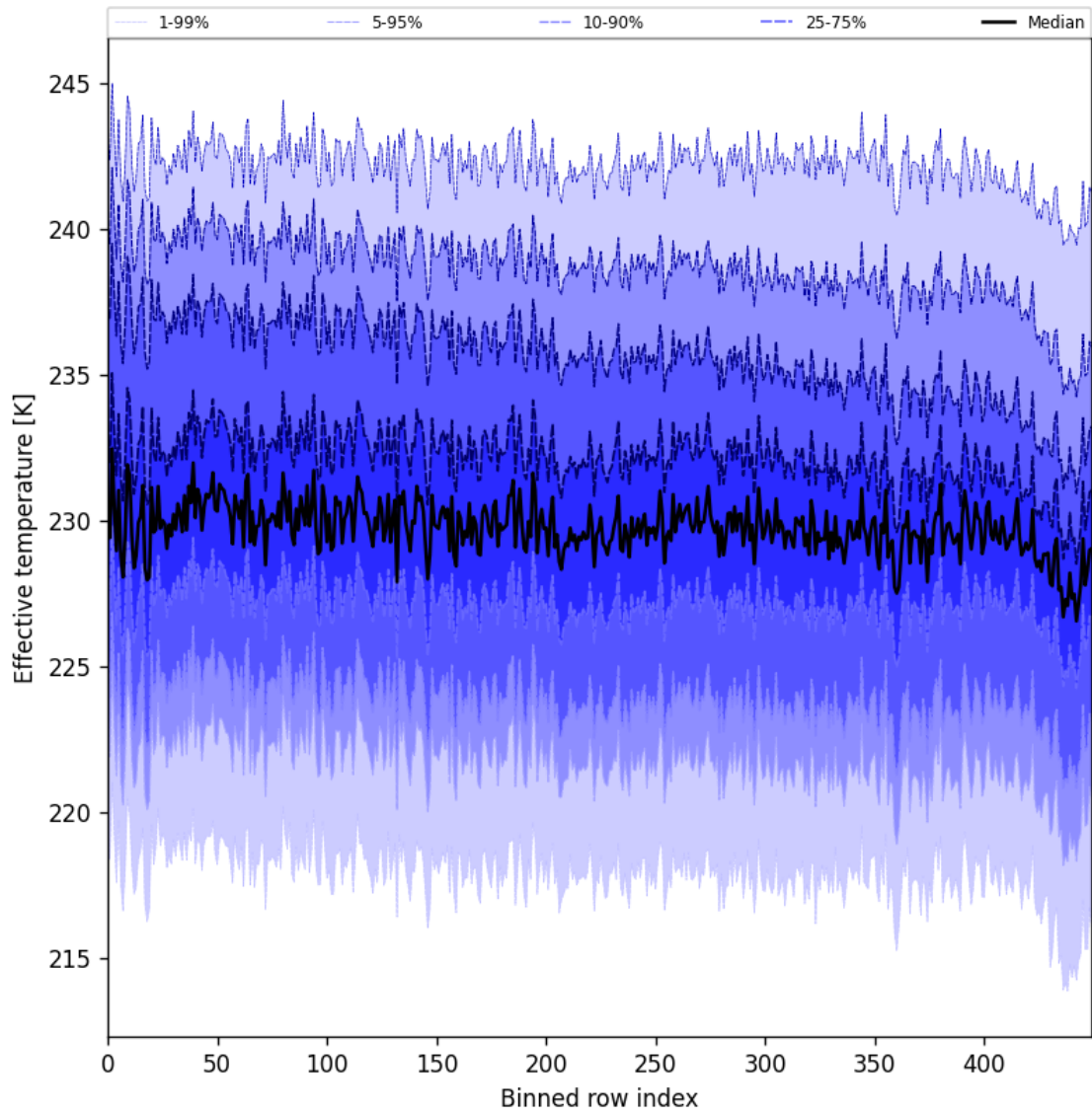
Figure 31: Along track statistics of “Effective temperature” for 2024-10-10 to 2024-10-12
