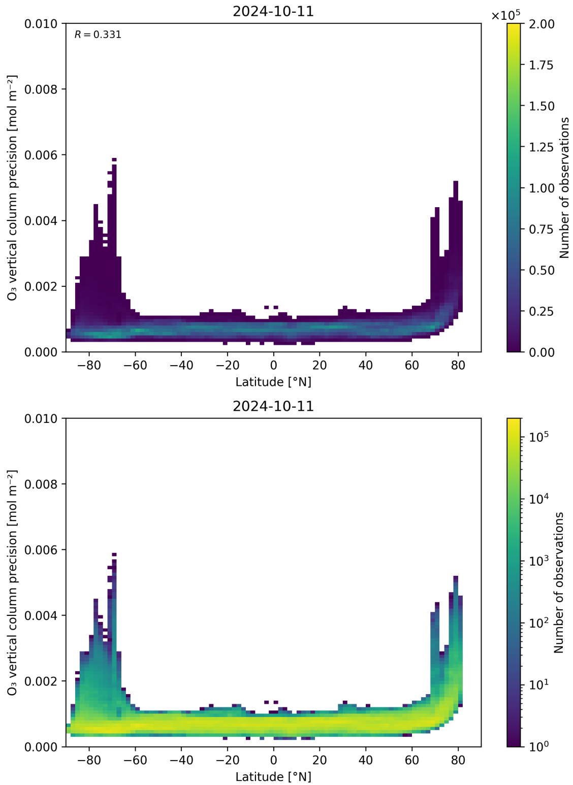
Figure 37: Scatter density plot of “Latitude” against “O 3 vertical column precision” for 2024-10-10 to 2024-10-12.
