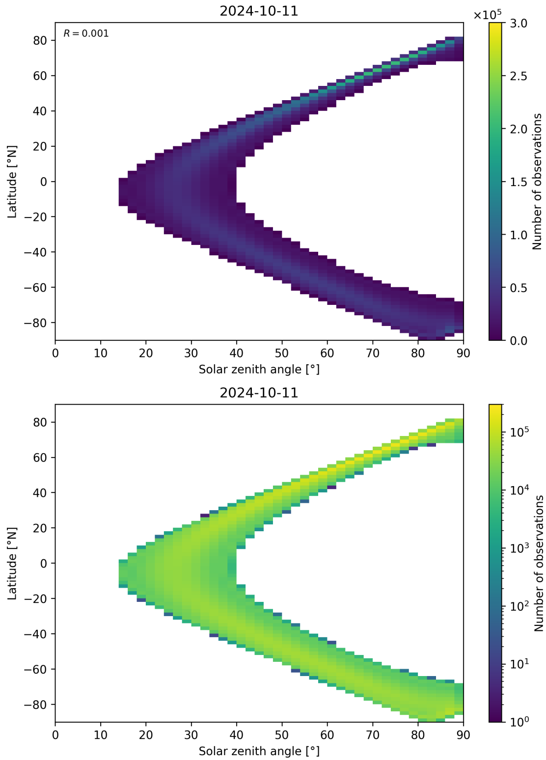
Figure 44: Scatter density plot of “Solar zenith angle” against “Latitude” for 2024-10-10 to 2024-10-12.
