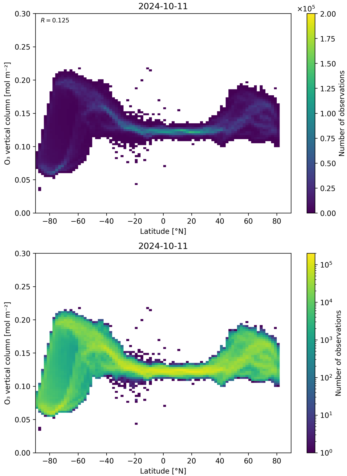
Figure 36: Scatter density plot of “Latitude” against “O 3 vertical column” for 2024-10-10 to 2024-10-12.
