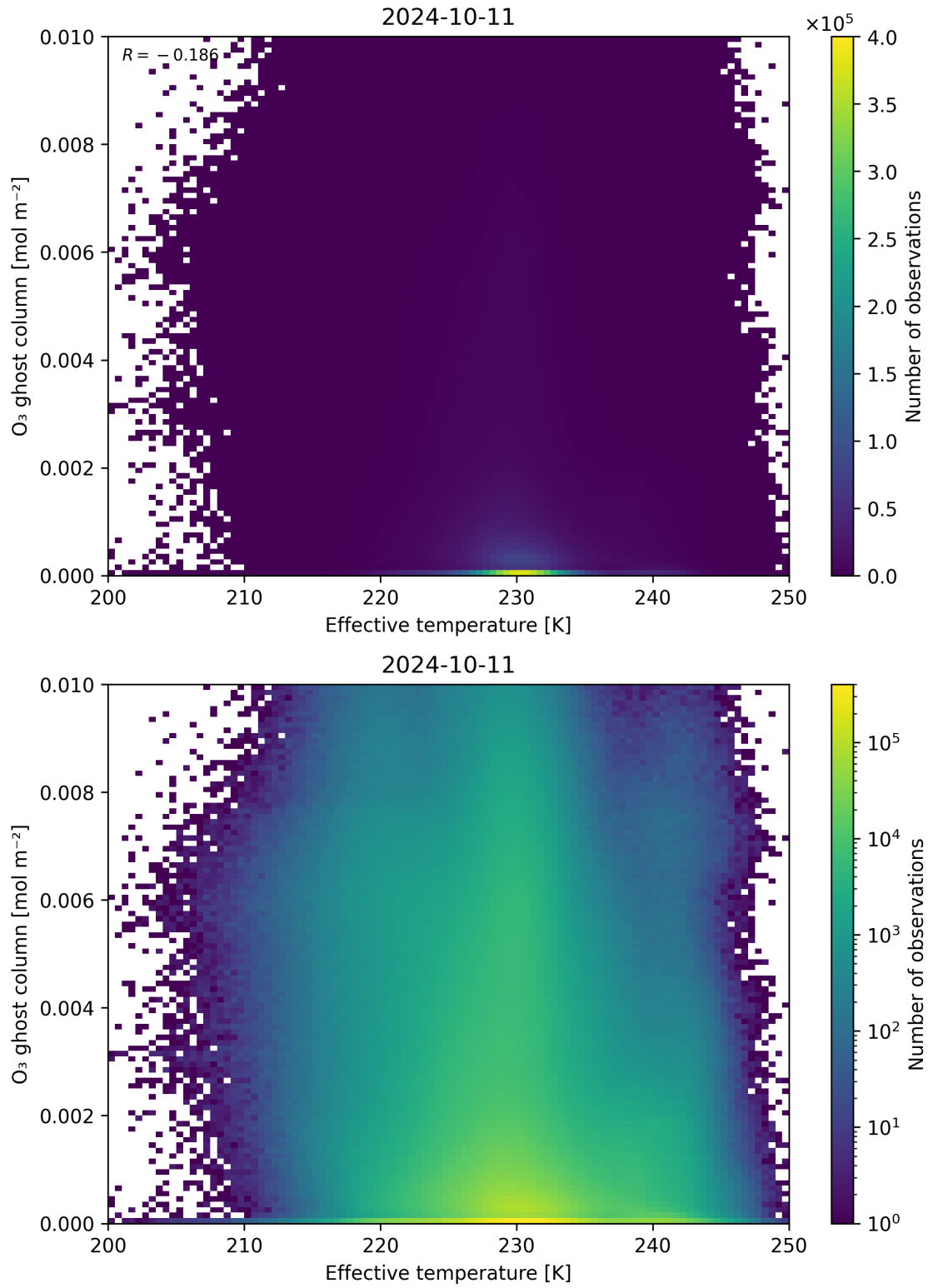
Figure 38: Scatter density plot of “Effective temperature” against “O 3 ghost column” for 2024-10-10 to 2024-10-12.
