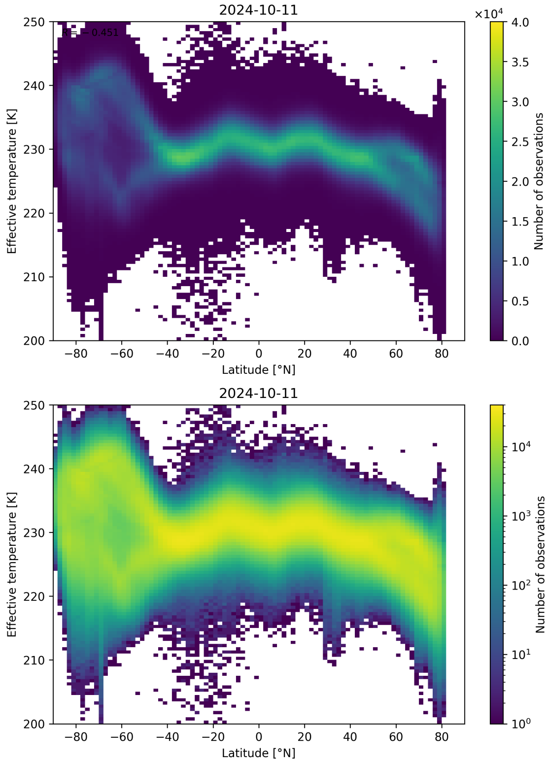
Figure 34: Scatter density plot of “Latitude” against “Effective temperature” for 2024-10-10 to 2024-10-12.
