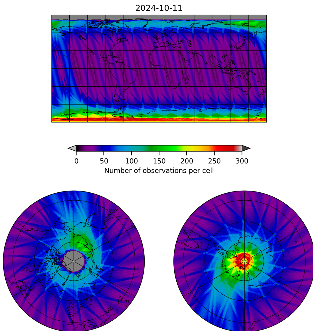
Figure 12: Map of the number of observations for 2024-10-10 to 2024-10-12
