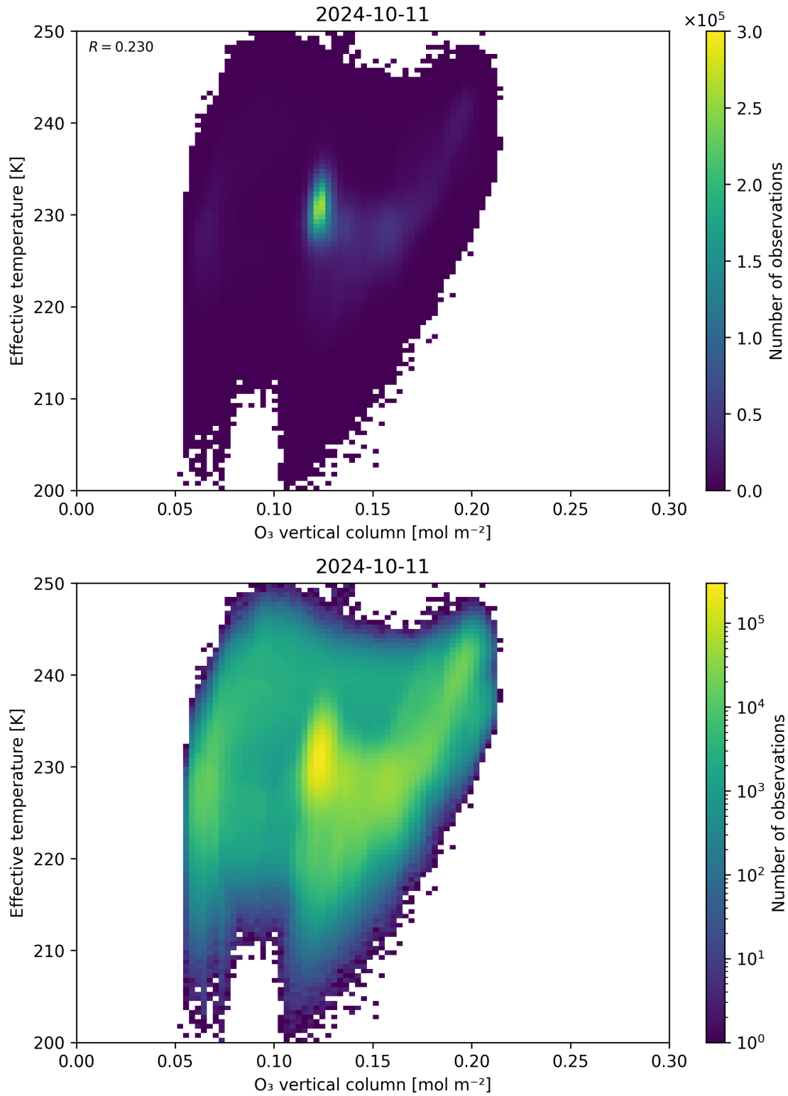
Figure 39: Scatter density plot of “O 3 vertical column” against “Effective temperature” for 2024-10-10 to 2024-10-12.
