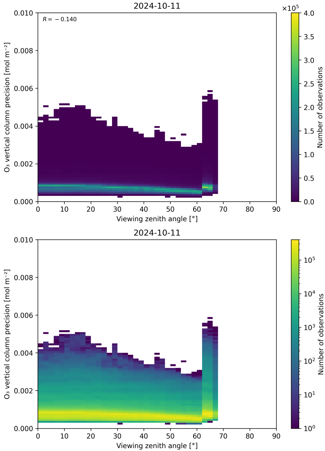
Figure 53: Scatter density plot of “Viewing zenith angle” against “O 3 vertical column precision” for 2024-10-10 to 2024-10-12.
