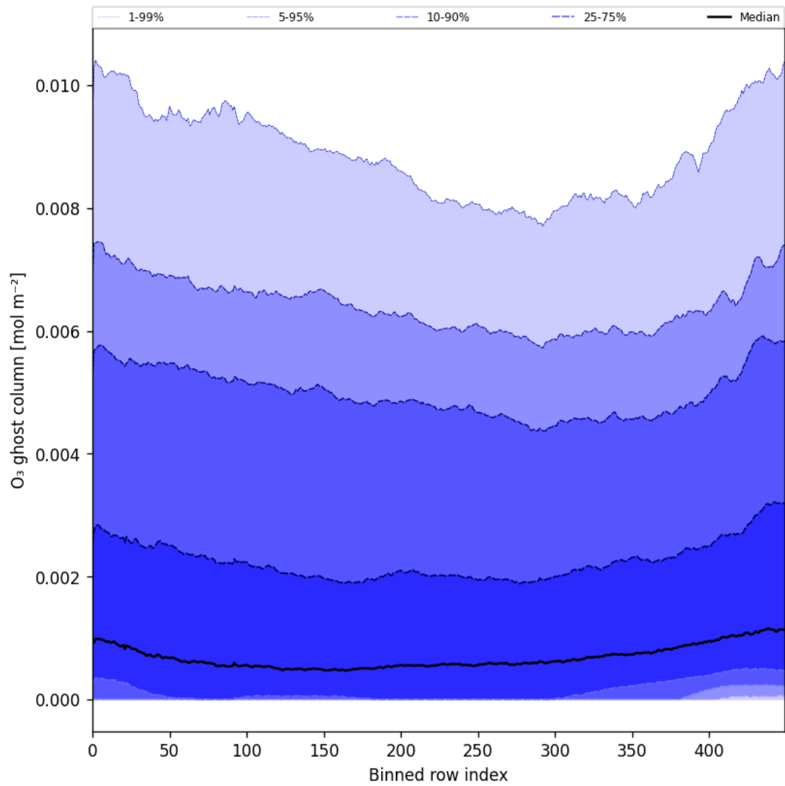
Figure 32: Along track statistics of “O 3 ghost column” for 2024-10-10 to 2024-10-12
