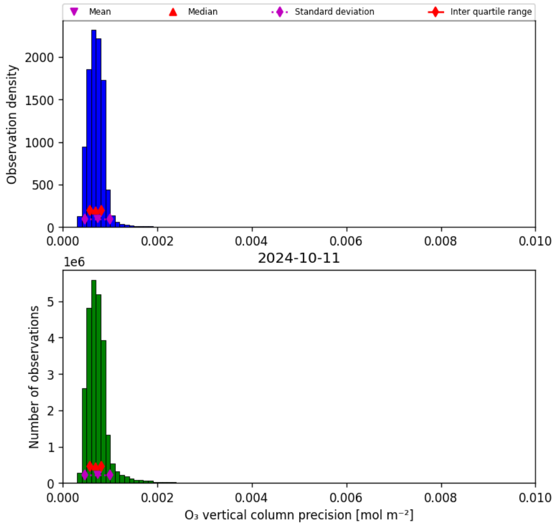
Figure 22: Histogram of “O 3 vertical column precision” for 2024-10-10 to 2024-10-12
