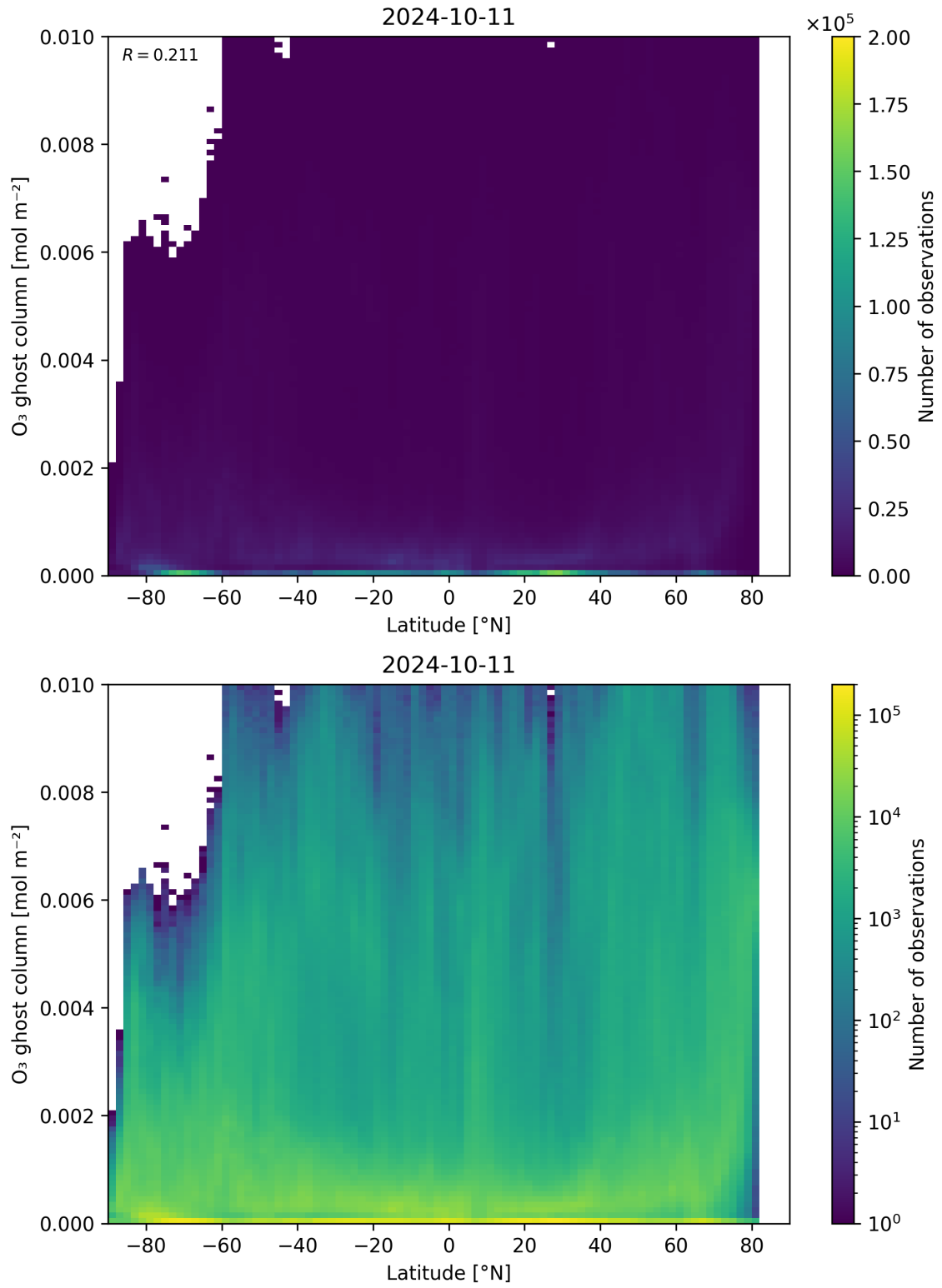
Figure 35: Scatter density plot of “Latitude” against “O 3 ghost column” for 2024-10-10 to 2024-10-12.
