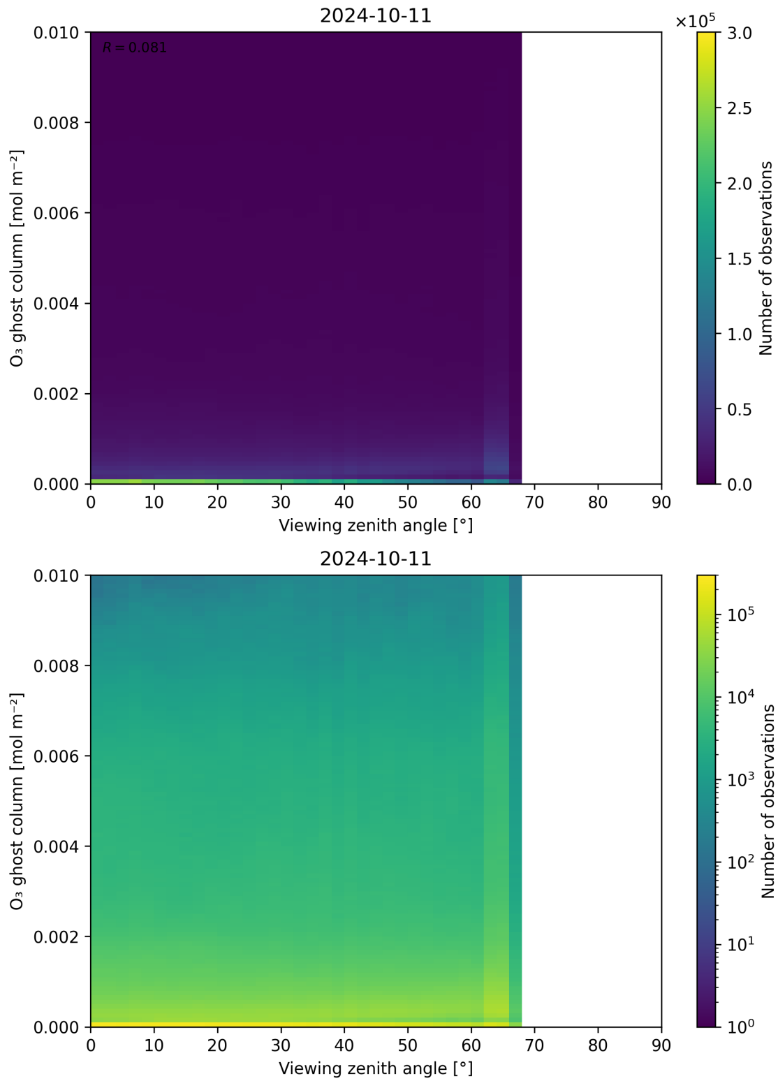
Figure 51: Scatter density plot of “Viewing zenith angle” against “O 3 ghost column” for 2024-10-10 to 2024-10-12.
