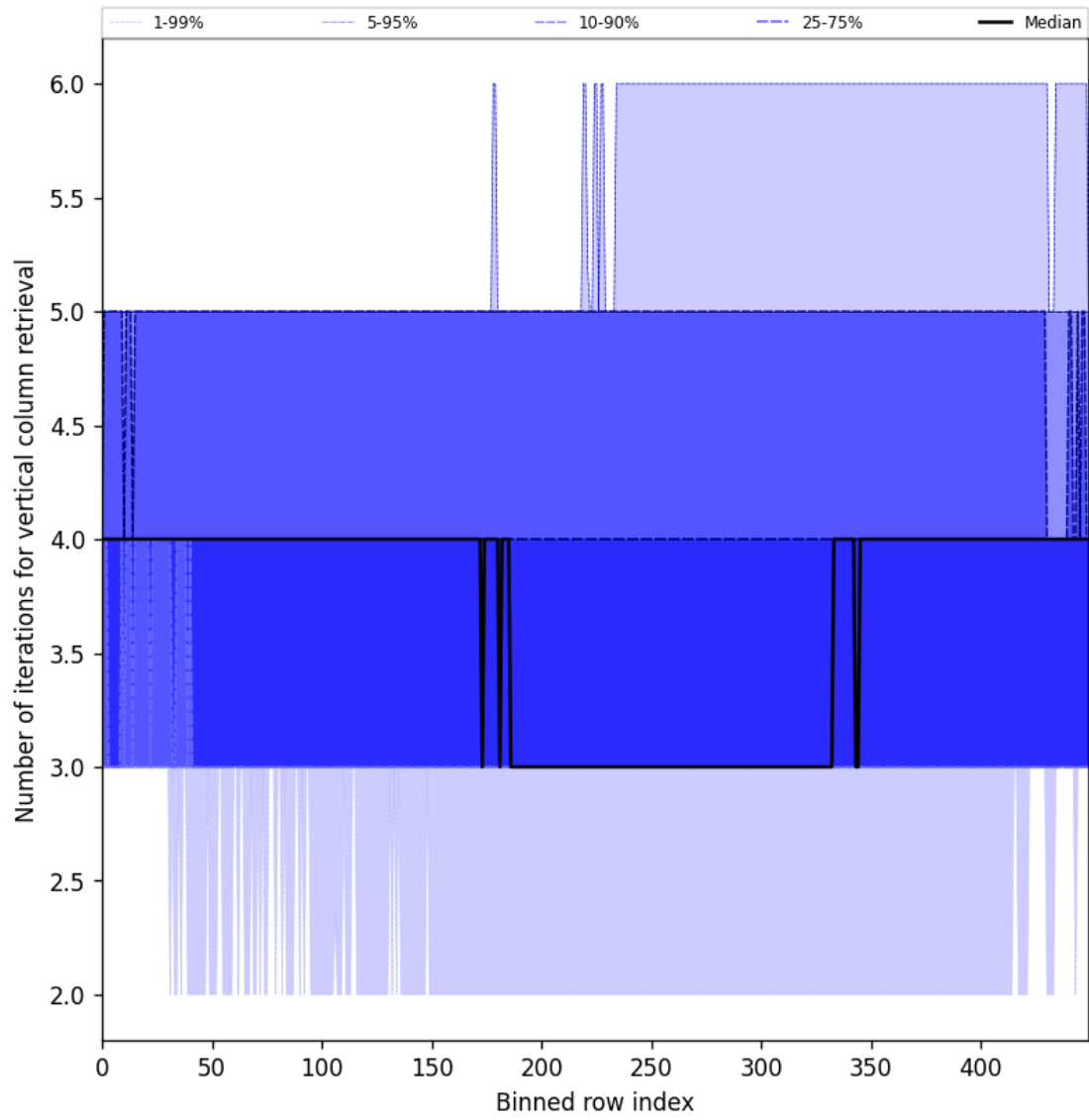
Figure 33: Along track statistics of “Number of iterations for vertical column retrieval” for 2024-10-10 to 2024-10-12
