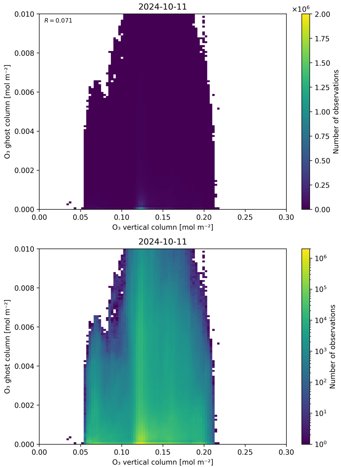
Figure 40: Scatter density plot of “O 3 vertical column” against “O 3 ghost column” for 2024-10-10 to 2024-10-12.
