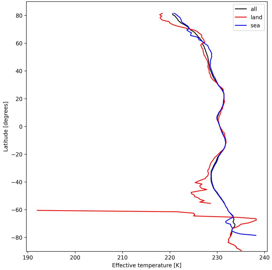
Figure 17: Zonal average of “Effective temperature” for 2024-10-10 to 2024-10-12.
