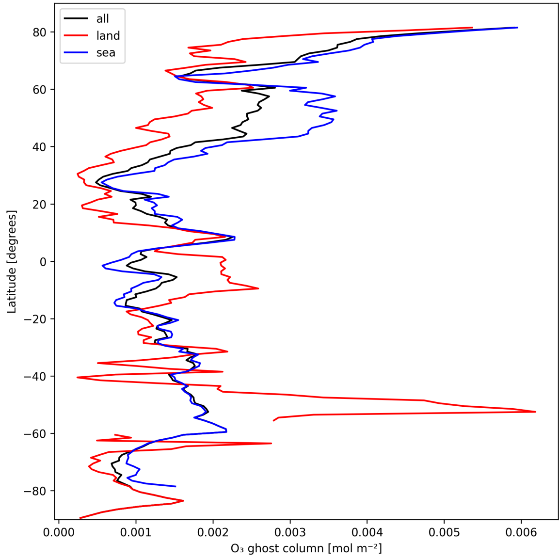
Figure 18: Zonal average of “O 3 ghost column” for 2024-10-10 to 2024-10-12.
