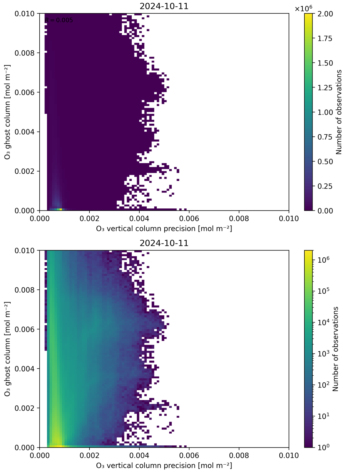
Figure 43: Scatter density plot of “O 3 vertical column precision” against “O 3 ghost column” for 2024-10-10 to 2024-10-12.
