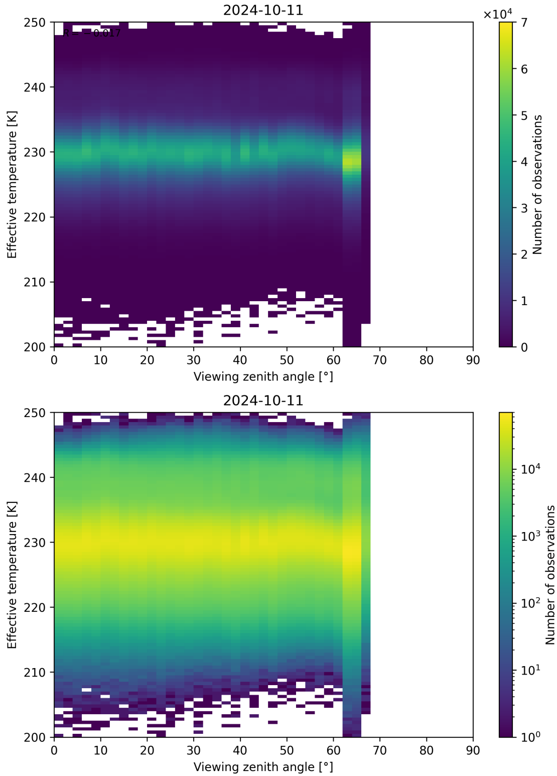
Figure 50: Scatter density plot of “Viewing zenith angle” against “Effective temperature” for 2024-10-10 to 2024-10-12.
