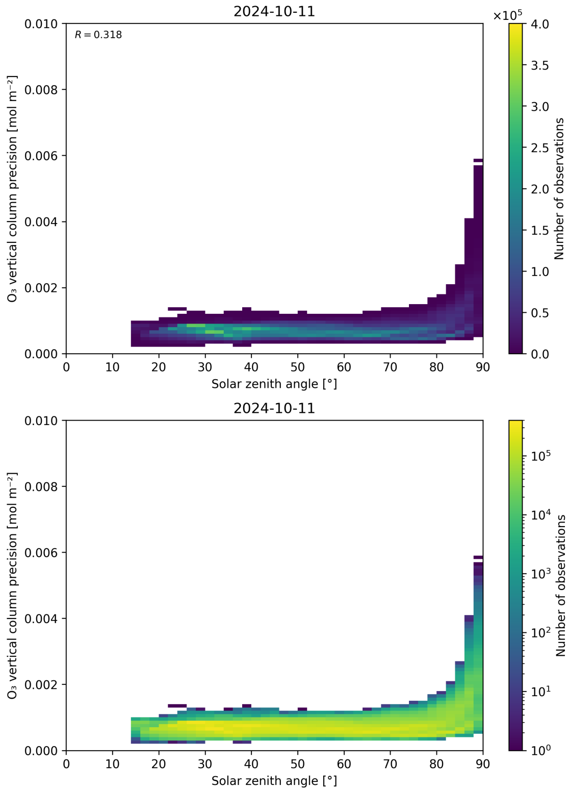
Figure 48: Scatter density plot of “Solar zenith angle” against “O 3 vertical column precision” for 2024-10-10 to 2024-10-12.
