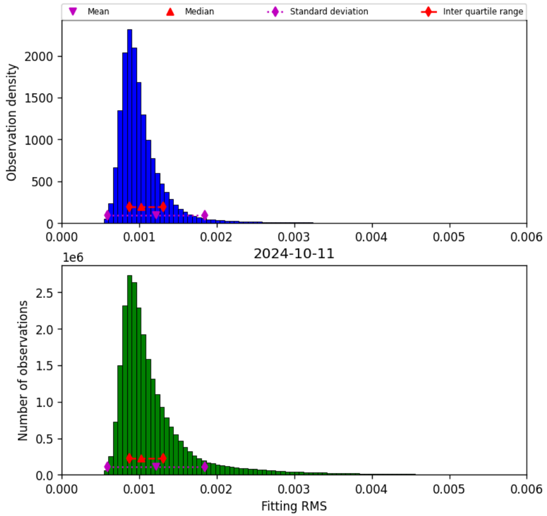
Figure 23: Histogram of “Fitting RMS” for 2024-10-10 to 2024-10-12
