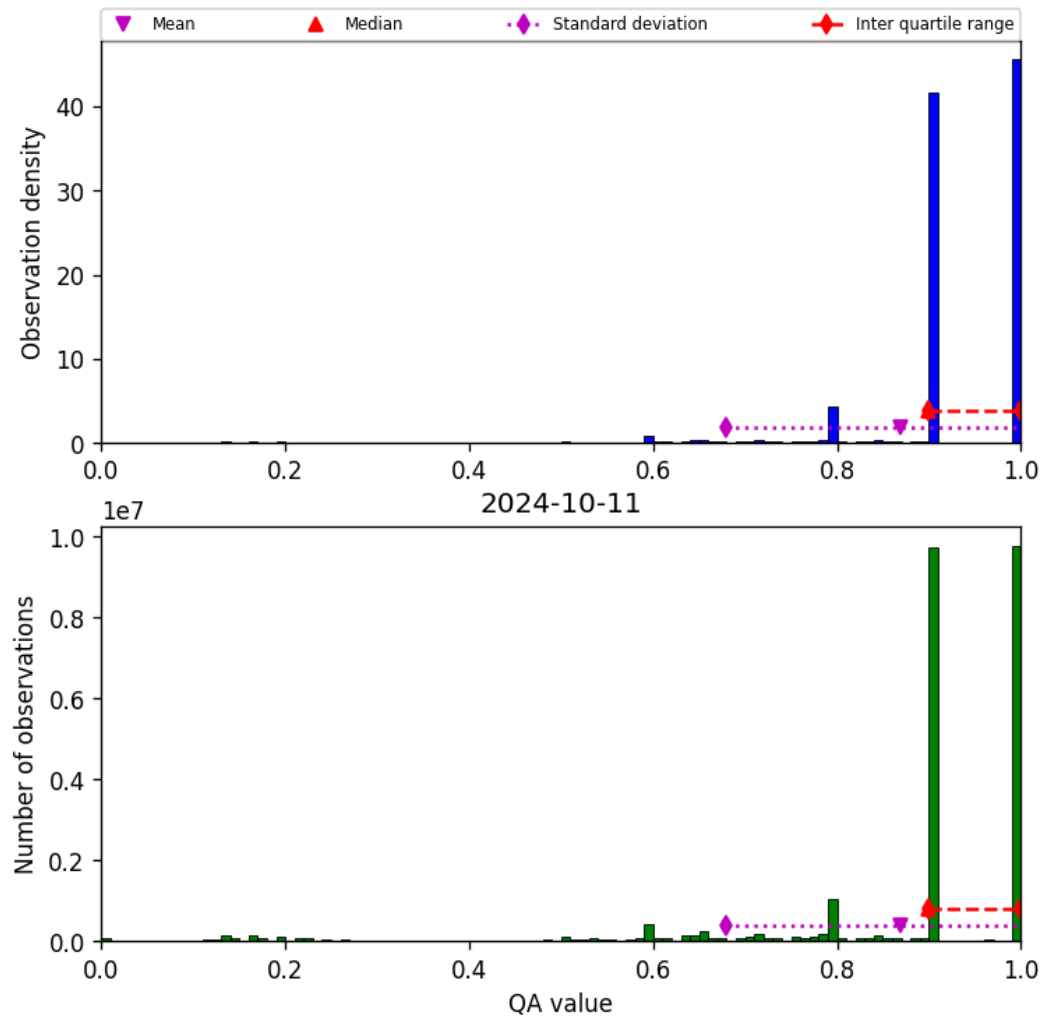
Figure 20: Histogram of “QA value” for 2024-10-10 to 2024-10-12
