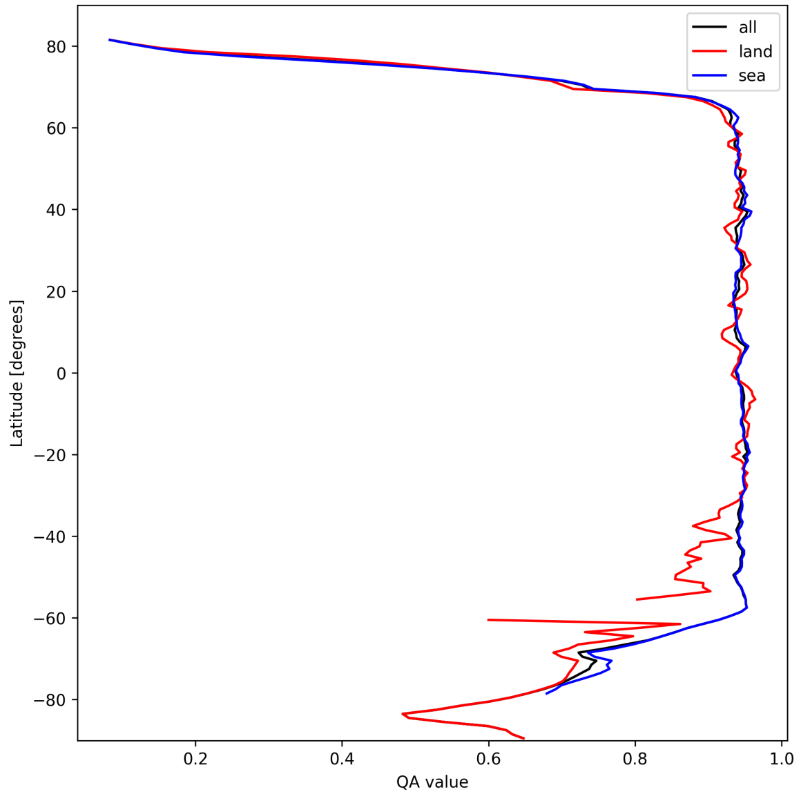
Figure 13: Zonal average of “QA value” for 2024-10-10 to 2024-10-12.
