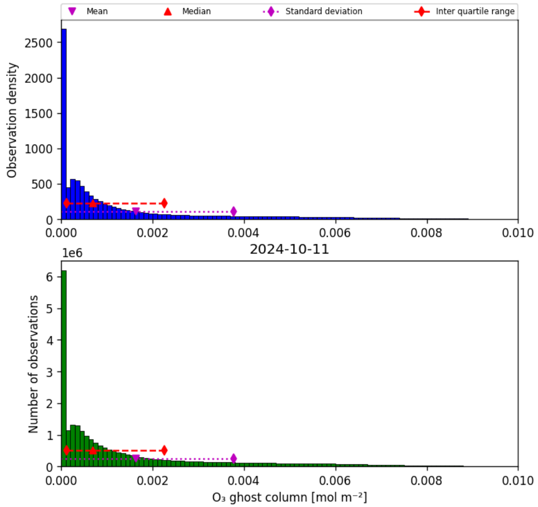
Figure 25: Histogram of “O 3 ghost column” for 2024-10-10 to 2024-10-12
