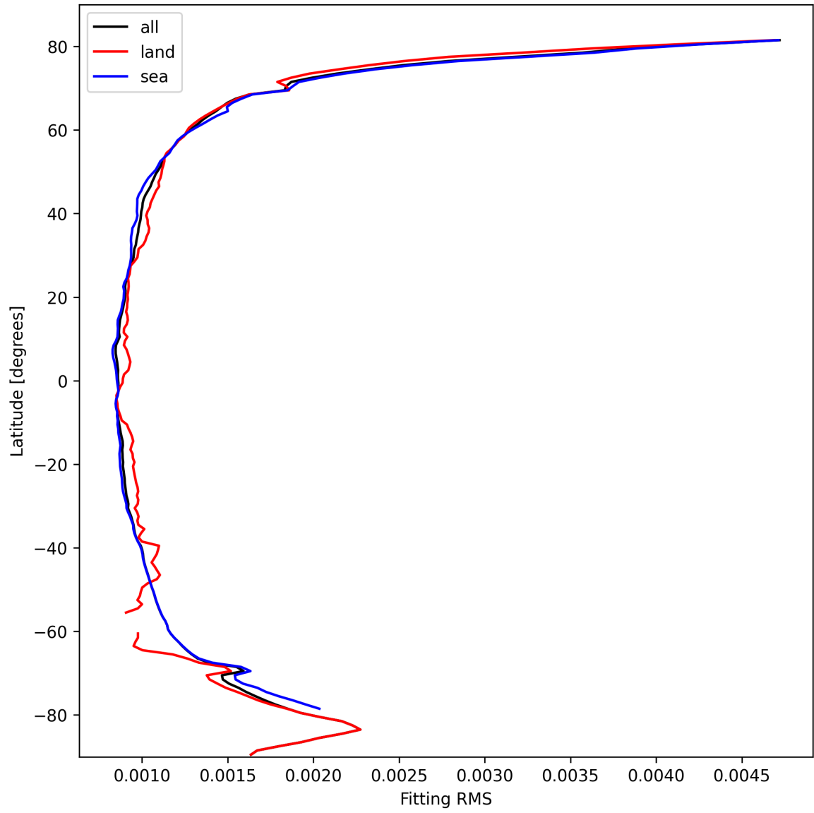
Figure 16: Zonal average of “Fitting RMS” for 2024-10-10 to 2024-10-12.
