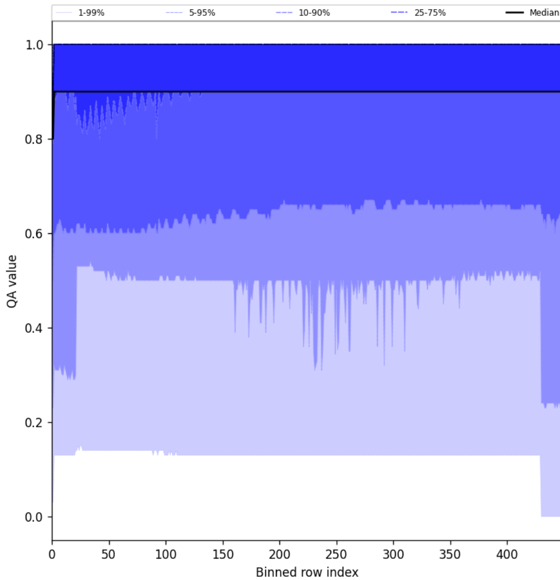
Figure 27: Along track statistics of “QA value” for 2024-10-10 to 2024-10-12
