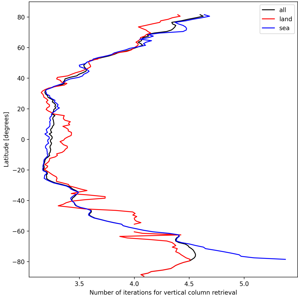
Figure 19: Zonal average of “Number of iterations for vertical column retrieval” for 2024-10-10 to 2024-10-12.
