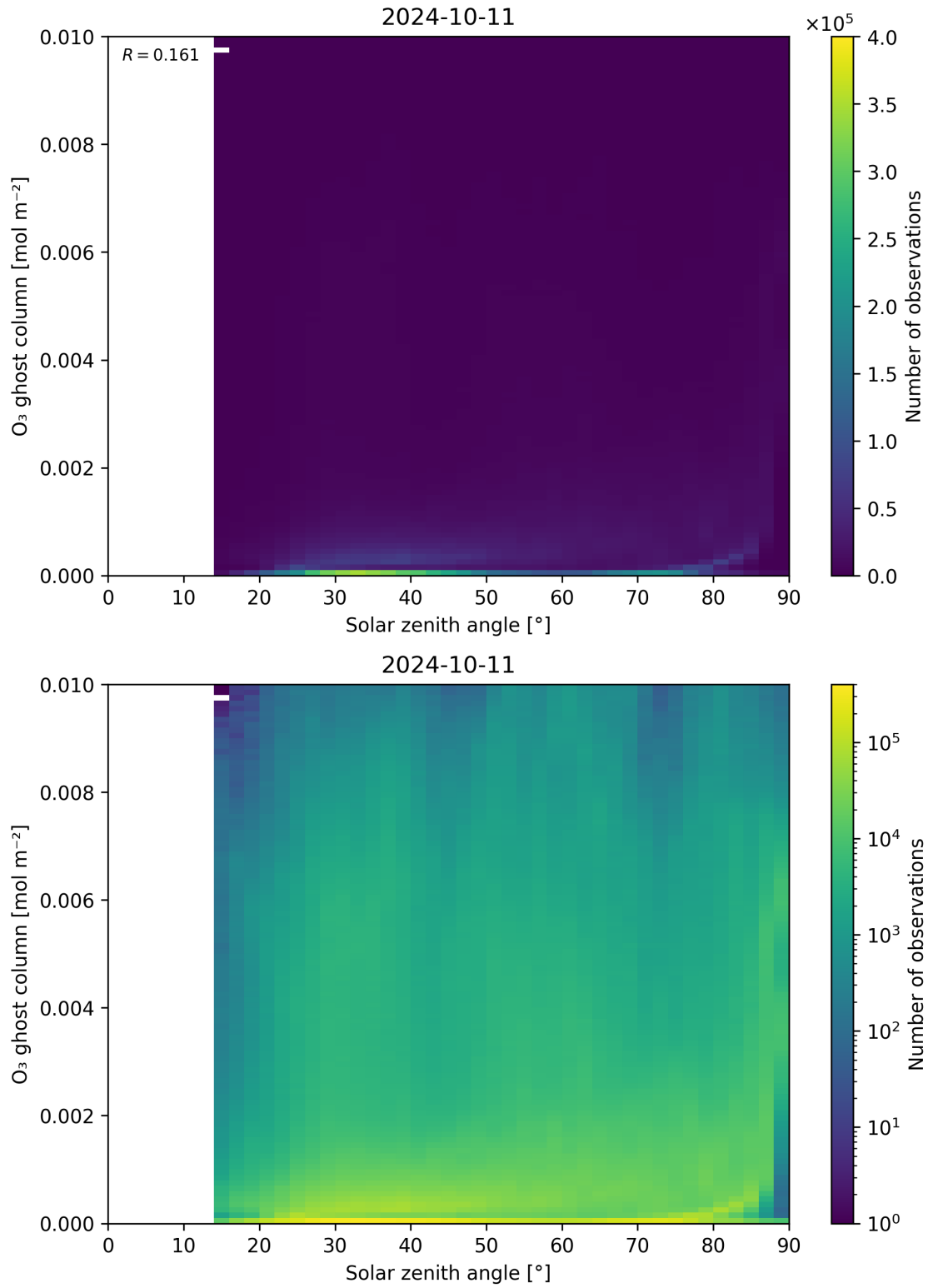
Figure 46: Scatter density plot of “Solar zenith angle” against “O 3 ghost column” for 2024-10-10 to 2024-10-12.
