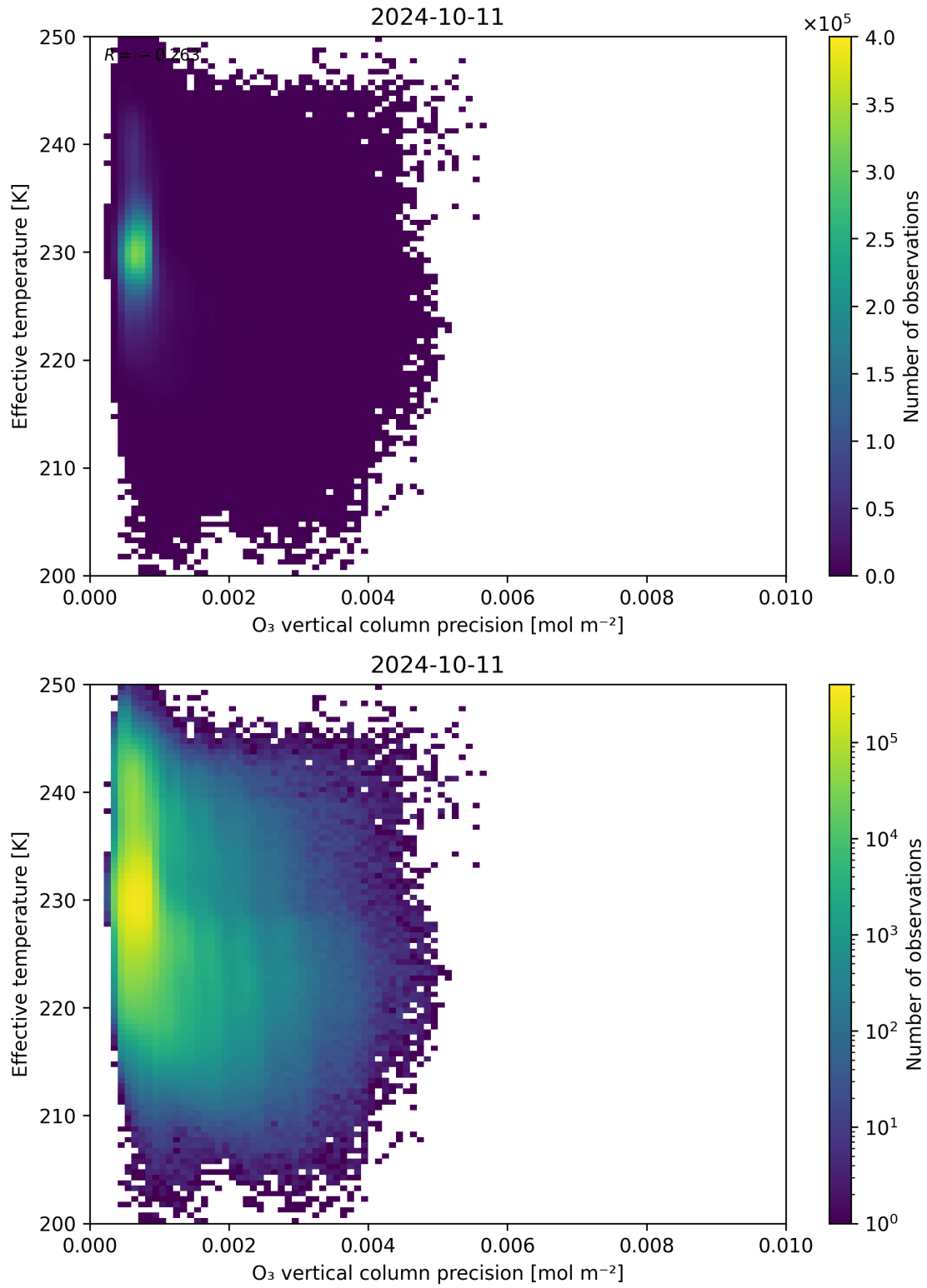
Figure 42: Scatter density plot of “O 3 vertical column precision” against “Effective temperature” for 2024-10-10 to 2024-10-12.
