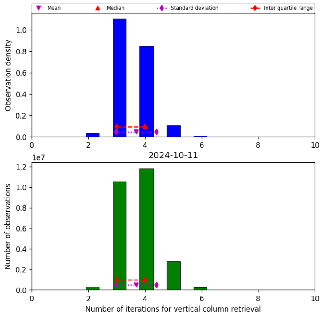
Figure 26: Histogram of “Number of iterations for vertical column retrieval” for 2024-10-10 to 2024-10-12
