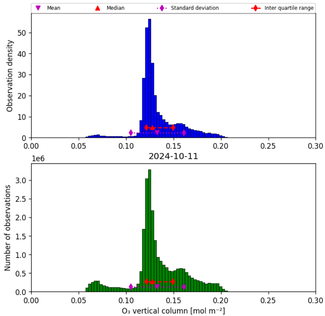
Figure 21: Histogram of “O 3 vertical column” for 2024-10-10 to 2024-10-12
