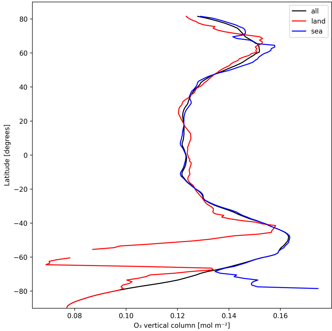
Figure 14: Zonal average of “O 3 vertical column” for 2024-10-10 to 2024-10-12.
