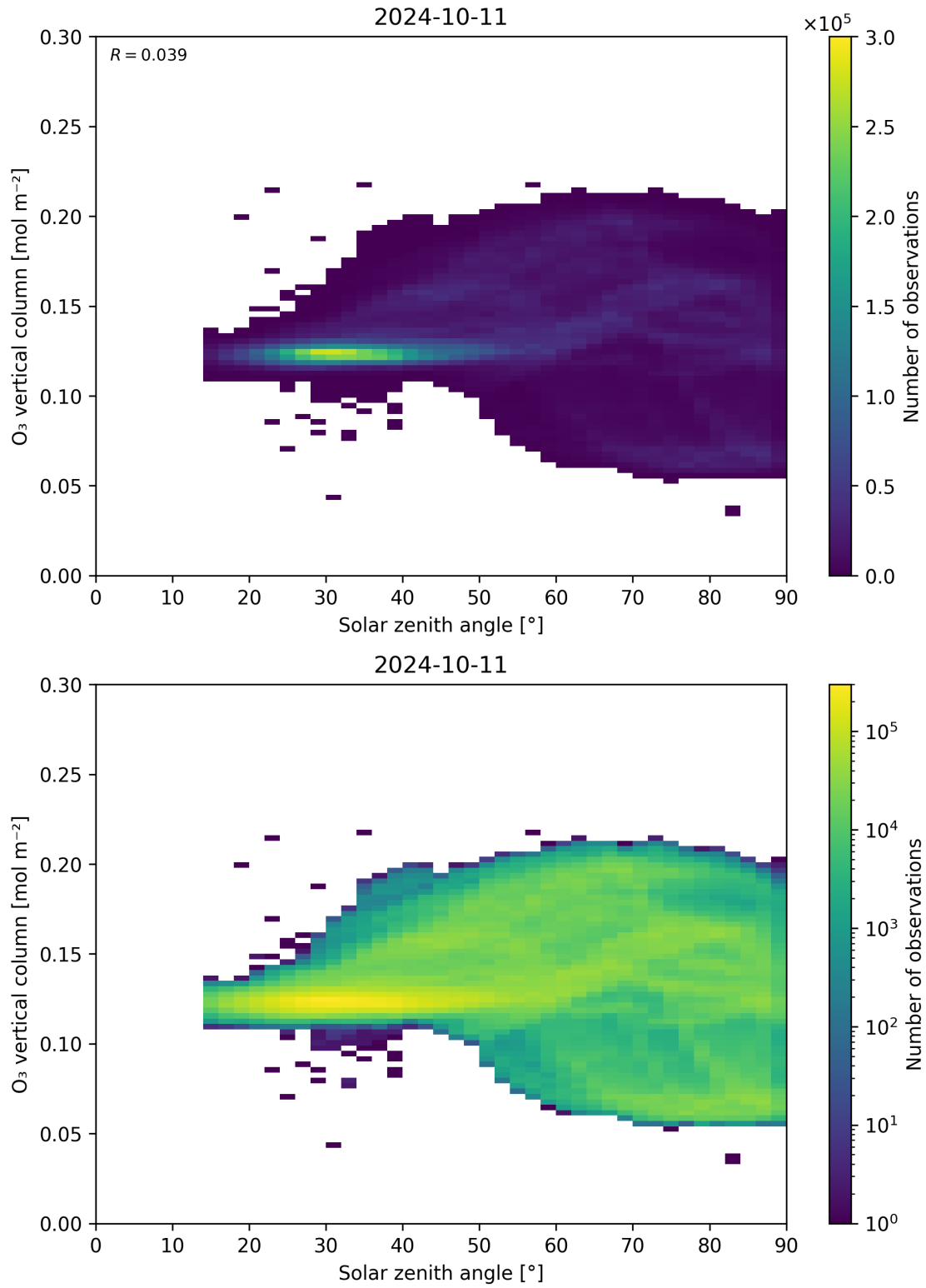
Figure 47: Scatter density plot of “Solar zenith angle” against “O 3 vertical column” for 2024-10-10 to 2024-10-12.
