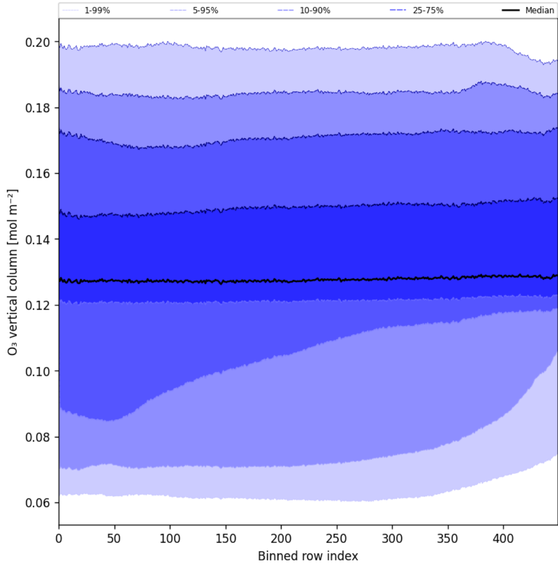
Figure 28: Along track statistics of “O 3 vertical column” for 2024-10-10 to 2024-10-12
