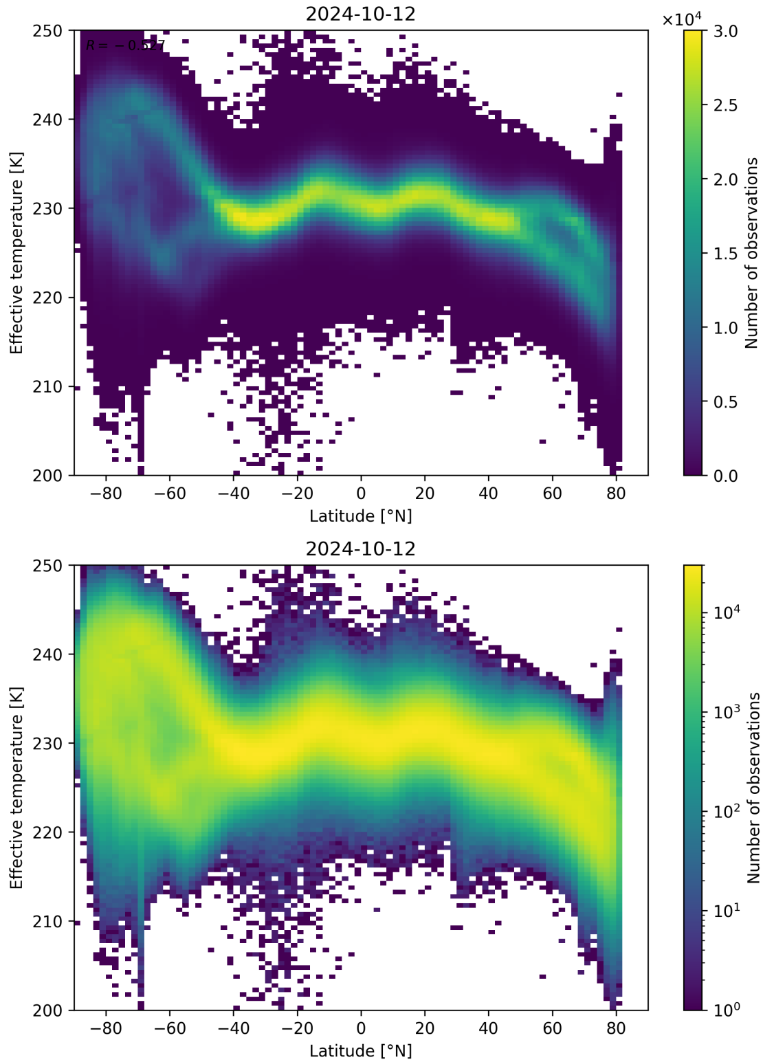
Figure 34: Scatter density plot of “Latitude” against “Effective temperature” for 2024-10-11 to 2024-10-13.
