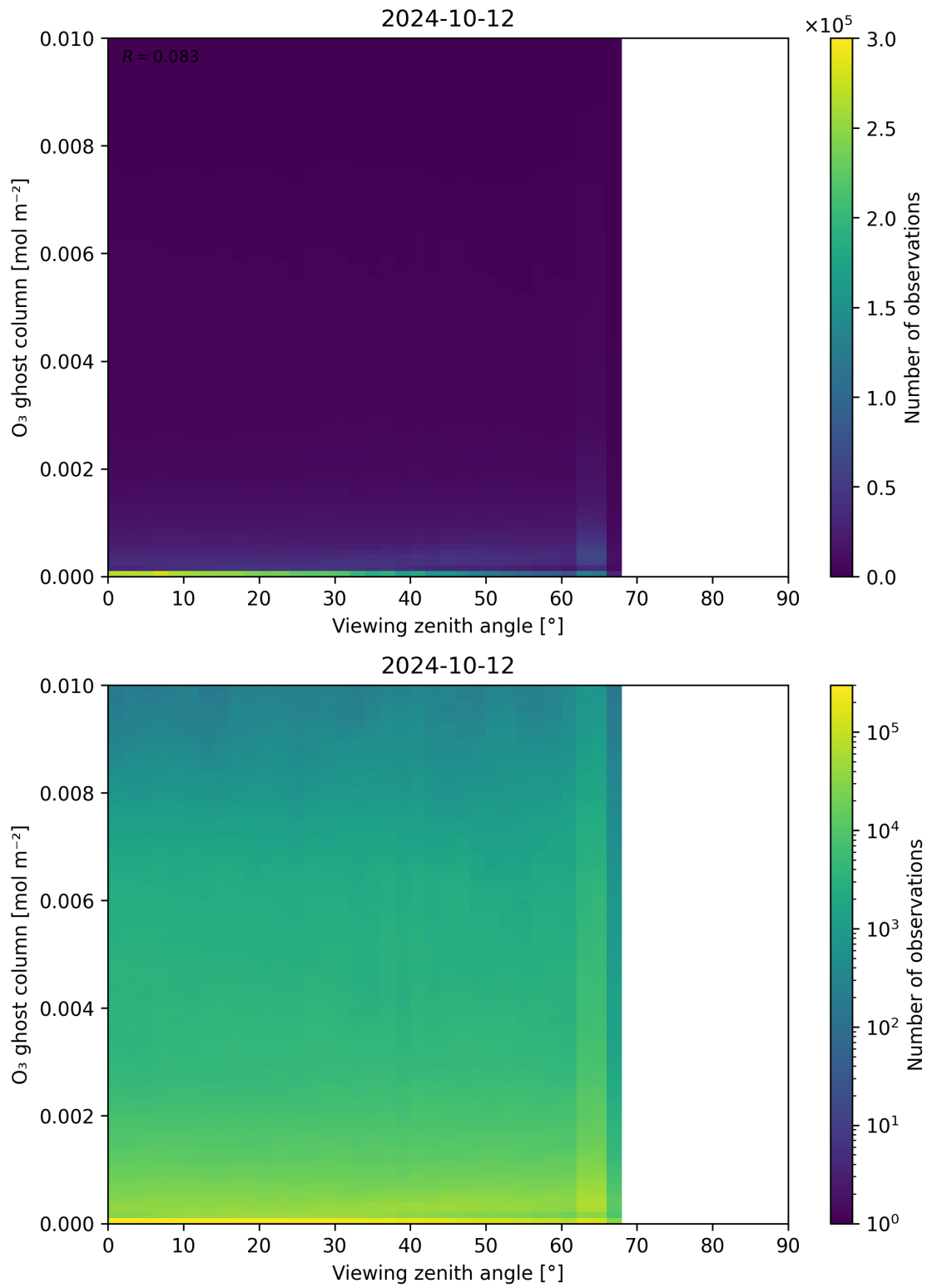
Figure 51: Scatter density plot of “Viewing zenith angle” against “O 3 ghost column” for 2024-10-11 to 2024-10-13.
