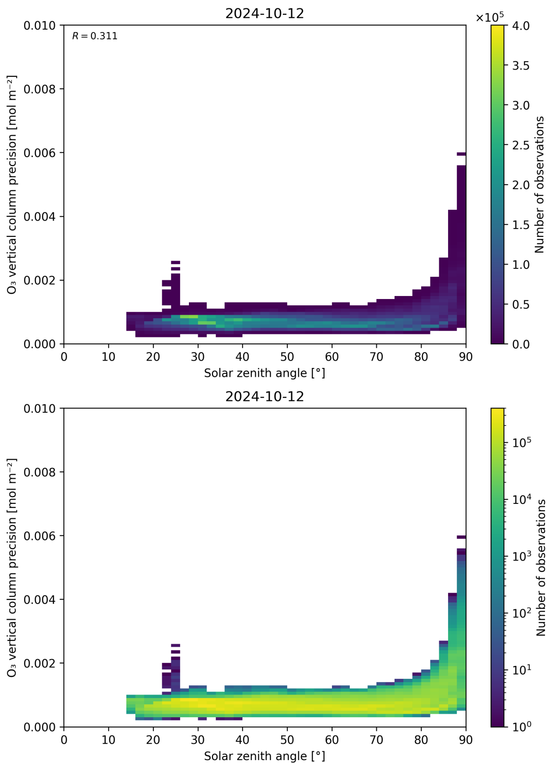
Figure 48: Scatter density plot of “Solar zenith angle” against “O 3 vertical column precision” for 2024-10-11 to 2024-10-13.
