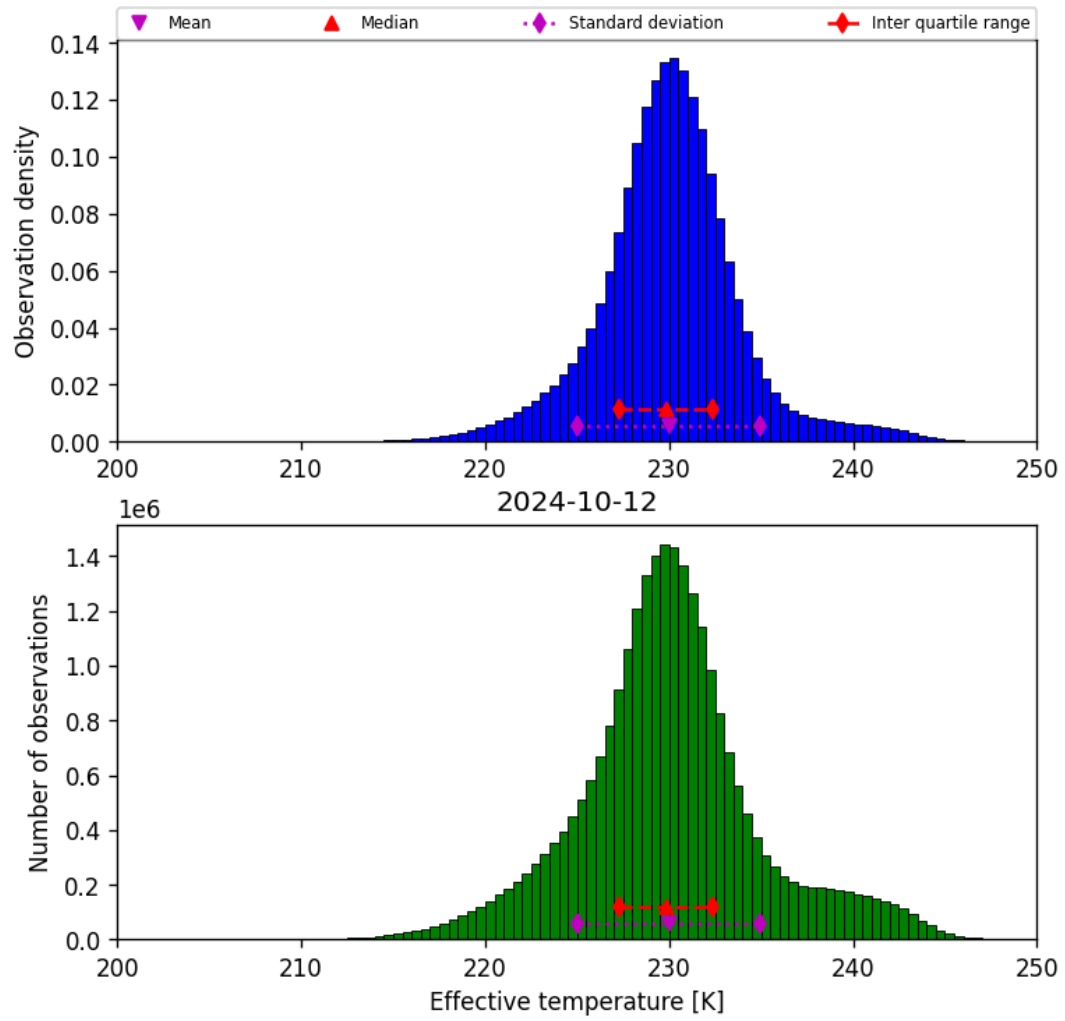
Figure 24: Histogram of “Effective temperature” for 2024-10-11 to 2024-10-13
