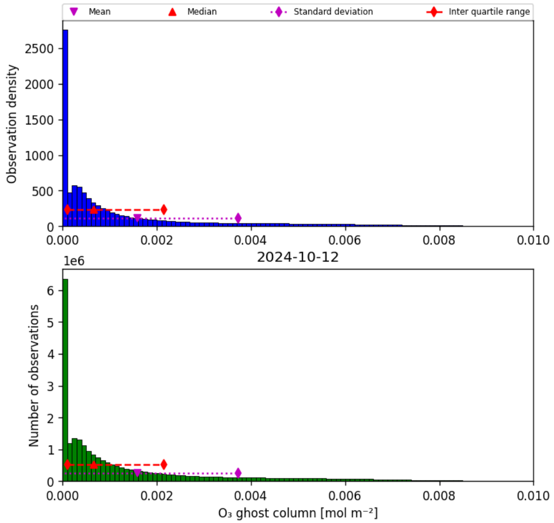
Figure 25: Histogram of “O 3 ghost column” for 2024-10-11 to 2024-10-13
