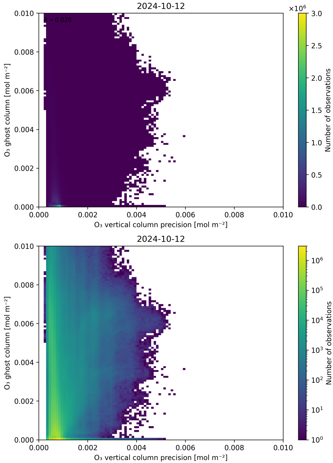
Figure 43: Scatter density plot of “ \text{O}_3 vertical column precision” against “ \text{O}_3 ghost column” for 2024-10-11 to 2024-10-13.
