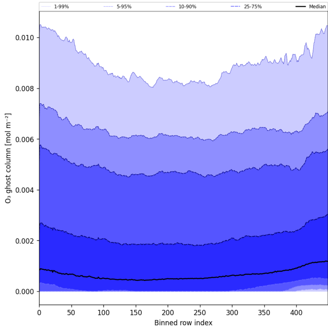
Figure 32: Along track statistics of “O 3 ghost column” for 2024-10-11 to 2024-10-13
