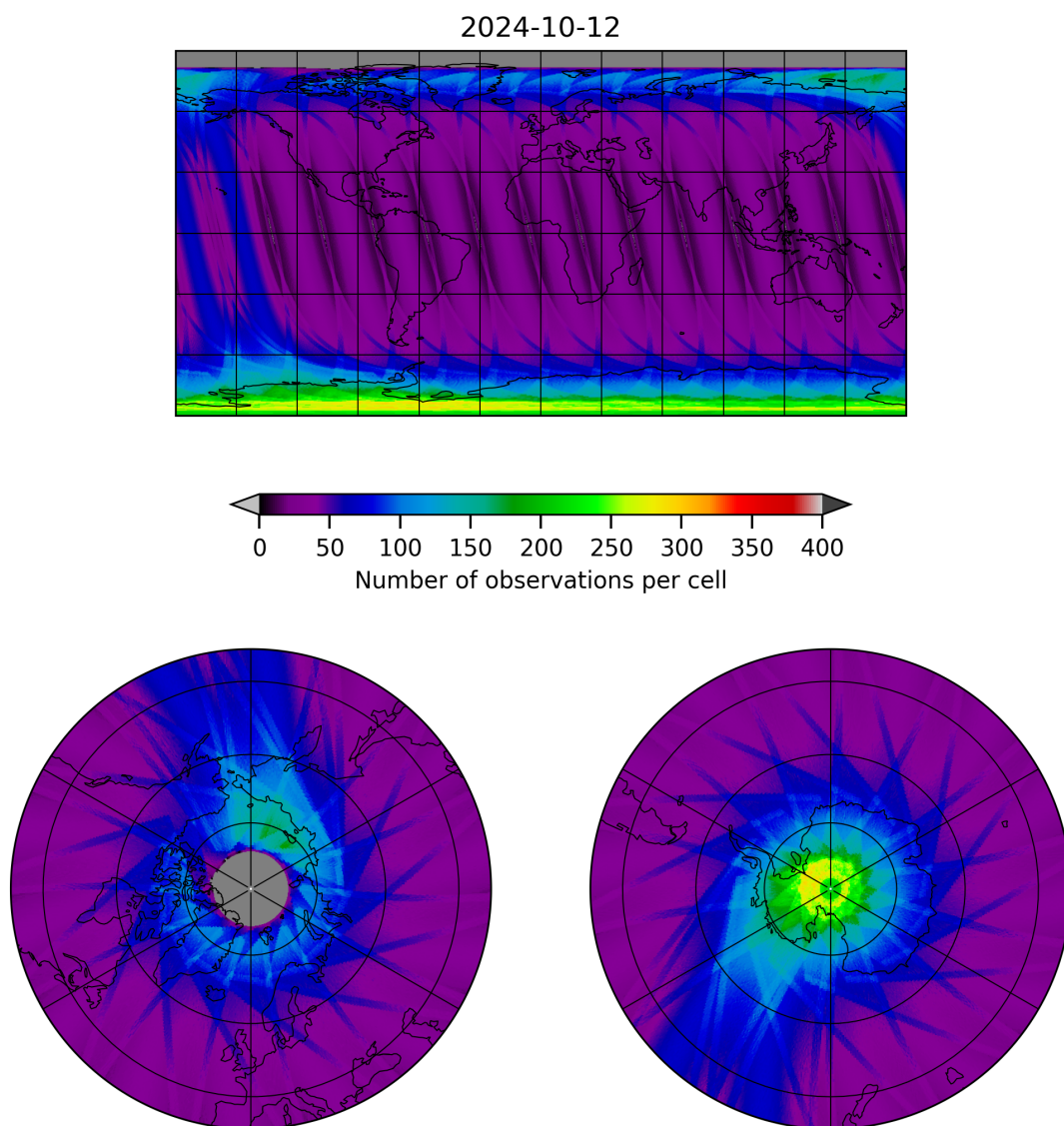
Figure 12: Map of the number of observations for 2024-10-11 to 2024-10-13
