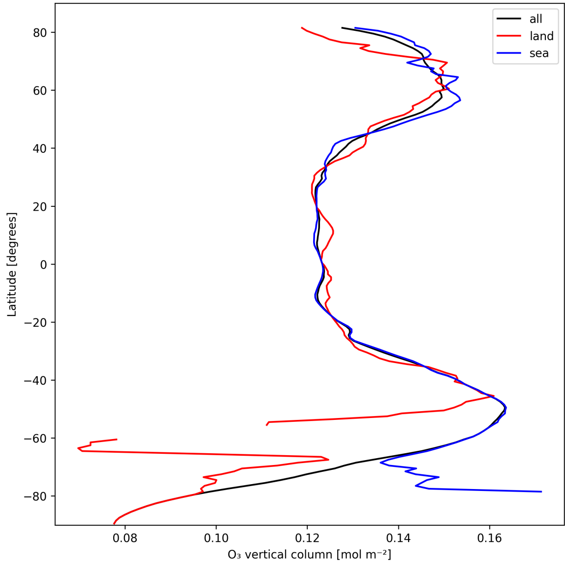
Figure 14: Zonal average of “O 3 vertical column” for 2024-10-11 to 2024-10-13.
