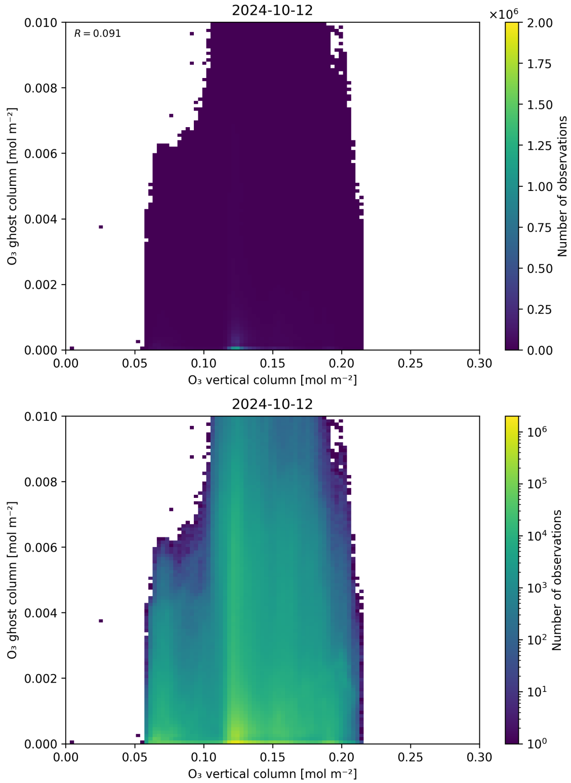
Figure 40: Scatter density plot of “O 3 vertical column” against “O 3 ghost column” for 2024-10-11 to 2024-10-13.
