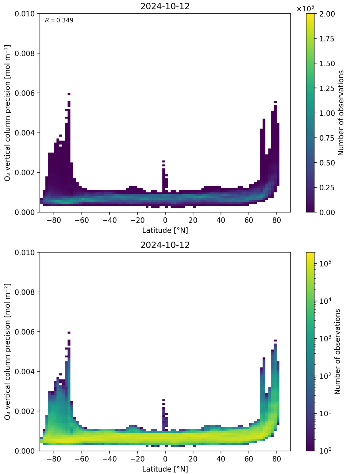
Figure 37: Scatter density plot of “Latitude” against “O 3 vertical column precision” for 2024-10-11 to 2024-10-13.
