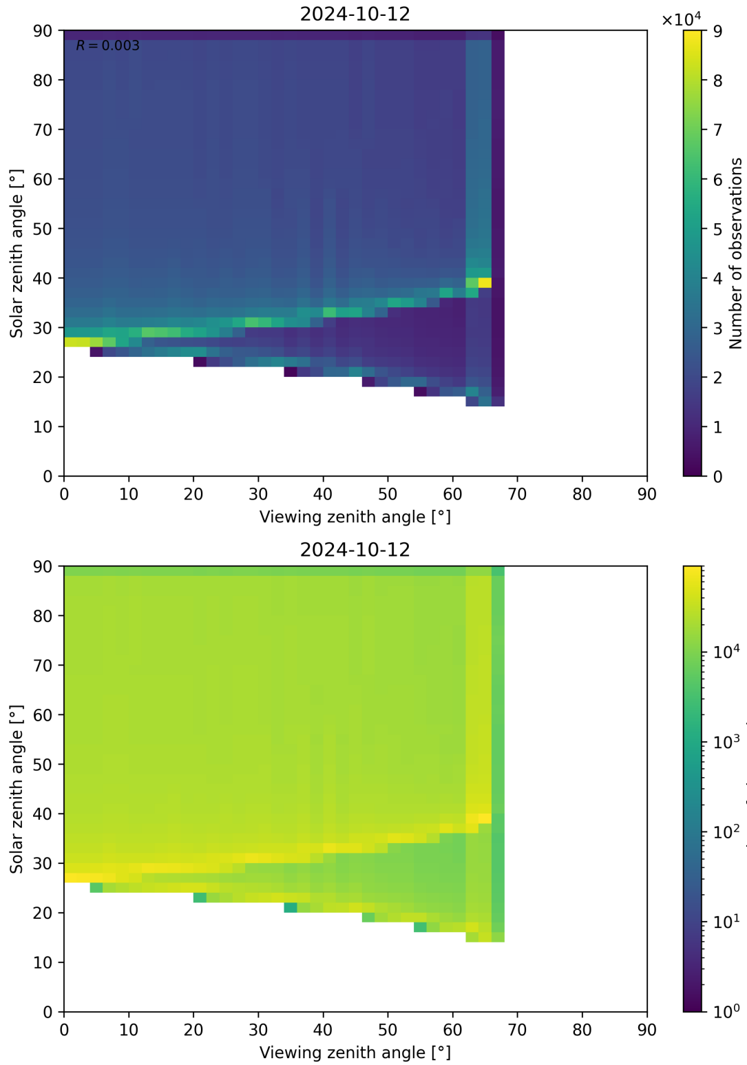
Figure 54: Scatter density plot of “Viewing zenith angle” against “Solar zenith angle” for 2024-10-11 to 2024-10-13.
