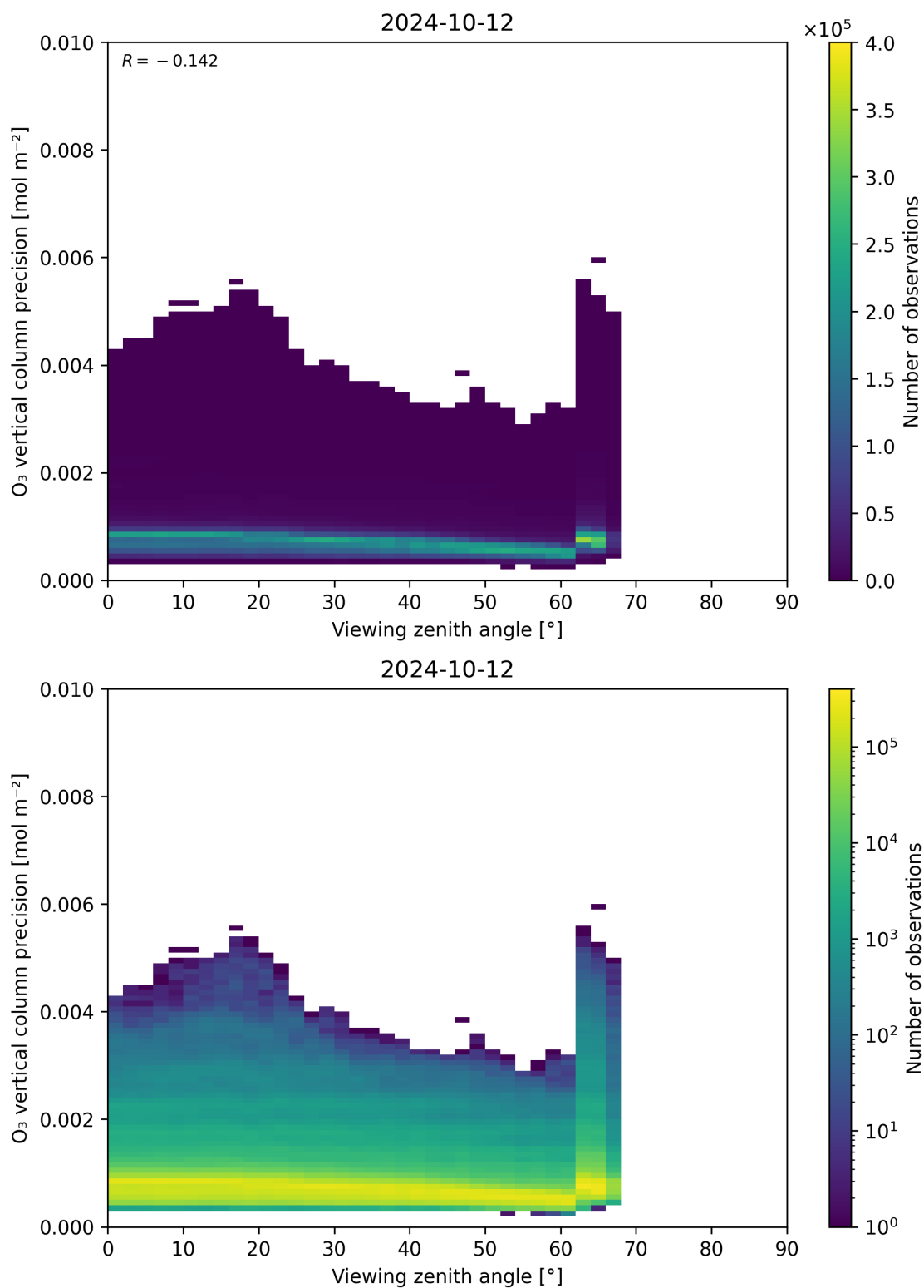
Figure 53: Scatter density plot of “Viewing zenith angle” against “O 3 vertical column precision” for 2024-10-11 to 2024-10-13.
