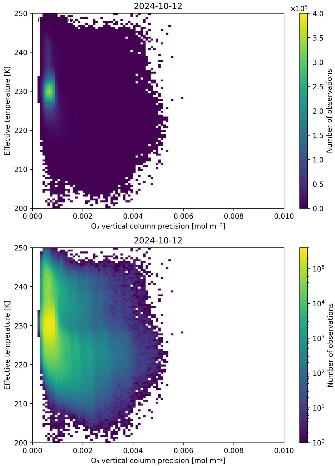
Figure 42: Scatter density plot of “ O_3 vertical column precision” against “Effective temperature” for 2024-10-11 to 2024-10-13.
