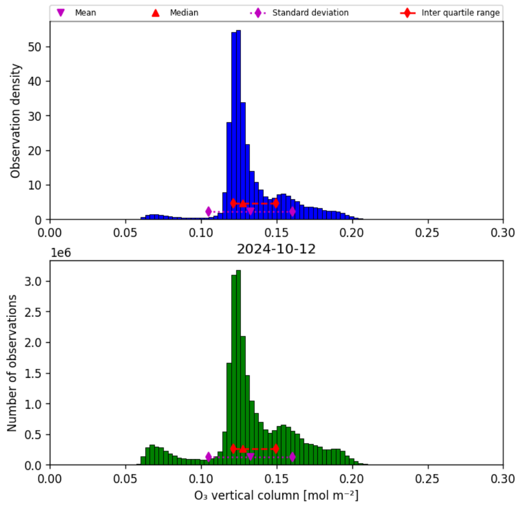
Figure 21: Histogram of “O 3 vertical column” for 2024-10-11 to 2024-10-13
