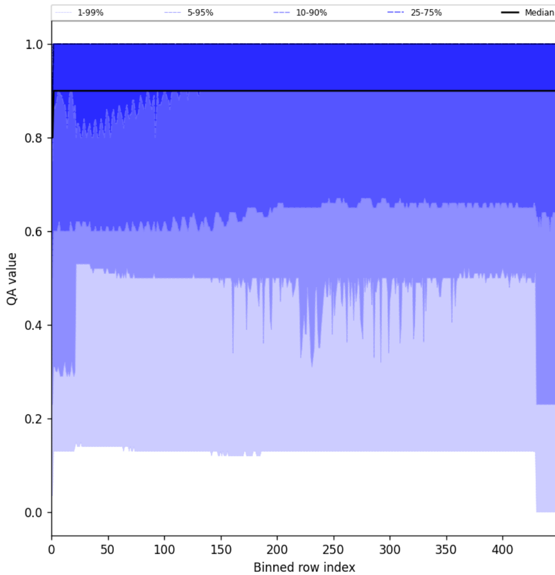
Figure 27: Along track statistics of “QA value” for 2024-10-11 to 2024-10-13
