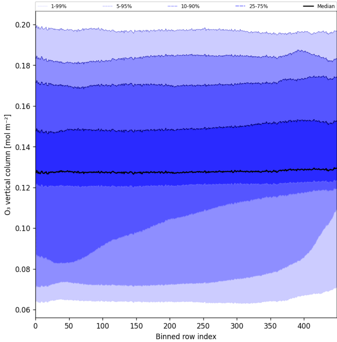
Figure 28: Along track statistics of “O 3 vertical column” for 2024-10-11 to 2024-10-13
