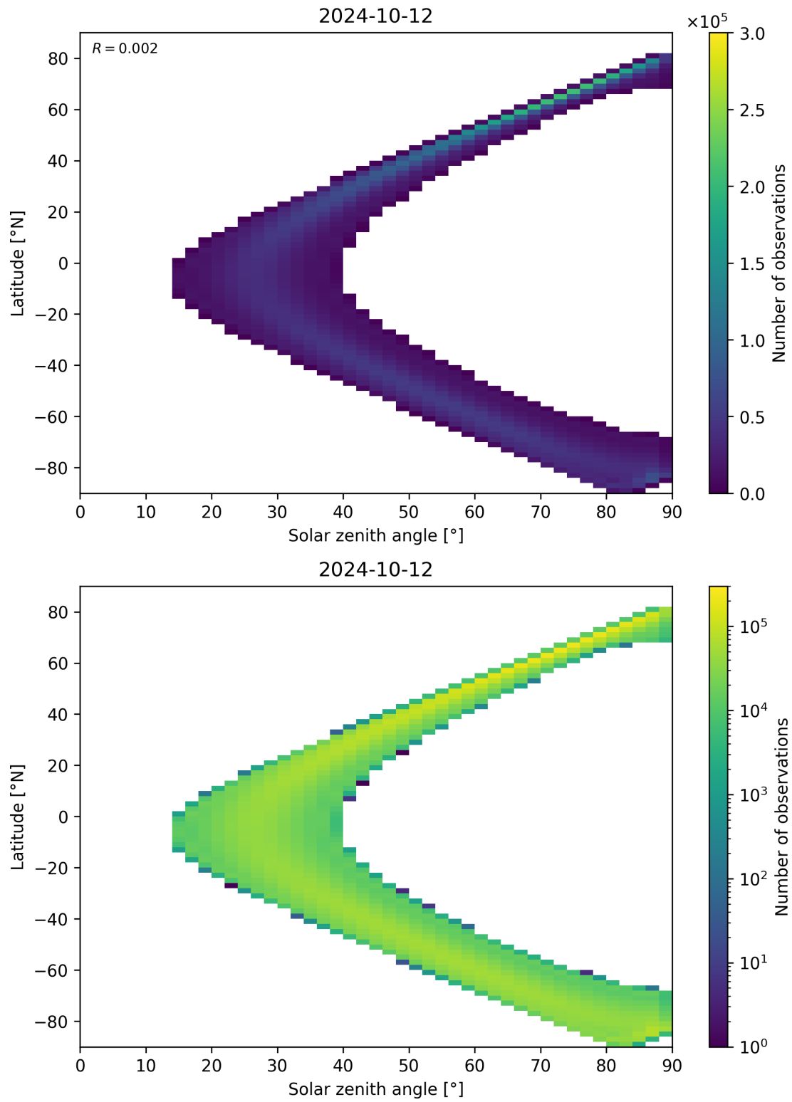
Figure 44: Scatter density plot of “Solar zenith angle” against “Latitude” for 2024-10-11 to 2024-10-13.
