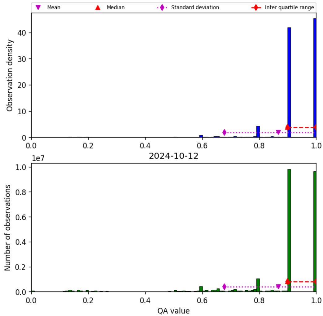
Figure 20: Histogram of “QA value” for 2024-10-11 to 2024-10-13
