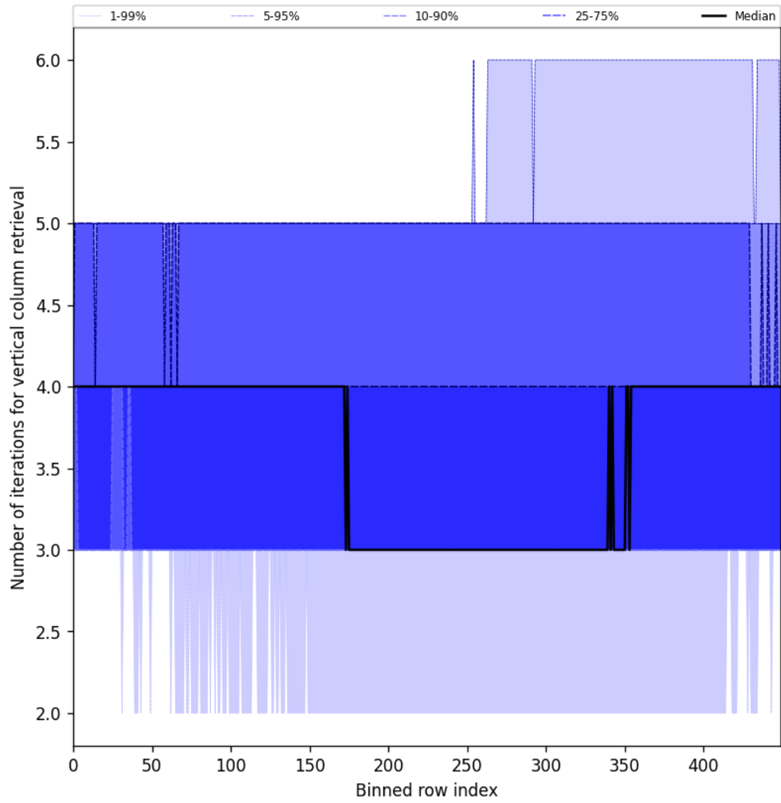
Figure 33: Along track statistics of “Number of iterations for vertical column retrieval” for 2024-10-11 to 2024-10-13
