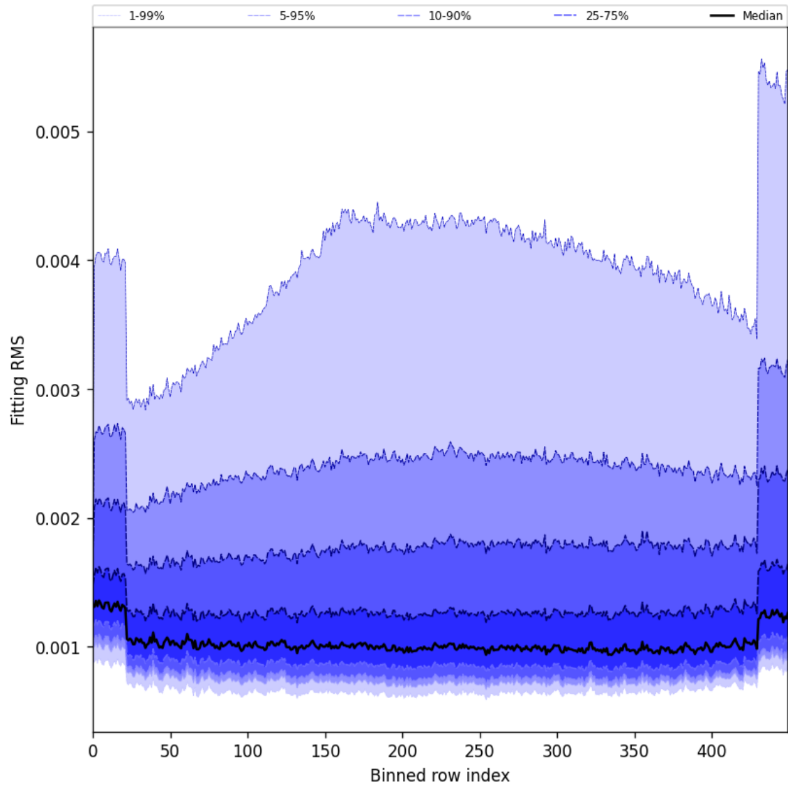
Figure 30: Along track statistics of “Fitting RMS” for 2024-10-11 to 2024-10-13
