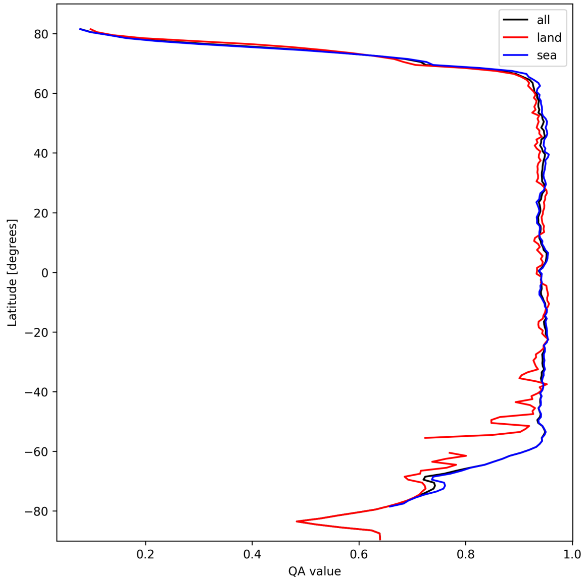
Figure 13: Zonal average of “QA value” for 2024-10-11 to 2024-10-13.
