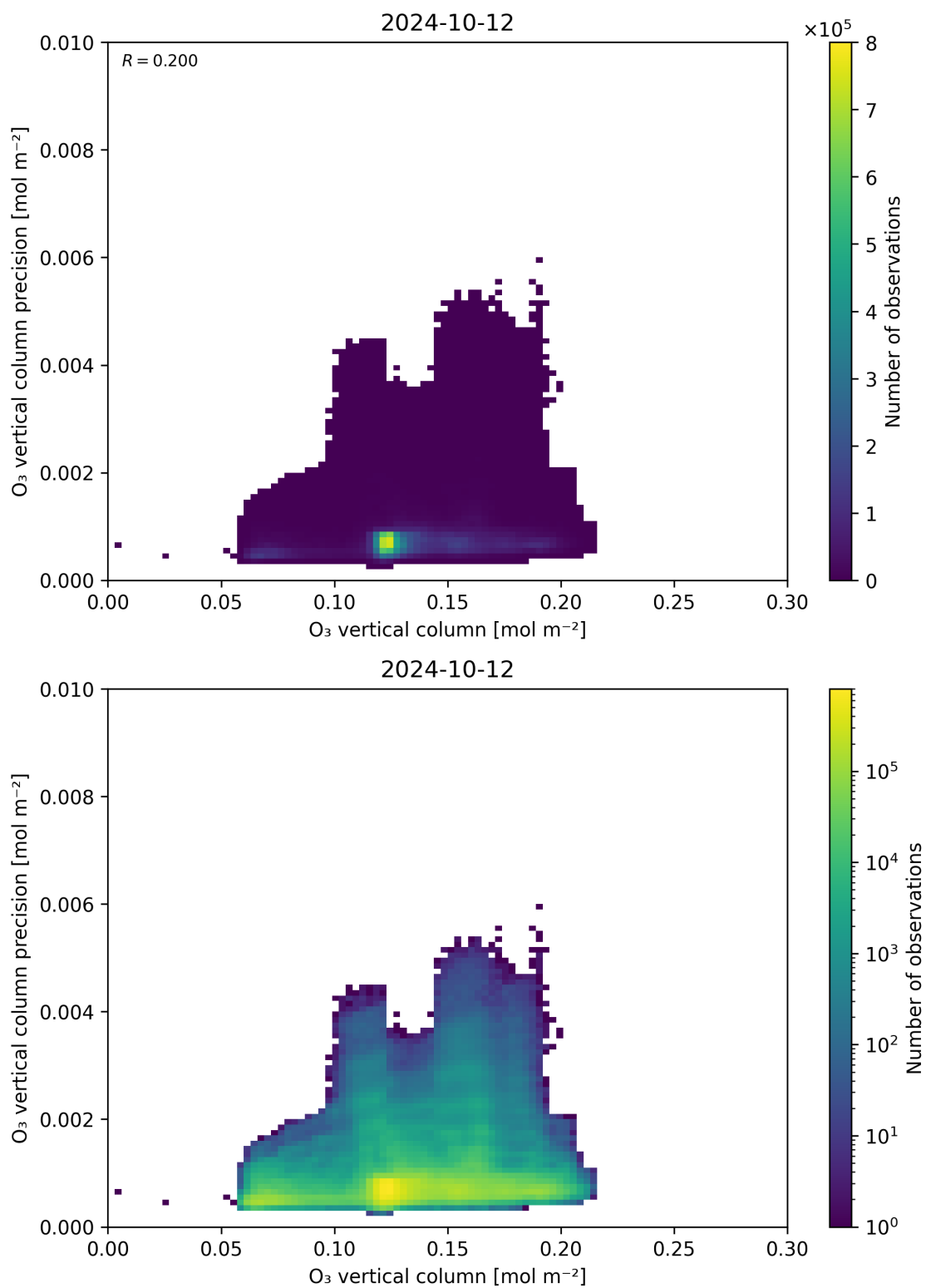
Figure 41: Scatter density plot of “O 3 vertical column” against “O 3 vertical column precision” for 2024-10-11 to 2024-10-13.
