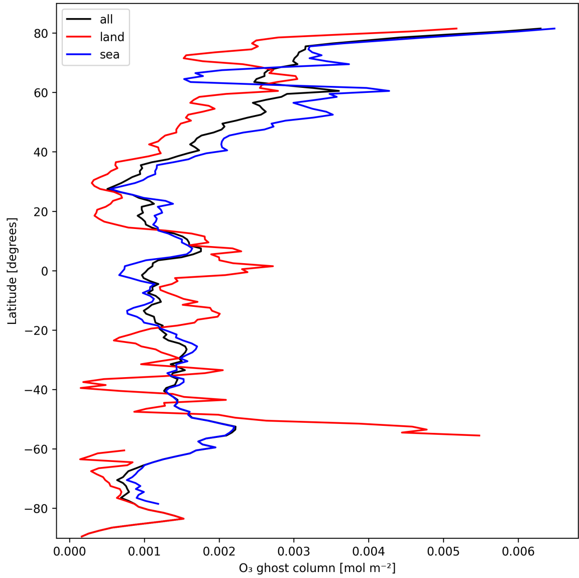
Figure 18: Zonal average of “O 3 ghost column” for 2024-10-11 to 2024-10-13.
