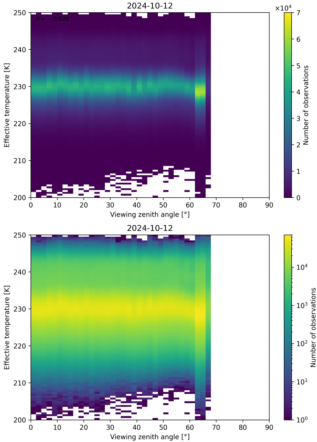
Figure 50: Scatter density plot of “Viewing zenith angle” against “Effective temperature” for 2024-10-11 to 2024-10-13.
