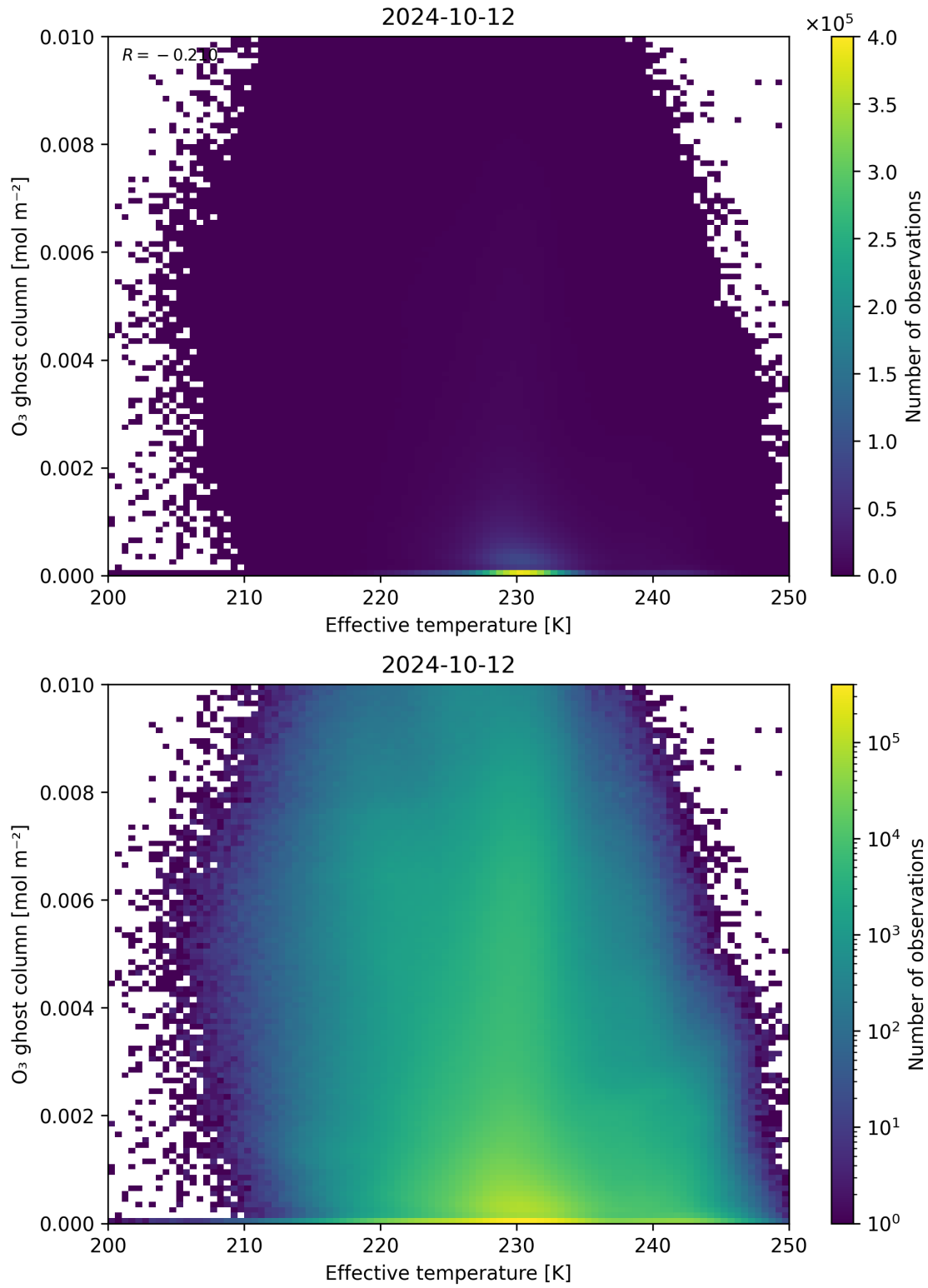
Figure 38: Scatter density plot of “Effective temperature” against “O 3 ghost column” for 2024-10-11 to 2024-10-13.
