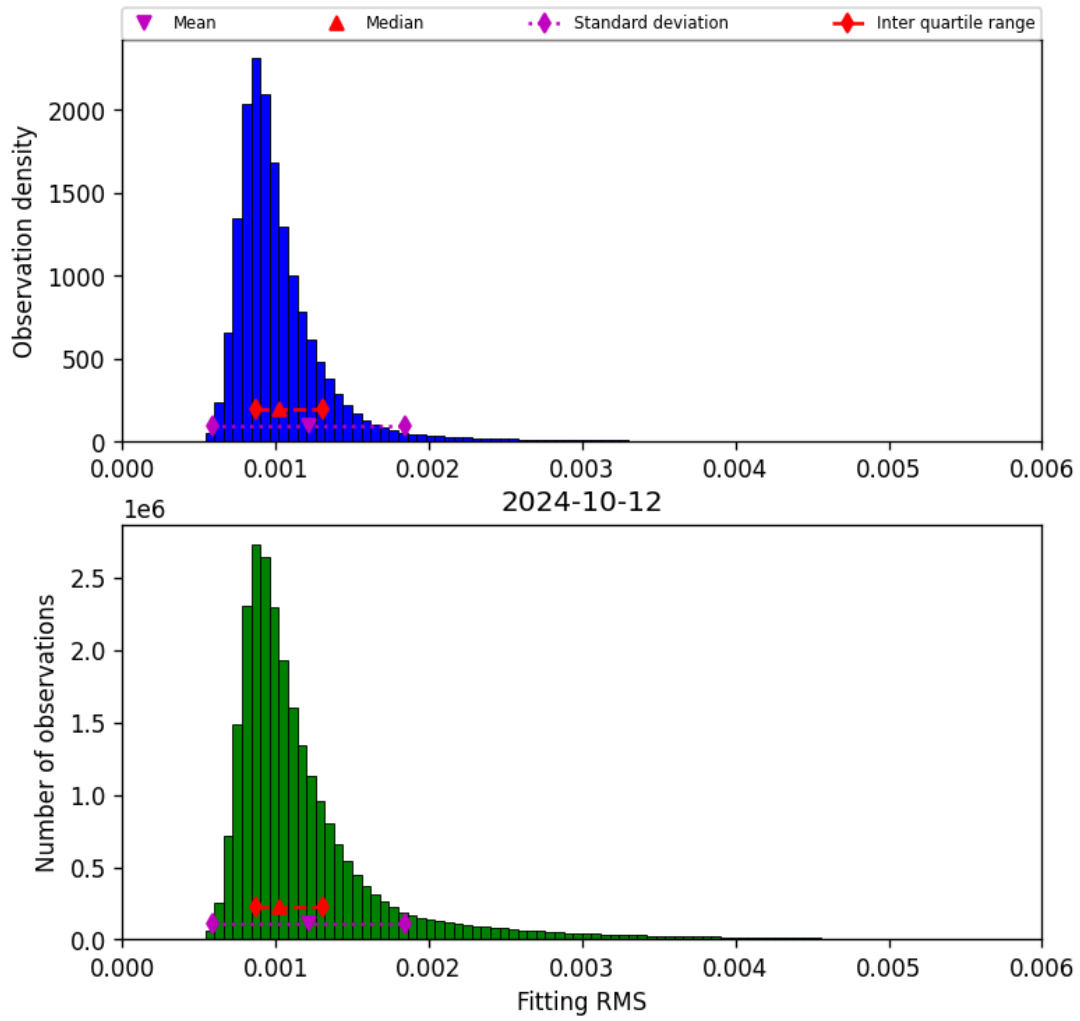
Figure 23: Histogram of “Fitting RMS” for 2024-10-11 to 2024-10-13
