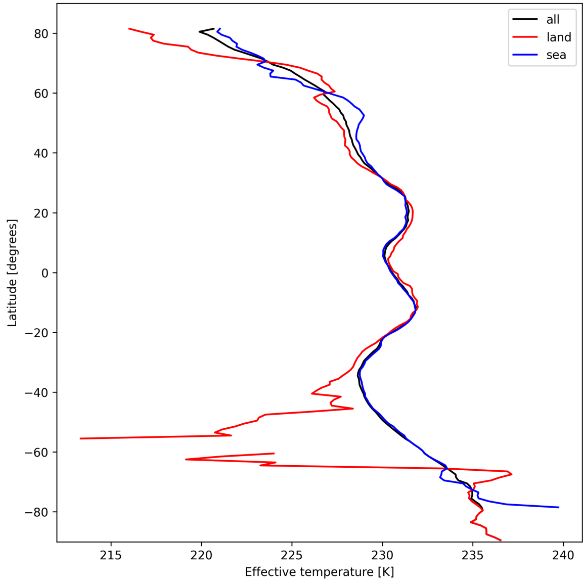
Figure 17: Zonal average of “Effective temperature” for 2024-10-11 to 2024-10-13.
