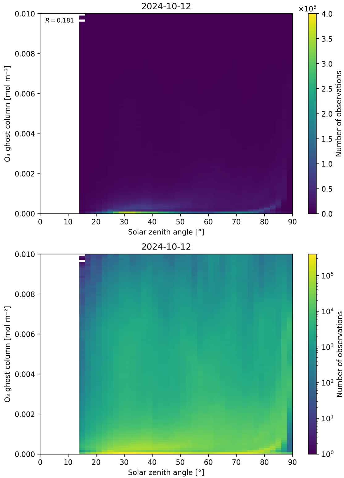
Figure 46: Scatter density plot of “Solar zenith angle” against “O 3 ghost column” for 2024-10-11 to 2024-10-13.
