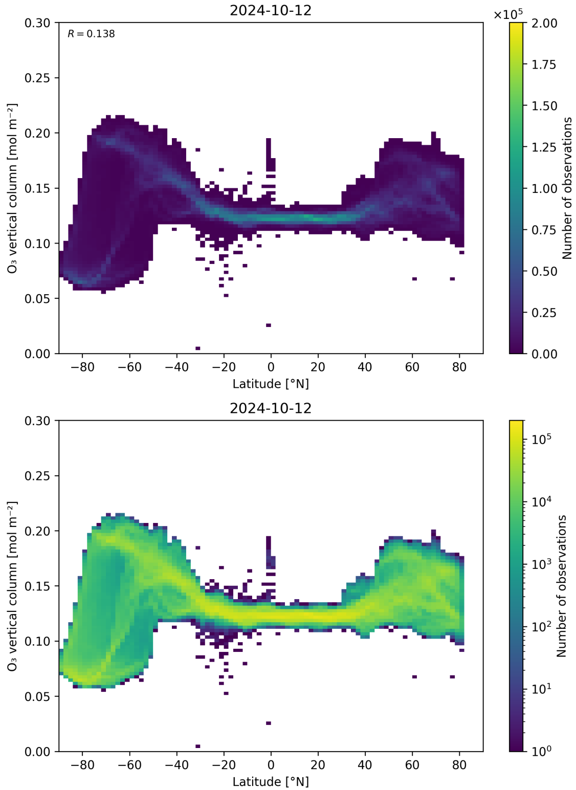
Figure 36: Scatter density plot of “Latitude” against “O 3 vertical column” for 2024-10-11 to 2024-10-13.
