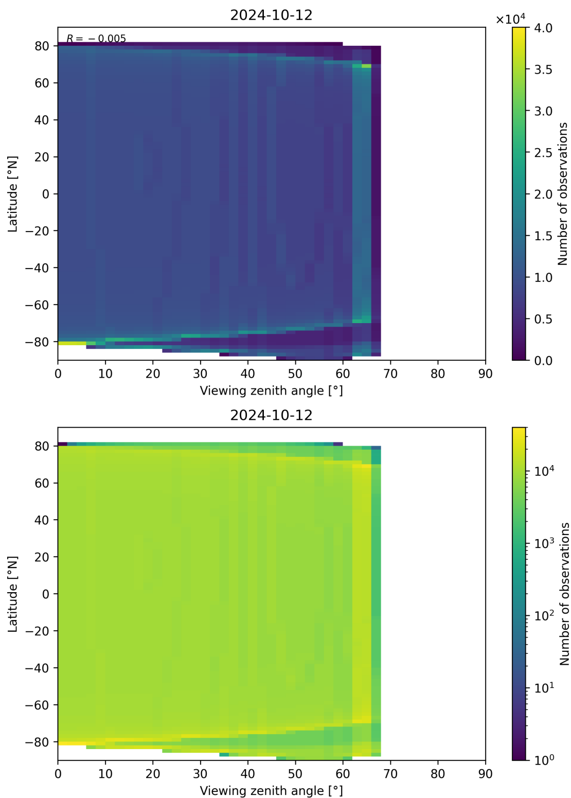
Figure 49: Scatter density plot of “Viewing zenith angle” against “Latitude” for 2024-10-11 to 2024-10-13.
