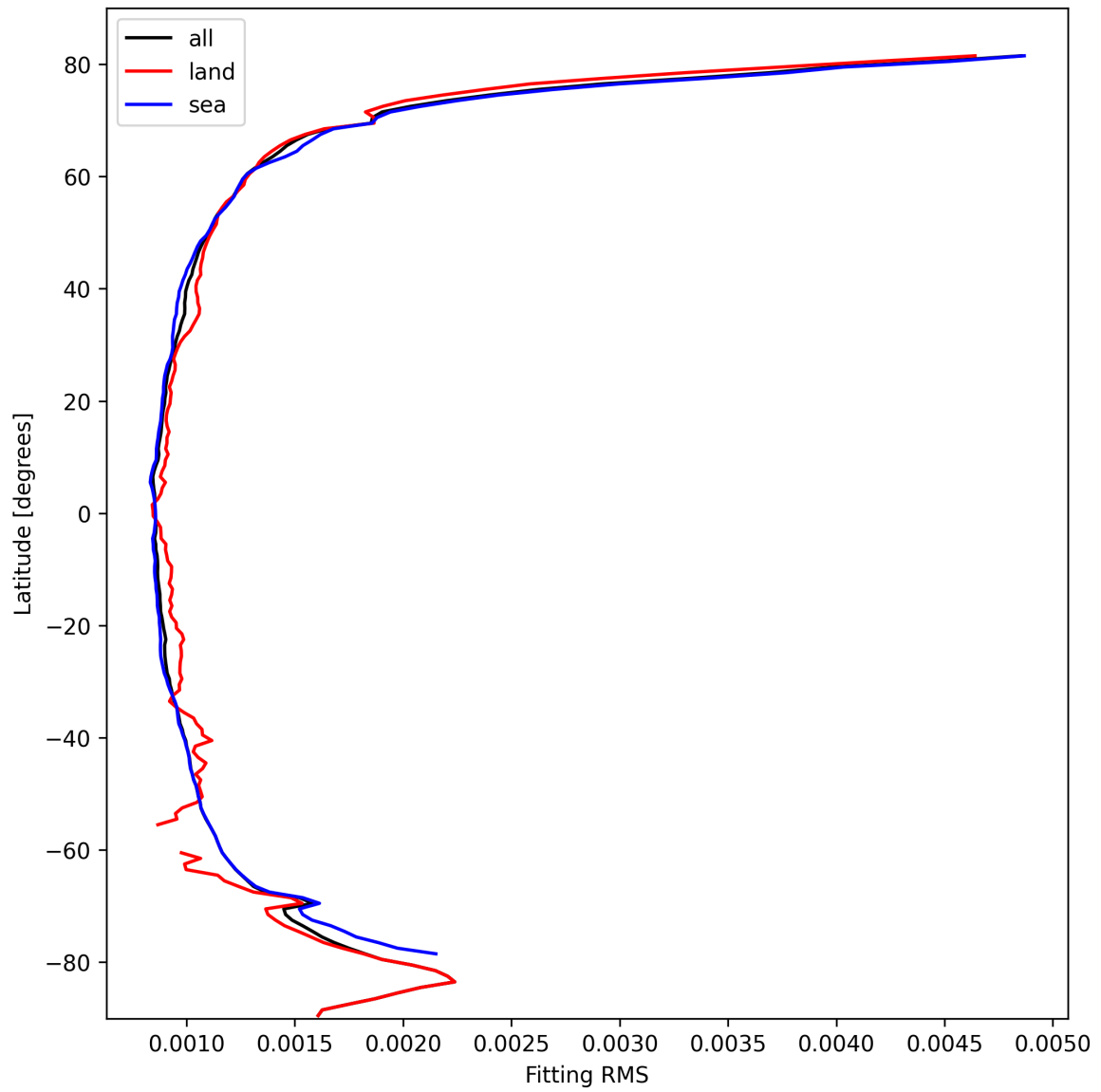
Figure 16: Zonal average of “Fitting RMS” for 2024-10-11 to 2024-10-13.
