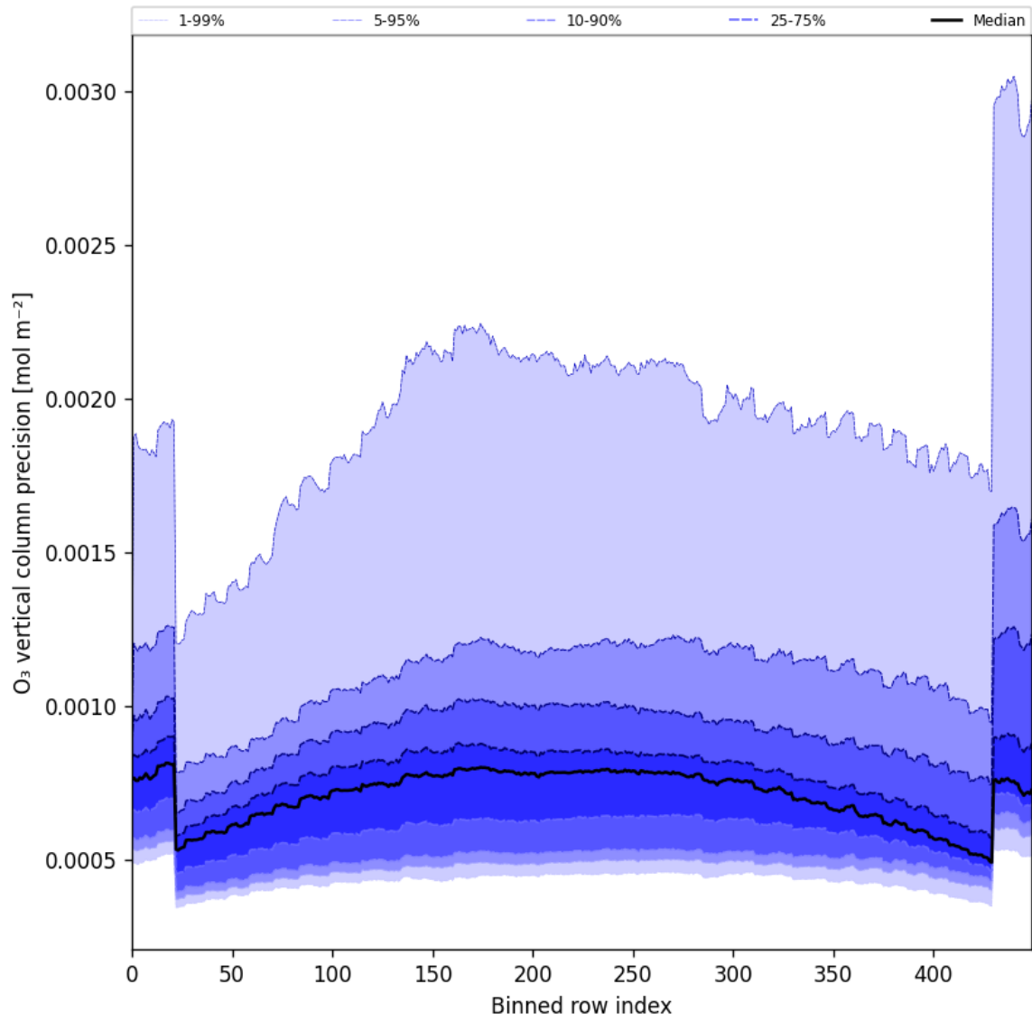
Figure 29: Along track statistics of “O 3 vertical column precision” for 2024-10-11 to 2024-10-13
