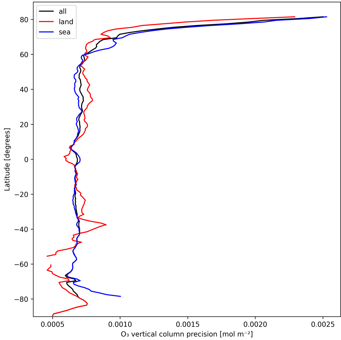
Figure 15: Zonal average of “O 3 vertical column precision” for 2024-10-11 to 2024-10-13.
