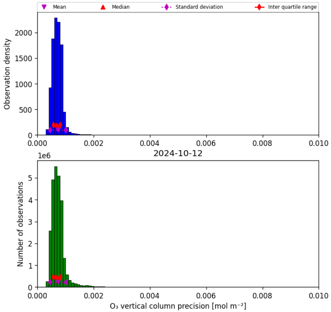
Figure 22: Histogram of “O 3 vertical column precision” for 2024-10-11 to 2024-10-13
