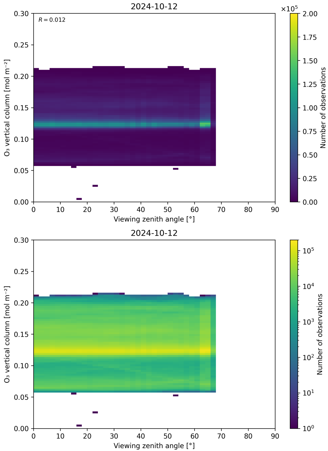
Figure 52: Scatter density plot of “Viewing zenith angle” against “O 3 vertical column” for 2024-10-11 to 2024-10-13.
