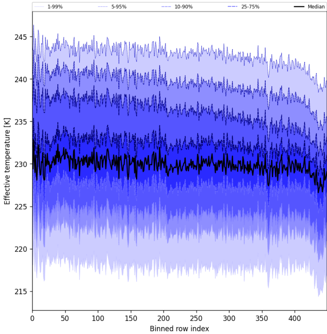
Figure 31: Along track statistics of “Effective temperature” for 2024-10-11 to 2024-10-13
