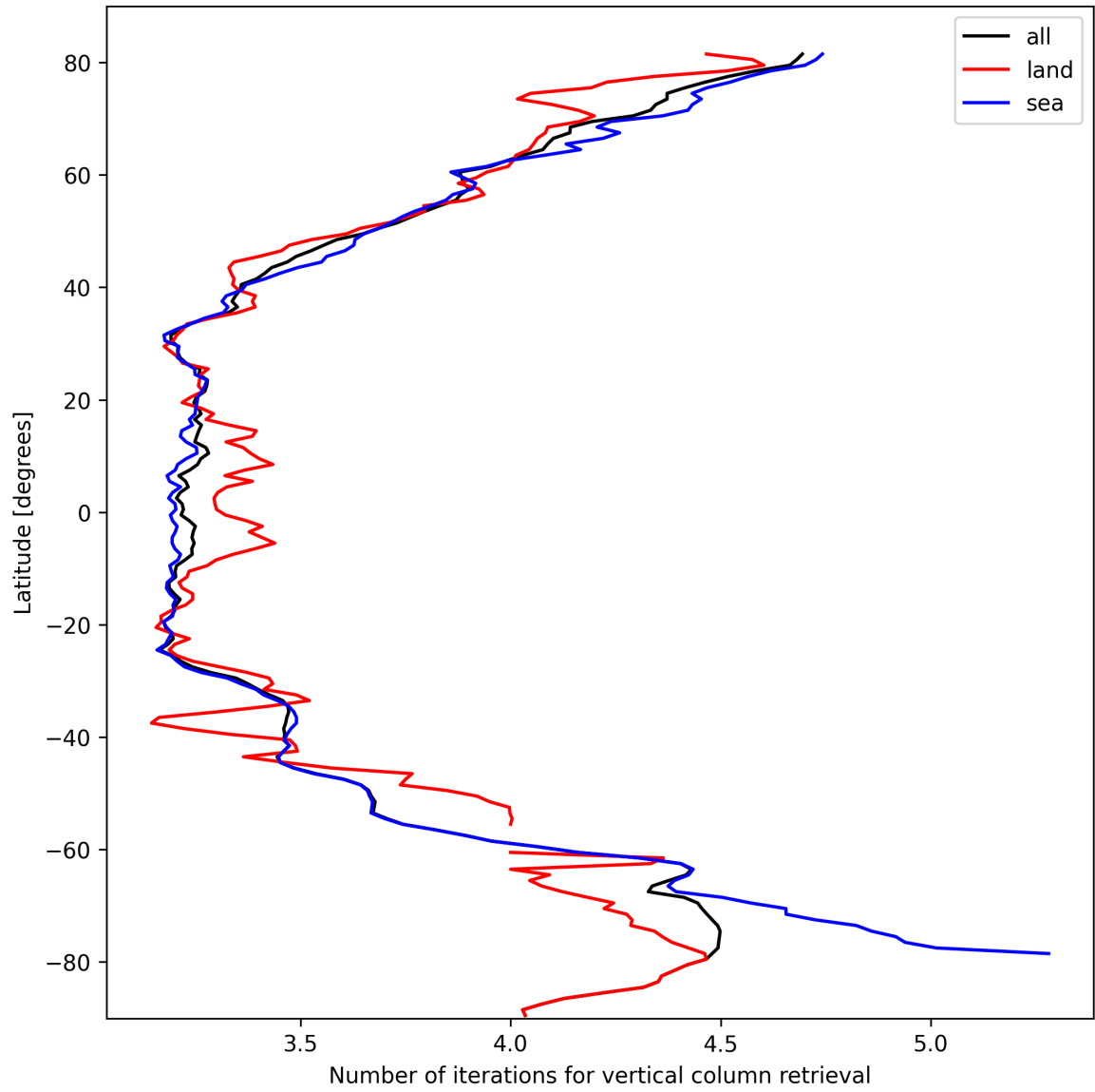
Figure 19: Zonal average of “Number of iterations for vertical column retrieval” for 2024-10-11 to 2024-10-13.
