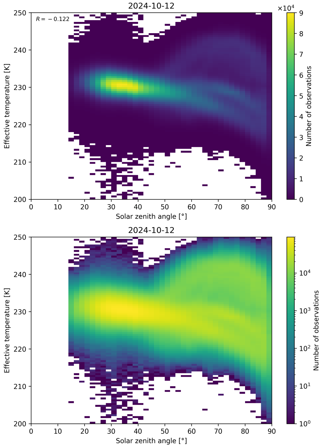
Figure 45: Scatter density plot of “Solar zenith angle” against “Effective temperature” for 2024-10-11 to 2024-10-13.
