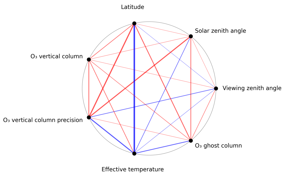
Figure 1: Map of correlation graph for 2024-10-11 to 2024-10-13.
