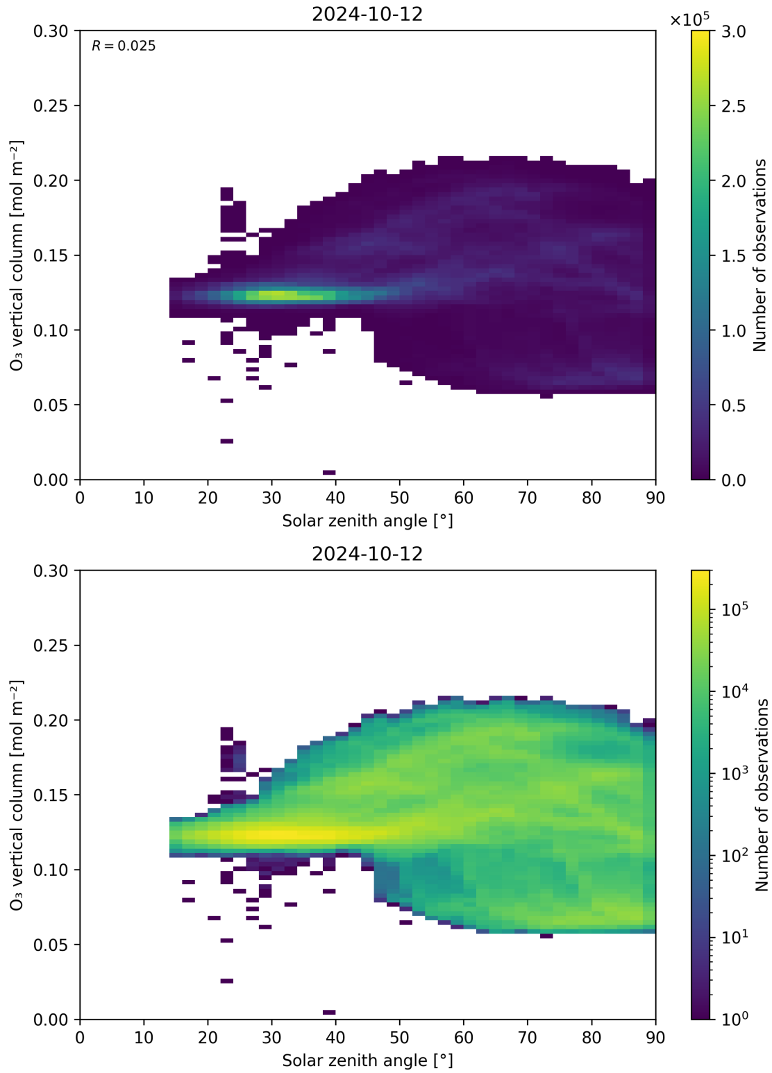
Figure 47: Scatter density plot of “Solar zenith angle” against “O 3 vertical column” for 2024-10-11 to 2024-10-13.
