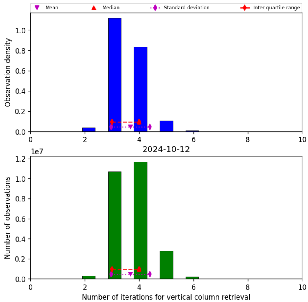
Figure 26: Histogram of “Number of iterations for vertical column retrieval” for 2024-10-11 to 2024-10-13
