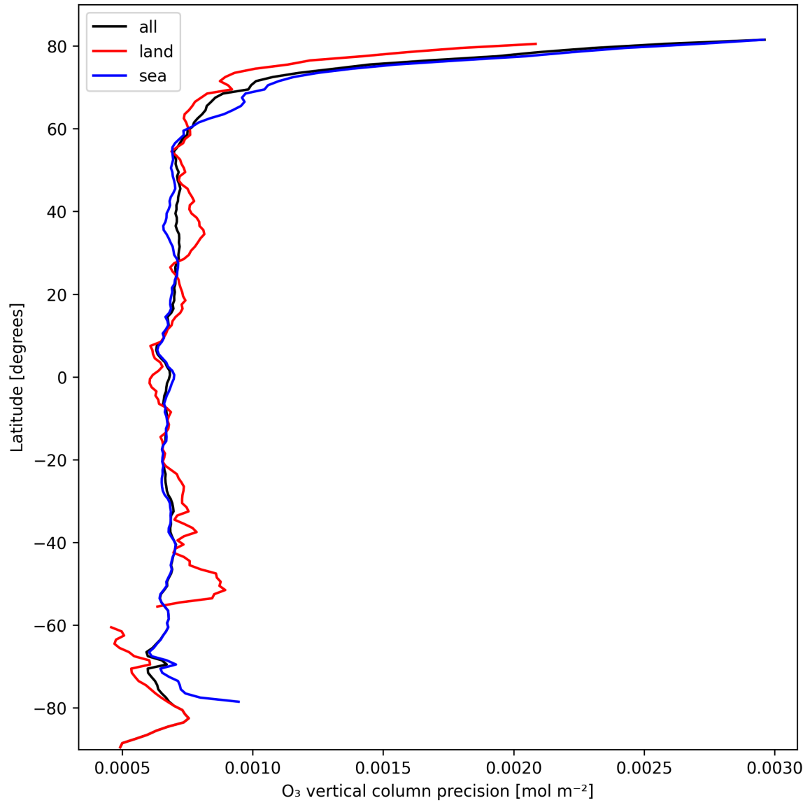
Figure 15: Zonal average of “O 3 vertical column precision” for 2024-10-12 to 2024-10-14.
