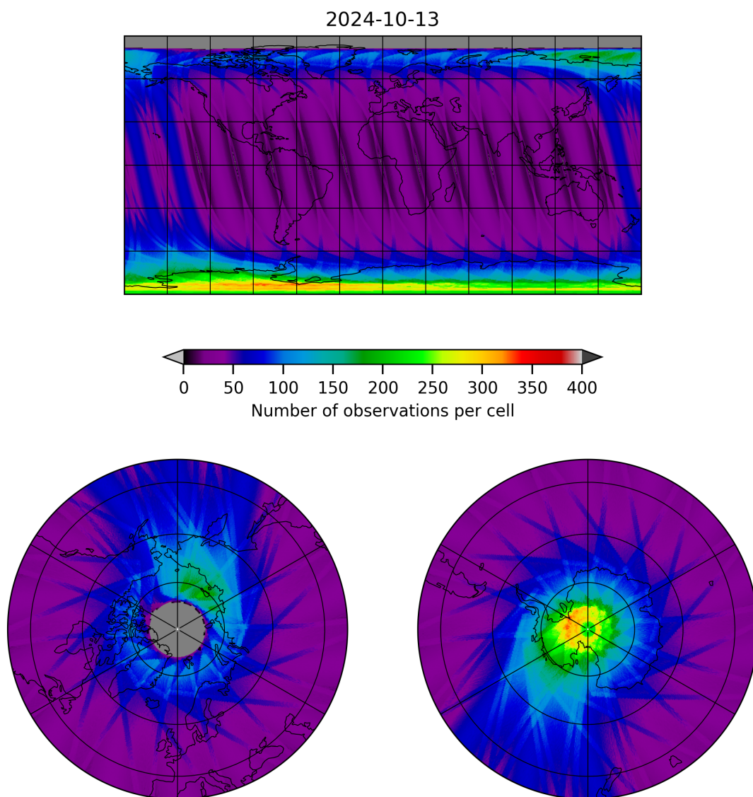
Figure 12: Map of the number of observations for 2024-10-12 to 2024-10-14
