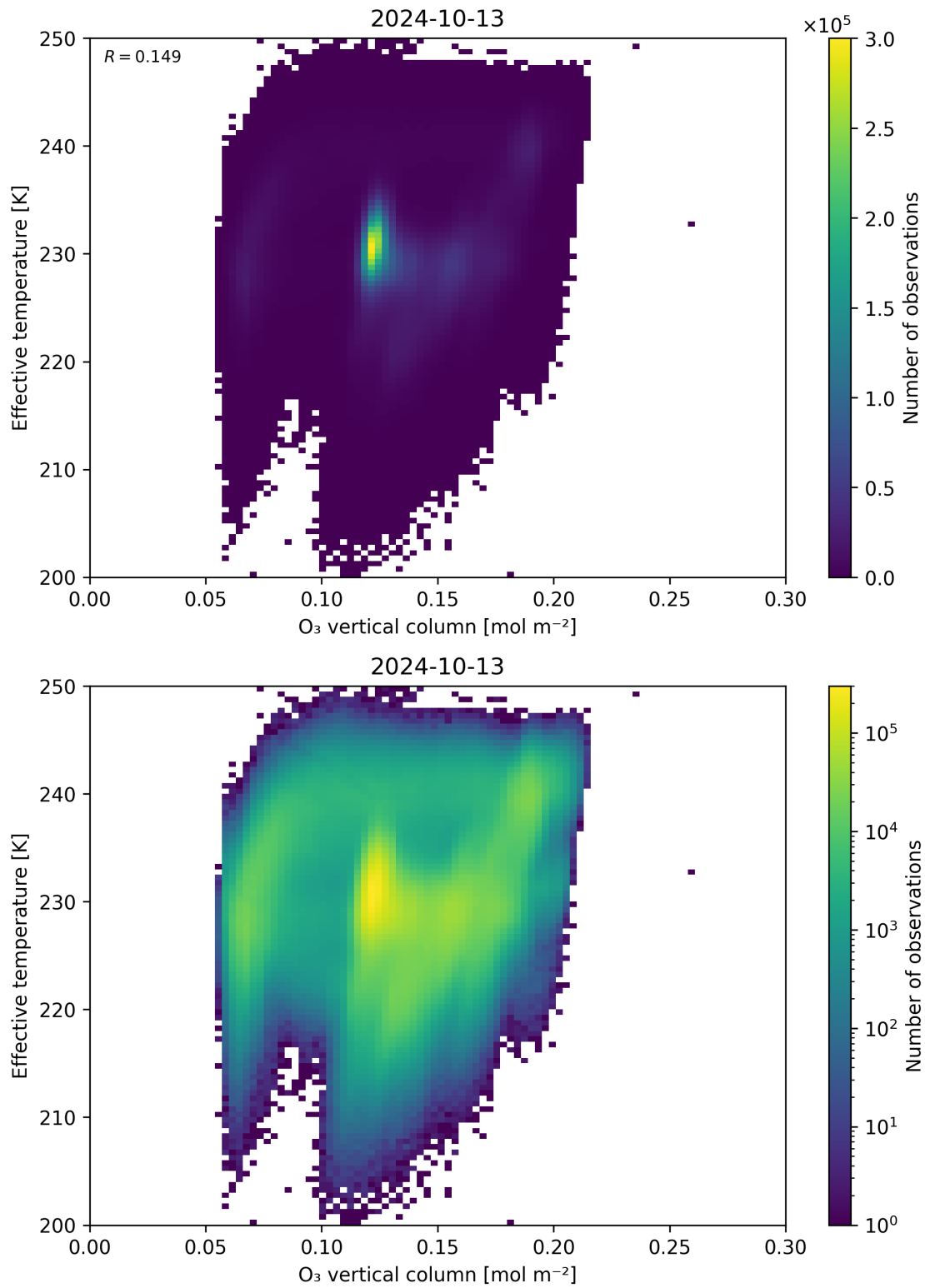
Figure 39: Scatter density plot of “O 3 vertical column” against “Effective temperature” for 2024-10-12 to 2024-10-14.
