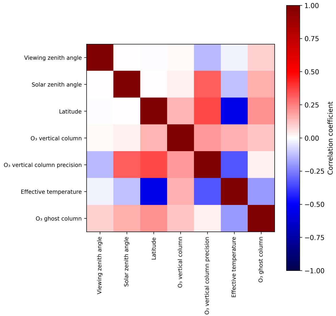
Figure 2: Map of correlation matrix for 2024-10-12 to 2024-10-14.
