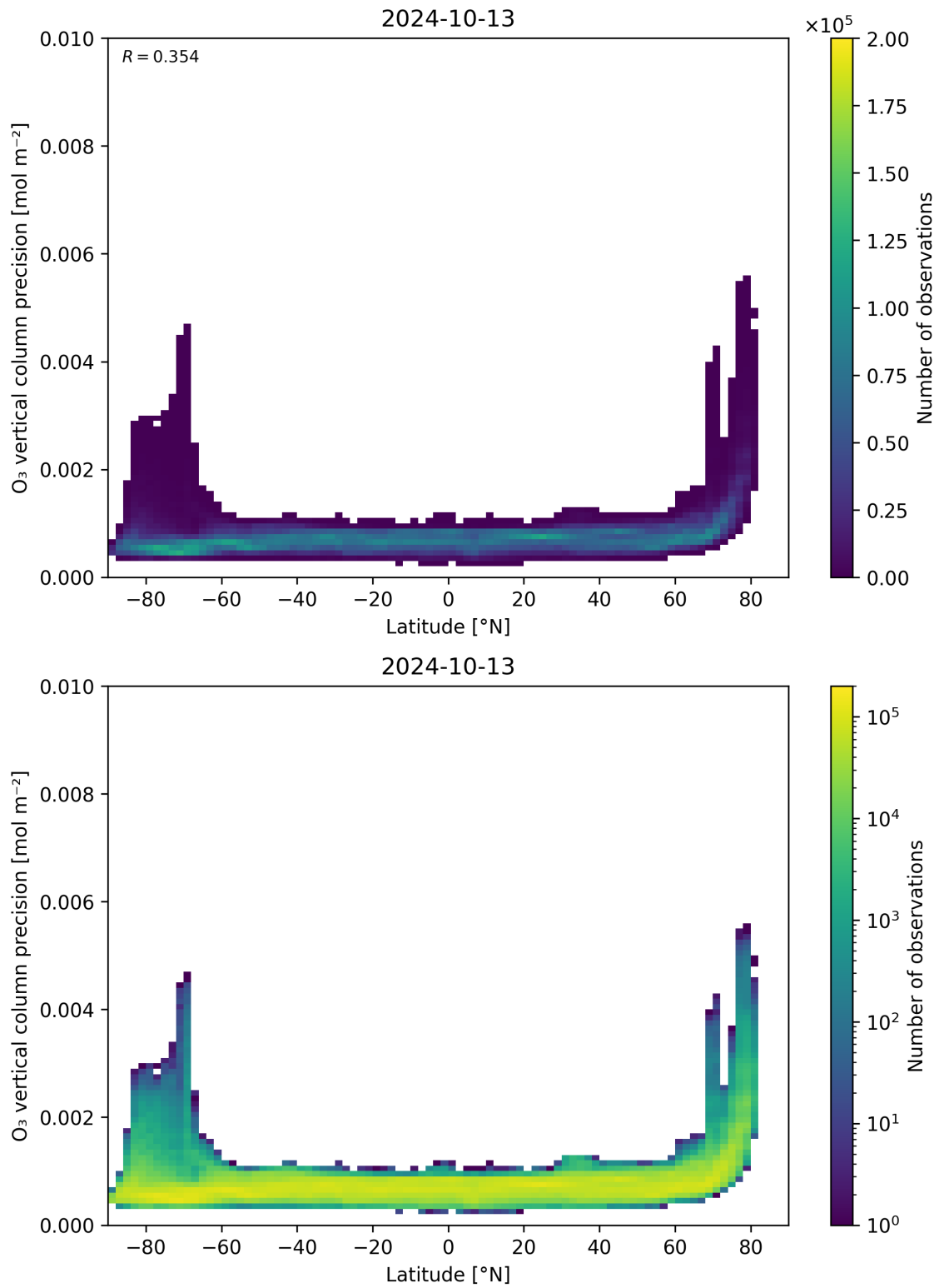
Figure 37: Scatter density plot of “Latitude” against “O 3 vertical column precision” for 2024-10-12 to 2024-10-14.
