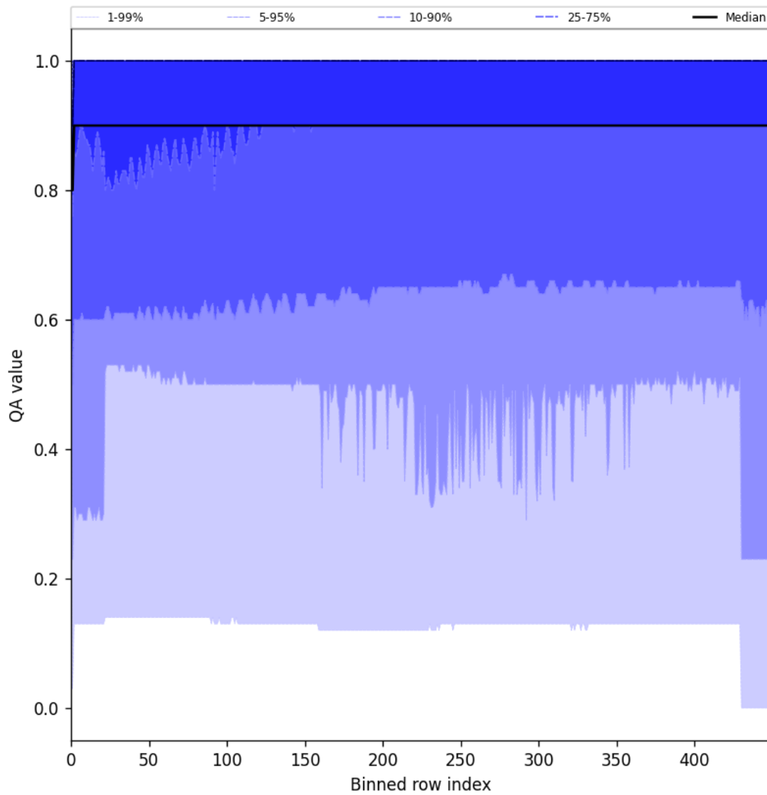
Figure 27: Along track statistics of “QA value” for 2024-10-12 to 2024-10-14
