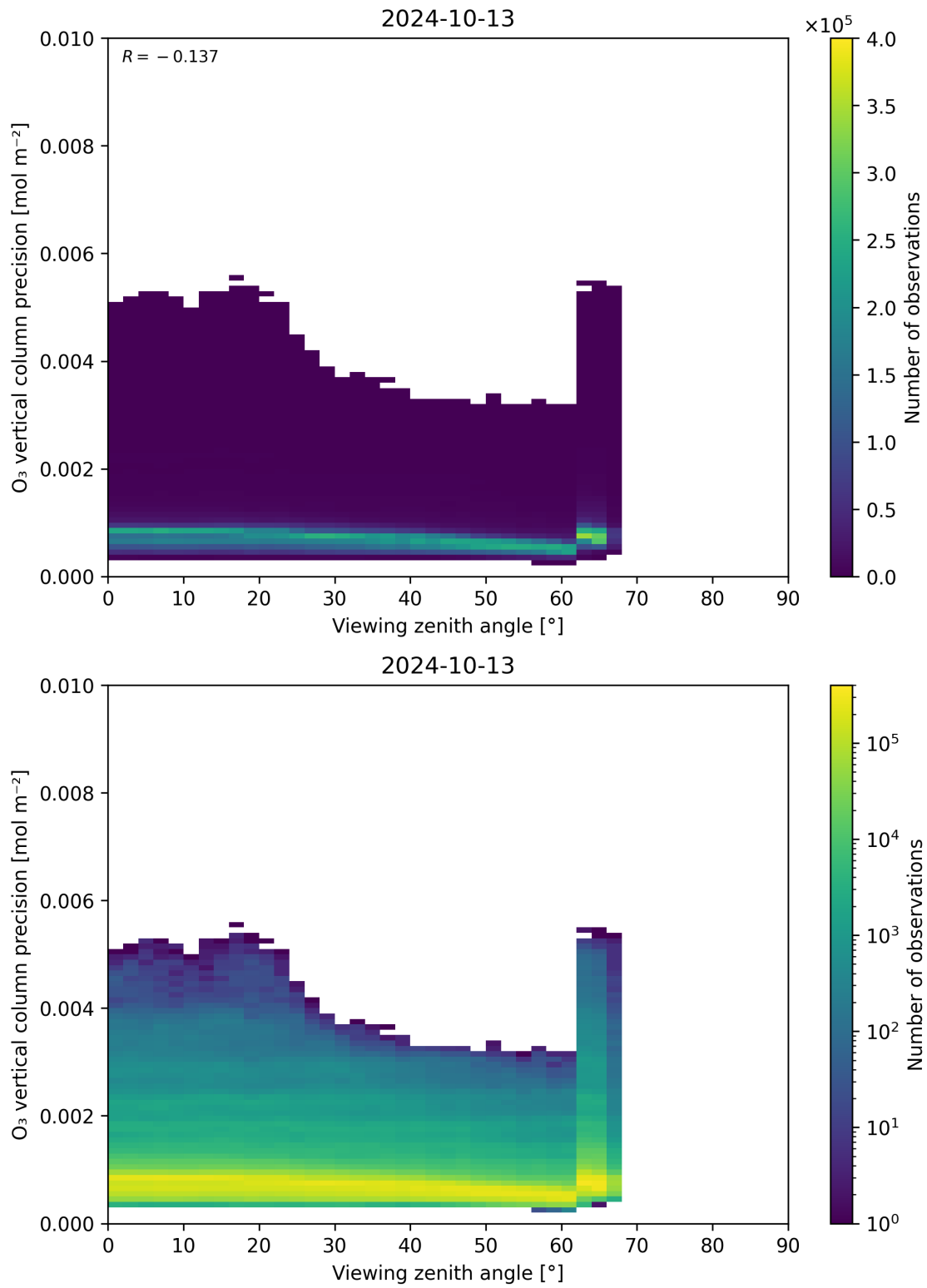
Figure 53: Scatter density plot of “Viewing zenith angle” against “O 3 vertical column precision” for 2024-10-12 to 2024-10-14.
