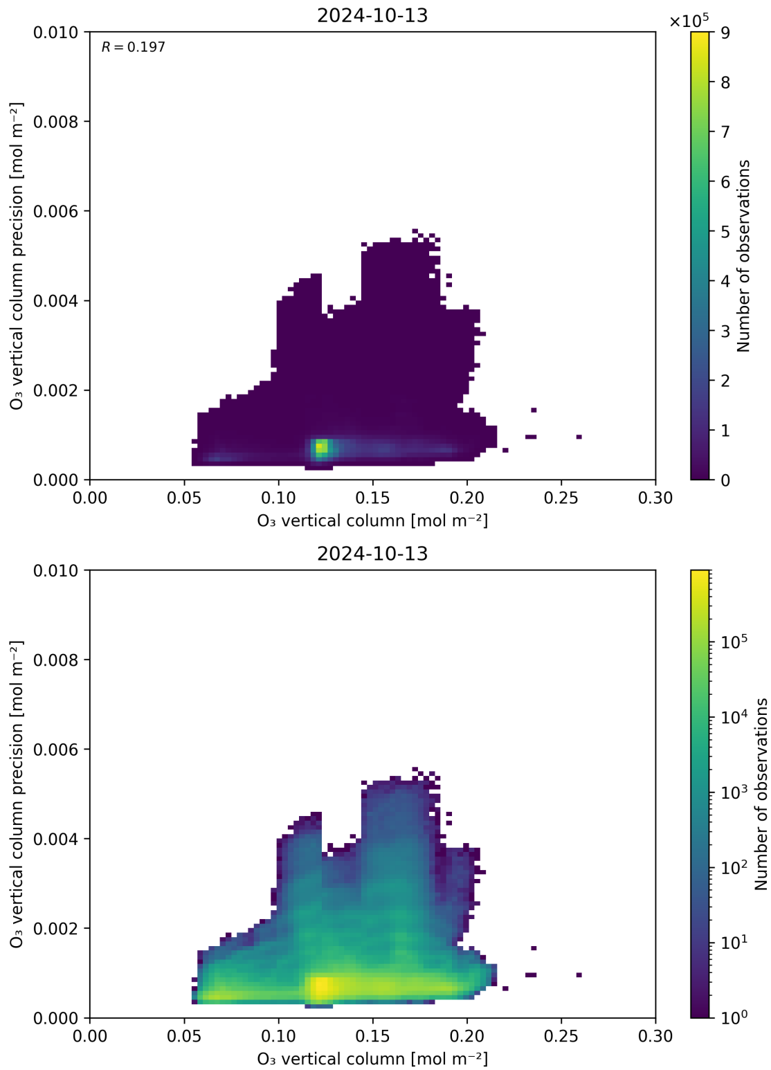
Figure 41: Scatter density plot of “O 3 vertical column” against “O 3 vertical column precision” for 2024-10-12 to 2024-10-14.
