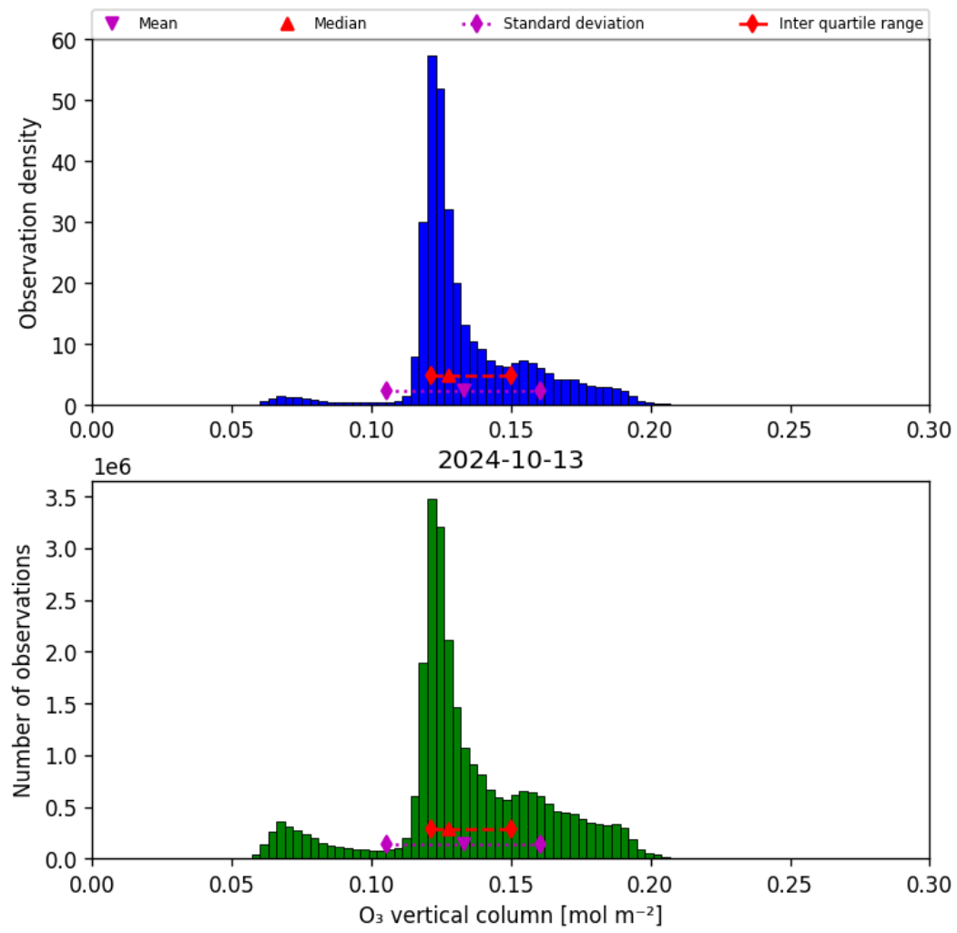
Figure 21: Histogram of “O 3 vertical column” for 2024-10-12 to 2024-10-14
