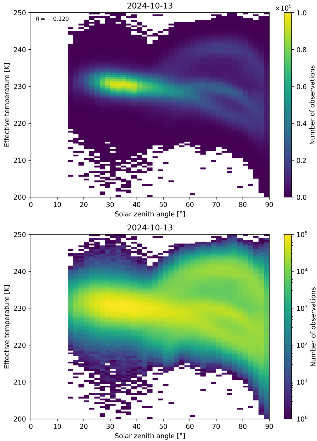
Figure 45: Scatter density plot of “Solar zenith angle” against “Effective temperature” for 2024-10-12 to 2024-10-14.
