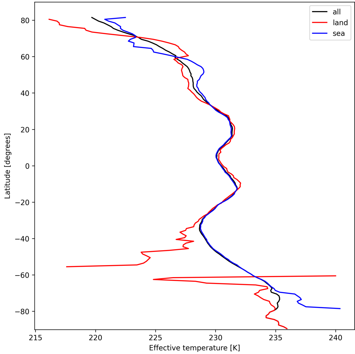
Figure 17: Zonal average of “Effective temperature” for 2024-10-12 to 2024-10-14.
