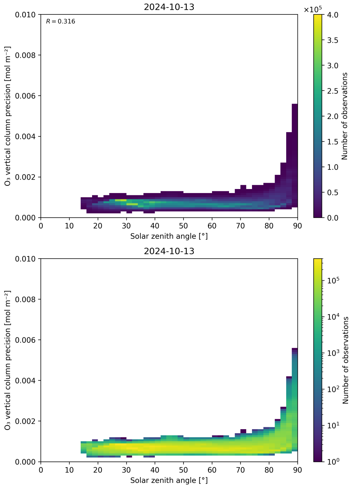
Figure 48: Scatter density plot of “Solar zenith angle” against “O 3 vertical column precision” for 2024-10-12 to 2024-10-14.
