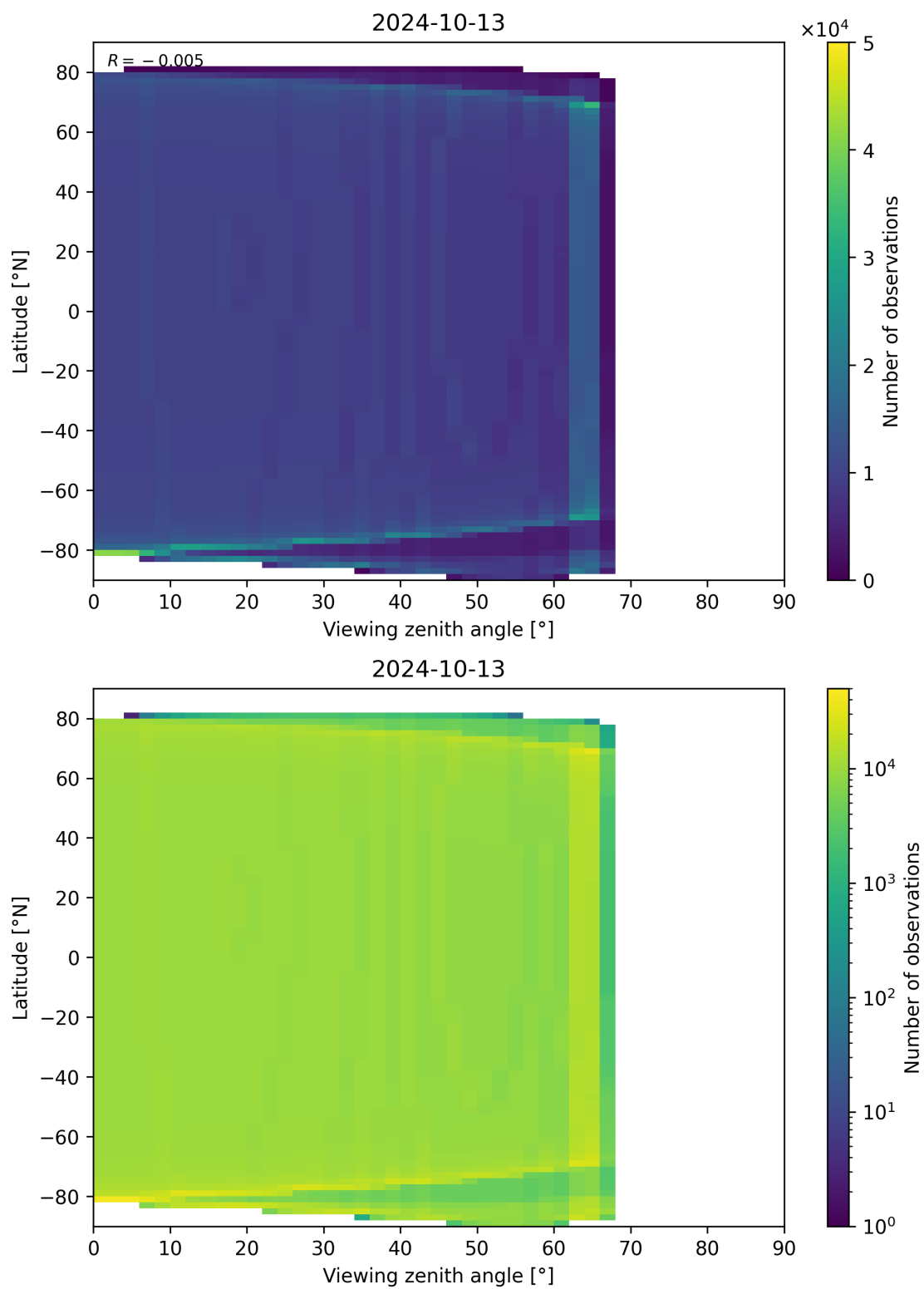
Figure 49: Scatter density plot of “Viewing zenith angle” against “Latitude” for 2024-10-12 to 2024-10-14.
