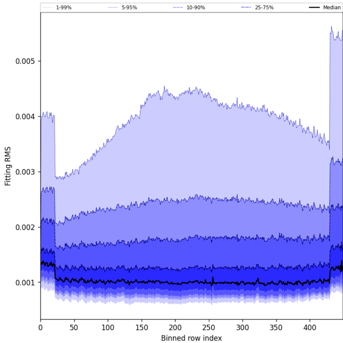
Figure 30: Along track statistics of “Fitting RMS” for 2024-10-12 to 2024-10-14
