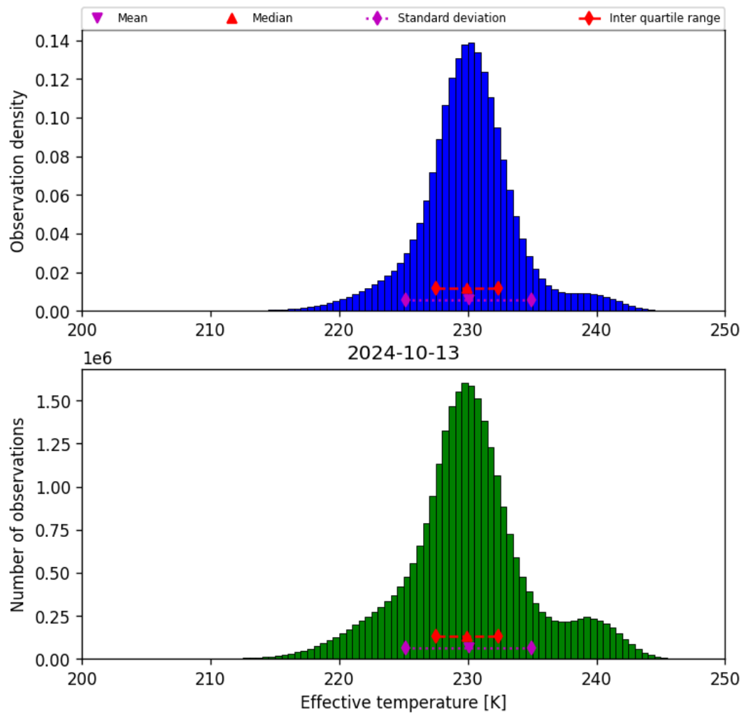
Figure 24: Histogram of “Effective temperature” for 2024-10-12 to 2024-10-14
