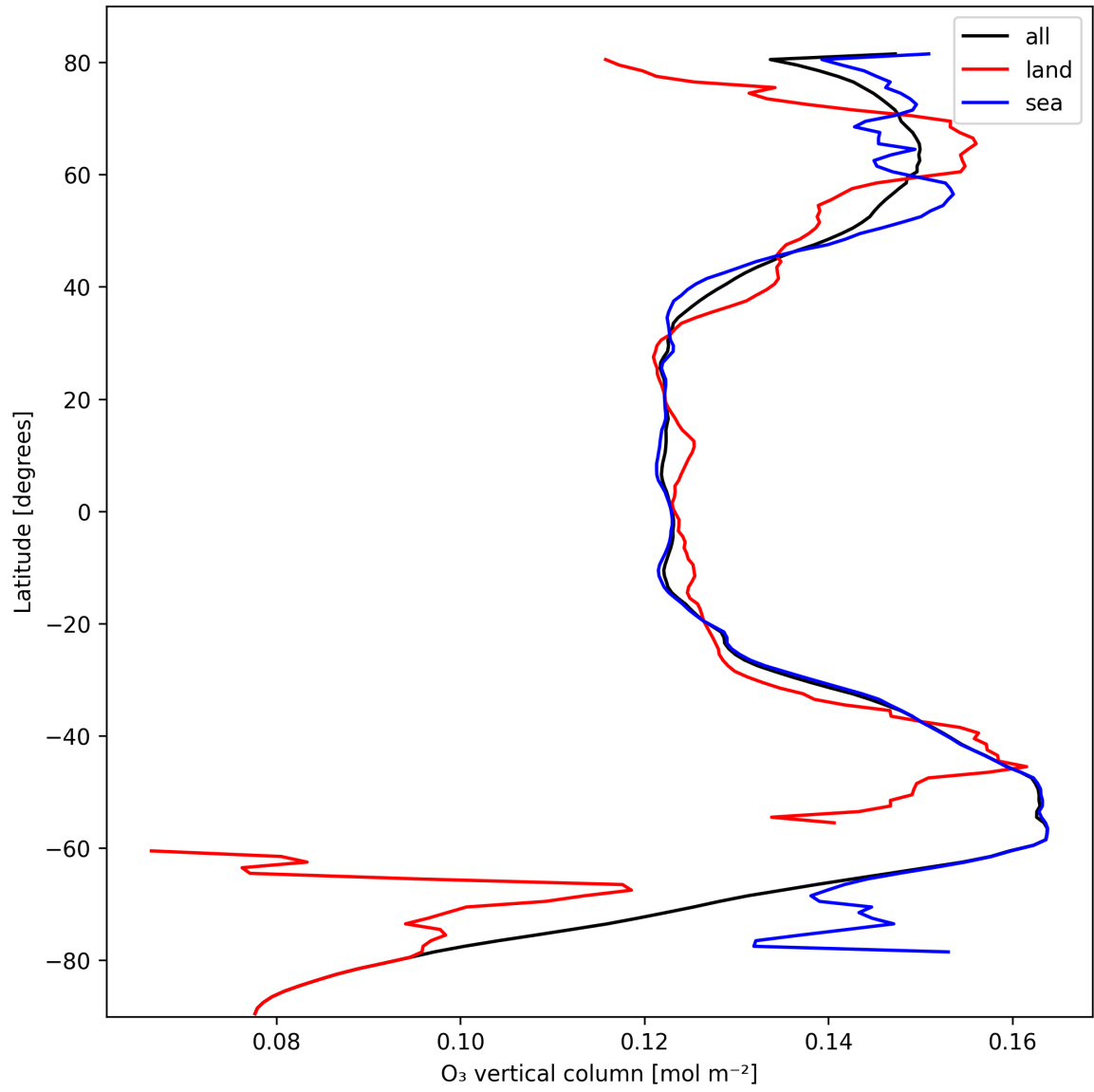
Figure 14: Zonal average of “O 3 vertical column” for 2024-10-12 to 2024-10-14.
