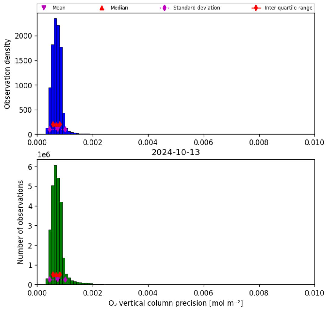
Figure 22: Histogram of “O 3 vertical column precision” for 2024-10-12 to 2024-10-14
