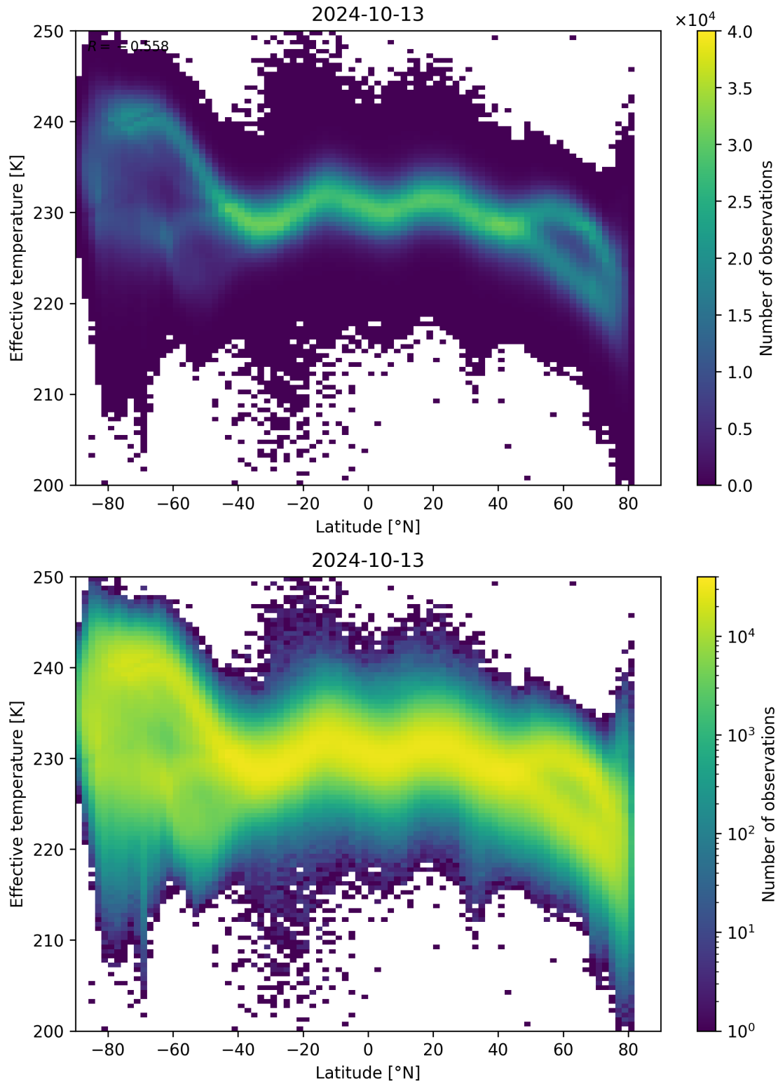
Figure 34: Scatter density plot of “Latitude” against “Effective temperature” for 2024-10-12 to 2024-10-14.
