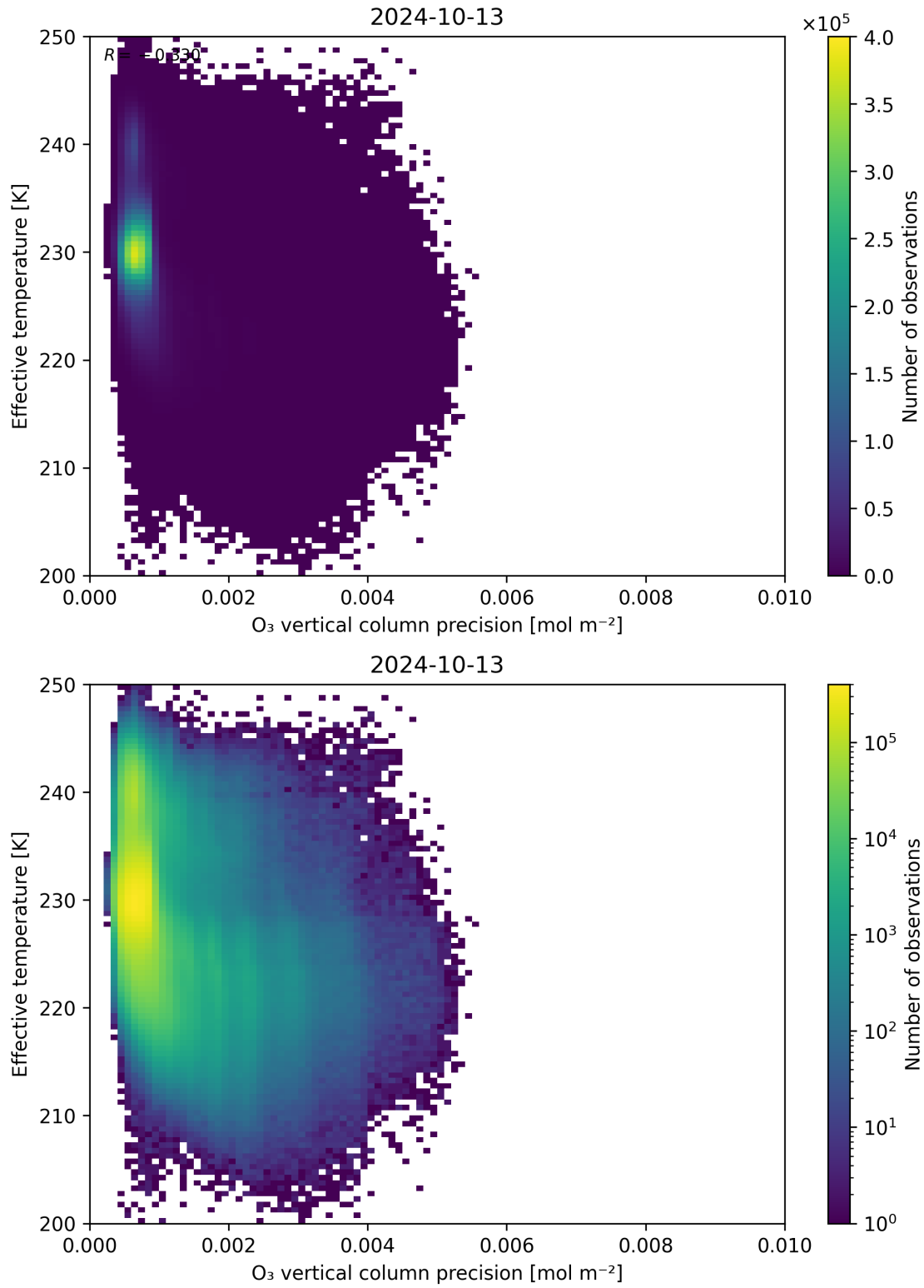
Figure 42: Scatter density plot of “ O_3 vertical column precision” against “Effective temperature” for 2024-10-12 to 2024-10-14.
