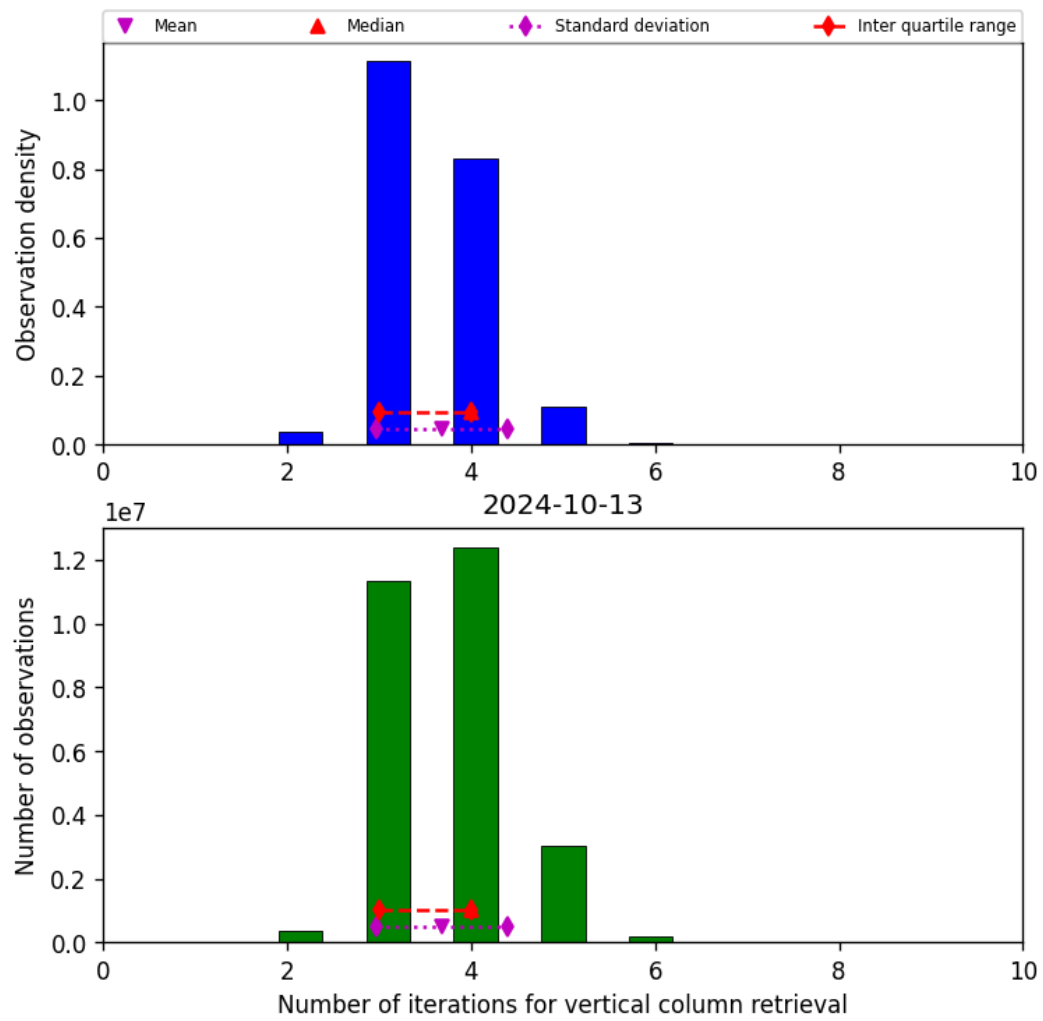
Figure 26: Histogram of “Number of iterations for vertical column retrieval” for 2024-10-12 to 2024-10-14
