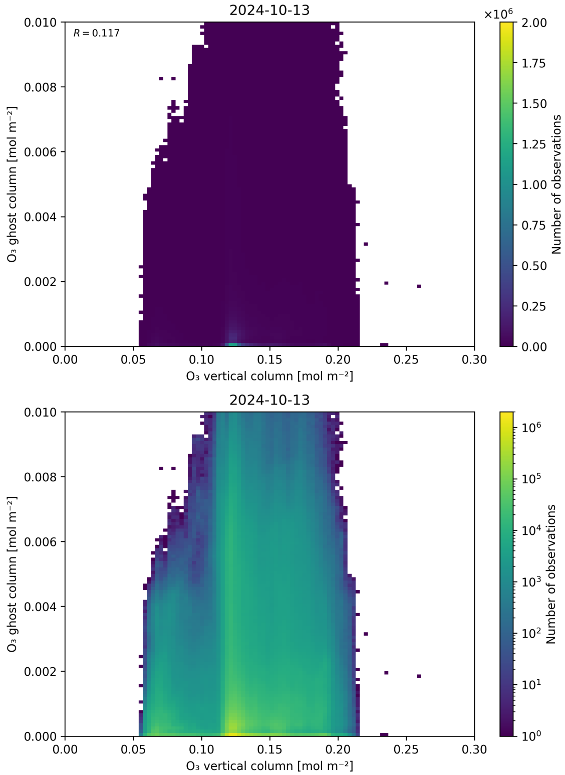
Figure 40: Scatter density plot of “O 3 vertical column” against “O 3 ghost column” for 2024-10-12 to 2024-10-14.
