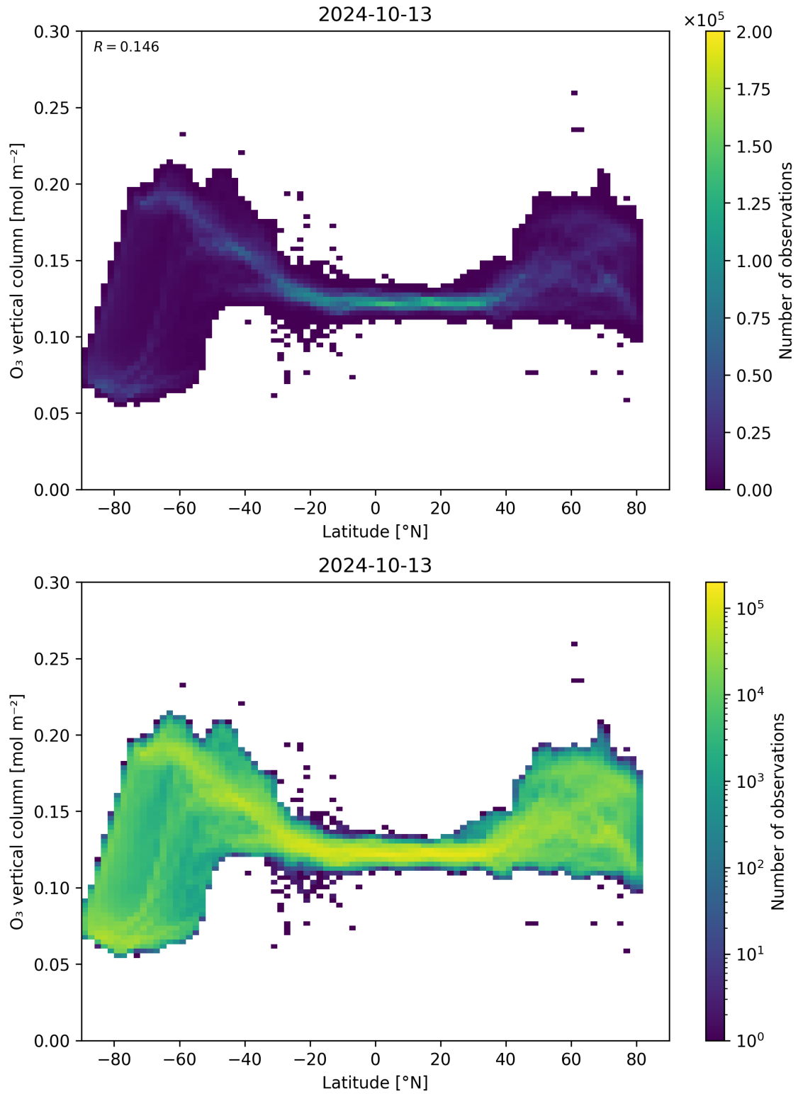
Figure 36: Scatter density plot of “Latitude” against “O 3 vertical column” for 2024-10-12 to 2024-10-14.
