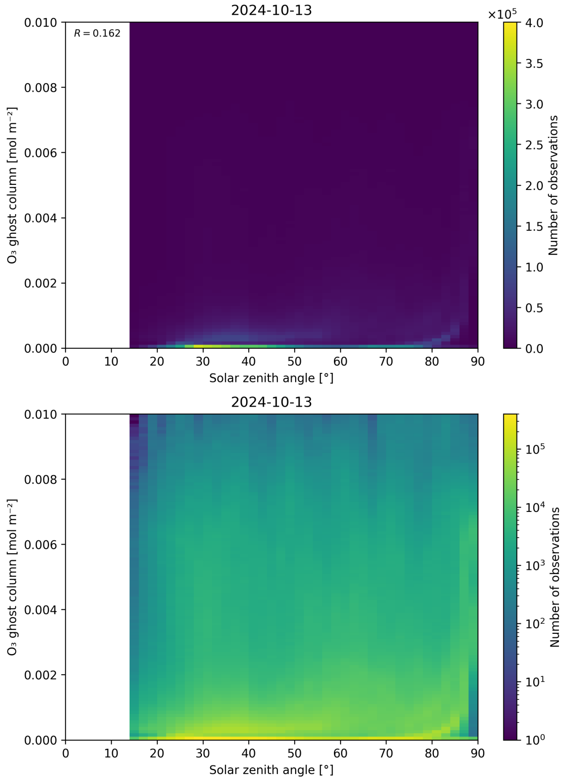
Figure 46: Scatter density plot of “Solar zenith angle” against “O 3 ghost column” for 2024-10-12 to 2024-10-14.
