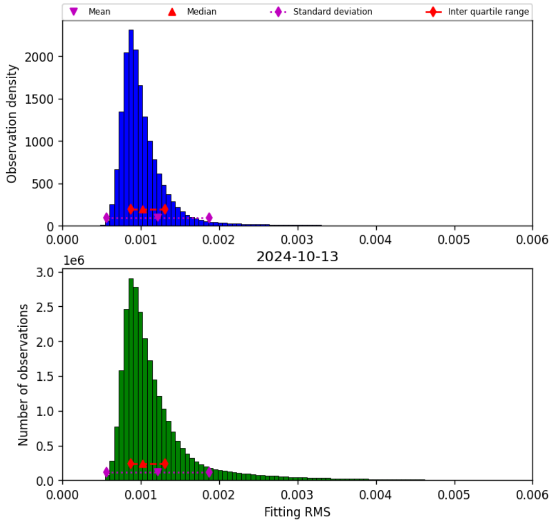
Figure 23: Histogram of “Fitting RMS” for 2024-10-12 to 2024-10-14
