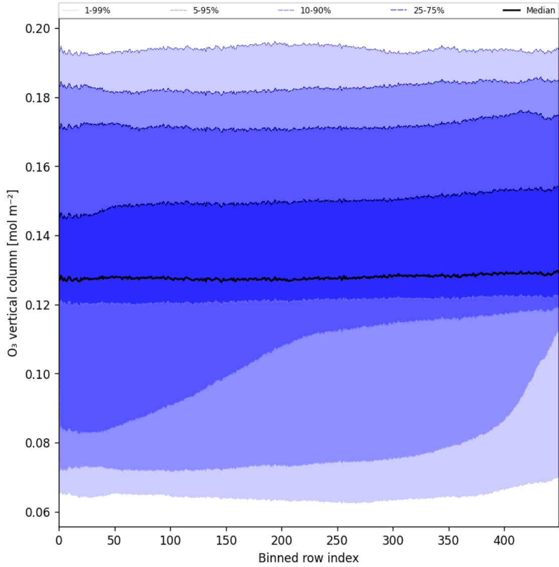
Figure 28: Along track statistics of “O 3 vertical column” for 2024-10-12 to 2024-10-14
