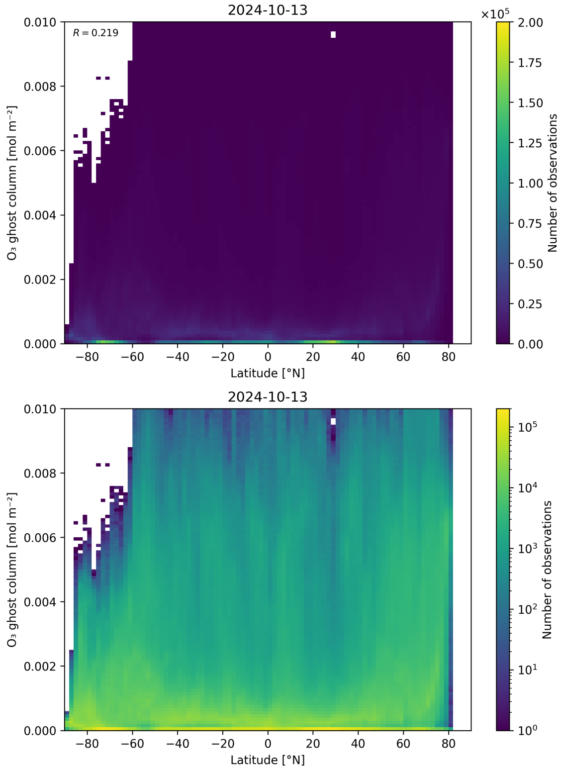
Figure 35: Scatter density plot of “Latitude” against “O 3 ghost column” for 2024-10-12 to 2024-10-14.
