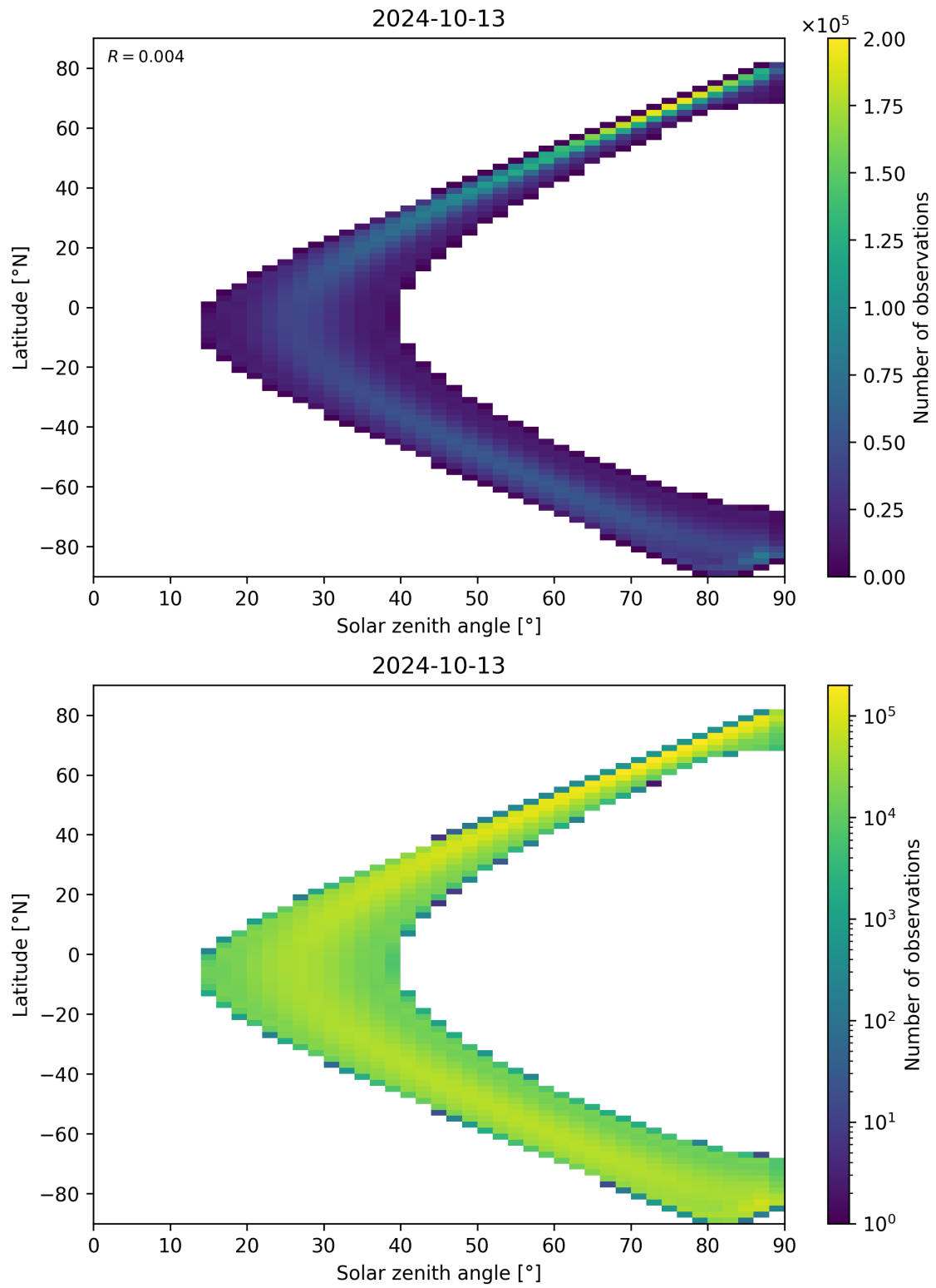
Figure 44: Scatter density plot of “Solar zenith angle” against “Latitude” for 2024-10-12 to 2024-10-14.
