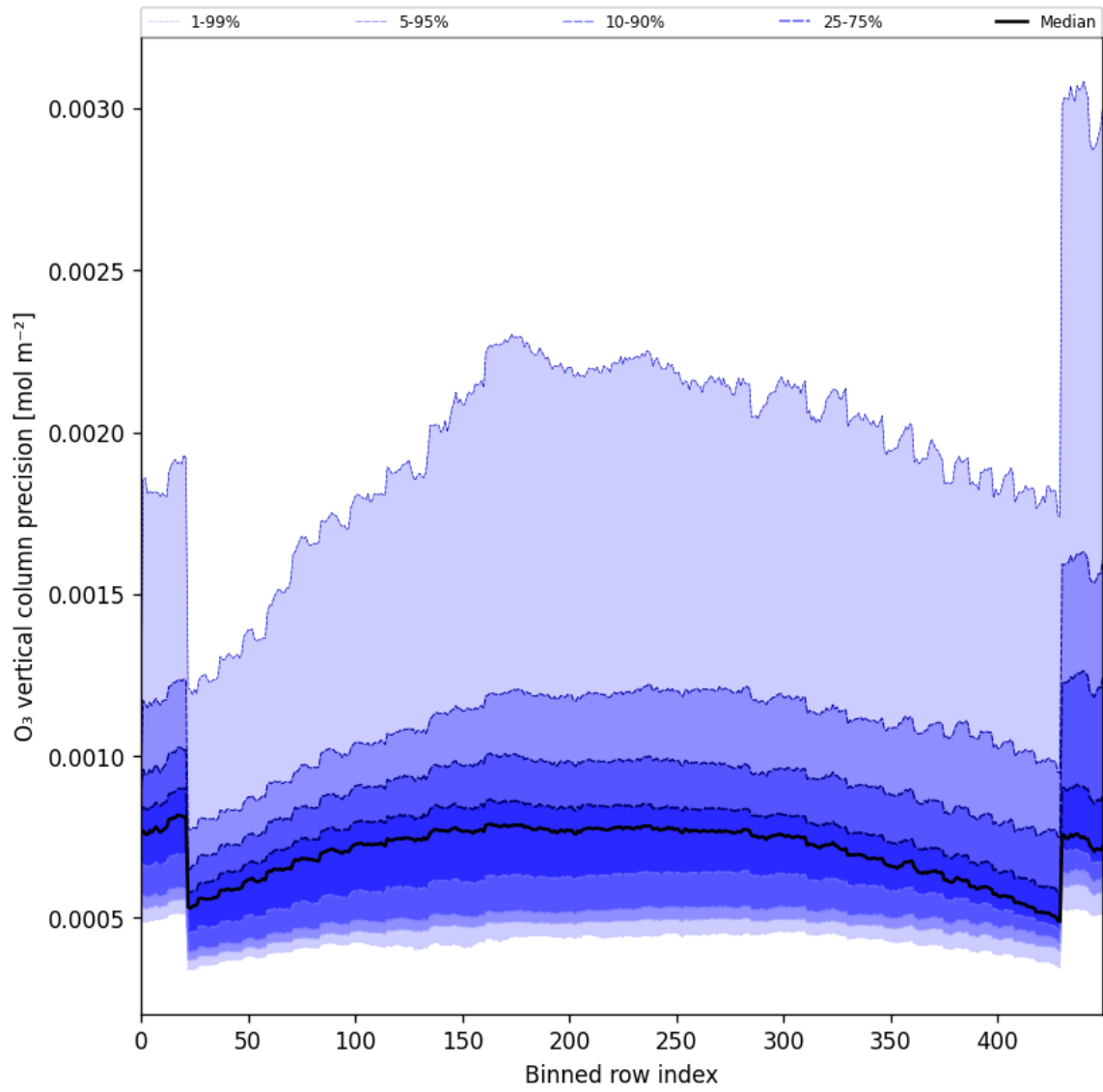
Figure 29: Along track statistics of “O 3 vertical column precision” for 2024-10-12 to 2024-10-14
