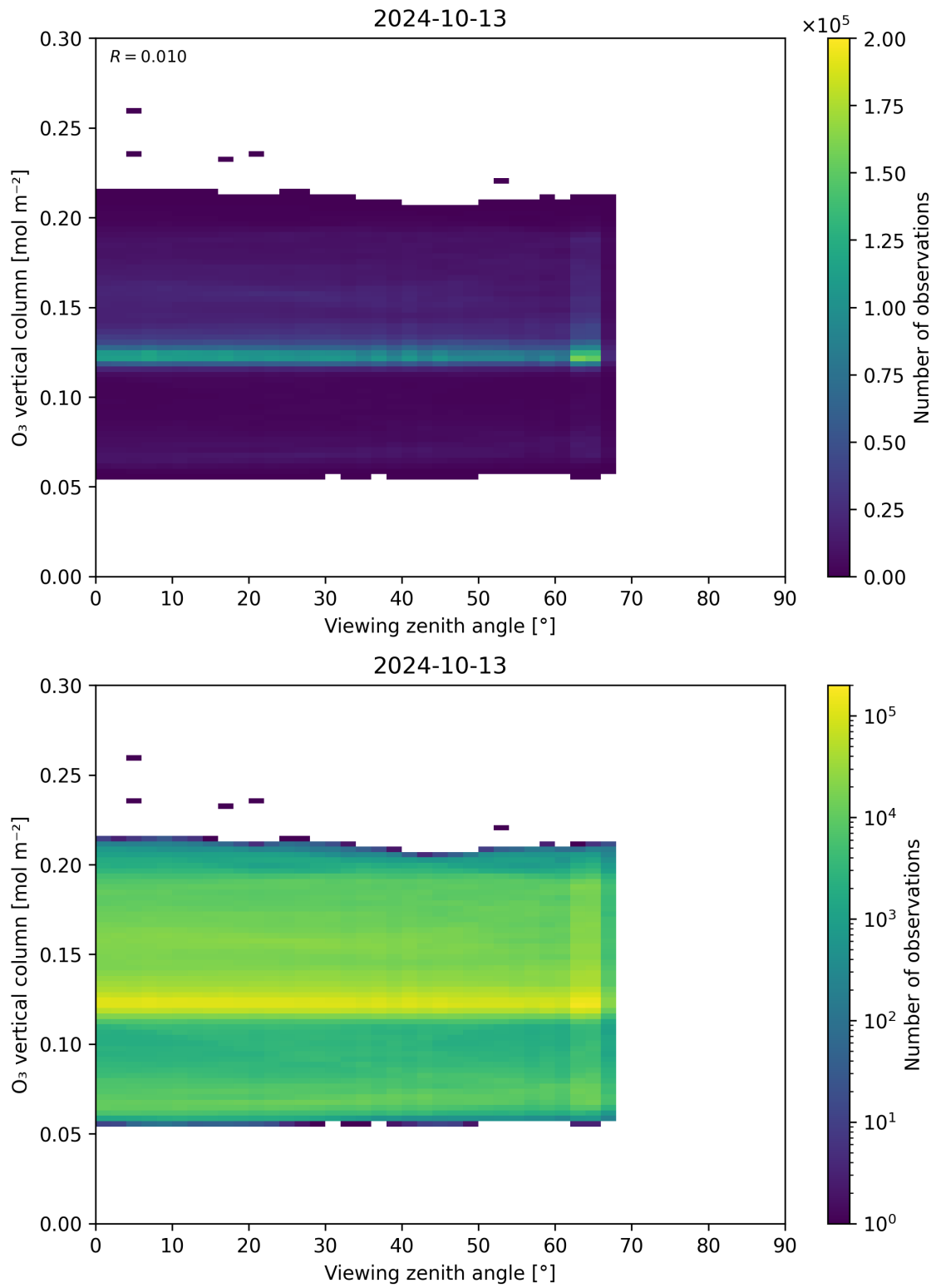
Figure 52: Scatter density plot of “Viewing zenith angle” against “O 3 vertical column” for 2024-10-12 to 2024-10-14.
