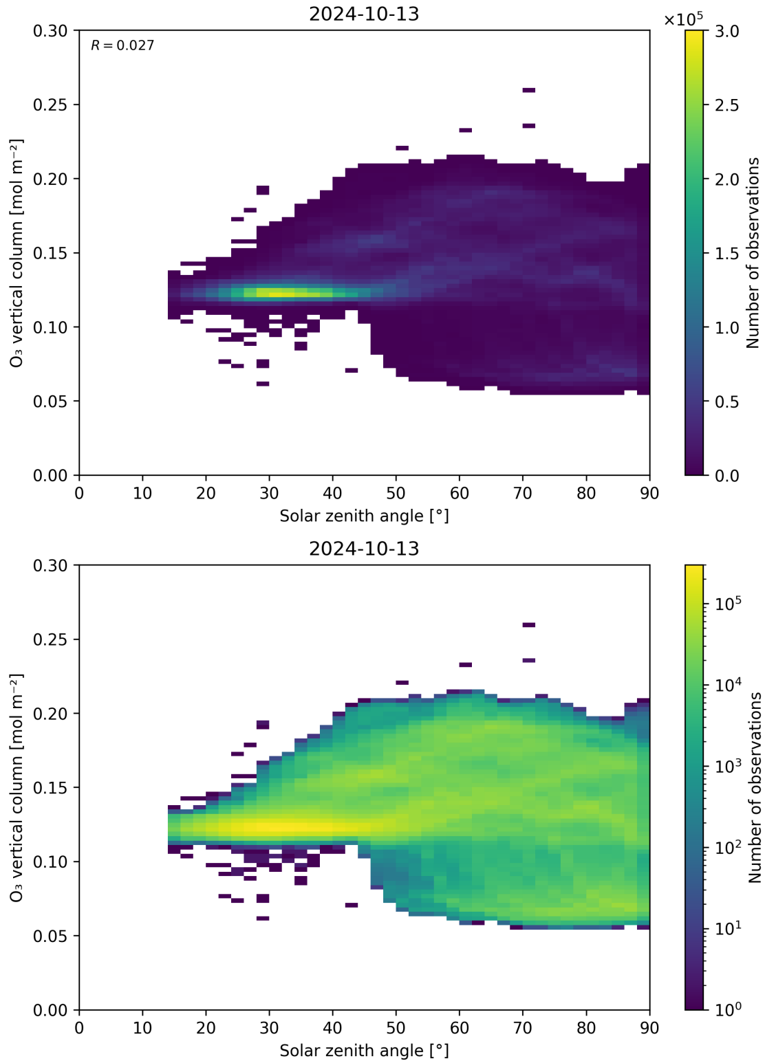
Figure 47: Scatter density plot of “Solar zenith angle” against “O 3 vertical column” for 2024-10-12 to 2024-10-14.
