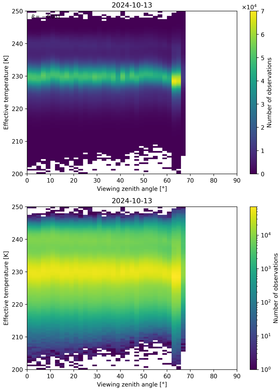
Figure 50: Scatter density plot of “Viewing zenith angle” against “Effective temperature” for 2024-10-12 to 2024-10-14.
