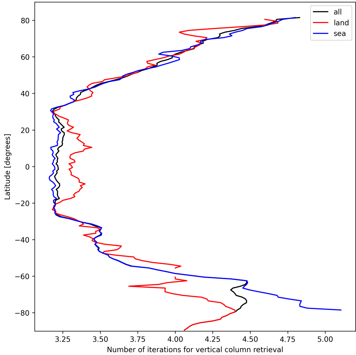
Figure 19: Zonal average of “Number of iterations for vertical column retrieval” for 2024-10-12 to 2024-10-14.
