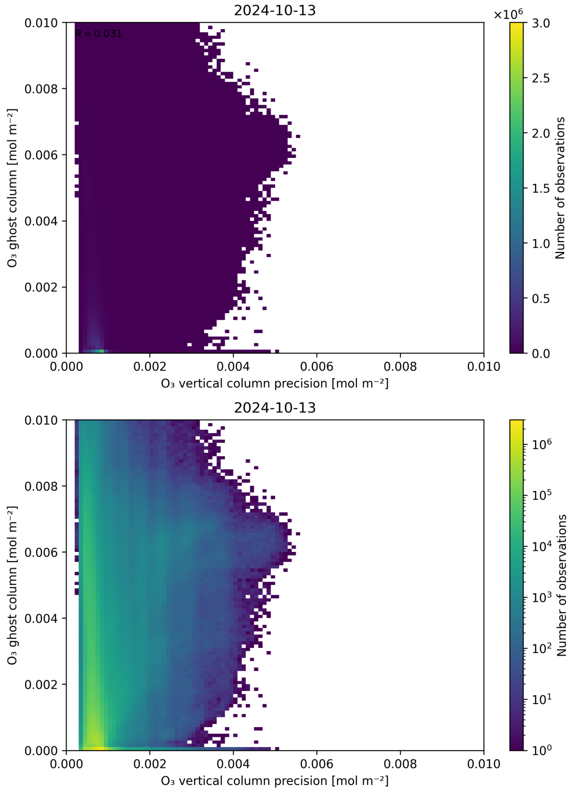
Figure 43: Scatter density plot of “ \text{O}_3 vertical column precision” against “ \text{O}_3 ghost column” for 2024-10-12 to 2024-10-14.
