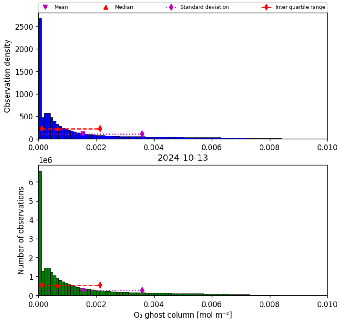
Figure 25: Histogram of “O 3 ghost column” for 2024-10-12 to 2024-10-14
