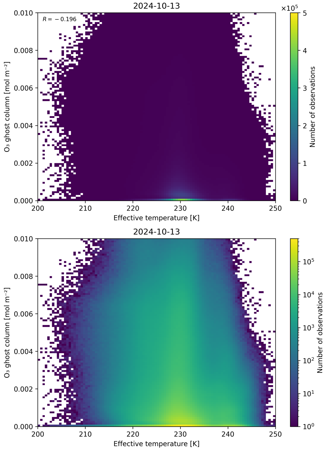
Figure 38: Scatter density plot of “Effective temperature” against “O 3 ghost column” for 2024-10-12 to 2024-10-14.
