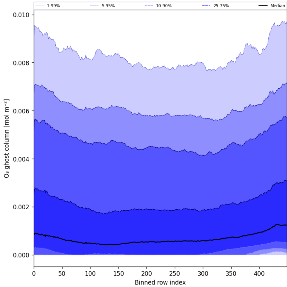
Figure 32: Along track statistics of “O 3 ghost column” for 2024-10-12 to 2024-10-14
