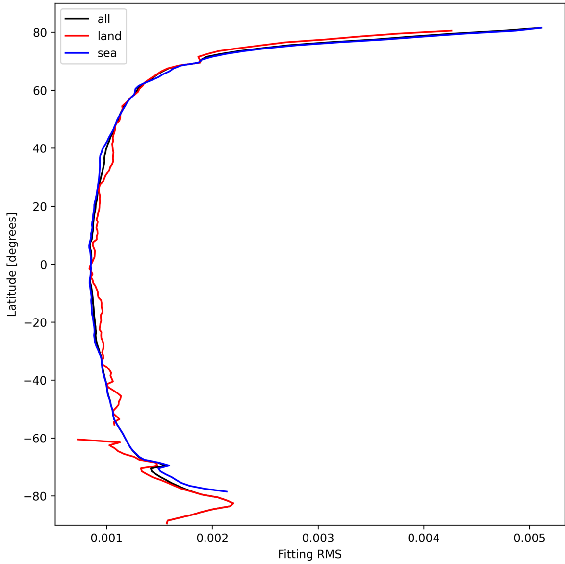
Figure 16: Zonal average of “Fitting RMS” for 2024-10-12 to 2024-10-14.
