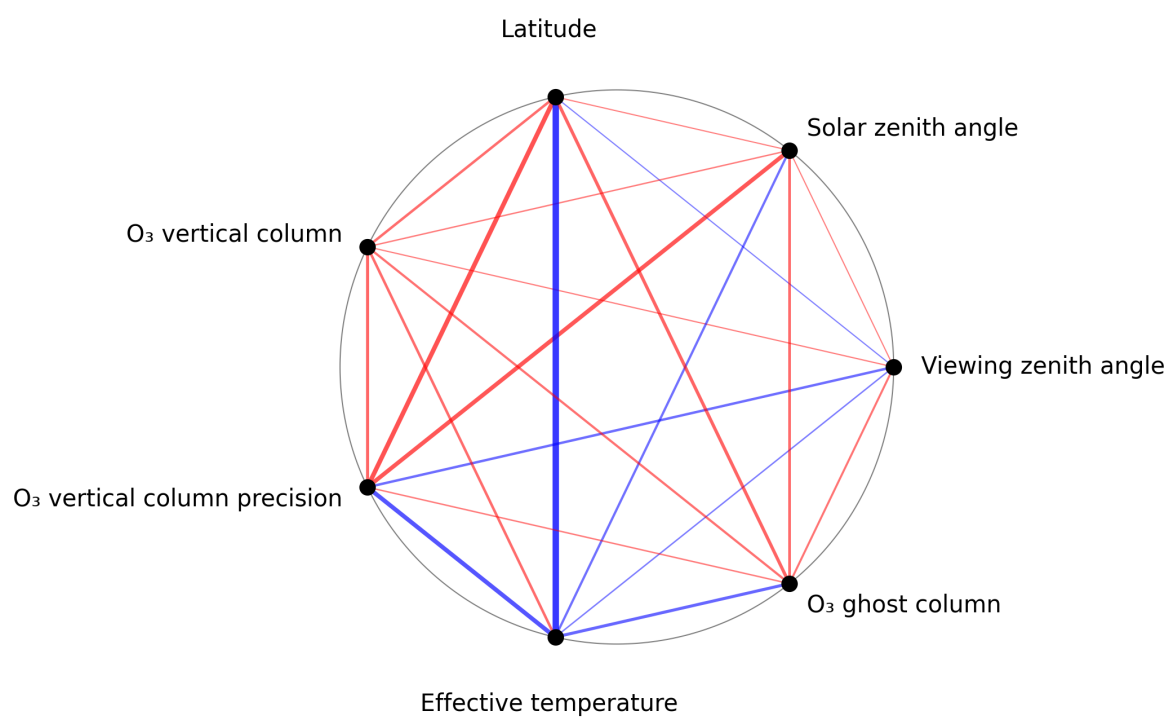
Figure 1: Map of correlation graph for 2024-10-12 to 2024-10-14.
