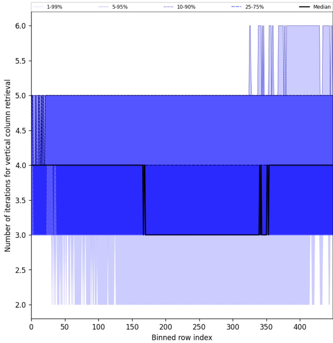
Figure 33: Along track statistics of “Number of iterations for vertical column retrieval” for 2024-10-12 to 2024-10-14
