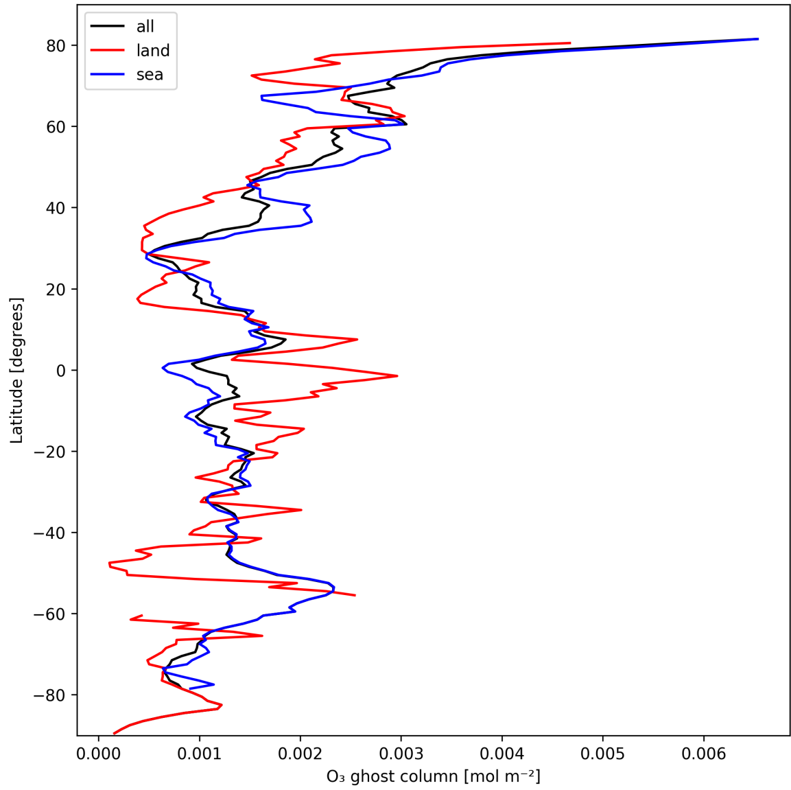
Figure 18: Zonal average of "O 3 ghost column" for 2024-10-12 to 2024-10-14.
