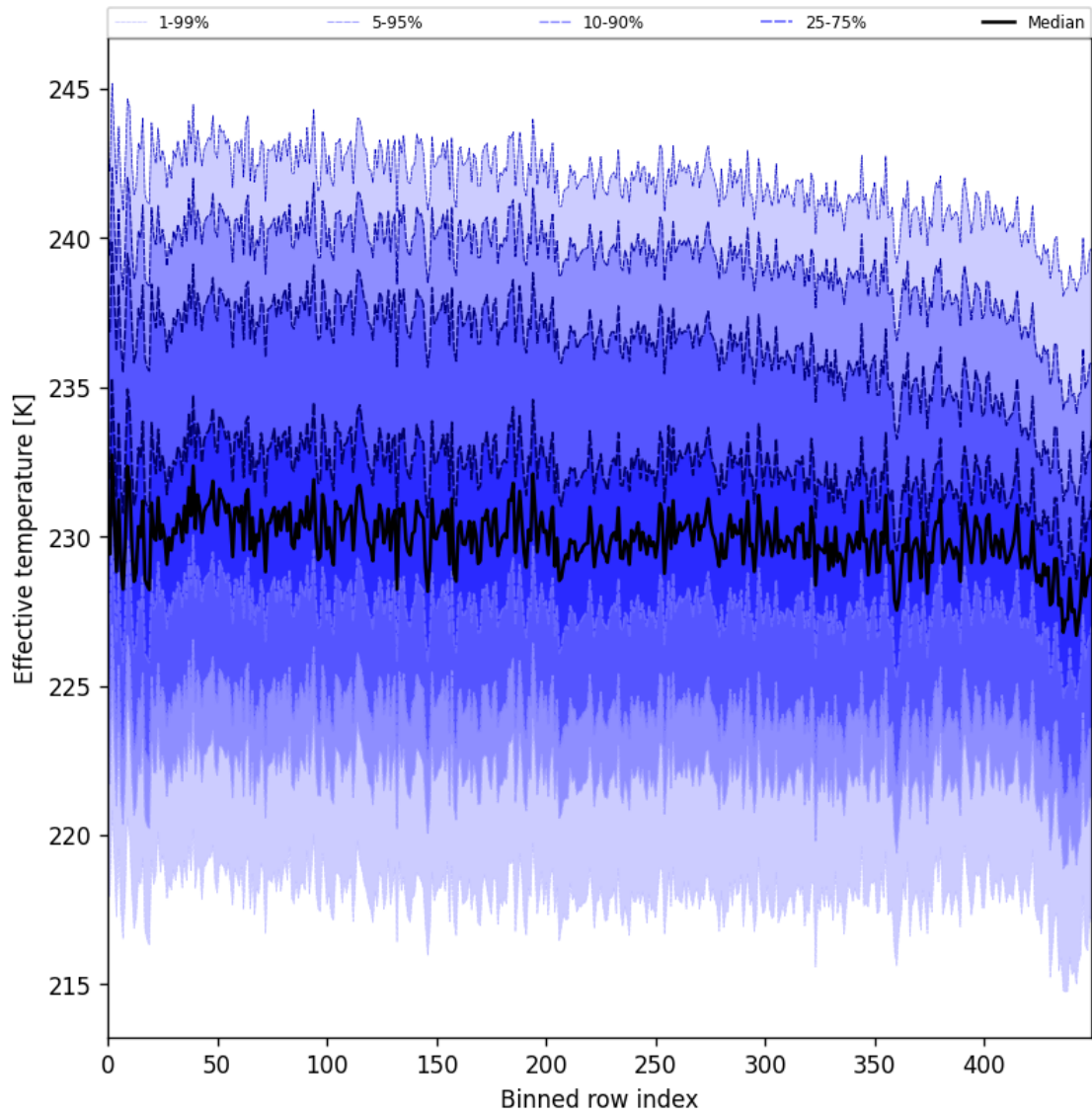
Figure 31: Along track statistics of “Effective temperature” for 2024-10-12 to 2024-10-14
