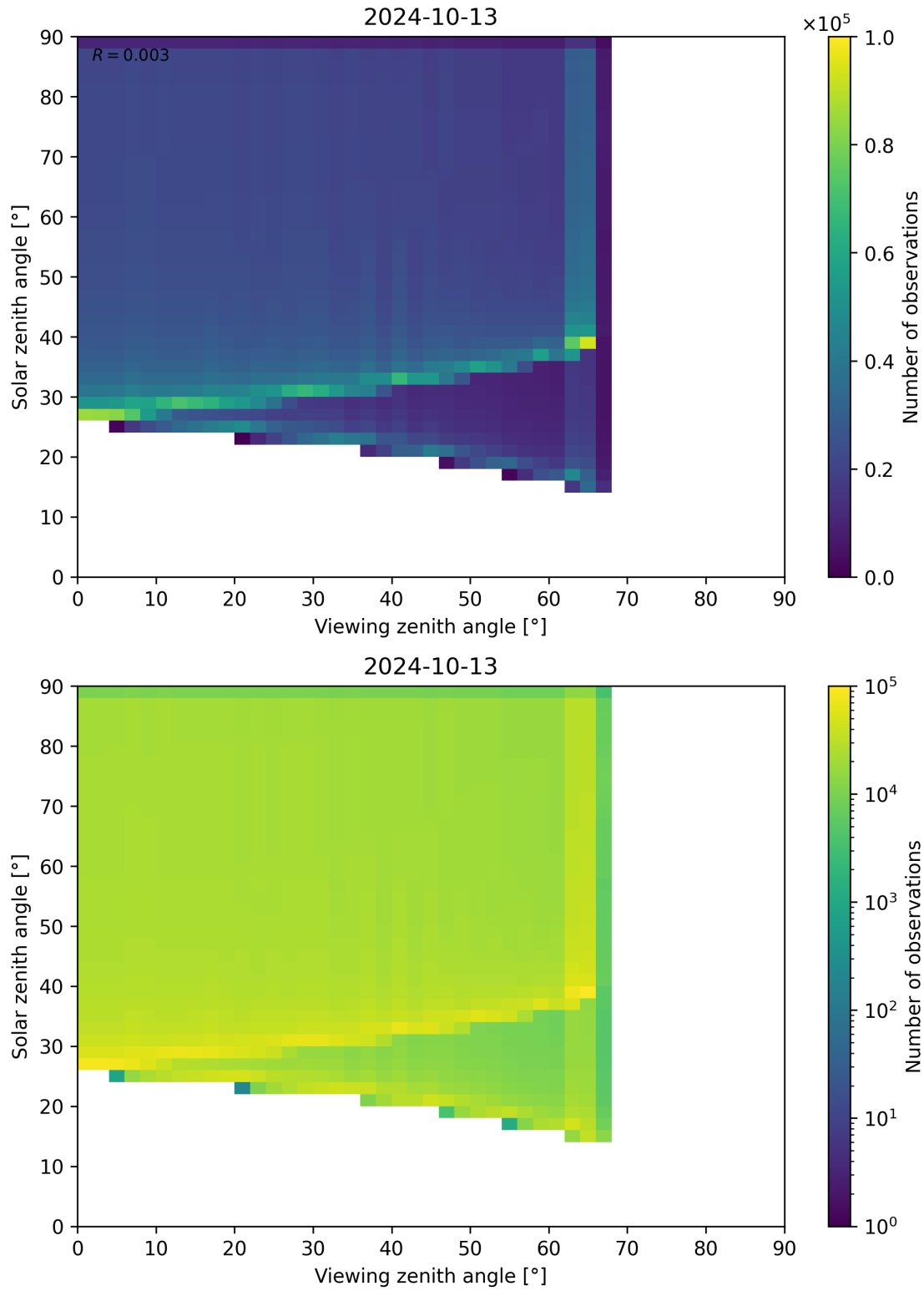
Figure 54: Scatter density plot of “Viewing zenith angle” against “Solar zenith angle” for 2024-10-12 to 2024-10-14.
