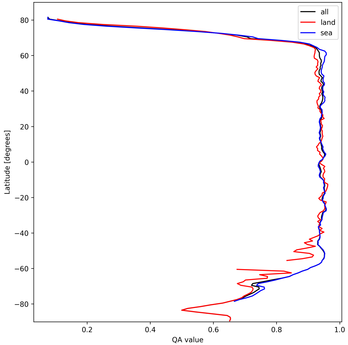
Figure 13: Zonal average of “QA value” for 2024-10-12 to 2024-10-14.
