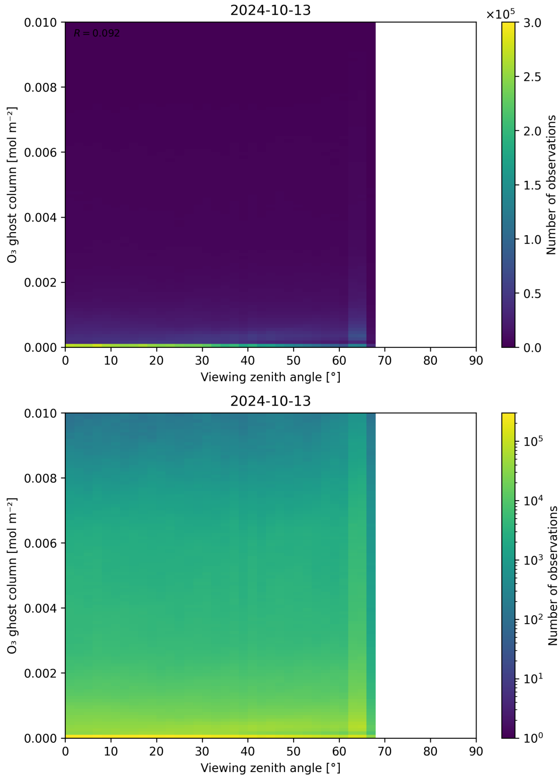
Figure 51: Scatter density plot of “Viewing zenith angle” against “O 3 ghost column” for 2024-10-12 to 2024-10-14.
