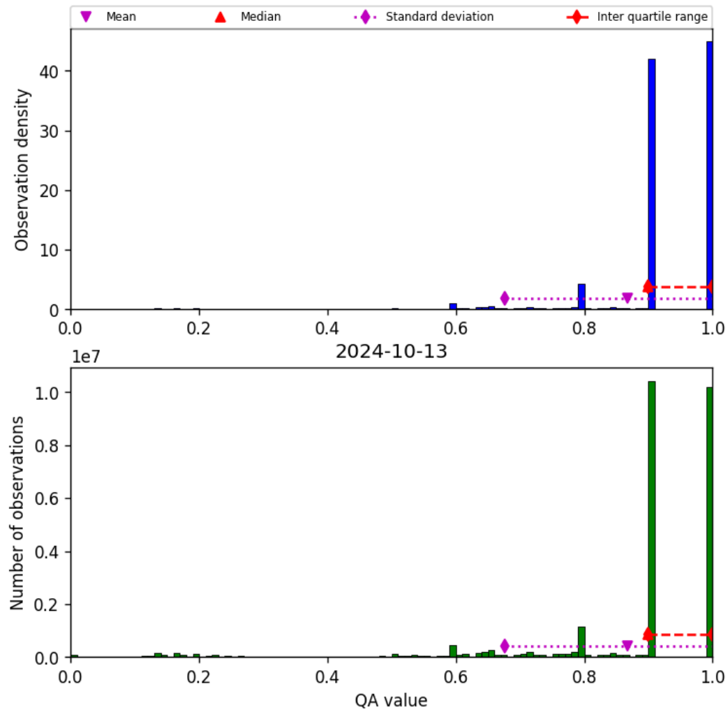
Figure 20: Histogram of “QA value” for 2024-10-12 to 2024-10-14
