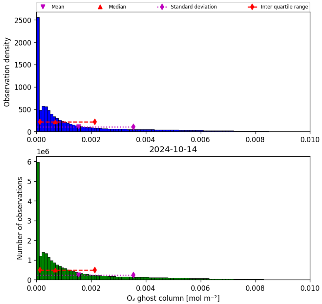
Figure 25: Histogram of “O 3 ghost column” for 2024-10-14 to 2024-10-15
