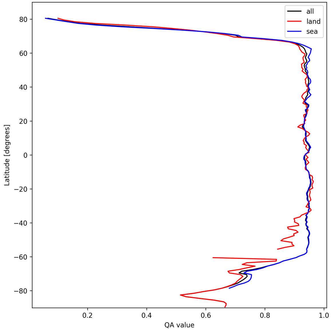
Figure 13: Zonal average of “QA value” for 2024-10-14 to 2024-10-15.
