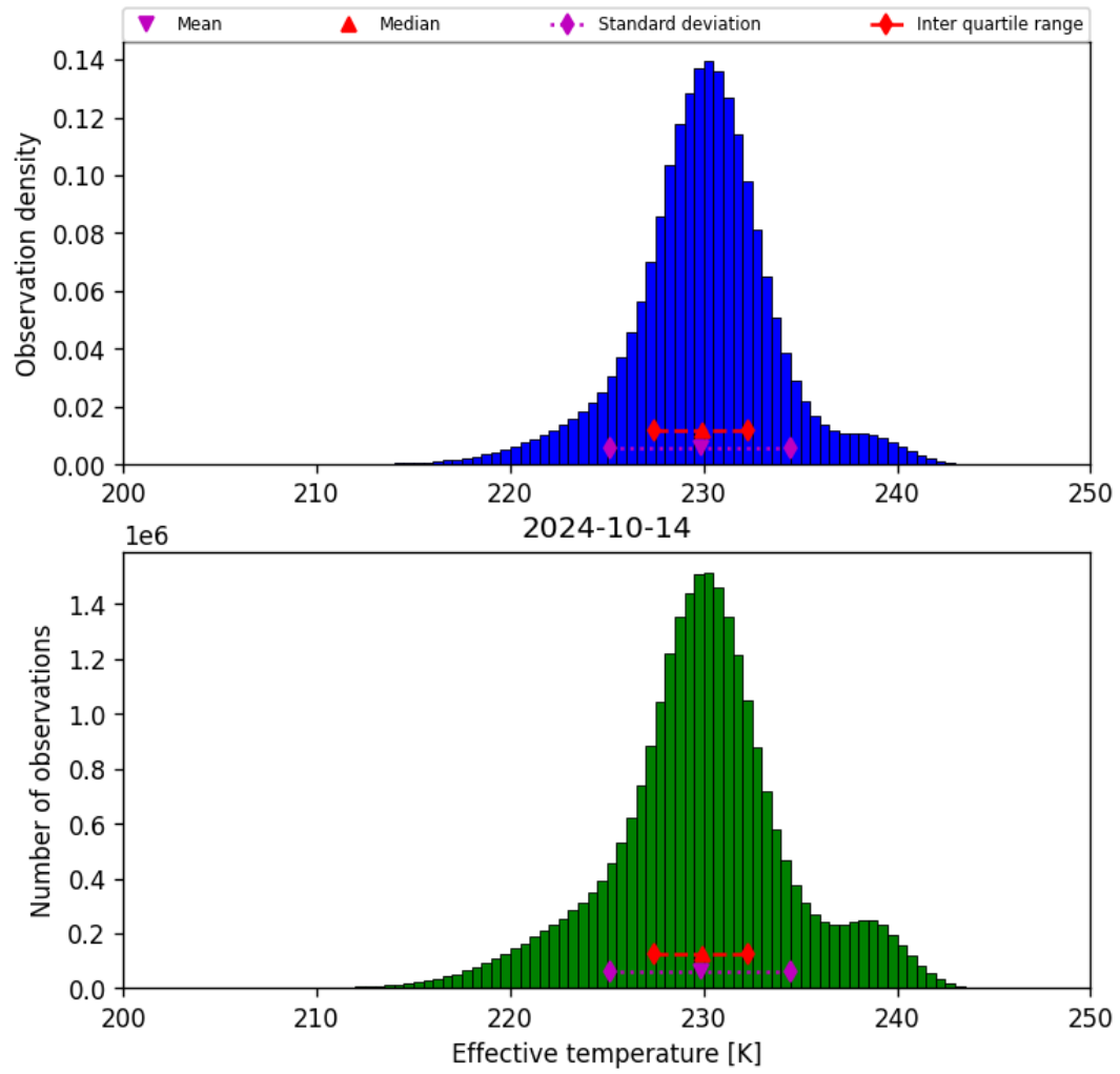
Figure 24: Histogram of “Effective temperature” for 2024-10-14 to 2024-10-15
