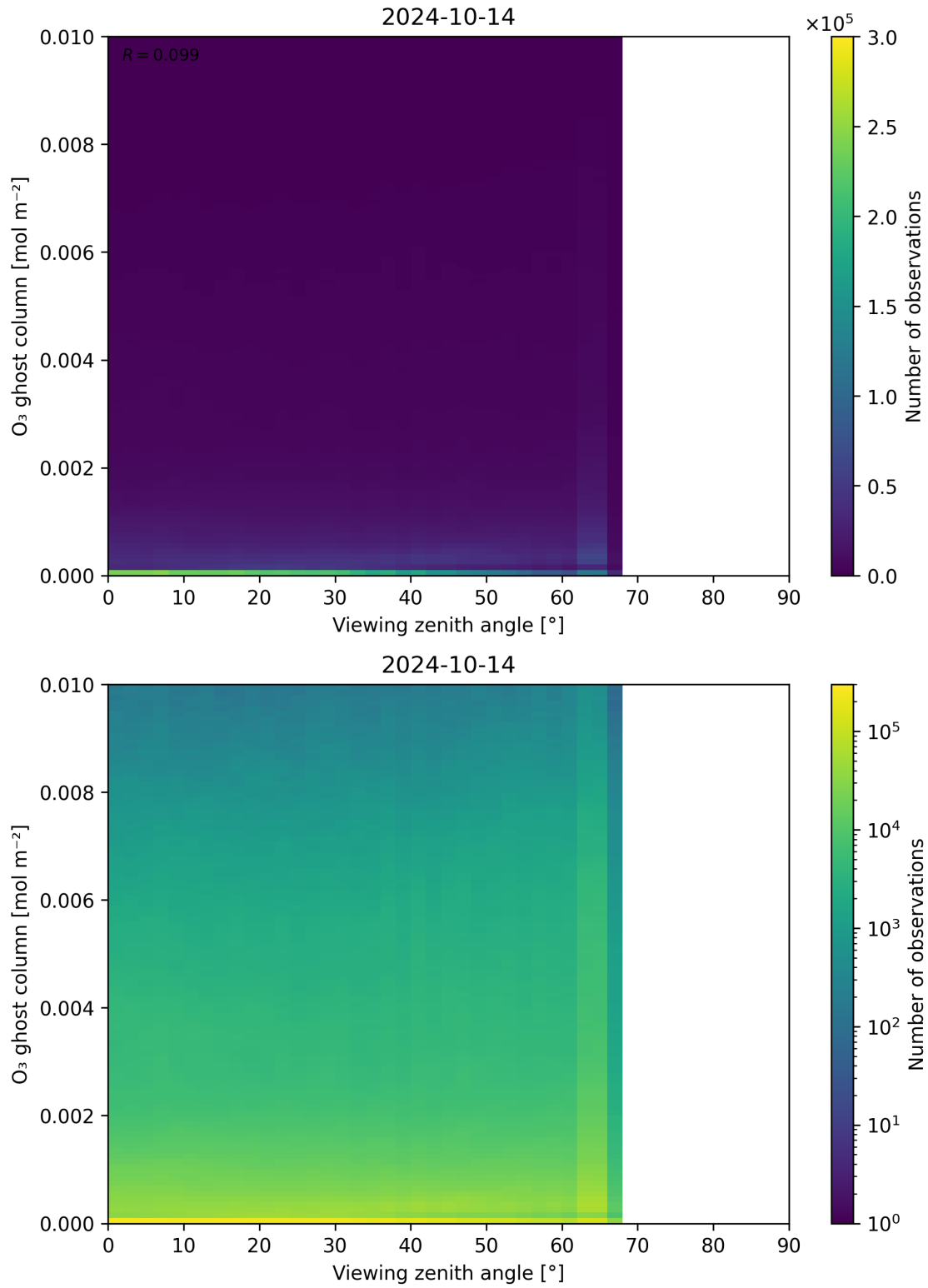
Figure 51: Scatter density plot of “Viewing zenith angle” against “O 3 ghost column” for 2024-10-14 to 2024-10-15.
