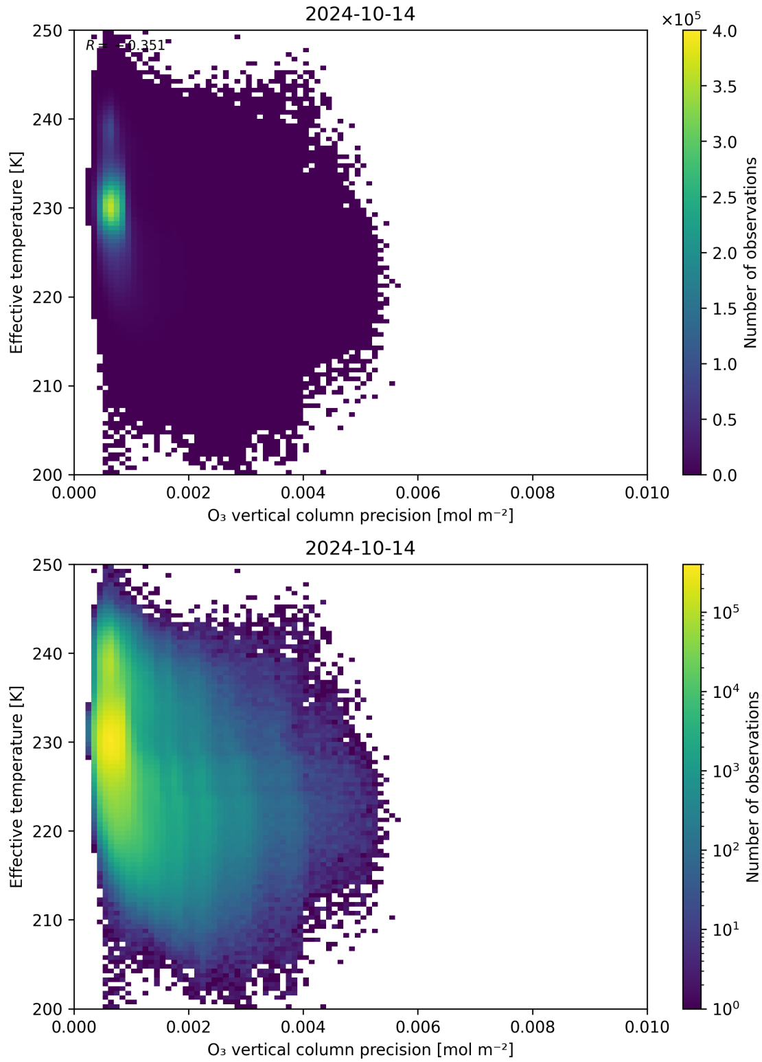
Figure 42: Scatter density plot of “O 3 vertical column precision” against “Effective temperature” for 2024-10-14 to 2024-10-15.
