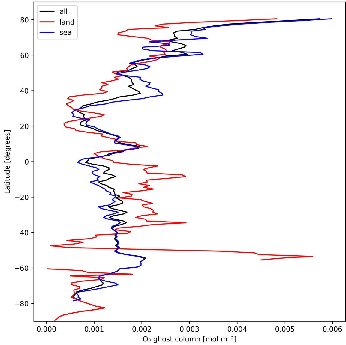
Figure 18: Zonal average of "O 3 ghost column" for 2024-10-14 to 2024-10-15.
