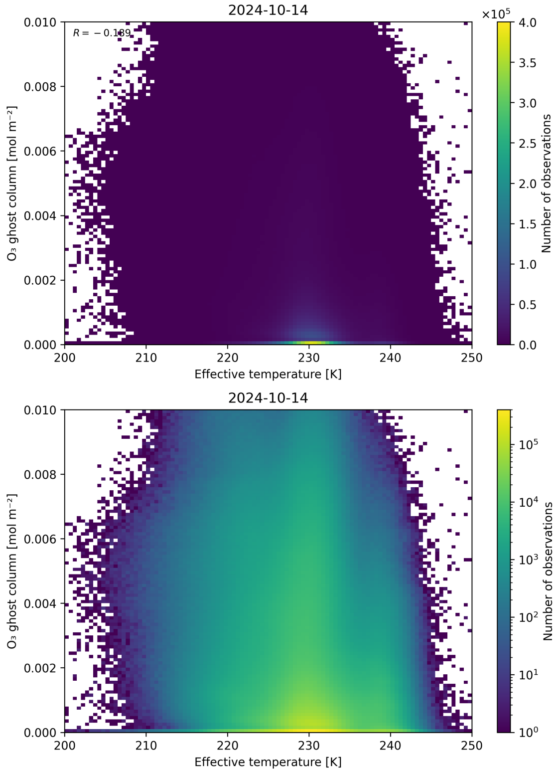
Figure 38: Scatter density plot of “Effective temperature” against “O 3 ghost column” for 2024-10-14 to 2024-10-15.
