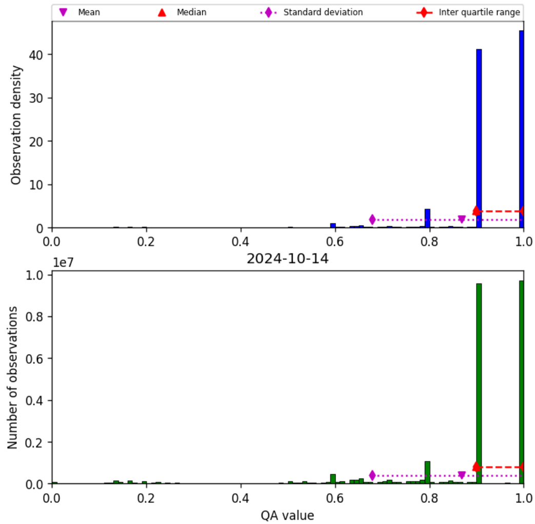
Figure 20: Histogram of “QA value” for 2024-10-14 to 2024-10-15
