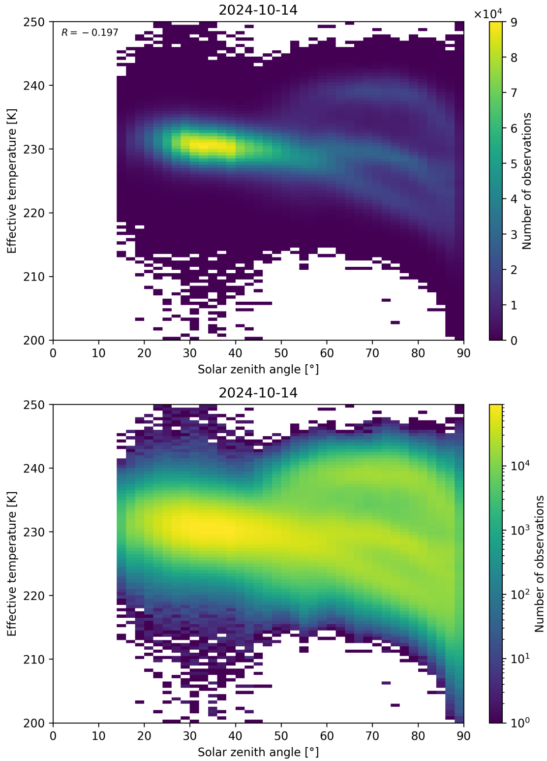
Figure 45: Scatter density plot of “Solar zenith angle” against “Effective temperature” for 2024-10-14 to 2024-10-15.
