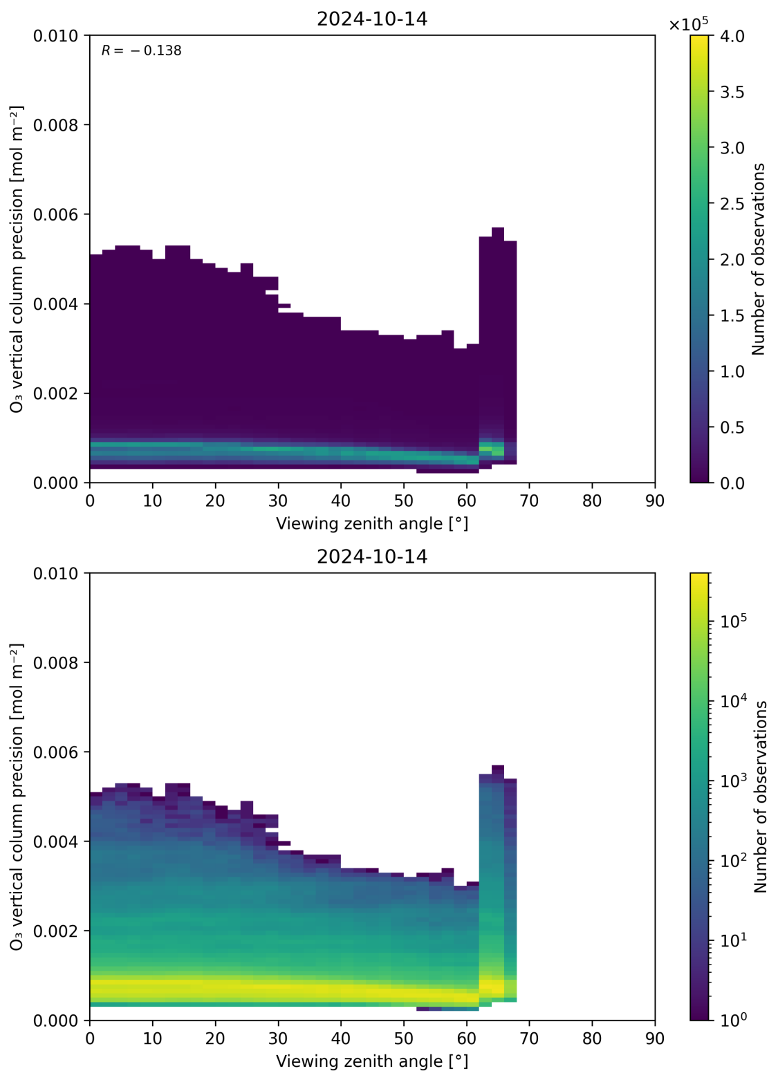
Figure 53: Scatter density plot of “Viewing zenith angle” against “O 3 vertical column precision” for 2024-10-14 to 2024-10-15.
