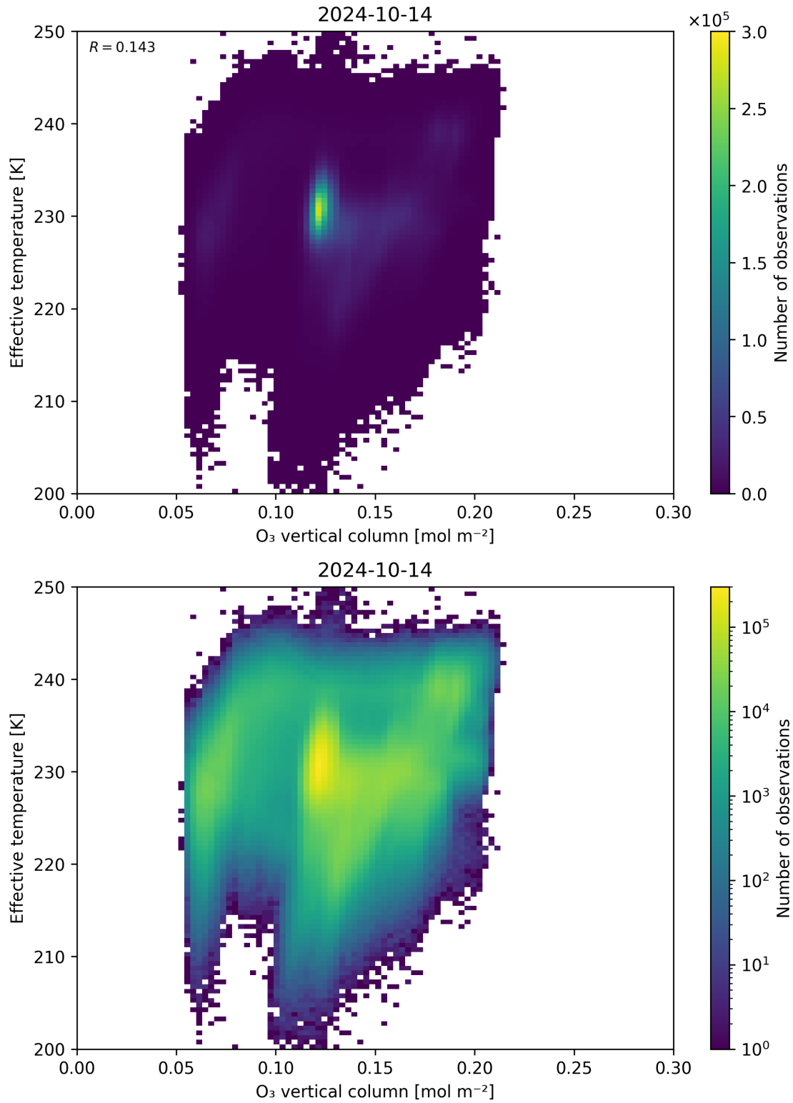
Figure 39: Scatter density plot of “O 3 vertical column” against “Effective temperature” for 2024-10-14 to 2024-10-15.
