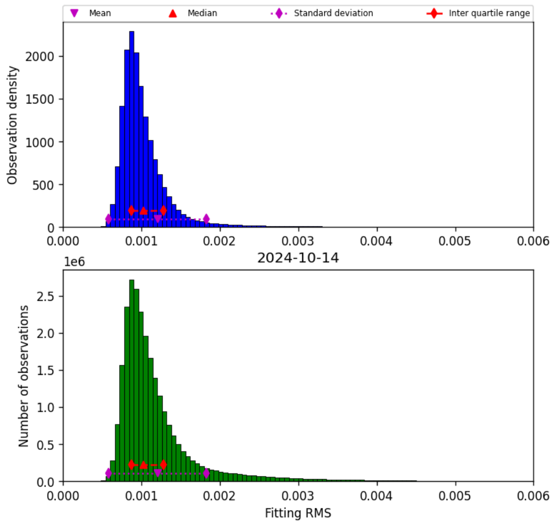
Figure 23: Histogram of “Fitting RMS” for 2024-10-14 to 2024-10-15
