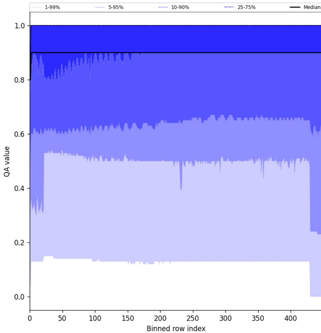
Figure 27: Along track statistics of “QA value” for 2024-10-14 to 2024-10-15
