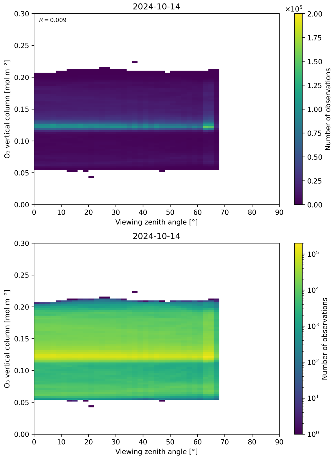
Figure 52: Scatter density plot of “Viewing zenith angle” against “O 3 vertical column” for 2024-10-14 to 2024-10-15.
