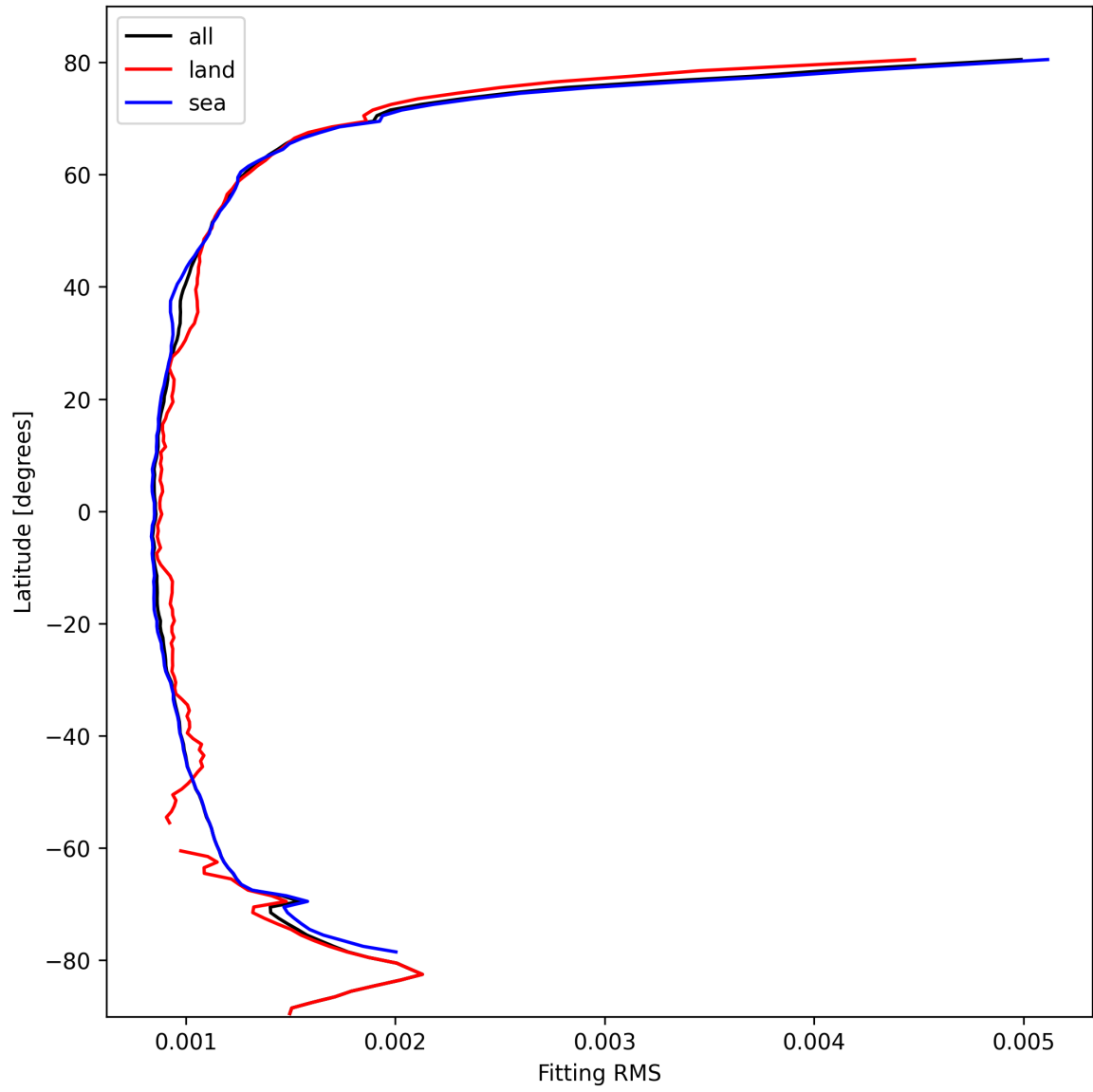
Figure 16: Zonal average of “Fitting RMS” for 2024-10-14 to 2024-10-15.
