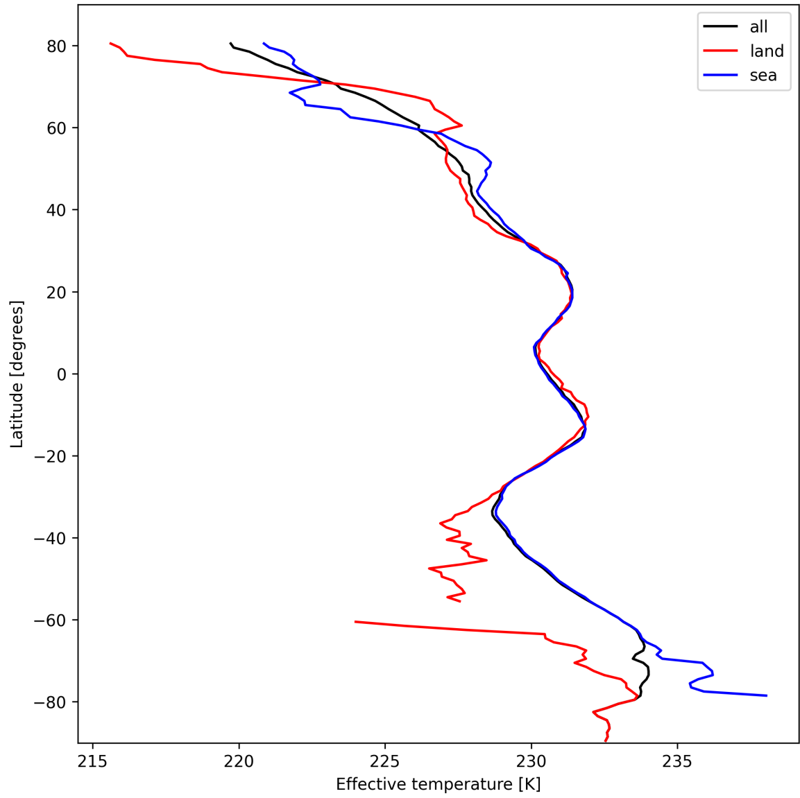
Figure 17: Zonal average of "Effective temperature" for 2024-10-14 to 2024-10-15.
