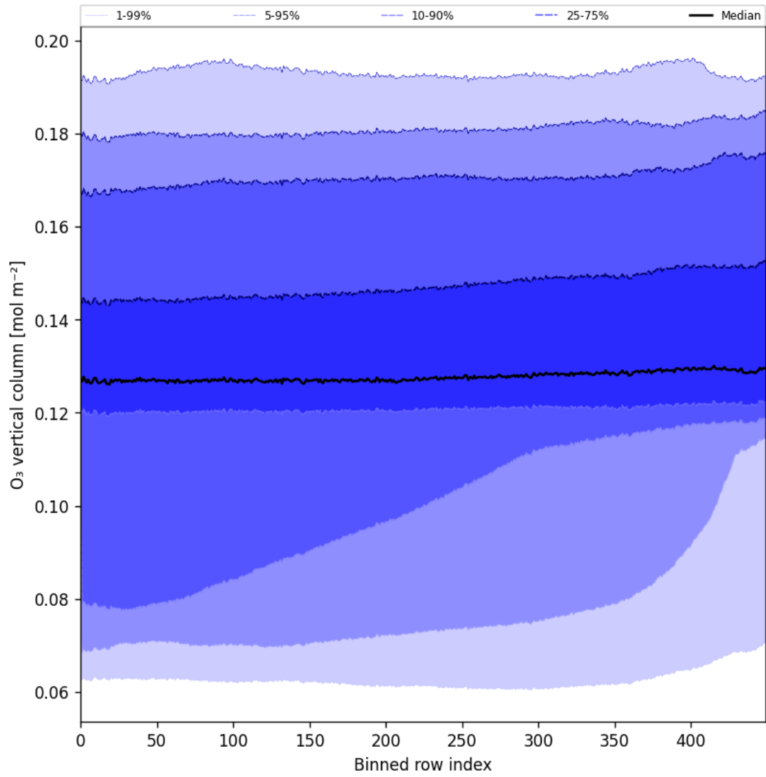
Figure 28: Along track statistics of “O 3 vertical column” for 2024-10-14 to 2024-10-15
