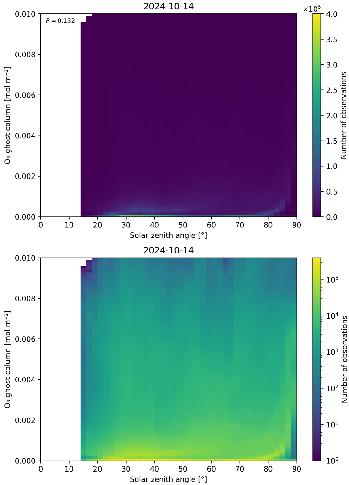
Figure 46: Scatter density plot of “Solar zenith angle” against “O 3 ghost column” for 2024-10-14 to 2024-10-15.
