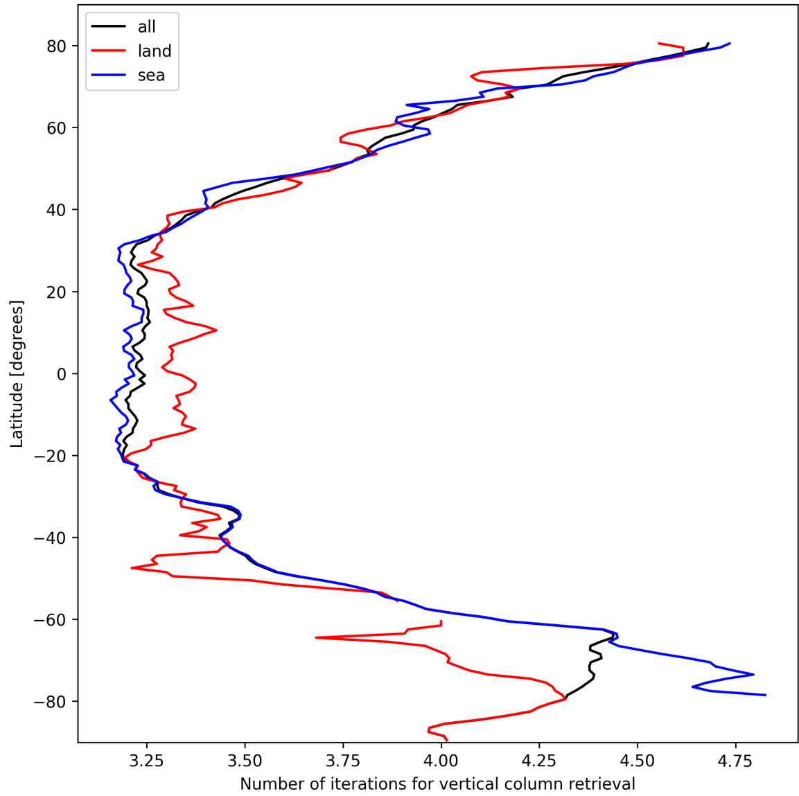
Figure 19: Zonal average of “Number of iterations for vertical column retrieval” for 2024-10-14 to 2024-10-15.
