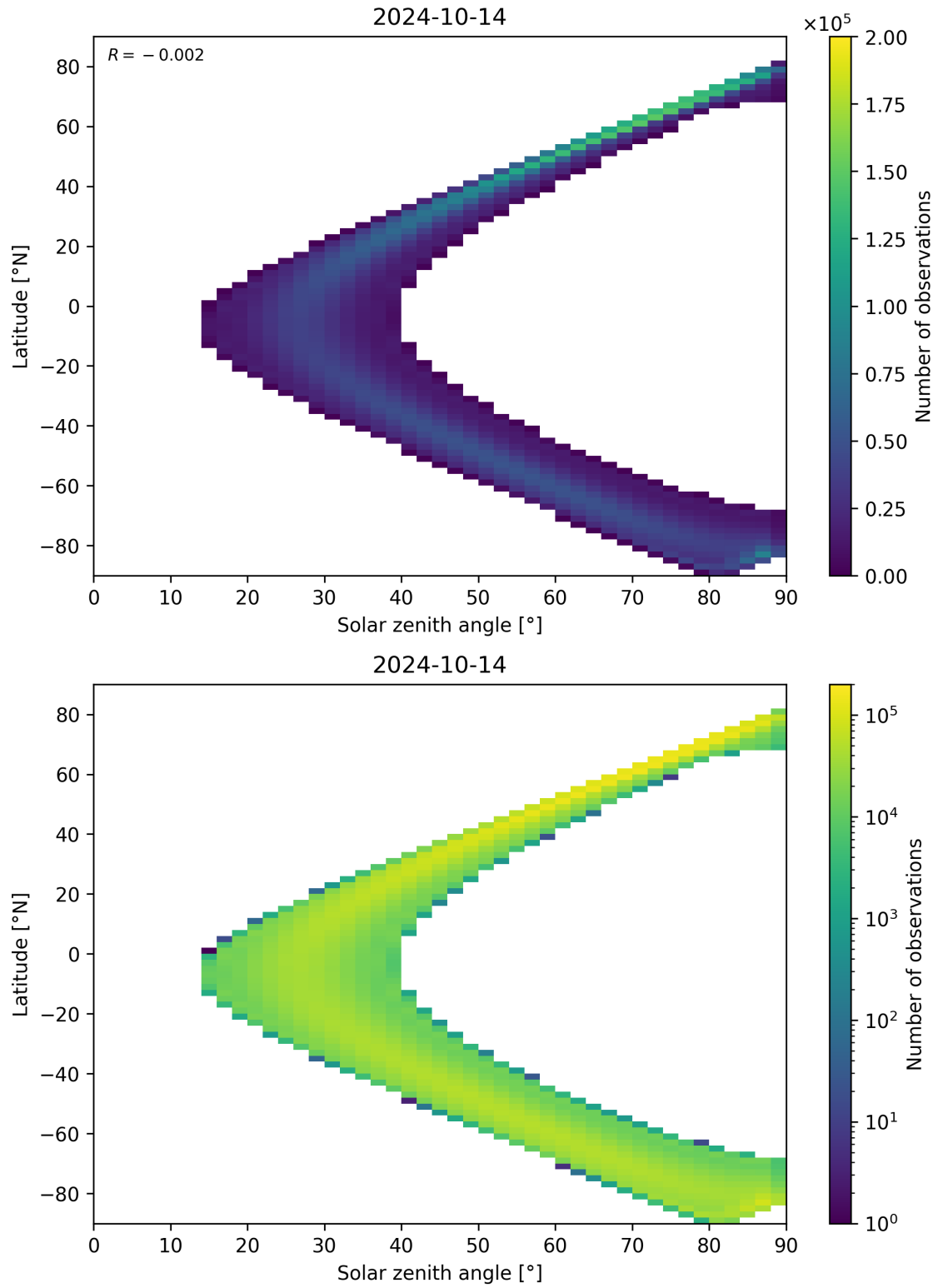
Figure 44: Scatter density plot of “Solar zenith angle” against “Latitude” for 2024-10-14 to 2024-10-15.
