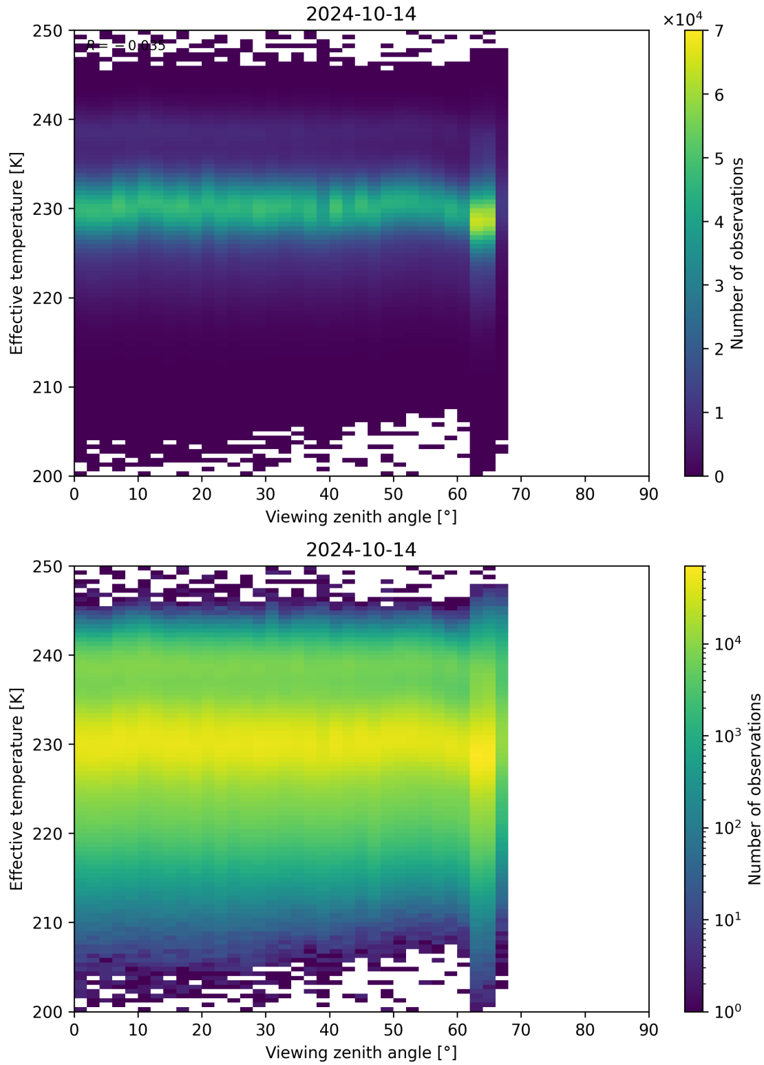
Figure 50: Scatter density plot of “Viewing zenith angle” against “Effective temperature” for 2024-10-14 to 2024-10-15.
