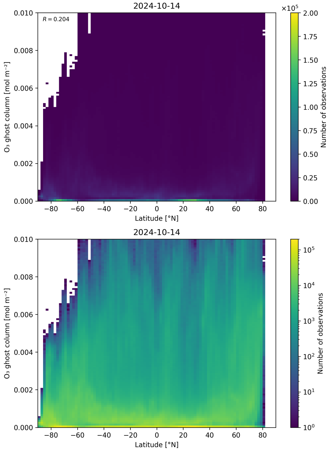
Figure 35: Scatter density plot of “Latitude” against “O 3 ghost column” for 2024-10-14 to 2024-10-15.
