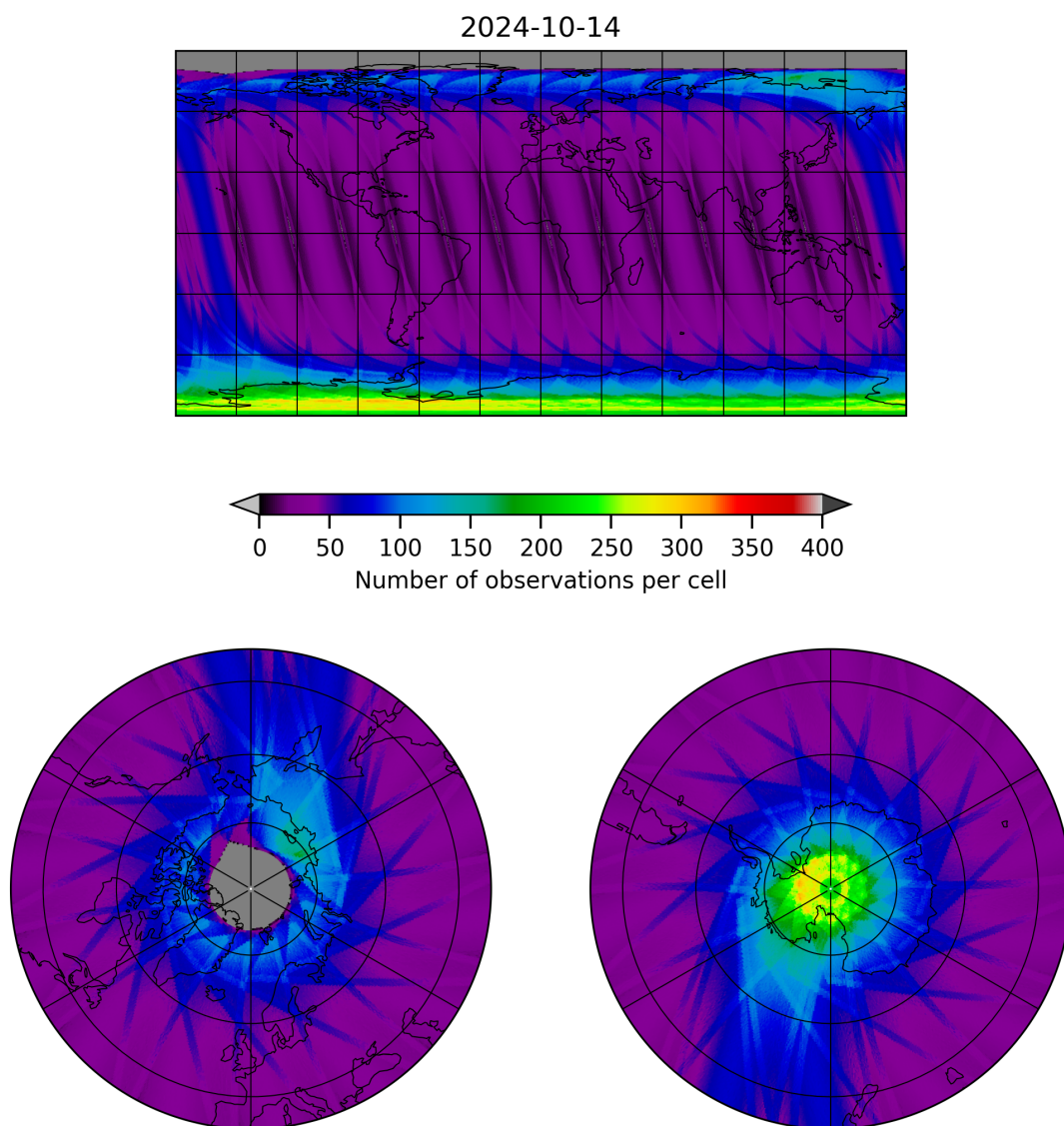
Figure 12: Map of the number of observations for 2024-10-14 to 2024-10-15
