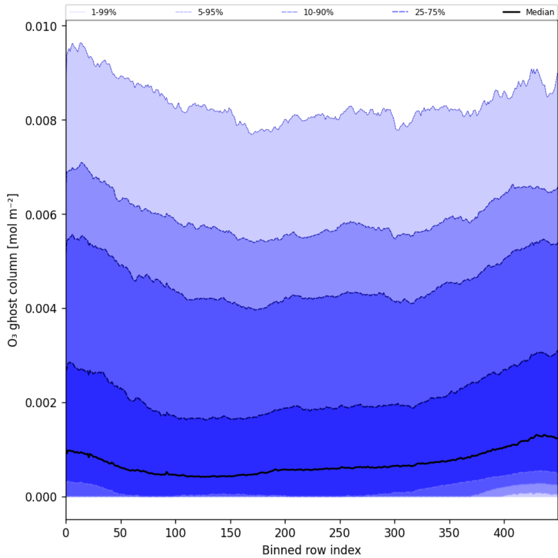
Figure 32: Along track statistics of “O 3 ghost column” for 2024-10-14 to 2024-10-15
