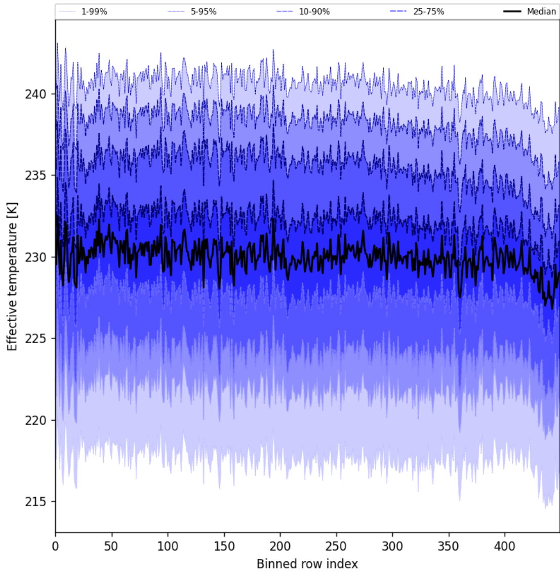
Figure 31: Along track statistics of “Effective temperature” for 2024-10-14 to 2024-10-15
