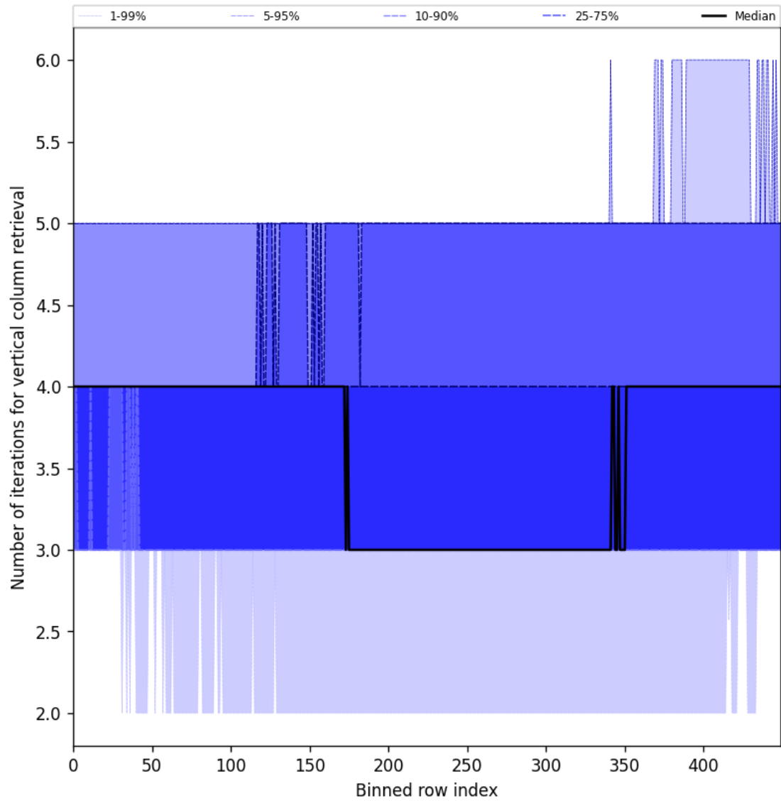
Figure 33: Along track statistics of “Number of iterations for vertical column retrieval” for 2024-10-14 to 2024-10-15
