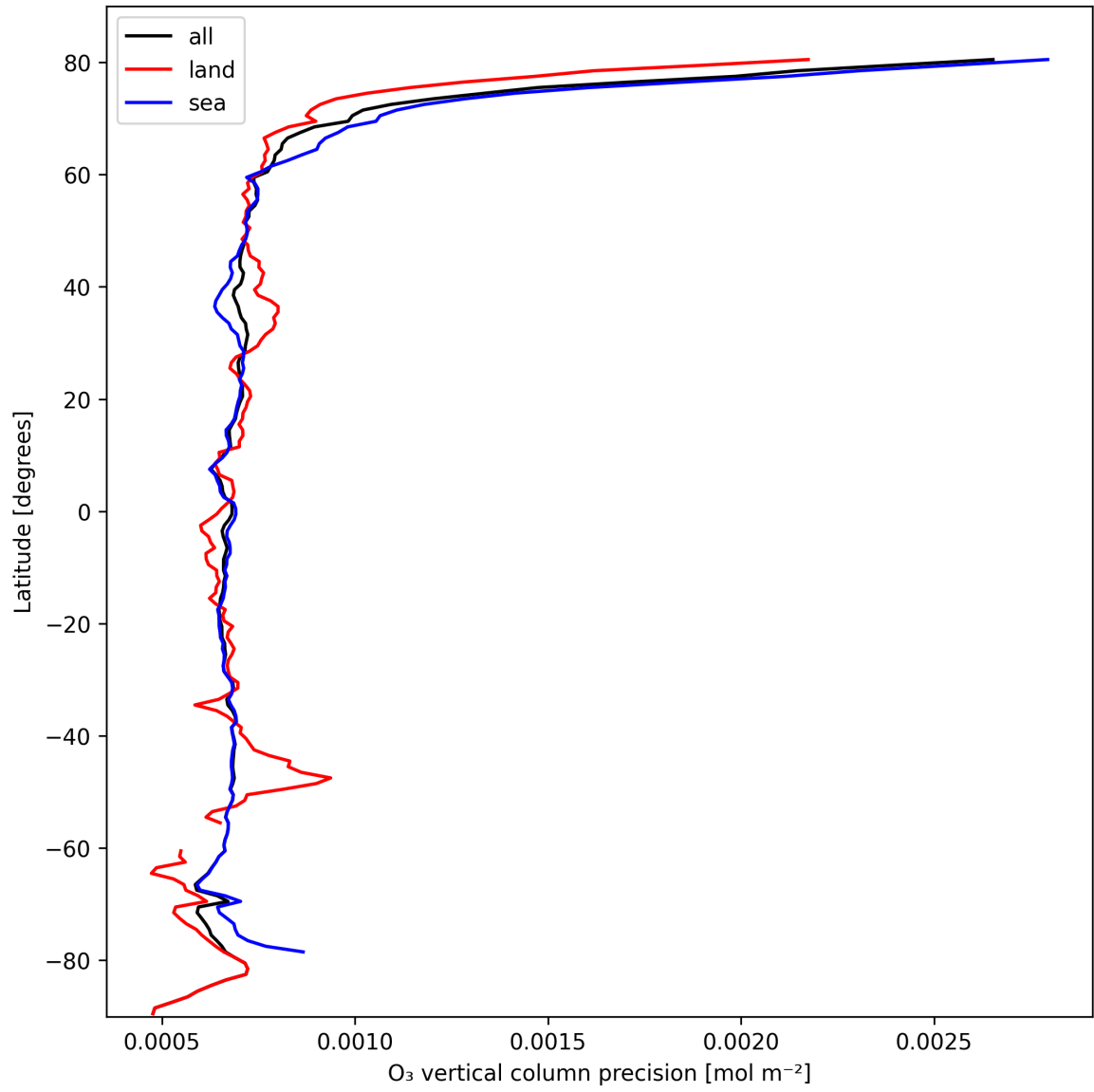
Figure 15: Zonal average of “O 3 vertical column precision” for 2024-10-14 to 2024-10-15.
