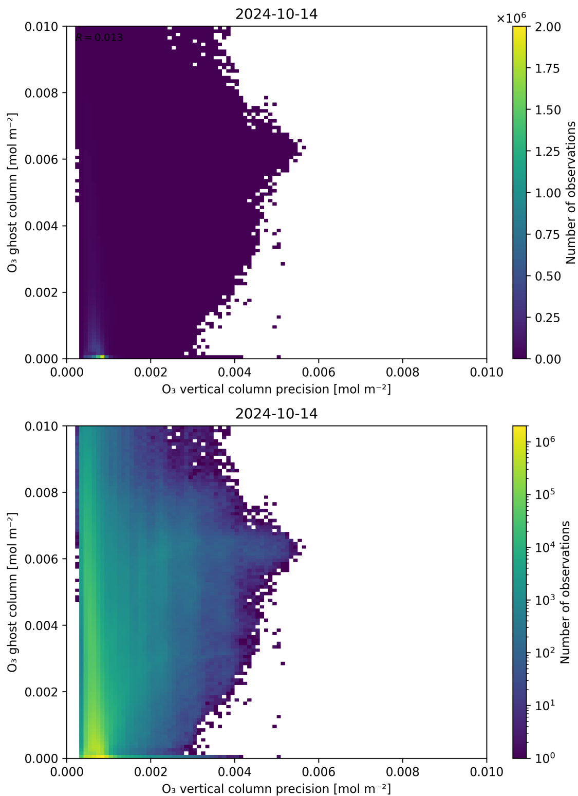
Figure 43: Scatter density plot of “O 3 vertical column precision” against “O 3 ghost column” for 2024-10-14 to 2024-10-15.
