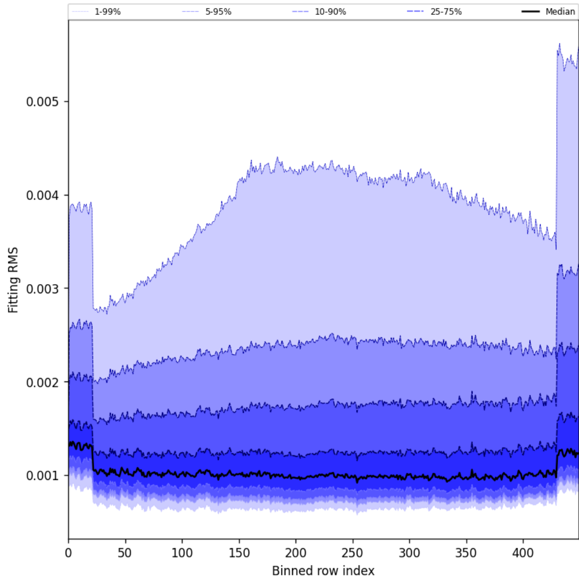
Figure 30: Along track statistics of “Fitting RMS” for 2024-10-14 to 2024-10-15
