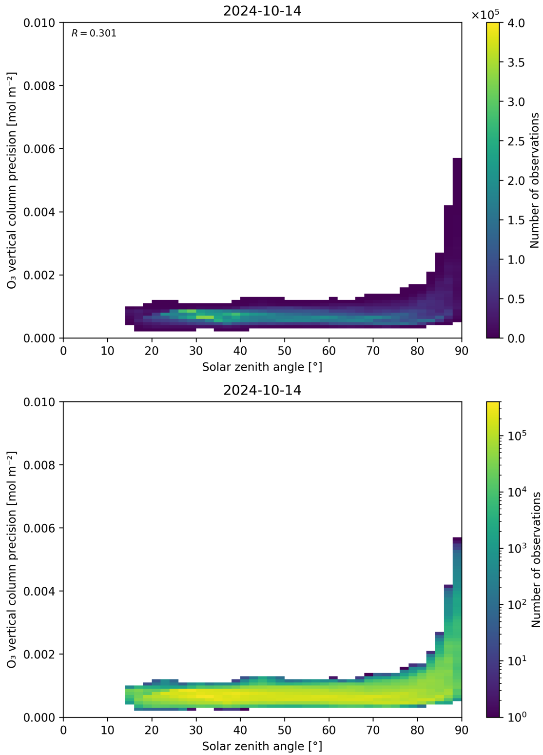
Figure 48: Scatter density plot of “Solar zenith angle” against “O 3 vertical column precision” for 2024-10-14 to 2024-10-15.
