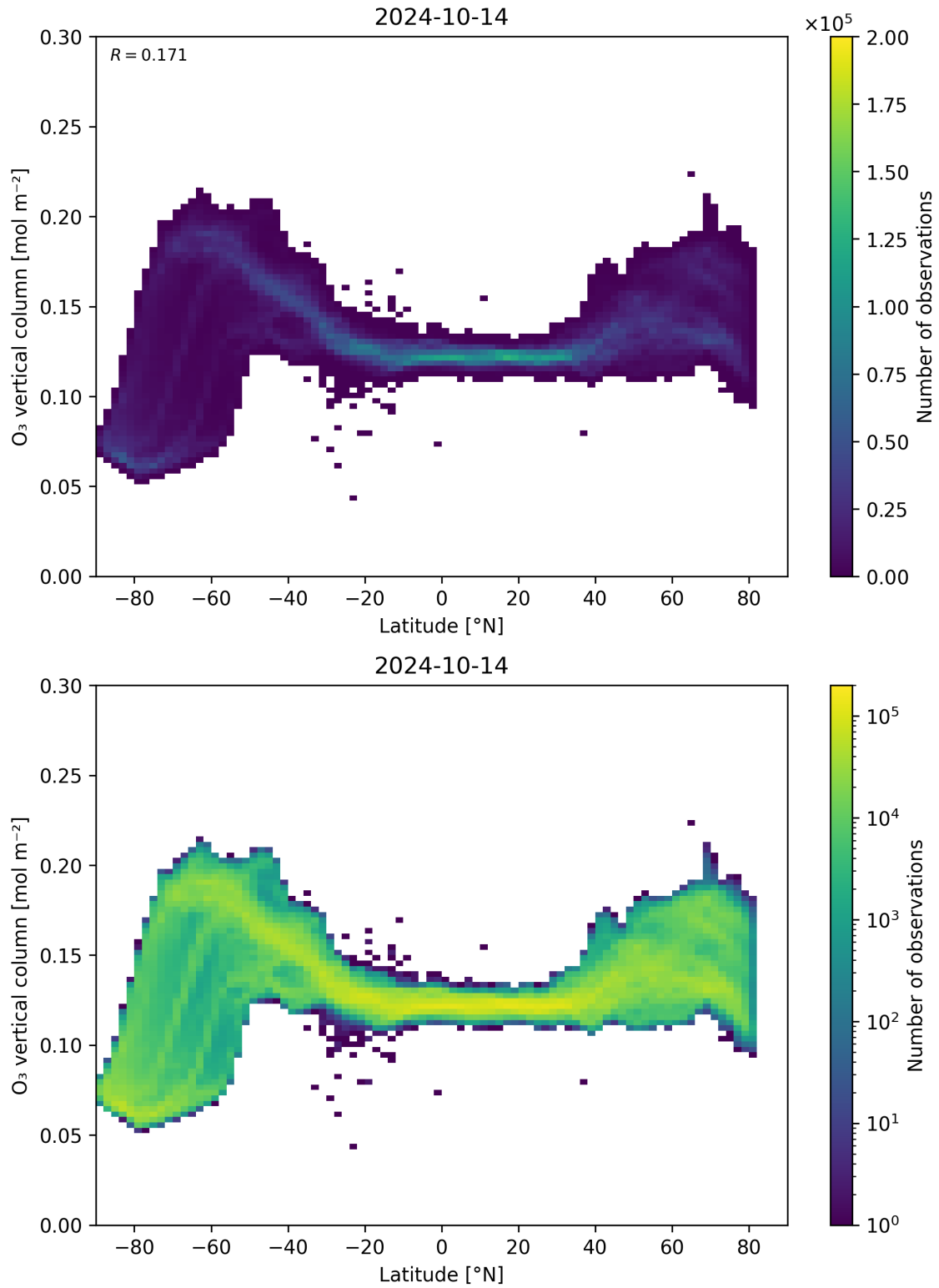
Figure 36: Scatter density plot of “Latitude” against “O 3 vertical column” for 2024-10-14 to 2024-10-15.
