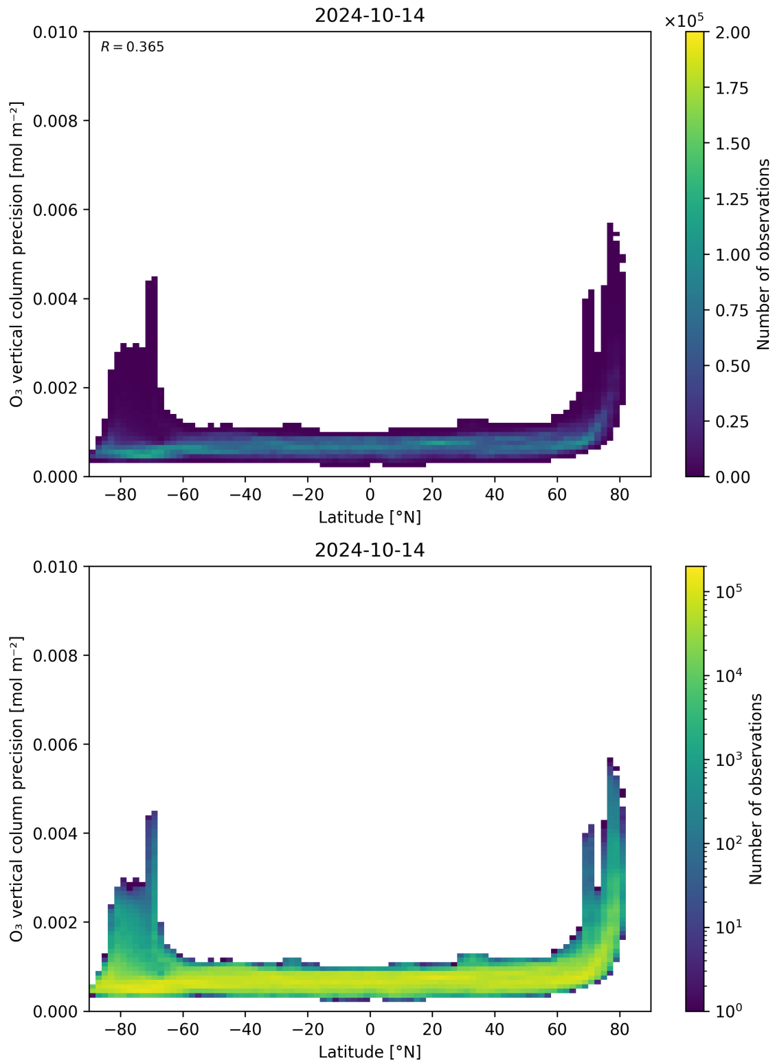
Figure 37: Scatter density plot of “Latitude” against “O 3 vertical column precision” for 2024-10-14 to 2024-10-15.
