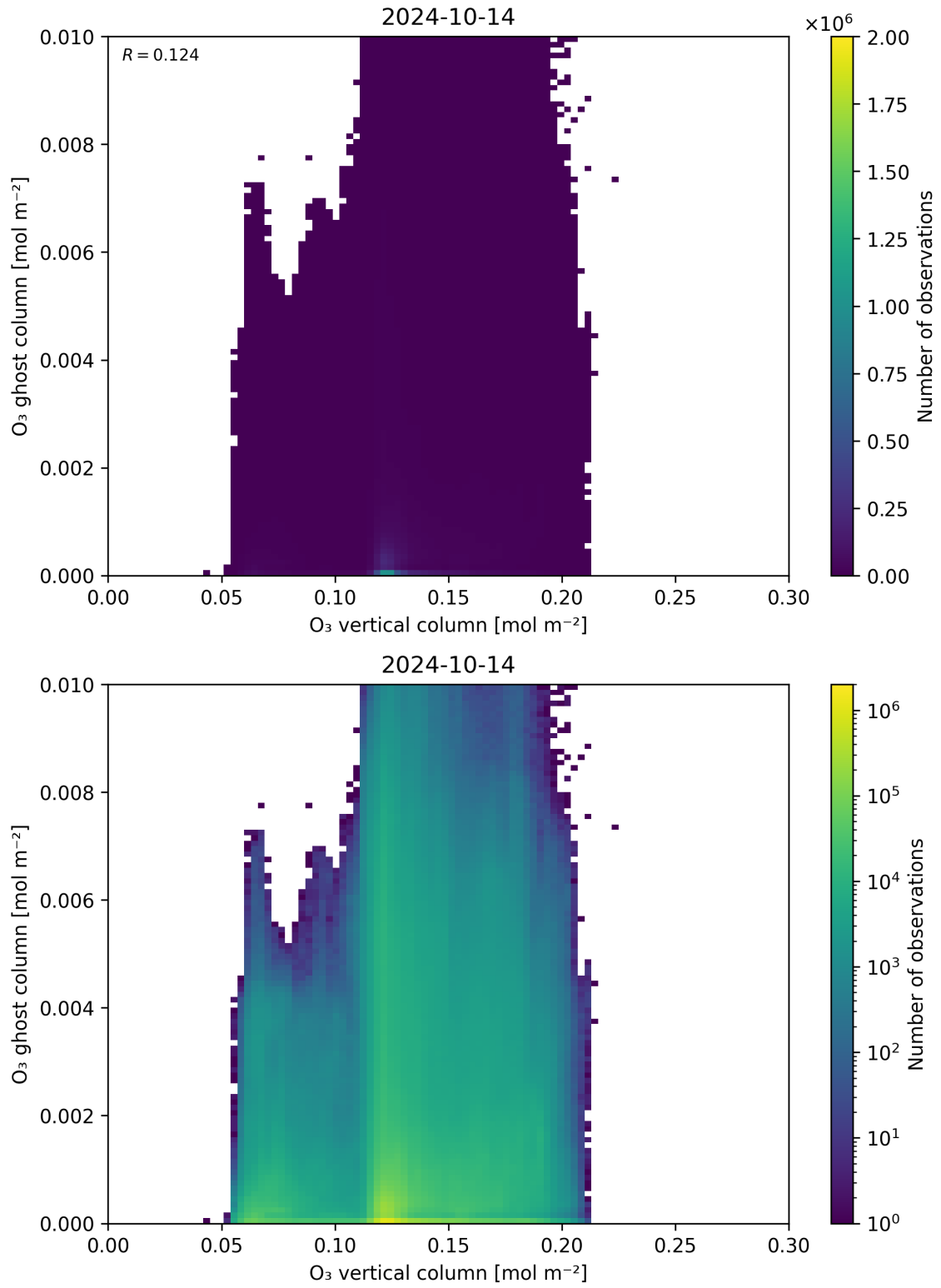
Figure 40: Scatter density plot of “O 3 vertical column” against “O 3 ghost column” for 2024-10-14 to 2024-10-15.
