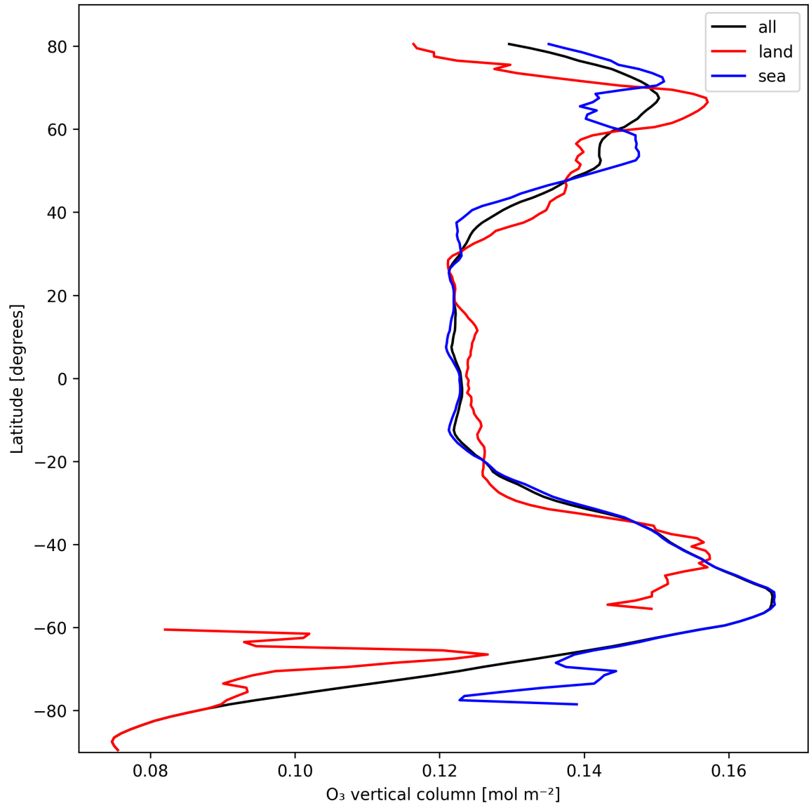
Figure 14: Zonal average of “O 3 vertical column” for 2024-10-14 to 2024-10-15.
