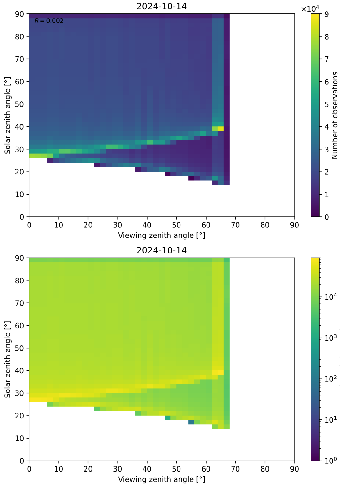
Figure 54: Scatter density plot of “Viewing zenith angle” against “Solar zenith angle” for 2024-10-14 to 2024-10-15.
