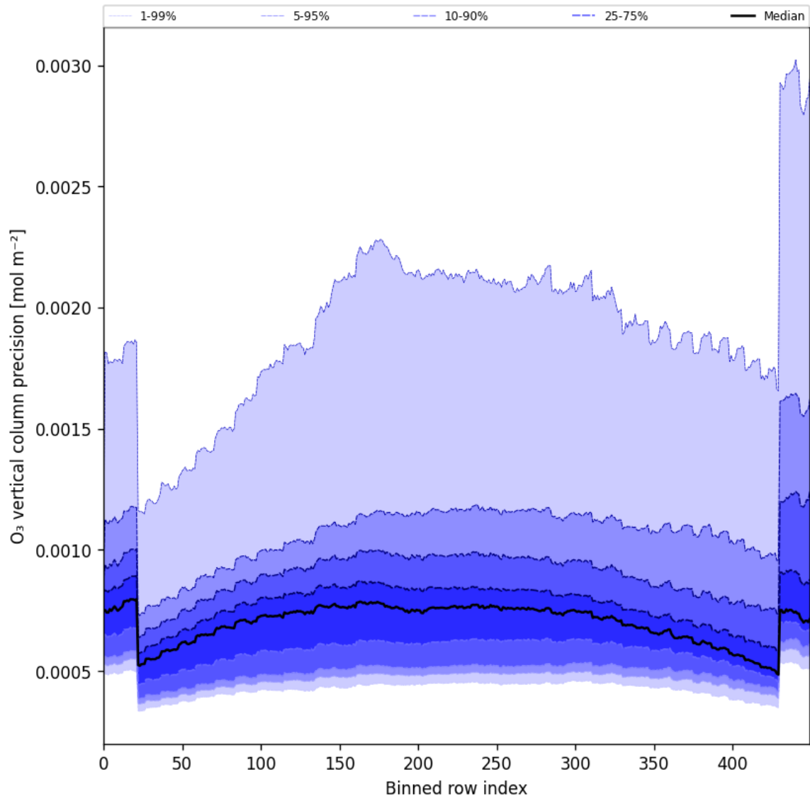
Figure 29: Along track statistics of “O 3 vertical column precision” for 2024-10-14 to 2024-10-15
