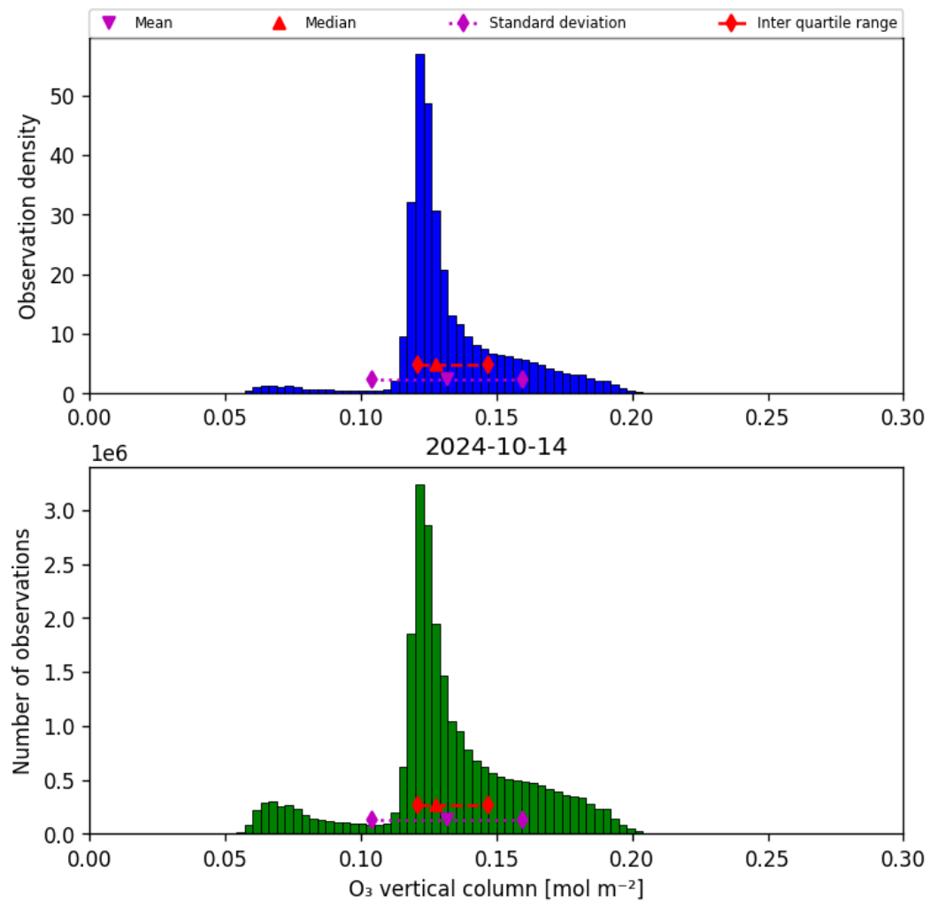
Figure 21: Histogram of “O 3 vertical column” for 2024-10-14 to 2024-10-15
