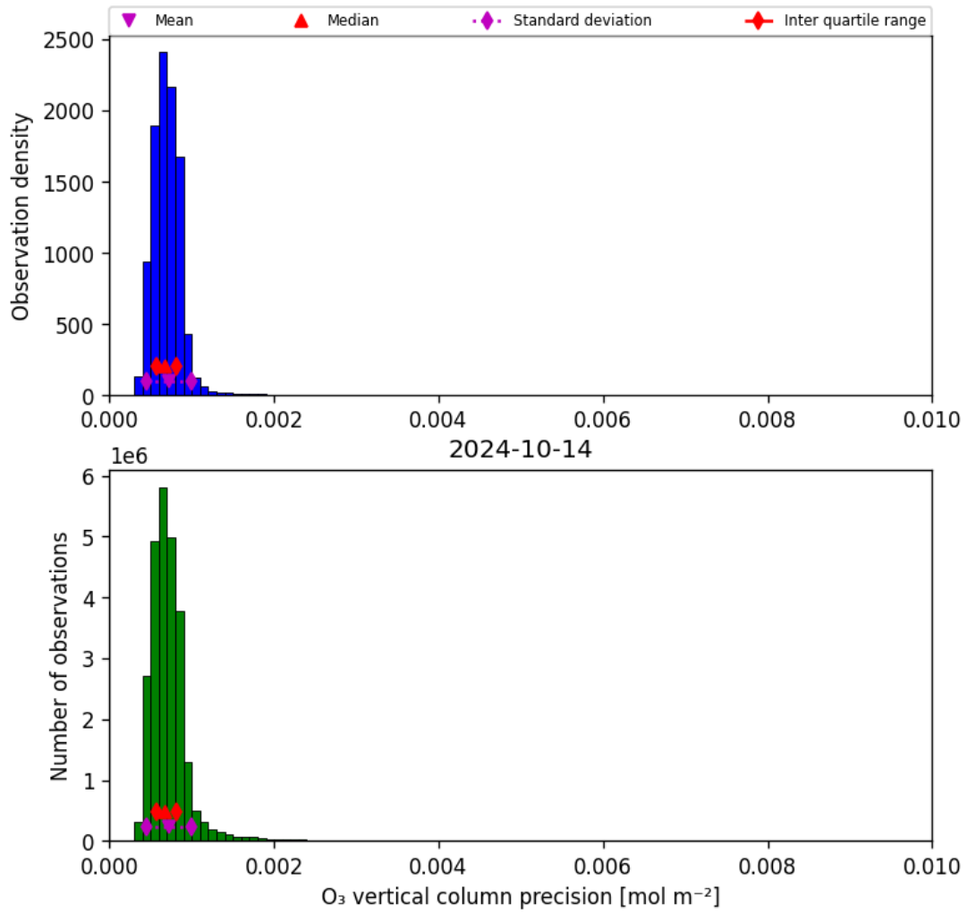
Figure 22: Histogram of “O 3 vertical column precision” for 2024-10-14 to 2024-10-15
