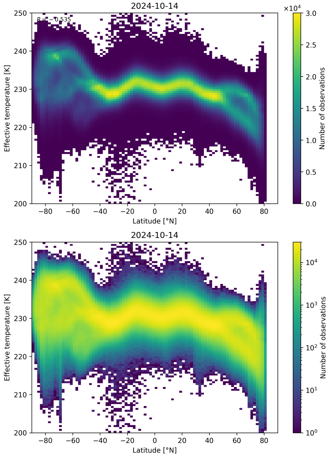
Figure 34: Scatter density plot of “Latitude” against “Effective temperature” for 2024-10-14 to 2024-10-15.
