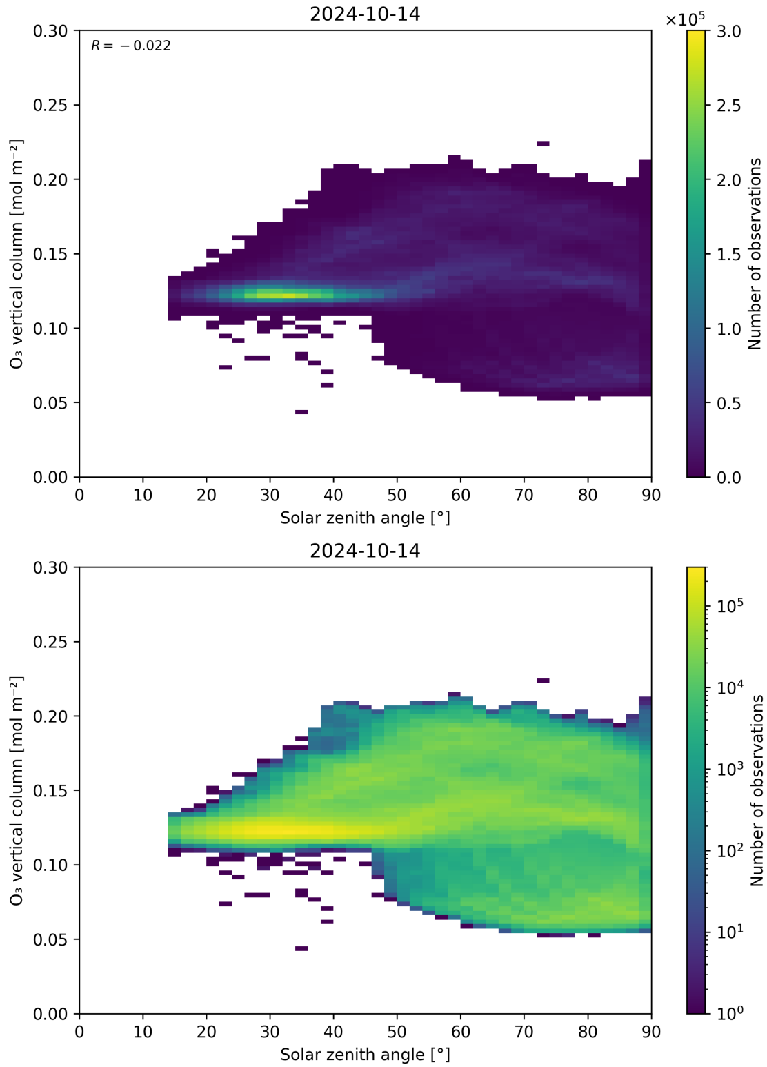
Figure 47: Scatter density plot of “Solar zenith angle” against “O 3 vertical column” for 2024-10-14 to 2024-10-15.
