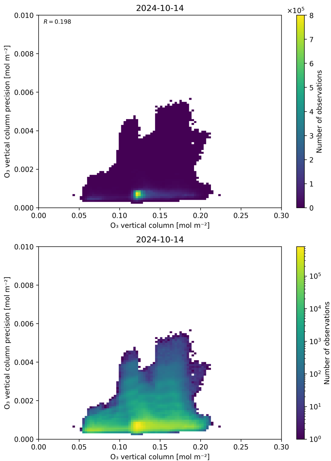
Figure 41: Scatter density plot of “O 3 vertical column” against “O 3 vertical column precision” for 2024-10-14 to 2024-10-15.
