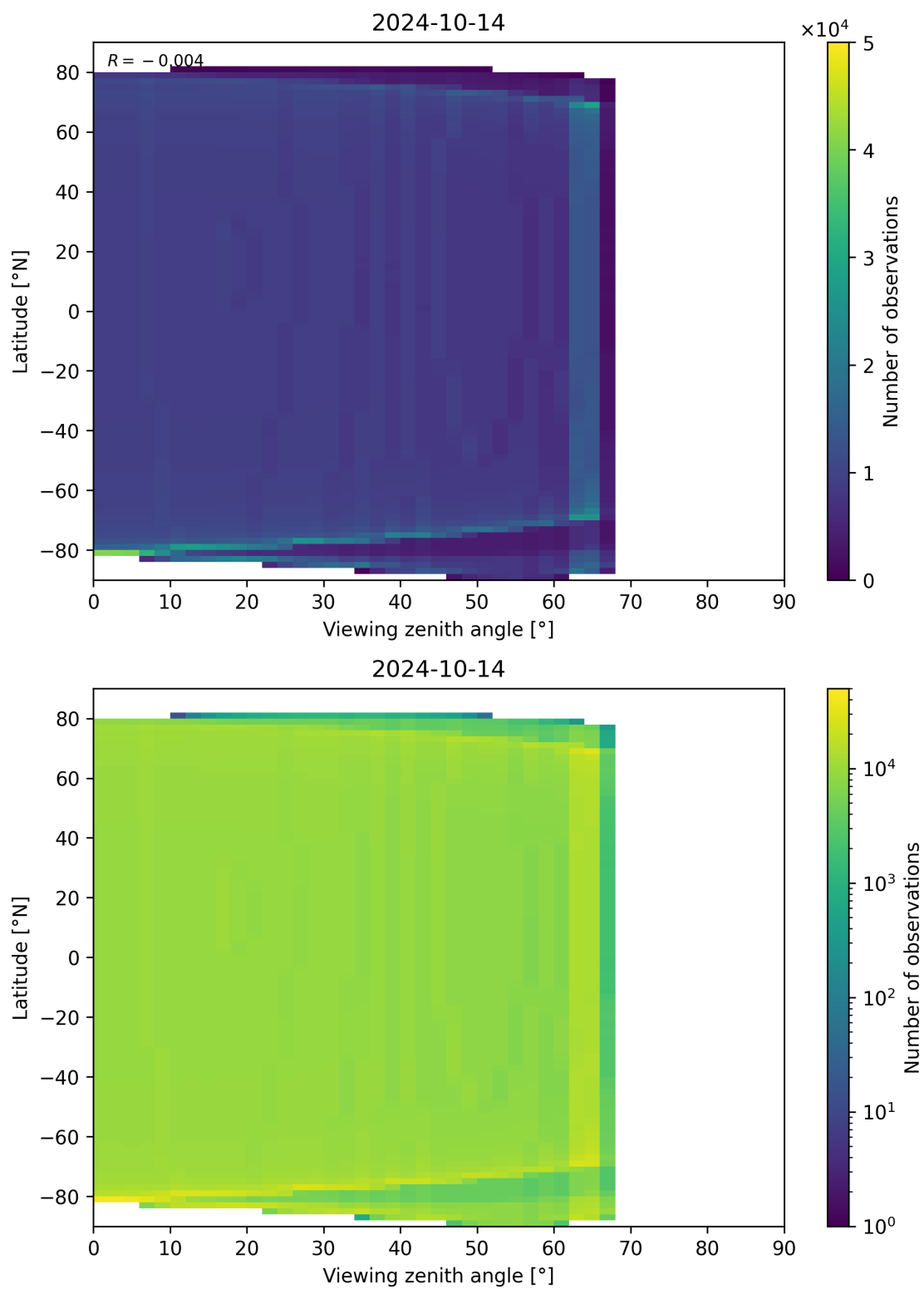
Figure 49: Scatter density plot of “Viewing zenith angle” against “Latitude” for 2024-10-14 to 2024-10-15.
