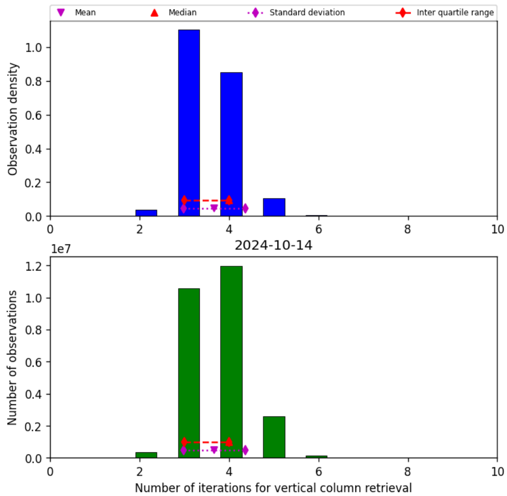
Figure 26: Histogram of “Number of iterations for vertical column retrieval” for 2024-10-14 to 2024-10-15
