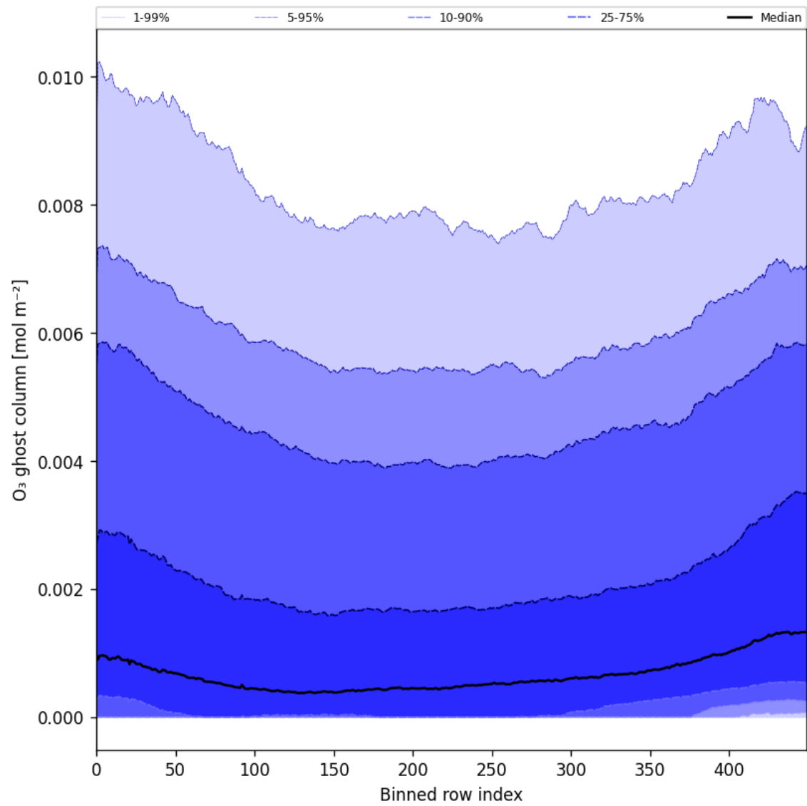
Figure 32: Along track statistics of "O 3 ghost column" for 2024-10-15 to 2024-10-17
