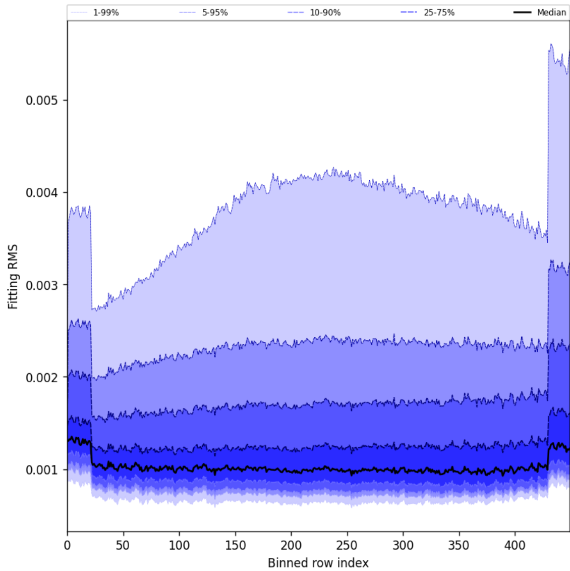
Figure 30: Along track statistics of “Fitting RMS” for 2024-10-15 to 2024-10-17
