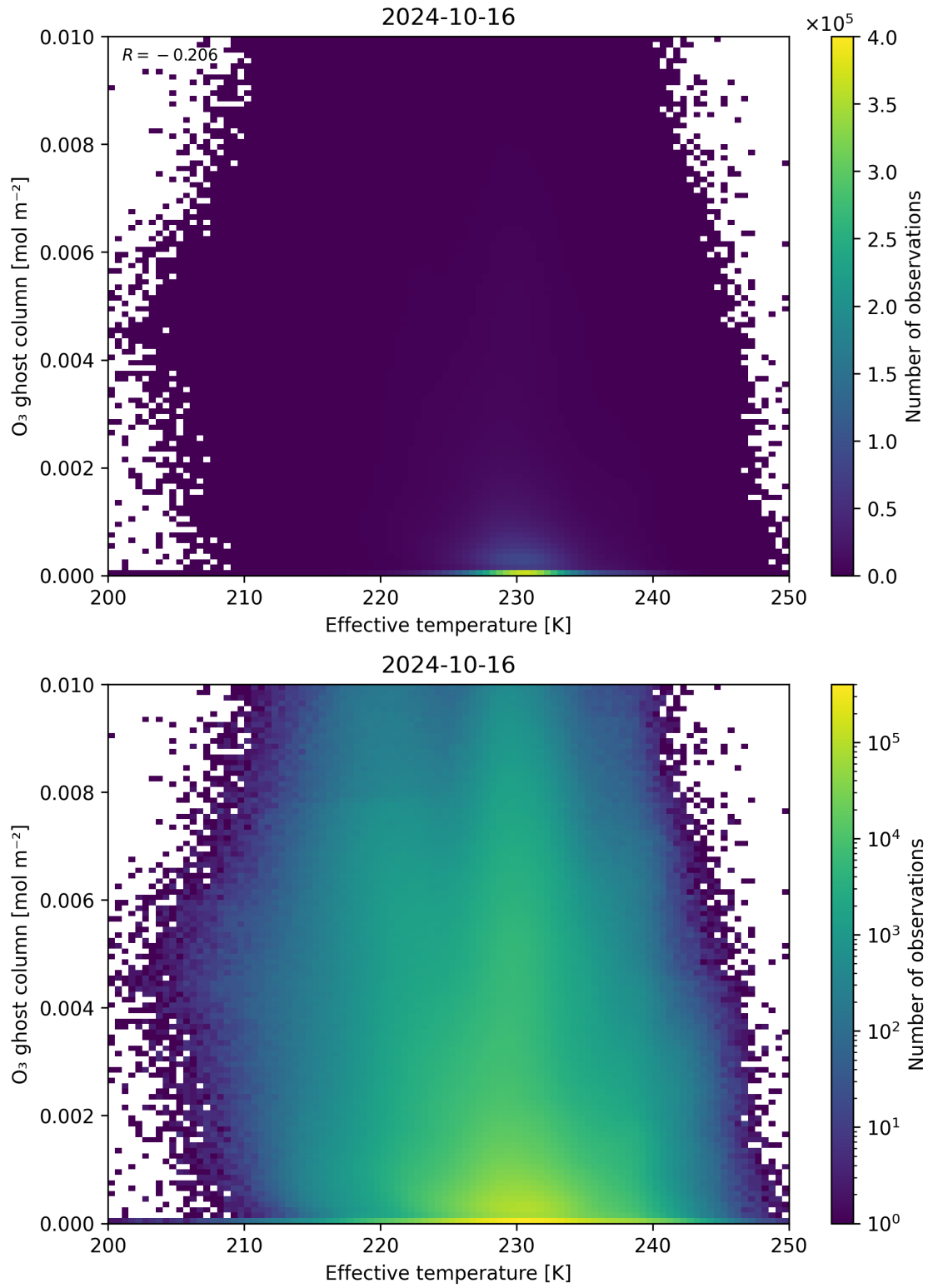
Figure 38: Scatter density plot of “Effective temperature” against “O 3 ghost column” for 2024-10-15 to 2024-10-17.
