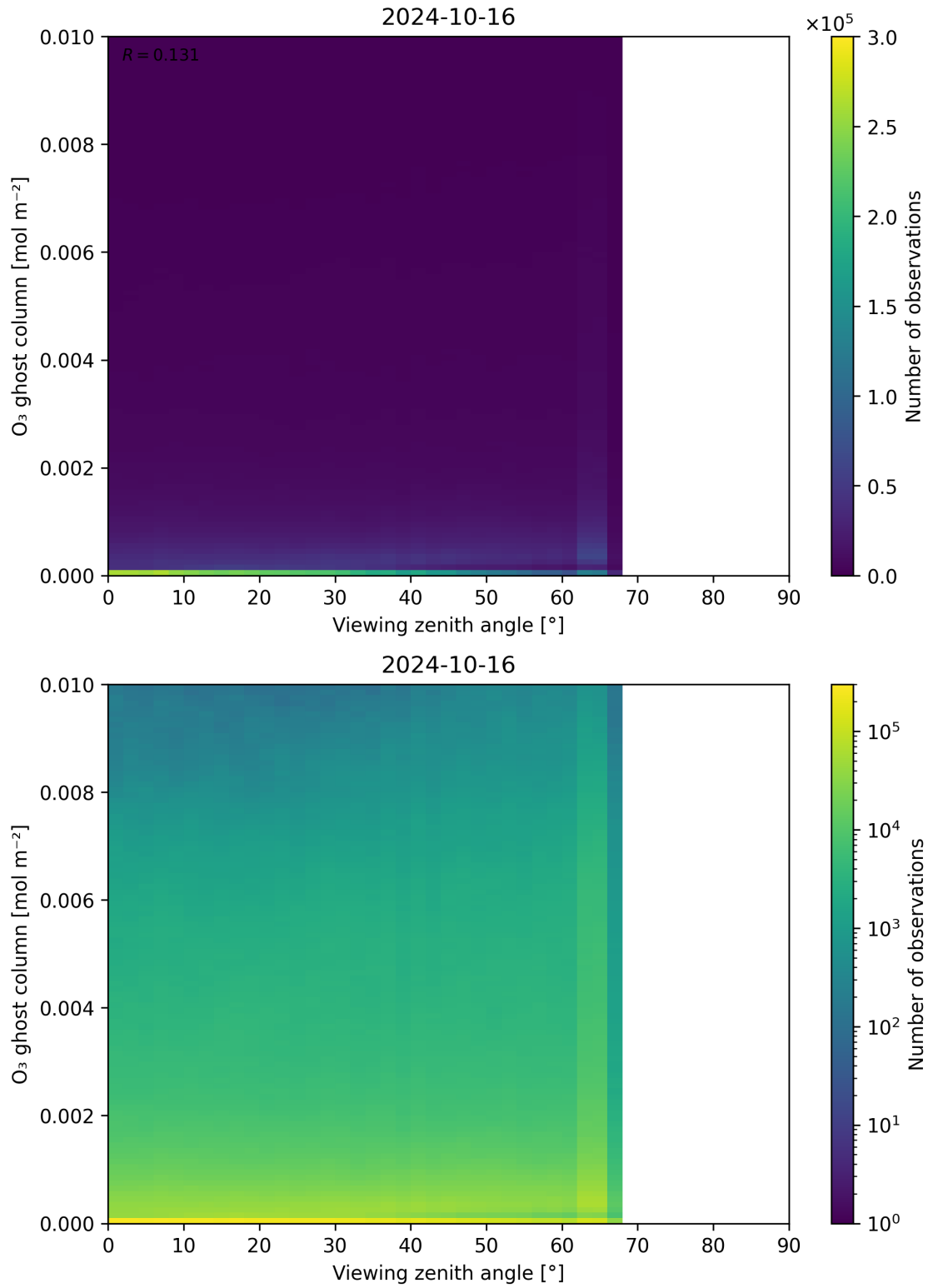
Figure 51: Scatter density plot of “Viewing zenith angle” against “O 3 ghost column” for 2024-10-15 to 2024-10-17.
