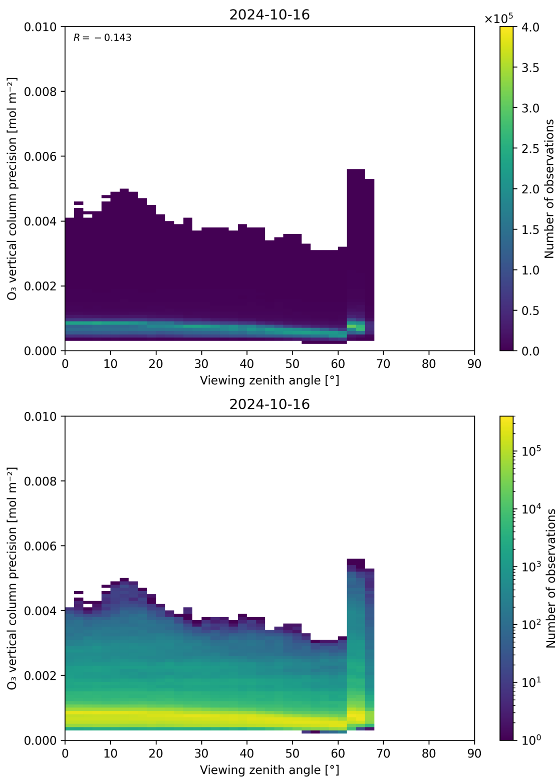
Figure 53: Scatter density plot of “Viewing zenith angle” against “O 3 vertical column precision” for 2024-10-15 to 2024-10-17.
