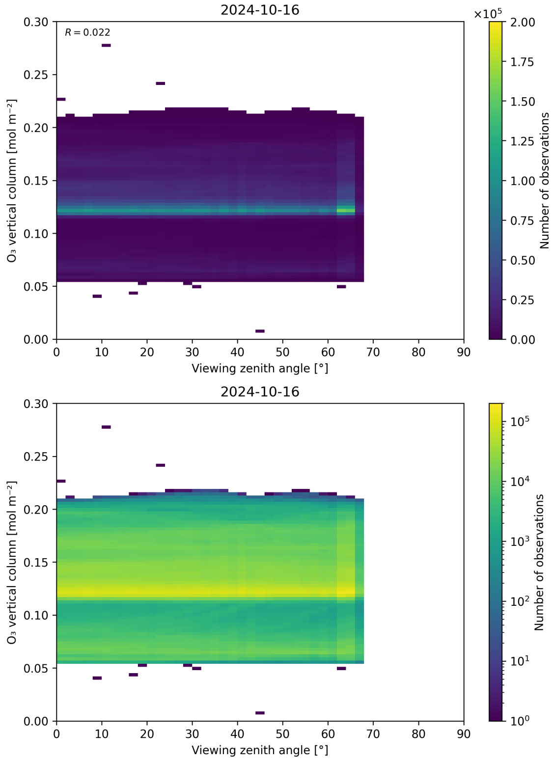
Figure 52: Scatter density plot of “Viewing zenith angle” against “O 3 vertical column” for 2024-10-15 to 2024-10-17.
