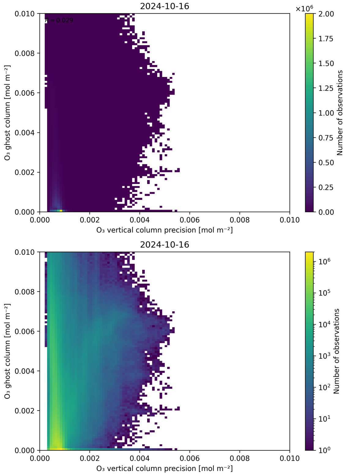
Figure 43: Scatter density plot of “O 3 vertical column precision” against “O 3 ghost column” for 2024-10-15 to 2024-10-17.
