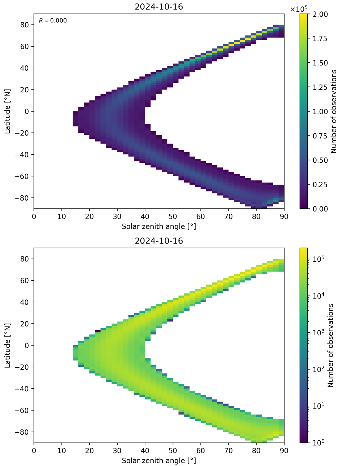
Figure 44: Scatter density plot of “Solar zenith angle” against “Latitude” for 2024-10-15 to 2024-10-17.
