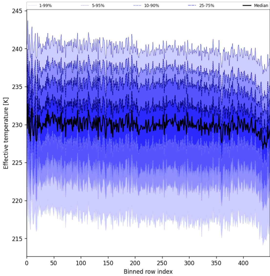
Figure 31: Along track statistics of “Effective temperature” for 2024-10-15 to 2024-10-17
