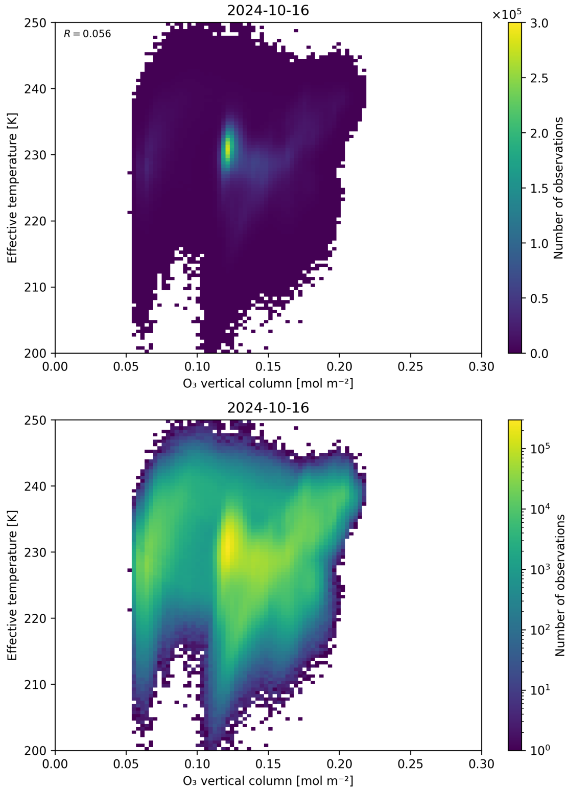
Figure 39: Scatter density plot of “O 3 vertical column” against “Effective temperature” for 2024-10-15 to 2024-10-17.
