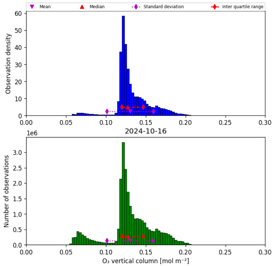
Figure 21: Histogram of “O 3 vertical column” for 2024-10-15 to 2024-10-17
