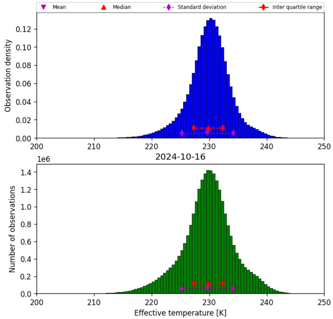
Figure 24: Histogram of “Effective temperature” for 2024-10-15 to 2024-10-17
