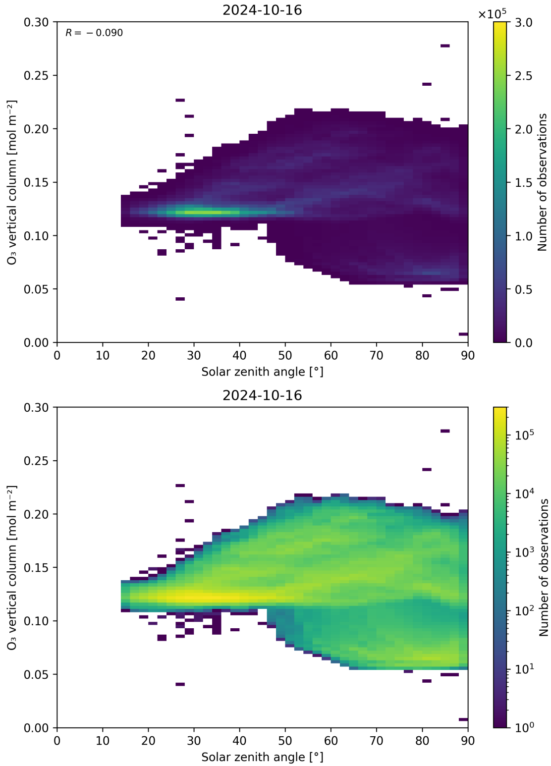
Figure 47: Scatter density plot of “Solar zenith angle” against “O 3 vertical column” for 2024-10-15 to 2024-10-17.
