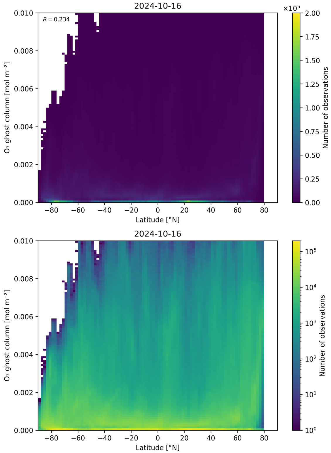
Figure 35: Scatter density plot of “Latitude” against “O 3 ghost column” for 2024-10-15 to 2024-10-17.
