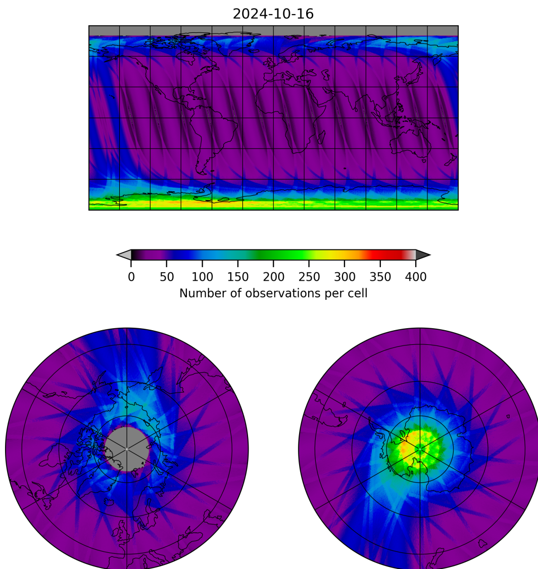
Figure 12: Map of the number of observations for 2024-10-15 to 2024-10-17
