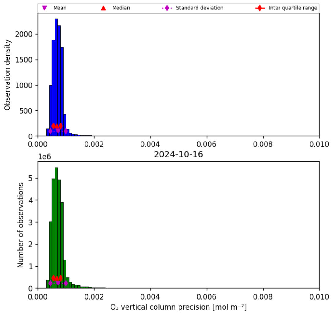
Figure 22: Histogram of “O 3 vertical column precision” for 2024-10-15 to 2024-10-17
