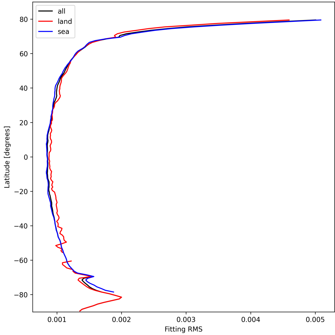
Figure 16: Zonal average of “Fitting RMS” for 2024-10-15 to 2024-10-17.
