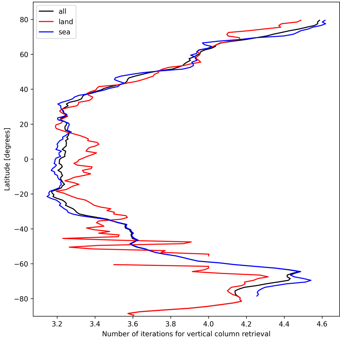
Figure 19: Zonal average of “Number of iterations for vertical column retrieval” for 2024-10-15 to 2024-10-17.
