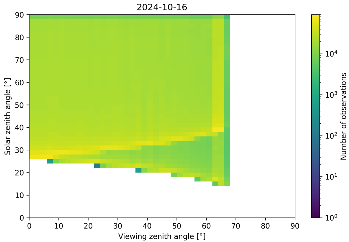
Figure 54: Scatter density plot of “Viewing zenith angle” against “Solar zenith angle” for 2024-10-15 to 2024-10-17.
