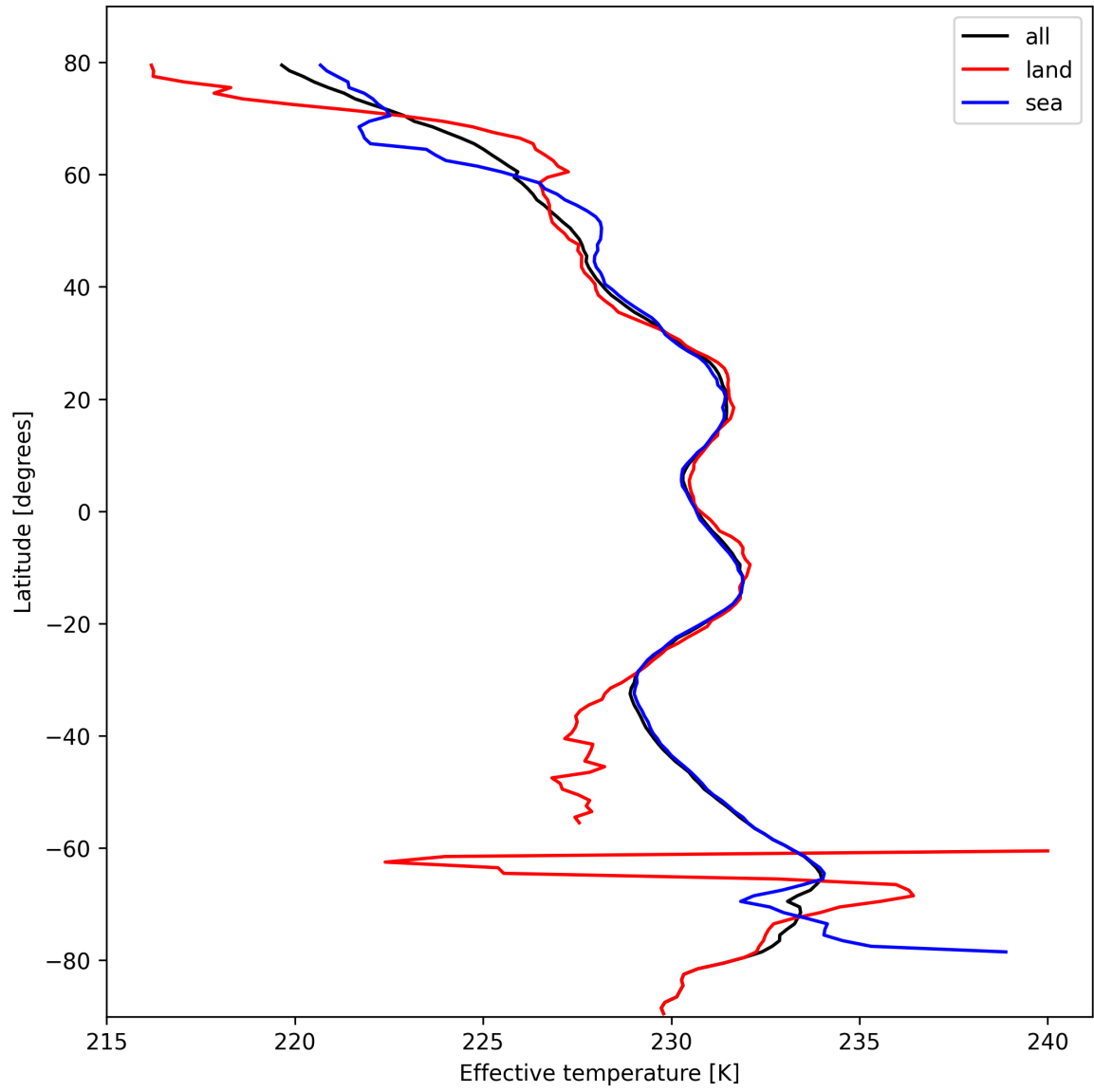
Figure 17: Zonal average of “Effective temperature” for 2024-10-15 to 2024-10-17.
