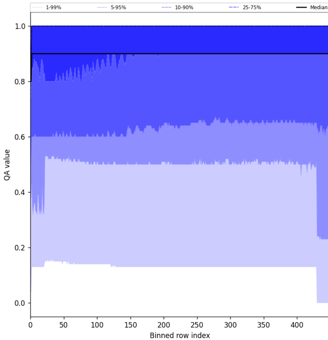
Figure 27: Along track statistics of “QA value” for 2024-10-15 to 2024-10-17
