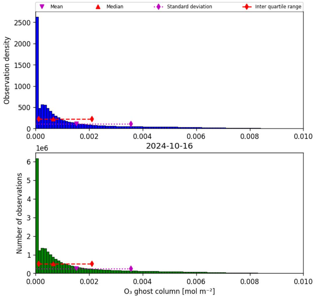
Figure 25: Histogram of "O 3 ghost column" for 2024-10-15 to 2024-10-17
