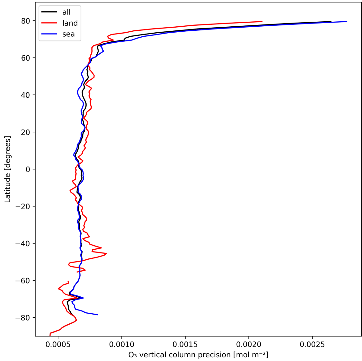
Figure 15: Zonal average of “O 3 vertical column precision” for 2024-10-15 to 2024-10-17.
