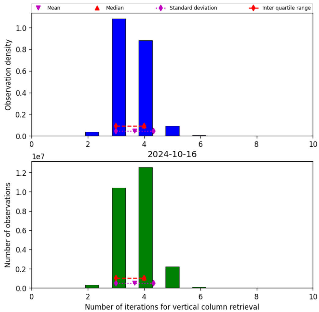
Figure 26: Histogram of “Number of iterations for vertical column retrieval” for 2024-10-15 to 2024-10-17
