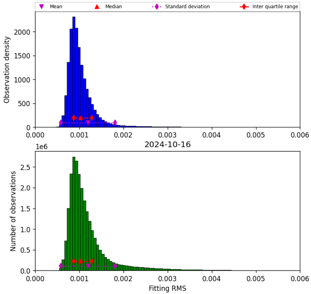
Figure 23: Histogram of “Fitting RMS” for 2024-10-15 to 2024-10-17
