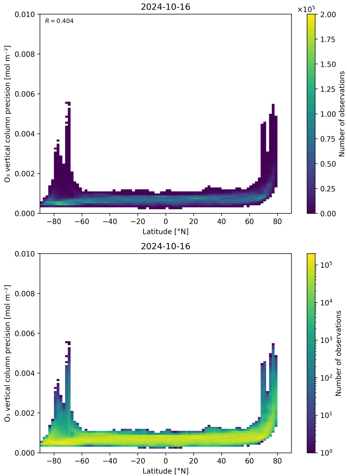
Figure 37: Scatter density plot of “Latitude” against “O 3 vertical column precision” for 2024-10-15 to 2024-10-17.
