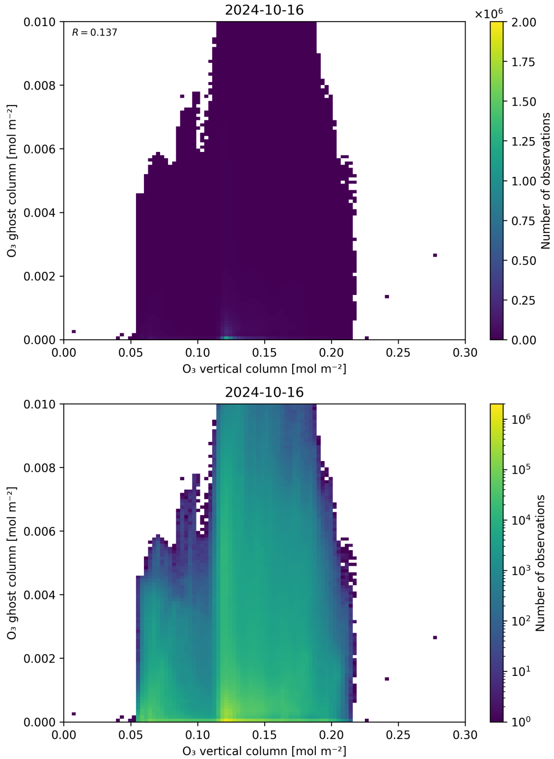
Figure 40: Scatter density plot of “O 3 vertical column” against “O 3 ghost column” for 2024-10-15 to 2024-10-17.
