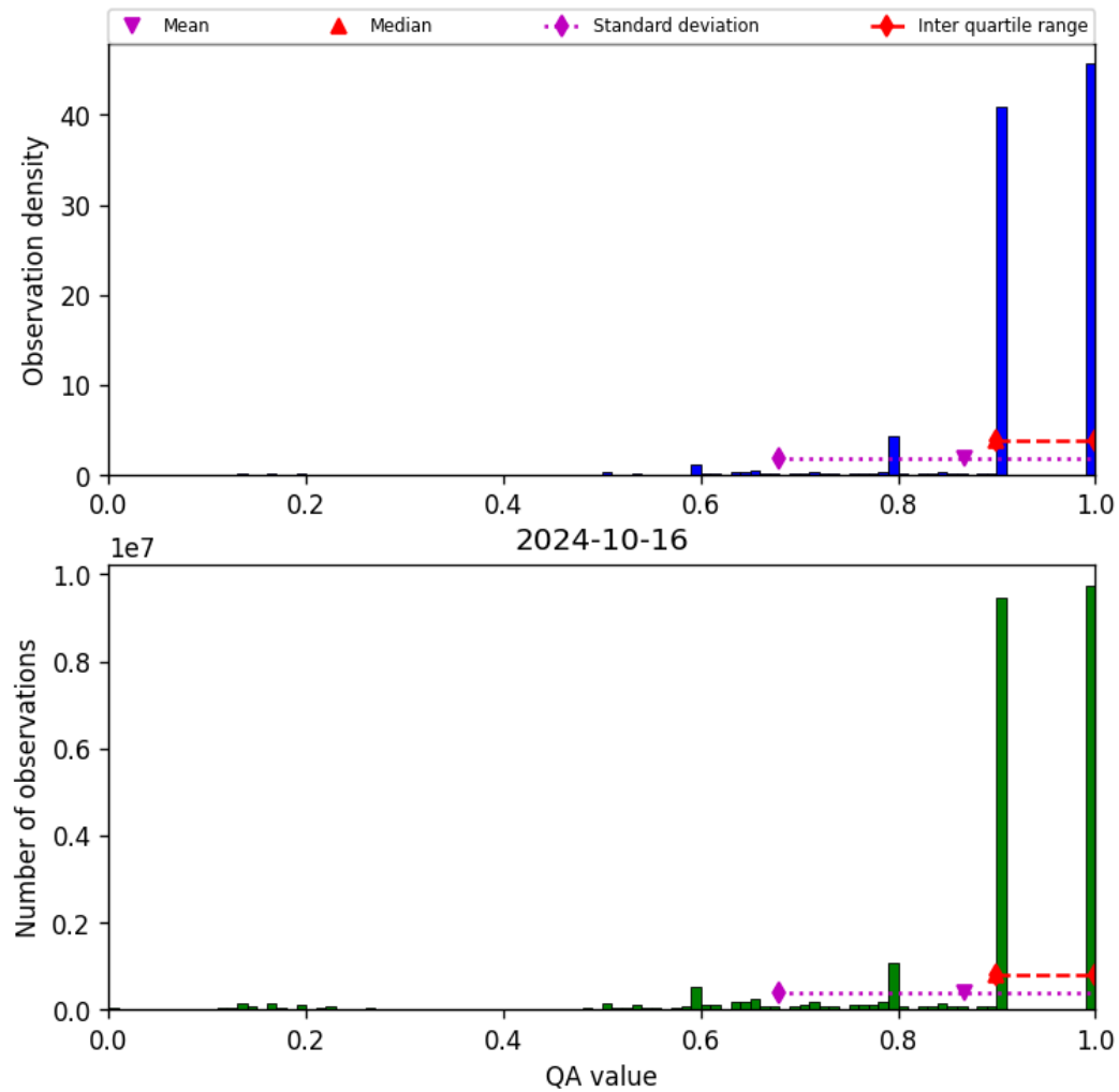
Figure 20: Histogram of “QA value” for 2024-10-15 to 2024-10-17
