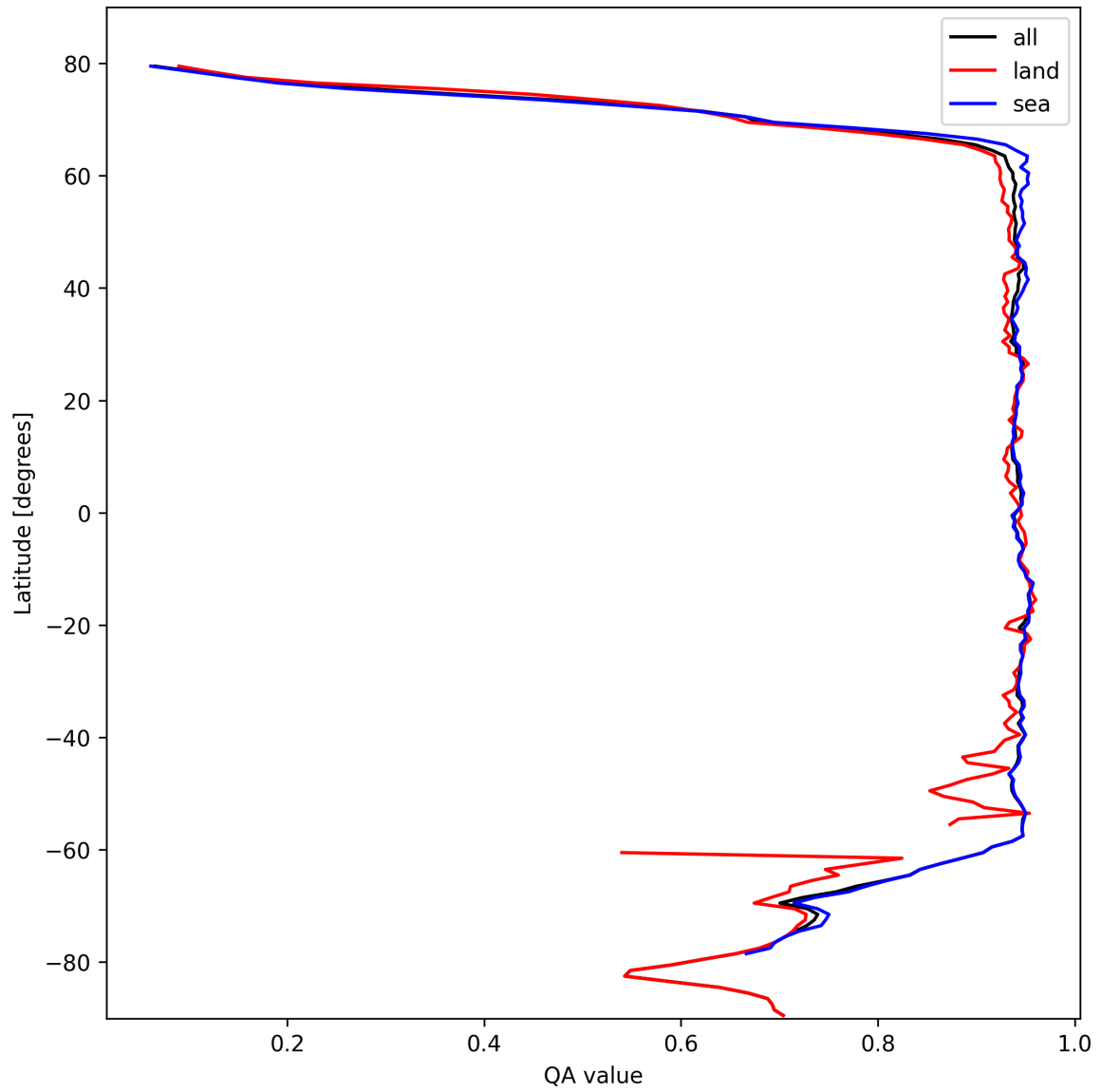
Figure 13: Zonal average of “QA value” for 2024-10-15 to 2024-10-17.
