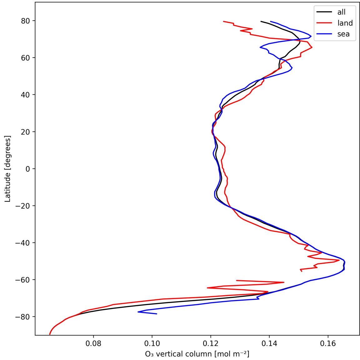
Figure 14: Zonal average of “O 3 vertical column” for 2024-10-15 to 2024-10-17.
