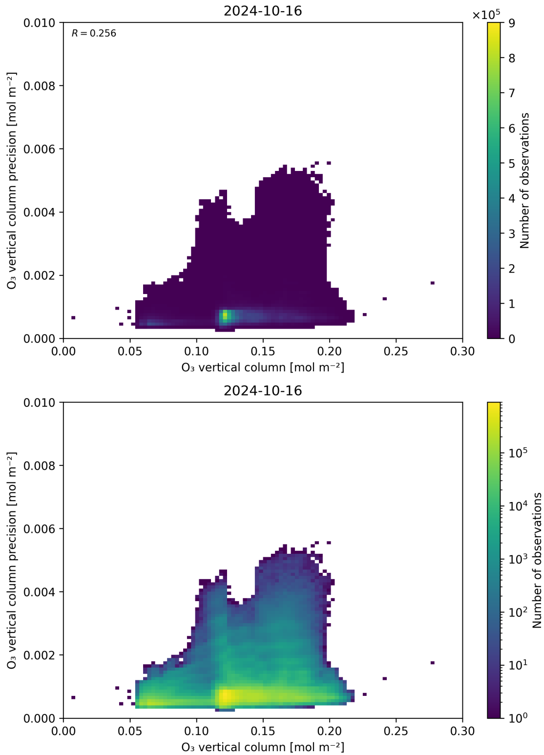
Figure 41: Scatter density plot of “O 3 vertical column” against “O 3 vertical column precision” for 2024-10-15 to 2024-10-17.
