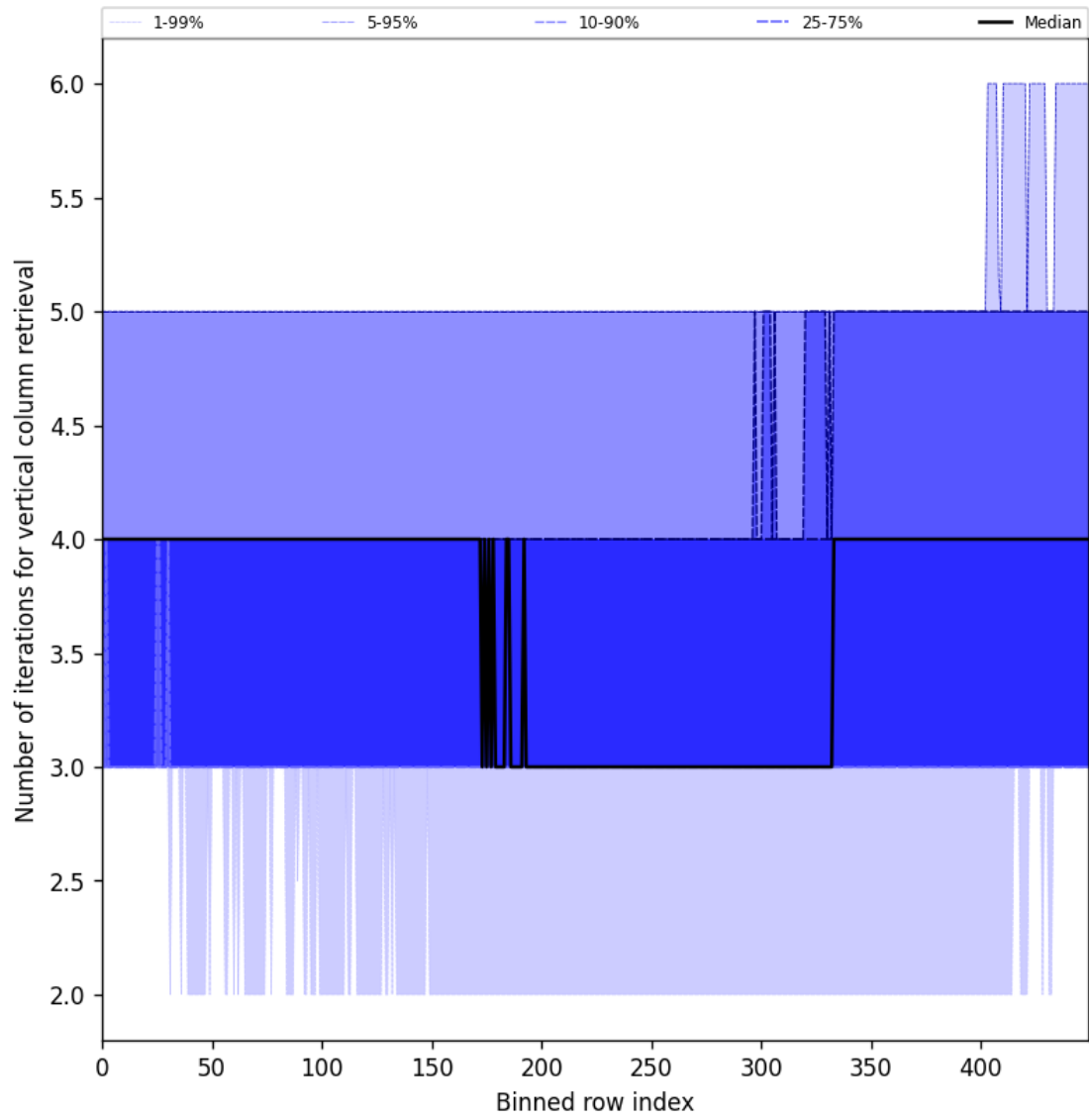
Figure 33: Along track statistics of “Number of iterations for vertical column retrieval” for 2024-10-15 to 2024-10-17
