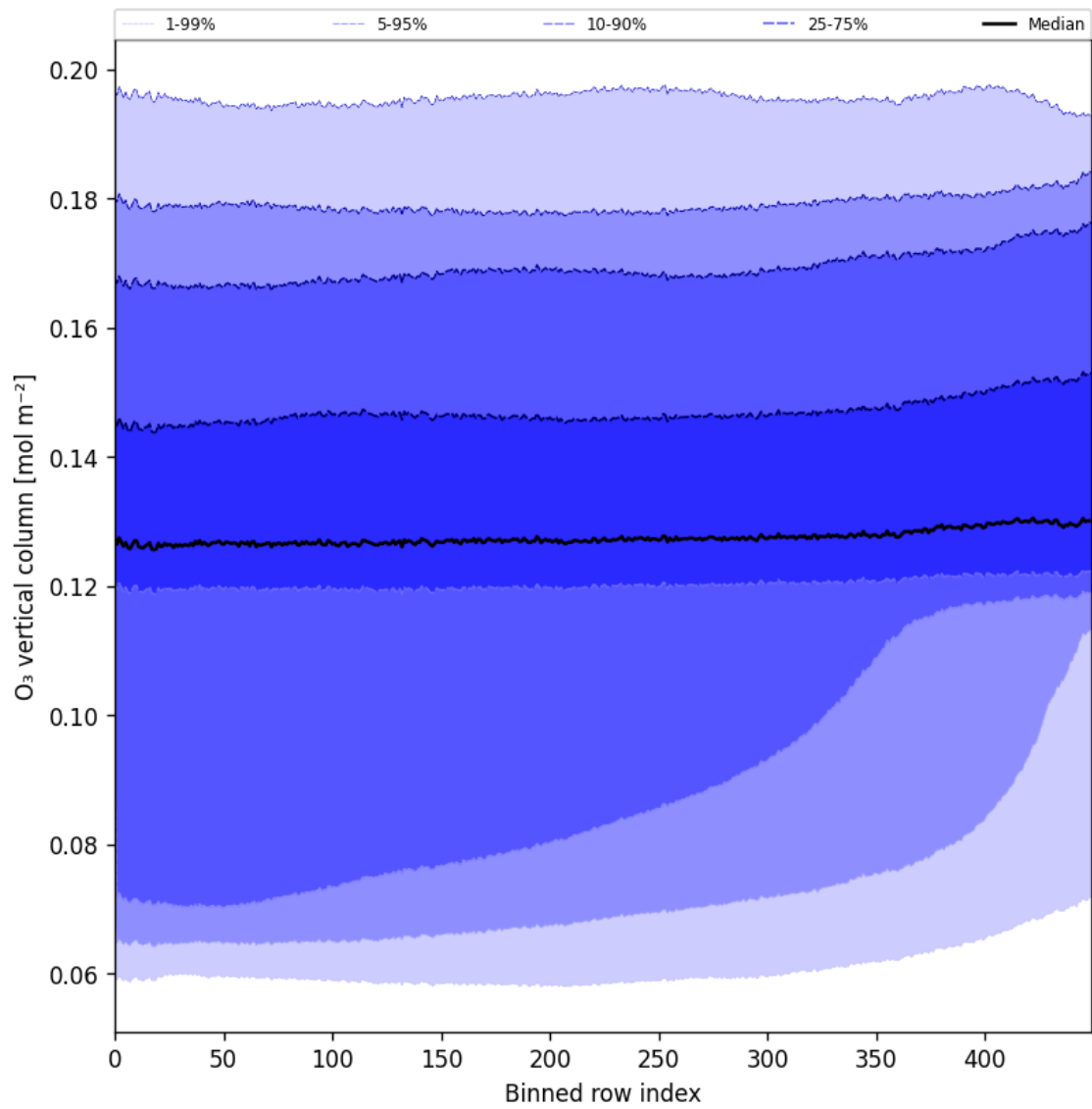
Figure 28: Along track statistics of “O 3 vertical column” for 2024-10-15 to 2024-10-17
