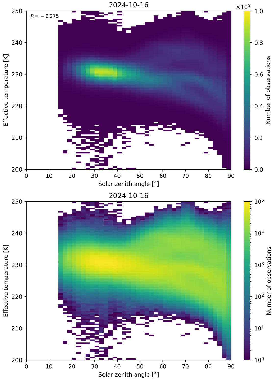
Figure 45: Scatter density plot of “Solar zenith angle” against “Effective temperature” for 2024-10-15 to 2024-10-17.
