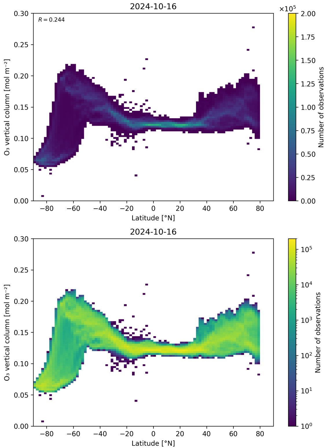
Figure 36: Scatter density plot of “Latitude” against “O 3 vertical column” for 2024-10-15 to 2024-10-17.
