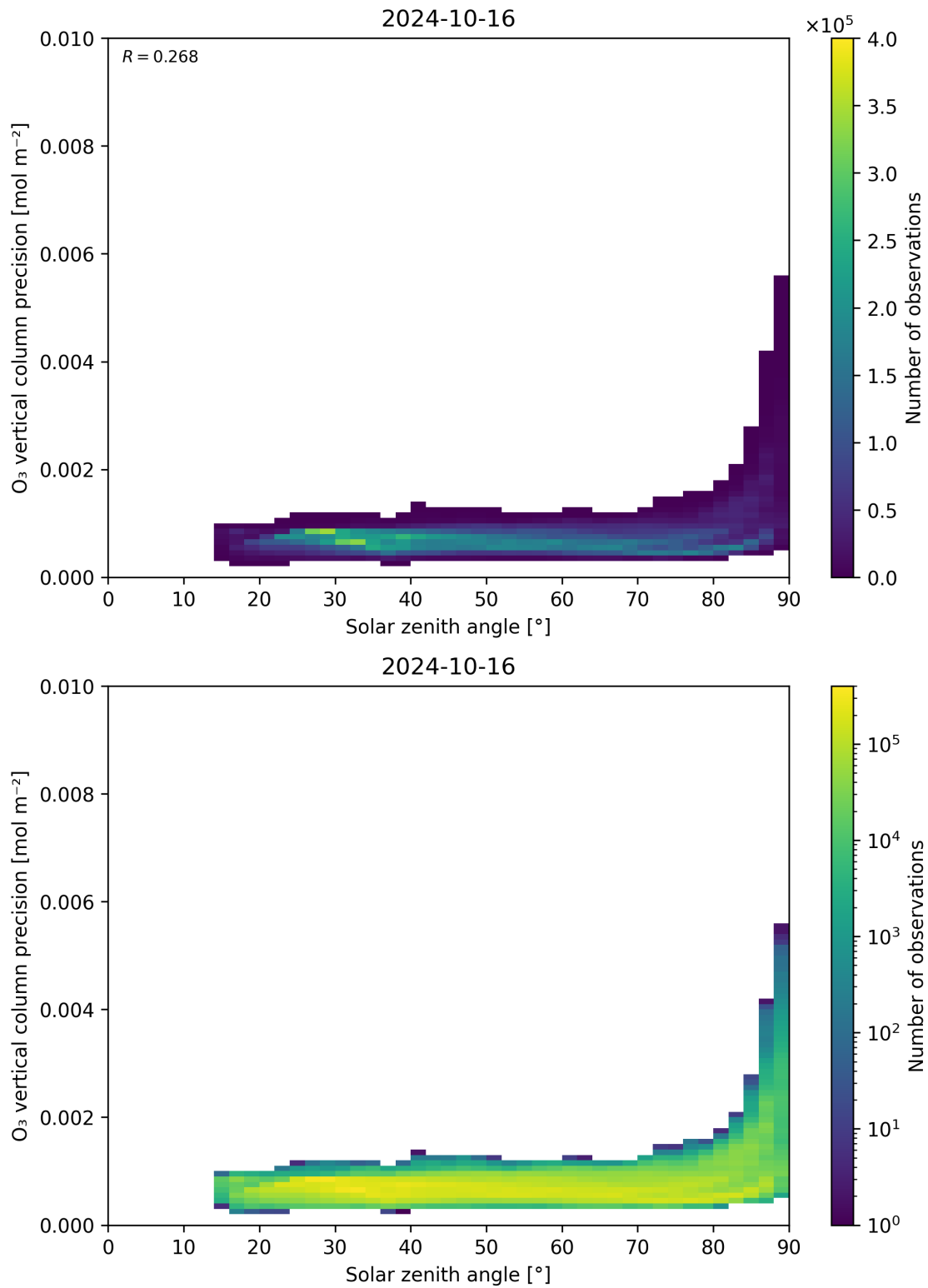
Figure 48: Scatter density plot of “Solar zenith angle” against “O 3 vertical column precision” for 2024-10-15 to 2024-10-17.
