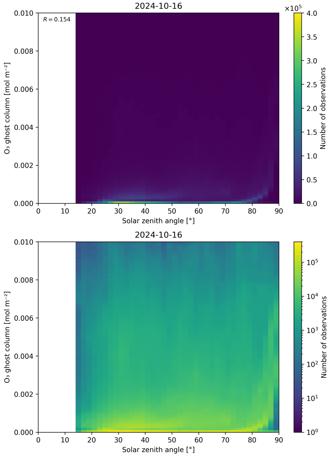
Figure 46: Scatter density plot of “Solar zenith angle” against “O 3 ghost column” for 2024-10-15 to 2024-10-17.
