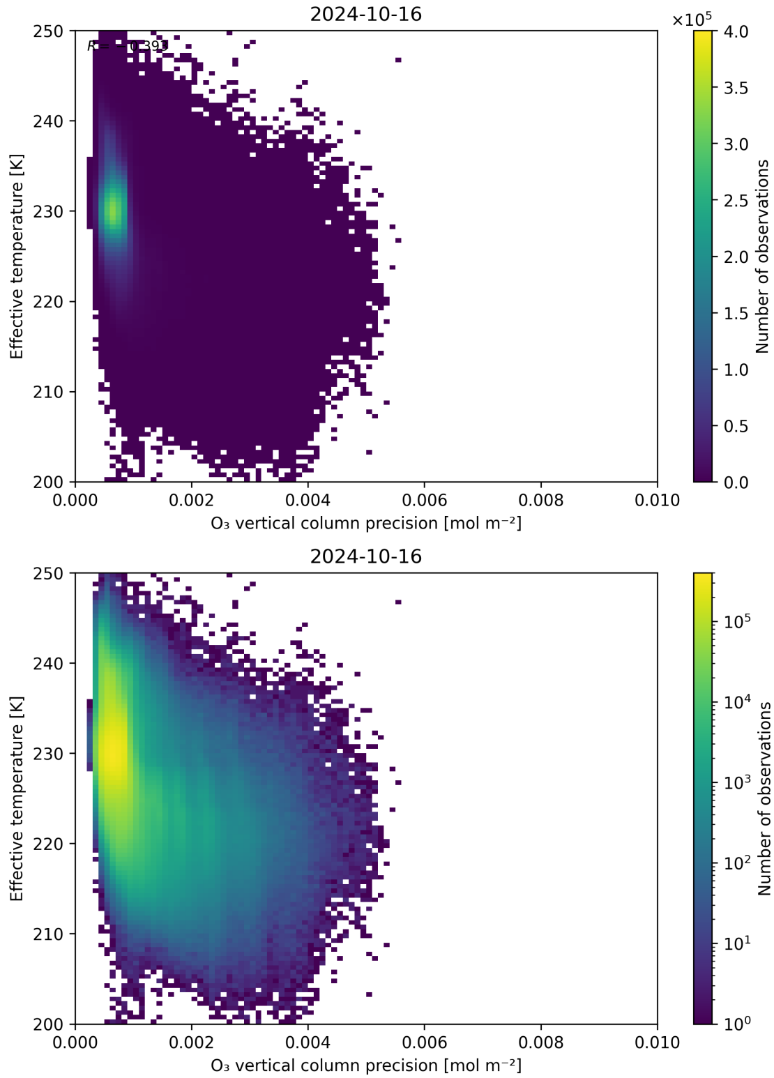
Figure 42: Scatter density plot of “O 3 vertical column precision” against “Effective temperature” for 2024-10-15 to 2024-10-17.
