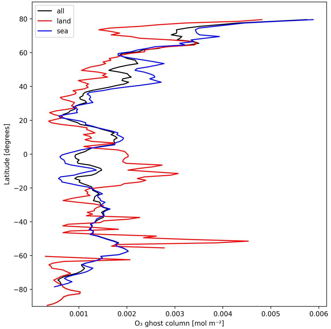
Figure 18: Zonal average of "O 3 ghost column" for 2024-10-15 to 2024-10-17.
