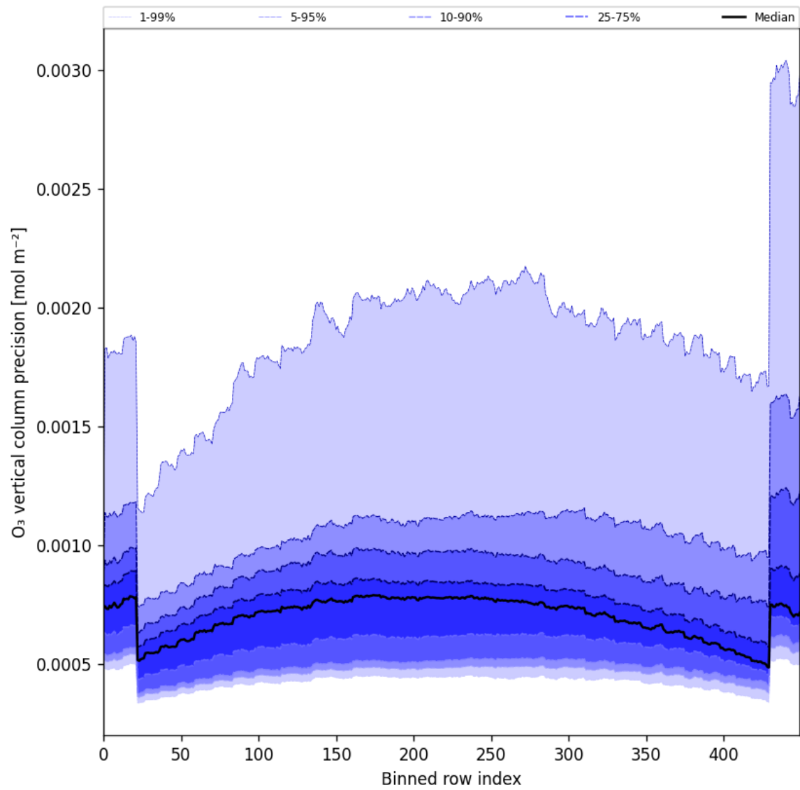
Figure 29: Along track statistics of “O 3 vertical column precision” for 2024-10-15 to 2024-10-17
