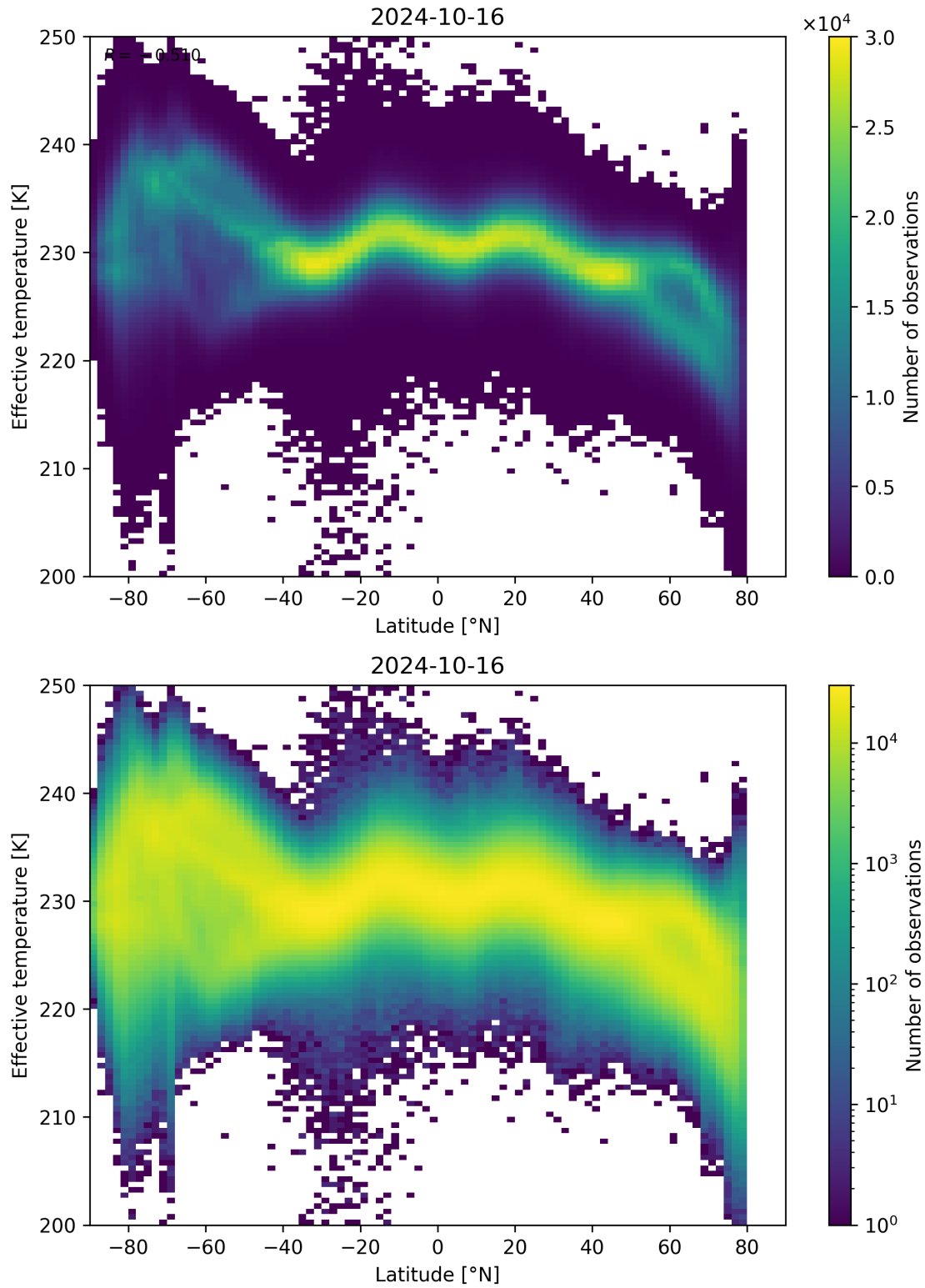
Figure 34: Scatter density plot of “Latitude” against “Effective temperature” for 2024-10-15 to 2024-10-17.
