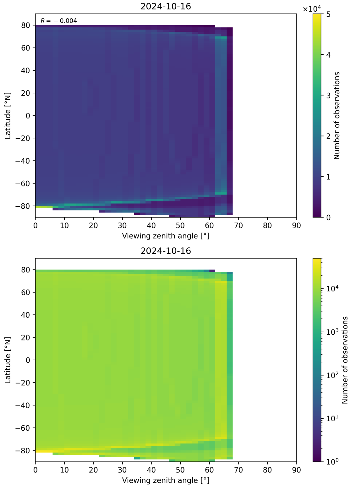
Figure 49: Scatter density plot of “Viewing zenith angle” against “Latitude” for 2024-10-15 to 2024-10-17.
