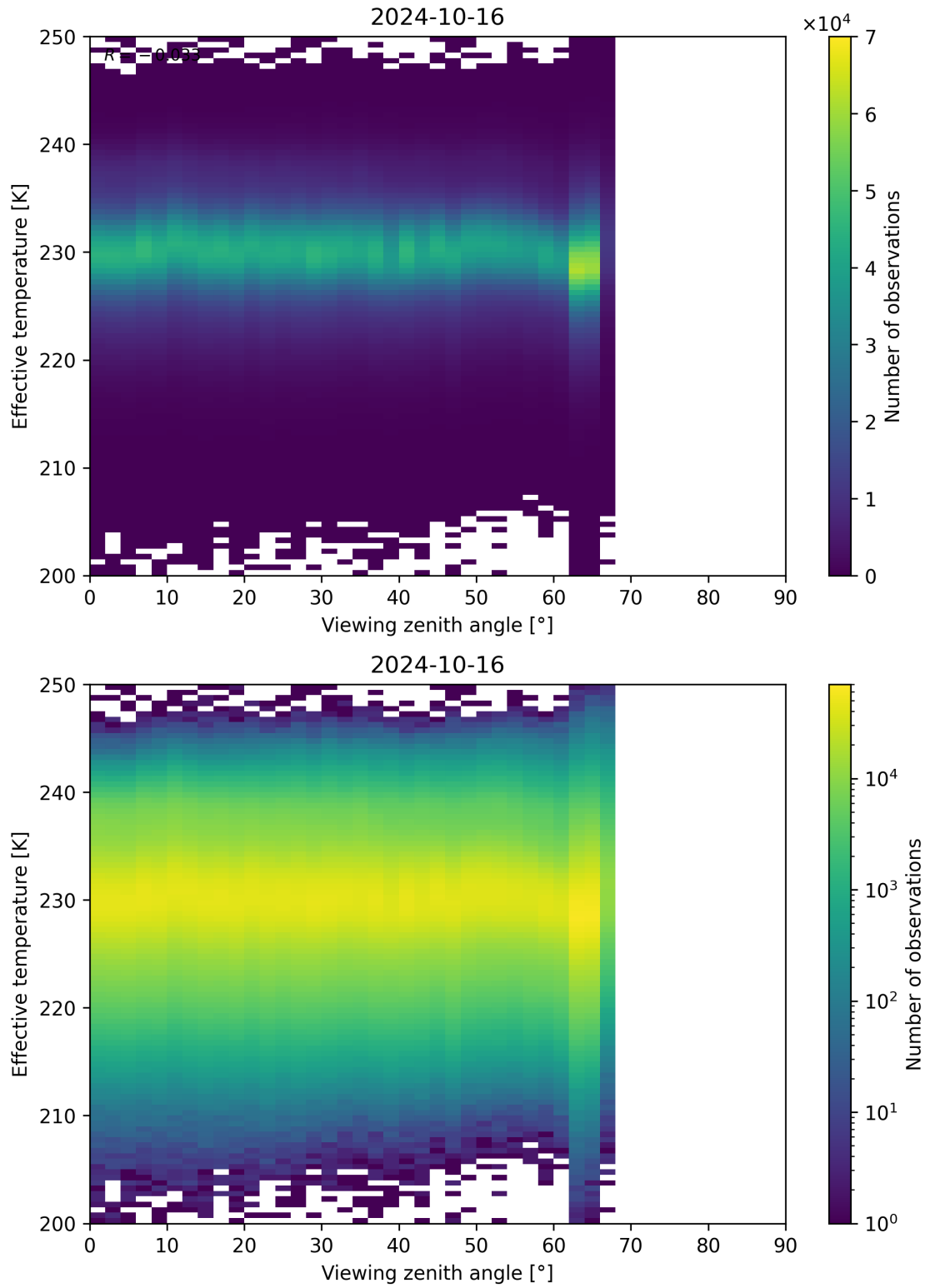
Figure 50: Scatter density plot of “Viewing zenith angle” against “Effective temperature” for 2024-10-15 to 2024-10-17.
