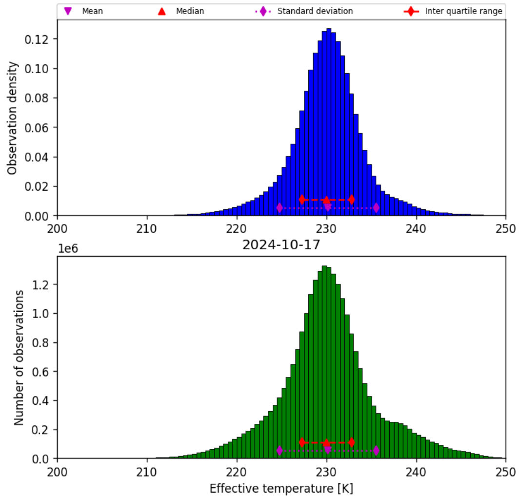
Figure 24: Histogram of “Effective temperature” for 2024-10-16 to 2024-10-18
