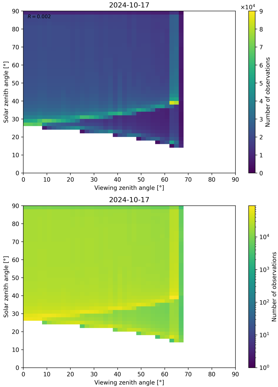
Figure 54: Scatter density plot of “Viewing zenith angle” against “Solar zenith angle” for 2024-10-16 to 2024-10-18.
