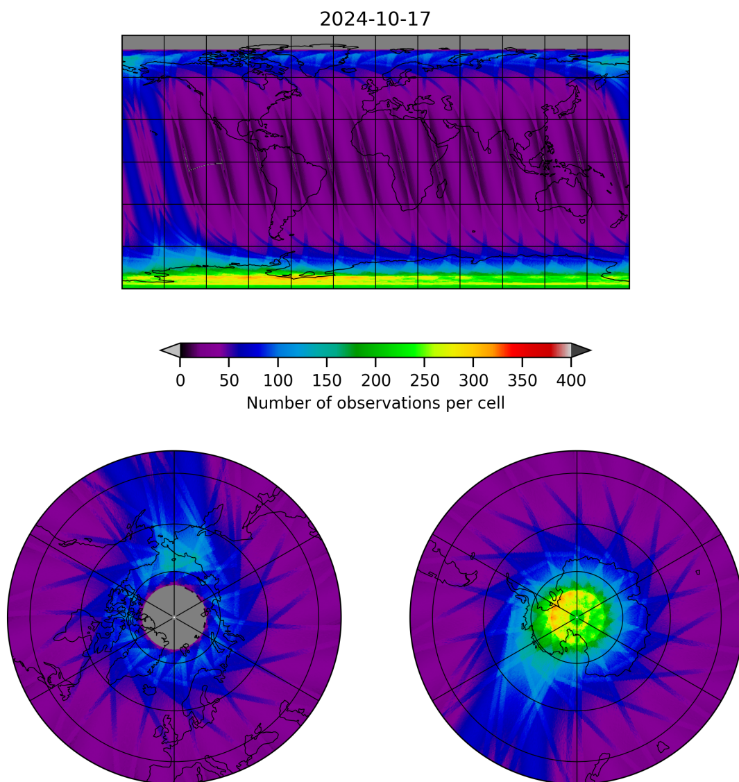
Figure 12: Map of the number of observations for 2024-10-16 to 2024-10-18
