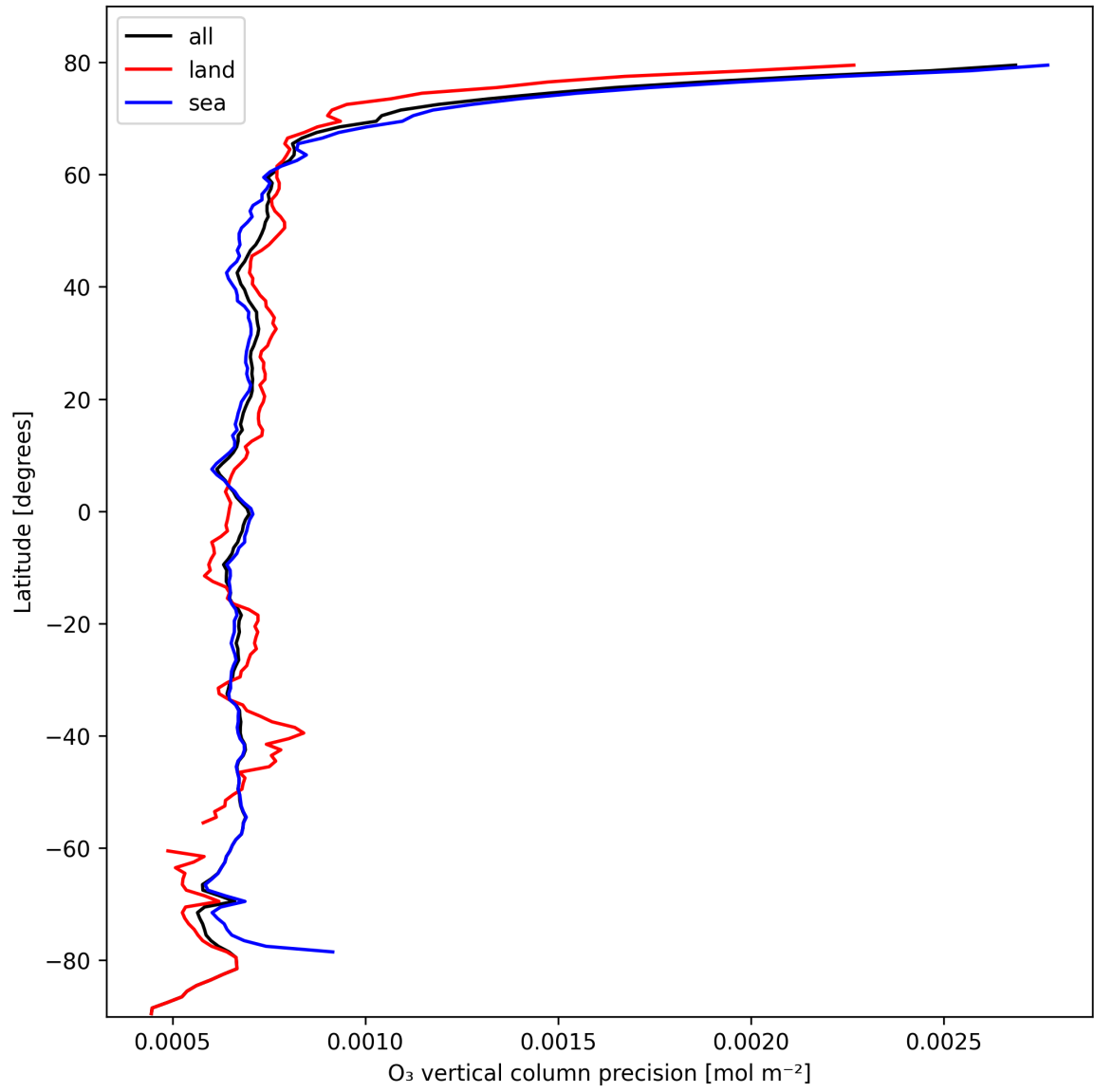
Figure 15: Zonal average of “O 3 vertical column precision” for 2024-10-16 to 2024-10-18.
