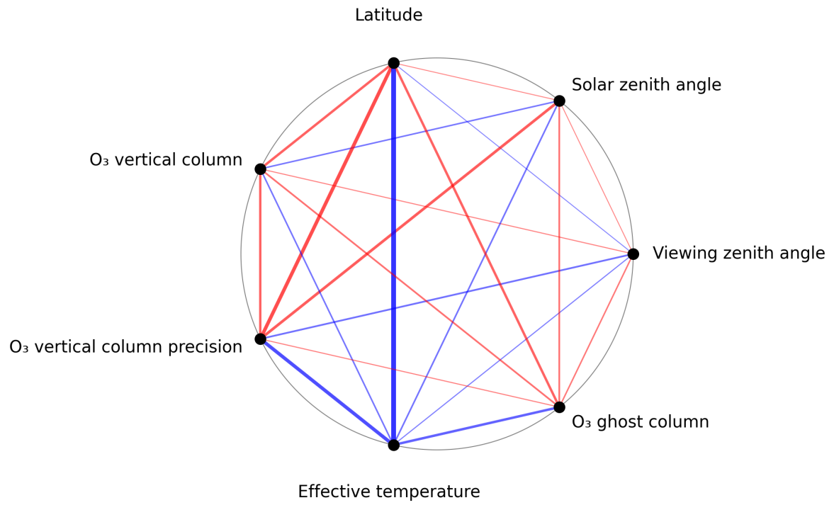
Figure 1: Map of correlation graph for 2024-10-16 to 2024-10-18.
