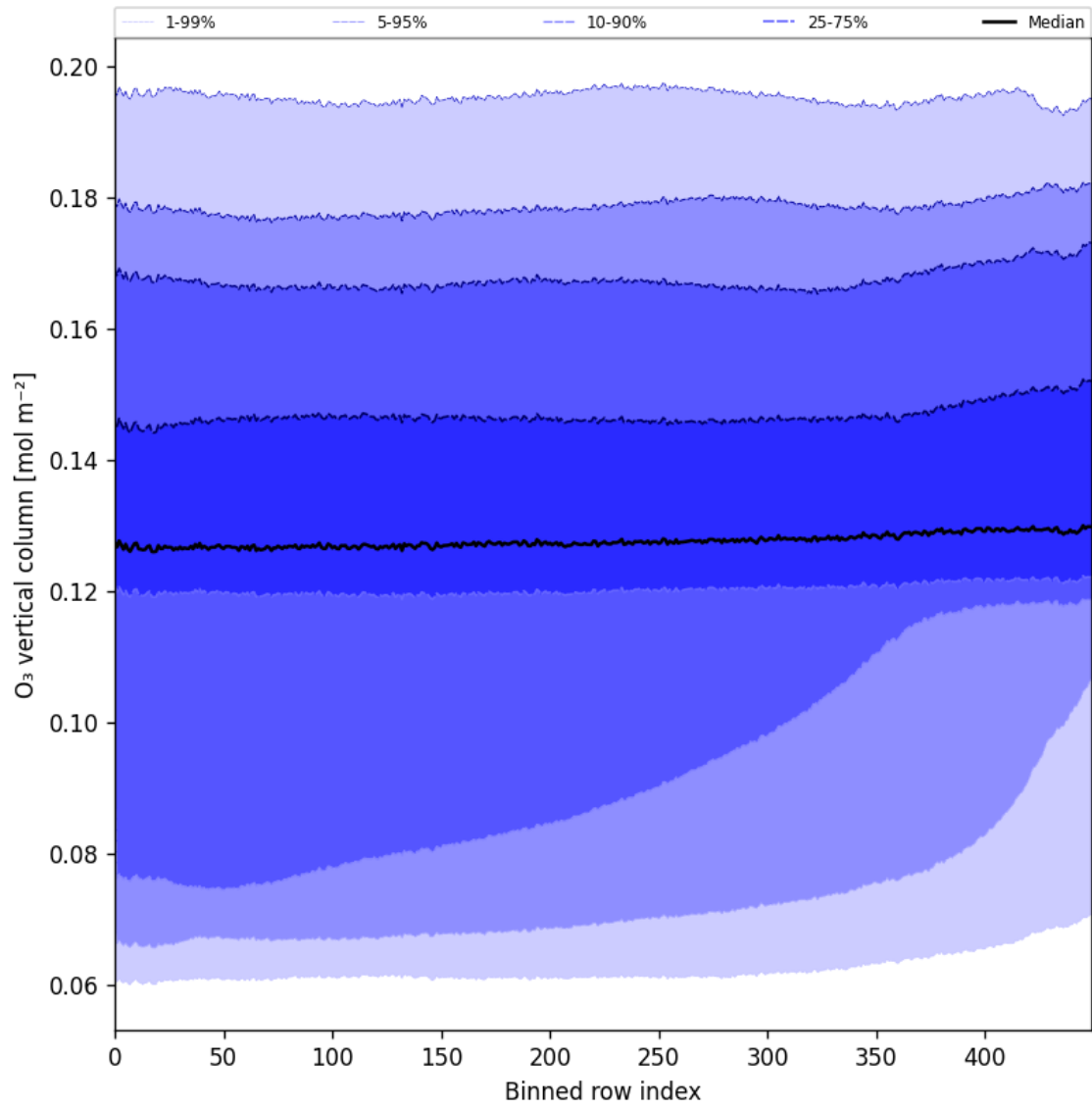
Figure 28: Along track statistics of “O 3 vertical column” for 2024-10-16 to 2024-10-18
