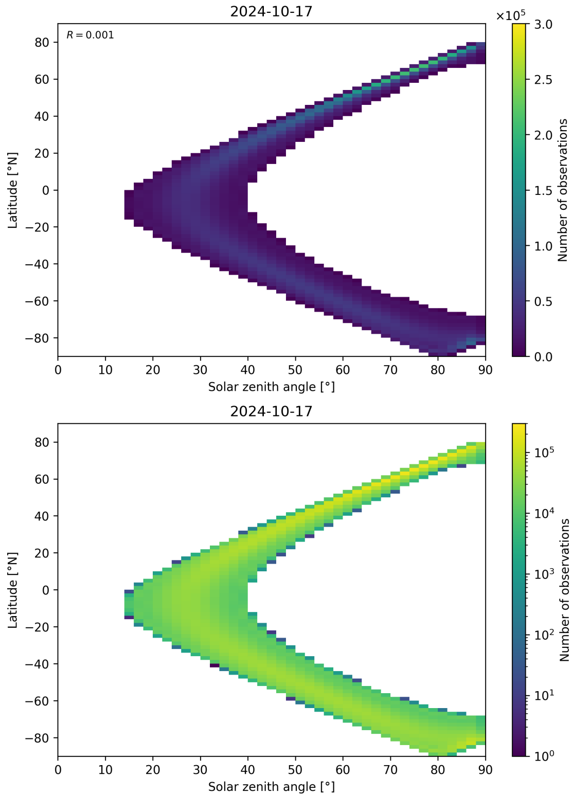
Figure 44: Scatter density plot of “Solar zenith angle” against “Latitude” for 2024-10-16 to 2024-10-18.
