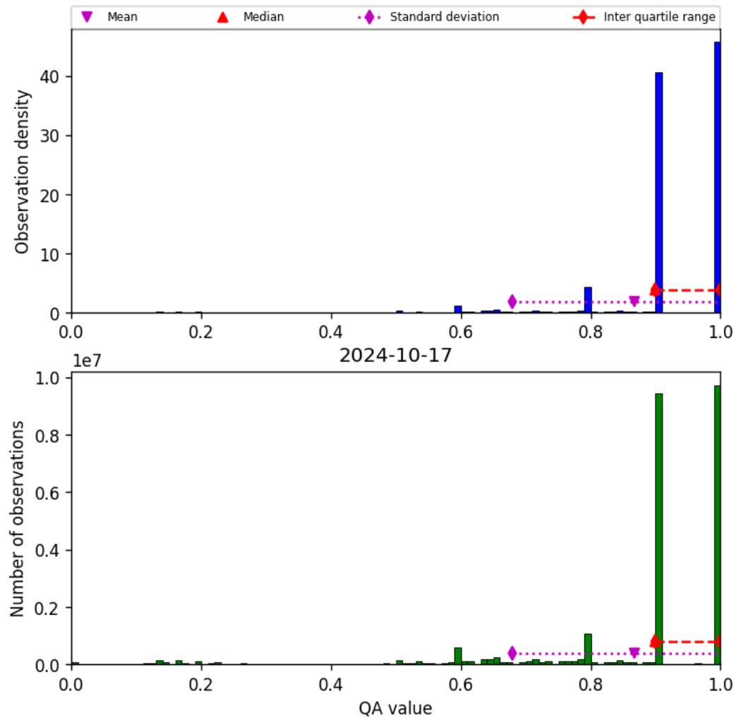
Figure 20: Histogram of “QA value” for 2024-10-16 to 2024-10-18
