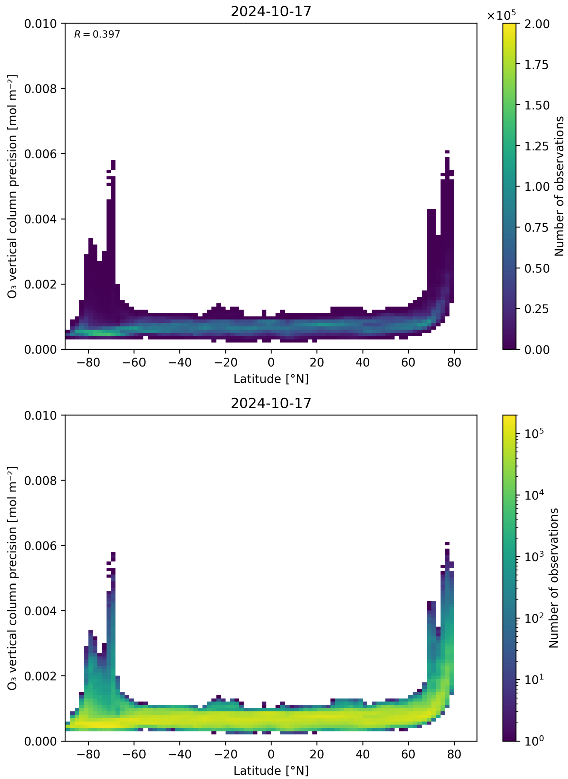
Figure 37: Scatter density plot of “Latitude” against “O 3 vertical column precision” for 2024-10-16 to 2024-10-18.
