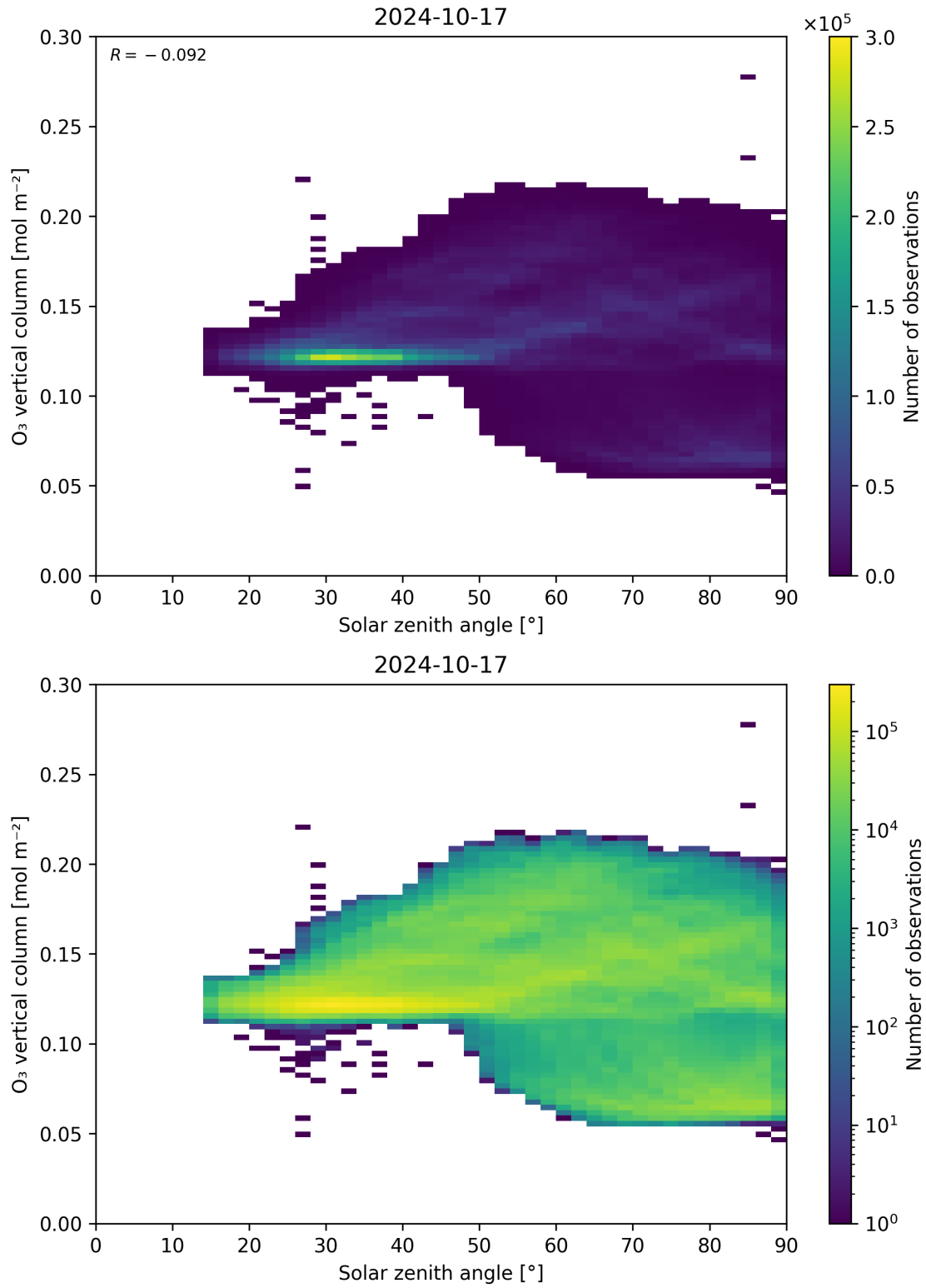
Figure 47: Scatter density plot of “Solar zenith angle” against “O 3 vertical column” for 2024-10-16 to 2024-10-18.
