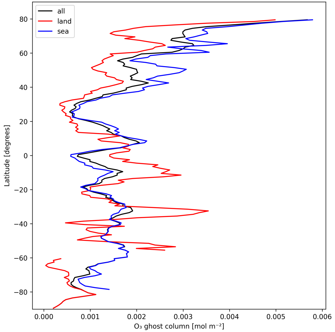
Figure 18: Zonal average of “O 3 ghost column” for 2024-10-16 to 2024-10-18.
