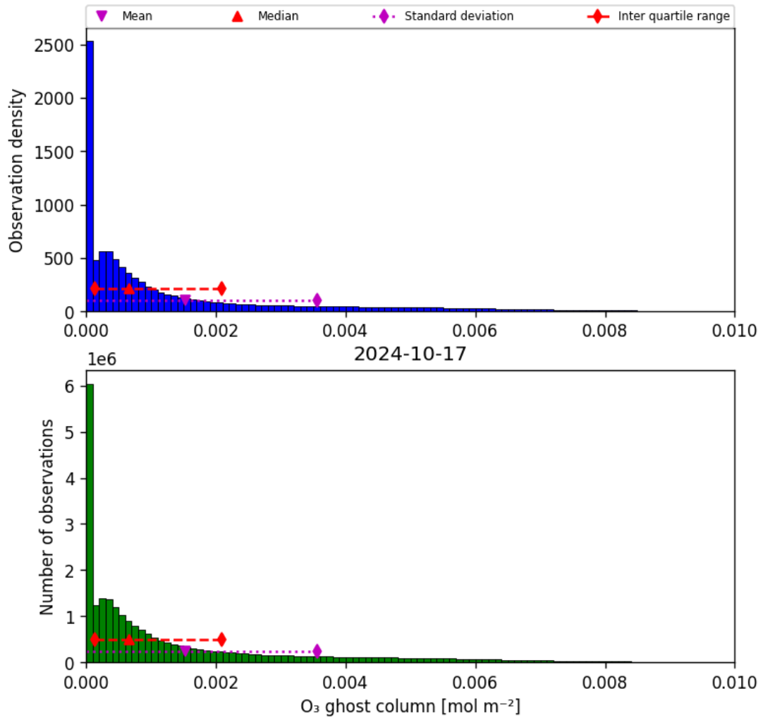
Figure 25: Histogram of “O 3 ghost column” for 2024-10-16 to 2024-10-18
