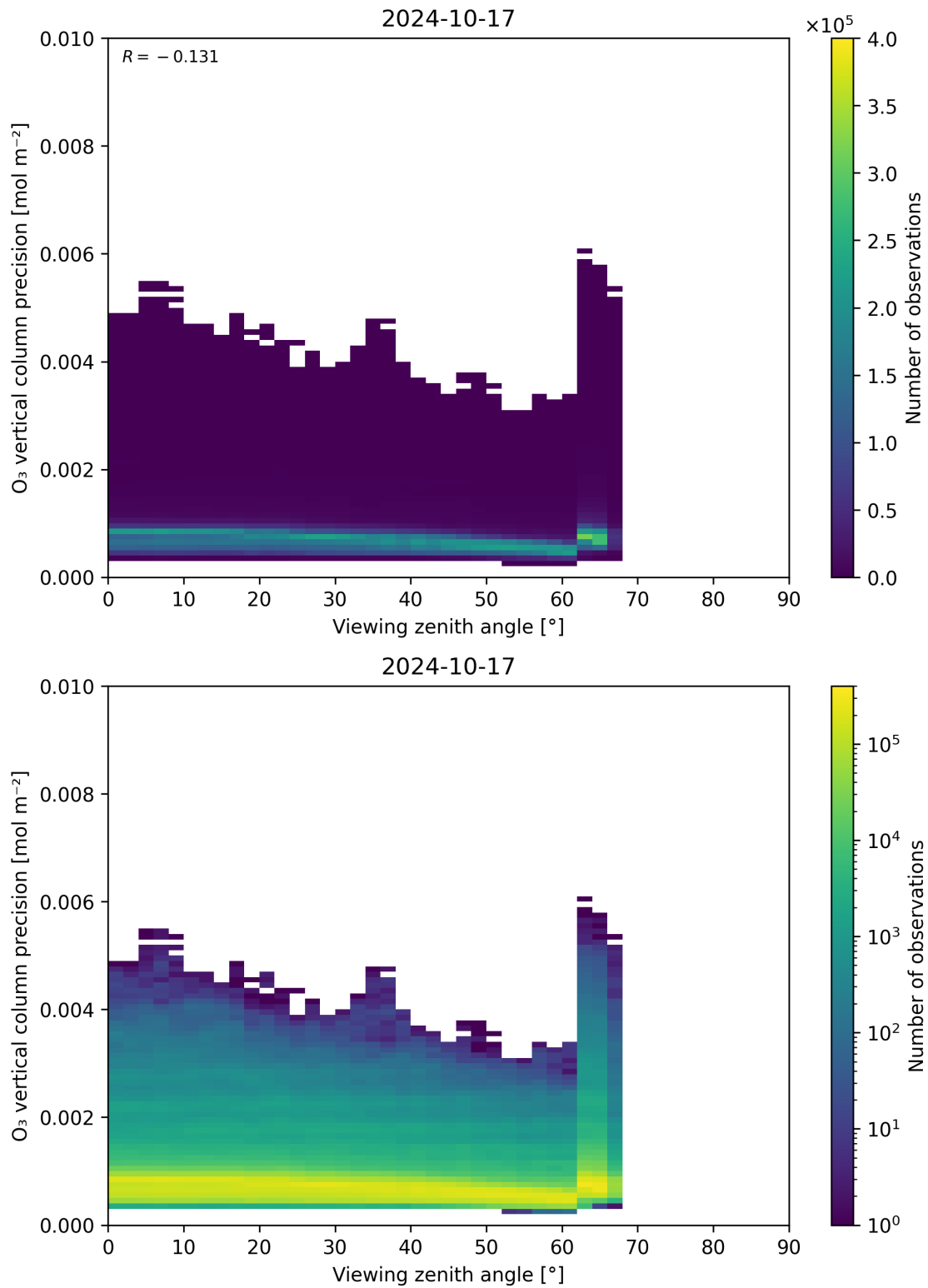
Figure 53: Scatter density plot of “Viewing zenith angle” against “O 3 vertical column precision” for 2024-10-16 to 2024-10-18.
