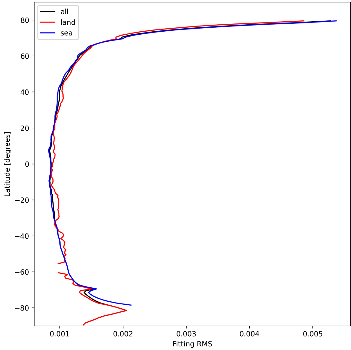
Figure 16: Zonal average of “Fitting RMS” for 2024-10-16 to 2024-10-18.
