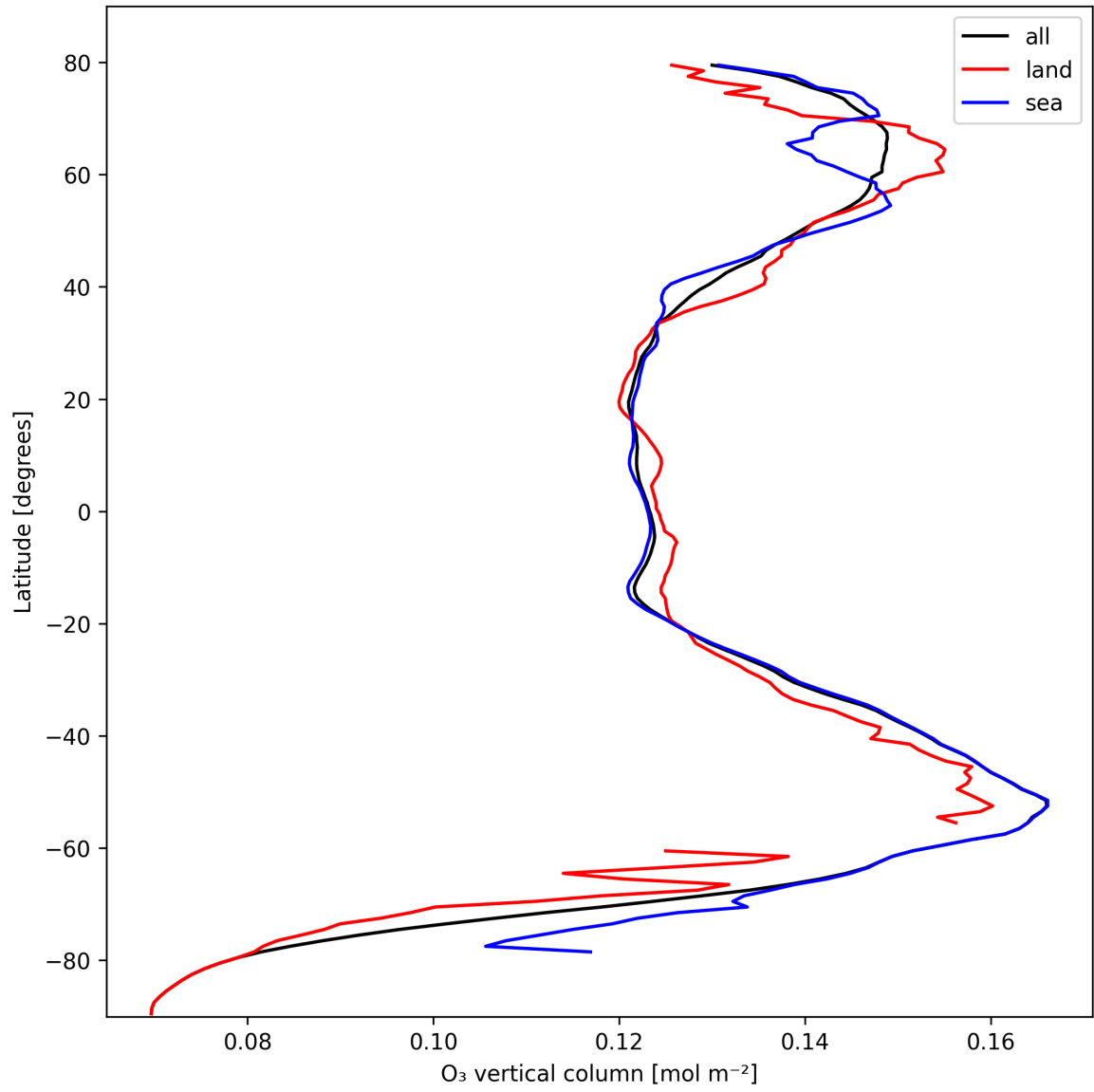
Figure 14: Zonal average of “O 3 vertical column” for 2024-10-16 to 2024-10-18.
