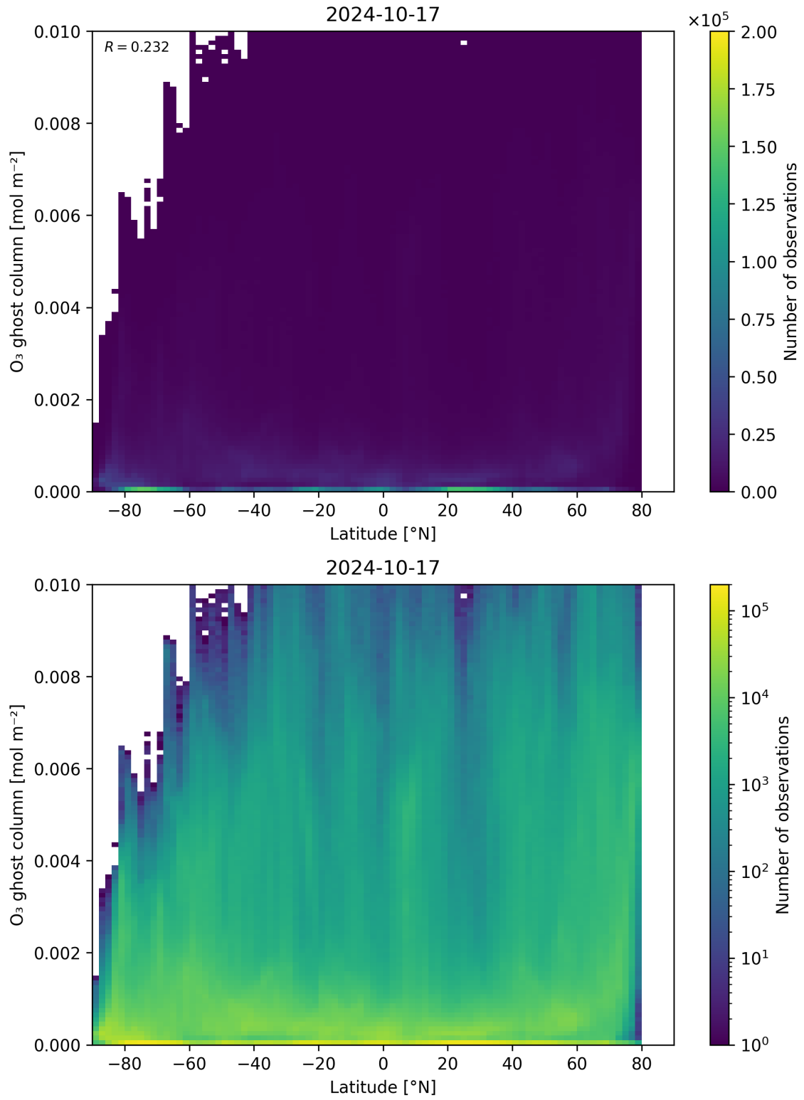
Figure 35: Scatter density plot of “Latitude” against “O 3 ghost column” for 2024-10-16 to 2024-10-18.
