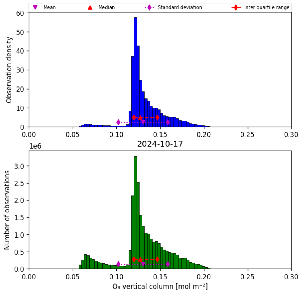
Figure 21: Histogram of “O 3 vertical column” for 2024-10-16 to 2024-10-18
