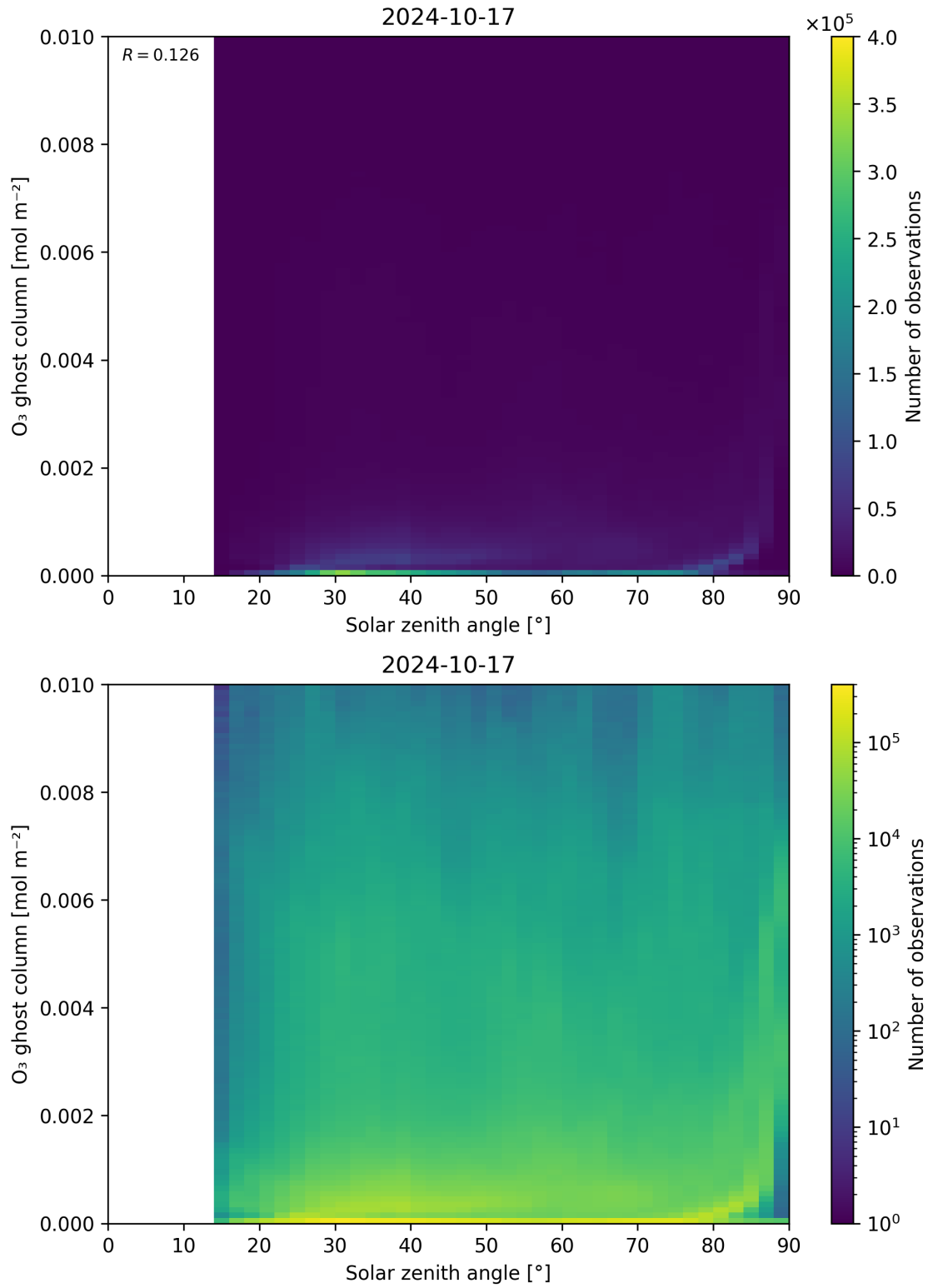
Figure 46: Scatter density plot of “Solar zenith angle” against “O 3 ghost column” for 2024-10-16 to 2024-10-18.
