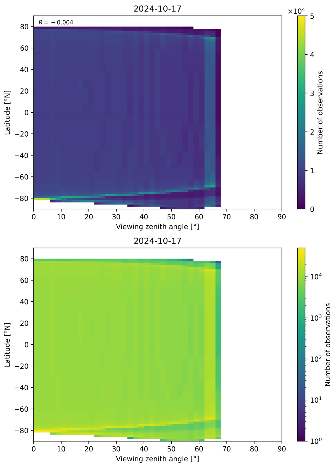
Figure 49: Scatter density plot of “Viewing zenith angle” against “Latitude” for 2024-10-16 to 2024-10-18.
