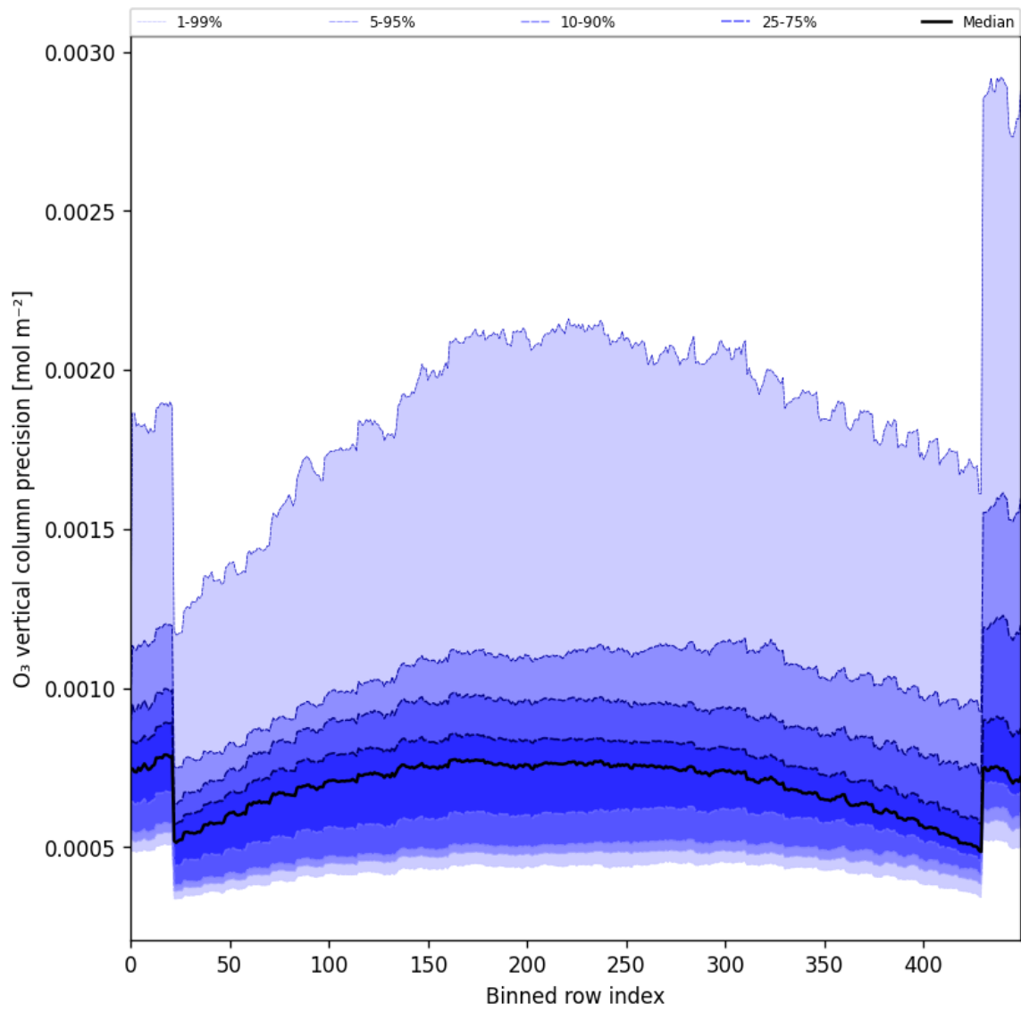
Figure 29: Along track statistics of “O 3 vertical column precision” for 2024-10-16 to 2024-10-18
