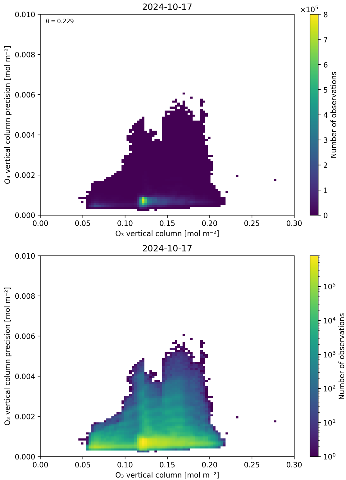
Figure 41: Scatter density plot of “O 3 vertical column” against “O 3 vertical column precision” for 2024-10-16 to 2024-10-18.
