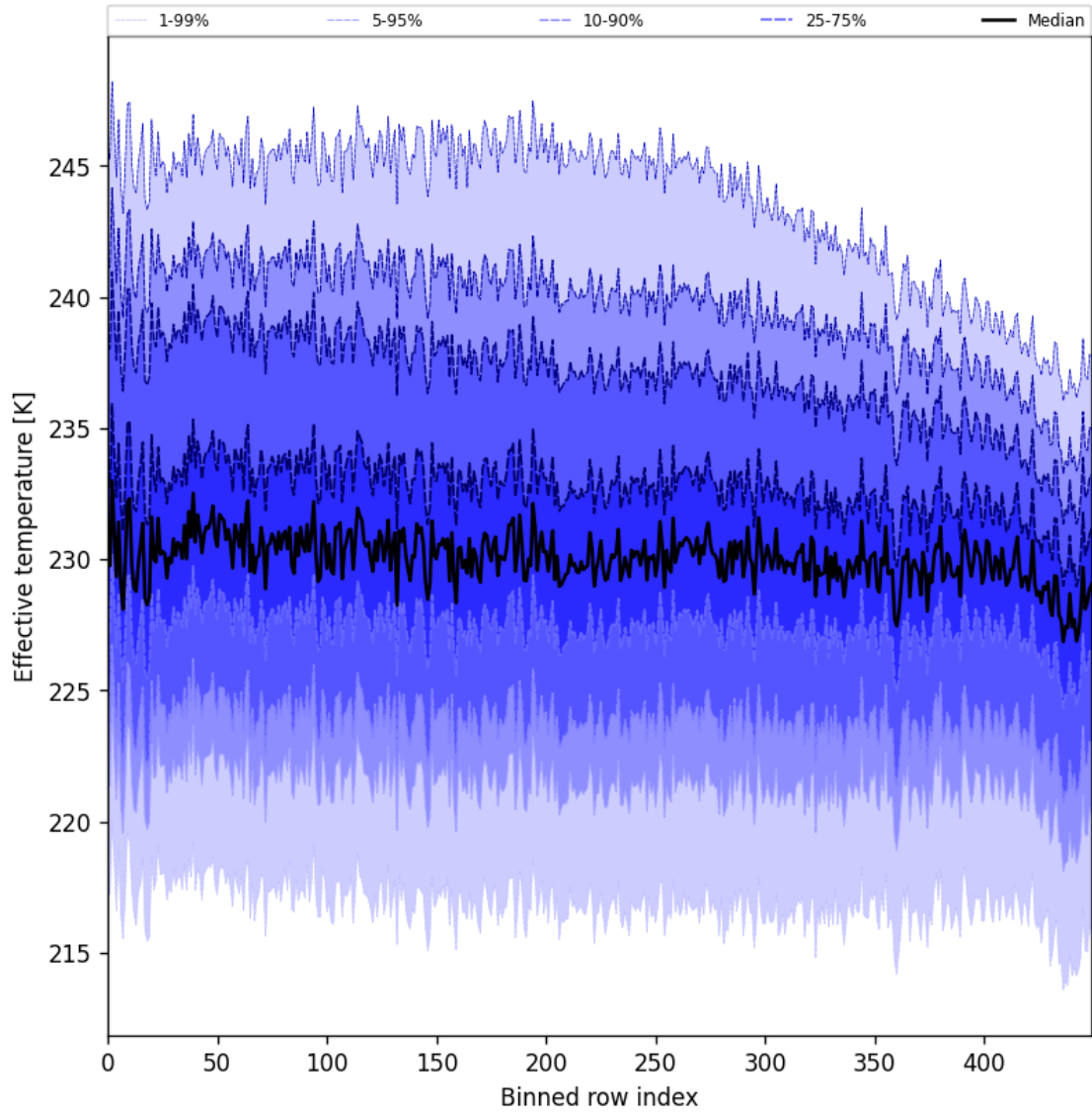
Figure 31: Along track statistics of “Effective temperature” for 2024-10-16 to 2024-10-18
