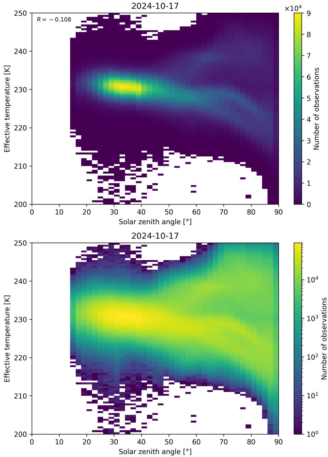
Figure 45: Scatter density plot of “Solar zenith angle” against “Effective temperature” for 2024-10-16 to 2024-10-18.
