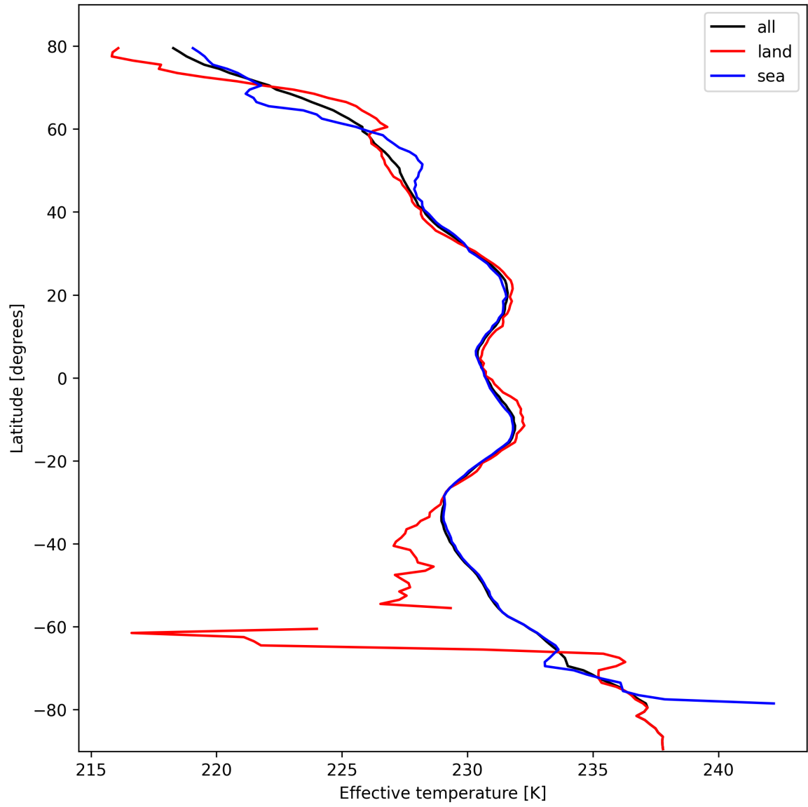
Figure 17: Zonal average of "Effective temperature" for 2024-10-16 to 2024-10-18.
