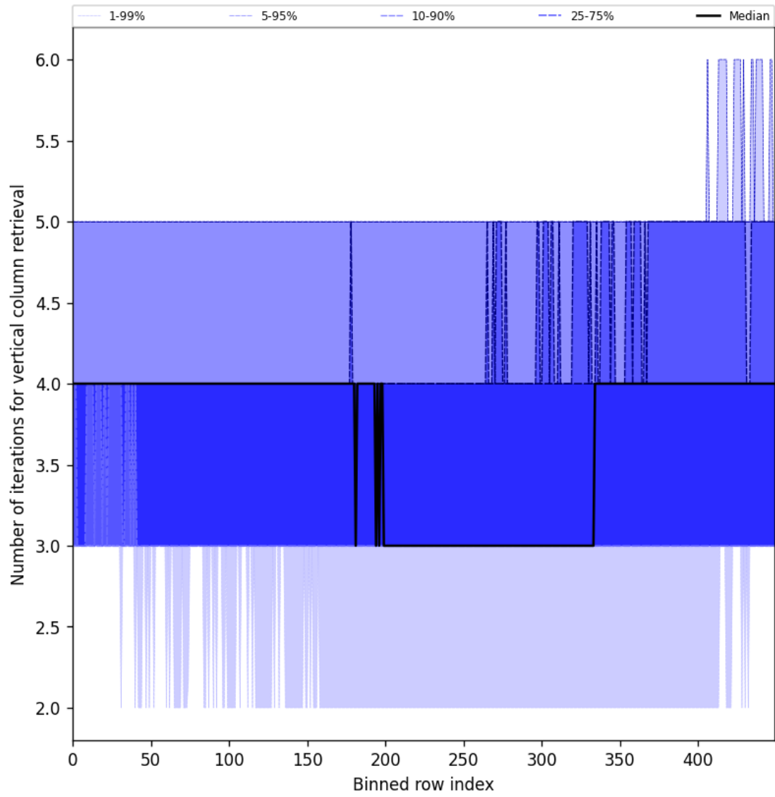
Figure 33: Along track statistics of “Number of iterations for vertical column retrieval” for 2024-10-16 to 2024-10-18
