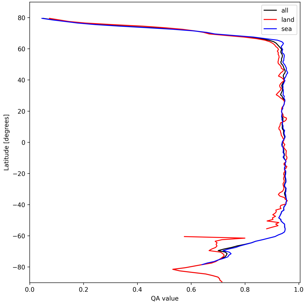
Figure 13: Zonal average of “QA value” for 2024-10-16 to 2024-10-18.
