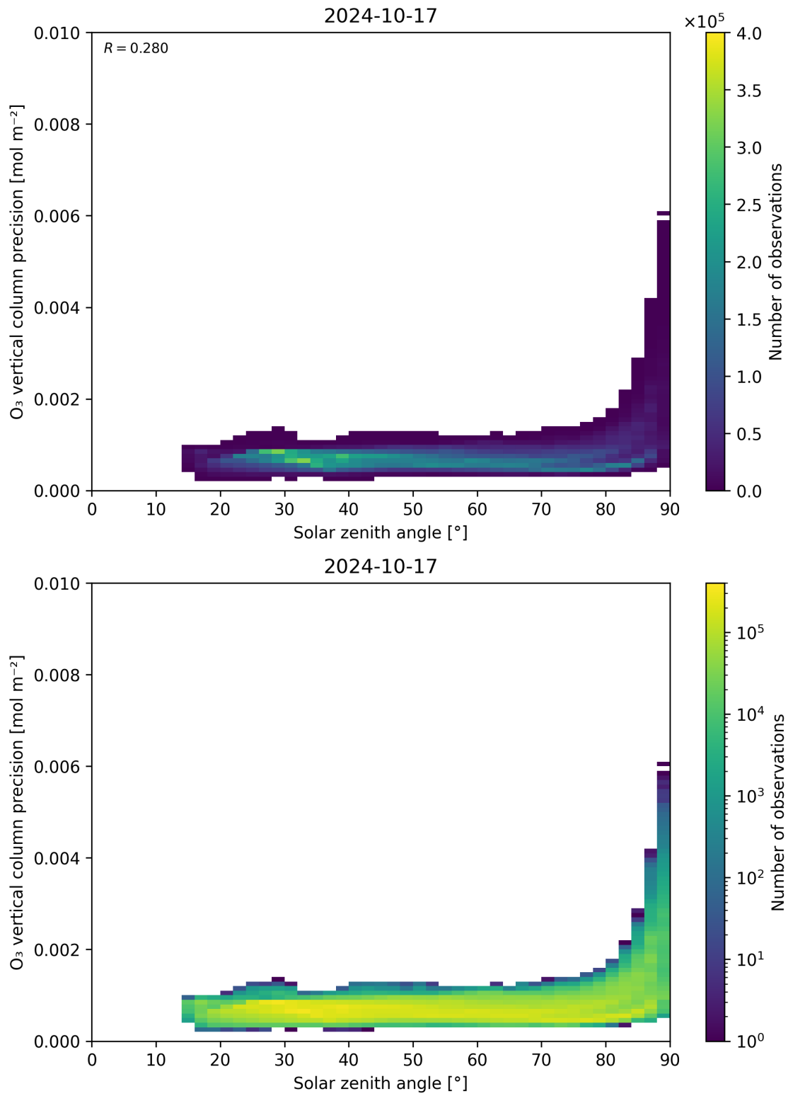
Figure 48: Scatter density plot of “Solar zenith angle” against “O 3 vertical column precision” for 2024-10-16 to 2024-10-18.
