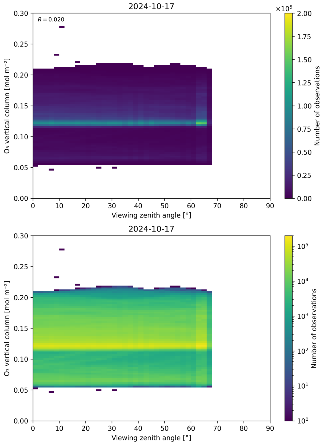
Figure 52: Scatter density plot of “Viewing zenith angle” against “O 3 vertical column” for 2024-10-16 to 2024-10-18.
