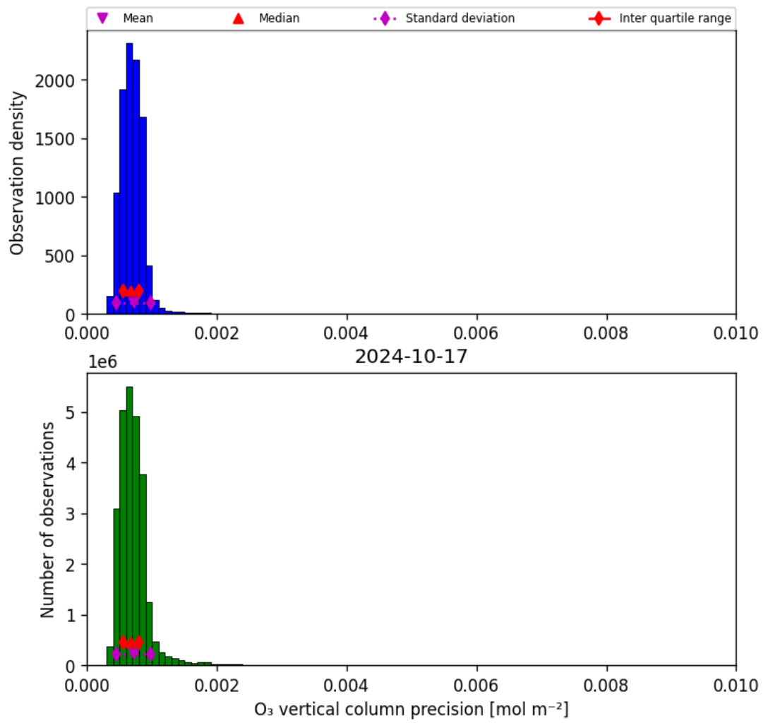
Figure 22: Histogram of “O 3 vertical column precision” for 2024-10-16 to 2024-10-18
