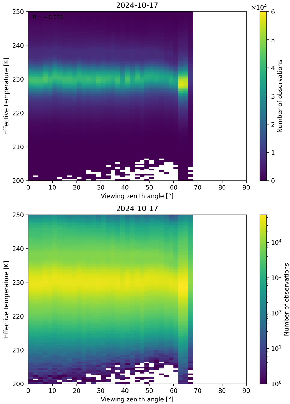
Figure 50: Scatter density plot of “Viewing zenith angle” against “Effective temperature” for 2024-10-16 to 2024-10-18.
