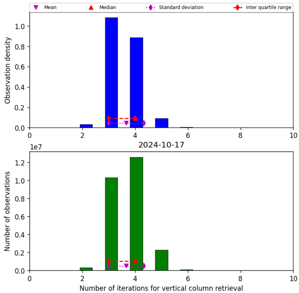
Figure 26: Histogram of “Number of iterations for vertical column retrieval” for 2024-10-16 to 2024-10-18
