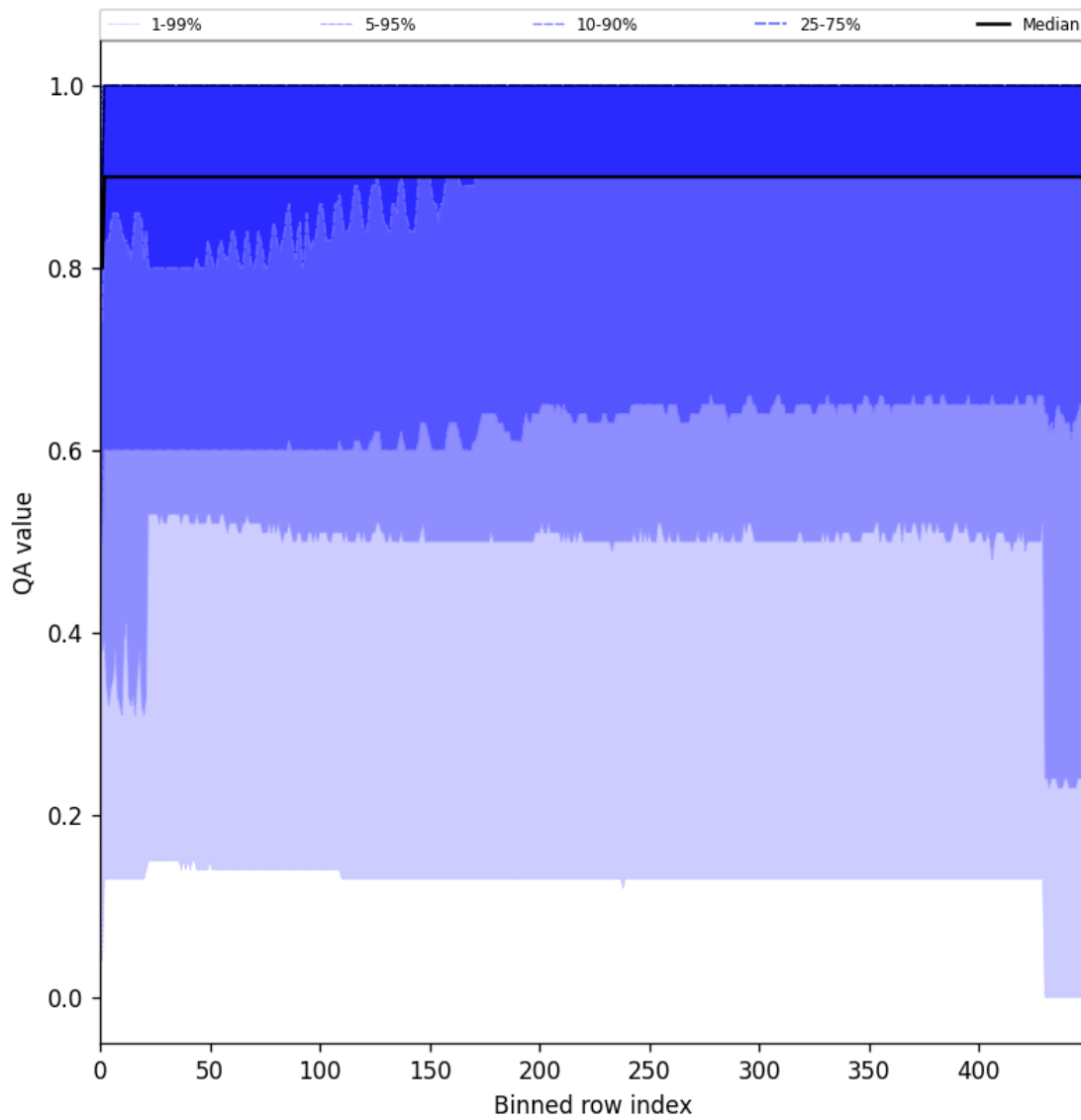
Figure 27: Along track statistics of “QA value” for 2024-10-16 to 2024-10-18
