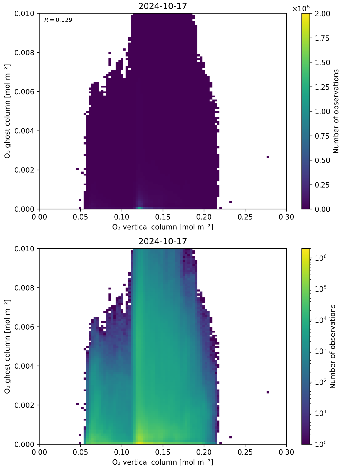
Figure 40: Scatter density plot of “O 3 vertical column” against “O 3 ghost column” for 2024-10-16 to 2024-10-18.
