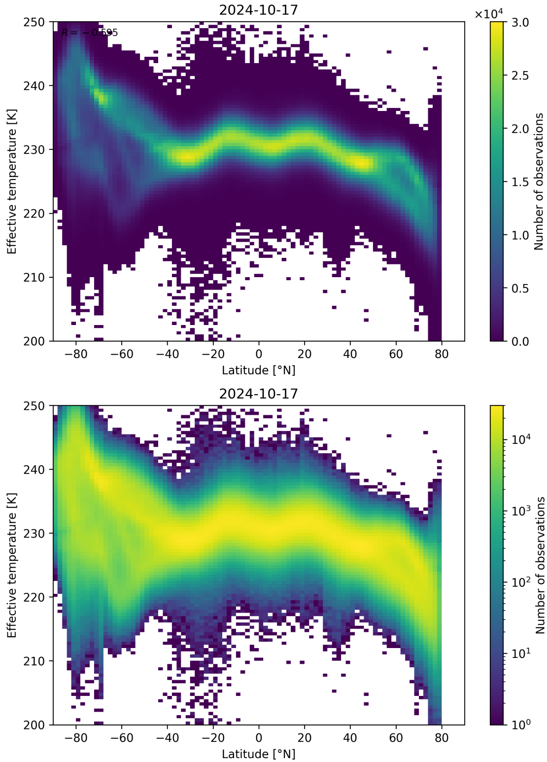
Figure 34: Scatter density plot of “Latitude” against “Effective temperature” for 2024-10-16 to 2024-10-18.
