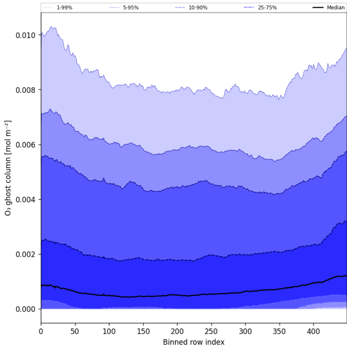
Figure 32: Along track statistics of “O 3 ghost column” for 2024-10-16 to 2024-10-18
