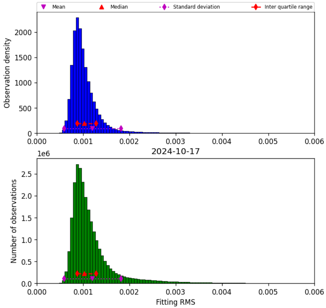
Figure 23: Histogram of “Fitting RMS” for 2024-10-16 to 2024-10-18
