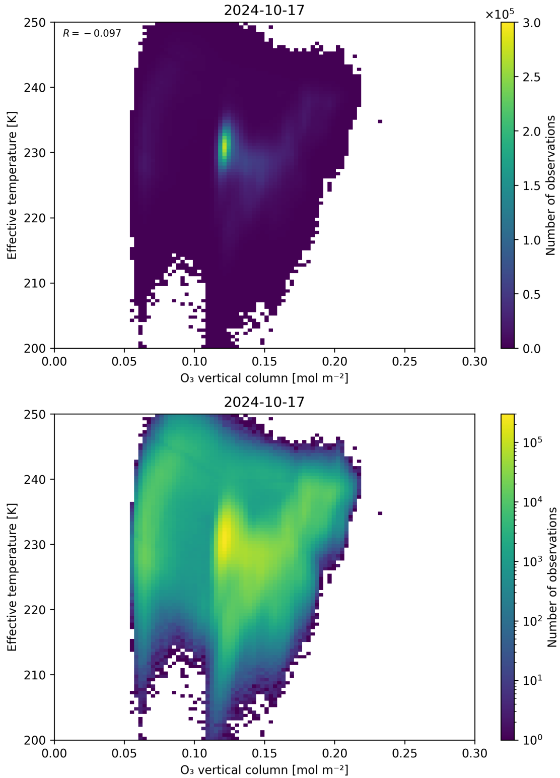
Figure 39: Scatter density plot of “O 3 vertical column” against “Effective temperature” for 2024-10-16 to 2024-10-18.
