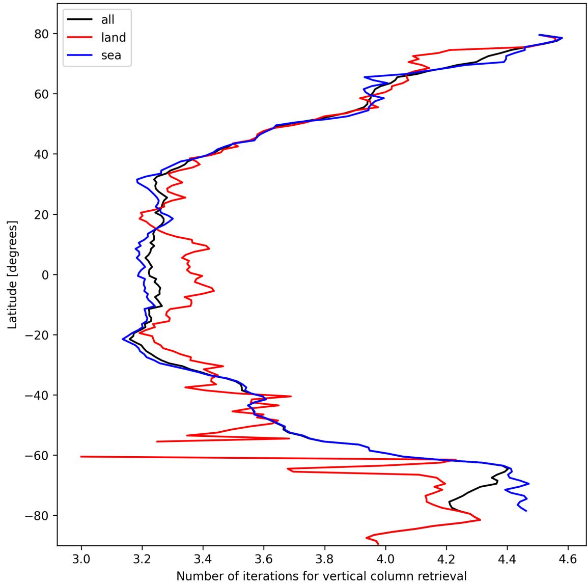
Figure 19: Zonal average of “Number of iterations for vertical column retrieval” for 2024-10-16 to 2024-10-18.
