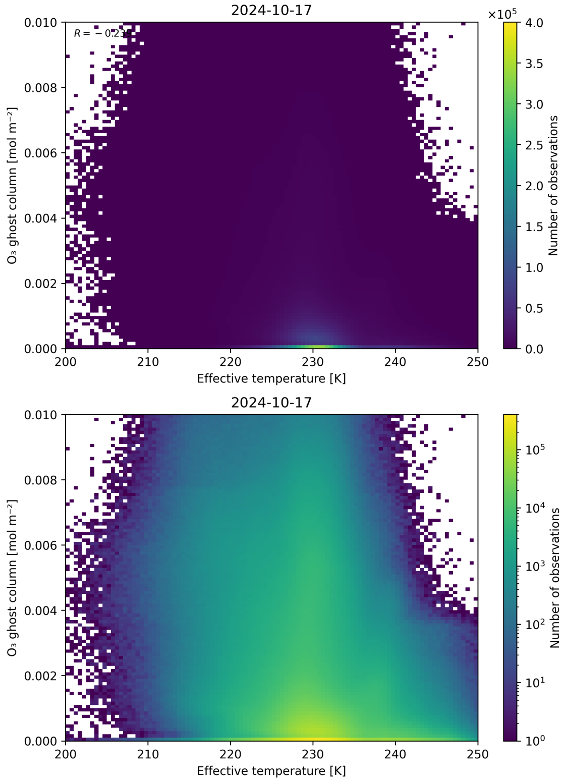
Figure 38: Scatter density plot of “Effective temperature” against “O 3 ghost column” for 2024-10-16 to 2024-10-18.
