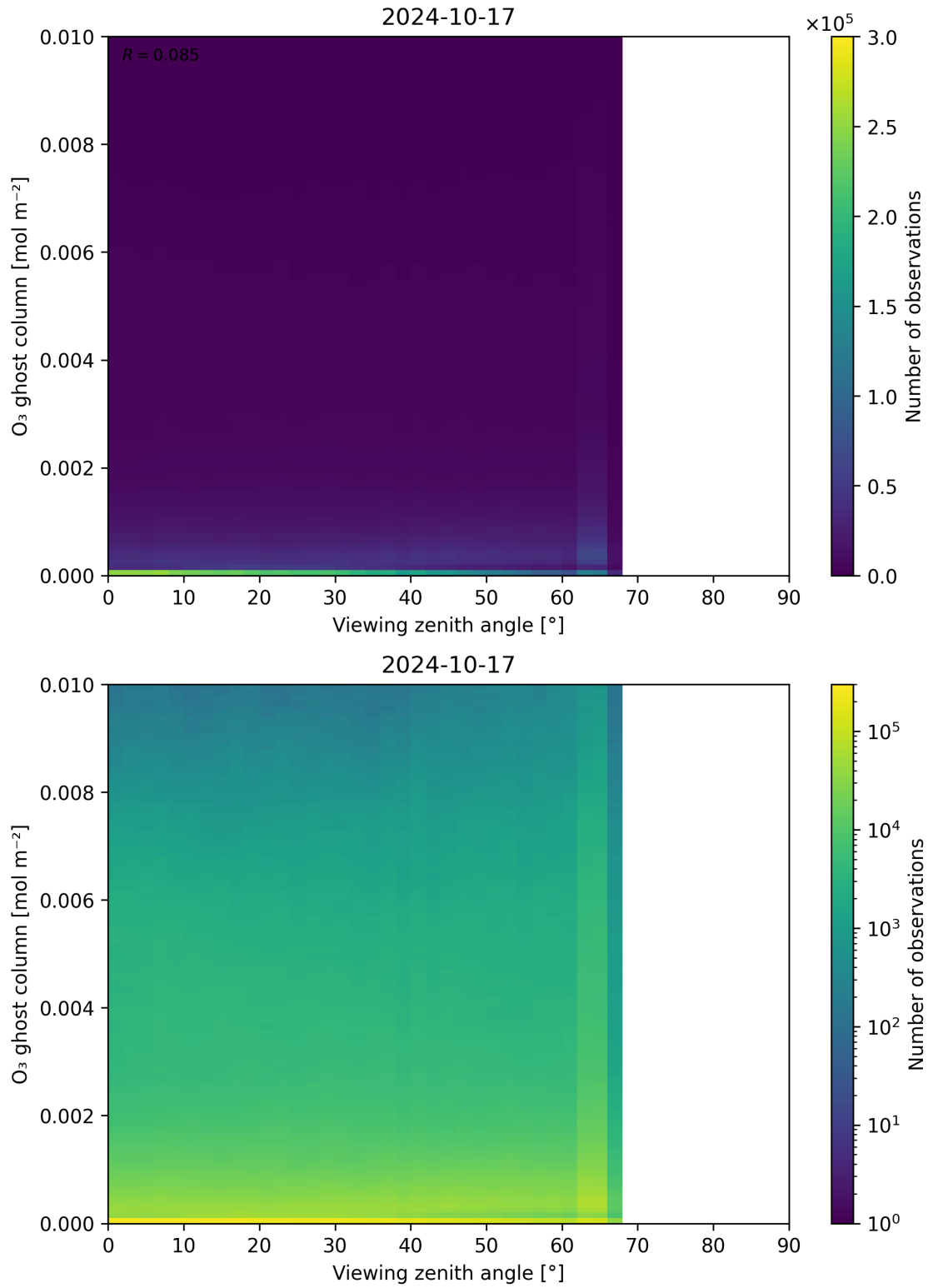
Figure 51: Scatter density plot of “Viewing zenith angle” against “O 3 ghost column” for 2024-10-16 to 2024-10-18.
