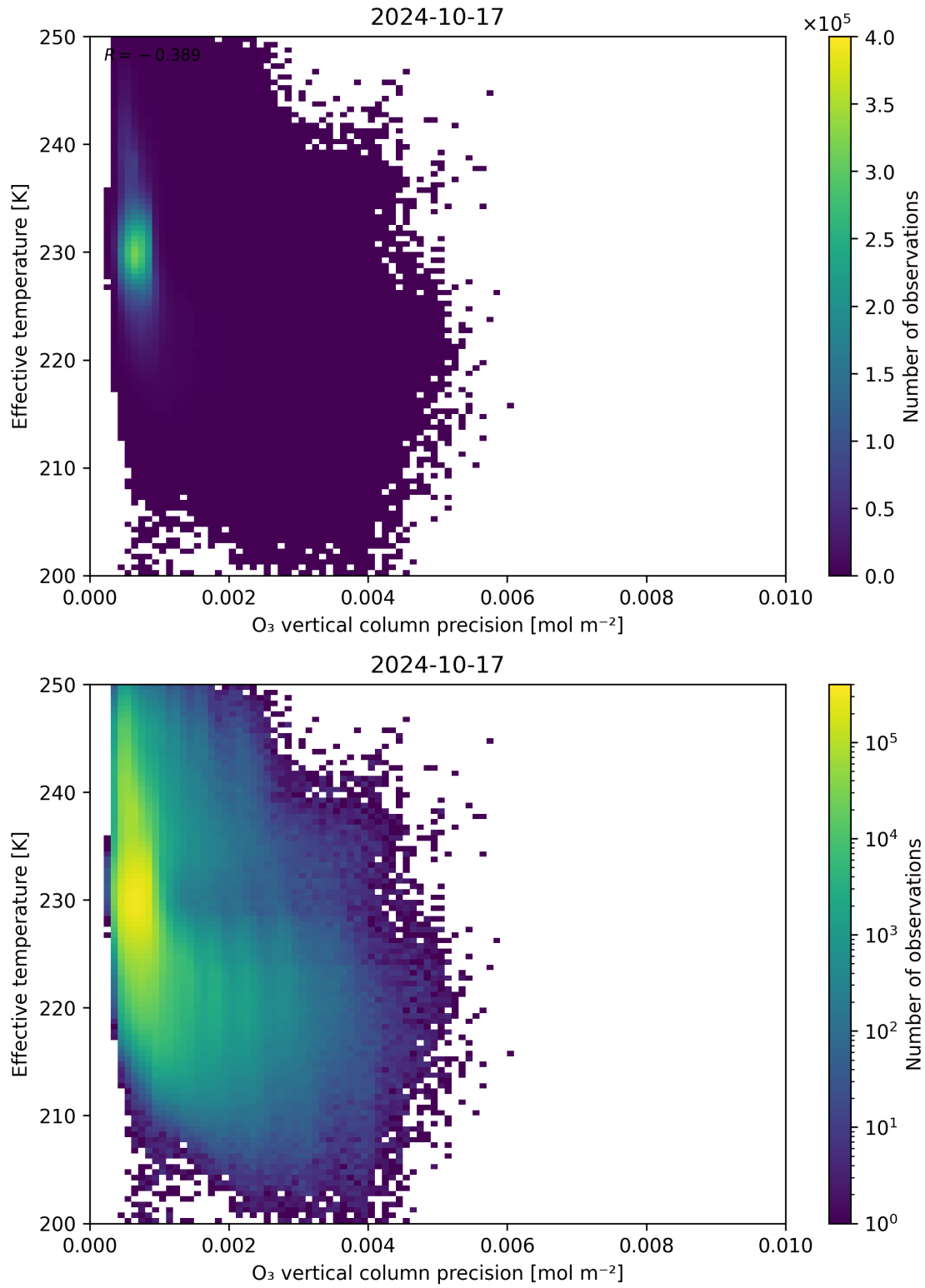
Figure 42: Scatter density plot of “ O_3 vertical column precision” against “Effective temperature” for 2024-10-16 to 2024-10-18.
