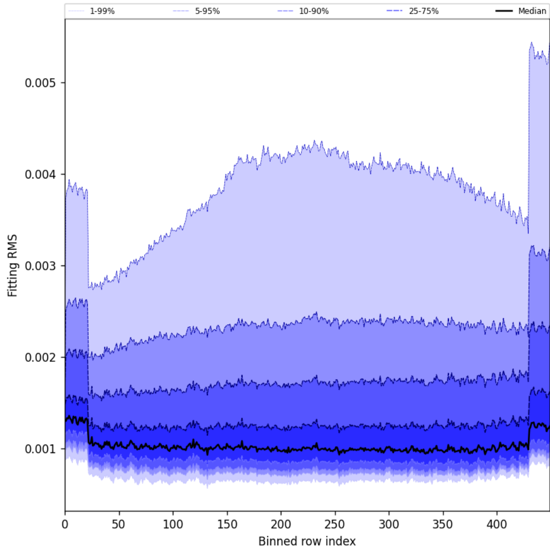
Figure 30: Along track statistics of “Fitting RMS” for 2024-10-16 to 2024-10-18
