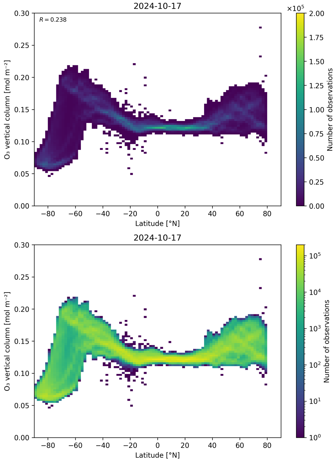
Figure 36: Scatter density plot of “Latitude” against “O 3 vertical column” for 2024-10-16 to 2024-10-18.
