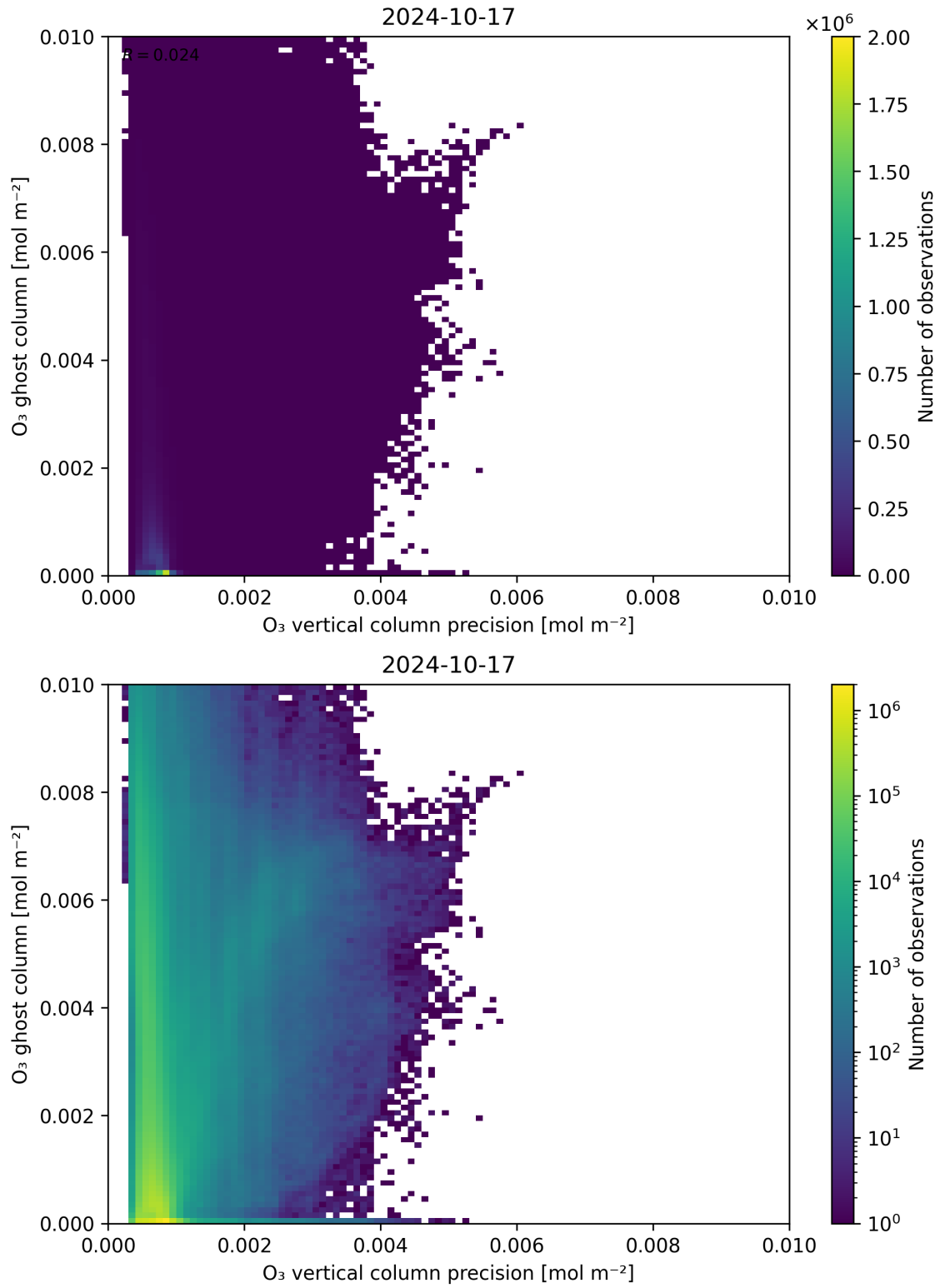
Figure 43: Scatter density plot of “ O_3 vertical column precision” against “ O_3 ghost column” for 2024-10-16 to 2024-10-18.
