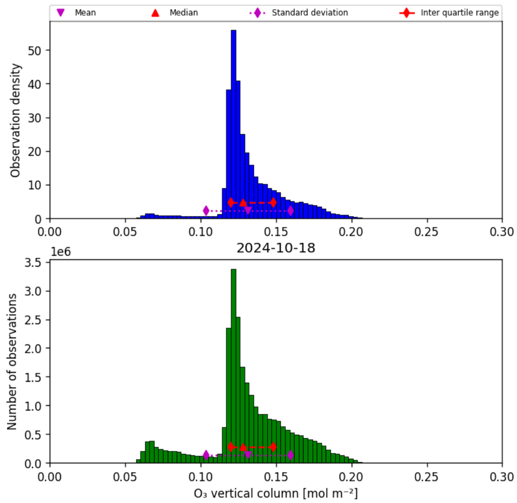
Figure 21: Histogram of “O 3 vertical column” for 2024-10-17 to 2024-10-19
