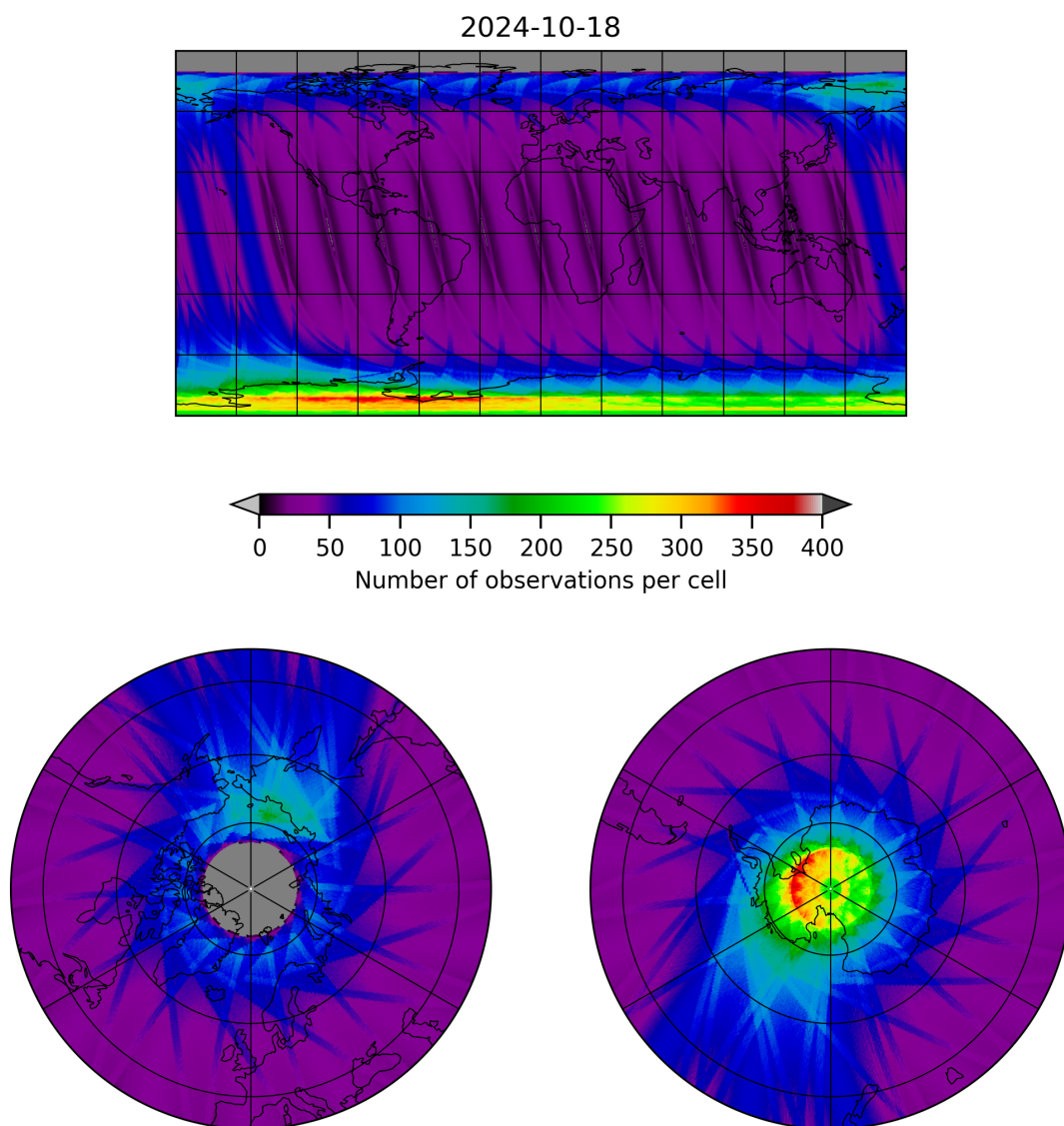
Figure 12: Map of the number of observations for 2024-10-17 to 2024-10-19
