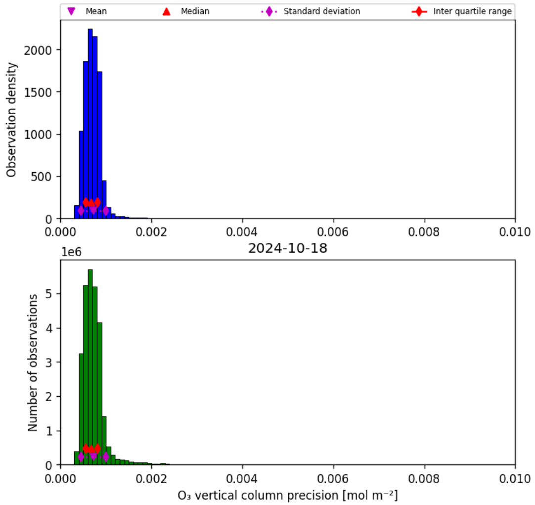
Figure 22: Histogram of "O 3 vertical column precision" for 2024-10-17 to 2024-10-19
