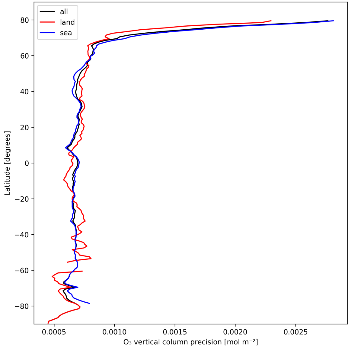
Figure 15: Zonal average of “O 3 vertical column precision” for 2024-10-17 to 2024-10-19.
