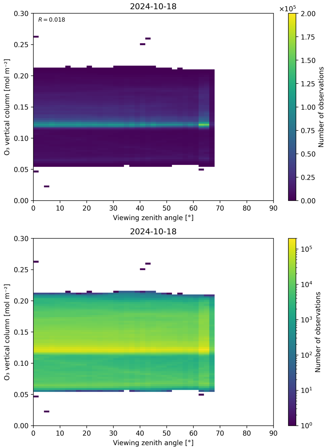
Figure 52: Scatter density plot of “Viewing zenith angle” against “O 3 vertical column” for 2024-10-17 to 2024-10-19.
