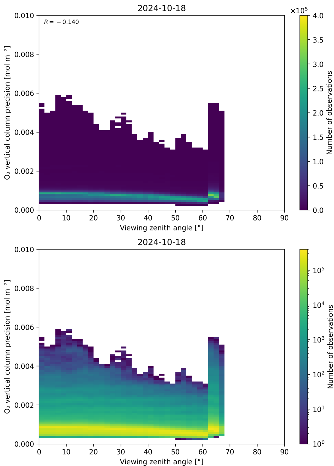
Figure 53: Scatter density plot of “Viewing zenith angle” against “O 3 vertical column precision” for 2024-10-17 to 2024-10-19.
