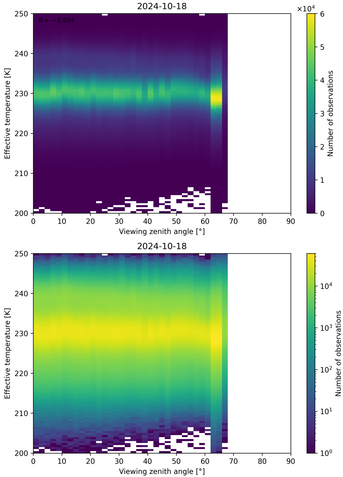
Figure 50: Scatter density plot of “Viewing zenith angle” against “Effective temperature” for 2024-10-17 to 2024-10-19.
