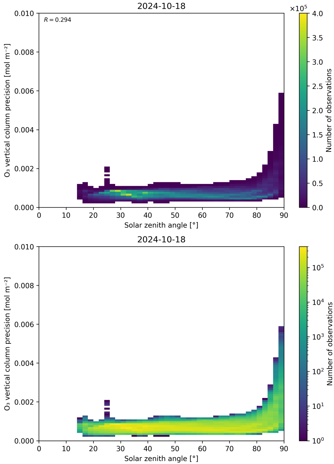
Figure 48: Scatter density plot of “Solar zenith angle” against “O 3 vertical column precision” for 2024-10-17 to 2024-10-19.
