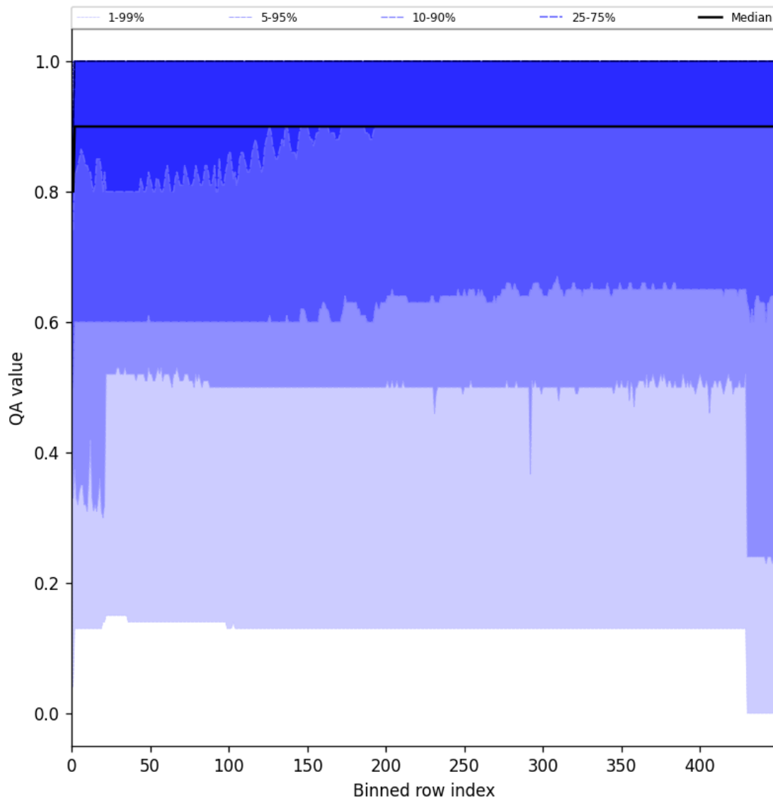
Figure 27: Along track statistics of “QA value” for 2024-10-17 to 2024-10-19
