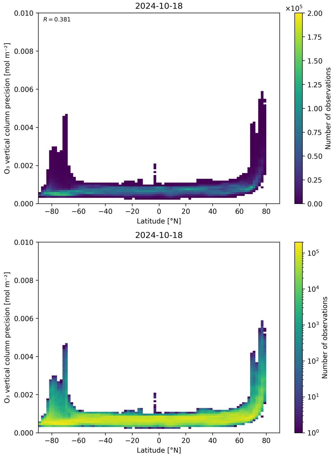
Figure 37: Scatter density plot of “Latitude” against “O 3 vertical column precision” for 2024-10-17 to 2024-10-19.
