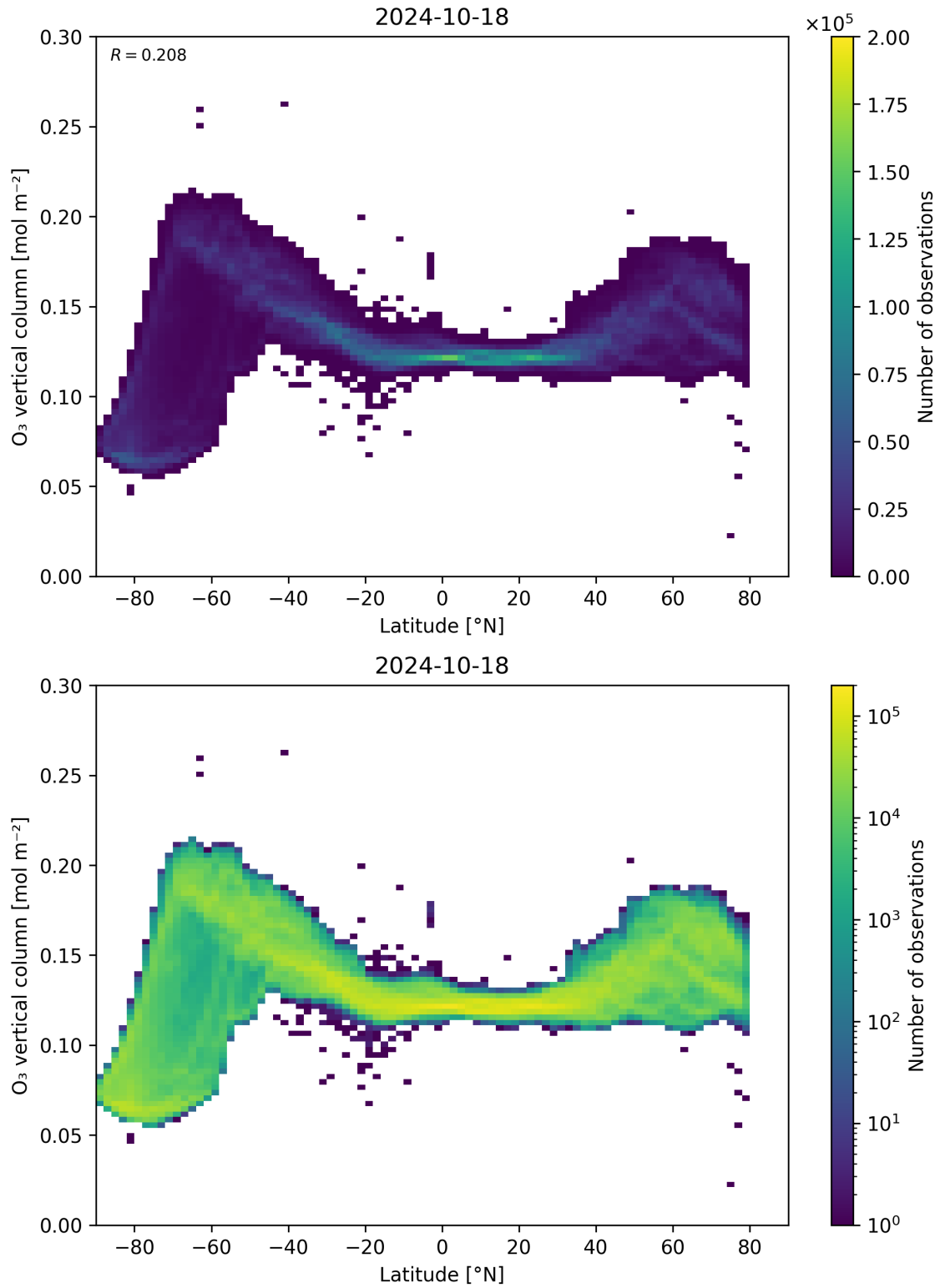
Figure 36: Scatter density plot of “Latitude” against “O 3 vertical column” for 2024-10-17 to 2024-10-19.
