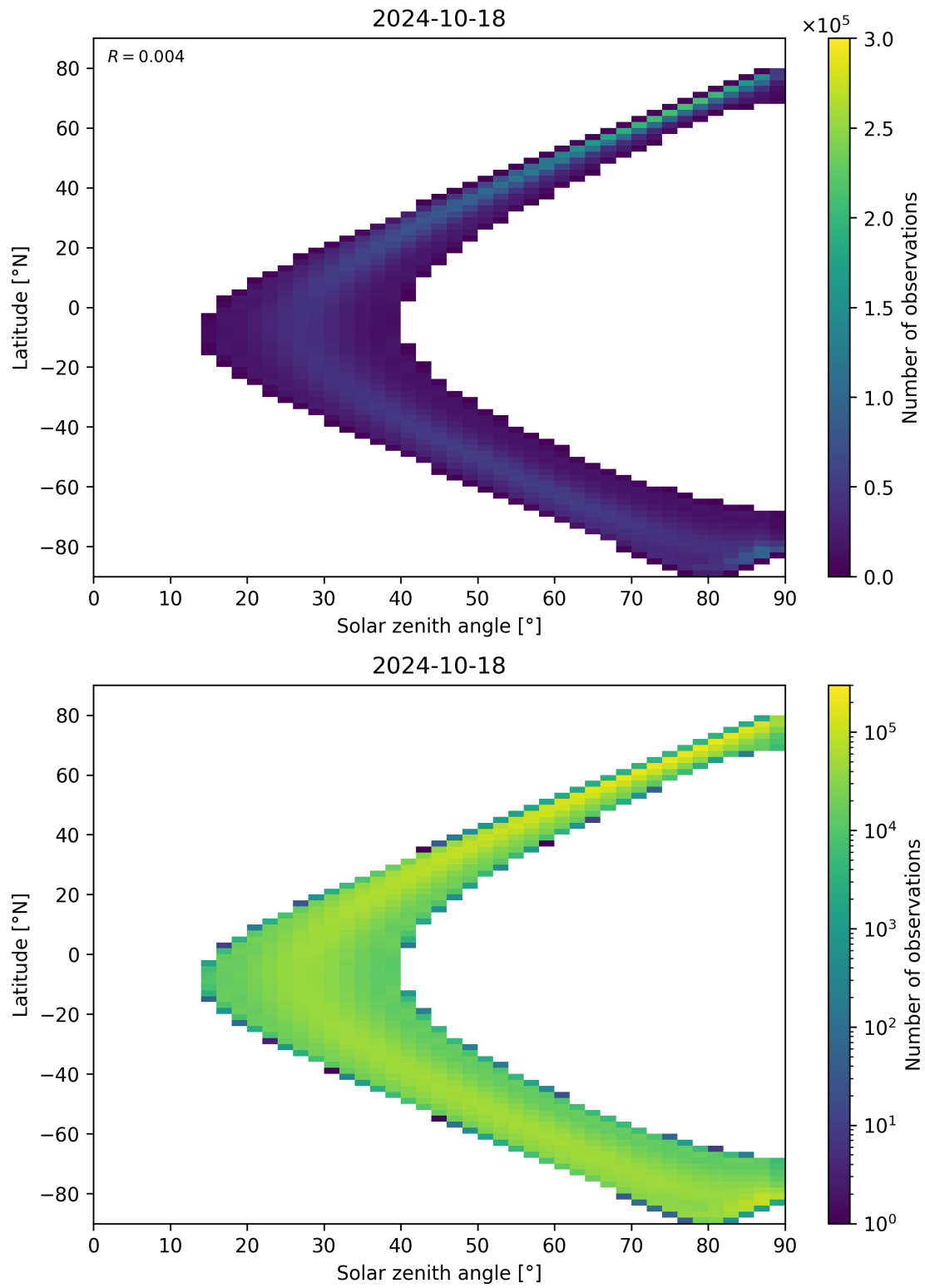
Figure 44: Scatter density plot of “Solar zenith angle” against “Latitude” for 2024-10-17 to 2024-10-19.
