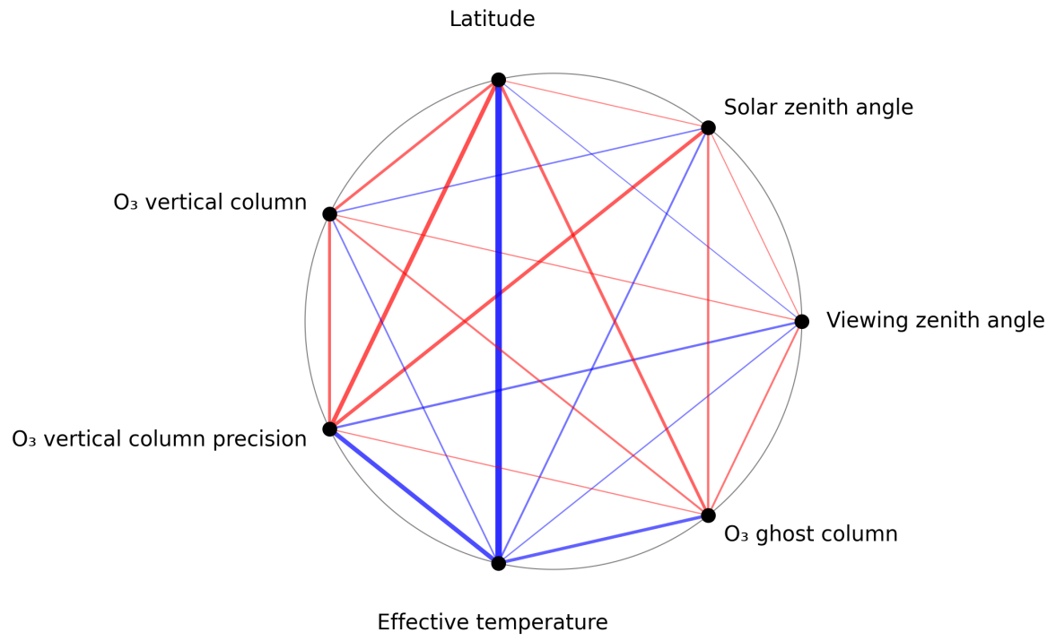
Figure 1: Map of correlation graph for 2024-10-17 to 2024-10-19.
