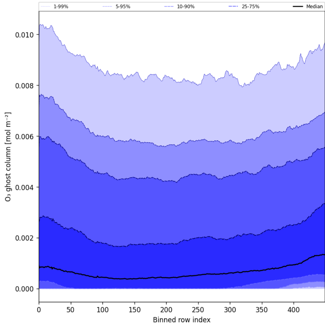
Figure 32: Along track statistics of “O 3 ghost column” for 2024-10-17 to 2024-10-19
