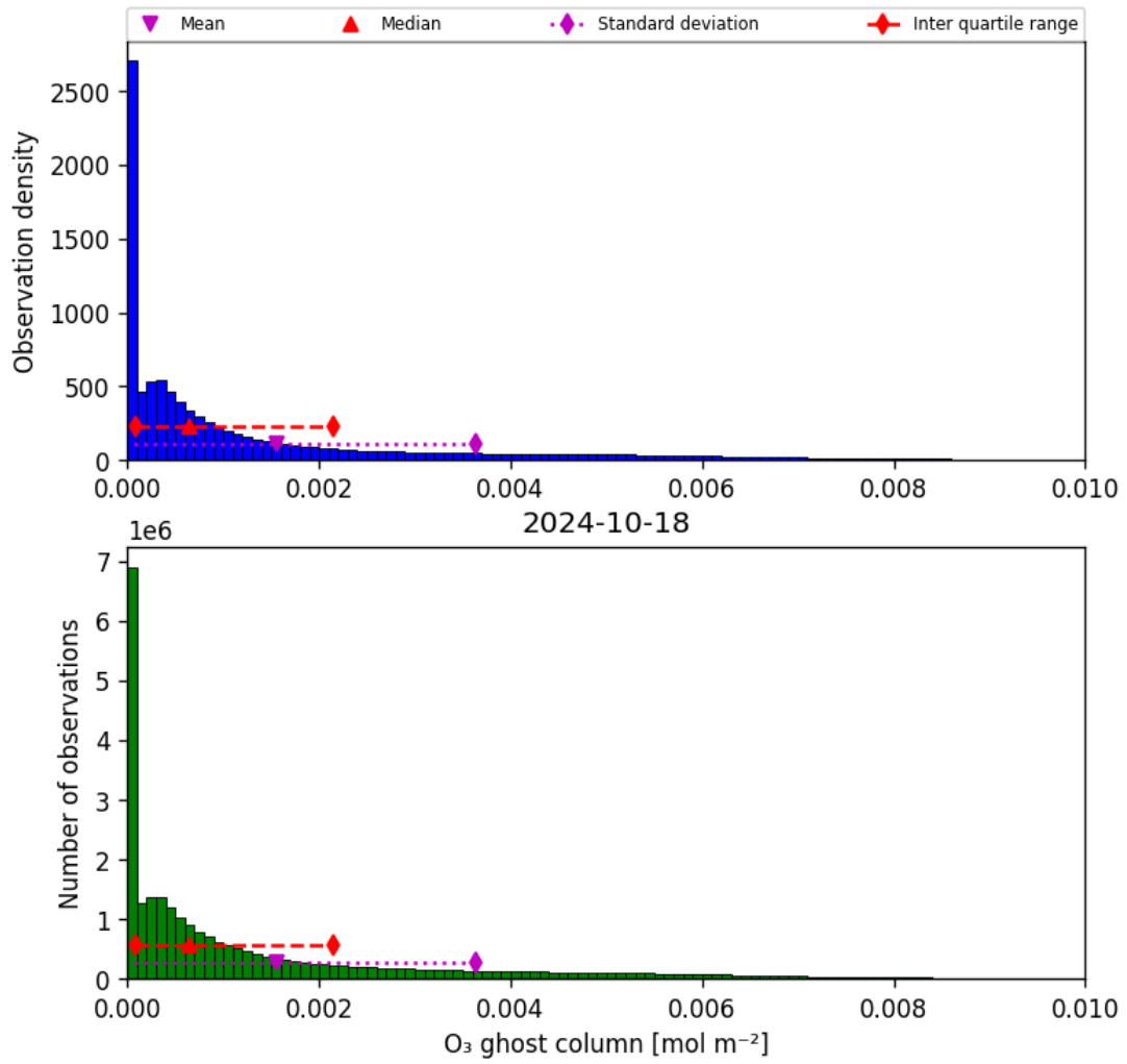
Figure 25: Histogram of “O 3 ghost column” for 2024-10-17 to 2024-10-19
