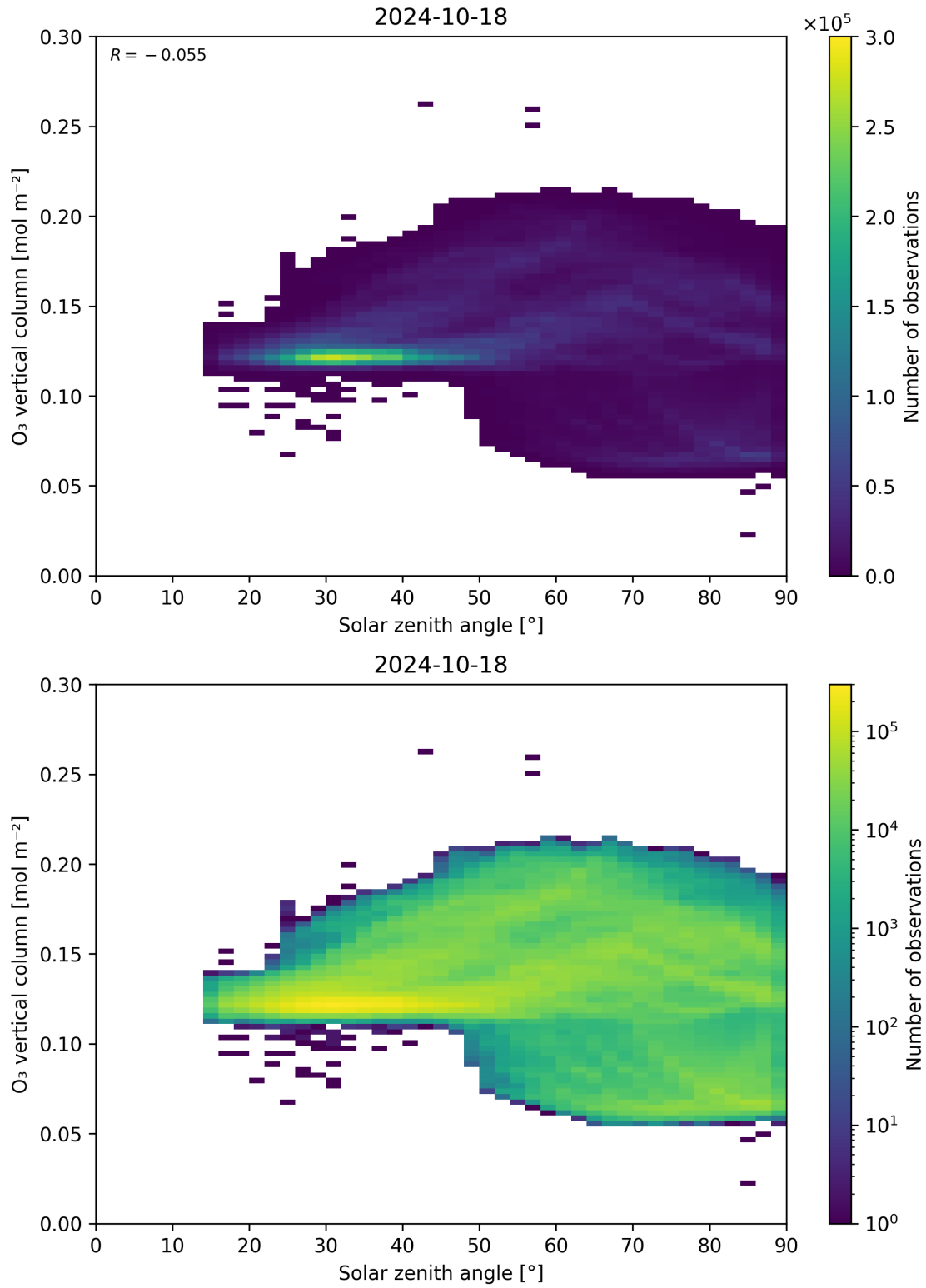
Figure 47: Scatter density plot of “Solar zenith angle” against “O 3 vertical column” for 2024-10-17 to 2024-10-19.
