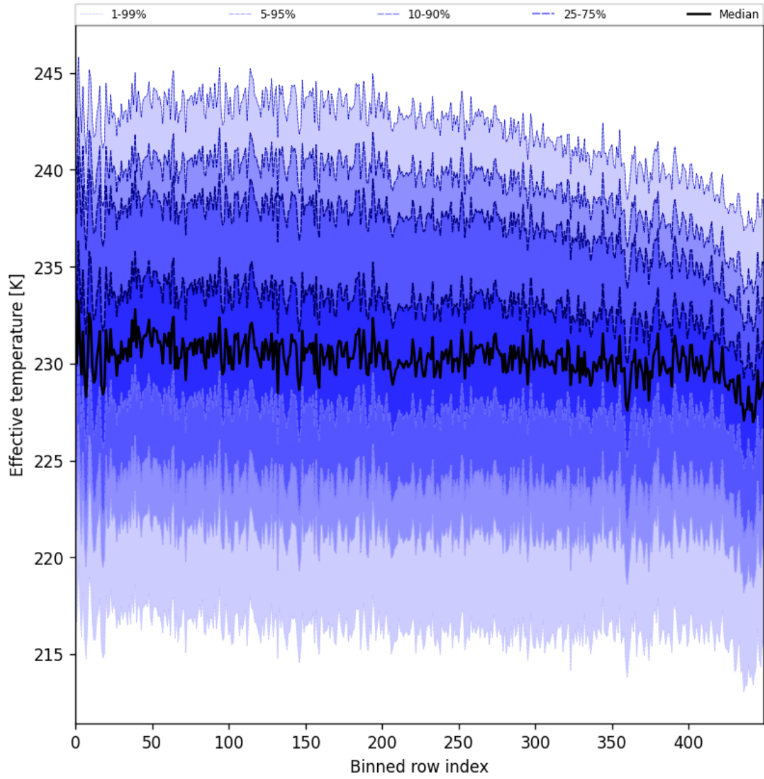
Figure 31: Along track statistics of “Effective temperature” for 2024-10-17 to 2024-10-19
