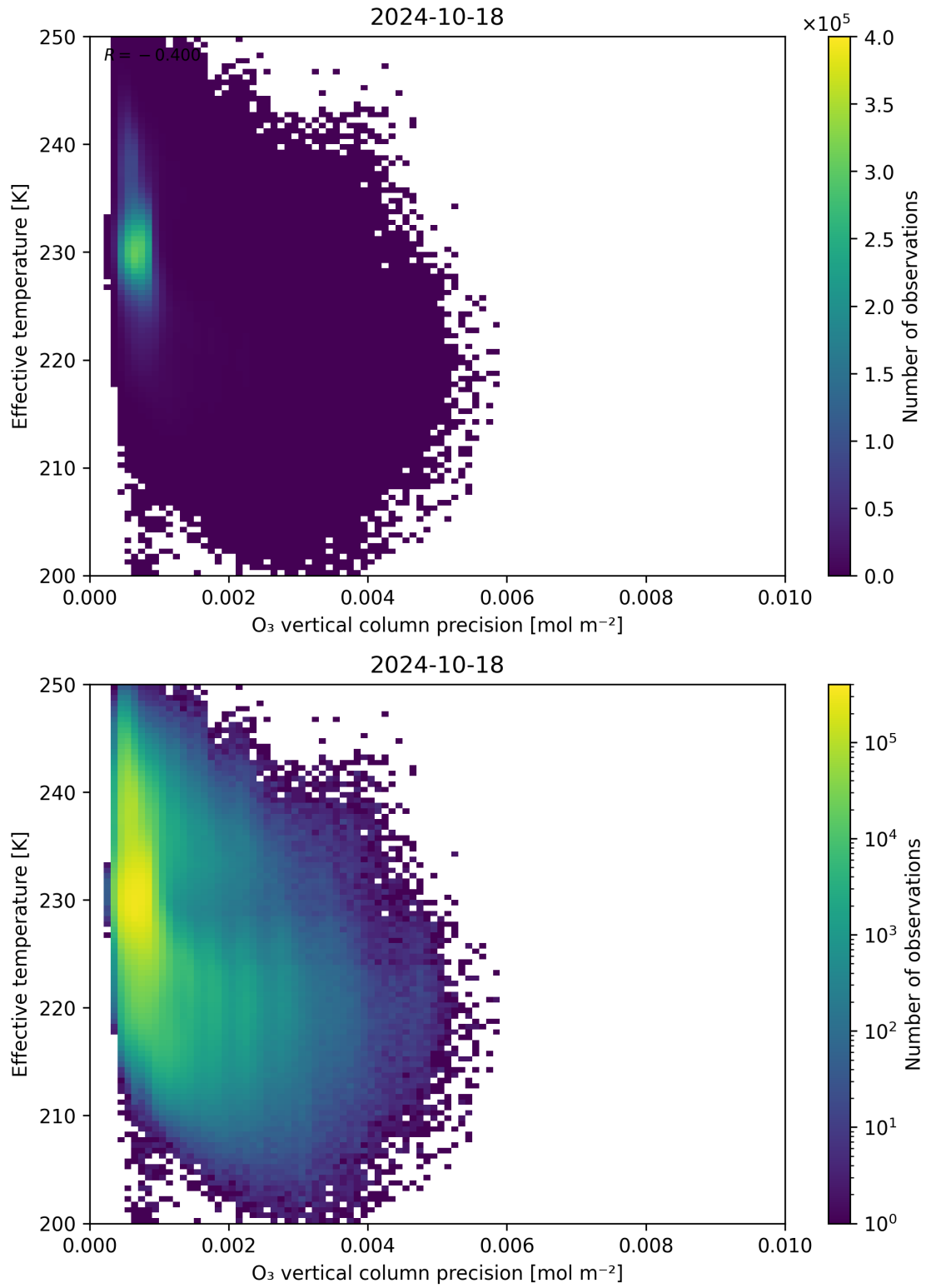
Figure 42: Scatter density plot of “ O_3 vertical column precision” against “Effective temperature” for 2024-10-17 to 2024-10-19.
