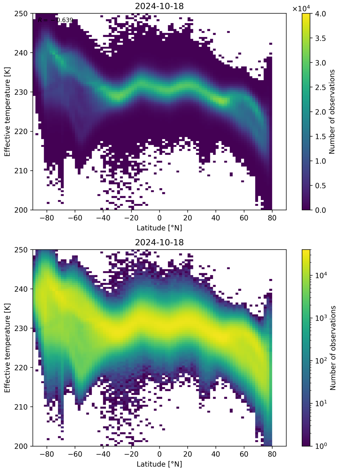
Figure 34: Scatter density plot of “Latitude” against “Effective temperature” for 2024-10-17 to 2024-10-19.
