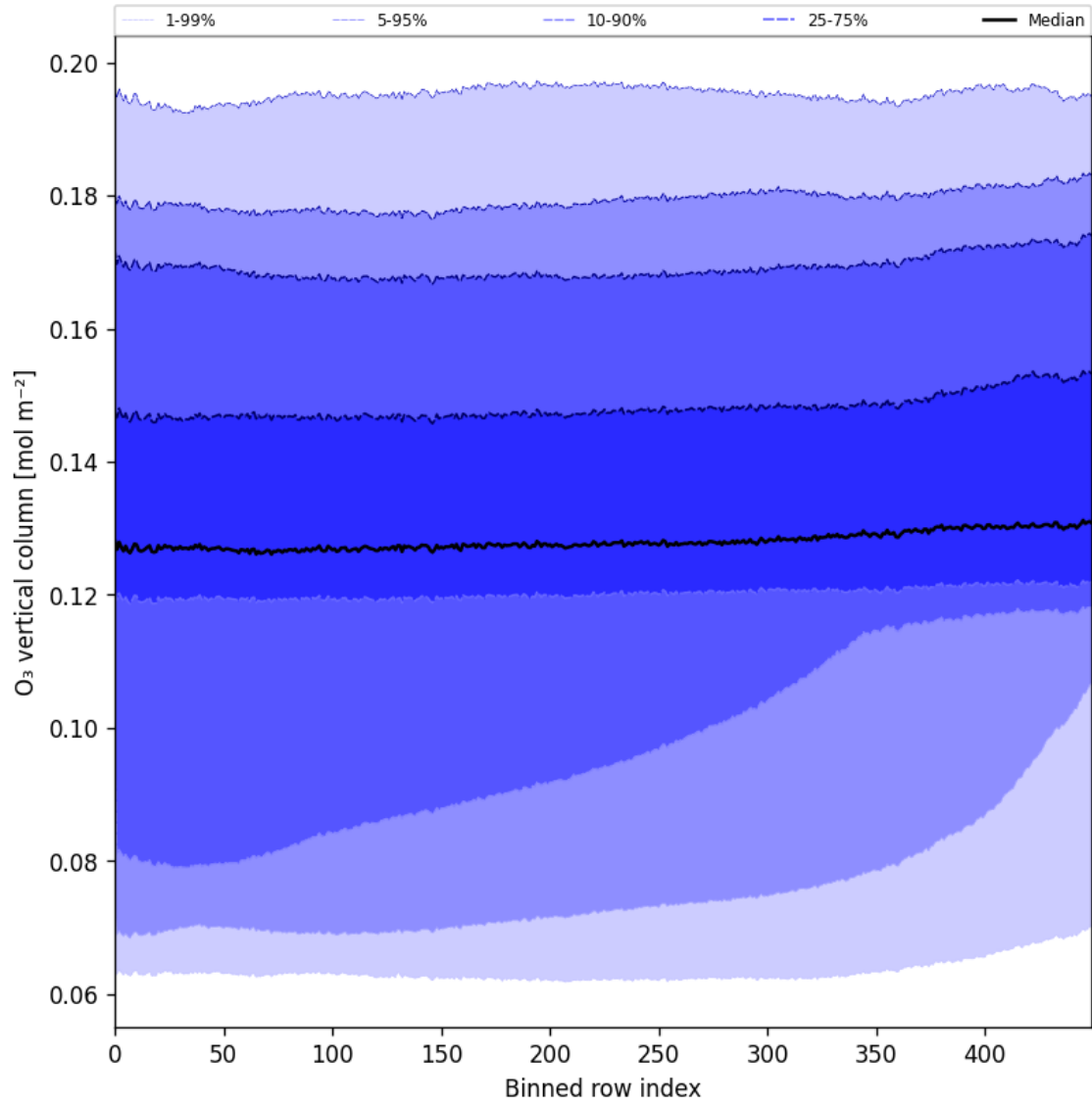
Figure 28: Along track statistics of “O 3 vertical column” for 2024-10-17 to 2024-10-19
