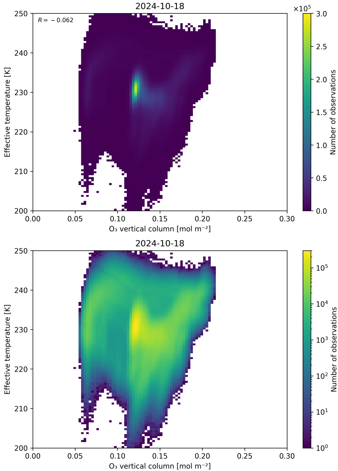
Figure 39: Scatter density plot of “O 3 vertical column” against “Effective temperature” for 2024-10-17 to 2024-10-19.
