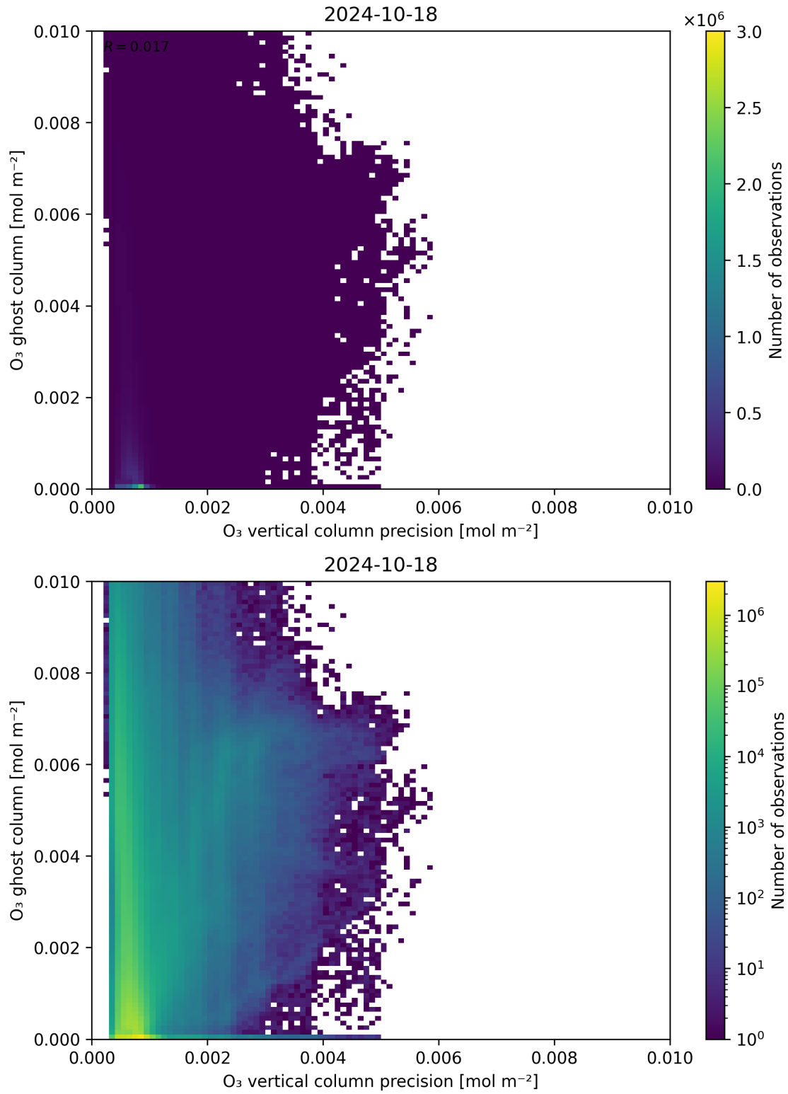
Figure 43: Scatter density plot of “O 3 vertical column precision” against “O 3 ghost column” for 2024-10-17 to 2024-10-19.
