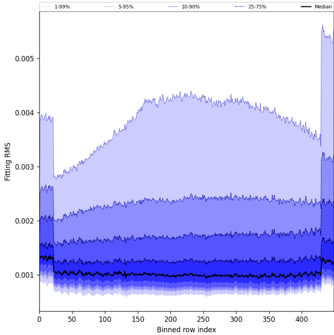
Figure 30: Along track statistics of “Fitting RMS” for 2024-10-17 to 2024-10-19
