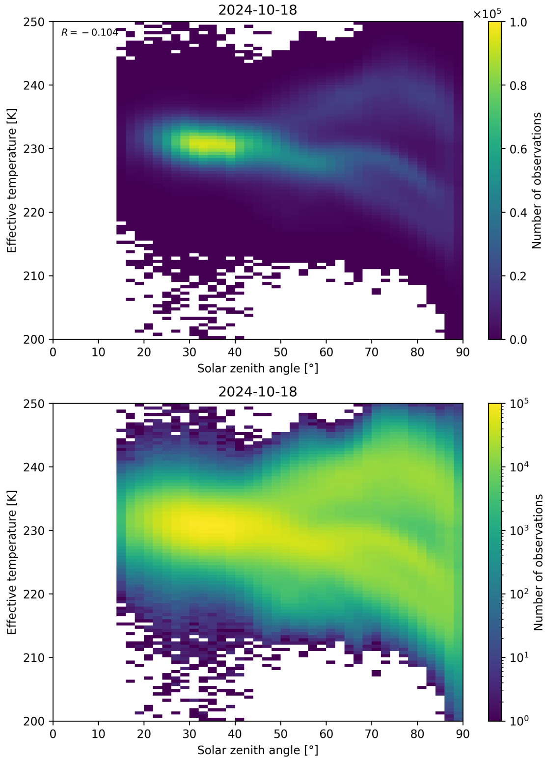
Figure 45: Scatter density plot of “Solar zenith angle” against “Effective temperature” for 2024-10-17 to 2024-10-19.
