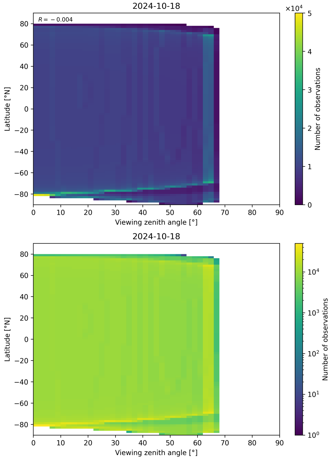
Figure 49: Scatter density plot of “Viewing zenith angle” against “Latitude” for 2024-10-17 to 2024-10-19.
