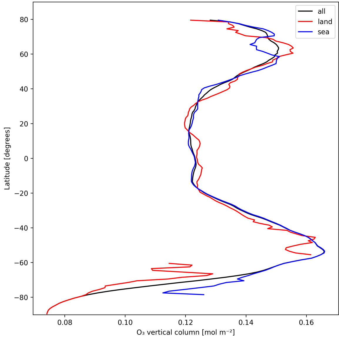
Figure 14: Zonal average of “O 3 vertical column” for 2024-10-17 to 2024-10-19.
