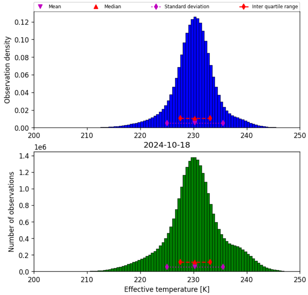
Figure 24: Histogram of “Effective temperature” for 2024-10-17 to 2024-10-19
