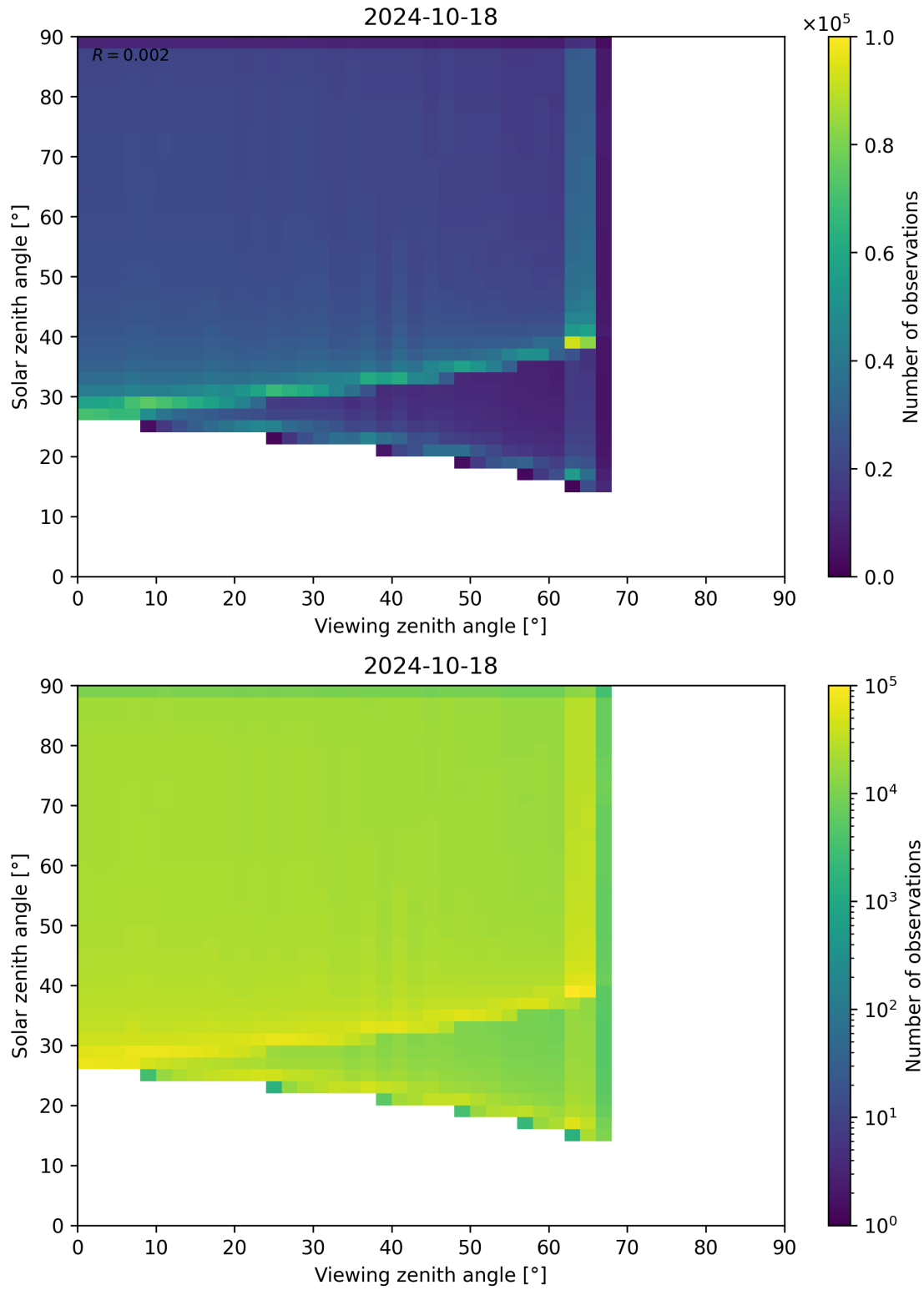
Figure 54: Scatter density plot of “Viewing zenith angle” against “Solar zenith angle” for 2024-10-17 to 2024-10-19.
