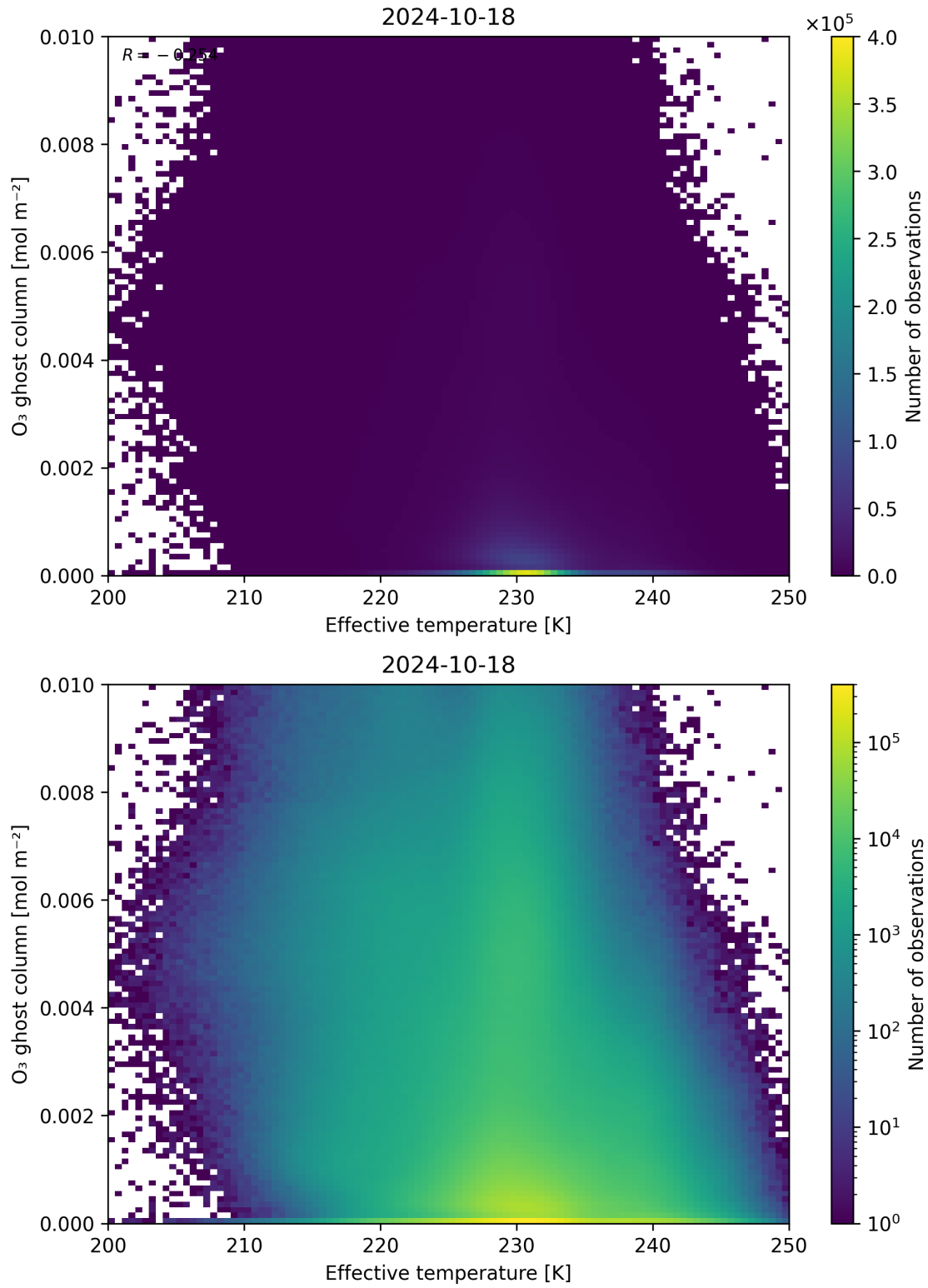
Figure 38: Scatter density plot of “Effective temperature” against “O 3 ghost column” for 2024-10-17 to 2024-10-19.
