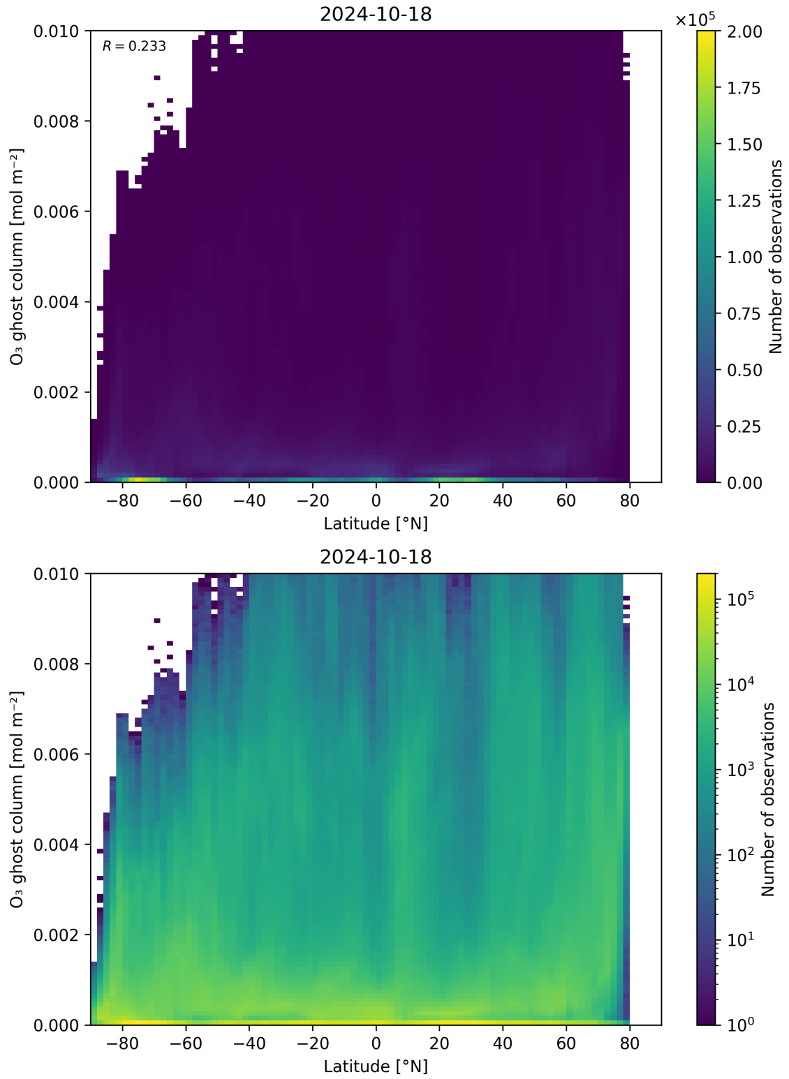
Figure 35: Scatter density plot of “Latitude” against “O 3 ghost column” for 2024-10-17 to 2024-10-19.
