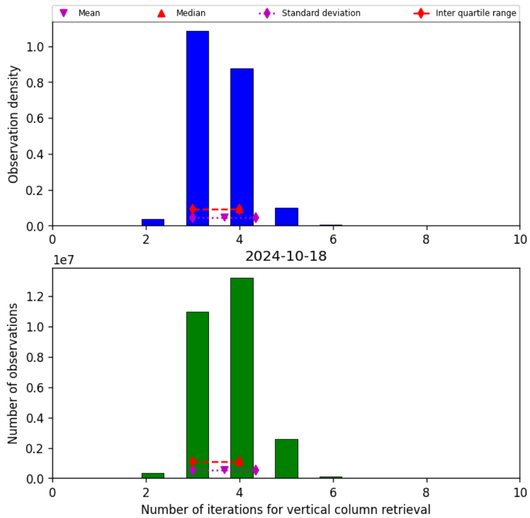
Figure 26: Histogram of “Number of iterations for vertical column retrieval” for 2024-10-17 to 2024-10-19
