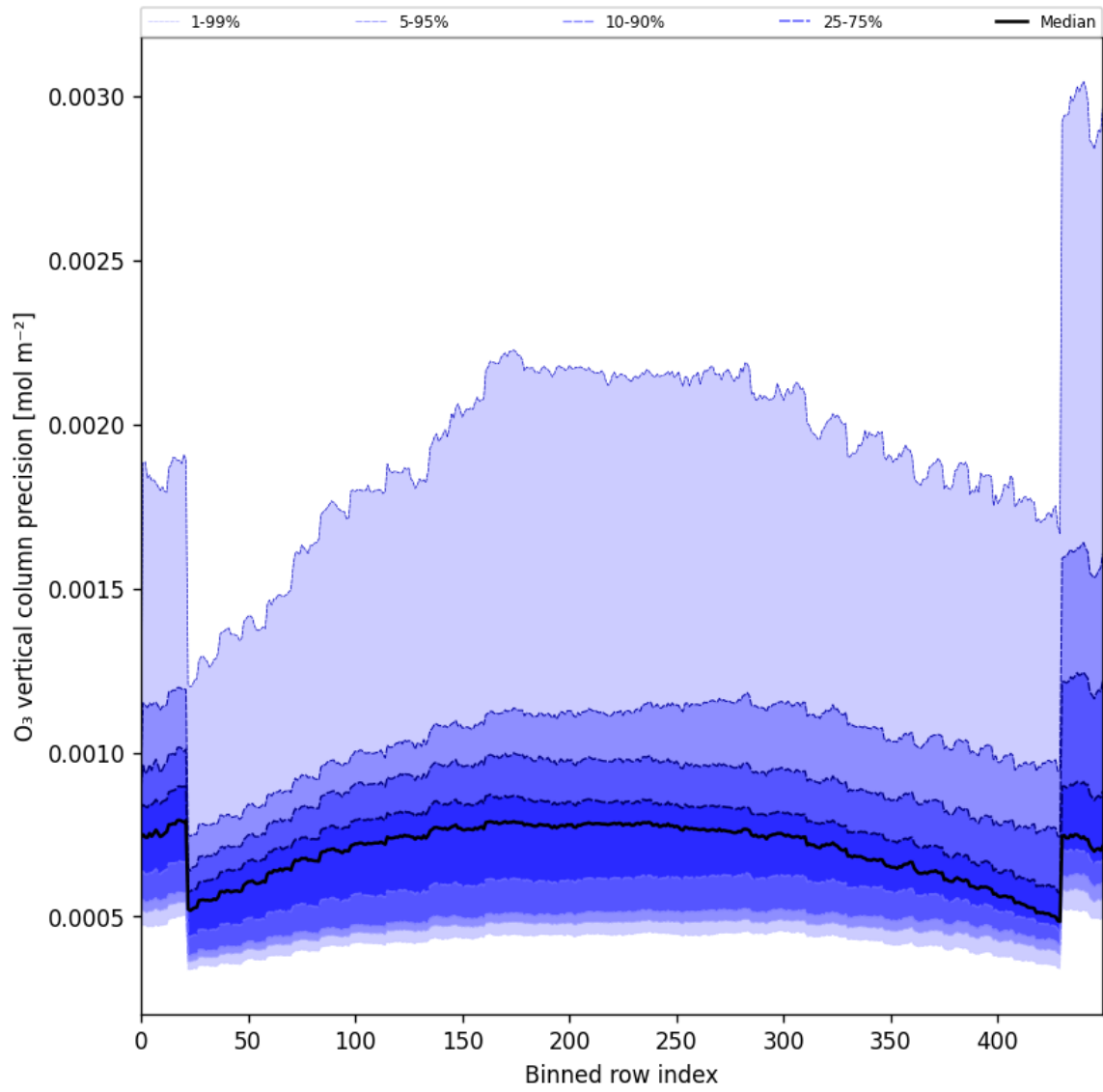
Figure 29: Along track statistics of “O 3 vertical column precision” for 2024-10-17 to 2024-10-19
