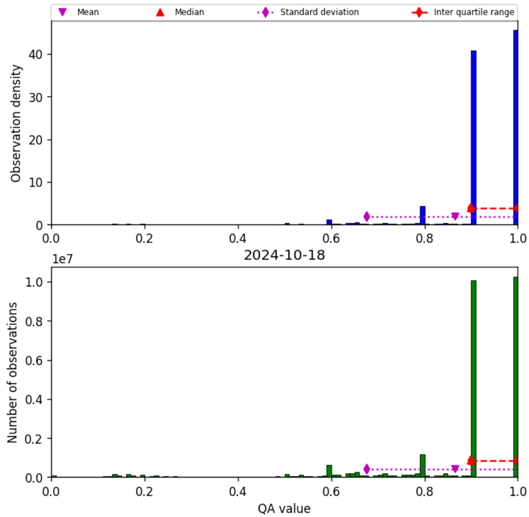
Figure 20: Histogram of “QA value” for 2024-10-17 to 2024-10-19
