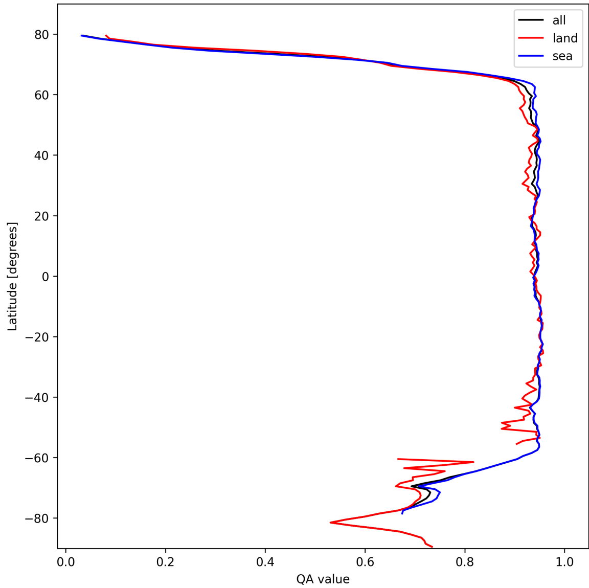
Figure 13: Zonal average of “QA value” for 2024-10-17 to 2024-10-19.
