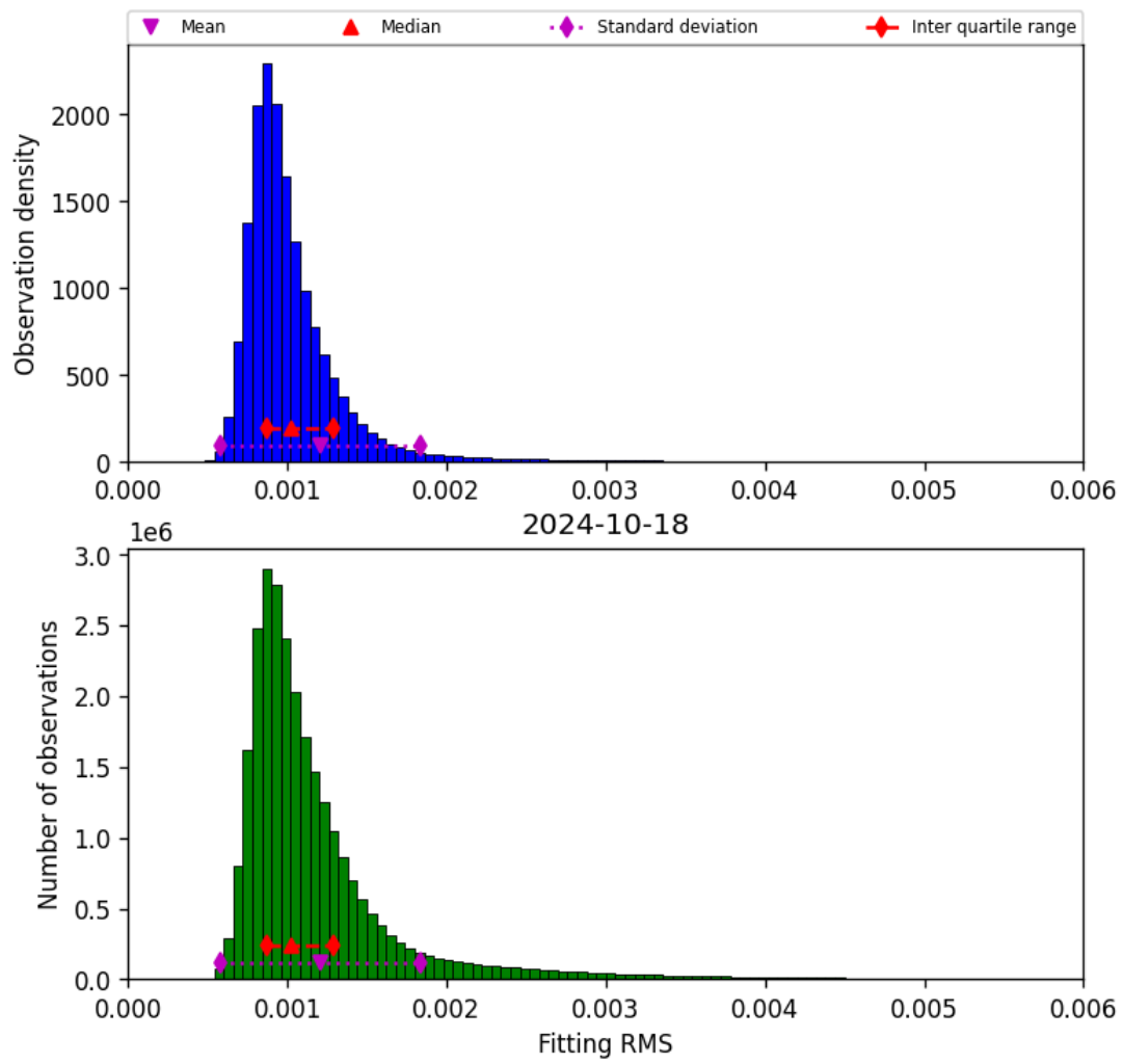
Figure 23: Histogram of “Fitting RMS” for 2024-10-17 to 2024-10-19
