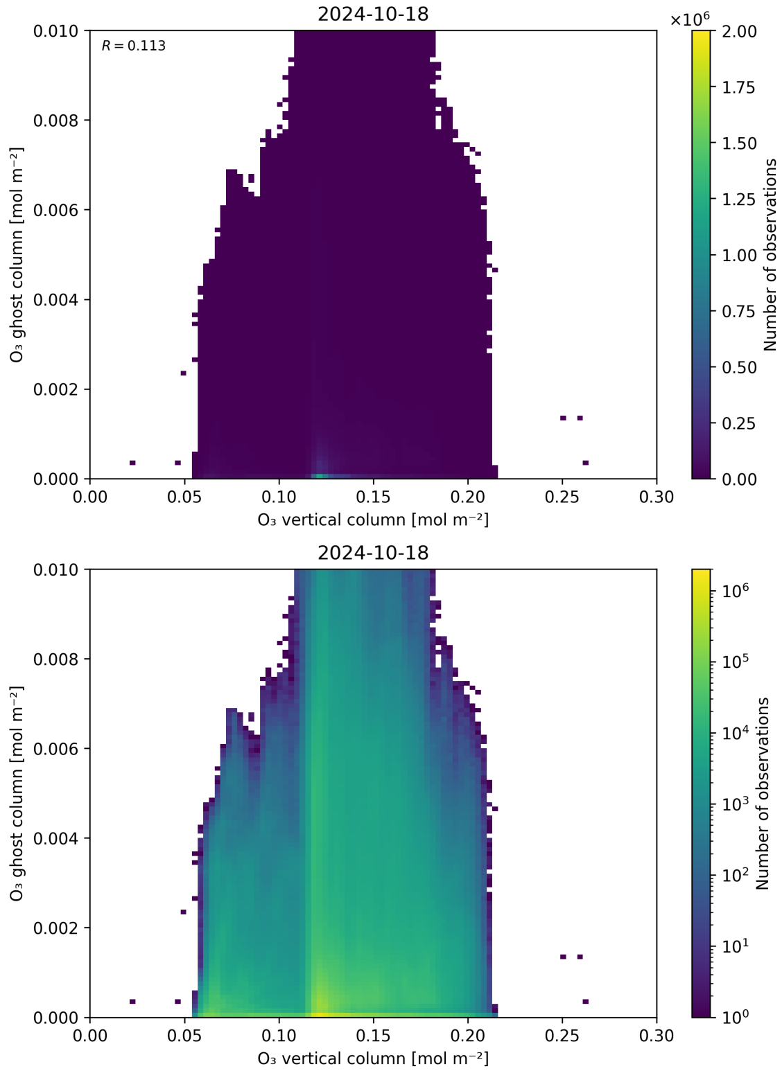
Figure 40: Scatter density plot of “O 3 vertical column” against “O 3 ghost column” for 2024-10-17 to 2024-10-19.
