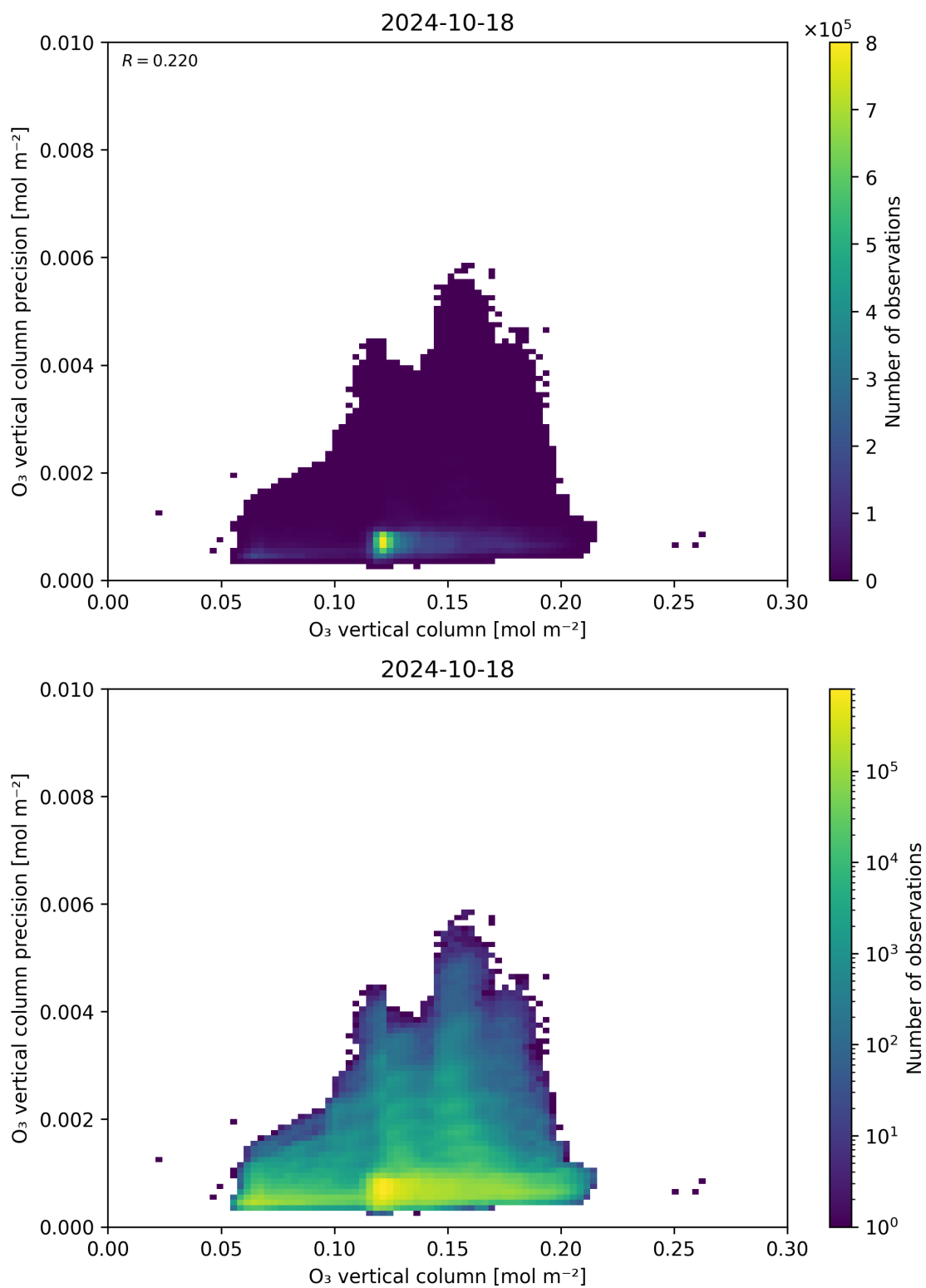
Figure 41: Scatter density plot of “O 3 vertical column” against “O 3 vertical column precision” for 2024-10-17 to 2024-10-19.
