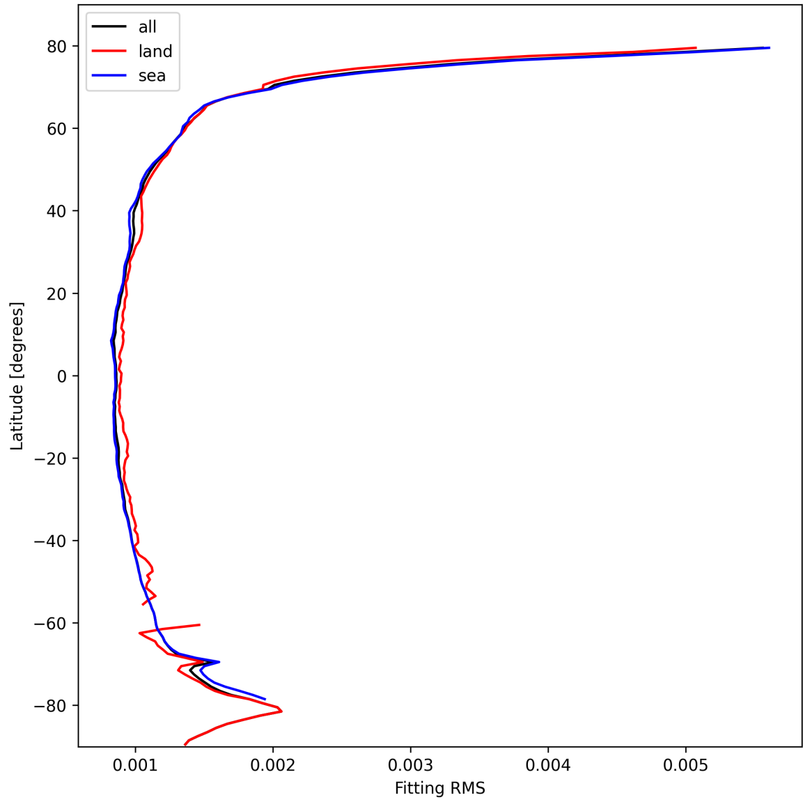
Figure 16: Zonal average of “Fitting RMS” for 2024-10-17 to 2024-10-19.
