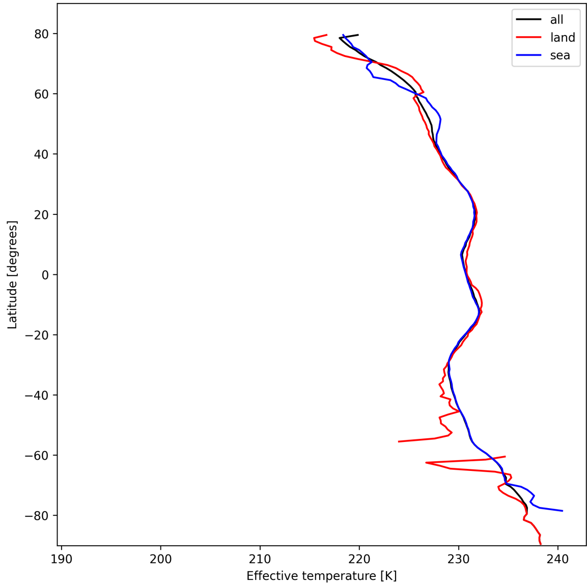
Figure 17: Zonal average of "Effective temperature" for 2024-10-17 to 2024-10-19.
