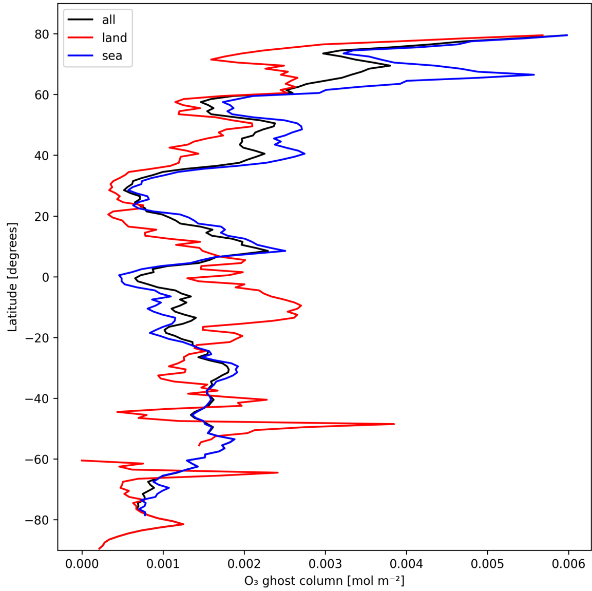
Figure 18: Zonal average of "O 3 ghost column" for 2024-10-17 to 2024-10-19.
