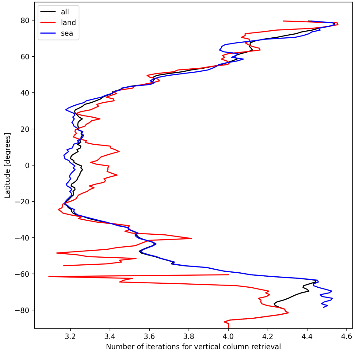
Figure 19: Zonal average of “Number of iterations for vertical column retrieval” for 2024-10-17 to 2024-10-19.
