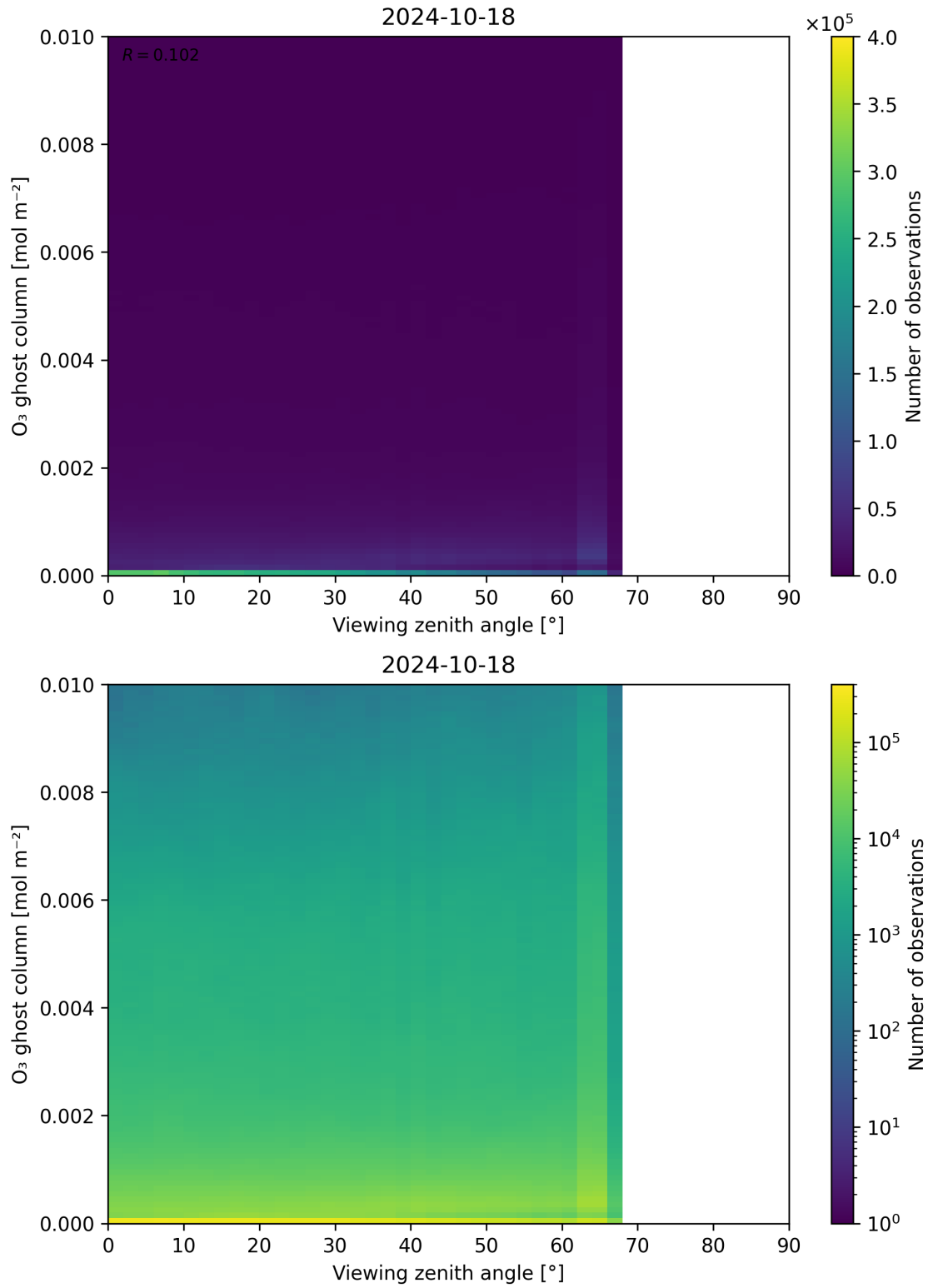
Figure 51: Scatter density plot of “Viewing zenith angle” against “O 3 ghost column” for 2024-10-17 to 2024-10-19.
