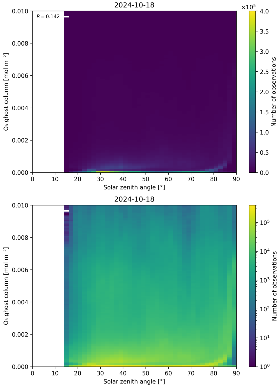
Figure 46: Scatter density plot of “Solar zenith angle” against “O 3 ghost column” for 2024-10-17 to 2024-10-19.
