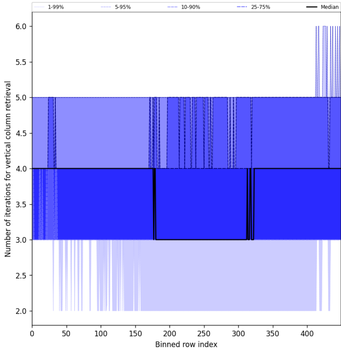
Figure 33: Along track statistics of “Number of iterations for vertical column retrieval” for 2024-10-17 to 2024-10-19
