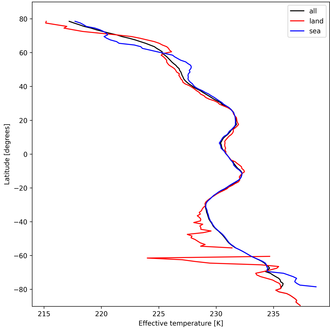
Figure 17: Zonal average of “Effective temperature” for 2024-10-19 to 2024-10-20.
