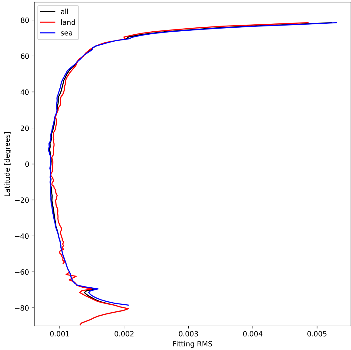
Figure 16: Zonal average of “Fitting RMS” for 2024-10-19 to 2024-10-20.
