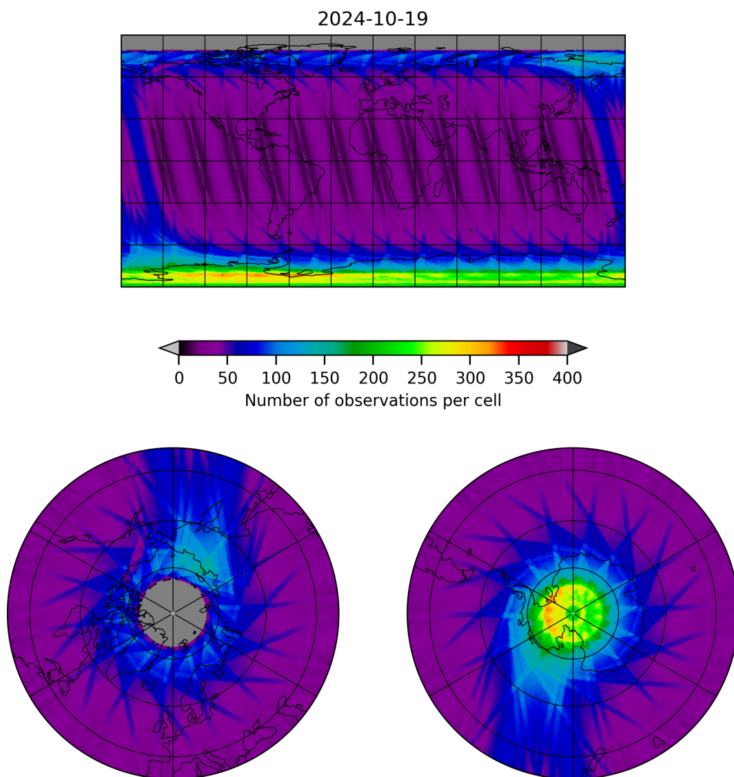
Figure 12: Map of the number of observations for 2024-10-19 to 2024-10-20
