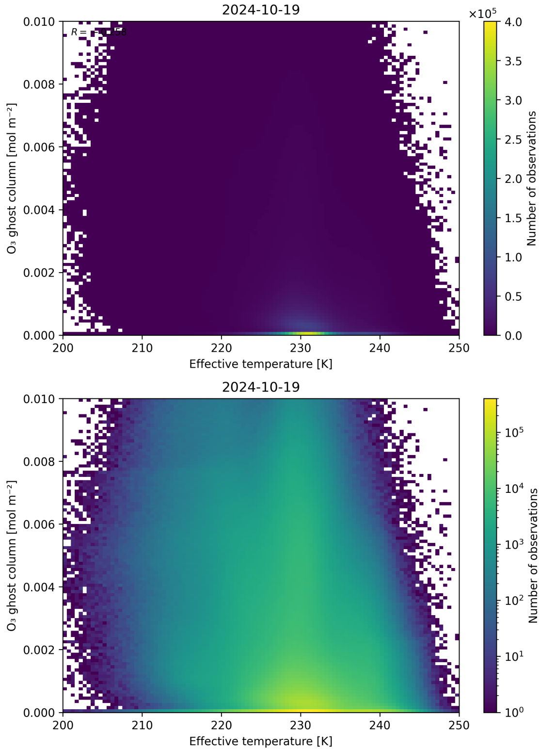
Figure 38: Scatter density plot of “Effective temperature” against “O 3 ghost column” for 2024-10-19 to 2024-10-20.
