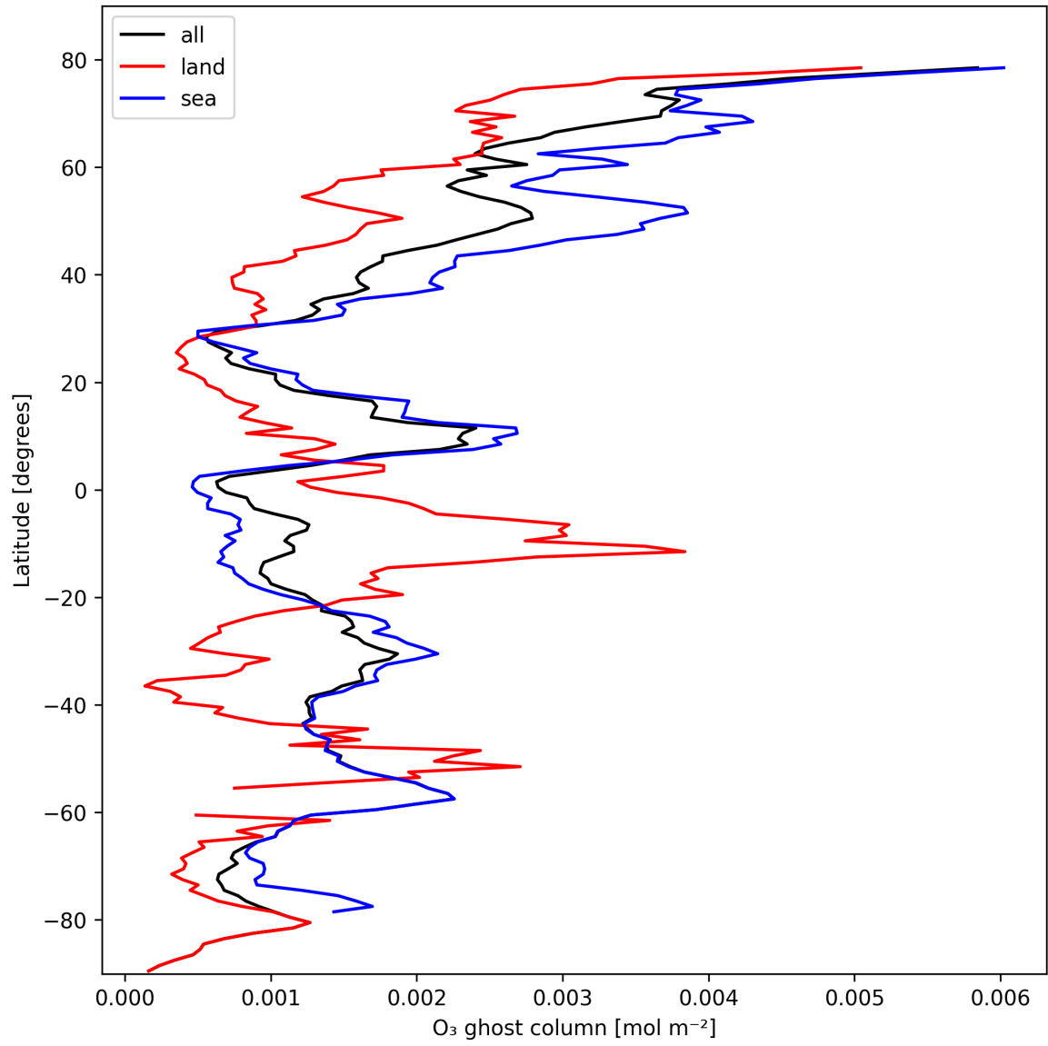
Figure 18: Zonal average of “O 3 ghost column” for 2024-10-19 to 2024-10-20.
