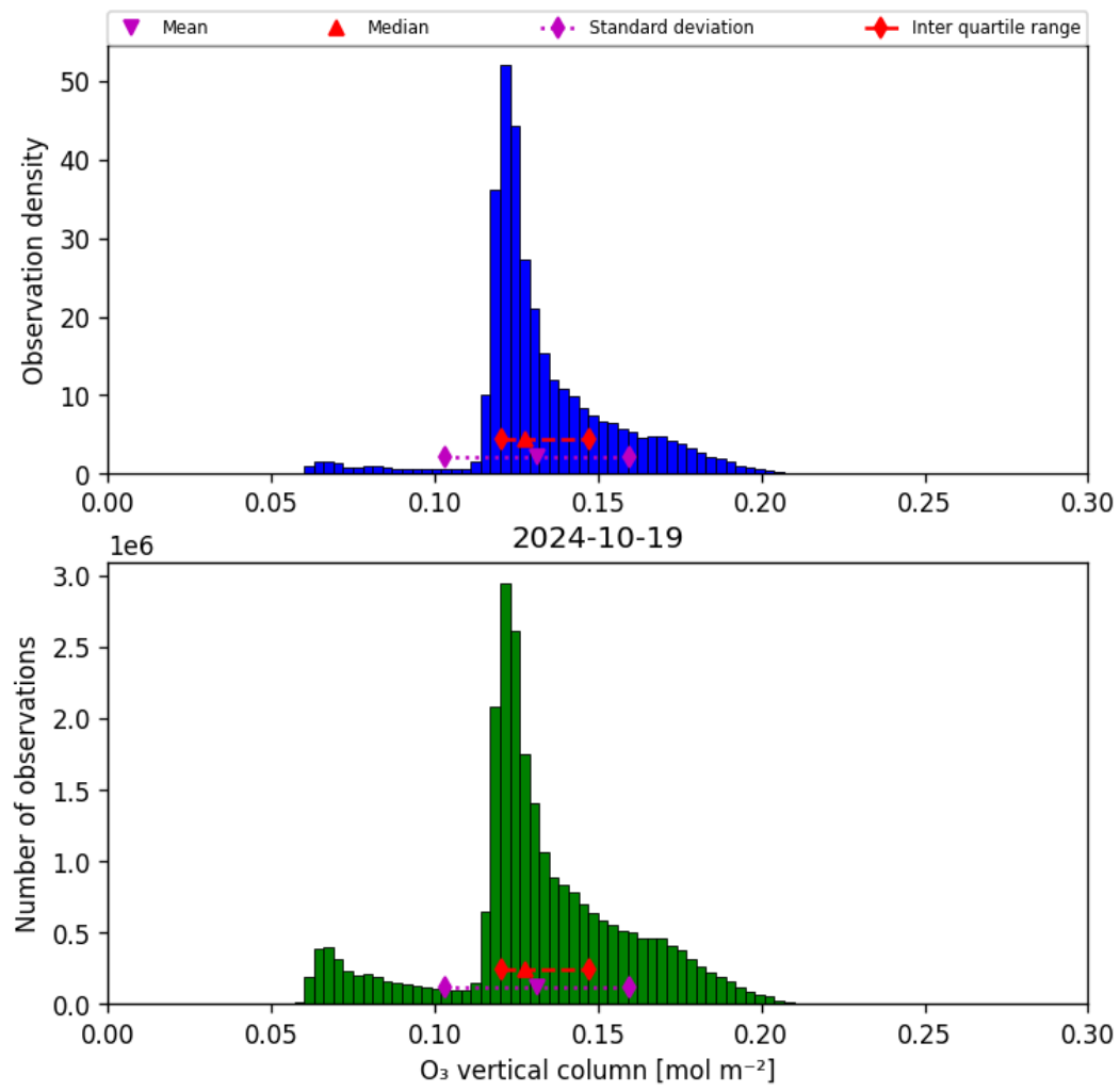
Figure 21: Histogram of “O 3 vertical column” for 2024-10-19 to 2024-10-20
