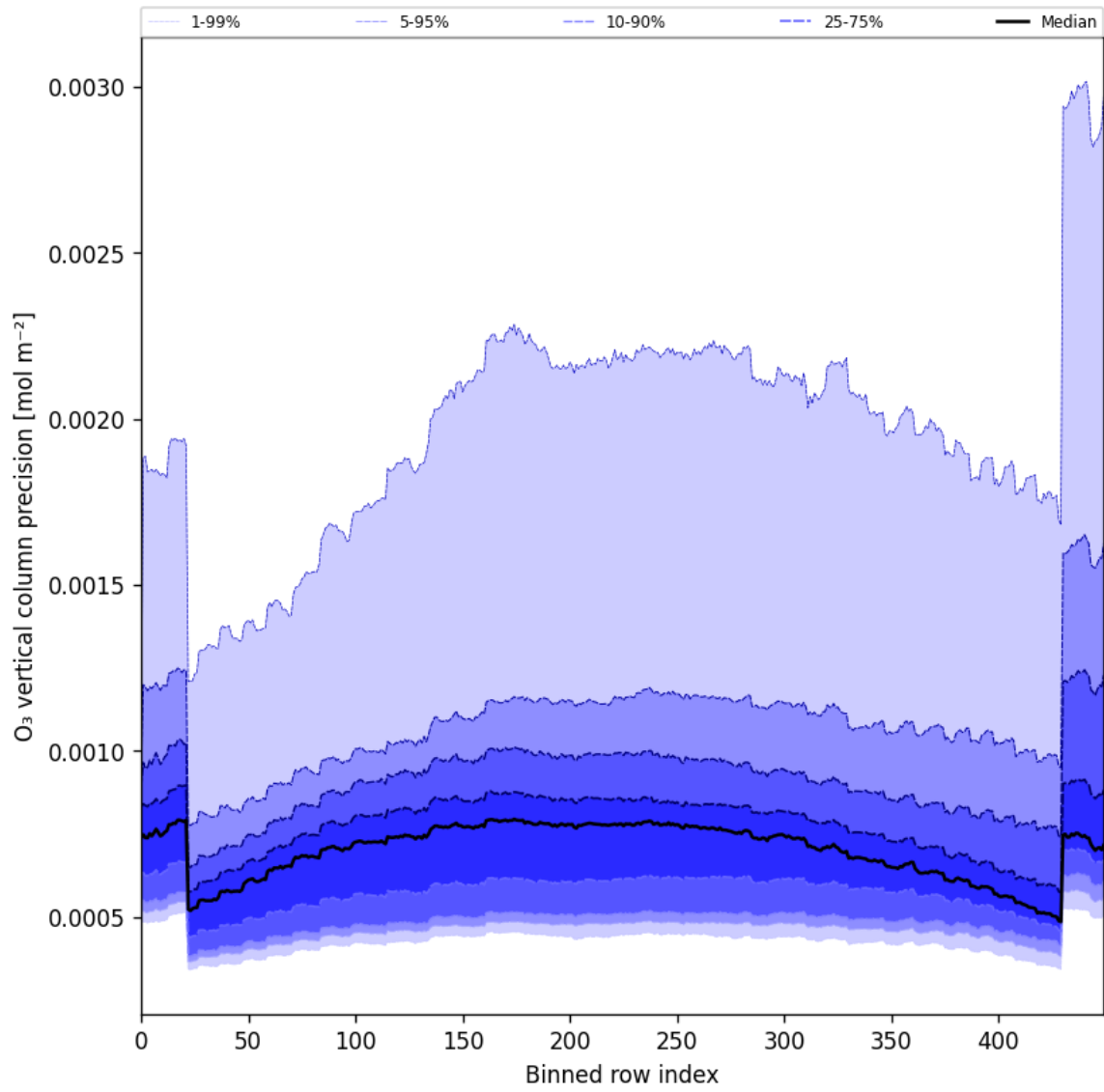
Figure 29: Along track statistics of “O 3 vertical column precision” for 2024-10-19 to 2024-10-20
