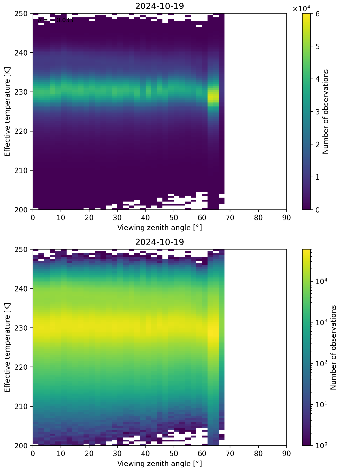
Figure 50: Scatter density plot of “Viewing zenith angle” against “Effective temperature” for 2024-10-19 to 2024-10-20.
