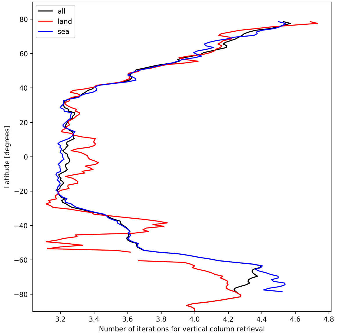
Figure 19: Zonal average of “Number of iterations for vertical column retrieval” for 2024-10-19 to 2024-10-20.
