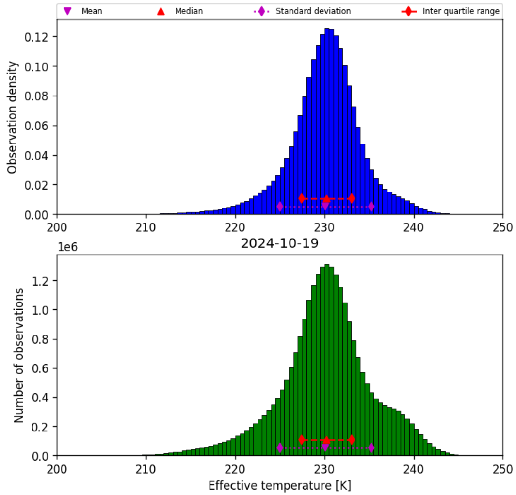
Figure 24: Histogram of “Effective temperature” for 2024-10-19 to 2024-10-20
