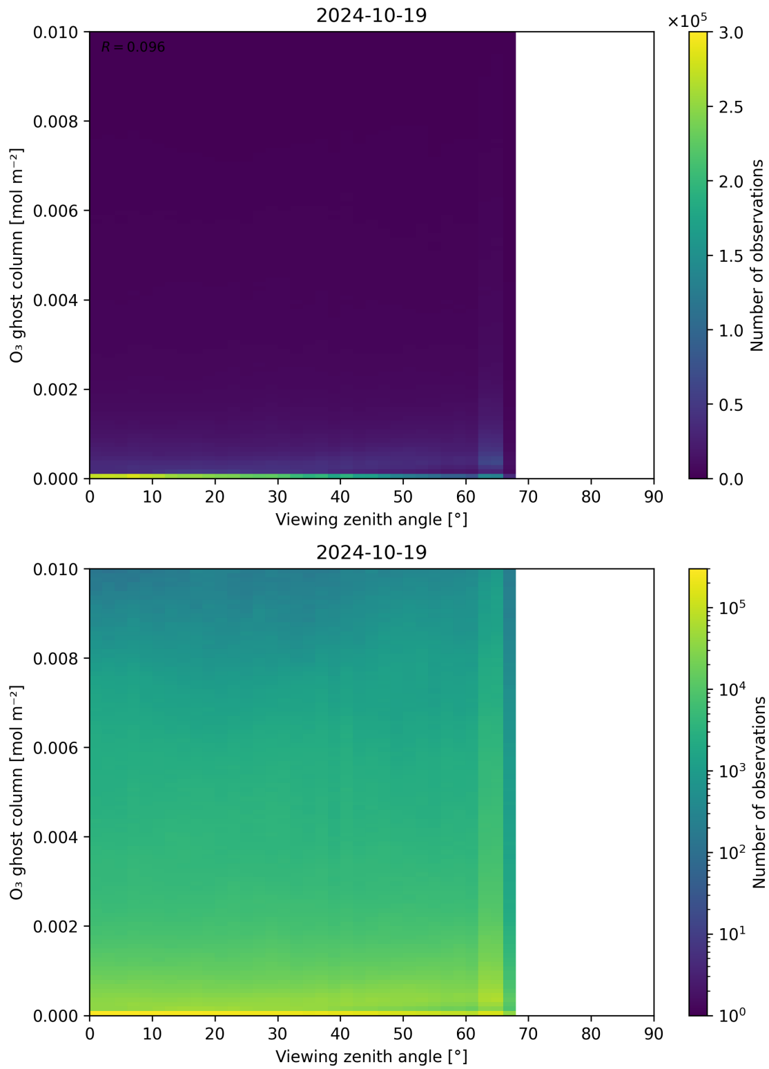
Figure 51: Scatter density plot of “Viewing zenith angle” against “O 3 ghost column” for 2024-10-19 to 2024-10-20.
