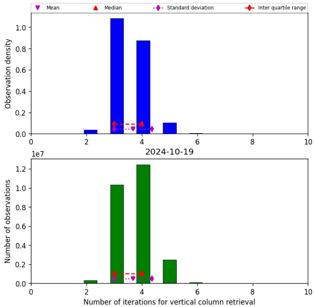
Figure 26: Histogram of “Number of iterations for vertical column retrieval” for 2024-10-19 to 2024-10-20
