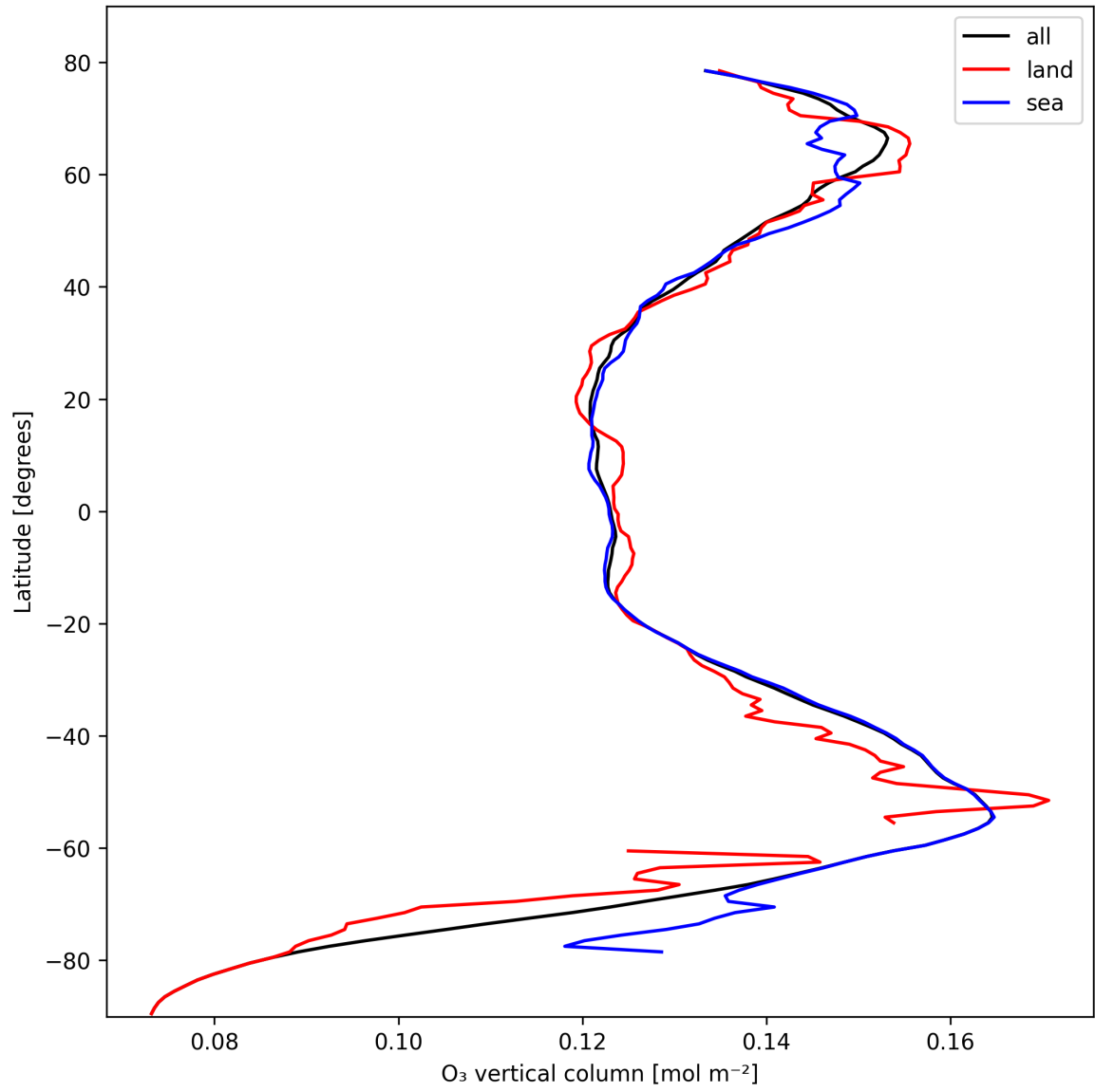
Figure 14: Zonal average of “O 3 vertical column” for 2024-10-19 to 2024-10-20.
