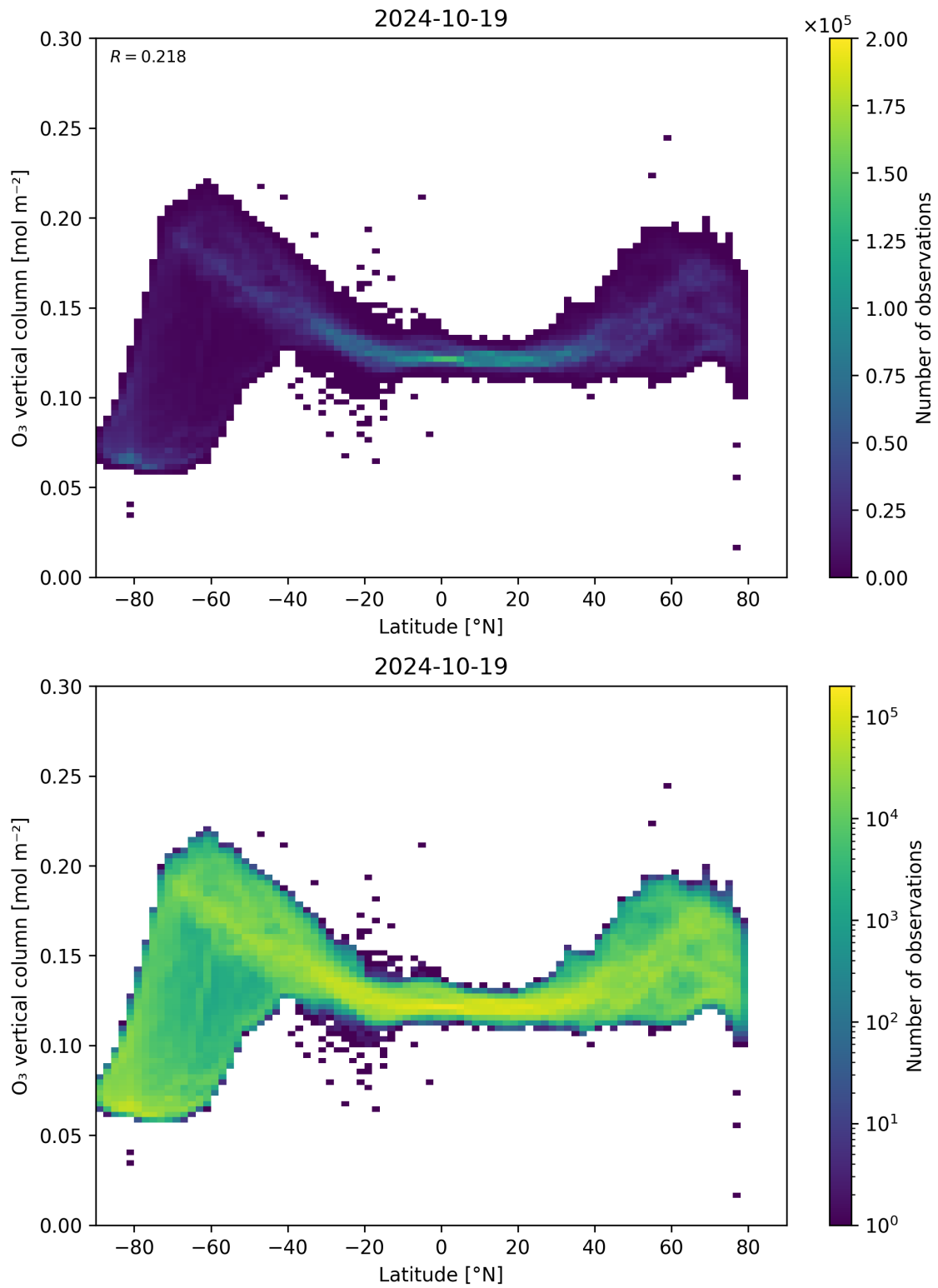
Figure 36: Scatter density plot of “Latitude” against “O 3 vertical column” for 2024-10-19 to 2024-10-20.
