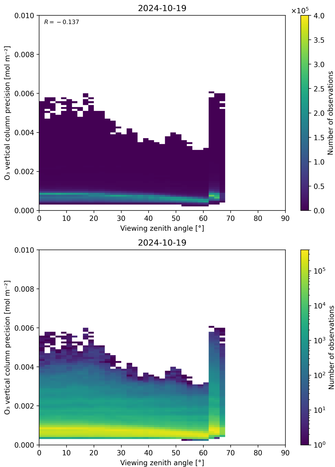
Figure 53: Scatter density plot of “Viewing zenith angle” against “O 3 vertical column precision” for 2024-10-19 to 2024-10-20.
