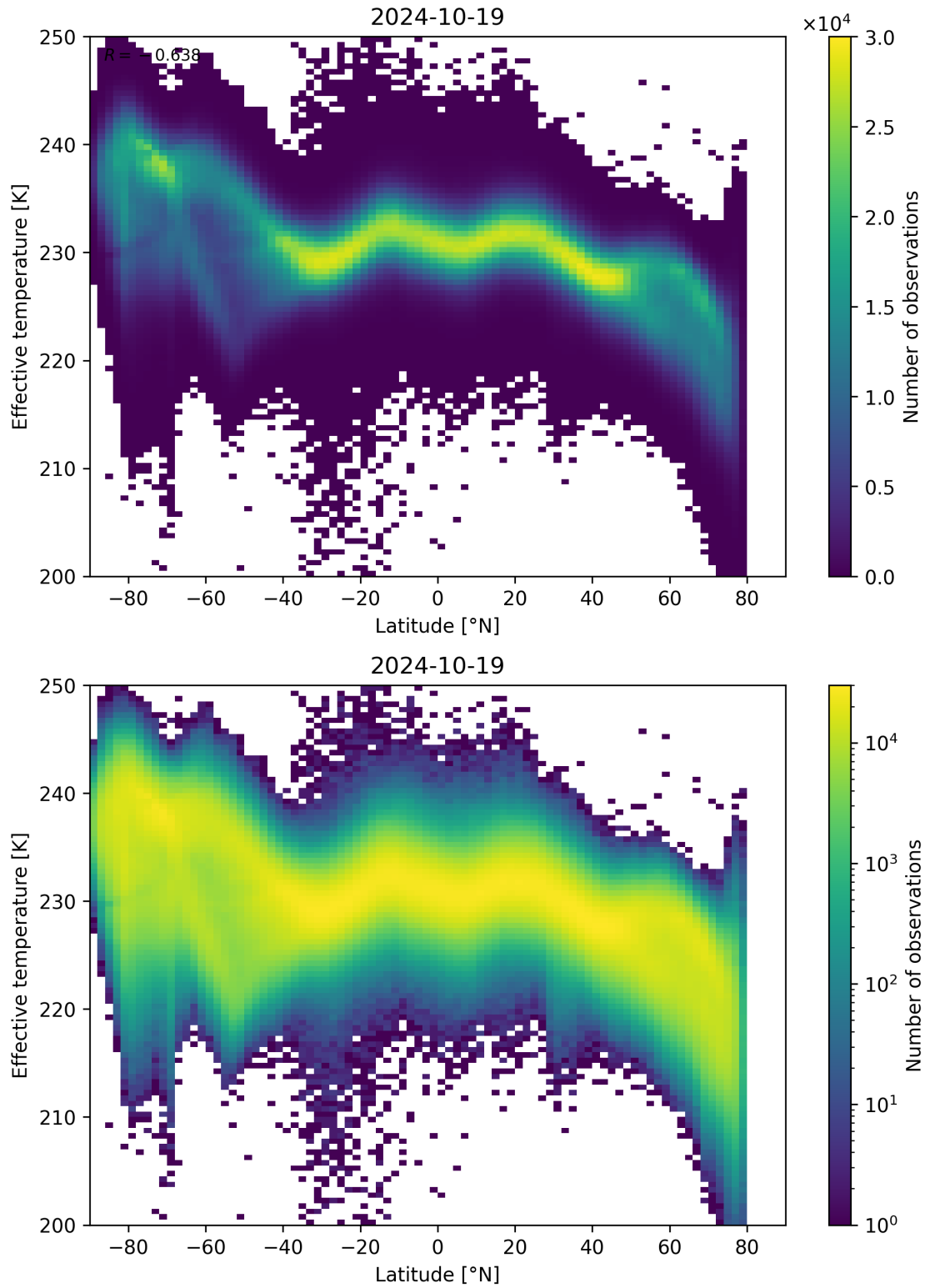
Figure 34: Scatter density plot of “Latitude” against “Effective temperature” for 2024-10-19 to 2024-10-20.
