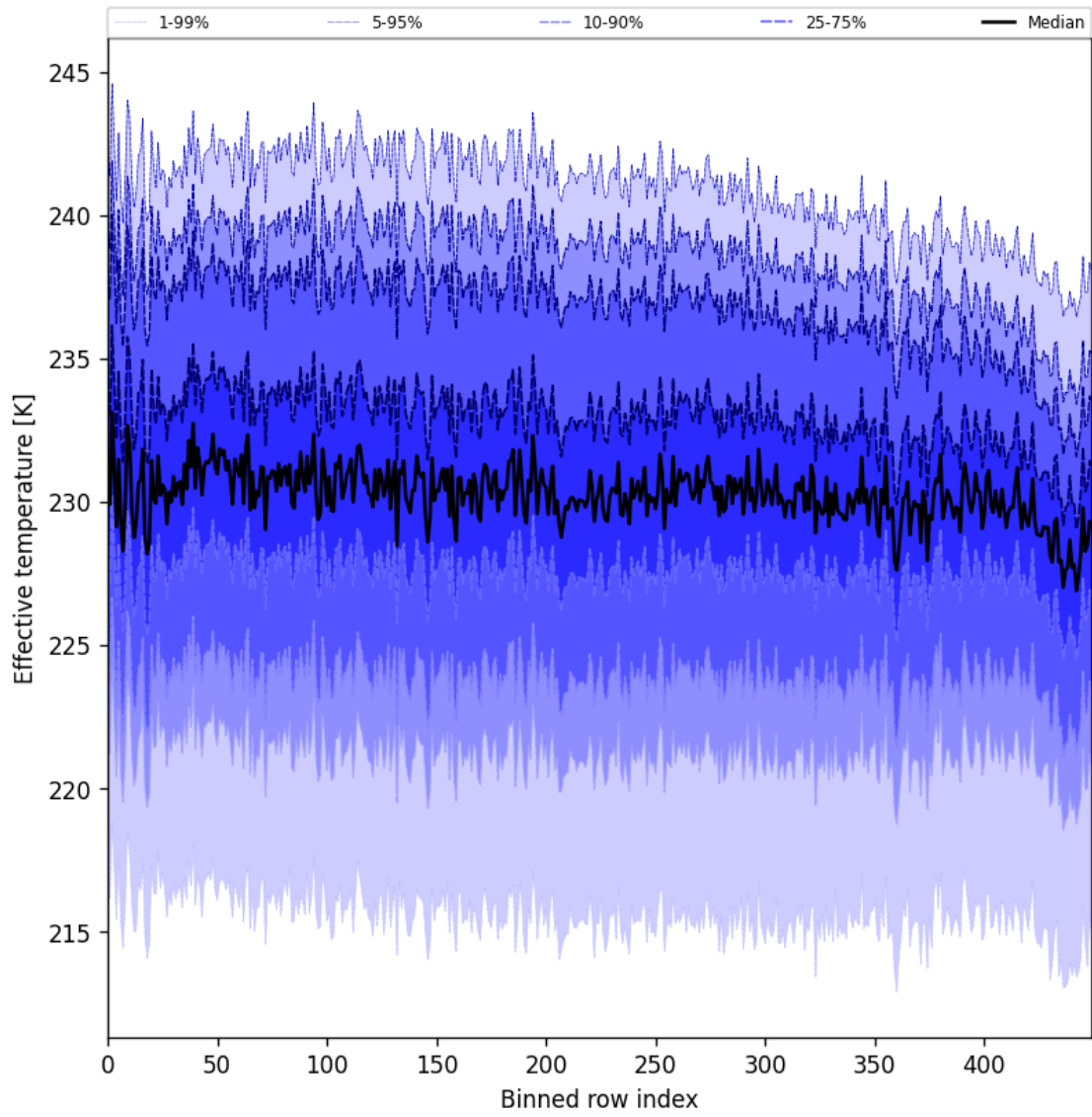
Figure 31: Along track statistics of “Effective temperature” for 2024-10-19 to 2024-10-20
