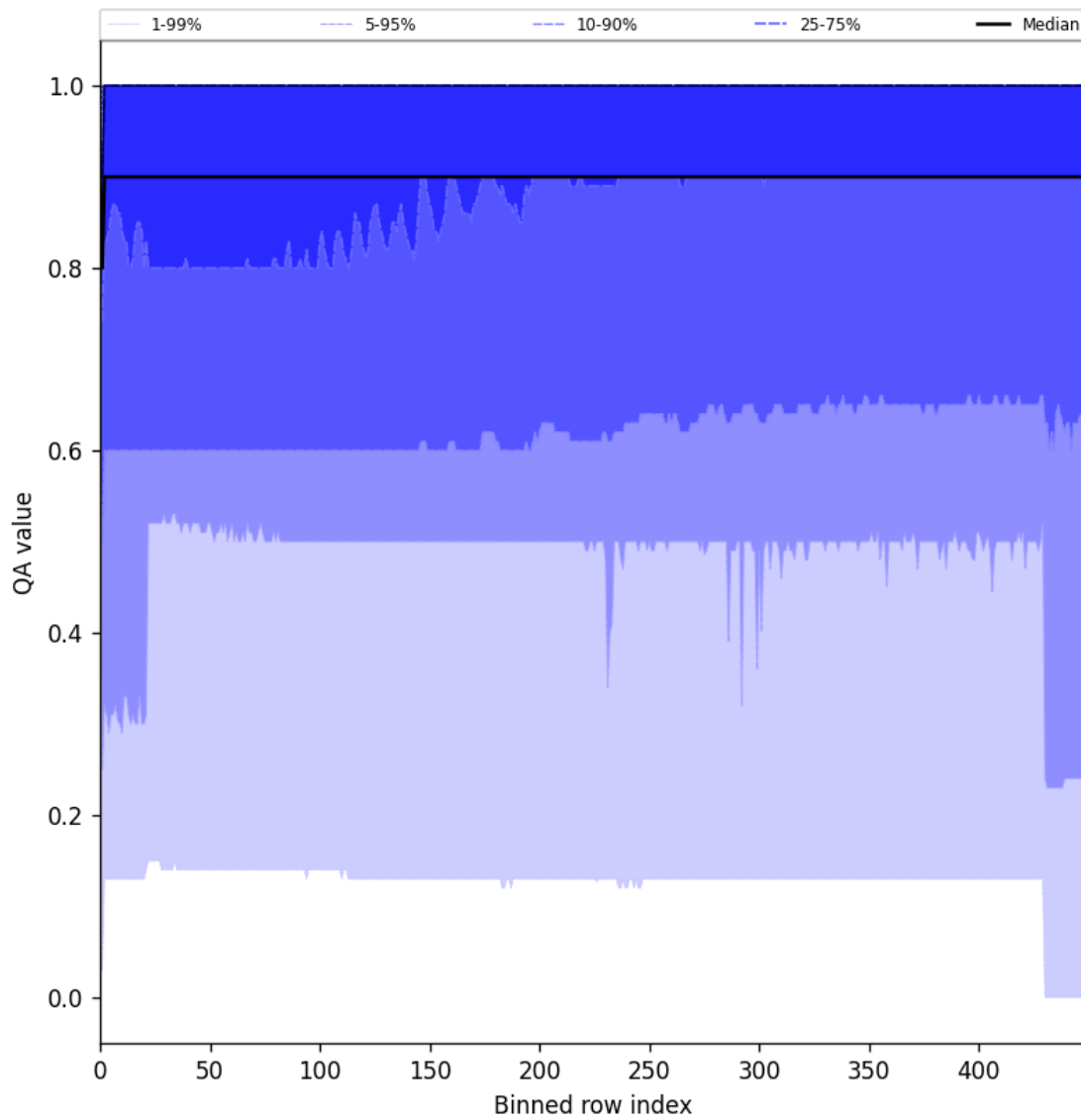
Figure 27: Along track statistics of “QA value” for 2024-10-19 to 2024-10-20
