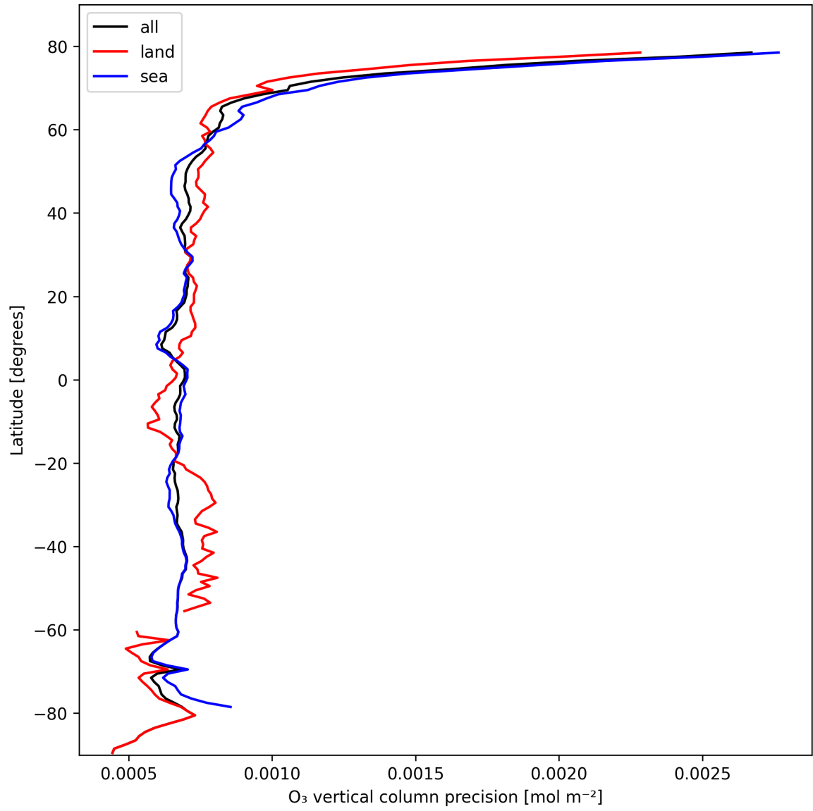
Figure 15: Zonal average of “O 3 vertical column precision” for 2024-10-19 to 2024-10-20.
