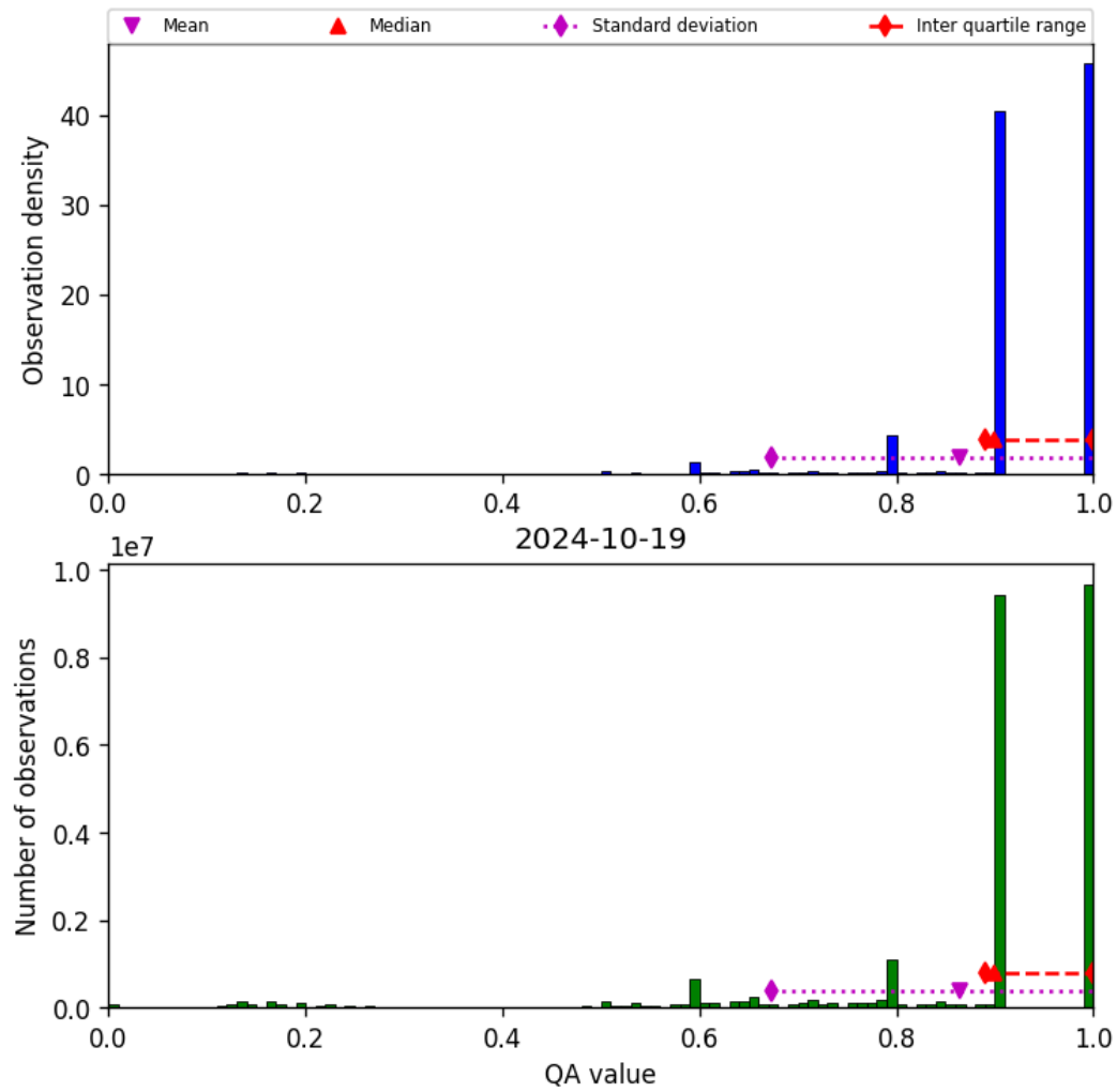
Figure 20: Histogram of “QA value” for 2024-10-19 to 2024-10-20
