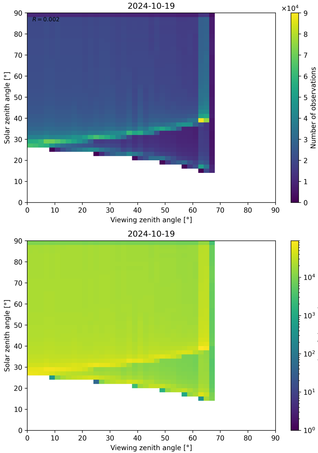
Figure 54: Scatter density plot of “Viewing zenith angle” against “Solar zenith angle” for 2024-10-19 to 2024-10-20.
