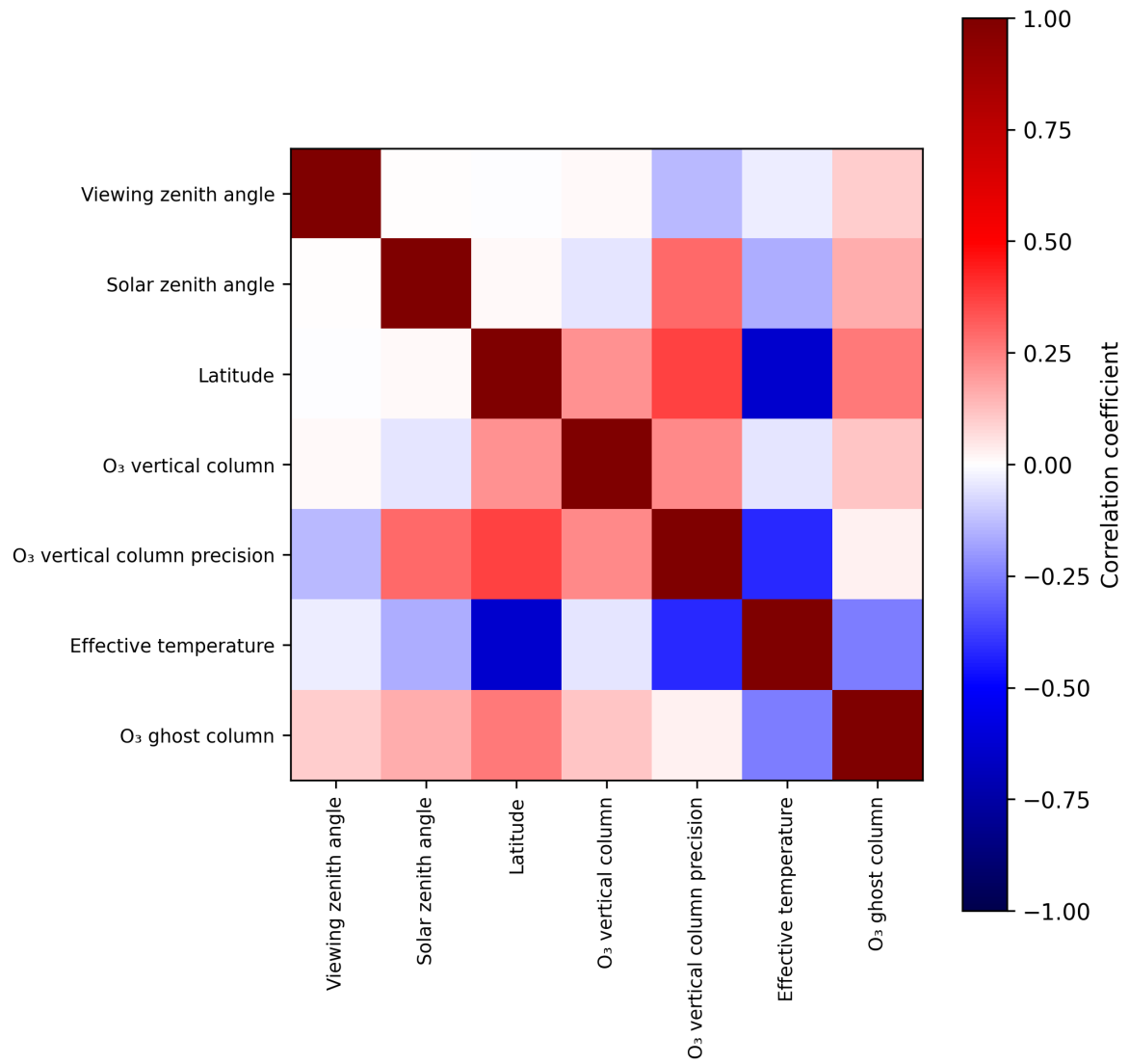
Figure 2: Map of correlation matrix for 2024-10-19 to 2024-10-20.
