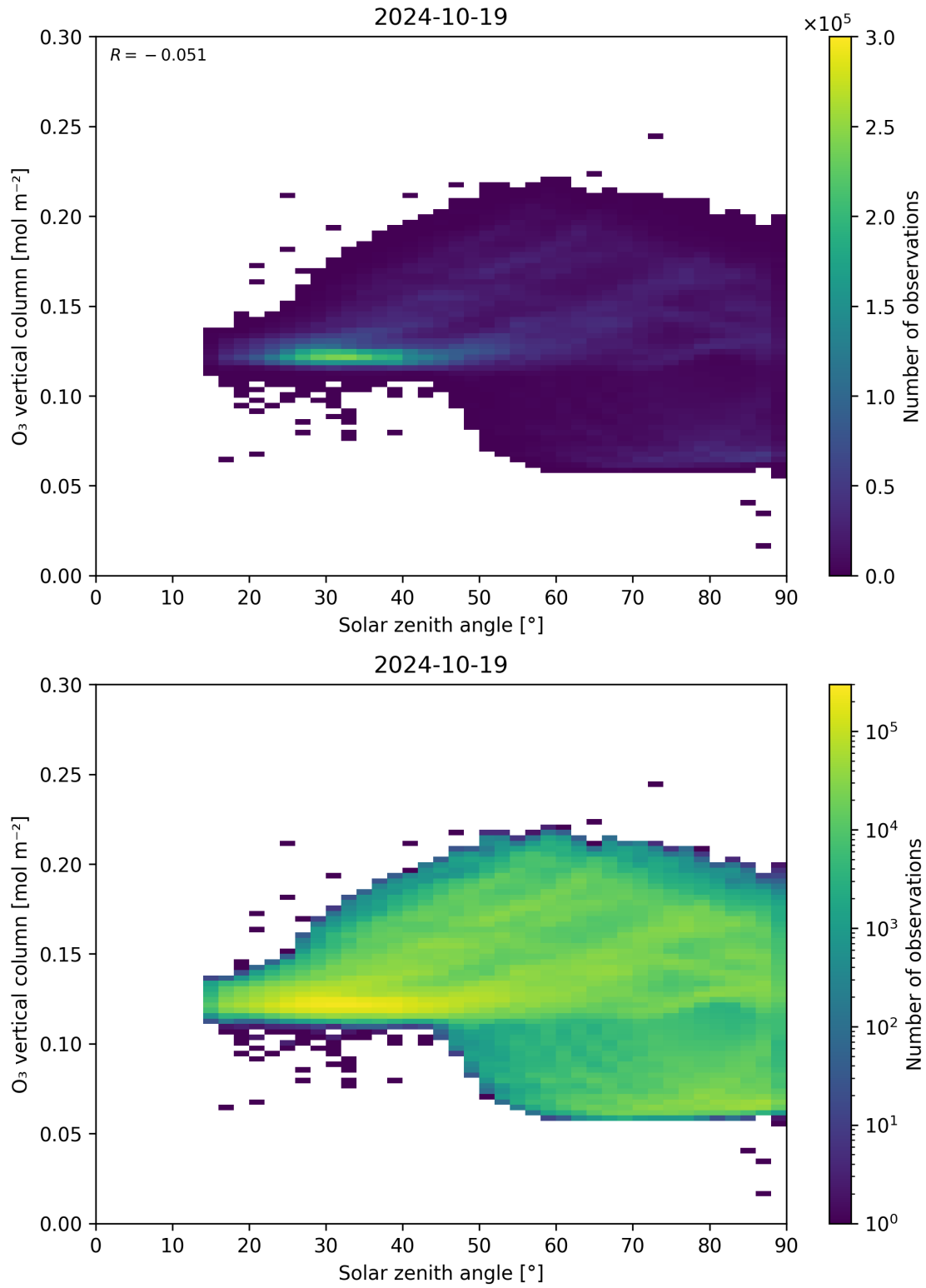
Figure 47: Scatter density plot of “Solar zenith angle” against “O 3 vertical column” for 2024-10-19 to 2024-10-20.
