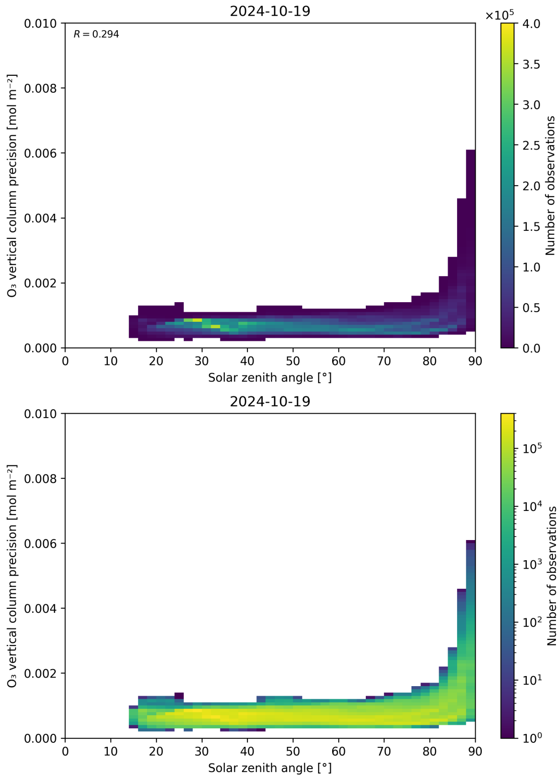
Figure 48: Scatter density plot of “Solar zenith angle” against “O 3 vertical column precision” for 2024-10-19 to 2024-10-20.
