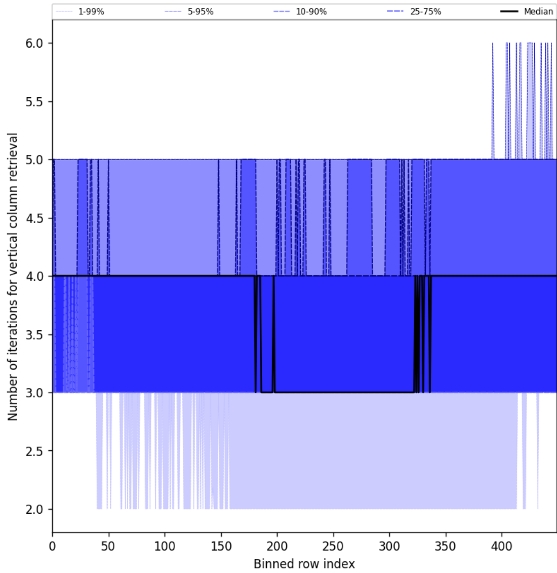
Figure 33: Along track statistics of “Number of iterations for vertical column retrieval” for 2024-10-19 to 2024-10-20
