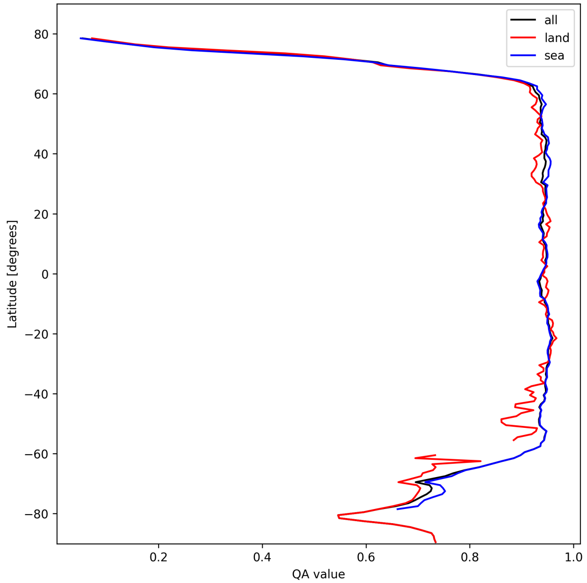
Figure 13: Zonal average of “QA value” for 2024-10-19 to 2024-10-20.
