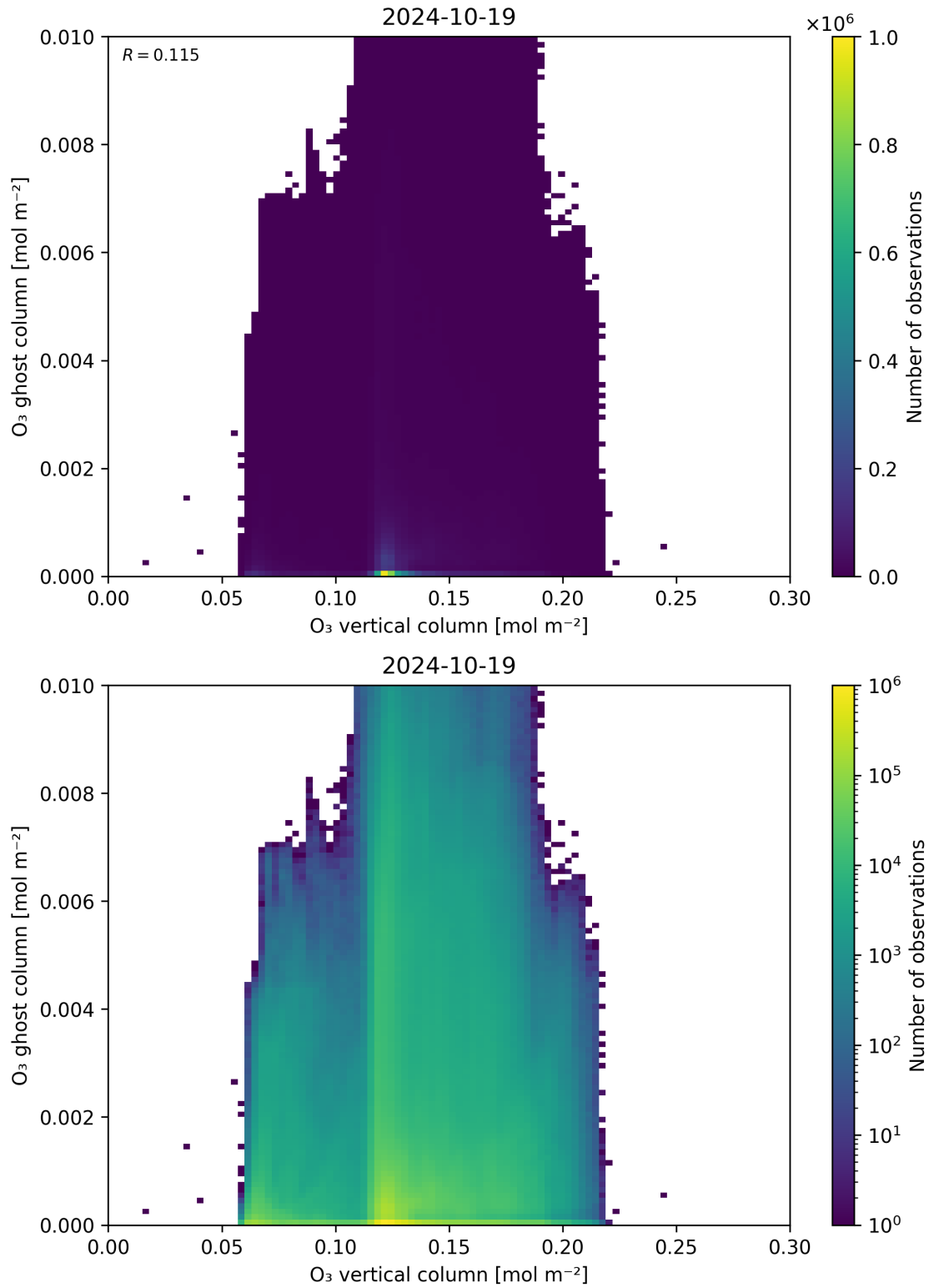
Figure 40: Scatter density plot of “O 3 vertical column” against “O 3 ghost column” for 2024-10-19 to 2024-10-20.
