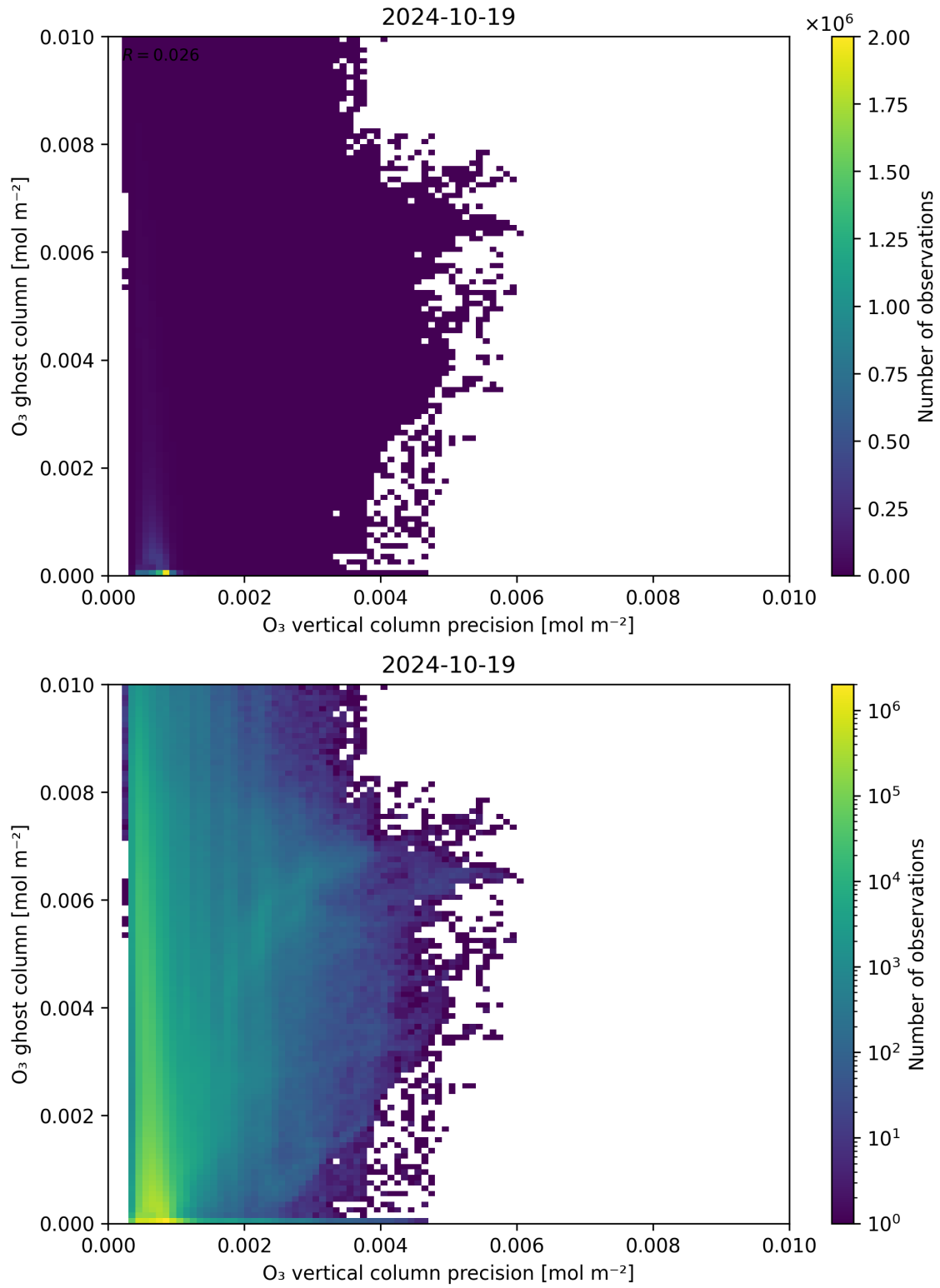
Figure 43: Scatter density plot of “O 3 vertical column precision” against “O 3 ghost column” for 2024-10-19 to 2024-10-20.
