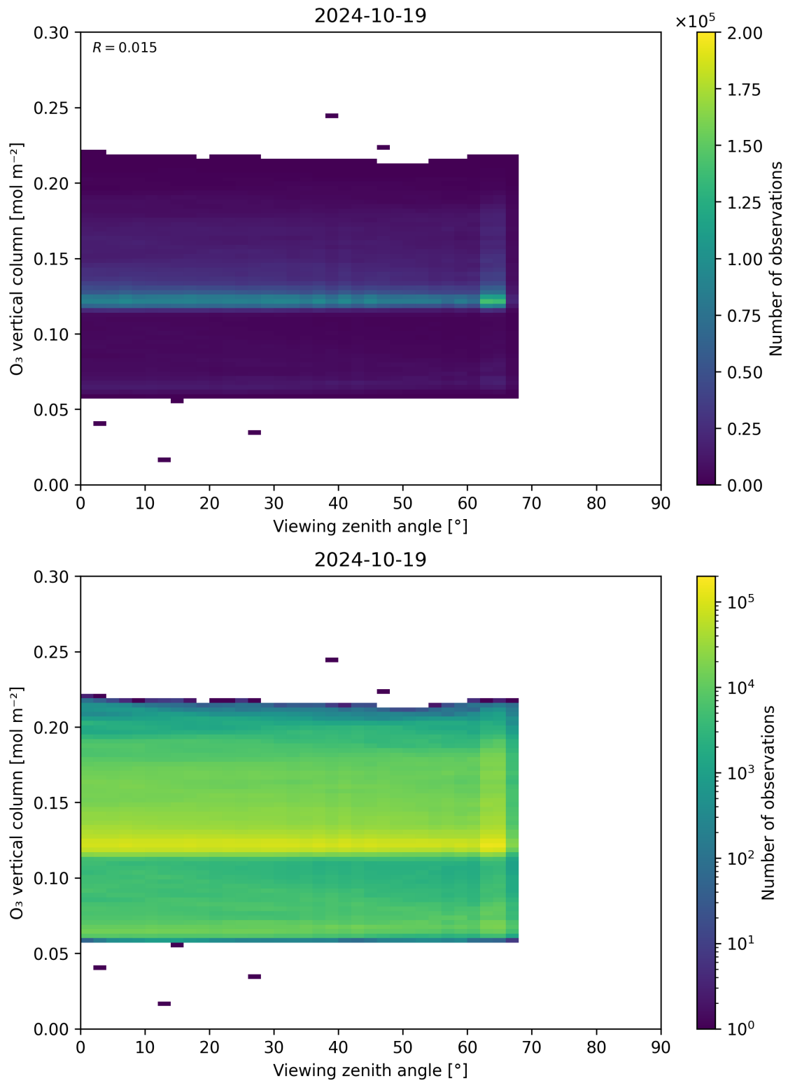
Figure 52: Scatter density plot of “Viewing zenith angle” against “O 3 vertical column” for 2024-10-19 to 2024-10-20.
