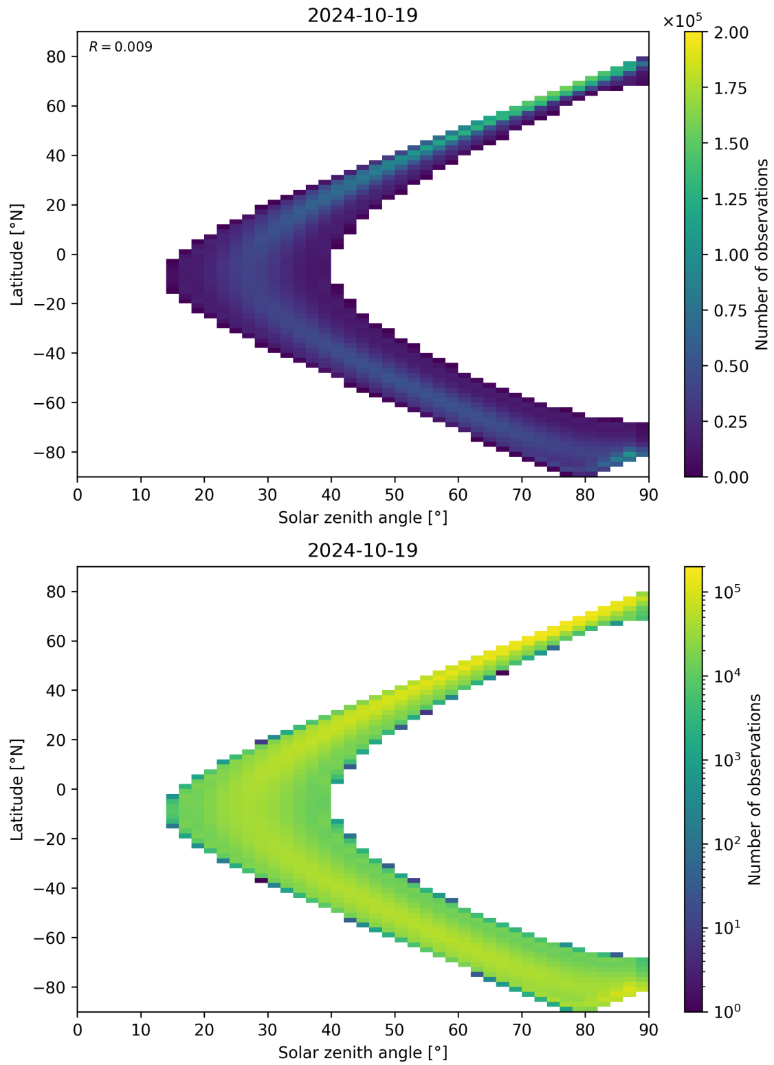
Figure 44: Scatter density plot of “Solar zenith angle” against “Latitude” for 2024-10-19 to 2024-10-20.
