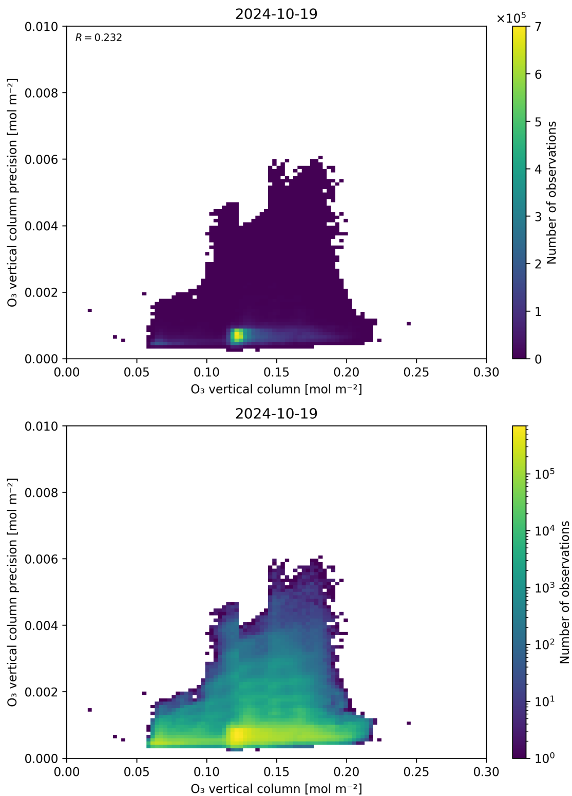
Figure 41: Scatter density plot of “O 3 vertical column” against “O 3 vertical column precision” for 2024-10-19 to 2024-10-20.
