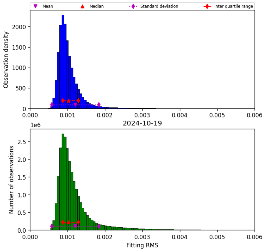
Figure 23: Histogram of “Fitting RMS” for 2024-10-19 to 2024-10-20
