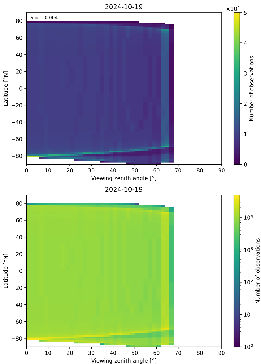
Figure 49: Scatter density plot of “Viewing zenith angle” against “Latitude” for 2024-10-19 to 2024-10-20.
