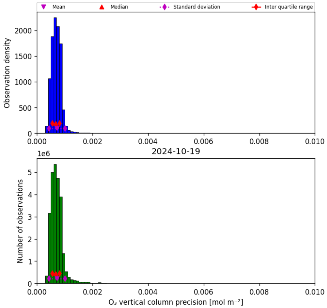
Figure 22: Histogram of “O 3 vertical column precision” for 2024-10-19 to 2024-10-20
