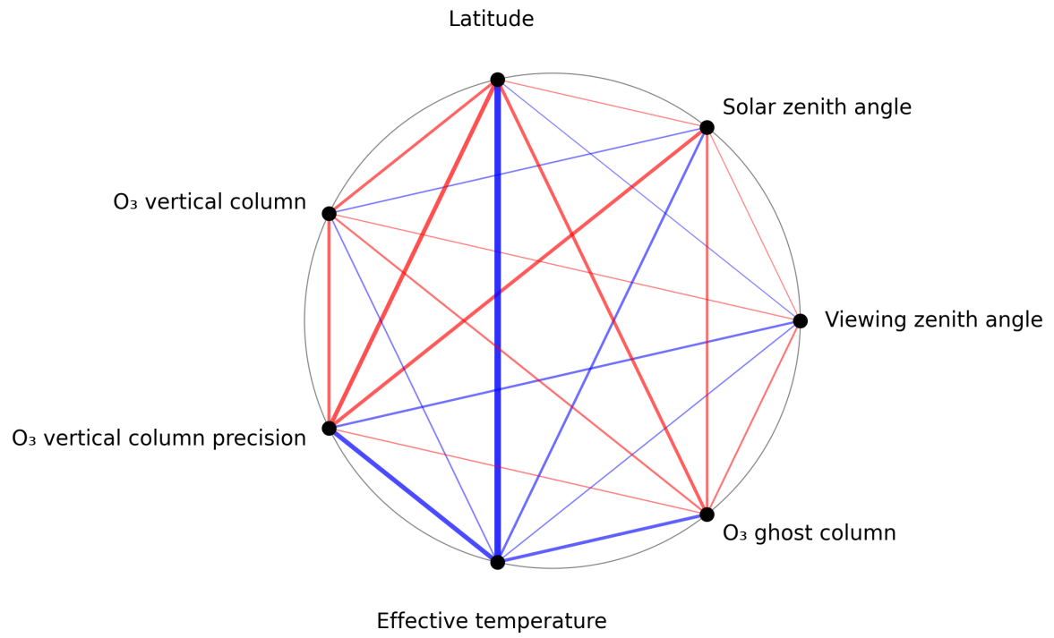
Figure 1: Map of correlation graph for 2024-10-19 to 2024-10-20.
