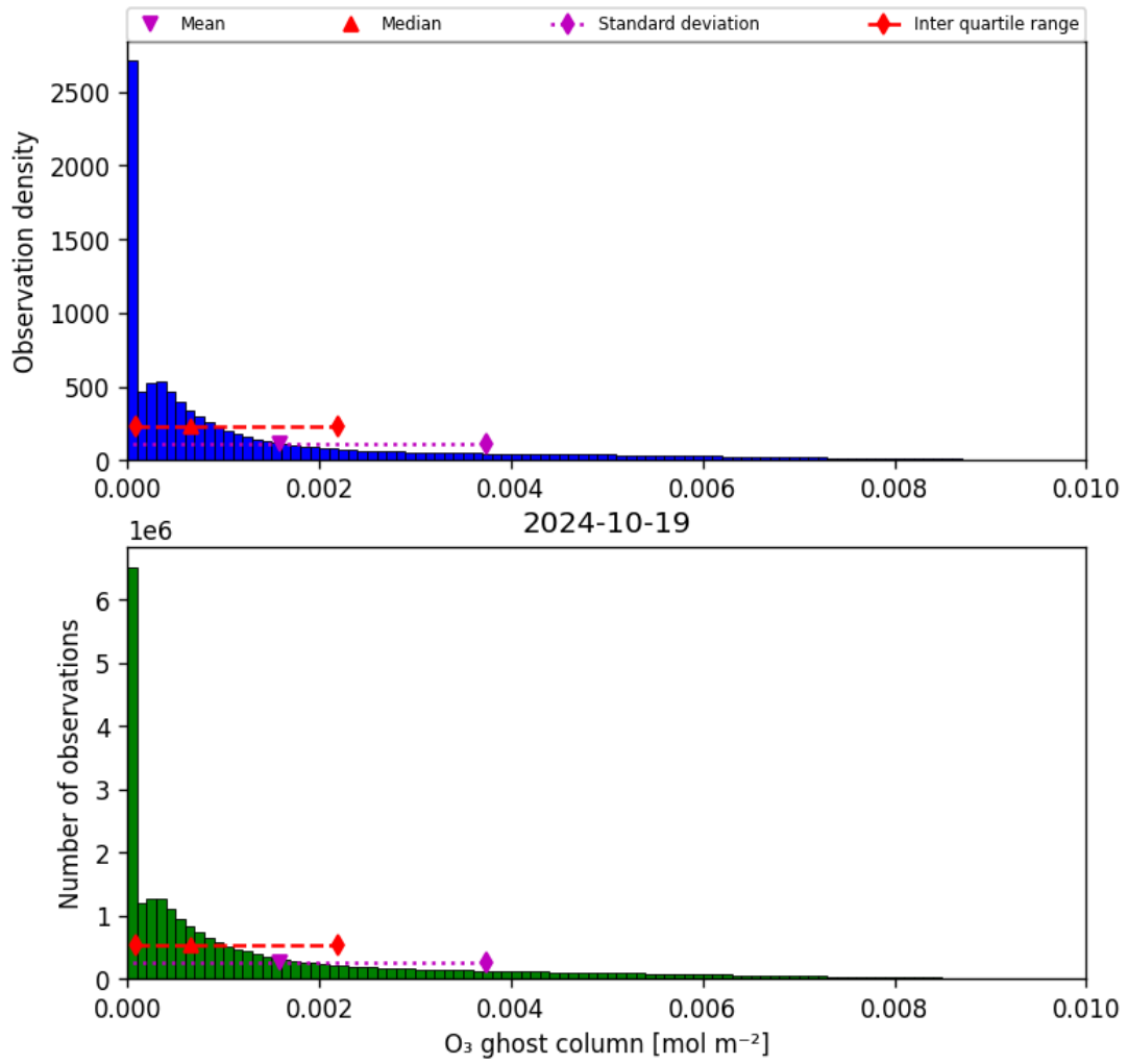
Figure 25: Histogram of “O 3 ghost column” for 2024-10-19 to 2024-10-20
