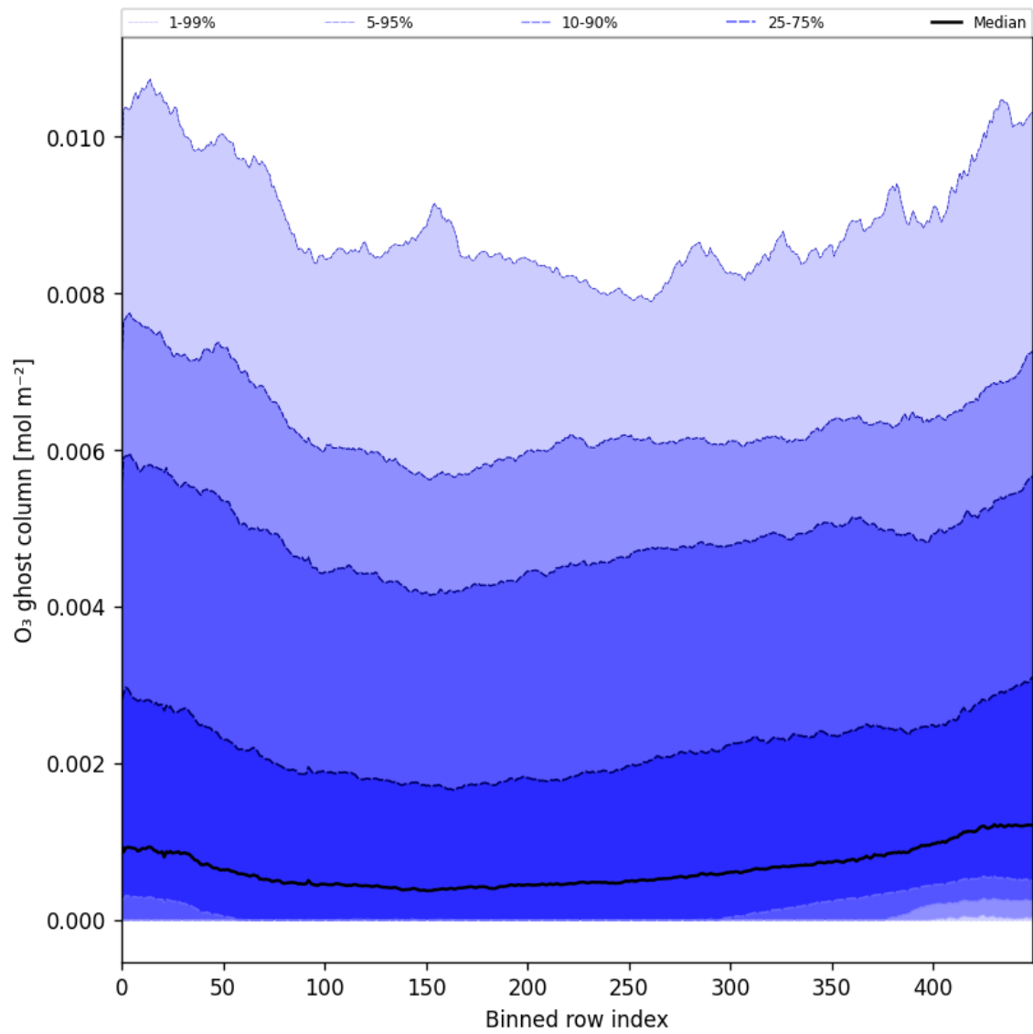
Figure 32: Along track statistics of “O 3 ghost column” for 2024-10-19 to 2024-10-20
