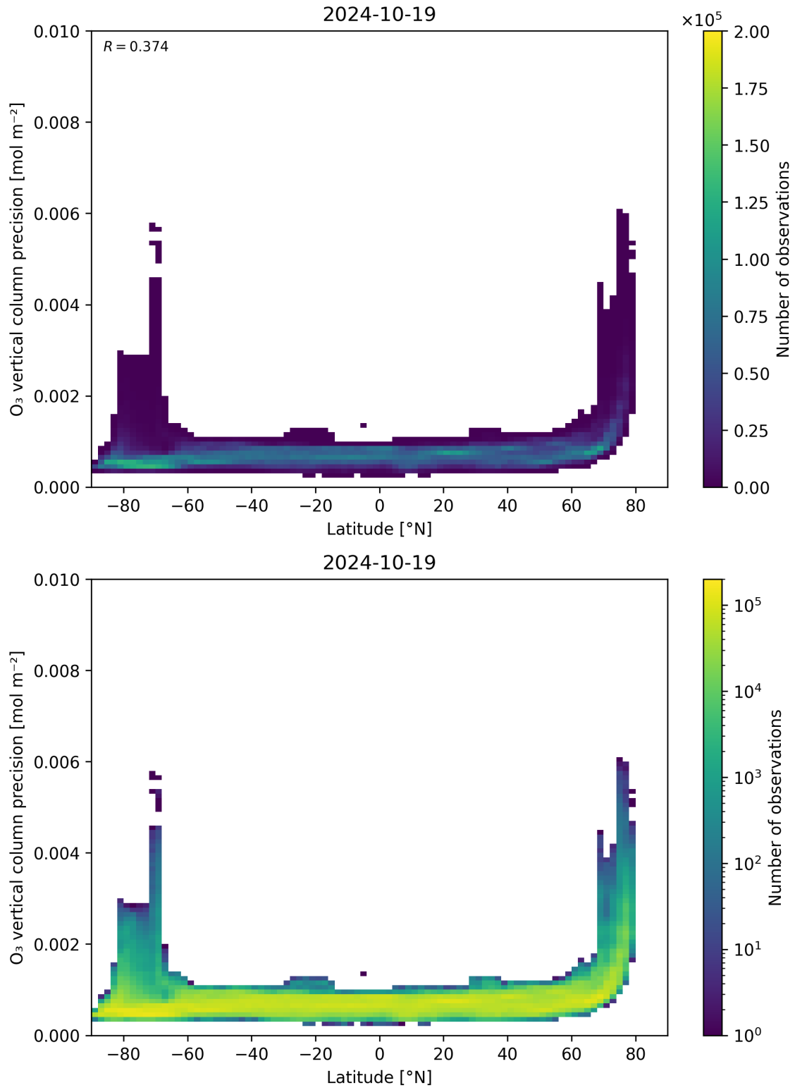
Figure 37: Scatter density plot of “Latitude” against “O 3 vertical column precision” for 2024-10-19 to 2024-10-20.
