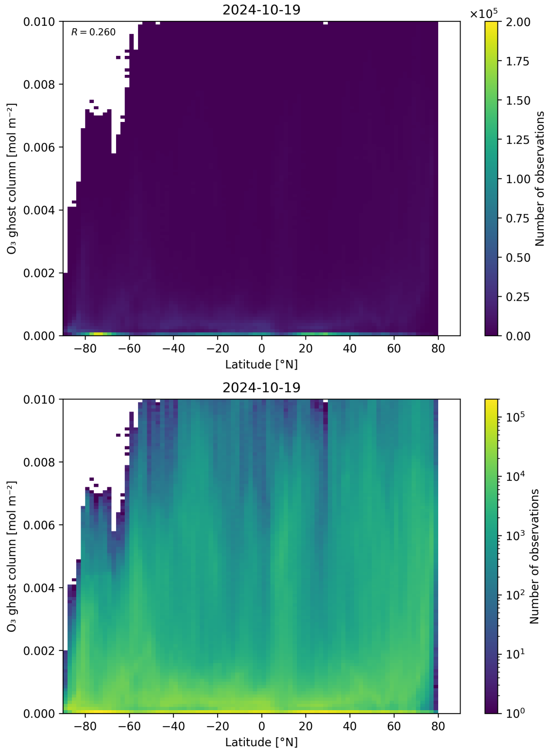
Figure 35: Scatter density plot of “Latitude” against “O 3 ghost column” for 2024-10-19 to 2024-10-20.
