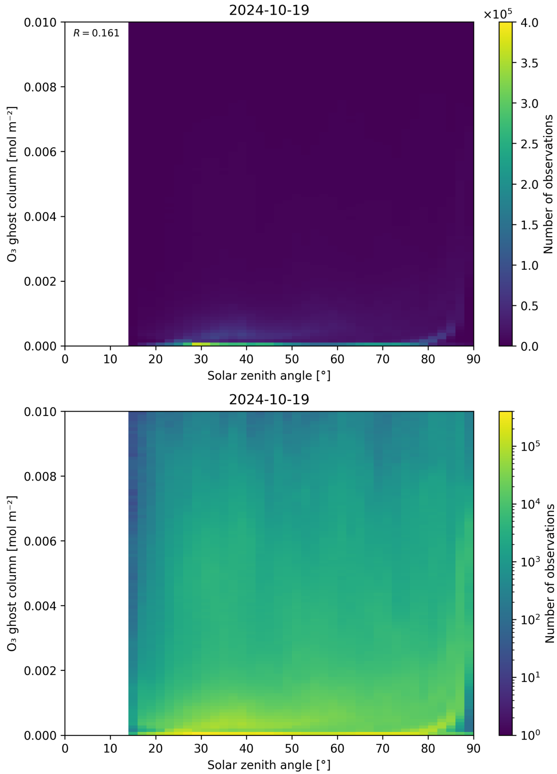
Figure 46: Scatter density plot of “Solar zenith angle” against “O 3 ghost column” for 2024-10-19 to 2024-10-20.
