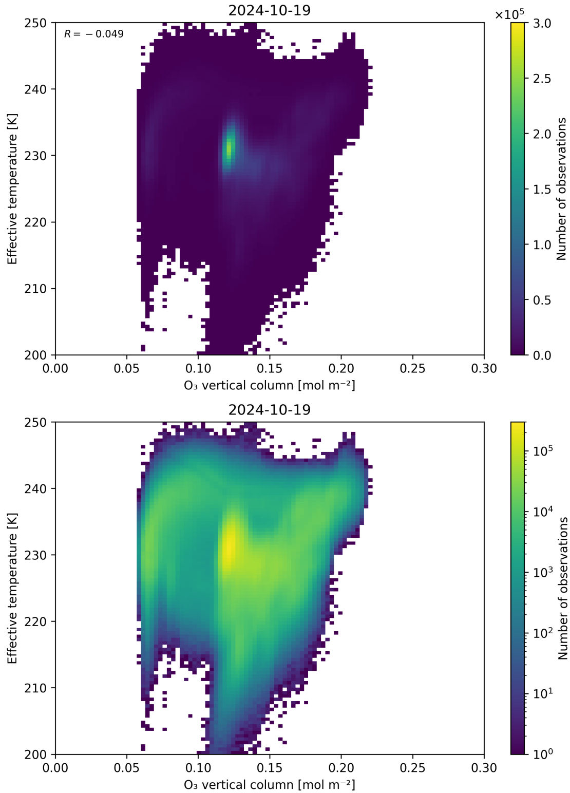
Figure 39: Scatter density plot of “O 3 vertical column” against “Effective temperature” for 2024-10-19 to 2024-10-20.
