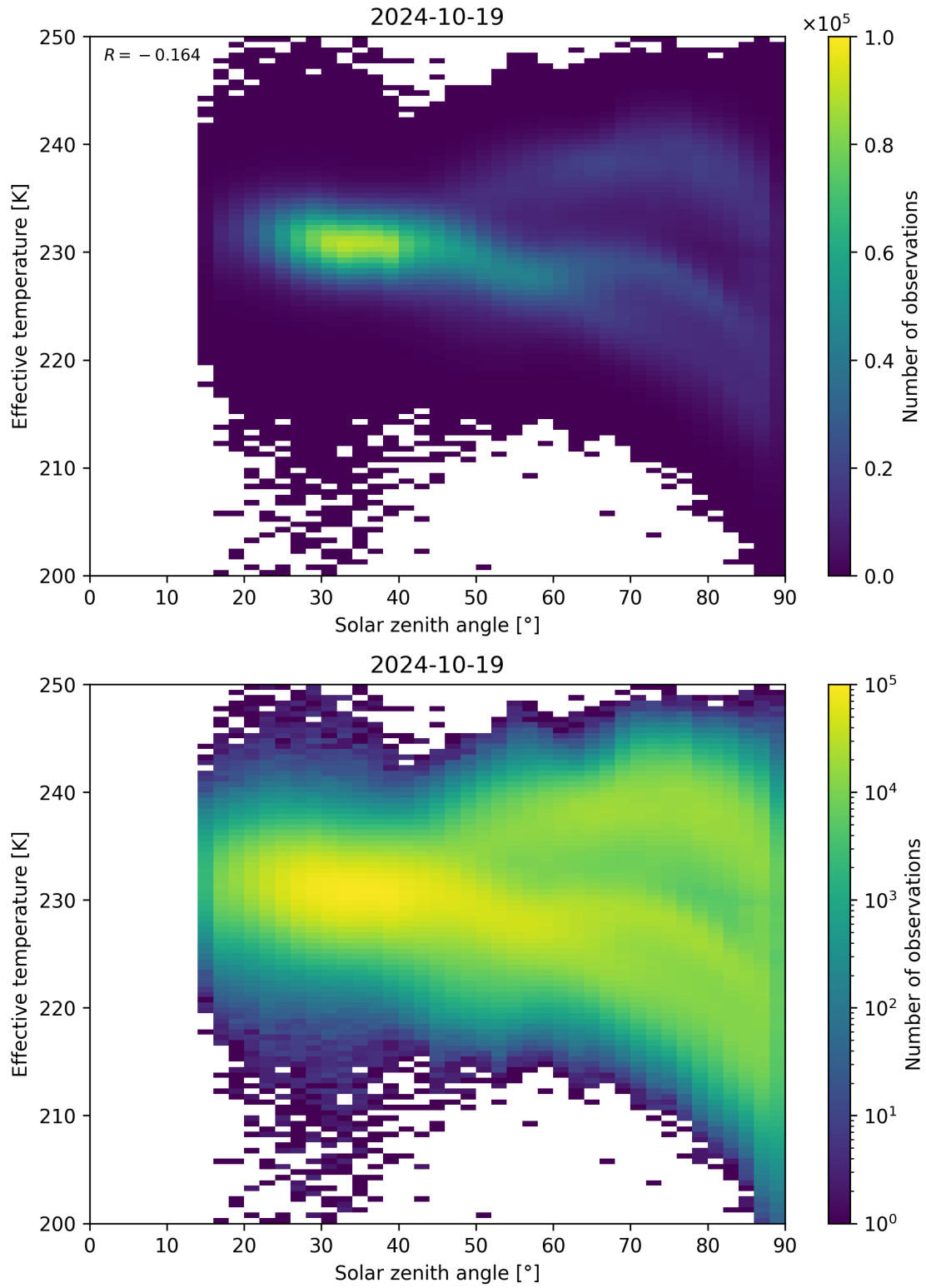
Figure 45: Scatter density plot of “Solar zenith angle” against “Effective temperature” for 2024-10-19 to 2024-10-20.
