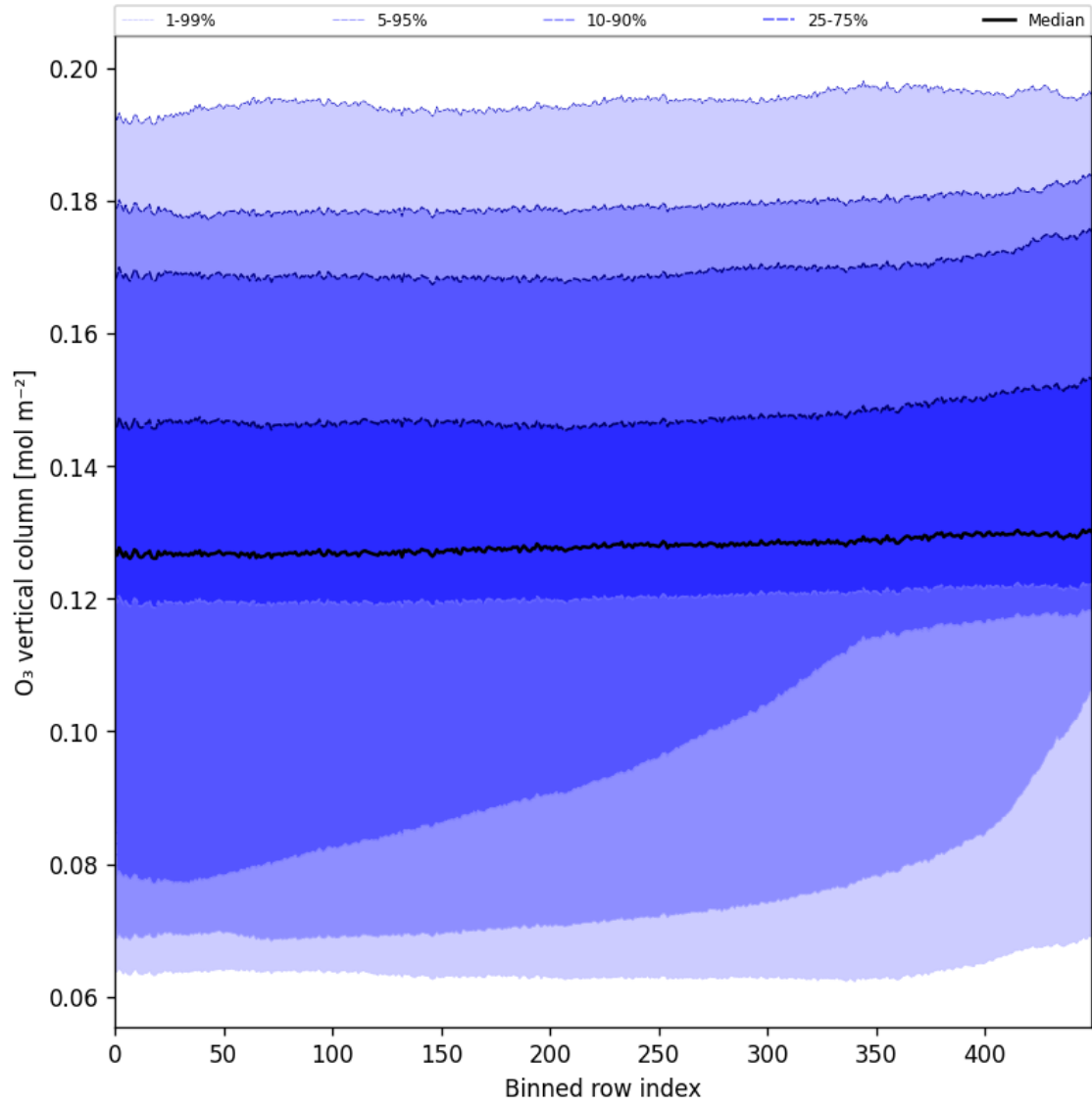
Figure 28: Along track statistics of “O 3 vertical column” for 2024-10-19 to 2024-10-20
