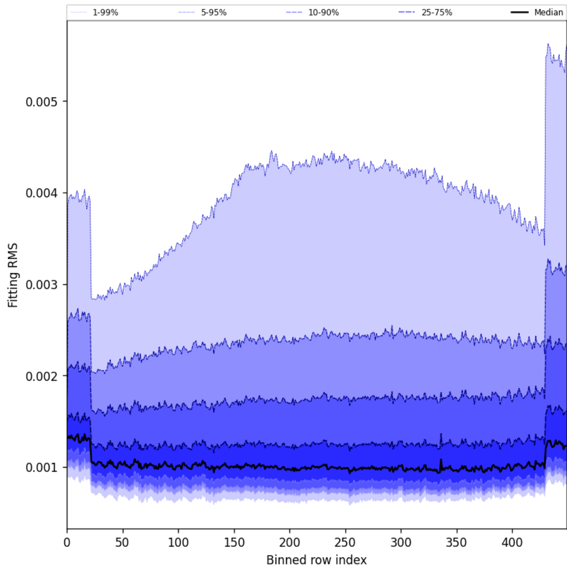
Figure 30: Along track statistics of “Fitting RMS” for 2024-10-19 to 2024-10-20
