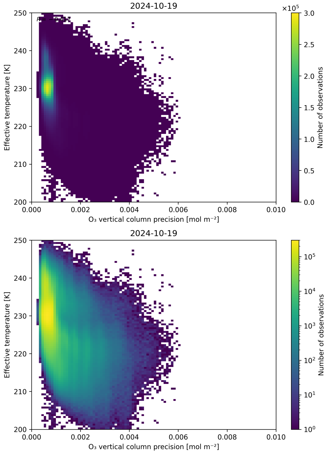
Figure 42: Scatter density plot of “ O_3 vertical column precision” against “Effective temperature” for 2024-10-19 to 2024-10-20.
