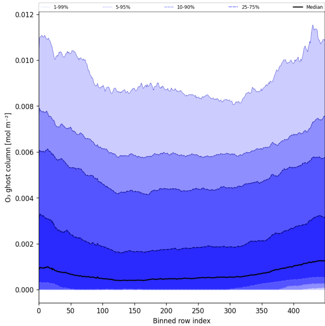
Figure 32: Along track statistics of "O 3 ghost column" for 2024-10-19 to 2024-10-21
