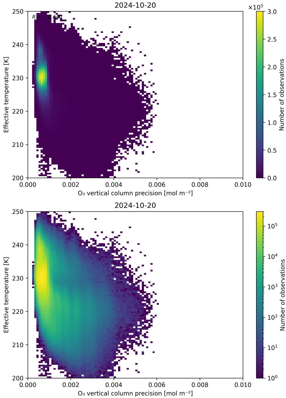
Figure 42: Scatter density plot of “O 3 vertical column precision” against “Effective temperature” for 2024-10-19 to 2024-10-21.
