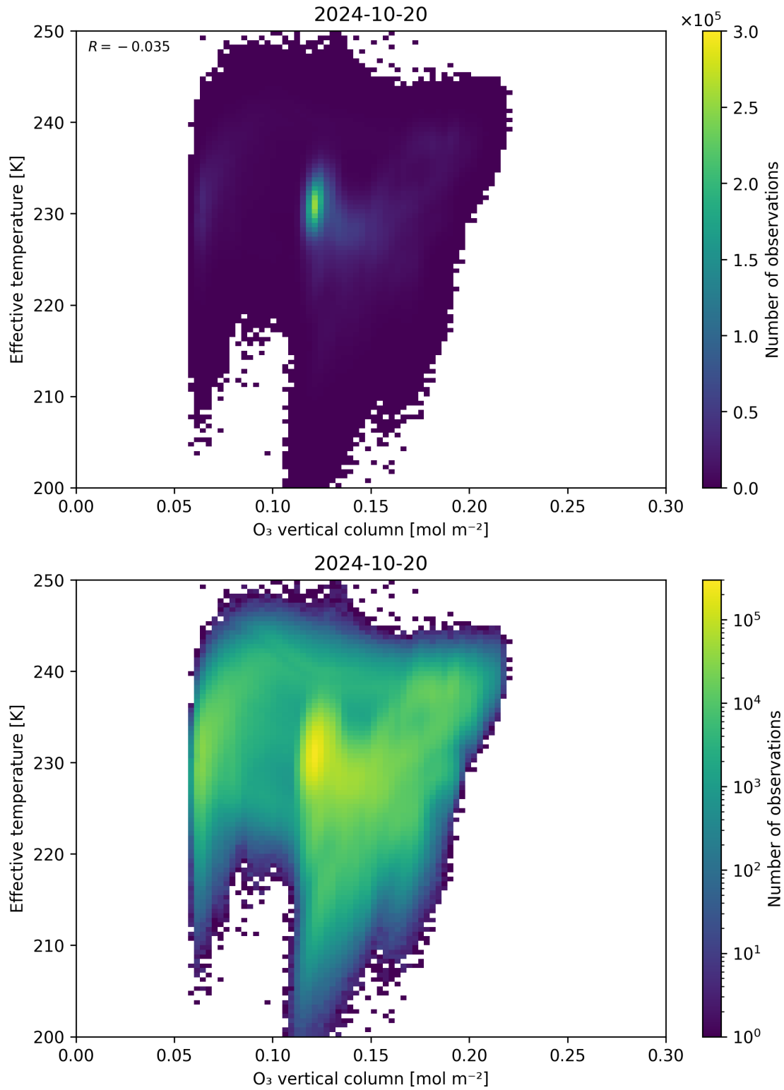
Figure 39: Scatter density plot of “O 3 vertical column” against “Effective temperature” for 2024-10-19 to 2024-10-21.
