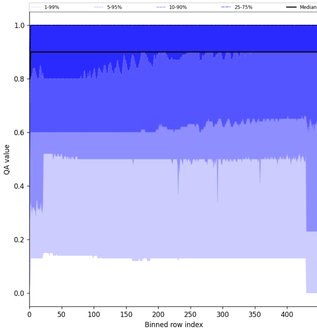
Figure 27: Along track statistics of “QA value” for 2024-10-19 to 2024-10-21
