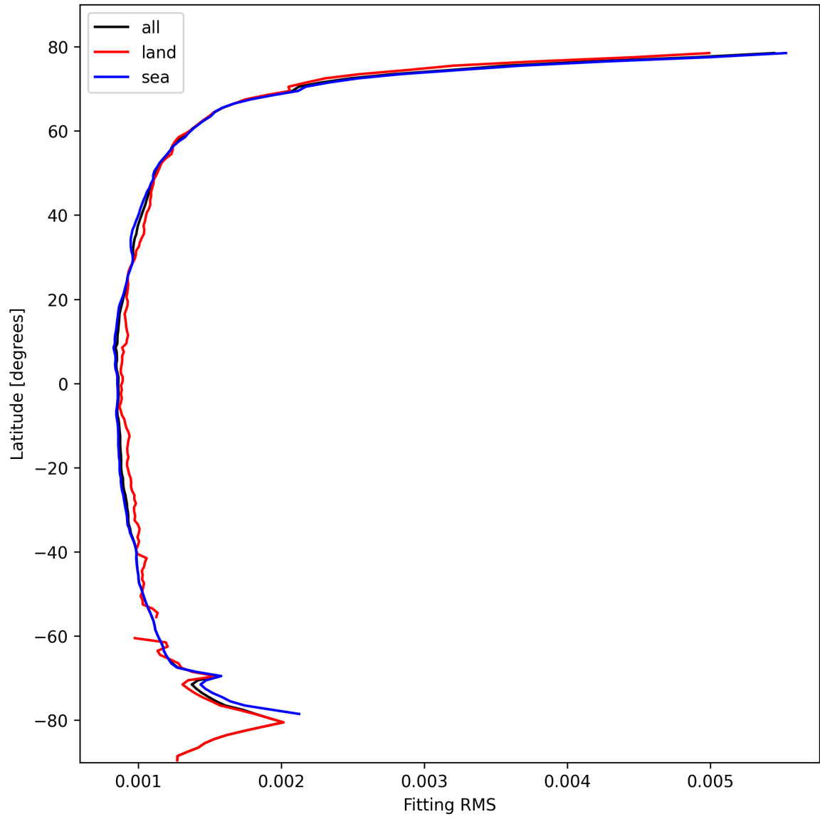
Figure 16: Zonal average of “Fitting RMS” for 2024-10-19 to 2024-10-21.
