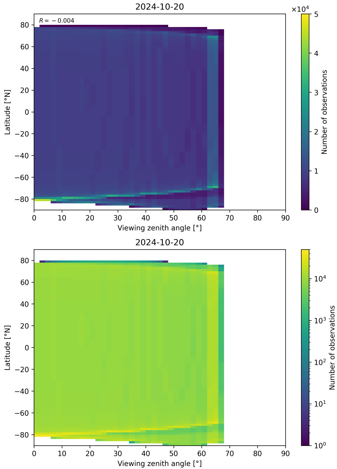
Figure 49: Scatter density plot of “Viewing zenith angle” against “Latitude” for 2024-10-19 to 2024-10-21.
