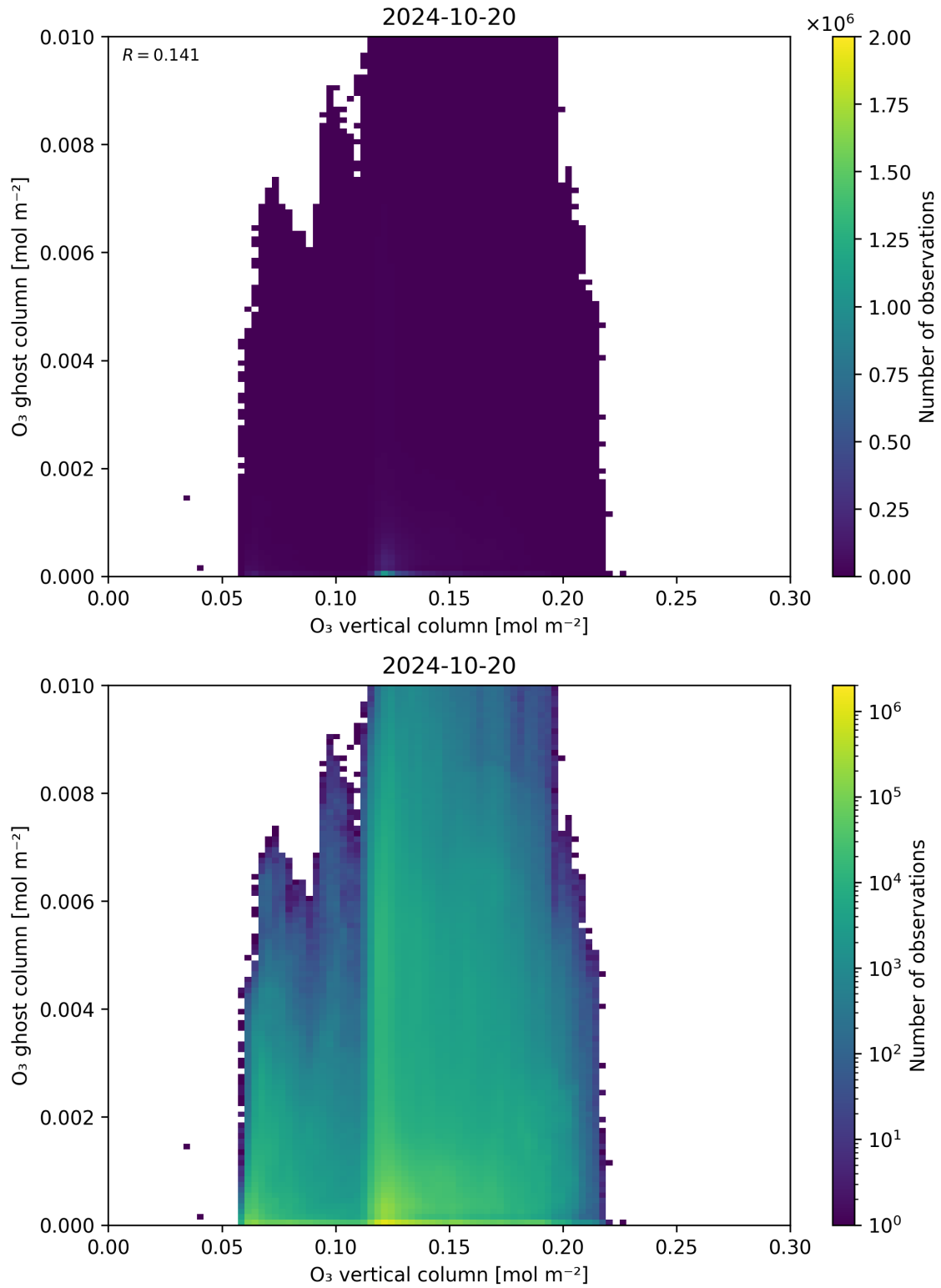
Figure 40: Scatter density plot of “O 3 vertical column” against “O 3 ghost column” for 2024-10-19 to 2024-10-21.
