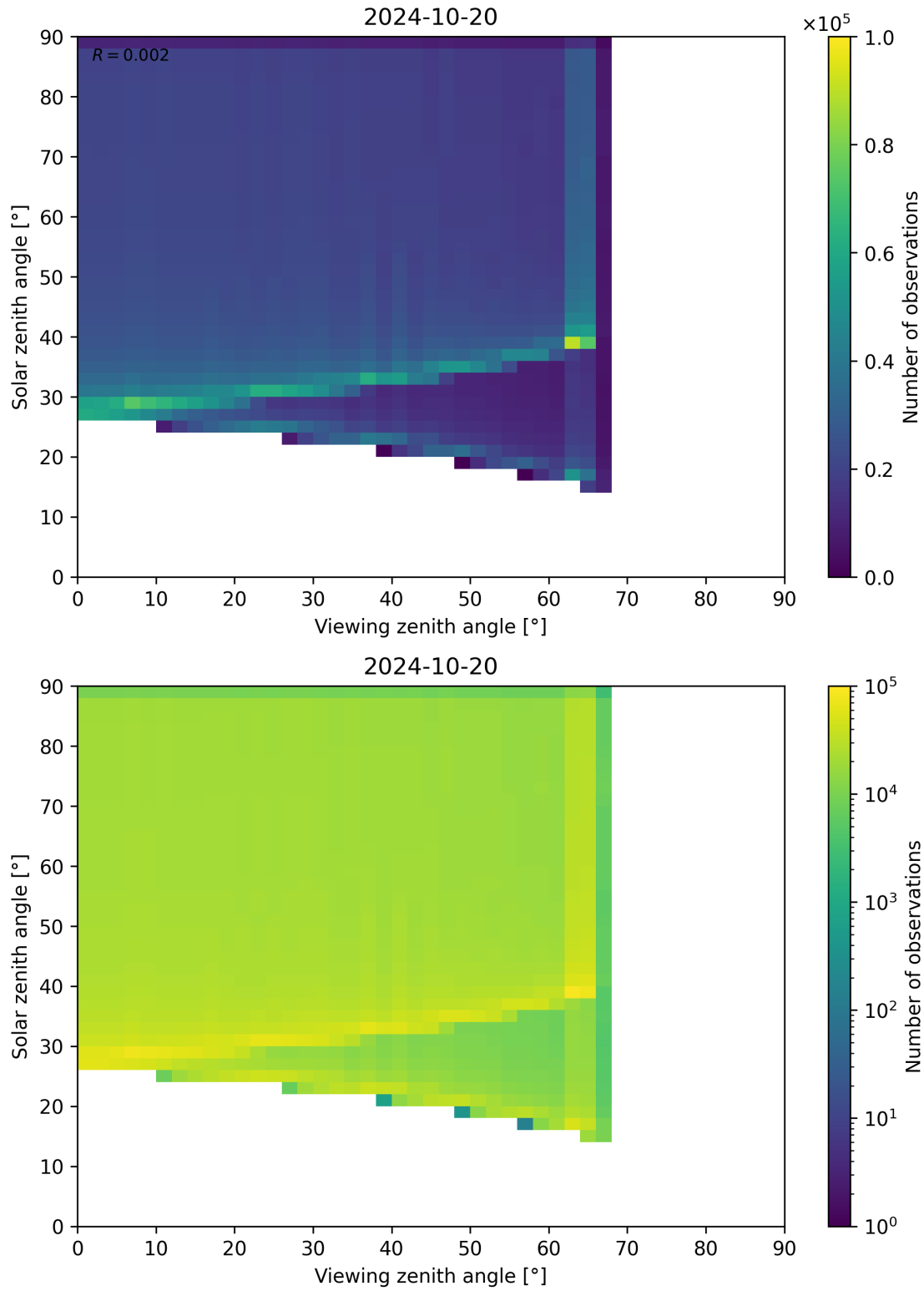
Figure 54: Scatter density plot of “Viewing zenith angle” against “Solar zenith angle” for 2024-10-19 to 2024-10-21.
