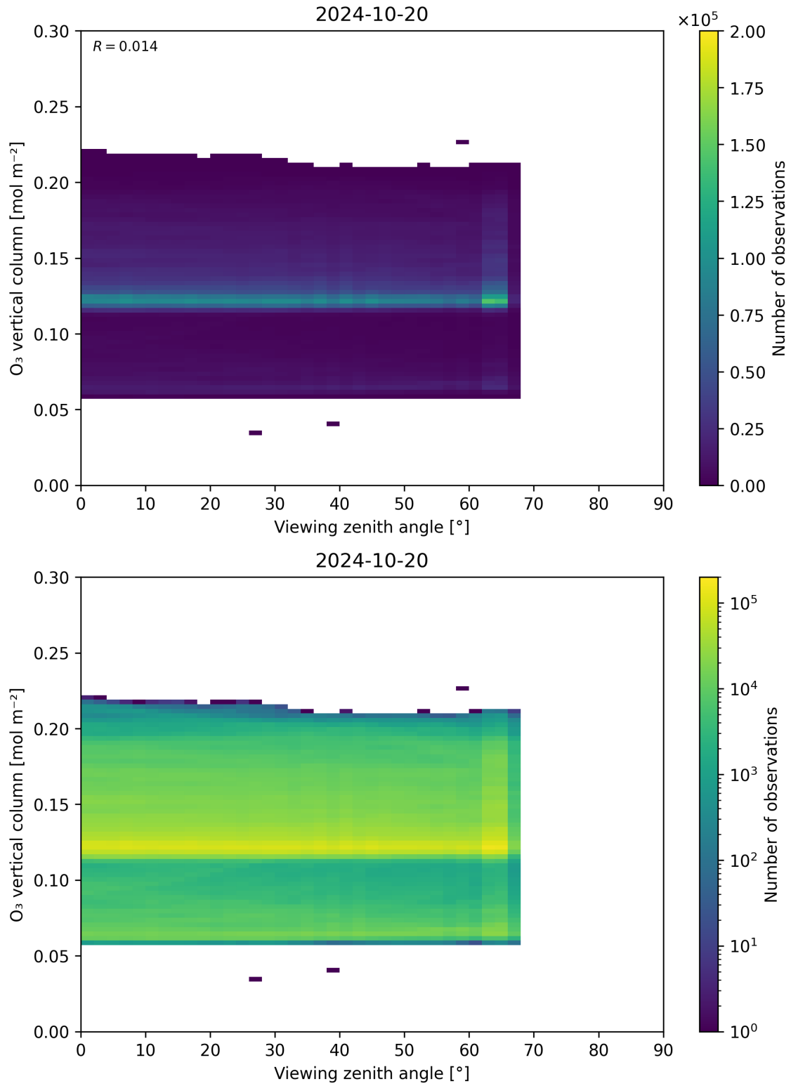
Figure 52: Scatter density plot of “Viewing zenith angle” against “O 3 vertical column” for 2024-10-19 to 2024-10-21.
