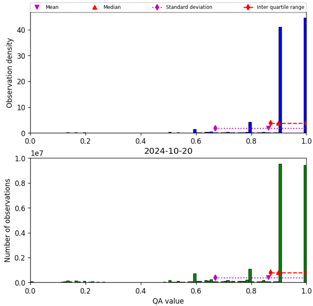
Figure 20: Histogram of “QA value” for 2024-10-19 to 2024-10-21
