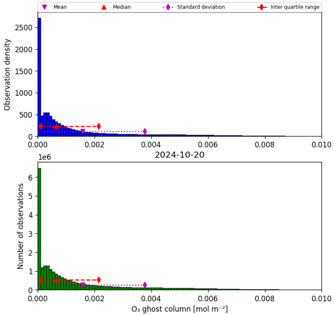
Figure 25: Histogram of “O 3 ghost column” for 2024-10-19 to 2024-10-21
