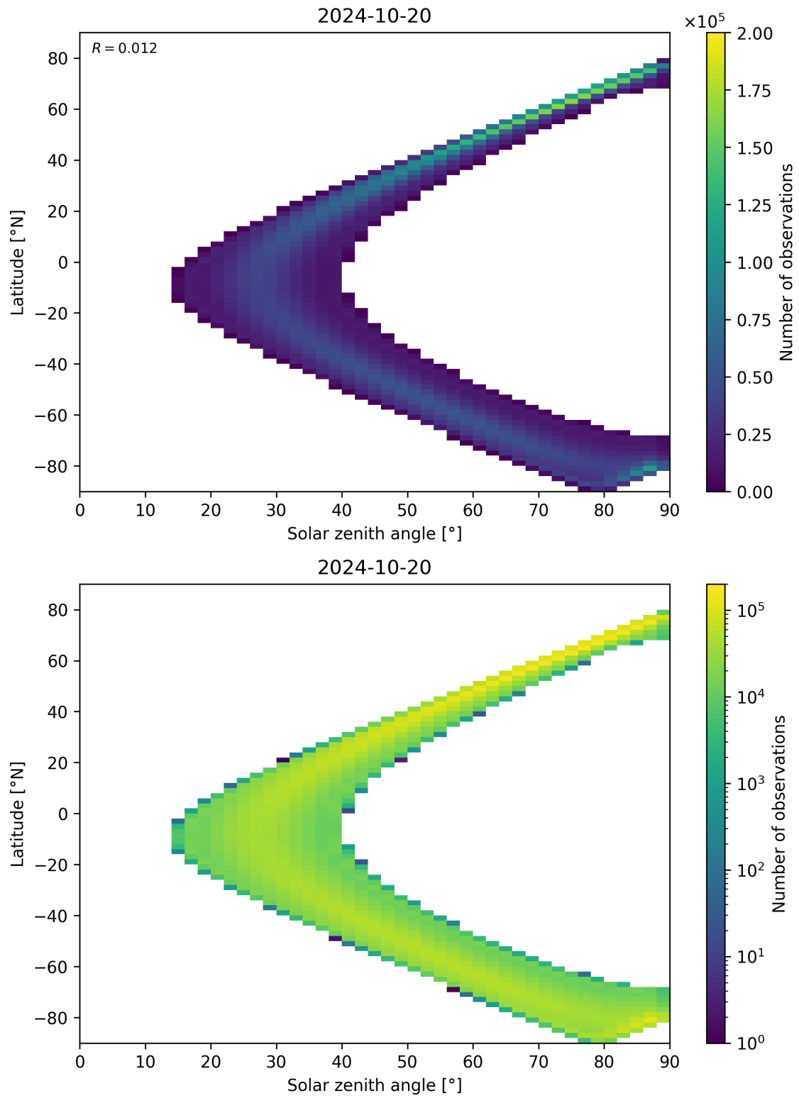
Figure 44: Scatter density plot of “Solar zenith angle” against “Latitude” for 2024-10-19 to 2024-10-21.
