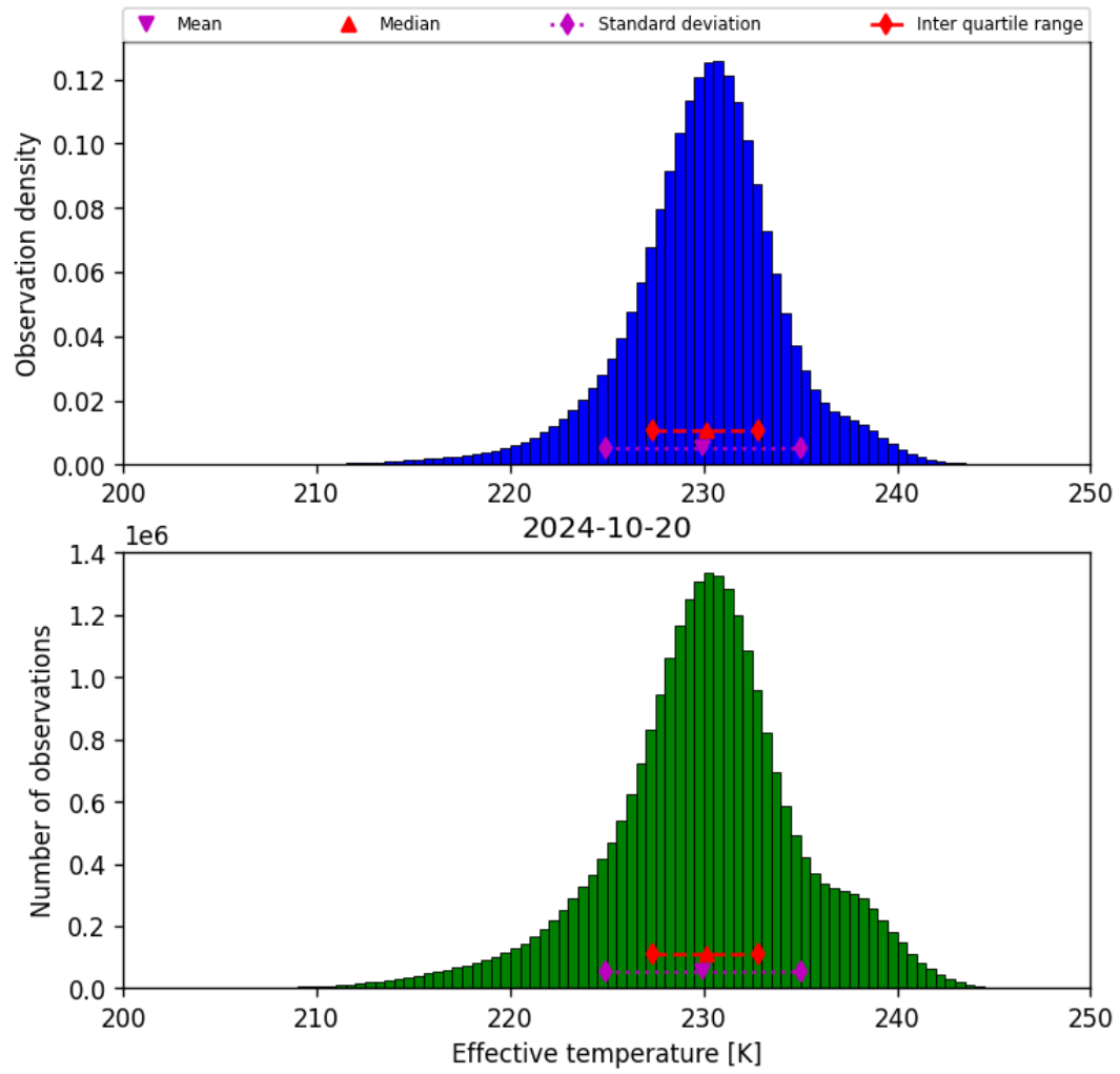
Figure 24: Histogram of “Effective temperature” for 2024-10-19 to 2024-10-21
