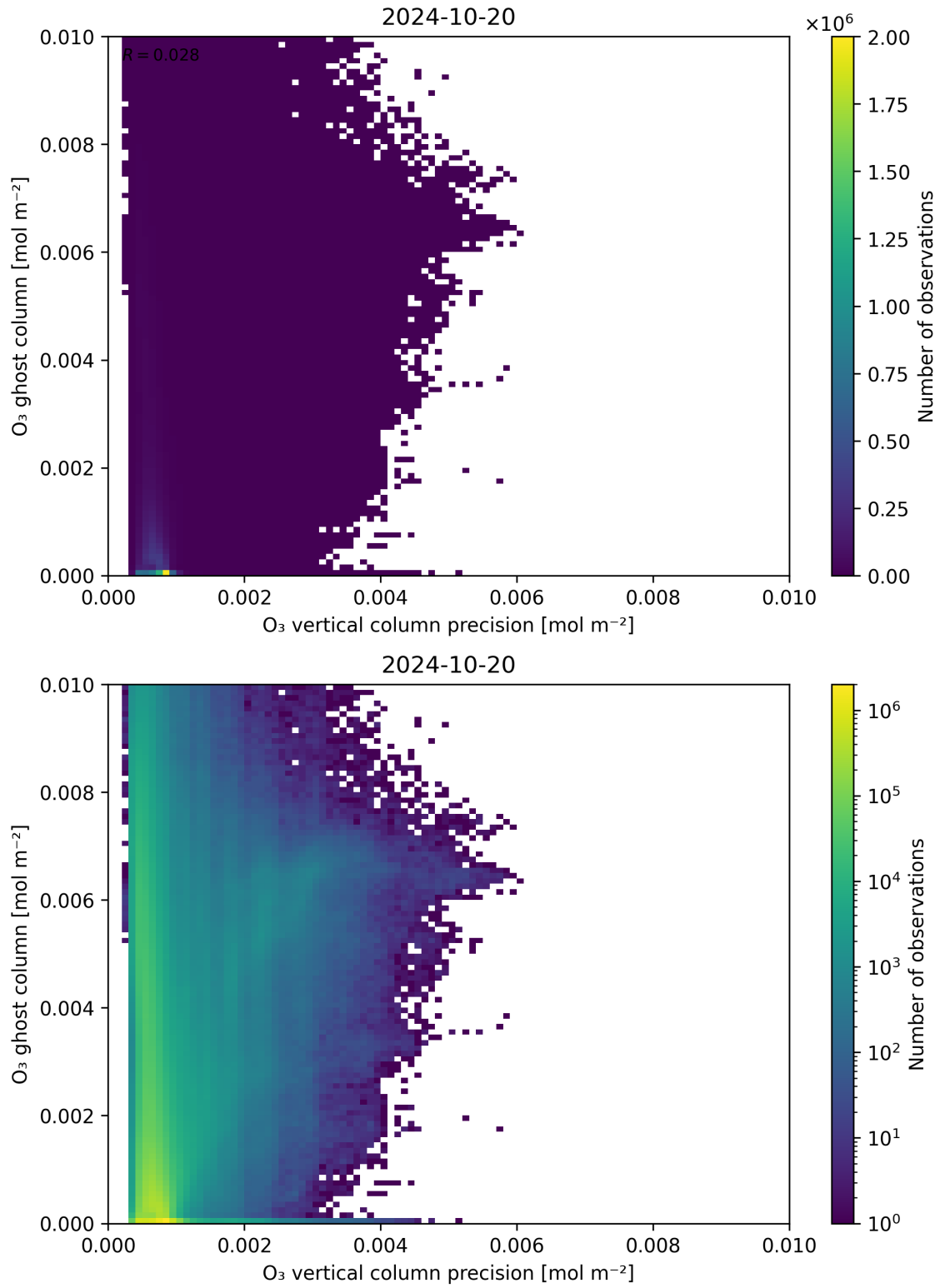
Figure 43: Scatter density plot of “O 3 vertical column precision” against “O 3 ghost column” for 2024-10-19 to 2024-10-21.
