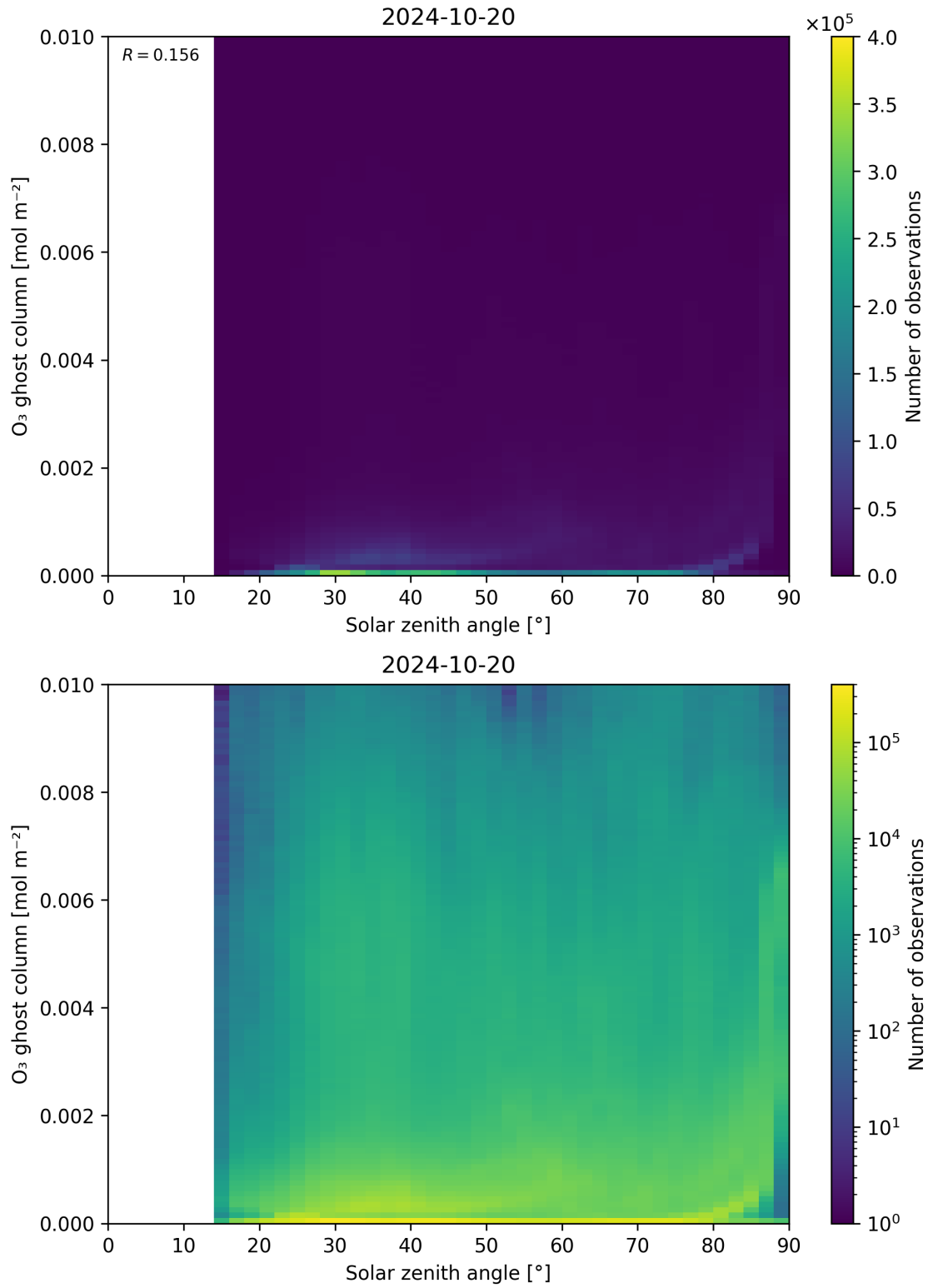
Figure 46: Scatter density plot of “Solar zenith angle” against “O 3 ghost column” for 2024-10-19 to 2024-10-21.
