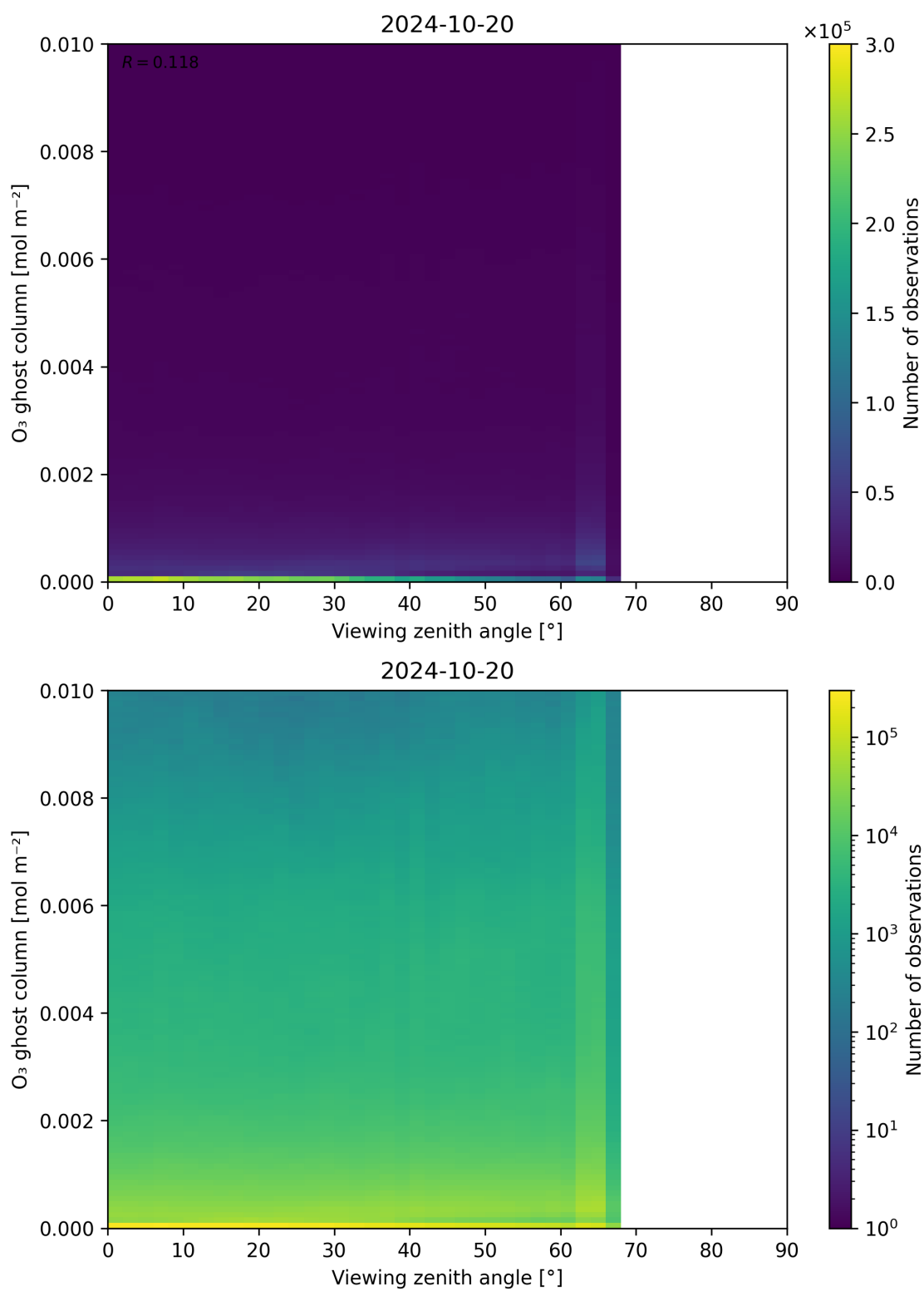
Figure 51: Scatter density plot of “Viewing zenith angle” against “O 3 ghost column” for 2024-10-19 to 2024-10-21.
