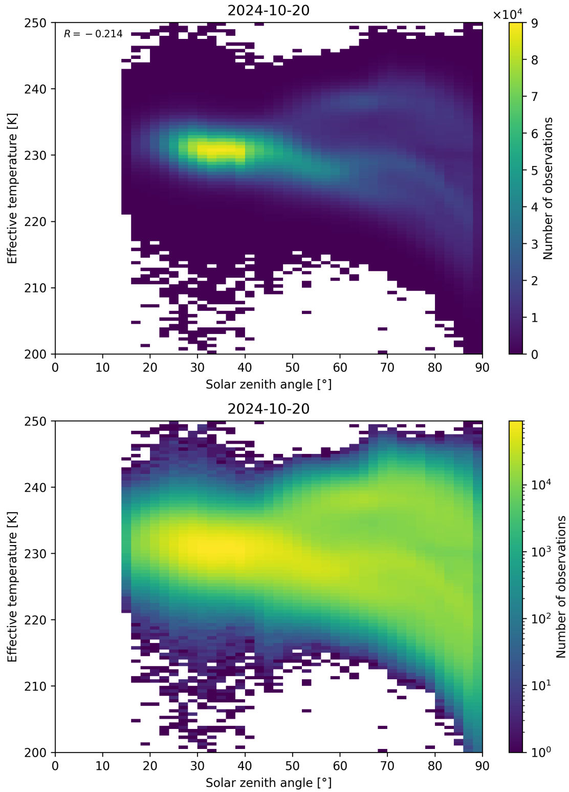
Figure 45: Scatter density plot of “Solar zenith angle” against “Effective temperature” for 2024-10-19 to 2024-10-21.
