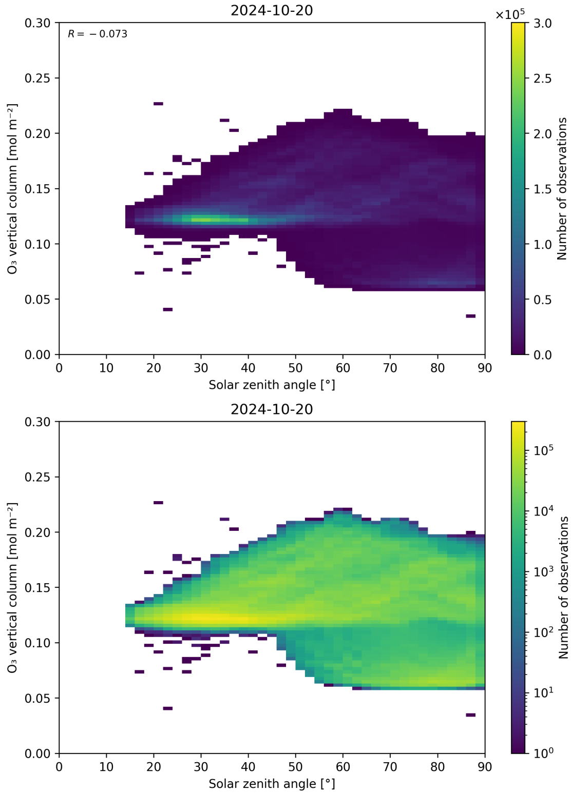
Figure 47: Scatter density plot of “Solar zenith angle” against “O 3 vertical column” for 2024-10-19 to 2024-10-21.
