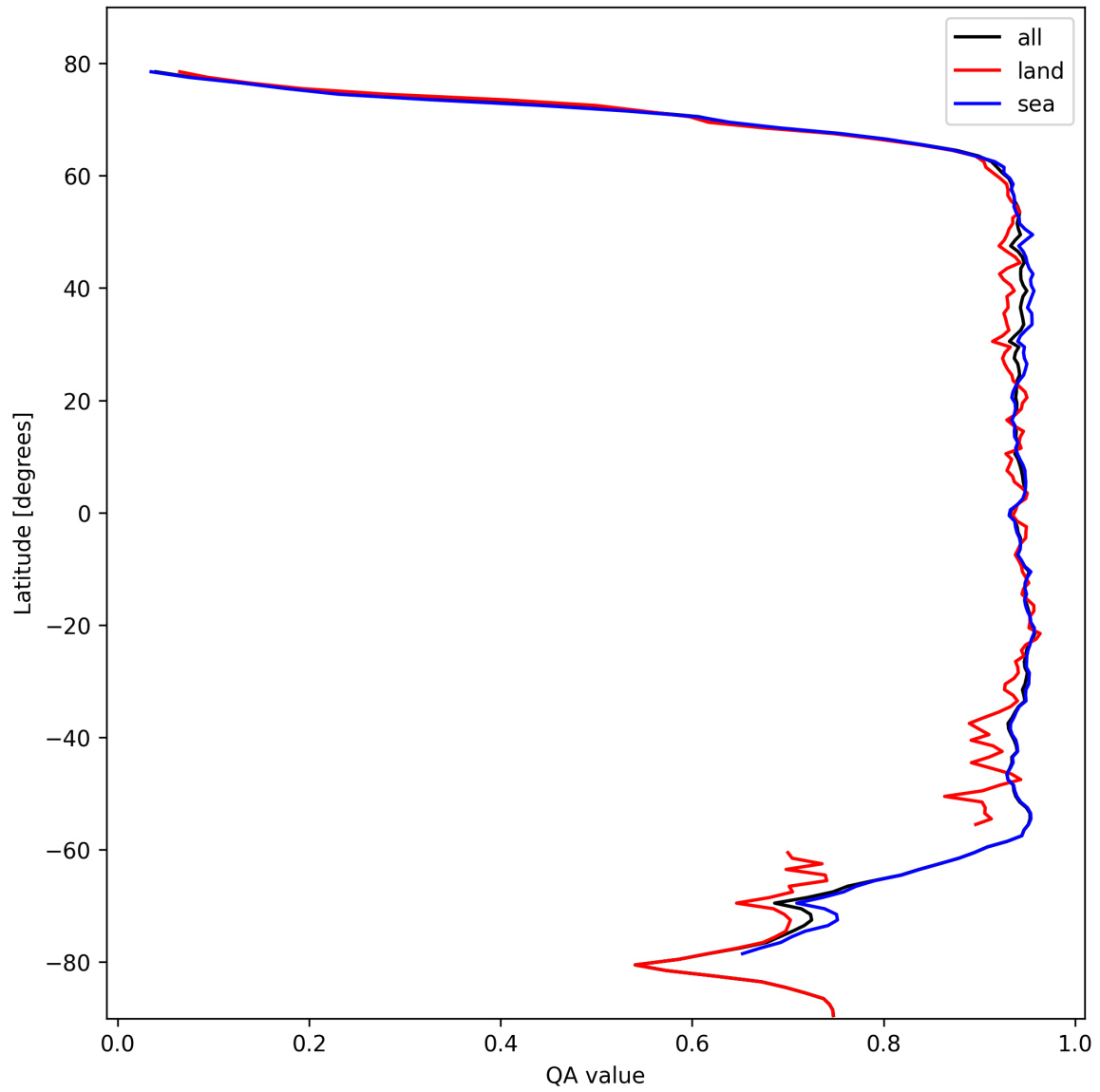
Figure 13: Zonal average of “QA value” for 2024-10-19 to 2024-10-21.
