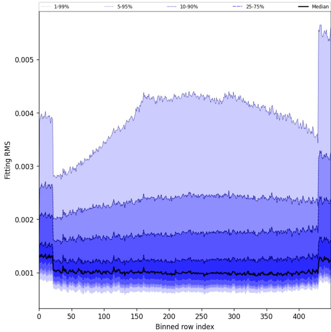
Figure 30: Along track statistics of “Fitting RMS” for 2024-10-19 to 2024-10-21
