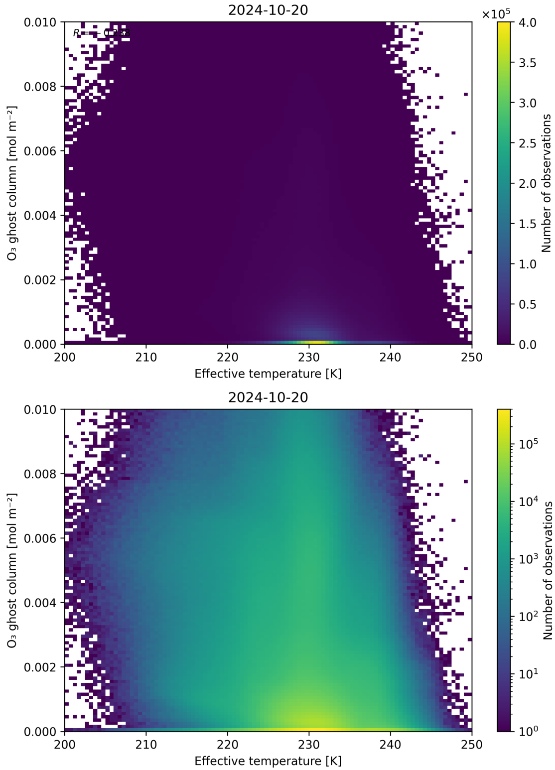
Figure 38: Scatter density plot of “Effective temperature” against “O 3 ghost column” for 2024-10-19 to 2024-10-21.
