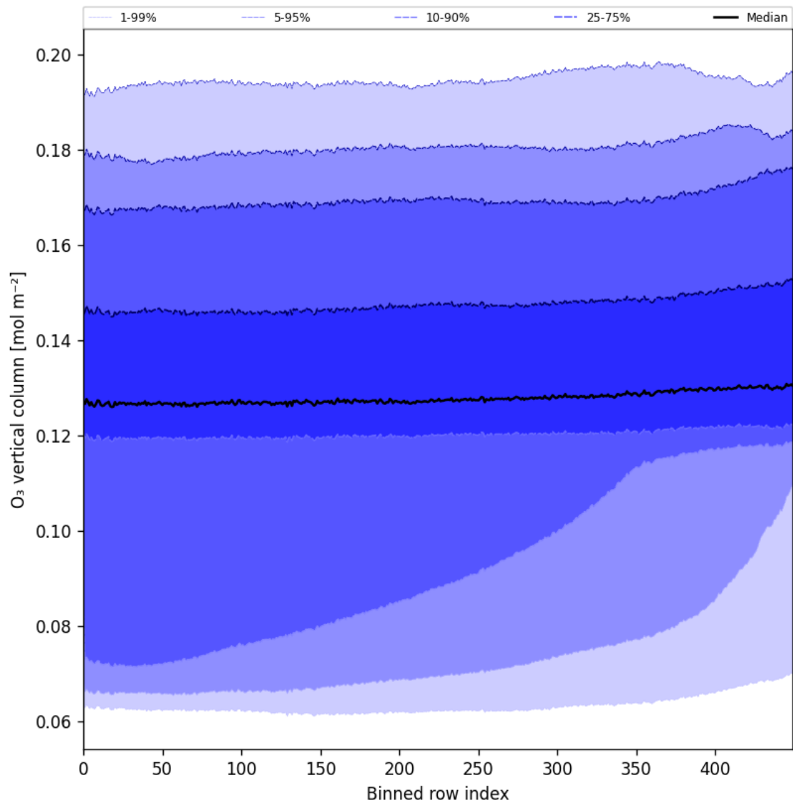
Figure 28: Along track statistics of “O 3 vertical column” for 2024-10-19 to 2024-10-21
