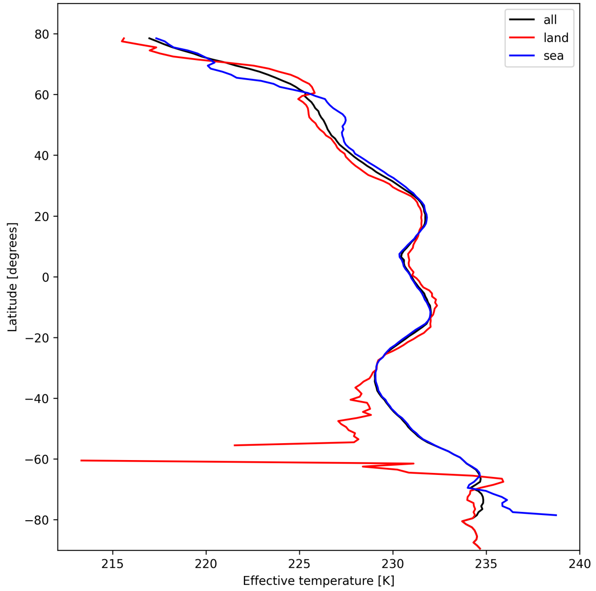
Figure 17: Zonal average of “Effective temperature” for 2024-10-19 to 2024-10-21.
