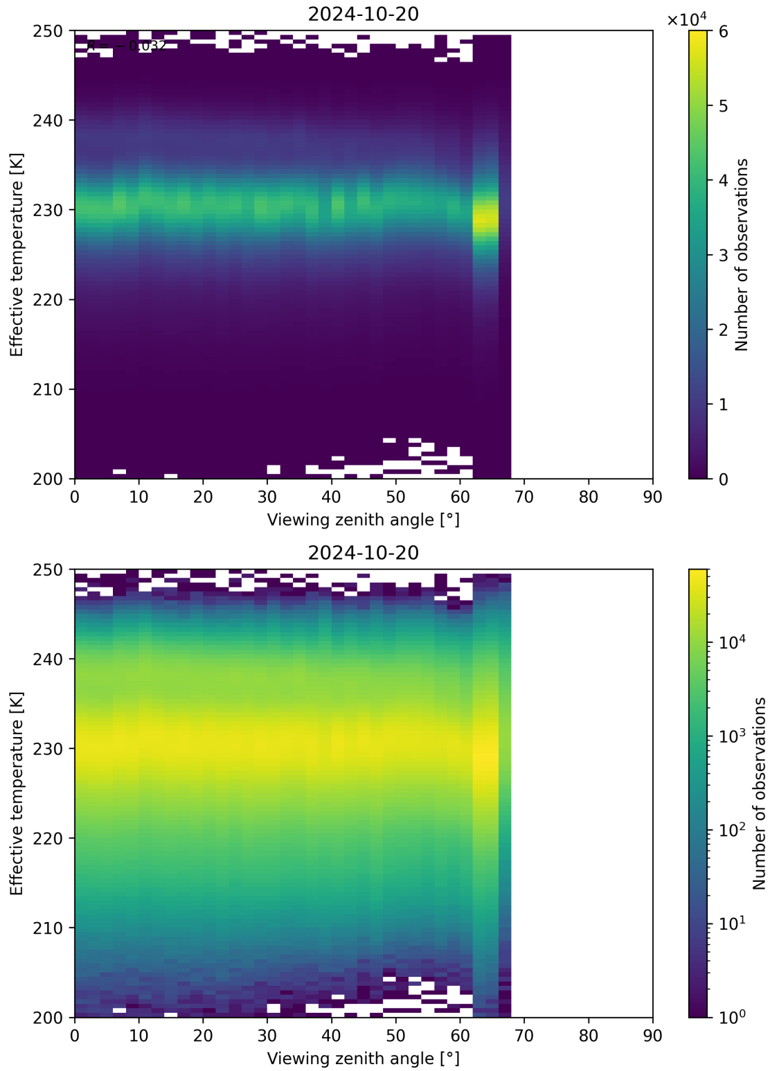
Figure 50: Scatter density plot of “Viewing zenith angle” against “Effective temperature” for 2024-10-19 to 2024-10-21.
