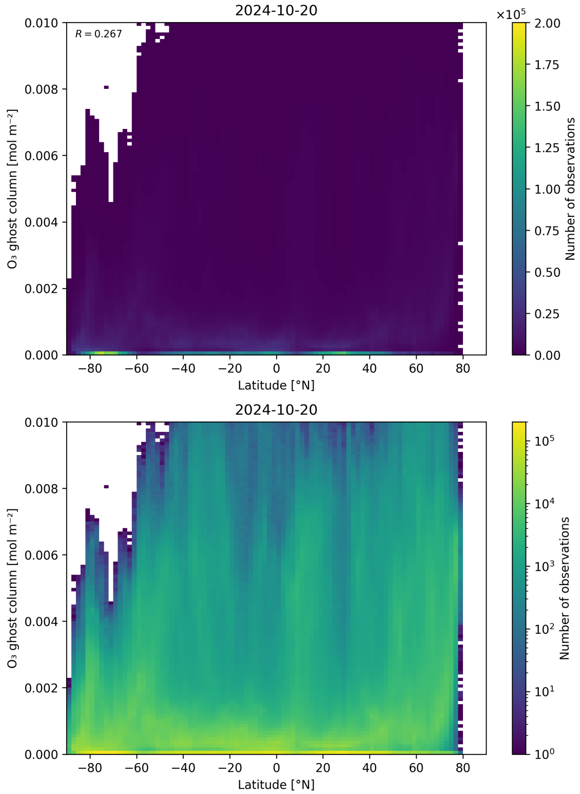
Figure 35: Scatter density plot of “Latitude” against “O 3 ghost column” for 2024-10-19 to 2024-10-21.
