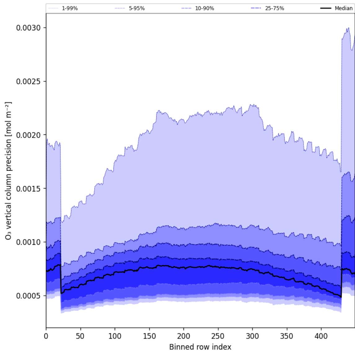
Figure 29: Along track statistics of “O 3 vertical column precision” for 2024-10-19 to 2024-10-21
