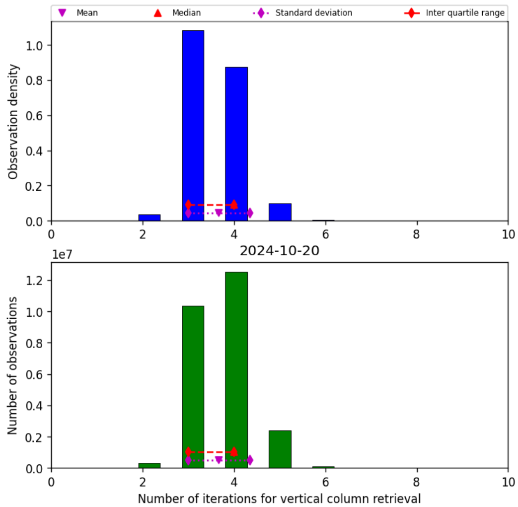
Figure 26: Histogram of “Number of iterations for vertical column retrieval” for 2024-10-19 to 2024-10-21
