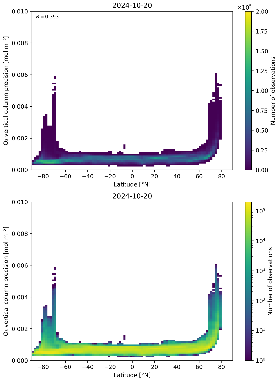
Figure 37: Scatter density plot of “Latitude” against “O 3 vertical column precision” for 2024-10-19 to 2024-10-21.
