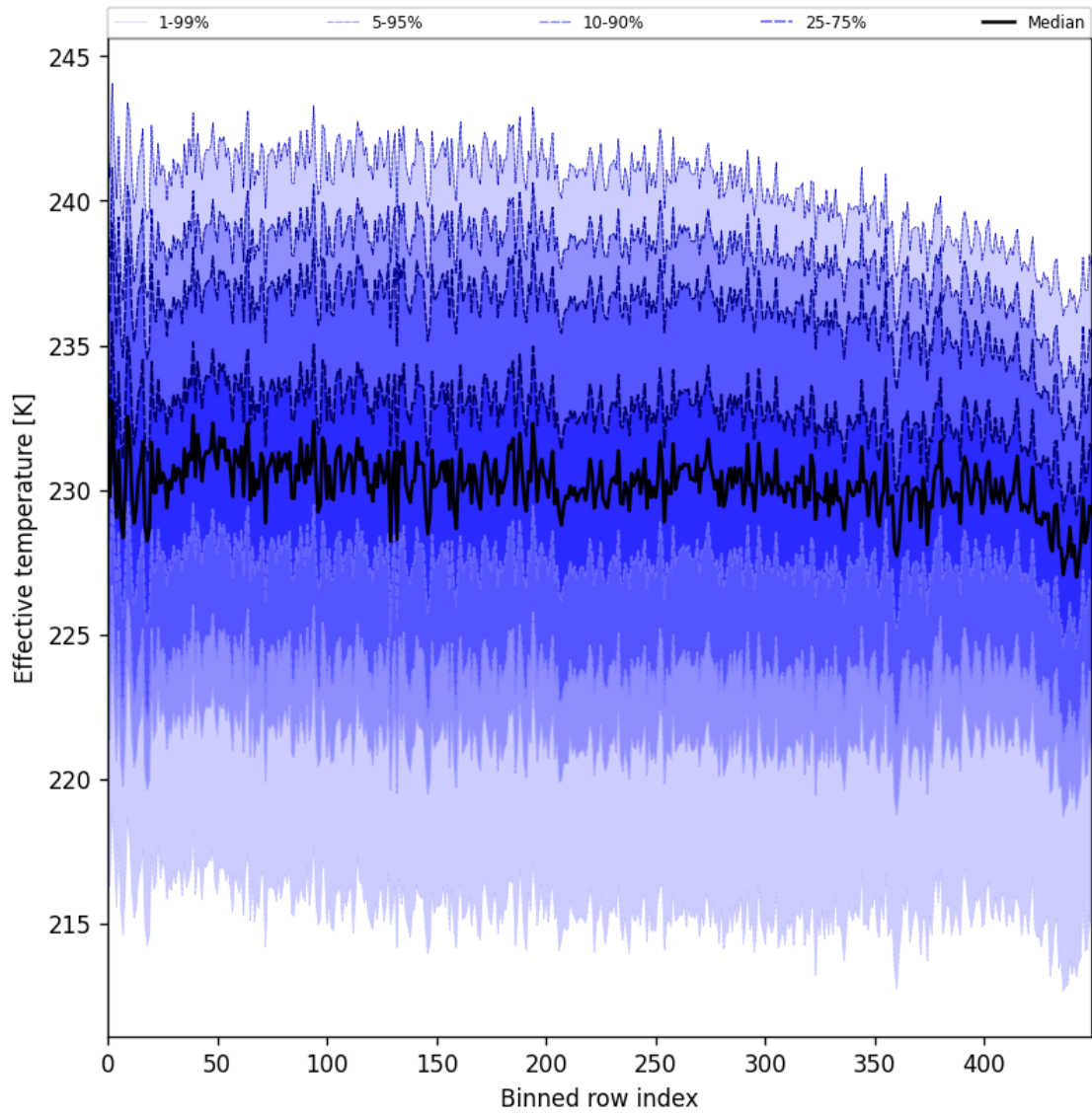
Figure 31: Along track statistics of “Effective temperature” for 2024-10-19 to 2024-10-21
