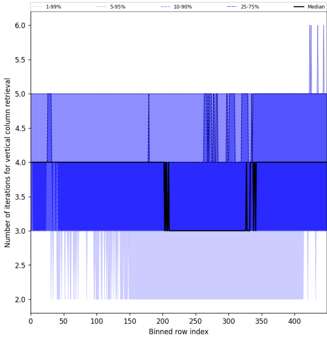
Figure 33: Along track statistics of “Number of iterations for vertical column retrieval” for 2024-10-19 to 2024-10-21
