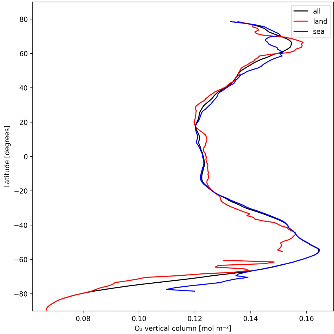
Figure 14: Zonal average of “O 3 vertical column” for 2024-10-19 to 2024-10-21.
