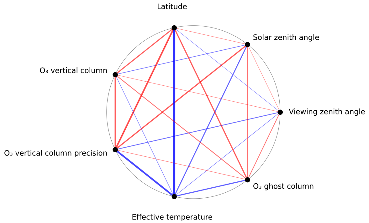
Figure 1: Map of correlation graph for 2024-10-19 to 2024-10-21.
