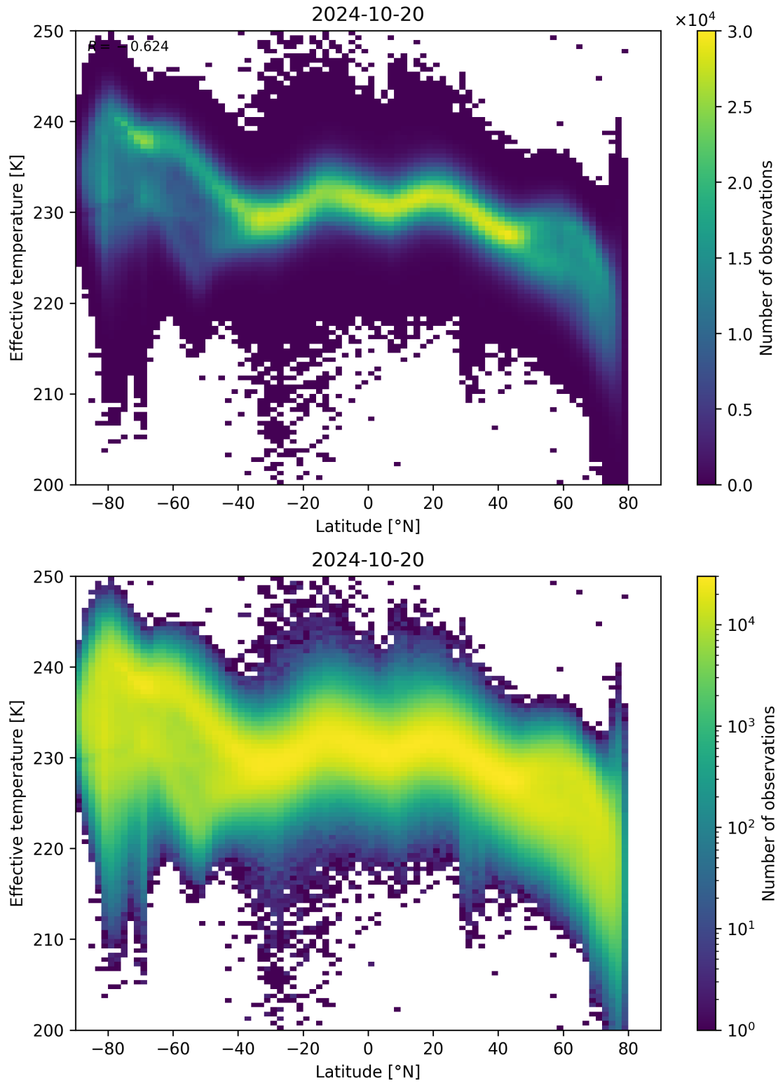
Figure 34: Scatter density plot of “Latitude” against “Effective temperature” for 2024-10-19 to 2024-10-21.
