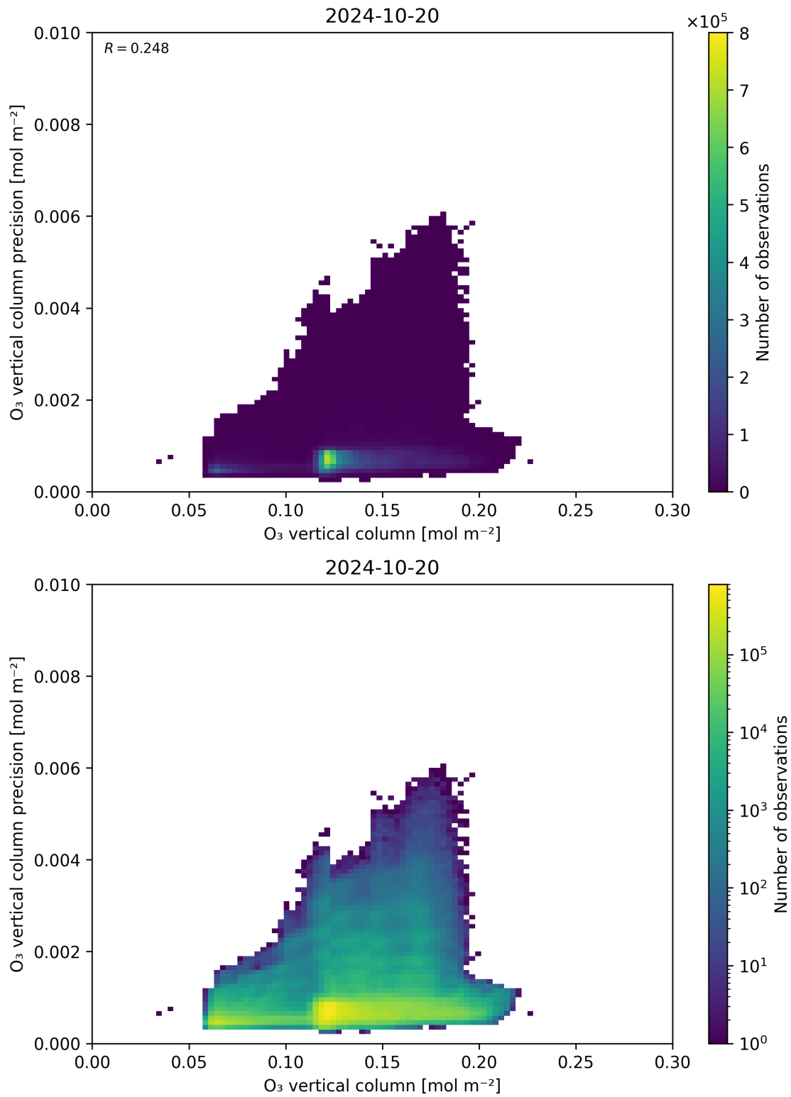
Figure 41: Scatter density plot of “O 3 vertical column” against “O 3 vertical column precision” for 2024-10-19 to 2024-10-21.
