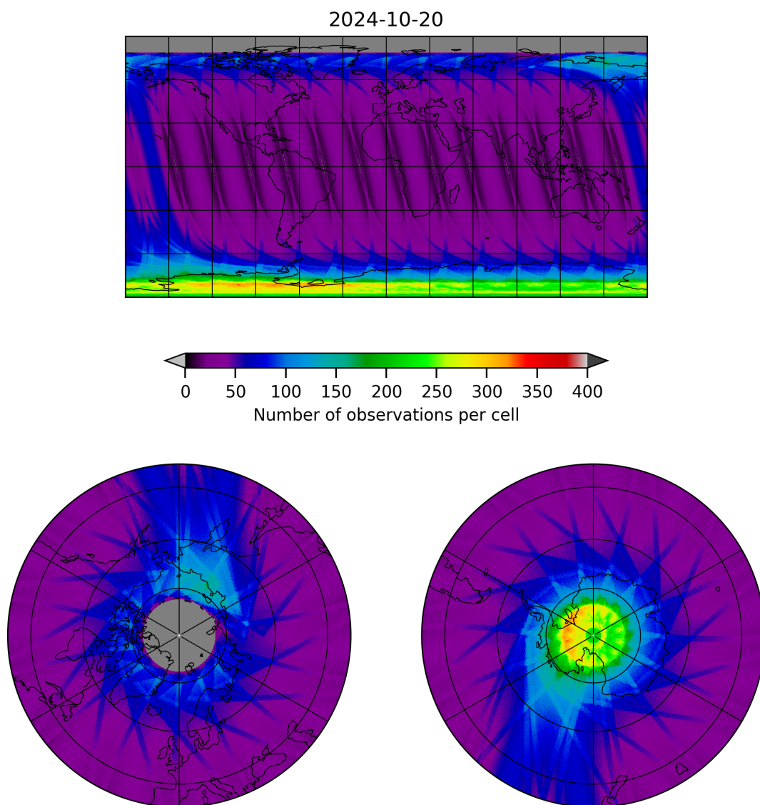
Figure 12: Map of the number of observations for 2024-10-19 to 2024-10-21
