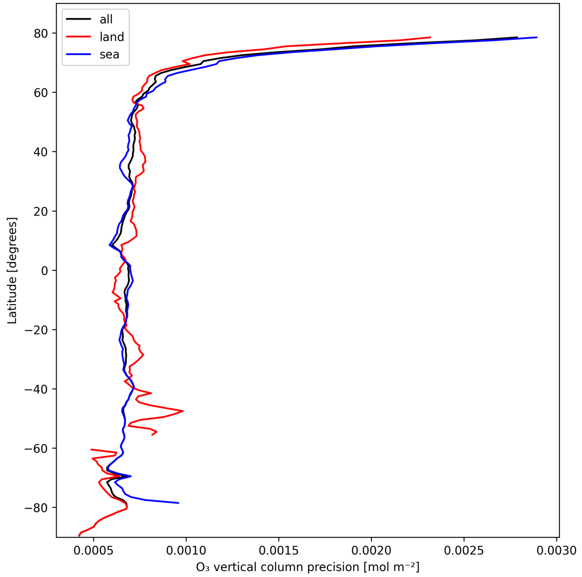
Figure 15: Zonal average of “O 3 vertical column precision” for 2024-10-19 to 2024-10-21.
