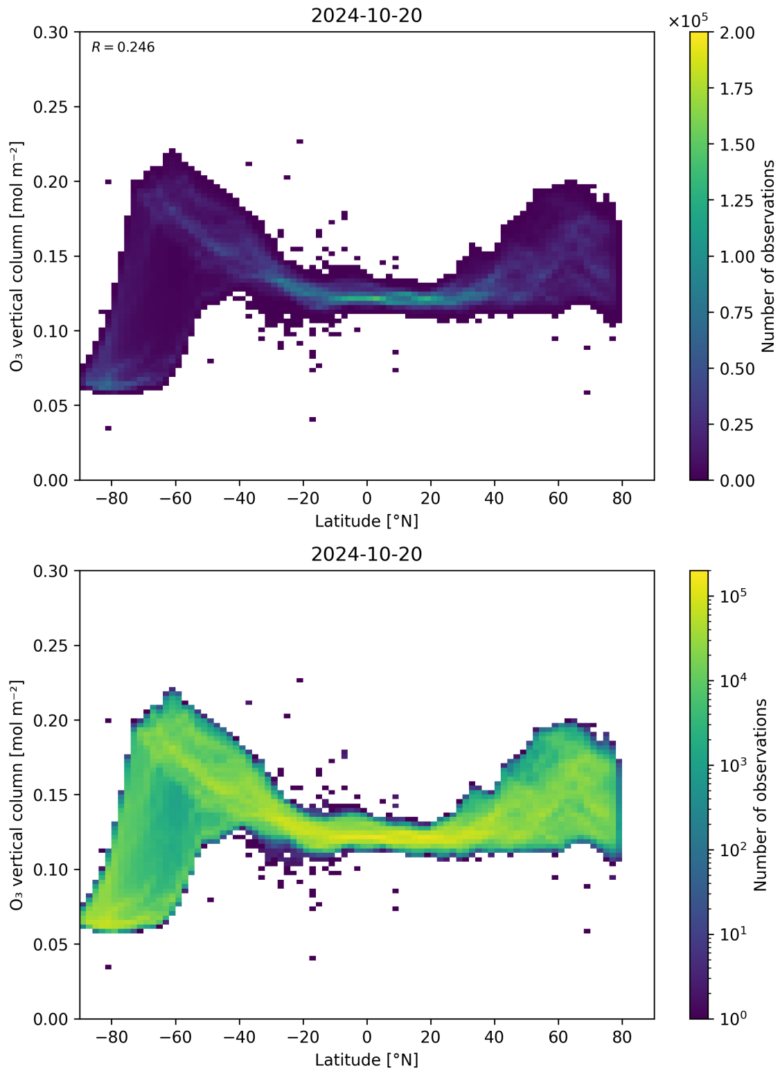
Figure 36: Scatter density plot of “Latitude” against “O 3 vertical column” for 2024-10-19 to 2024-10-21.
