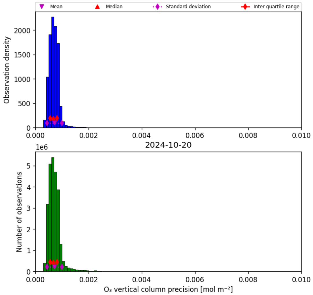
Figure 22: Histogram of “O 3 vertical column precision” for 2024-10-19 to 2024-10-21
