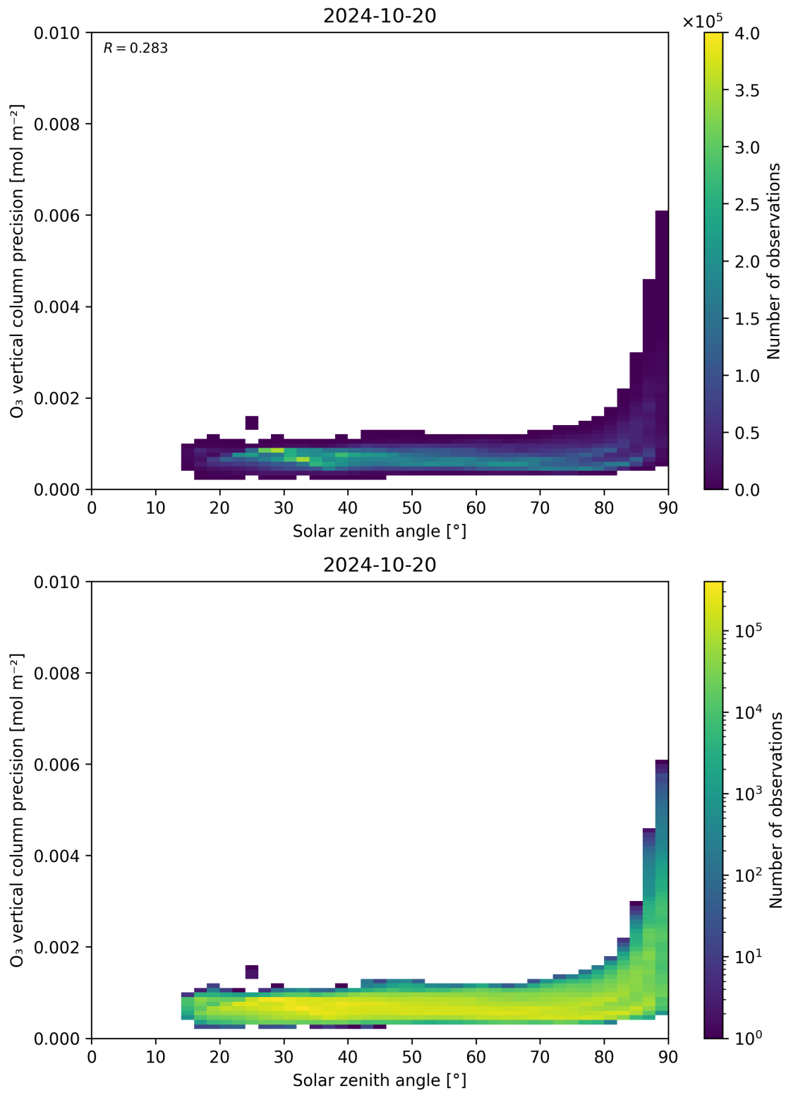
Figure 48: Scatter density plot of “Solar zenith angle” against “O 3 vertical column precision” for 2024-10-19 to 2024-10-21.
