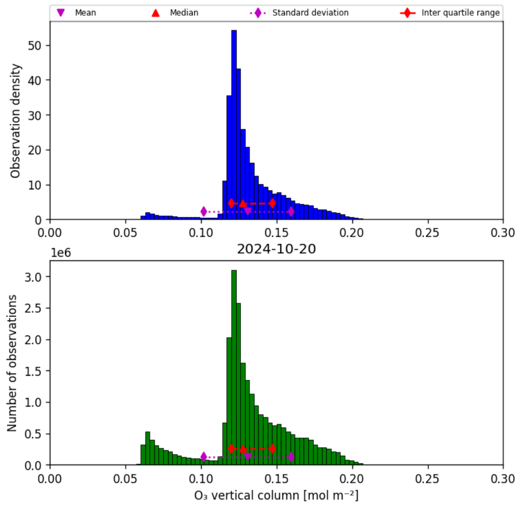
Figure 21: Histogram of “O 3 vertical column” for 2024-10-19 to 2024-10-21
