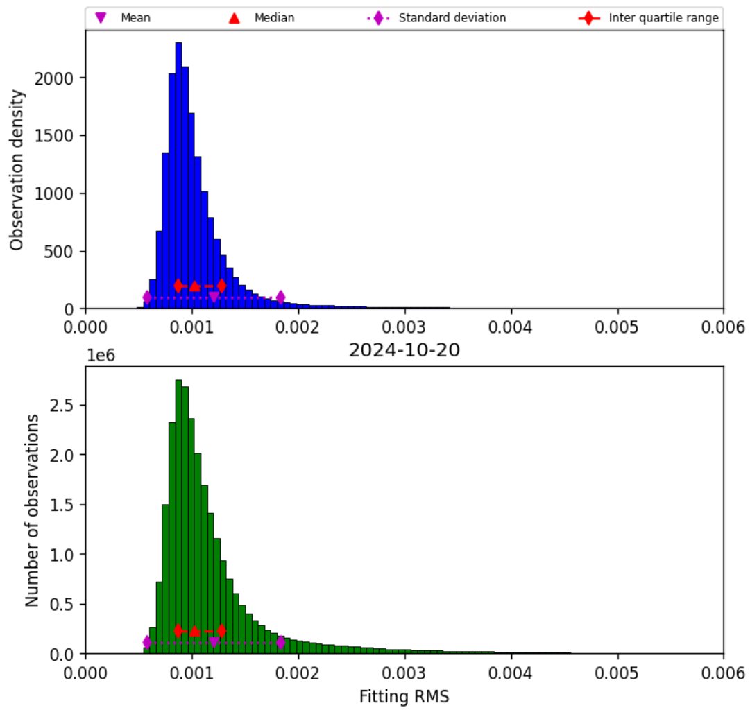
Figure 23: Histogram of “Fitting RMS” for 2024-10-19 to 2024-10-21
