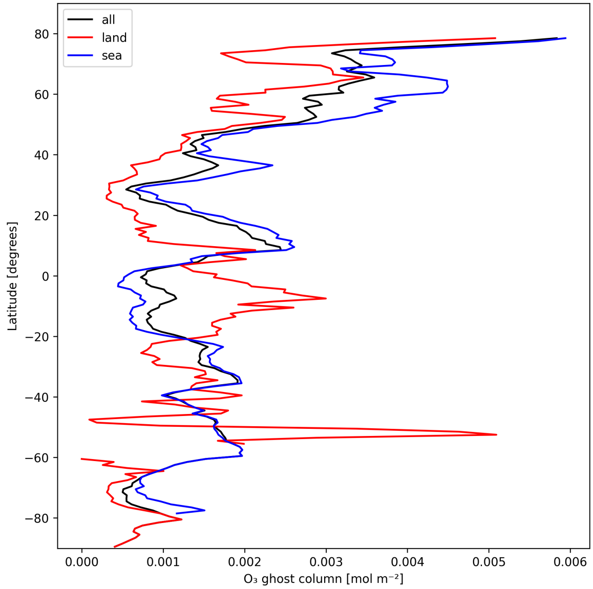
Figure 18: Zonal average of “O 3 ghost column” for 2024-10-19 to 2024-10-21.
