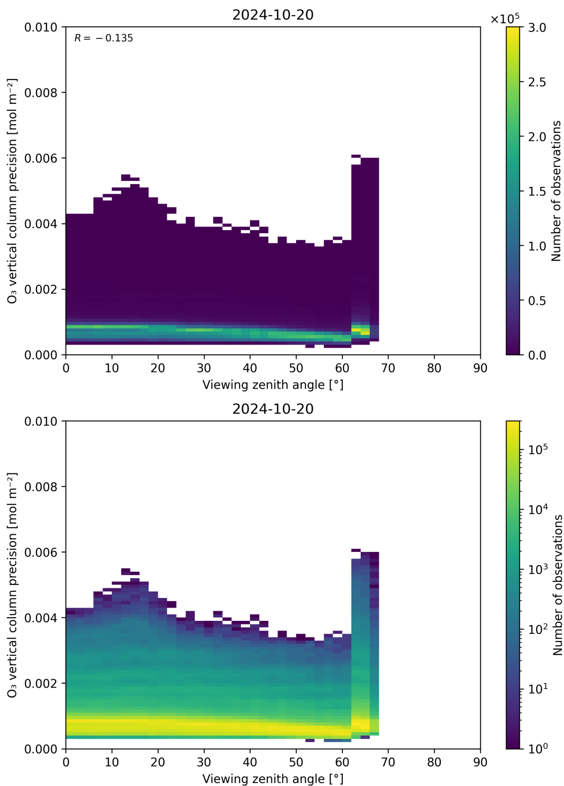
Figure 53: Scatter density plot of “Viewing zenith angle” against “O 3 vertical column precision” for 2024-10-19 to 2024-10-21.
