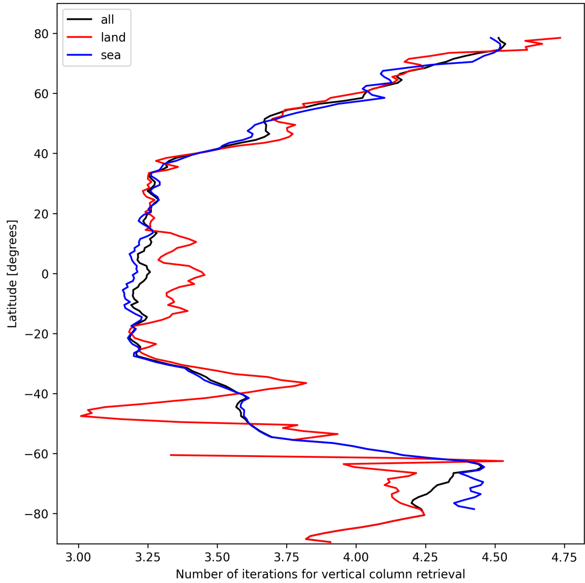
Figure 19: Zonal average of “Number of iterations for vertical column retrieval” for 2024-10-19 to 2024-10-21.
