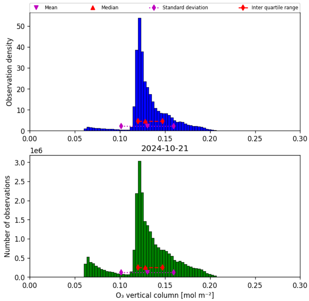
Figure 21: Histogram of “O 3 vertical column” for 2024-10-20 to 2024-10-22
