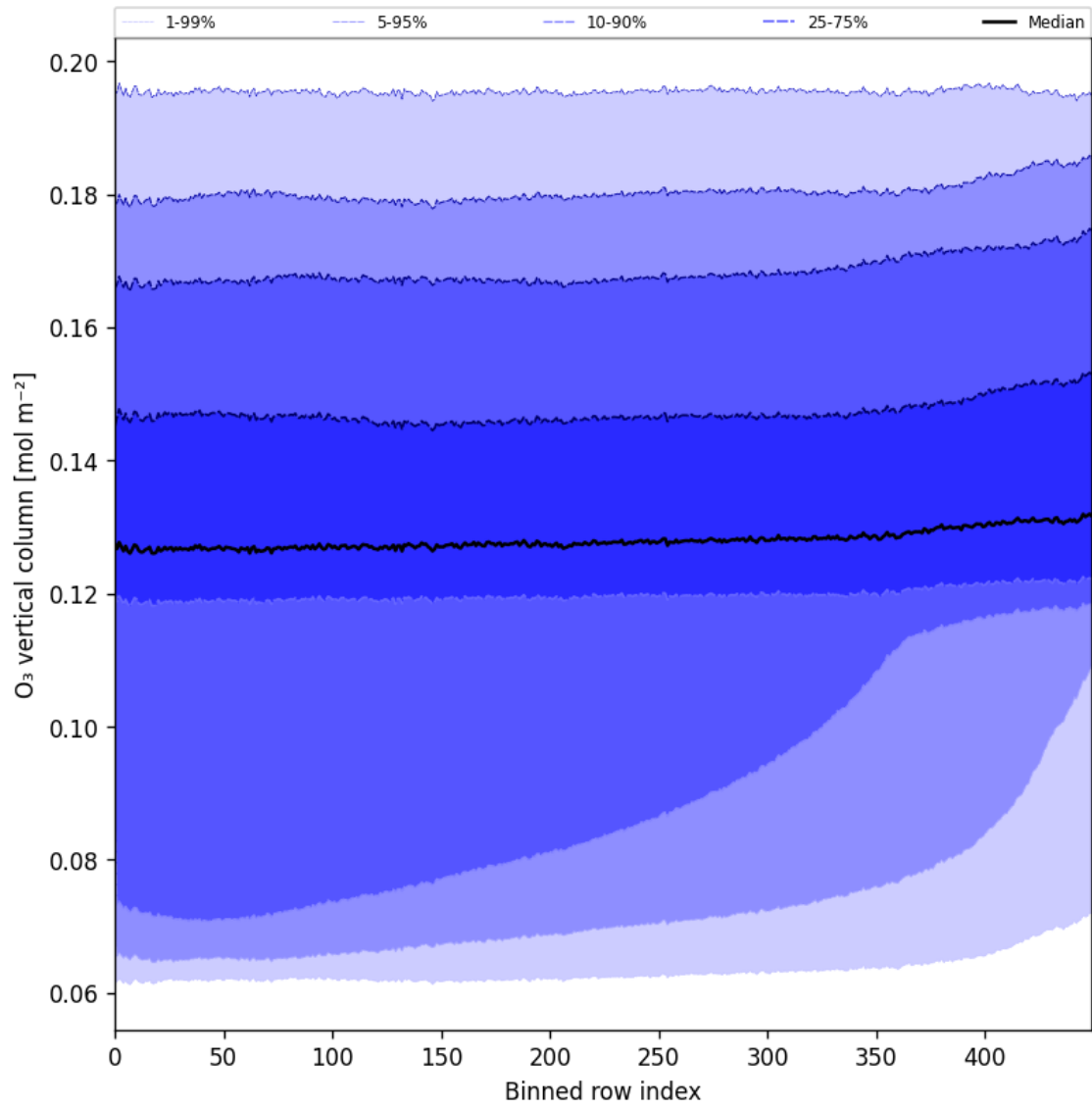
Figure 28: Along track statistics of "O 3 vertical column" for 2024-10-20 to 2024-10-22
