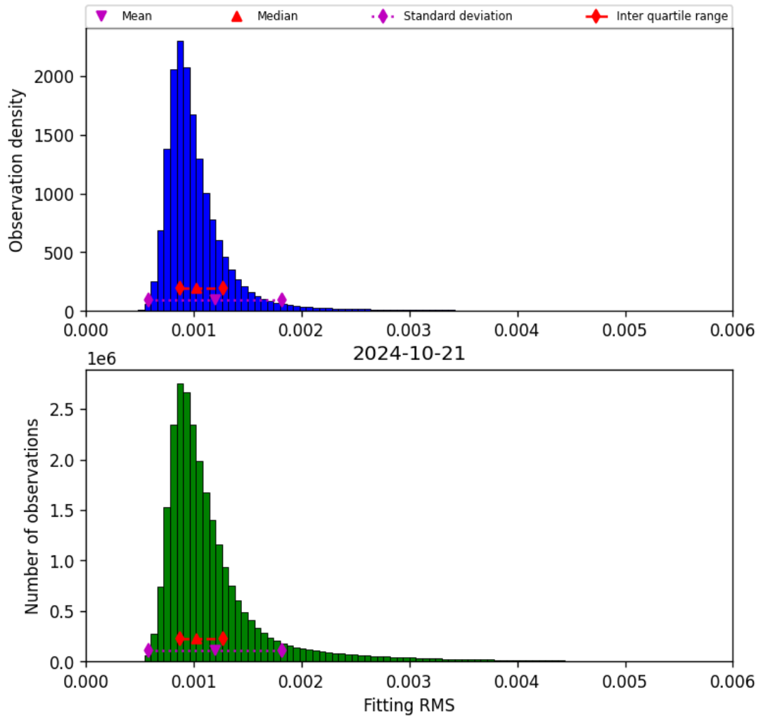
Figure 23: Histogram of “Fitting RMS” for 2024-10-20 to 2024-10-22
