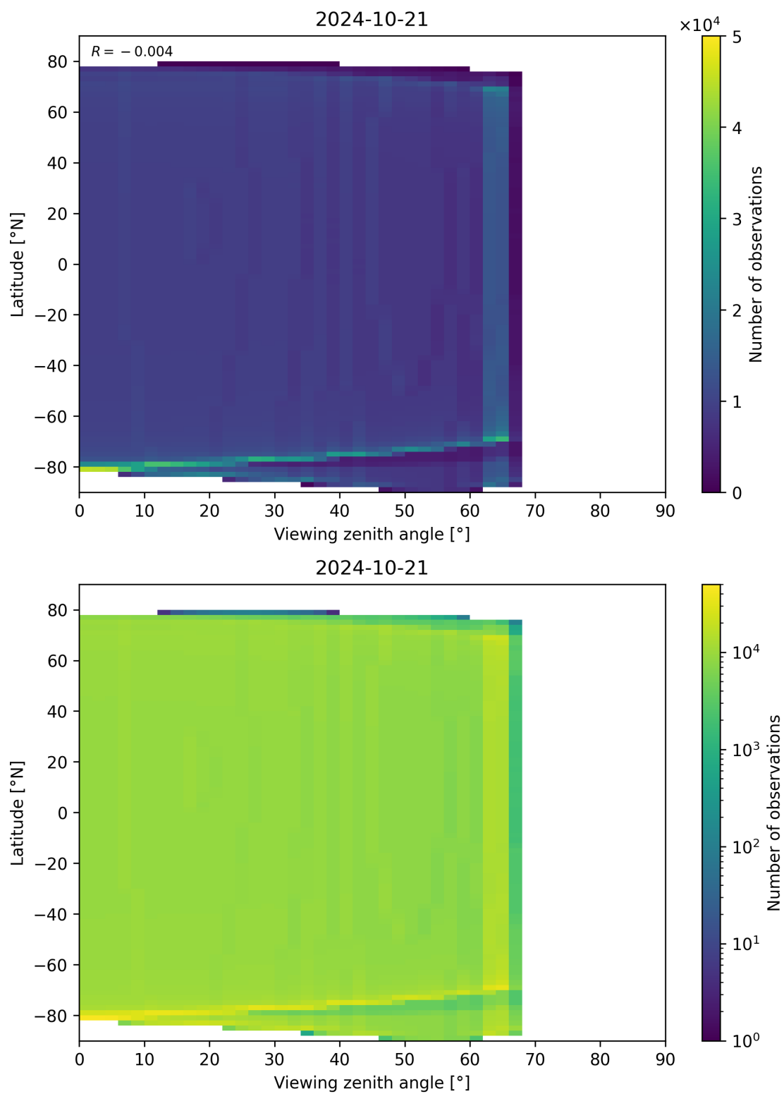
Figure 49: Scatter density plot of “Viewing zenith angle” against “Latitude” for 2024-10-20 to 2024-10-22.
