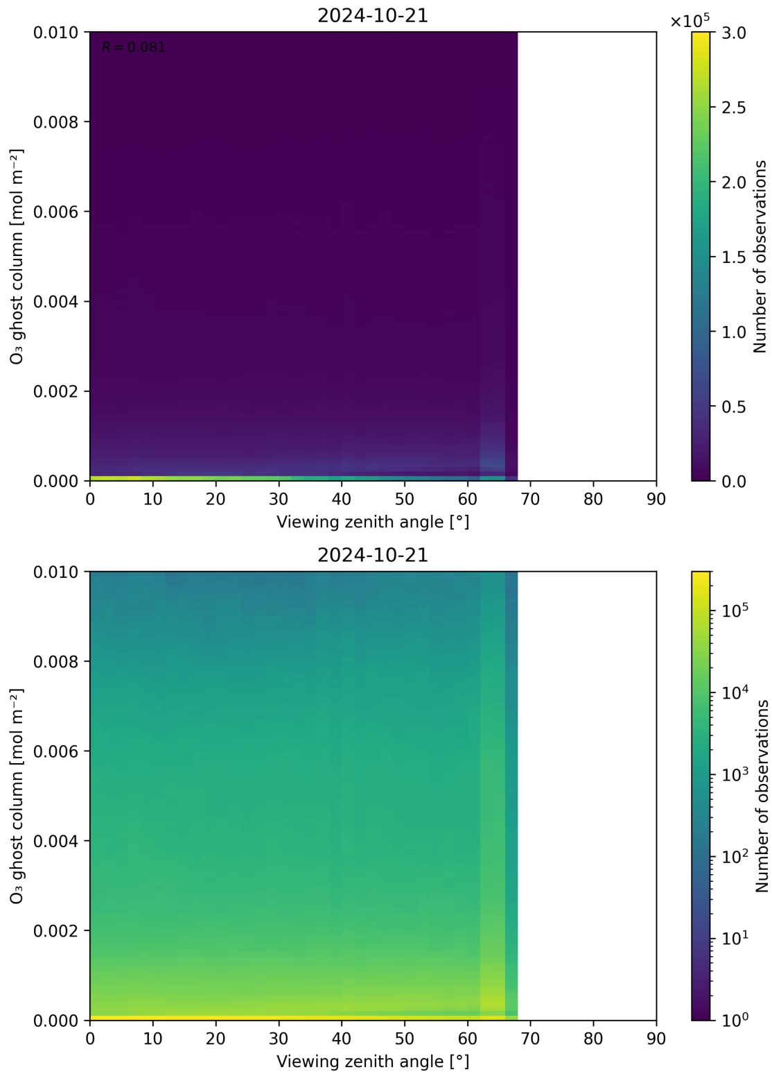
Figure 51: Scatter density plot of “Viewing zenith angle” against “O 3 ghost column” for 2024-10-20 to 2024-10-22.
