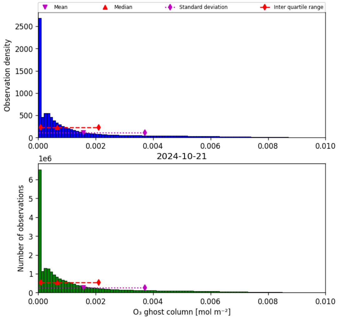
Figure 25: Histogram of “O 3 ghost column” for 2024-10-20 to 2024-10-22
