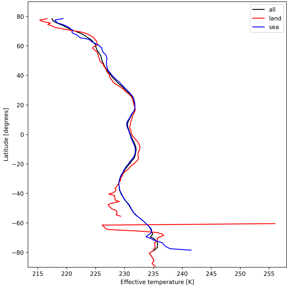
Figure 17: Zonal average of “Effective temperature” for 2024-10-20 to 2024-10-22.
