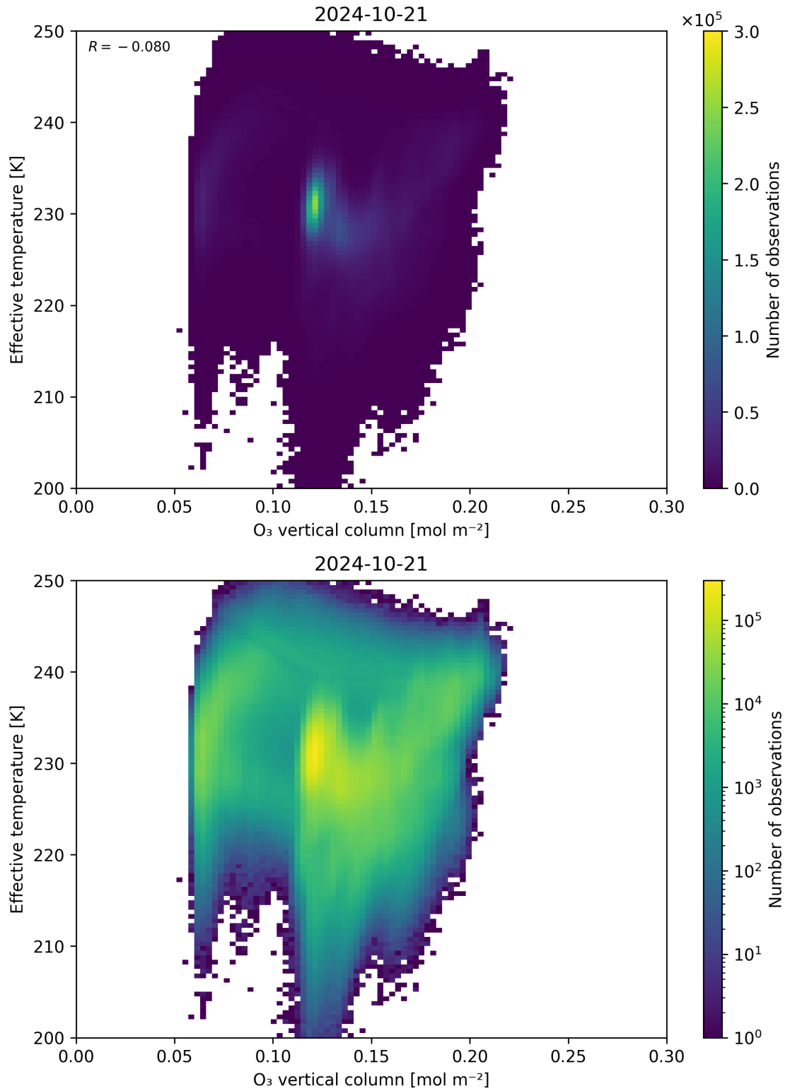
Figure 39: Scatter density plot of “O 3 vertical column” against “Effective temperature” for 2024-10-20 to 2024-10-22.
