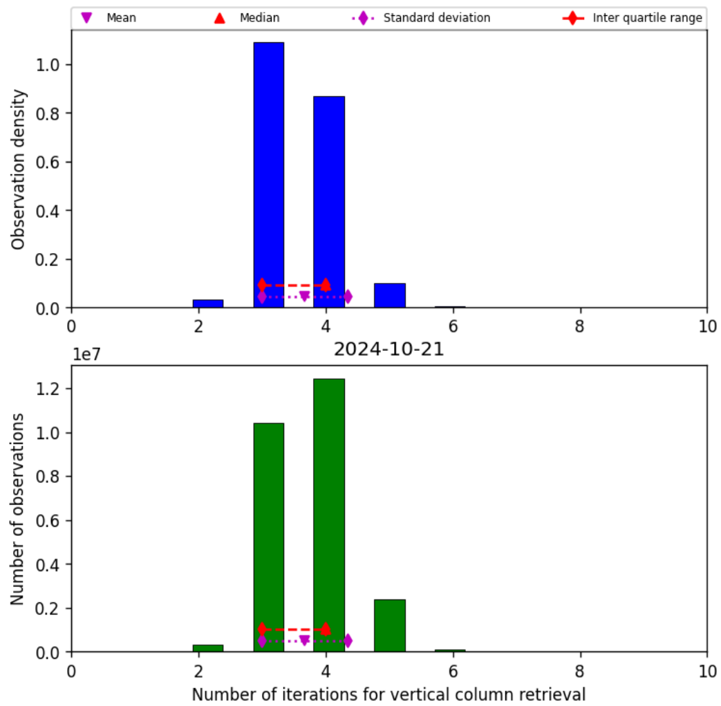
Figure 26: Histogram of “Number of iterations for vertical column retrieval” for 2024-10-20 to 2024-10-22
