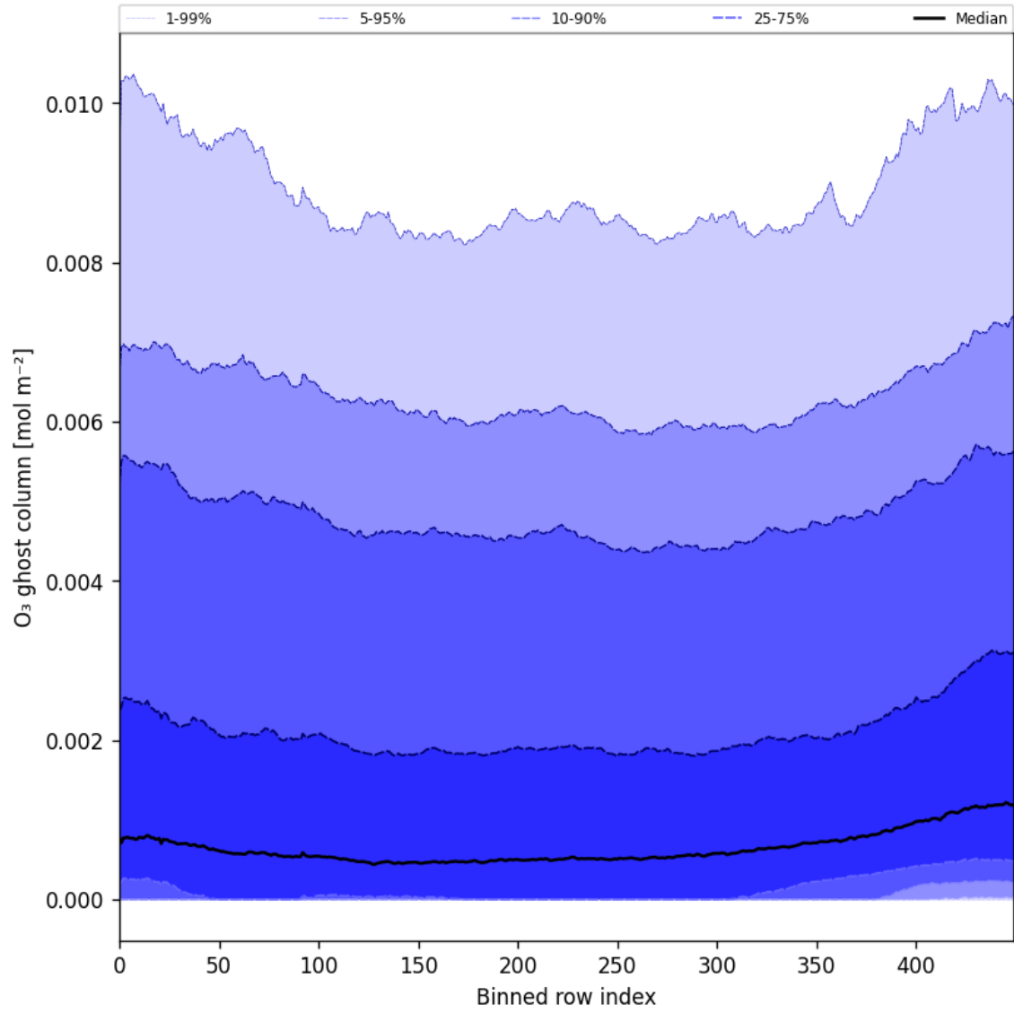
Figure 32: Along track statistics of “O 3 ghost column” for 2024-10-20 to 2024-10-22
