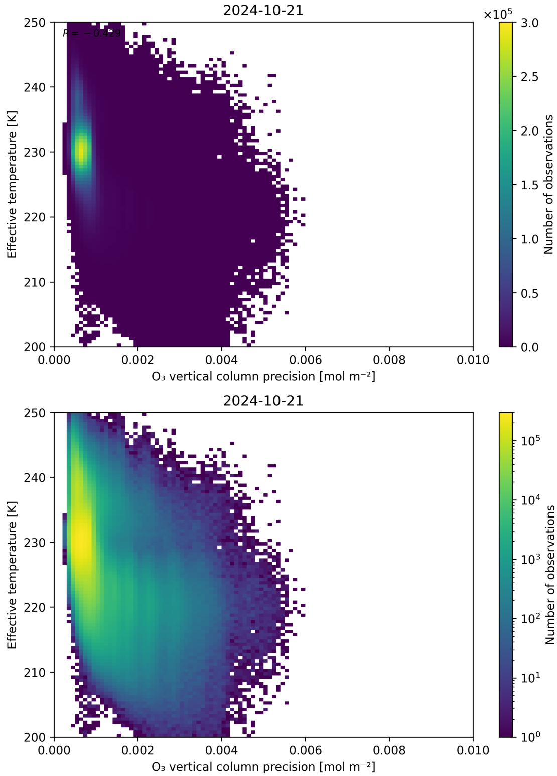
Figure 42: Scatter density plot of “O 3 vertical column precision” against “Effective temperature” for 2024-10-20 to 2024-10-22.
