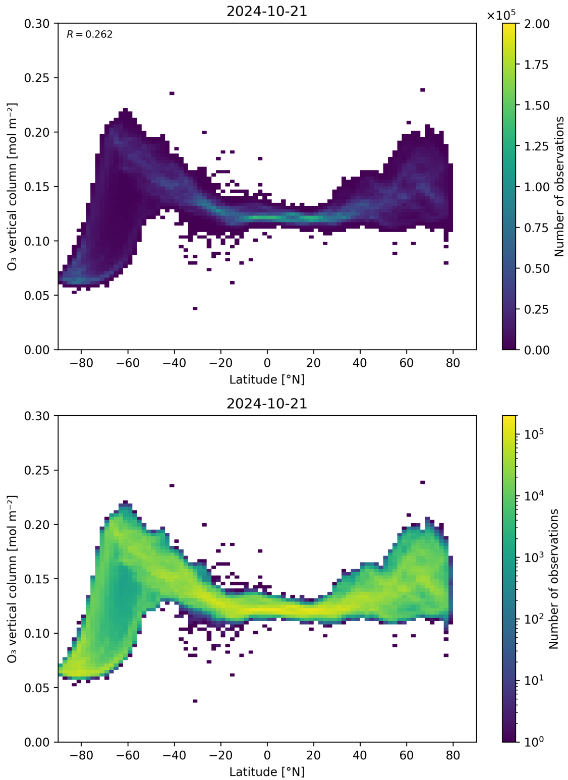
Figure 36: Scatter density plot of “Latitude” against “O 3 vertical column” for 2024-10-20 to 2024-10-22.
