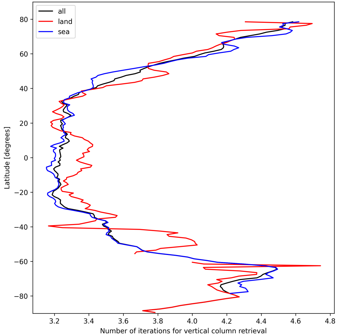
Figure 19: Zonal average of “Number of iterations for vertical column retrieval” for 2024-10-20 to 2024-10-22.
