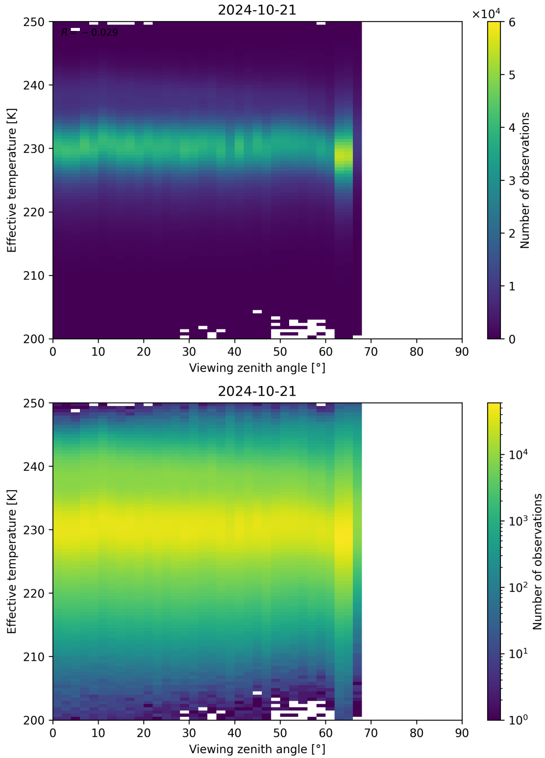
Figure 50: Scatter density plot of “Viewing zenith angle” against “Effective temperature” for 2024-10-20 to 2024-10-22.
