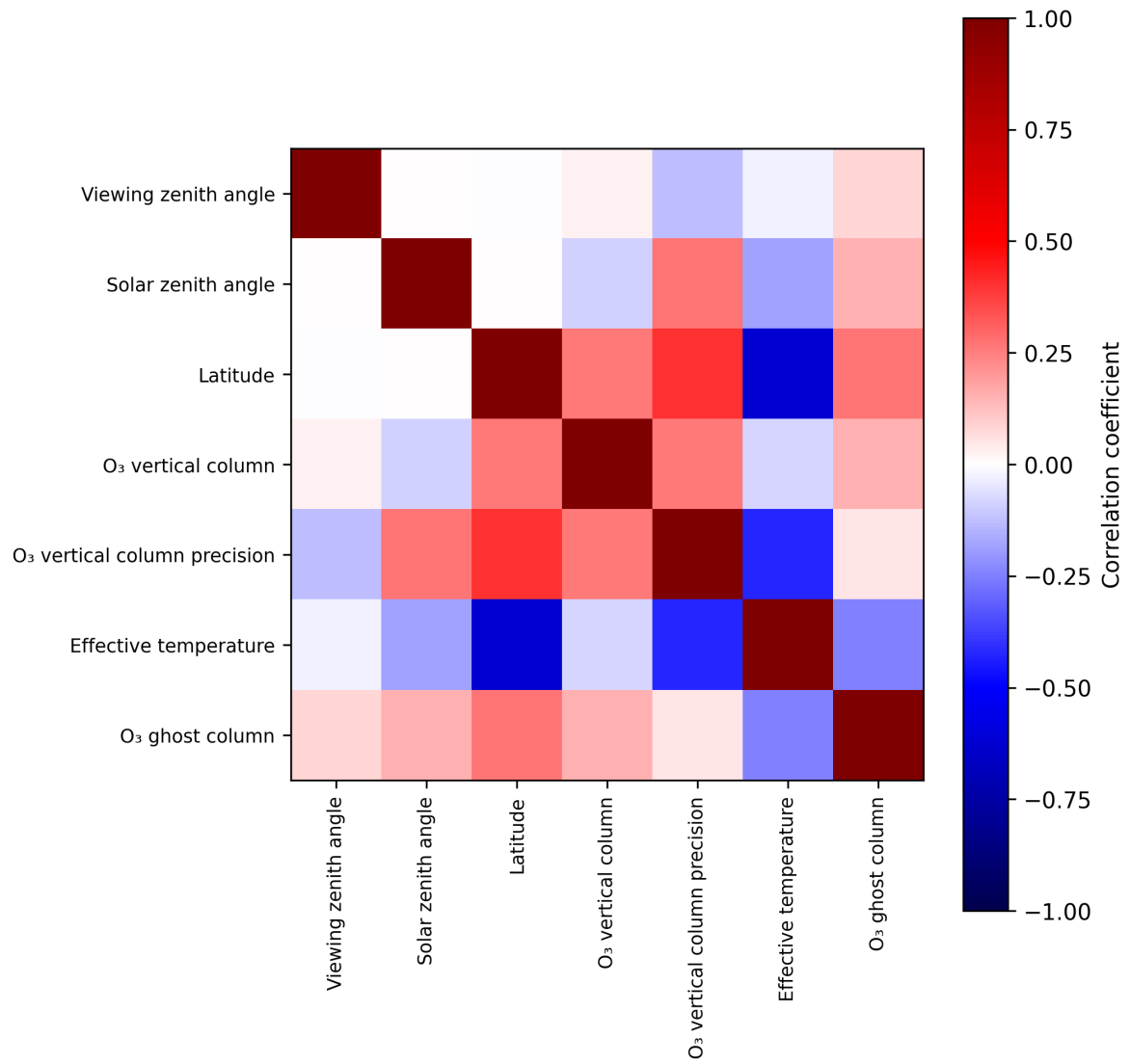
Figure 2: Map of correlation matrix for 2024-10-20 to 2024-10-22.
