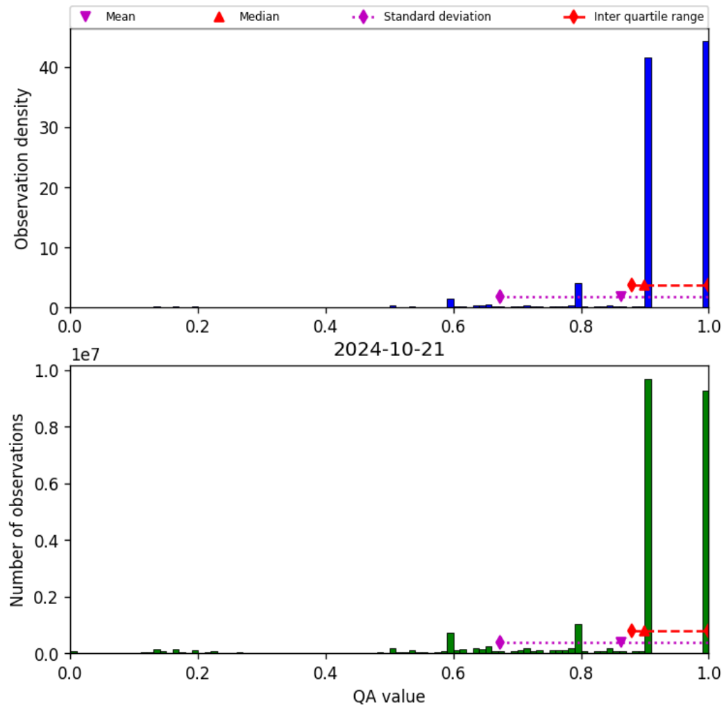
Figure 20: Histogram of “QA value” for 2024-10-20 to 2024-10-22
