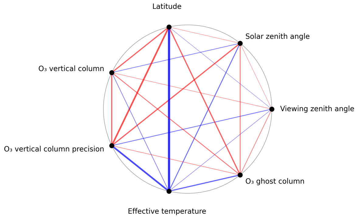
Figure 1: Map of correlation graph for 2024-10-20 to 2024-10-22.
