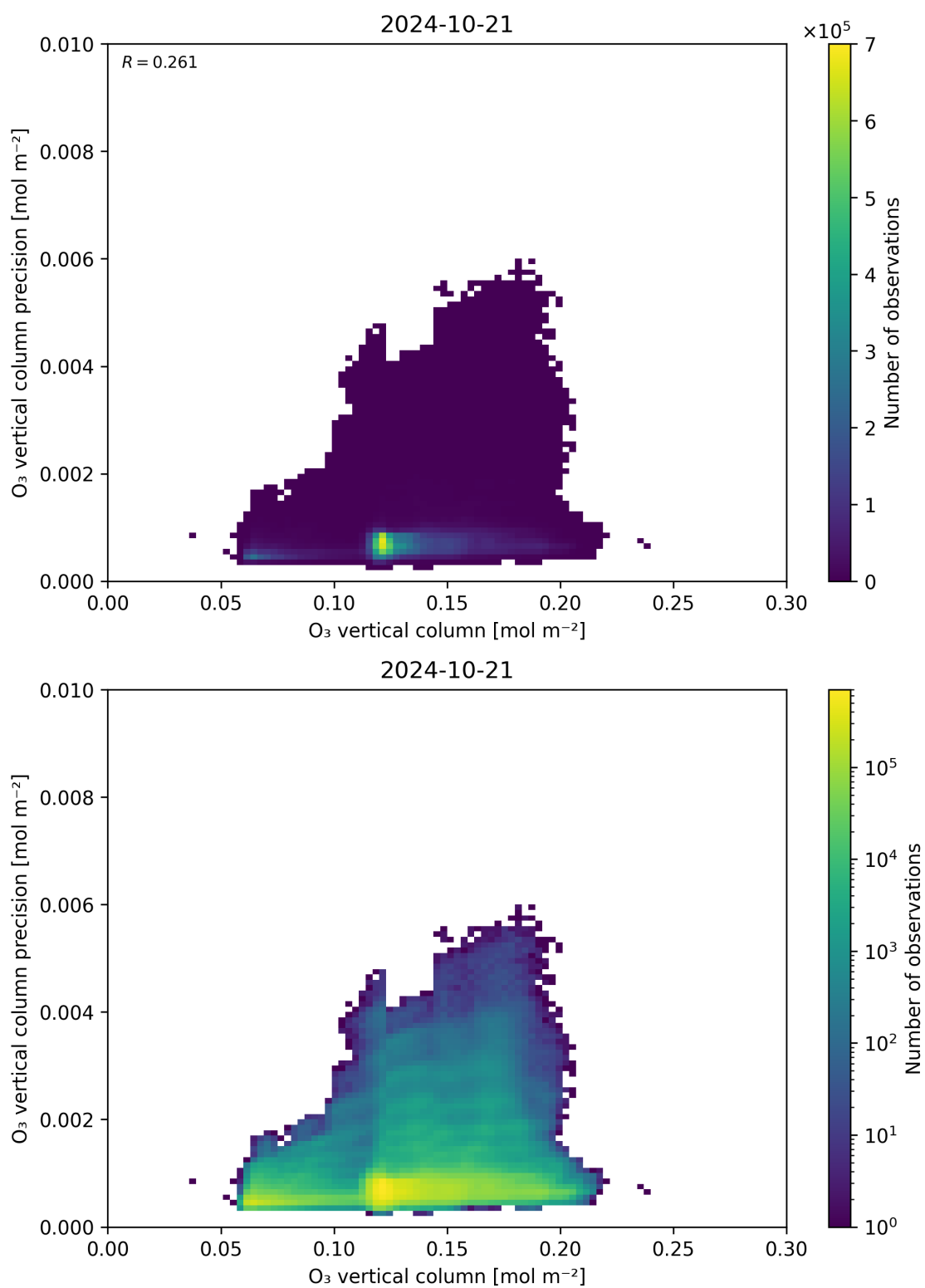
Figure 41: Scatter density plot of “O 3 vertical column” against “O 3 vertical column precision” for 2024-10-20 to 2024-10-22.
