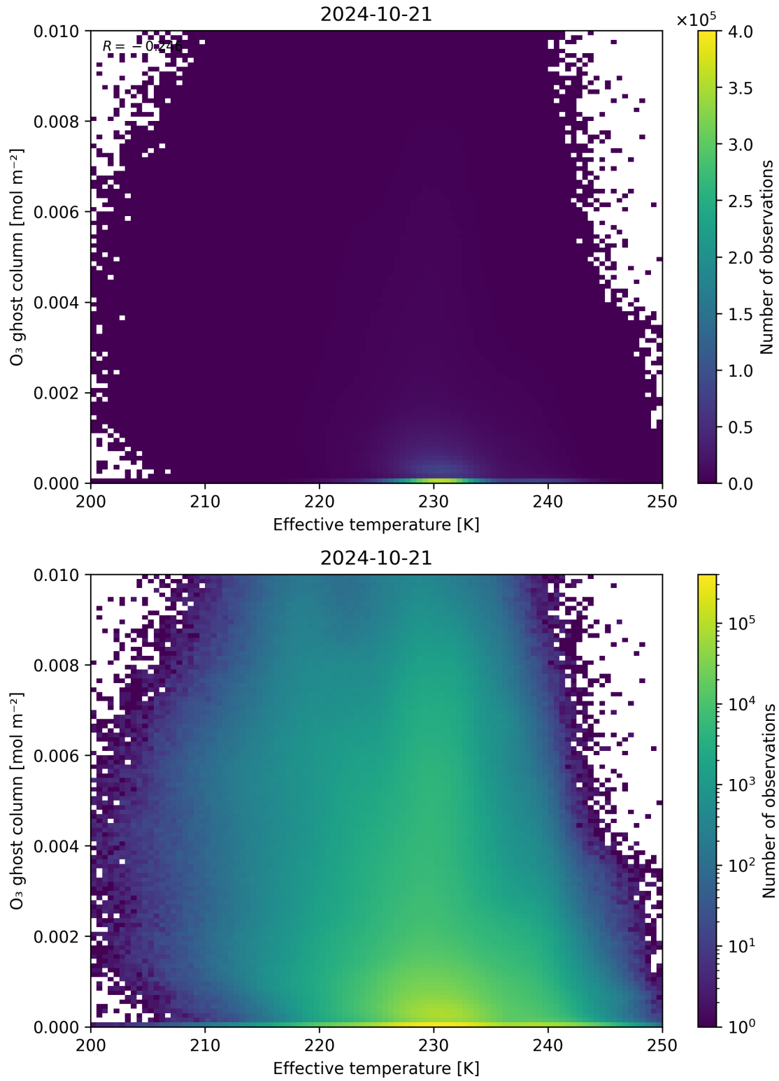
Figure 38: Scatter density plot of “Effective temperature” against “O 3 ghost column” for 2024-10-20 to 2024-10-22.
