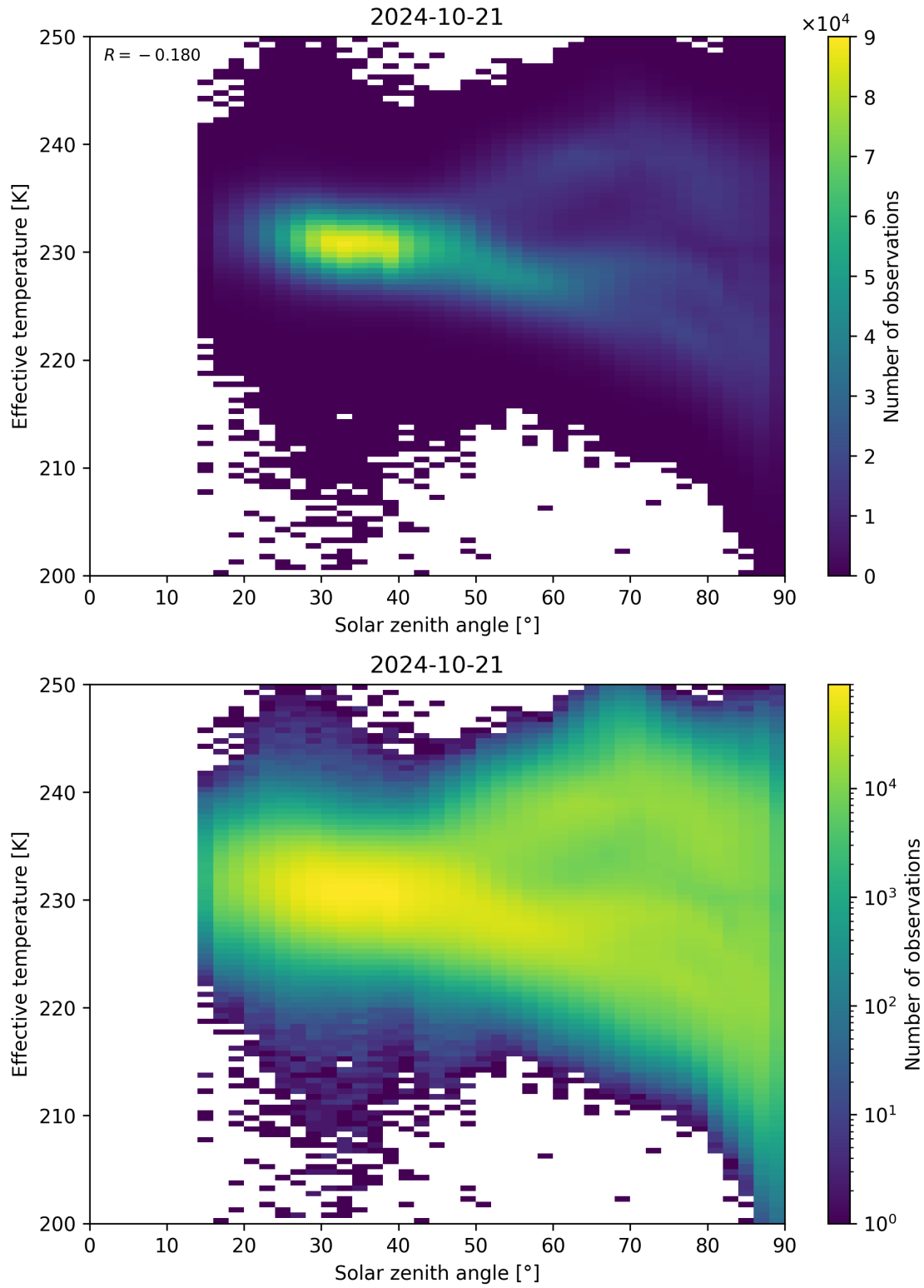
Figure 45: Scatter density plot of “Solar zenith angle” against “Effective temperature” for 2024-10-20 to 2024-10-22.
