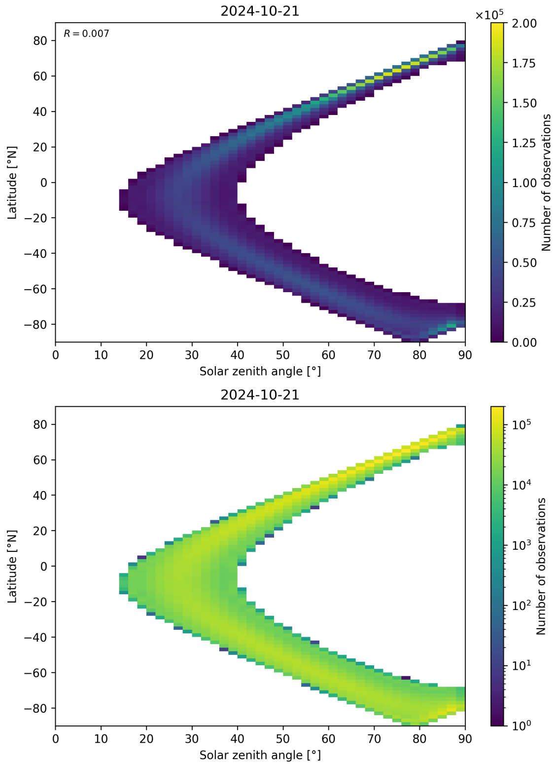
Figure 44: Scatter density plot of “Solar zenith angle” against “Latitude” for 2024-10-20 to 2024-10-22.
