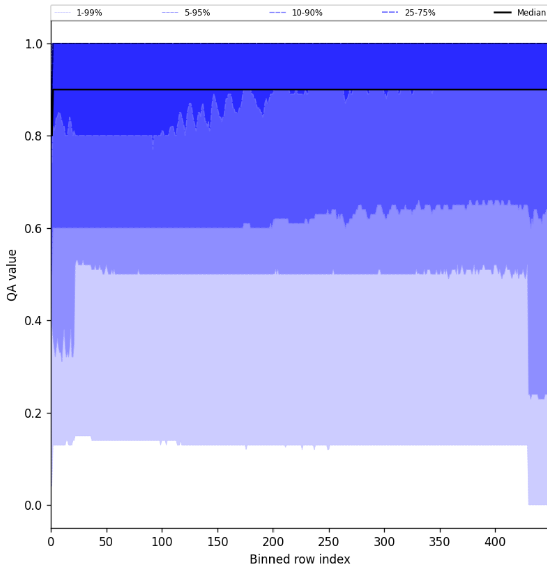
Figure 27: Along track statistics of “QA value” for 2024-10-20 to 2024-10-22
