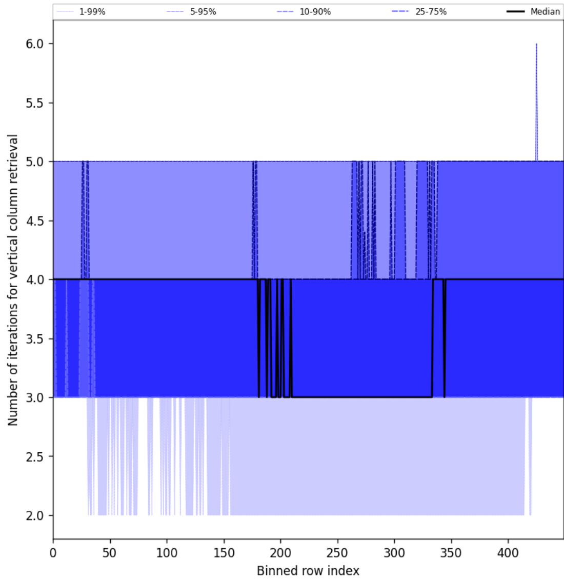
Figure 33: Along track statistics of “Number of iterations for vertical column retrieval” for 2024-10-20 to 2024-10-22
