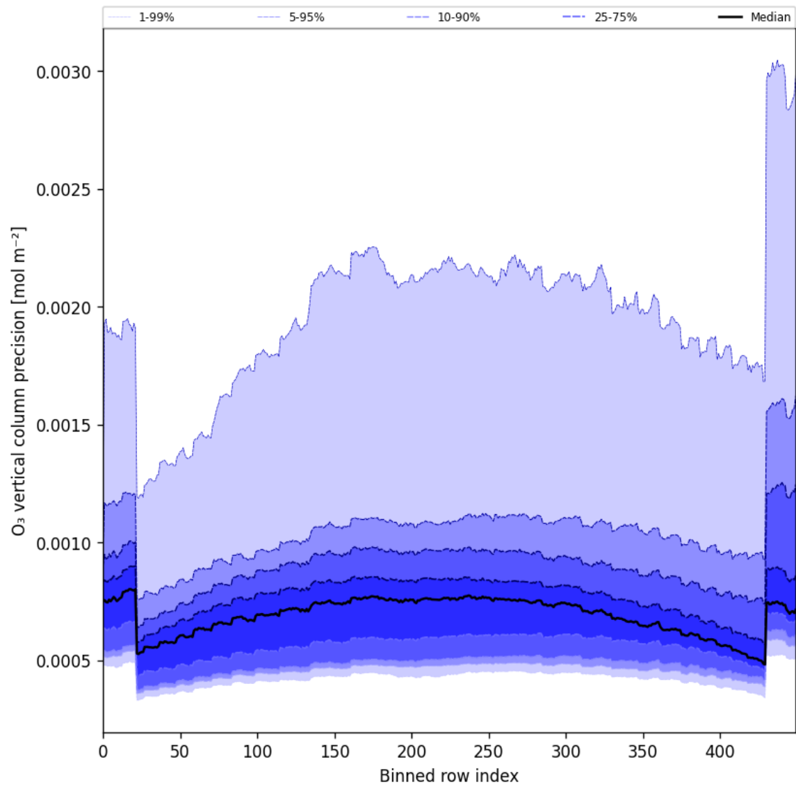
Figure 29: Along track statistics of “O 3 vertical column precision” for 2024-10-20 to 2024-10-22
