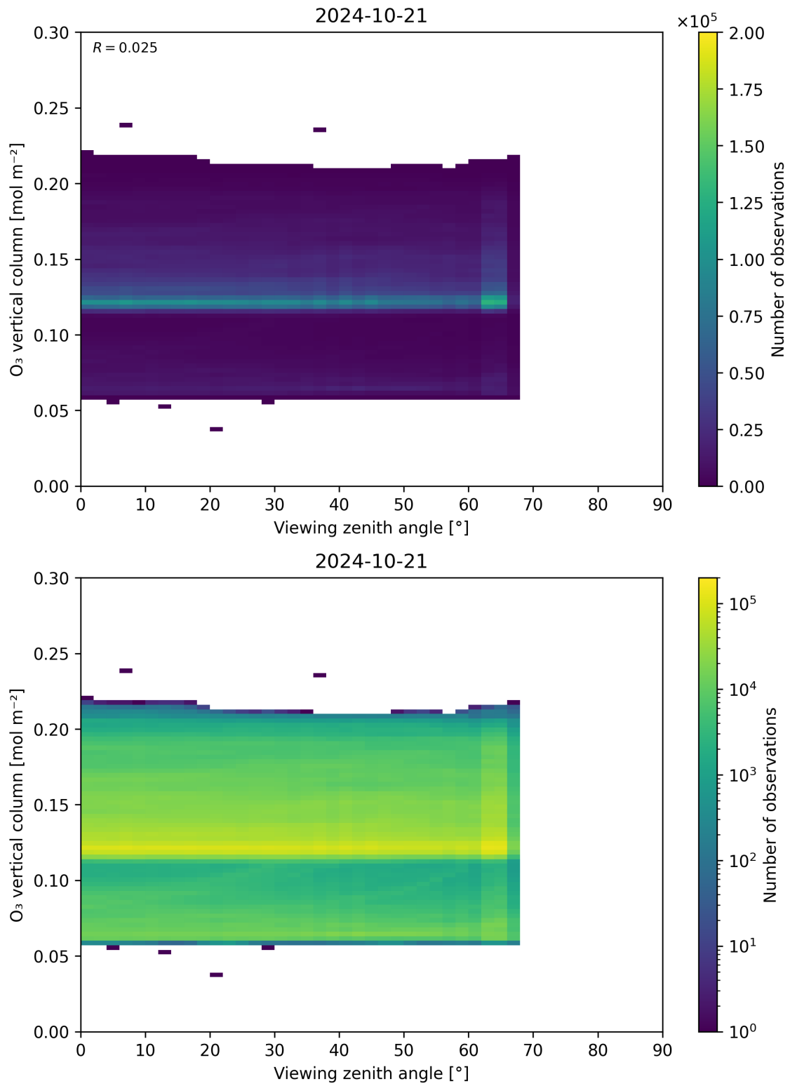
Figure 52: Scatter density plot of “Viewing zenith angle” against “O 3 vertical column” for 2024-10-20 to 2024-10-22.
