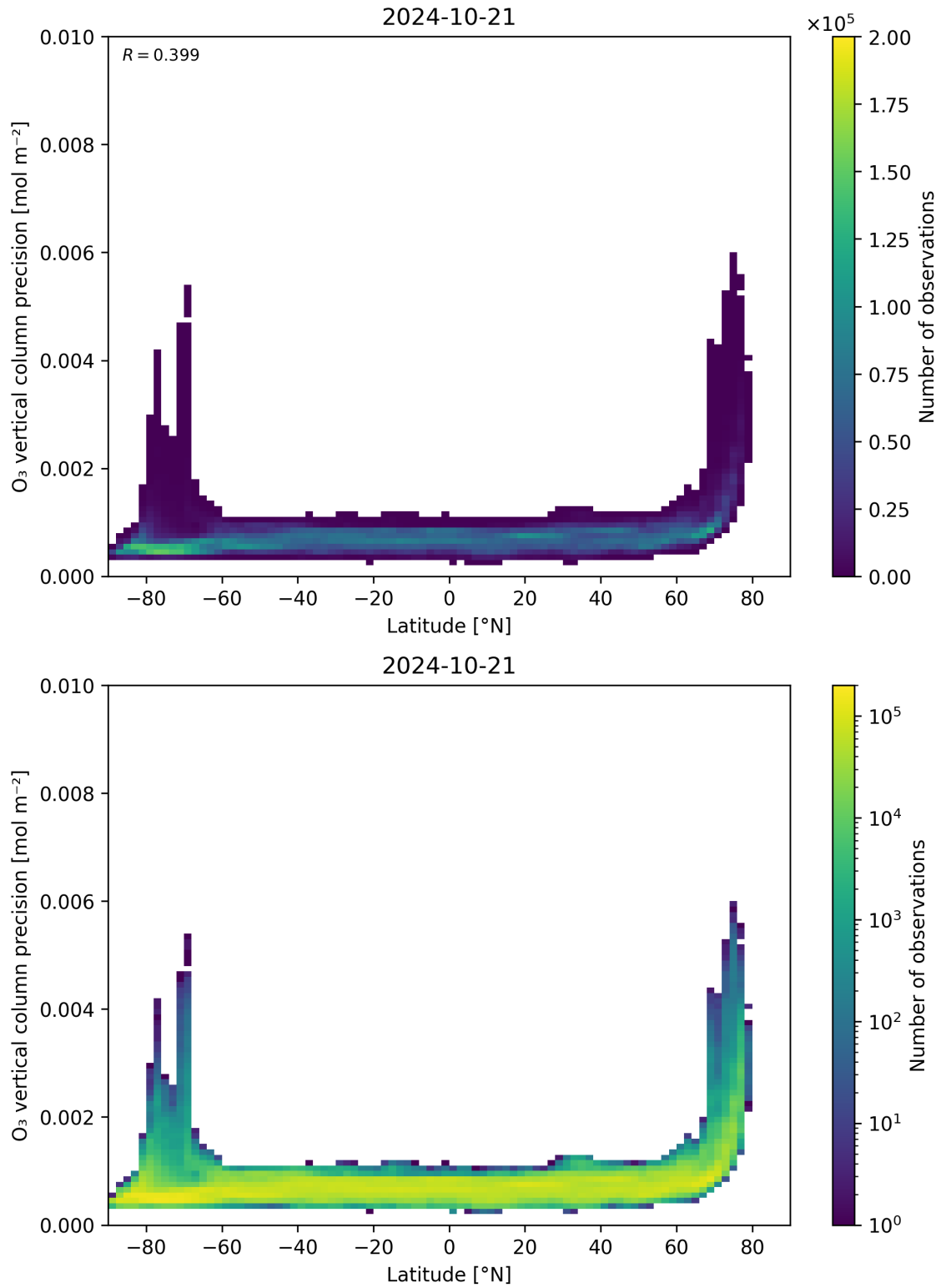
Figure 37: Scatter density plot of “Latitude” against “O 3 vertical column precision” for 2024-10-20 to 2024-10-22.
