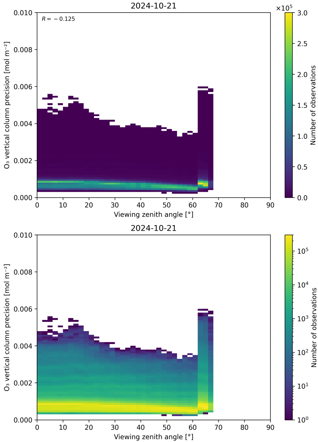
Figure 53: Scatter density plot of “Viewing zenith angle” against “O 3 vertical column precision” for 2024-10-20 to 2024-10-22.
