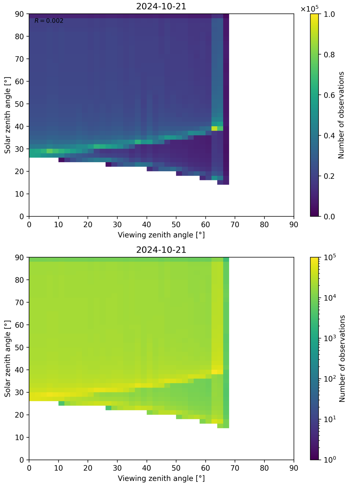
Figure 54: Scatter density plot of “Viewing zenith angle” against “Solar zenith angle” for 2024-10-20 to 2024-10-22.
