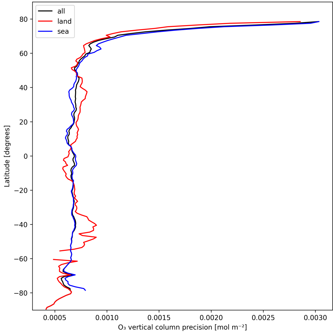
Figure 15: Zonal average of “O 3 vertical column precision” for 2024-10-20 to 2024-10-22.
