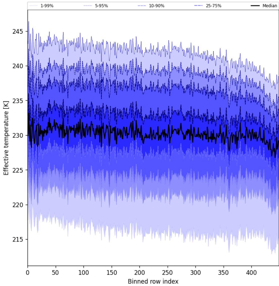
Figure 31: Along track statistics of “Effective temperature” for 2024-10-20 to 2024-10-22
