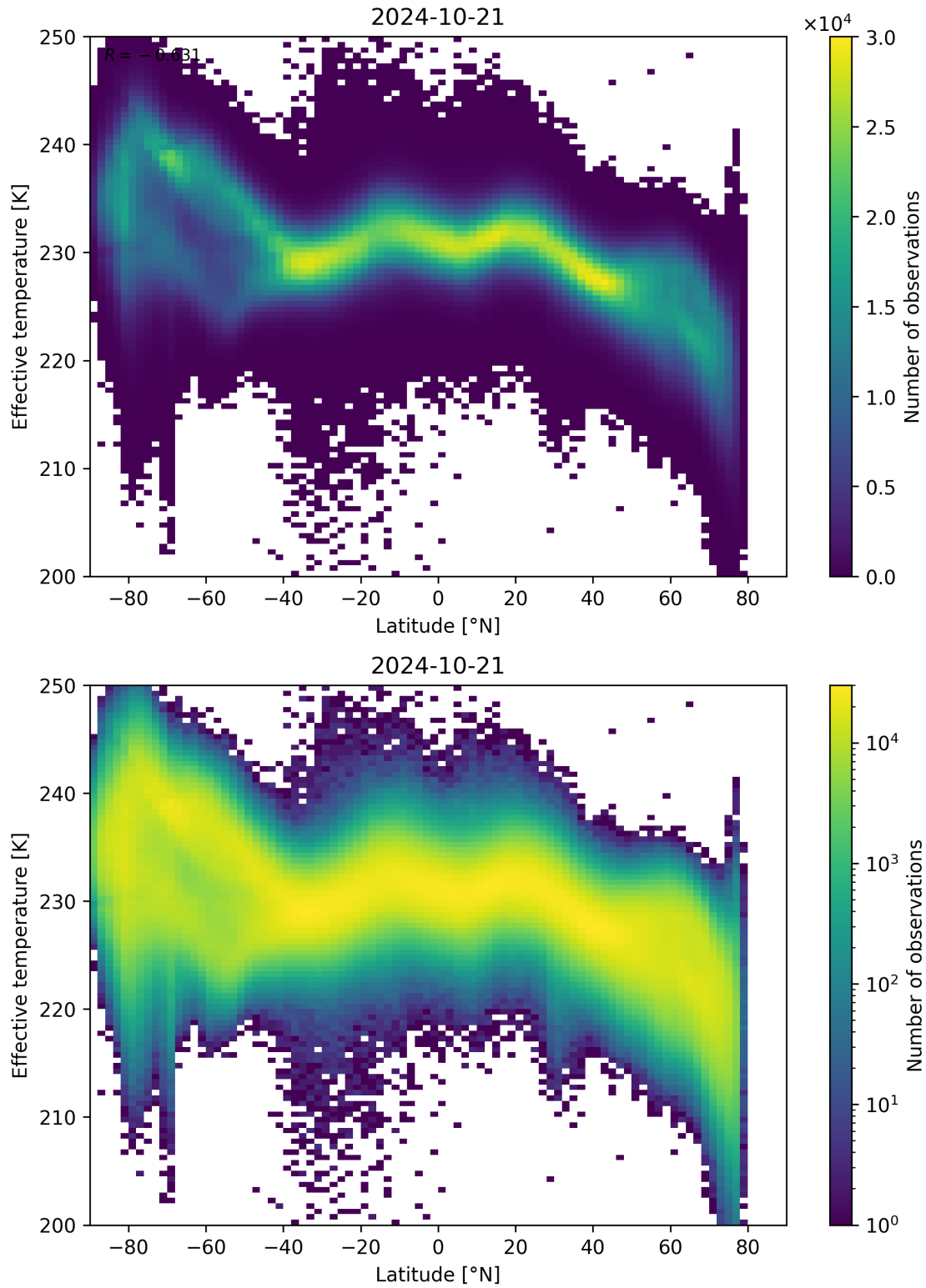
Figure 34: Scatter density plot of “Latitude” against “Effective temperature” for 2024-10-20 to 2024-10-22.
