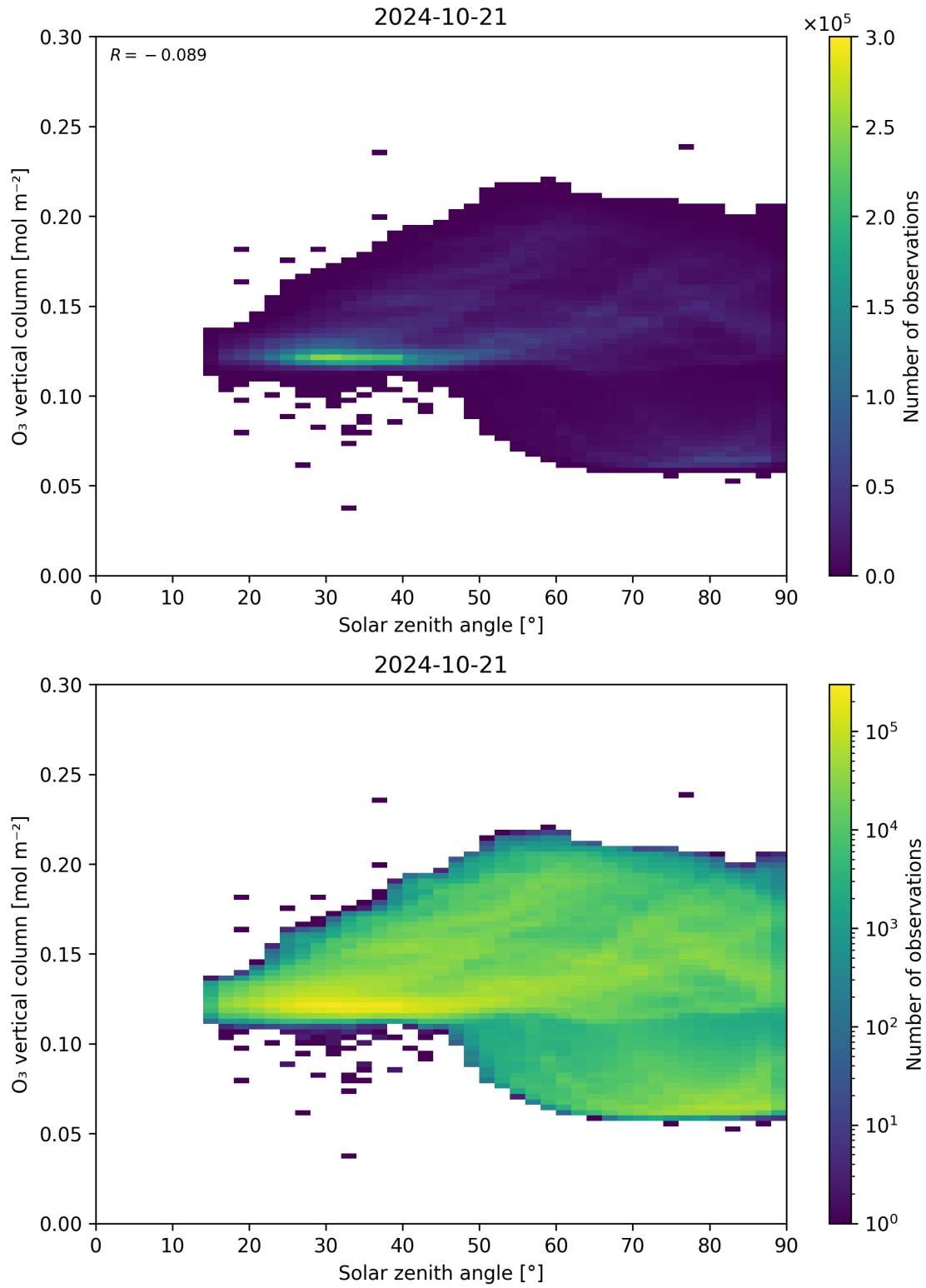
Figure 47: Scatter density plot of “Solar zenith angle” against “O 3 vertical column” for 2024-10-20 to 2024-10-22.
