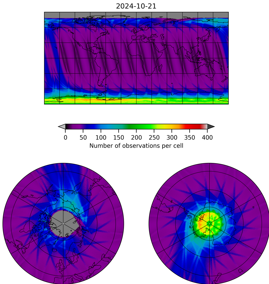
Figure 12: Map of the number of observations for 2024-10-20 to 2024-10-22
