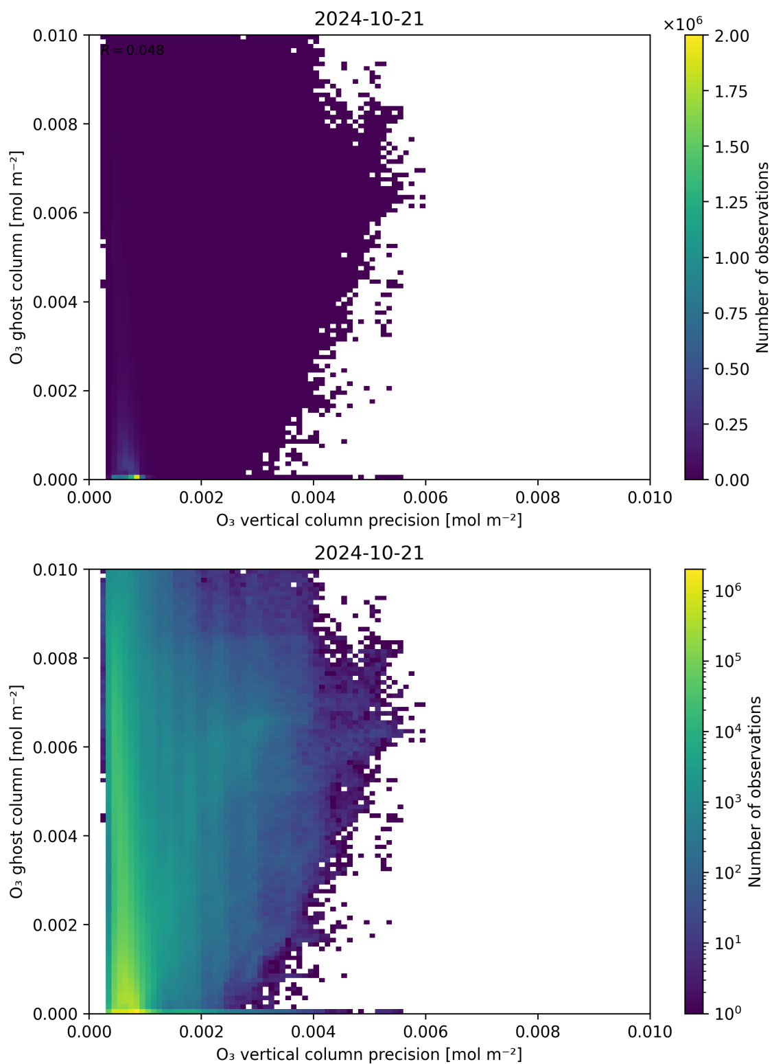
Figure 43: Scatter density plot of “O 3 vertical column precision” against “O 3 ghost column” for 2024-10-20 to 2024-10-22.
