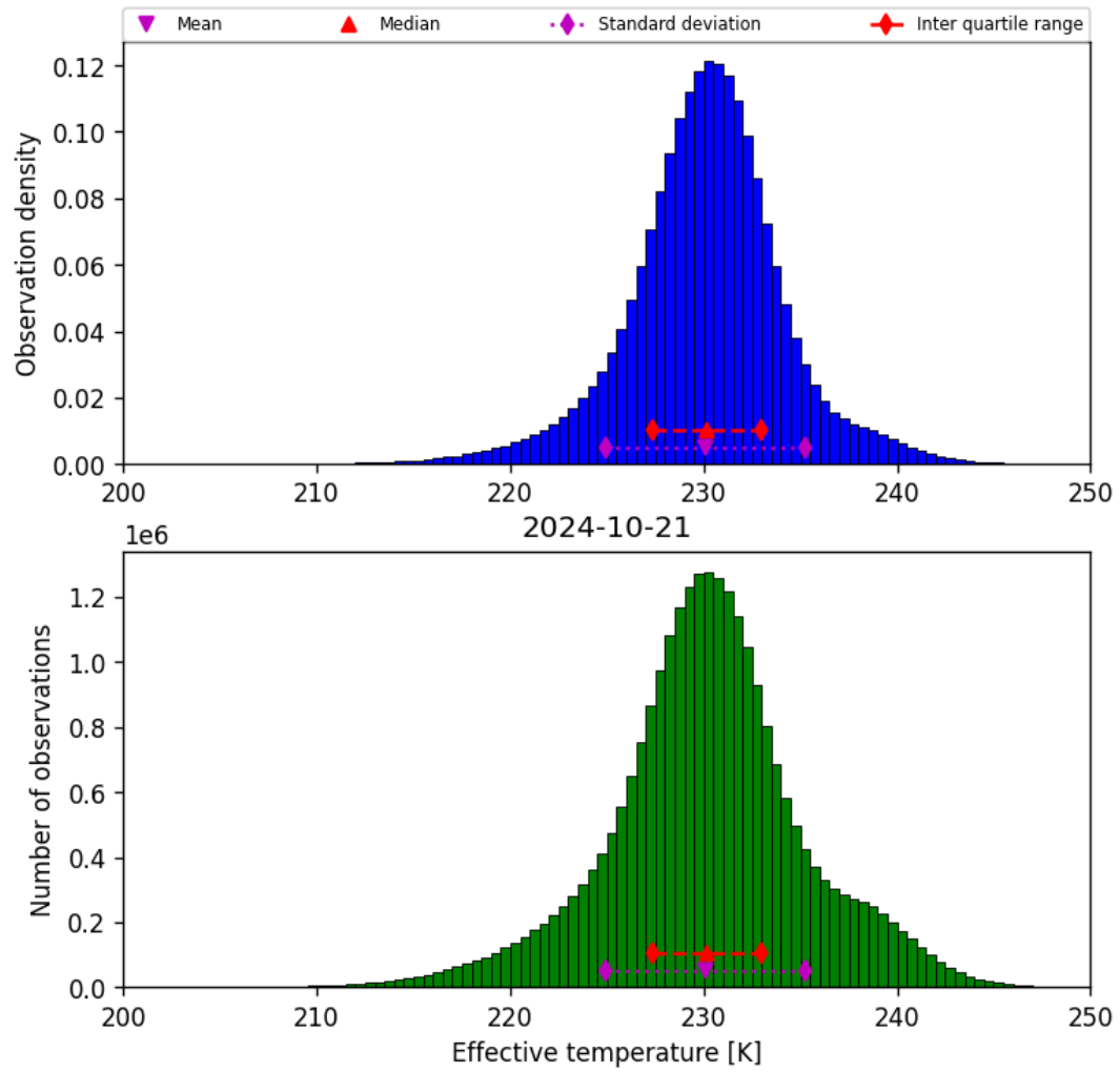
Figure 24: Histogram of “Effective temperature” for 2024-10-20 to 2024-10-22
