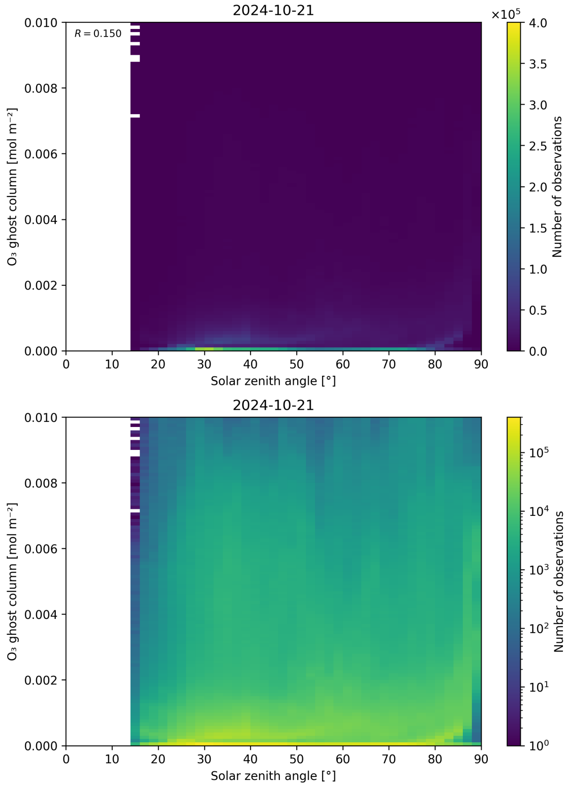
Figure 46: Scatter density plot of “Solar zenith angle” against “O 3 ghost column” for 2024-10-20 to 2024-10-22.
