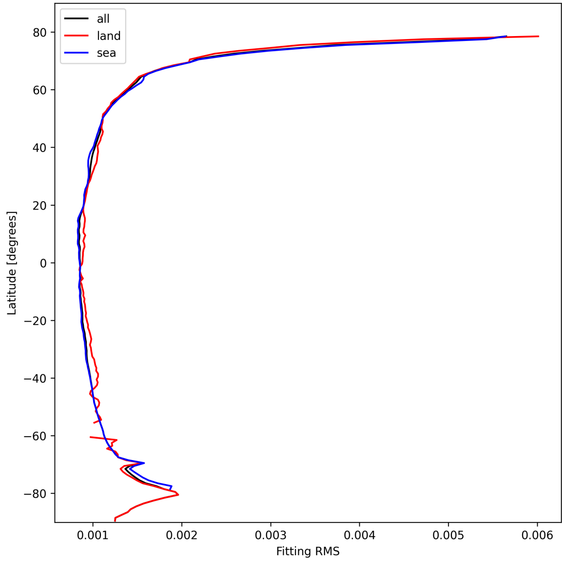
Figure 16: Zonal average of “Fitting RMS” for 2024-10-20 to 2024-10-22.
