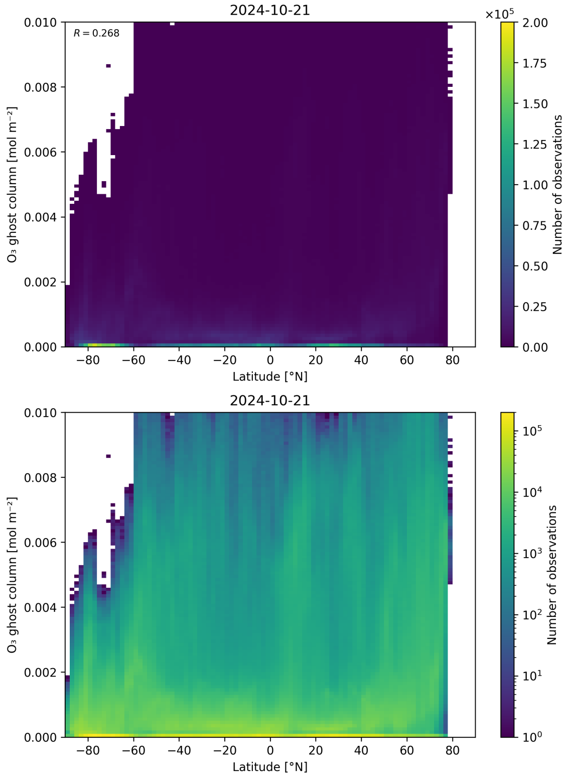
Figure 35: Scatter density plot of “Latitude” against “O 3 ghost column” for 2024-10-20 to 2024-10-22.
