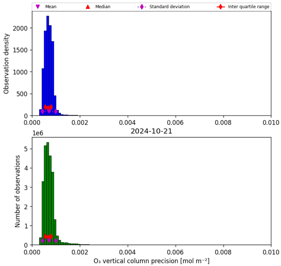
Figure 22: Histogram of “O 3 vertical column precision” for 2024-10-20 to 2024-10-22
