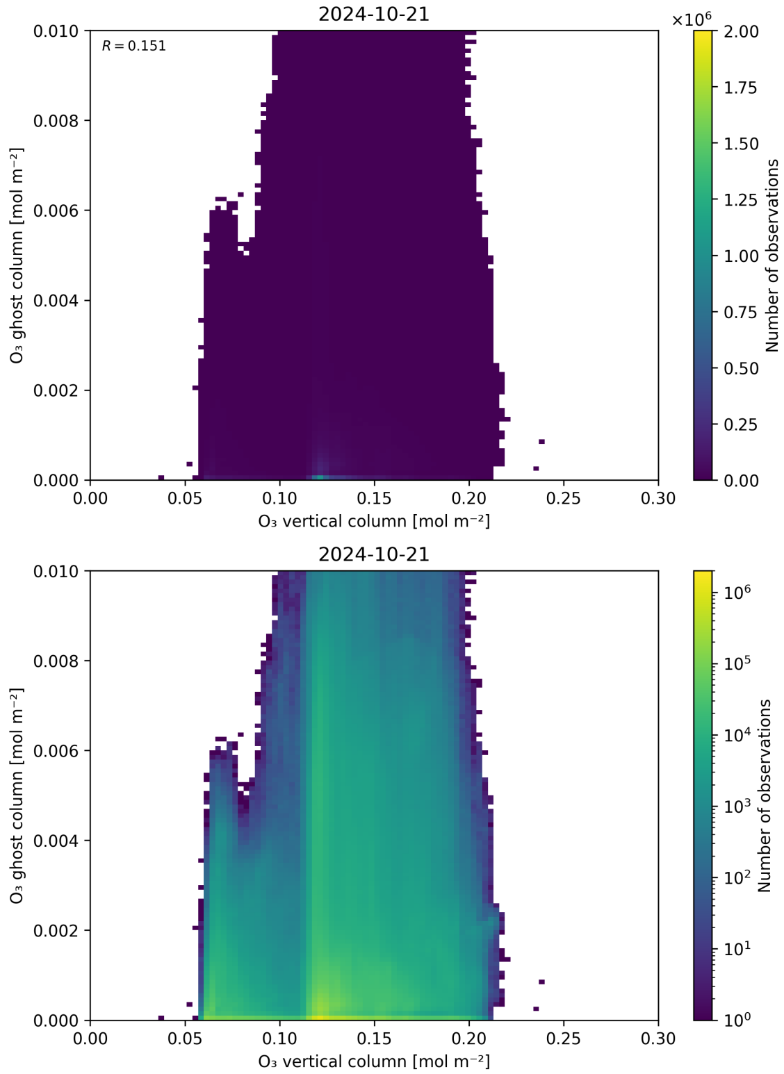
Figure 40: Scatter density plot of “O 3 vertical column” against “O 3 ghost column” for 2024-10-20 to 2024-10-22.
