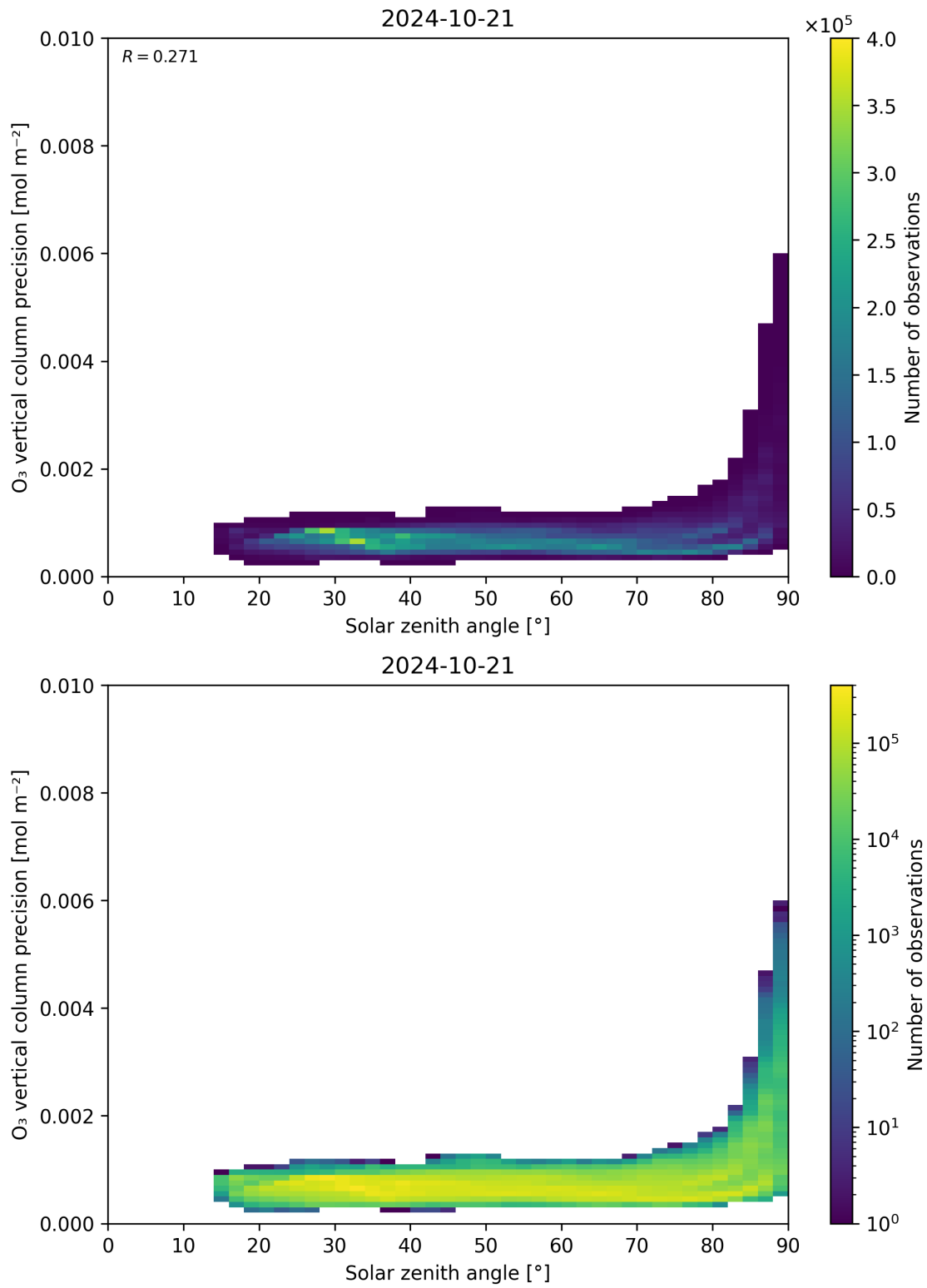
Figure 48: Scatter density plot of “Solar zenith angle” against “O 3 vertical column precision” for 2024-10-20 to 2024-10-22.
