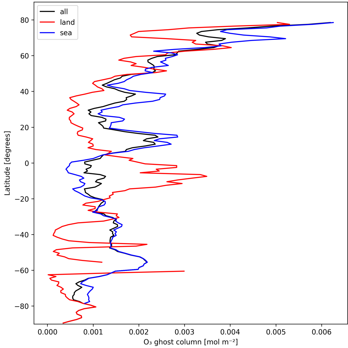
Figure 18: Zonal average of "O 3 ghost column" for 2024-10-20 to 2024-10-22.
