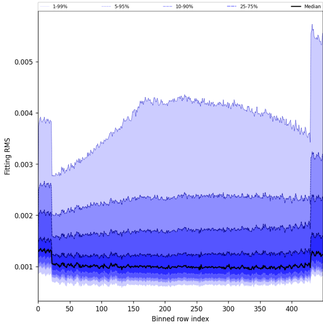
Figure 30: Along track statistics of “Fitting RMS” for 2024-10-20 to 2024-10-22
