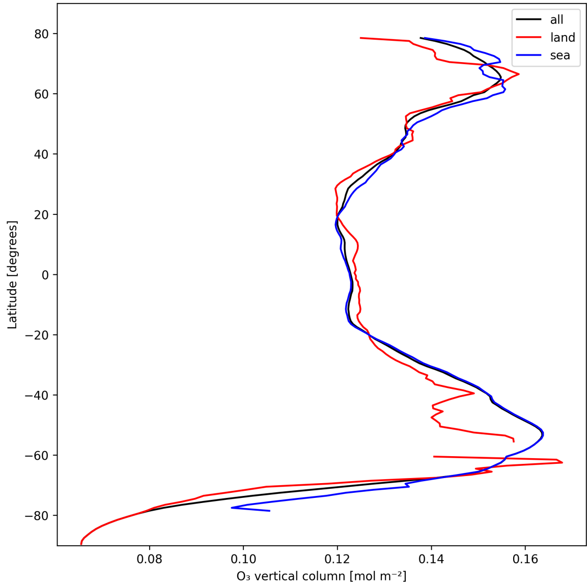
Figure 14: Zonal average of “O 3 vertical column” for 2024-10-20 to 2024-10-22.
