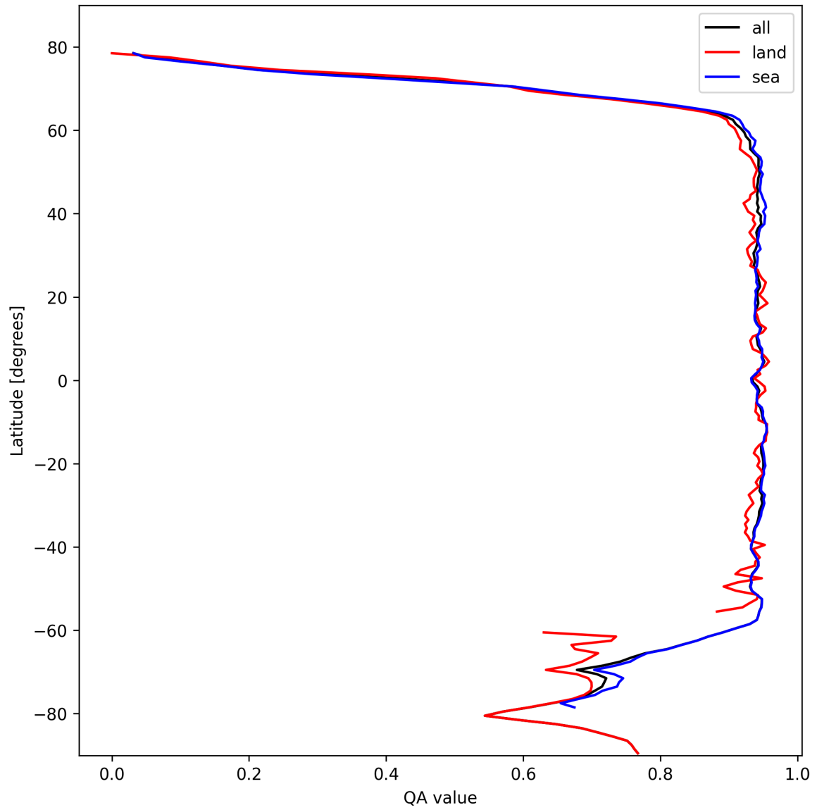
Figure 13: Zonal average of “QA value” for 2024-10-20 to 2024-10-22.
